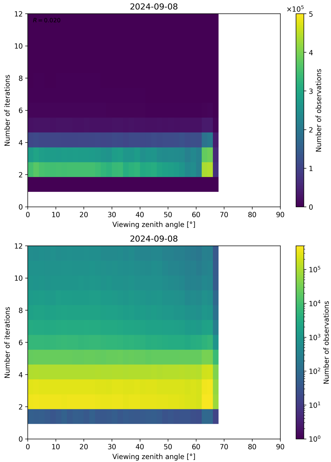
Figure 136: Scatter density plot of “Viewing zenith angle” against “Number of iterations” for 2024-09-07 to 2024-09-09.
