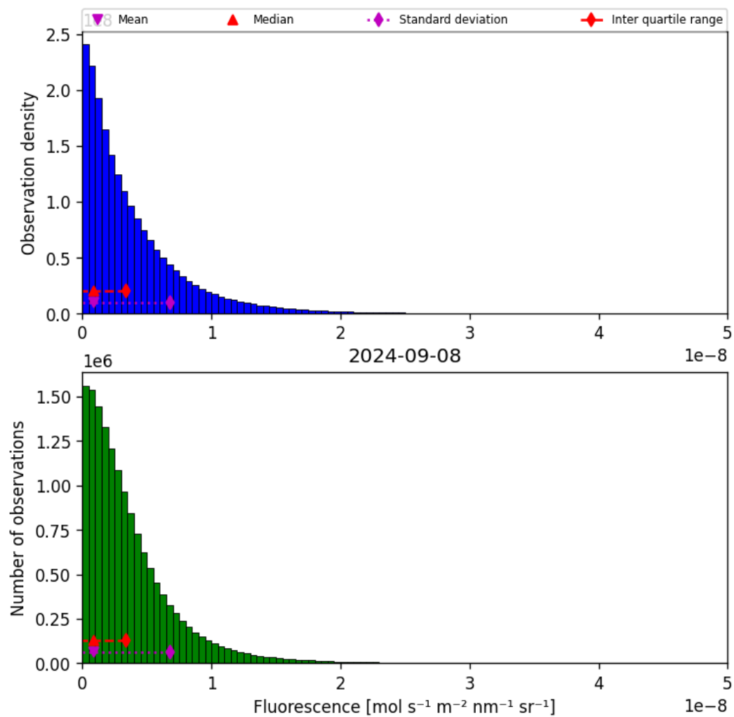
Figure 40: Histogram of “Fluorescence” for 2024-09-07 to 2024-09-09
