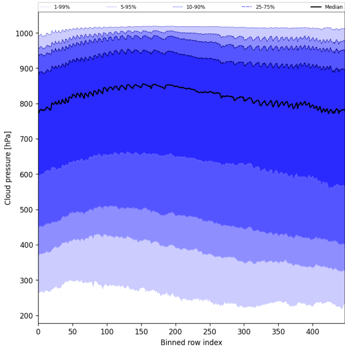
Figure 47: Along track statistics of “Cloud pressure” for 2024-09-07 to 2024-09-09
