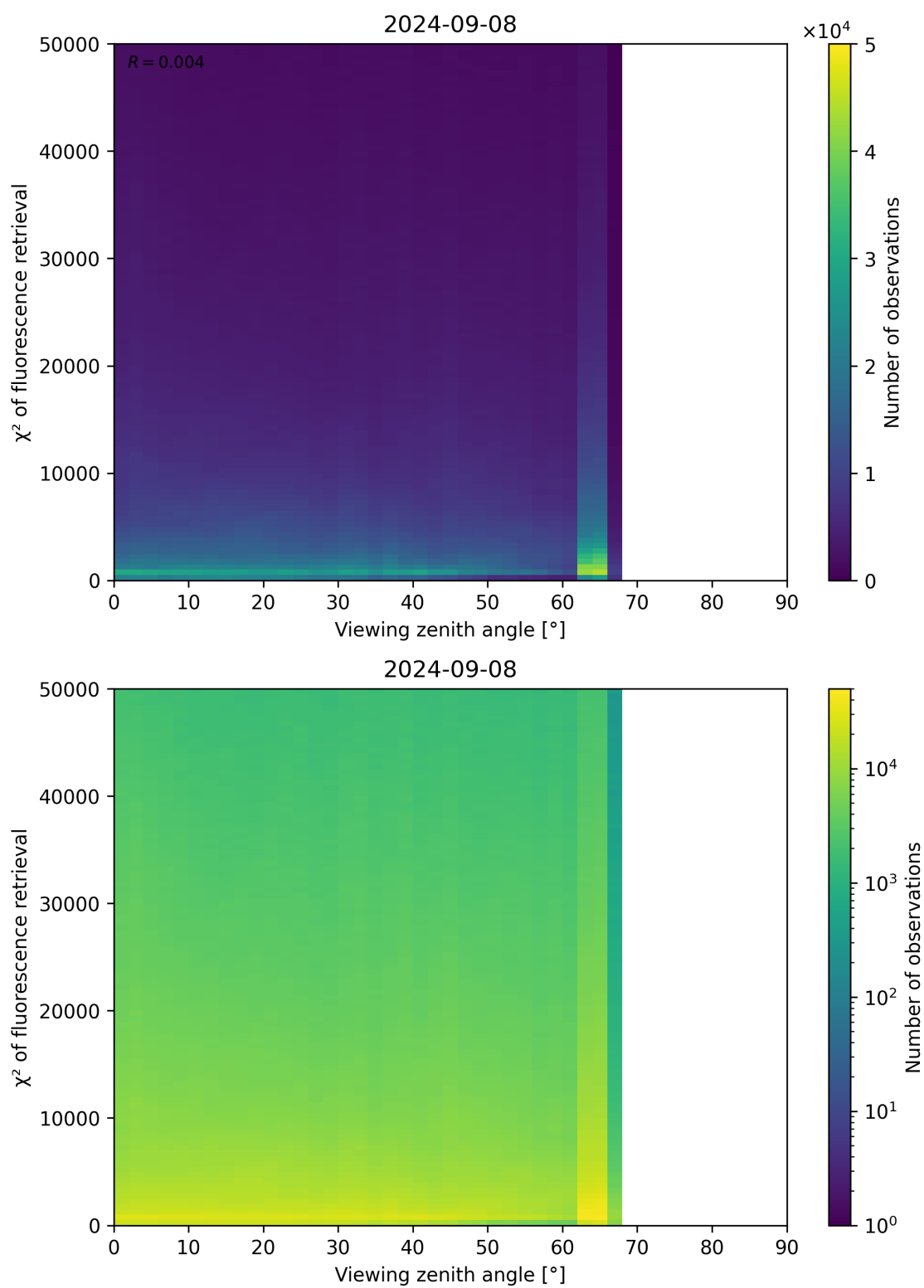
Figure 131: Scatter density plot of “Viewing zenith angle” against “ \chi^2 of fluorescence retrieval” for 2024-09-07 to 2024-09-09.
