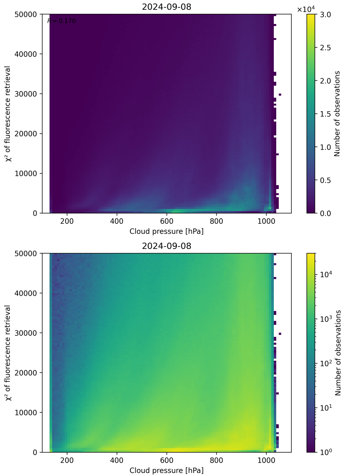
Figure 86: Scatter density plot of “Cloud pressure” against “ \chi^2 of fluorescence retrieval” for 2024-09-07 to 2024-09-09.
