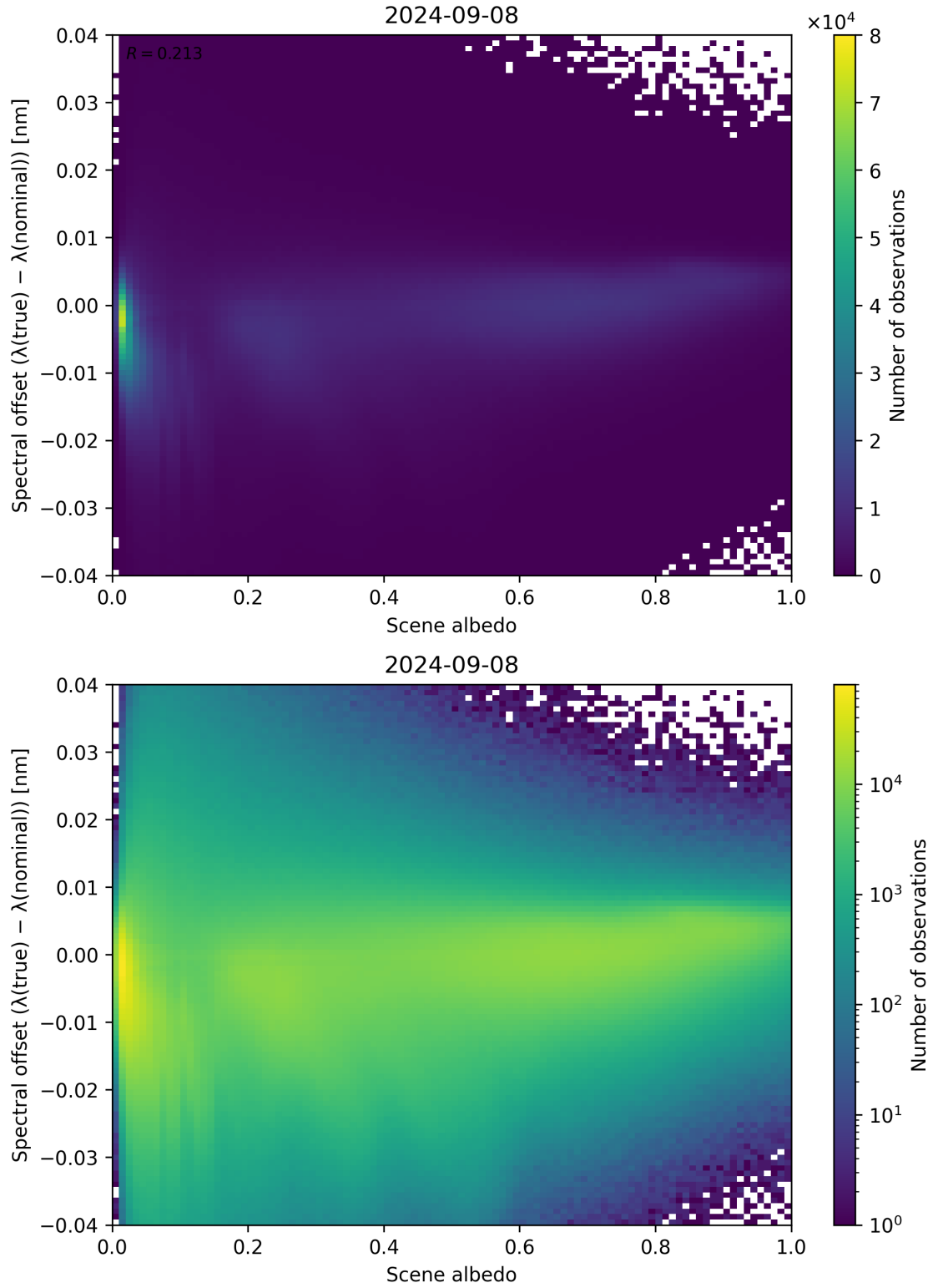
Figure 117: Scatter density plot of “Scene albedo” against “Spectral offset ( \lambda_{\text{true}} - \lambda_{\text{nominal}} )” for 2024-09-07 to 2024-09-09.
