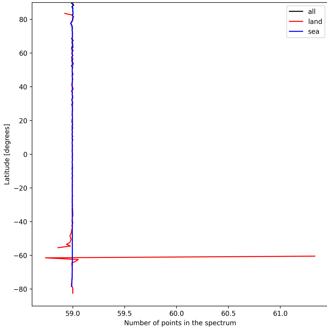
Figure 27: Zonal average of “Number of points in the spectrum” for 2024-09-07 to 2024-09-09.
