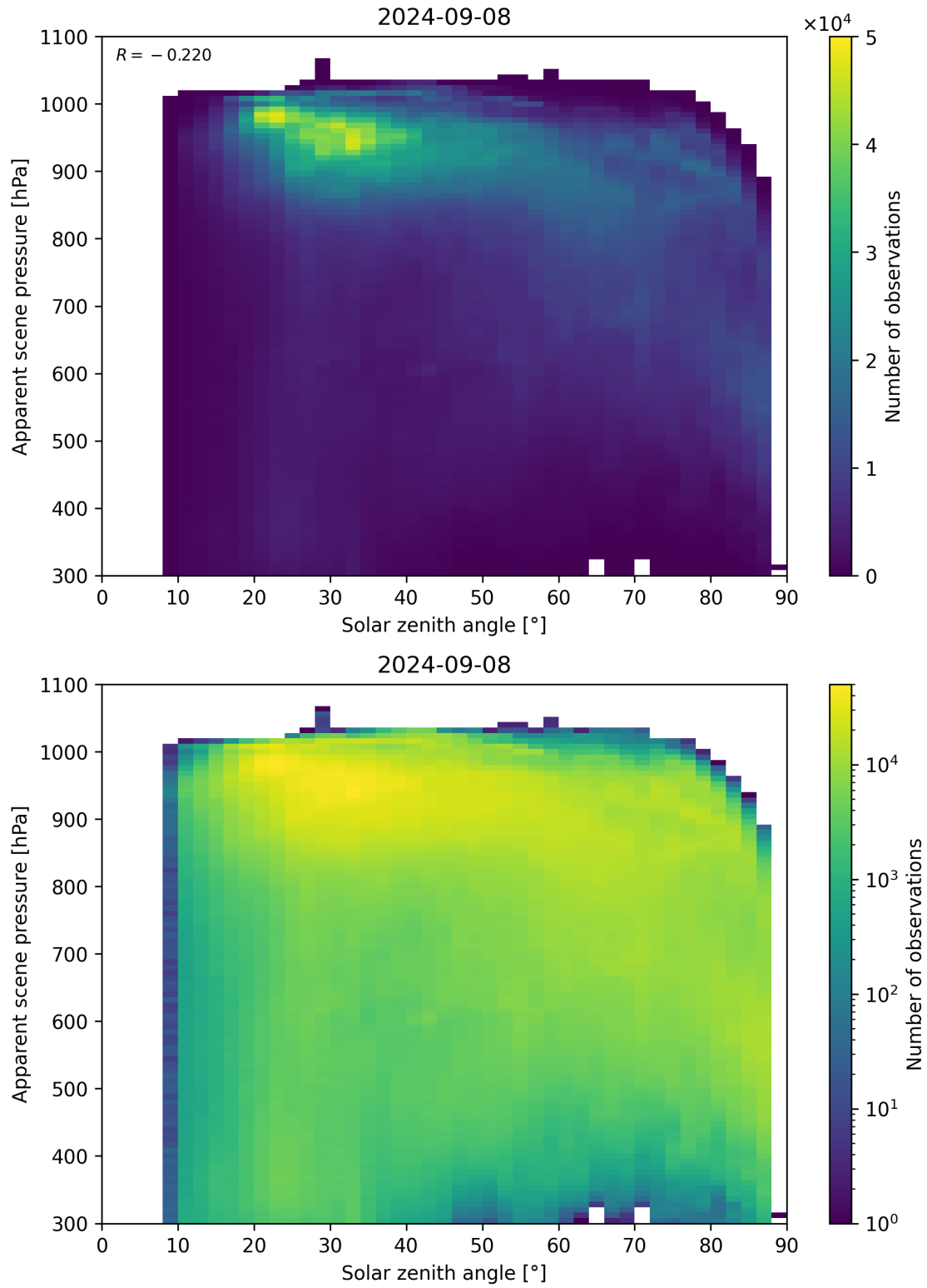
Figure 118: Scatter density plot of “Solar zenith angle” against “Apparent scene pressure” for 2024-09-07 to 2024-09-09.
