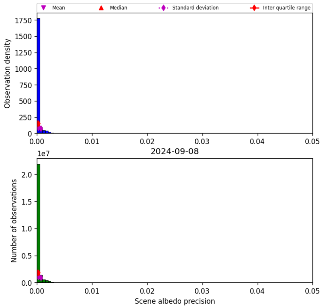
Figure 35: Histogram of “Scene albedo precision” for 2024-09-07 to 2024-09-09
