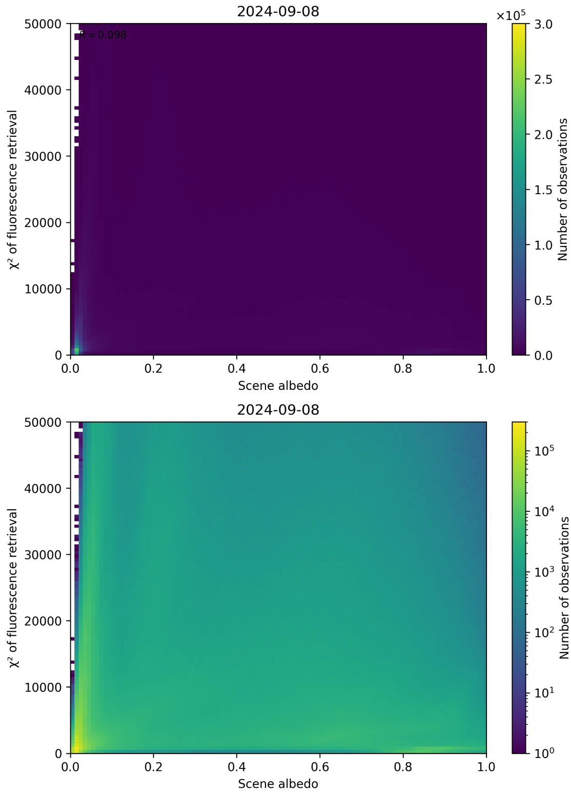
Figure 113: Scatter density plot of “Scene albedo” against “ \chi^2 of fluorescence retrieval” for 2024-09-07 to 2024-09-09.
