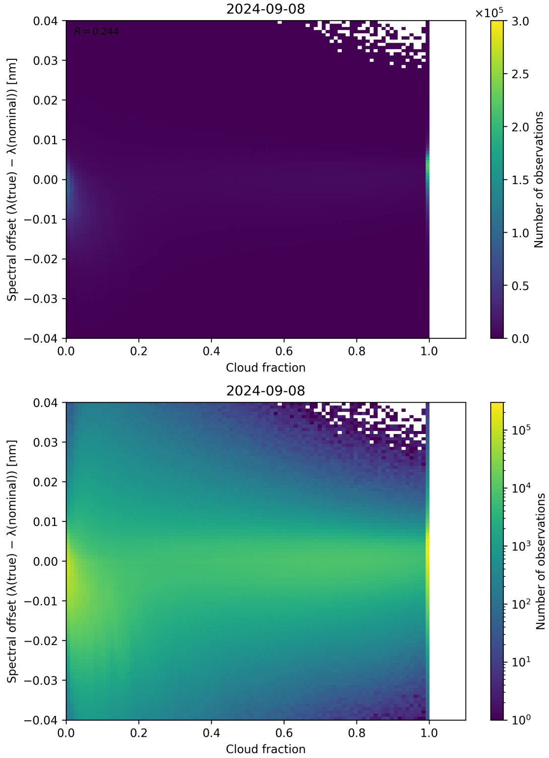
Figure 83: Scatter density plot of “Cloud fraction” against “Spectral offset ( \lambda_{\text{true}} - \lambda_{\text{nominal}} )” for 2024-09-07 to 2024-09-09.
