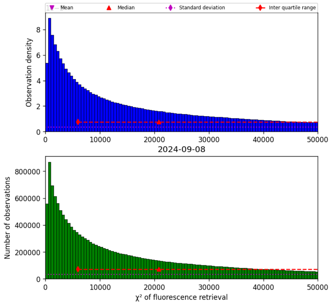
Figure 42: Histogram of “ \chi^2 of fluorescence retrieval” for 2024-09-07 to 2024-09-09
