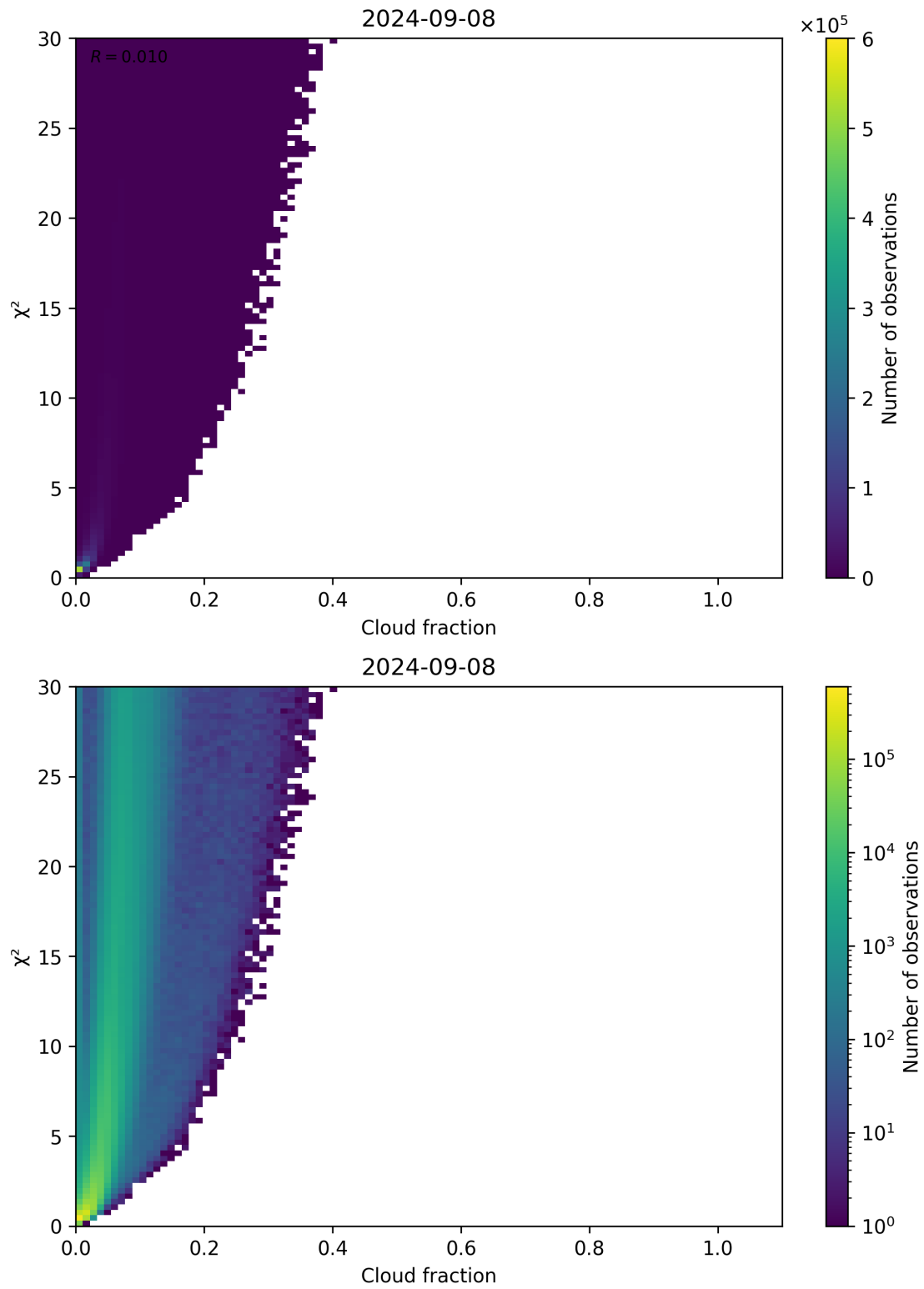
Figure 77: Scatter density plot of “Cloud fraction” against “ \chi^2 ” for 2024-09-07 to 2024-09-09.
