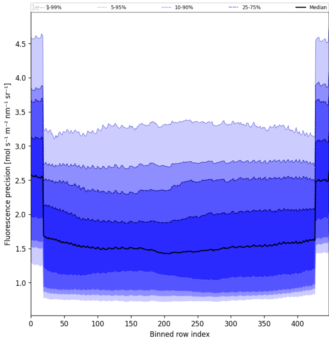
Figure 58: Along track statistics of “Fluorescence precision” for 2024-09-07 to 2024-09-09
