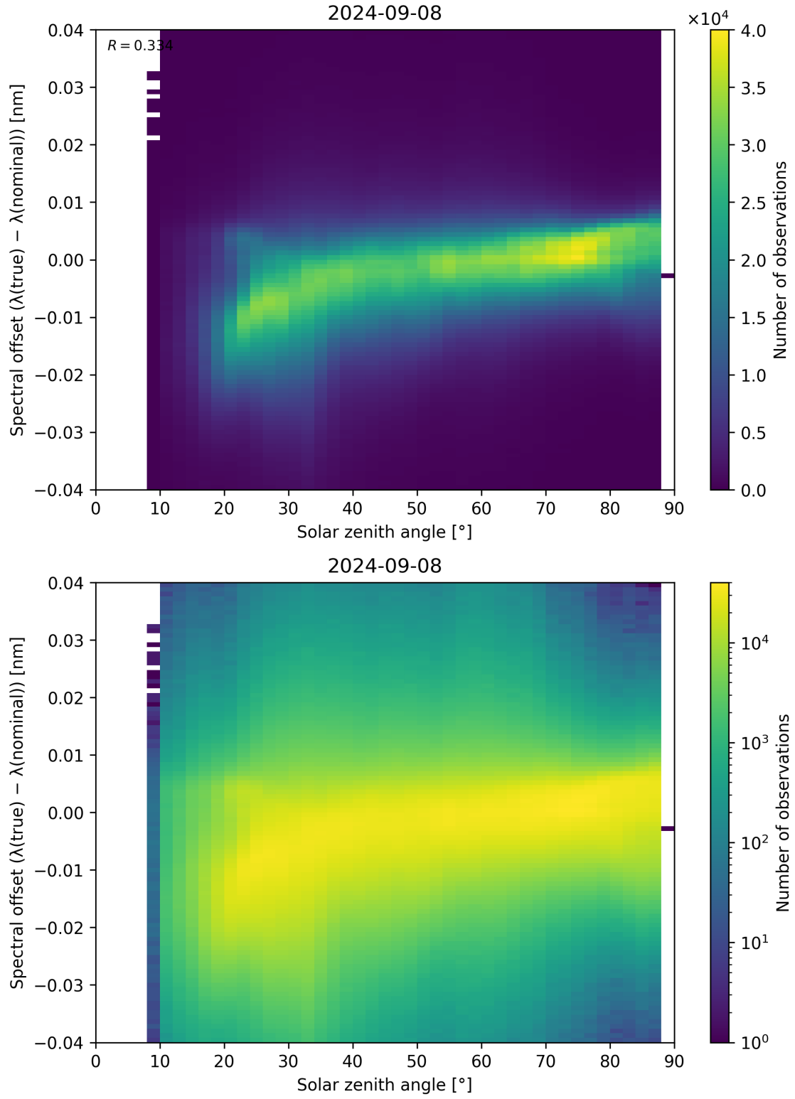
Figure 128: Scatter density plot of “Solar zenith angle” against “Spectral offset ( \lambda_{\text{true}} - \lambda_{\text{nominal}} )” for 2024-09-07 to 2024-09-09.
