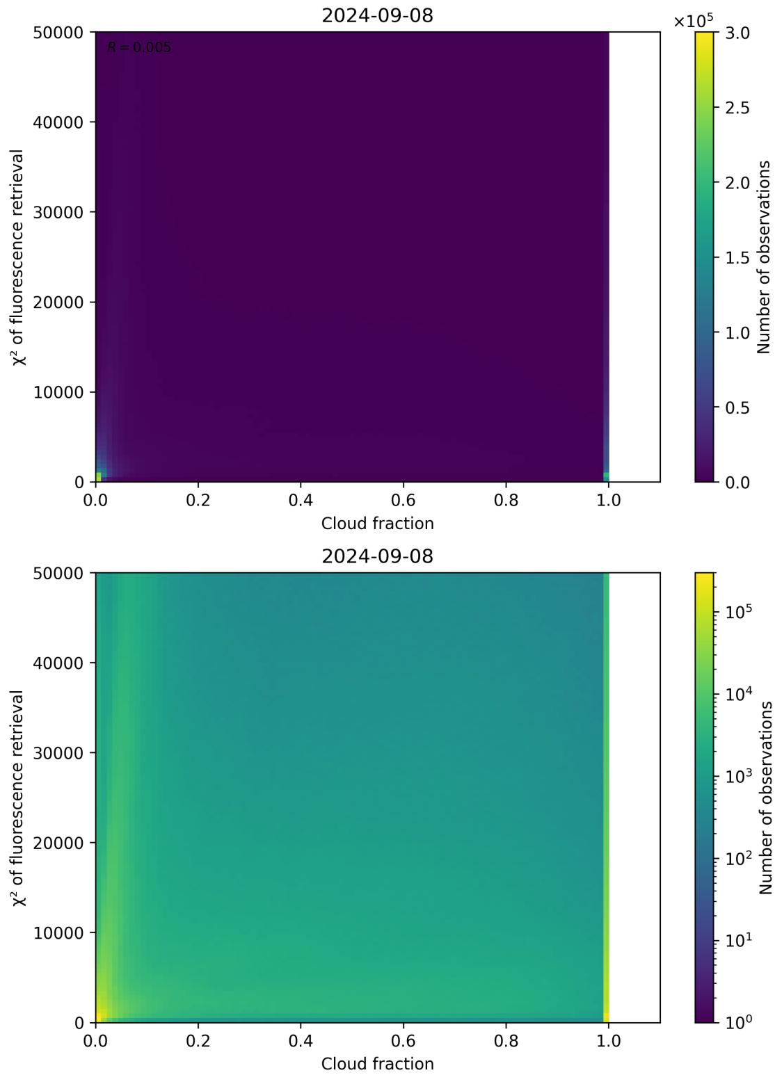
Figure 78: Scatter density plot of “Cloud fraction” against “ \chi^2 of fluorescence retrieval” for 2024-09-07 to 2024-09-09.
