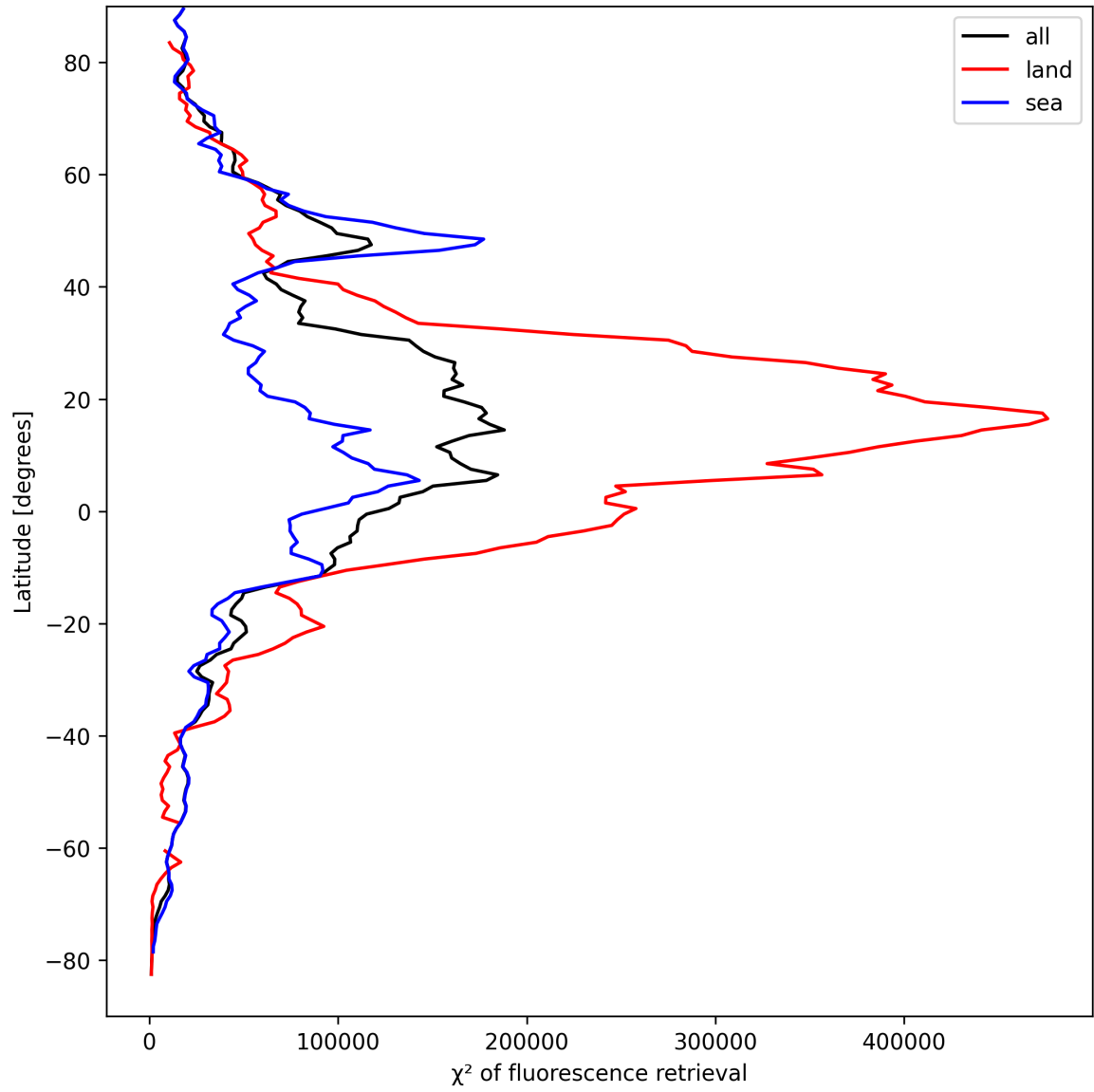
Figure 25: Zonal average of “ \chi^2 of fluorescence retrieval” for 2024-09-07 to 2024-09-09.
