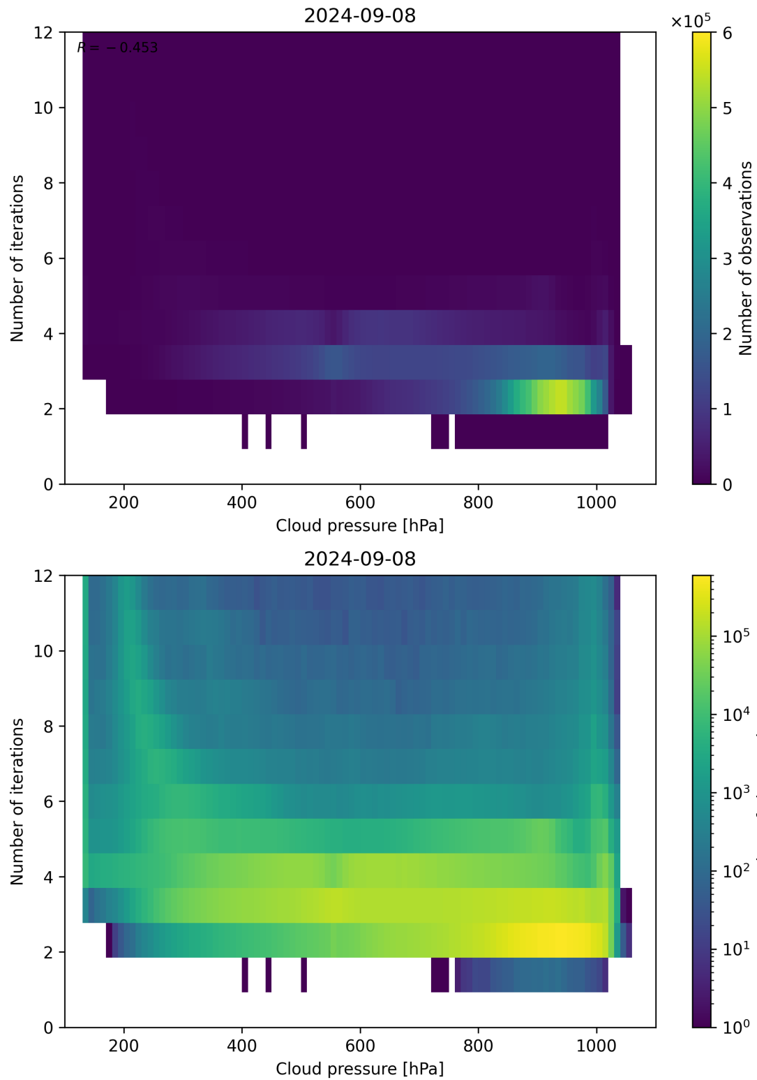
Figure 89: Scatter density plot of “Cloud pressure” against “Number of iterations” for 2024-09-07 to 2024-09-09.
