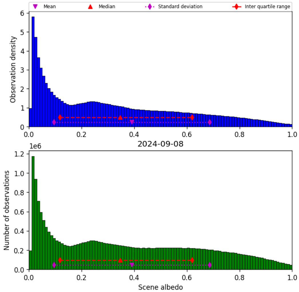
Figure 34: Histogram of “Scene albedo” for 2024-09-07 to 2024-09-09
