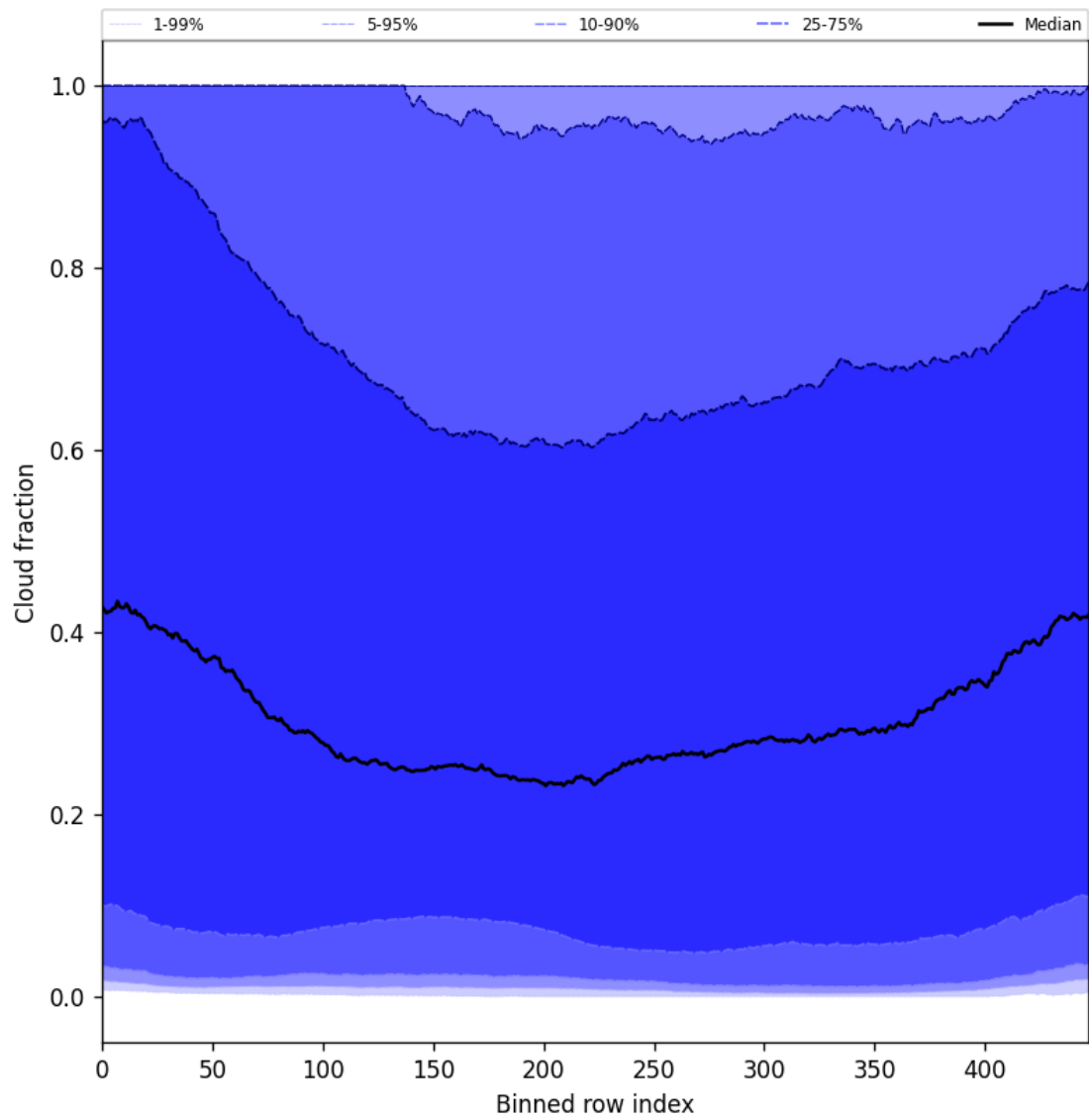
Figure 49: Along track statistics of “Cloud fraction” for 2024-09-07 to 2024-09-09
