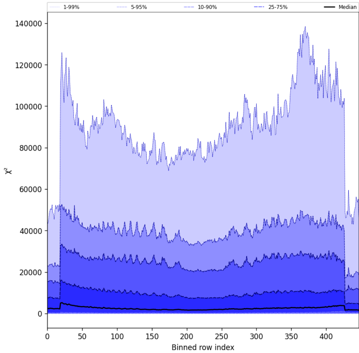
Figure 55: Along track statistics of “ \chi^2 ” for 2024-09-07 to 2024-09-09
