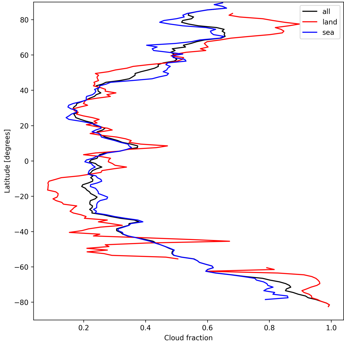
Figure 15: Zonal average of “Cloud fraction” for 2024-09-07 to 2024-09-09.
