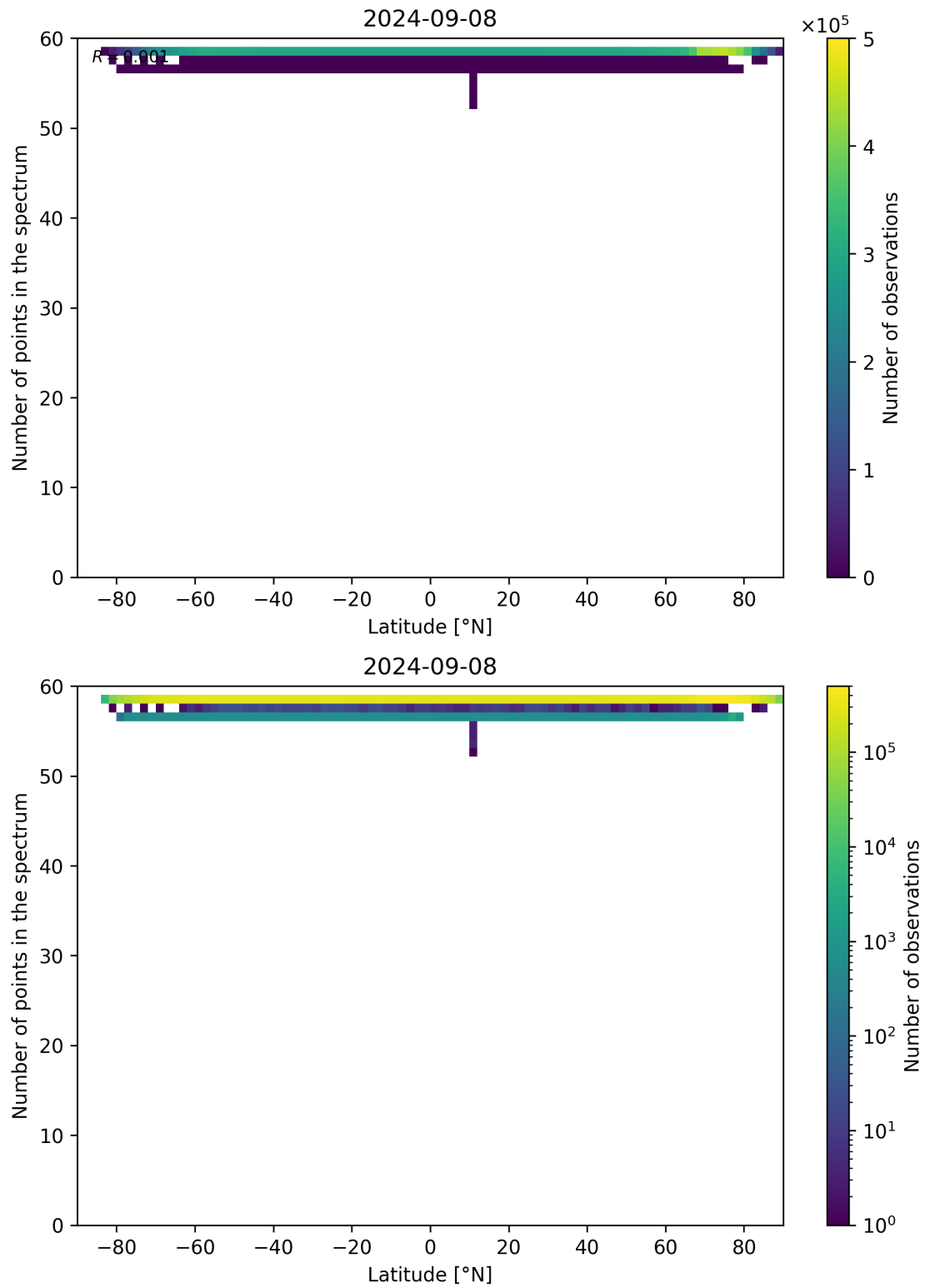
Figure 103: Scatter density plot of “Latitude” against “Number of points in the spectrum” for 2024-09-07 to 2024-09-09.
