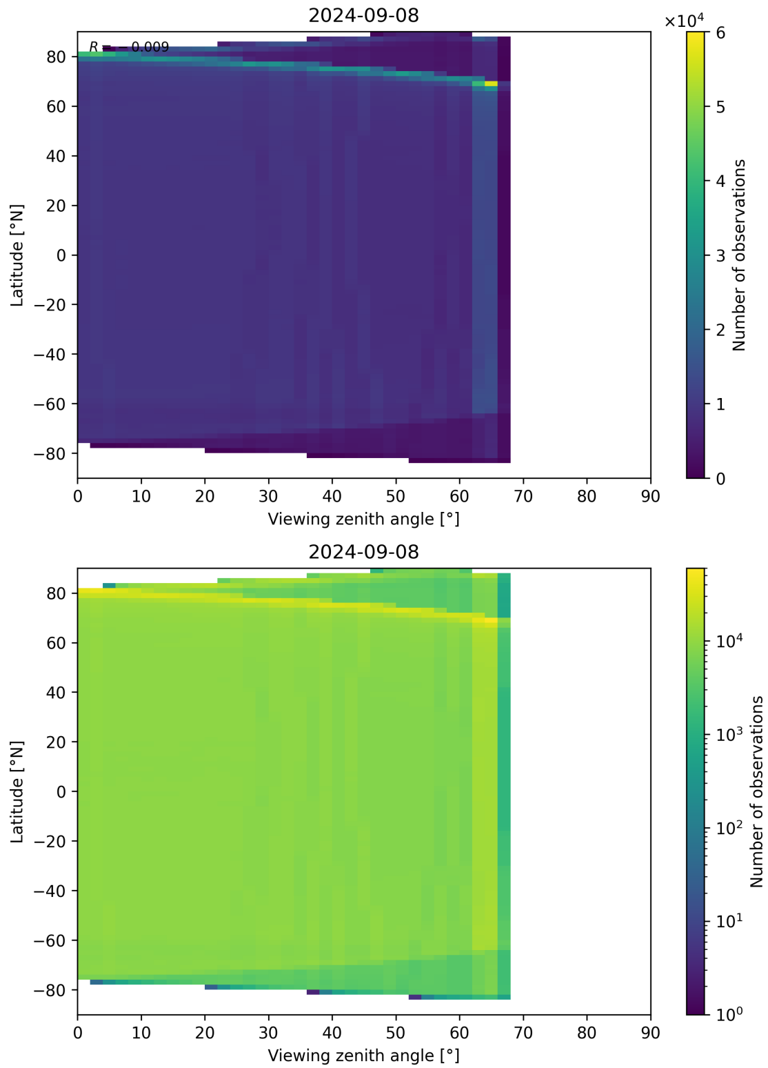
Figure 135: Scatter density plot of “Viewing zenith angle” against “Latitude” for 2024-09-07 to 2024-09-09.
