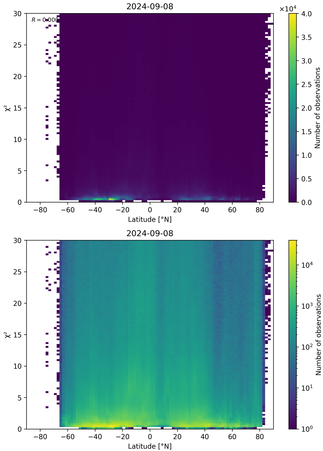
Figure 97: Scatter density plot of “Latitude” against “ \chi^2 ” for 2024-09-07 to 2024-09-09.
