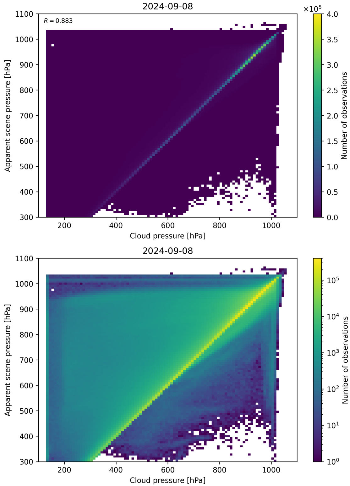
Figure 84: Scatter density plot of “Cloud pressure” against “Apparent scene pressure” for 2024-09-07 to 2024-09-09.
