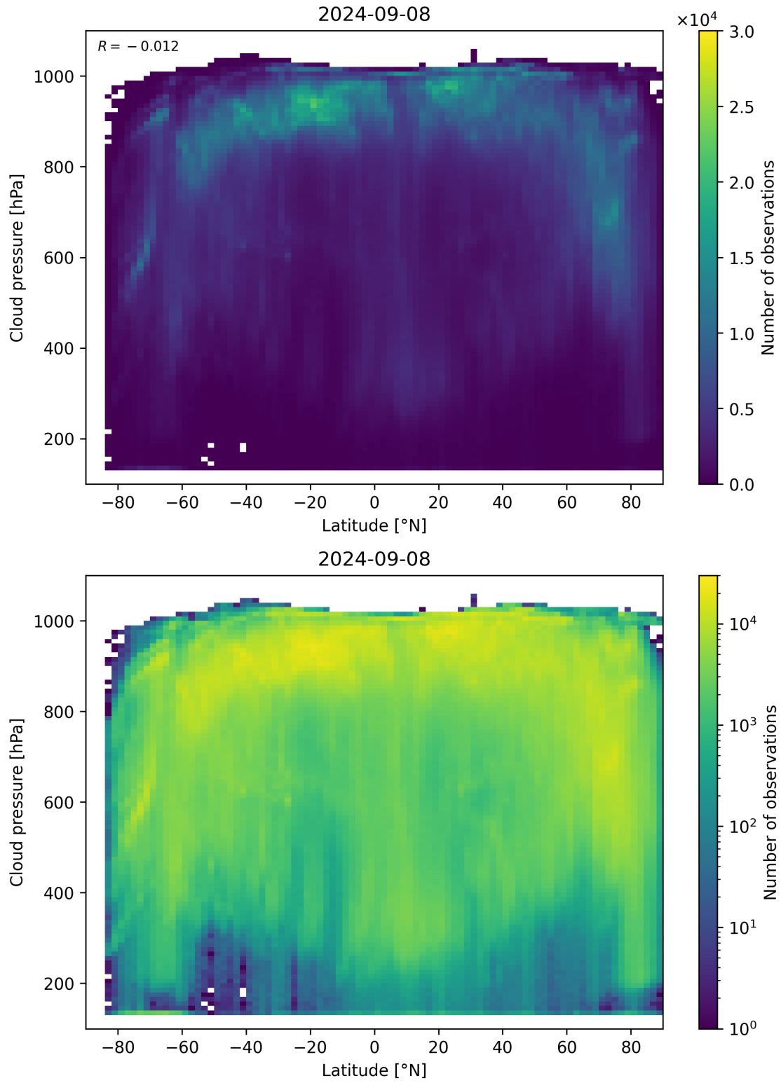
Figure 100: Scatter density plot of “Latitude” against “Cloud pressure” for 2024-09-07 to 2024-09-09.
