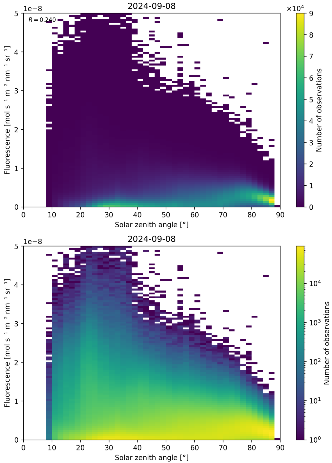
Figure 123: Scatter density plot of “Solar zenith angle” against “Fluorescence” for 2024-09-07 to 2024-09-09.
