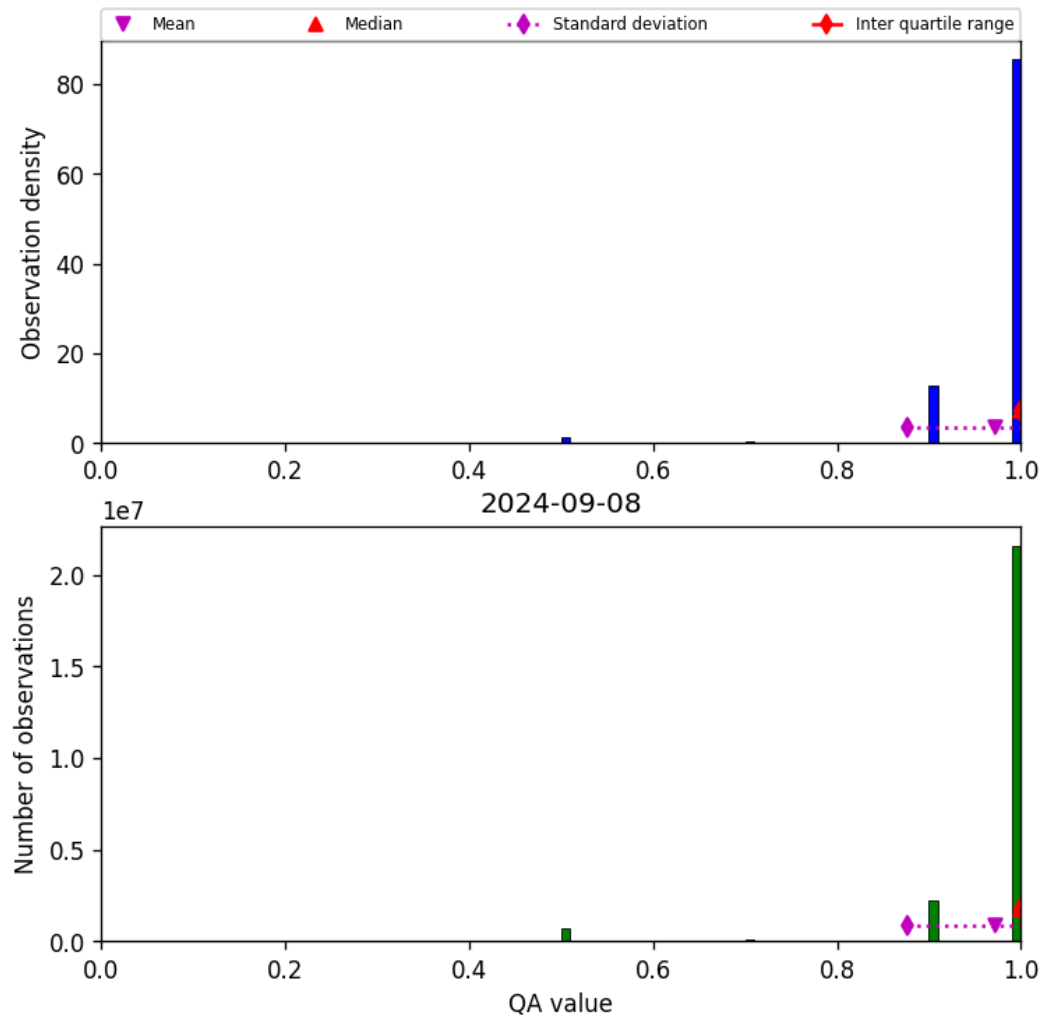
Figure 29: Histogram of “QA value” for 2024-09-07 to 2024-09-09
