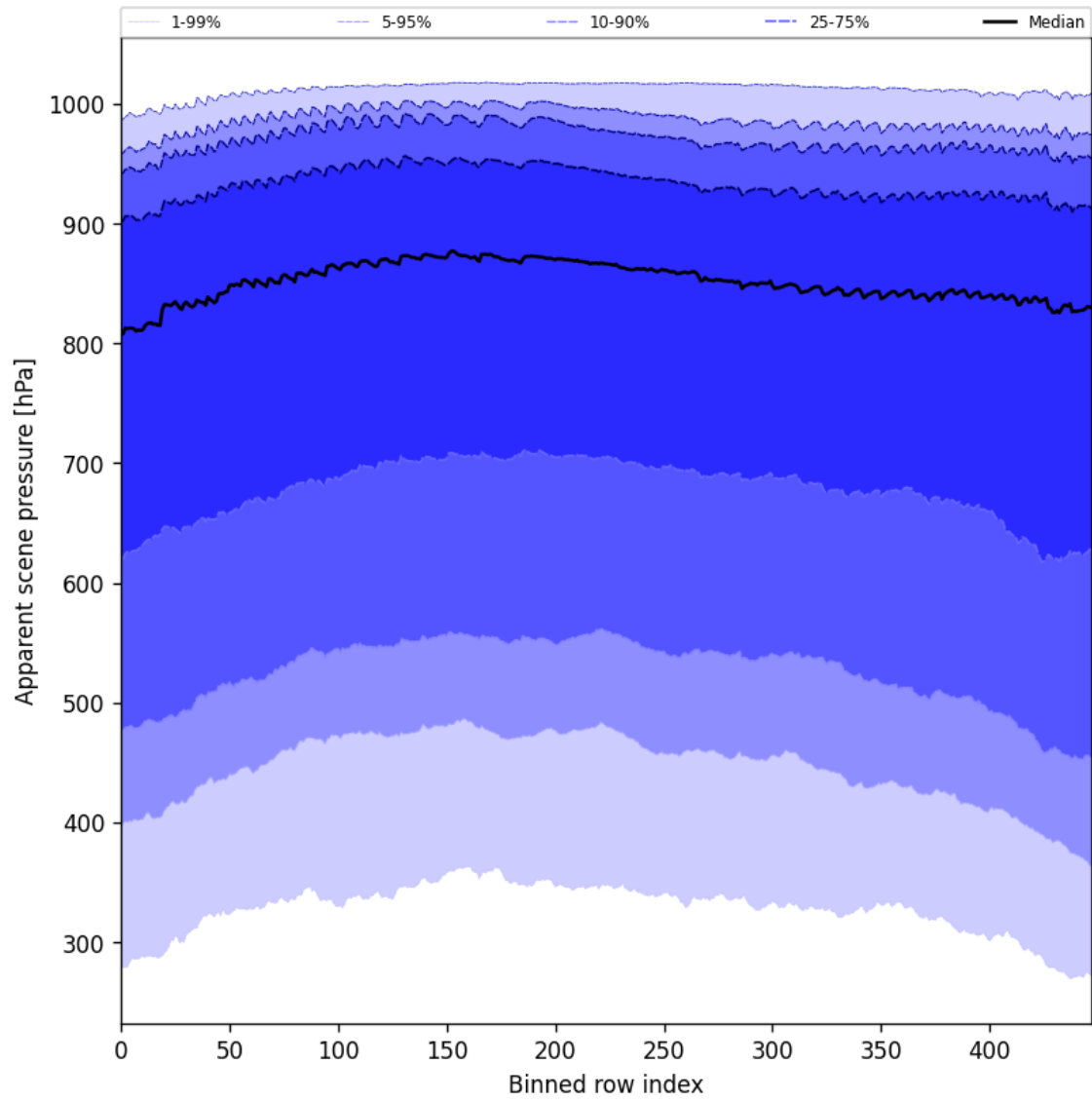
Figure 53: Along track statistics of “Apparent scene pressure” for 2024-09-07 to 2024-09-09
