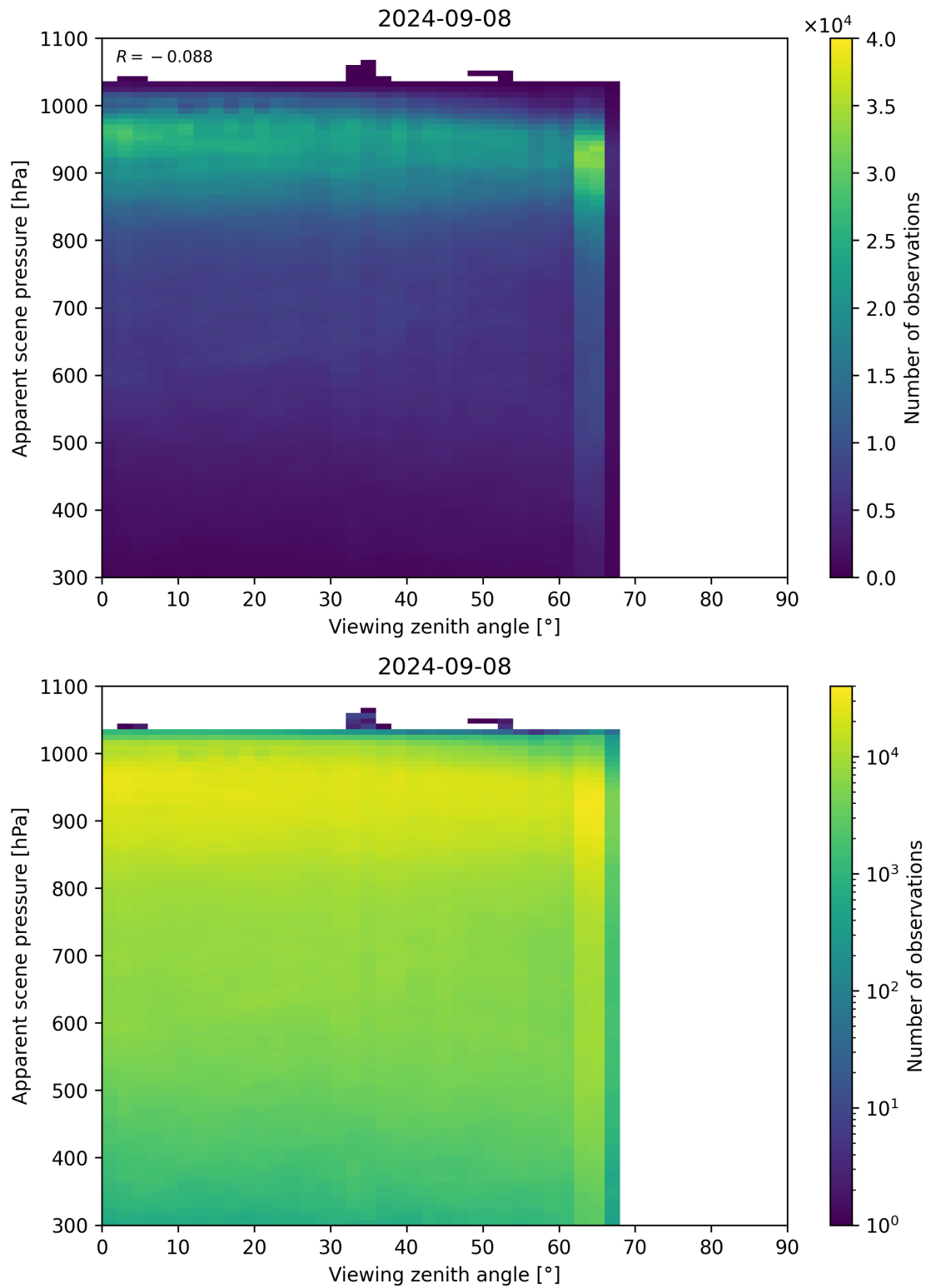
Figure 129: Scatter density plot of “Viewing zenith angle” against “Apparent scene pressure” for 2024-09-07 to 2024-09-09.
