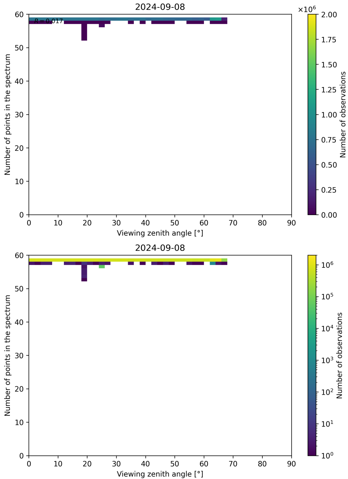
Figure 137: Scatter density plot of “Viewing zenith angle” against “Number of points in the spectrum” for 2024-09-07 to 2024-09-09.
