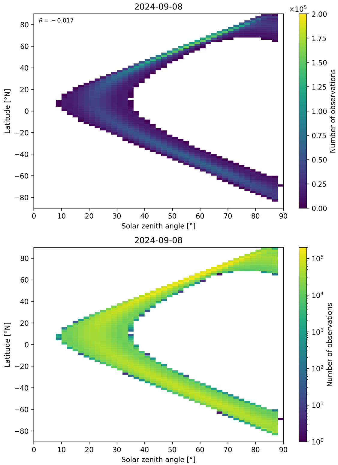
Figure 124: Scatter density plot of “Solar zenith angle” against “Latitude” for 2024-09-07 to 2024-09-09.
