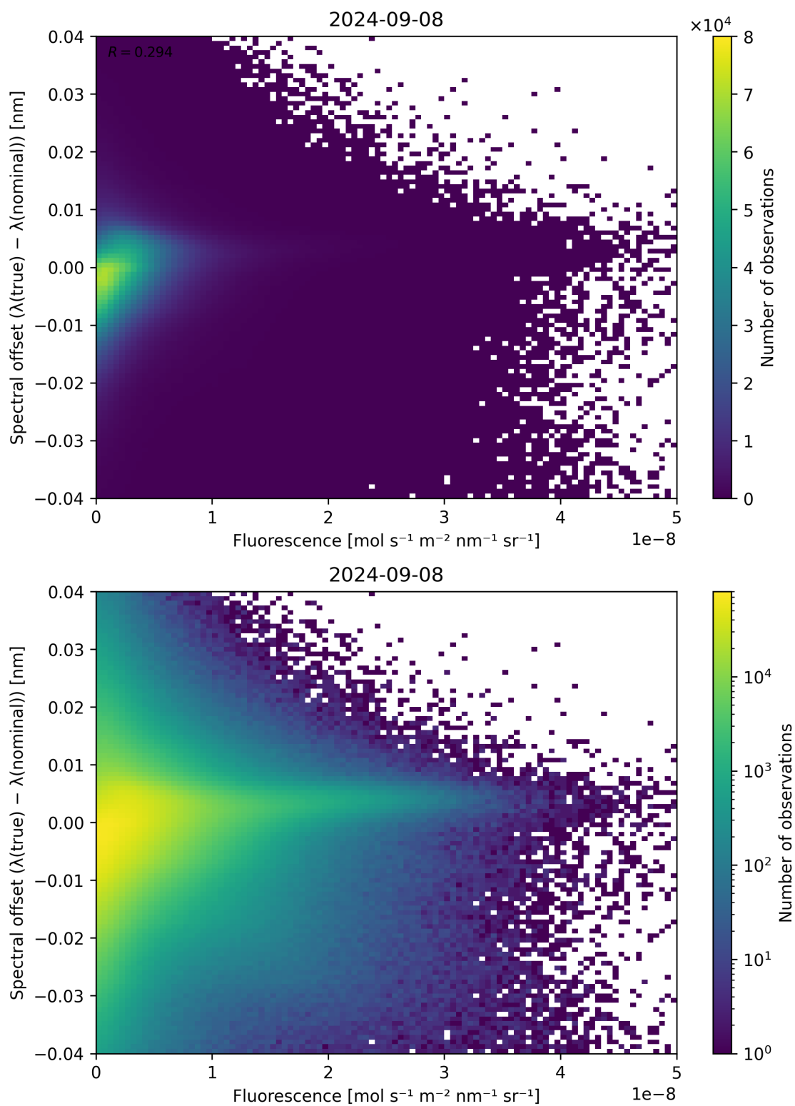
Figure 95: Scatter density plot of “Fluorescence” against “Spectral offset ( \lambda_{\text{true}} - \lambda_{\text{nominal}} )” for 2024-09-07 to 2024-09-09.
