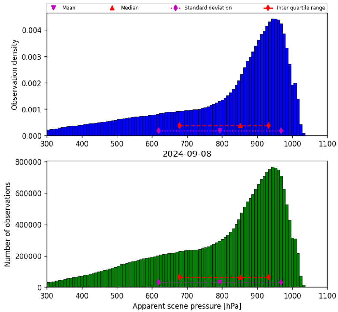
Figure 36: Histogram of “Apparent scene pressure” for 2024-09-07 to 2024-09-09
