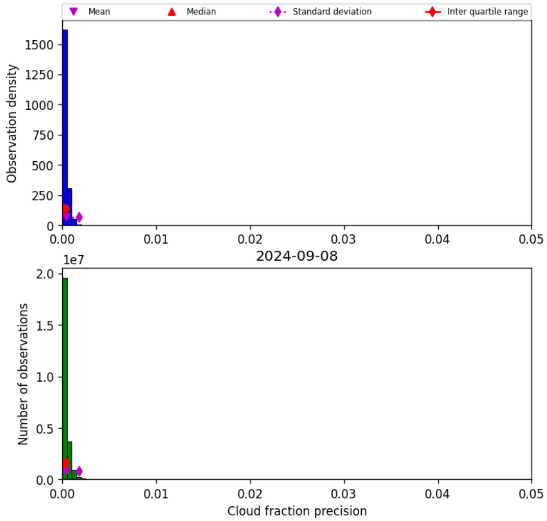
Figure 33: Histogram of “Cloud fraction precision” for 2024-09-07 to 2024-09-09
