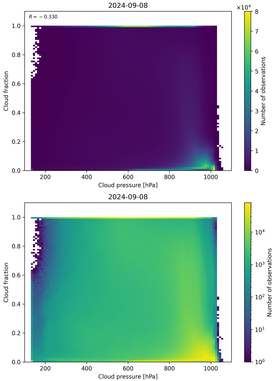
Figure 87: Scatter density plot of “Cloud pressure” against “Cloud fraction” for 2024-09-07 to 2024-09-09.
