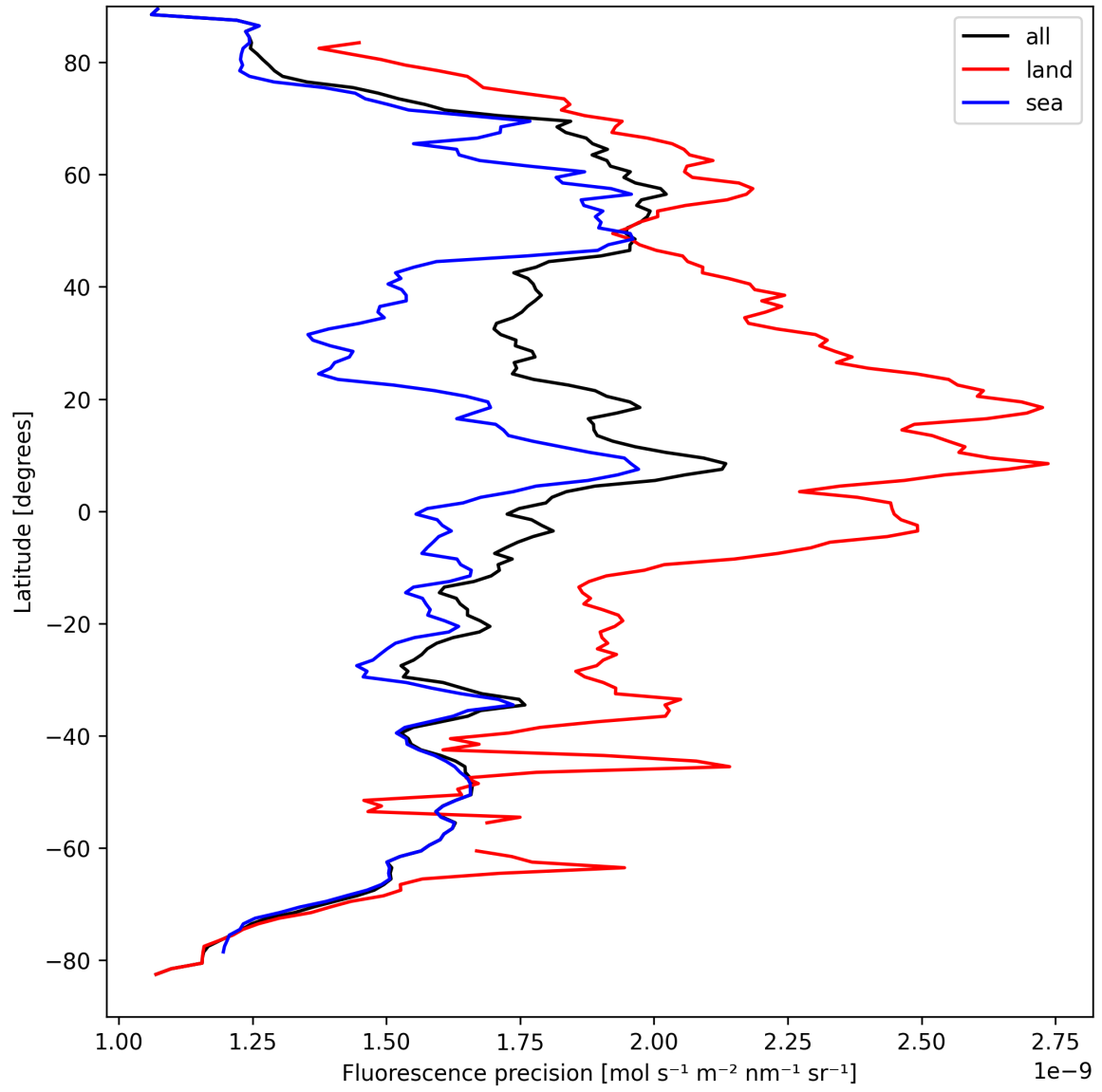
Figure 24: Zonal average of “Fluorescence precision” for 2024-09-07 to 2024-09-09.
