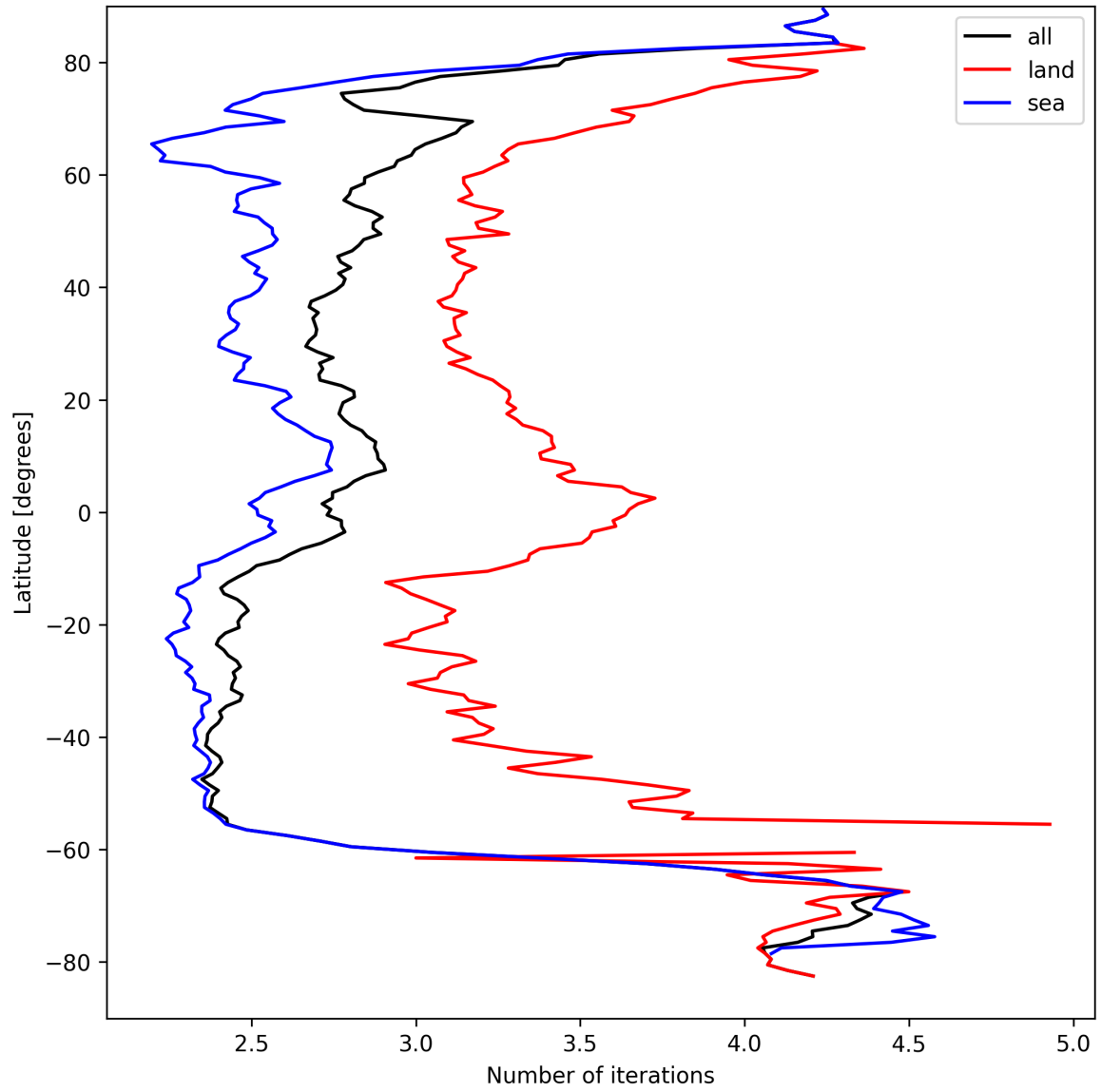
Figure 22: Zonal average of “Number of iterations” for 2024-09-07 to 2024-09-09.
