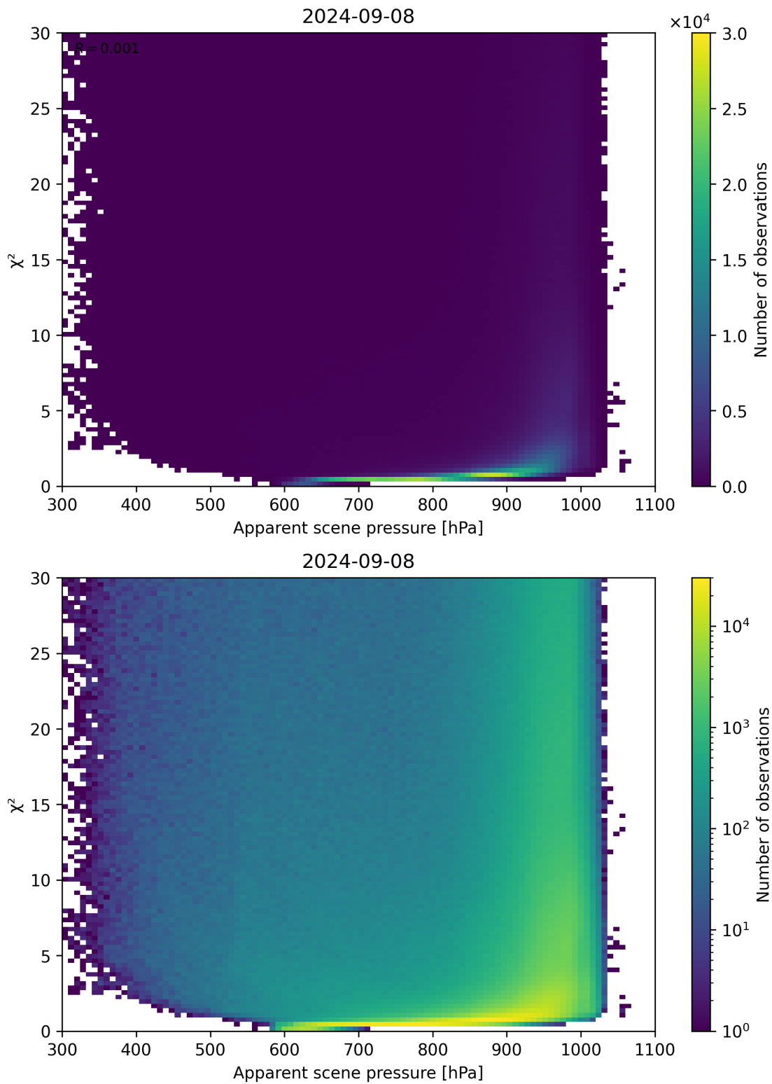
Figure 63: Scatter density plot of “Apparent scene pressure” against “ \chi^2 ” for 2024-09-07 to 2024-09-09.
