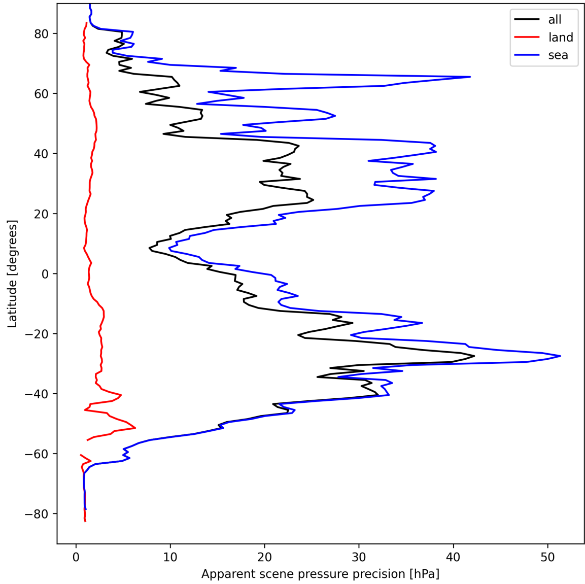
Figure 20: Zonal average of “Apparent scene pressure precision” for 2024-09-07 to 2024-09-09.
