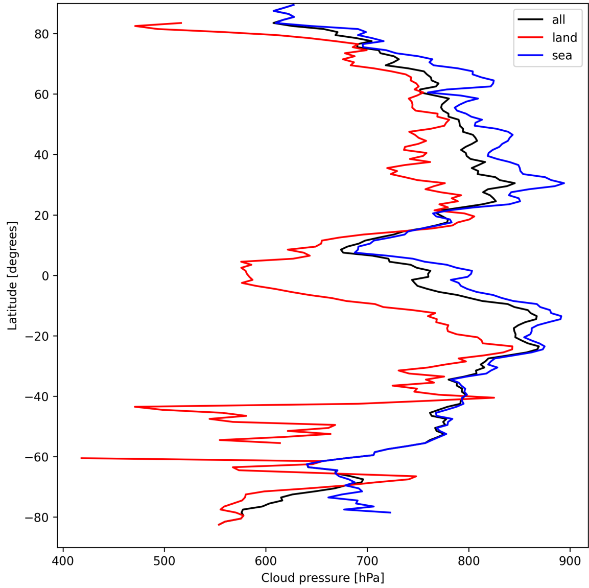
Figure 13: Zonal average of “Cloud pressure” for 2024-09-07 to 2024-09-09.
