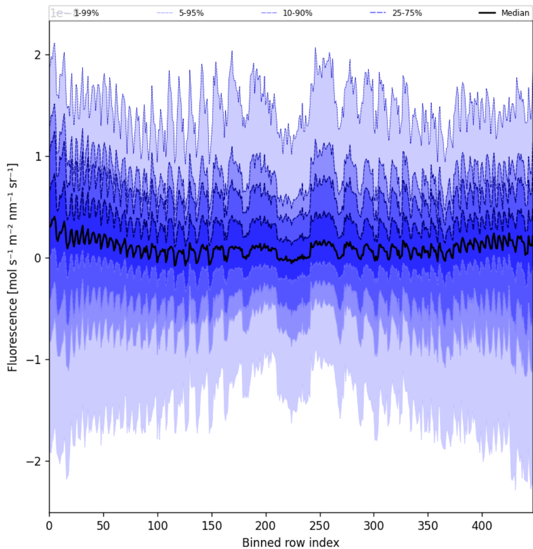
Figure 57: Along track statistics of “Fluorescence” for 2024-09-07 to 2024-09-09
