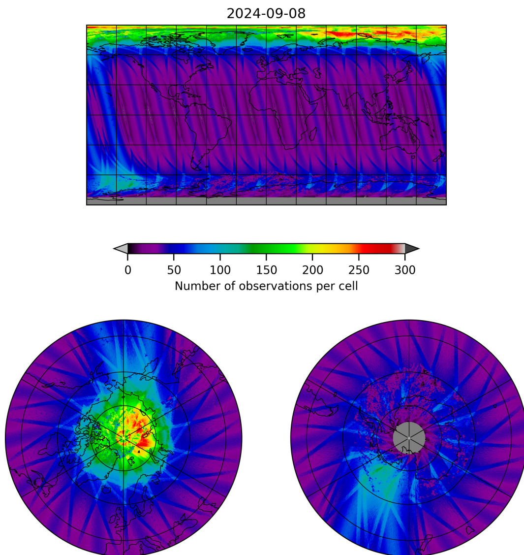
Figure 11: Map of the number of observations for 2024-09-07 to 2024-09-09
