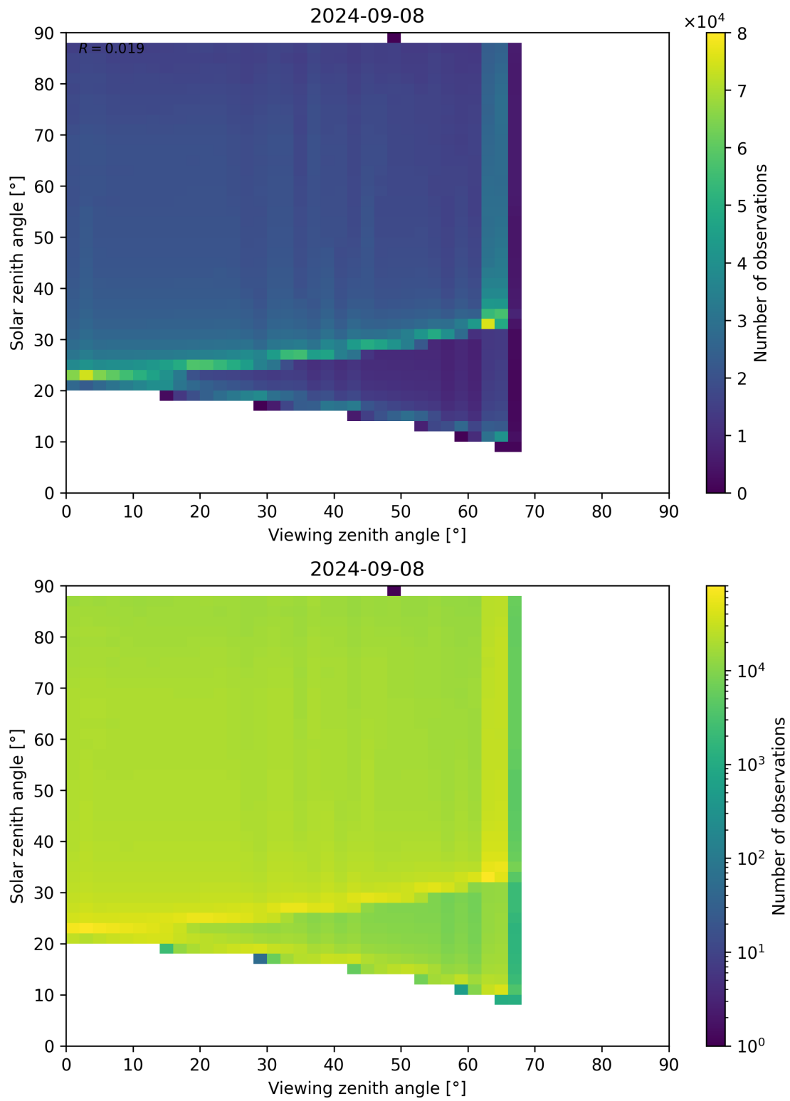
Figure 139: Scatter density plot of “Viewing zenith angle” against “Solar zenith angle” for 2024-09-07 to 2024-09-09.
