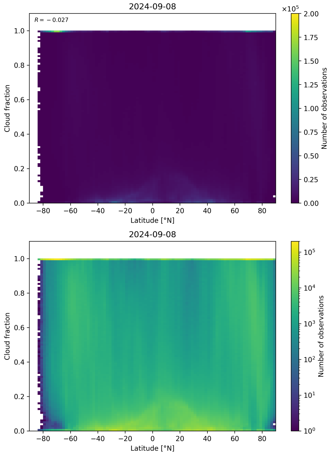
Figure 99: Scatter density plot of “Latitude” against “Cloud fraction” for 2024-09-07 to 2024-09-09.
