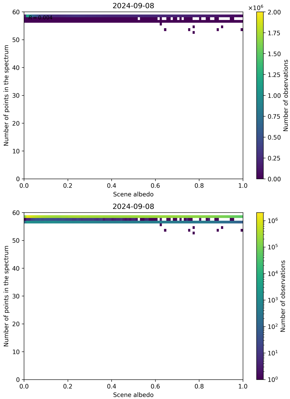
Figure 116: Scatter density plot of “Scene albedo” against “Number of points in the spectrum” for 2024-09-07 to 2024-09-09.
