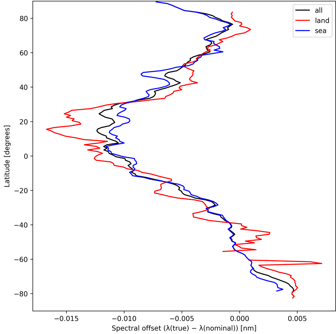
Figure 28: Zonal average of “Spectral offset ( \lambda_{\text{true}} - \lambda_{\text{nominal}} )” for 2024-09-07 to 2024-09-09.
