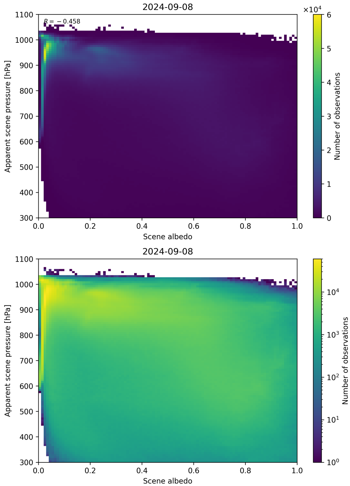
Figure 111: Scatter density plot of “Scene albedo” against “Apparent scene pressure” for 2024-09-07 to 2024-09-09.
