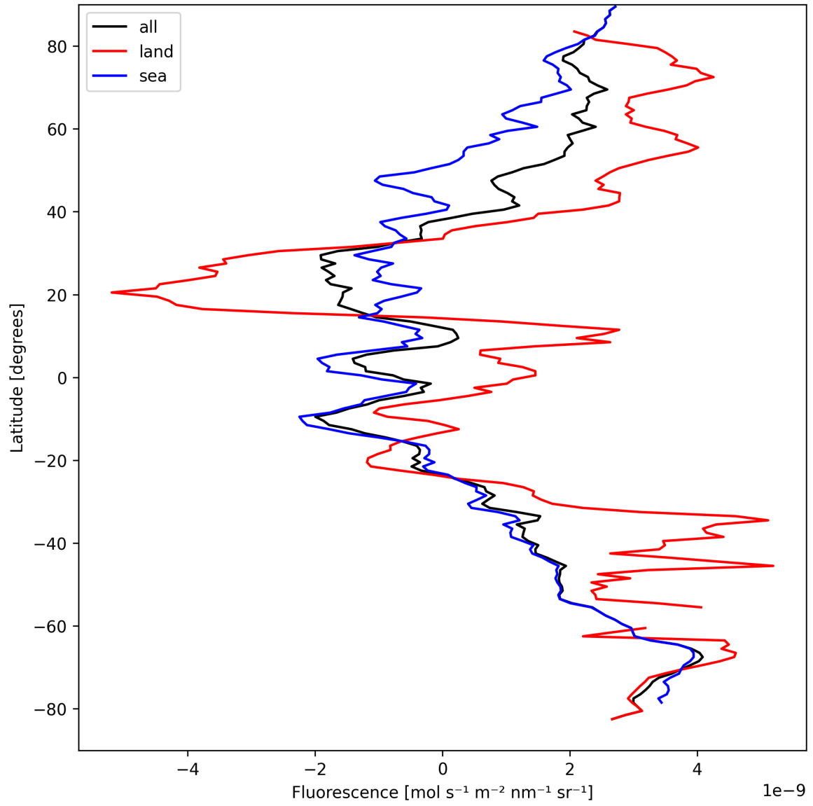
Figure 23: Zonal average of “Fluorescence” for 2024-09-07 to 2024-09-09.
