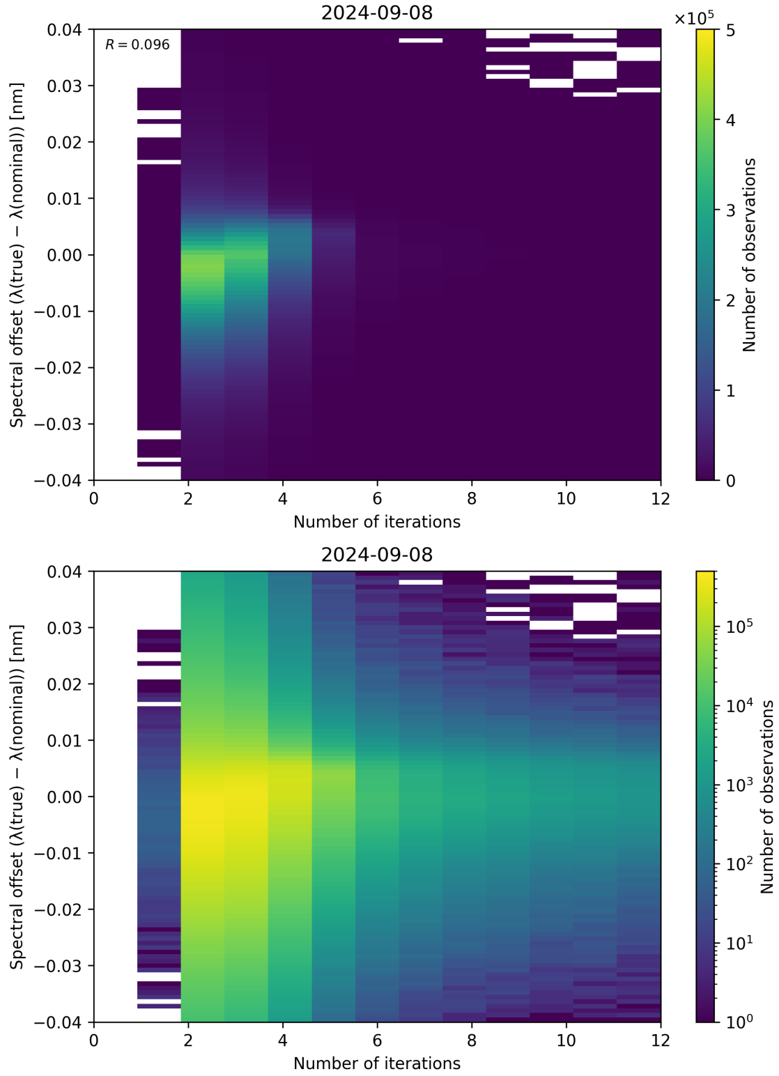
Figure 109: Scatter density plot of “Number of iterations” against “Spectral offset ( \lambda_{\text{true}} - \lambda_{\text{nominal}} )” for 2024-09-07 to 2024-09-09.
