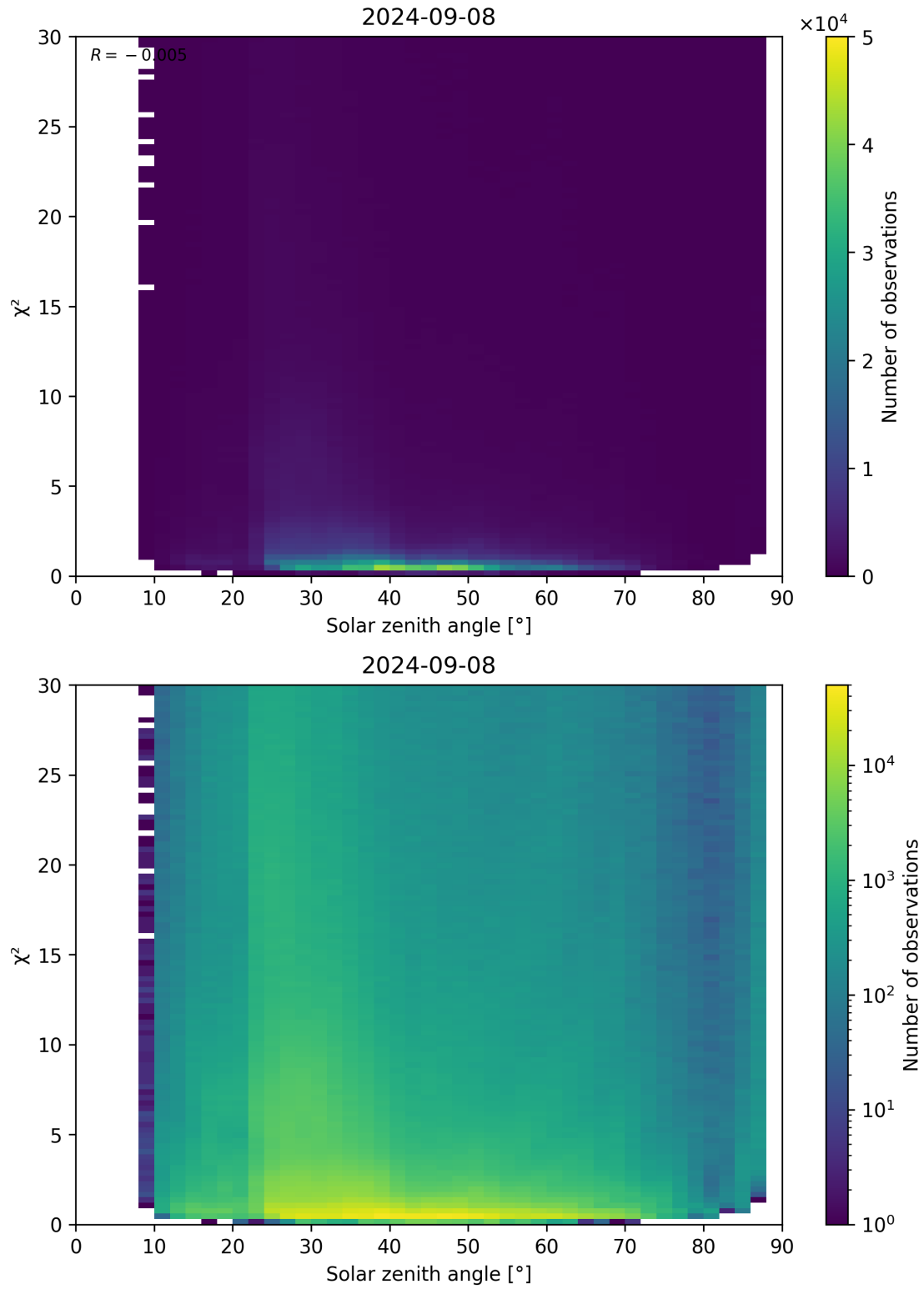
Figure 119: Scatter density plot of “Solar zenith angle” against “ \chi^2 ” for 2024-09-07 to 2024-09-09.
