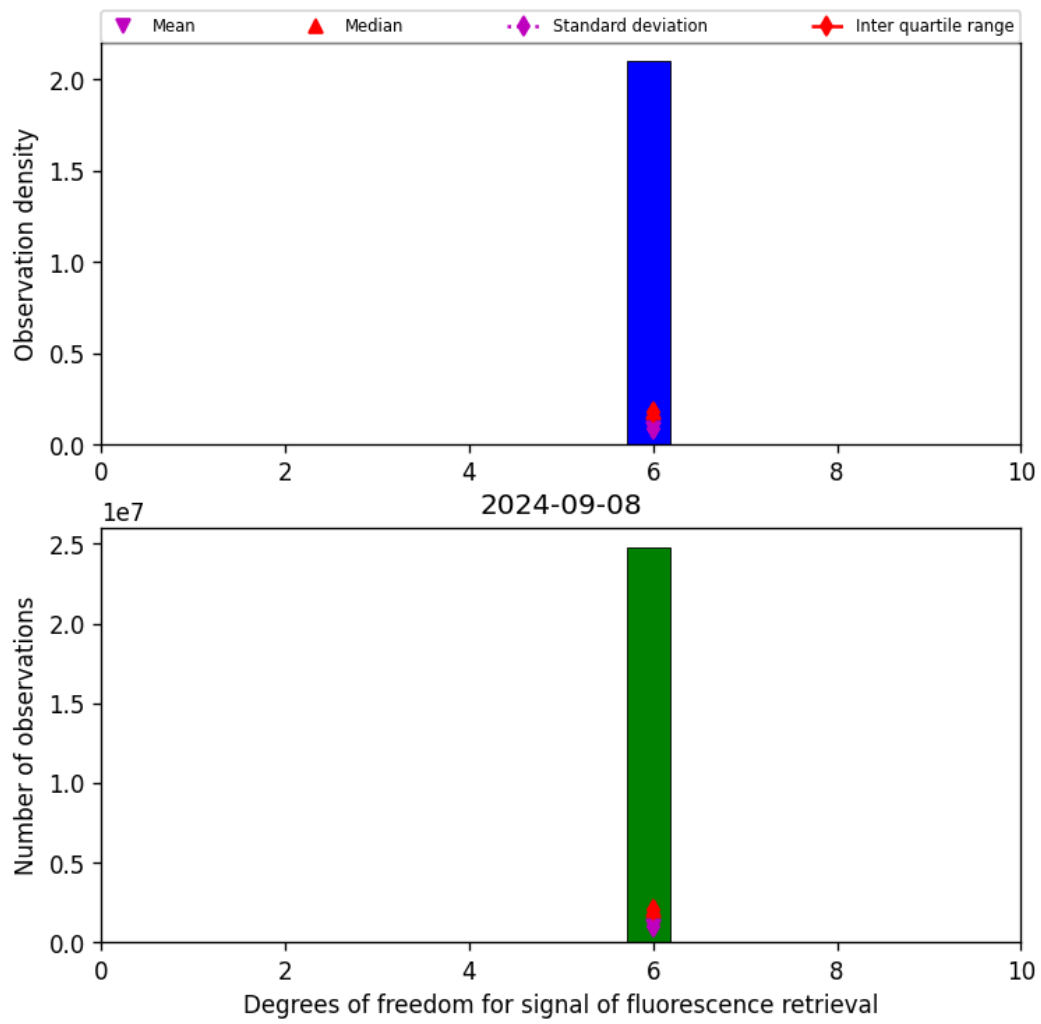
Figure 43: Histogram of "Degrees of freedom for signal of fluorescence retrieval" for 2024-09-07 to 2024-09-09
