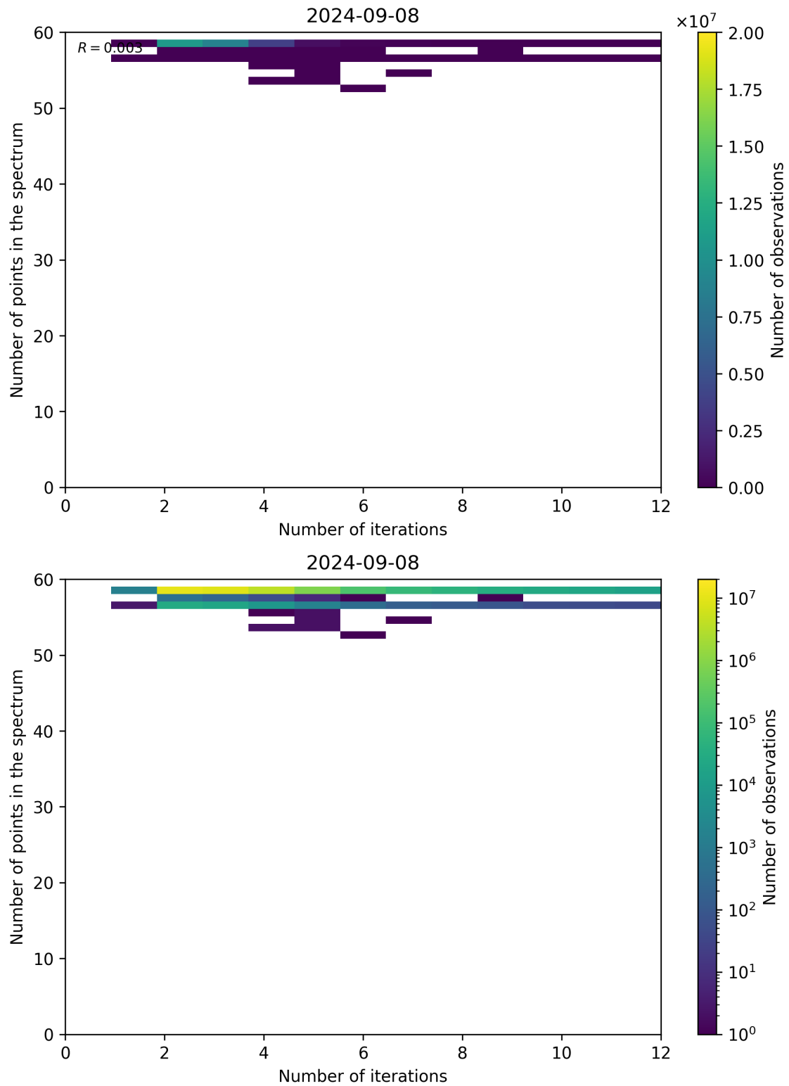
Figure 108: Scatter density plot of “Number of iterations” against “Number of points in the spectrum” for 2024-09-07 to 2024-09-09.
