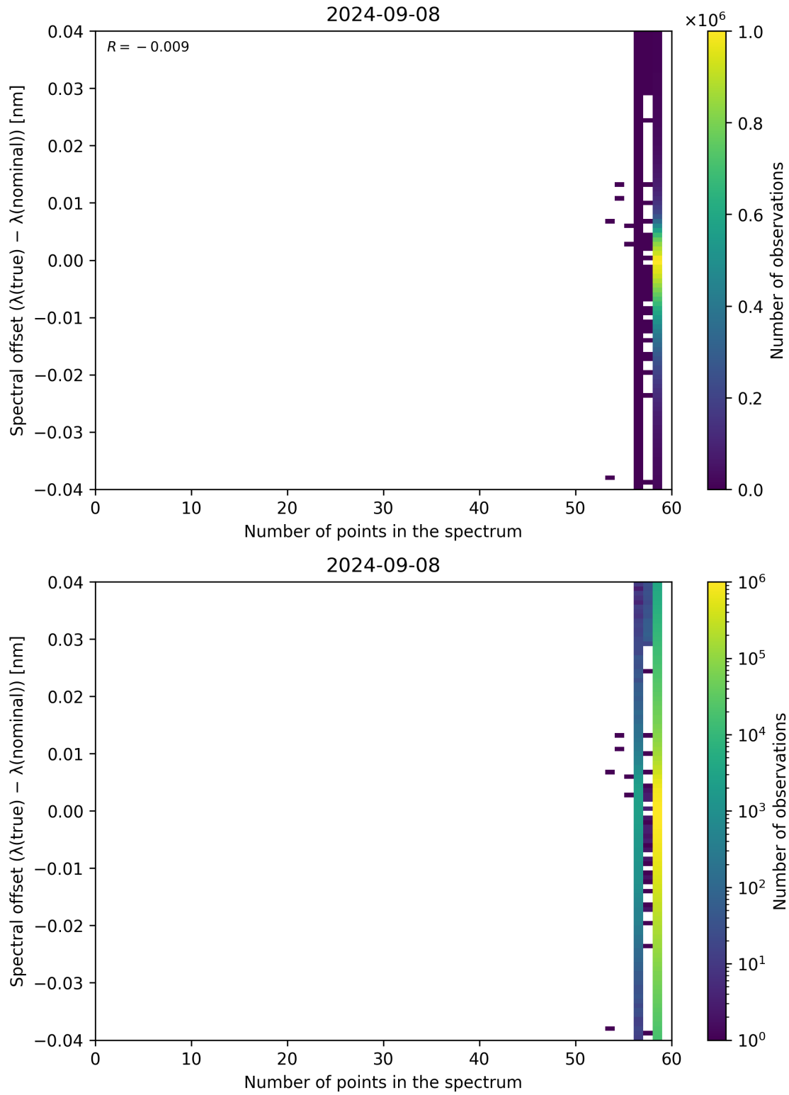
Figure 110: Scatter density plot of “Number of points in the spectrum” against “Spectral offset ( \lambda_{\text{true}} - \lambda_{\text{nominal}} )” for 2024-09-07 to 2024-09-09.
