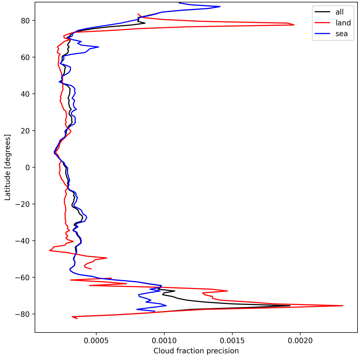
Figure 16: Zonal average of “Cloud fraction precision” for 2024-09-07 to 2024-09-09.
