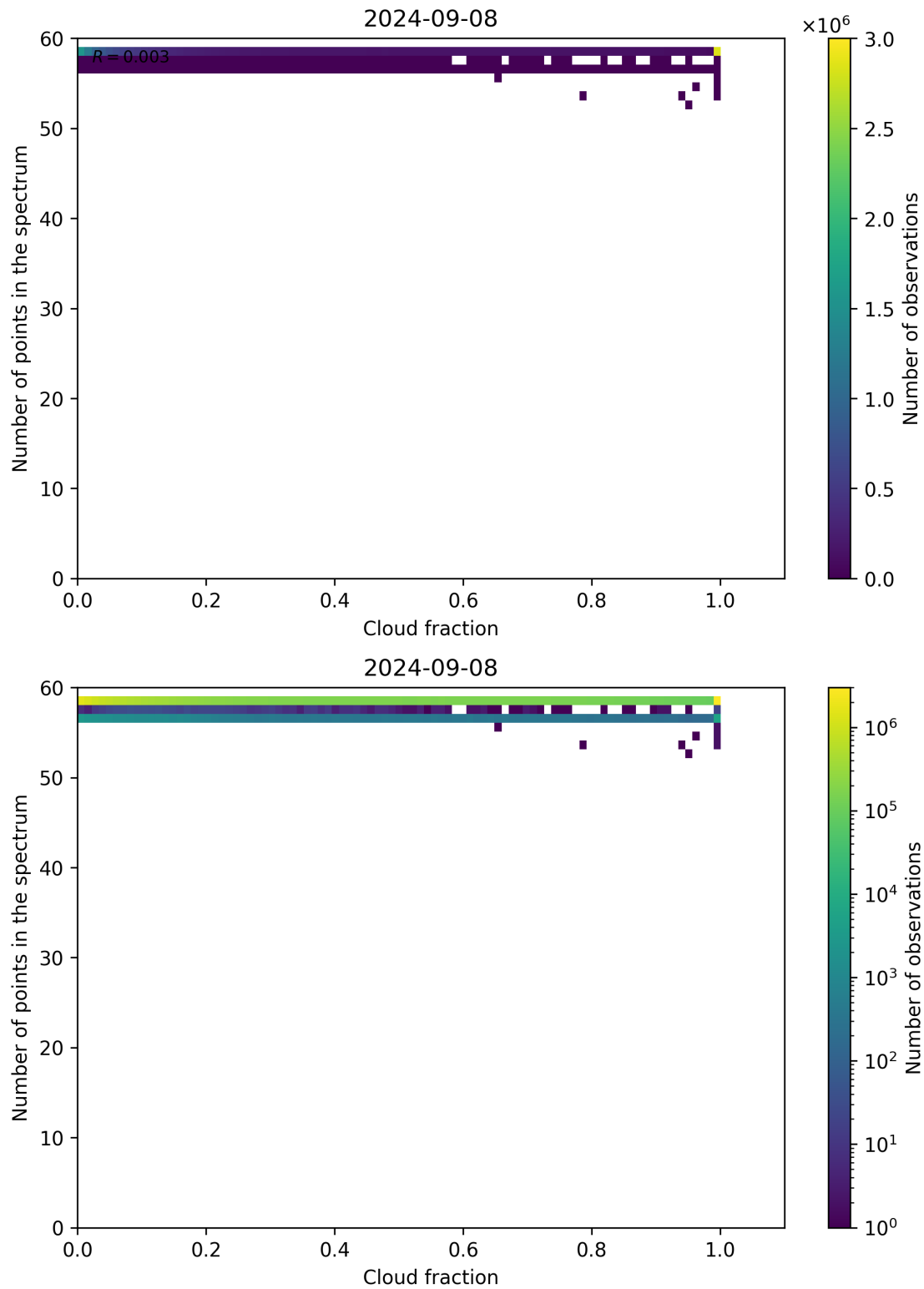
Figure 81: Scatter density plot of “Cloud fraction” against “Number of points in the spectrum” for 2024-09-07 to 2024-09-09.
