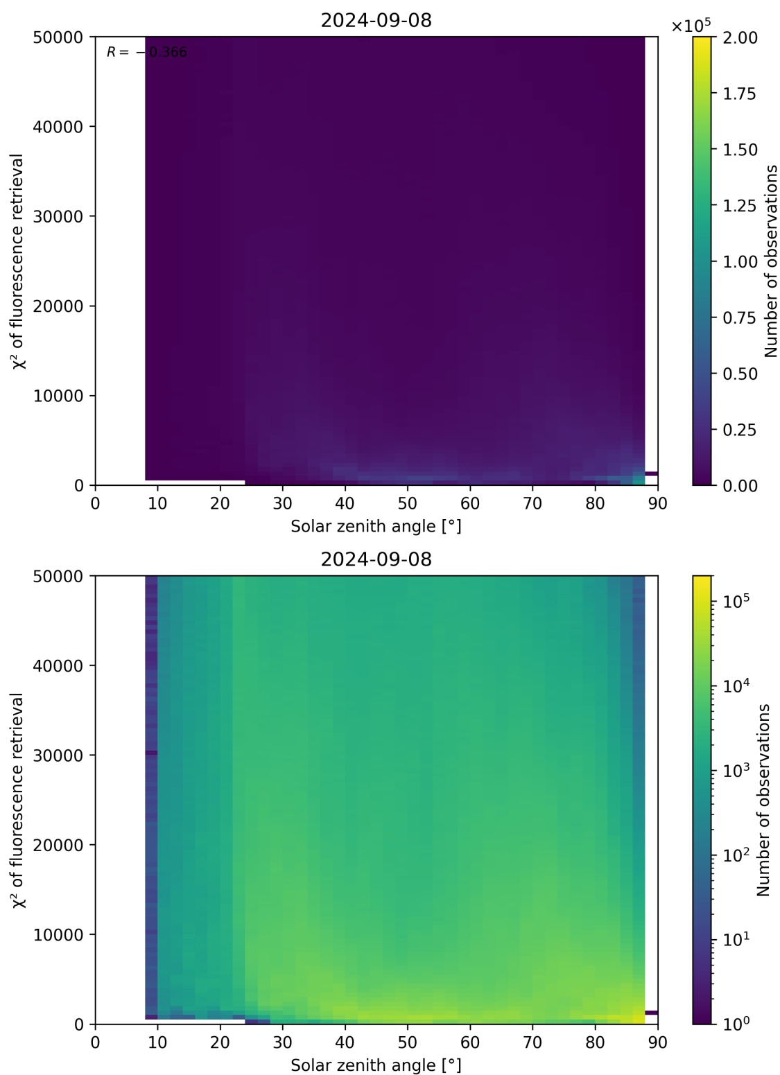
Figure 120: Scatter density plot of “Solar zenith angle” against “ \chi^2 of fluorescence retrieval” for 2024-09-07 to 2024-09-09.
