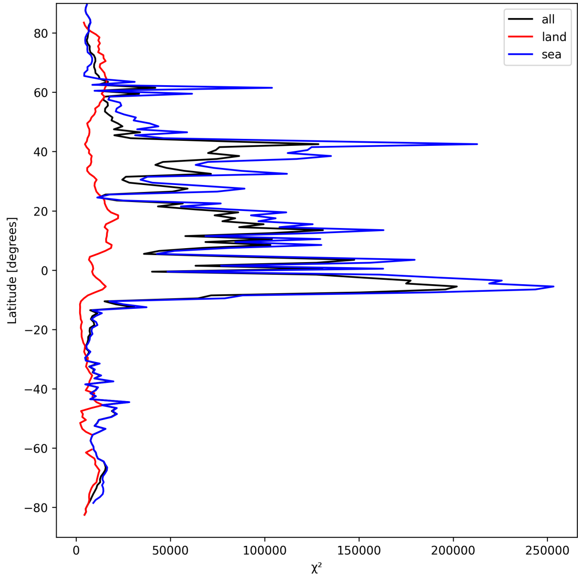
Figure 21: Zonal average of “ \chi^2 ” for 2024-09-07 to 2024-09-09.
