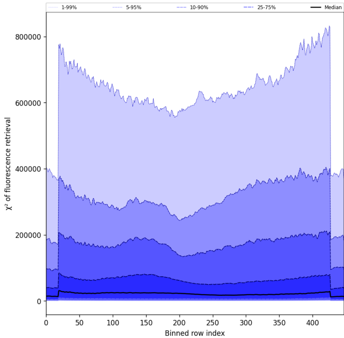
Figure 59: Along track statistics of “ \chi^2 of fluorescence retrieval” for 2024-09-07 to 2024-09-09
