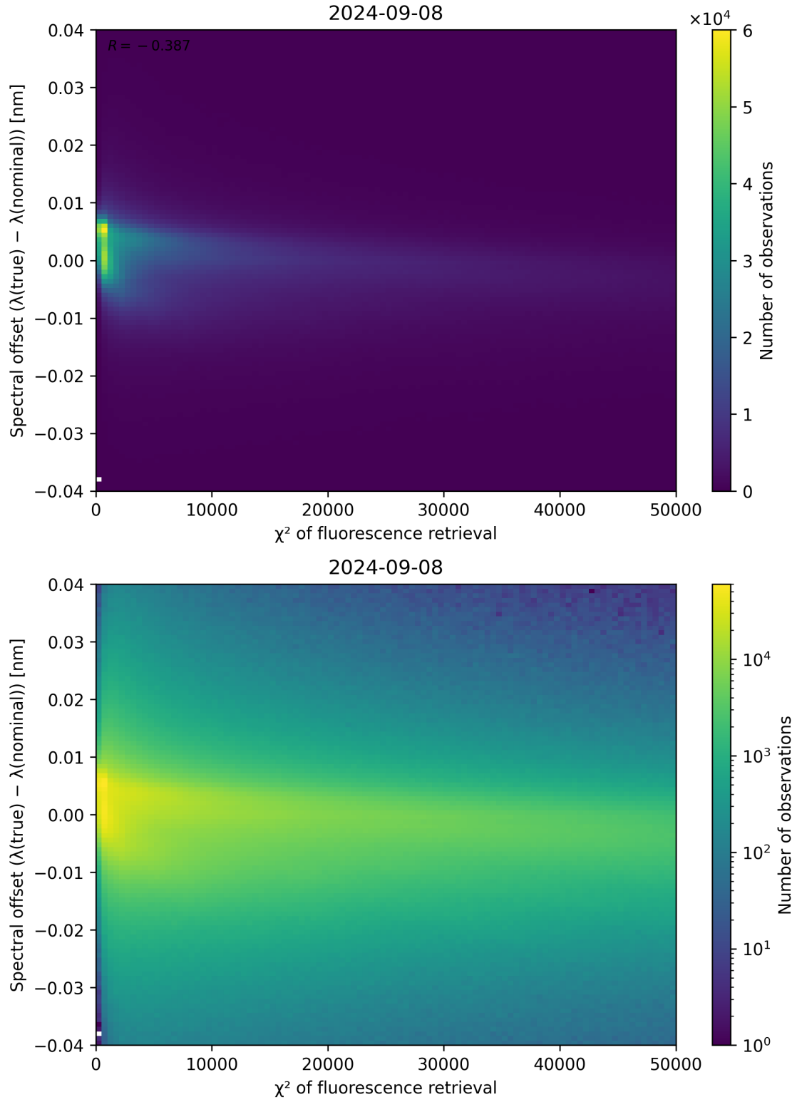
Figure 72: Scatter density plot of “ \chi^2 of fluorescence retrieval” against “Spectral offset ( \lambda_{\text{true}} - \lambda_{\text{nominal}} )” for 2024-09-07 to 2024-09-09.
