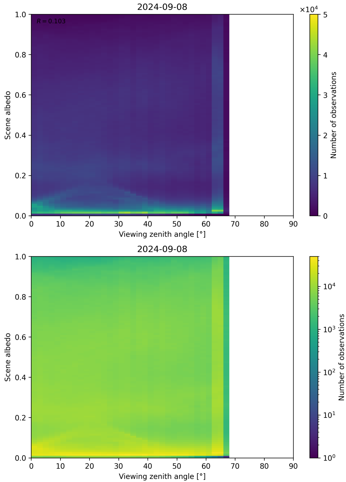
Figure 138: Scatter density plot of “Viewing zenith angle” against “Scene albedo” for 2024-09-07 to 2024-09-09.
