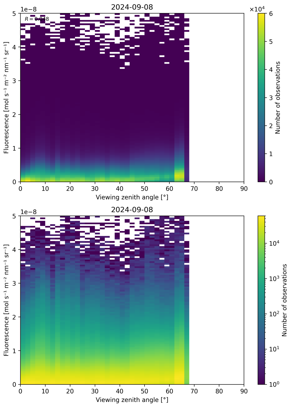
Figure 134: Scatter density plot of “Viewing zenith angle” against “Fluorescence” for 2024-09-07 to 2024-09-09.
