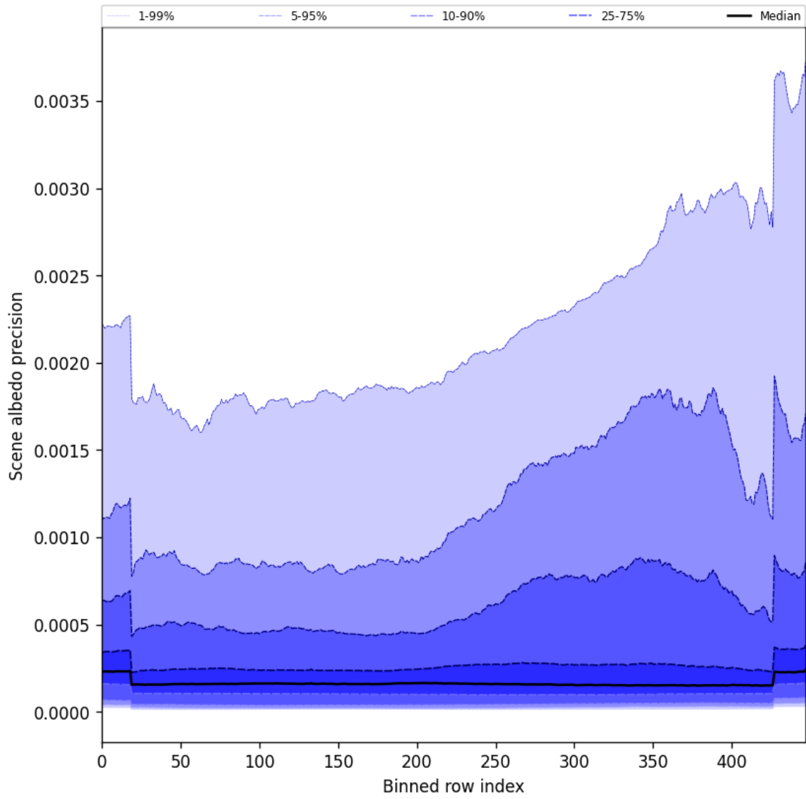
Figure 52: Along track statistics of “Scene albedo precision” for 2024-09-07 to 2024-09-09
