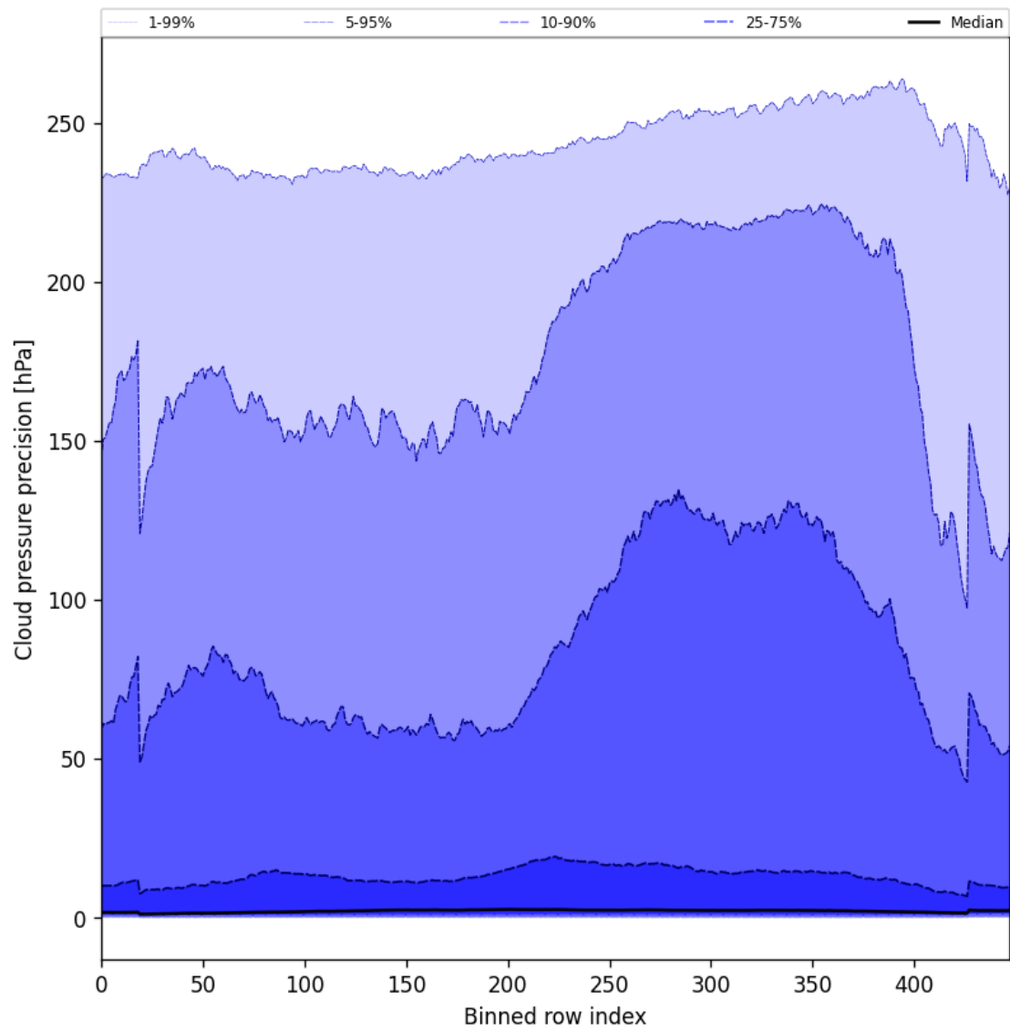
Figure 48: Along track statistics of “Cloud pressure precision” for 2024-09-07 to 2024-09-09
