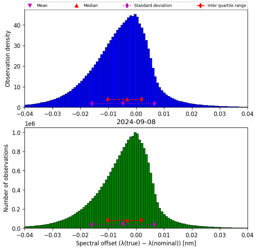
Figure 45: Histogram of “Spectral offset ( \lambda_{\text{true}} - \lambda_{\text{nominal}} )” for 2024-09-07 to 2024-09-09
