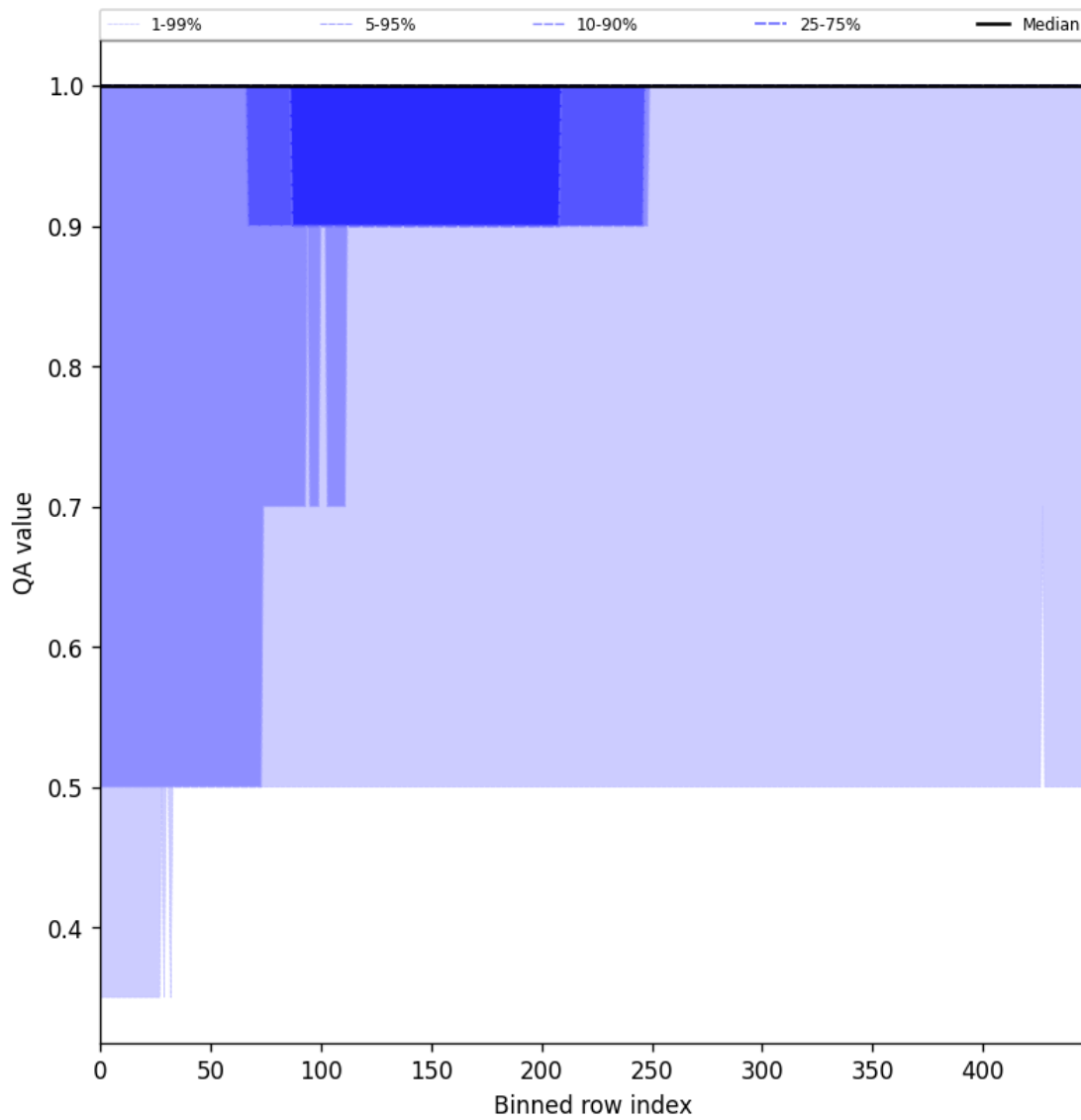
Figure 46: Along track statistics of “QA value” for 2024-09-07 to 2024-09-09
