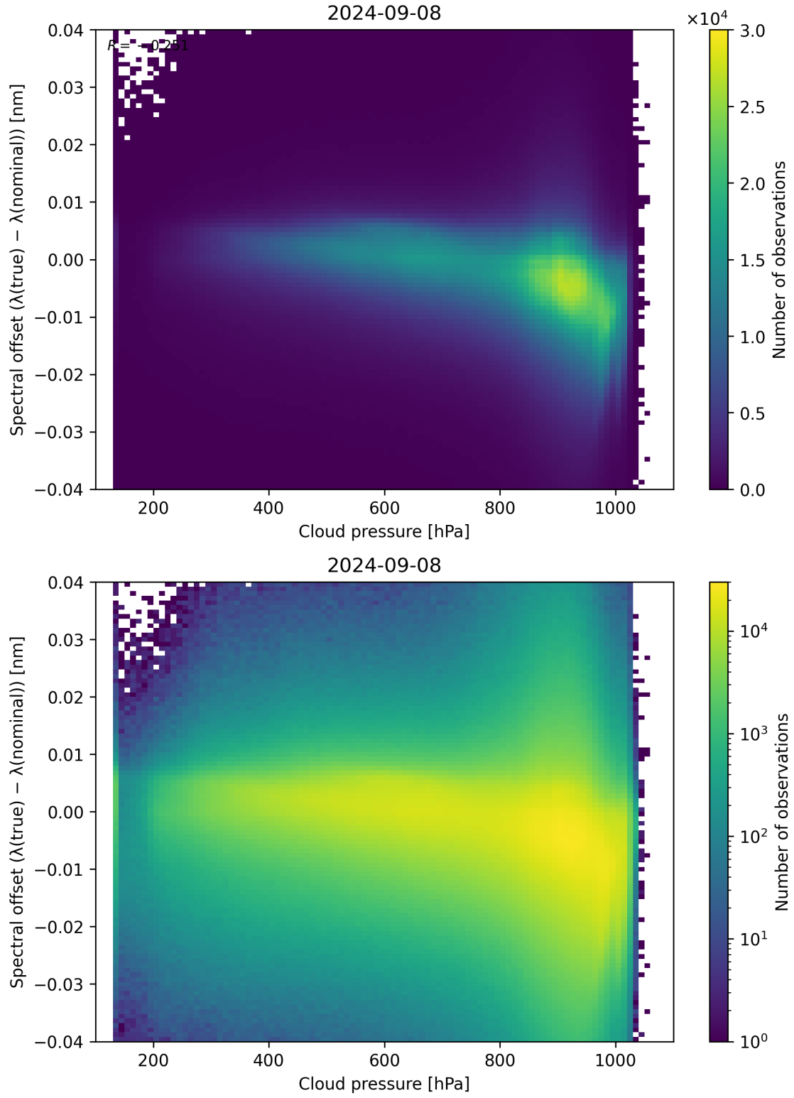
Figure 92: Scatter density plot of “Cloud pressure” against “Spectral offset ( \lambda_{\text{true}} - \lambda_{\text{nominal}} )” for 2024-09-07 to 2024-09-09.
