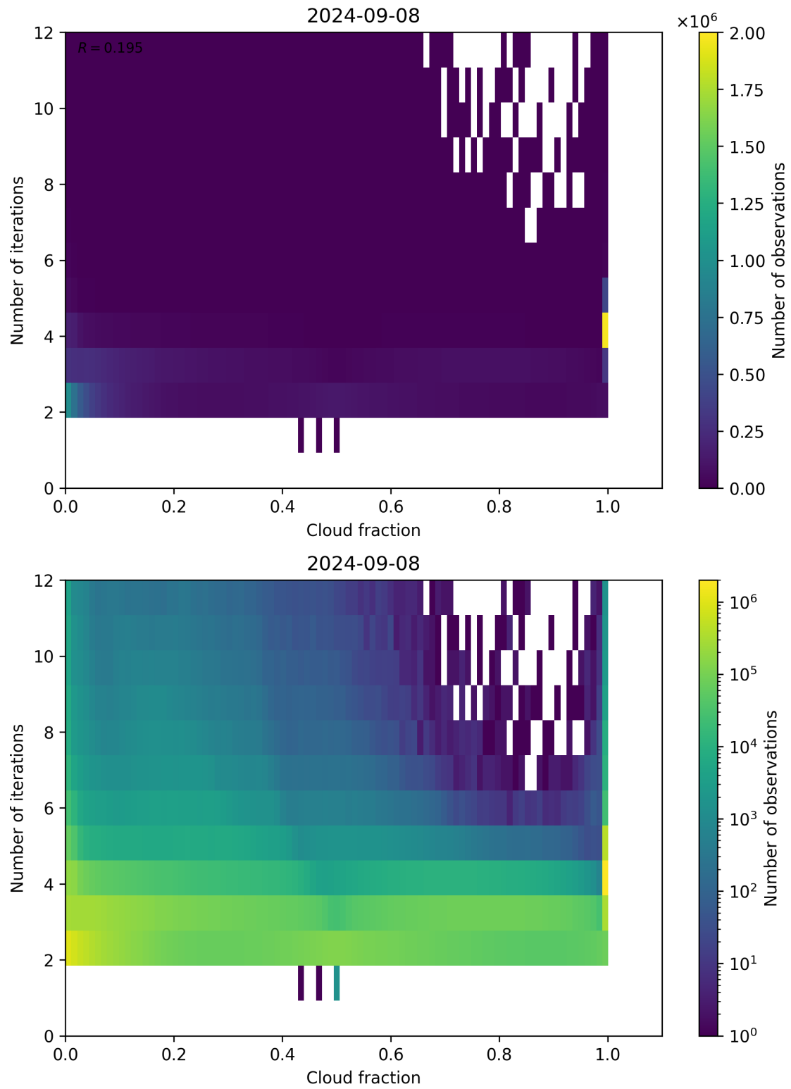
Figure 80: Scatter density plot of “Cloud fraction” against “Number of iterations” for 2024-09-07 to 2024-09-09.
