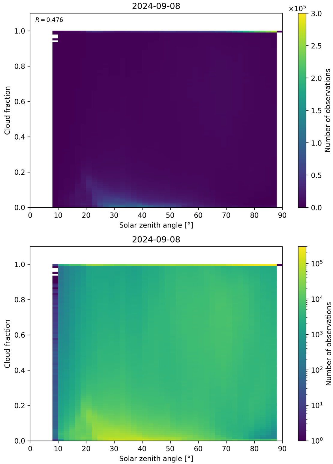
Figure 121: Scatter density plot of “Solar zenith angle” against “Cloud fraction” for 2024-09-07 to 2024-09-09.
