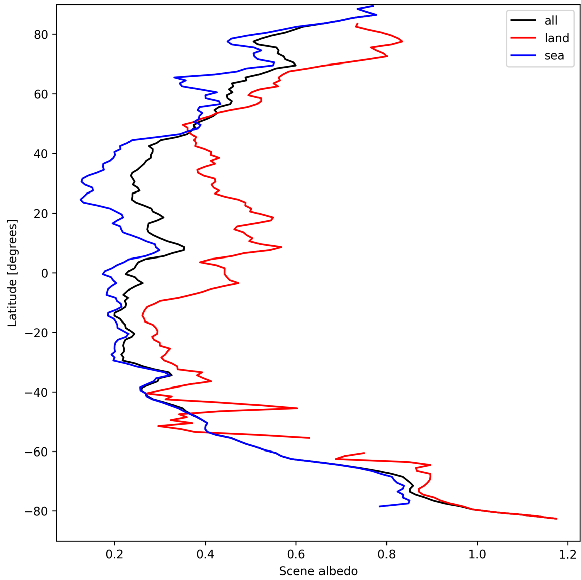
Figure 17: Zonal average of “Scene albedo” for 2024-09-07 to 2024-09-09.
