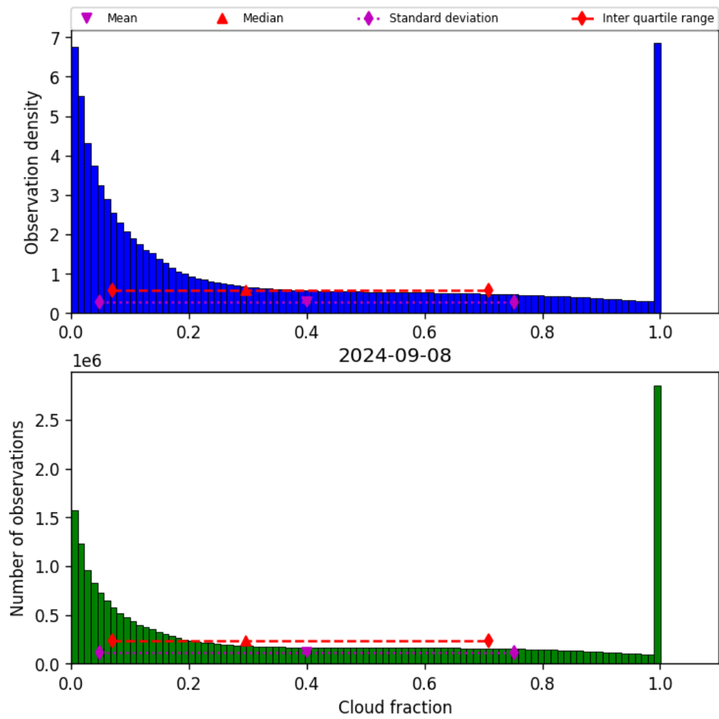
Figure 32: Histogram of “Cloud fraction” for 2024-09-07 to 2024-09-09
