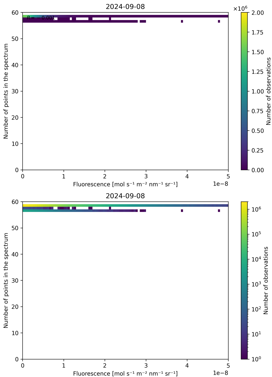
Figure 94: Scatter density plot of “Fluorescence” against “Number of points in the spectrum” for 2024-09-07 to 2024-09-09.
