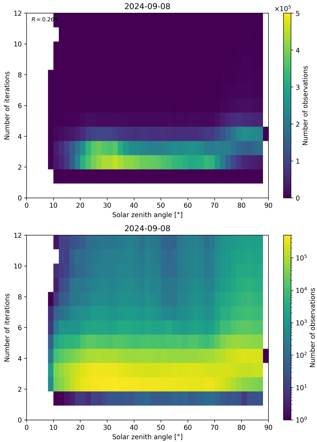
Figure 125: Scatter density plot of “Solar zenith angle” against “Number of iterations” for 2024-09-07 to 2024-09-09.
