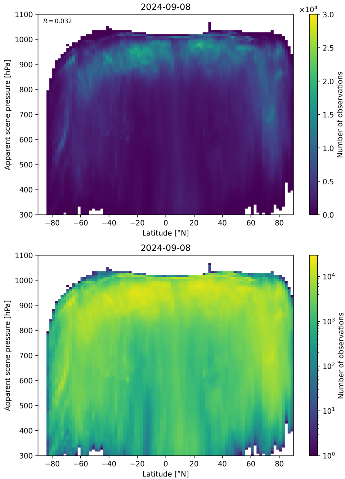
Figure 96: Scatter density plot of “Latitude” against “Apparent scene pressure” for 2024-09-07 to 2024-09-09.
