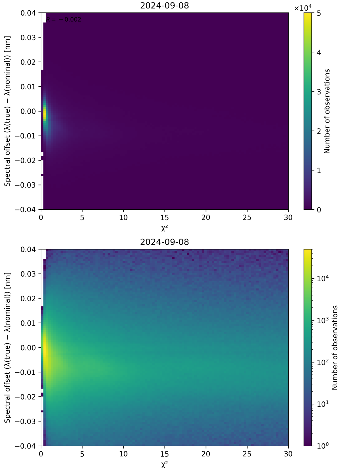
Figure 75: Scatter density plot of “ \chi^2 ” against “Spectral offset ( \lambda_{\text{true}} - \lambda_{\text{nominal}} )” for 2024-09-07 to 2024-09-09.
