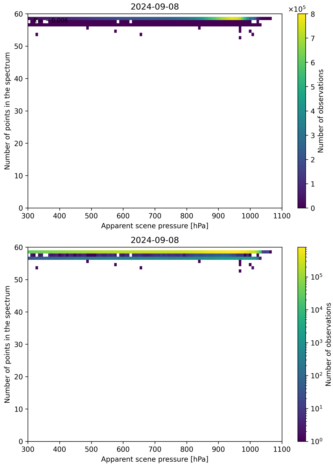
Figure 67: Scatter density plot of “Apparent scene pressure” against “Number of points in the spectrum” for 2024-09-07 to 2024-09-09.
