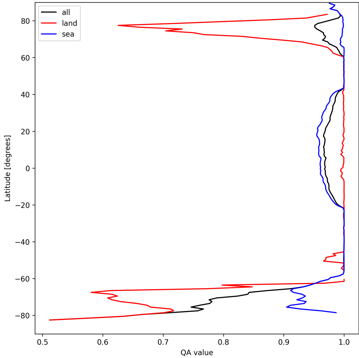
Figure 12: Zonal average of “QA value” for 2024-09-07 to 2024-09-09.
