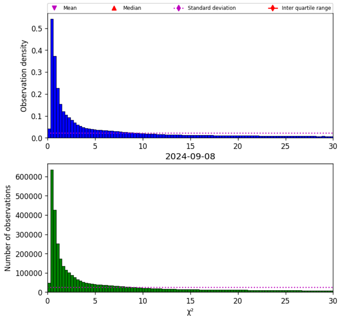
Figure 38: Histogram of " \chi^2 " for 2024-09-07 to 2024-09-09
