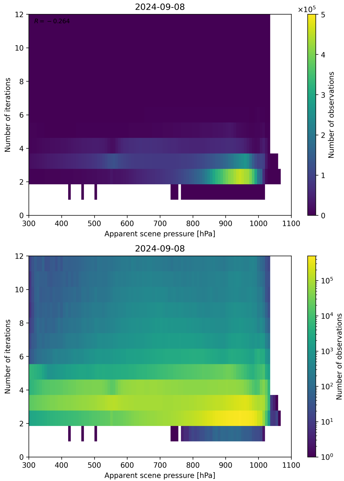
Figure 66: Scatter density plot of “Apparent scene pressure” against “Number of iterations” for 2024-09-07 to 2024-09-09.
