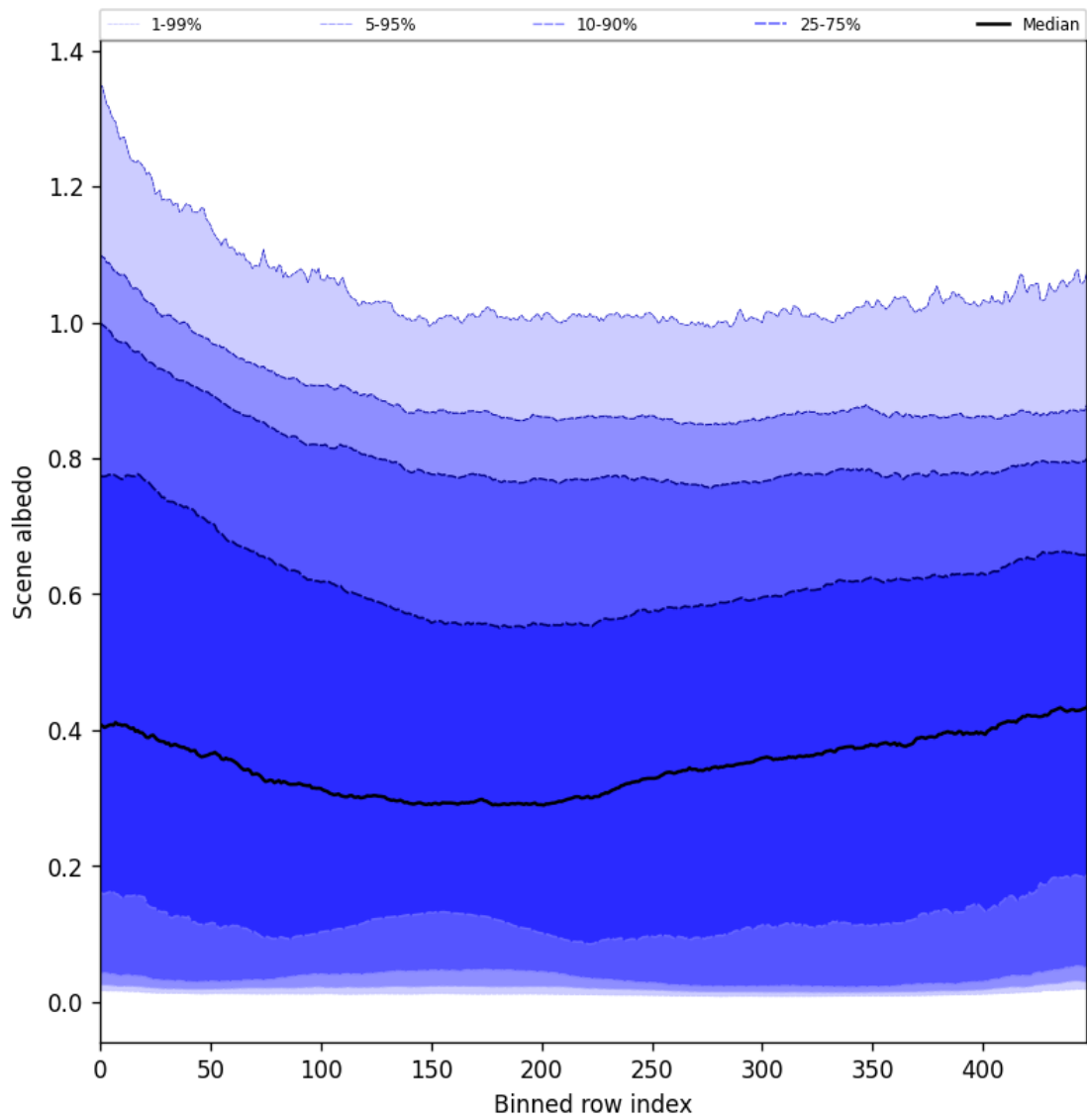
Figure 51: Along track statistics of “Scene albedo” for 2024-09-07 to 2024-09-09
