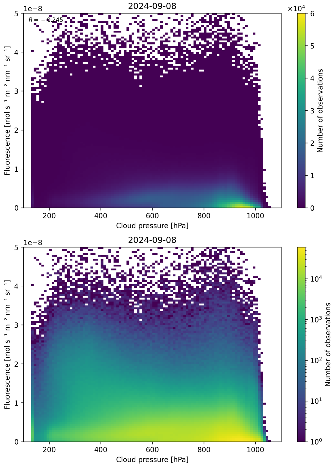
Figure 88: Scatter density plot of “Cloud pressure” against “Fluorescence” for 2024-09-07 to 2024-09-09.
