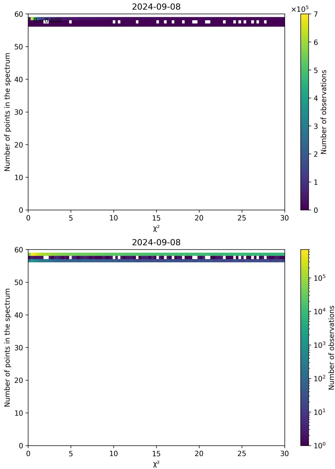
Figure 74: Scatter density plot of " \chi^2 " against "Number of points in the spectrum" for 2024-09-07 to 2024-09-09.
