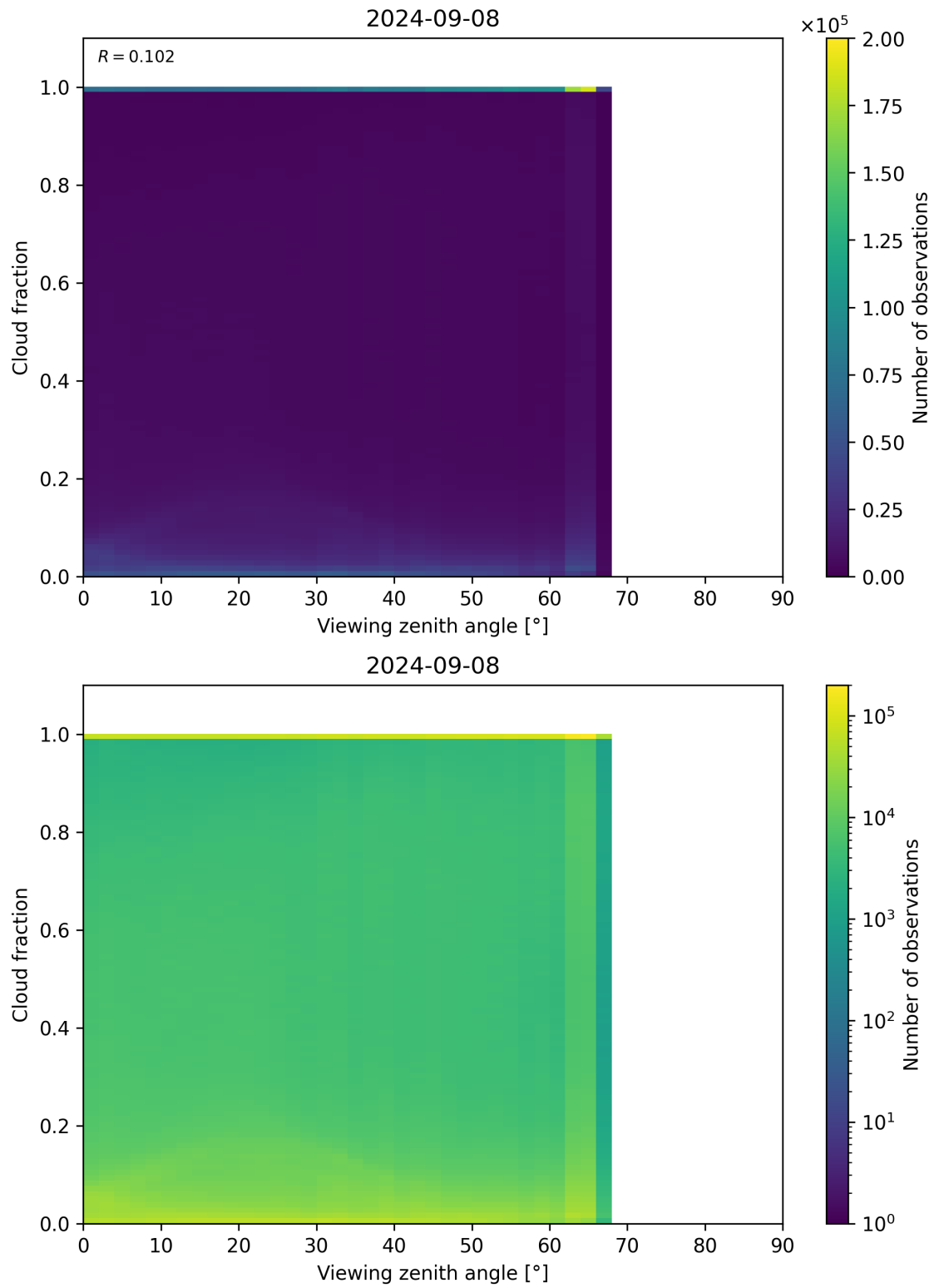
Figure 132: Scatter density plot of “Viewing zenith angle” against “Cloud fraction” for 2024-09-07 to 2024-09-09.
