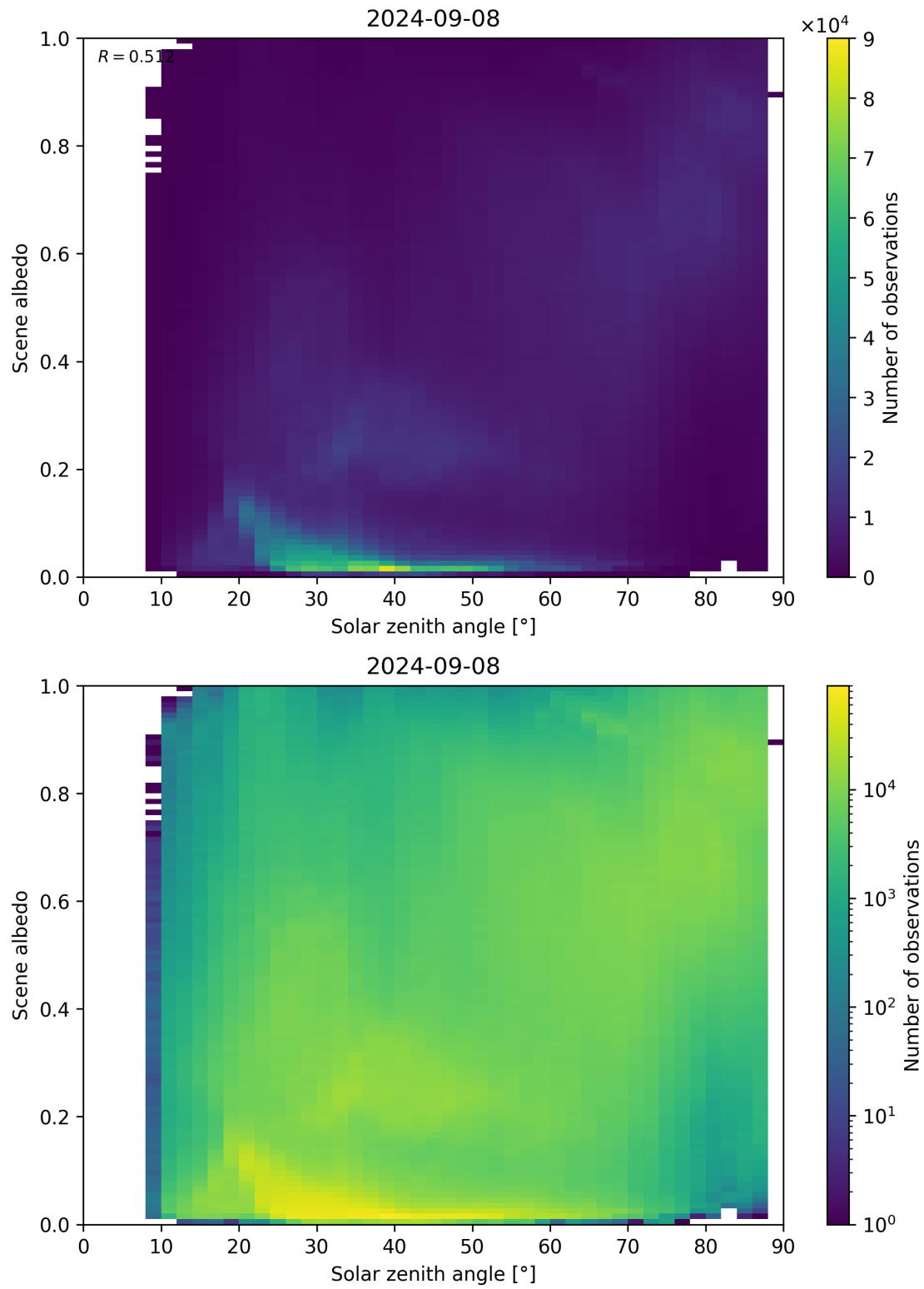
Figure 127: Scatter density plot of “Solar zenith angle” against “Scene albedo” for 2024-09-07 to 2024-09-09.
