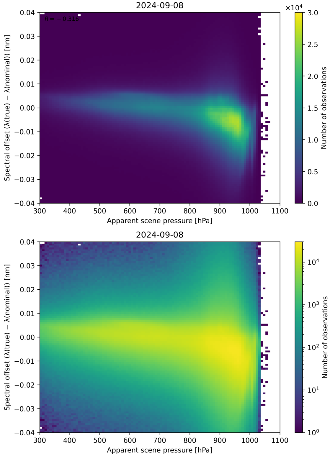
Figure 68: Scatter density plot of “Apparent scene pressure” against “Spectral offset ( \lambda_{\text{true}} - \lambda_{\text{nominal}} )” for 2024-09-07 to 2024-09-09.
