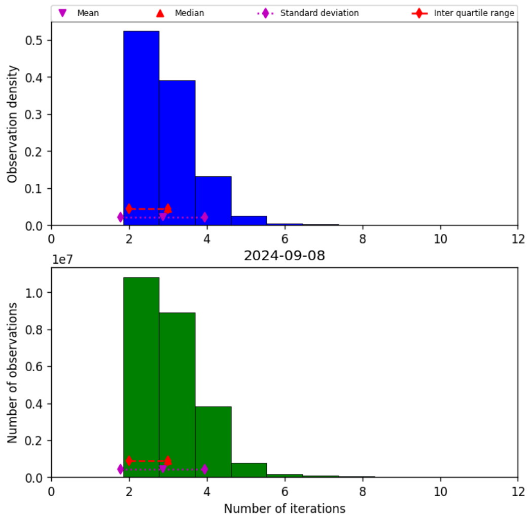
Figure 39: Histogram of “Number of iterations” for 2024-09-07 to 2024-09-09
