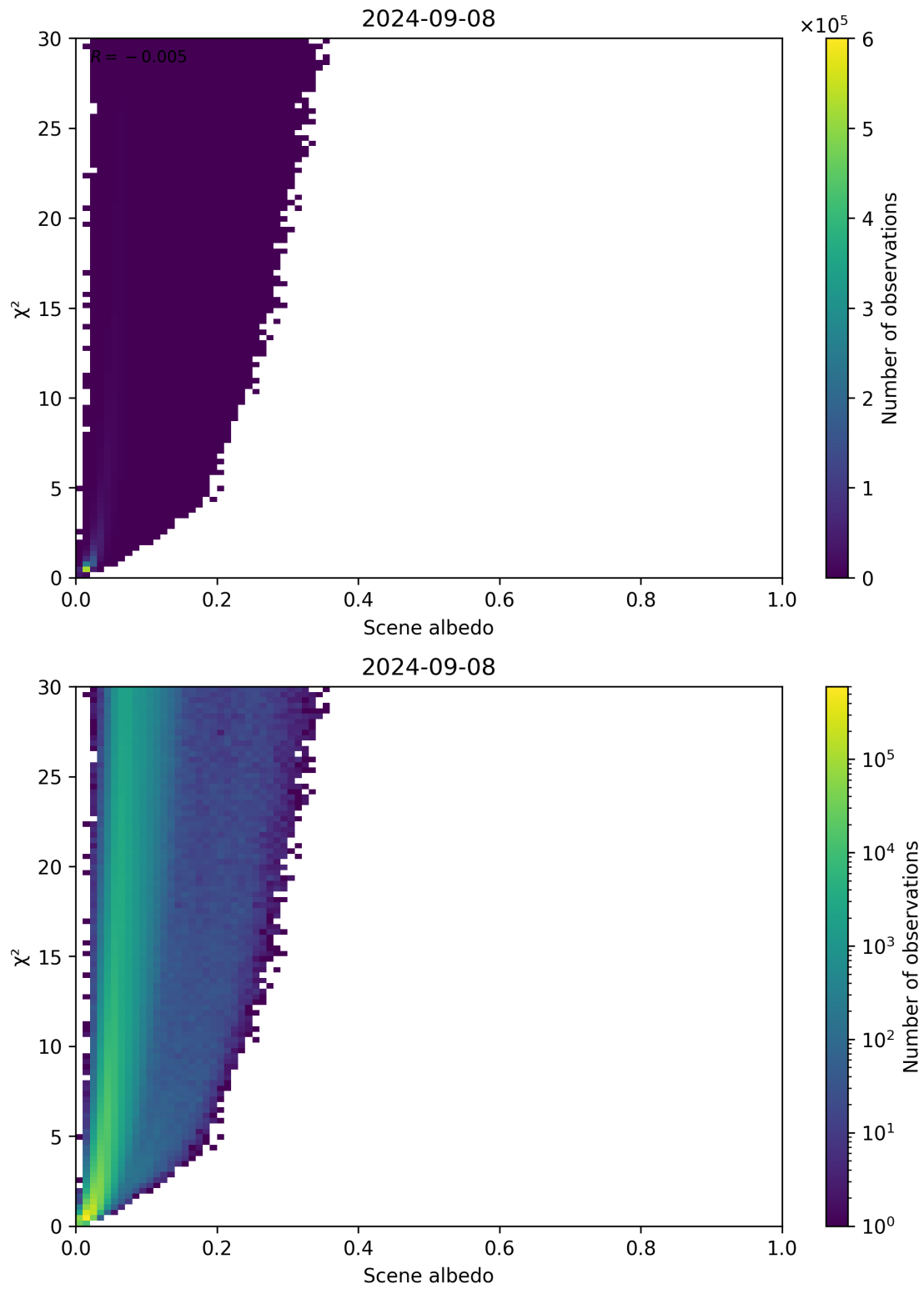
Figure 112: Scatter density plot of “Scene albedo” against “ \chi^2 ” for 2024-09-07 to 2024-09-09.
