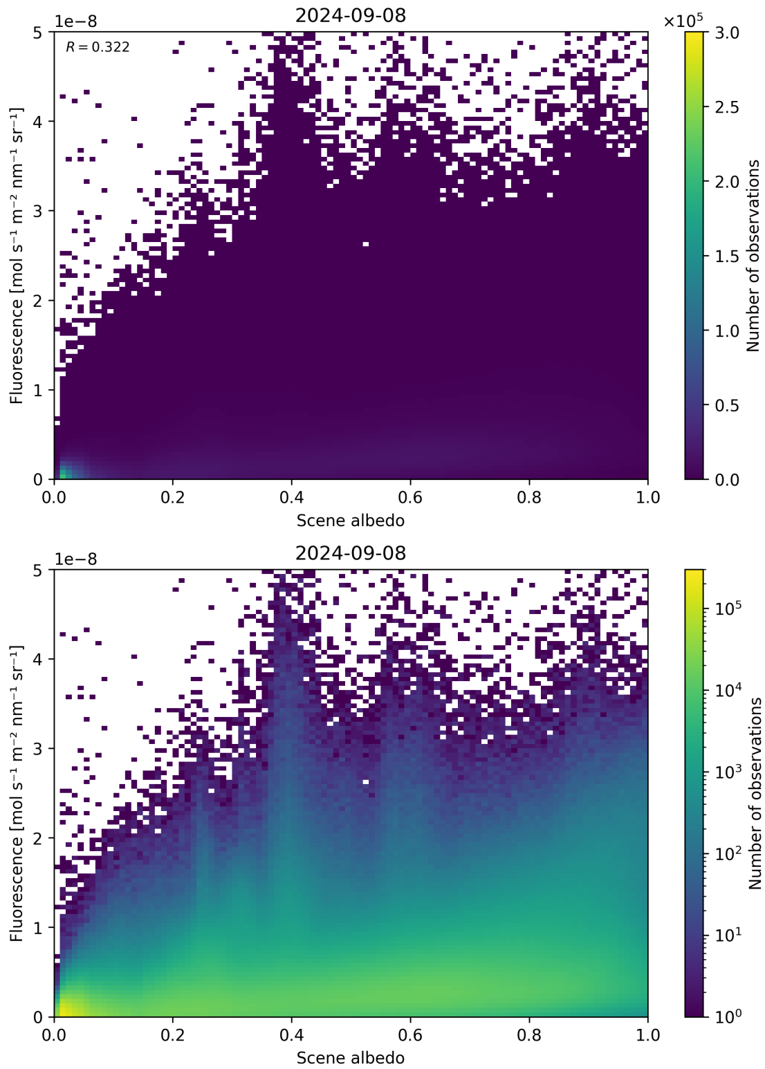
Figure 114: Scatter density plot of “Scene albedo” against “Fluorescence” for 2024-09-07 to 2024-09-09.
