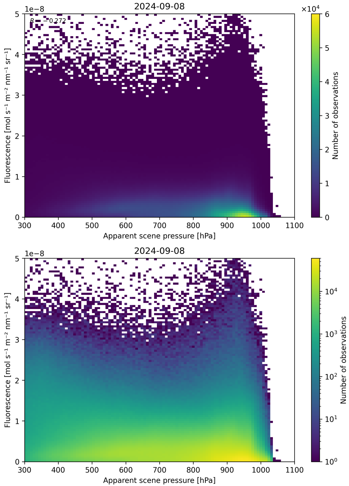
Figure 65: Scatter density plot of “Apparent scene pressure” against “Fluorescence” for 2024-09-07 to 2024-09-09.
