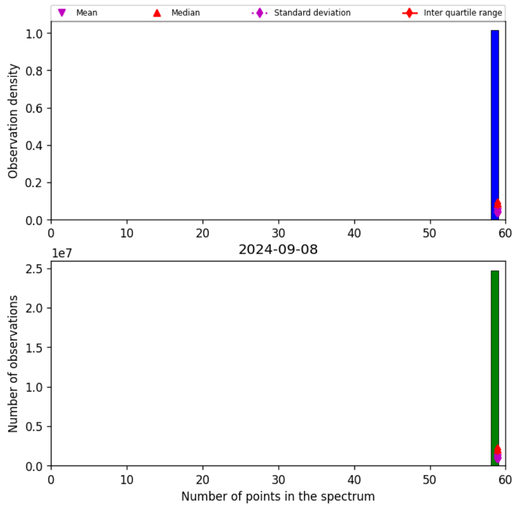
Figure 44: Histogram of “Number of points in the spectrum” for 2024-09-07 to 2024-09-09
