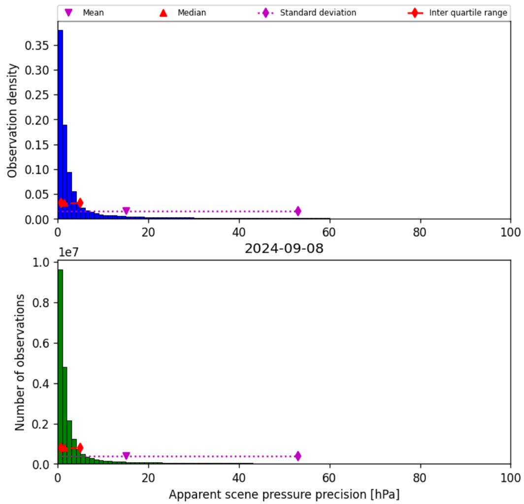
Figure 37: Histogram of “Apparent scene pressure precision” for 2024-09-07 to 2024-09-09
