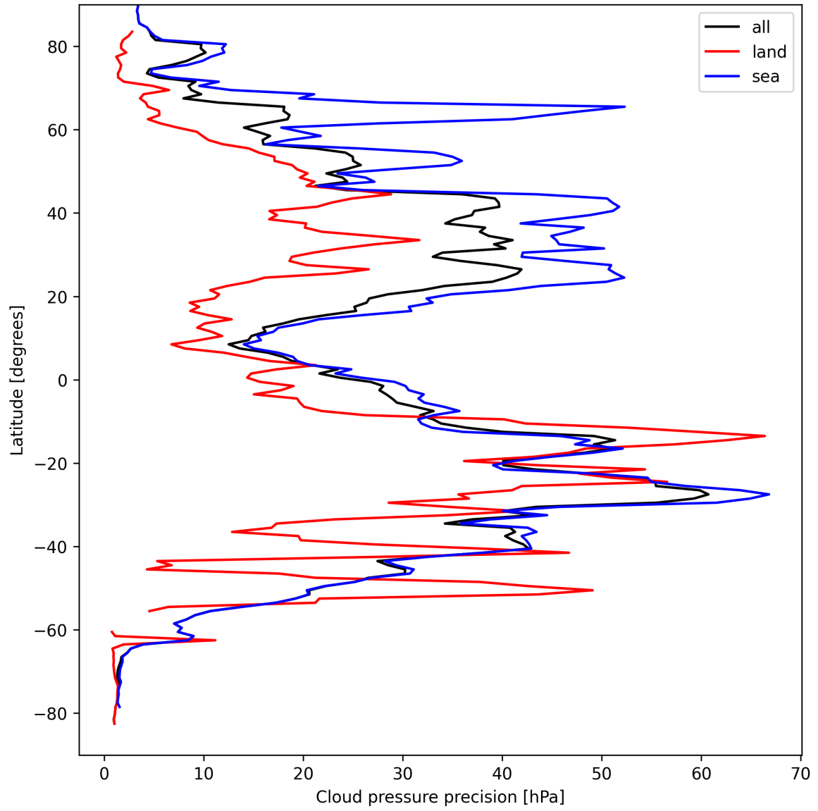
Figure 14: Zonal average of “Cloud pressure precision” for 2024-09-07 to 2024-09-09.
