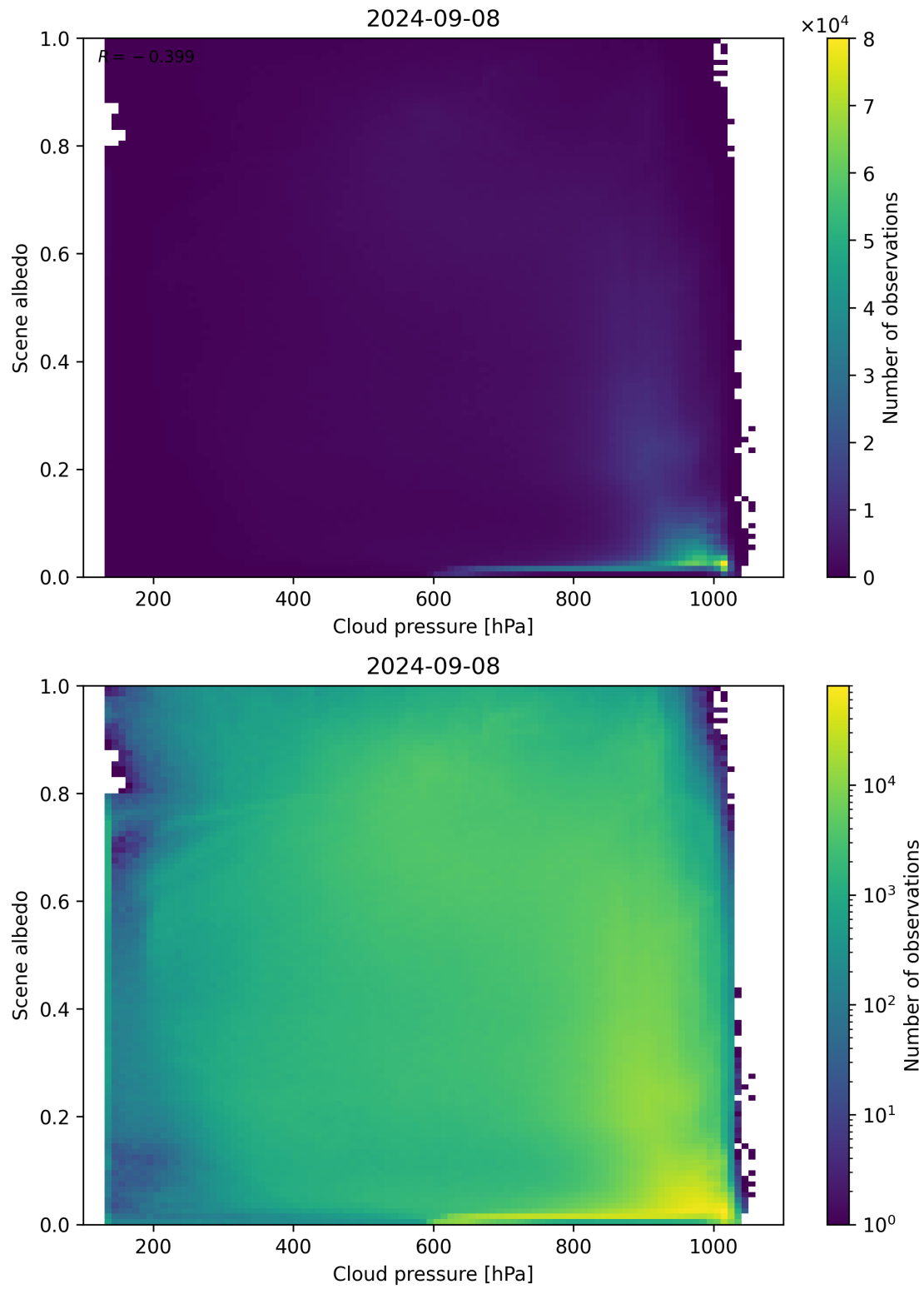
Figure 91: Scatter density plot of “Cloud pressure” against “Scene albedo” for 2024-09-07 to 2024-09-09.
