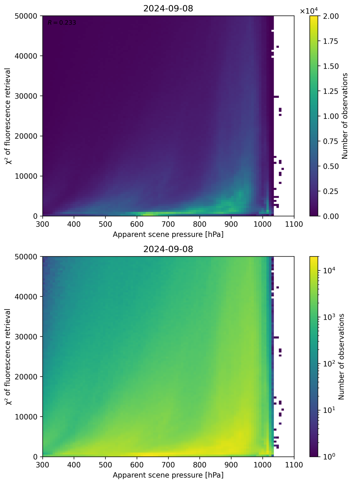
Figure 64: Scatter density plot of “Apparent scene pressure” against “ \chi^2 of fluorescence retrieval” for 2024-09-07 to 2024-09-09.
