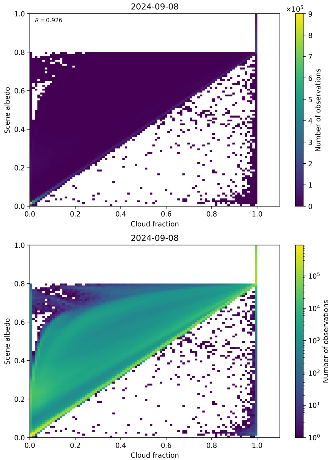
Figure 82: Scatter density plot of “Cloud fraction” against “Scene albedo” for 2024-09-07 to 2024-09-09.
