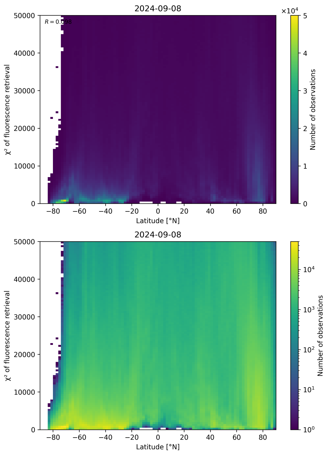
Figure 98: Scatter density plot of “Latitude” against “ \chi^2 of fluorescence retrieval” for 2024-09-07 to 2024-09-09.
