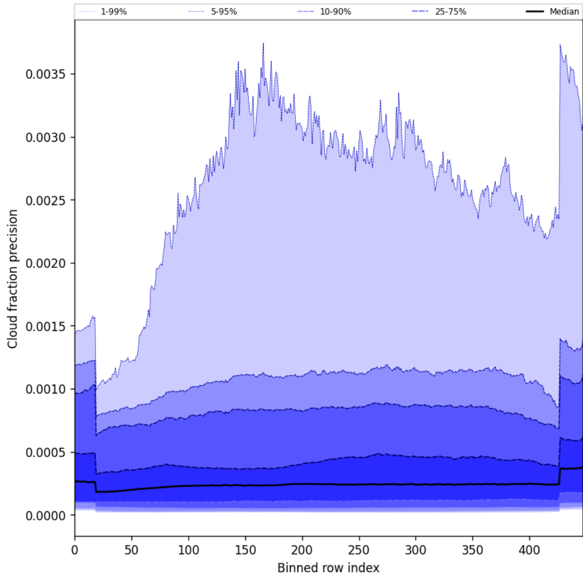
Figure 50: Along track statistics of “Cloud fraction precision” for 2024-09-07 to 2024-09-09
