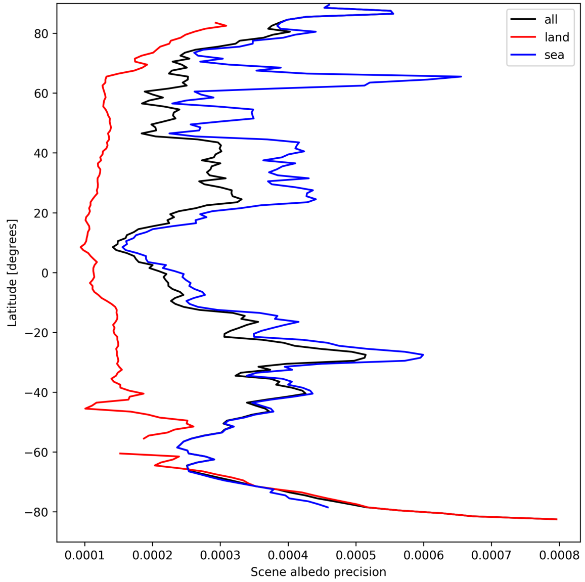
Figure 18: Zonal average of “Scene albedo precision” for 2024-09-07 to 2024-09-09.
