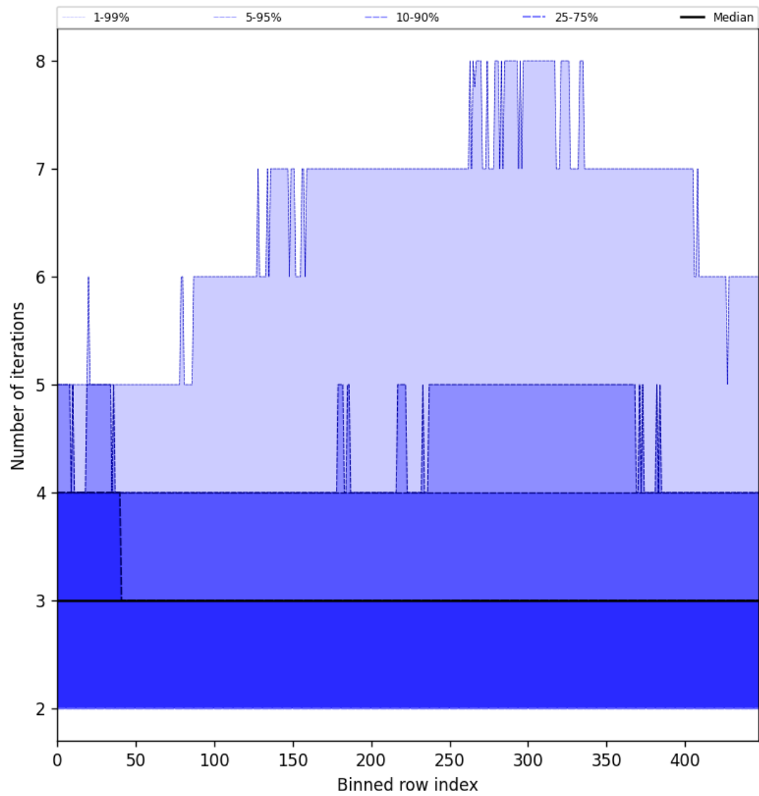
Figure 56: Along track statistics of “Number of iterations” for 2024-09-07 to 2024-09-09
