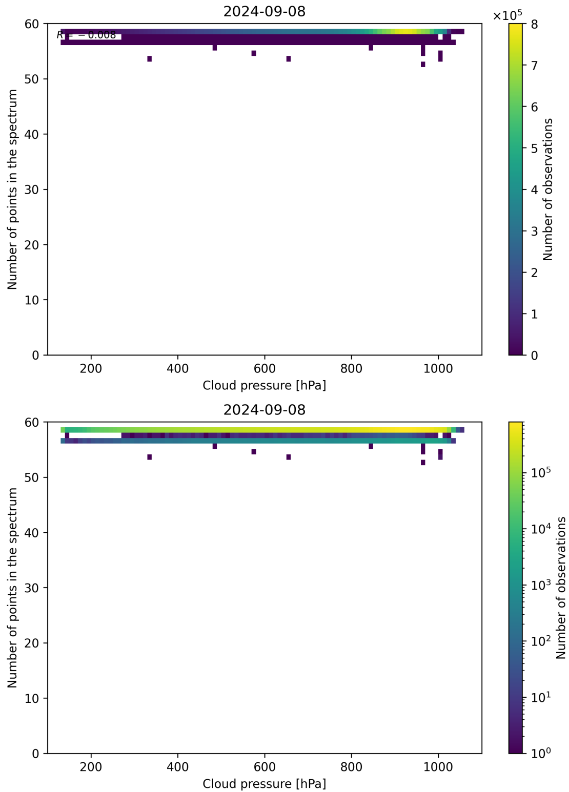
Figure 90: Scatter density plot of “Cloud pressure” against “Number of points in the spectrum” for 2024-09-07 to 2024-09-09.
