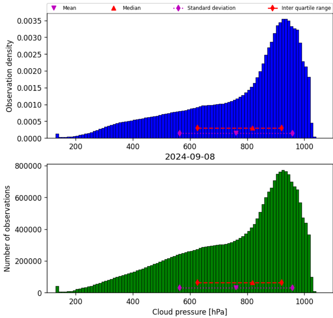
Figure 30: Histogram of “Cloud pressure” for 2024-09-07 to 2024-09-09
