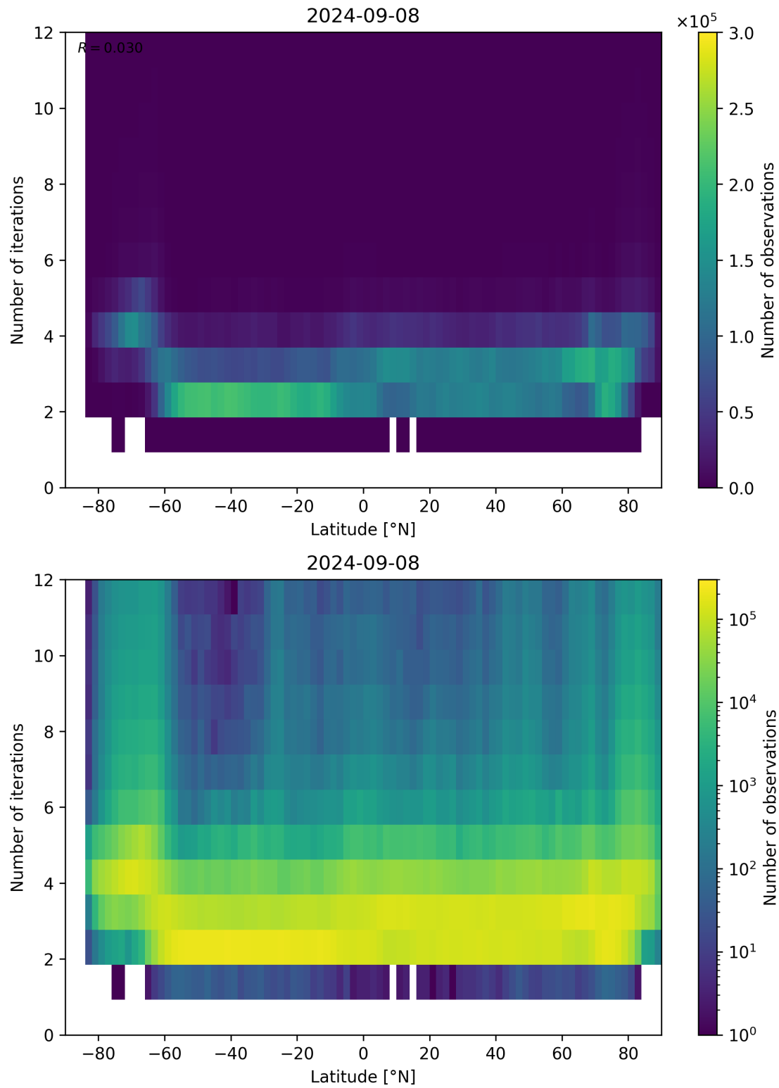
Figure 102: Scatter density plot of “Latitude” against “Number of iterations” for 2024-09-07 to 2024-09-09.
