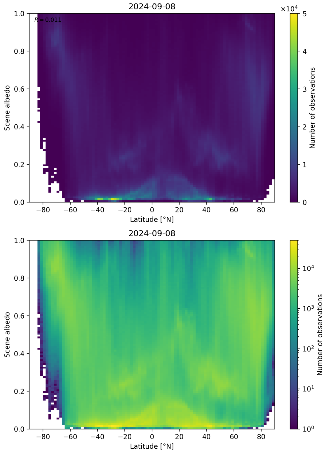
Figure 104: Scatter density plot of “Latitude” against “Scene albedo” for 2024-09-07 to 2024-09-09.
