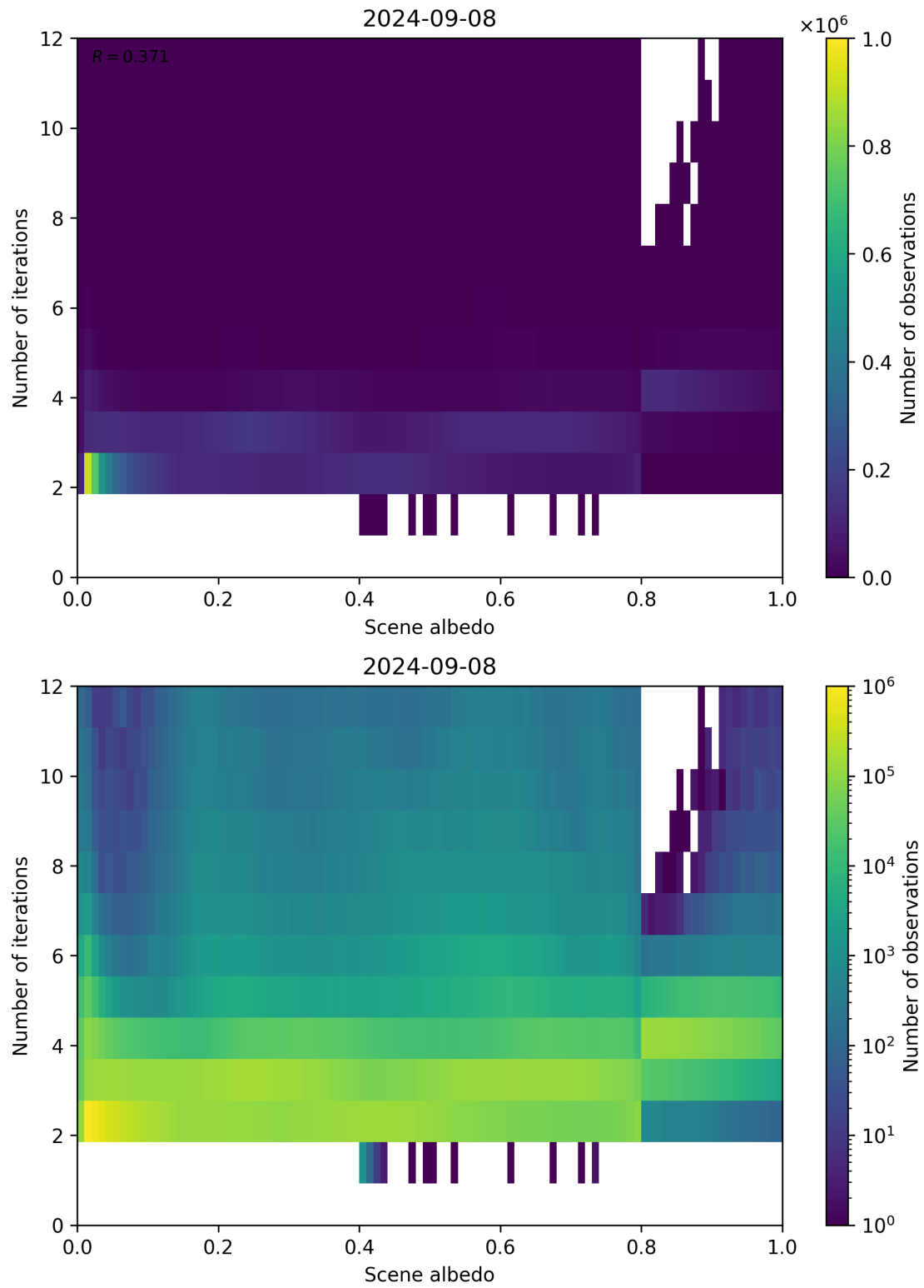
Figure 115: Scatter density plot of “Scene albedo” against “Number of iterations” for 2024-09-07 to 2024-09-09.
