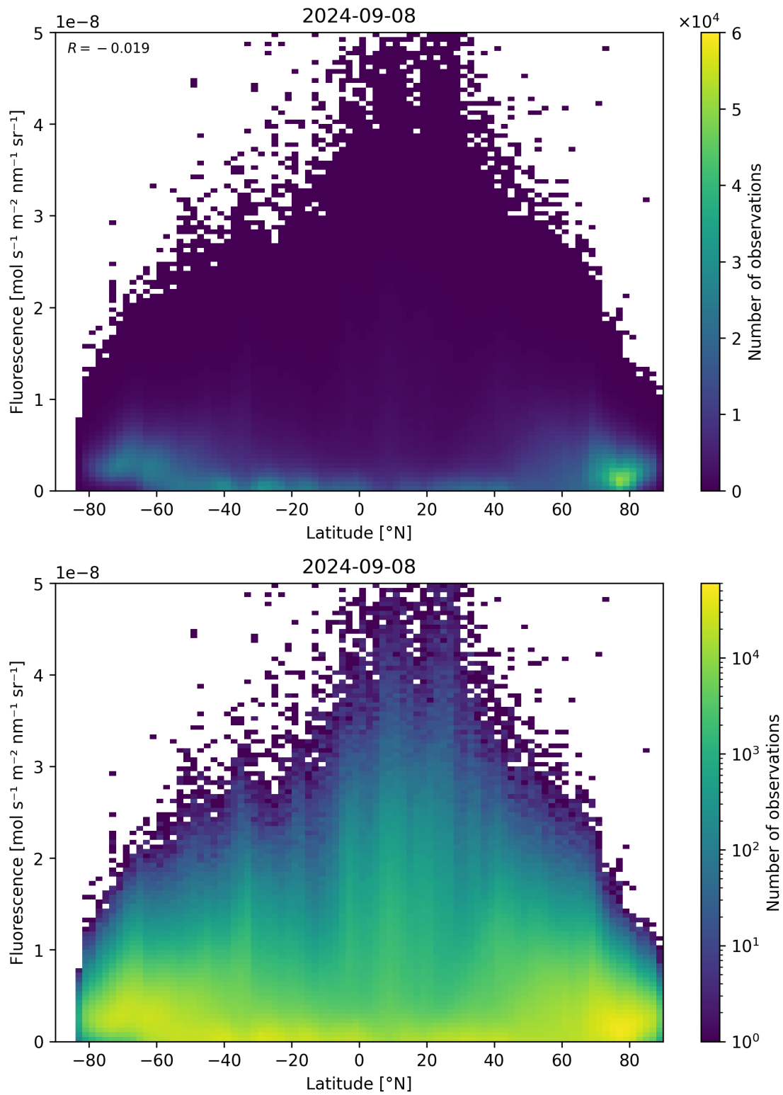
Figure 101: Scatter density plot of “Latitude” against “Fluorescence” for 2024-09-07 to 2024-09-09.
