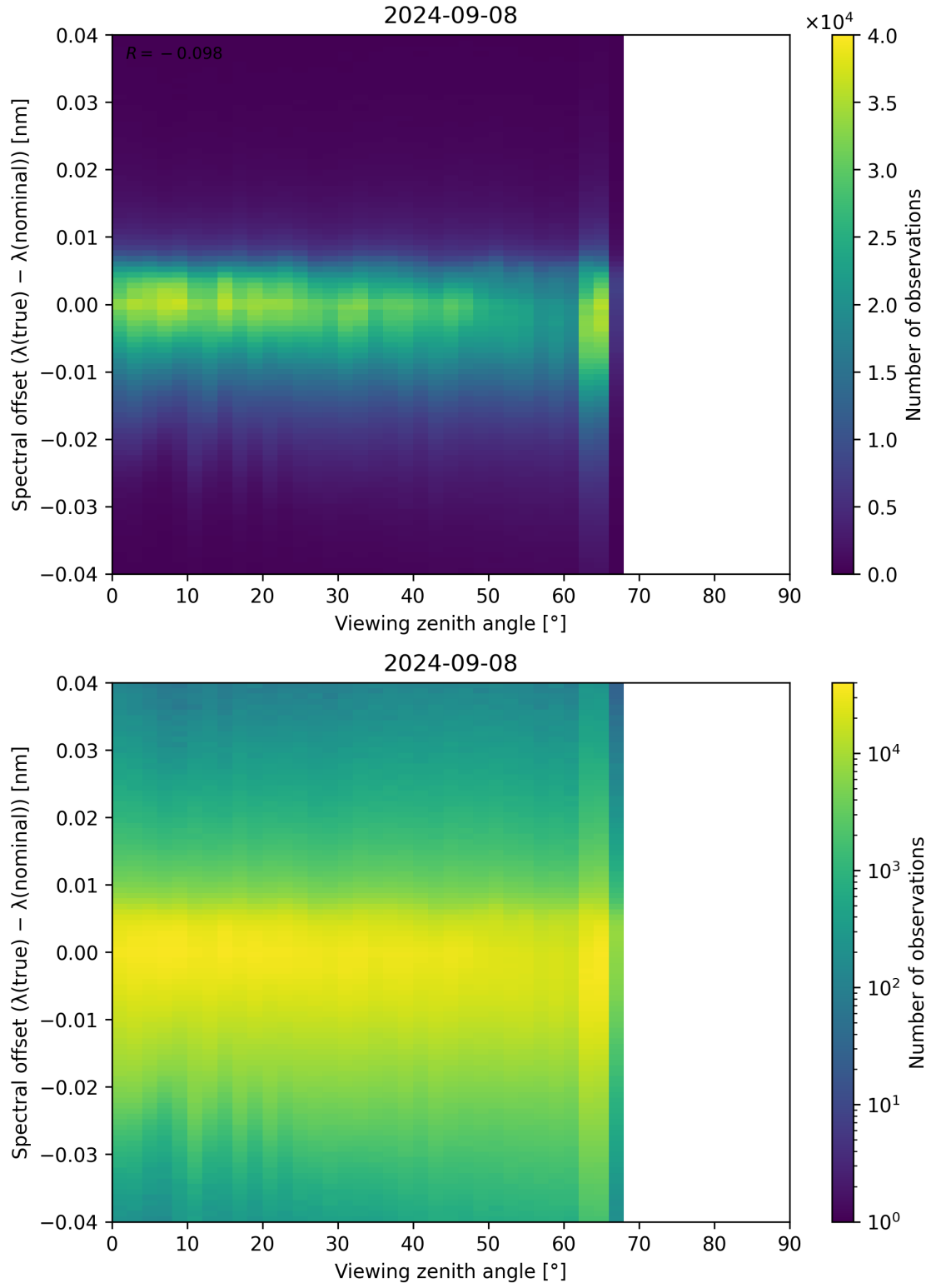
Figure 140: Scatter density plot of “Viewing zenith angle” against “Spectral offset ( \lambda_{\text{true}} - \lambda_{\text{nominal}} )” for 2024-09-07 to 2024-09-09.
