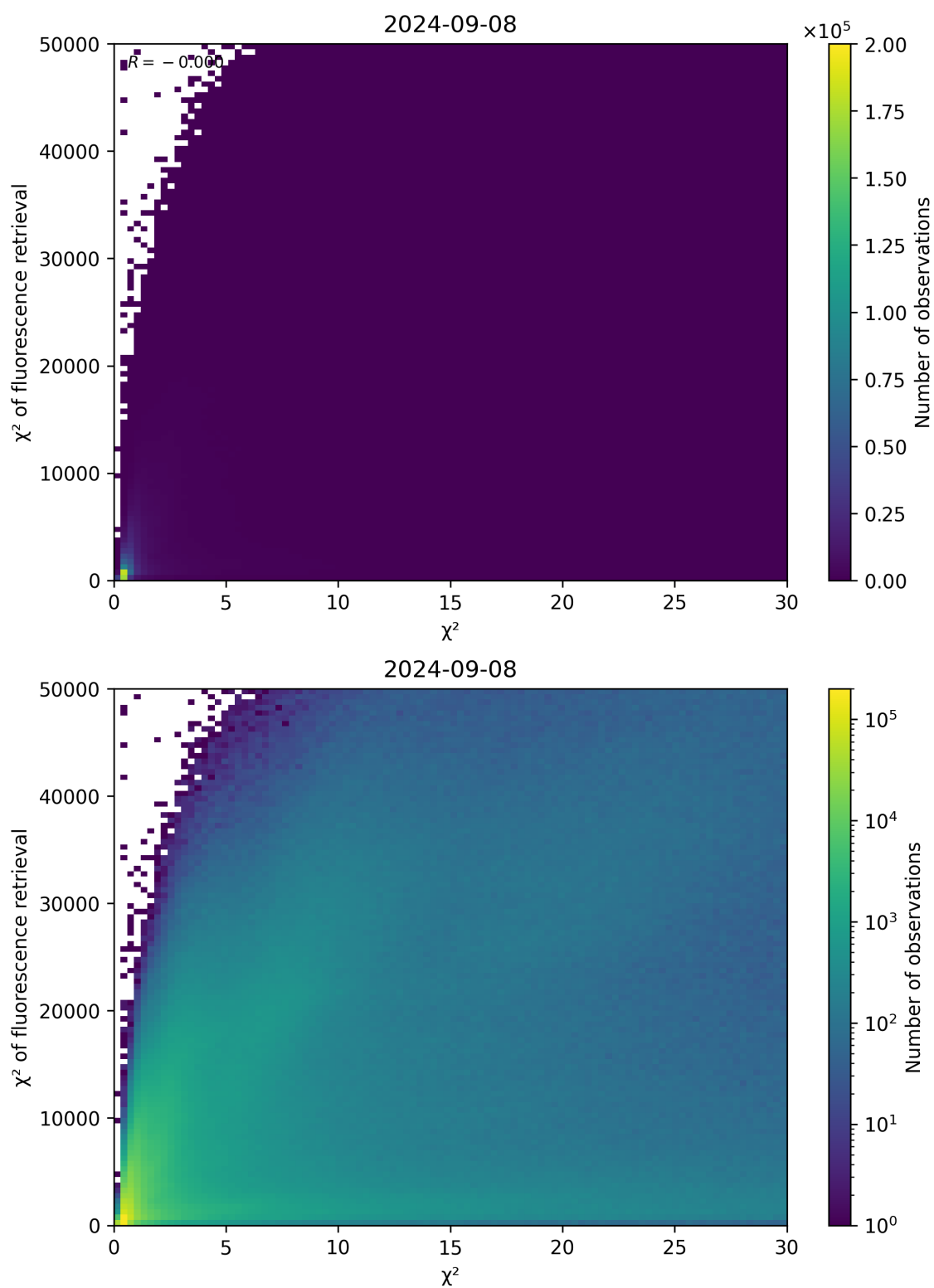
Figure 69: Scatter density plot of “ \chi^2 ” against “ \chi^2 of fluorescence retrieval” for 2024-09-07 to 2024-09-09.
