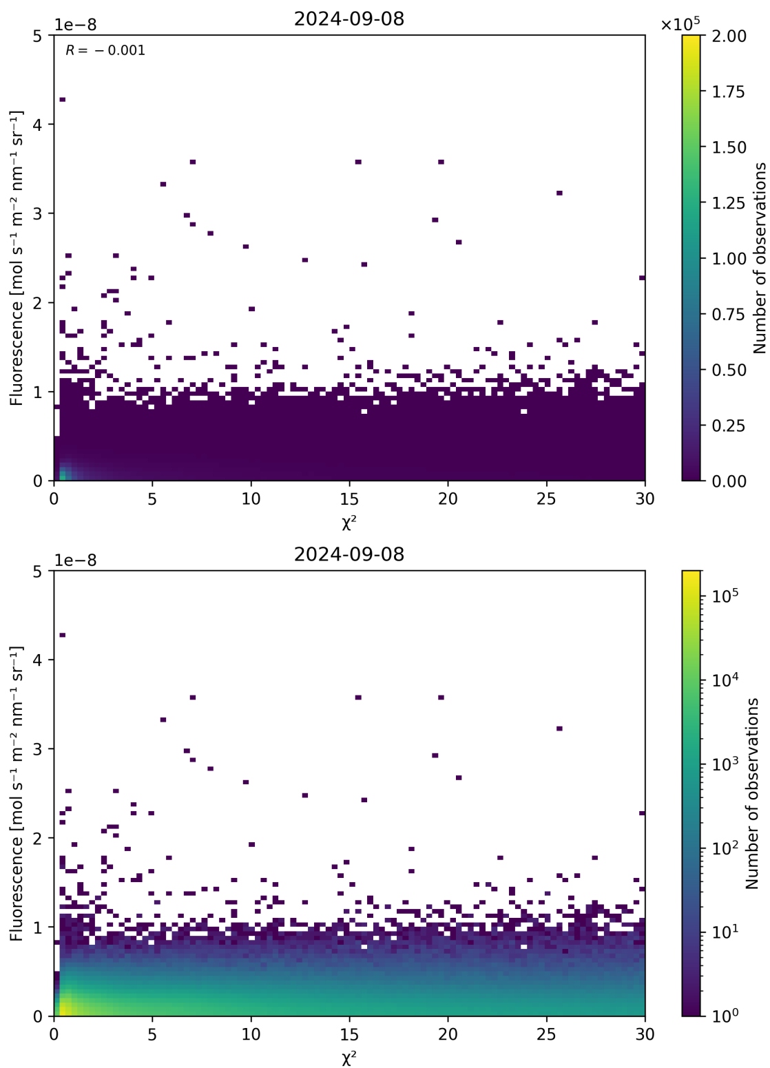
Figure 70: Scatter density plot of “ \chi^2 ” against “Fluorescence” for 2024-09-07 to 2024-09-09.
