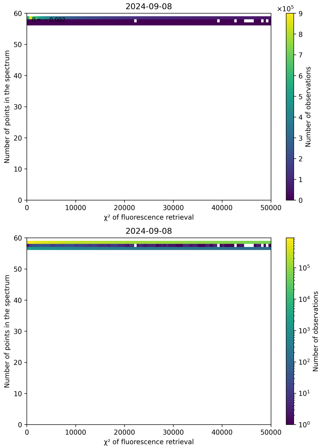
Figure 71: Scatter density plot of “ \chi^2 of fluorescence retrieval” against “Number of points in the spectrum” for 2024-09-07 to 2024-09-09.
