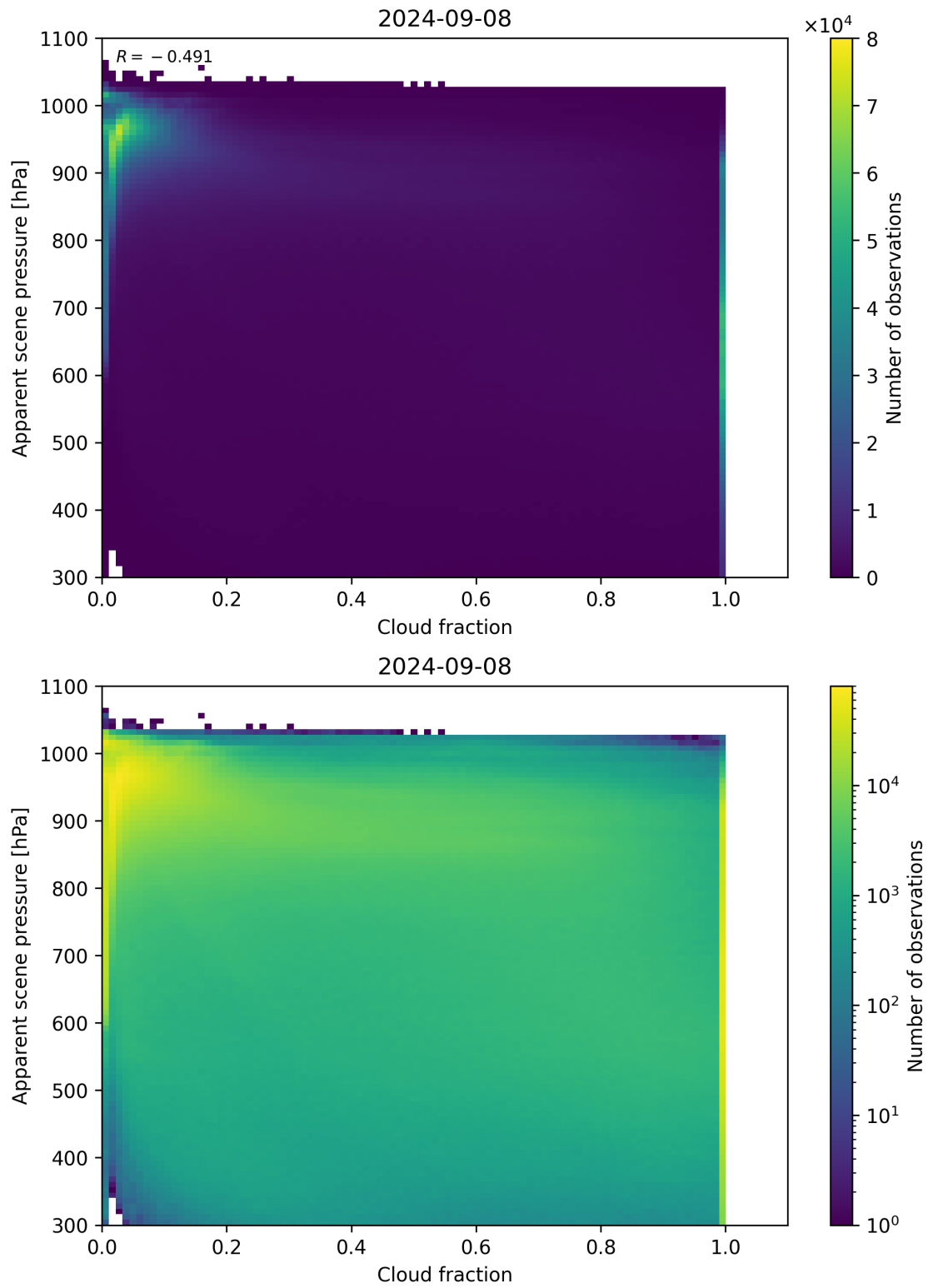
Figure 76: Scatter density plot of “Cloud fraction” against “Apparent scene pressure” for 2024-09-07 to 2024-09-09.
