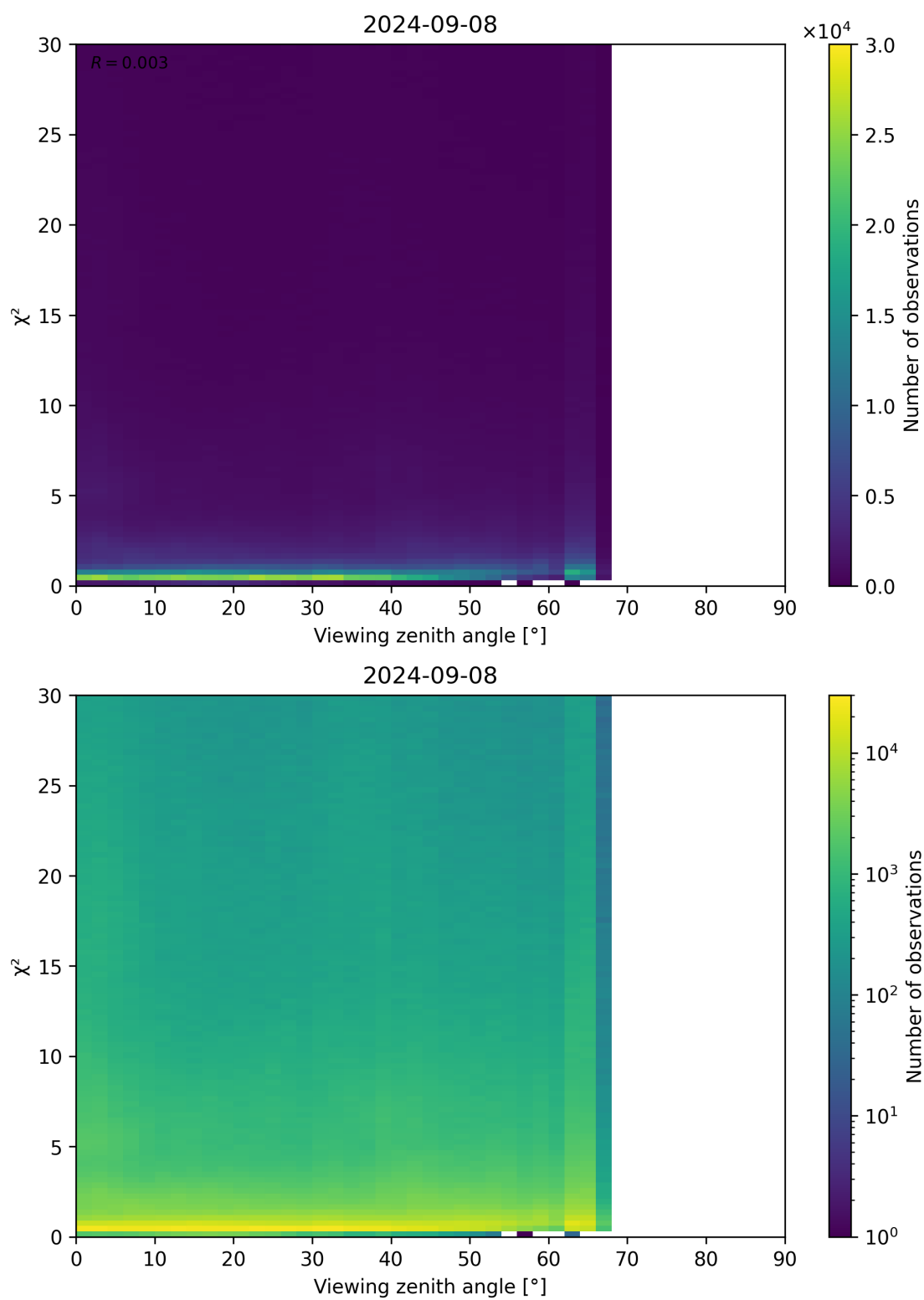
Figure 130: Scatter density plot of “Viewing zenith angle” against “ \chi^2 ” for 2024-09-07 to 2024-09-09.
