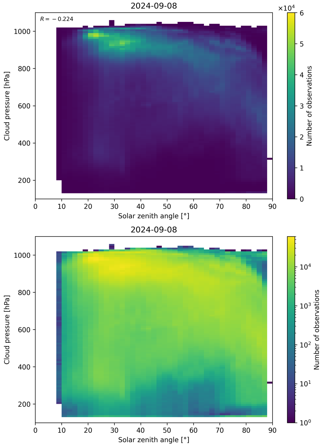
Figure 122: Scatter density plot of “Solar zenith angle” against “Cloud pressure” for 2024-09-07 to 2024-09-09.
