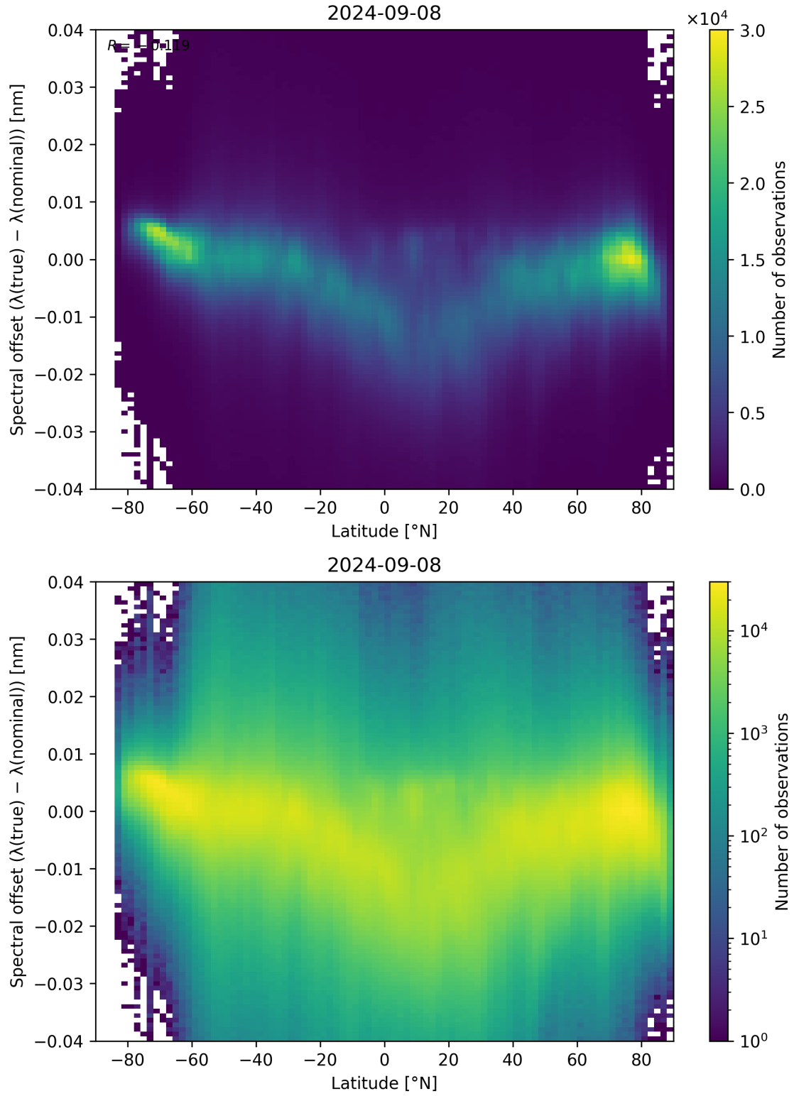
Figure 105: Scatter density plot of “Latitude” against “Spectral offset ( \lambda_{\text{true}} - \lambda_{\text{nominal}} )” for 2024-09-07 to 2024-09-09.
