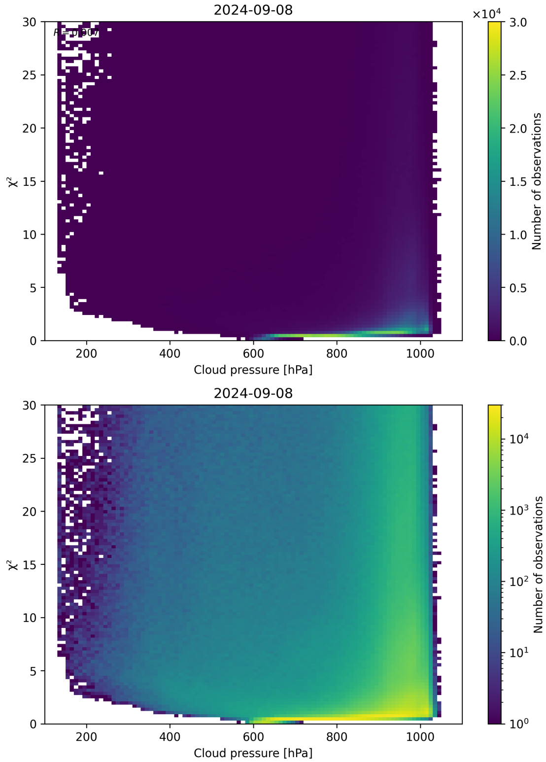
Figure 85: Scatter density plot of “Cloud pressure” against “ \chi^2 ” for 2024-09-07 to 2024-09-09.
