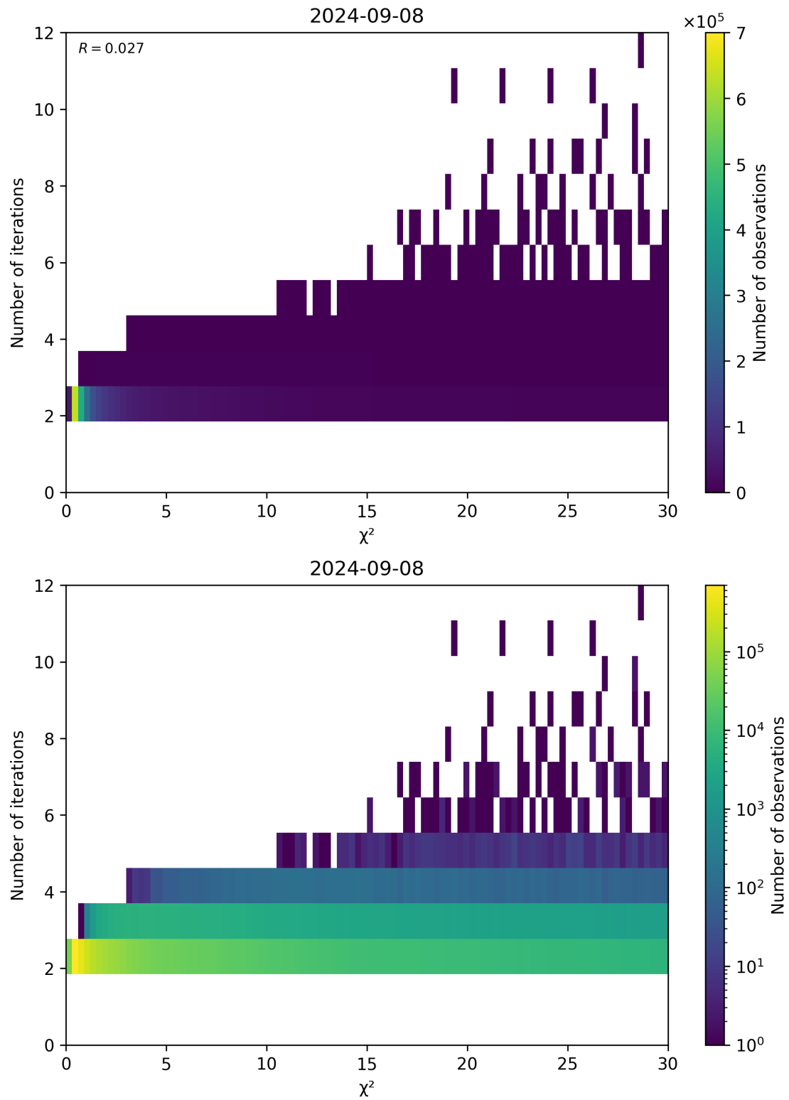
Figure 73: Scatter density plot of “ \chi^2 ” against “Number of iterations” for 2024-09-07 to 2024-09-09.
