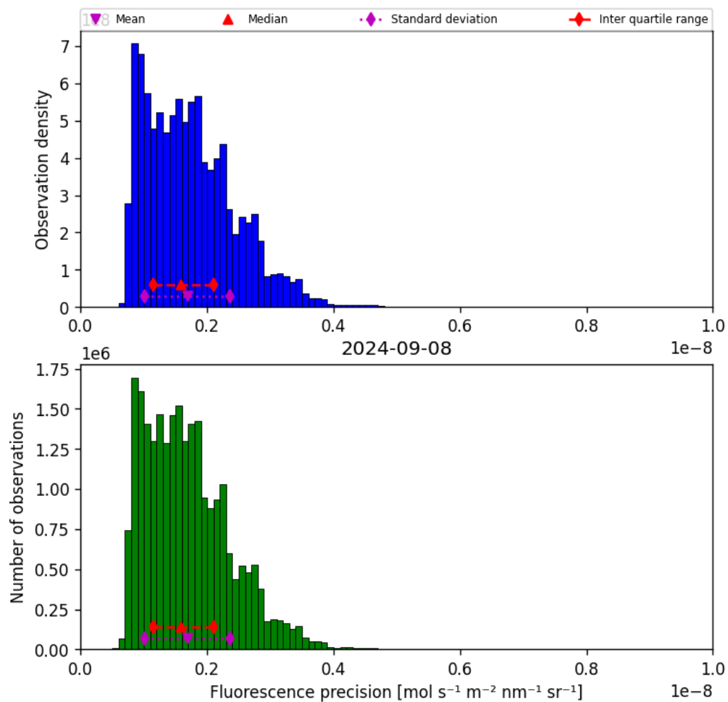
Figure 41: Histogram of “Fluorescence precision” for 2024-09-07 to 2024-09-09
