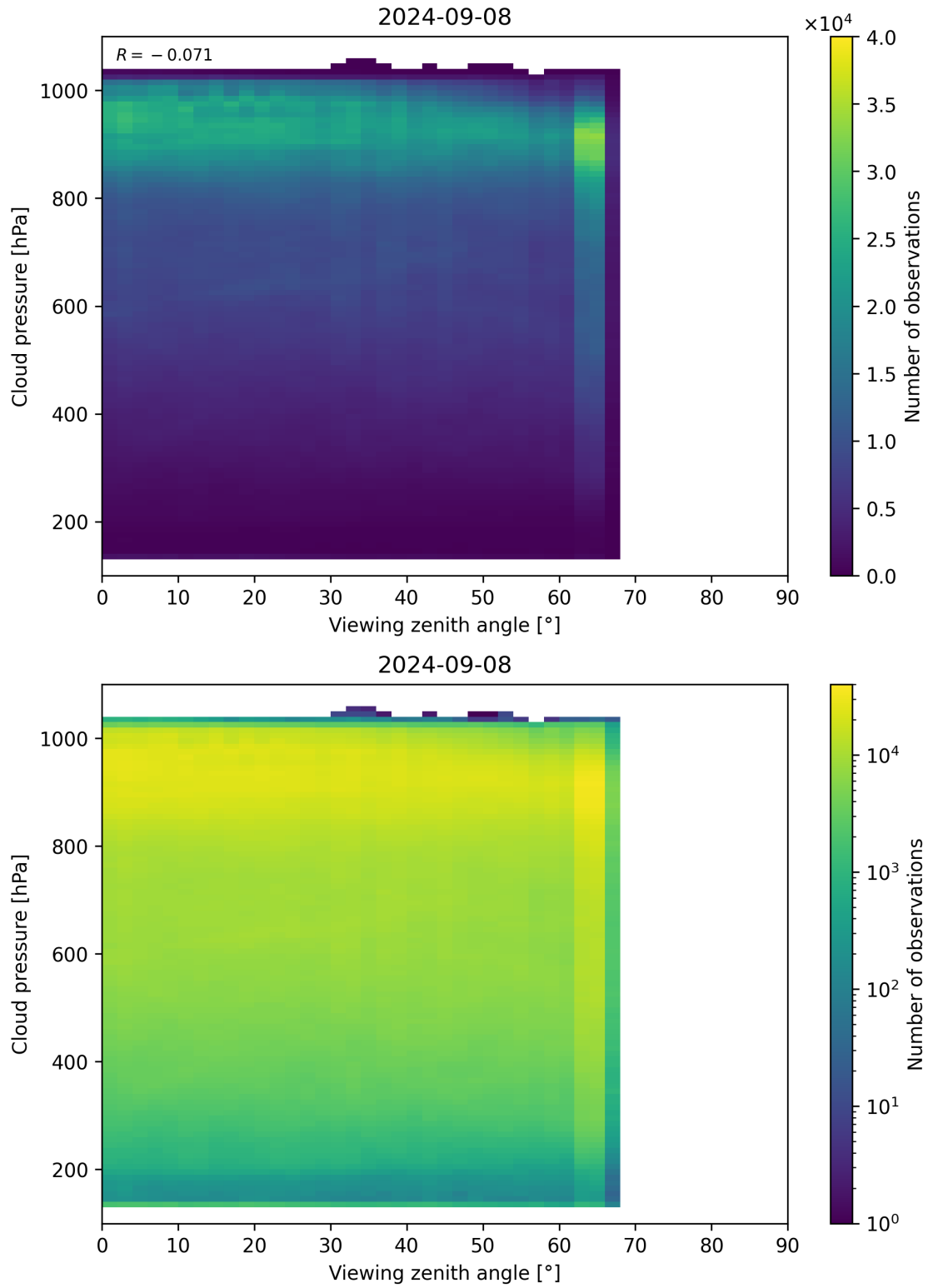
Figure 133: Scatter density plot of “Viewing zenith angle” against “Cloud pressure” for 2024-09-07 to 2024-09-09.
