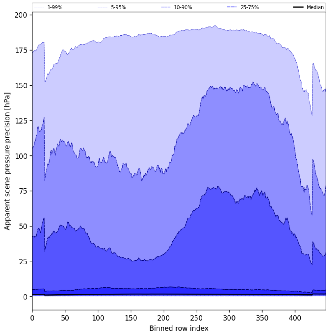
Figure 54: Along track statistics of “Apparent scene pressure precision” for 2024-09-07 to 2024-09-09
