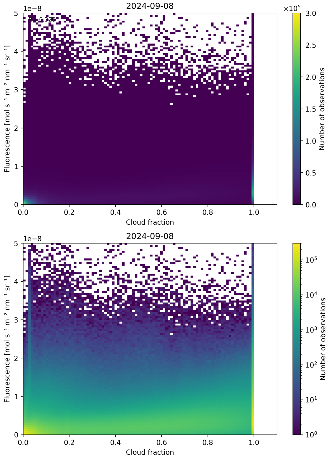
Figure 79: Scatter density plot of “Cloud fraction” against “Fluorescence” for 2024-09-07 to 2024-09-09.
