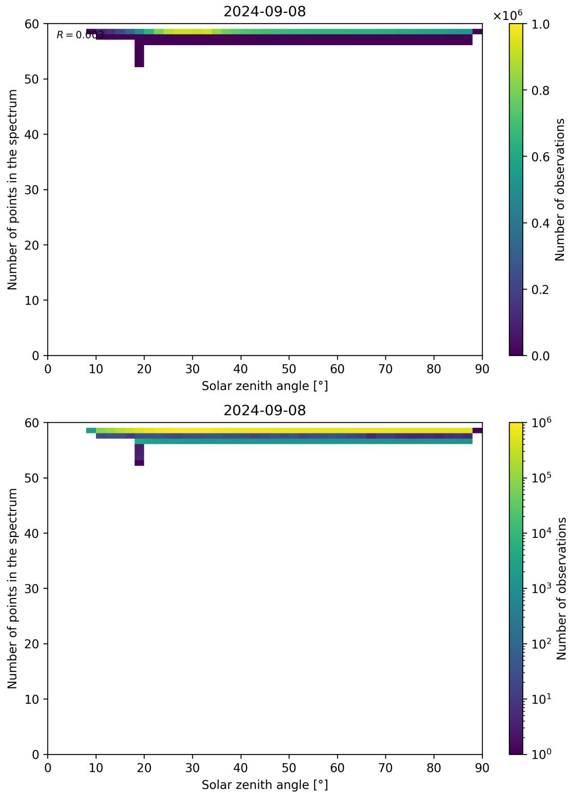
Figure 126: Scatter density plot of “Solar zenith angle” against “Number of points in the spectrum” for 2024-09-07 to 2024-09-09.
