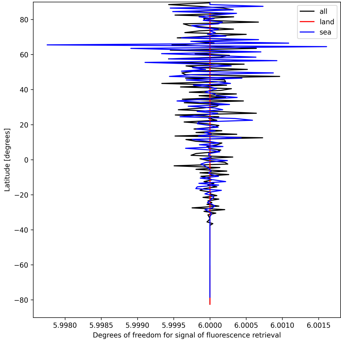
Figure 26: Zonal average of “Degrees of freedom for signal of fluorescence retrieval” for 2024-09-07 to 2024-09-09.
