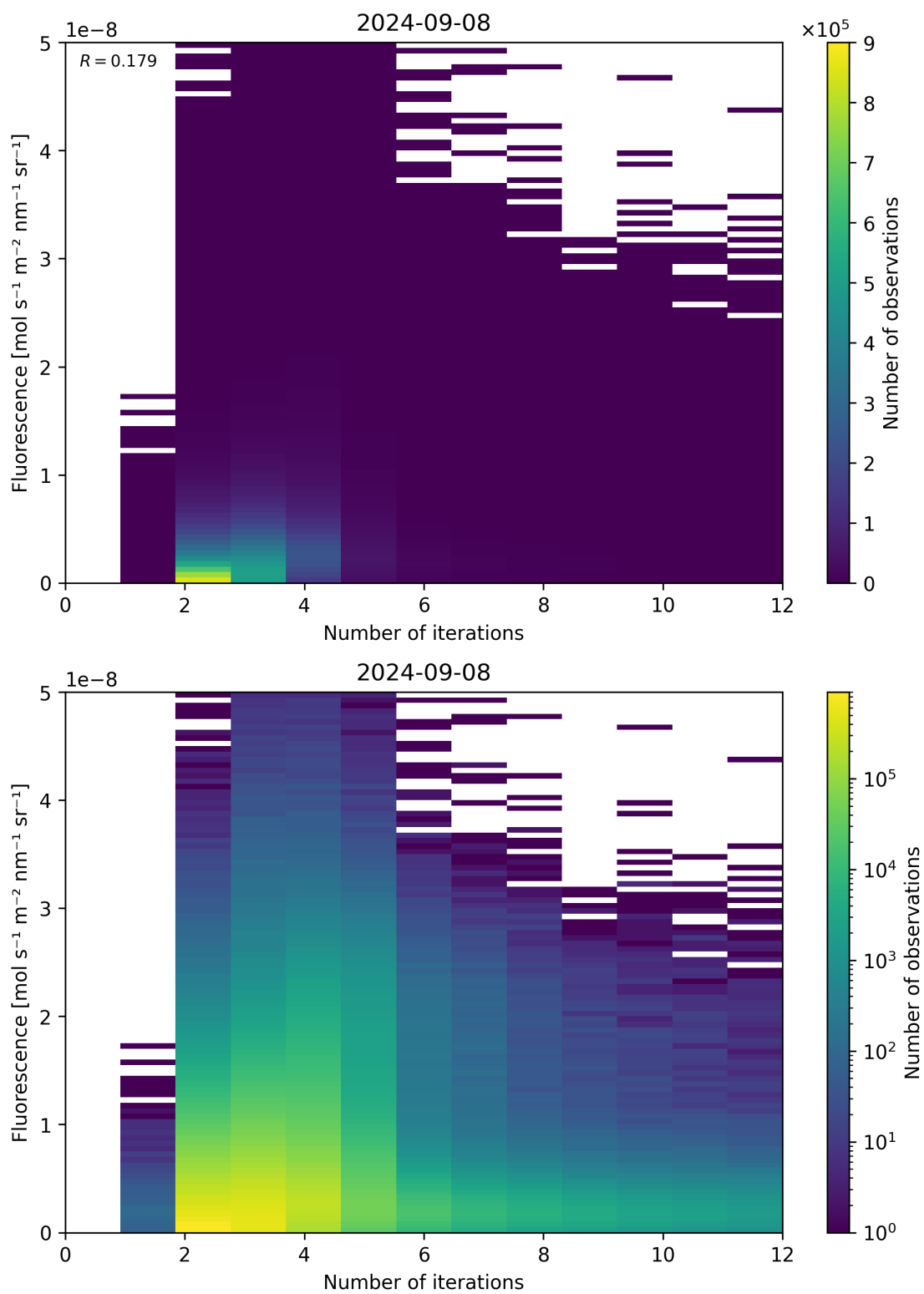
Figure 107: Scatter density plot of "Number of iterations" against "Fluorescence" for 2024-09-07 to 2024-09-09.
