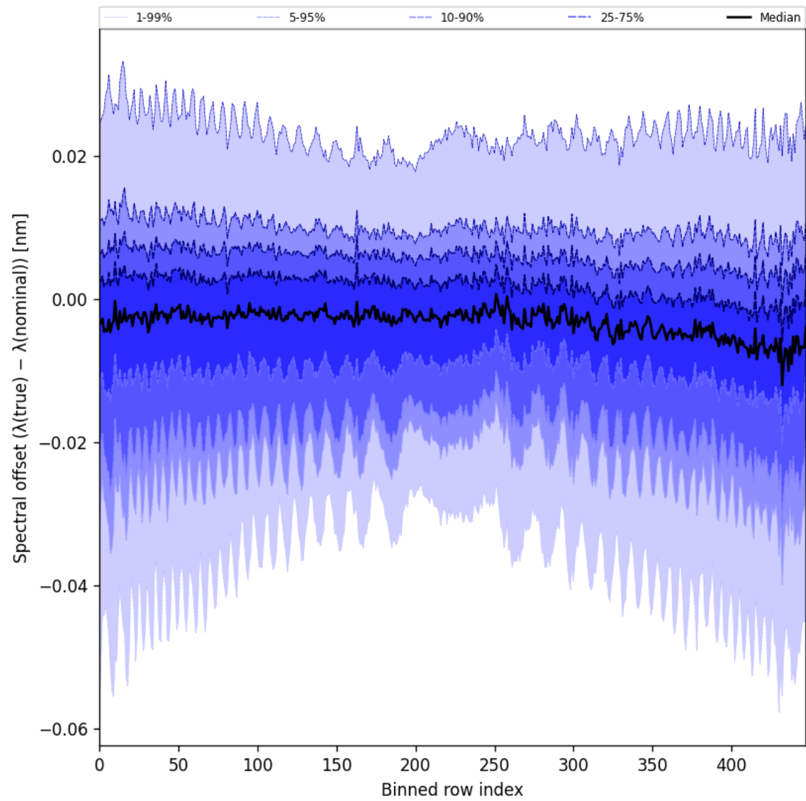
Figure 62: Along track statistics of “Spectral offset ( \lambda_{\text{true}} - \lambda_{\text{nominal}} )” for 2024-09-07 to 2024-09-09
