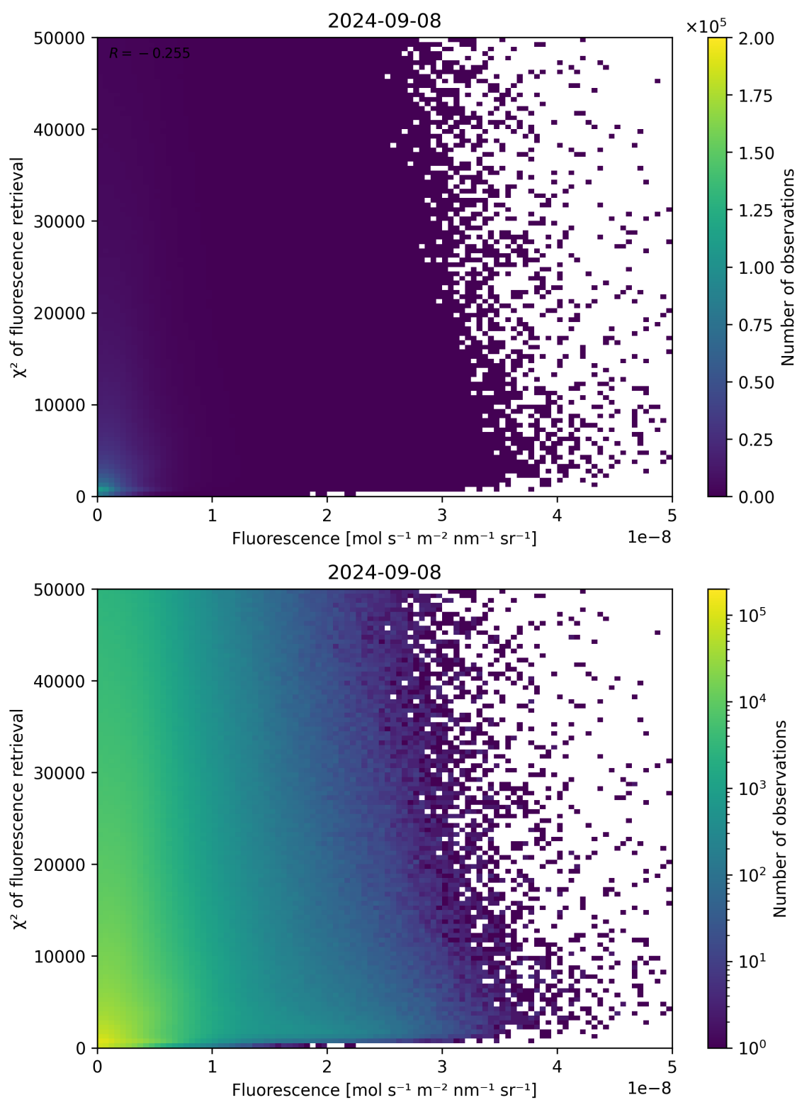
Figure 93: Scatter density plot of “Fluorescence” against “ \chi^2 of fluorescence retrieval” for 2024-09-07 to 2024-09-09.
