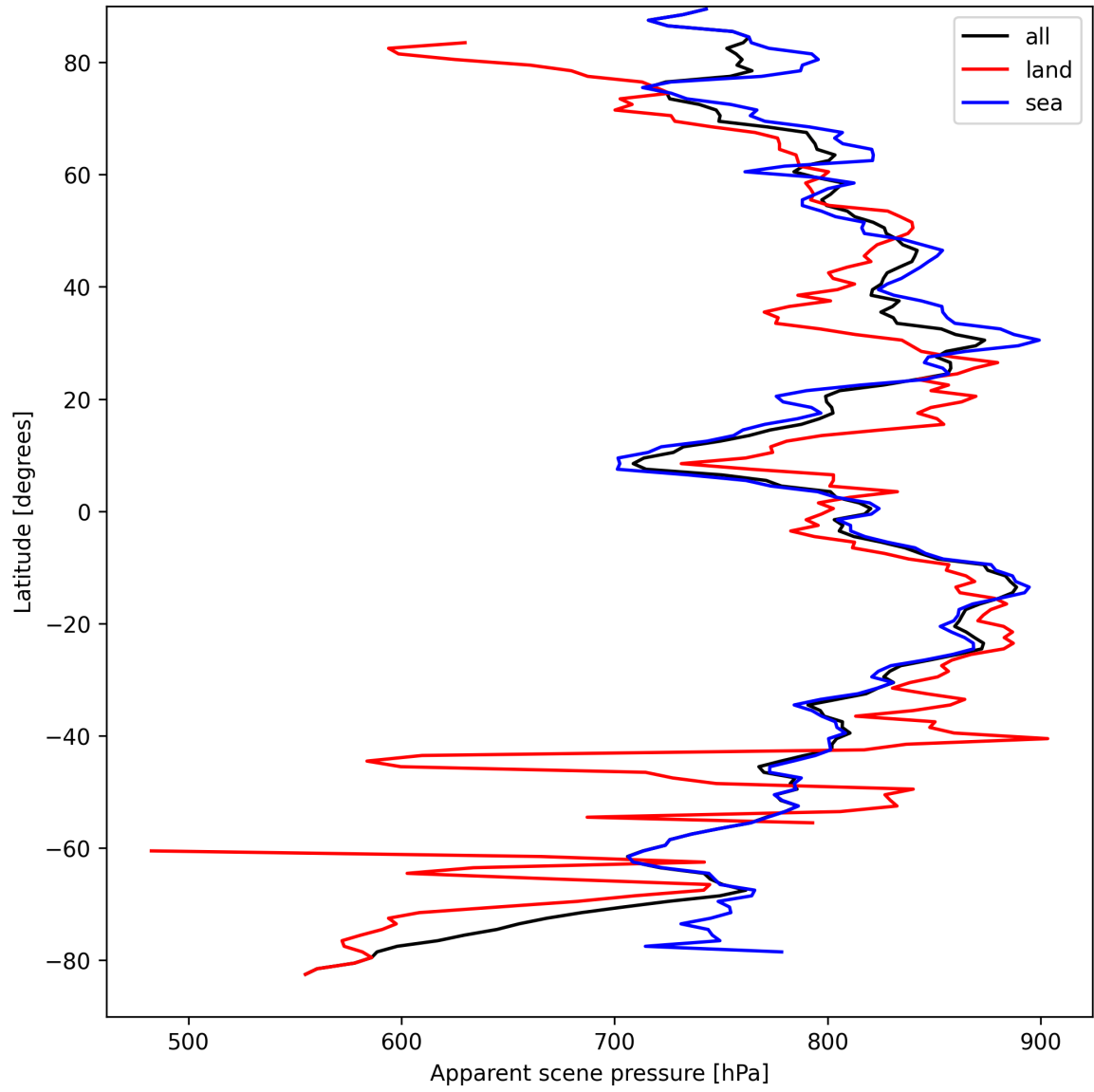
Figure 19: Zonal average of “Apparent scene pressure” for 2024-09-07 to 2024-09-09.
