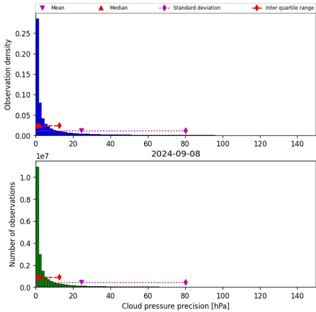
Figure 31: Histogram of “Cloud pressure precision” for 2024-09-07 to 2024-09-09
