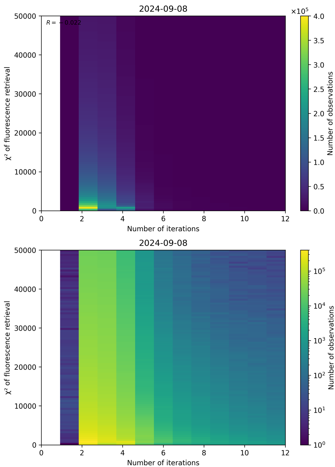
Figure 106: Scatter density plot of “Number of iterations” against “ \chi^2 of fluorescence retrieval” for 2024-09-07 to 2024-09-09.
