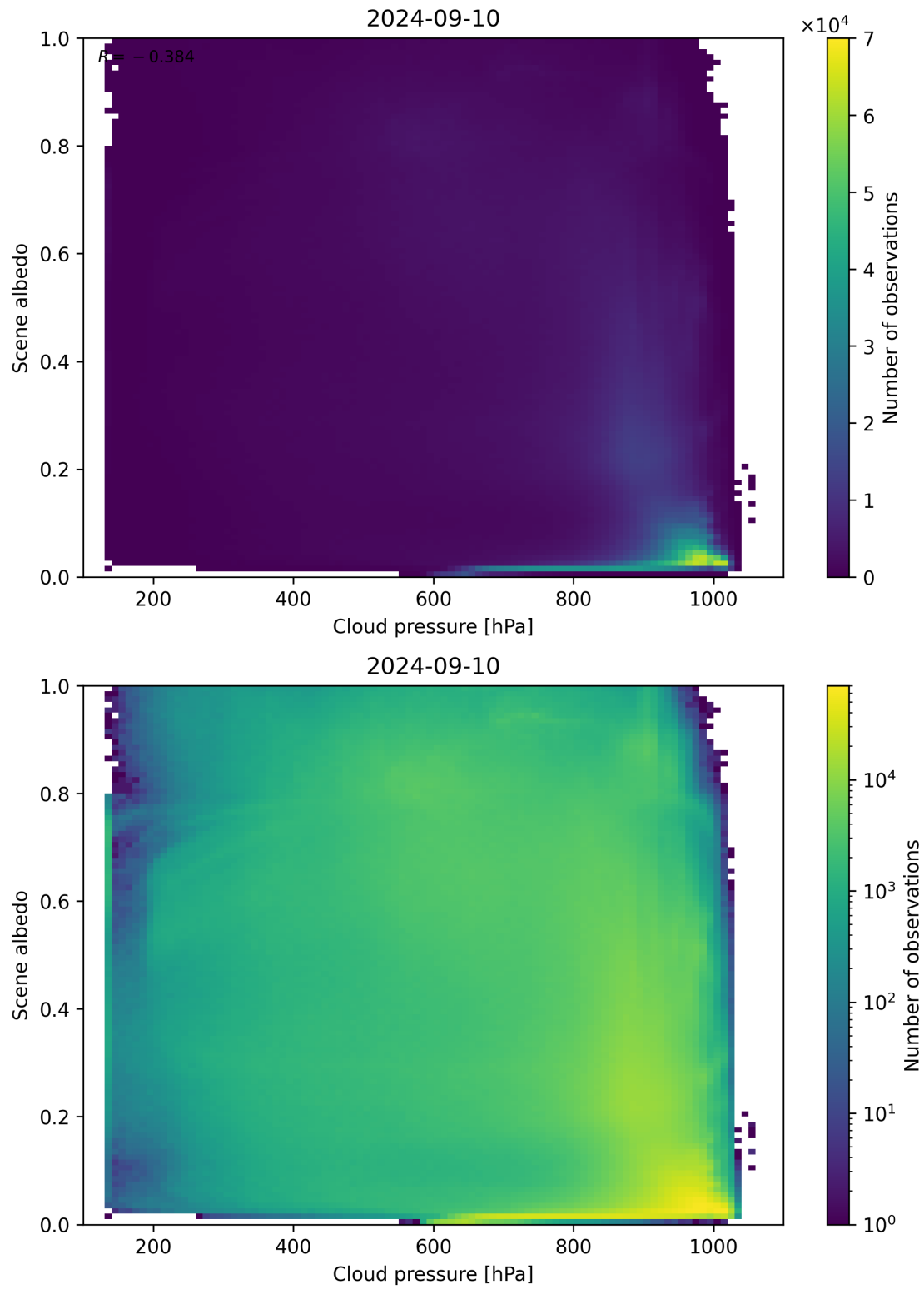
Figure 91: Scatter density plot of “Cloud pressure” against “Scene albedo” for 2024-09-09 to 2024-09-11.
