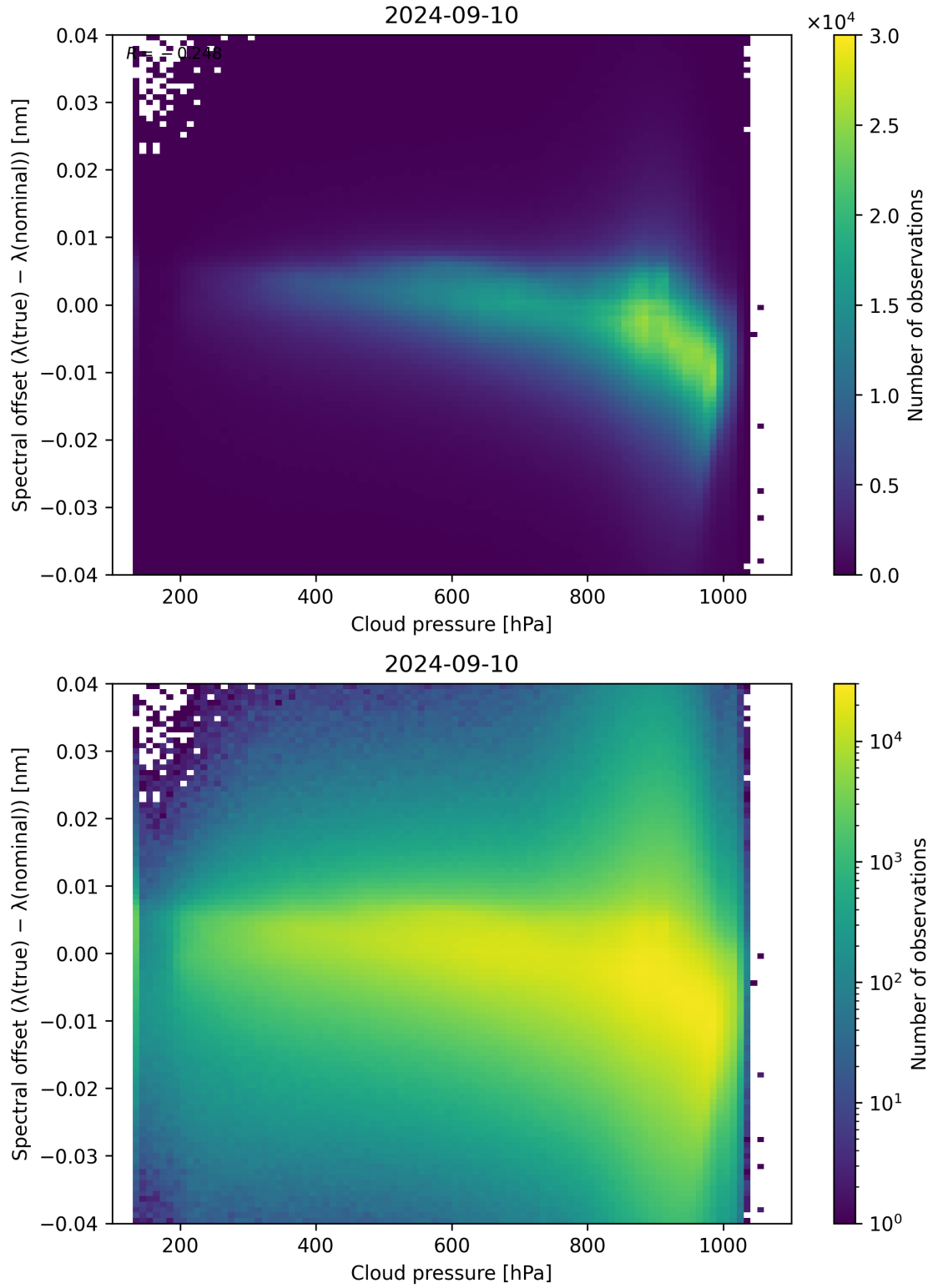
Figure 92: Scatter density plot of “Cloud pressure” against “Spectral offset ( \lambda_{\text{true}} - \lambda_{\text{nominal}} )” for 2024-09-09 to 2024-09-11.
