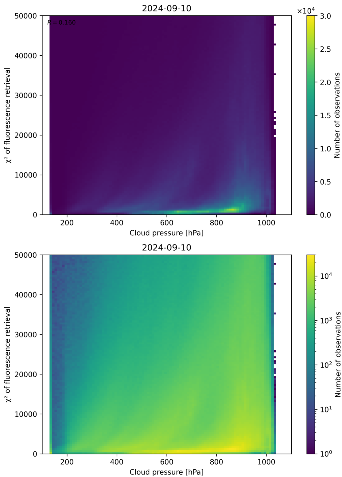
Figure 86: Scatter density plot of “Cloud pressure” against “ \chi^2 of fluorescence retrieval” for 2024-09-09 to 2024-09-11.
