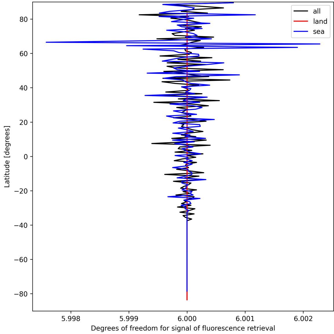
Figure 26: Zonal average of “Degrees of freedom for signal of fluorescence retrieval” for 2024-09-09 to 2024-09-11.
