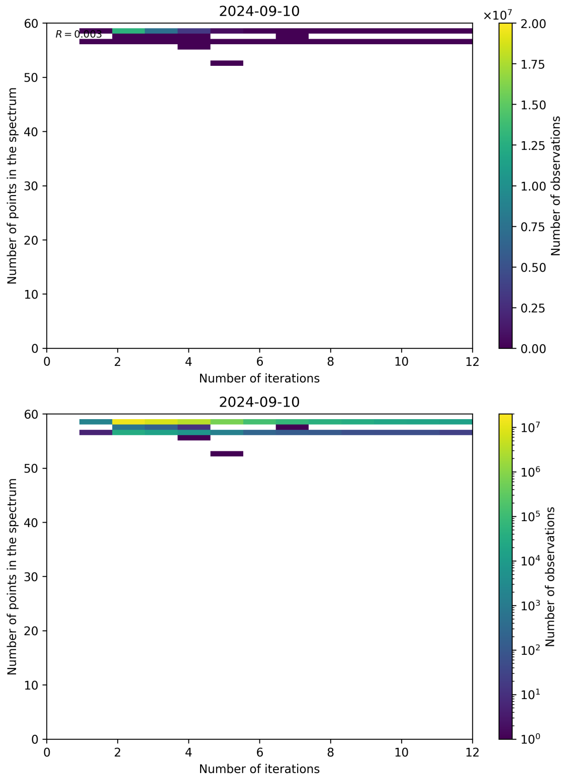
Figure 108: Scatter density plot of “Number of iterations” against “Number of points in the spectrum” for 2024-09-09 to 2024-09-11.
