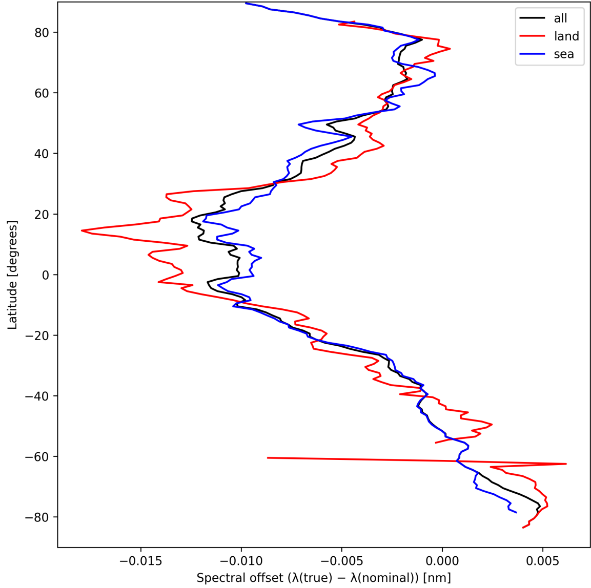
Figure 28: Zonal average of “Spectral offset ( \lambda_{\text{true}} - \lambda_{\text{nominal}} )” for 2024-09-09 to 2024-09-11.
