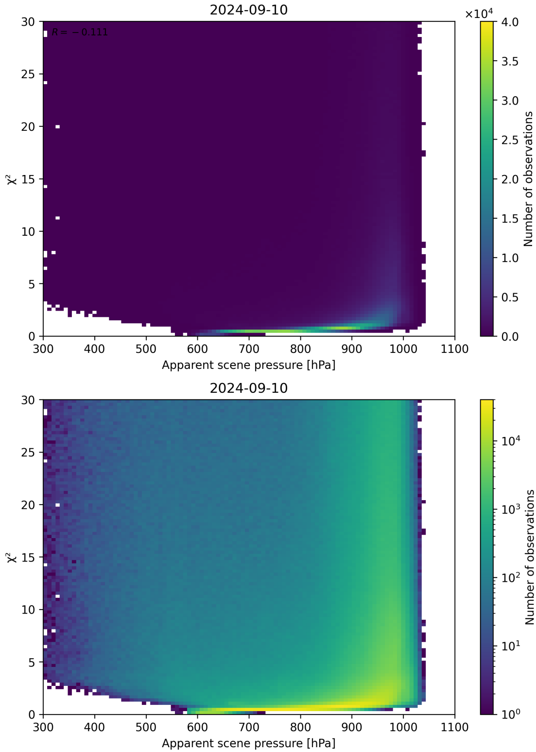
Figure 63: Scatter density plot of “Apparent scene pressure” against “ \chi^2 ” for 2024-09-09 to 2024-09-11.
