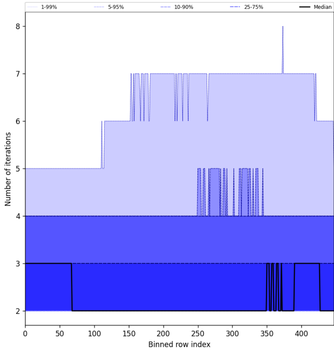
Figure 56: Along track statistics of “Number of iterations” for 2024-09-09 to 2024-09-11
