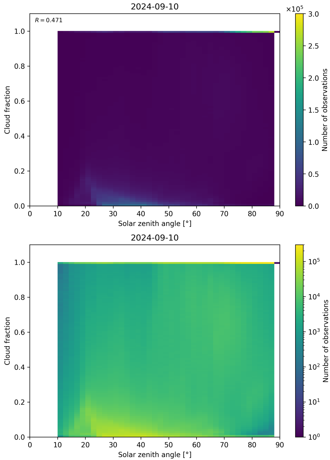
Figure 121: Scatter density plot of “Solar zenith angle” against “Cloud fraction” for 2024-09-09 to 2024-09-11.
