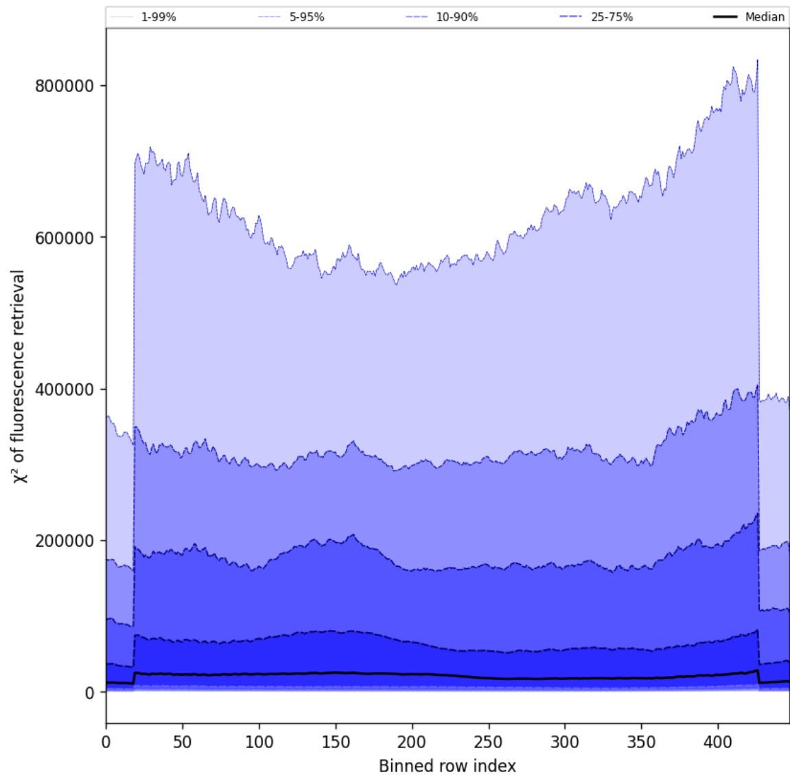
Figure 59: Along track statistics of “ \chi^2 of fluorescence retrieval” for 2024-09-09 to 2024-09-11
