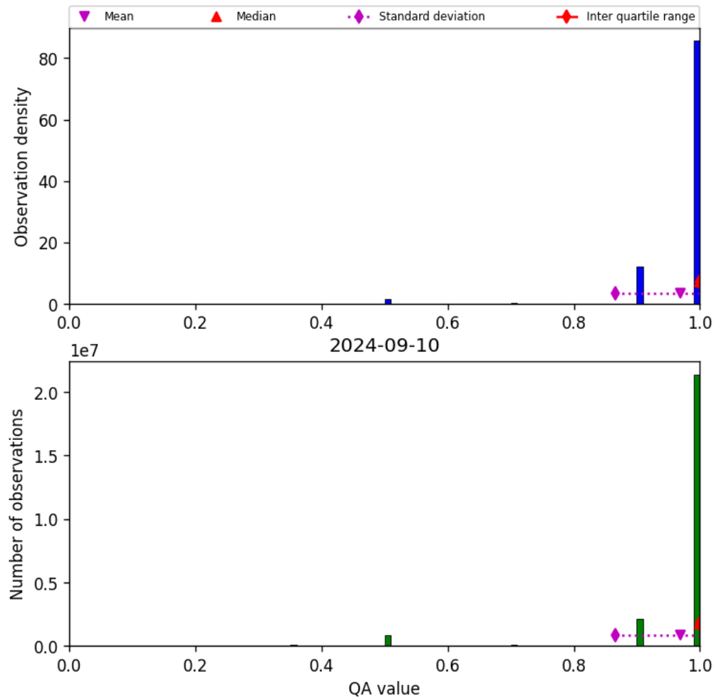
Figure 29: Histogram of “QA value” for 2024-09-09 to 2024-09-11
