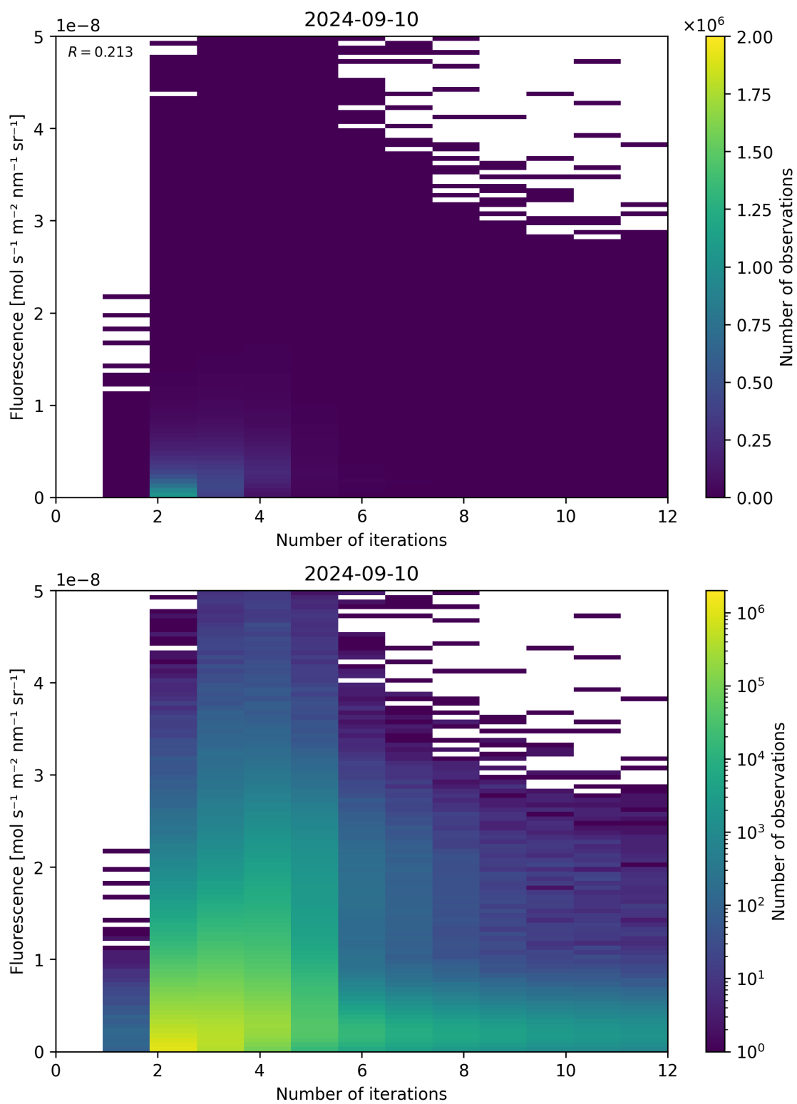
Figure 107: Scatter density plot of “Number of iterations” against “Fluorescence” for 2024-09-09 to 2024-09-11.
