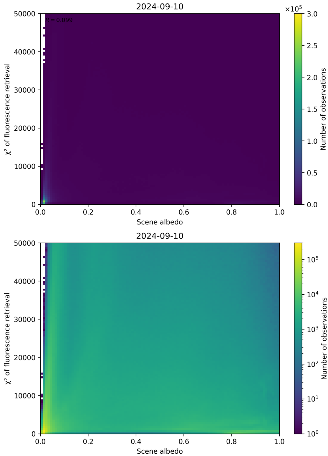
Figure 113: Scatter density plot of “Scene albedo” against “ \chi^2 of fluorescence retrieval” for 2024-09-09 to 2024-09-11.
