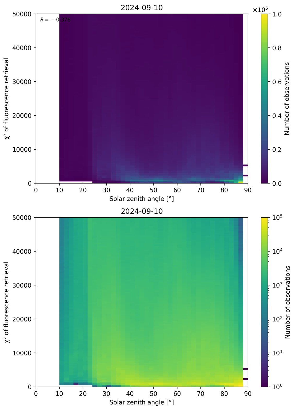
Figure 120: Scatter density plot of “Solar zenith angle” against “ \chi^2 of fluorescence retrieval” for 2024-09-09 to 2024-09-11.
