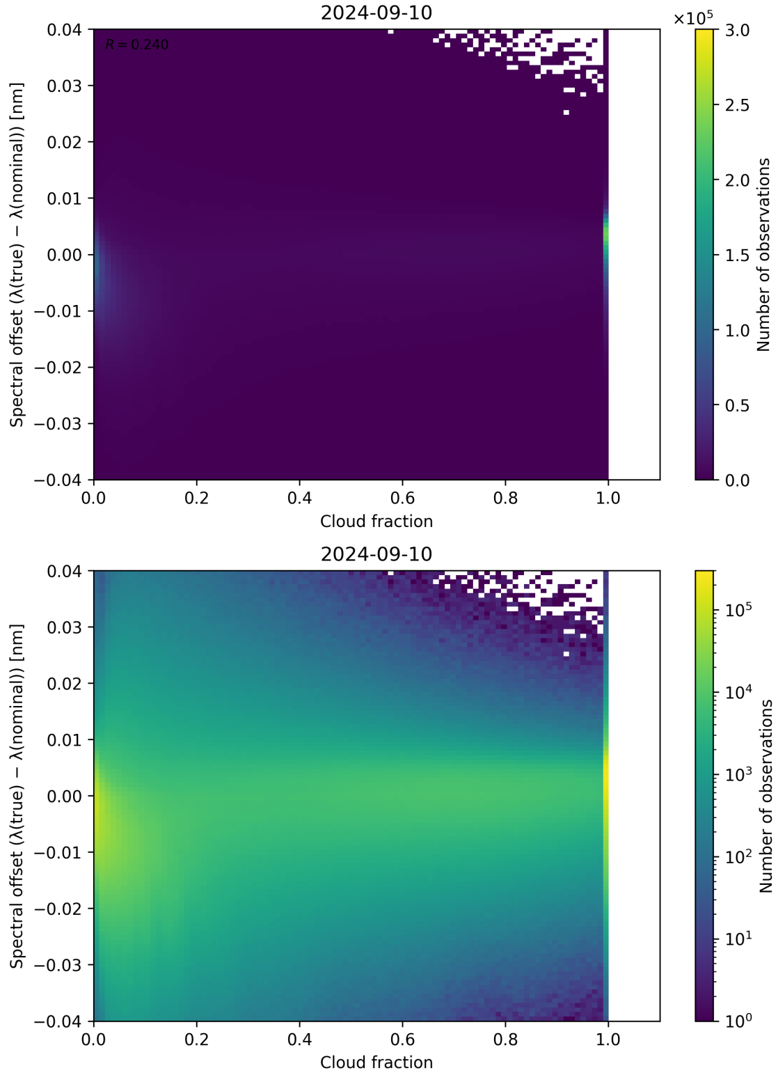
Figure 83: Scatter density plot of “Cloud fraction” against “Spectral offset ( \lambda_{\text{true}} - \lambda_{\text{nominal}} )” for 2024-09-09 to 2024-09-11.
