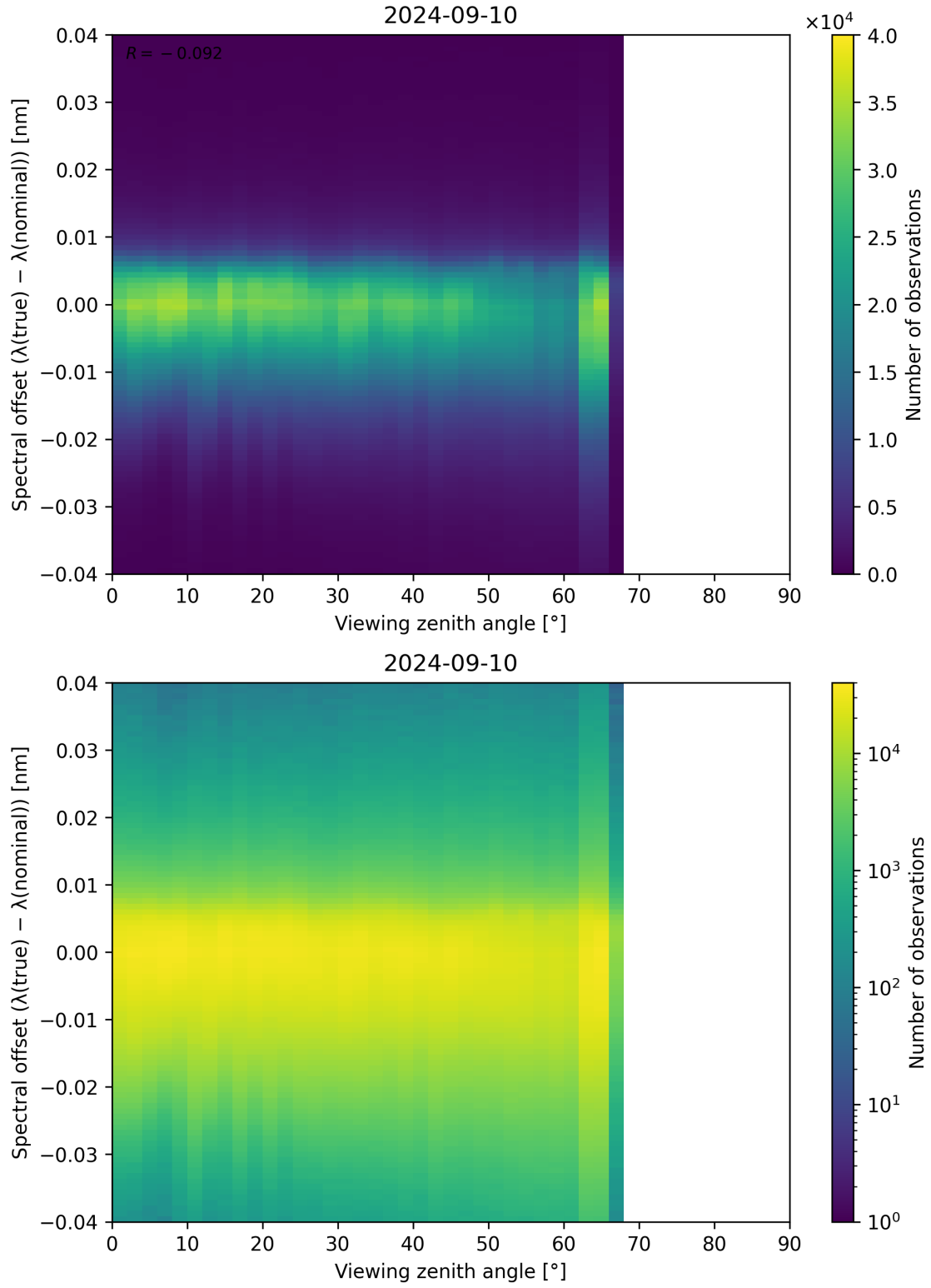
Figure 140: Scatter density plot of “Viewing zenith angle” against “Spectral offset ( \lambda_{\text{true}} - \lambda_{\text{nominal}} )” for 2024-09-09 to 2024-09-11.
