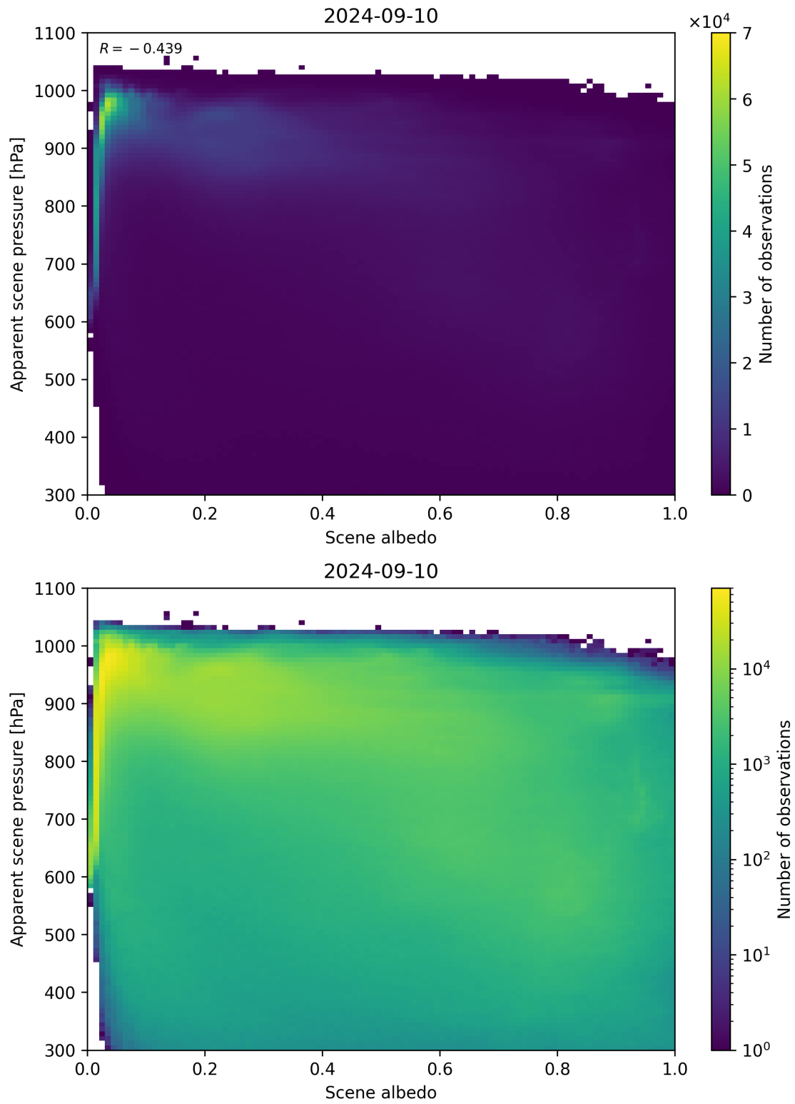
Figure 111: Scatter density plot of “Scene albedo” against “Apparent scene pressure” for 2024-09-09 to 2024-09-11.
