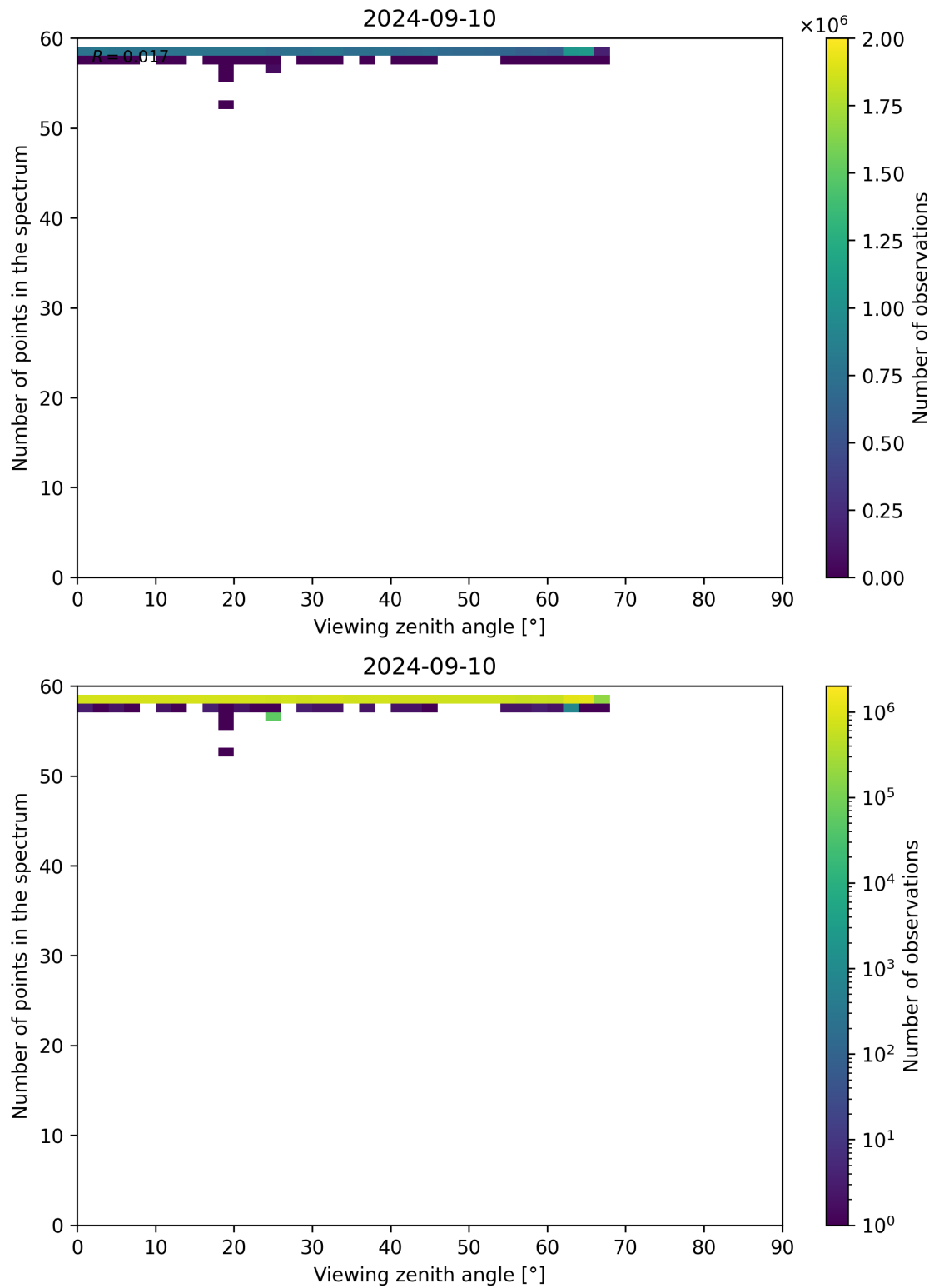
Figure 137: Scatter density plot of “Viewing zenith angle” against “Number of points in the spectrum” for 2024-09-09 to 2024-09-11.
