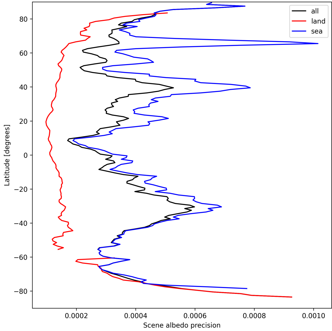
Figure 18: Zonal average of “Scene albedo precision” for 2024-09-09 to 2024-09-11.
