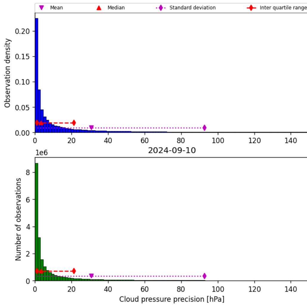
Figure 31: Histogram of “Cloud pressure precision” for 2024-09-09 to 2024-09-11
