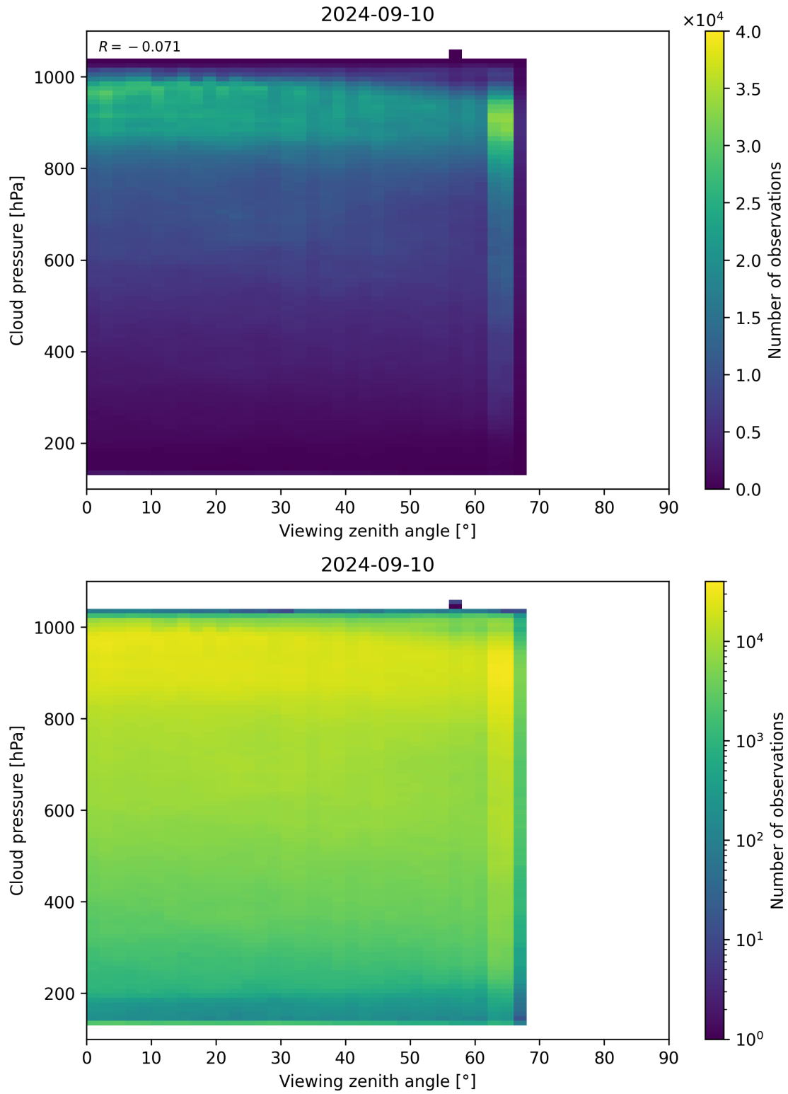
Figure 133: Scatter density plot of “Viewing zenith angle” against “Cloud pressure” for 2024-09-09 to 2024-09-11.
