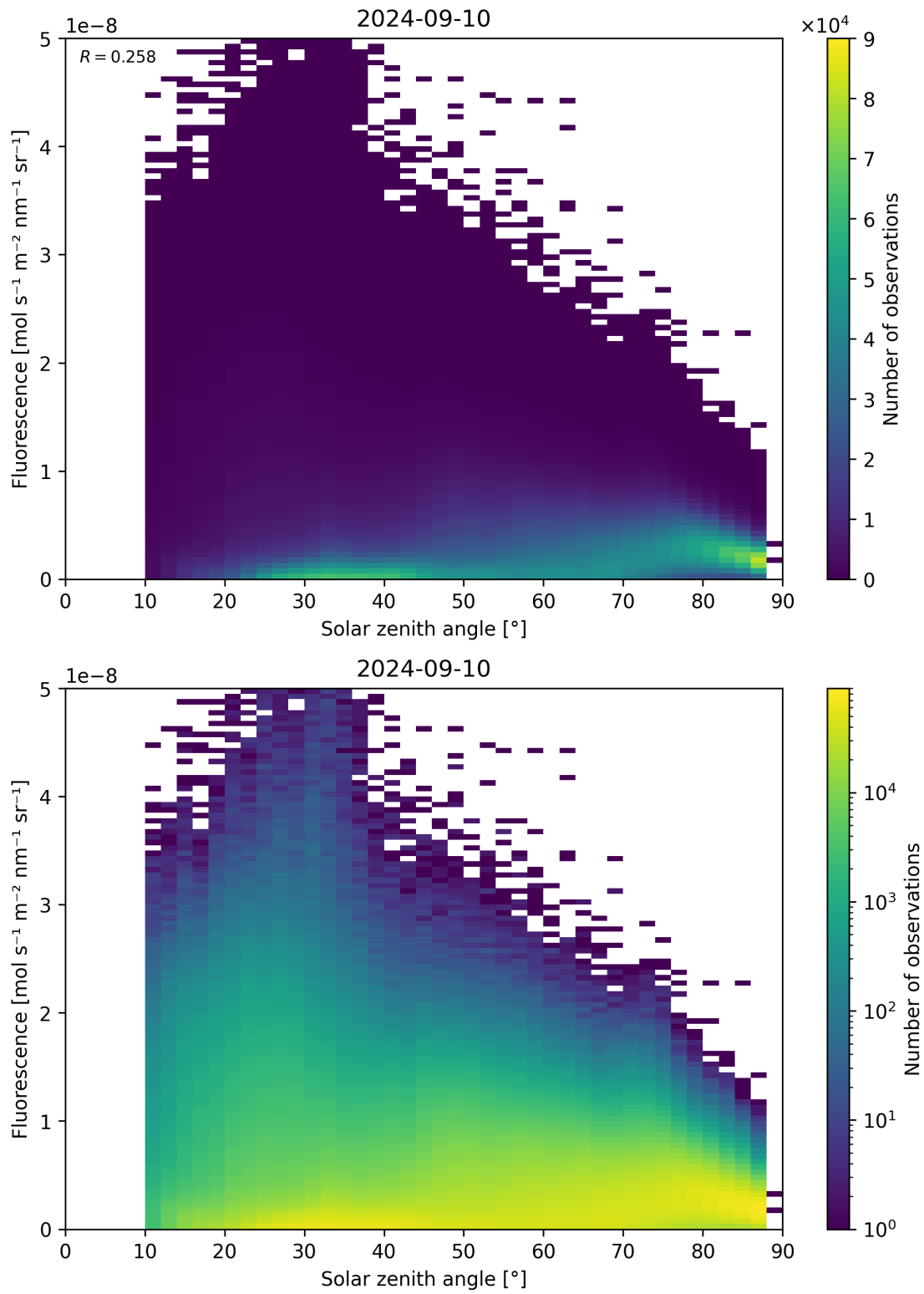
Figure 123: Scatter density plot of “Solar zenith angle” against “Fluorescence” for 2024-09-09 to 2024-09-11.
