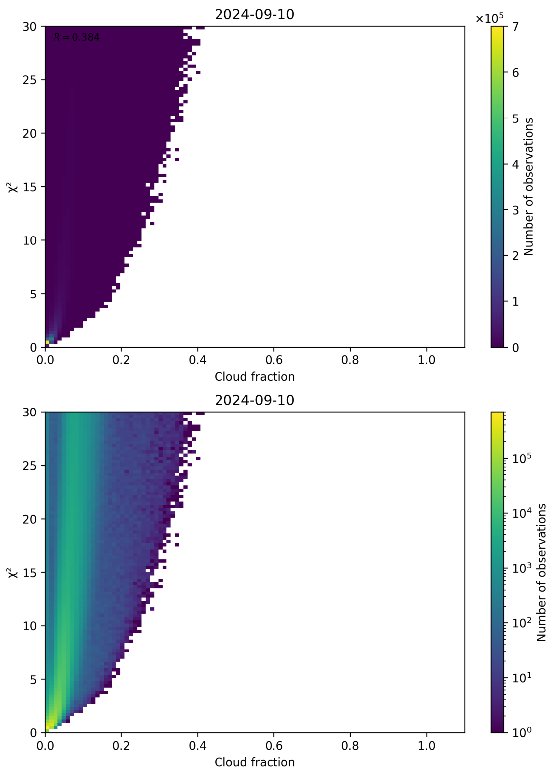
Figure 77: Scatter density plot of “Cloud fraction” against “ \chi^2 ” for 2024-09-09 to 2024-09-11.
