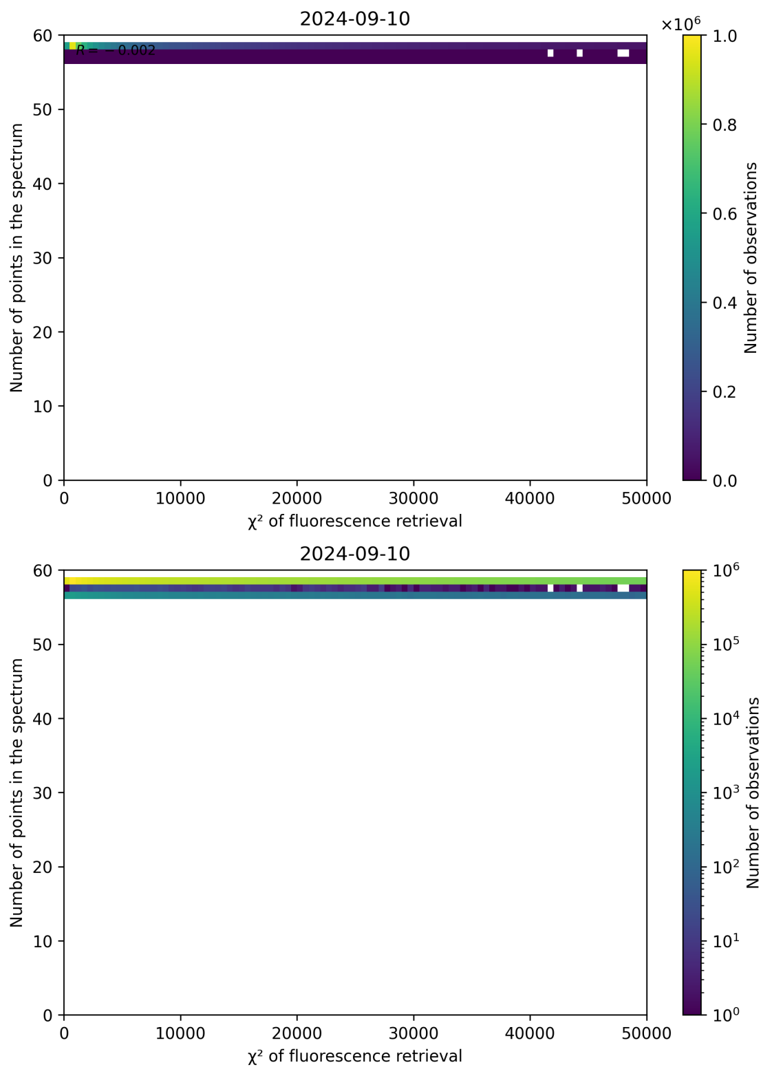
Figure 71: Scatter density plot of “ \chi^2 of fluorescence retrieval” against “Number of points in the spectrum” for 2024-09-09 to 2024-09-11.
