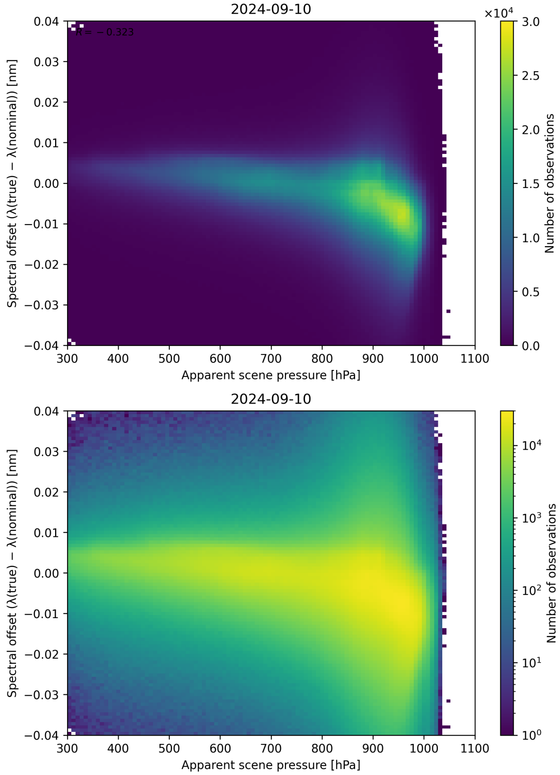
Figure 68: Scatter density plot of “Apparent scene pressure” against “Spectral offset ( \lambda_{\text{true}} - \lambda_{\text{nominal}} )” for 2024-09-09 to 2024-09-11.
