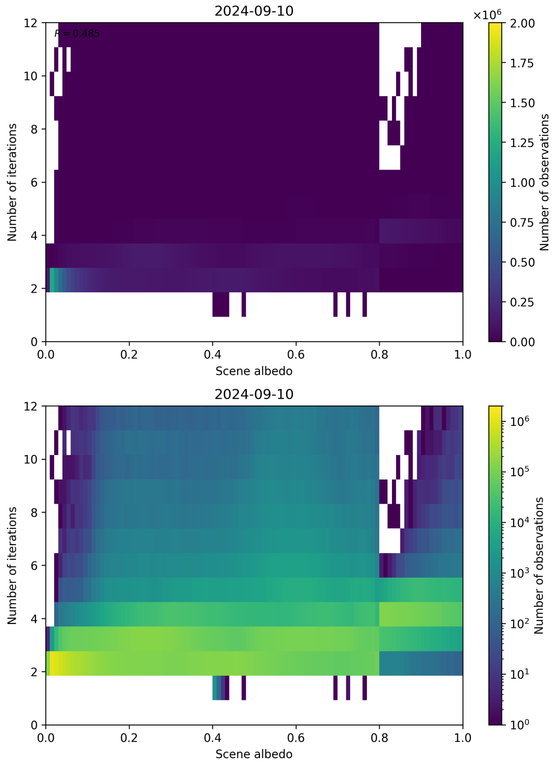
Figure 115: Scatter density plot of “Scene albedo” against “Number of iterations” for 2024-09-09 to 2024-09-11.
