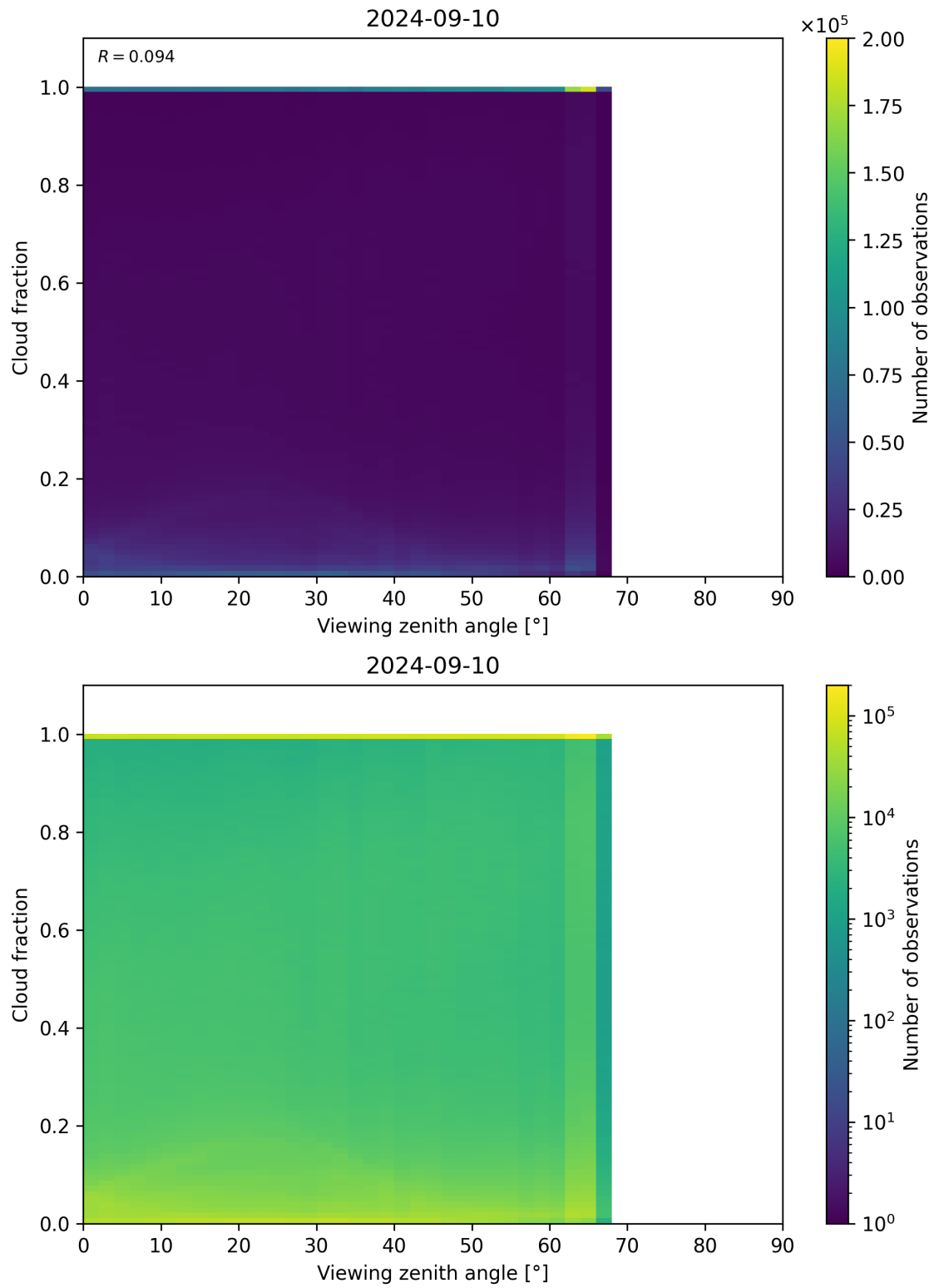
Figure 132: Scatter density plot of “Viewing zenith angle” against “Cloud fraction” for 2024-09-09 to 2024-09-11.
