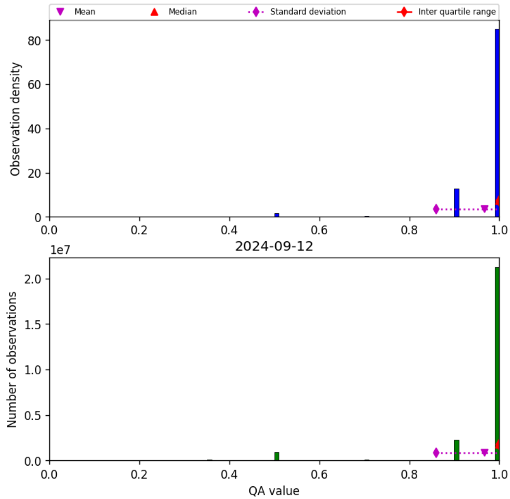
Figure 29: Histogram of “QA value” for 2024-09-12 to 2024-09-13
