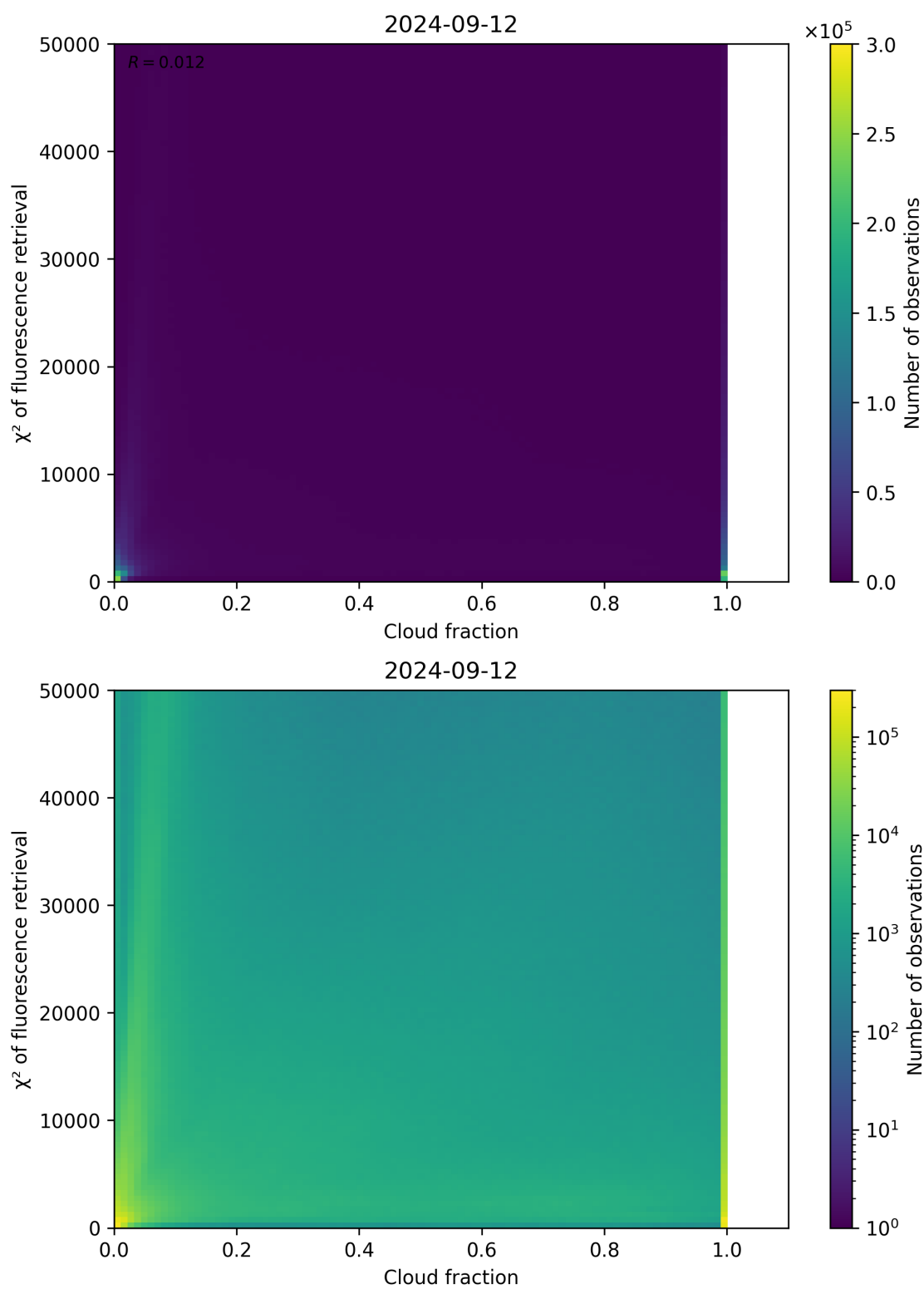
Figure 78: Scatter density plot of “Cloud fraction” against “ \chi^2 of fluorescence retrieval” for 2024-09-12 to 2024-09-13.
