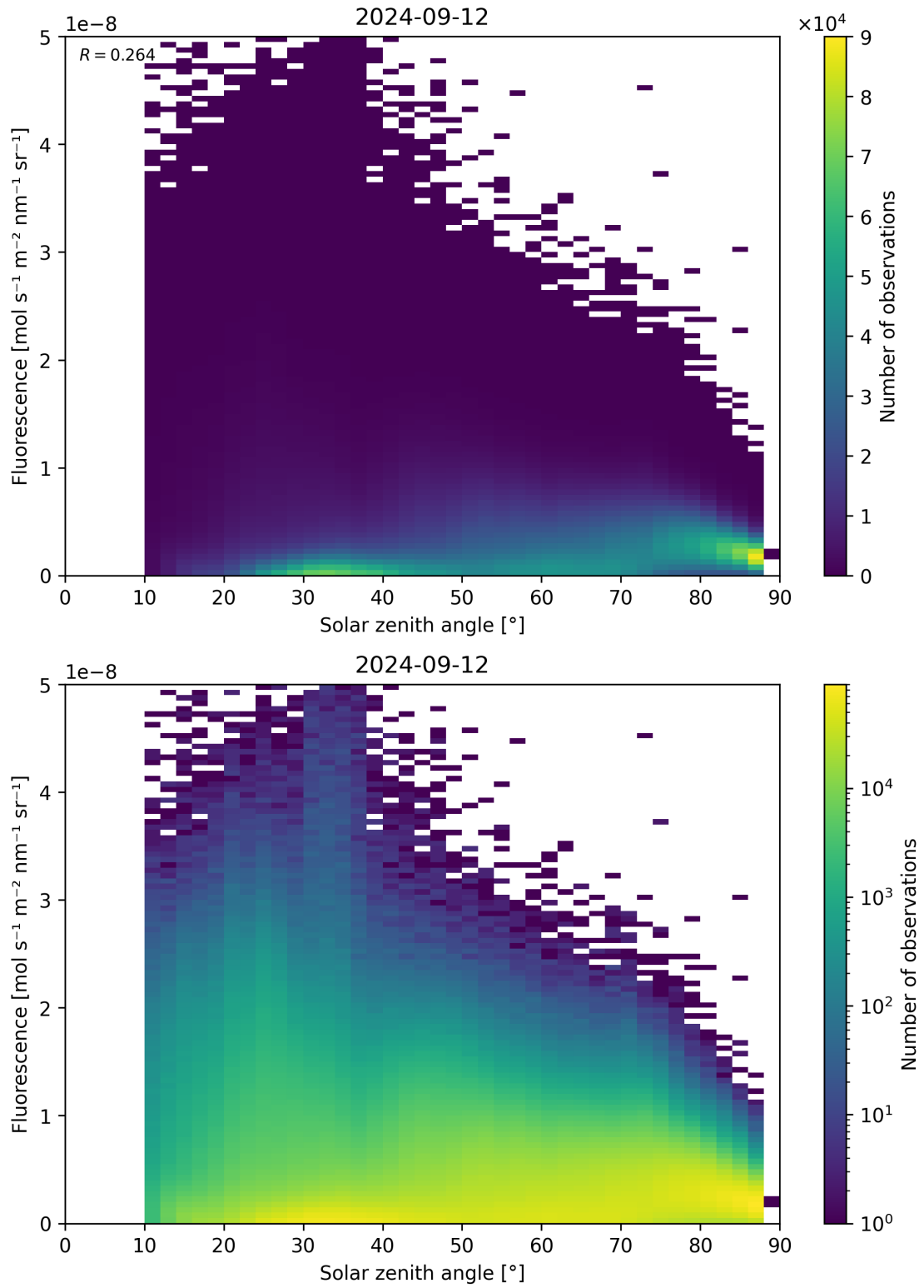
Figure 123: Scatter density plot of “Solar zenith angle” against “Fluorescence” for 2024-09-12 to 2024-09-13.
