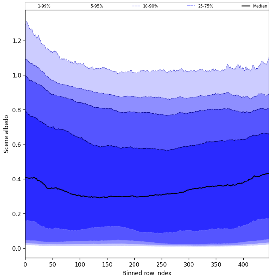
Figure 51: Along track statistics of “Scene albedo” for 2024-09-12 to 2024-09-13
