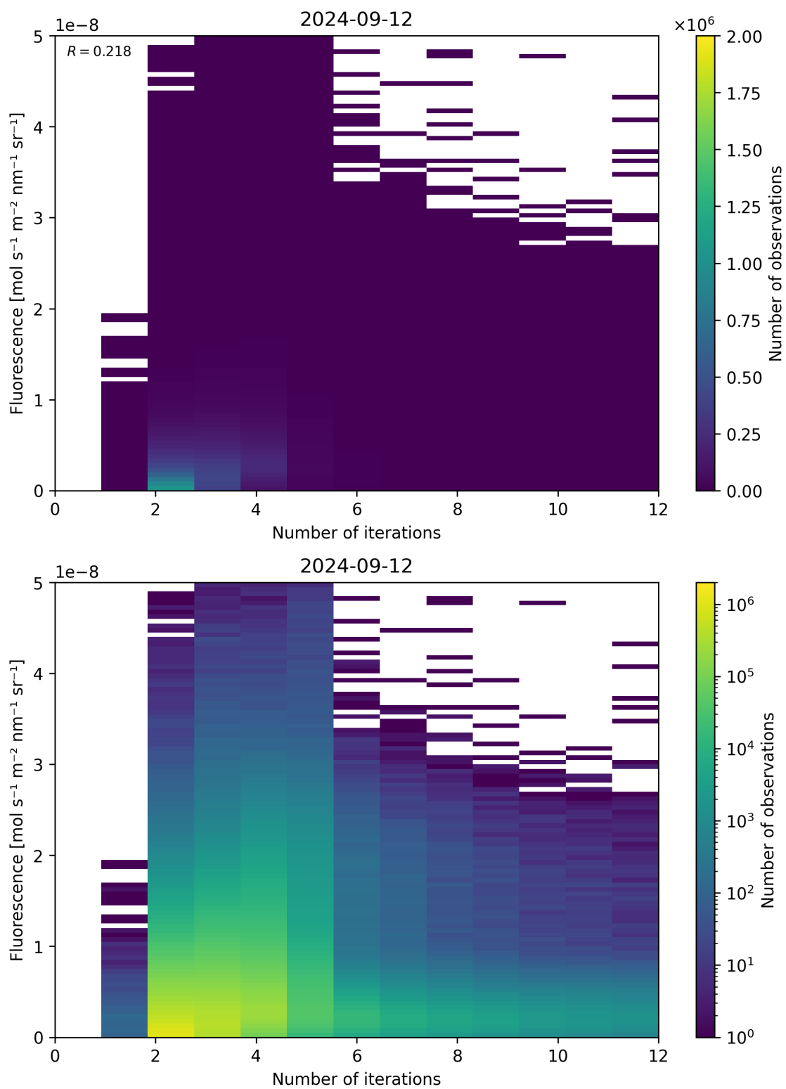
Figure 107: Scatter density plot of “Number of iterations” against “Fluorescence” for 2024-09-12 to 2024-09-13.
