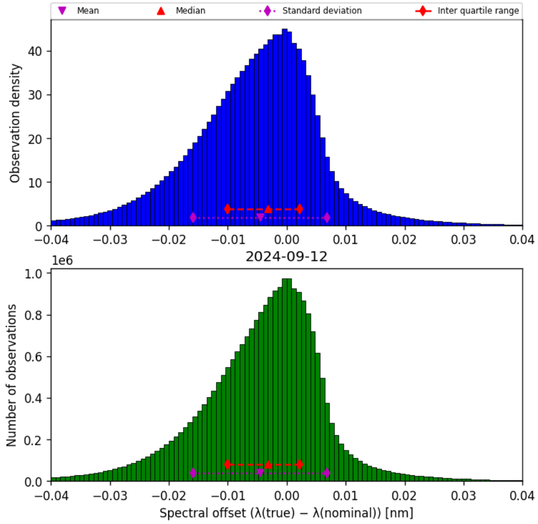
Figure 45: Histogram of “Spectral offset ( \lambda_{\text{true}} - \lambda_{\text{nominal}} )” for 2024-09-12 to 2024-09-13
