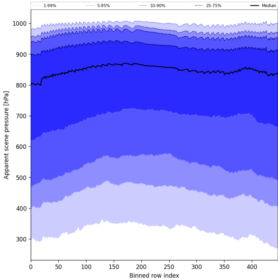
Figure 53: Along track statistics of “Apparent scene pressure” for 2024-09-12 to 2024-09-13
