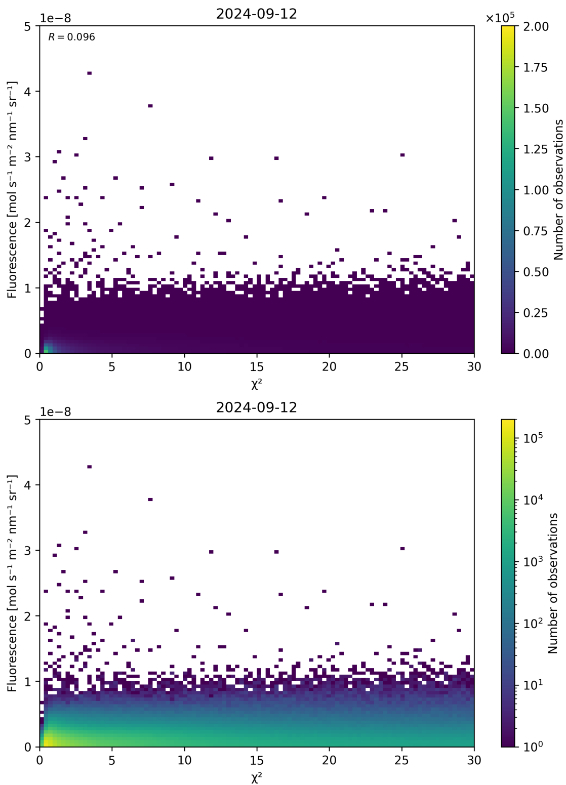
Figure 70: Scatter density plot of “ \chi^2 ” against “Fluorescence” for 2024-09-12 to 2024-09-13.
