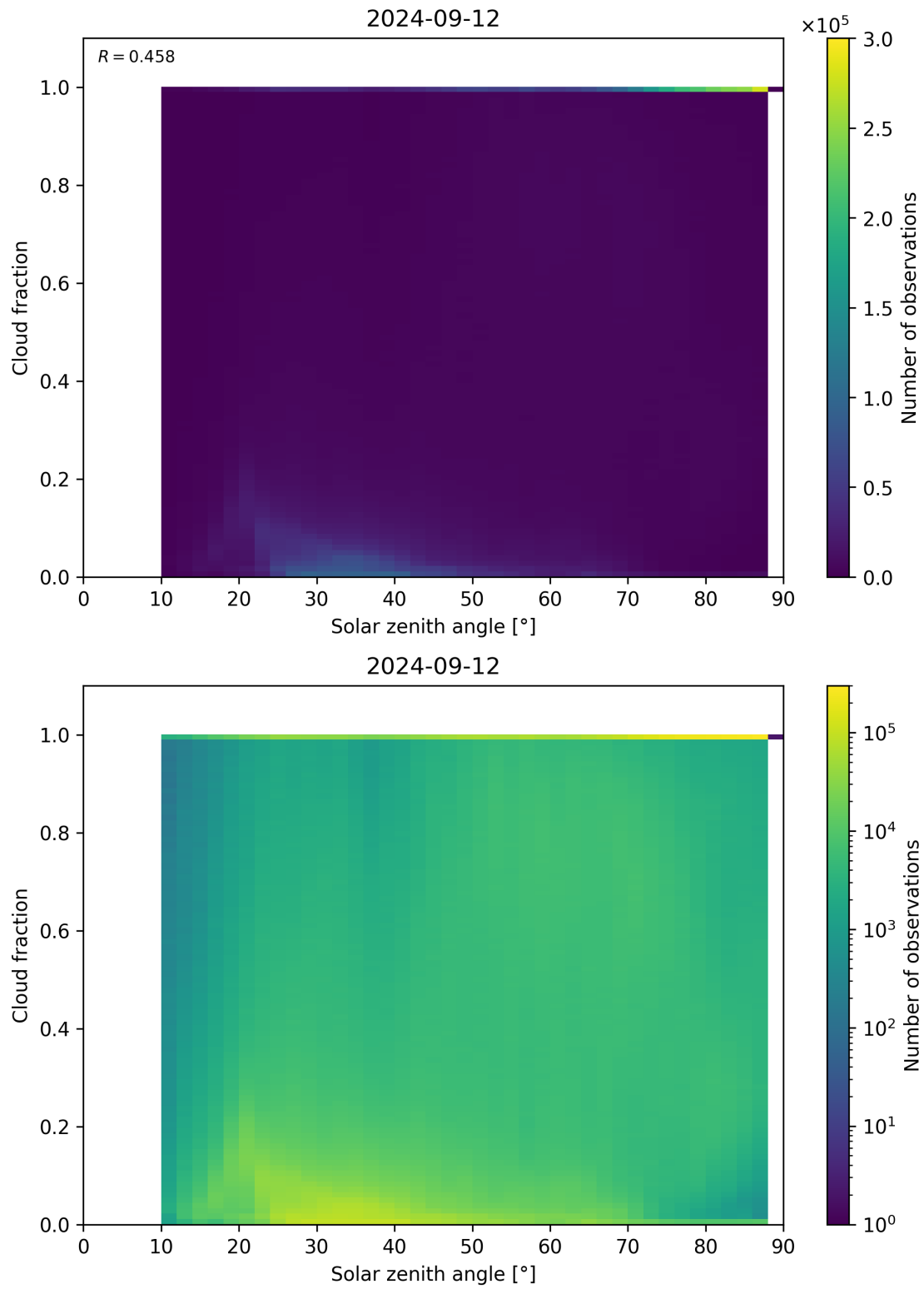
Figure 121: Scatter density plot of “Solar zenith angle” against “Cloud fraction” for 2024-09-12 to 2024-09-13.
