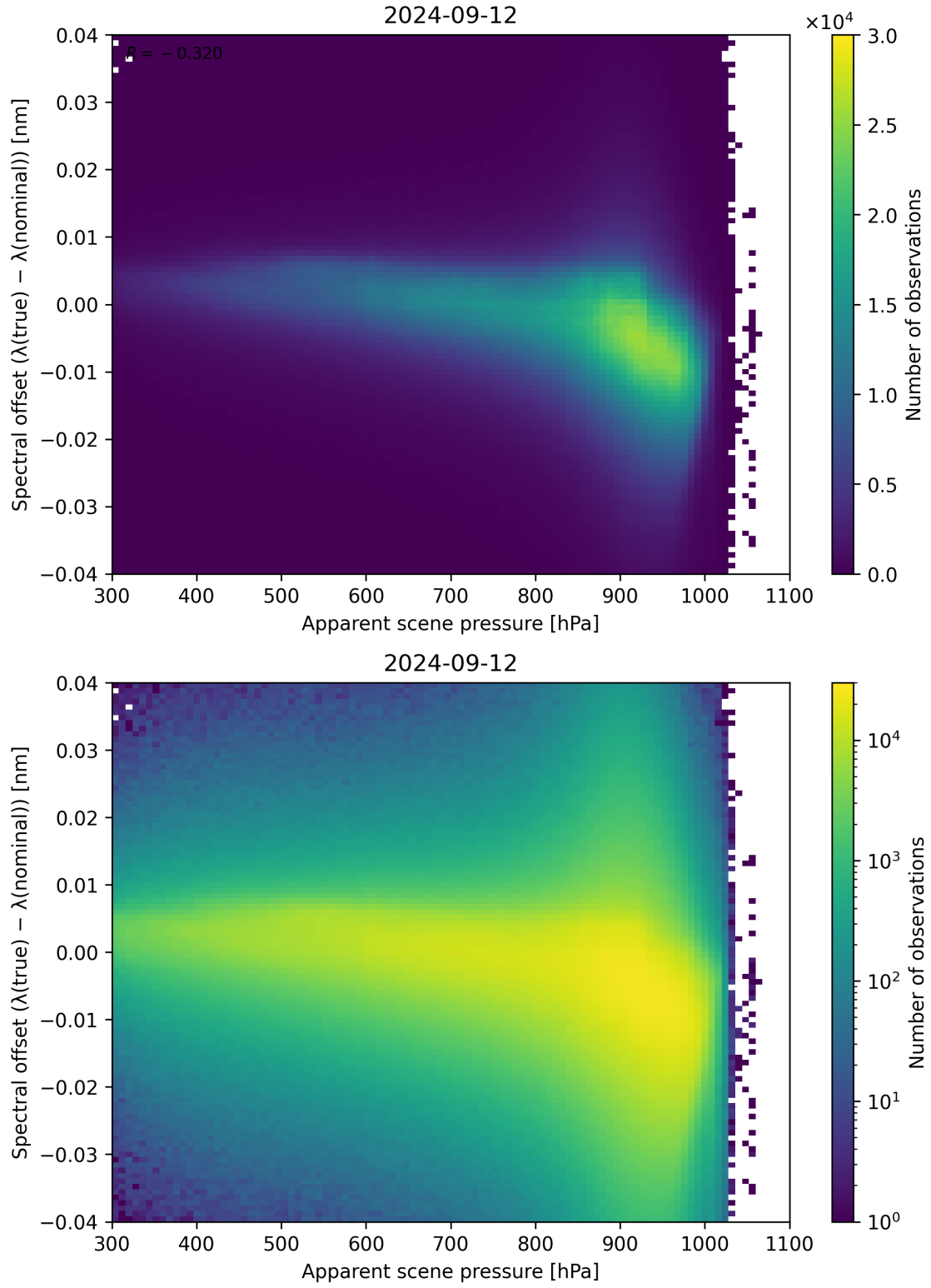
Figure 68: Scatter density plot of “Apparent scene pressure” against “Spectral offset ( \lambda_{\text{true}} - \lambda_{\text{nominal}} )” for 2024-09-12 to 2024-09-13.
