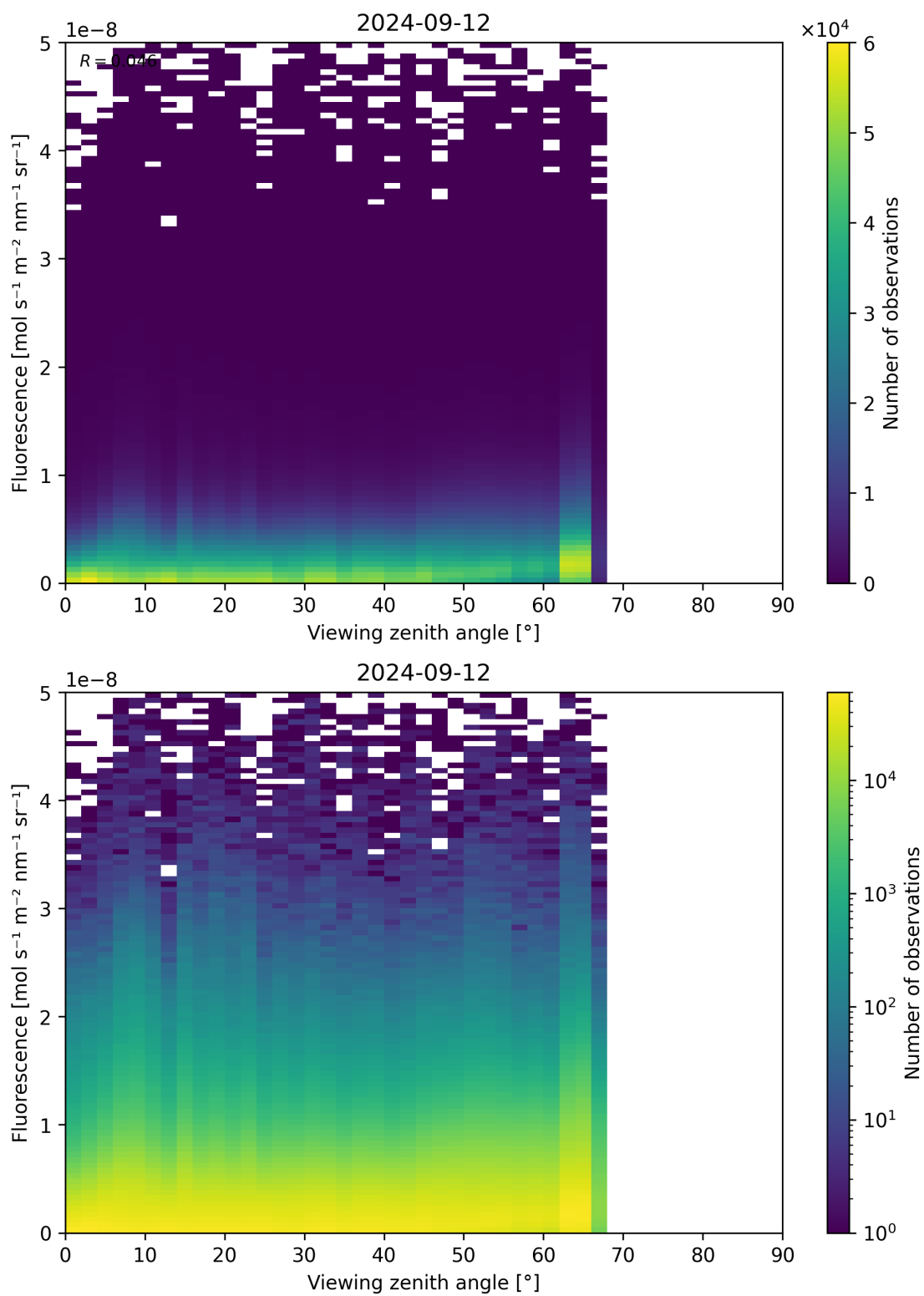
Figure 134: Scatter density plot of “Viewing zenith angle” against “Fluorescence” for 2024-09-12 to 2024-09-13.
