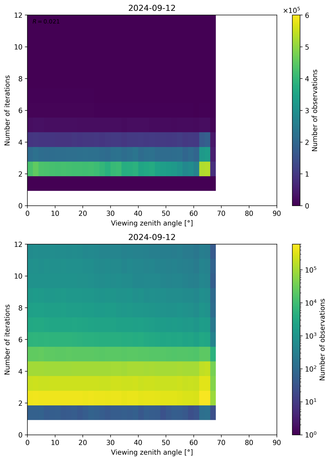
Figure 136: Scatter density plot of “Viewing zenith angle” against “Number of iterations” for 2024-09-12 to 2024-09-13.
