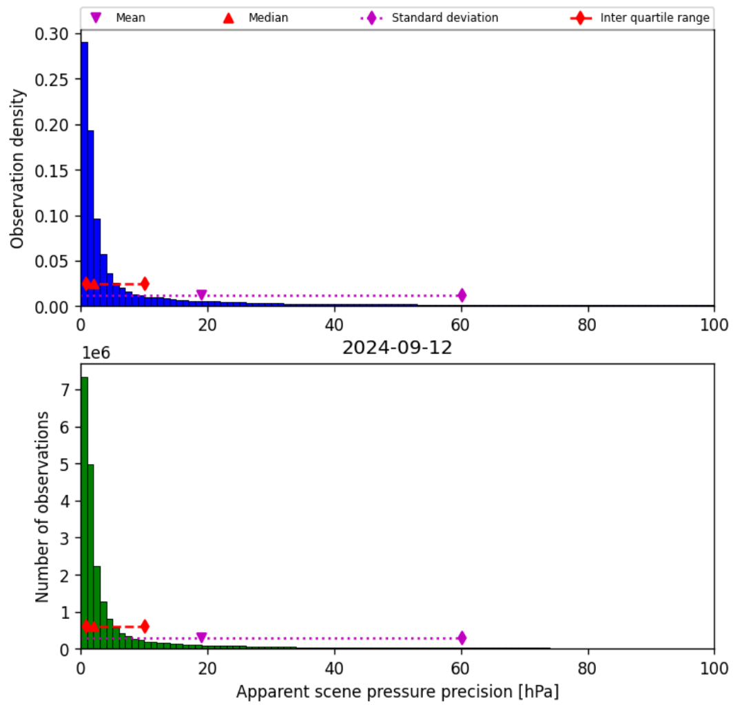
Figure 37: Histogram of “Apparent scene pressure precision” for 2024-09-12 to 2024-09-13
