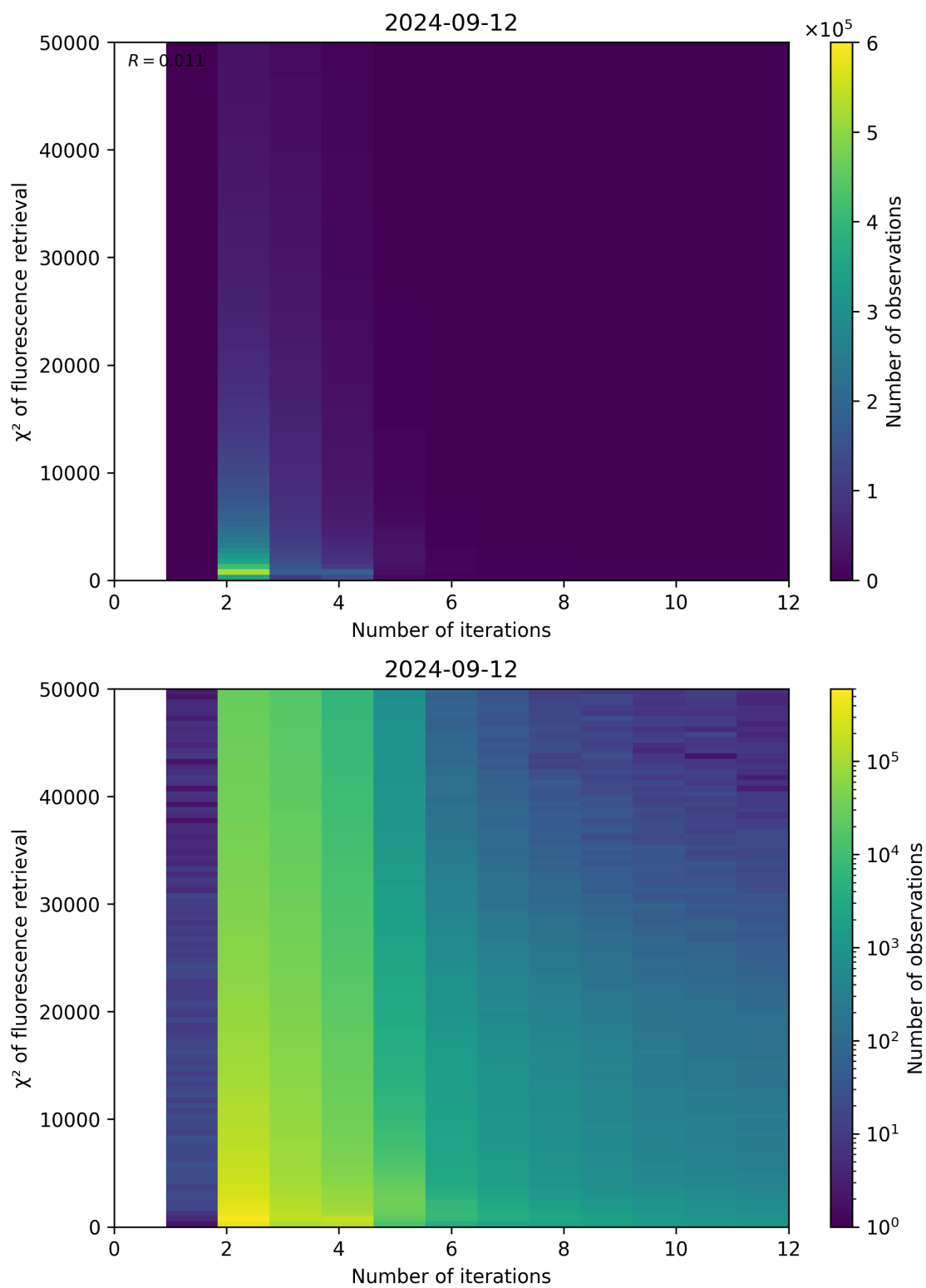
Figure 106: Scatter density plot of “Number of iterations” against “ \chi^2 of fluorescence retrieval” for 2024-09-12 to 2024-09-13.
