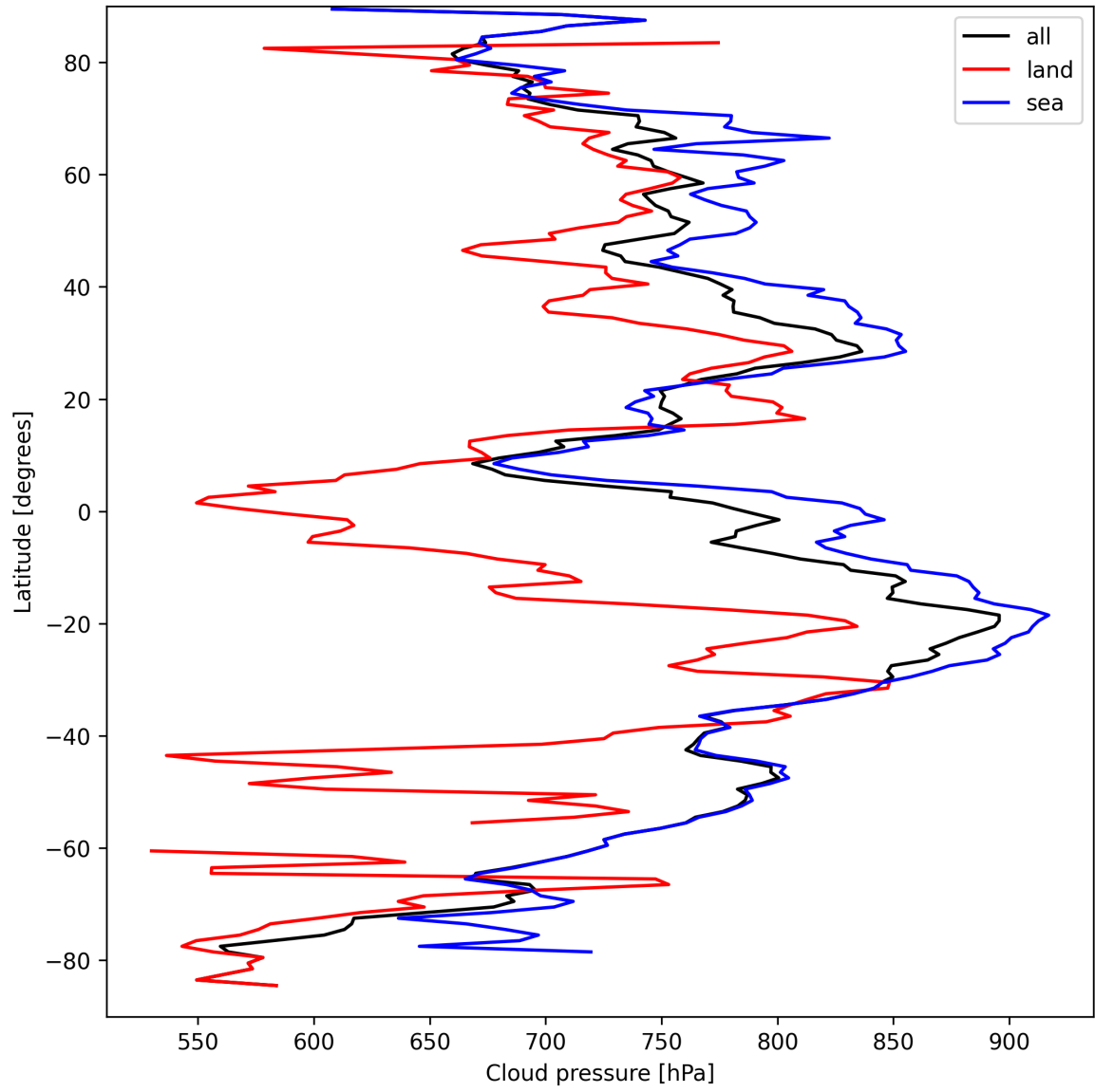
Figure 13: Zonal average of “Cloud pressure” for 2024-09-12 to 2024-09-13.
