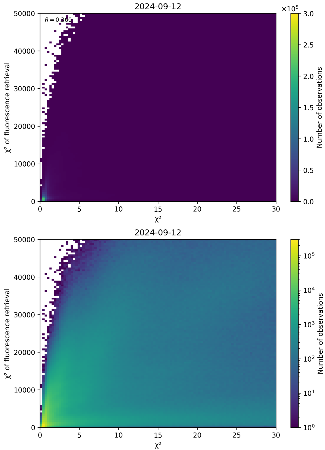
Figure 69: Scatter density plot of “ \chi^2 ” against “ \chi^2 of fluorescence retrieval” for 2024-09-12 to 2024-09-13.
