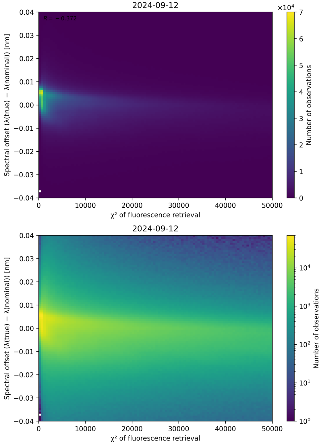
Figure 72: Scatter density plot of “ \chi^2 of fluorescence retrieval” against “Spectral offset ( \lambda_{\text{true}} - \lambda_{\text{nominal}} )” for 2024-09-12 to 2024-09-13.
