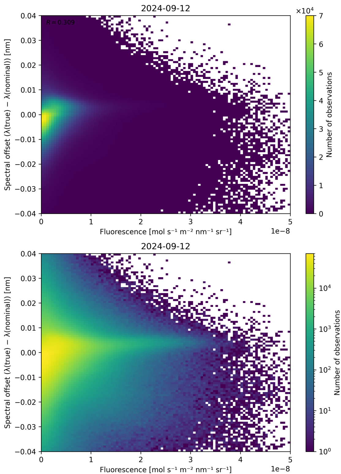
Figure 95: Scatter density plot of “Fluorescence” against “Spectral offset ( \lambda_{\text{true}} - \lambda_{\text{nominal}} )” for 2024-09-12 to 2024-09-13.
