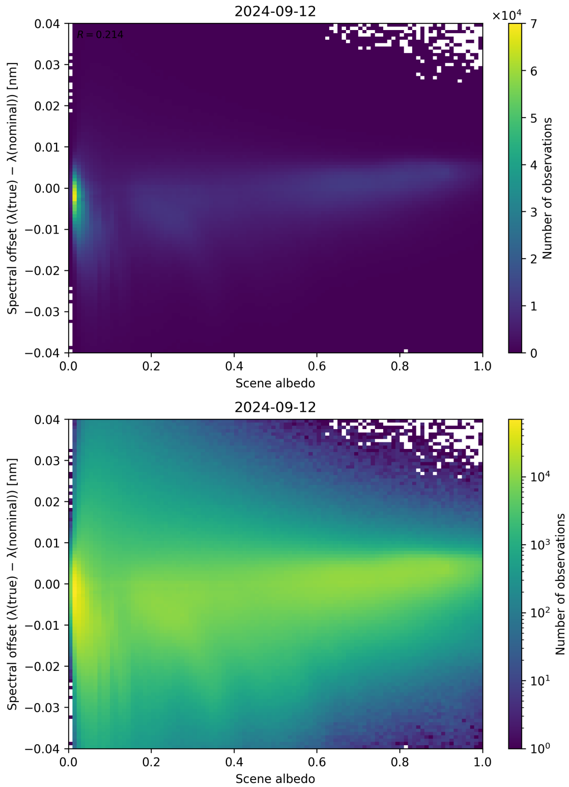
Figure 117: Scatter density plot of “Scene albedo” against “Spectral offset ( \lambda_{\text{true}} - \lambda_{\text{nominal}} )” for 2024-09-12 to 2024-09-13.
