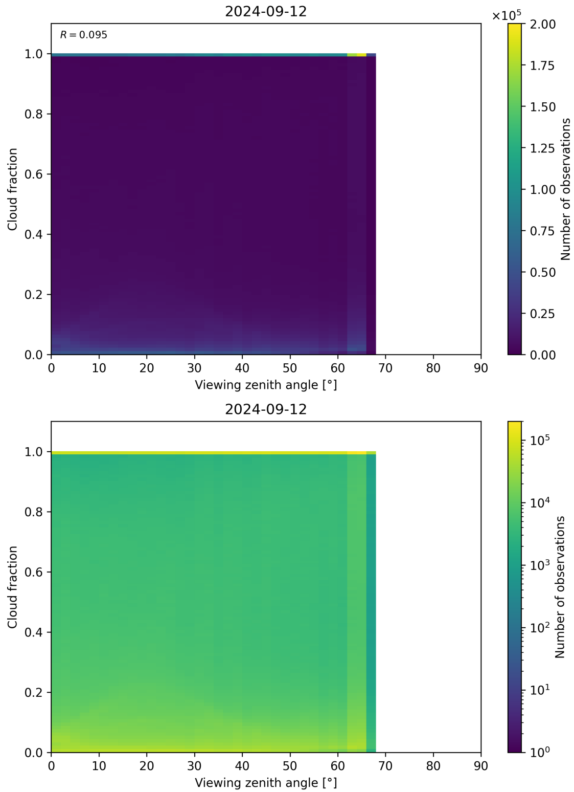
Figure 132: Scatter density plot of “Viewing zenith angle” against “Cloud fraction” for 2024-09-12 to 2024-09-13.
