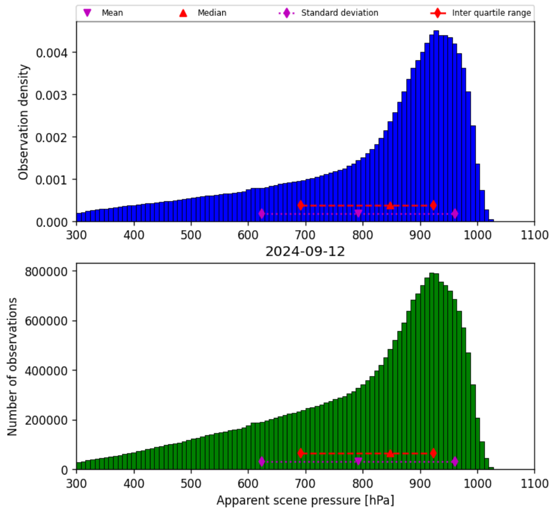
Figure 36: Histogram of “Apparent scene pressure” for 2024-09-12 to 2024-09-13
