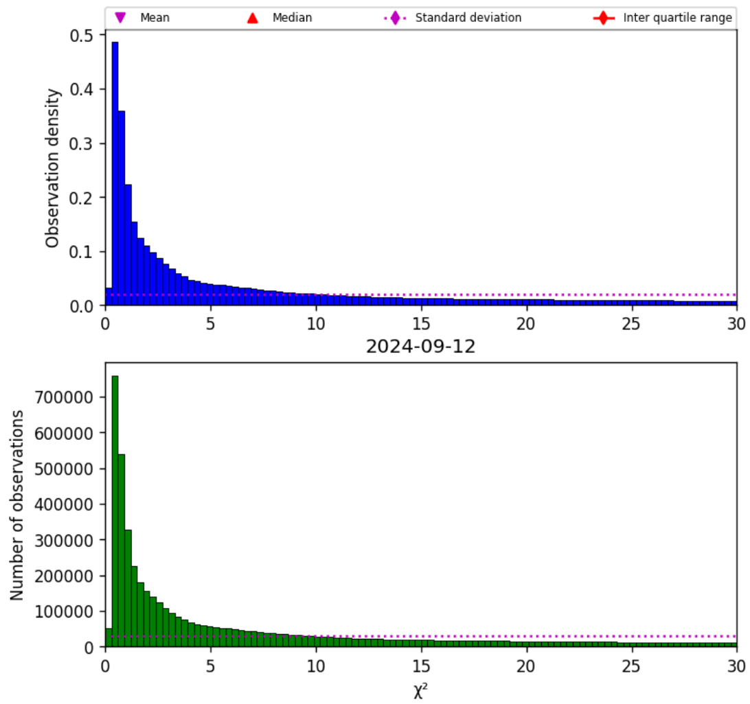
Figure 38: Histogram of “ \chi^2 ” for 2024-09-12 to 2024-09-13
