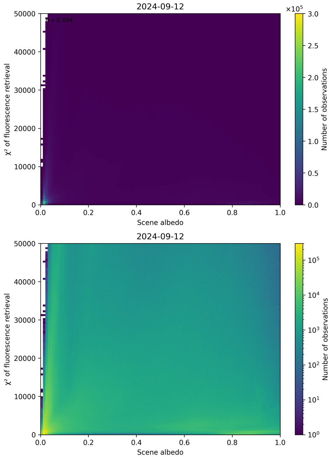
Figure 113: Scatter density plot of “Scene albedo” against “ \chi^2 of fluorescence retrieval” for 2024-09-12 to 2024-09-13.
