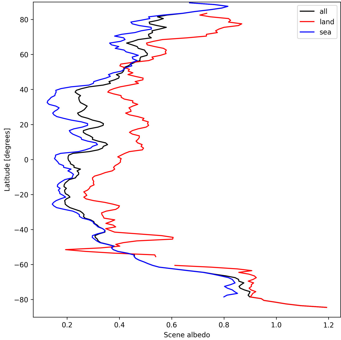
Figure 17: Zonal average of “Scene albedo” for 2024-09-12 to 2024-09-13.
