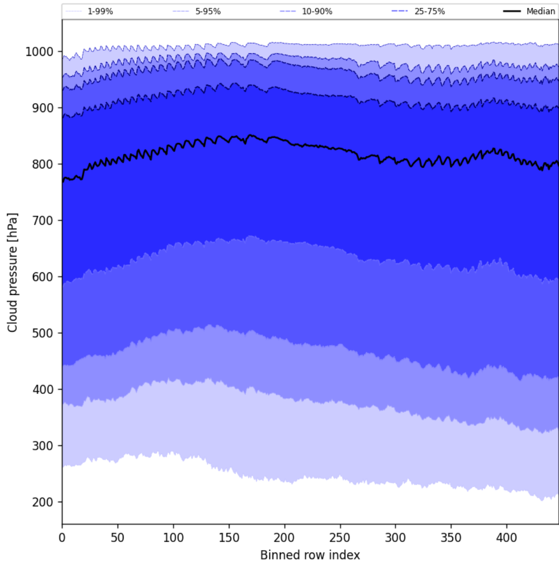
Figure 47: Along track statistics of “Cloud pressure” for 2024-09-12 to 2024-09-13
