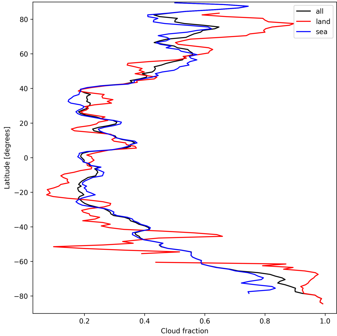
Figure 15: Zonal average of “Cloud fraction” for 2024-09-12 to 2024-09-13.
