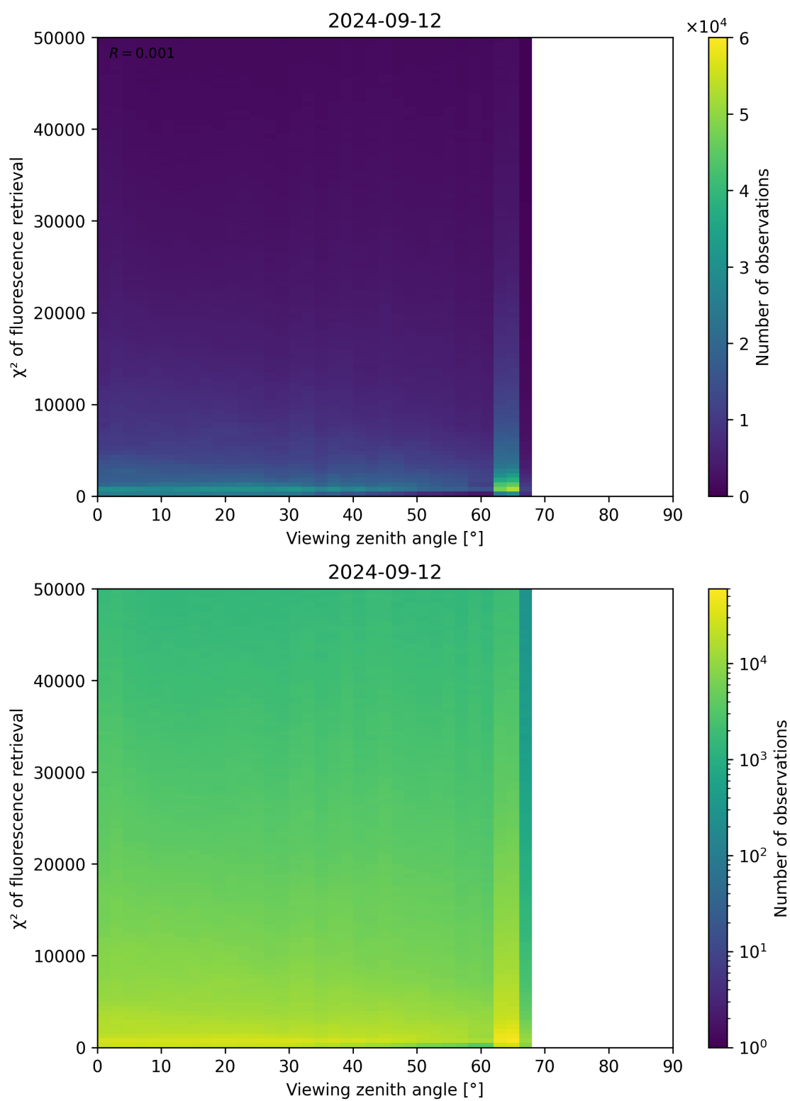
Figure 131: Scatter density plot of “Viewing zenith angle” against “ \chi^2 of fluorescence retrieval” for 2024-09-12 to 2024-09-13.
