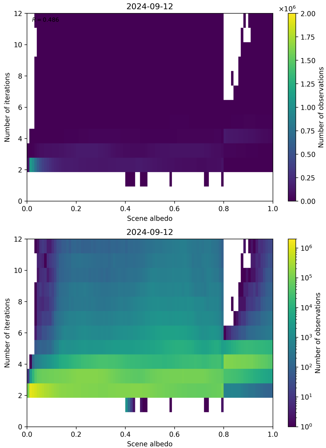
Figure 115: Scatter density plot of “Scene albedo” against “Number of iterations” for 2024-09-12 to 2024-09-13.
