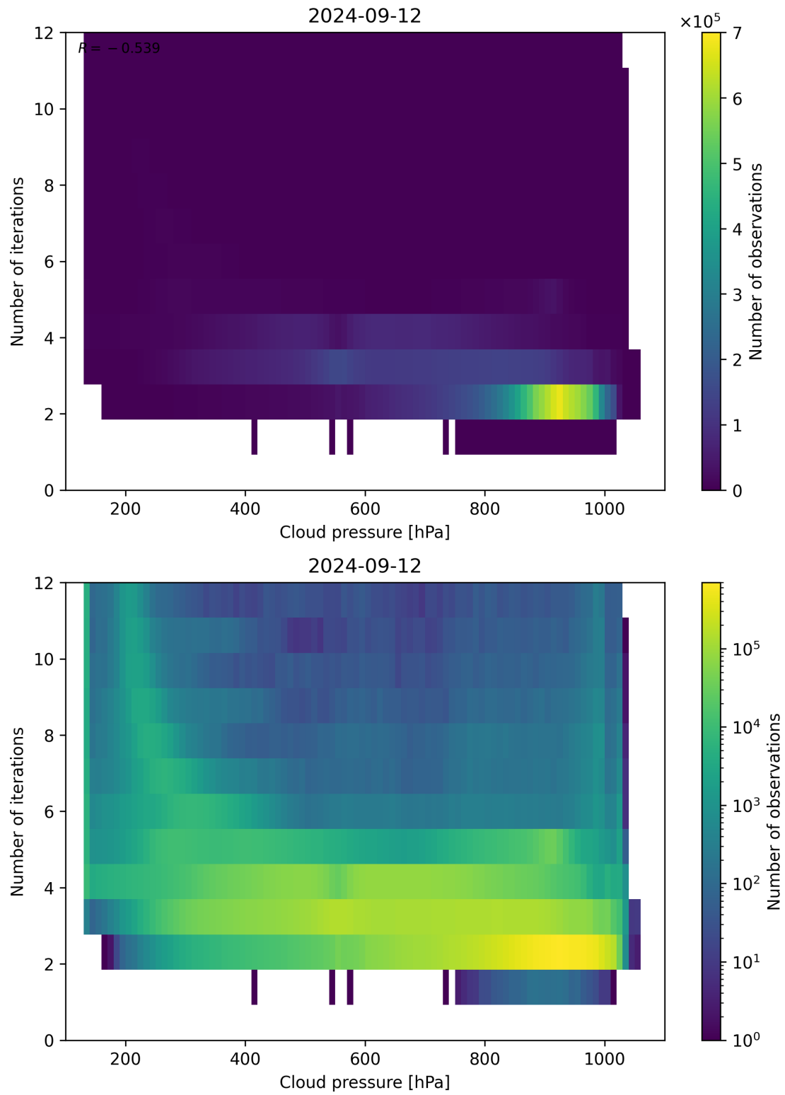
Figure 89: Scatter density plot of “Cloud pressure” against “Number of iterations” for 2024-09-12 to 2024-09-13.
