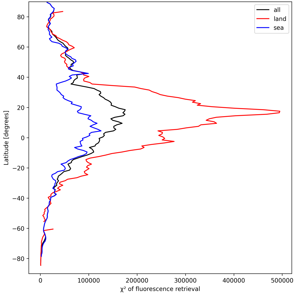
Figure 25: Zonal average of “ \chi^2 of fluorescence retrieval” for 2024-09-12 to 2024-09-13.
