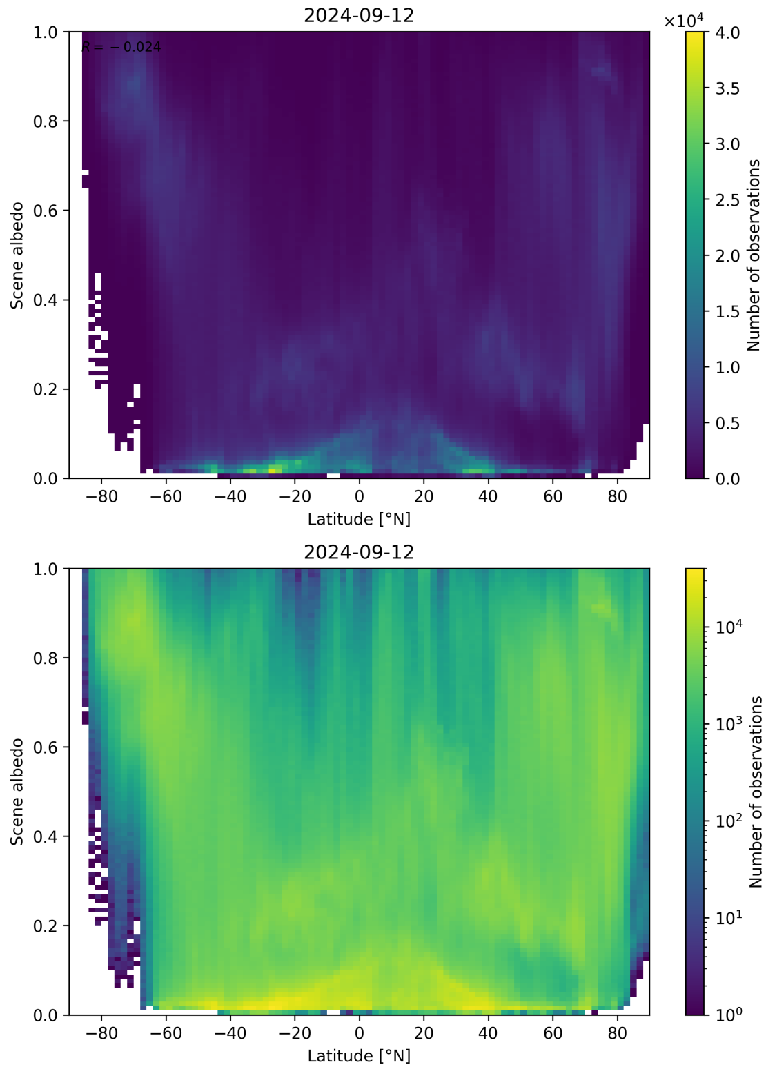
Figure 104: Scatter density plot of “Latitude” against “Scene albedo” for 2024-09-12 to 2024-09-13.
