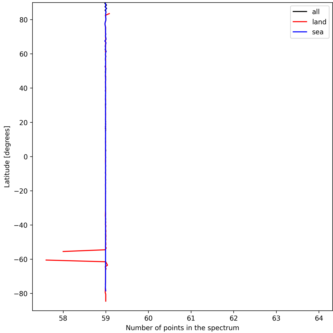
Figure 27: Zonal average of “Number of points in the spectrum” for 2024-09-12 to 2024-09-13.
