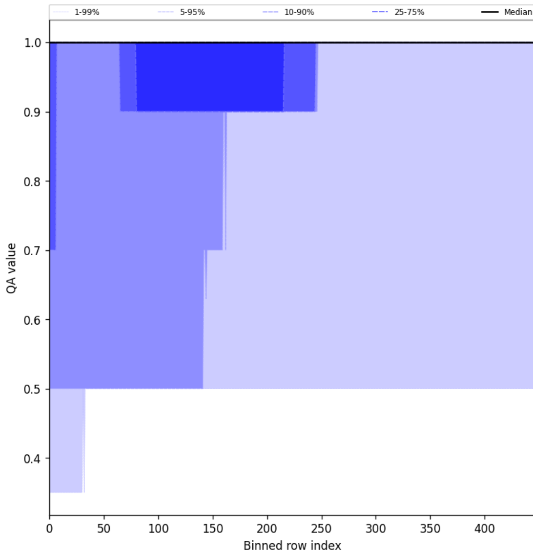
Figure 46: Along track statistics of “QA value” for 2024-09-12 to 2024-09-13
