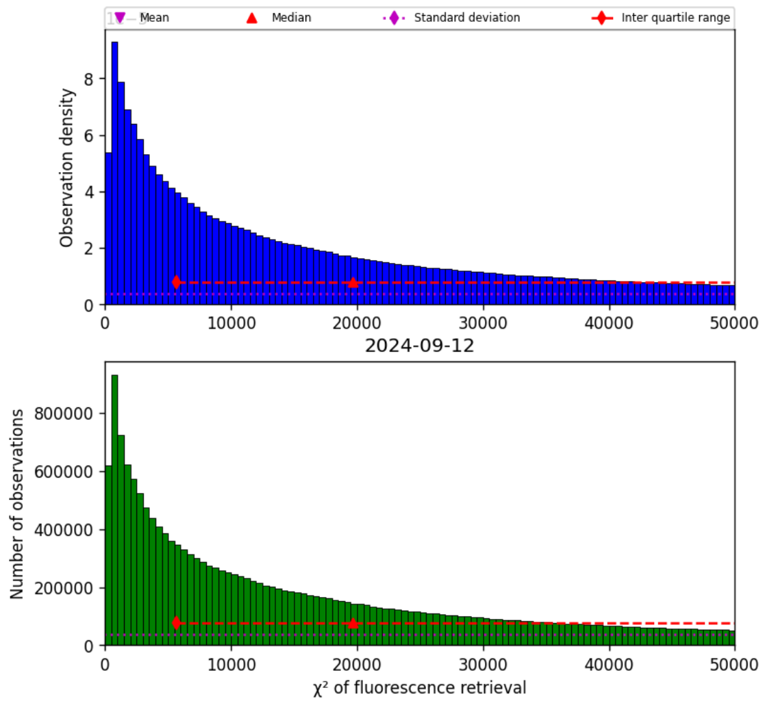
Figure 42: Histogram of “ \chi^2 of fluorescence retrieval” for 2024-09-12 to 2024-09-13
