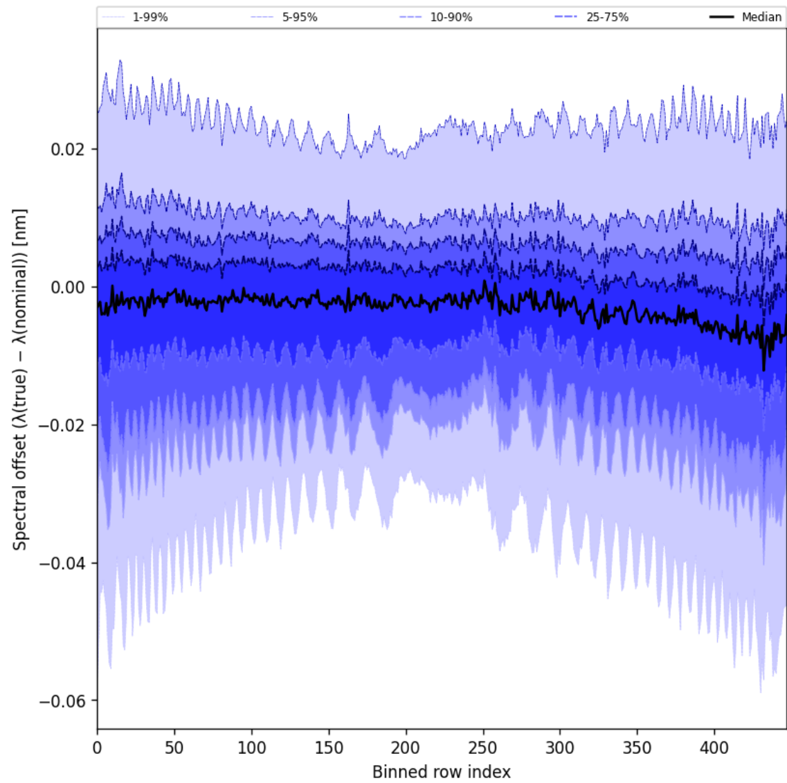
Figure 62: Along track statistics of “Spectral offset ( \lambda_{\text{true}} - \lambda_{\text{nominal}} )” for 2024-09-12 to 2024-09-13
