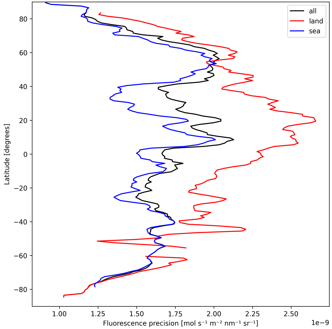
Figure 24: Zonal average of “Fluorescence precision” for 2024-09-12 to 2024-09-13.
