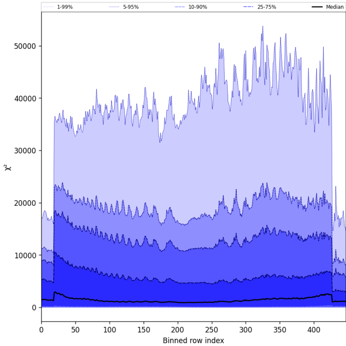
Figure 55: Along track statistics of “ \chi^2 ” for 2024-09-12 to 2024-09-13
