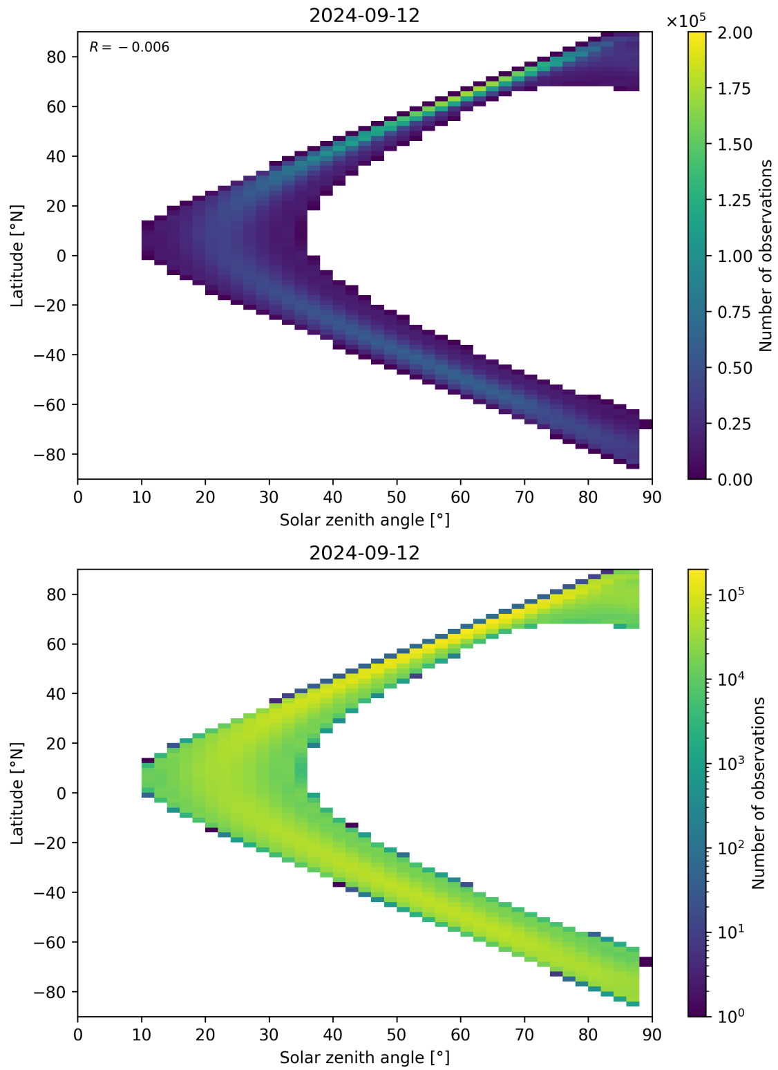
Figure 124: Scatter density plot of “Solar zenith angle” against “Latitude” for 2024-09-12 to 2024-09-13.
