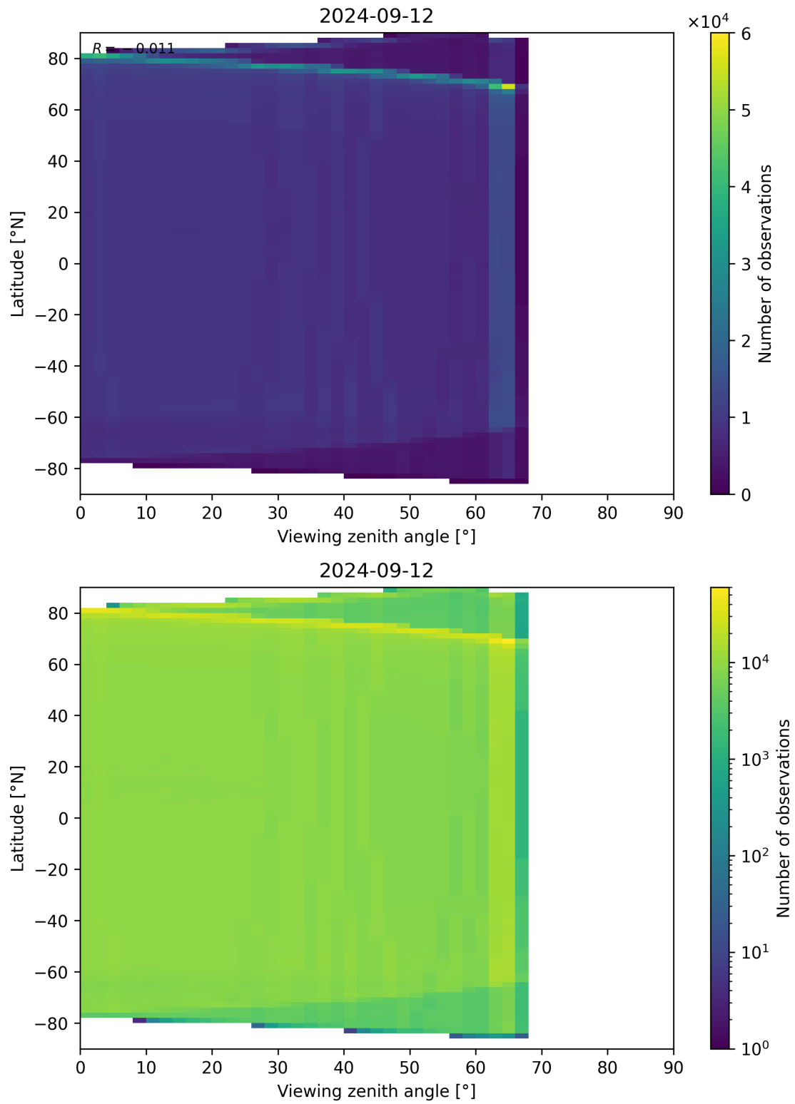
Figure 135: Scatter density plot of “Viewing zenith angle” against “Latitude” for 2024-09-12 to 2024-09-13.
