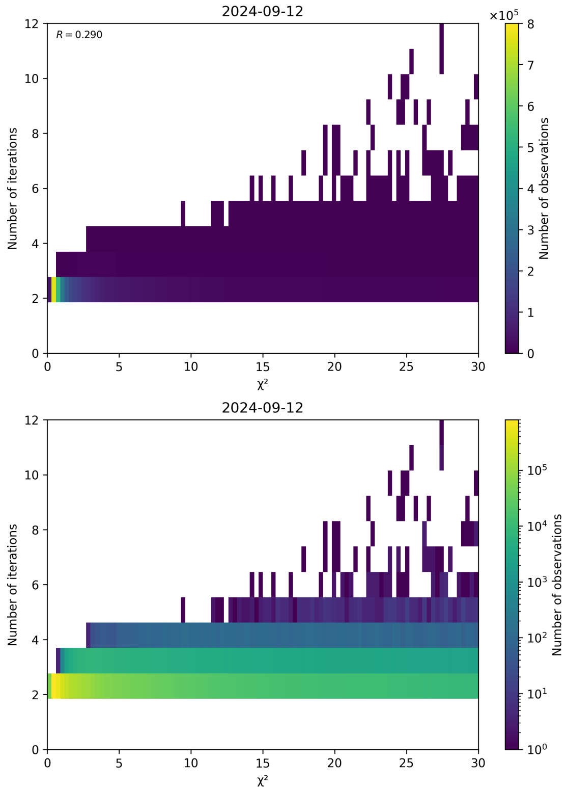
Figure 73: Scatter density plot of " \chi^2 " against "Number of iterations" for 2024-09-12 to 2024-09-13.
