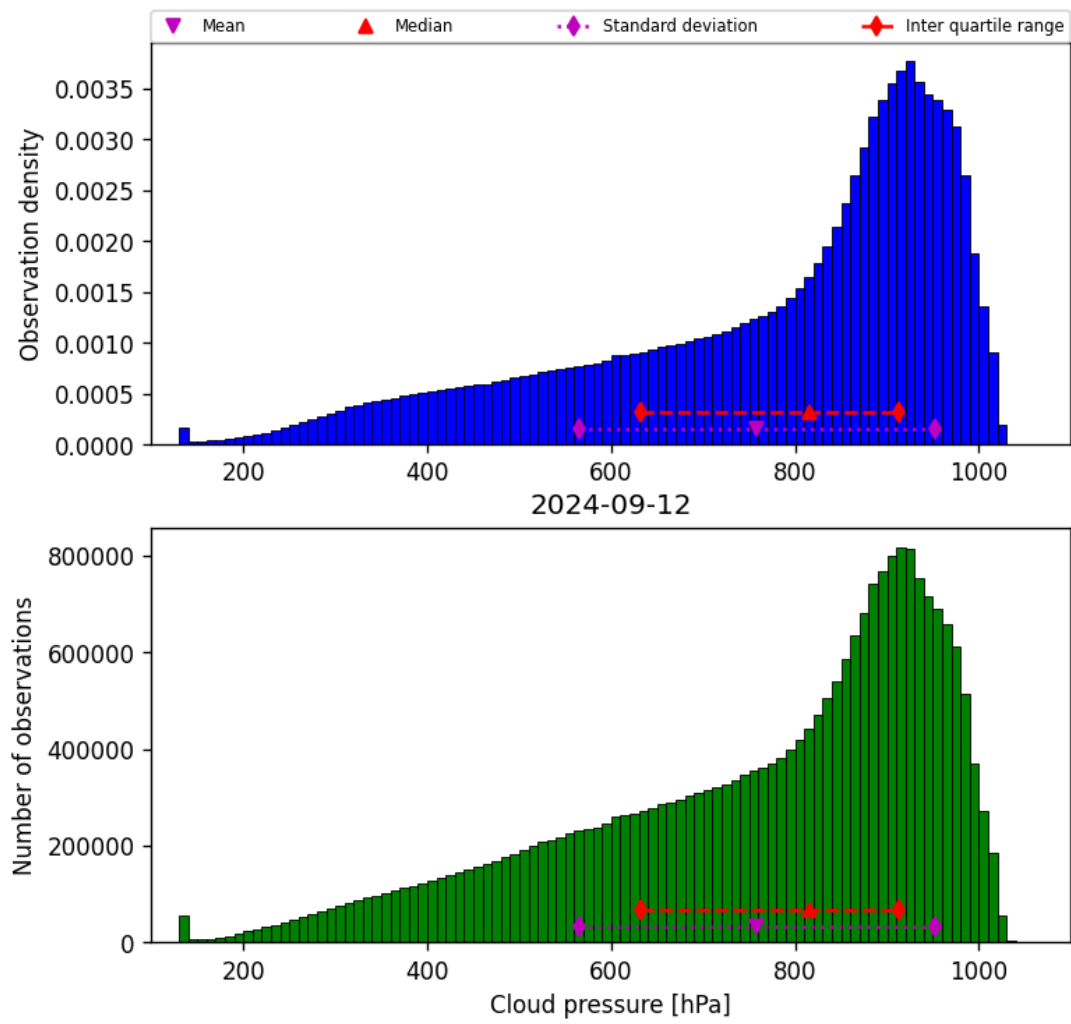
Figure 30: Histogram of “Cloud pressure” for 2024-09-12 to 2024-09-13
