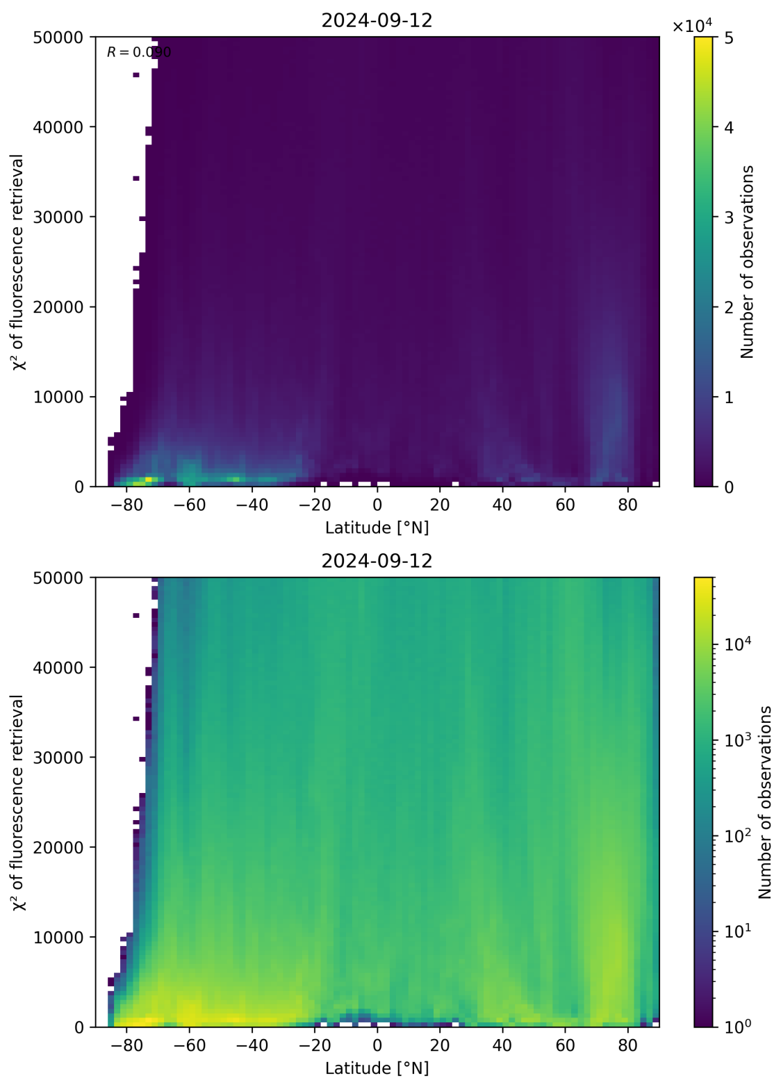
Figure 98: Scatter density plot of “Latitude” against “ \chi^2 of fluorescence retrieval” for 2024-09-12 to 2024-09-13.
