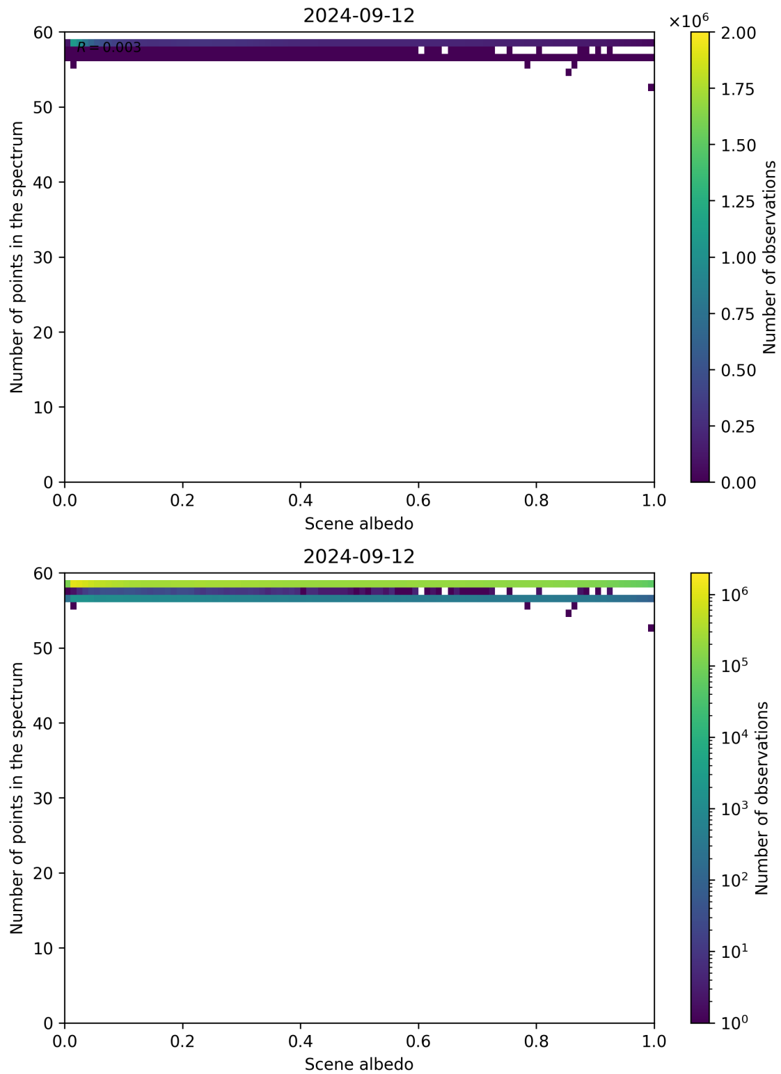
Figure 116: Scatter density plot of “Scene albedo” against “Number of points in the spectrum” for 2024-09-12 to 2024-09-13.
