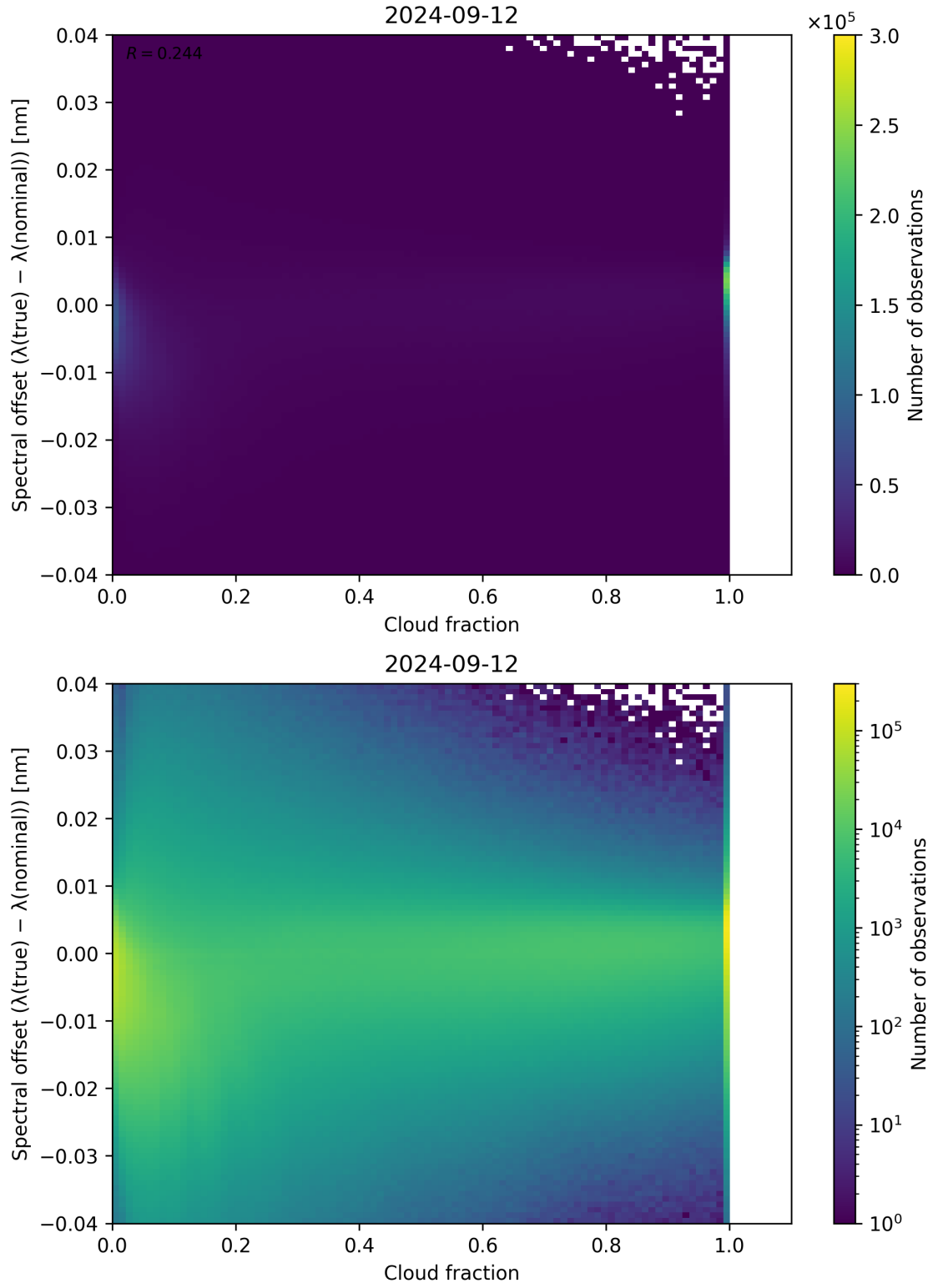
Figure 83: Scatter density plot of “Cloud fraction” against “Spectral offset ( \lambda_{\text{true}} - \lambda_{\text{nominal}} )” for 2024-09-12 to 2024-09-13.
