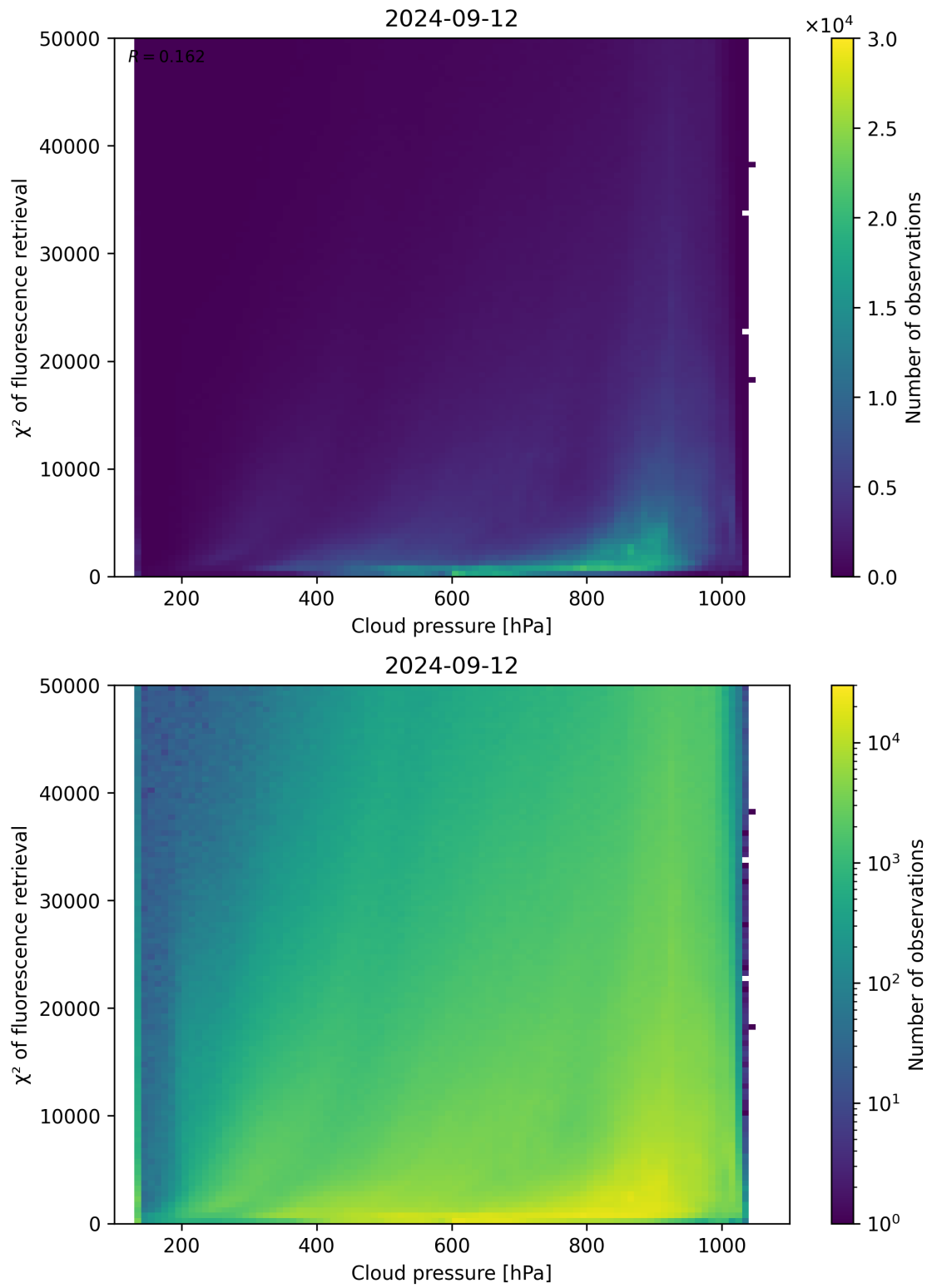
Figure 86: Scatter density plot of “Cloud pressure” against “ \chi^2 of fluorescence retrieval” for 2024-09-12 to 2024-09-13.
