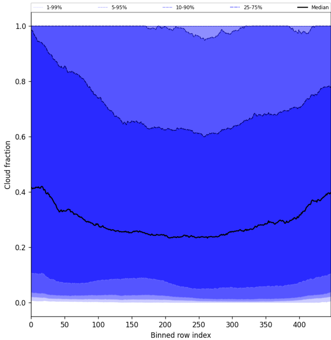
Figure 49: Along track statistics of “Cloud fraction” for 2024-09-12 to 2024-09-13
