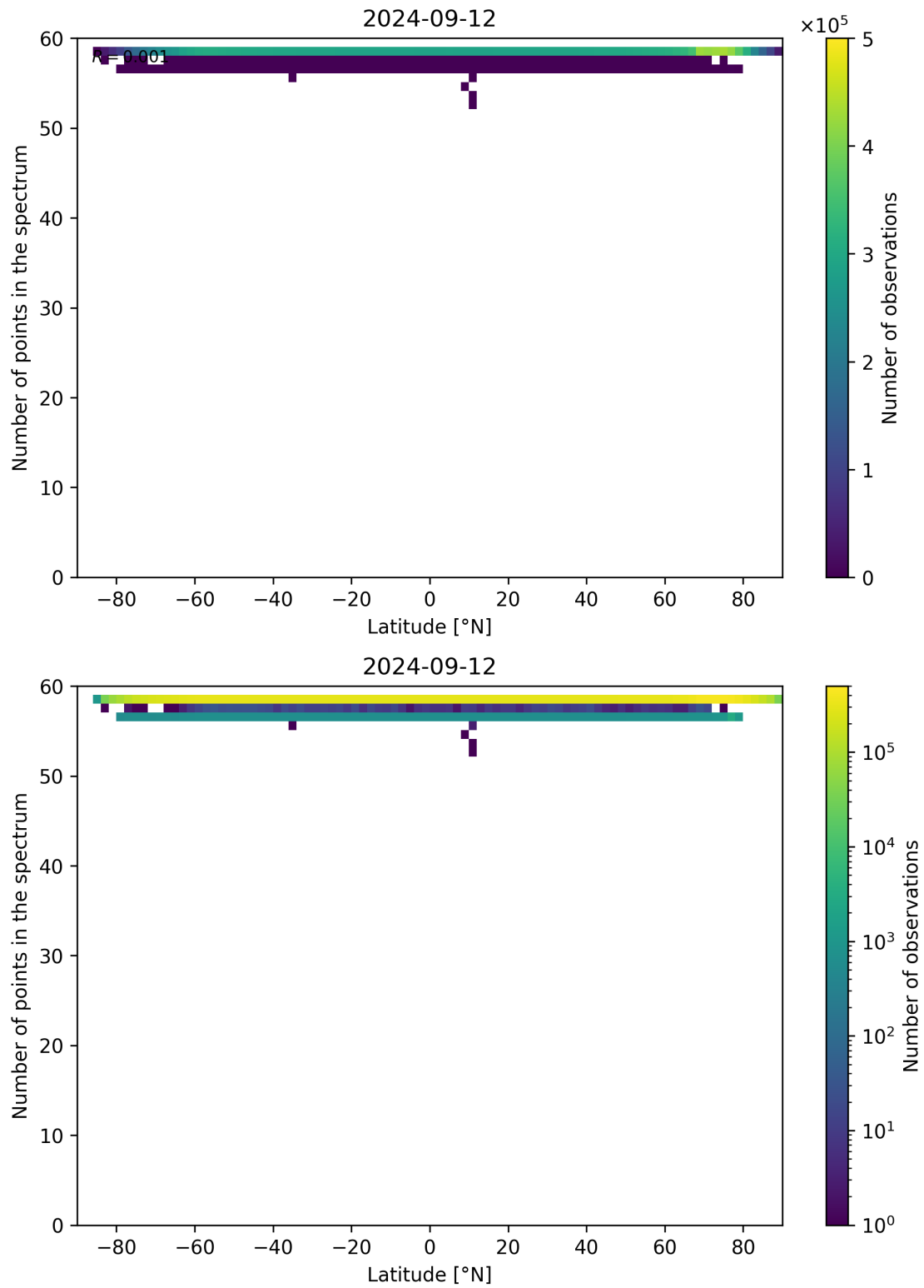
Figure 103: Scatter density plot of “Latitude” against “Number of points in the spectrum” for 2024-09-12 to 2024-09-13.
