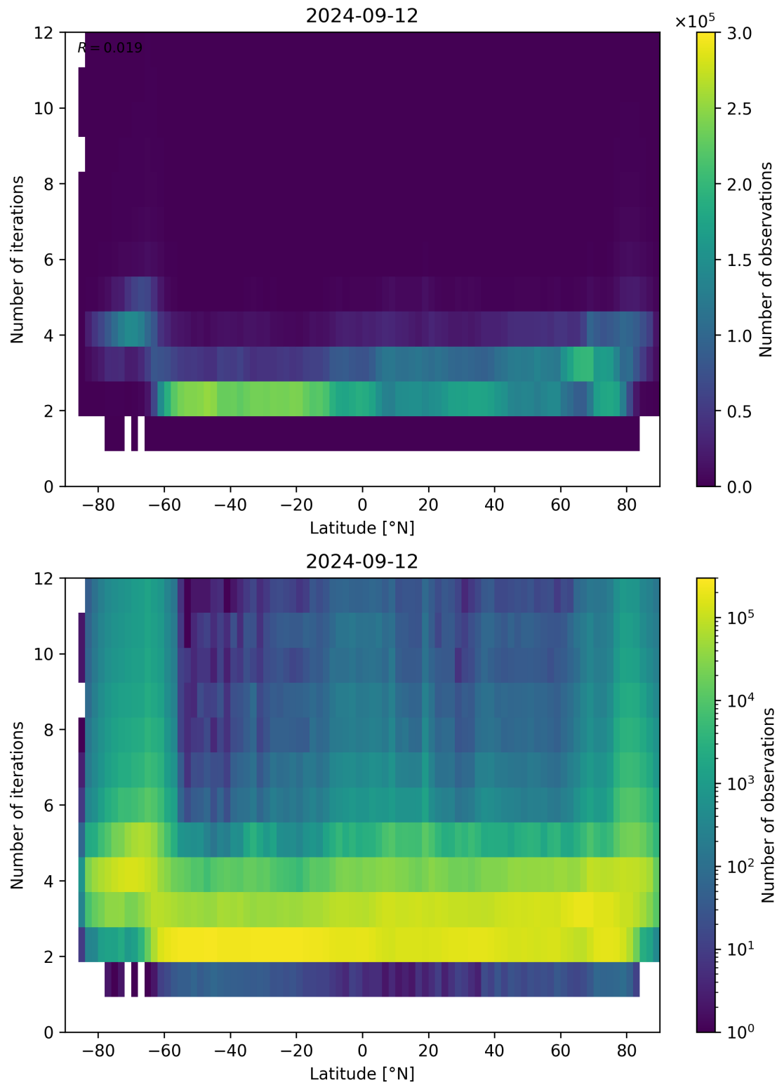
Figure 102: Scatter density plot of “Latitude” against “Number of iterations” for 2024-09-12 to 2024-09-13.
