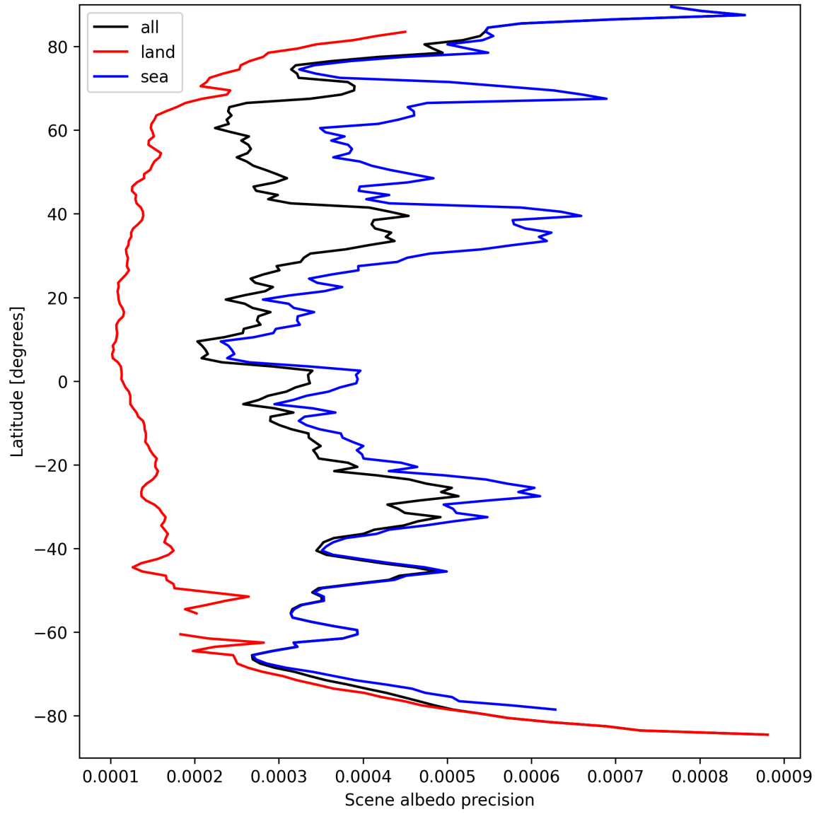
Figure 18: Zonal average of “Scene albedo precision” for 2024-09-12 to 2024-09-13.
