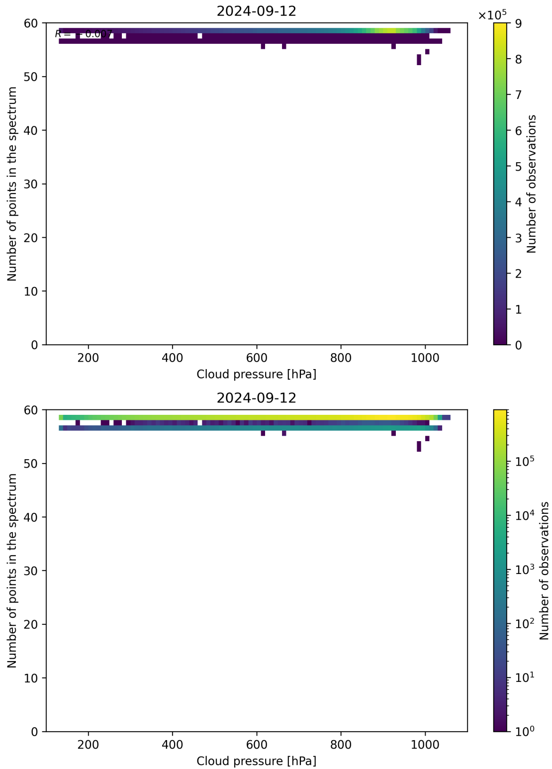
Figure 90: Scatter density plot of “Cloud pressure” against “Number of points in the spectrum” for 2024-09-12 to 2024-09-13.
