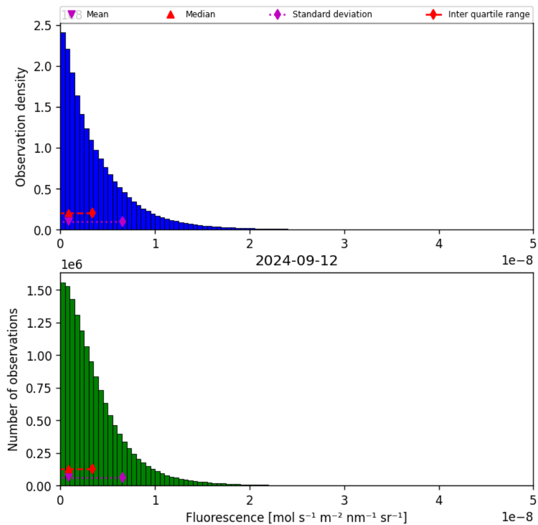
Figure 40: Histogram of “Fluorescence” for 2024-09-12 to 2024-09-13
