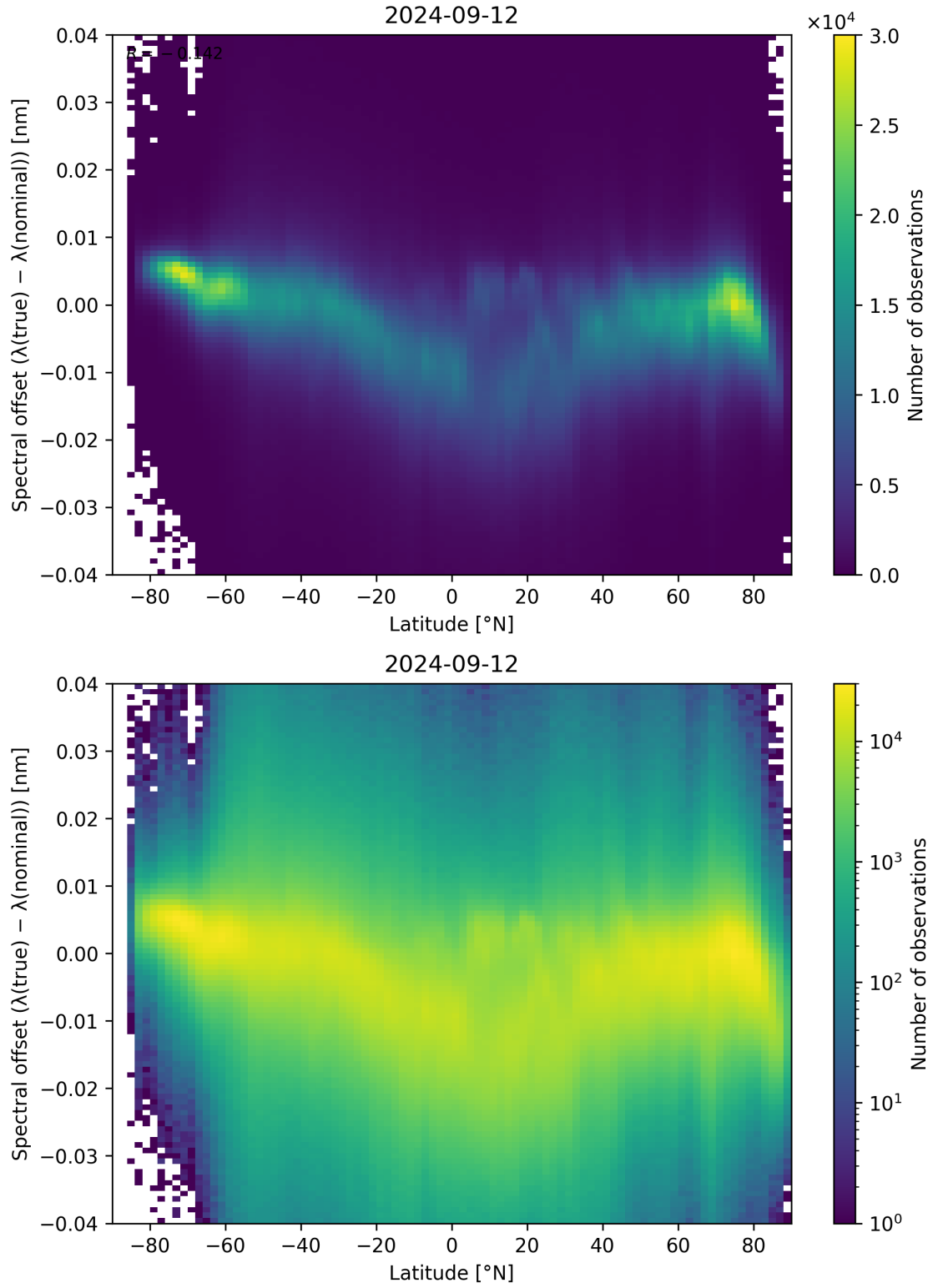
Figure 105: Scatter density plot of “Latitude” against “Spectral offset ( \lambda_{\text{true}} - \lambda_{\text{nominal}} )” for 2024-09-12 to 2024-09-13.
