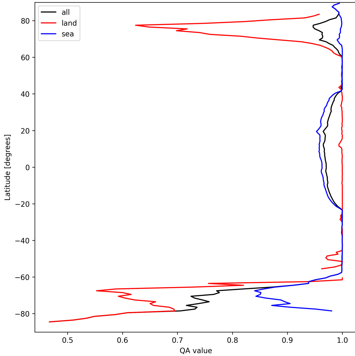
Figure 12: Zonal average of “QA value” for 2024-09-12 to 2024-09-13.
