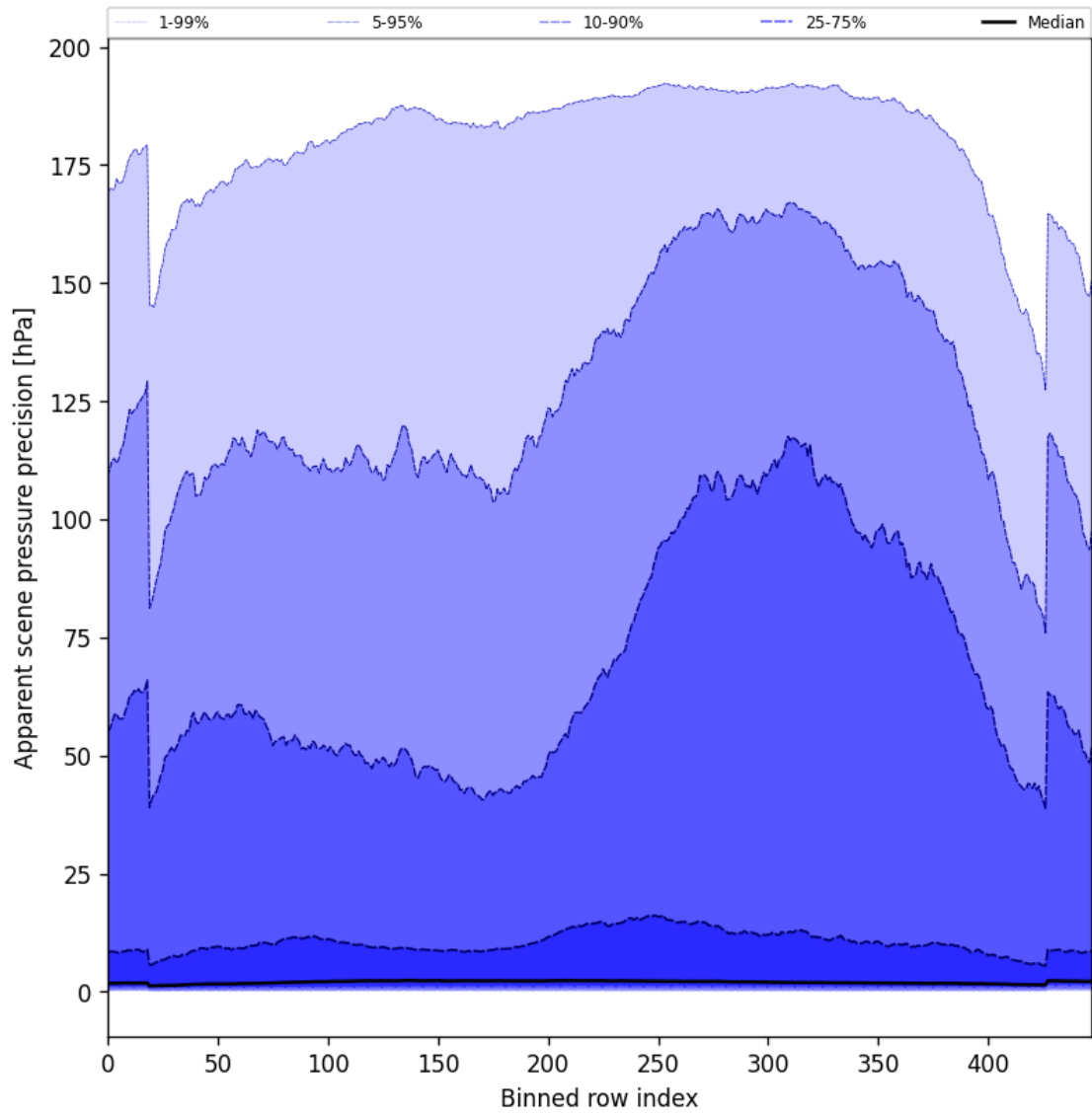
Figure 54: Along track statistics of “Apparent scene pressure precision” for 2024-09-12 to 2024-09-13
