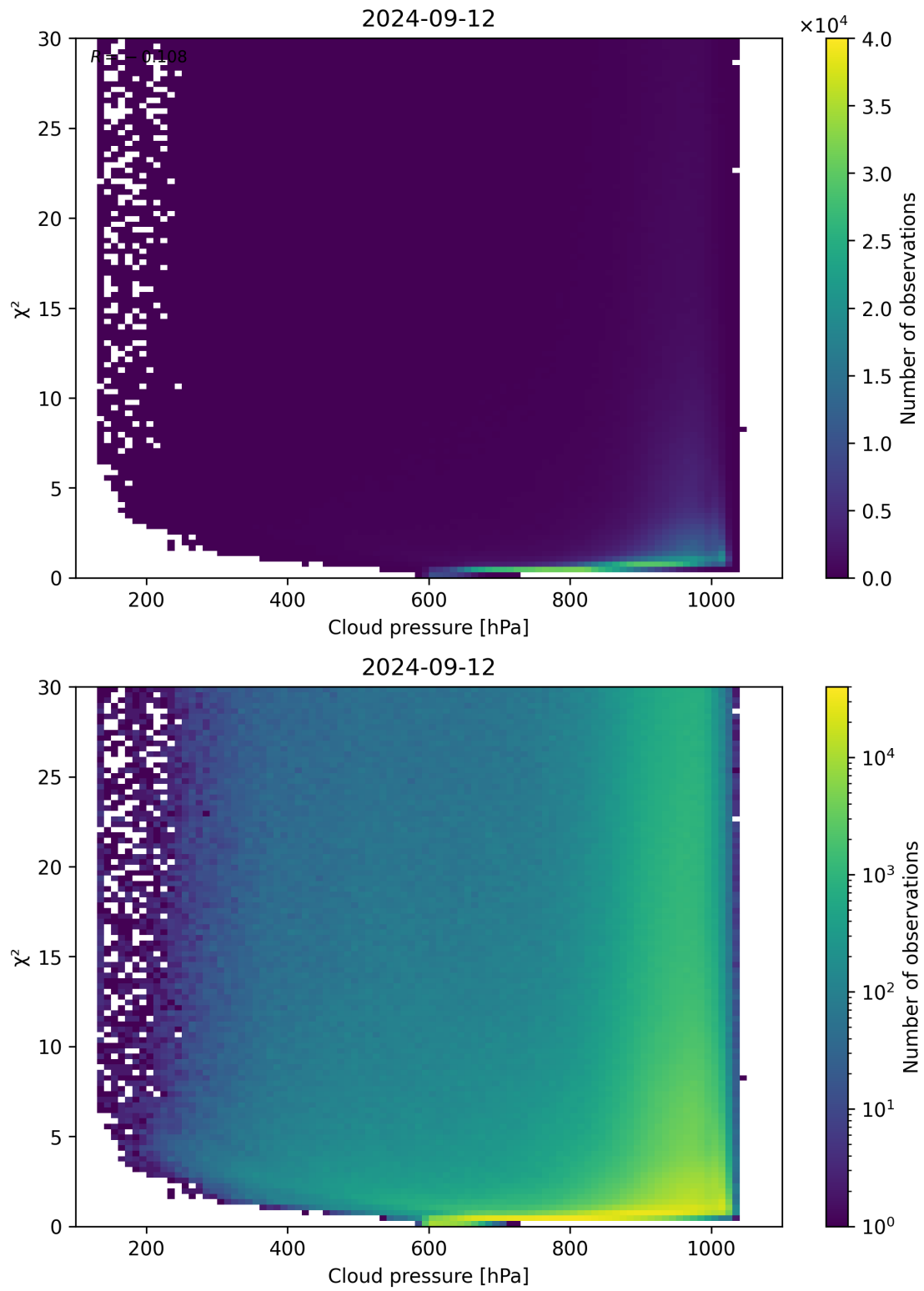
Figure 85: Scatter density plot of “Cloud pressure” against “ \chi^2 ” for 2024-09-12 to 2024-09-13.
