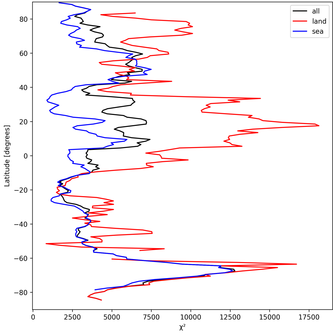
Figure 21: Zonal average of “ \chi^2 ” for 2024-09-12 to 2024-09-13.
