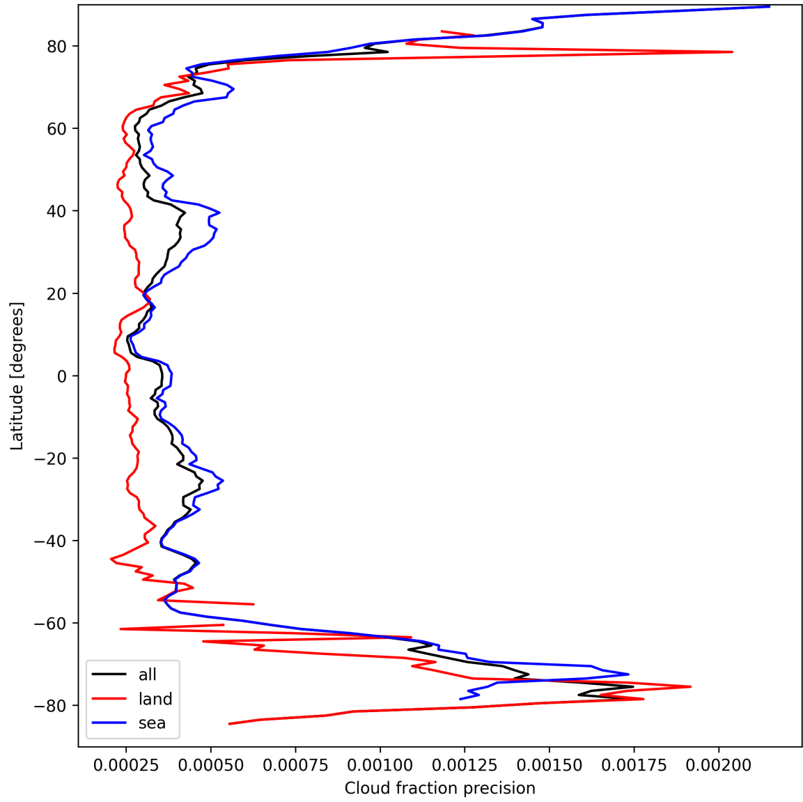
Figure 16: Zonal average of “Cloud fraction precision” for 2024-09-12 to 2024-09-13.
