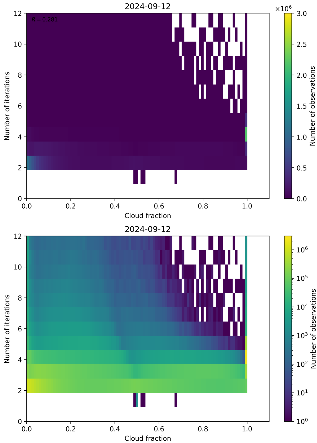
Figure 80: Scatter density plot of “Cloud fraction” against “Number of iterations” for 2024-09-12 to 2024-09-13.
