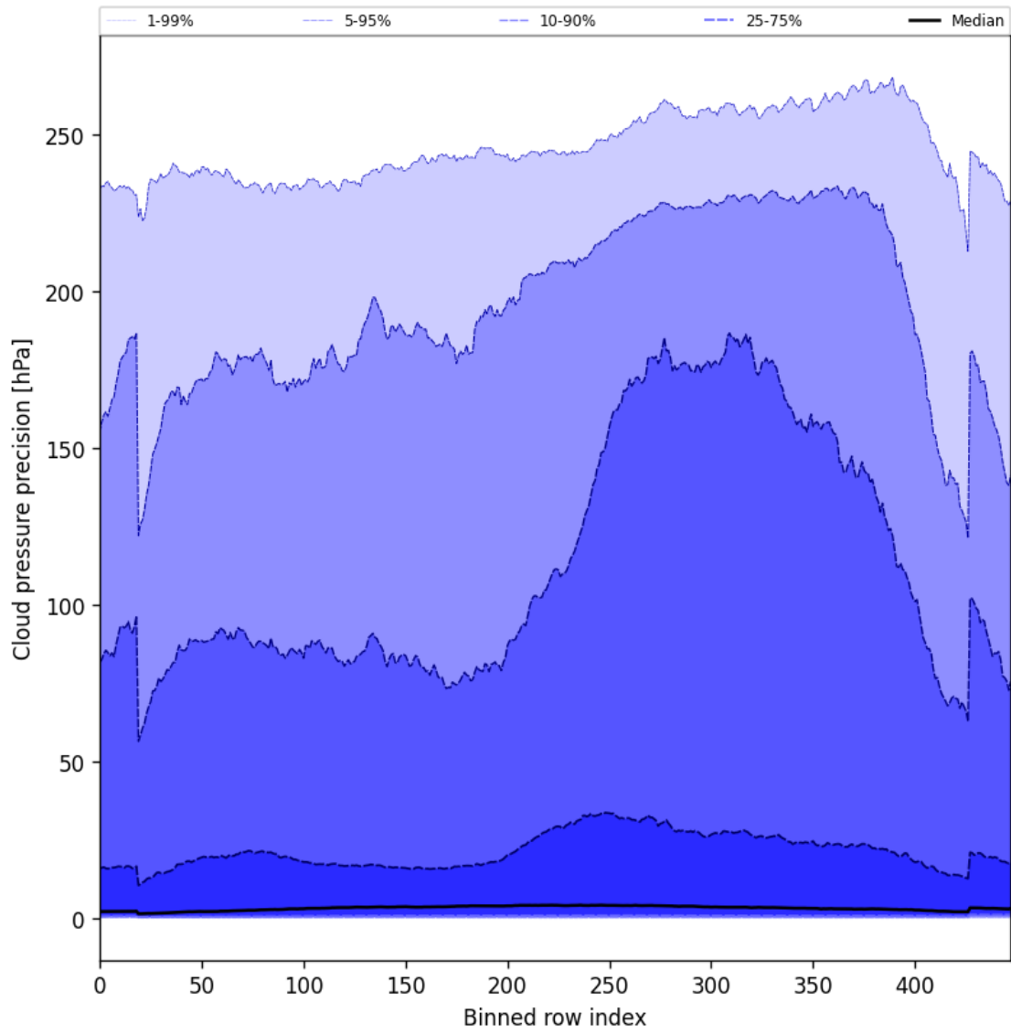
Figure 48: Along track statistics of “Cloud pressure precision” for 2024-09-12 to 2024-09-13
