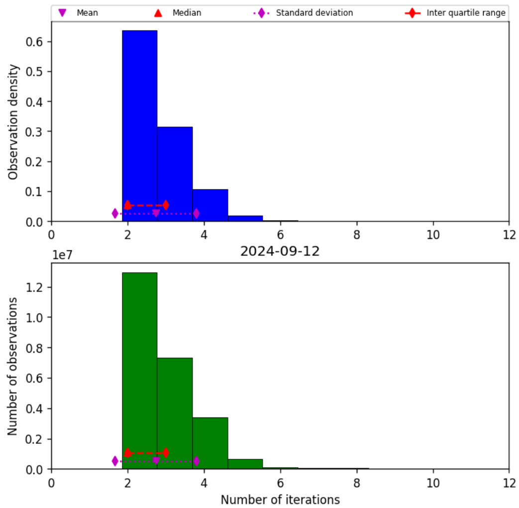
Figure 39: Histogram of “Number of iterations” for 2024-09-12 to 2024-09-13
