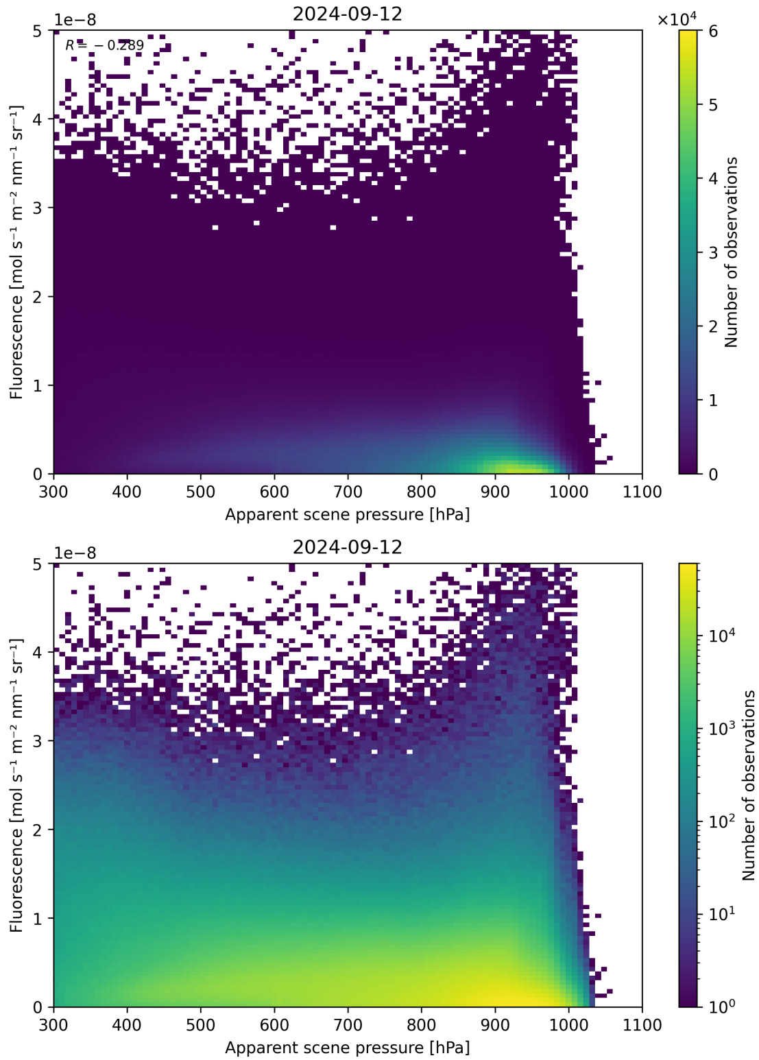
Figure 65: Scatter density plot of “Apparent scene pressure” against “Fluorescence” for 2024-09-12 to 2024-09-13.
