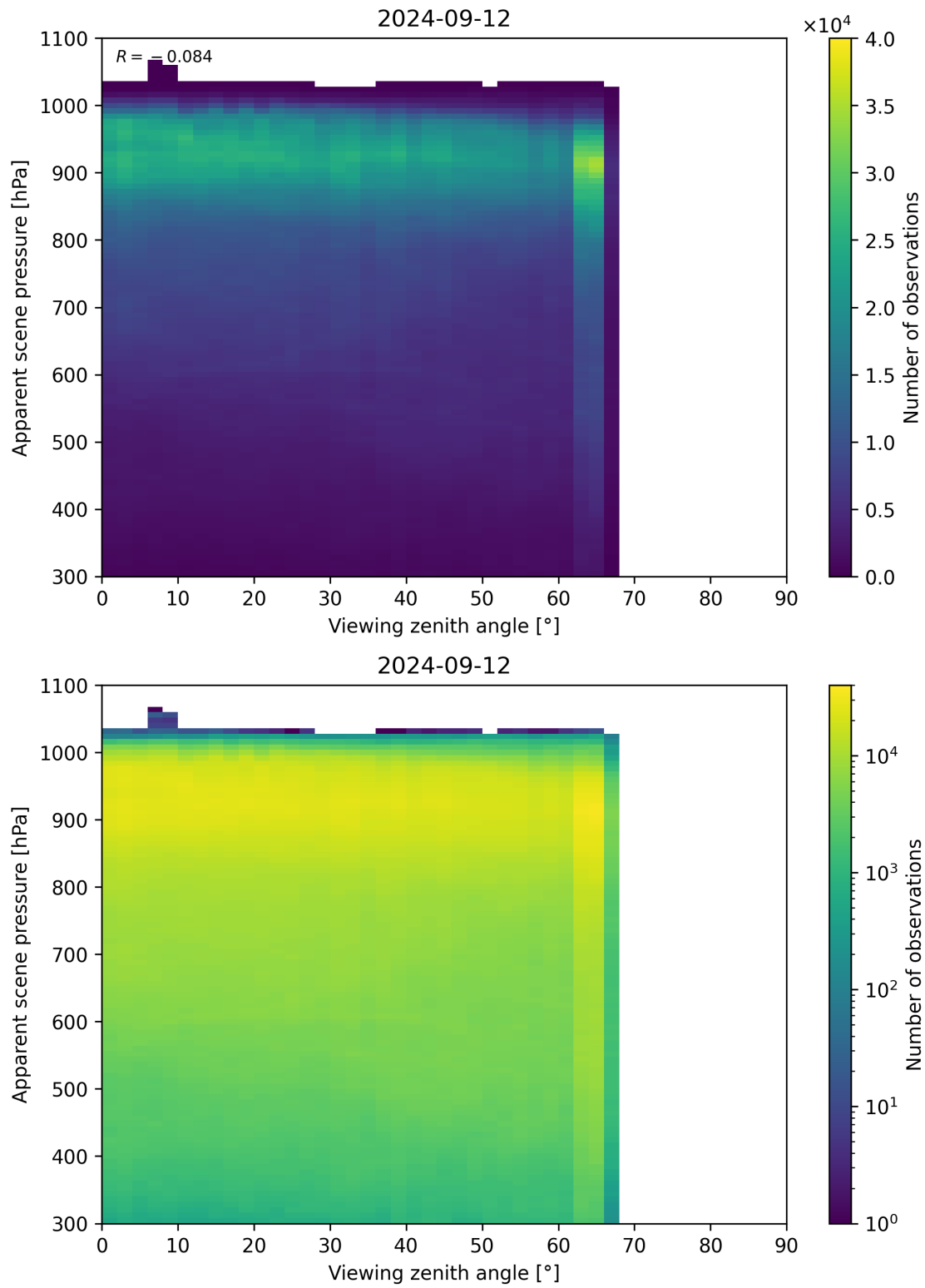
Figure 129: Scatter density plot of “Viewing zenith angle” against “Apparent scene pressure” for 2024-09-12 to 2024-09-13.
