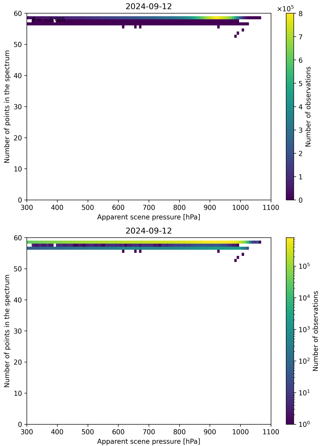
Figure 67: Scatter density plot of “Apparent scene pressure” against “Number of points in the spectrum” for 2024-09-12 to 2024-09-13.
