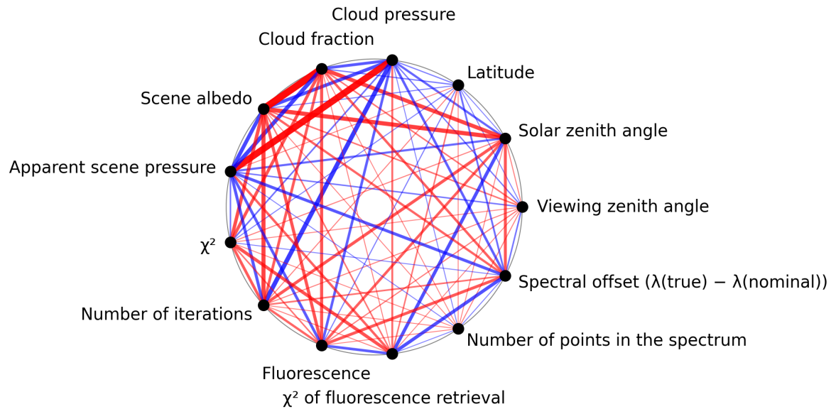
Figure 1: Map of correlation graph for 2024-09-12 to 2024-09-13.
