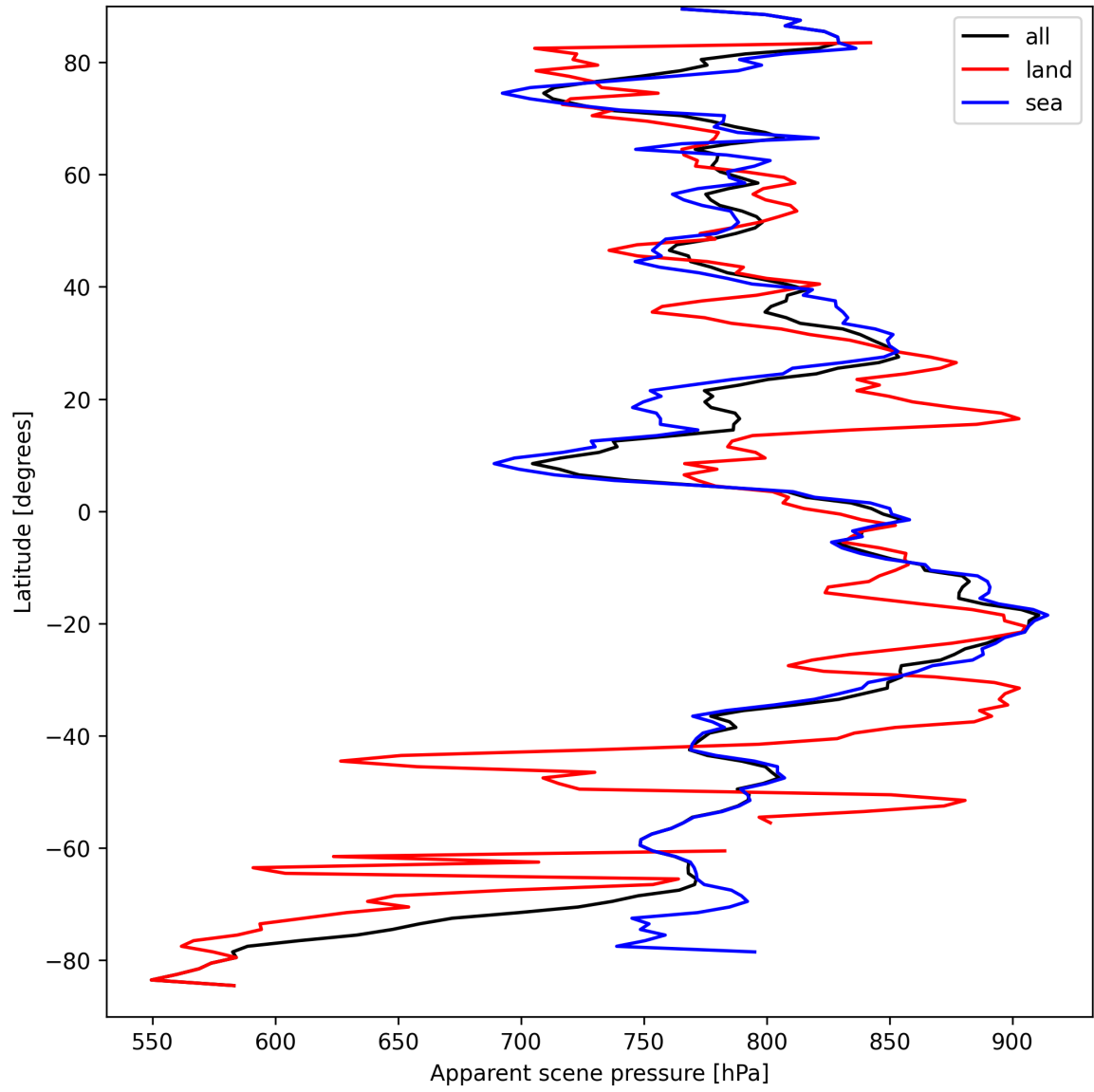
Figure 19: Zonal average of “Apparent scene pressure” for 2024-09-12 to 2024-09-13.
