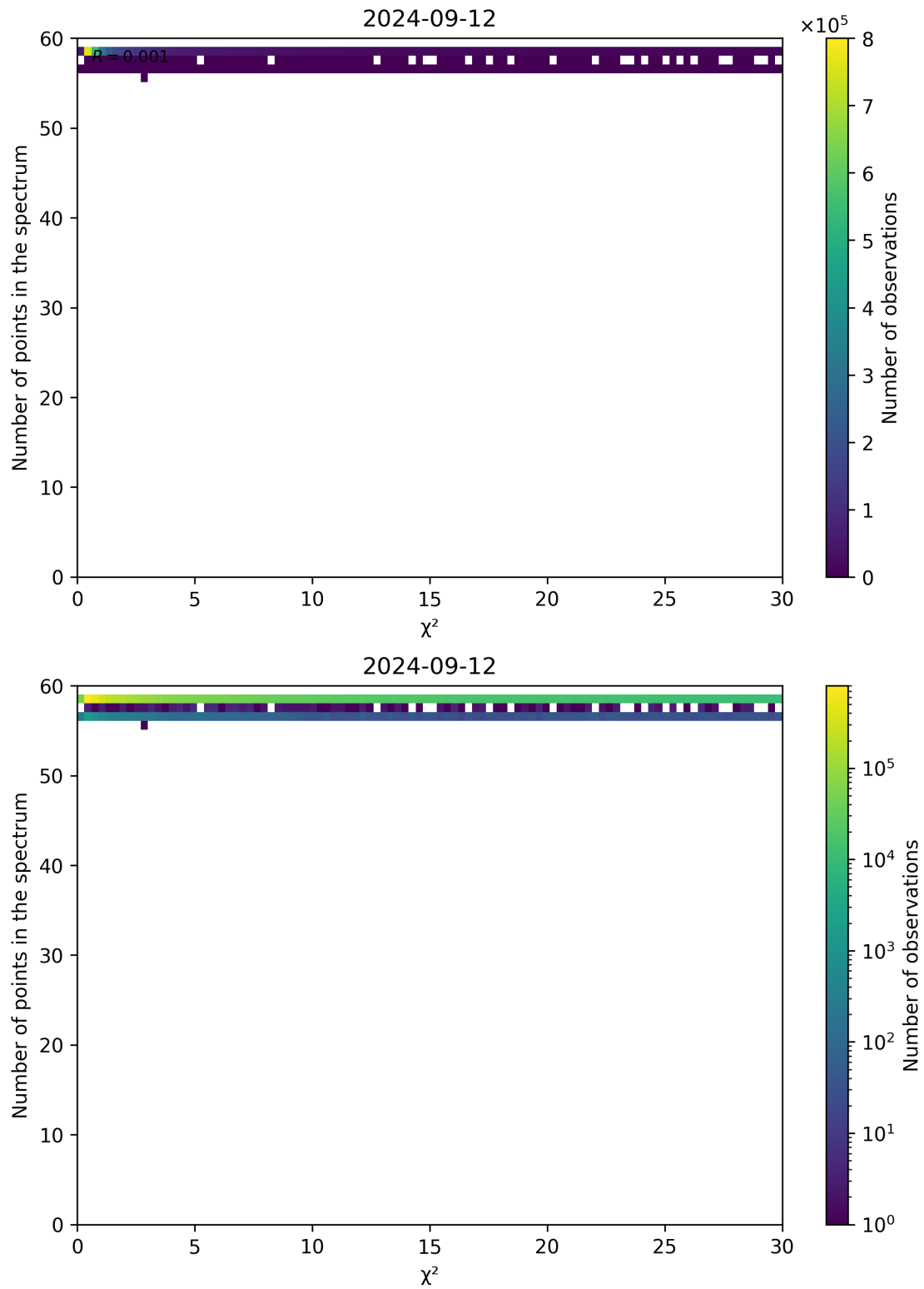
Figure 74: Scatter density plot of " \chi^2 " against "Number of points in the spectrum" for 2024-09-12 to 2024-09-13.
