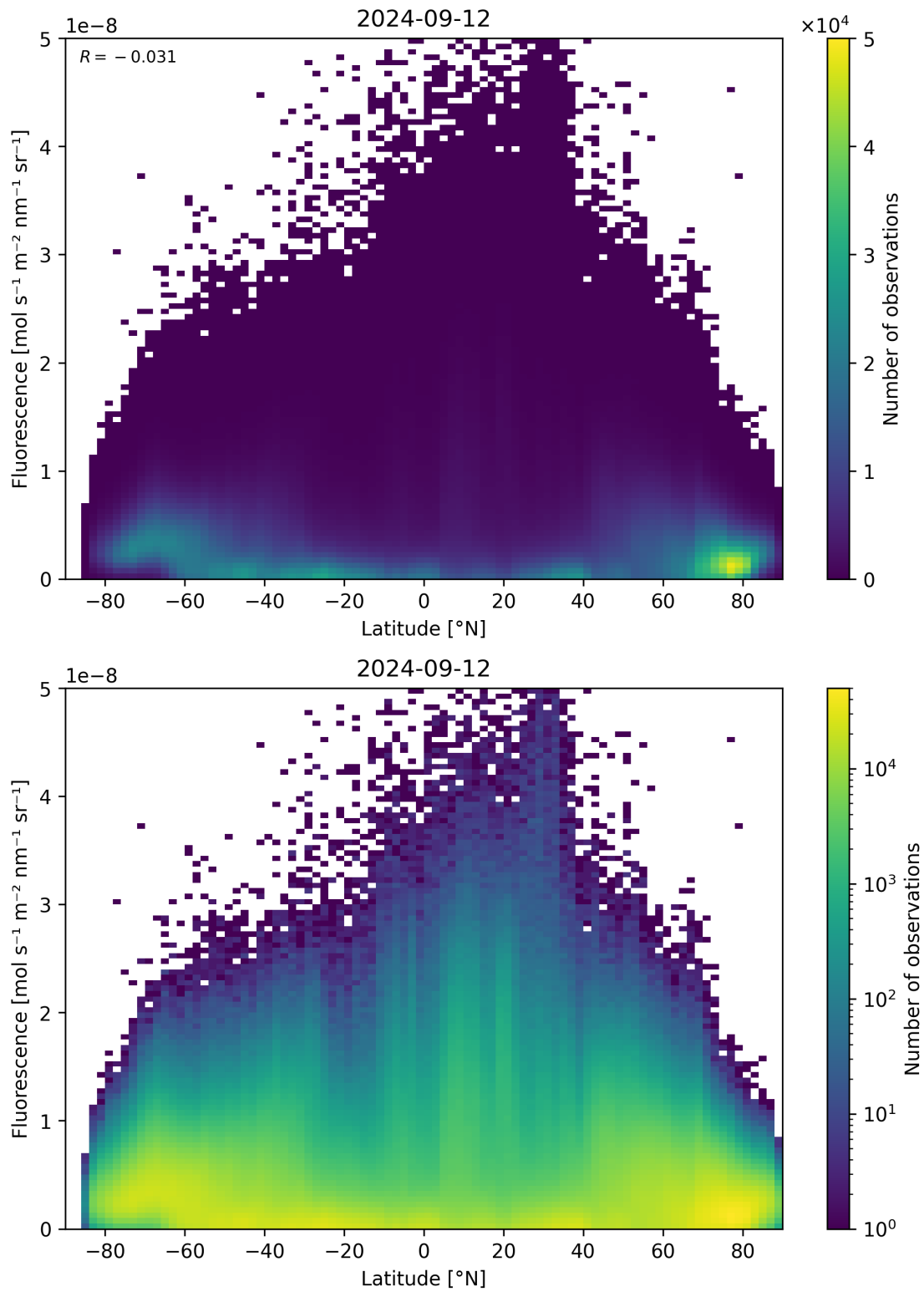
Figure 101: Scatter density plot of “Latitude” against “Fluorescence” for 2024-09-12 to 2024-09-13.
