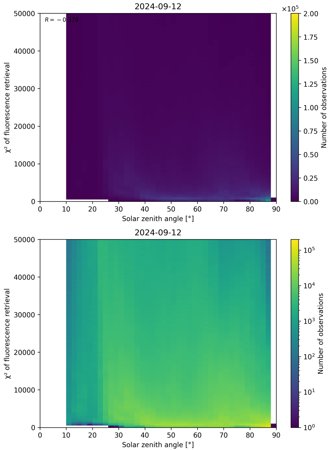
Figure 120: Scatter density plot of “Solar zenith angle” against “ \chi^2 of fluorescence retrieval” for 2024-09-12 to 2024-09-13.
