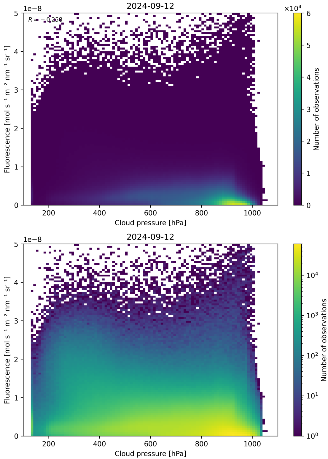
Figure 88: Scatter density plot of “Cloud pressure” against “Fluorescence” for 2024-09-12 to 2024-09-13.
