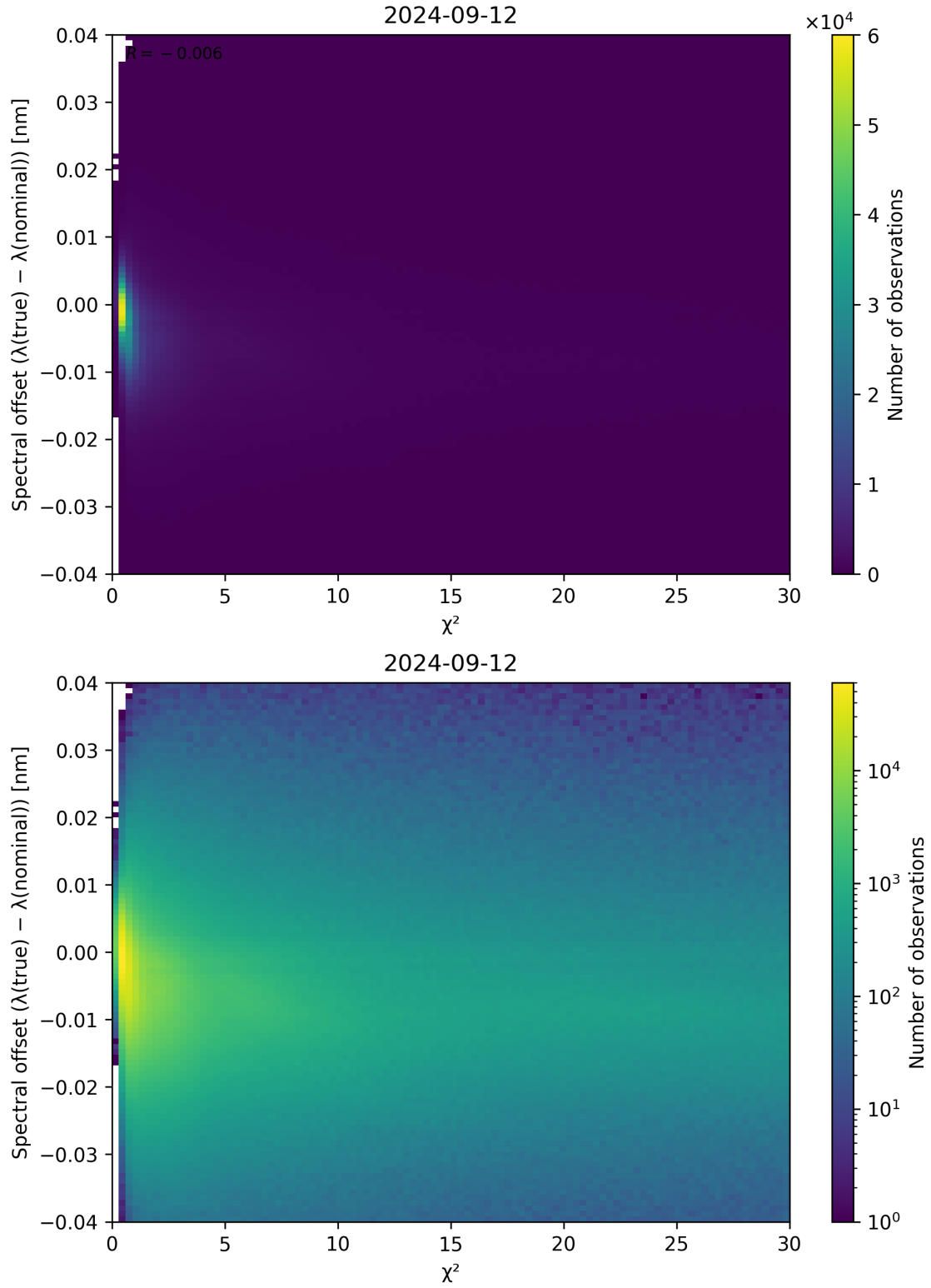
Figure 75: Scatter density plot of “ \chi^2 ” against “Spectral offset ( \lambda_{\text{true}} - \lambda_{\text{nominal}} )” for 2024-09-12 to 2024-09-13.
