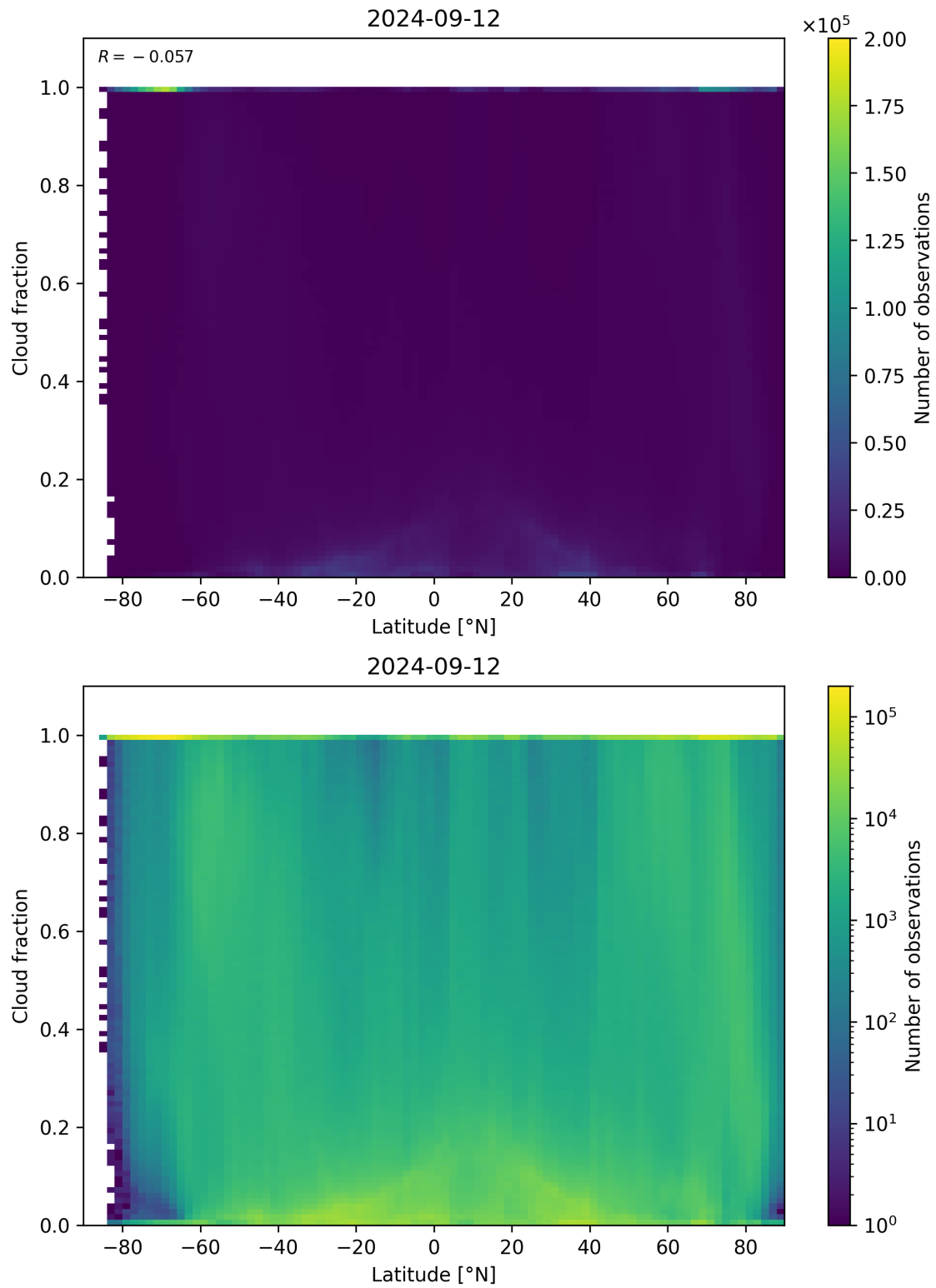
Figure 99: Scatter density plot of “Latitude” against “Cloud fraction” for 2024-09-12 to 2024-09-13.
