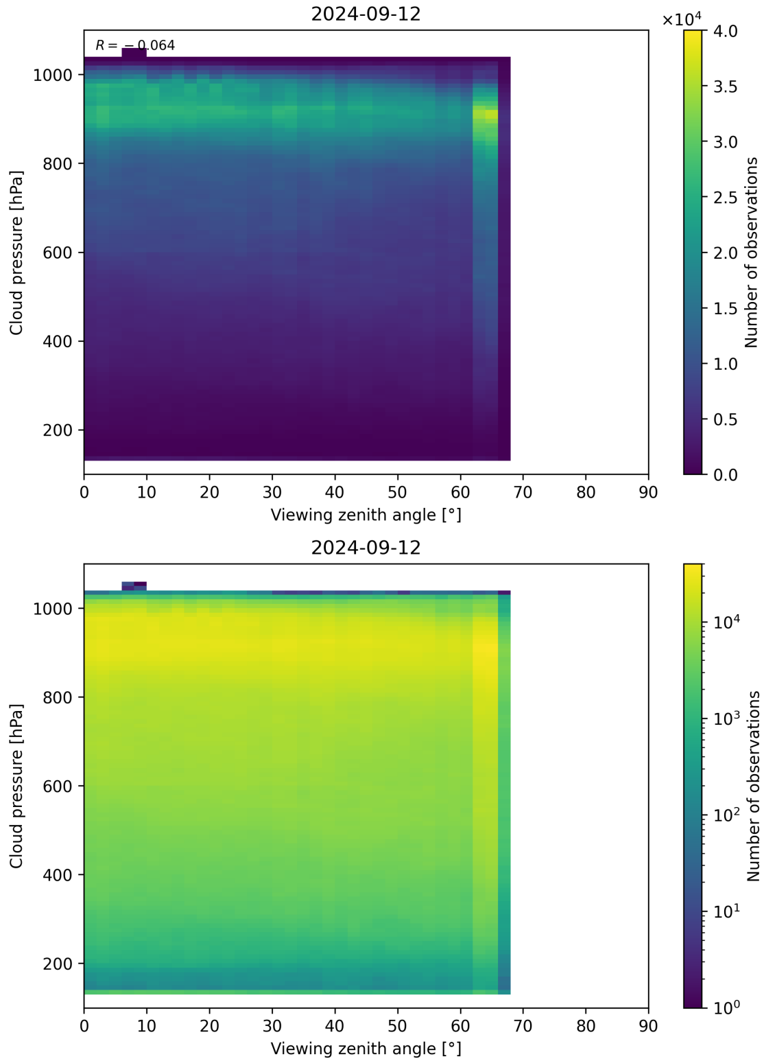
Figure 133: Scatter density plot of “Viewing zenith angle” against “Cloud pressure” for 2024-09-12 to 2024-09-13.
