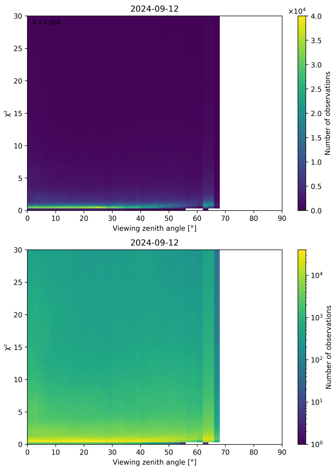
Figure 130: Scatter density plot of “Viewing zenith angle” against “ \chi^2 ” for 2024-09-12 to 2024-09-13.
