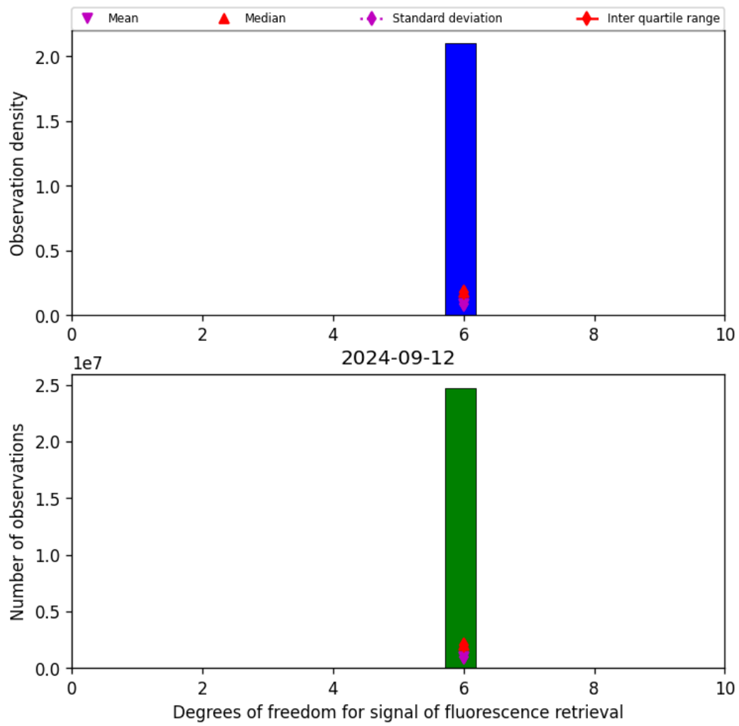
Figure 43: Histogram of “Degrees of freedom for signal of fluorescence retrieval” for 2024-09-12 to 2024-09-13
