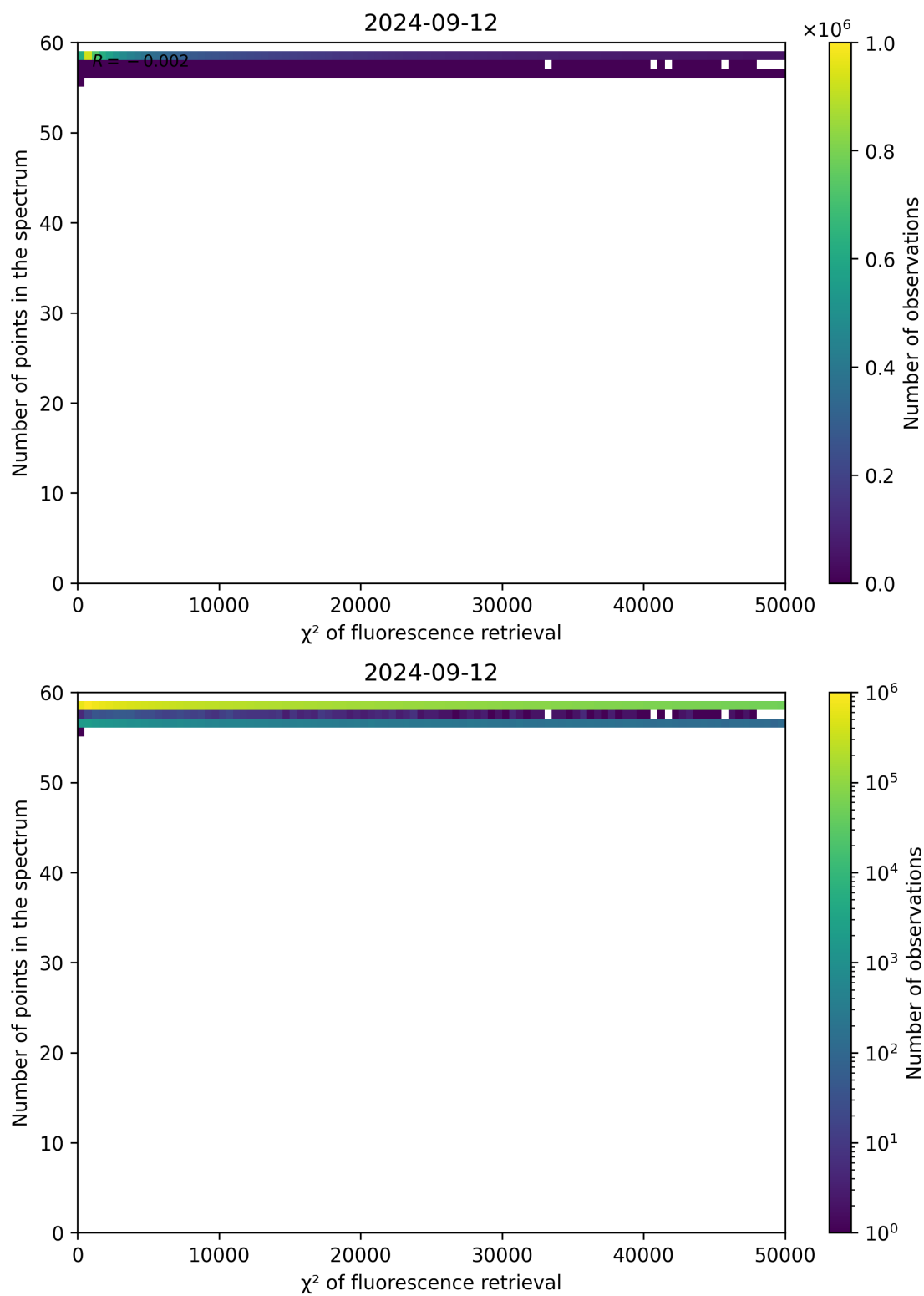
Figure 71: Scatter density plot of " \chi^2 of fluorescence retrieval" against "Number of points in the spectrum" for 2024-09-12 to 2024-09-13.
