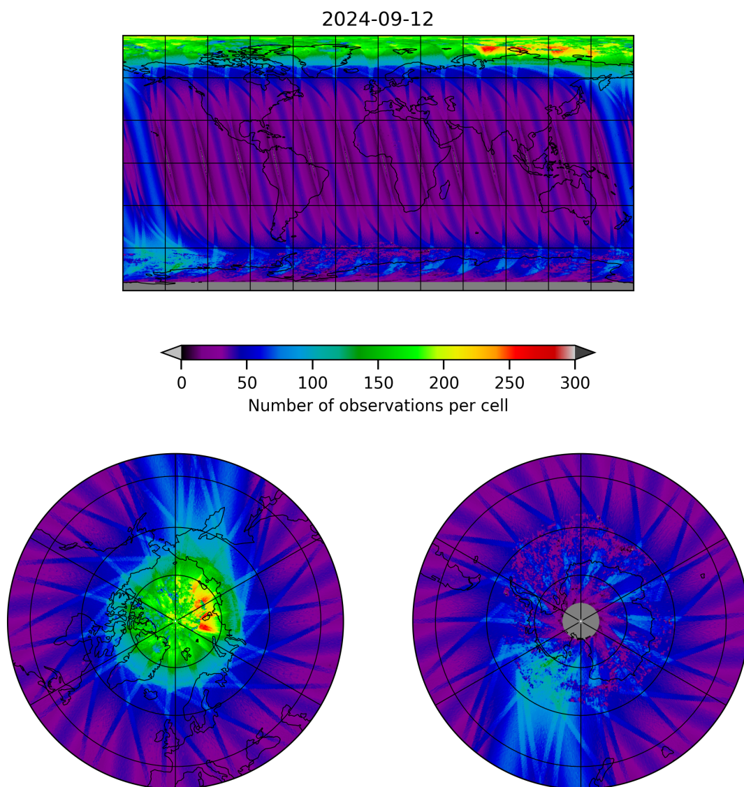
Figure 11: Map of the number of observations for 2024-09-12 to 2024-09-13
