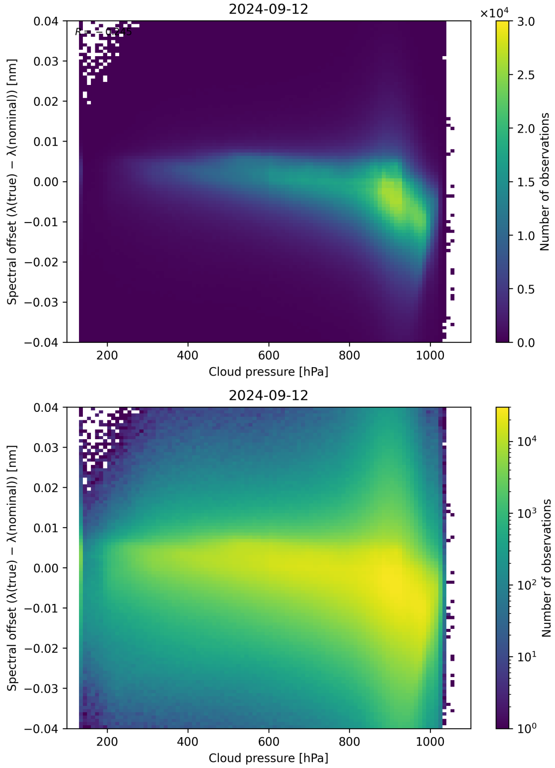
Figure 92: Scatter density plot of “Cloud pressure” against “Spectral offset ( \lambda_{\text{true}} - \lambda_{\text{nominal}} )” for 2024-09-12 to 2024-09-13.
