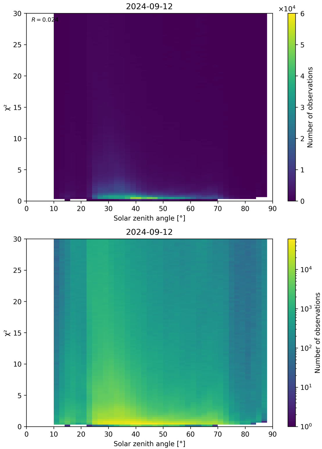
Figure 119: Scatter density plot of “Solar zenith angle” against “ \chi^2 ” for 2024-09-12 to 2024-09-13.
