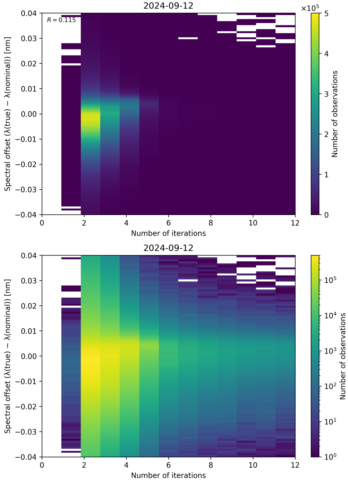
Figure 109: Scatter density plot of “Number of iterations” against “Spectral offset ( \lambda_{\text{true}} - \lambda_{\text{nominal}} )” for 2024-09-12 to 2024-09-13.
