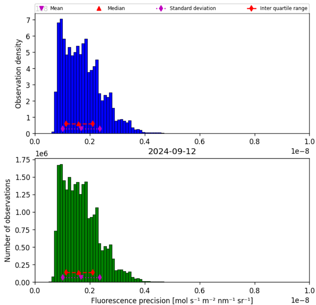
Figure 41: Histogram of “Fluorescence precision” for 2024-09-12 to 2024-09-13
