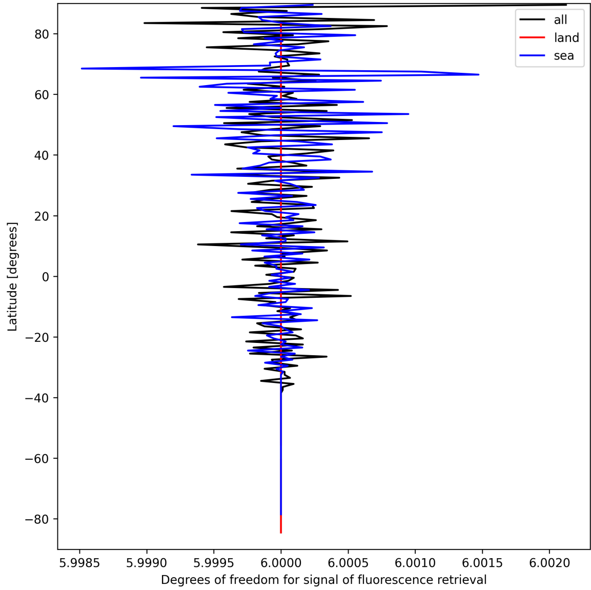
Figure 26: Zonal average of “Degrees of freedom for signal of fluorescence retrieval” for 2024-09-12 to 2024-09-13.
