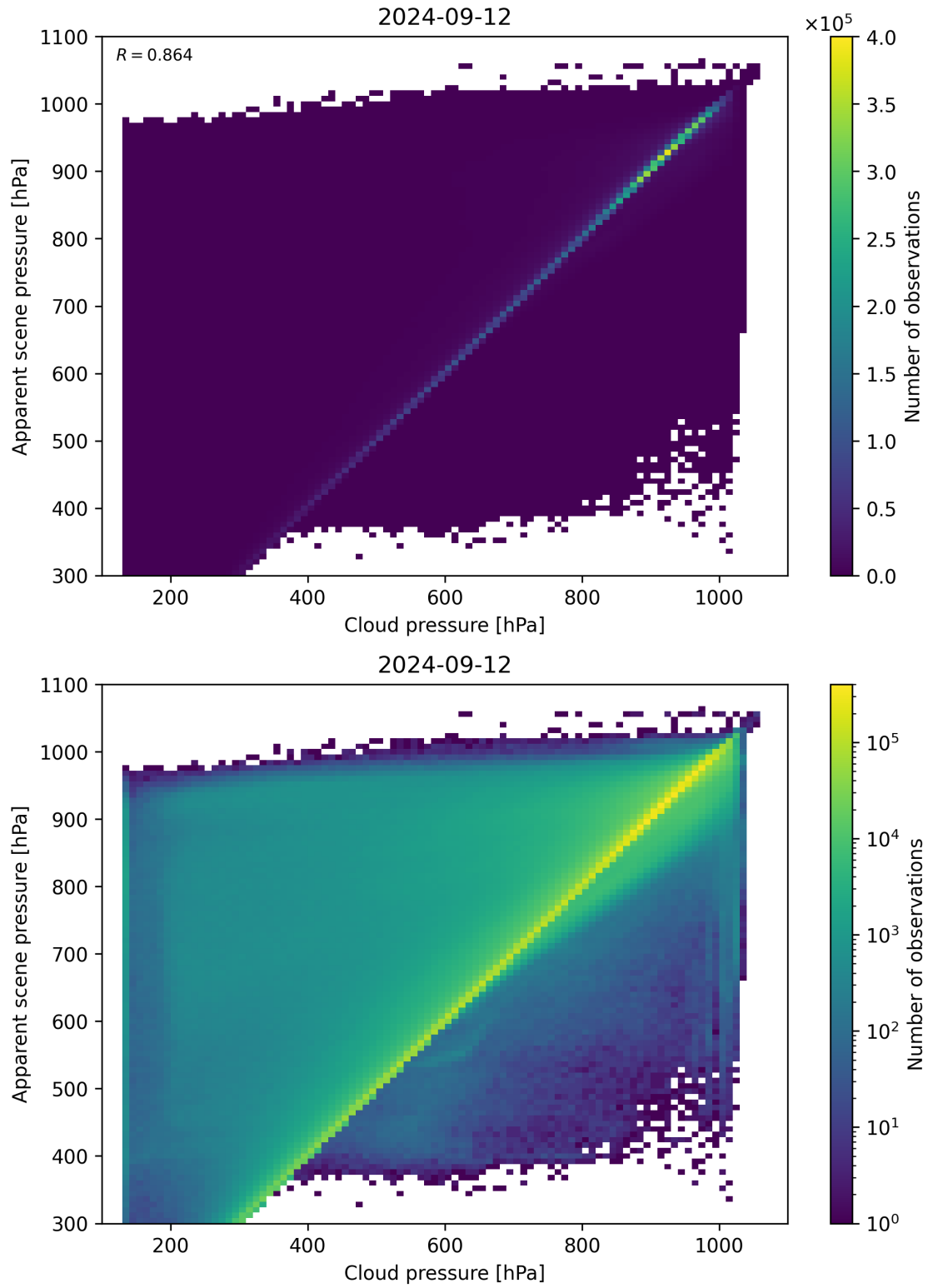
Figure 84: Scatter density plot of “Cloud pressure” against “Apparent scene pressure” for 2024-09-12 to 2024-09-13.
