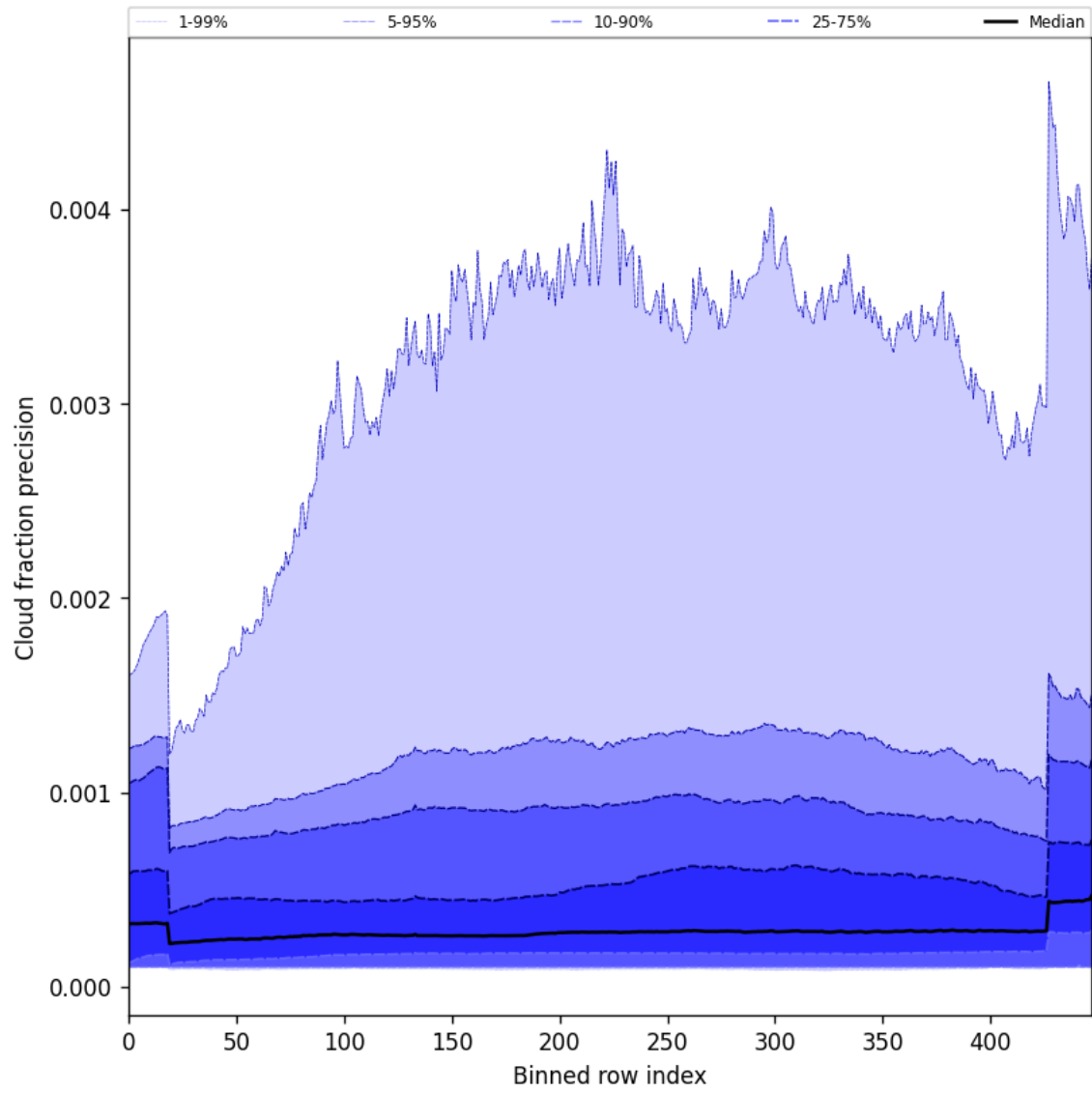
Figure 50: Along track statistics of “Cloud fraction precision” for 2024-09-12 to 2024-09-13
