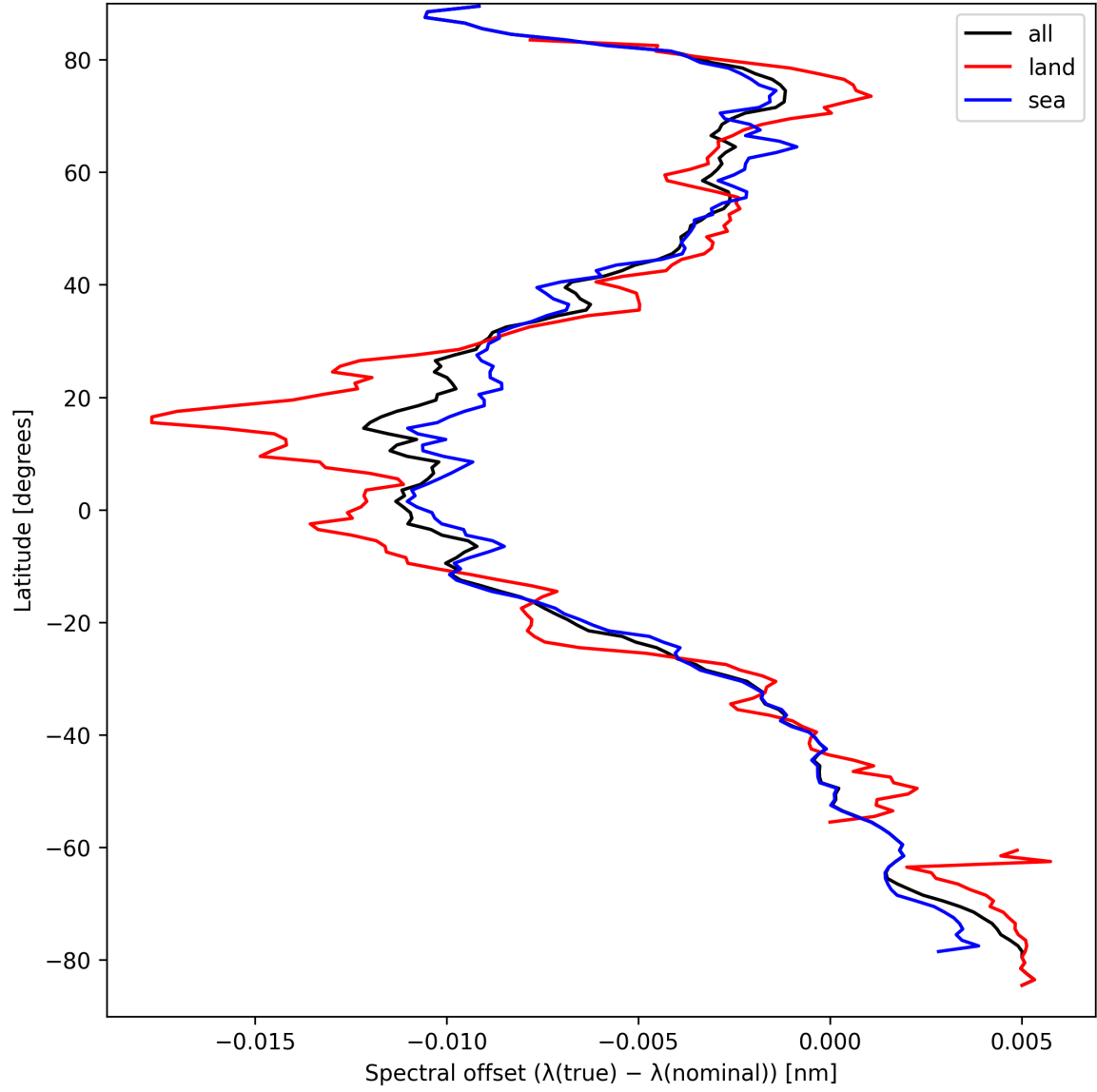
Figure 28: Zonal average of “Spectral offset ( \lambda_{\text{true}} - \lambda_{\text{nominal}} )” for 2024-09-12 to 2024-09-13.
