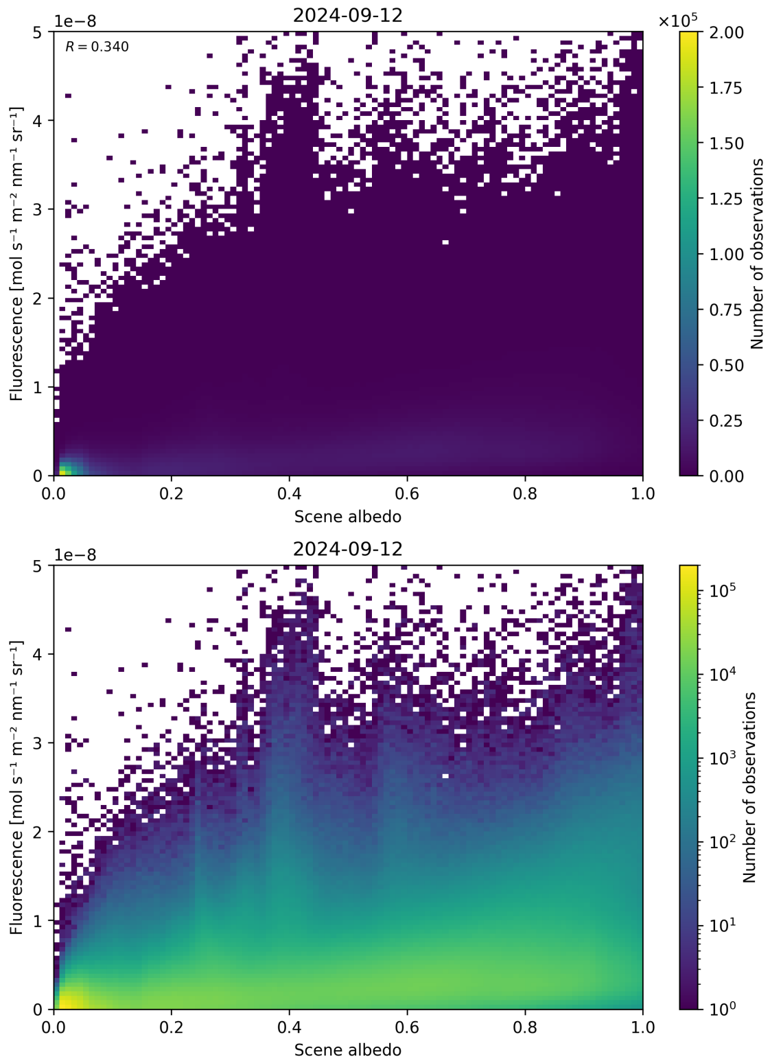
Figure 114: Scatter density plot of “Scene albedo” against “Fluorescence” for 2024-09-12 to 2024-09-13.
