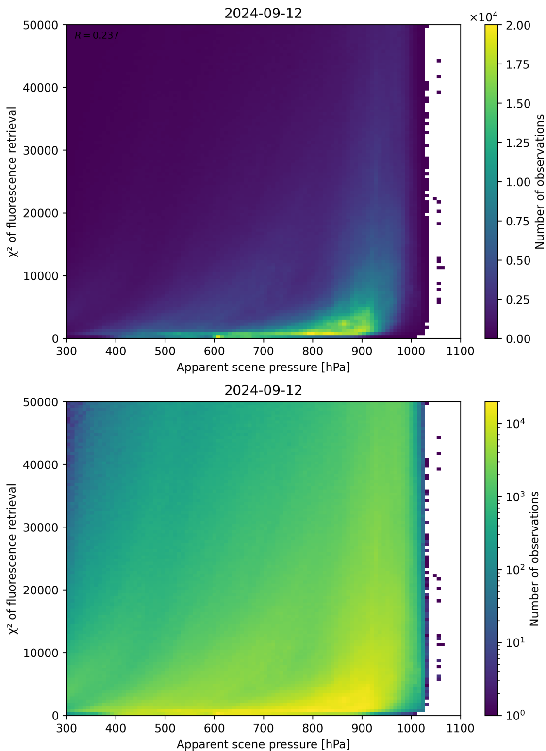
Figure 64: Scatter density plot of “Apparent scene pressure” against “ \chi^2 of fluorescence retrieval” for 2024-09-12 to 2024-09-13.
