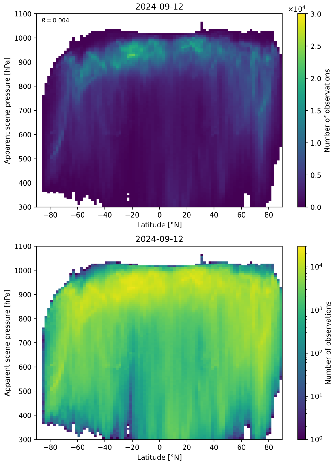
Figure 96: Scatter density plot of “Latitude” against “Apparent scene pressure” for 2024-09-12 to 2024-09-13.
