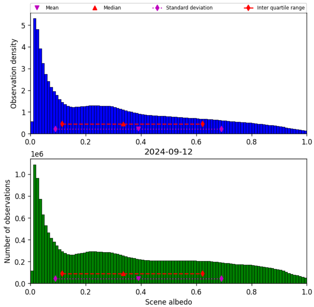
Figure 34: Histogram of “Scene albedo” for 2024-09-12 to 2024-09-13
