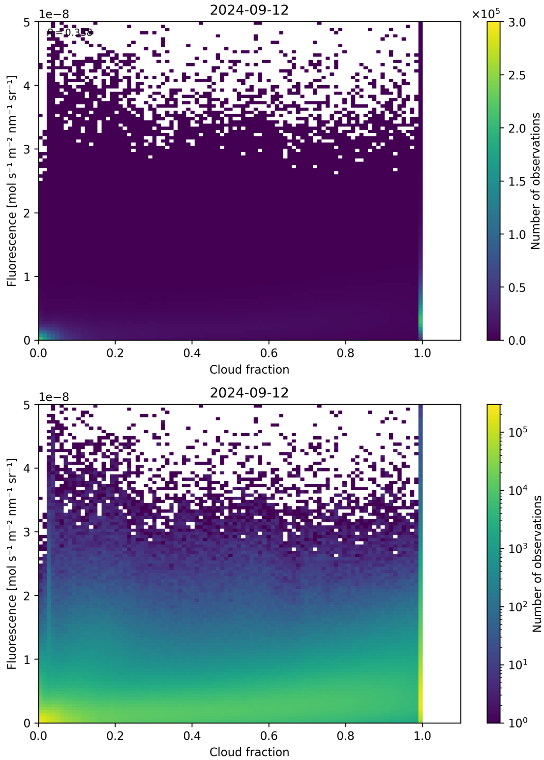
Figure 79: Scatter density plot of “Cloud fraction” against “Fluorescence” for 2024-09-12 to 2024-09-13.
