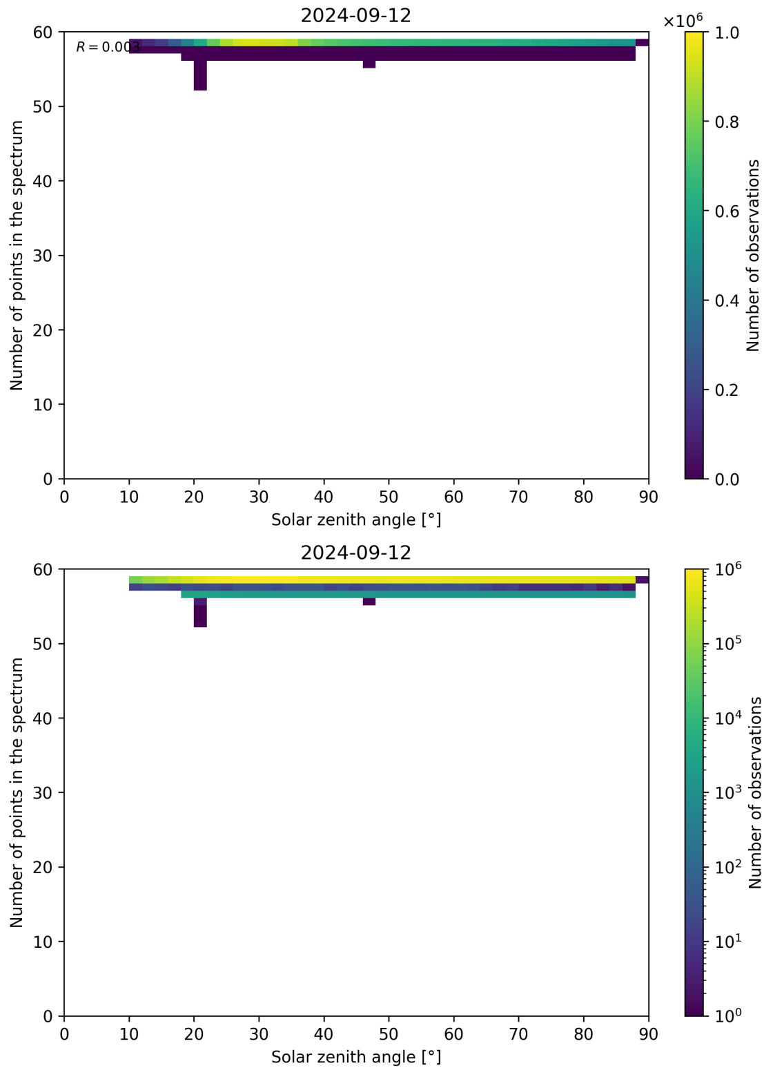
Figure 126: Scatter density plot of “Solar zenith angle” against “Number of points in the spectrum” for 2024-09-12 to 2024-09-13.
