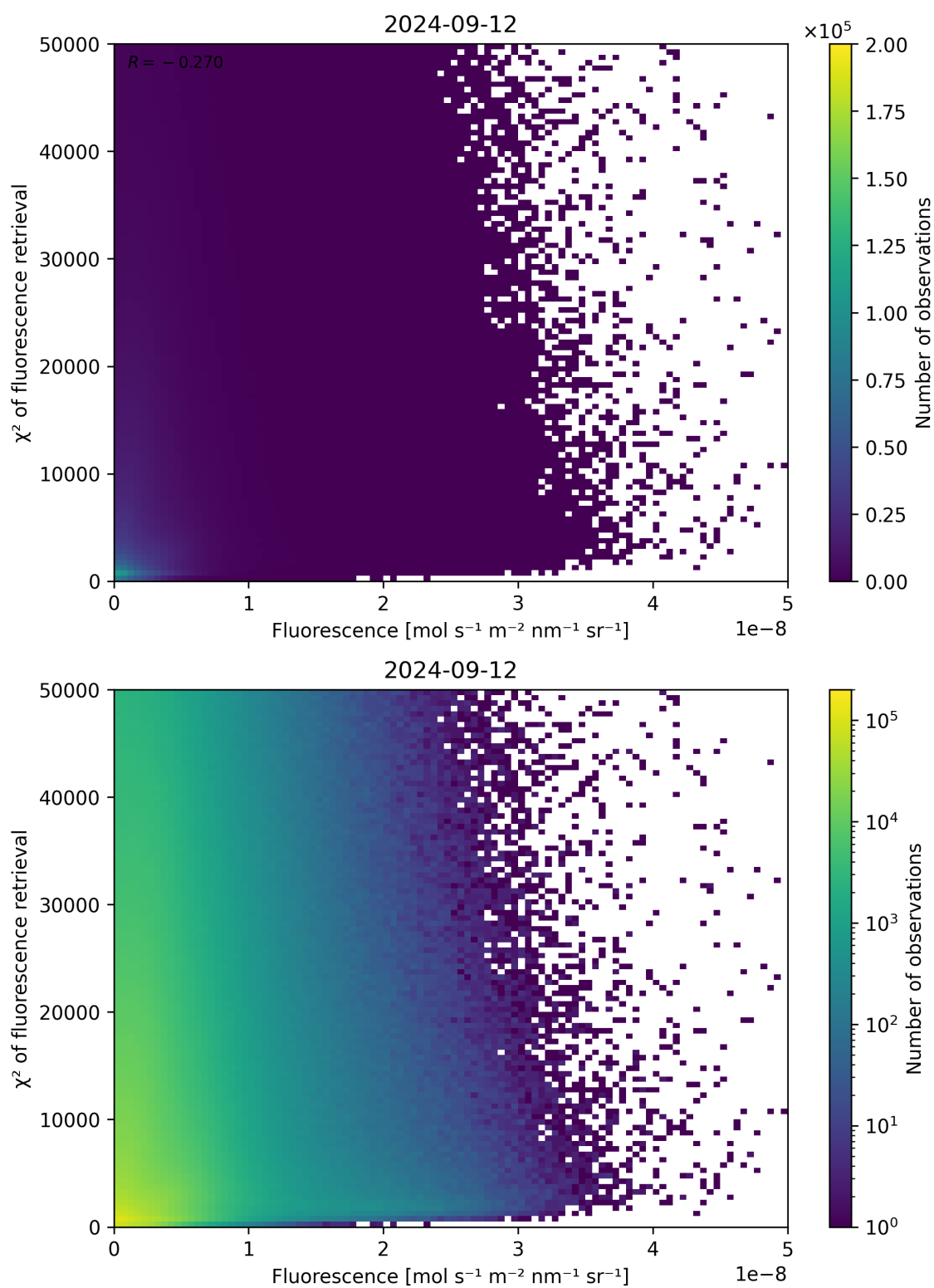
Figure 93: Scatter density plot of “Fluorescence” against “ \chi^2 of fluorescence retrieval” for 2024-09-12 to 2024-09-13.
