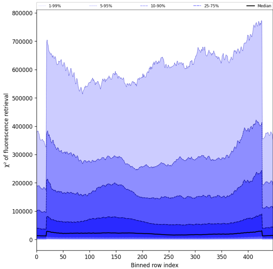
Figure 59: Along track statistics of “ \chi^2 of fluorescence retrieval” for 2024-09-12 to 2024-09-13
