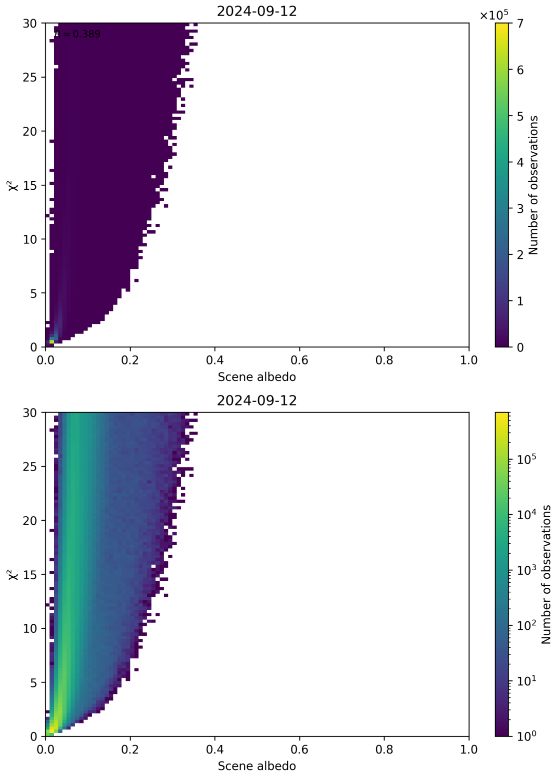
Figure 112: Scatter density plot of “Scene albedo” against “ \chi^2 ” for 2024-09-12 to 2024-09-13.
