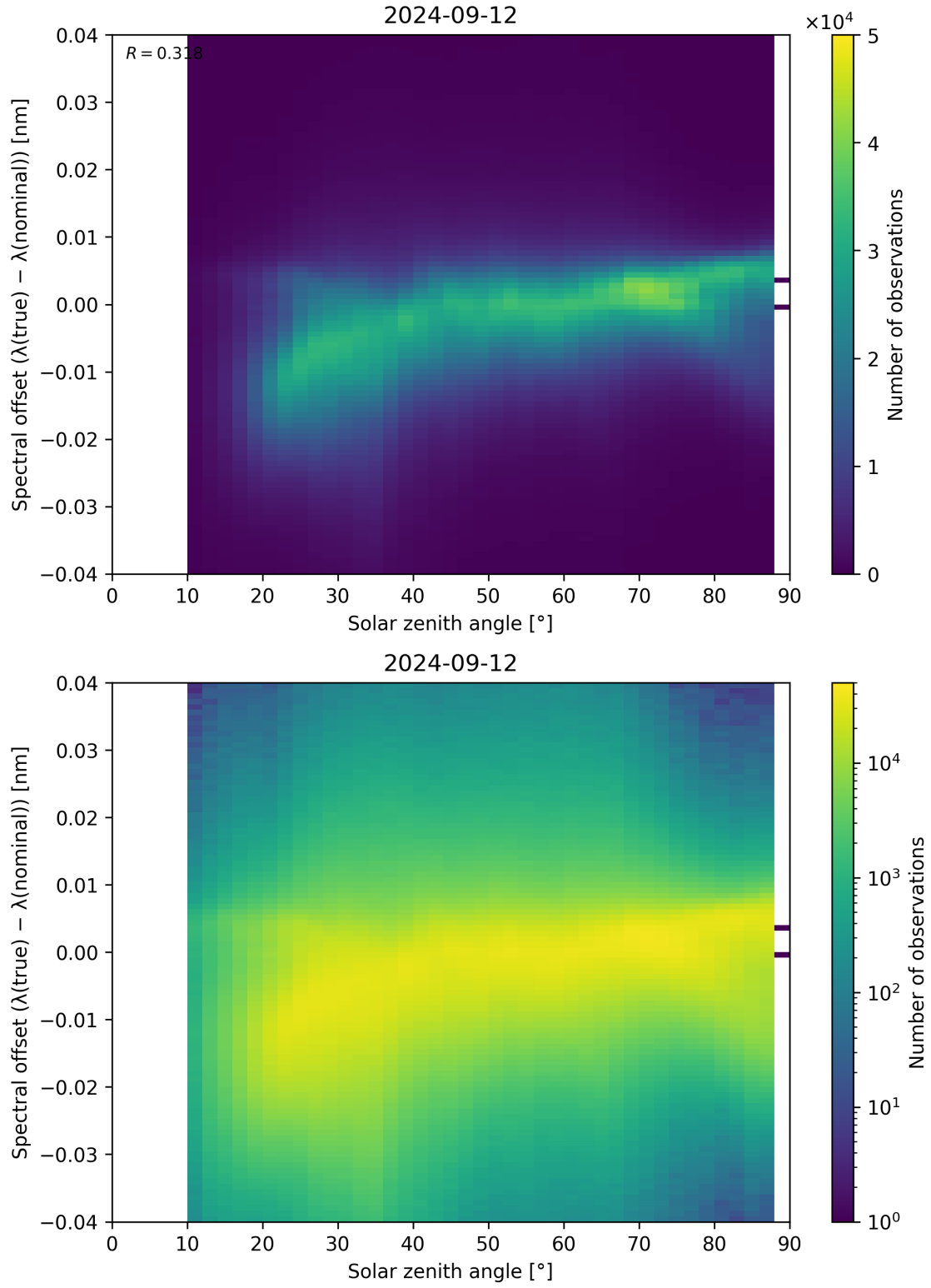
Figure 128: Scatter density plot of “Solar zenith angle” against “Spectral offset ( \lambda_{\text{true}} - \lambda_{\text{nominal}} )” for 2024-09-12 to 2024-09-13.
