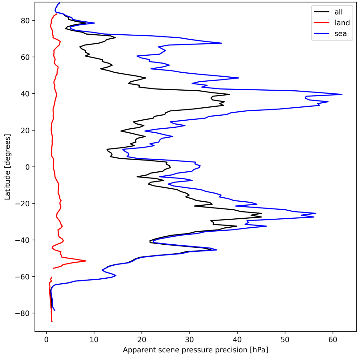
Figure 20: Zonal average of “Apparent scene pressure precision” for 2024-09-12 to 2024-09-13.
