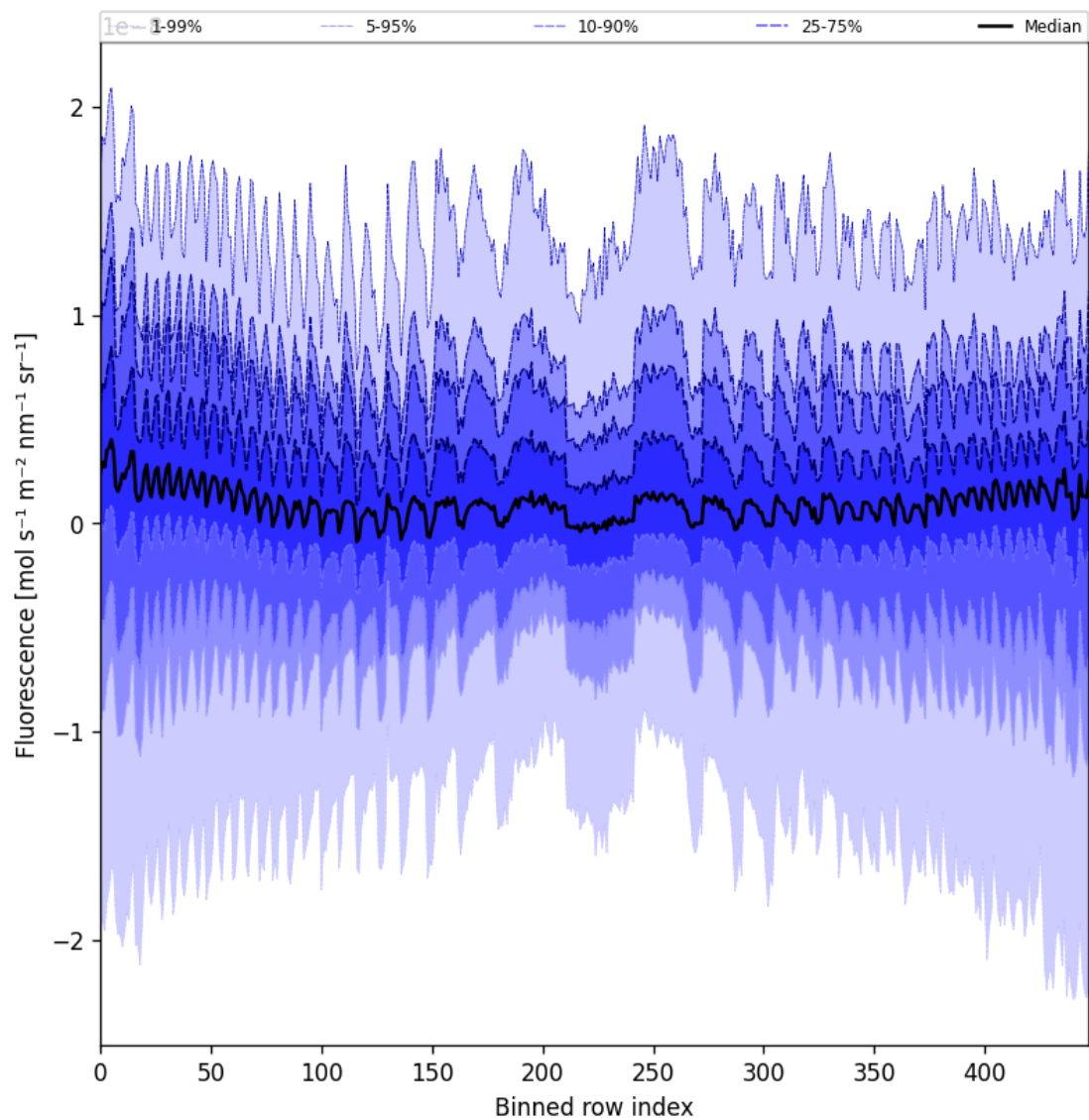
Figure 57: Along track statistics of “Fluorescence” for 2024-09-12 to 2024-09-13
