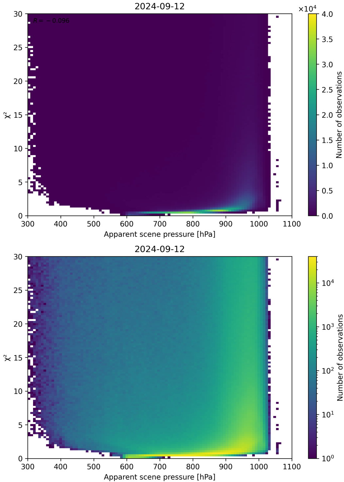
Figure 63: Scatter density plot of “Apparent scene pressure” against “ \chi^2 ” for 2024-09-12 to 2024-09-13.
