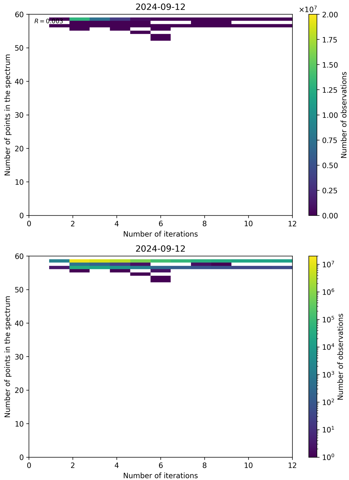
Figure 108: Scatter density plot of “Number of iterations” against “Number of points in the spectrum” for 2024-09-12 to 2024-09-13.
