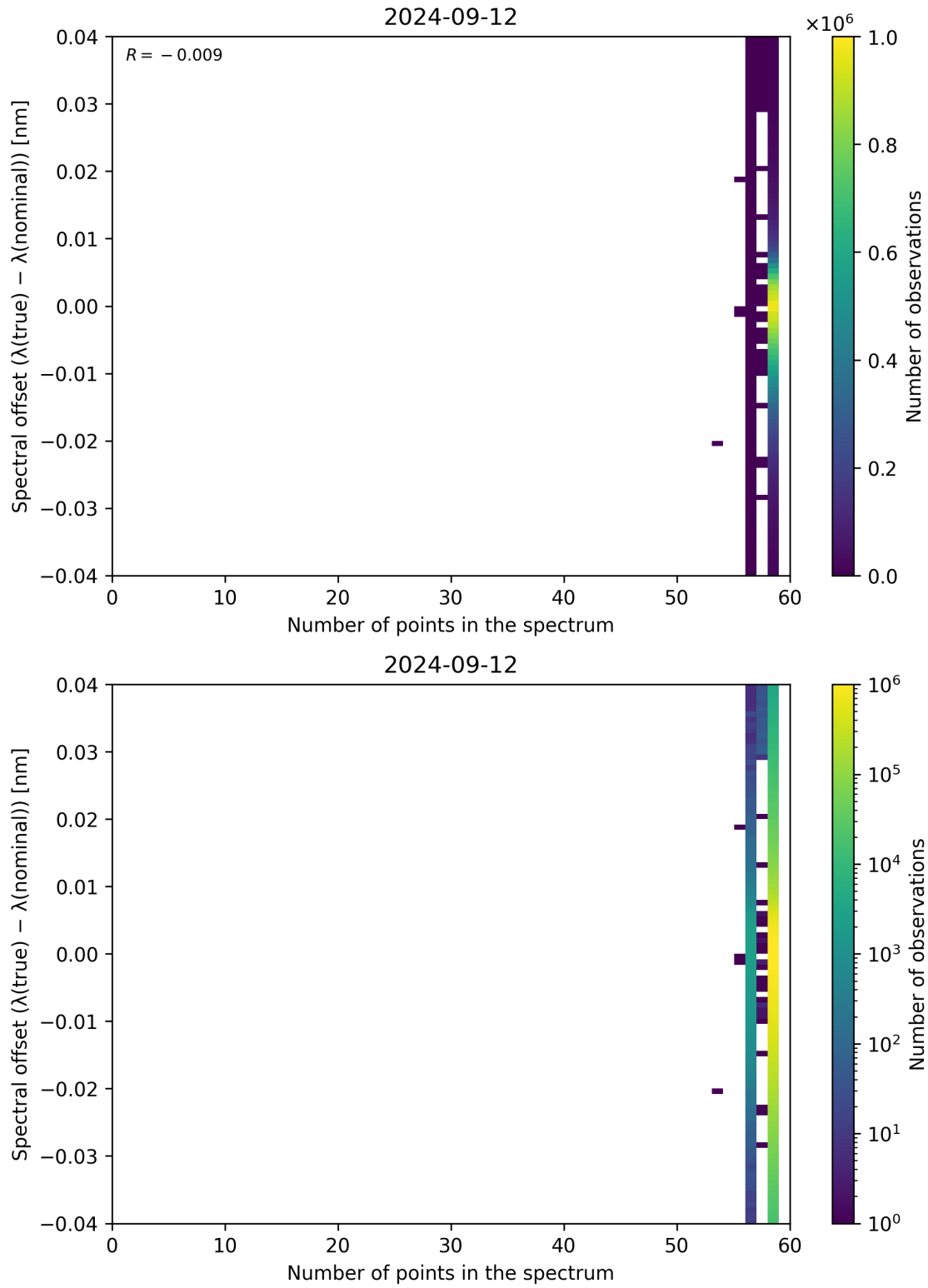
Figure 110: Scatter density plot of “Number of points in the spectrum” against “Spectral offset ( \lambda_{\text{true}} - \lambda_{\text{nominal}} )” for 2024-09-12 to 2024-09-13.
