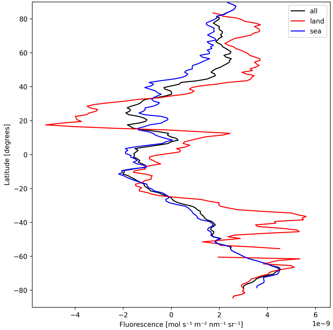
Figure 23: Zonal average of “Fluorescence” for 2024-09-12 to 2024-09-13.
