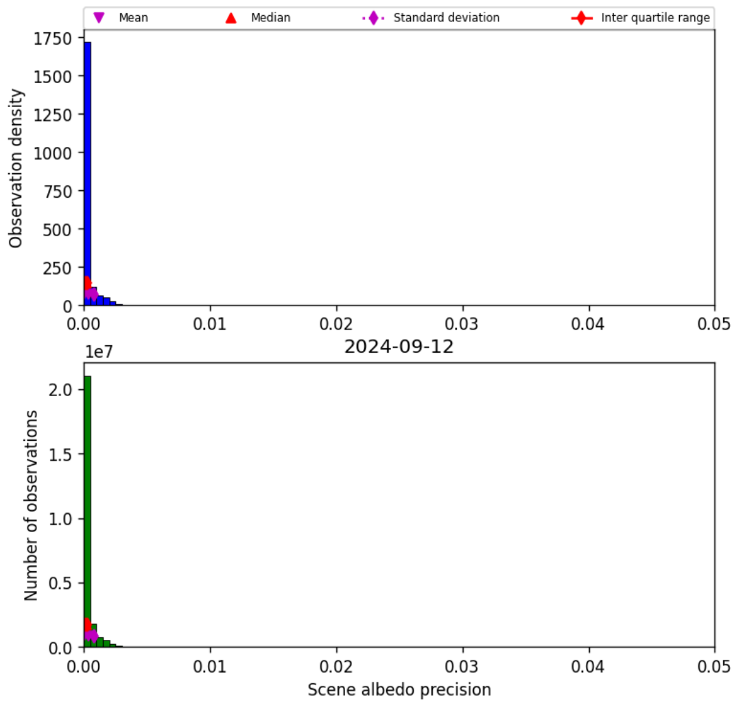
Figure 35: Histogram of “Scene albedo precision” for 2024-09-12 to 2024-09-13
