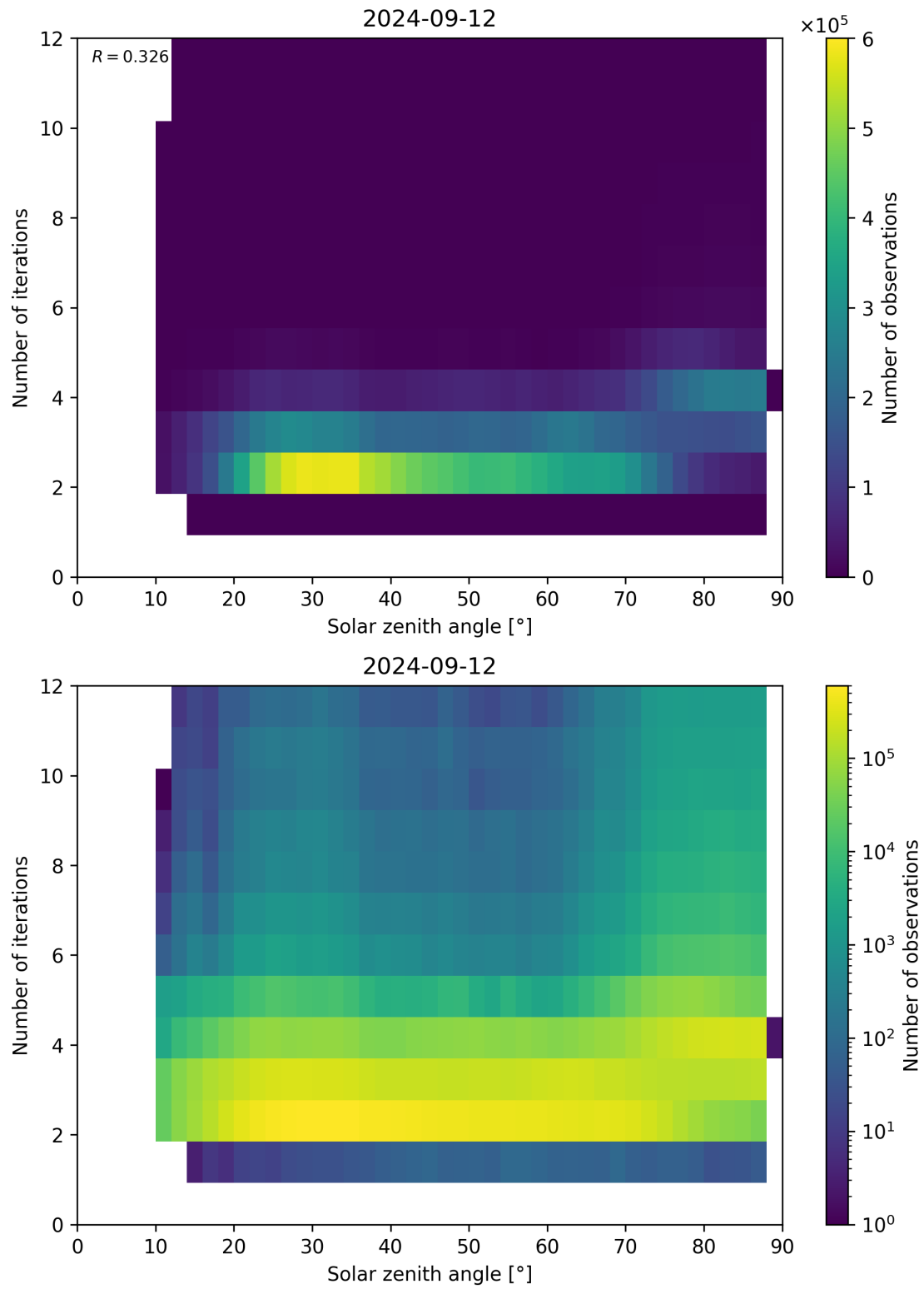
Figure 125: Scatter density plot of “Solar zenith angle” against “Number of iterations” for 2024-09-12 to 2024-09-13.
