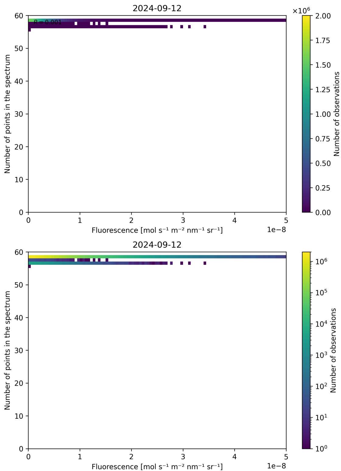
Figure 94: Scatter density plot of “Fluorescence” against “Number of points in the spectrum” for 2024-09-12 to 2024-09-13.
