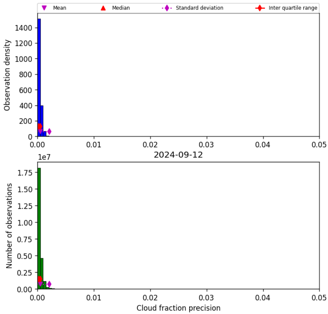
Figure 33: Histogram of “Cloud fraction precision” for 2024-09-12 to 2024-09-13
