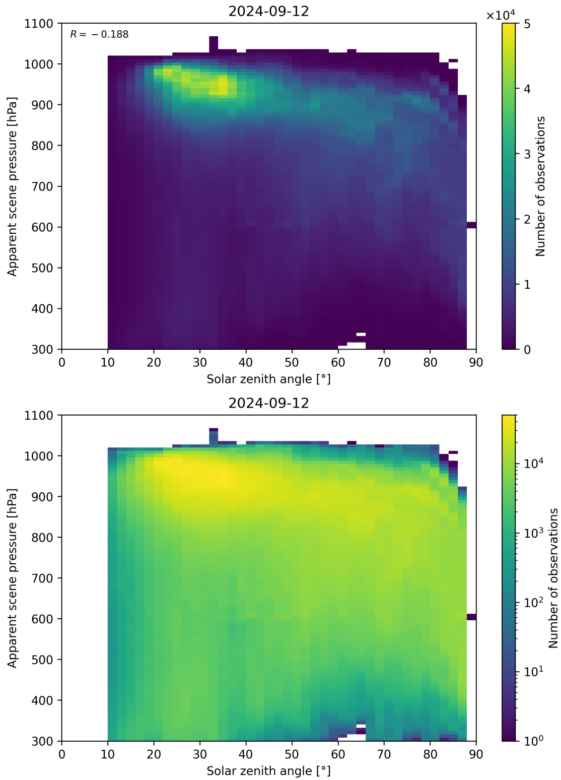
Figure 118: Scatter density plot of “Solar zenith angle” against “Apparent scene pressure” for 2024-09-12 to 2024-09-13.
