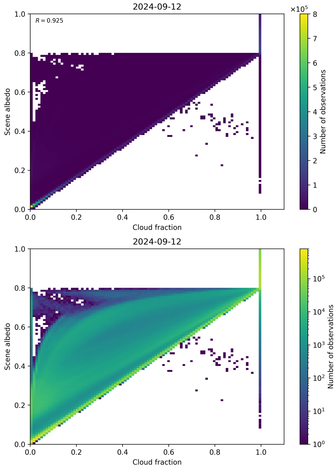
Figure 82: Scatter density plot of “Cloud fraction” against “Scene albedo” for 2024-09-12 to 2024-09-13.
