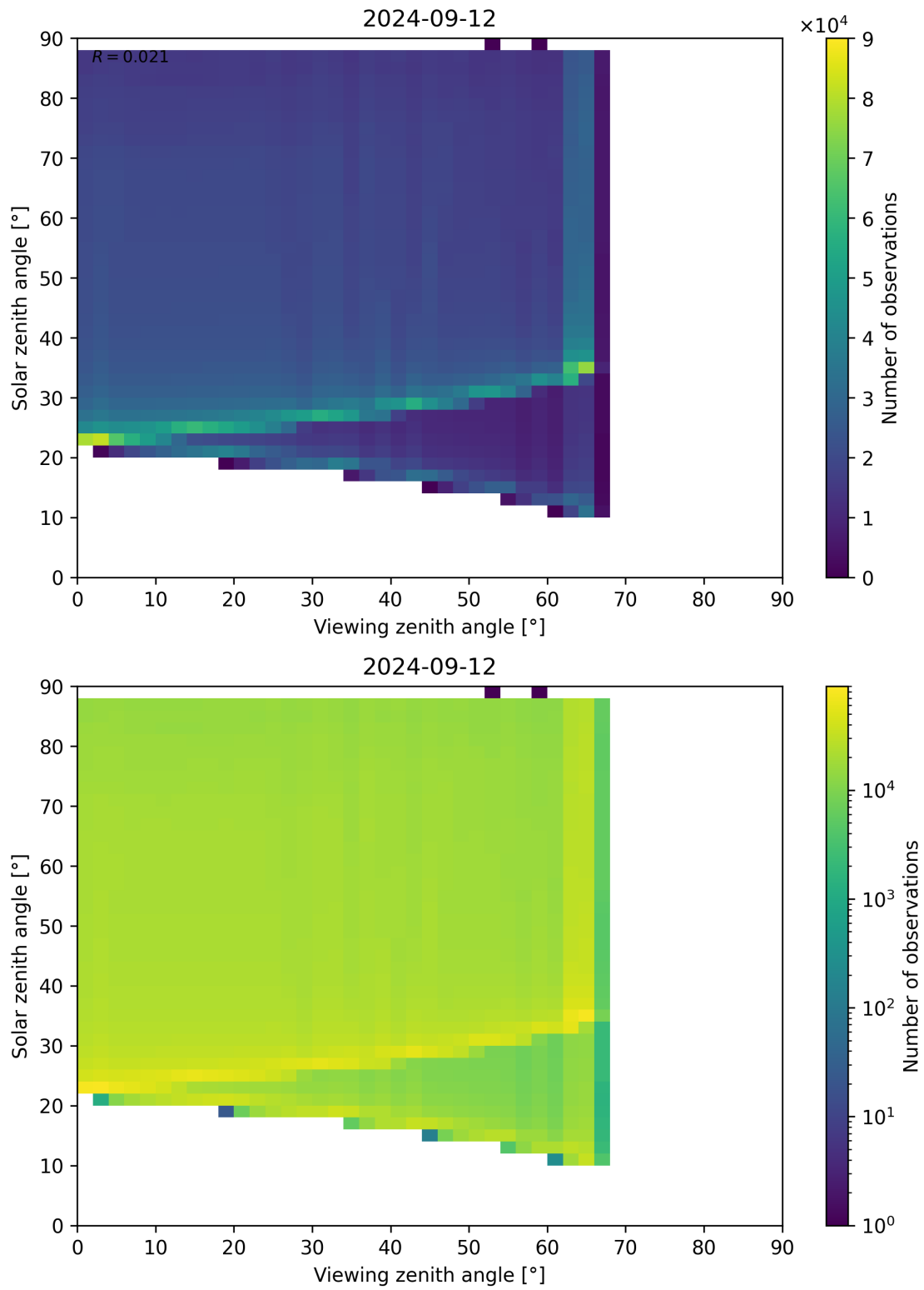
Figure 139: Scatter density plot of “Viewing zenith angle” against “Solar zenith angle” for 2024-09-12 to 2024-09-13.
