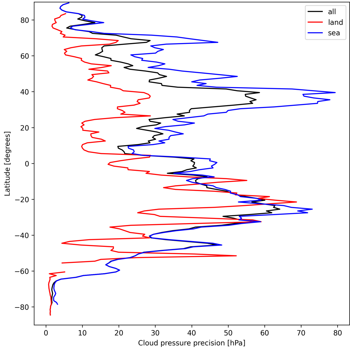
Figure 14: Zonal average of “Cloud pressure precision” for 2024-09-12 to 2024-09-13.
