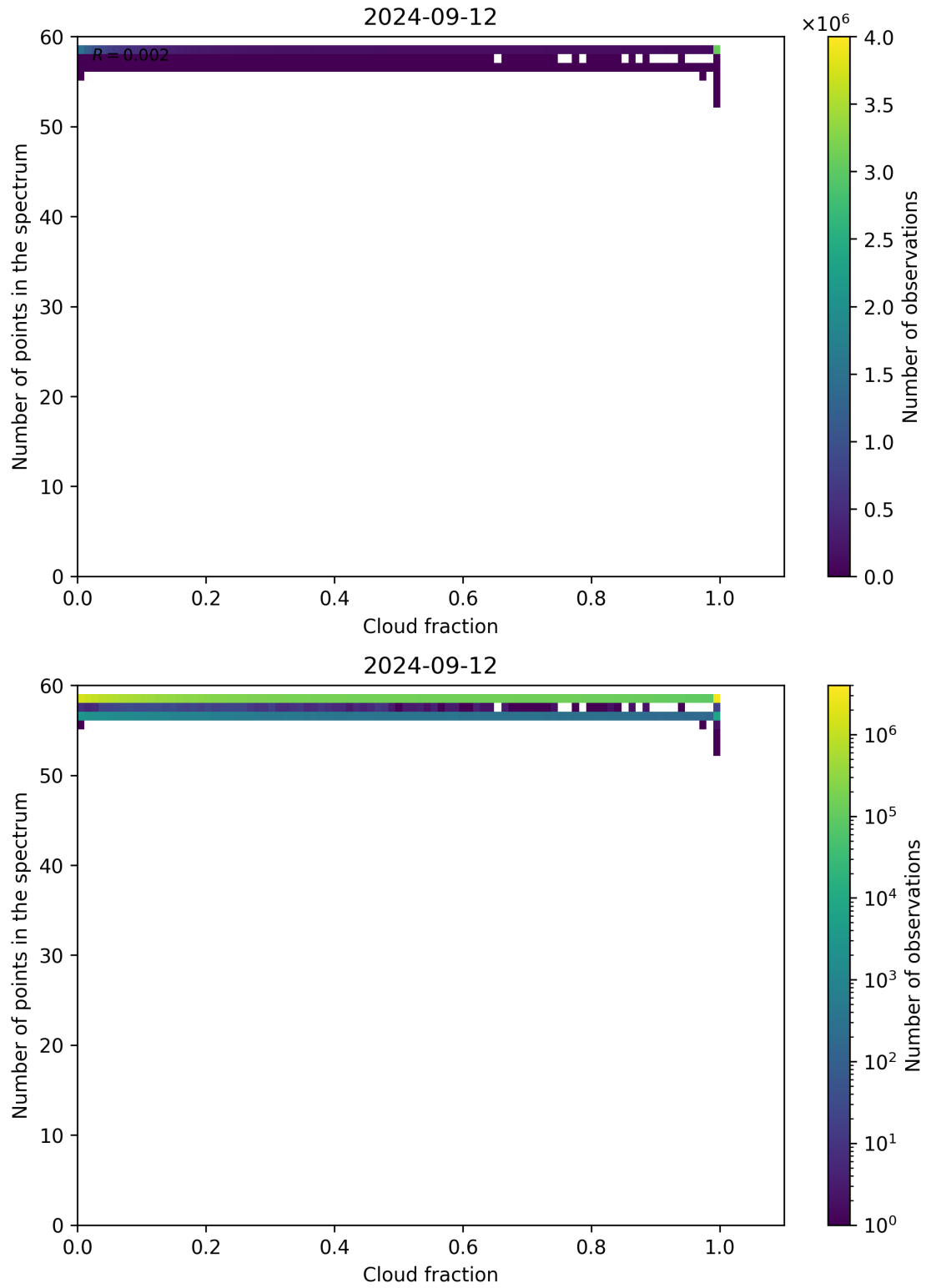
Figure 81: Scatter density plot of “Cloud fraction” against “Number of points in the spectrum” for 2024-09-12 to 2024-09-13.
