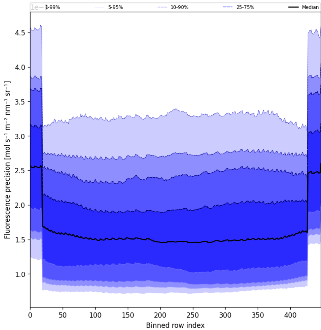
Figure 58: Along track statistics of “Fluorescence precision” for 2024-09-12 to 2024-09-13
