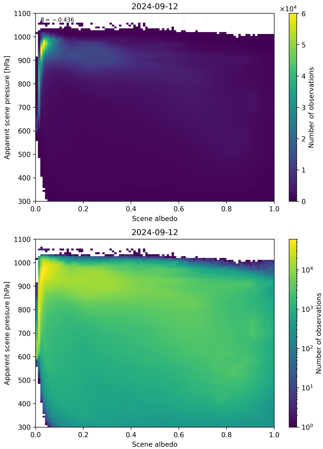
Figure 111: Scatter density plot of “Scene albedo” against “Apparent scene pressure” for 2024-09-12 to 2024-09-13.
