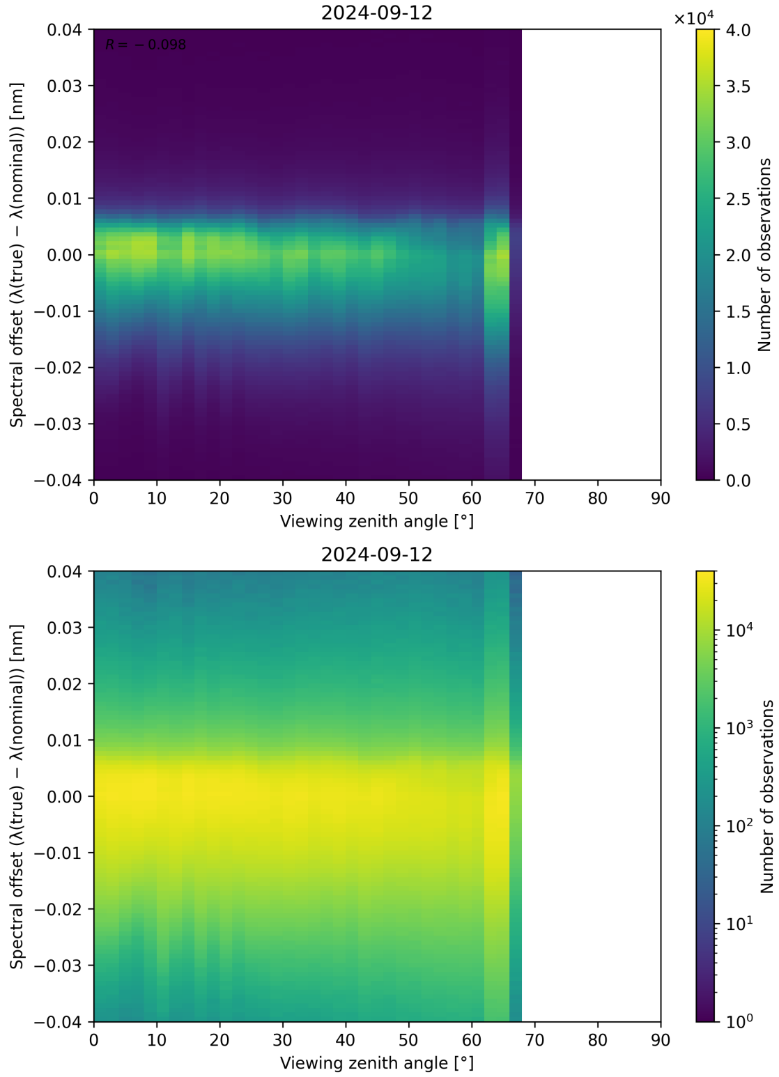
Figure 140: Scatter density plot of “Viewing zenith angle” against “Spectral offset ( \lambda_{\text{true}} - \lambda_{\text{nominal}} )” for 2024-09-12 to 2024-09-13.
