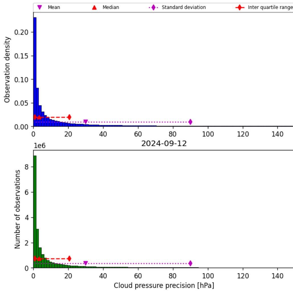
Figure 31: Histogram of “Cloud pressure precision” for 2024-09-12 to 2024-09-13
