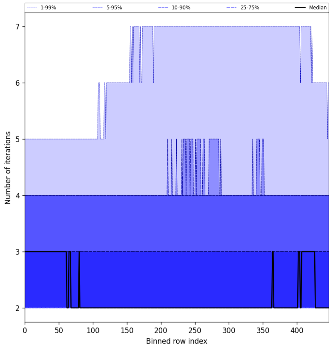
Figure 56: Along track statistics of “Number of iterations” for 2024-09-12 to 2024-09-13
