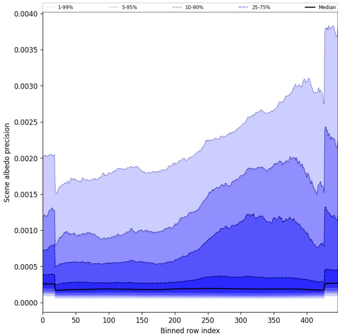
Figure 52: Along track statistics of “Scene albedo precision” for 2024-09-12 to 2024-09-13
