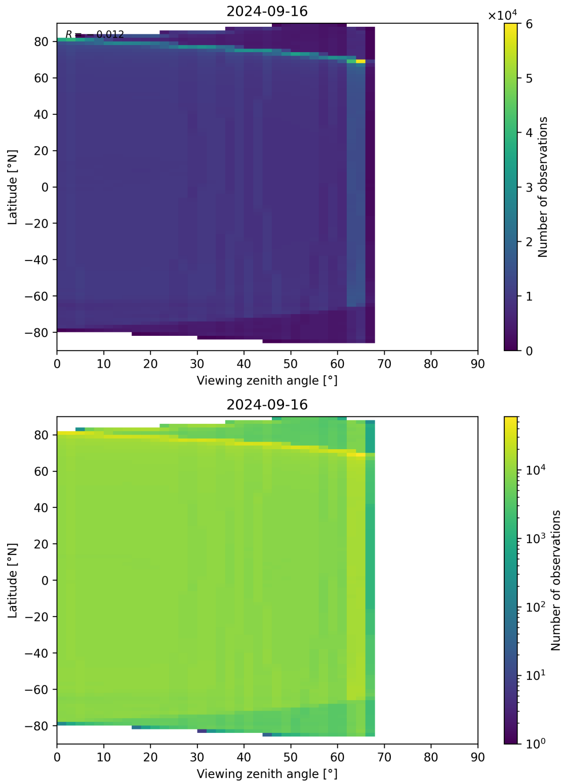
Figure 135: Scatter density plot of “Viewing zenith angle” against “Latitude” for 2024-09-15 to 2024-09-17.
