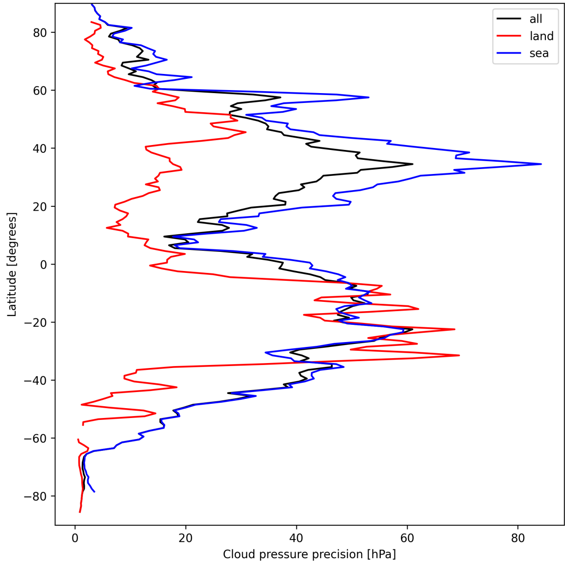
Figure 14: Zonal average of “Cloud pressure precision” for 2024-09-15 to 2024-09-17.
