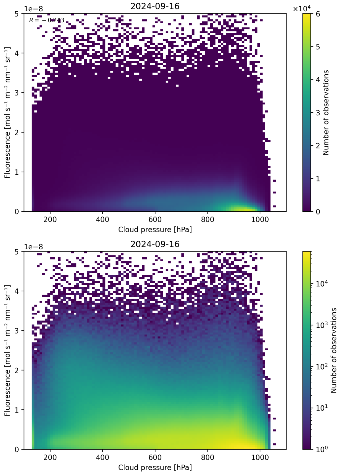
Figure 88: Scatter density plot of “Cloud pressure” against “Fluorescence” for 2024-09-15 to 2024-09-17.
