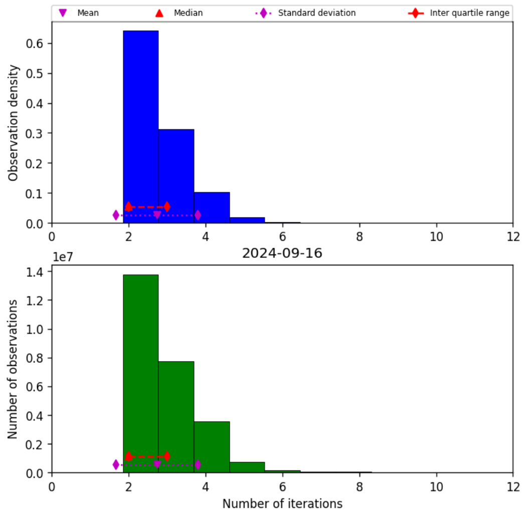
Figure 39: Histogram of “Number of iterations” for 2024-09-15 to 2024-09-17
