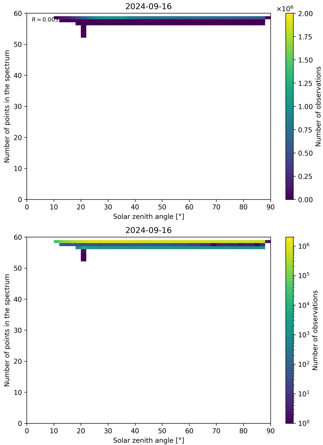
Figure 126: Scatter density plot of “Solar zenith angle” against “Number of points in the spectrum” for 2024-09-15 to 2024-09-17.
