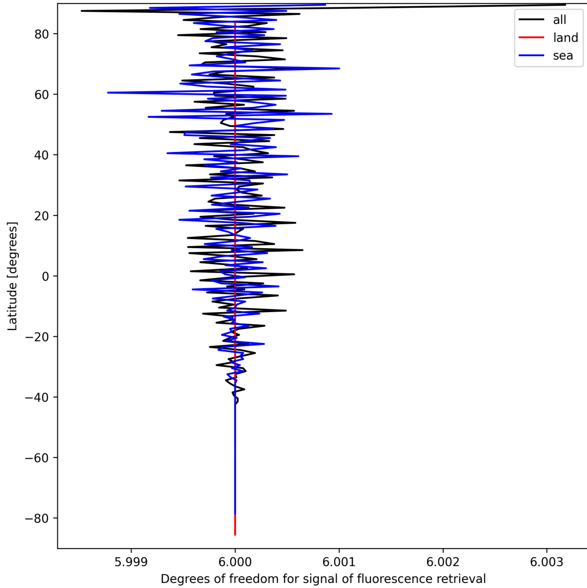
Figure 26: Zonal average of “Degrees of freedom for signal of fluorescence retrieval” for 2024-09-15 to 2024-09-17.
