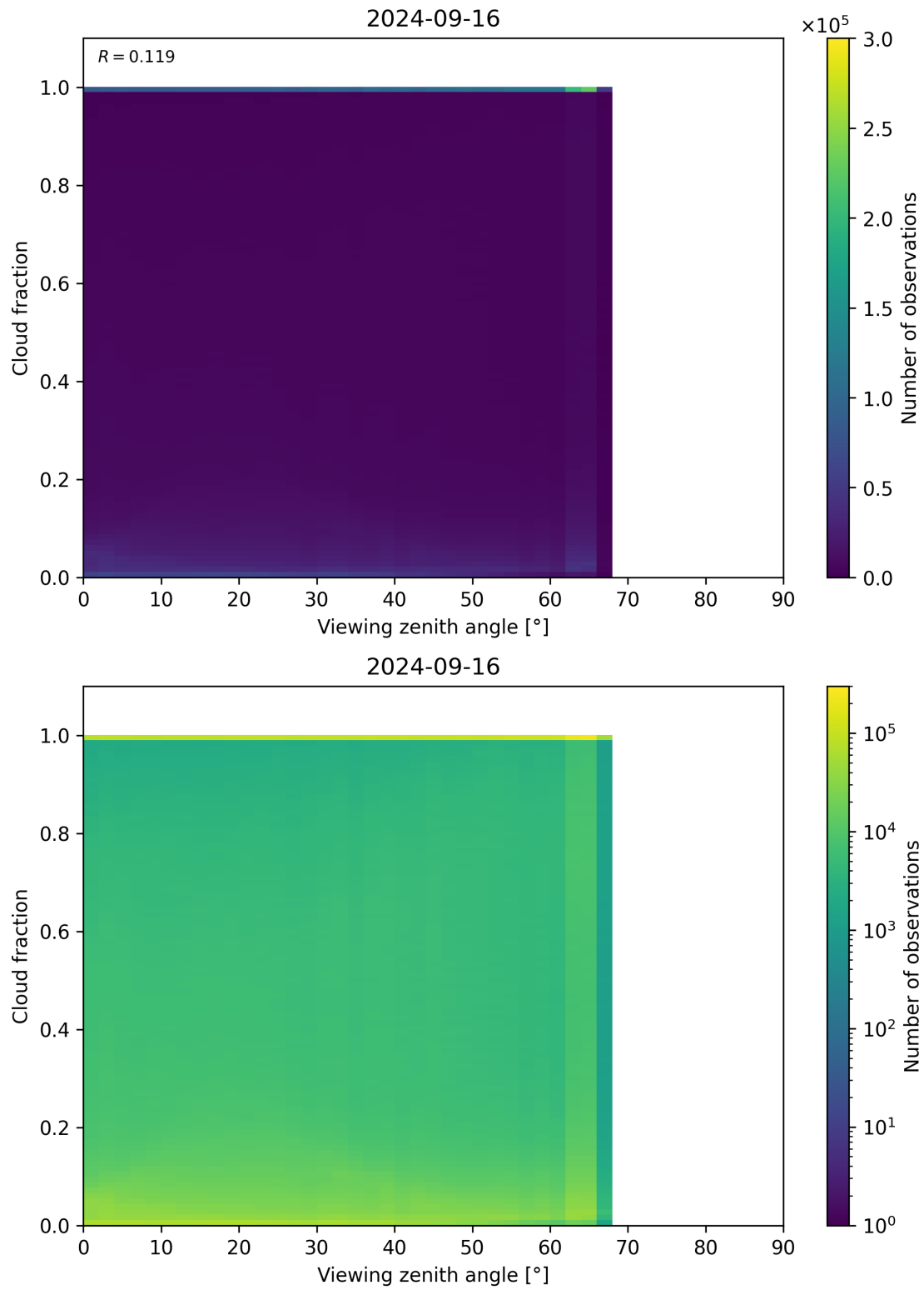
Figure 132: Scatter density plot of “Viewing zenith angle” against “Cloud fraction” for 2024-09-15 to 2024-09-17.
