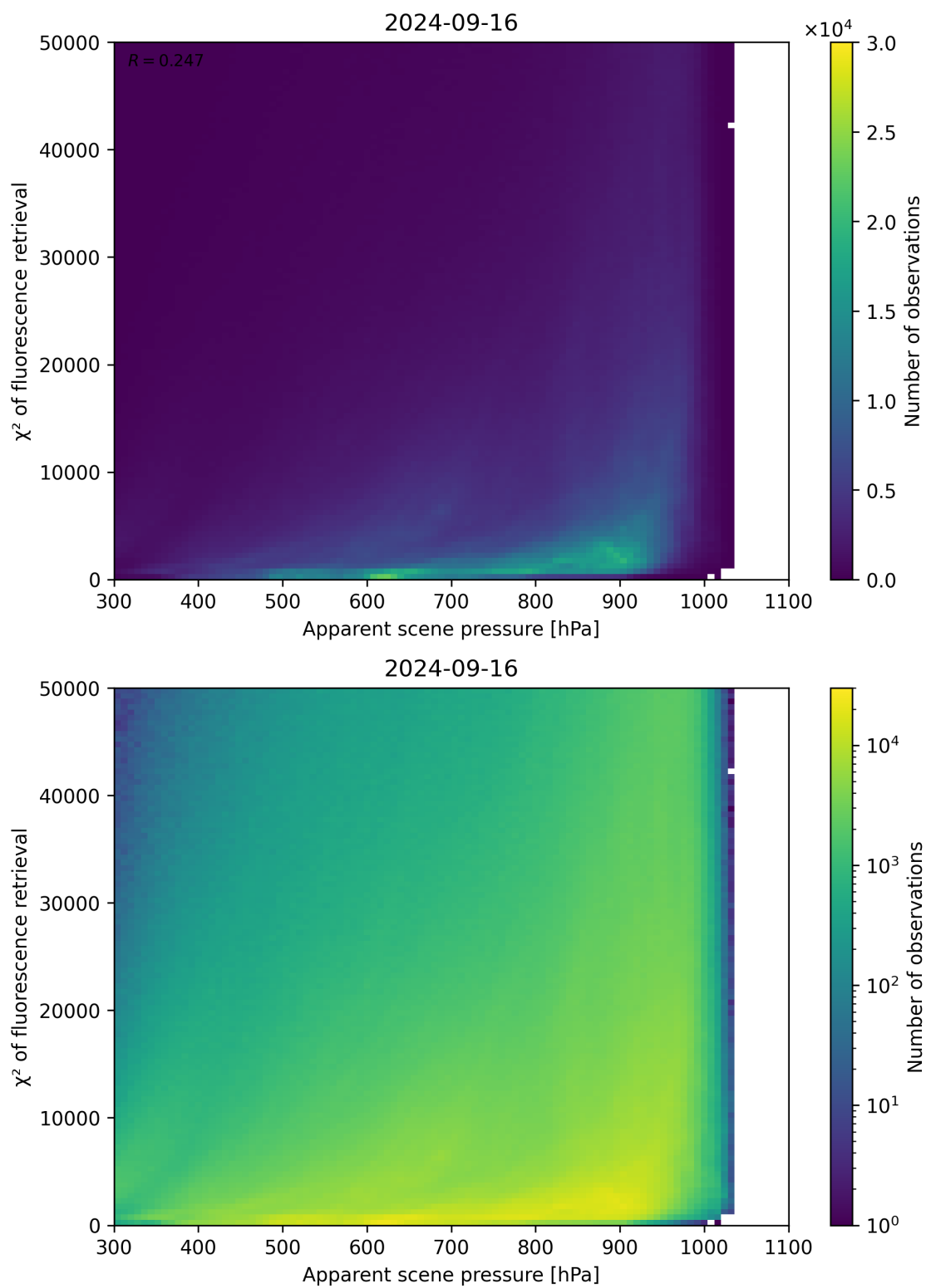
Figure 64: Scatter density plot of “Apparent scene pressure” against “ \chi^2 of fluorescence retrieval” for 2024-09-15 to 2024-09-17.
