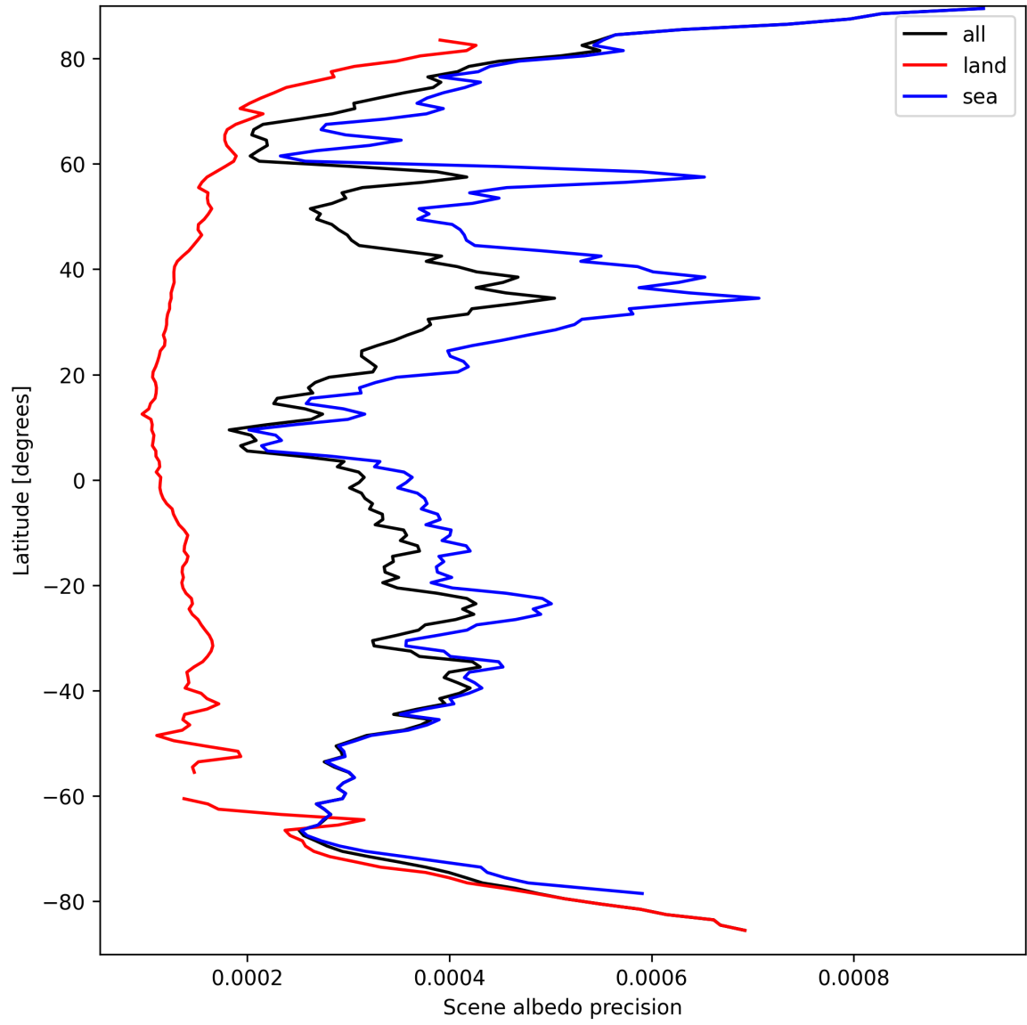
Figure 18: Zonal average of “Scene albedo precision” for 2024-09-15 to 2024-09-17.
