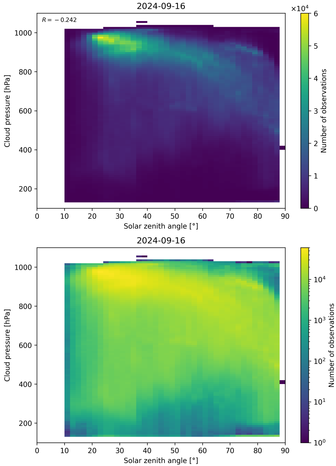
Figure 122: Scatter density plot of “Solar zenith angle” against “Cloud pressure” for 2024-09-15 to 2024-09-17.
