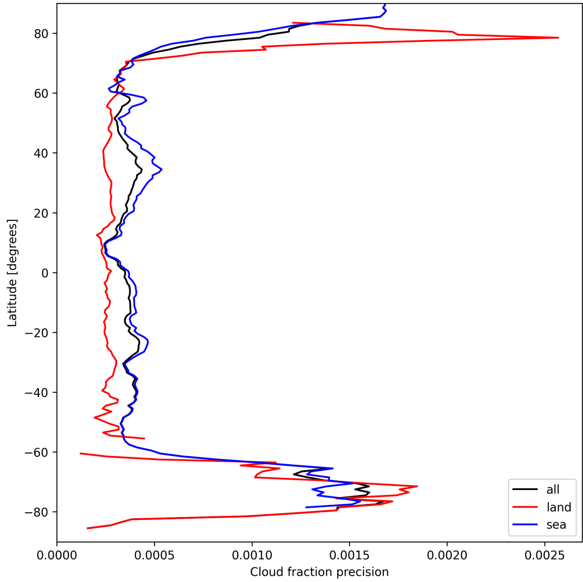
Figure 16: Zonal average of “Cloud fraction precision” for 2024-09-15 to 2024-09-17.
