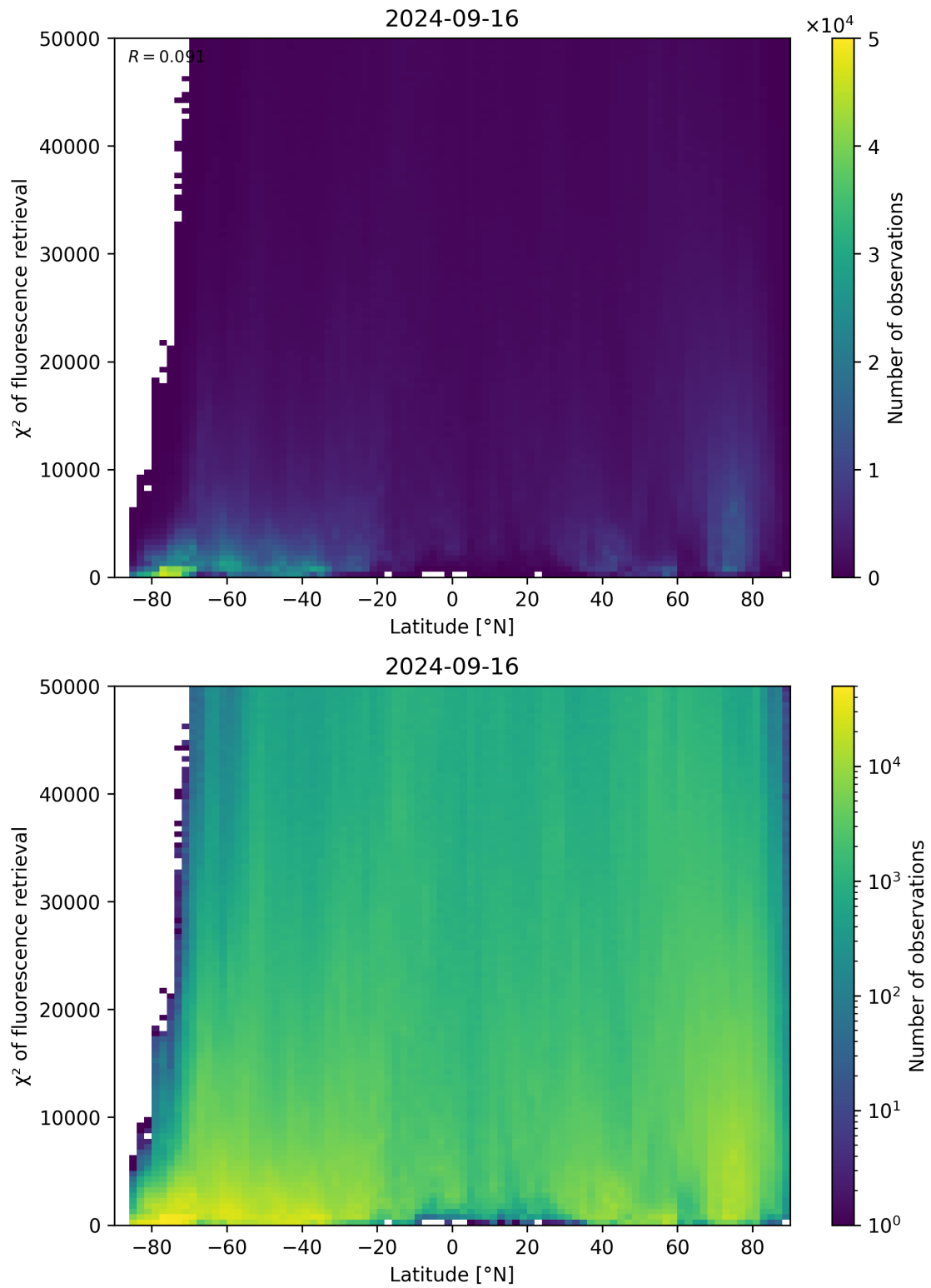
Figure 98: Scatter density plot of “Latitude” against “ \chi^2 of fluorescence retrieval” for 2024-09-15 to 2024-09-17.
