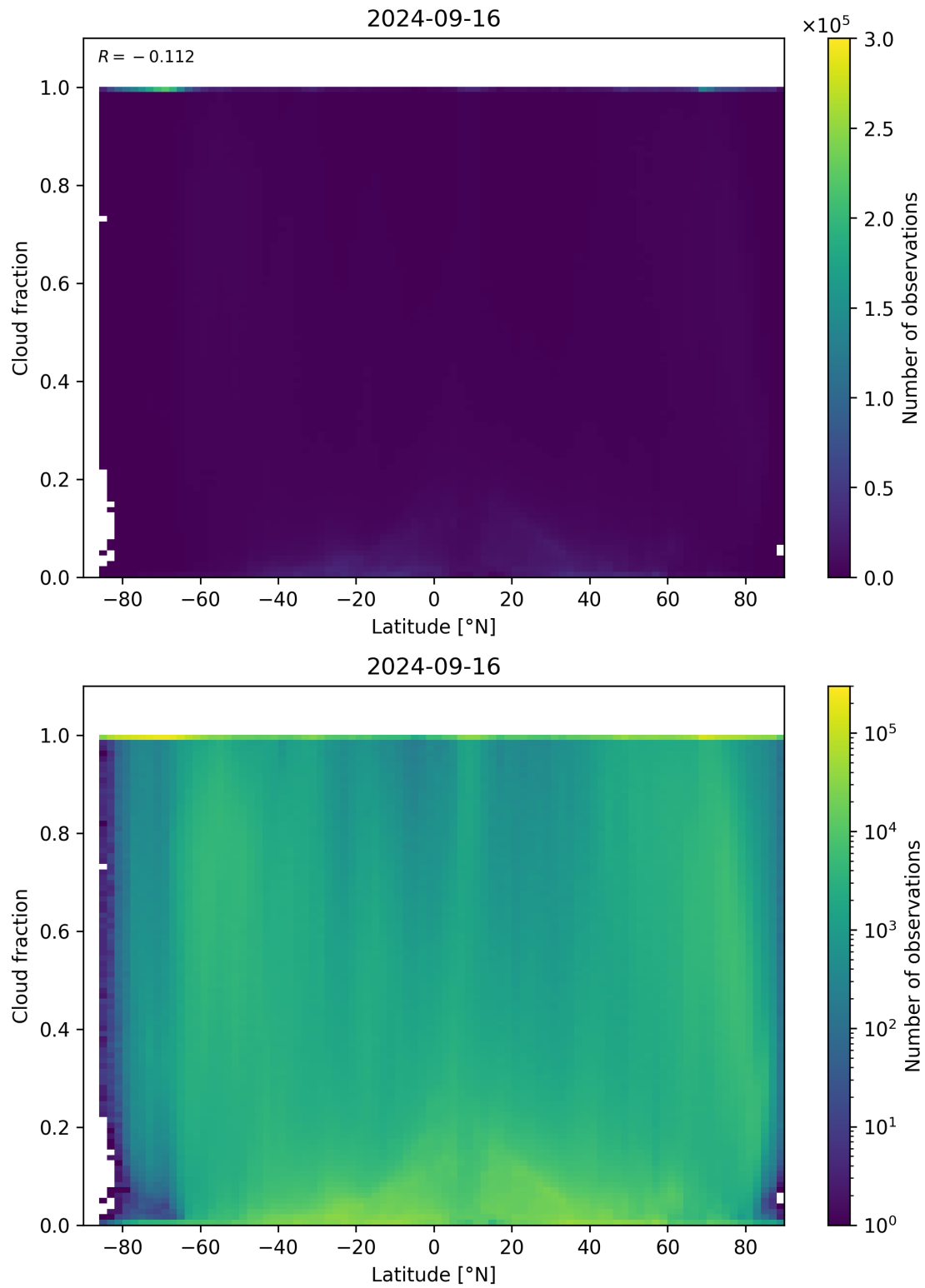
Figure 99: Scatter density plot of “Latitude” against “Cloud fraction” for 2024-09-15 to 2024-09-17.
