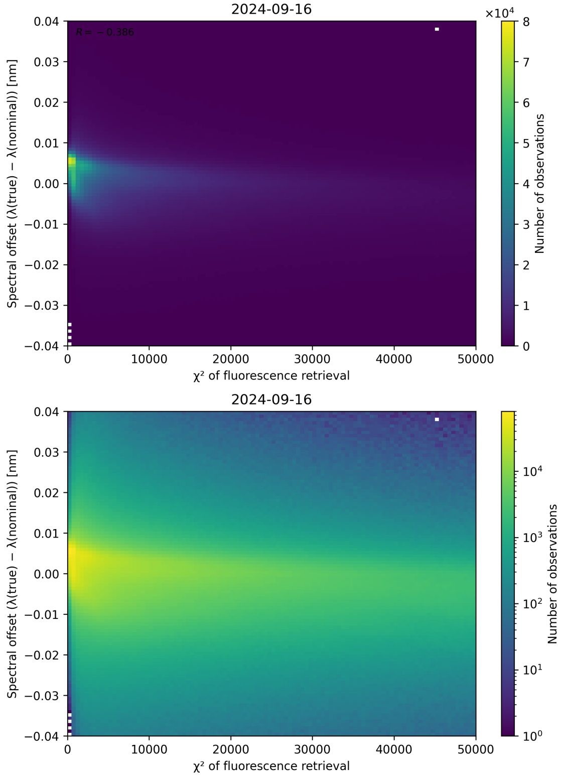
Figure 72: Scatter density plot of “ \chi^2 of fluorescence retrieval” against “Spectral offset ( \lambda_{\text{true}} - \lambda_{\text{nominal}} )” for 2024-09-15 to 2024-09-17.
