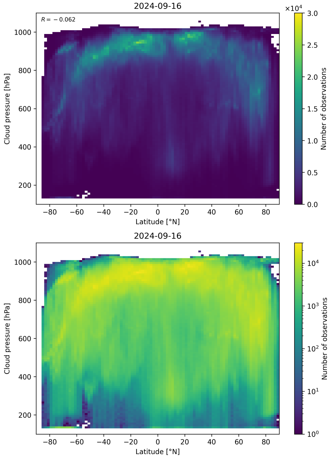
Figure 100: Scatter density plot of “Latitude” against “Cloud pressure” for 2024-09-15 to 2024-09-17.
