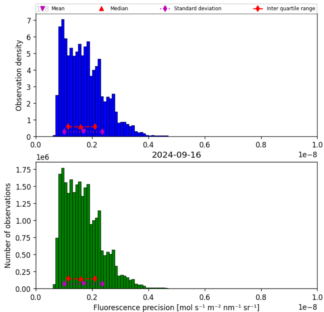
Figure 41: Histogram of “Fluorescence precision” for 2024-09-15 to 2024-09-17
