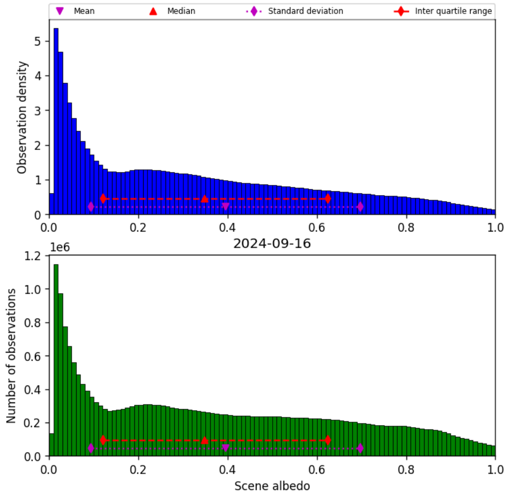
Figure 34: Histogram of “Scene albedo” for 2024-09-15 to 2024-09-17
