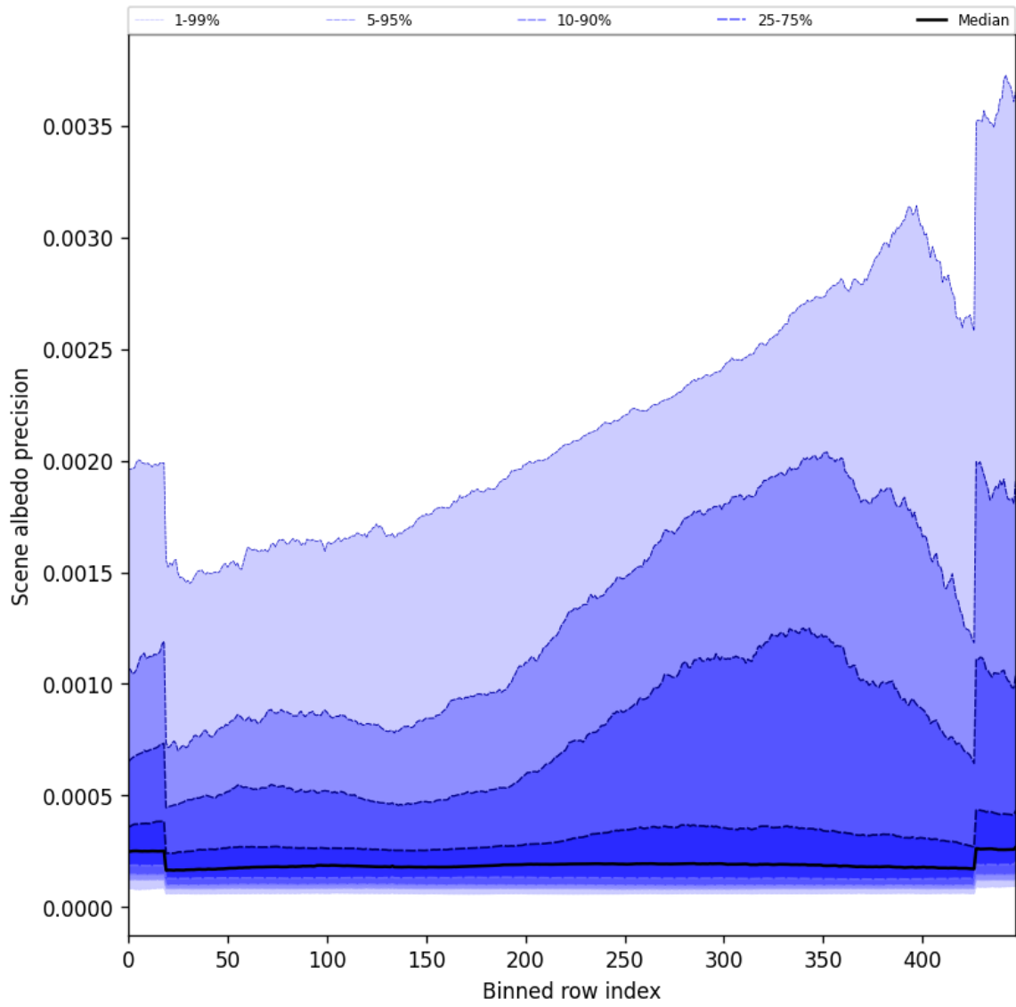
Figure 52: Along track statistics of “Scene albedo precision” for 2024-09-15 to 2024-09-17
