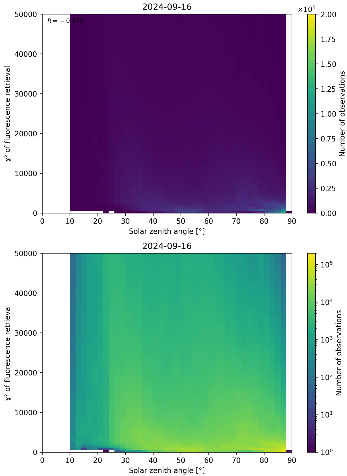
Figure 120: Scatter density plot of “Solar zenith angle” against “ \chi^2 of fluorescence retrieval” for 2024-09-15 to 2024-09-17.
