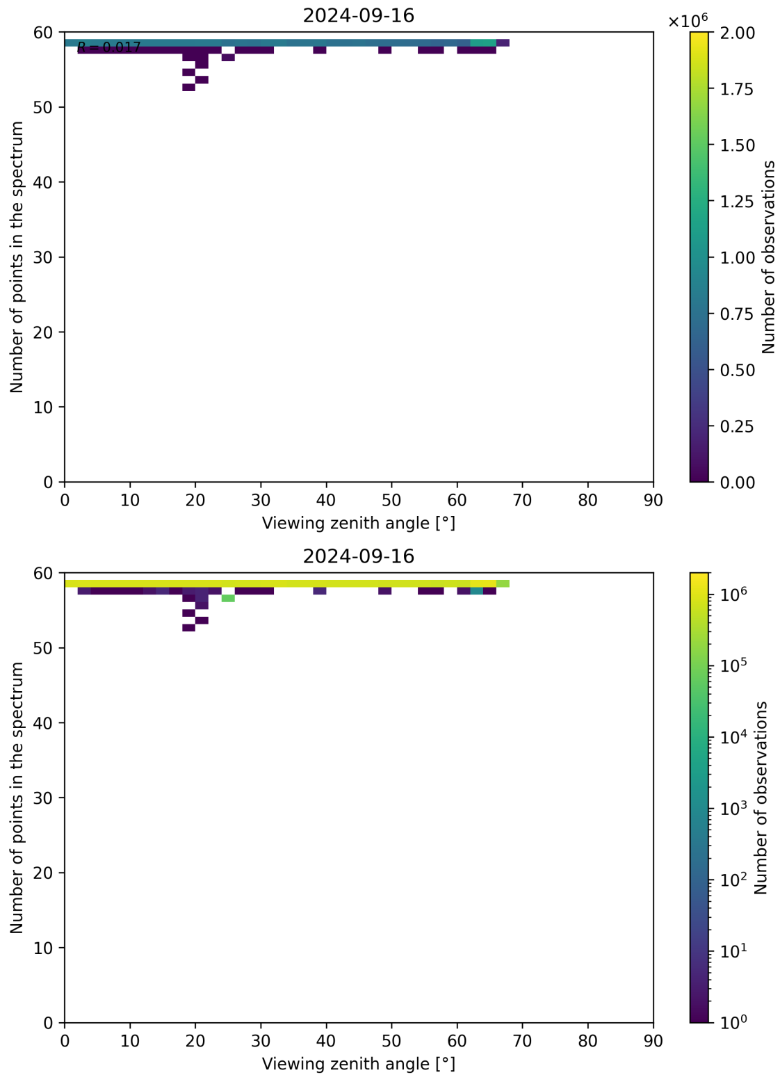
Figure 137: Scatter density plot of “Viewing zenith angle” against “Number of points in the spectrum” for 2024-09-15 to 2024-09-17.
