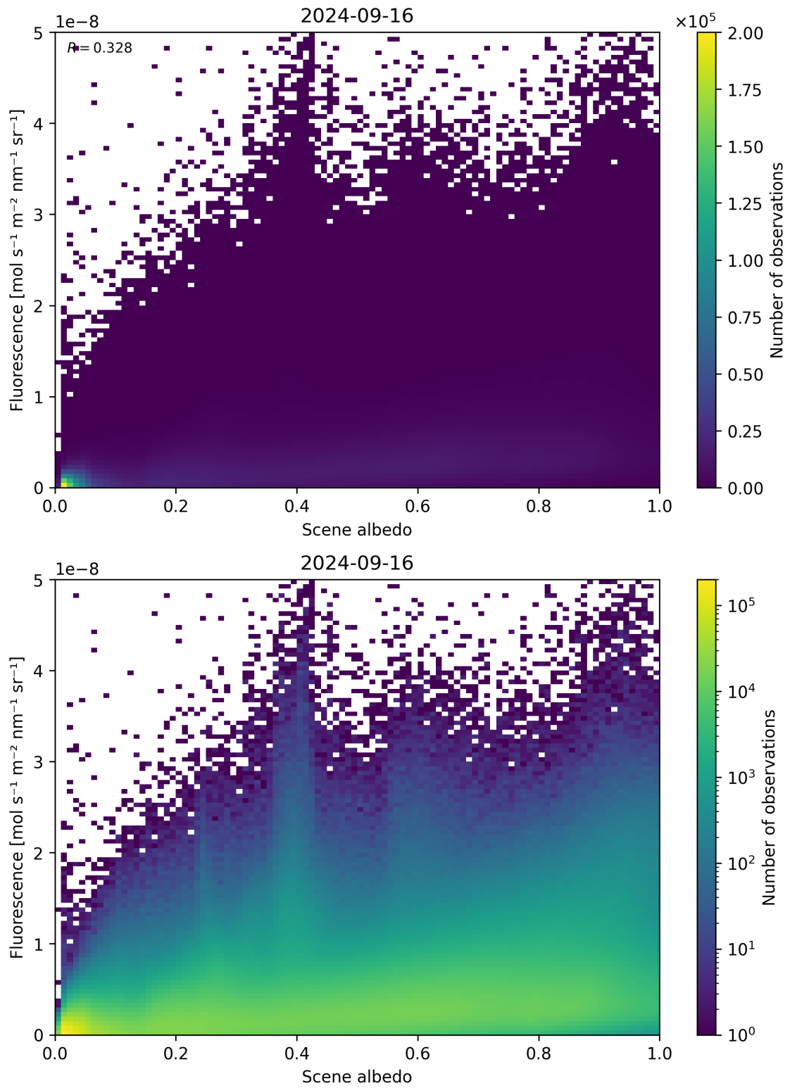
Figure 114: Scatter density plot of “Scene albedo” against “Fluorescence” for 2024-09-15 to 2024-09-17.
