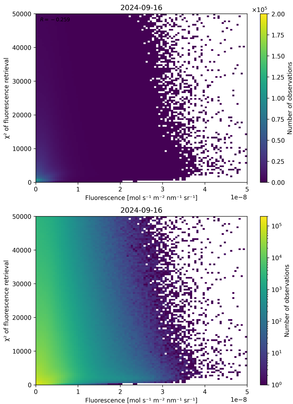
Figure 93: Scatter density plot of “Fluorescence” against “ \chi^2 of fluorescence retrieval” for 2024-09-15 to 2024-09-17.
