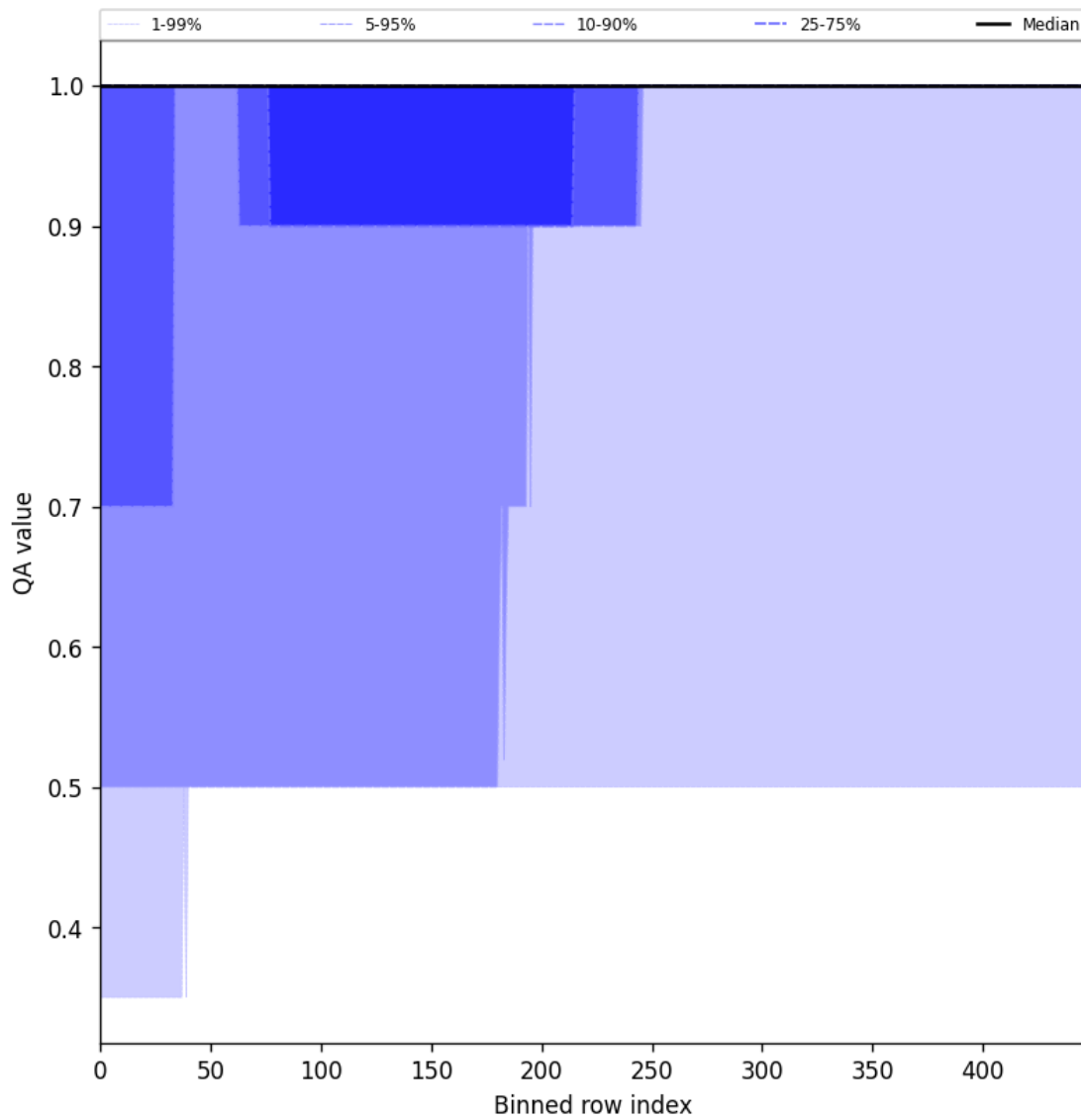
Figure 46: Along track statistics of “QA value” for 2024-09-15 to 2024-09-17
