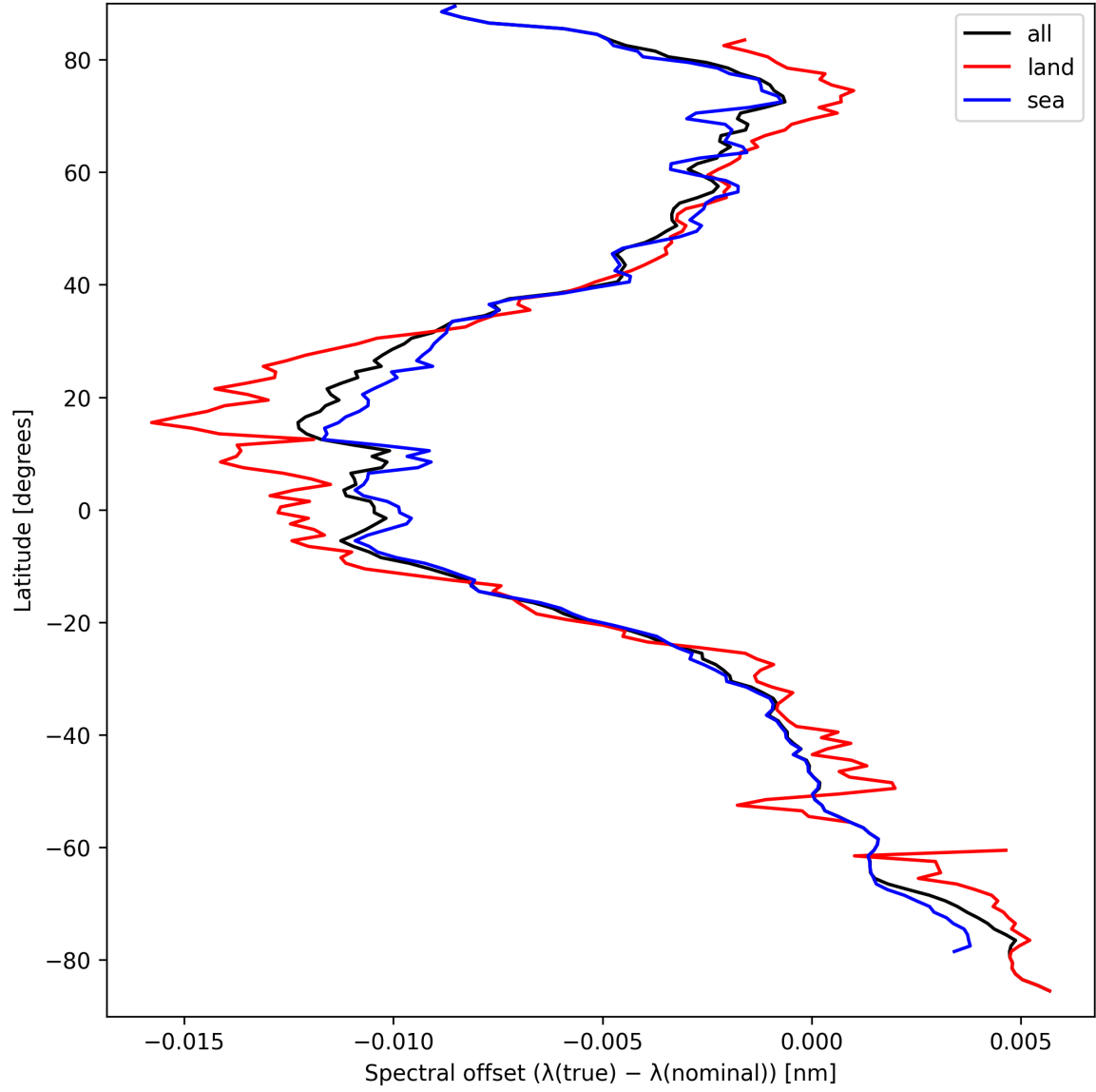
Figure 28: Zonal average of “Spectral offset ( \lambda_{\text{true}} - \lambda_{\text{nominal}} )” for 2024-09-15 to 2024-09-17.
