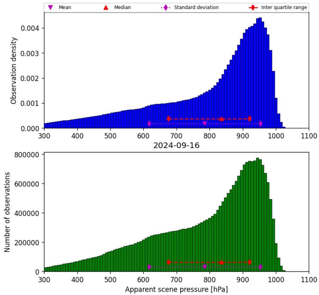
Figure 36: Histogram of “Apparent scene pressure” for 2024-09-15 to 2024-09-17
