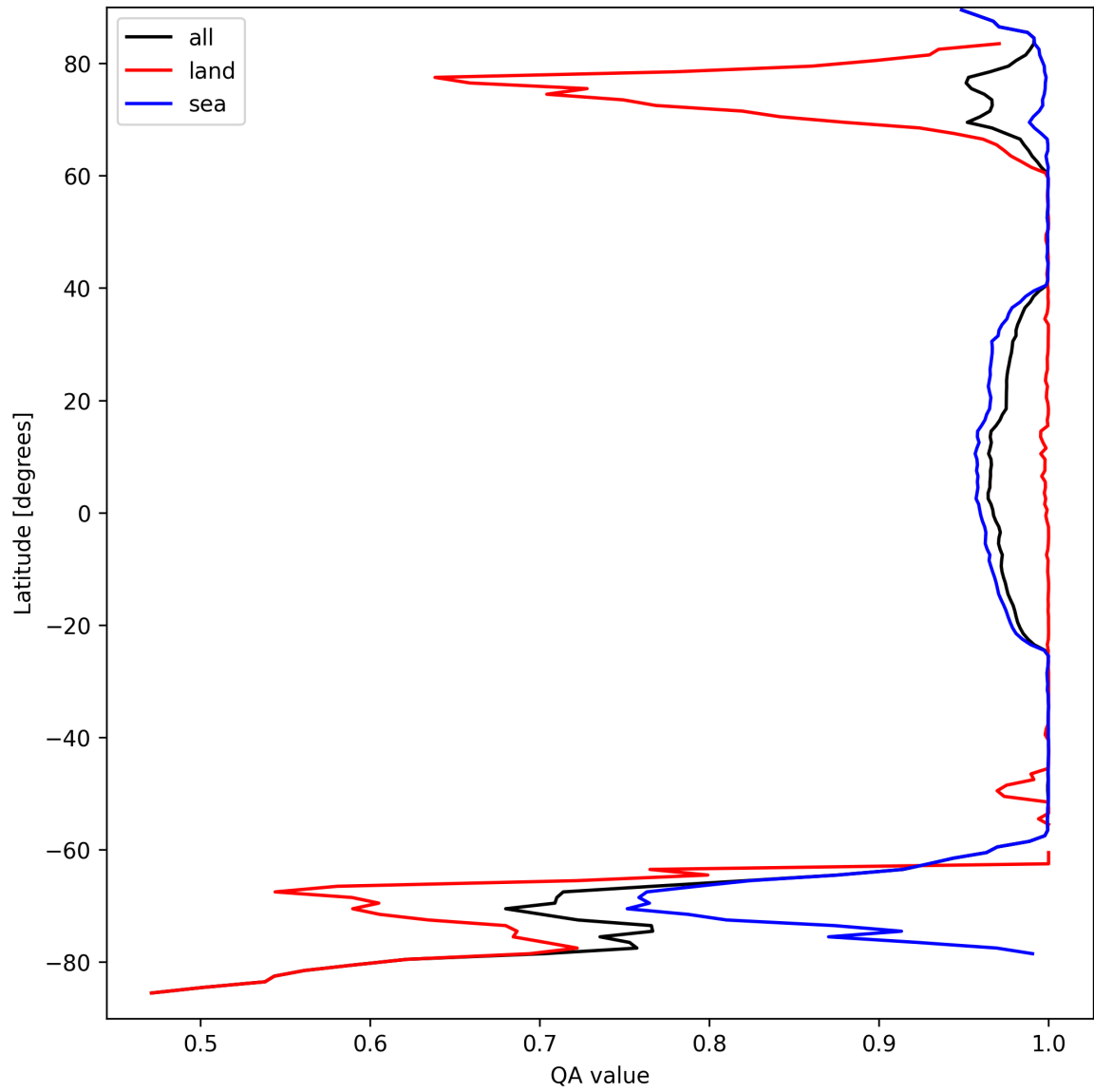
Figure 12: Zonal average of "QA value" for 2024-09-15 to 2024-09-17.
