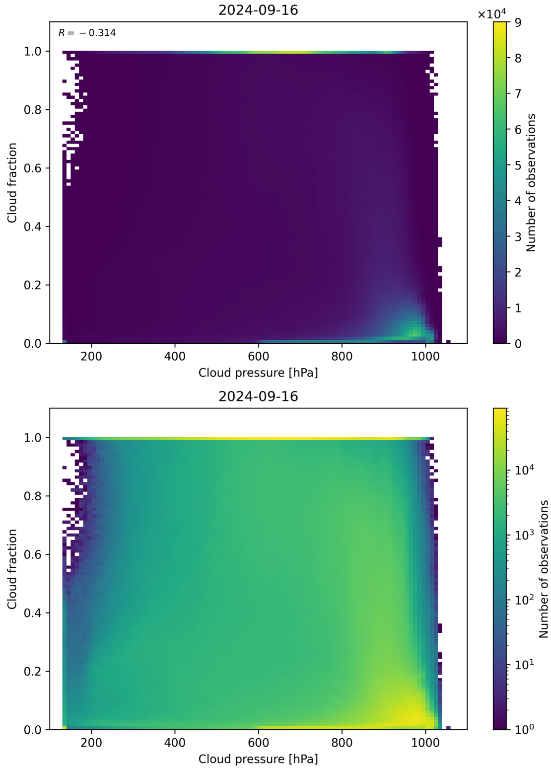
Figure 87: Scatter density plot of “Cloud pressure” against “Cloud fraction” for 2024-09-15 to 2024-09-17.
