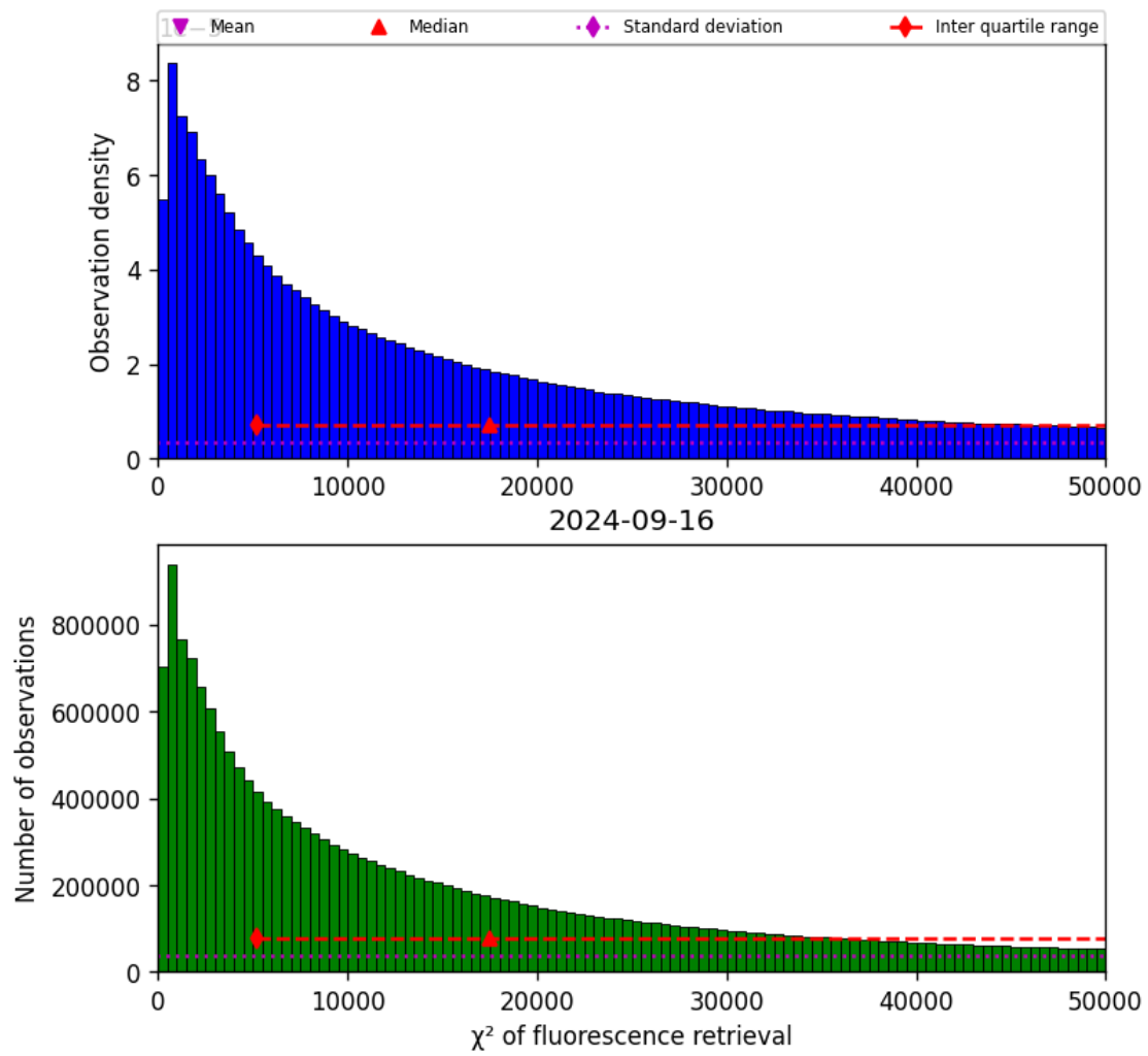
Figure 42: Histogram of “ \chi^2 of fluorescence retrieval” for 2024-09-15 to 2024-09-17
