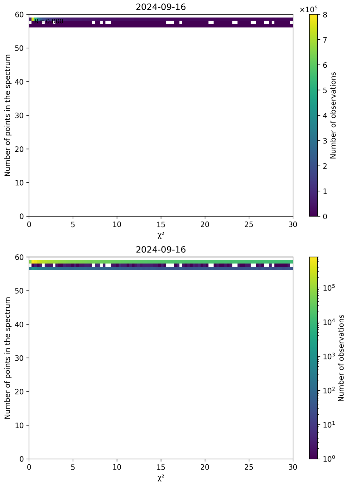
Figure 74: Scatter density plot of “ \chi^2 ” against “Number of points in the spectrum” for 2024-09-15 to 2024-09-17.
