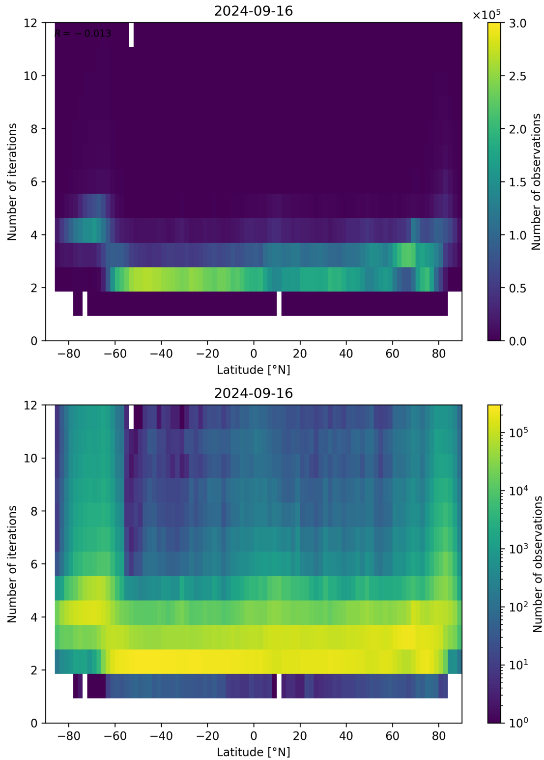
Figure 102: Scatter density plot of “Latitude” against “Number of iterations” for 2024-09-15 to 2024-09-17.
