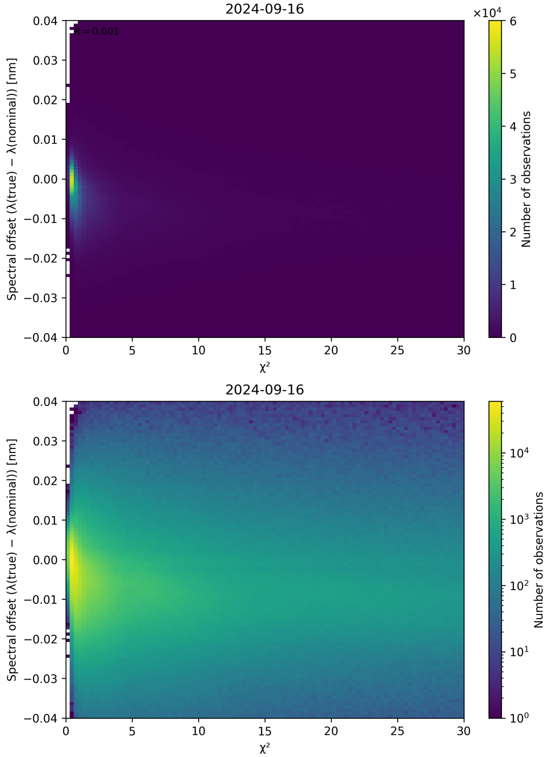
Figure 75: Scatter density plot of “ \chi^2 ” against “Spectral offset ( \lambda_{\text{true}} - \lambda_{\text{nominal}} )” for 2024-09-15 to 2024-09-17.
