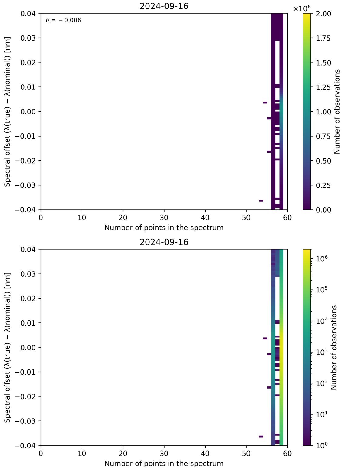
Figure 110: Scatter density plot of “Number of points in the spectrum” against “Spectral offset ( \lambda_{\text{true}} - \lambda_{\text{nominal}} )” for 2024-09-15 to 2024-09-17.
