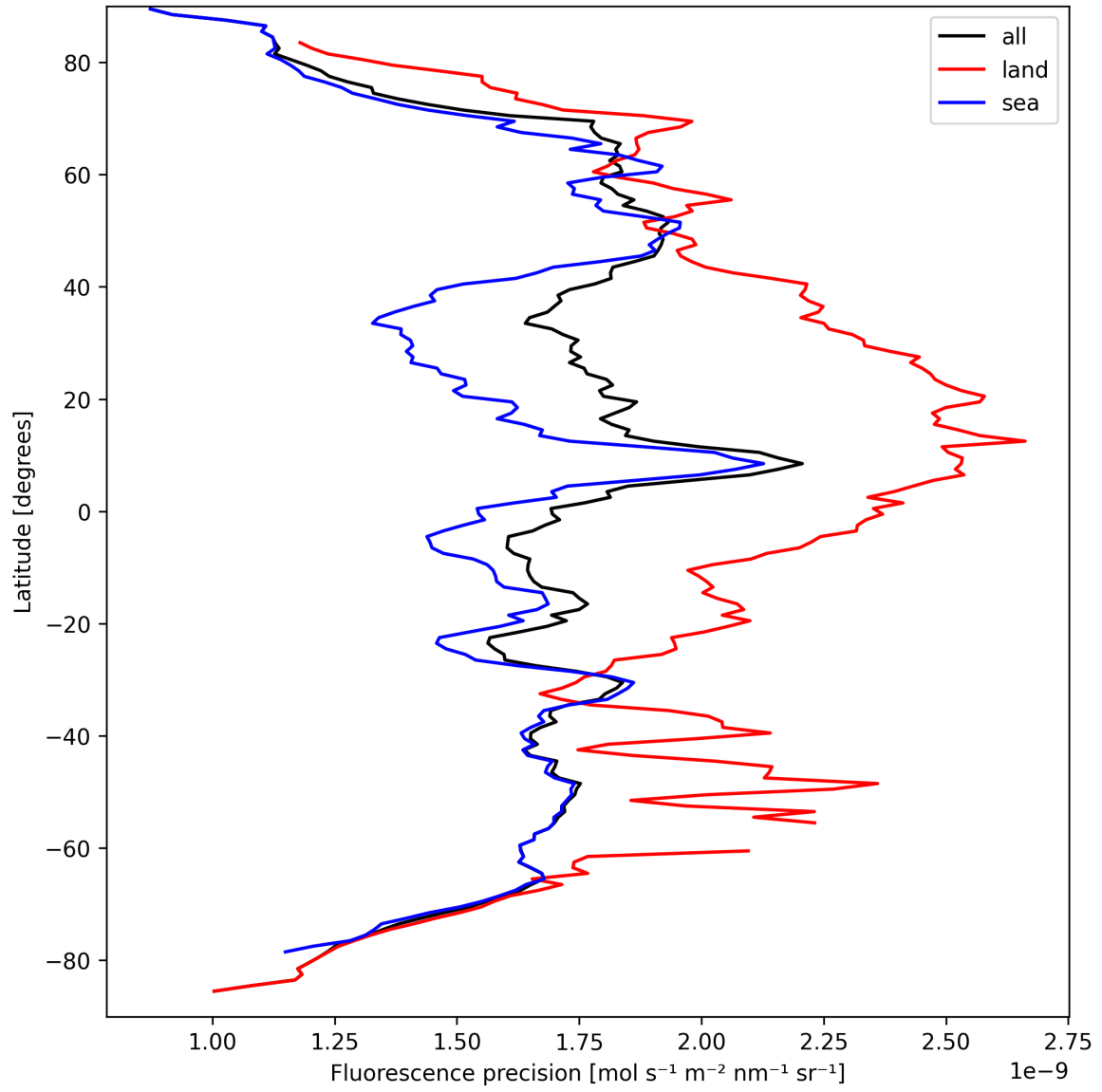
Figure 24: Zonal average of “Fluorescence precision” for 2024-09-15 to 2024-09-17.
