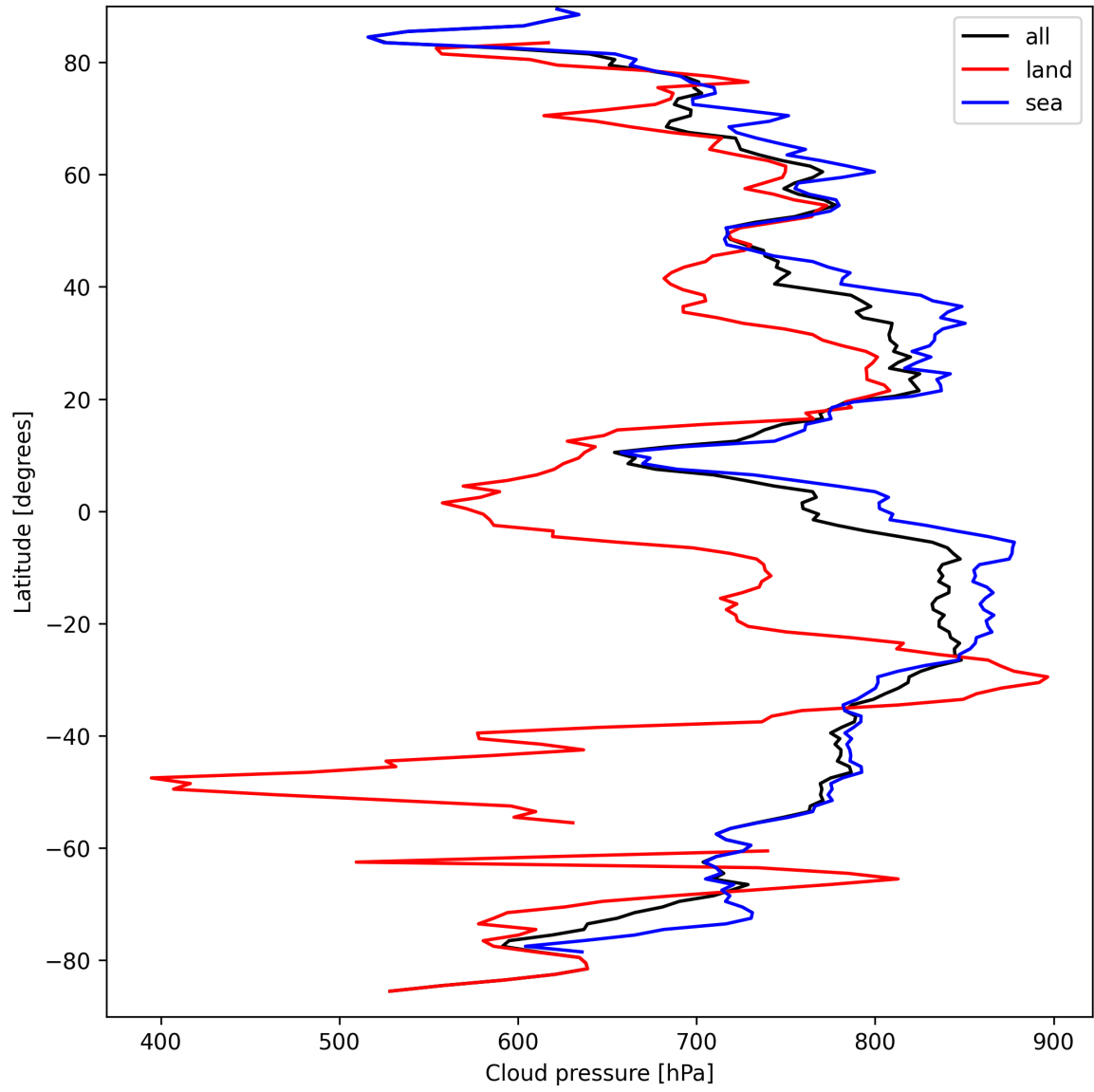
Figure 13: Zonal average of “Cloud pressure” for 2024-09-15 to 2024-09-17.
