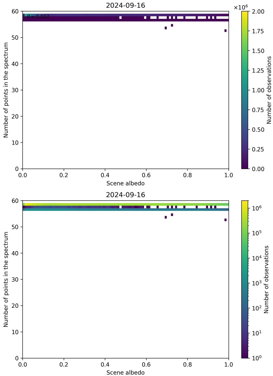
Figure 116: Scatter density plot of “Scene albedo” against “Number of points in the spectrum” for 2024-09-15 to 2024-09-17.
