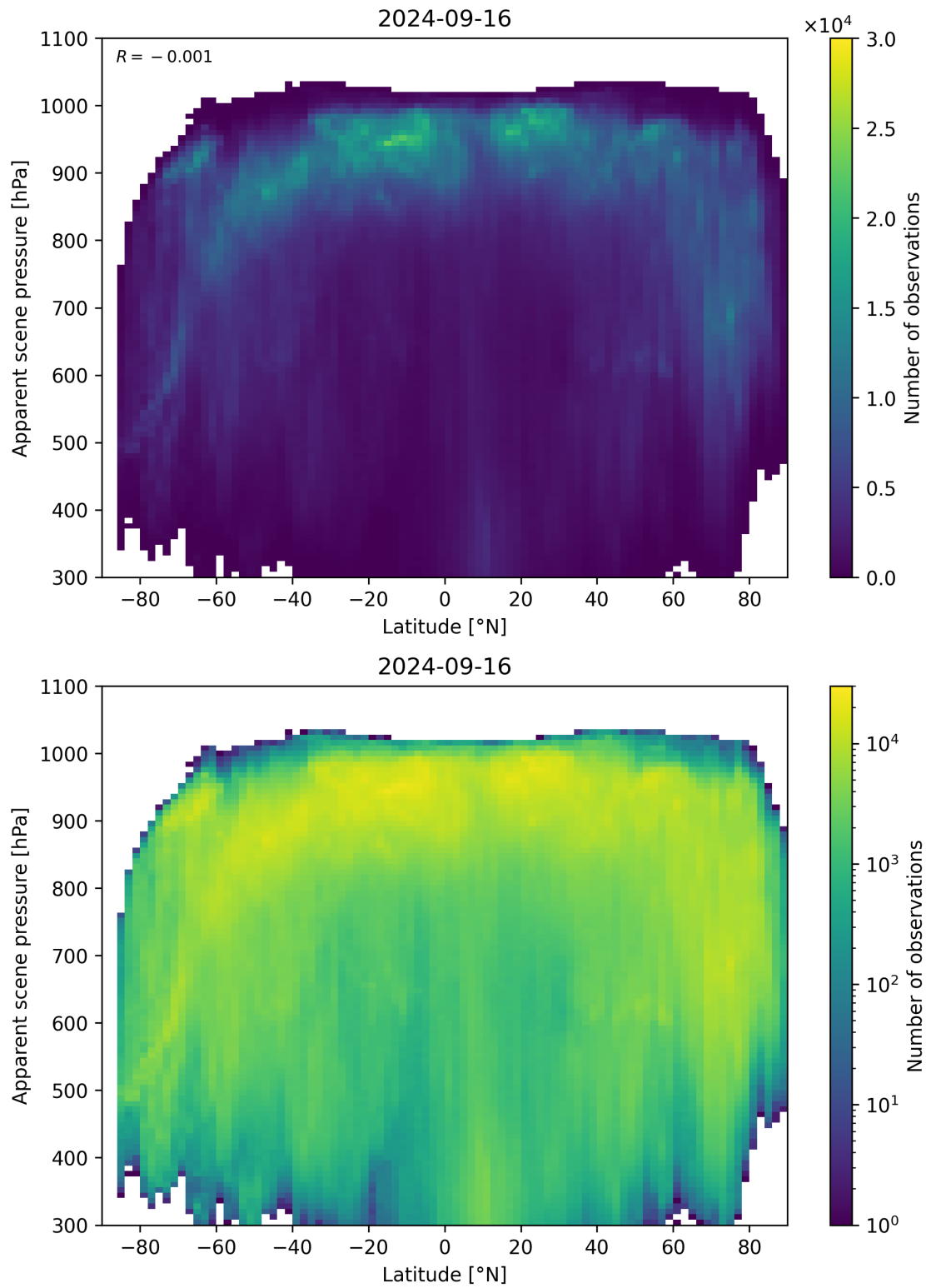
Figure 96: Scatter density plot of “Latitude” against “Apparent scene pressure” for 2024-09-15 to 2024-09-17.
