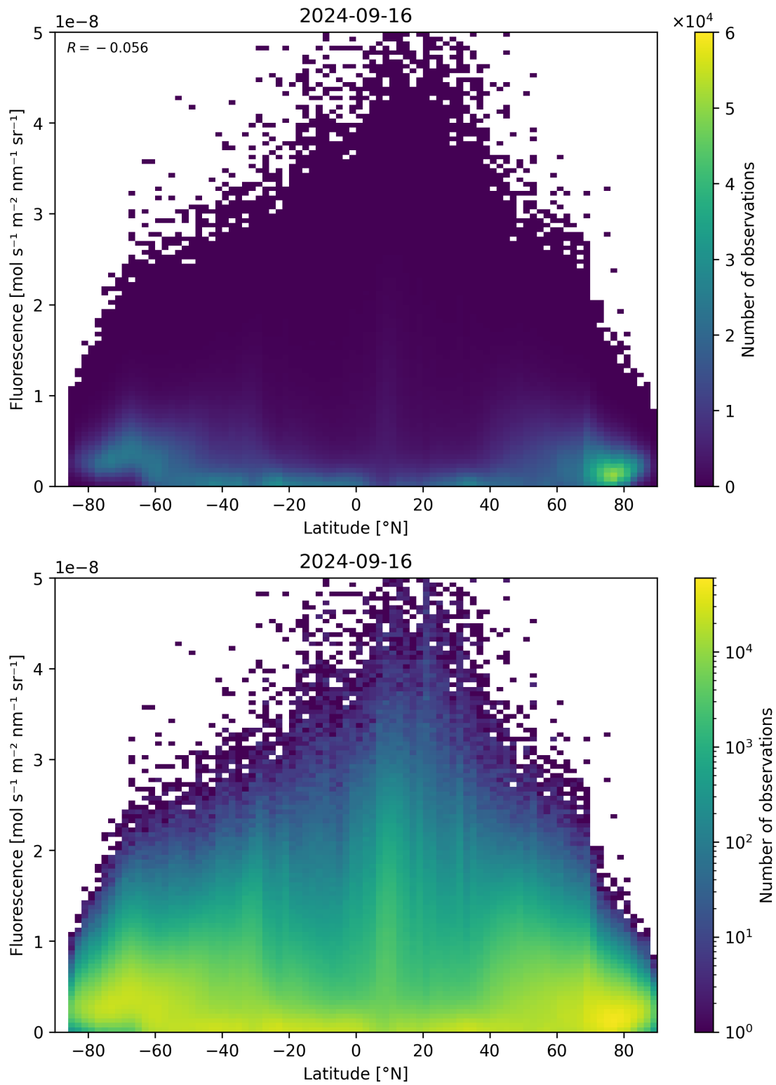
Figure 101: Scatter density plot of “Latitude” against “Fluorescence” for 2024-09-15 to 2024-09-17.
