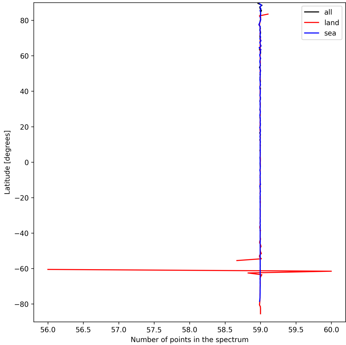
Figure 27: Zonal average of “Number of points in the spectrum” for 2024-09-15 to 2024-09-17.
