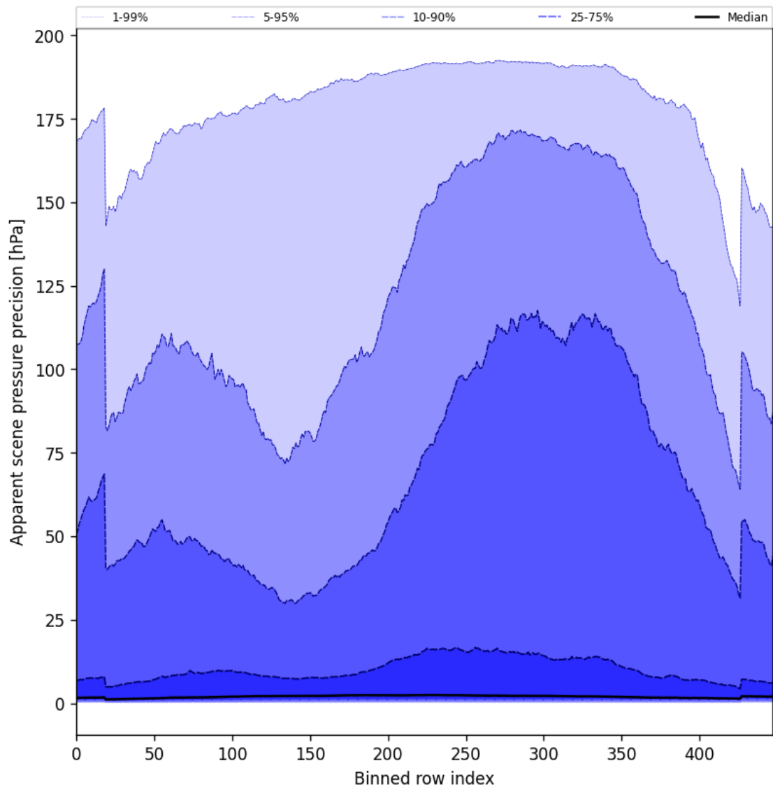
Figure 54: Along track statistics of “Apparent scene pressure precision” for 2024-09-15 to 2024-09-17
