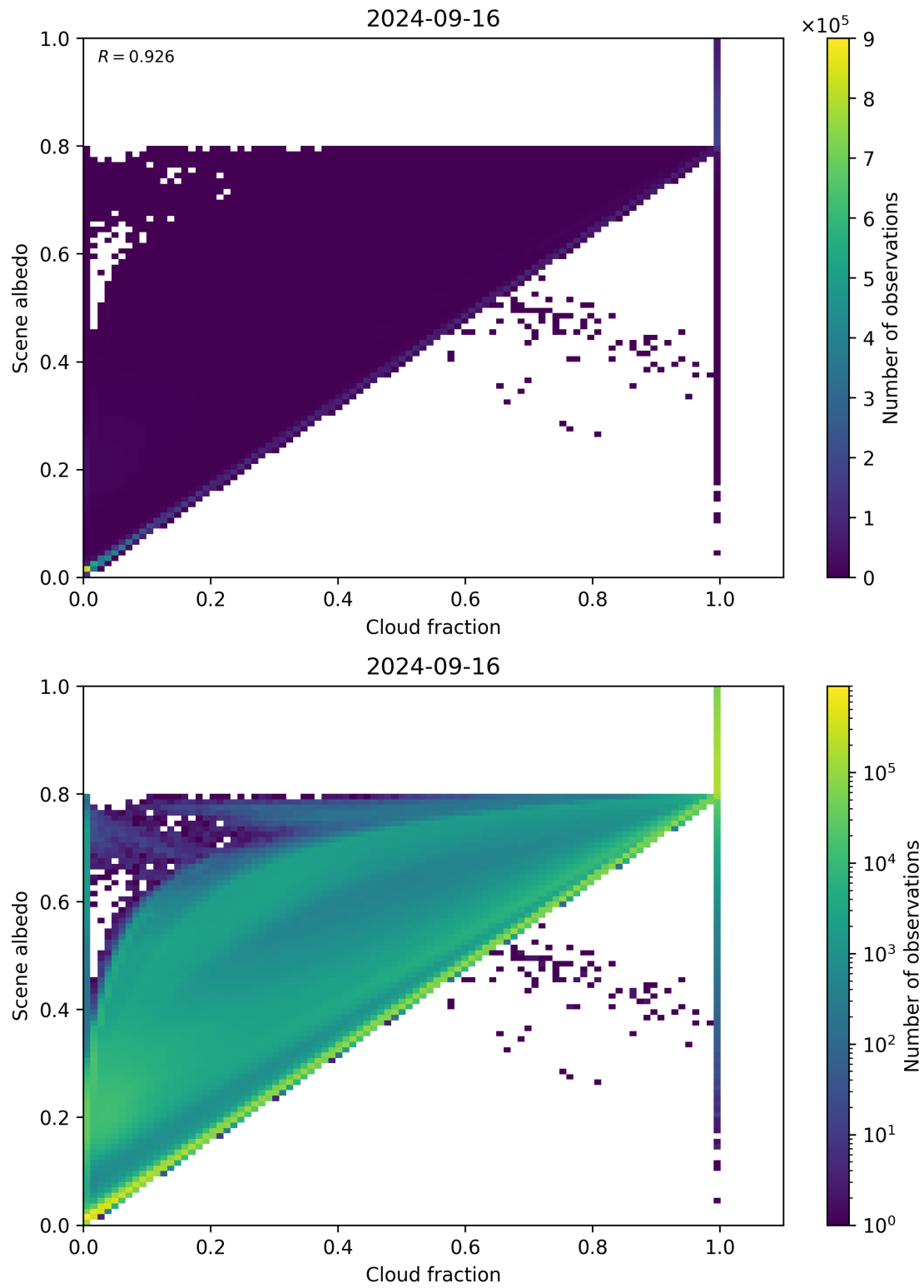
Figure 82: Scatter density plot of “Cloud fraction” against “Scene albedo” for 2024-09-15 to 2024-09-17.
