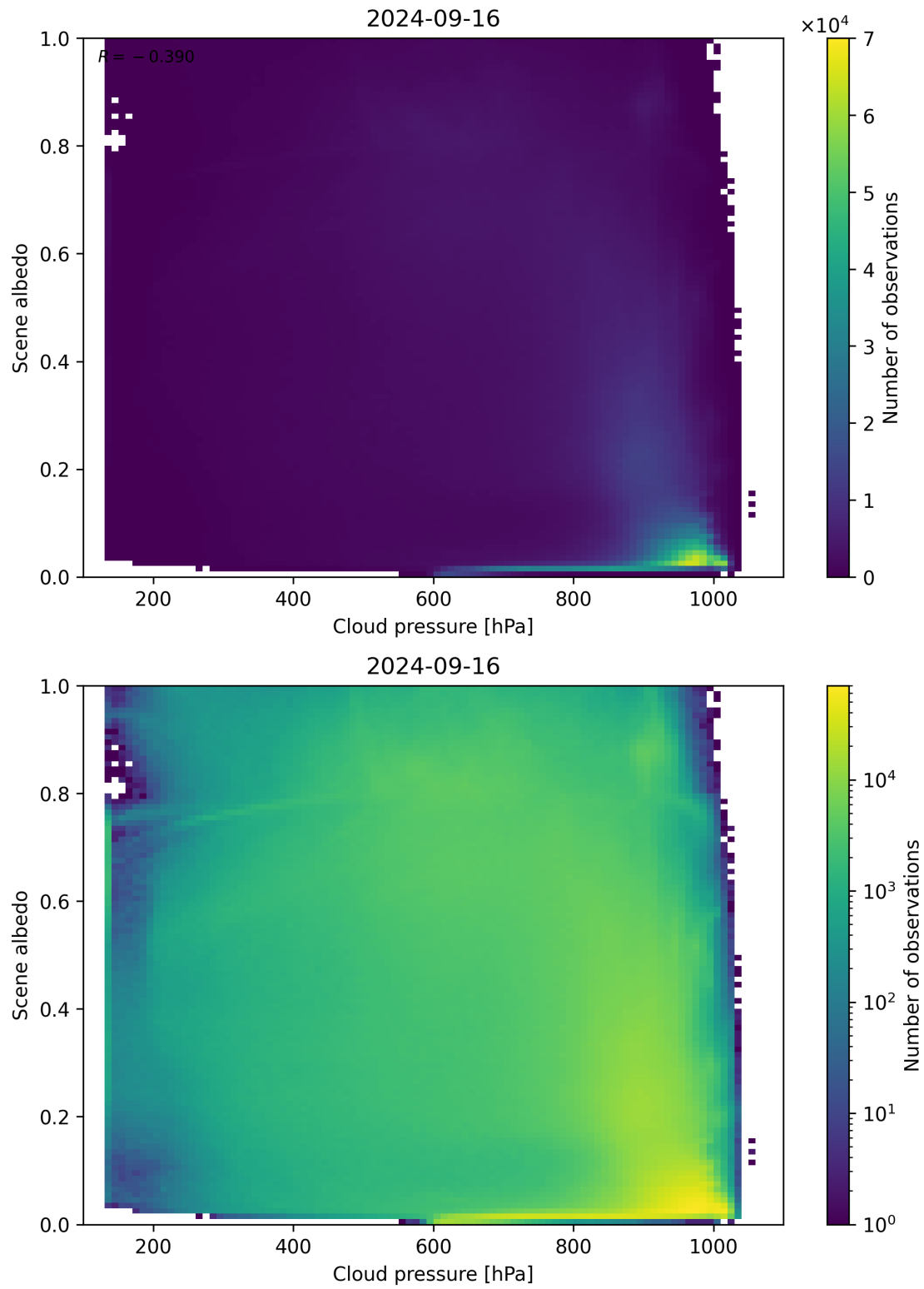
Figure 91: Scatter density plot of “Cloud pressure” against “Scene albedo” for 2024-09-15 to 2024-09-17.
