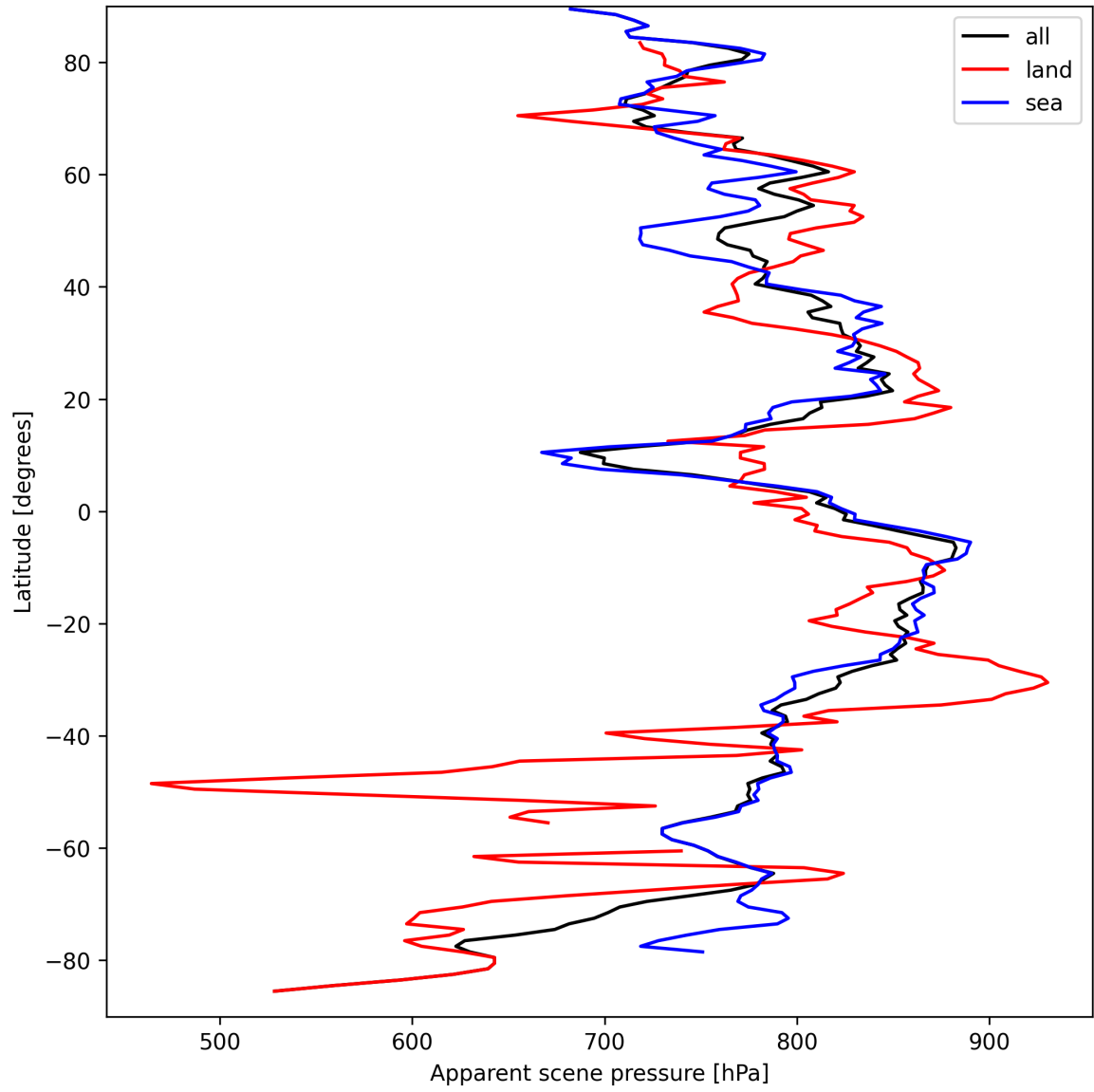
Figure 19: Zonal average of “Apparent scene pressure” for 2024-09-15 to 2024-09-17.
