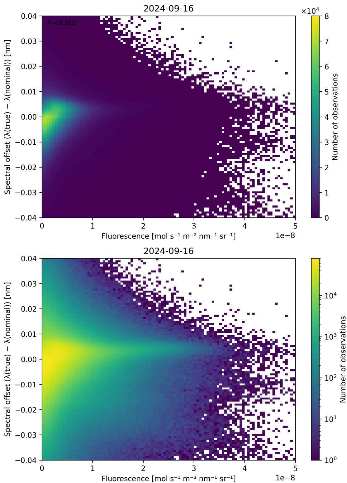
Figure 95: Scatter density plot of “Fluorescence” against “Spectral offset ( \lambda_{\text{true}} - \lambda_{\text{nominal}} )” for 2024-09-15 to 2024-09-17.
