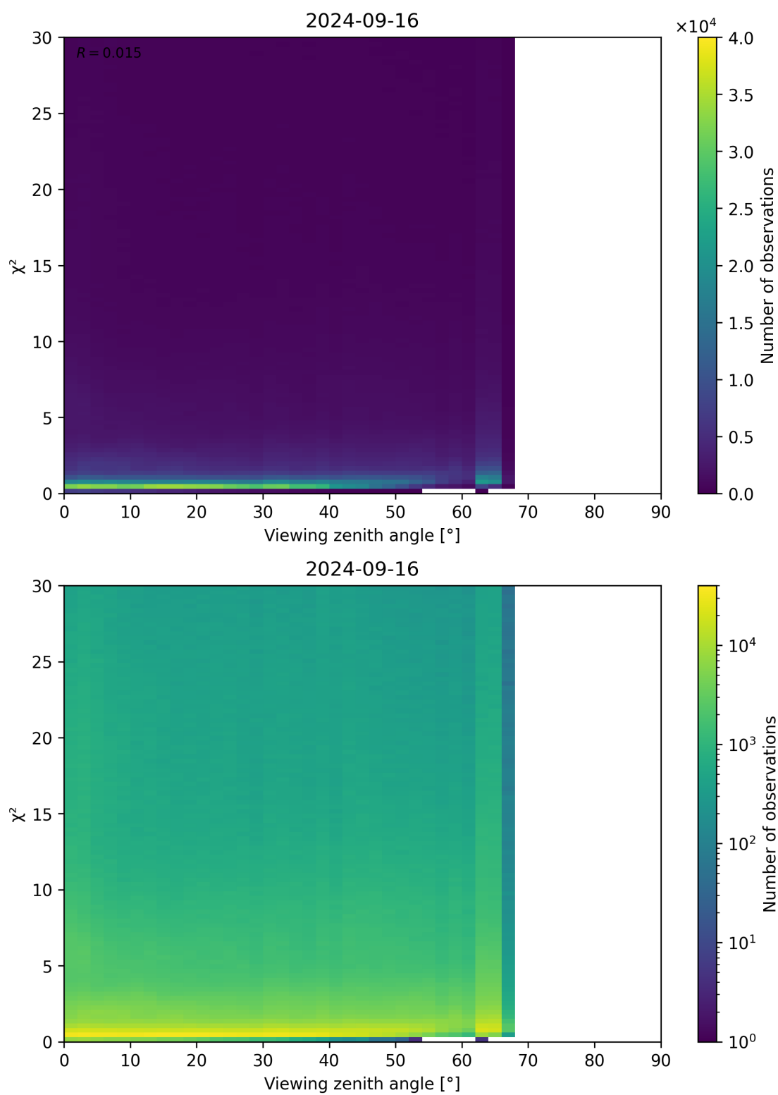
Figure 130: Scatter density plot of “Viewing zenith angle” against “ \chi^2 ” for 2024-09-15 to 2024-09-17.
