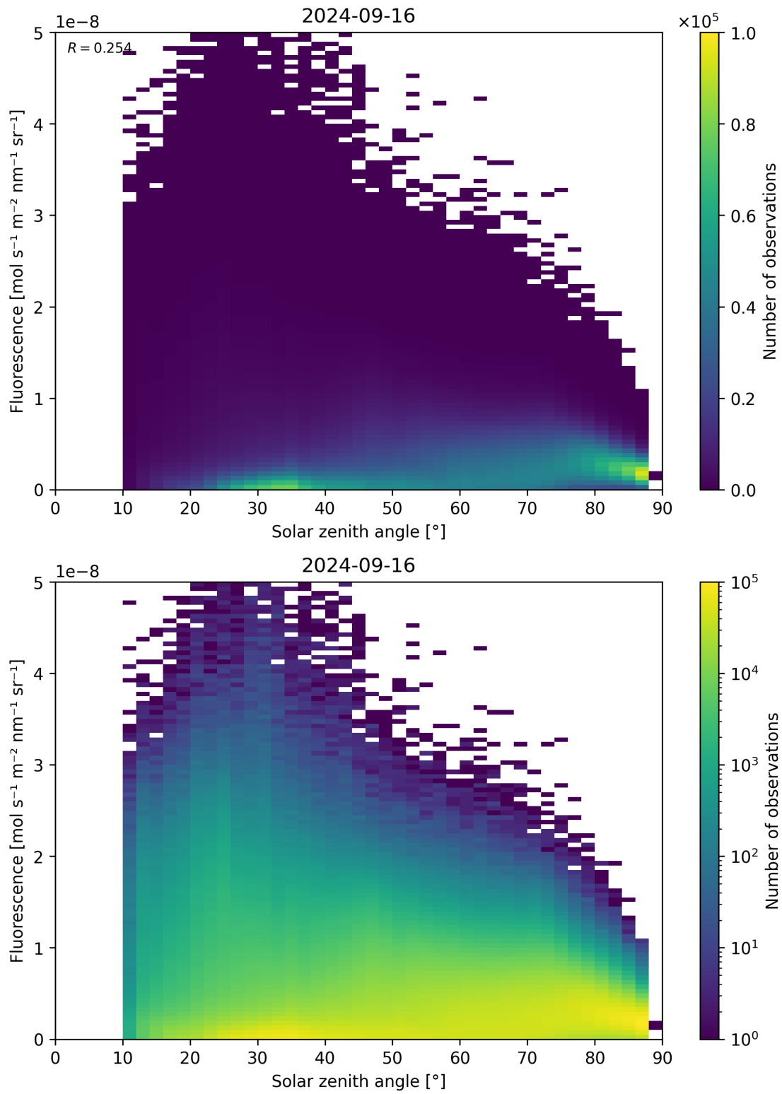
Figure 123: Scatter density plot of “Solar zenith angle” against “Fluorescence” for 2024-09-15 to 2024-09-17.
