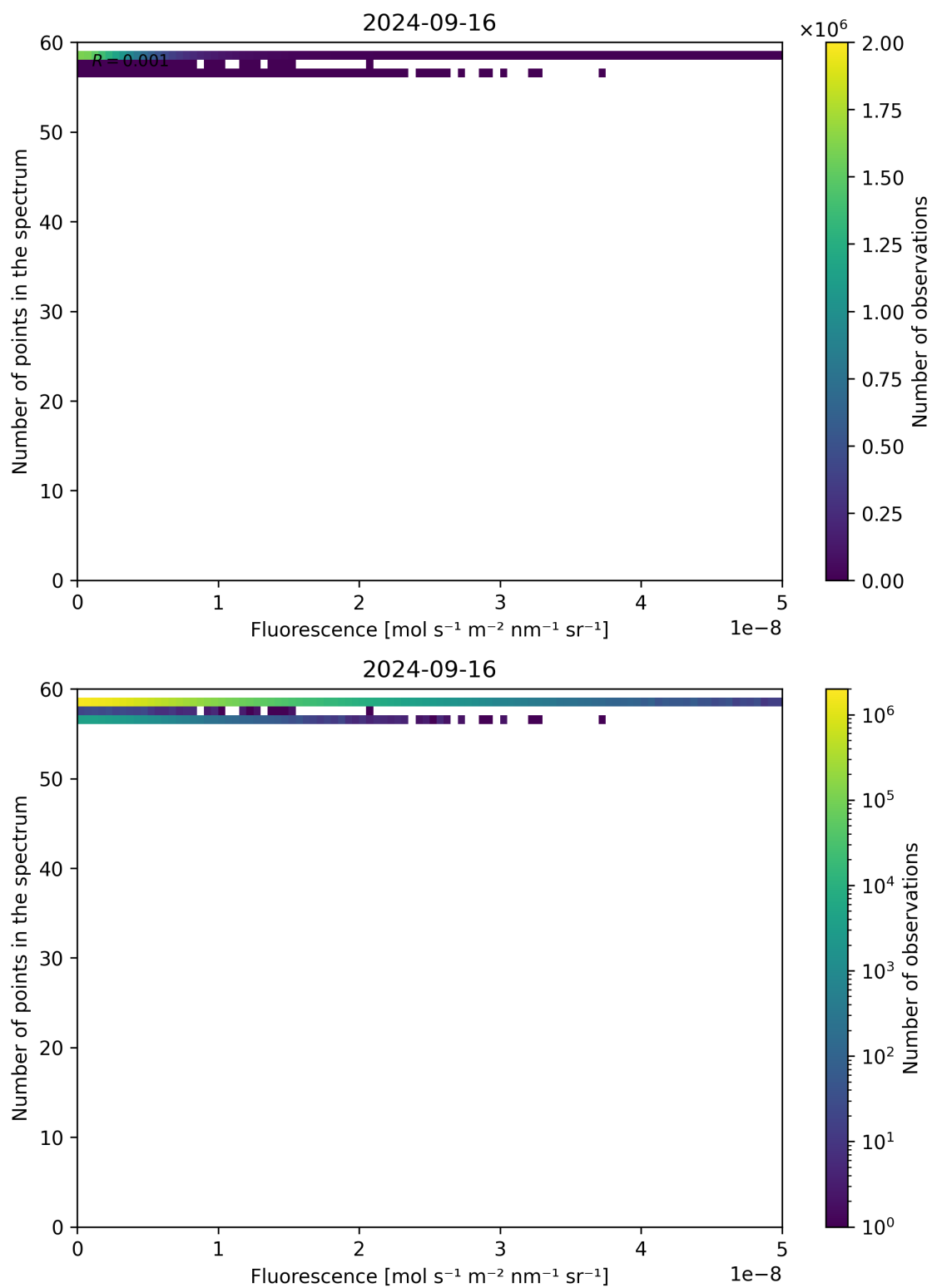
Figure 94: Scatter density plot of “Fluorescence” against “Number of points in the spectrum” for 2024-09-15 to 2024-09-17.
