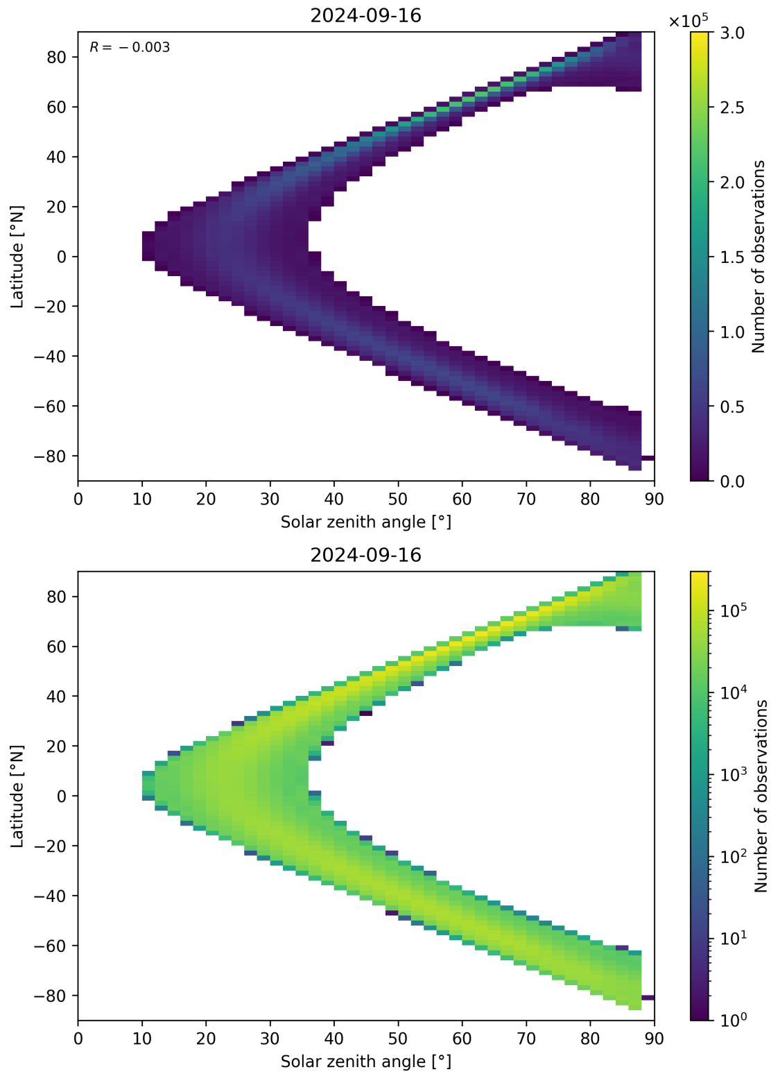
Figure 124: Scatter density plot of “Solar zenith angle” against “Latitude” for 2024-09-15 to 2024-09-17.
