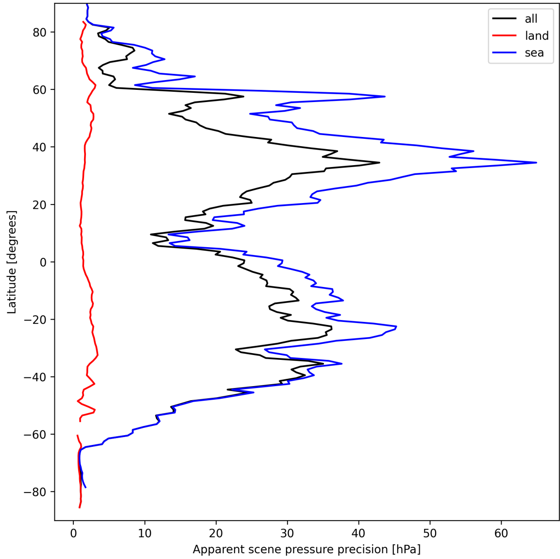
Figure 20: Zonal average of “Apparent scene pressure precision” for 2024-09-15 to 2024-09-17.
