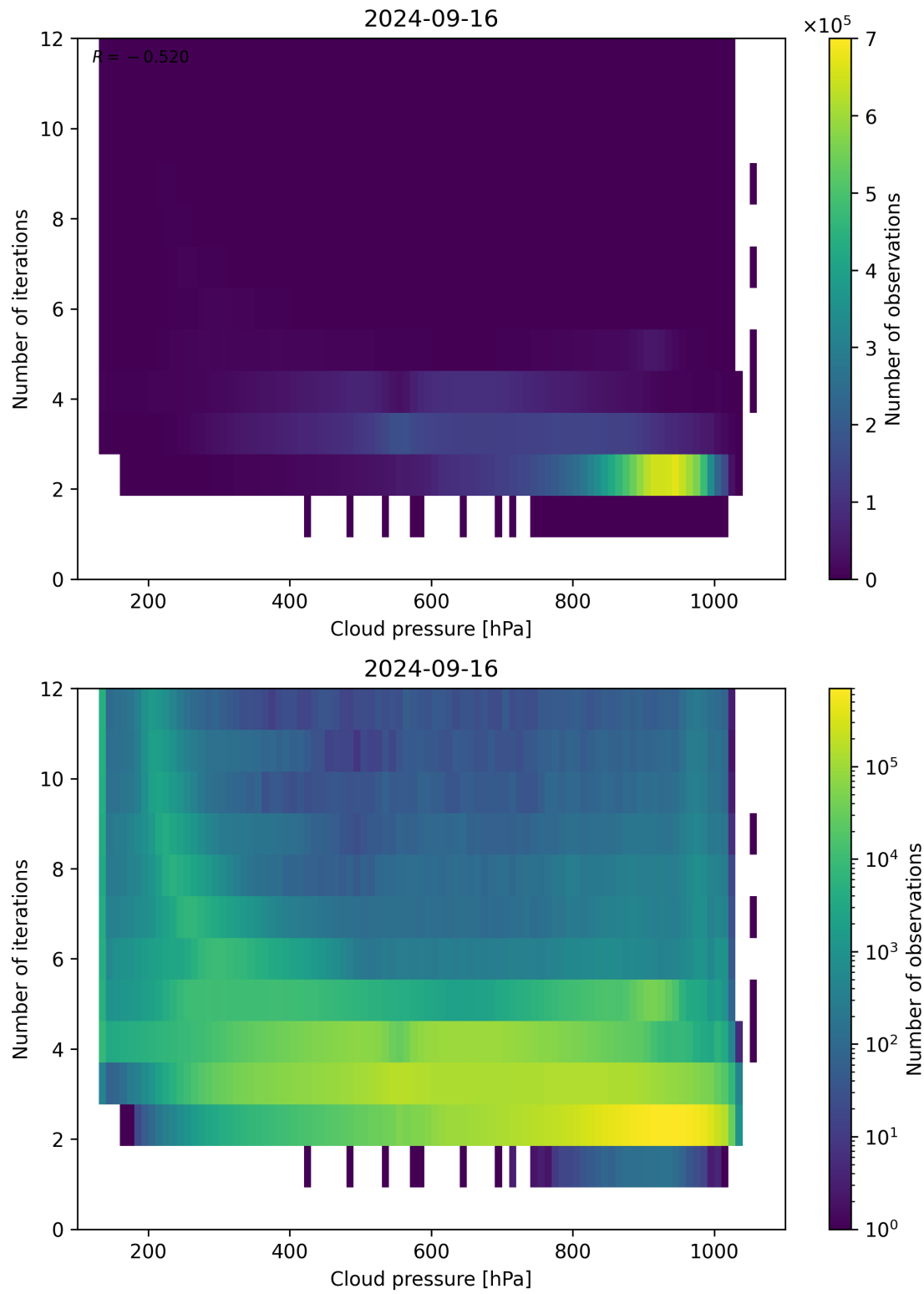
Figure 89: Scatter density plot of “Cloud pressure” against “Number of iterations” for 2024-09-15 to 2024-09-17.
