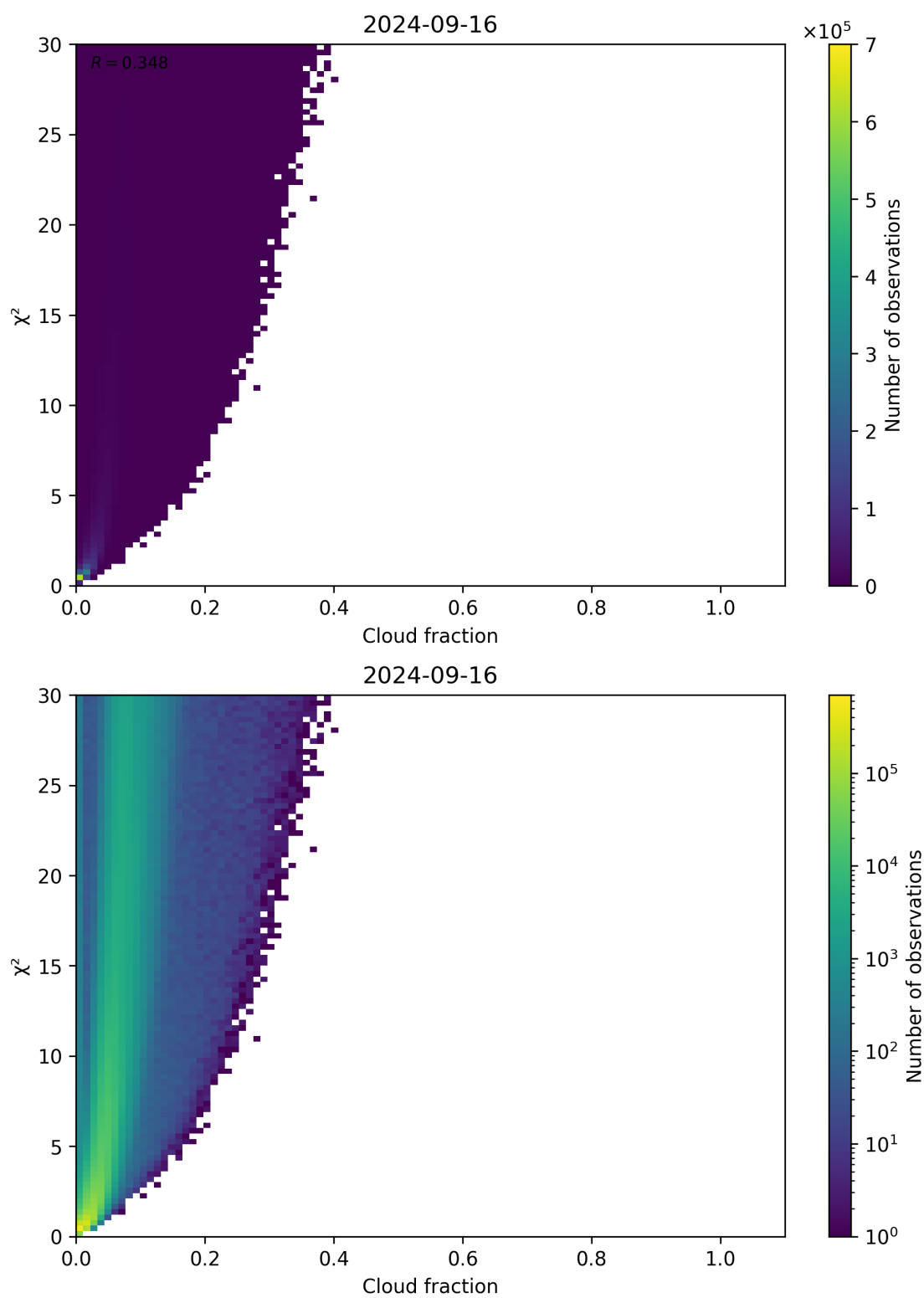
Figure 77: Scatter density plot of “Cloud fraction” against “ \chi^2 ” for 2024-09-15 to 2024-09-17.
