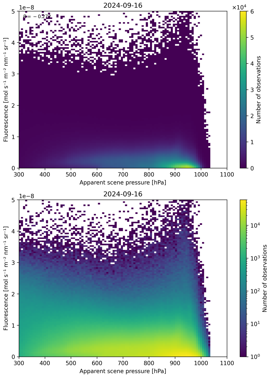
Figure 65: Scatter density plot of “Apparent scene pressure” against “Fluorescence” for 2024-09-15 to 2024-09-17.
