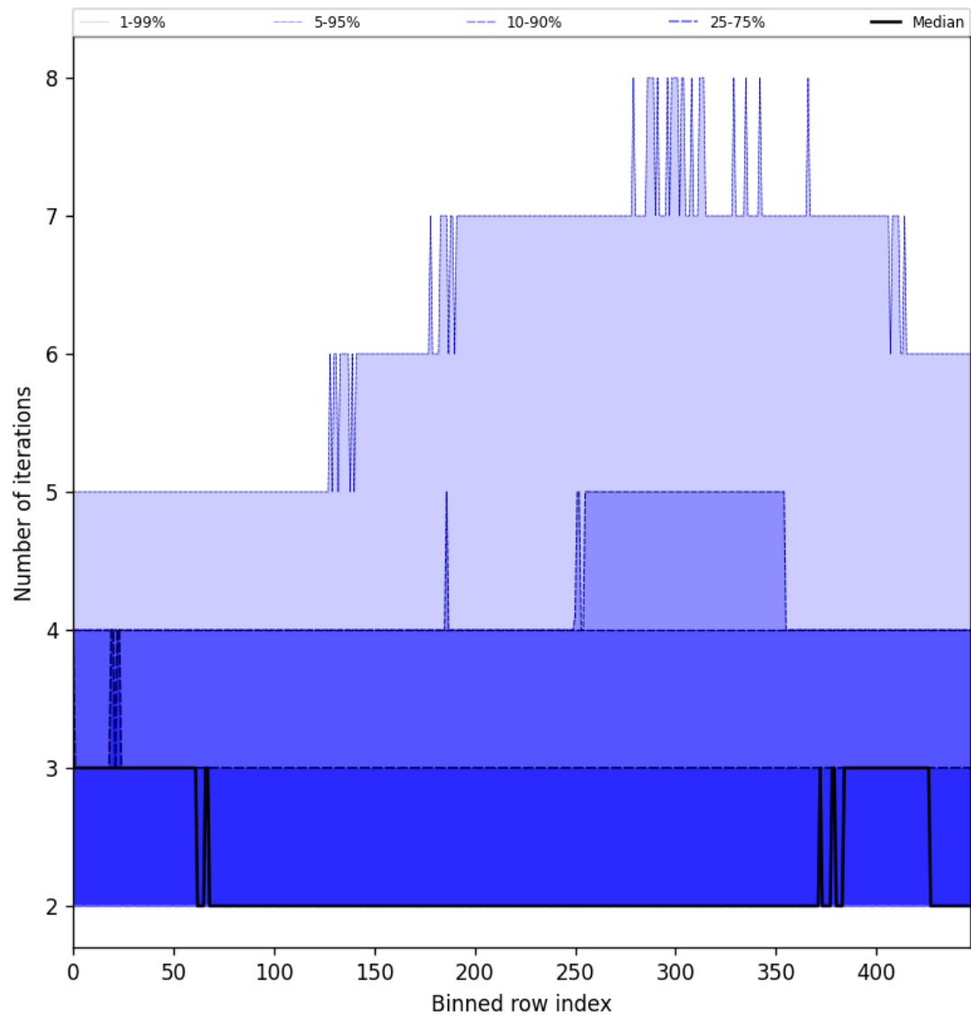
Figure 56: Along track statistics of “Number of iterations” for 2024-09-15 to 2024-09-17
