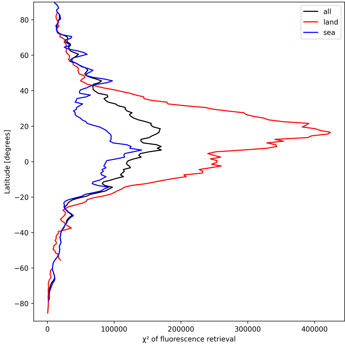
Figure 25: Zonal average of “ \chi^2 of fluorescence retrieval” for 2024-09-15 to 2024-09-17.
