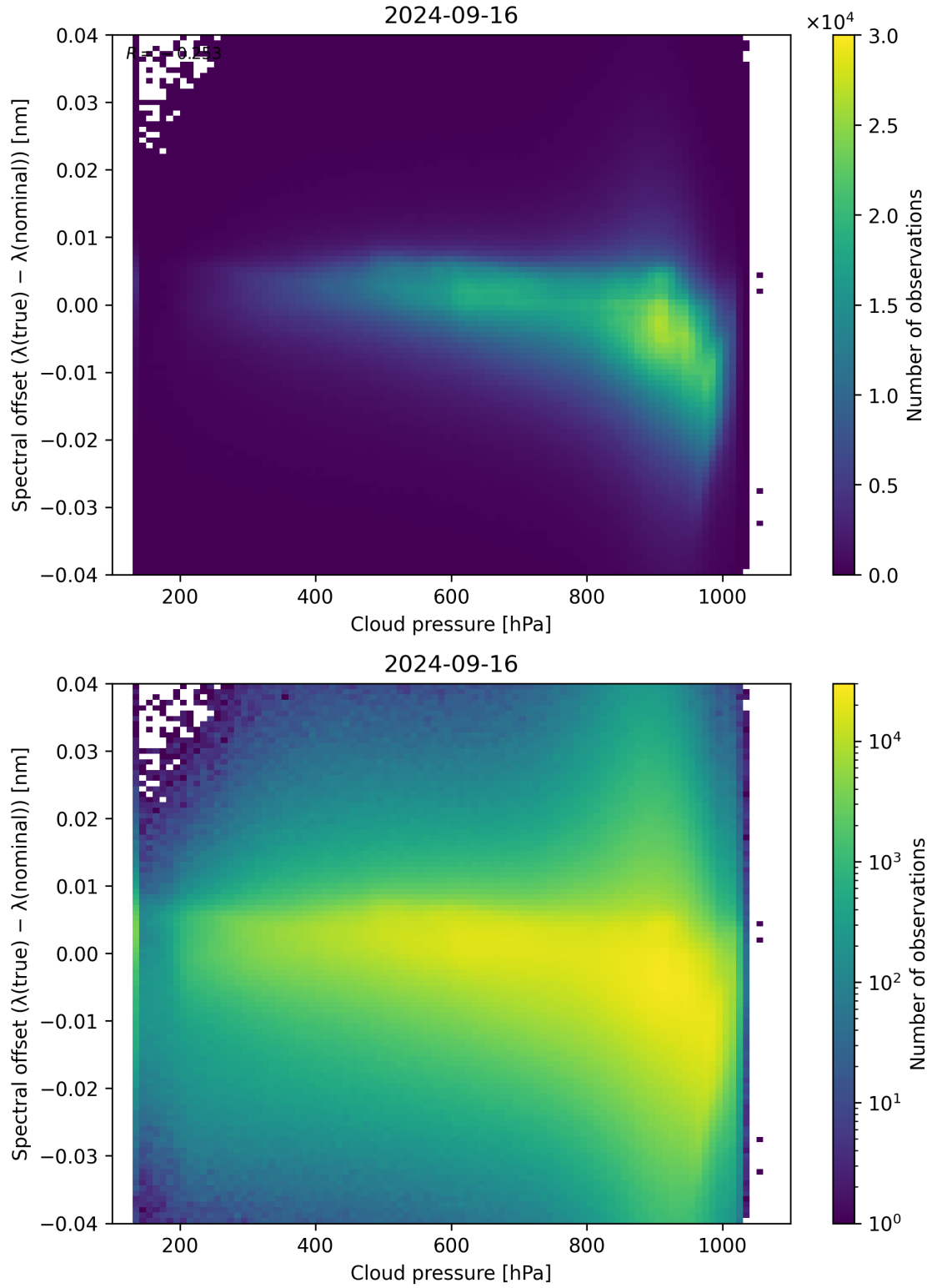
Figure 92: Scatter density plot of “Cloud pressure” against “Spectral offset ( \lambda_{\text{true}} - \lambda_{\text{nominal}} )” for 2024-09-15 to 2024-09-17.
