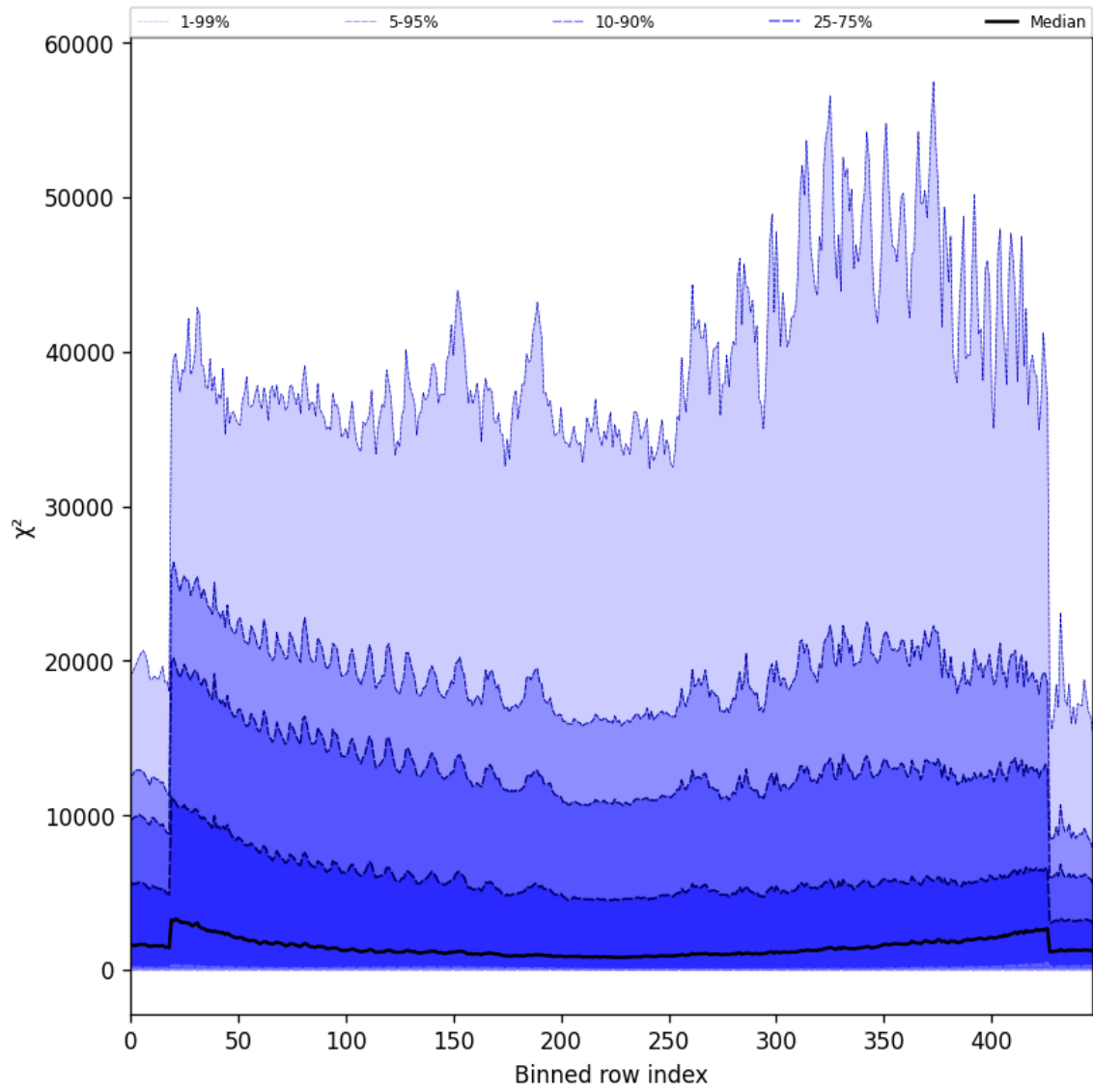
Figure 55: Along track statistics of “ \chi^2 ” for 2024-09-15 to 2024-09-17
