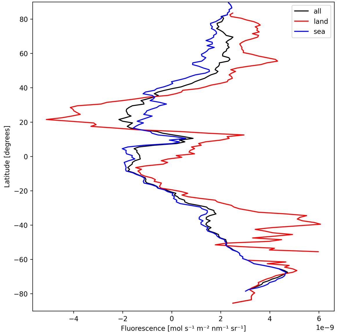
Figure 23: Zonal average of “Fluorescence” for 2024-09-15 to 2024-09-17.
