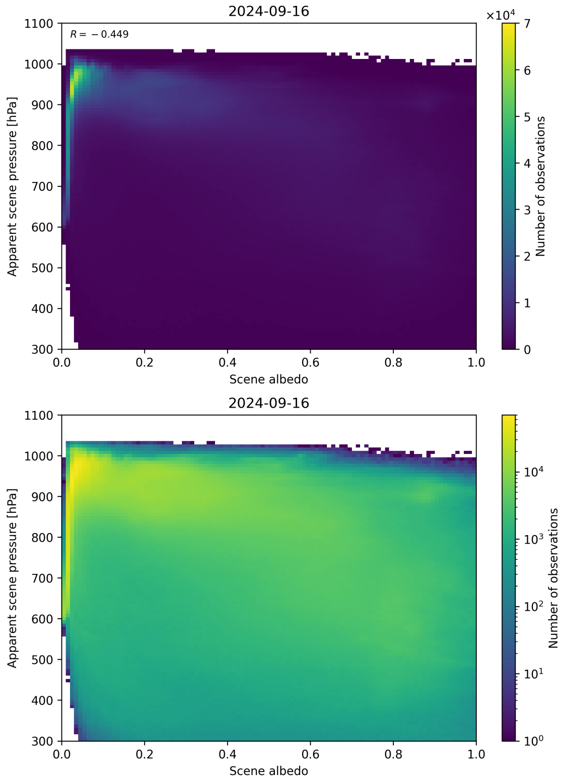
Figure 111: Scatter density plot of “Scene albedo” against “Apparent scene pressure” for 2024-09-15 to 2024-09-17.
