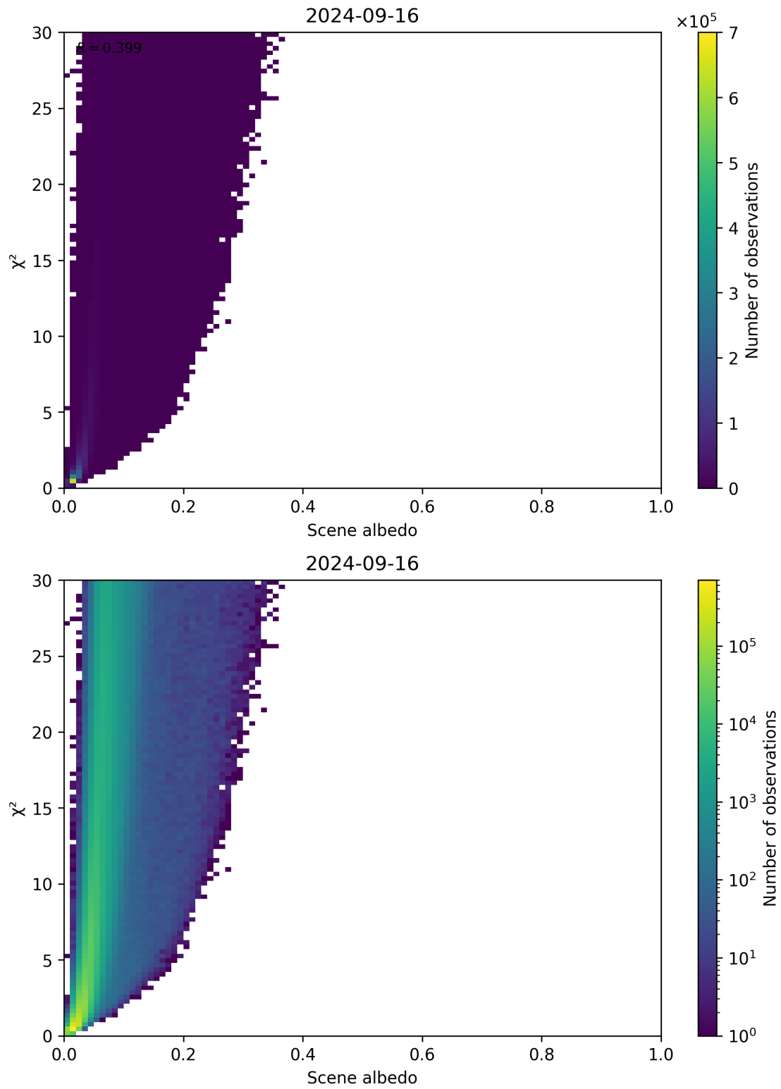
Figure 112: Scatter density plot of “Scene albedo” against “ \chi^2 ” for 2024-09-15 to 2024-09-17.
