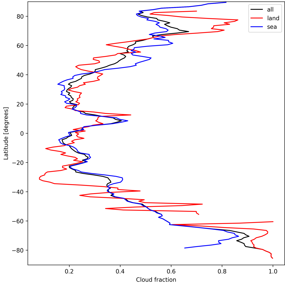
Figure 15: Zonal average of “Cloud fraction” for 2024-09-15 to 2024-09-17.
