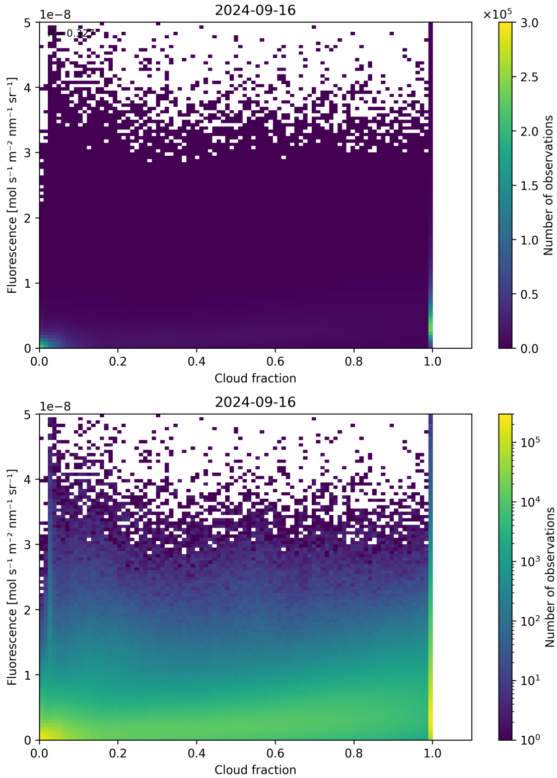
Figure 79: Scatter density plot of “Cloud fraction” against “Fluorescence” for 2024-09-15 to 2024-09-17.
