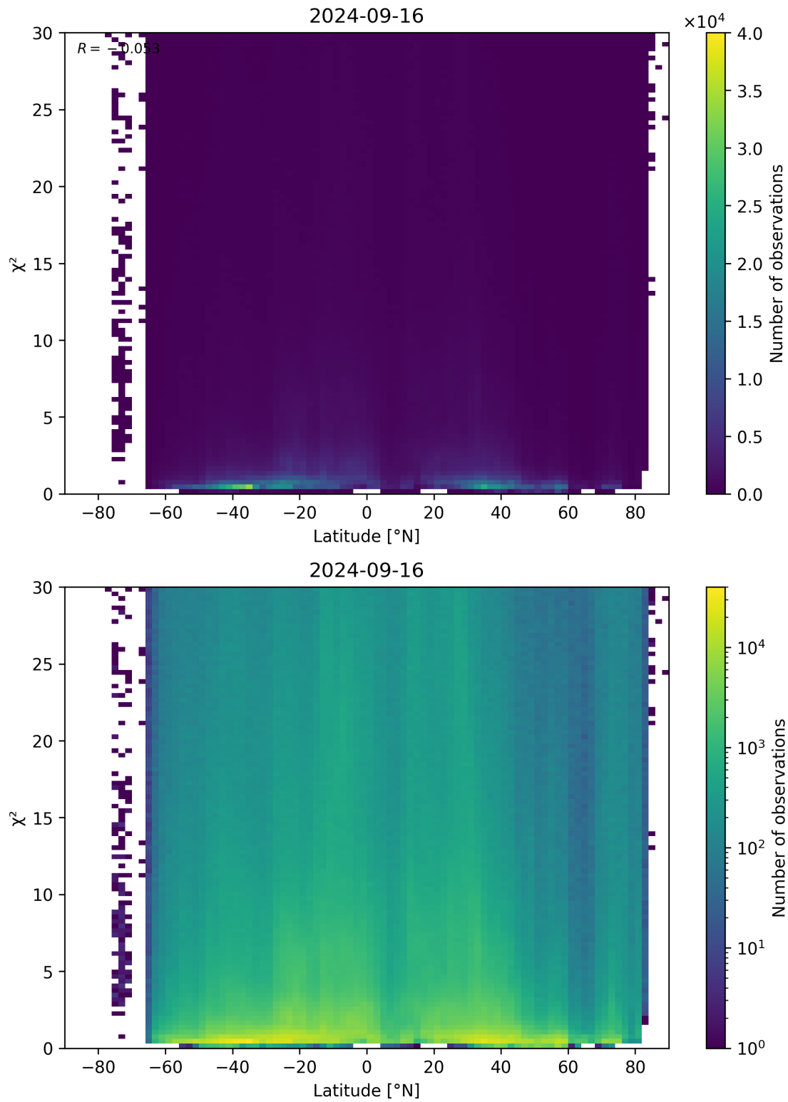
Figure 97: Scatter density plot of “Latitude” against “ \chi^2 ” for 2024-09-15 to 2024-09-17.
