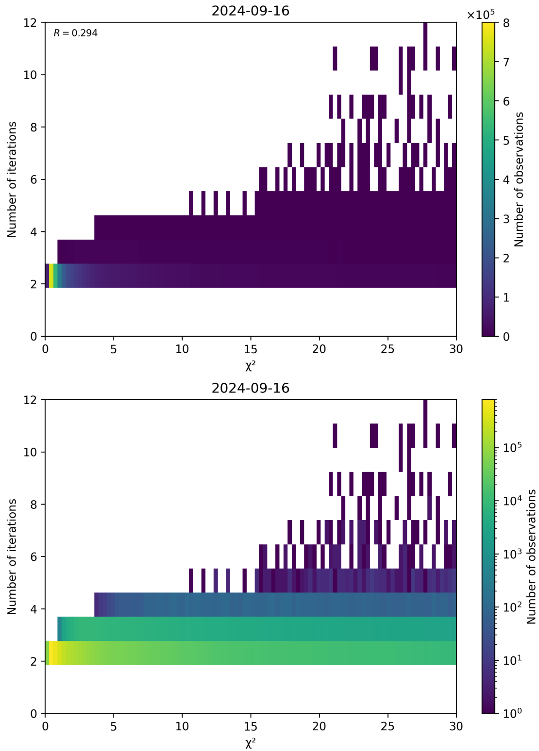
Figure 73: Scatter density plot of “ \chi^2 ” against “Number of iterations” for 2024-09-15 to 2024-09-17.
