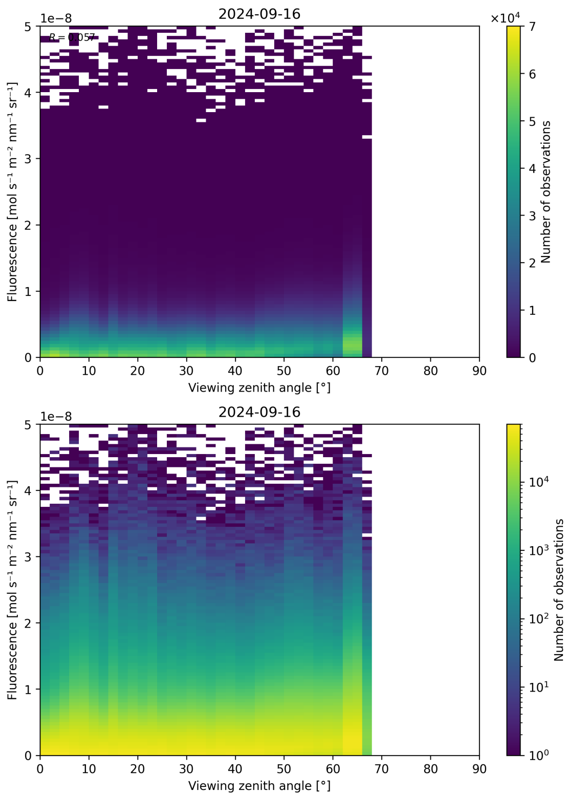
Figure 134: Scatter density plot of “Viewing zenith angle” against “Fluorescence” for 2024-09-15 to 2024-09-17.
