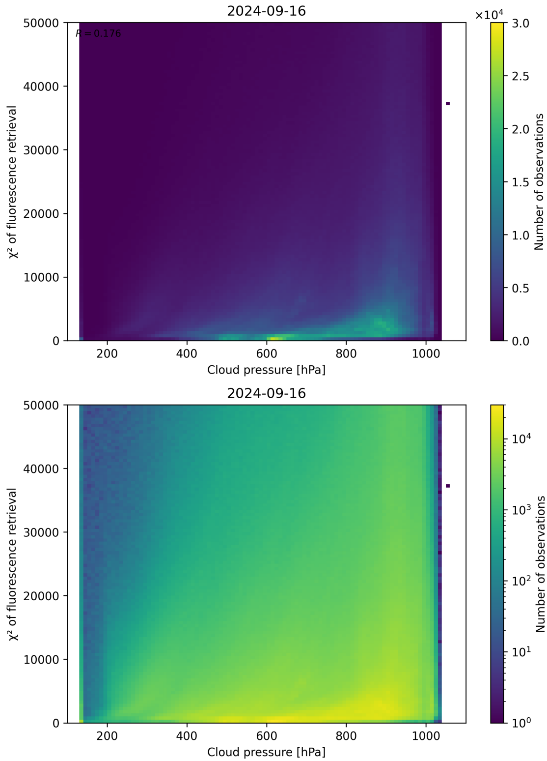
Figure 86: Scatter density plot of “Cloud pressure” against “ \chi^2 of fluorescence retrieval” for 2024-09-15 to 2024-09-17.
