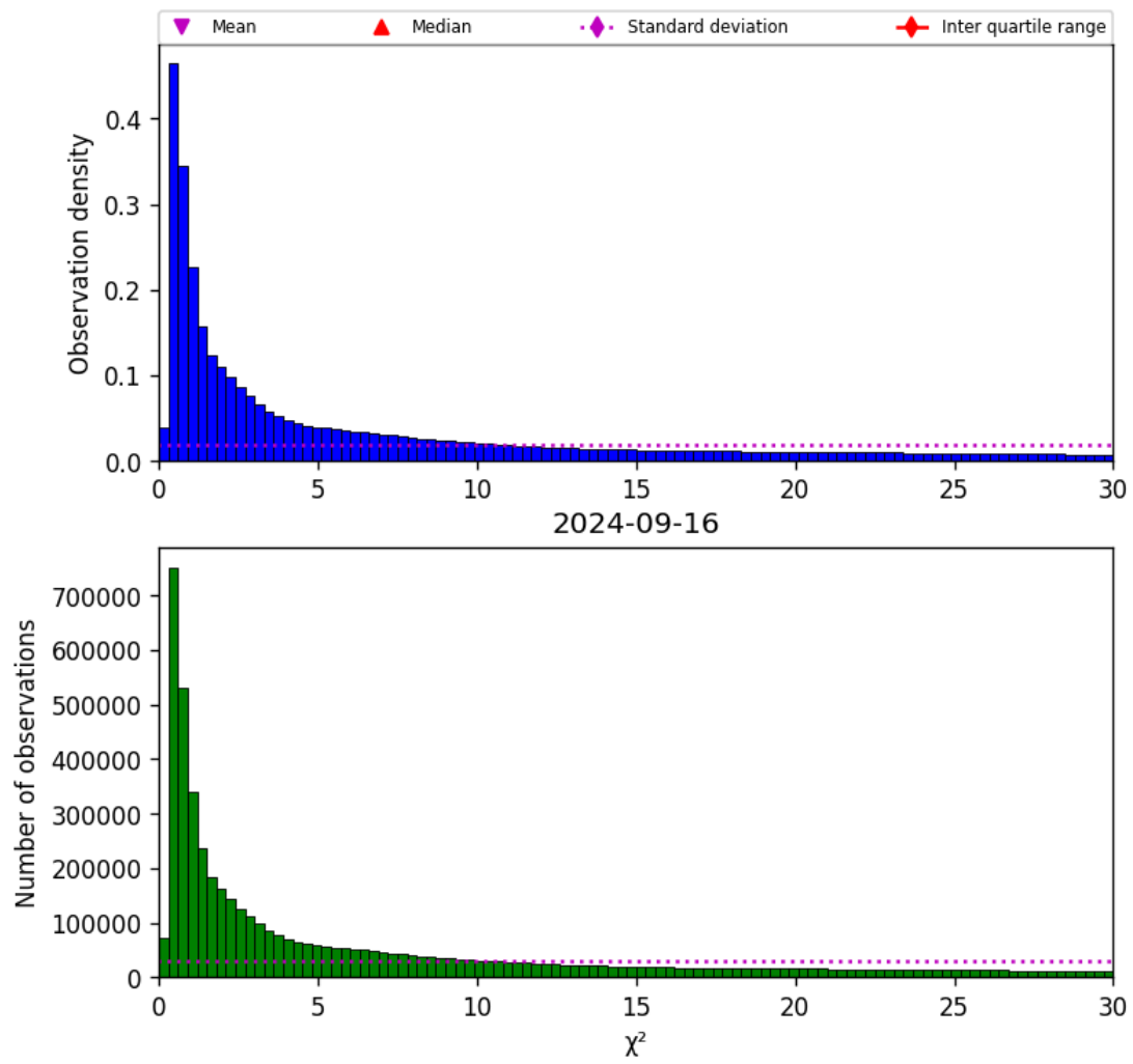
Figure 38: Histogram of " \chi^2 " for 2024-09-15 to 2024-09-17
