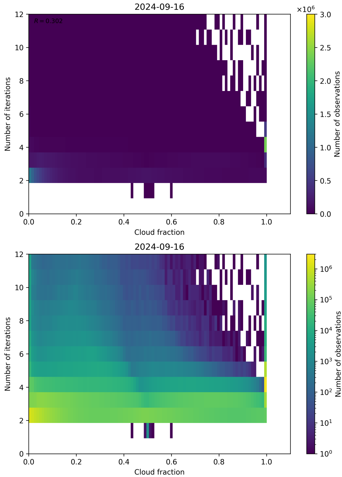
Figure 80: Scatter density plot of “Cloud fraction” against “Number of iterations” for 2024-09-15 to 2024-09-17.
