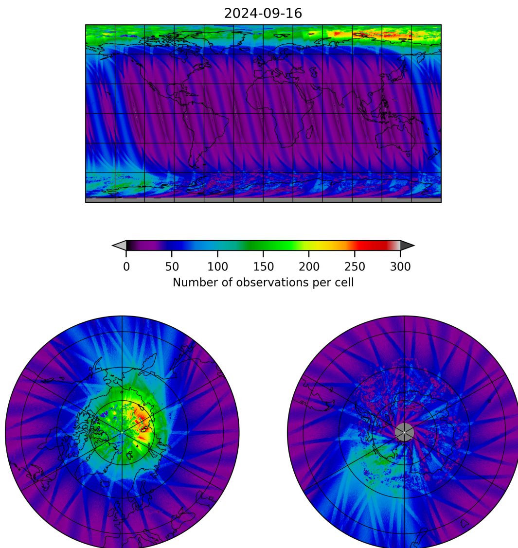
Figure 11: Map of the number of observations for 2024-09-15 to 2024-09-17
