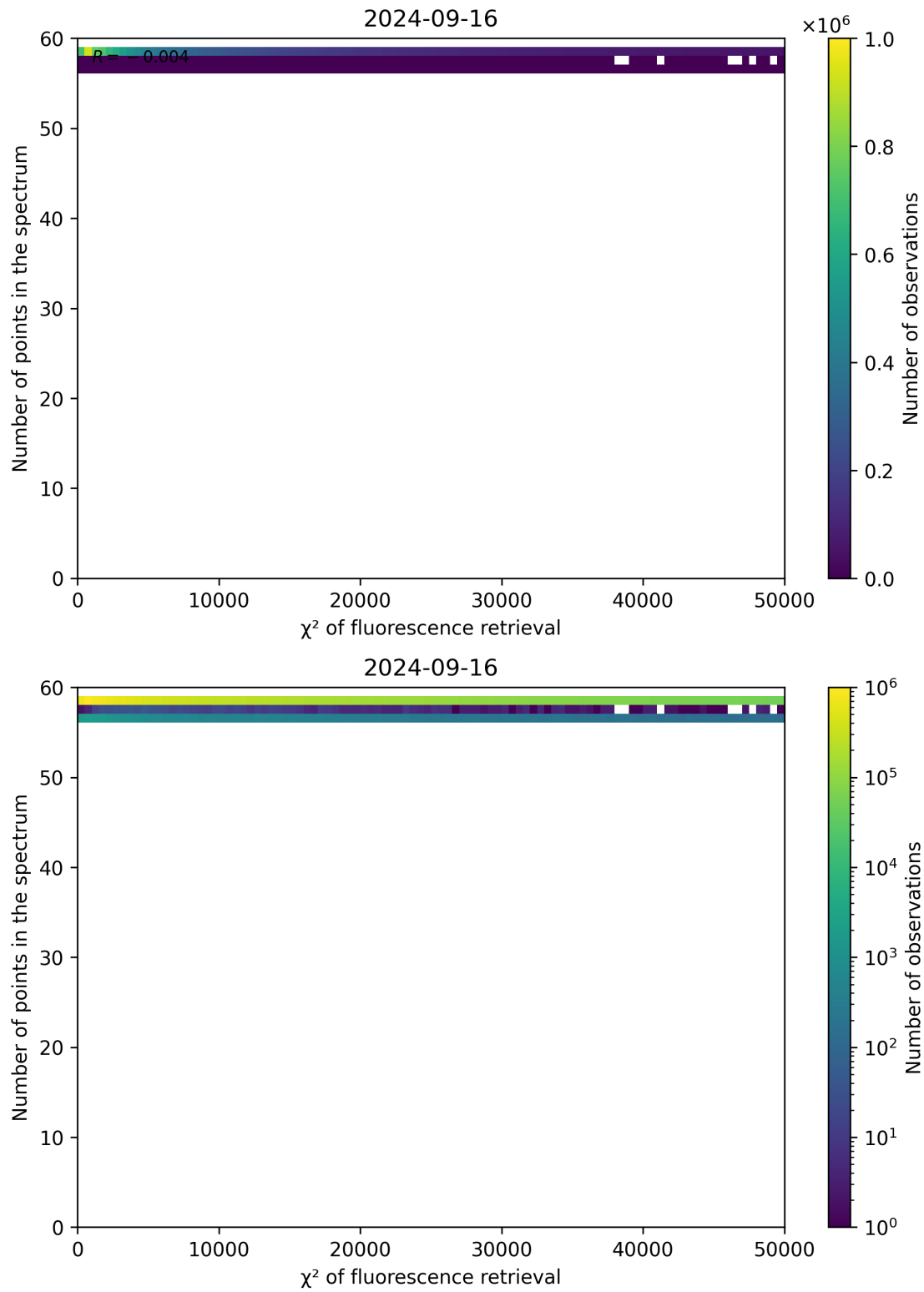
Figure 71: Scatter density plot of " \chi^2 of fluorescence retrieval" against "Number of points in the spectrum" for 2024-09-15 to 2024-09-17.
