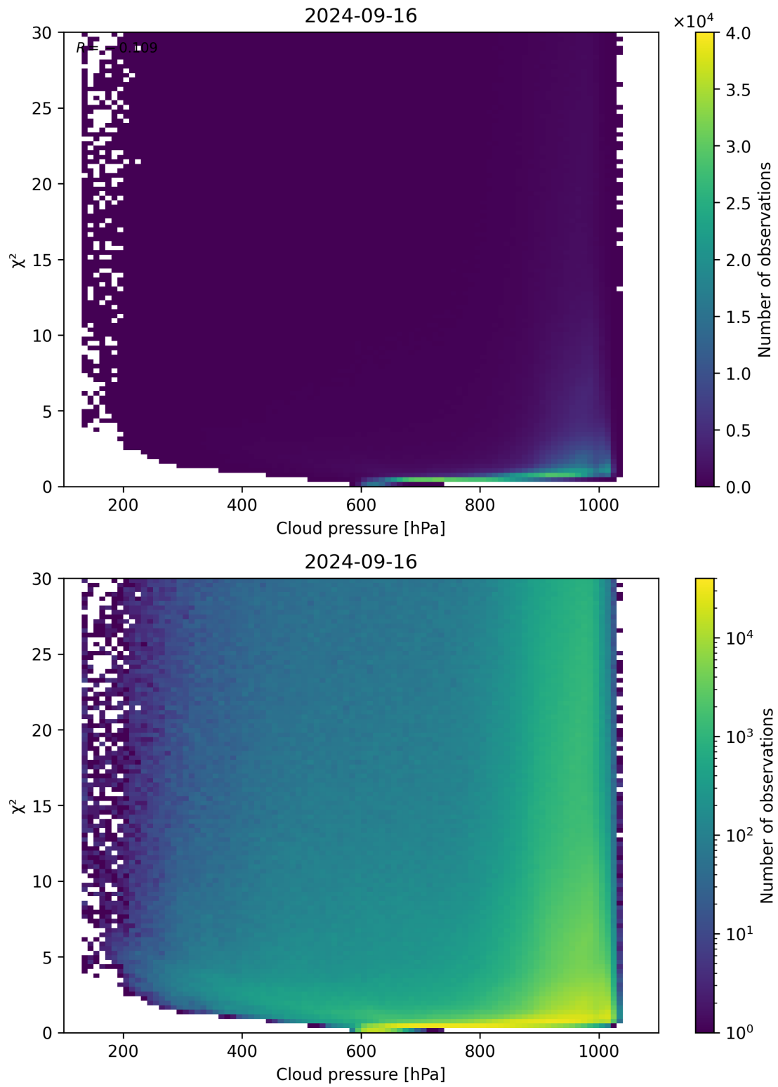
Figure 85: Scatter density plot of “Cloud pressure” against “ \chi^2 ” for 2024-09-15 to 2024-09-17.
