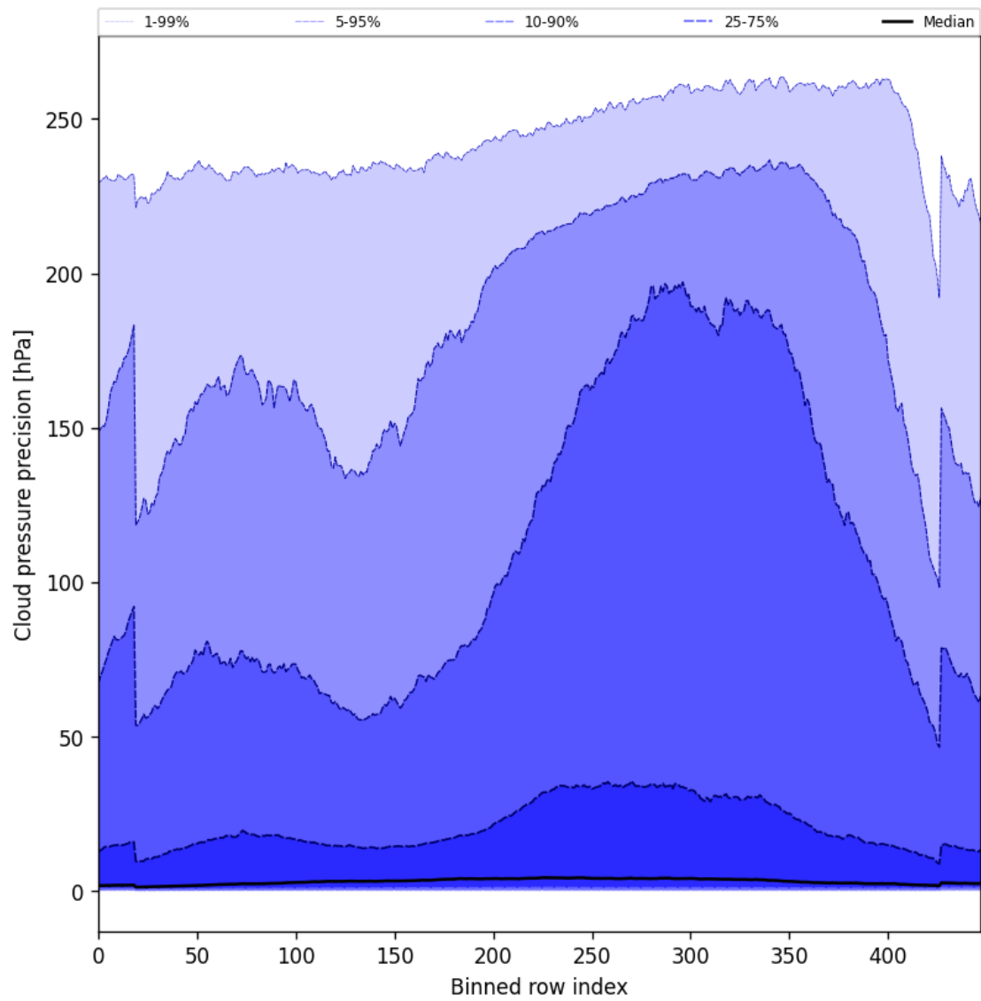
Figure 48: Along track statistics of “Cloud pressure precision” for 2024-09-15 to 2024-09-17
