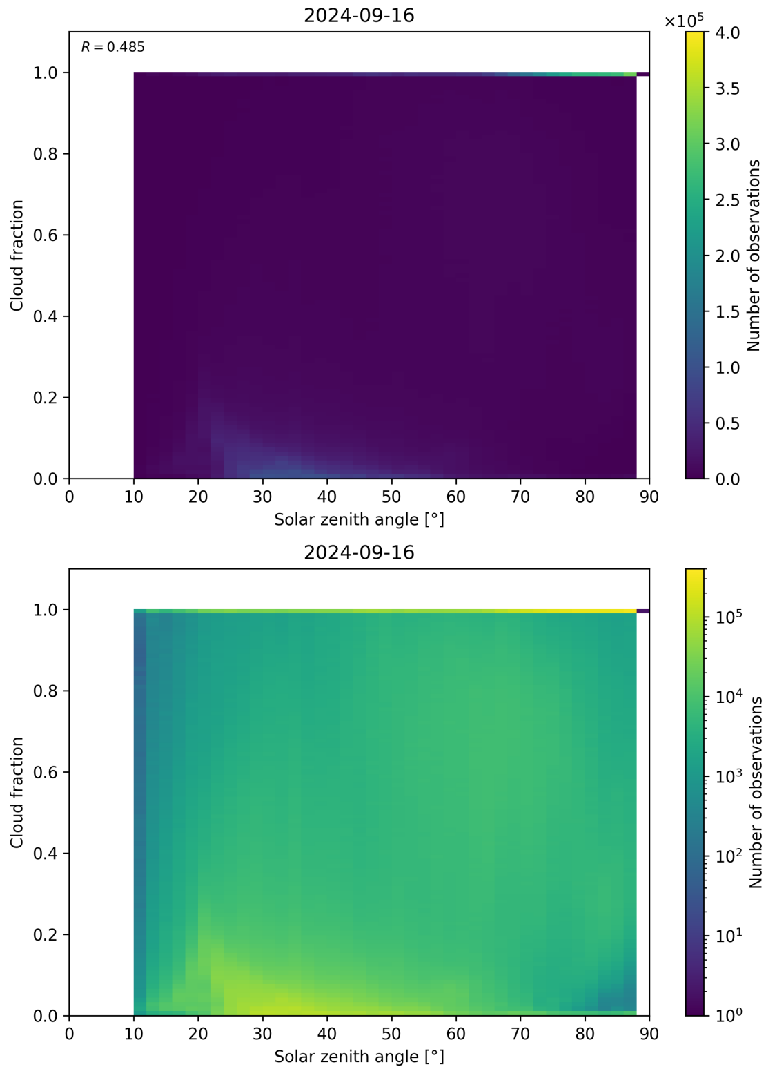
Figure 121: Scatter density plot of “Solar zenith angle” against “Cloud fraction” for 2024-09-15 to 2024-09-17.
