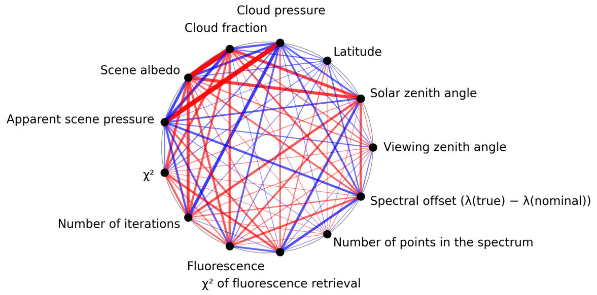
Figure 1: Map of correlation graph for 2024-09-15 to 2024-09-17.
