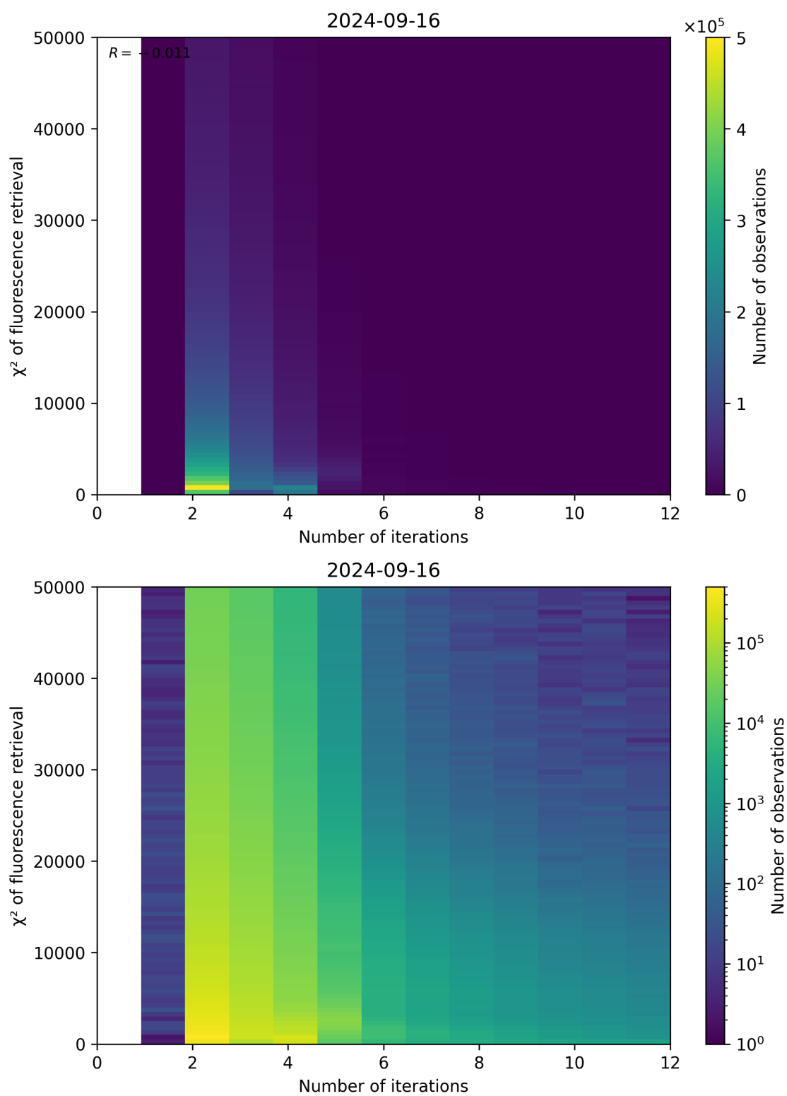
Figure 106: Scatter density plot of “Number of iterations” against “ \chi^2 of fluorescence retrieval” for 2024-09-15 to 2024-09-17.
