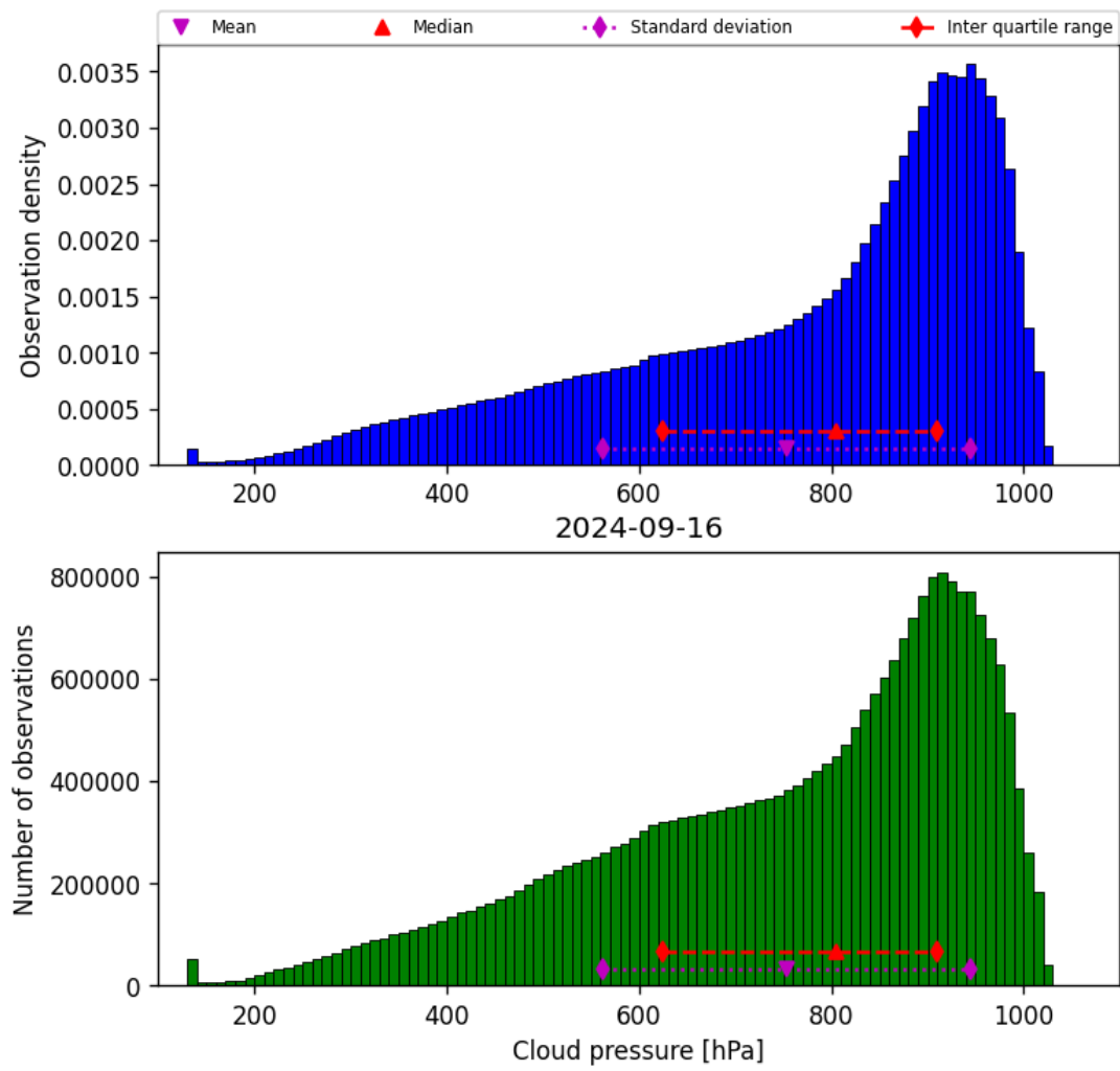
Figure 30: Histogram of “Cloud pressure” for 2024-09-15 to 2024-09-17
