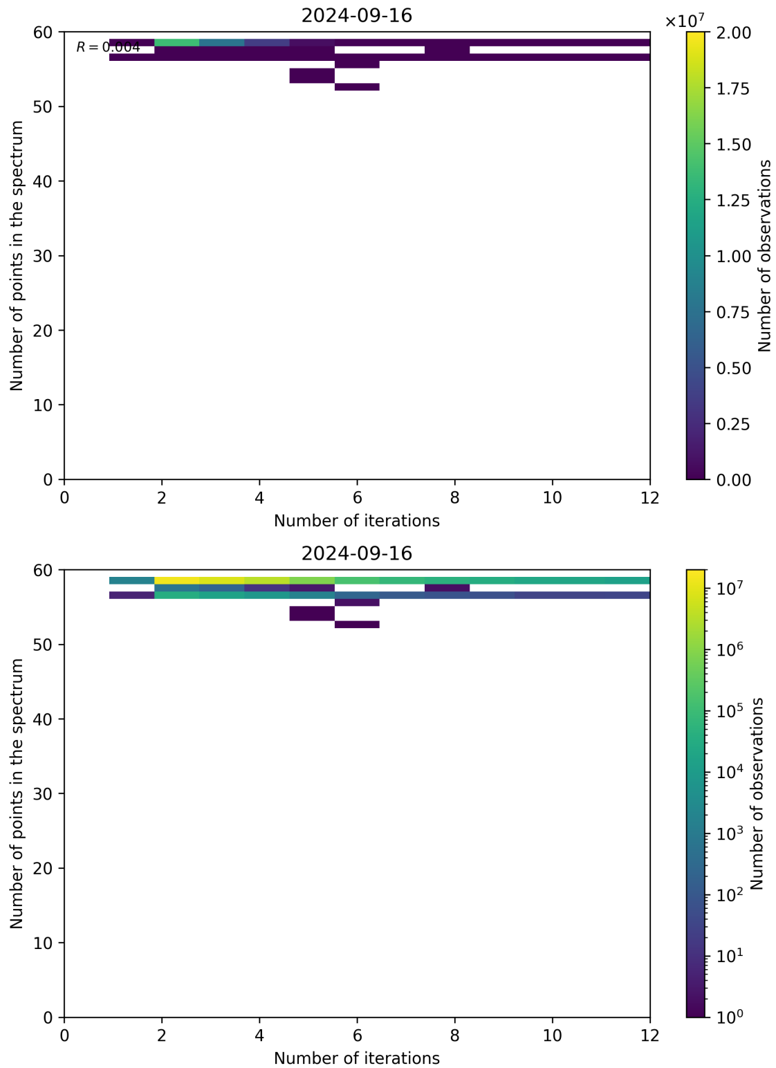
Figure 108: Scatter density plot of “Number of iterations” against “Number of points in the spectrum” for 2024-09-15 to 2024-09-17.
