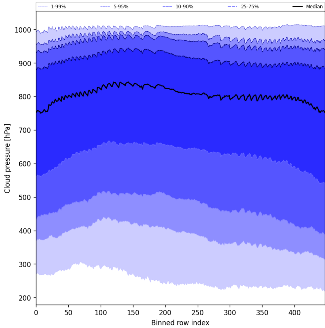
Figure 47: Along track statistics of “Cloud pressure” for 2024-09-15 to 2024-09-17
