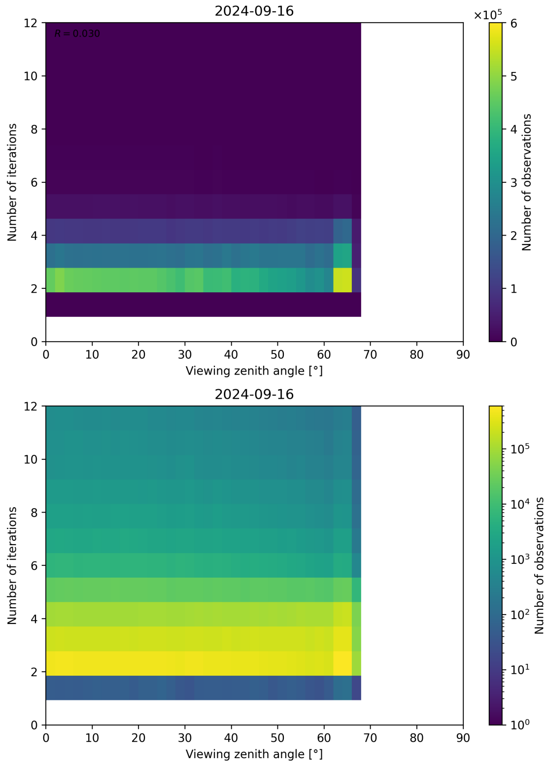
Figure 136: Scatter density plot of “Viewing zenith angle” against “Number of iterations” for 2024-09-15 to 2024-09-17.
