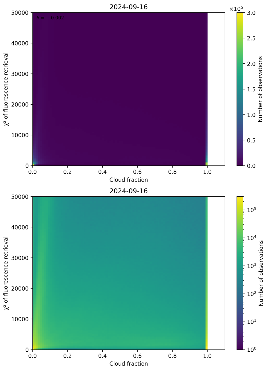
Figure 78: Scatter density plot of “Cloud fraction” against “ \chi^2 of fluorescence retrieval” for 2024-09-15 to 2024-09-17.
