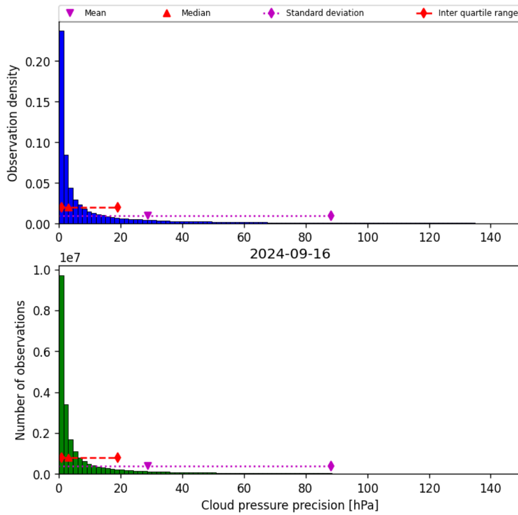
Figure 31: Histogram of “Cloud pressure precision” for 2024-09-15 to 2024-09-17
