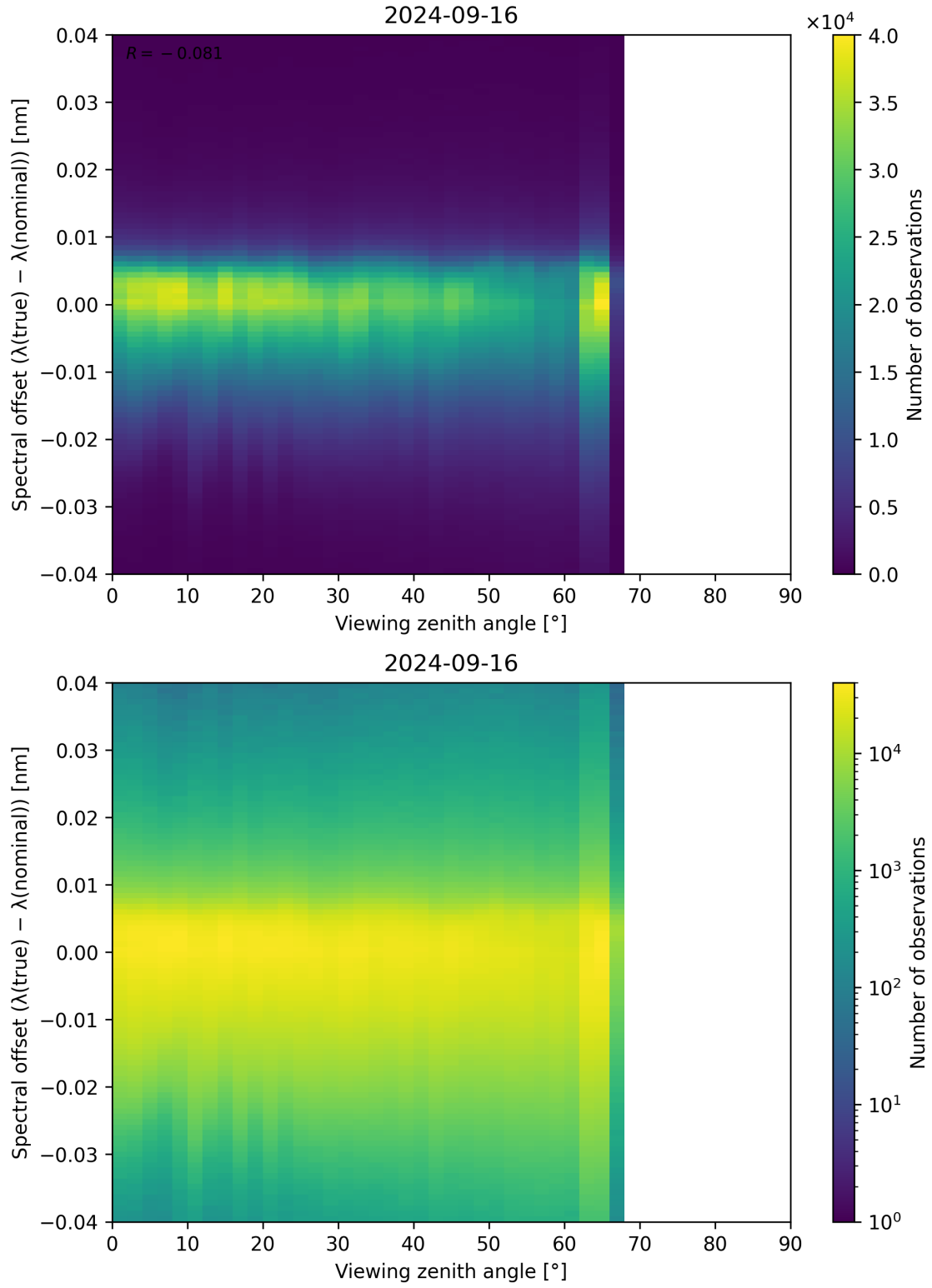
Figure 140: Scatter density plot of “Viewing zenith angle” against “Spectral offset ( \lambda_{\text{true}} - \lambda_{\text{nominal}} )” for 2024-09-15 to 2024-09-17.
