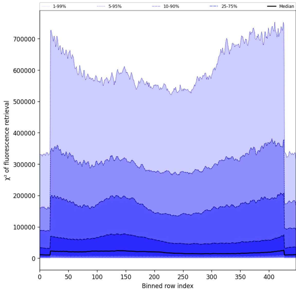
Figure 59: Along track statistics of “ \chi^2 of fluorescence retrieval” for 2024-09-15 to 2024-09-17
