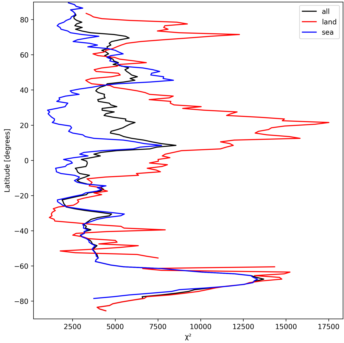
Figure 21: Zonal average of “ \chi^2 ” for 2024-09-15 to 2024-09-17.
