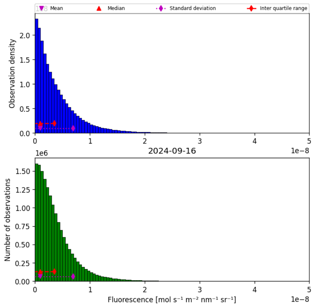
Figure 40: Histogram of “Fluorescence” for 2024-09-15 to 2024-09-17
