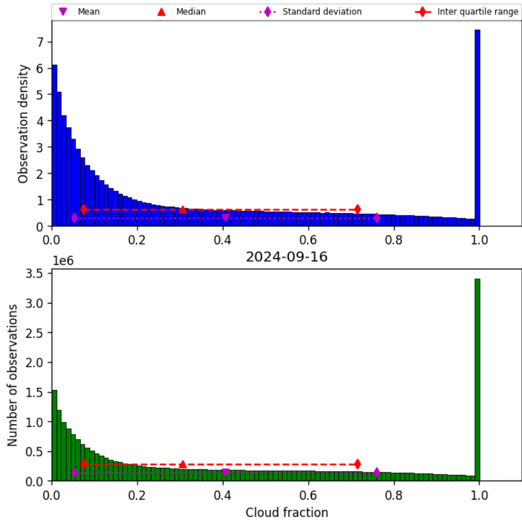
Figure 32: Histogram of “Cloud fraction” for 2024-09-15 to 2024-09-17
