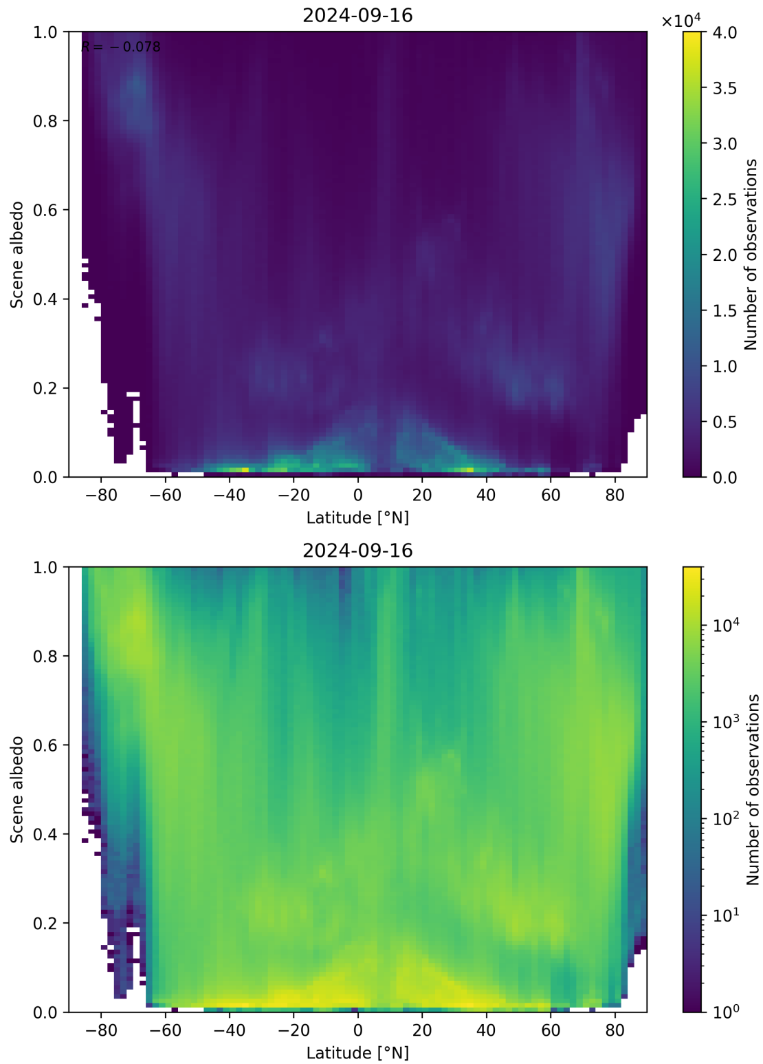
Figure 104: Scatter density plot of “Latitude” against “Scene albedo” for 2024-09-15 to 2024-09-17.
