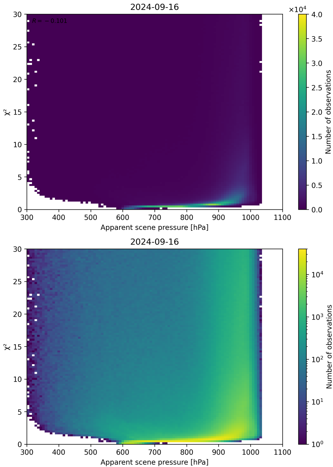
Figure 63: Scatter density plot of “Apparent scene pressure” against “ \chi^2 ” for 2024-09-15 to 2024-09-17.
