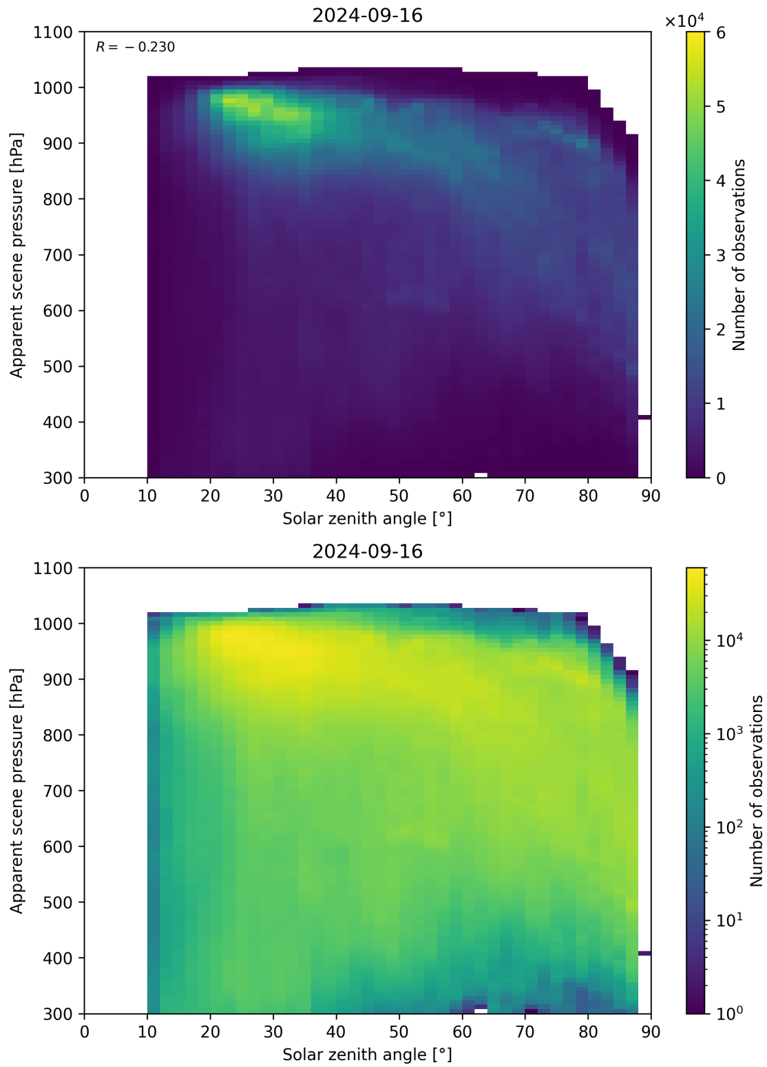
Figure 118: Scatter density plot of “Solar zenith angle” against “Apparent scene pressure” for 2024-09-15 to 2024-09-17.
