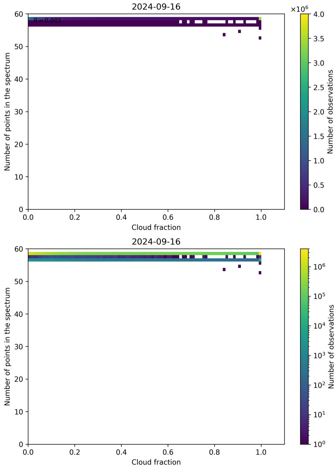
Figure 81: Scatter density plot of “Cloud fraction” against “Number of points in the spectrum” for 2024-09-15 to 2024-09-17.
