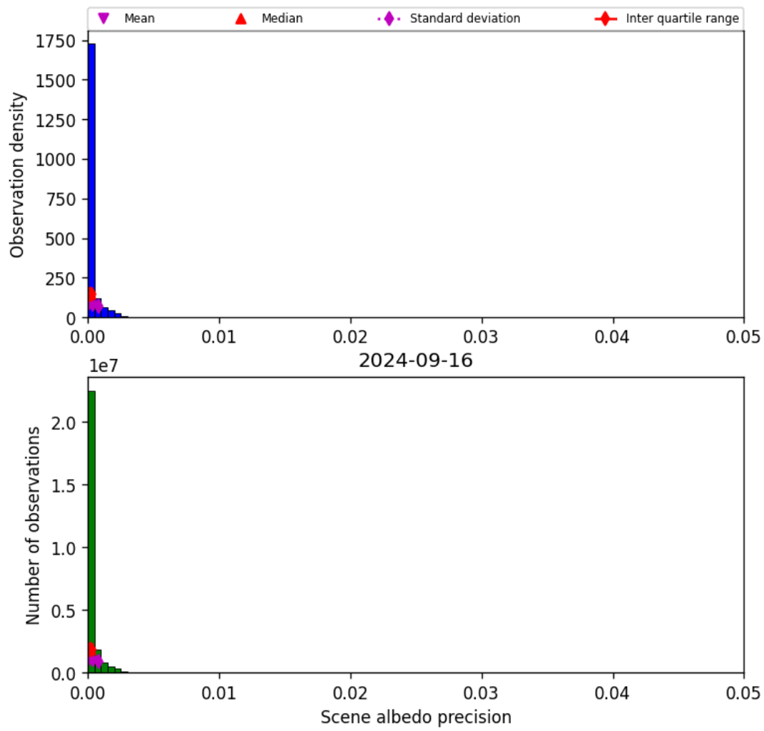
Figure 35: Histogram of “Scene albedo precision” for 2024-09-15 to 2024-09-17
