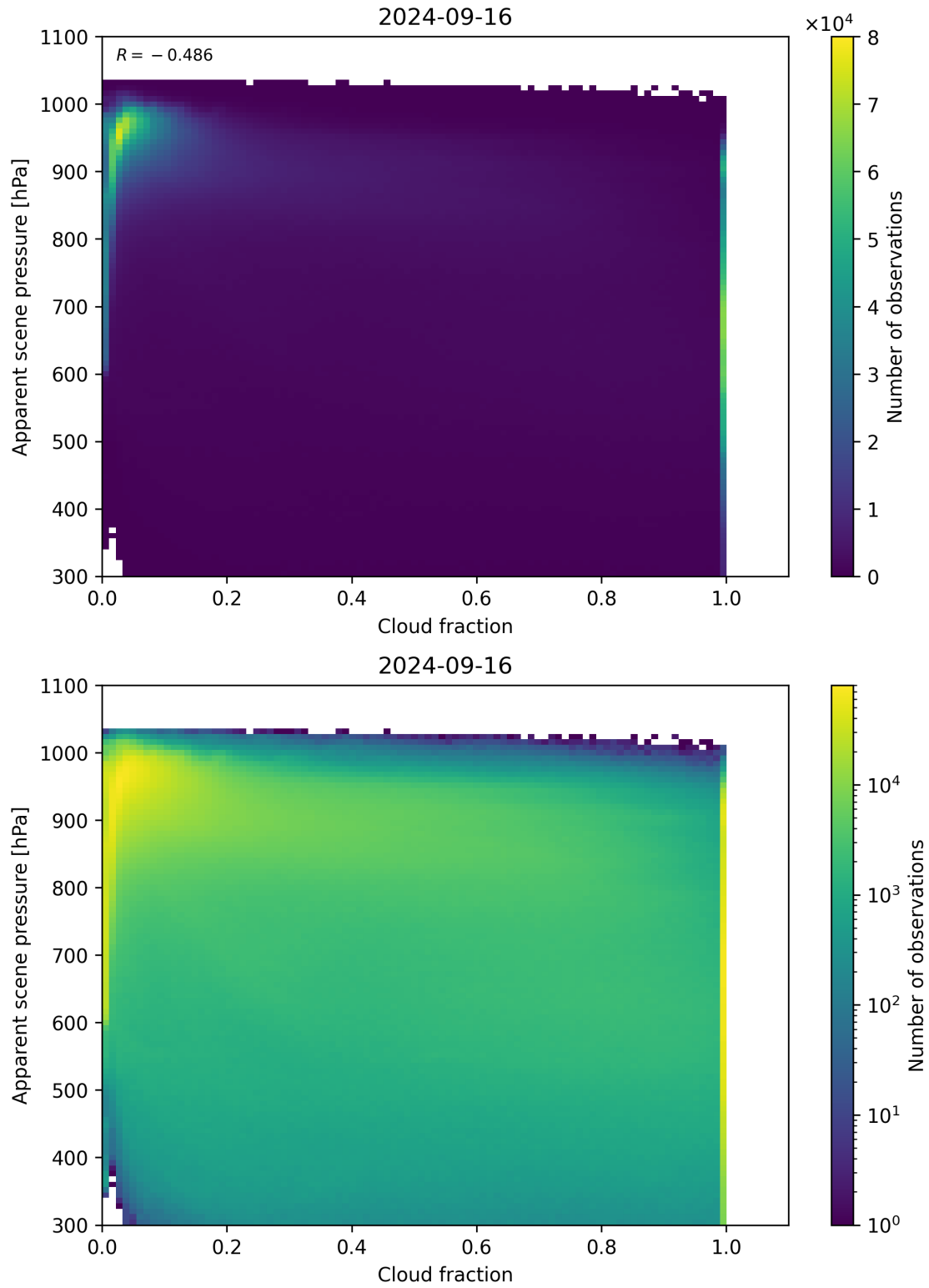
Figure 76: Scatter density plot of “Cloud fraction” against “Apparent scene pressure” for 2024-09-15 to 2024-09-17.
