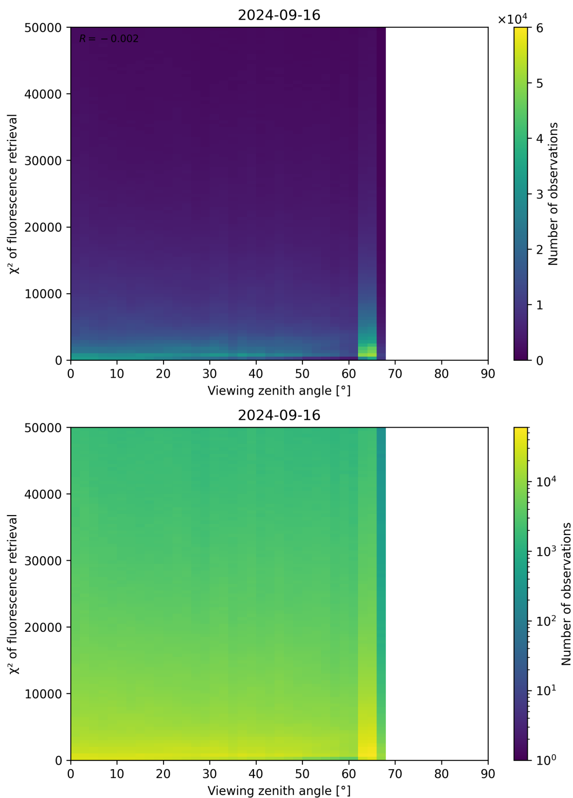
Figure 131: Scatter density plot of “Viewing zenith angle” against “ \chi^2 of fluorescence retrieval” for 2024-09-15 to 2024-09-17.
