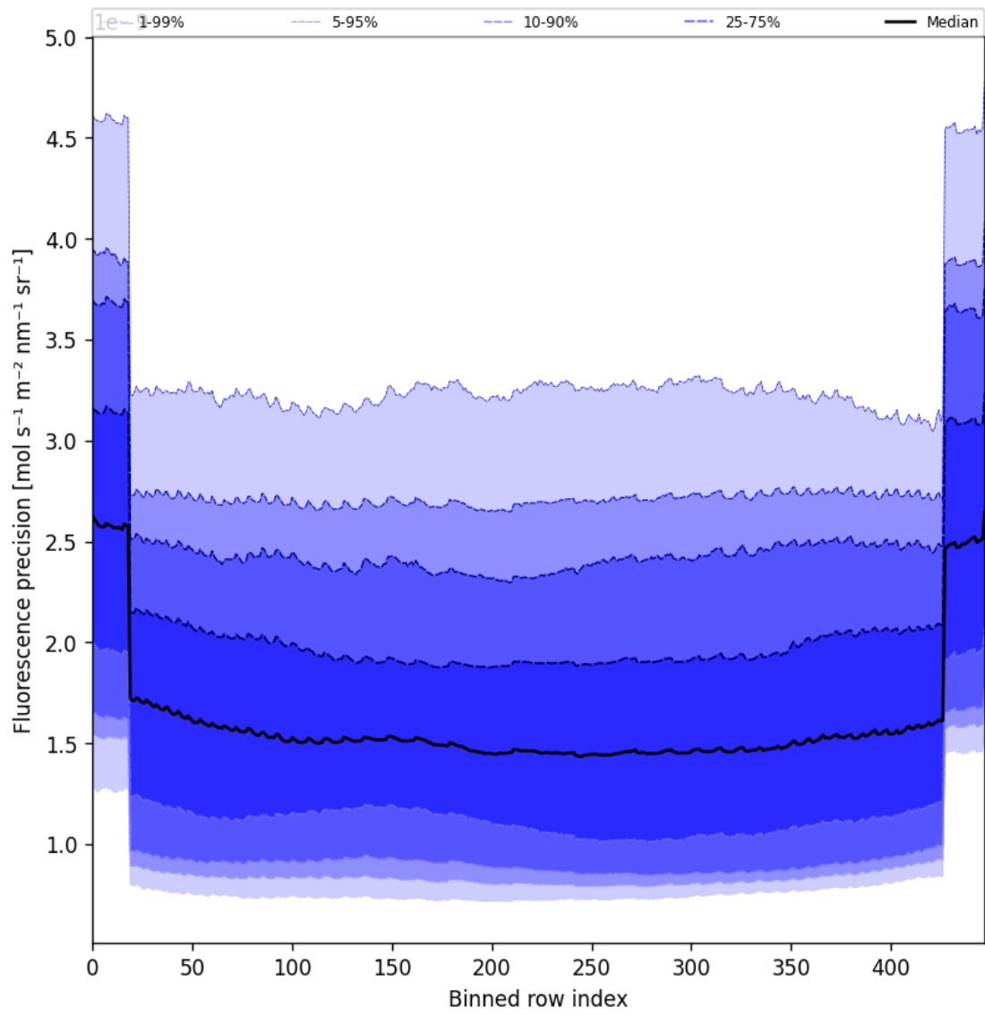
Figure 58: Along track statistics of “Fluorescence precision” for 2024-09-15 to 2024-09-17
