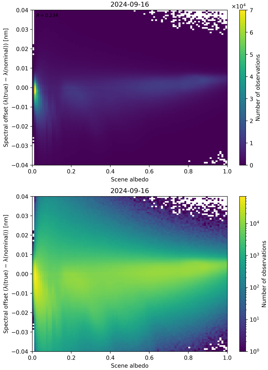
Figure 117: Scatter density plot of “Scene albedo” against “Spectral offset ( \lambda_{\text{true}} - \lambda_{\text{nominal}} )” for 2024-09-15 to 2024-09-17.
