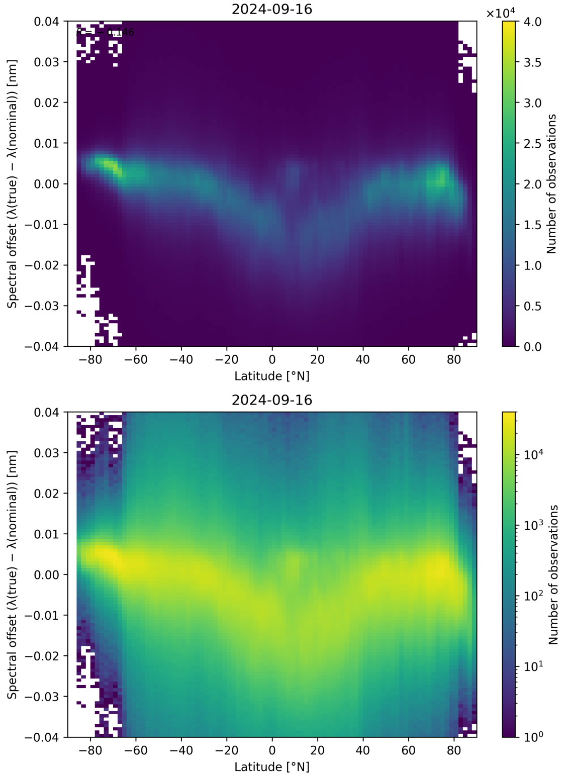
Figure 105: Scatter density plot of “Latitude” against “Spectral offset ( \lambda_{\text{true}} - \lambda_{\text{nominal}} )” for 2024-09-15 to 2024-09-17.
