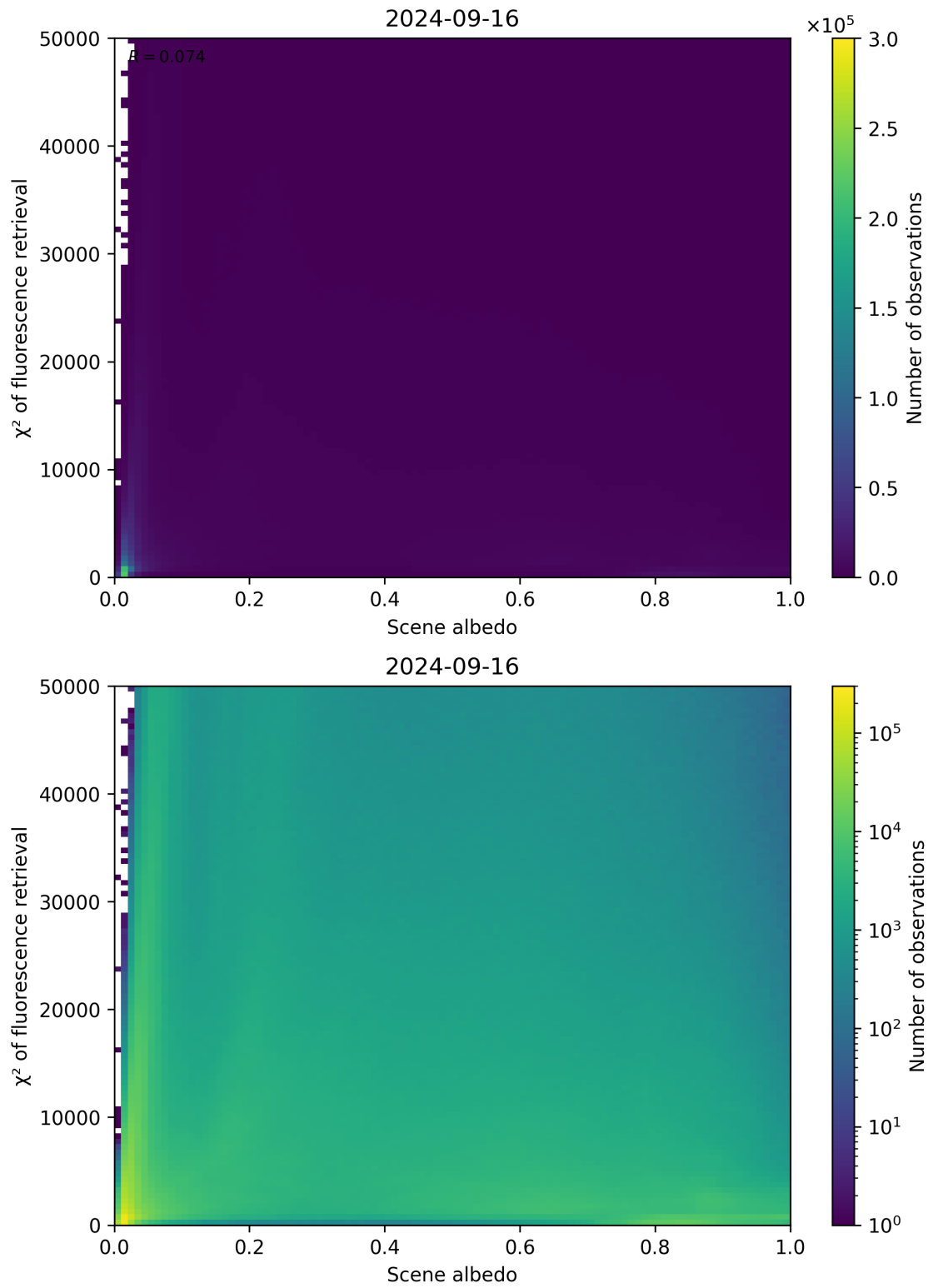
Figure 113: Scatter density plot of “Scene albedo” against “ \chi^2 of fluorescence retrieval” for 2024-09-15 to 2024-09-17.
