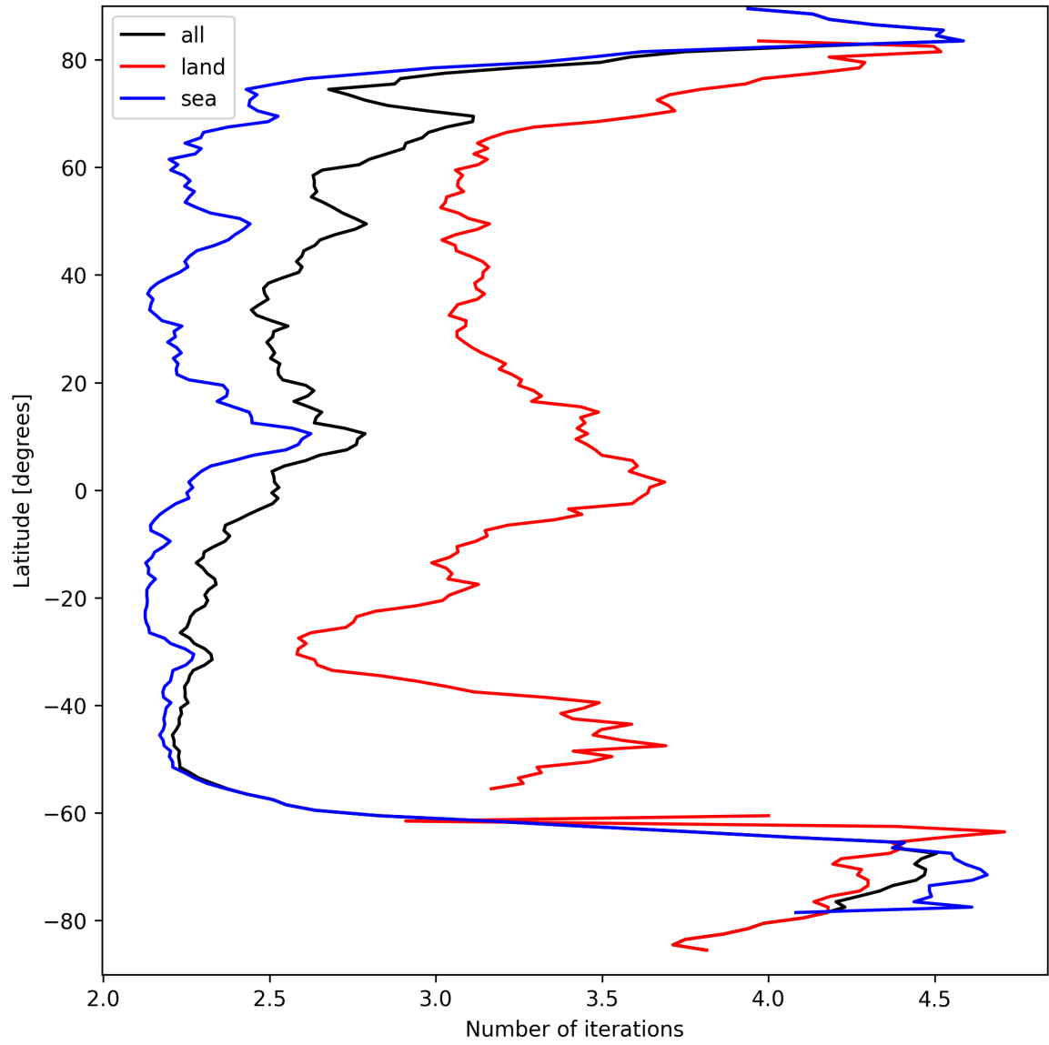
Figure 22: Zonal average of “Number of iterations” for 2024-09-15 to 2024-09-17.
