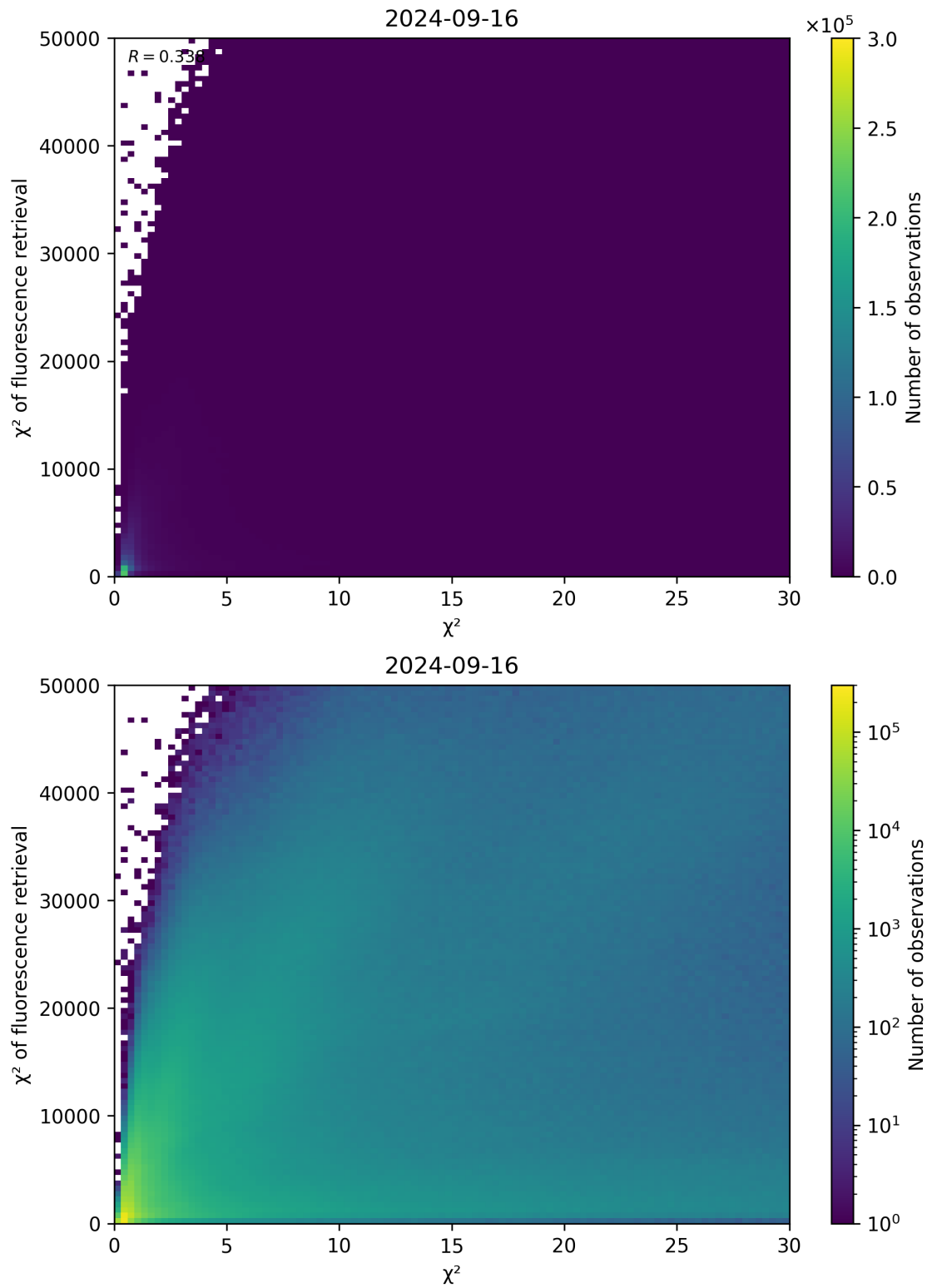
Figure 69: Scatter density plot of “ \chi^2 ” against “ \chi^2 of fluorescence retrieval” for 2024-09-15 to 2024-09-17.
