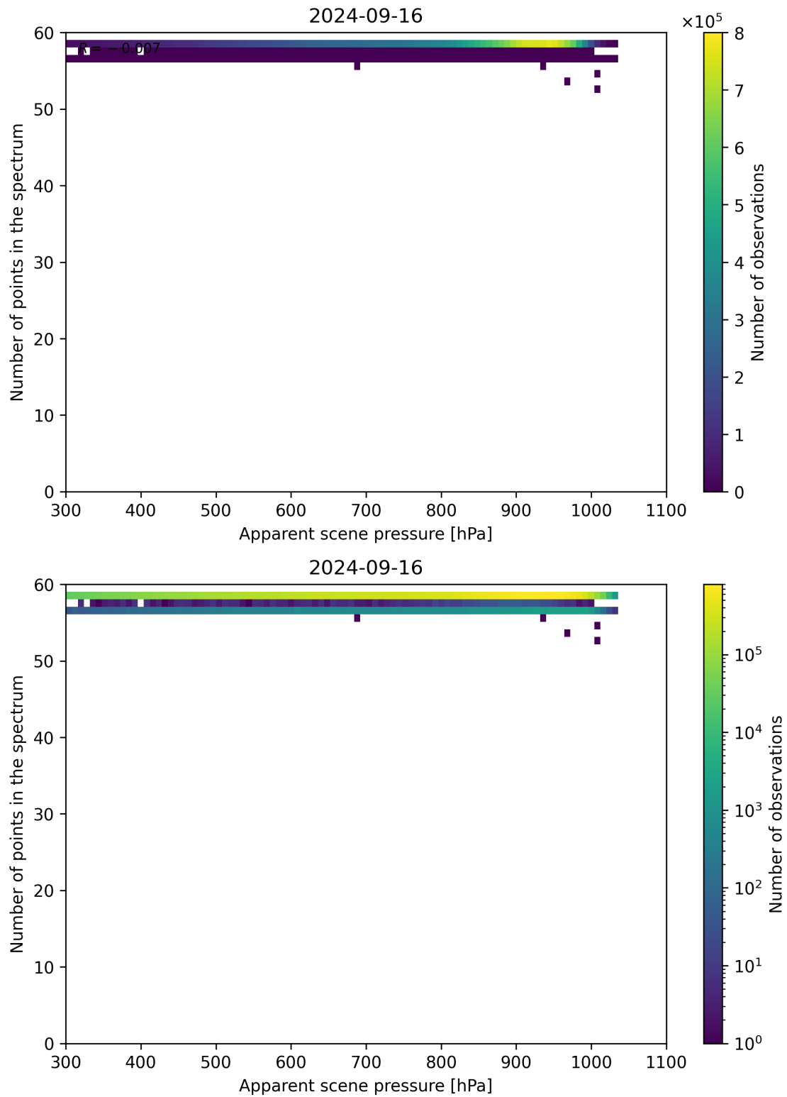
Figure 67: Scatter density plot of “Apparent scene pressure” against “Number of points in the spectrum” for 2024-09-15 to 2024-09-17.
