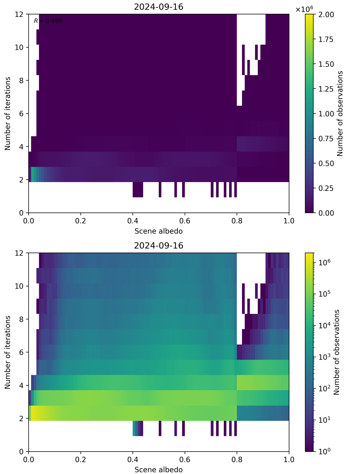
Figure 115: Scatter density plot of “Scene albedo” against “Number of iterations” for 2024-09-15 to 2024-09-17.
