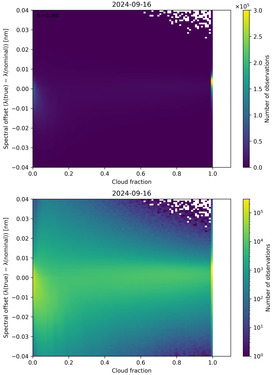
Figure 83: Scatter density plot of “Cloud fraction” against “Spectral offset ( \lambda_{\text{true}} - \lambda_{\text{nominal}} )” for 2024-09-15 to 2024-09-17.
