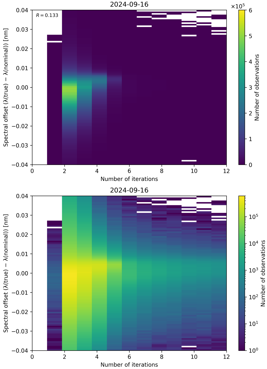
Figure 109: Scatter density plot of “Number of iterations” against “Spectral offset ( \lambda_{\text{true}} - \lambda_{\text{nominal}} )” for 2024-09-15 to 2024-09-17.
