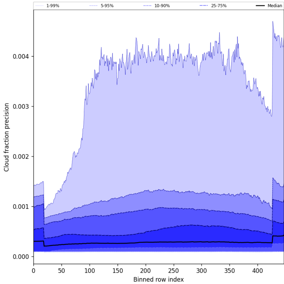
Figure 50: Along track statistics of “Cloud fraction precision” for 2024-09-15 to 2024-09-17
