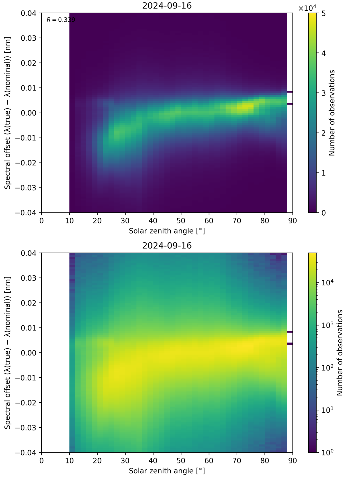
Figure 128: Scatter density plot of “Solar zenith angle” against “Spectral offset ( \lambda_{\text{true}} - \lambda_{\text{nominal}} )” for 2024-09-15 to 2024-09-17.
