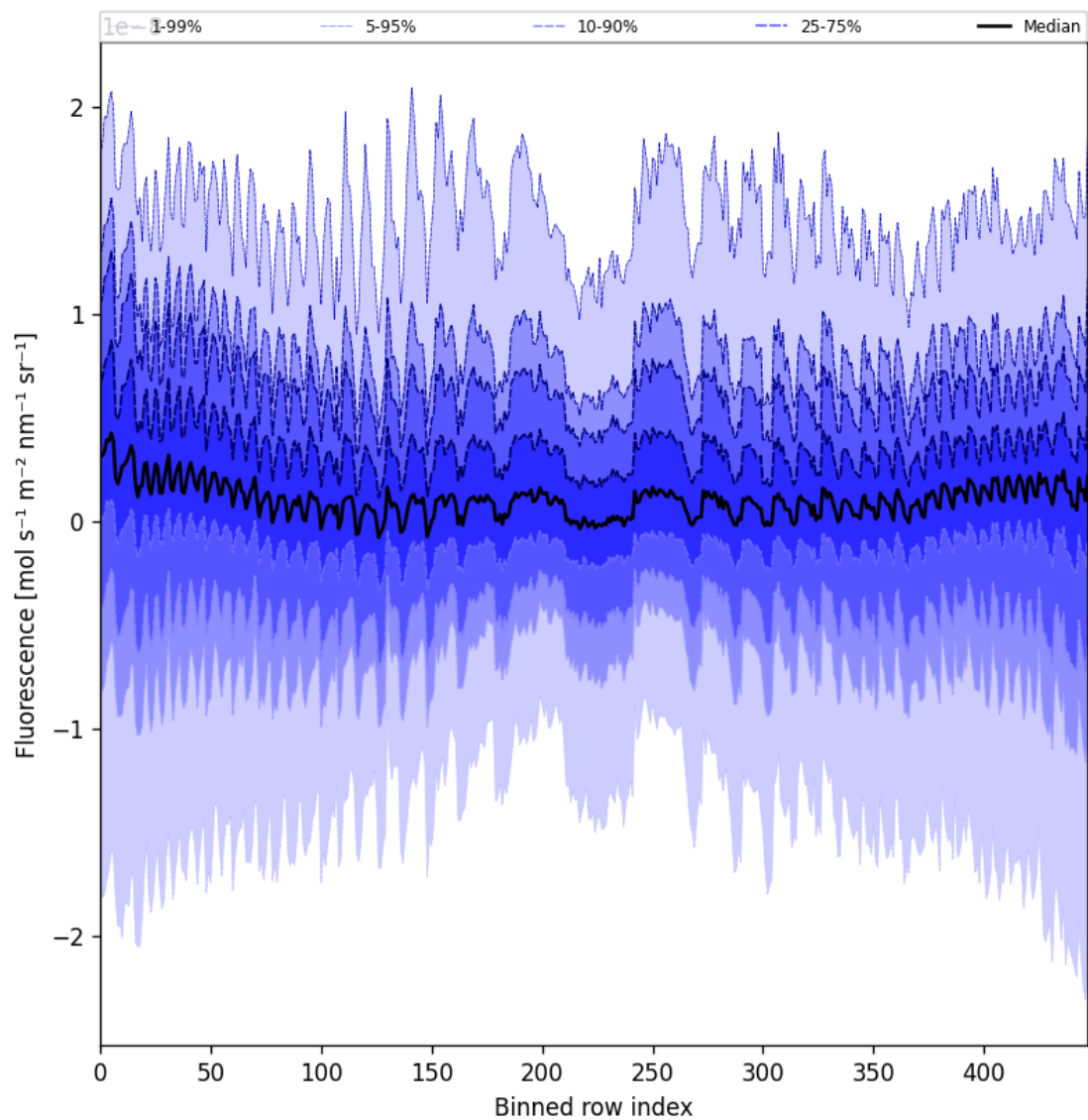
Figure 57: Along track statistics of “Fluorescence” for 2024-09-17 to 2024-09-18
