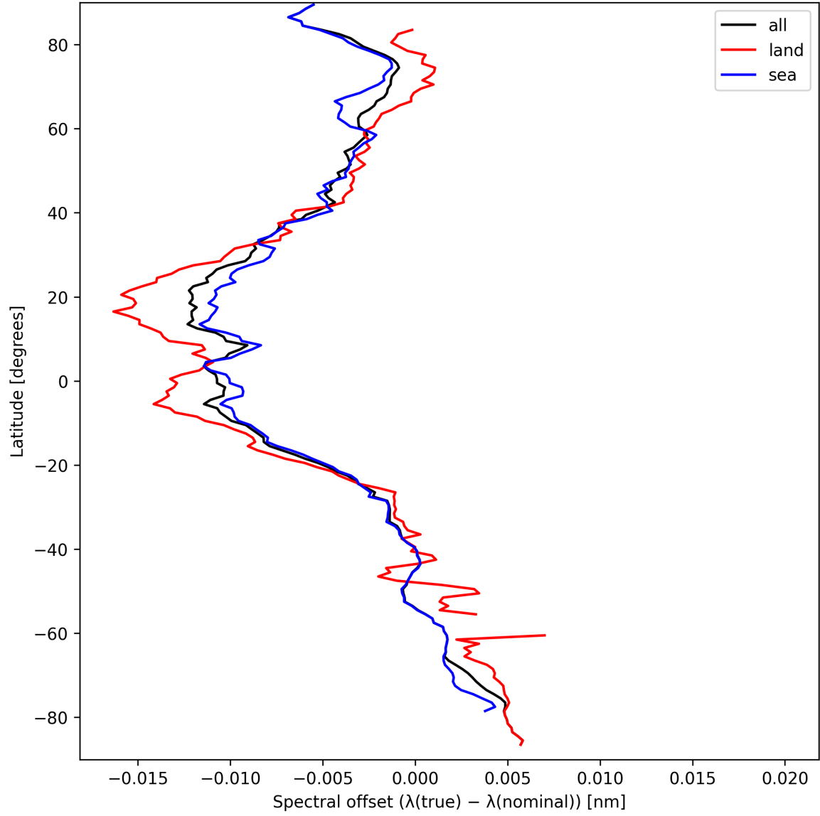
Figure 28: Zonal average of “Spectral offset ( \lambda_{\text{true}} - \lambda_{\text{nominal}} )” for 2024-09-17 to 2024-09-18.
