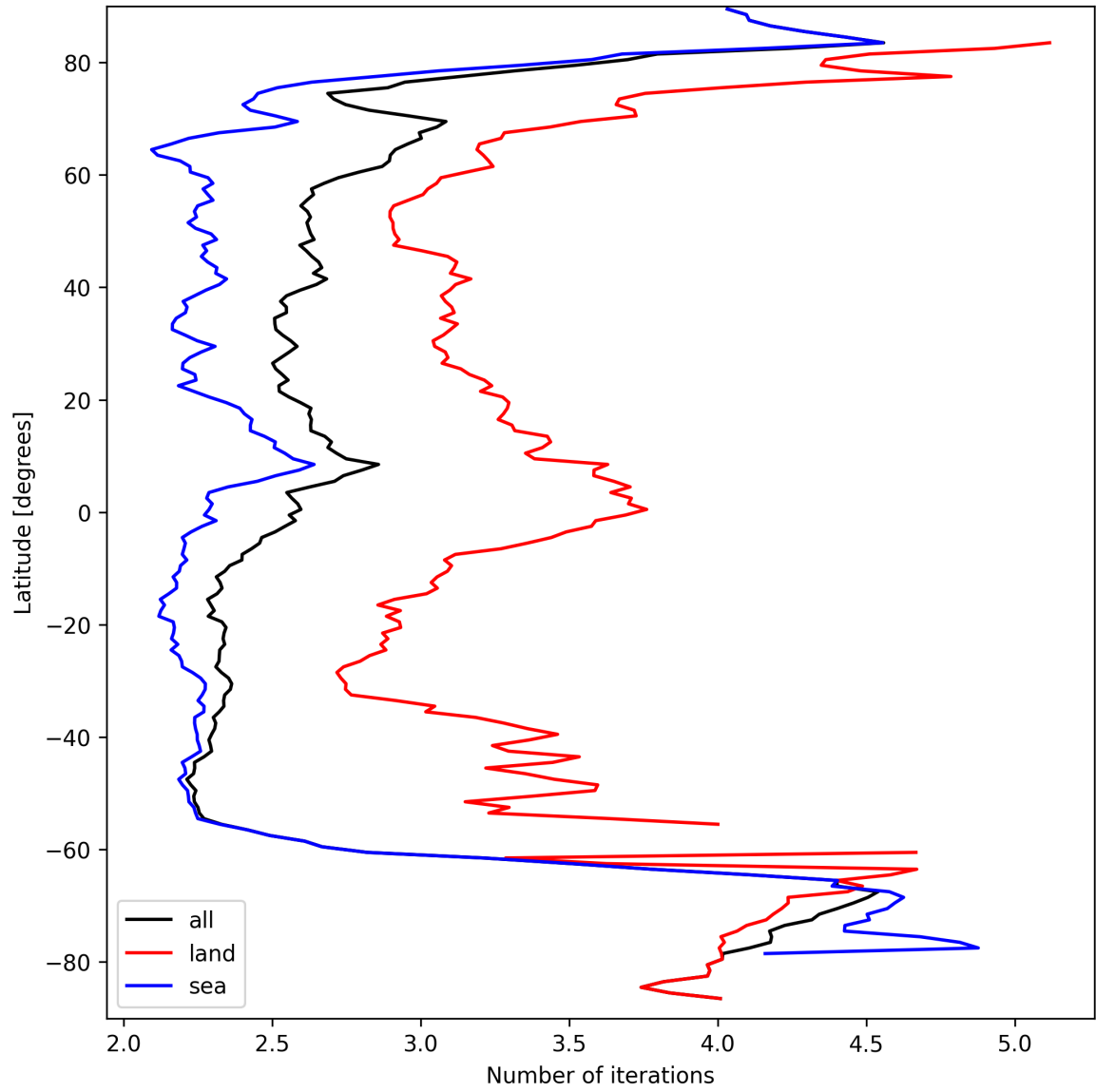
Figure 22: Zonal average of “Number of iterations” for 2024-09-17 to 2024-09-18.
