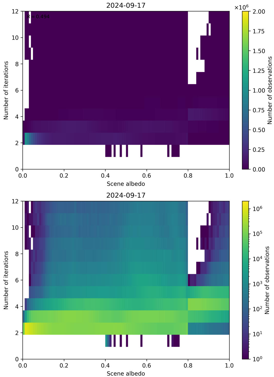
Figure 115: Scatter density plot of “Scene albedo” against “Number of iterations” for 2024-09-17 to 2024-09-18.
