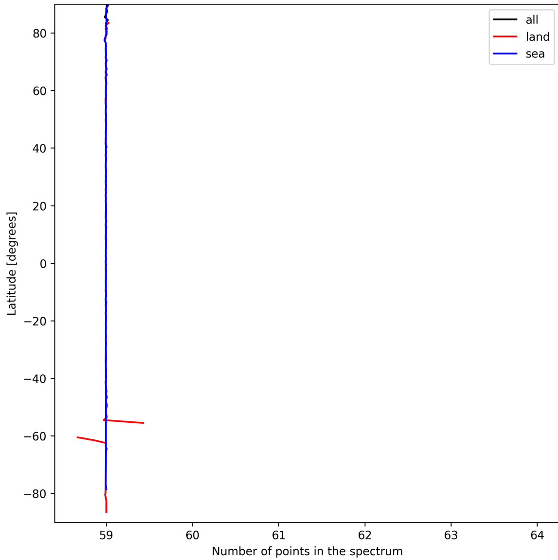
Figure 27: Zonal average of “Number of points in the spectrum” for 2024-09-17 to 2024-09-18.
