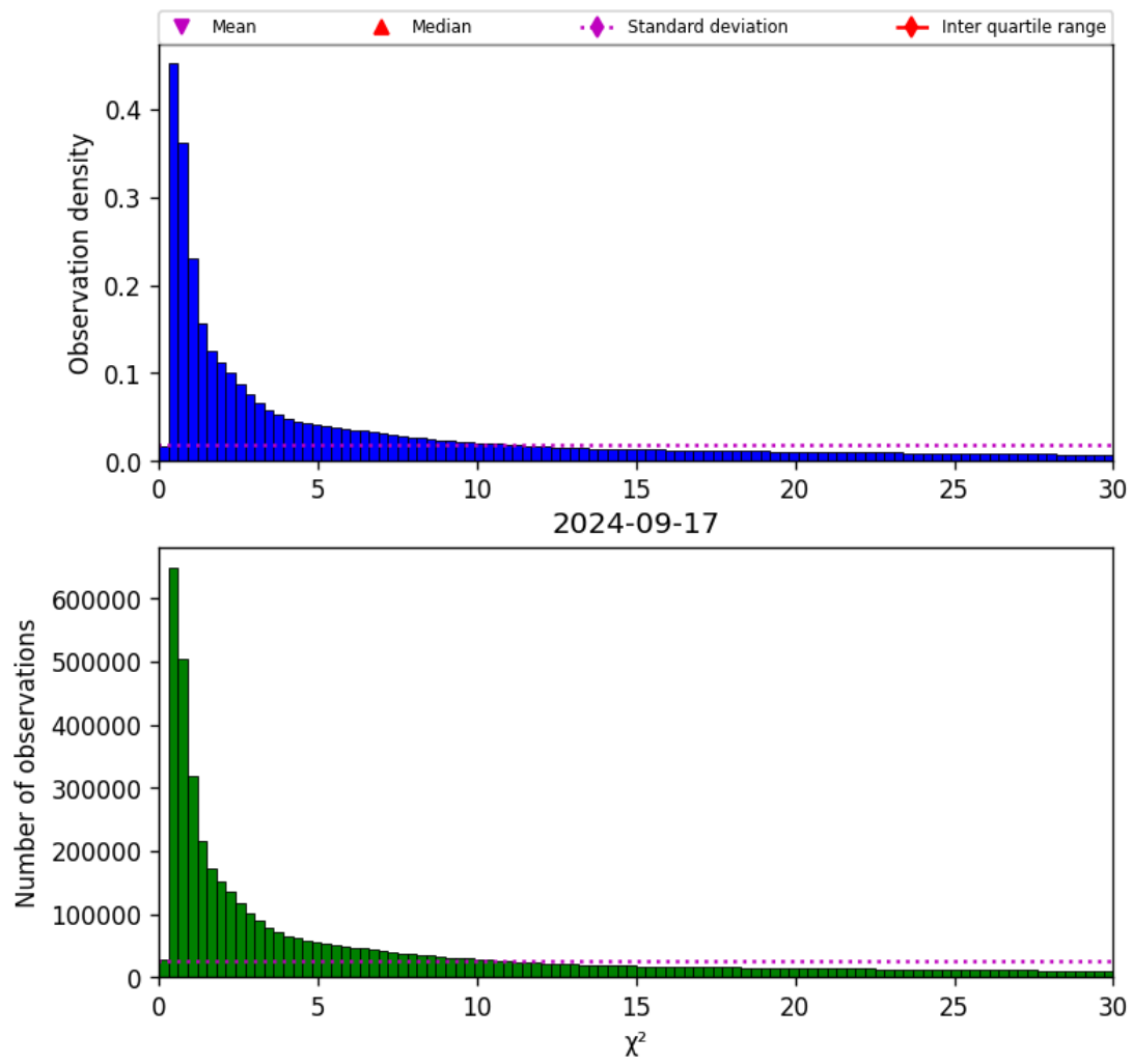
Figure 38: Histogram of “ \chi^2 ” for 2024-09-17 to 2024-09-18
