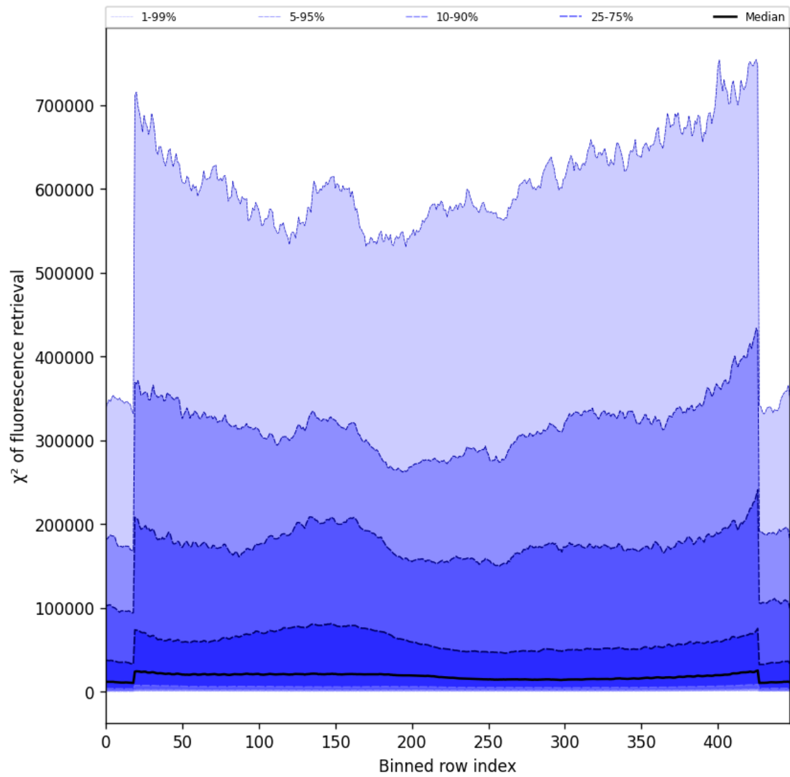
Figure 59: Along track statistics of “ \chi^2 of fluorescence retrieval” for 2024-09-17 to 2024-09-18
