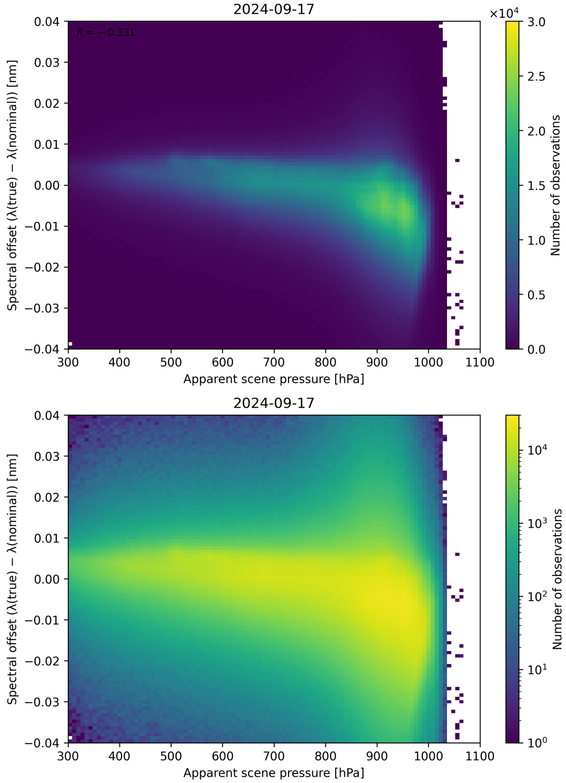
Figure 68: Scatter density plot of “Apparent scene pressure” against “Spectral offset ( \lambda_{\text{true}} - \lambda_{\text{nominal}} )” for 2024-09-17 to 2024-09-18.
