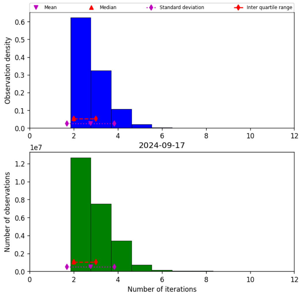
Figure 39: Histogram of “Number of iterations” for 2024-09-17 to 2024-09-18
