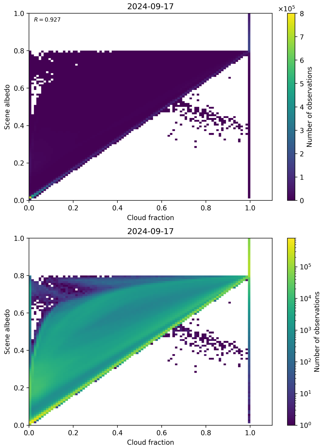
Figure 82: Scatter density plot of “Cloud fraction” against “Scene albedo” for 2024-09-17 to 2024-09-18.
