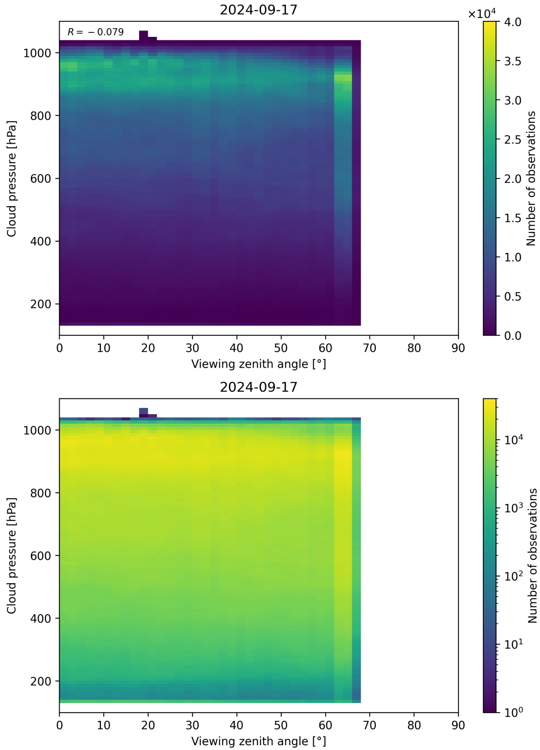
Figure 133: Scatter density plot of “Viewing zenith angle” against “Cloud pressure” for 2024-09-17 to 2024-09-18.
