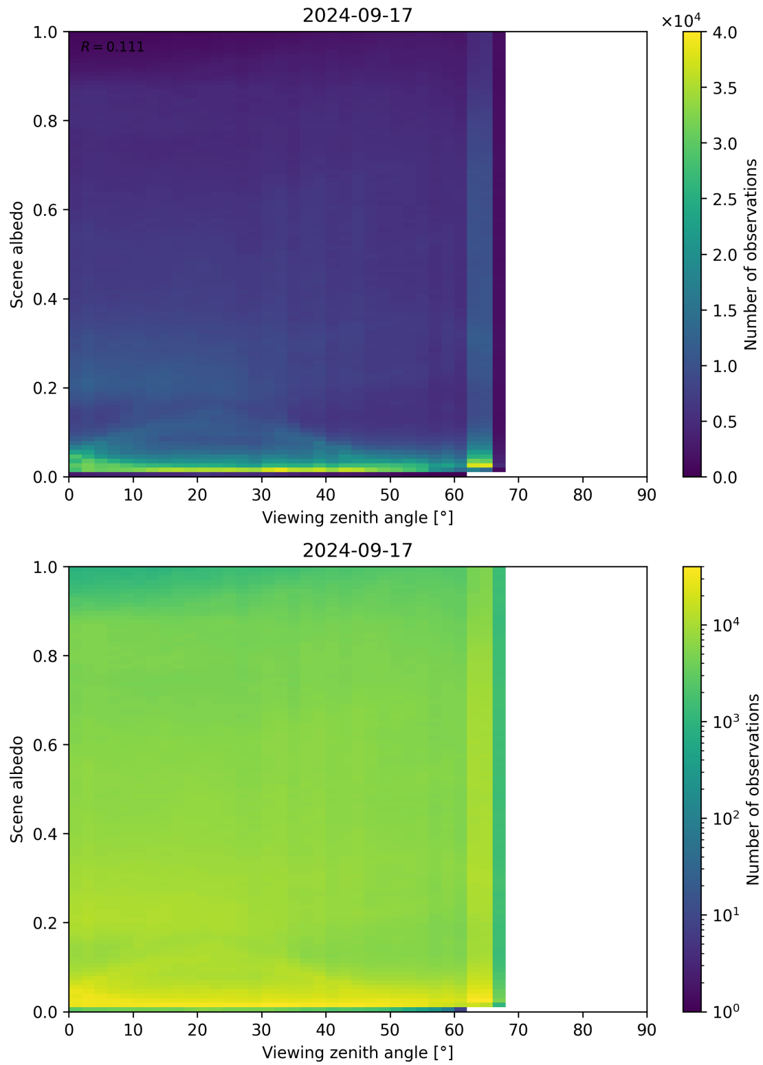
Figure 138: Scatter density plot of “Viewing zenith angle” against “Scene albedo” for 2024-09-17 to 2024-09-18.
