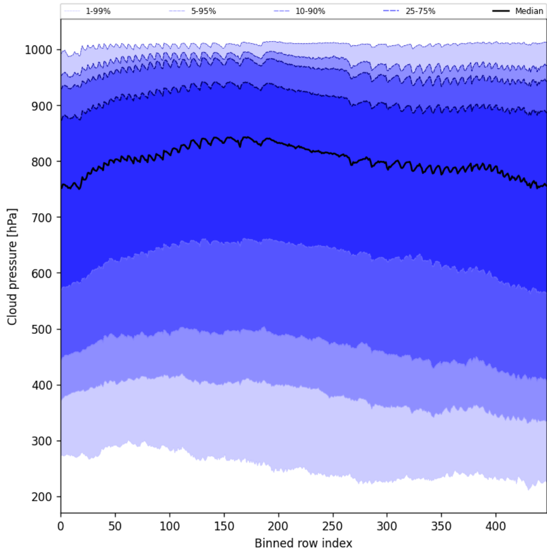
Figure 47: Along track statistics of “Cloud pressure” for 2024-09-17 to 2024-09-18
