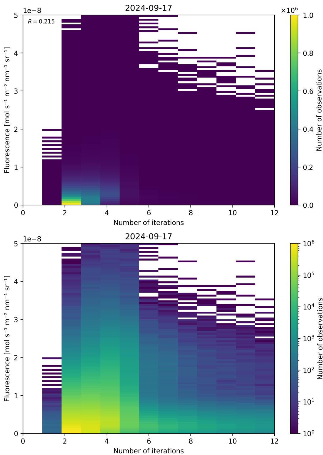
Figure 107: Scatter density plot of “Number of iterations” against “Fluorescence” for 2024-09-17 to 2024-09-18.
