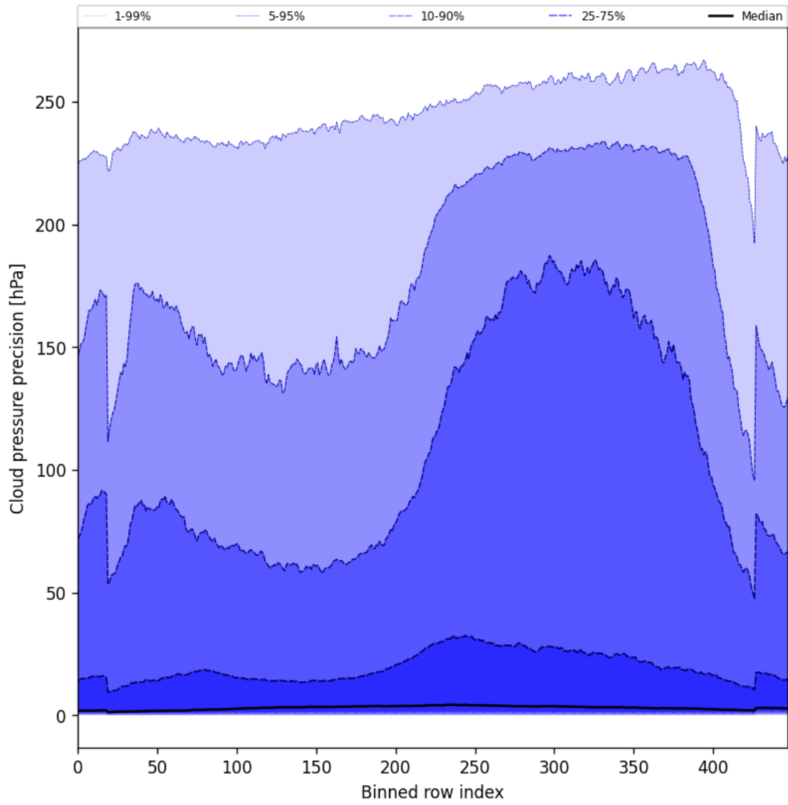
Figure 48: Along track statistics of “Cloud pressure precision” for 2024-09-17 to 2024-09-18
