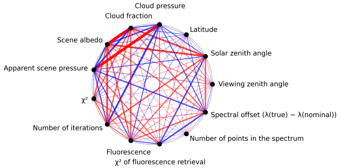
Figure 1: Map of correlation graph for 2024-09-17 to 2024-09-18.
