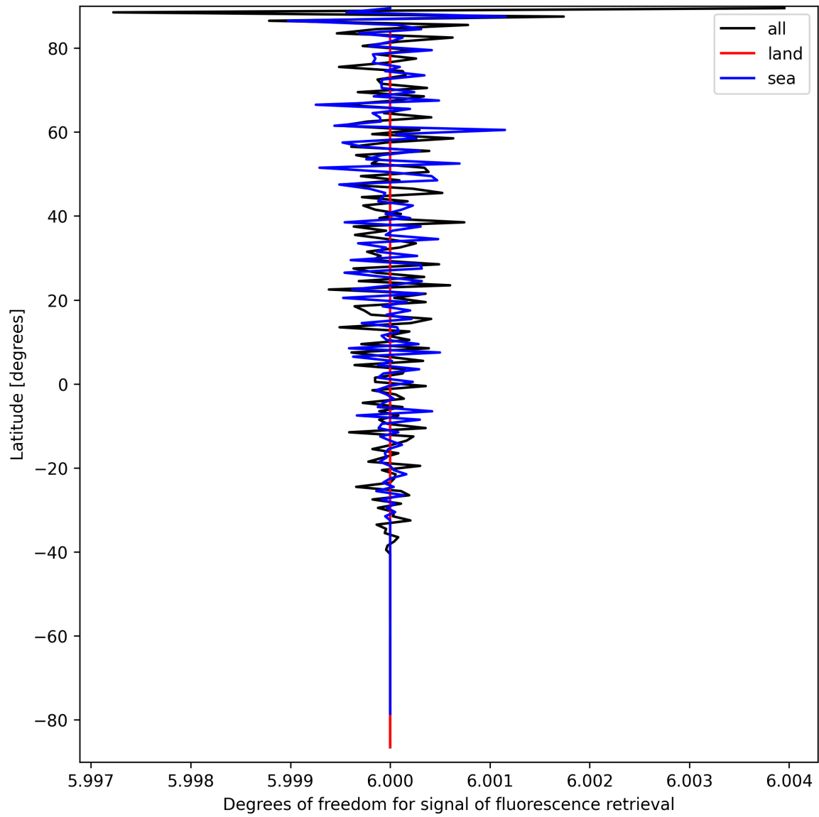
Figure 26: Zonal average of “Degrees of freedom for signal of fluorescence retrieval” for 2024-09-17 to 2024-09-18.
