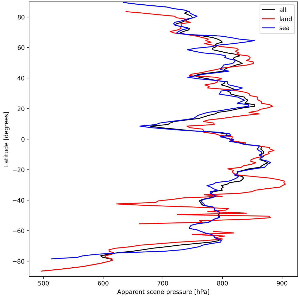
Figure 19: Zonal average of “Apparent scene pressure” for 2024-09-17 to 2024-09-18.
