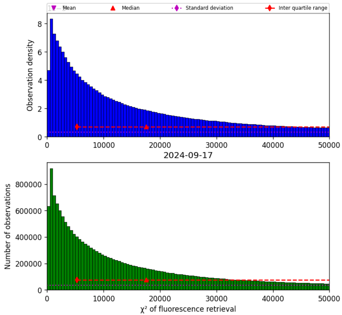
Figure 42: Histogram of “ \chi^2 of fluorescence retrieval” for 2024-09-17 to 2024-09-18
