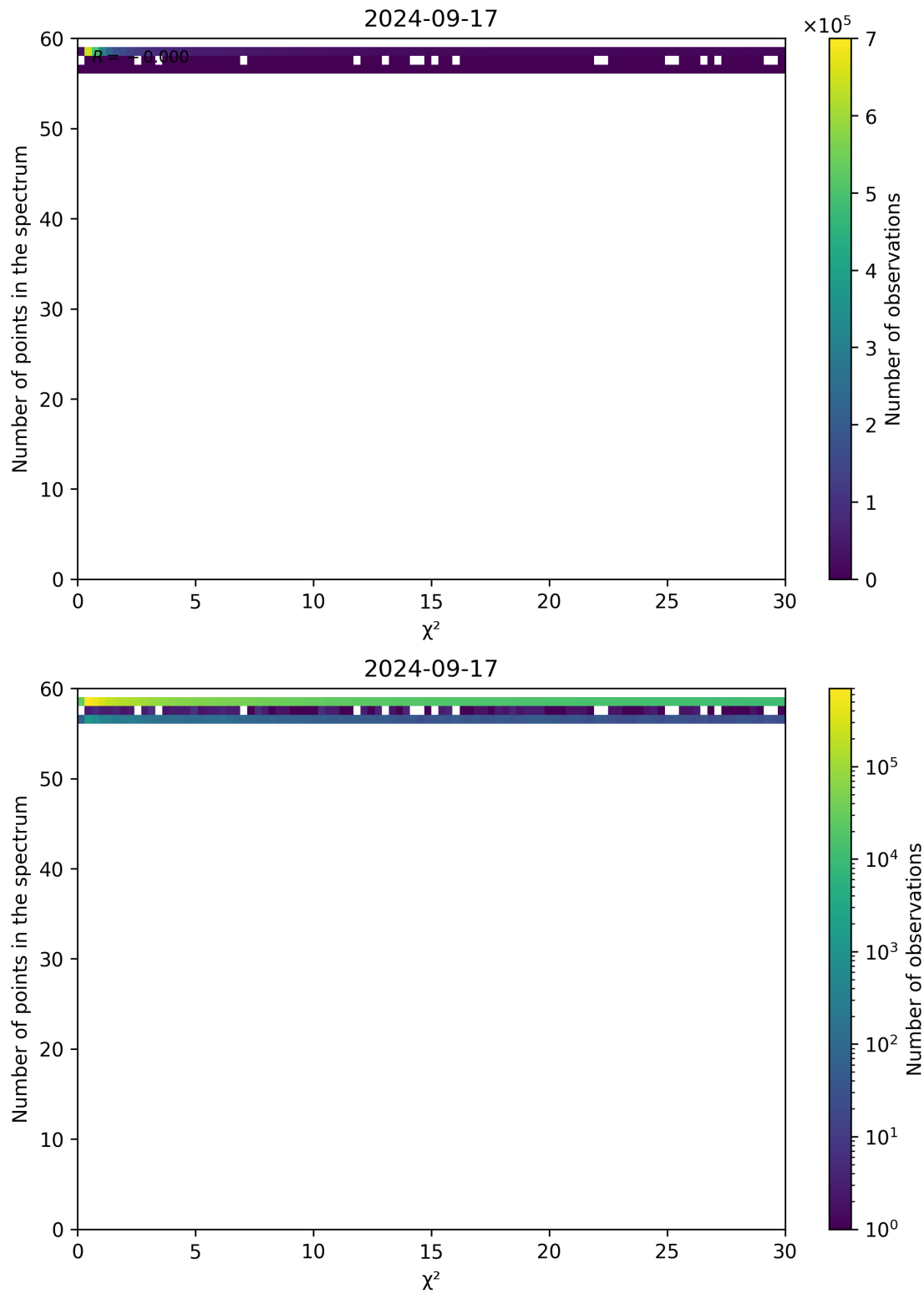
Figure 74: Scatter density plot of " \chi^2 " against "Number of points in the spectrum" for 2024-09-17 to 2024-09-18.
