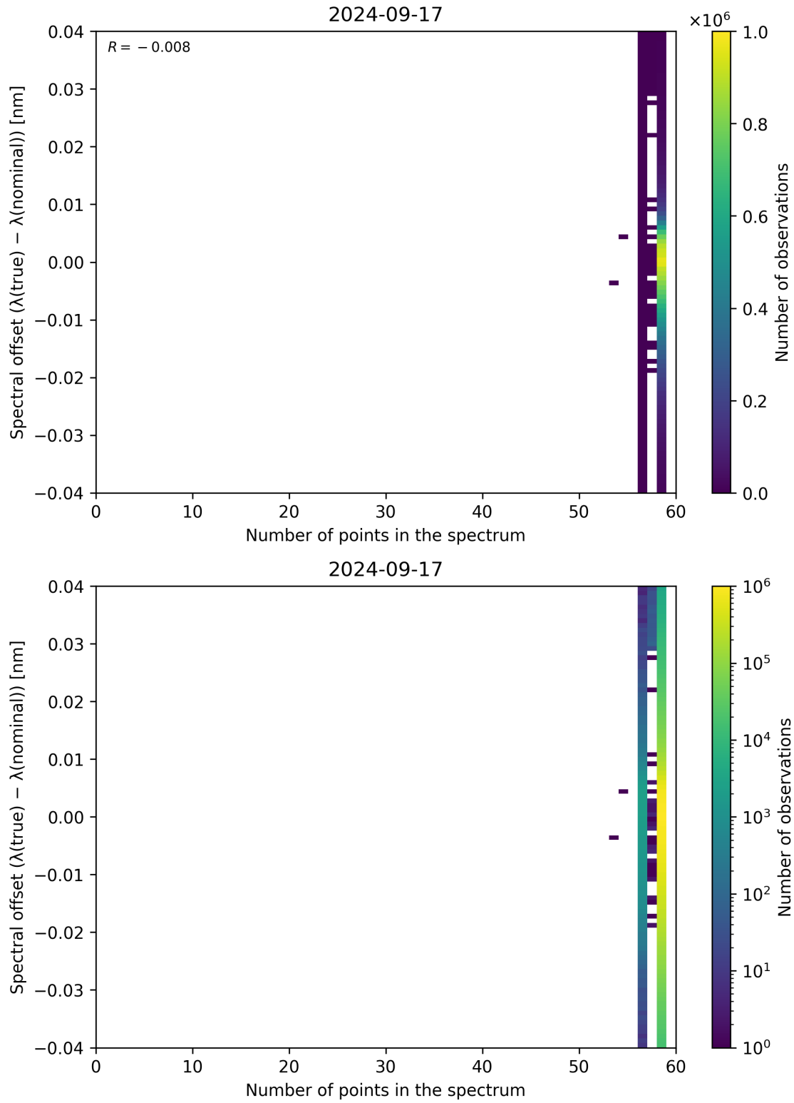
Figure 110: Scatter density plot of “Number of points in the spectrum” against “Spectral offset ( \lambda_{\text{true}} - \lambda_{\text{nominal}} )” for 2024-09-17 to 2024-09-18.
