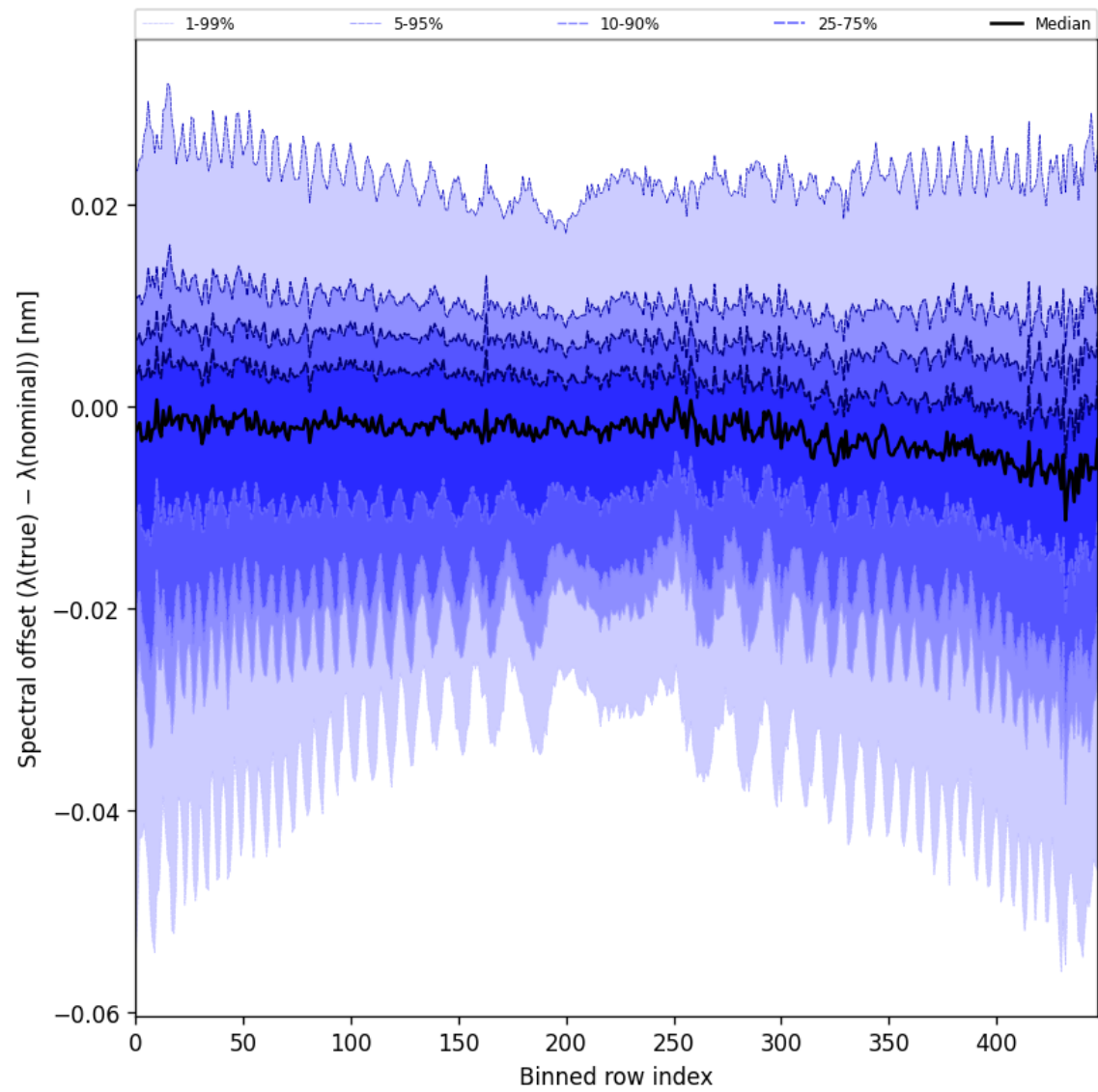
Figure 62: Along track statistics of “Spectral offset ( \lambda_{\text{true}} - \lambda_{\text{nominal}} )” for 2024-09-17 to 2024-09-18
