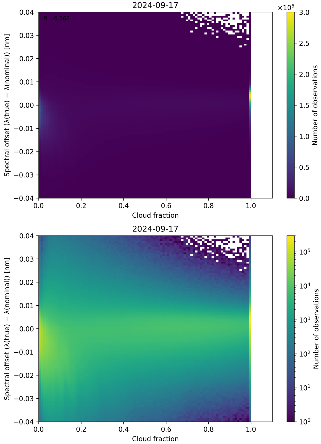
Figure 83: Scatter density plot of “Cloud fraction” against “Spectral offset ( \lambda_{\text{true}} - \lambda_{\text{nominal}} )” for 2024-09-17 to 2024-09-18.
