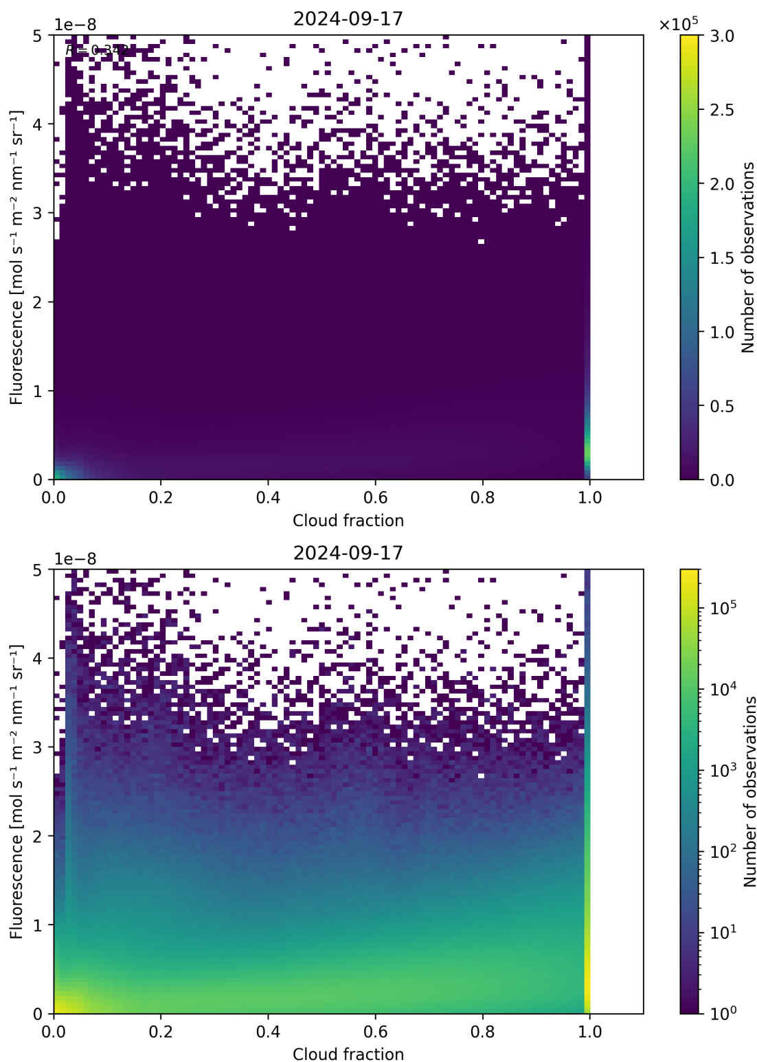
Figure 79: Scatter density plot of “Cloud fraction” against “Fluorescence” for 2024-09-17 to 2024-09-18.
