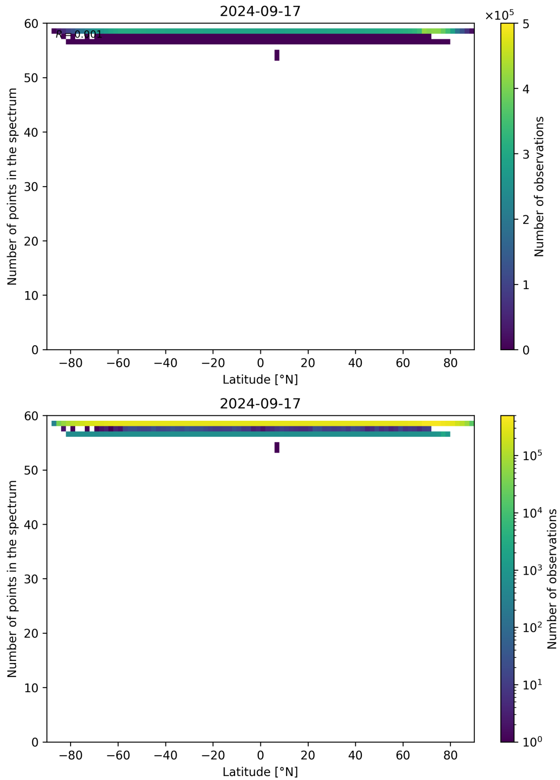
Figure 103: Scatter density plot of “Latitude” against “Number of points in the spectrum” for 2024-09-17 to 2024-09-18.
