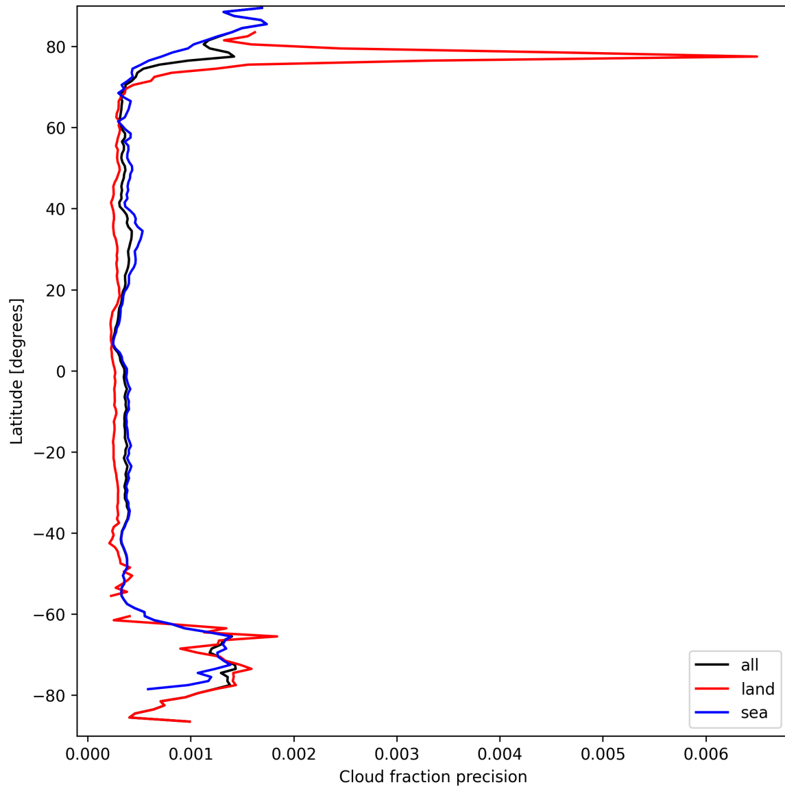
Figure 16: Zonal average of “Cloud fraction precision” for 2024-09-17 to 2024-09-18.
