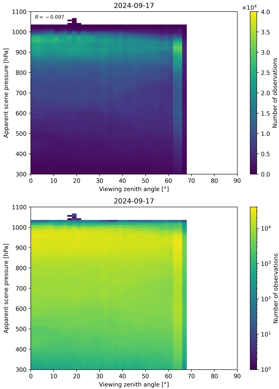
Figure 129: Scatter density plot of “Viewing zenith angle” against “Apparent scene pressure” for 2024-09-17 to 2024-09-18.
