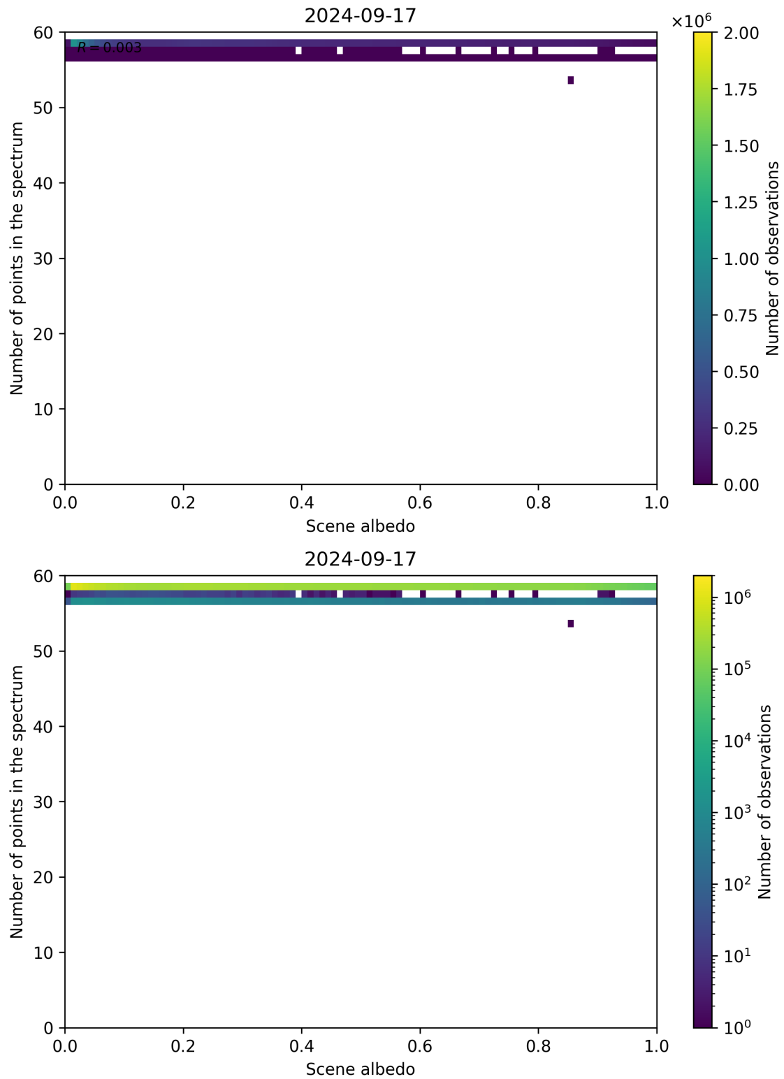
Figure 116: Scatter density plot of “Scene albedo” against “Number of points in the spectrum” for 2024-09-17 to 2024-09-18.
