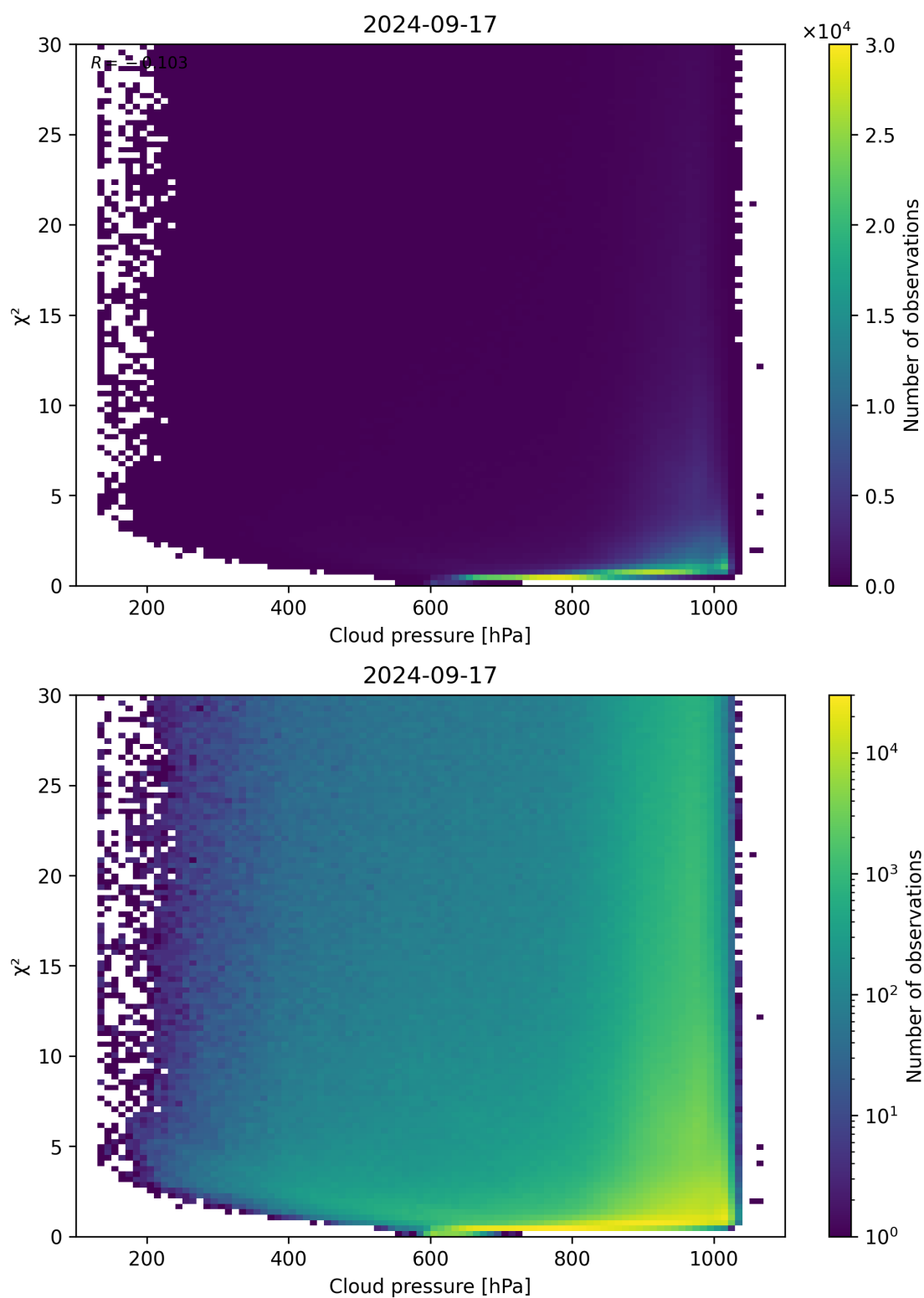
Figure 85: Scatter density plot of “Cloud pressure” against “ \chi^2 ” for 2024-09-17 to 2024-09-18.
