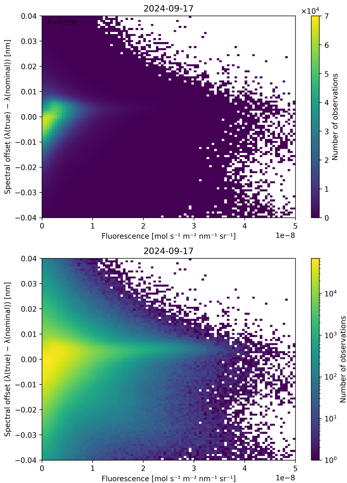
Figure 95: Scatter density plot of “Fluorescence” against “Spectral offset ( \lambda_{\text{true}} - \lambda_{\text{nominal}} )” for 2024-09-17 to 2024-09-18.
