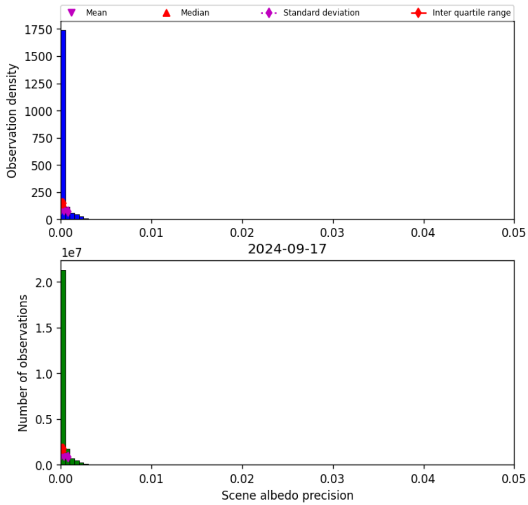
Figure 35: Histogram of “Scene albedo precision” for 2024-09-17 to 2024-09-18
