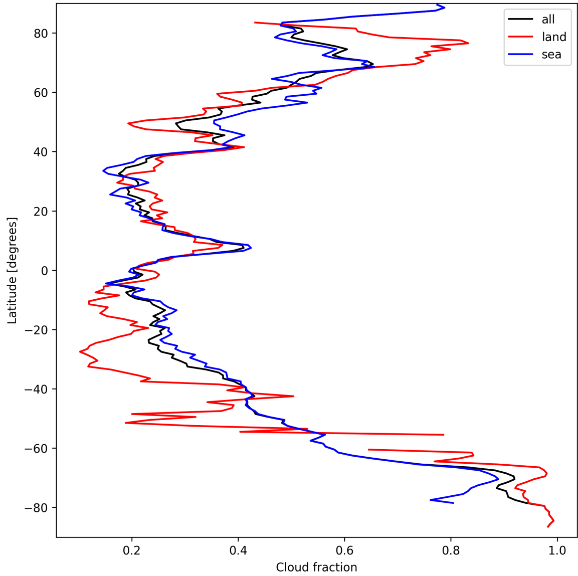
Figure 15: Zonal average of “Cloud fraction” for 2024-09-17 to 2024-09-18.
