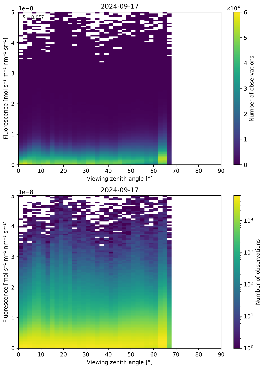
Figure 134: Scatter density plot of “Viewing zenith angle” against “Fluorescence” for 2024-09-17 to 2024-09-18.
