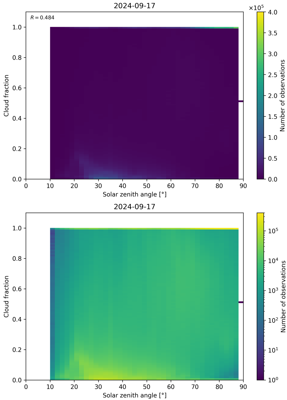
Figure 121: Scatter density plot of “Solar zenith angle” against “Cloud fraction” for 2024-09-17 to 2024-09-18.
