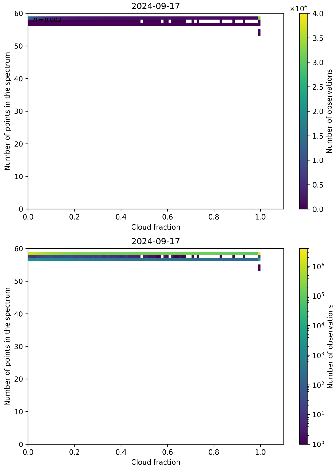
Figure 81: Scatter density plot of “Cloud fraction” against “Number of points in the spectrum” for 2024-09-17 to 2024-09-18.
