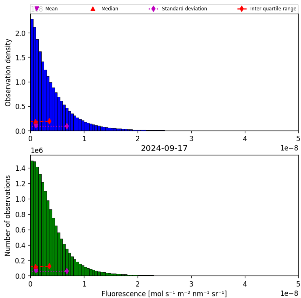
Figure 40: Histogram of “Fluorescence” for 2024-09-17 to 2024-09-18
