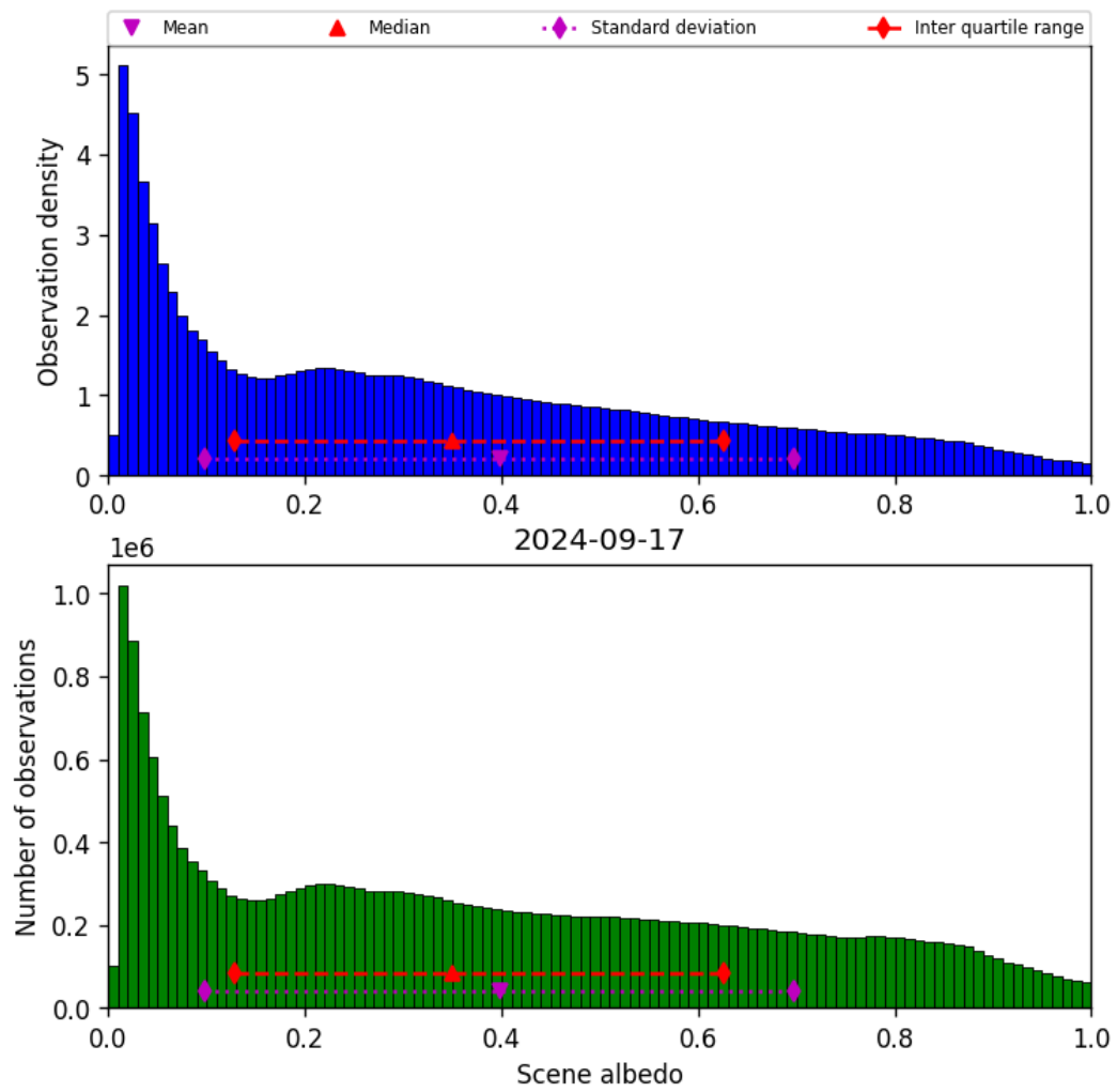
Figure 34: Histogram of “Scene albedo” for 2024-09-17 to 2024-09-18
