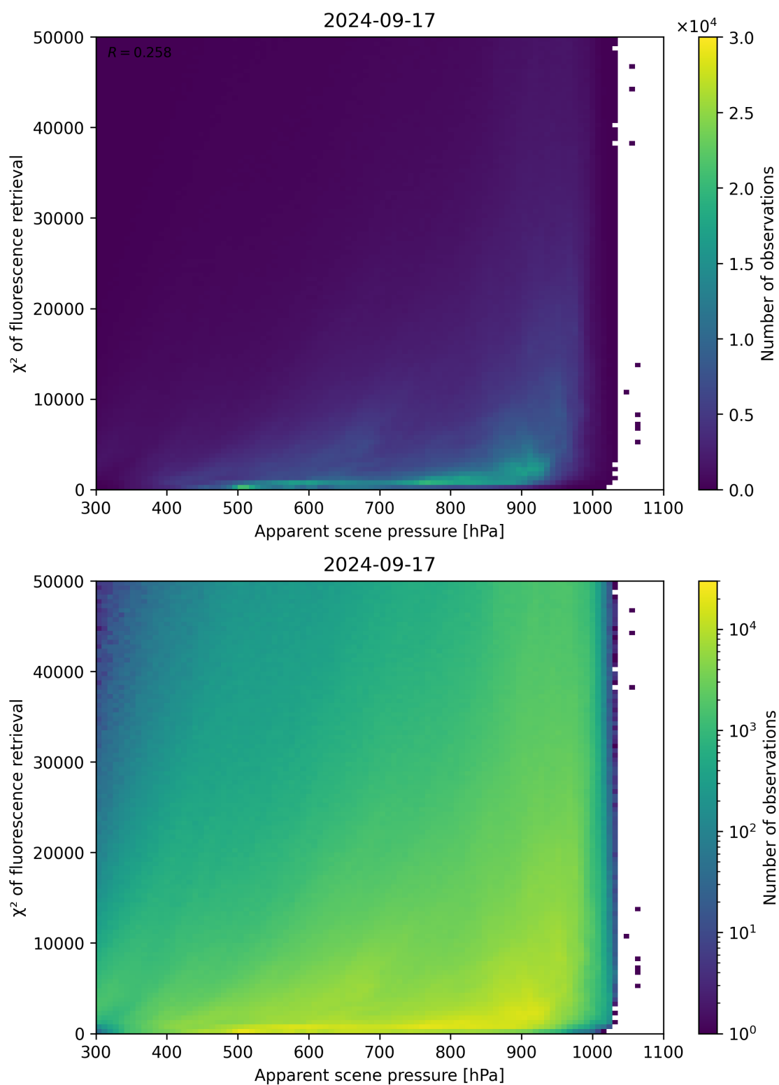
Figure 64: Scatter density plot of “Apparent scene pressure” against “ \chi^2 of fluorescence retrieval” for 2024-09-17 to 2024-09-18.
