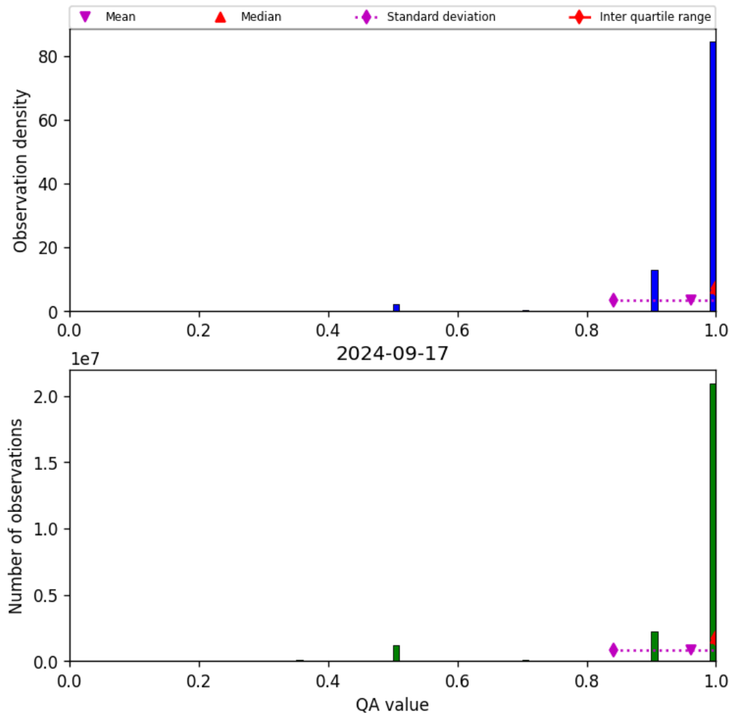
Figure 29: Histogram of “QA value” for 2024-09-17 to 2024-09-18
