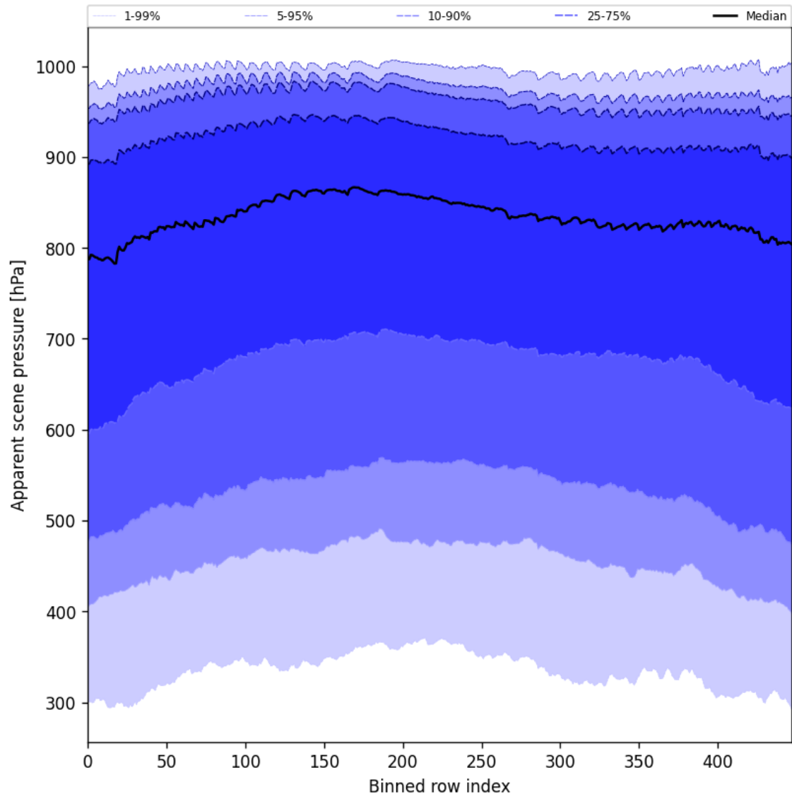
Figure 53: Along track statistics of “Apparent scene pressure” for 2024-09-17 to 2024-09-18
