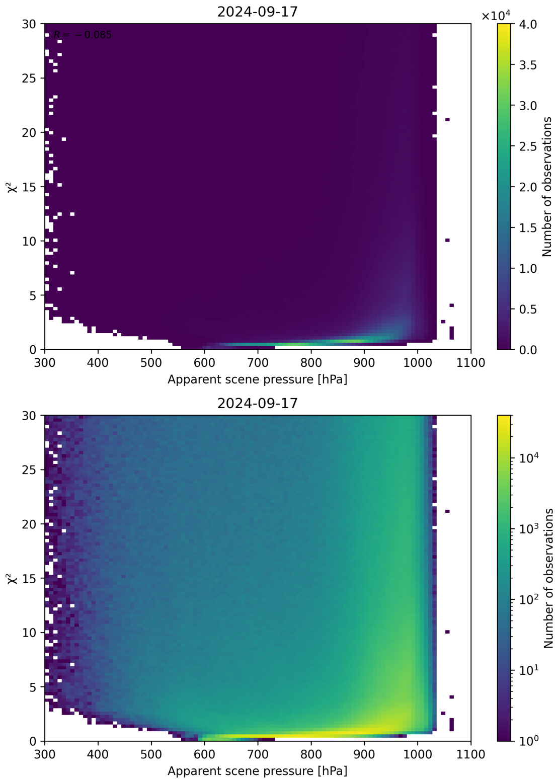
Figure 63: Scatter density plot of “Apparent scene pressure” against “ \chi^2 ” for 2024-09-17 to 2024-09-18.
