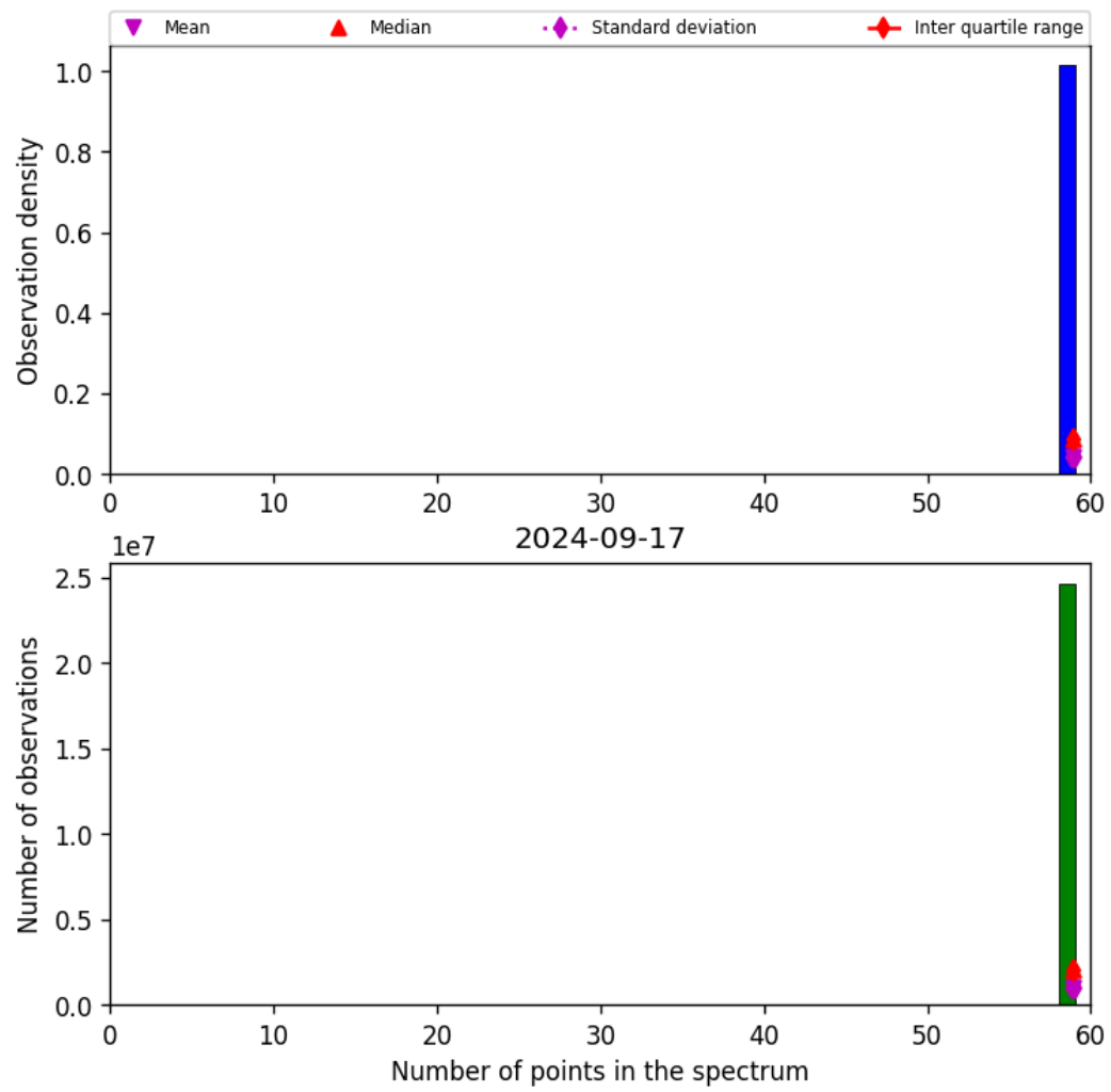
Figure 44: Histogram of “Number of points in the spectrum” for 2024-09-17 to 2024-09-18
