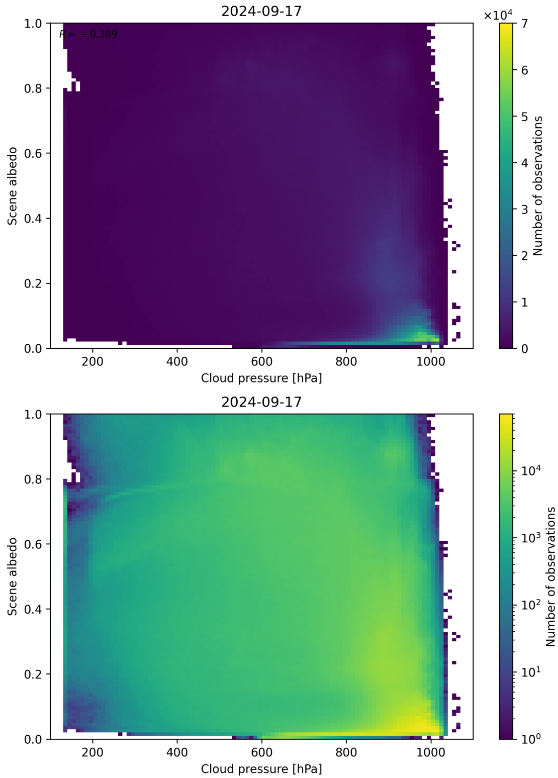
Figure 91: Scatter density plot of “Cloud pressure” against “Scene albedo” for 2024-09-17 to 2024-09-18.
