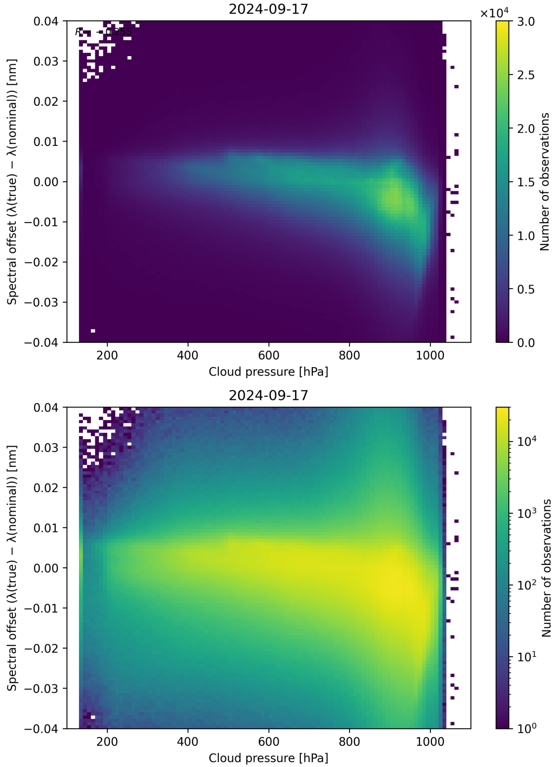
Figure 92: Scatter density plot of “Cloud pressure” against “Spectral offset ( \lambda_{\text{true}} - \lambda_{\text{nominal}} )” for 2024-09-17 to 2024-09-18.
