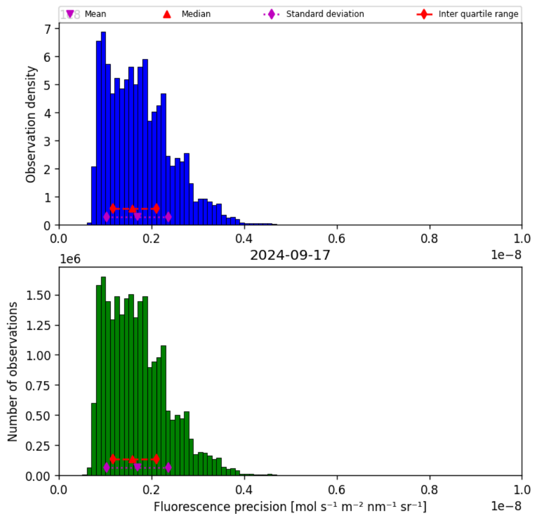
Figure 41: Histogram of “Fluorescence precision” for 2024-09-17 to 2024-09-18
