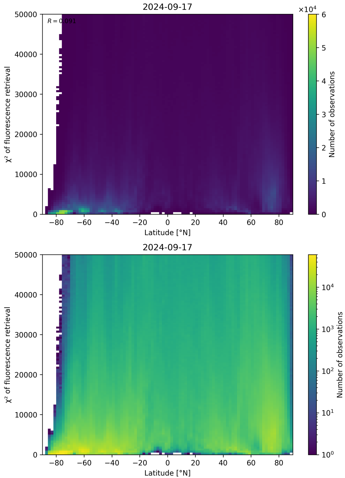
Figure 98: Scatter density plot of “Latitude” against “ \chi^2 of fluorescence retrieval” for 2024-09-17 to 2024-09-18.
