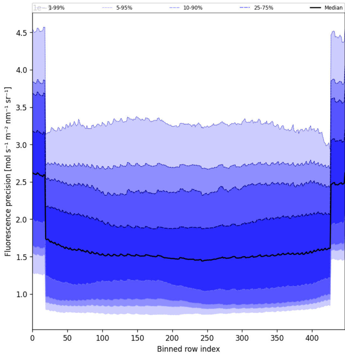
Figure 58: Along track statistics of “Fluorescence precision” for 2024-09-17 to 2024-09-18
