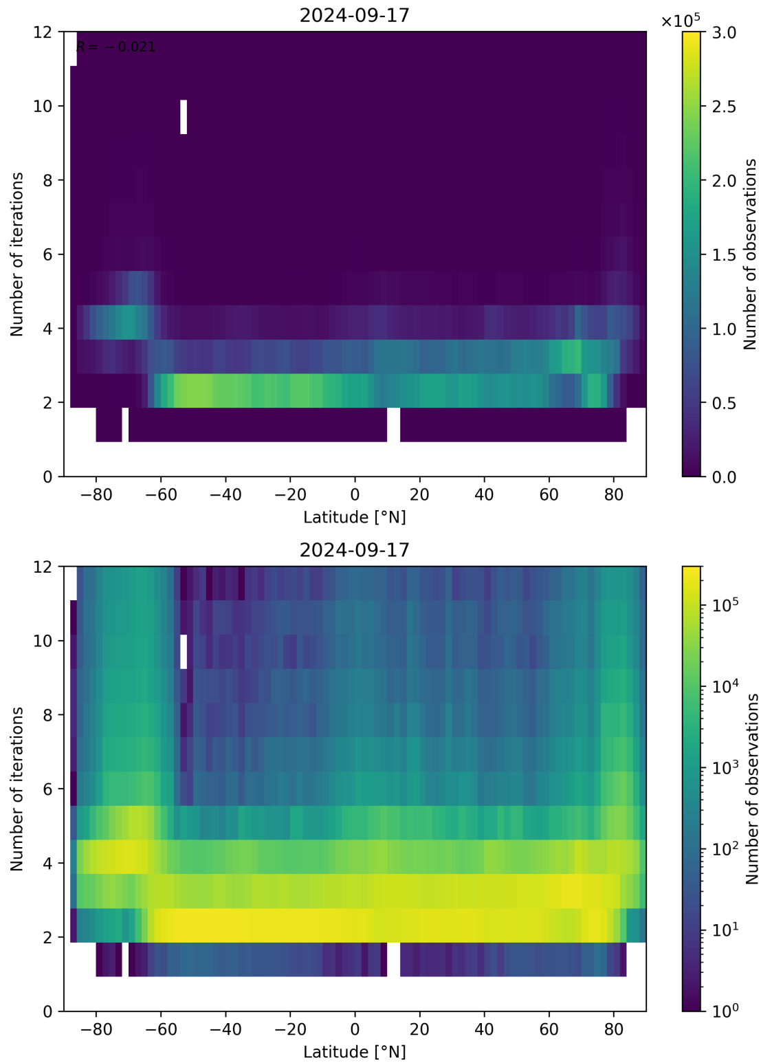
Figure 102: Scatter density plot of “Latitude” against “Number of iterations” for 2024-09-17 to 2024-09-18.
