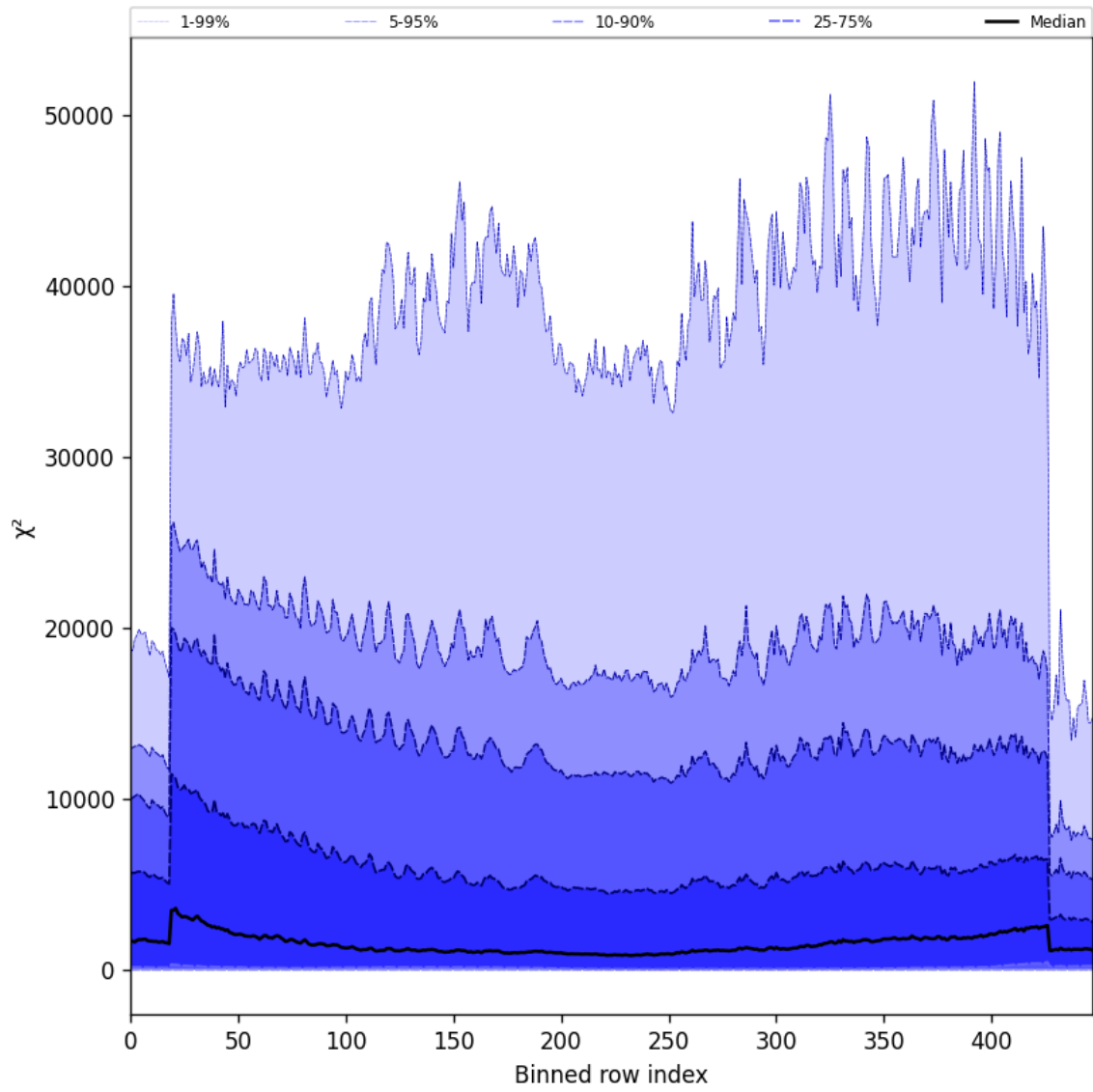
Figure 55: Along track statistics of “ \chi^2 ” for 2024-09-17 to 2024-09-18
