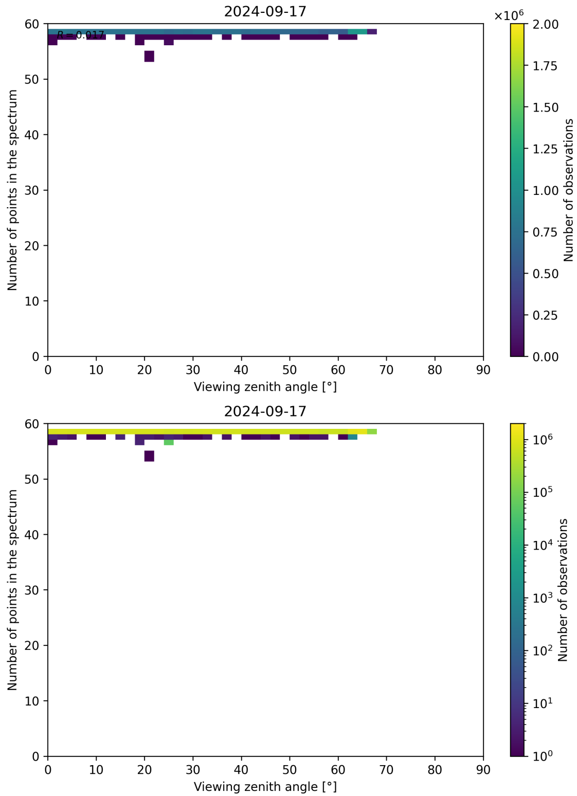
Figure 137: Scatter density plot of “Viewing zenith angle” against “Number of points in the spectrum” for 2024-09-17 to 2024-09-18.
