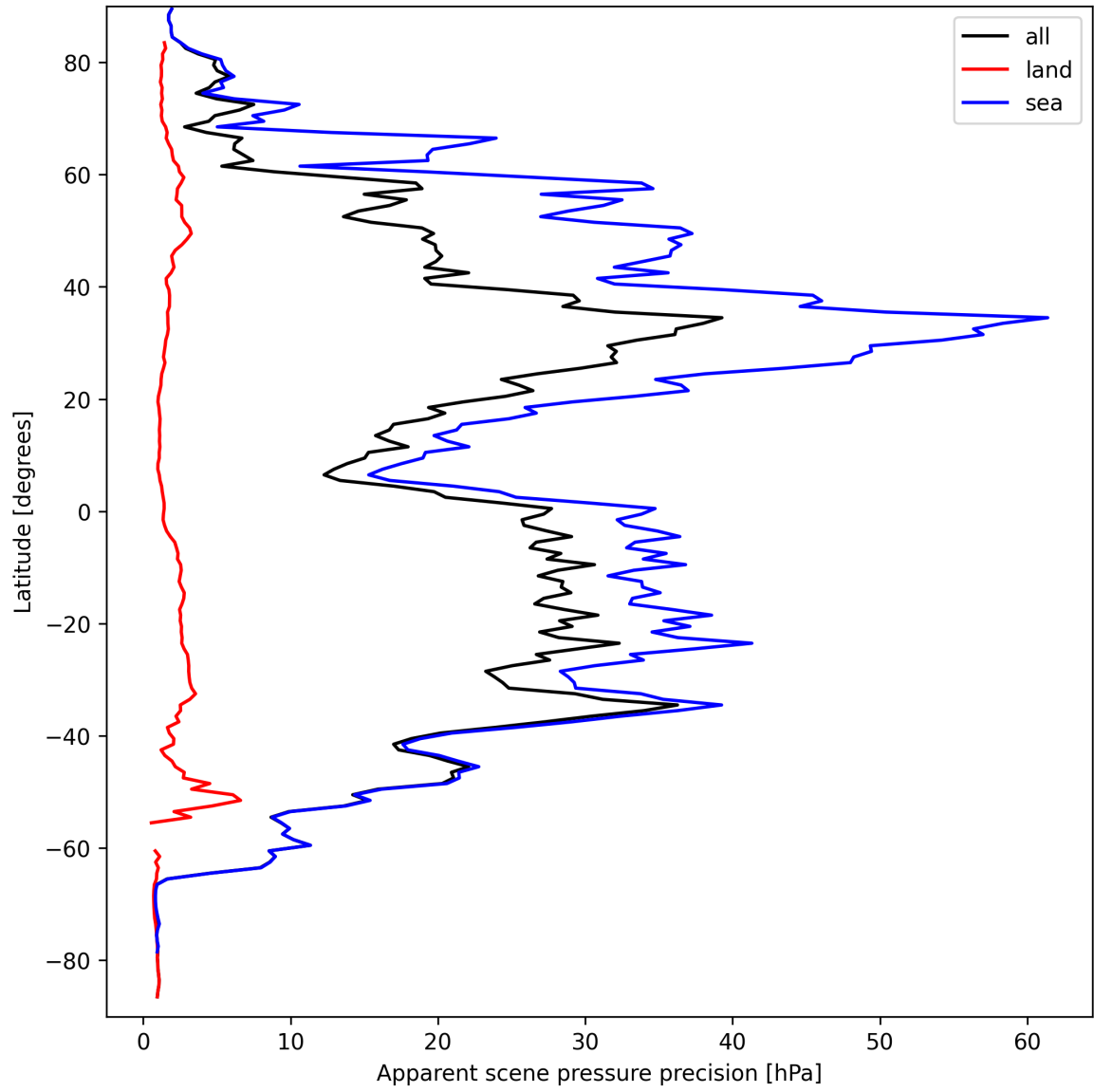
Figure 20: Zonal average of “Apparent scene pressure precision” for 2024-09-17 to 2024-09-18.
