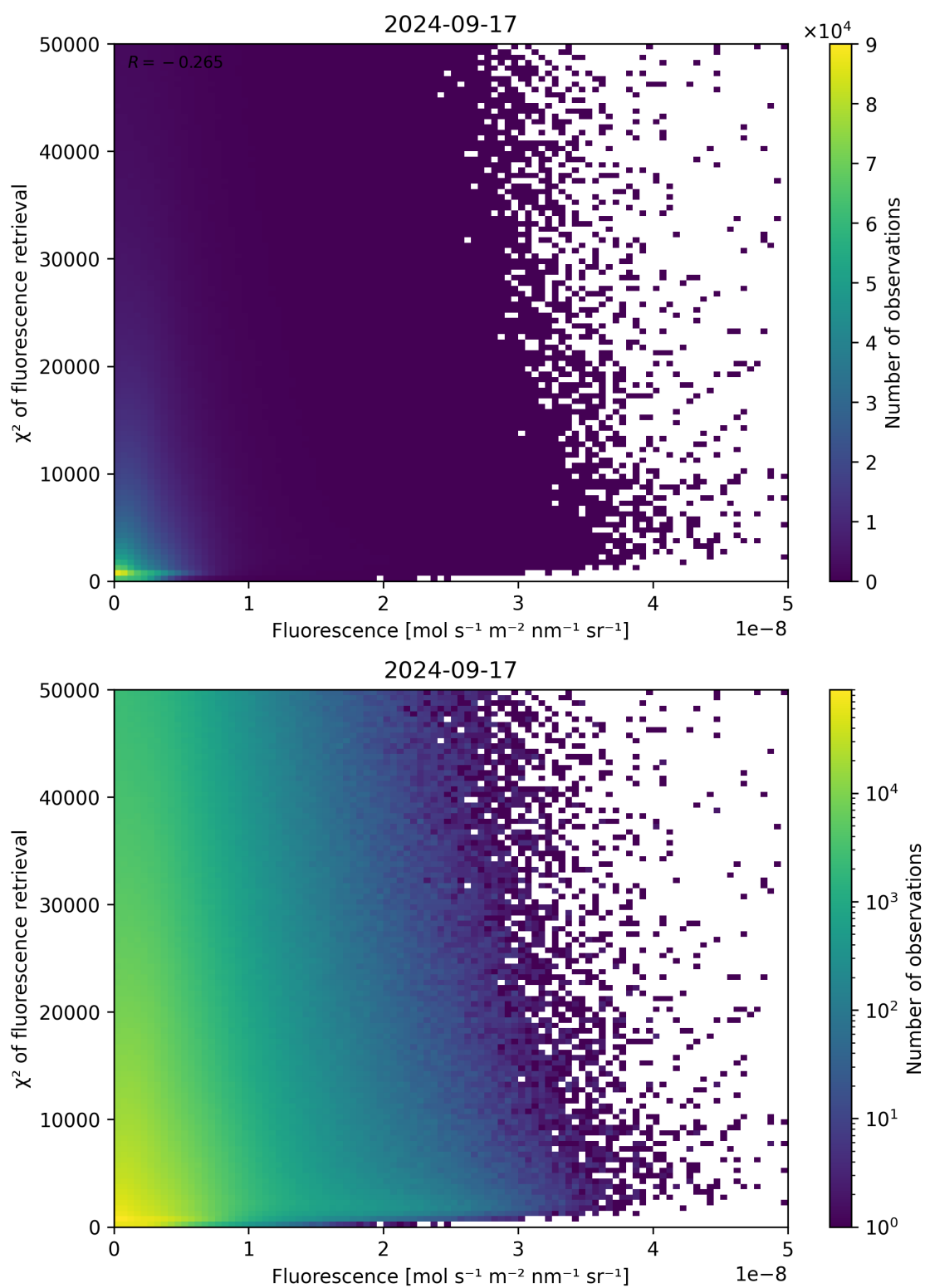
Figure 93: Scatter density plot of “Fluorescence” against “ \chi^2 of fluorescence retrieval” for 2024-09-17 to 2024-09-18.
