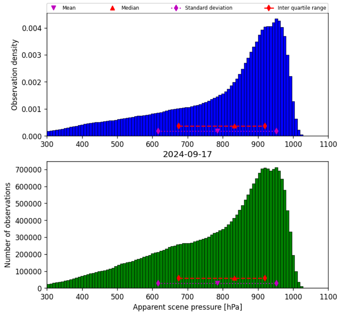
Figure 36: Histogram of “Apparent scene pressure” for 2024-09-17 to 2024-09-18
