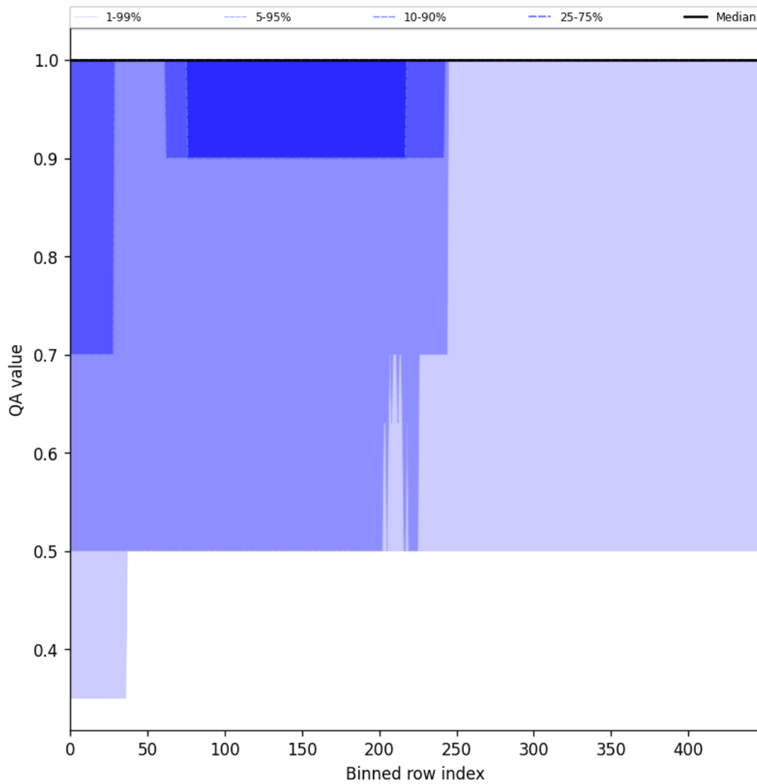
Figure 46: Along track statistics of “QA value” for 2024-09-17 to 2024-09-18
