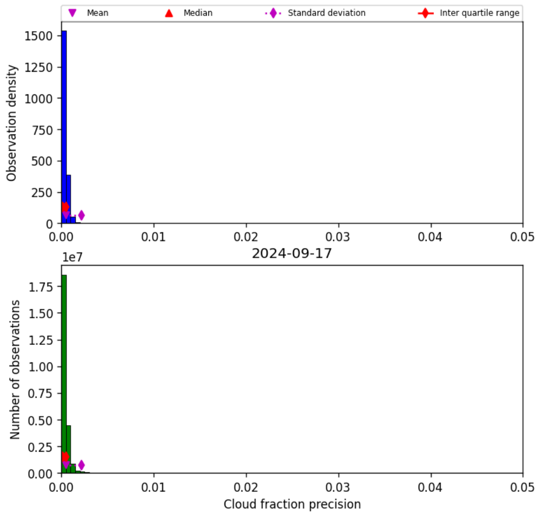
Figure 33: Histogram of “Cloud fraction precision” for 2024-09-17 to 2024-09-18
