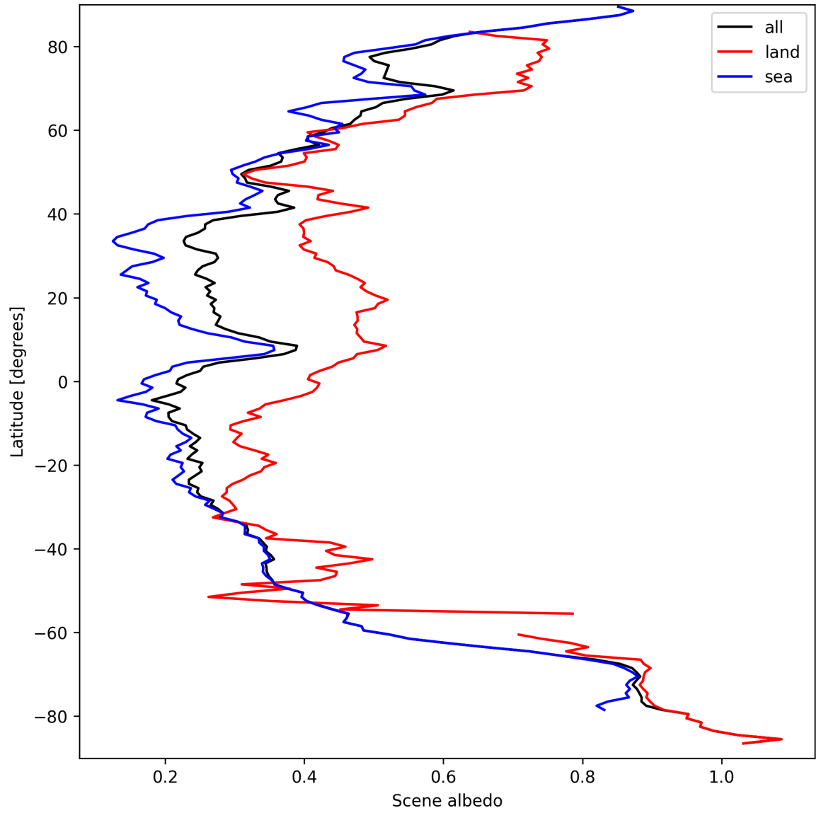
Figure 17: Zonal average of “Scene albedo” for 2024-09-17 to 2024-09-18.
