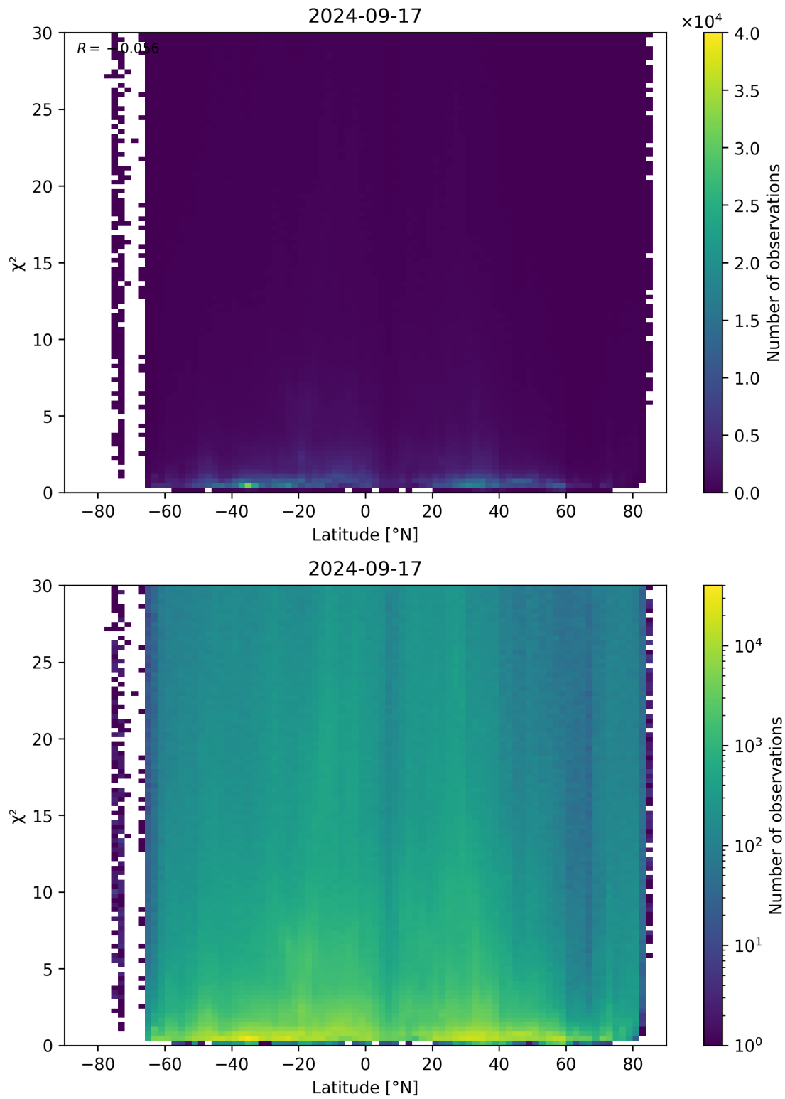
Figure 97: Scatter density plot of “Latitude” against “ \chi^2 ” for 2024-09-17 to 2024-09-18.
