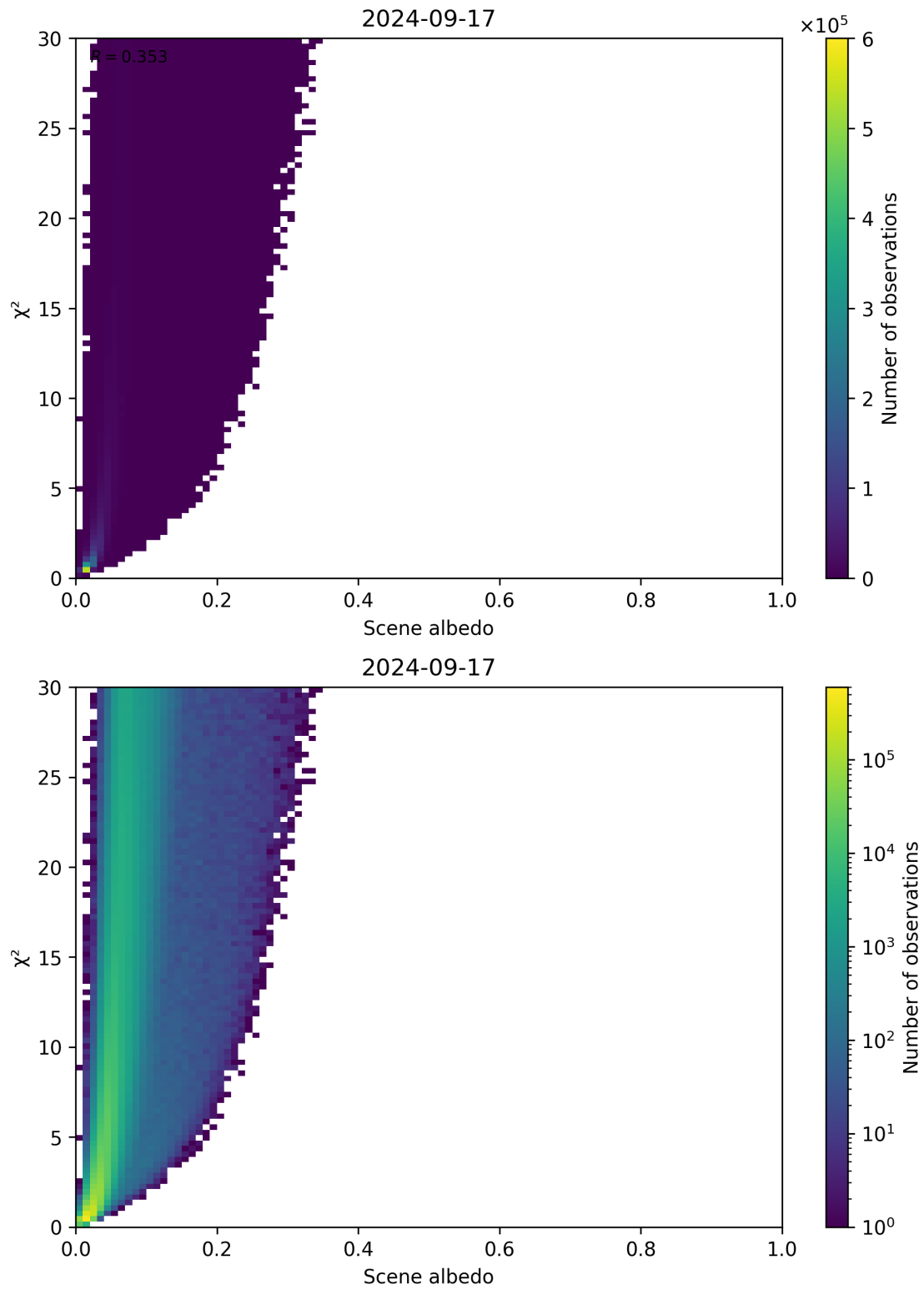
Figure 112: Scatter density plot of “Scene albedo” against “ \chi^2 ” for 2024-09-17 to 2024-09-18.
