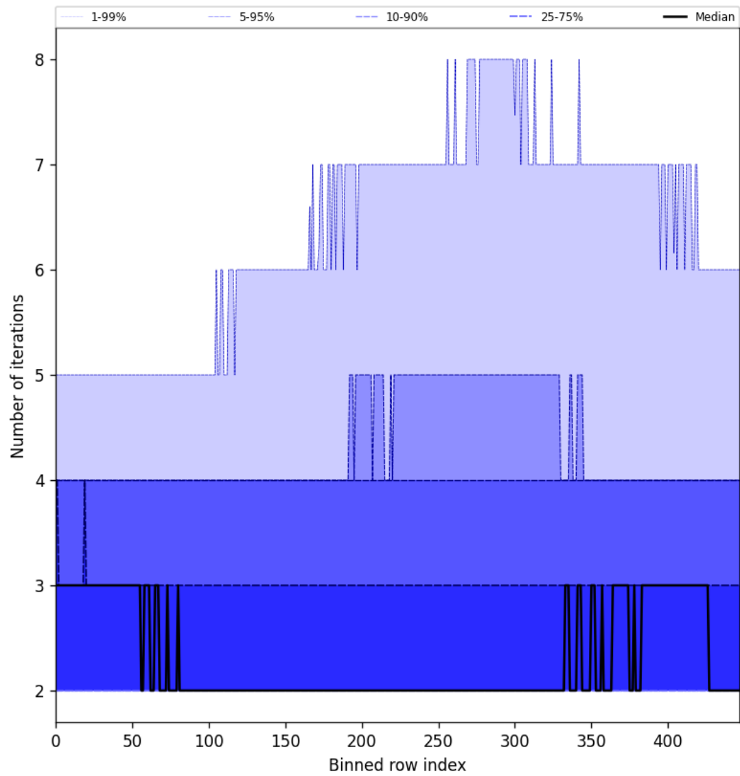
Figure 56: Along track statistics of “Number of iterations” for 2024-09-17 to 2024-09-18
