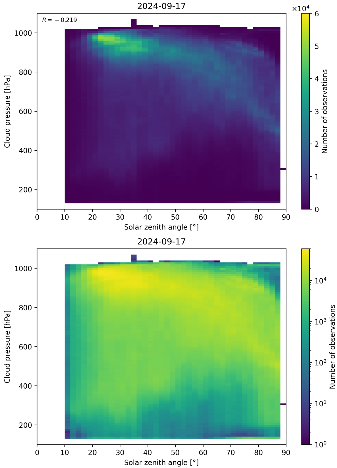
Figure 122: Scatter density plot of “Solar zenith angle” against “Cloud pressure” for 2024-09-17 to 2024-09-18.
