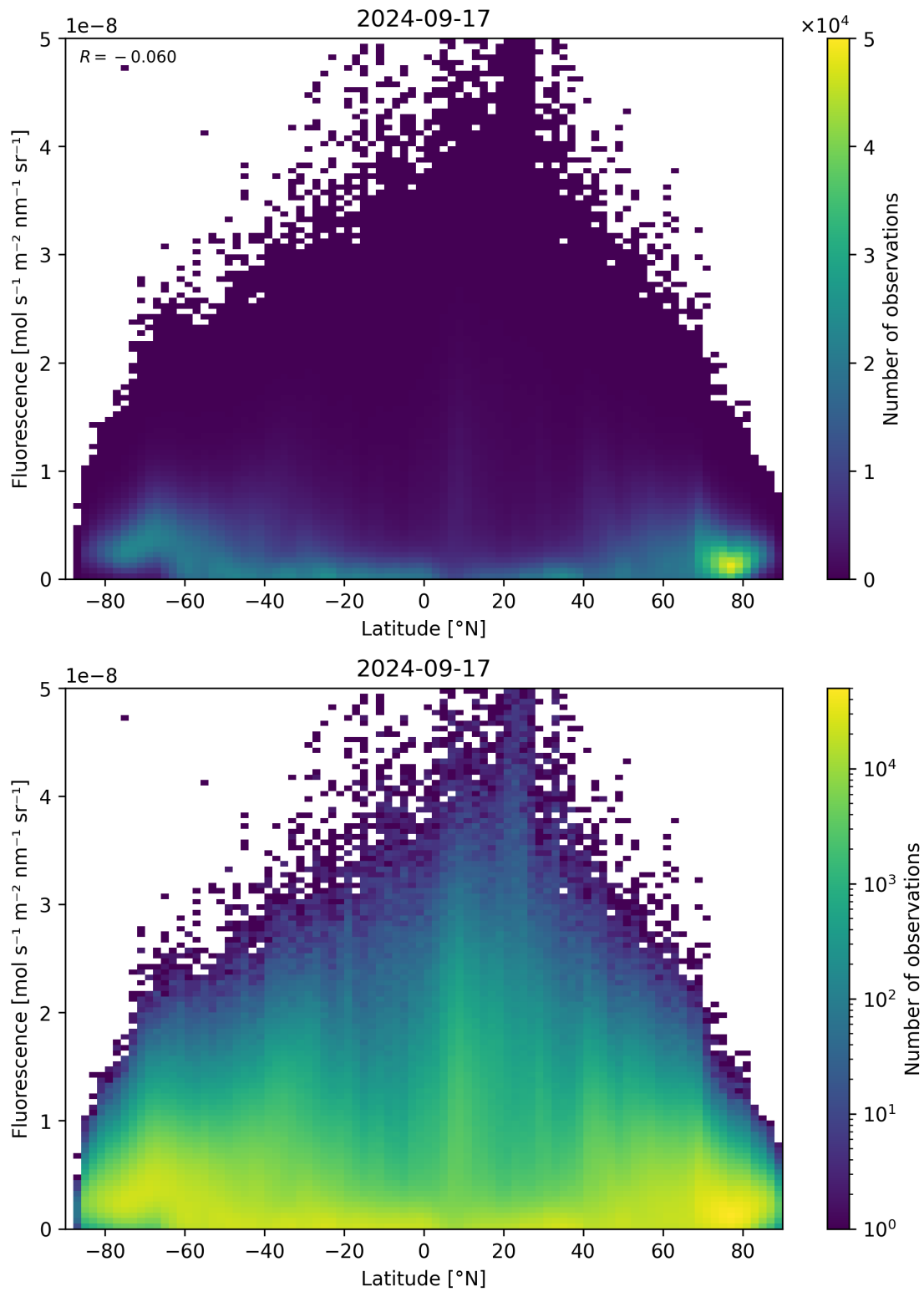
Figure 101: Scatter density plot of “Latitude” against “Fluorescence” for 2024-09-17 to 2024-09-18.
