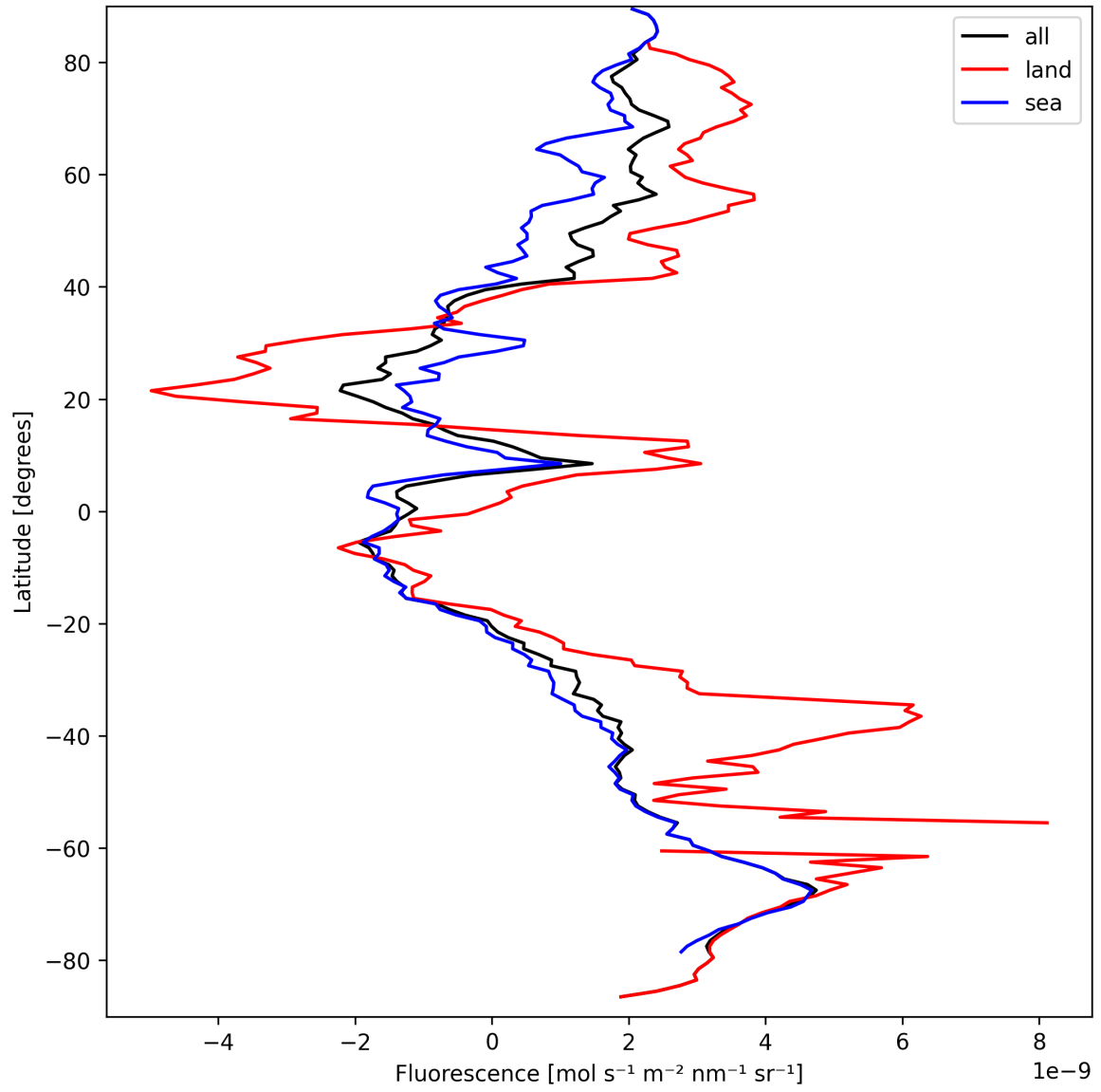
Figure 23: Zonal average of “Fluorescence” for 2024-09-17 to 2024-09-18.
