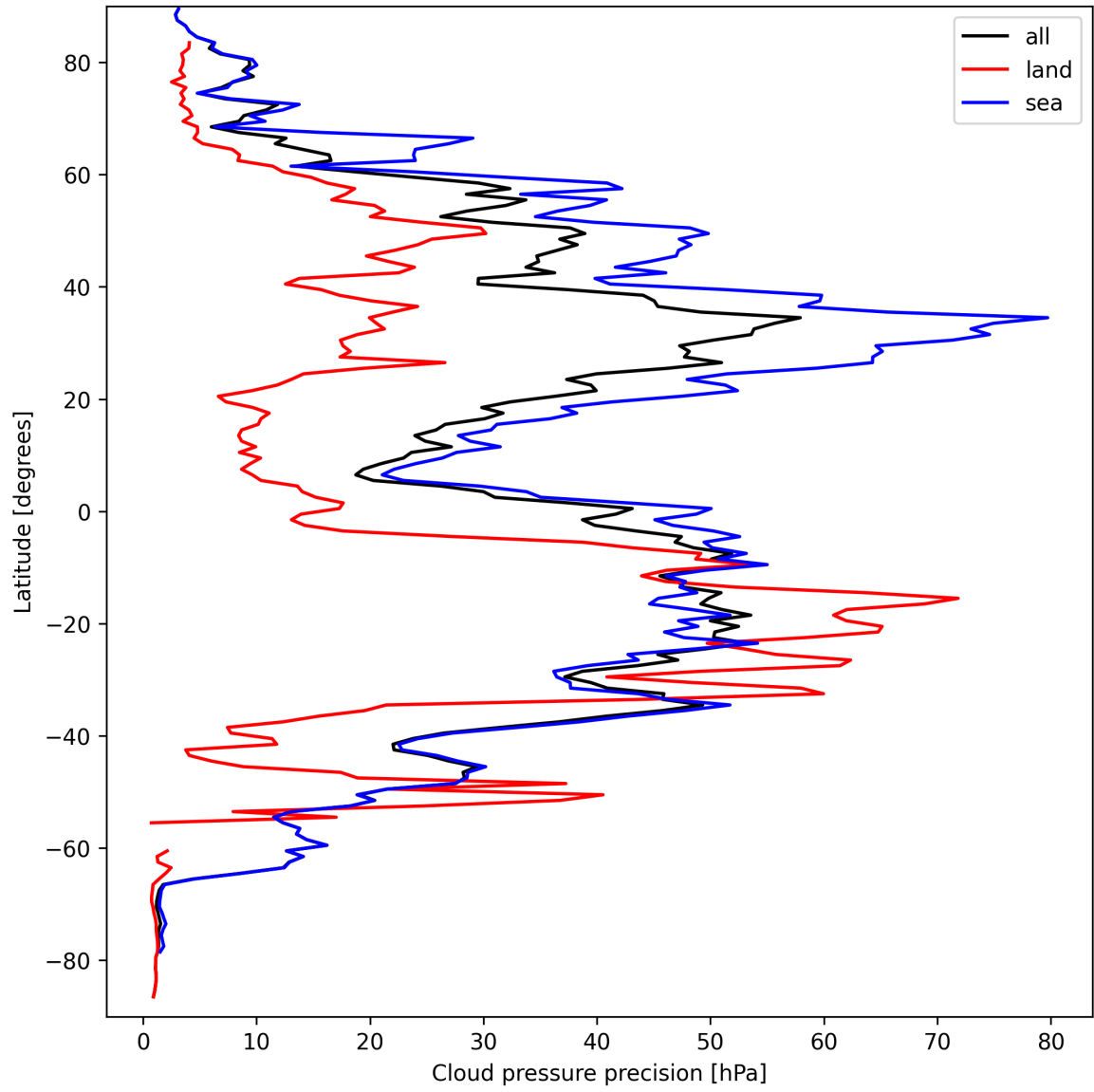
Figure 14: Zonal average of “Cloud pressure precision” for 2024-09-17 to 2024-09-18.
