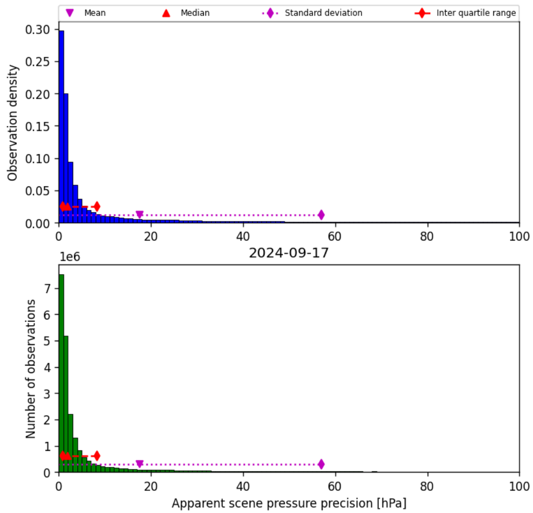
Figure 37: Histogram of “Apparent scene pressure precision” for 2024-09-17 to 2024-09-18
