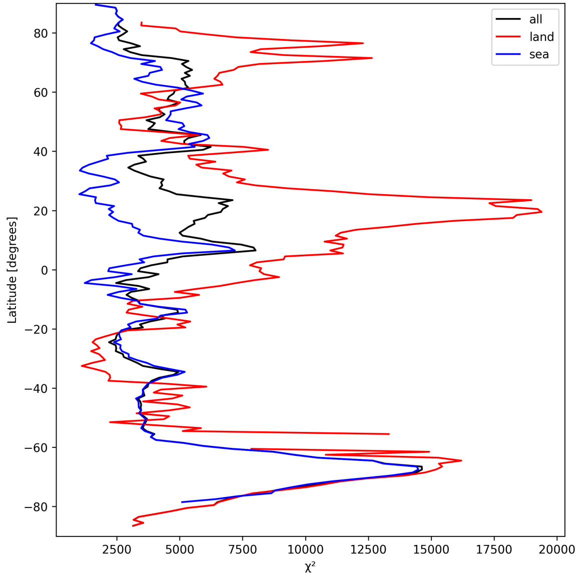
Figure 21: Zonal average of “ \chi^2 ” for 2024-09-17 to 2024-09-18.
