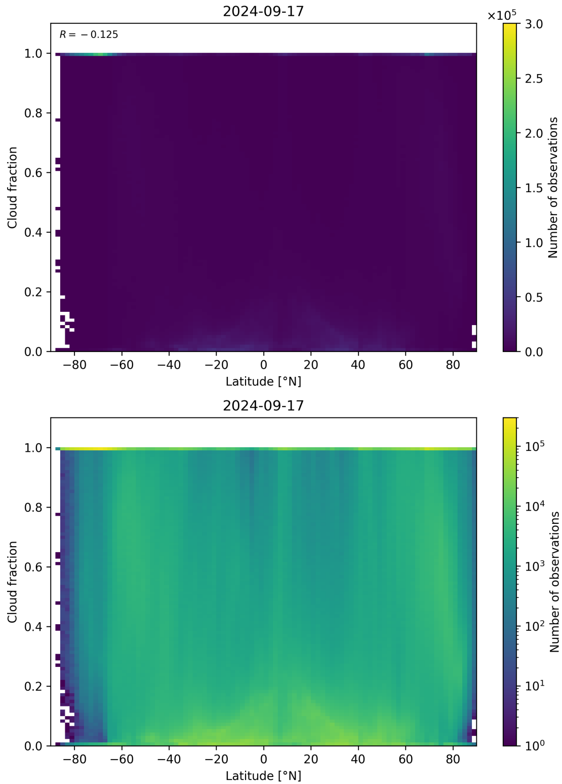
Figure 99: Scatter density plot of “Latitude” against “Cloud fraction” for 2024-09-17 to 2024-09-18.
