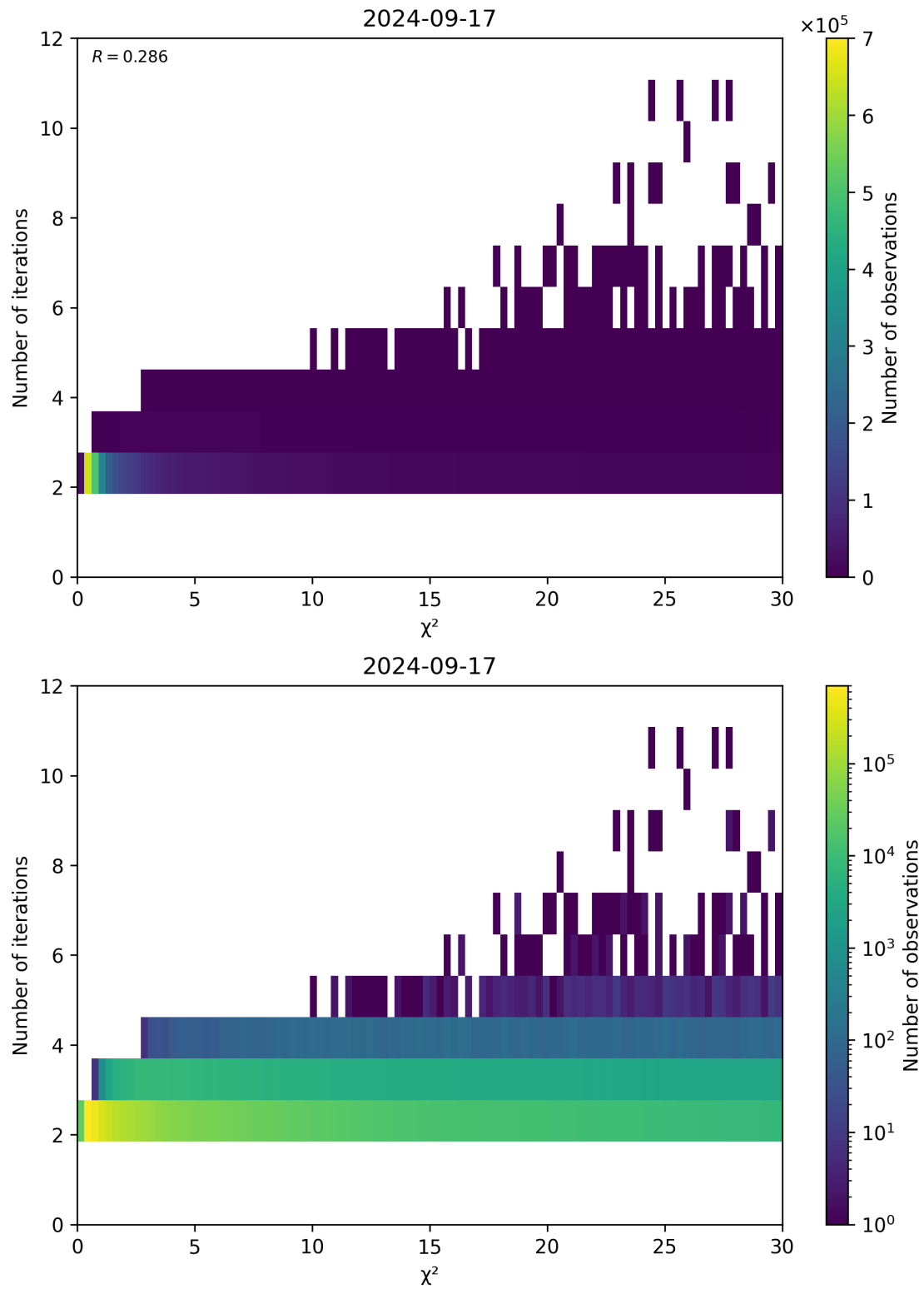
Figure 73: Scatter density plot of “ \chi^2 ” against “Number of iterations” for 2024-09-17 to 2024-09-18.
