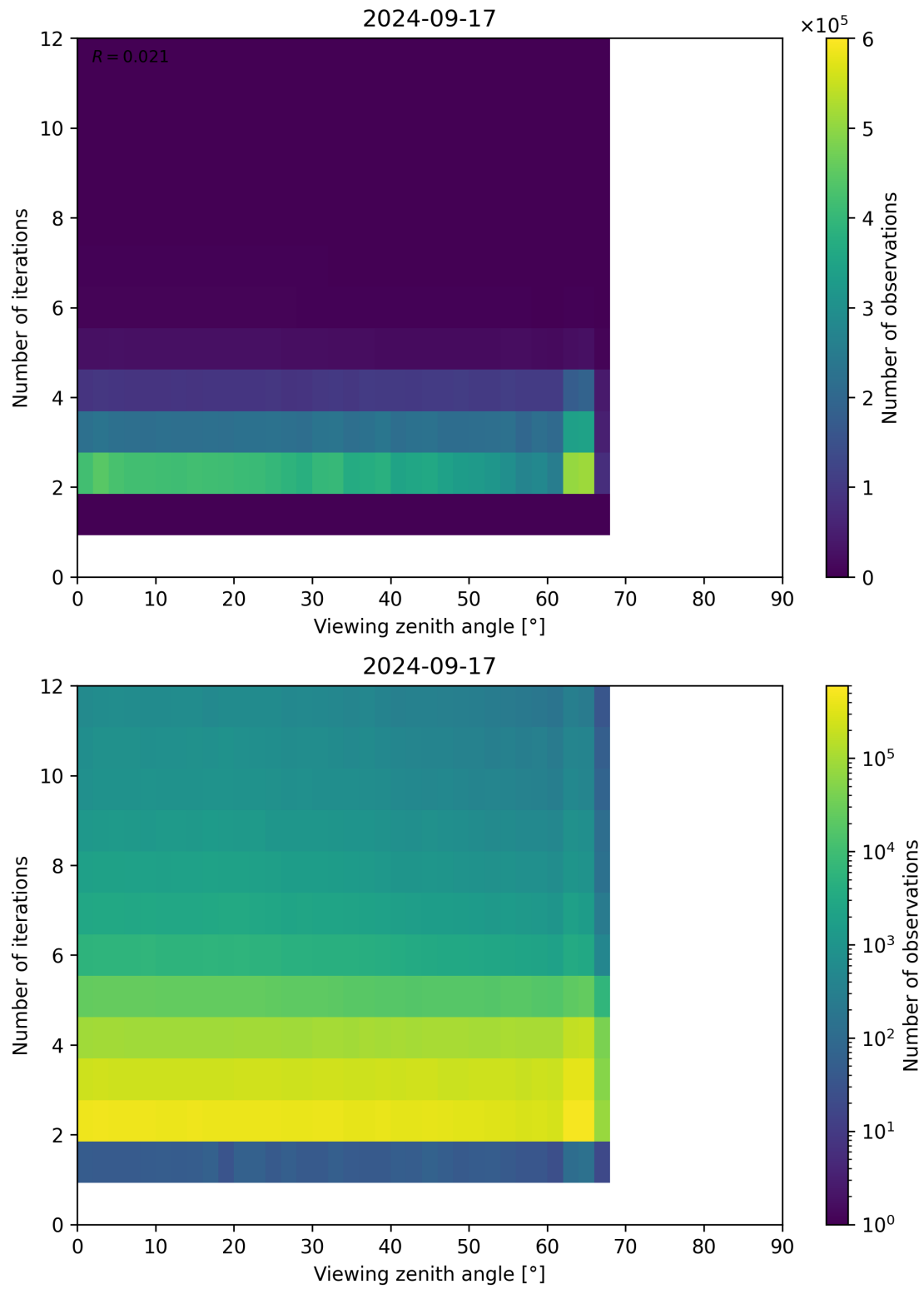
Figure 136: Scatter density plot of “Viewing zenith angle” against “Number of iterations” for 2024-09-17 to 2024-09-18.
