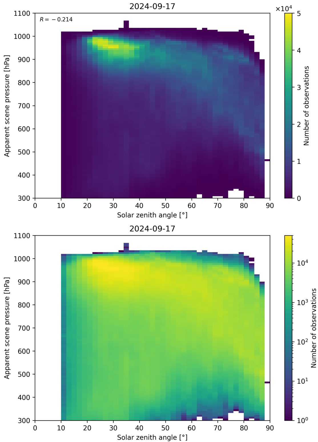
Figure 118: Scatter density plot of “Solar zenith angle” against “Apparent scene pressure” for 2024-09-17 to 2024-09-18.
