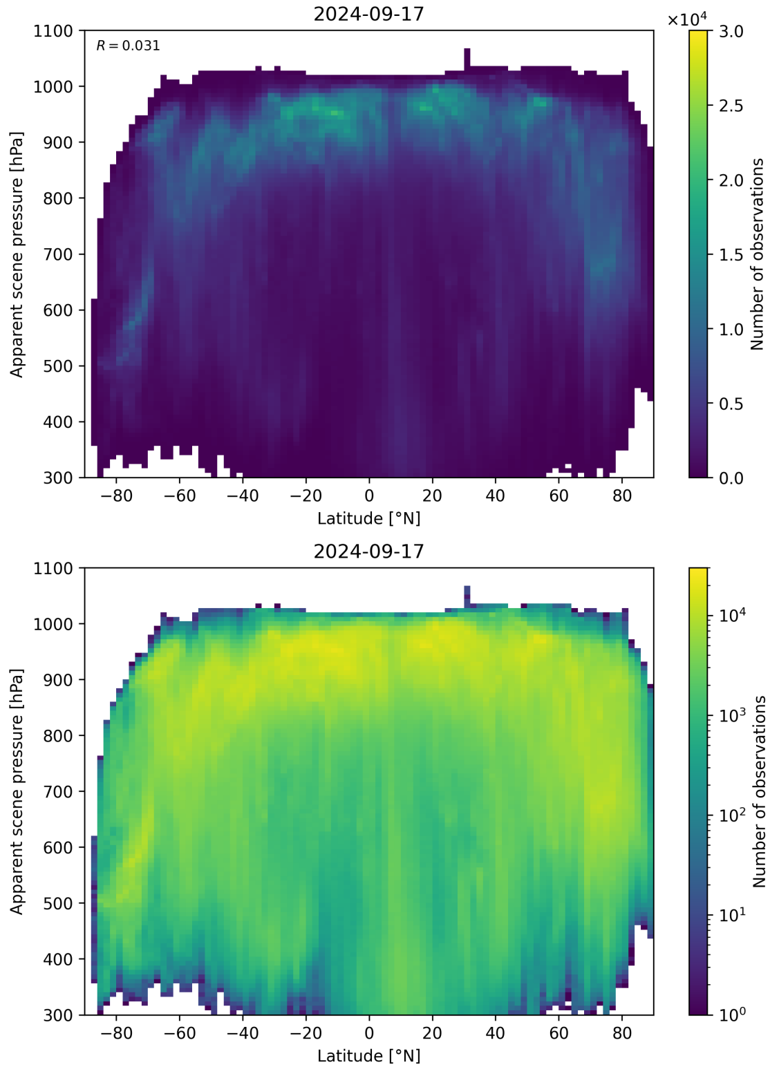
Figure 96: Scatter density plot of “Latitude” against “Apparent scene pressure” for 2024-09-17 to 2024-09-18.
