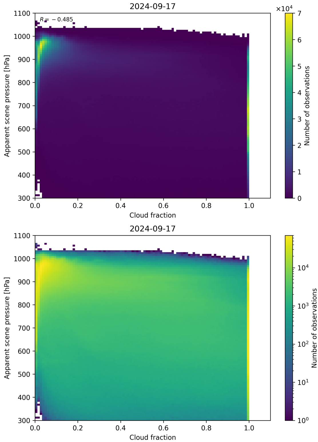
Figure 76: Scatter density plot of “Cloud fraction” against “Apparent scene pressure” for 2024-09-17 to 2024-09-18.
