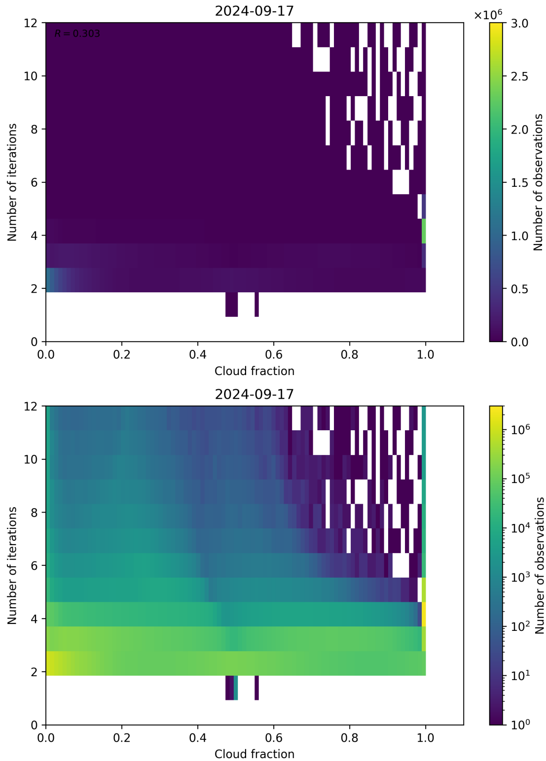
Figure 80: Scatter density plot of “Cloud fraction” against “Number of iterations” for 2024-09-17 to 2024-09-18.
