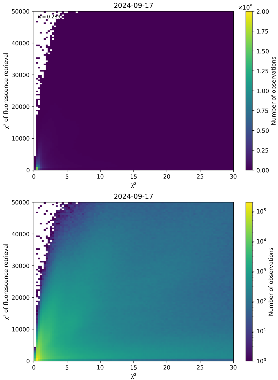
Figure 69: Scatter density plot of “ \chi^2 ” against “ \chi^2 of fluorescence retrieval” for 2024-09-17 to 2024-09-18.
