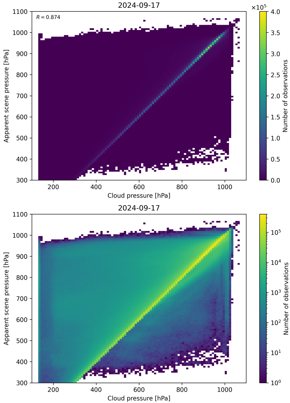
Figure 84: Scatter density plot of “Cloud pressure” against “Apparent scene pressure” for 2024-09-17 to 2024-09-18.
