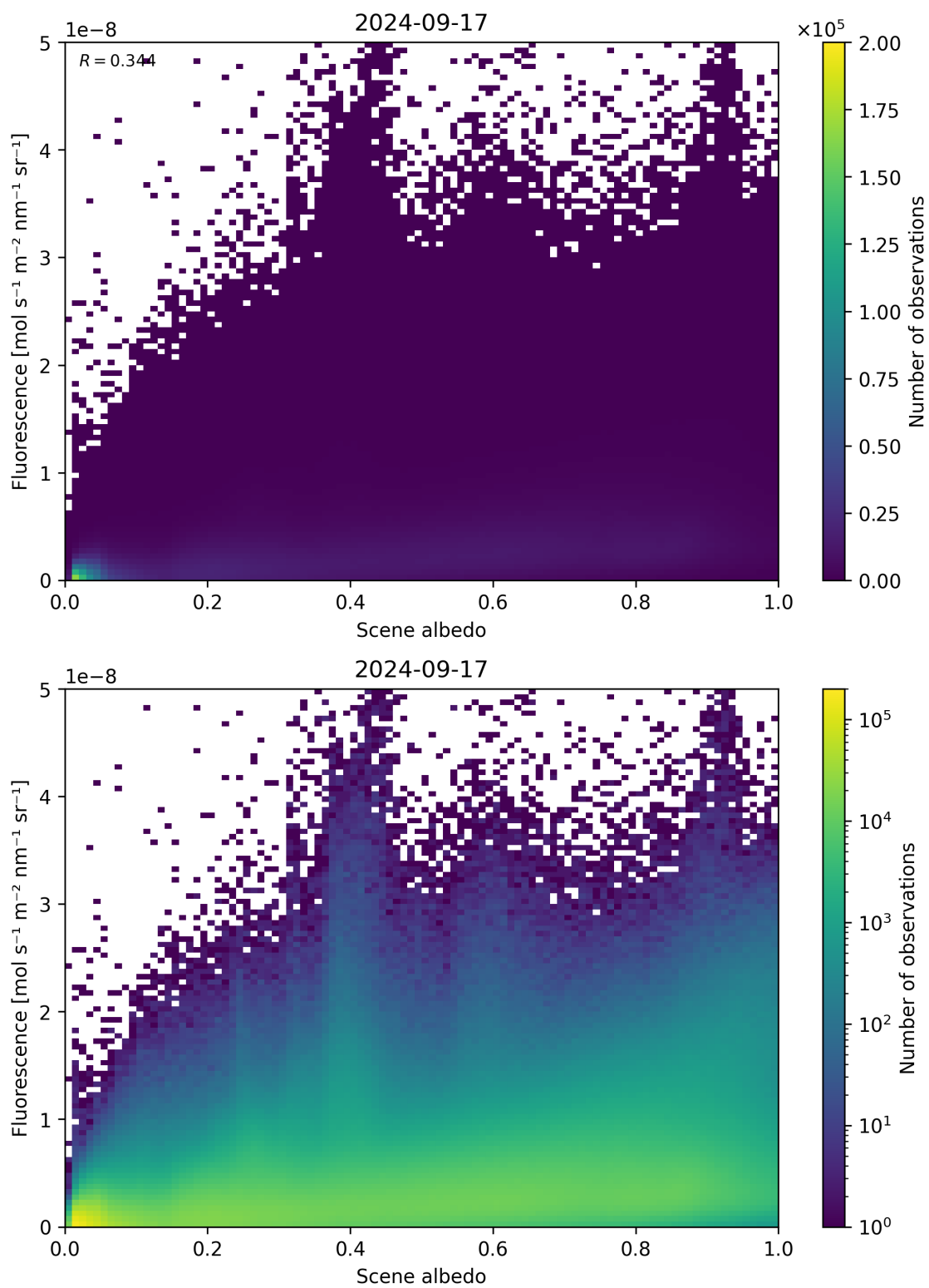
Figure 114: Scatter density plot of “Scene albedo” against “Fluorescence” for 2024-09-17 to 2024-09-18.
