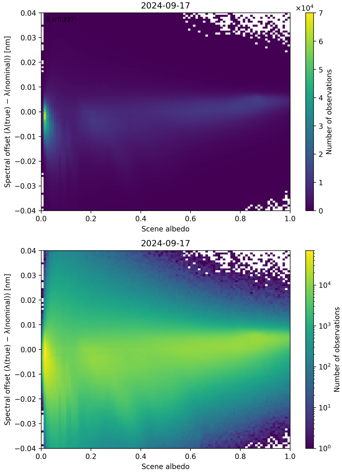
Figure 117: Scatter density plot of “Scene albedo” against “Spectral offset ( \lambda_{\text{true}} - \lambda_{\text{nominal}} )” for 2024-09-17 to 2024-09-18.
