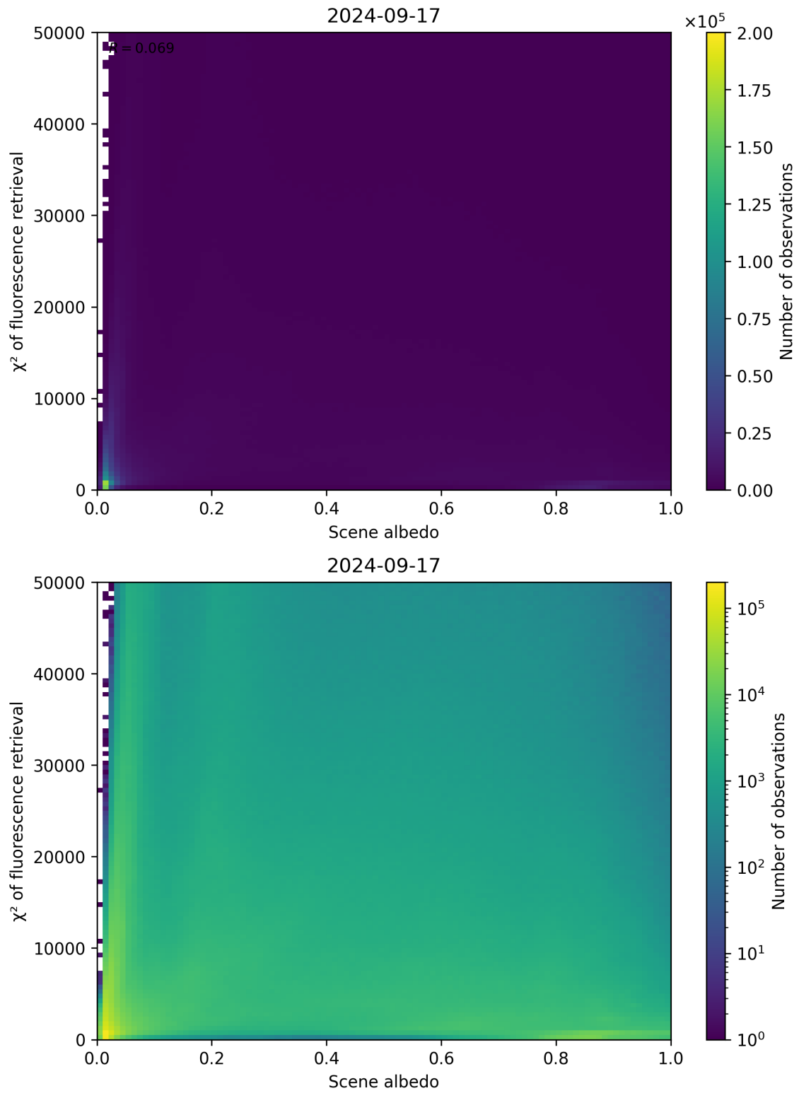
Figure 113: Scatter density plot of “Scene albedo” against “ \chi^2 of fluorescence retrieval” for 2024-09-17 to 2024-09-18.
