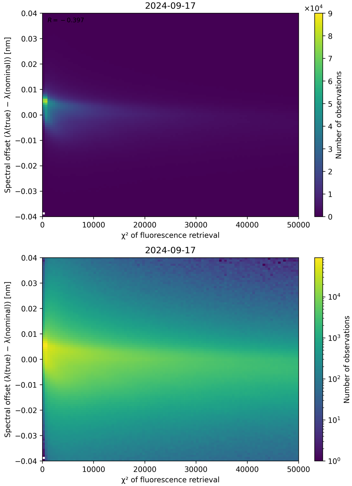
Figure 72: Scatter density plot of “ \chi^2 of fluorescence retrieval” against “Spectral offset ( \lambda_{\text{true}} - \lambda_{\text{nominal}} )” for 2024-09-17 to 2024-09-18.
