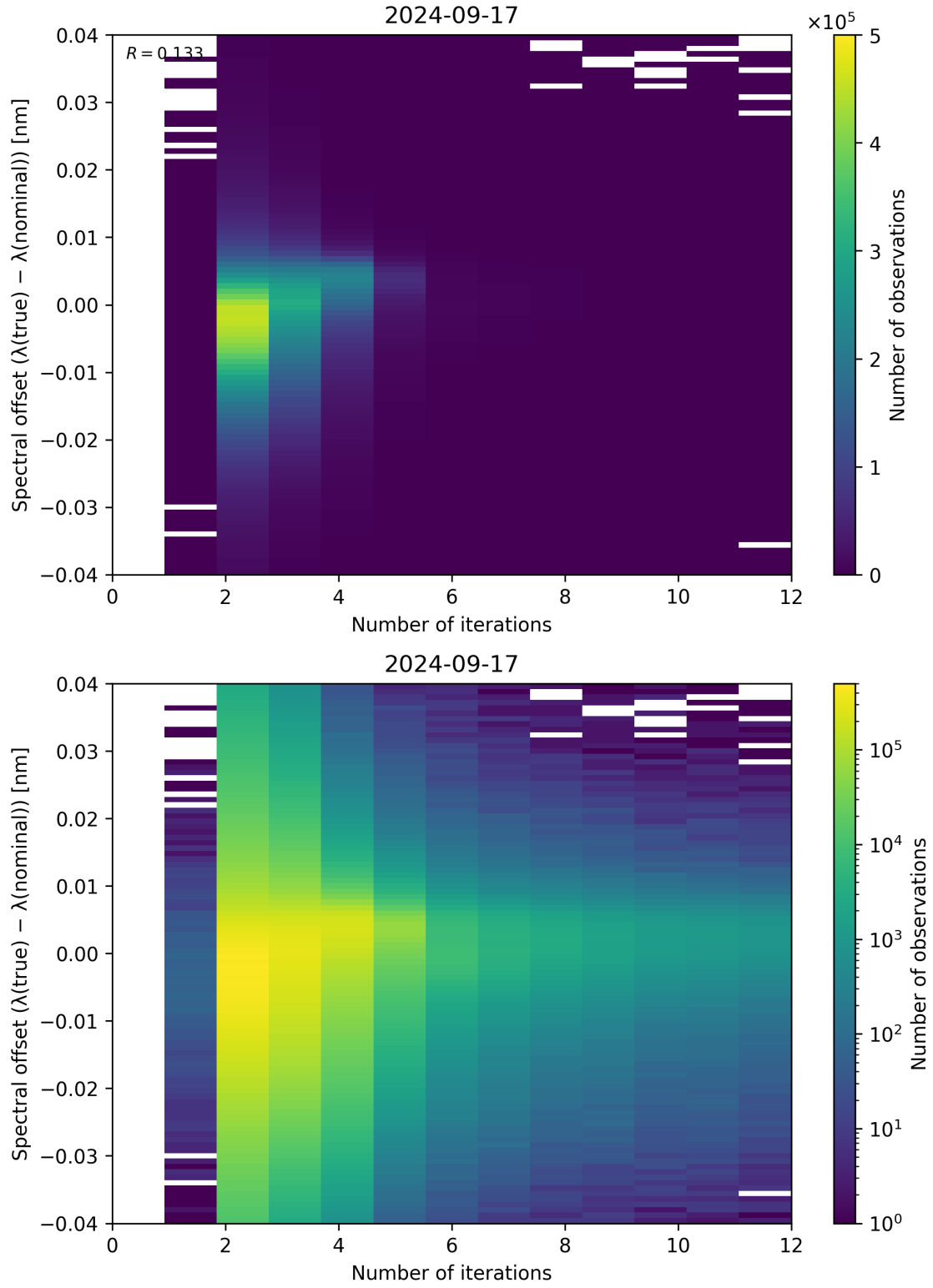
Figure 109: Scatter density plot of “Number of iterations” against “Spectral offset ( \lambda_{\text{true}} - \lambda_{\text{nominal}} )” for 2024-09-17 to 2024-09-18.
