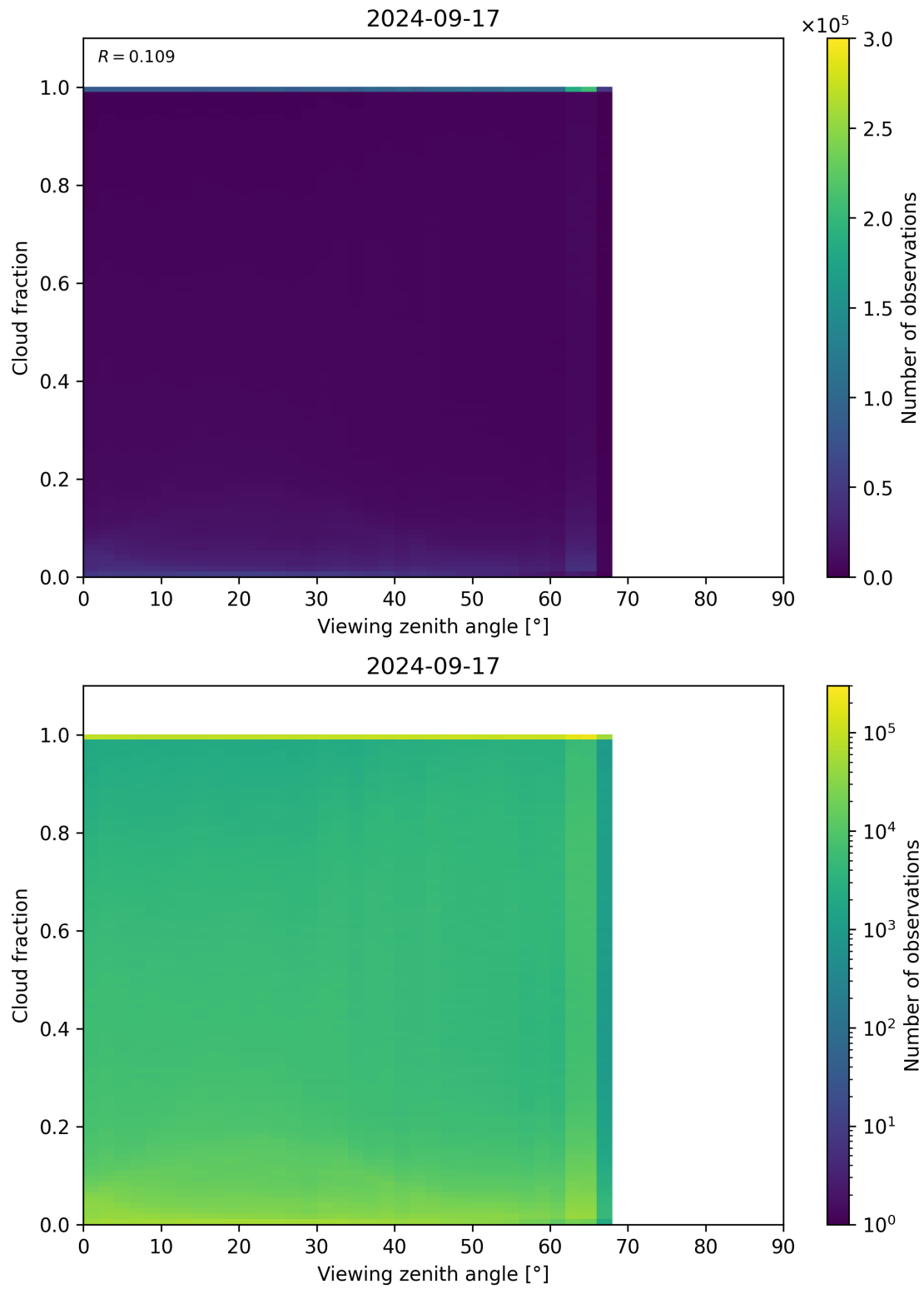
Figure 132: Scatter density plot of “Viewing zenith angle” against “Cloud fraction” for 2024-09-17 to 2024-09-18.
