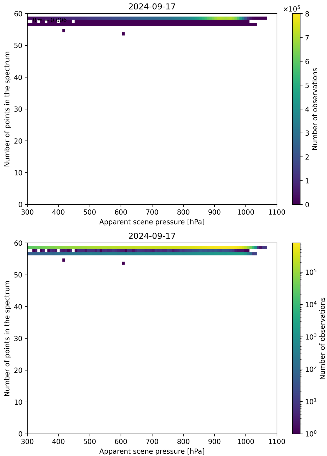
Figure 67: Scatter density plot of “Apparent scene pressure” against “Number of points in the spectrum” for 2024-09-17 to 2024-09-18.
