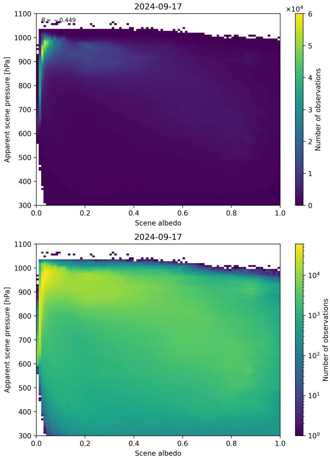
Figure 111: Scatter density plot of “Scene albedo” against “Apparent scene pressure” for 2024-09-17 to 2024-09-18.
