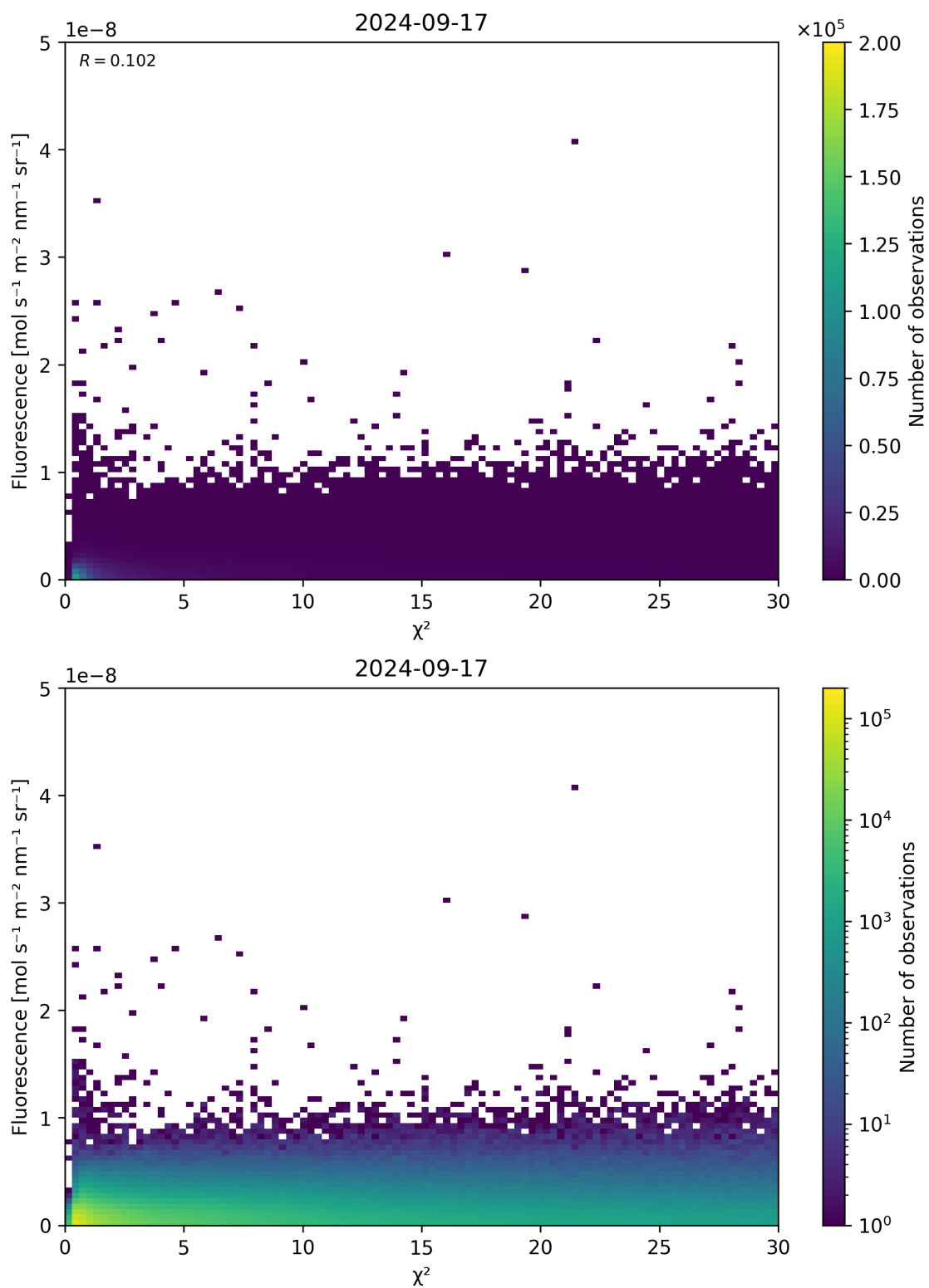
Figure 70: Scatter density plot of “ \chi^2 ” against “Fluorescence” for 2024-09-17 to 2024-09-18.
