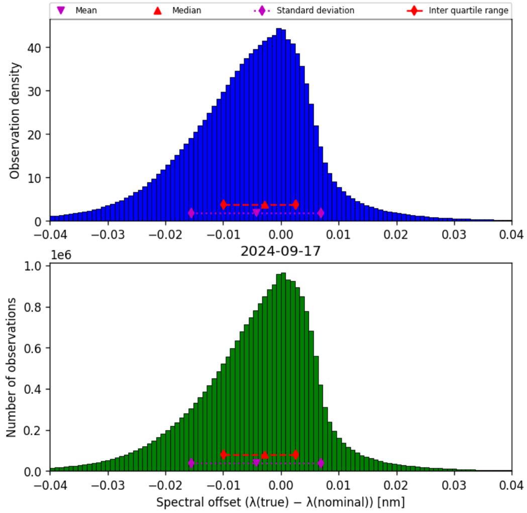
Figure 45: Histogram of “Spectral offset ( \lambda_{\text{true}} - \lambda_{\text{nominal}} )” for 2024-09-17 to 2024-09-18
