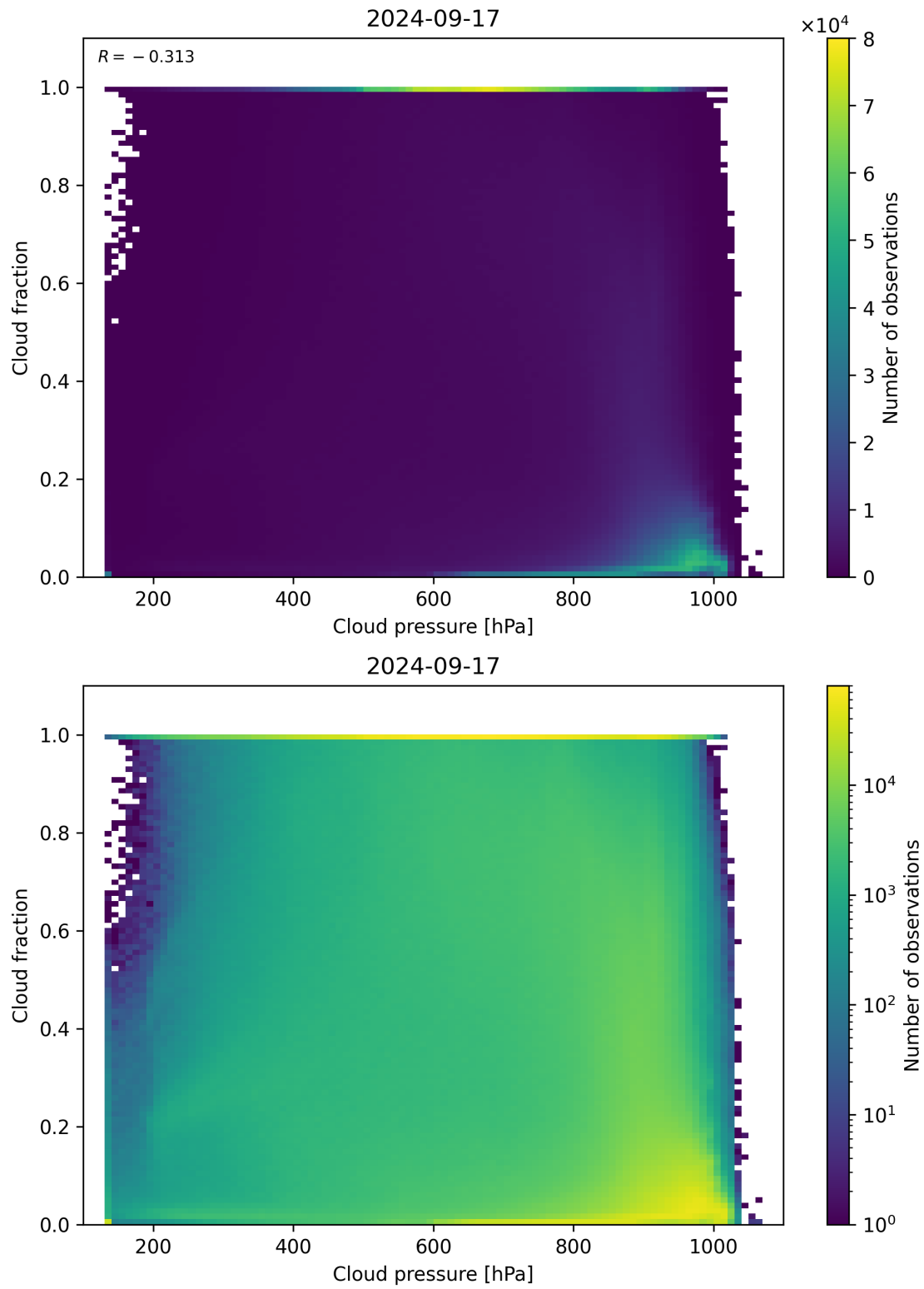
Figure 87: Scatter density plot of “Cloud pressure” against “Cloud fraction” for 2024-09-17 to 2024-09-18.
