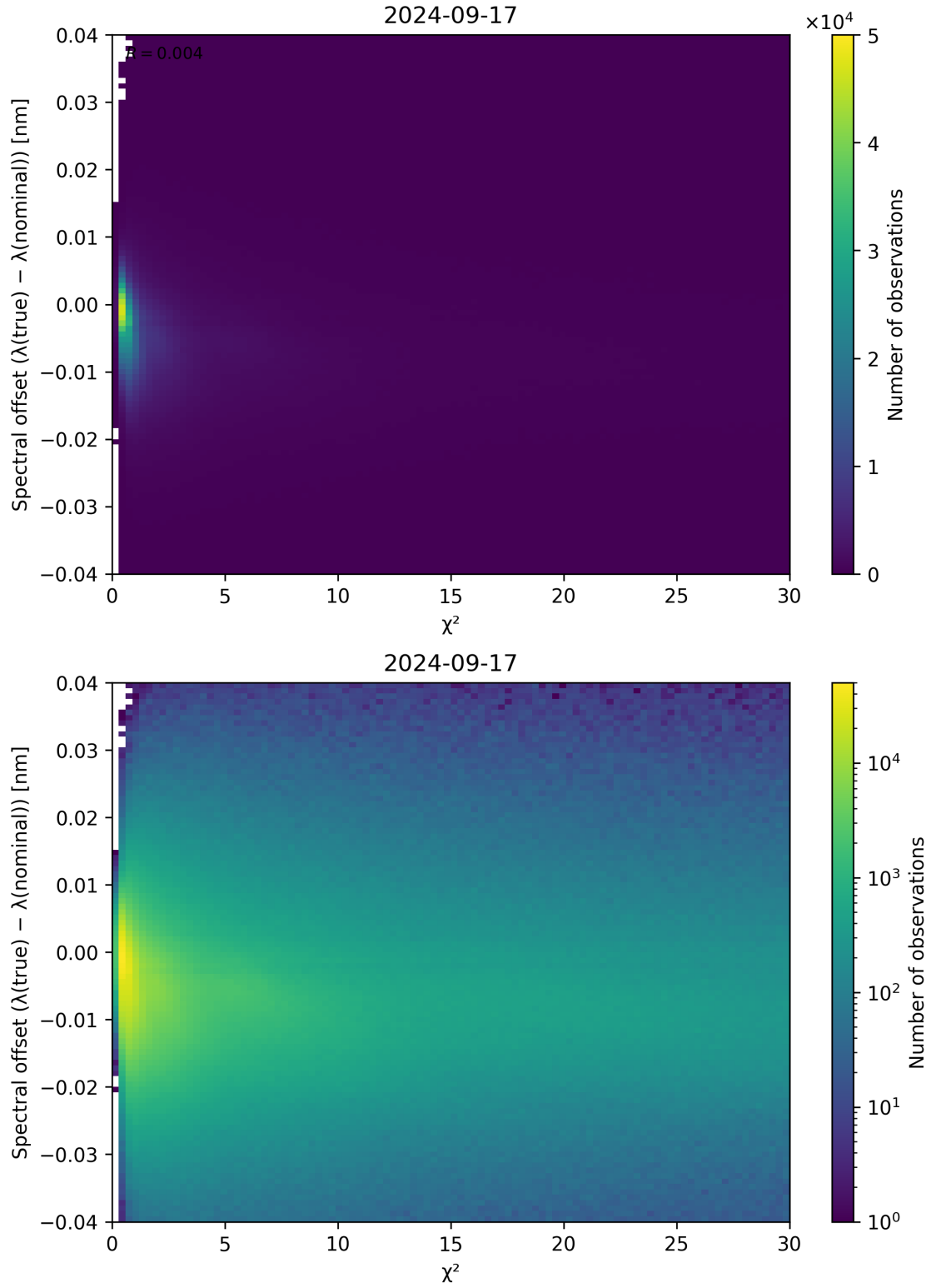
Figure 75: Scatter density plot of “ \chi^2 ” against “Spectral offset ( \lambda_{\text{true}} - \lambda_{\text{nominal}} )” for 2024-09-17 to 2024-09-18.
