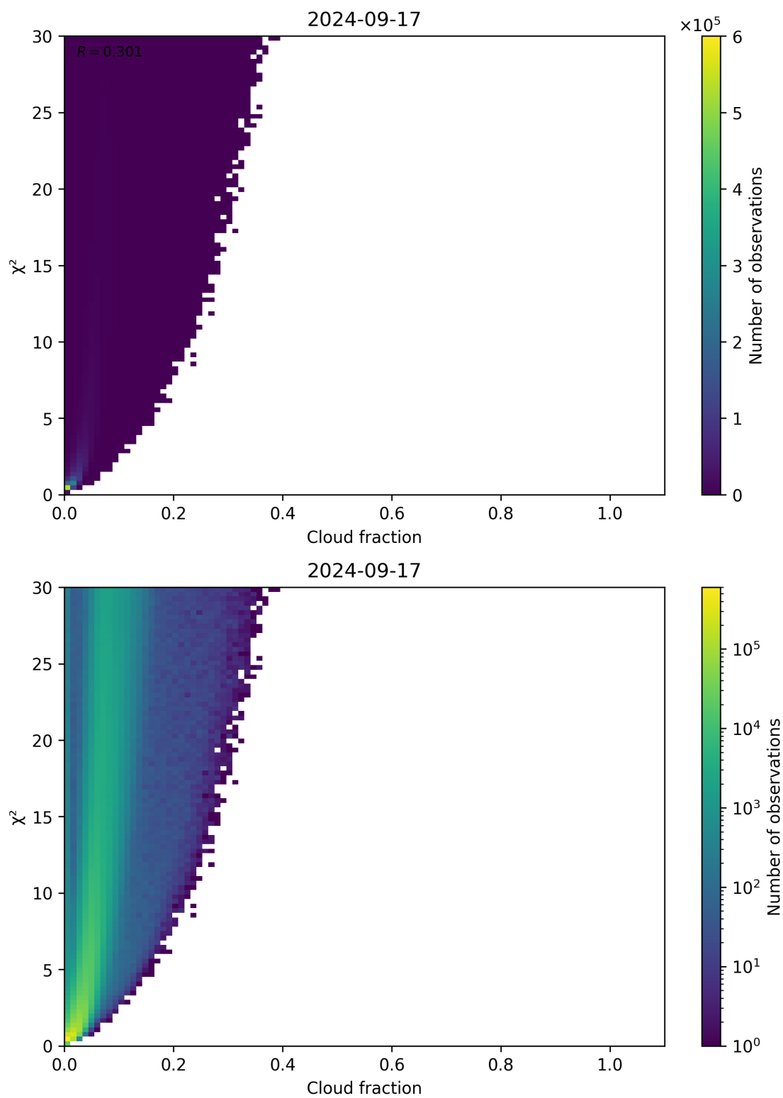
Figure 77: Scatter density plot of “Cloud fraction” against “ \chi^2 ” for 2024-09-17 to 2024-09-18.
