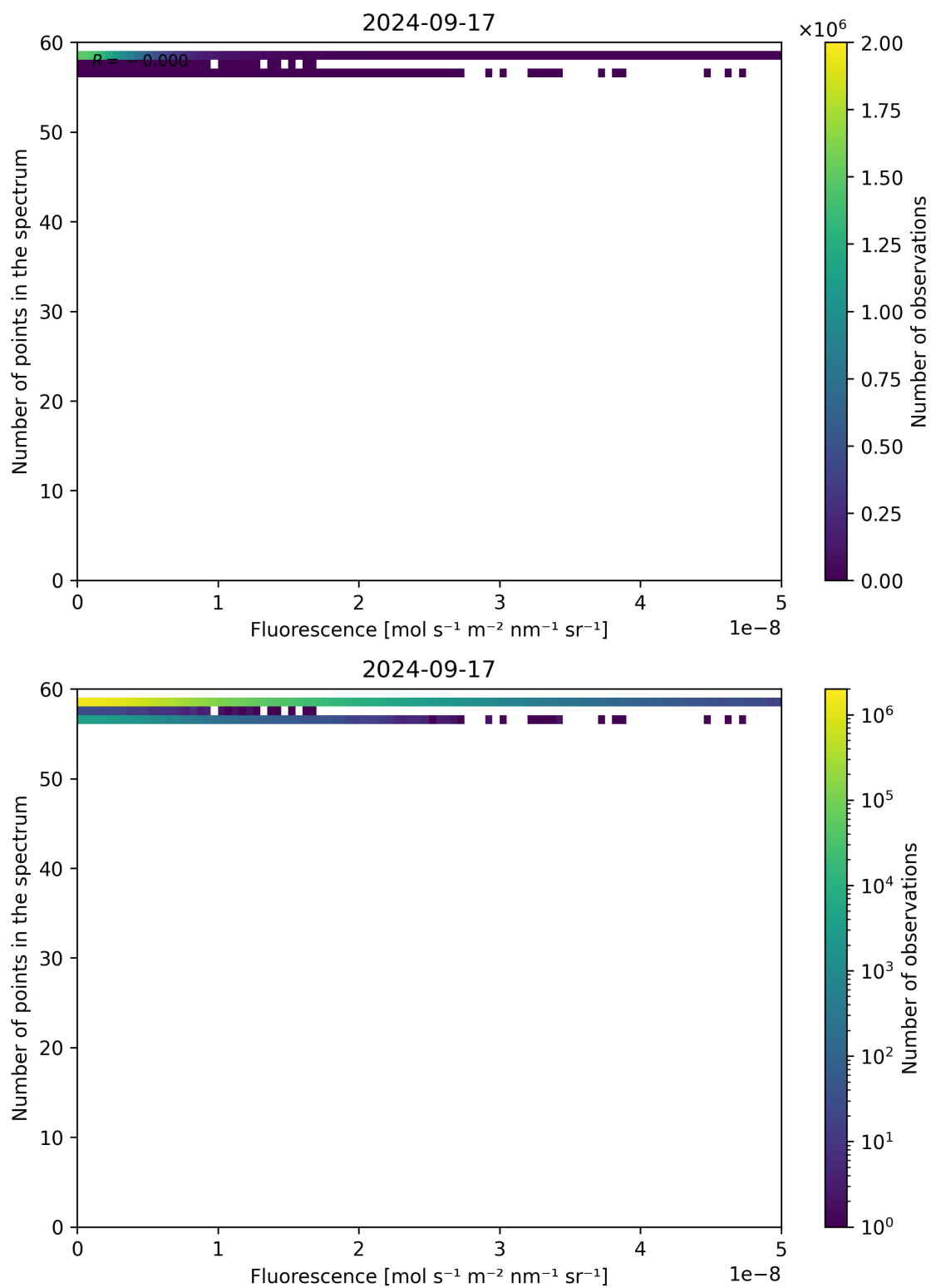
Figure 94: Scatter density plot of “Fluorescence” against “Number of points in the spectrum” for 2024-09-17 to 2024-09-18.
