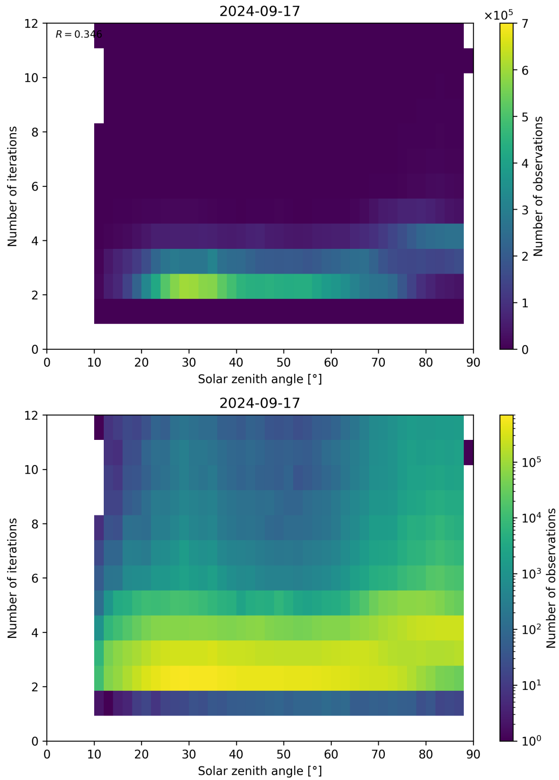
Figure 125: Scatter density plot of “Solar zenith angle” against “Number of iterations” for 2024-09-17 to 2024-09-18.
