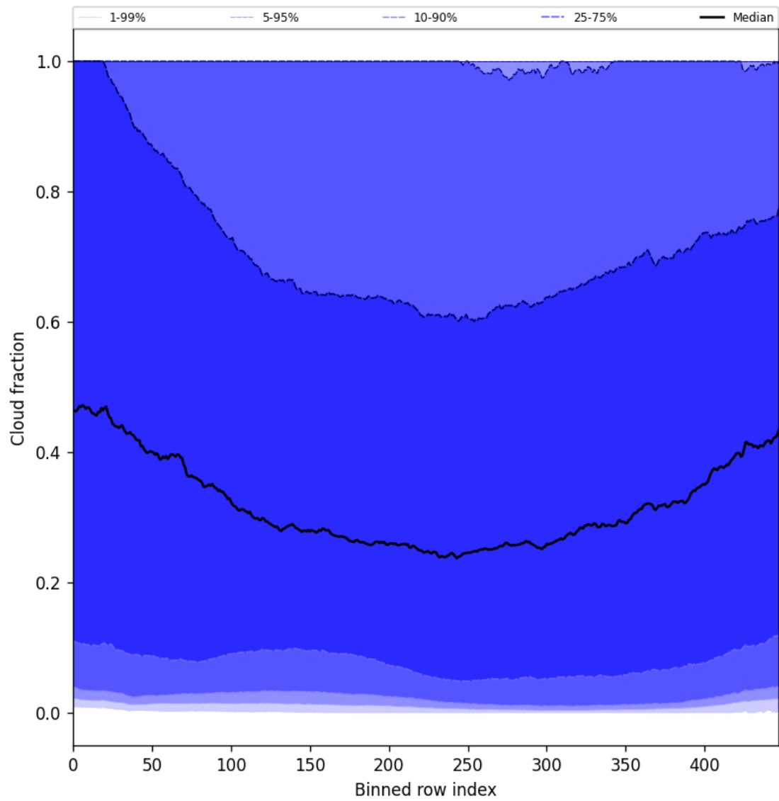
Figure 49: Along track statistics of “Cloud fraction” for 2024-09-17 to 2024-09-18
