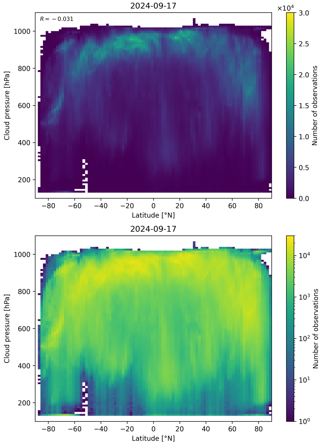
Figure 100: Scatter density plot of “Latitude” against “Cloud pressure” for 2024-09-17 to 2024-09-18.
