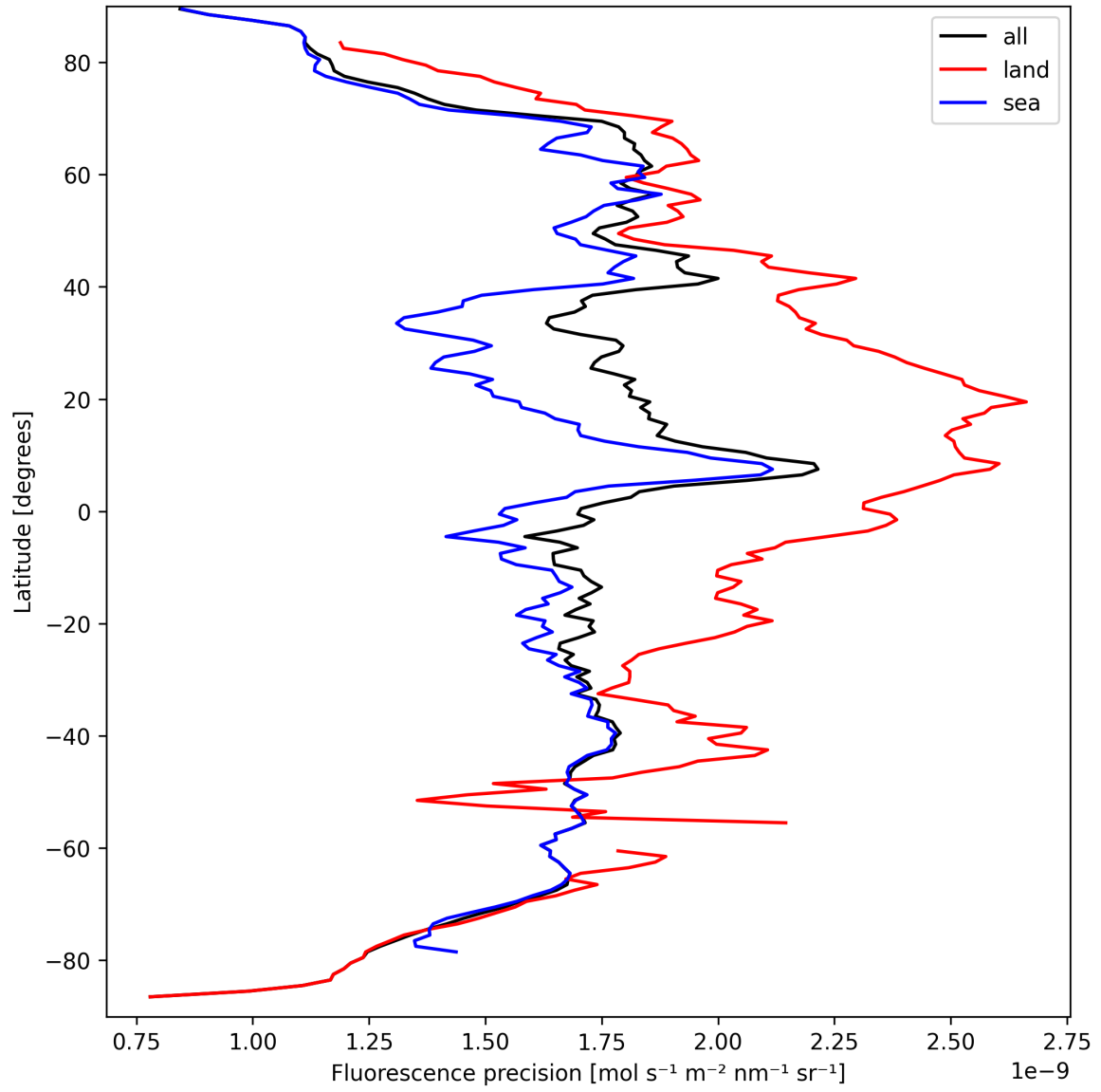
Figure 24: Zonal average of “Fluorescence precision” for 2024-09-17 to 2024-09-18.
