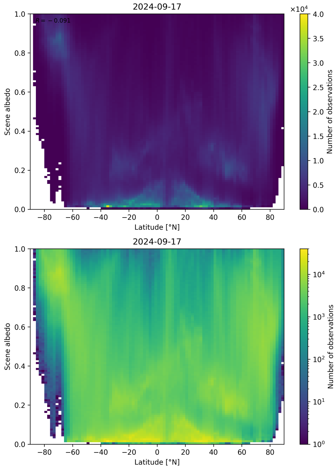
Figure 104: Scatter density plot of “Latitude” against “Scene albedo” for 2024-09-17 to 2024-09-18.
