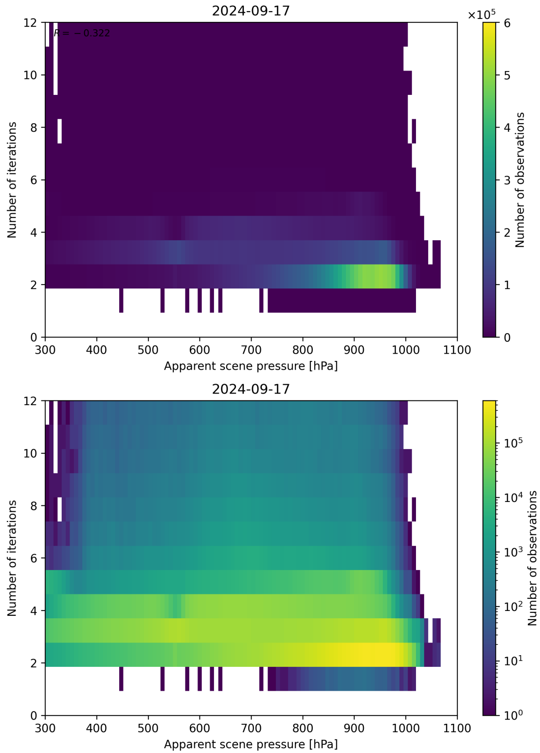
Figure 66: Scatter density plot of “Apparent scene pressure” against “Number of iterations” for 2024-09-17 to 2024-09-18.
