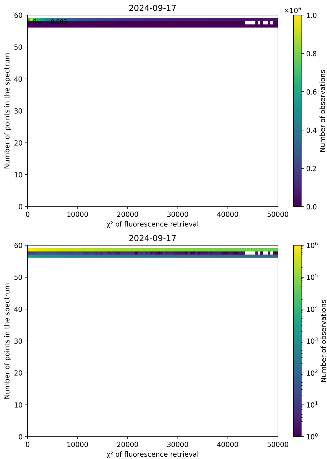
Figure 71: Scatter density plot of “ \chi^2 of fluorescence retrieval” against “Number of points in the spectrum” for 2024-09-17 to 2024-09-18.
