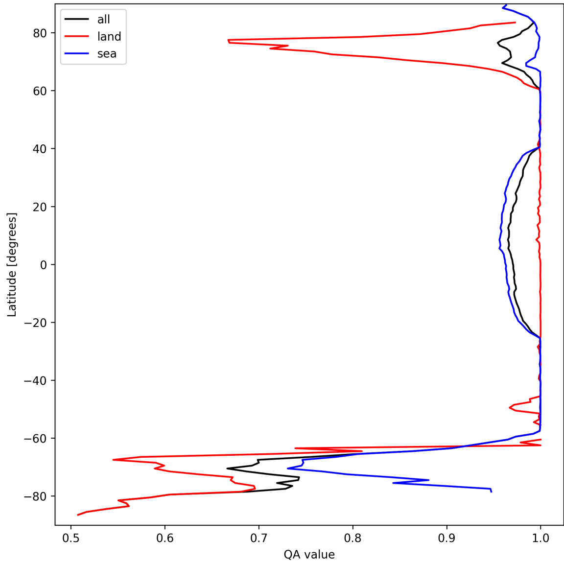
Figure 12: Zonal average of "QA value" for 2024-09-17 to 2024-09-18.
