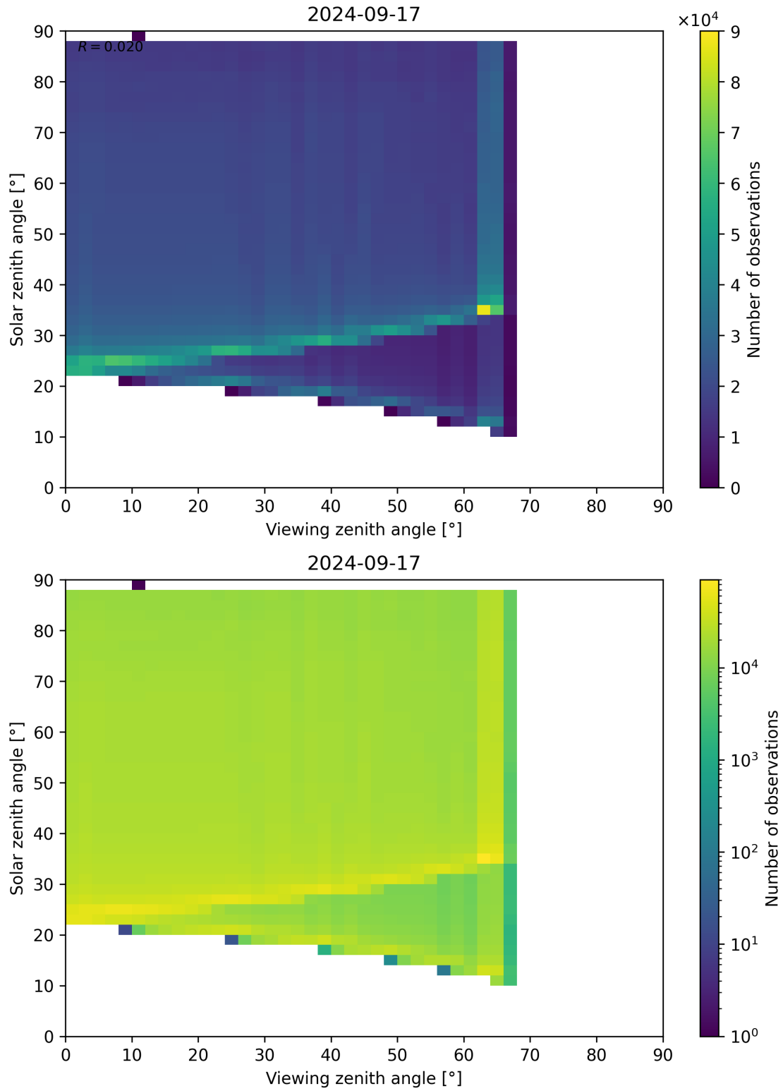
Figure 139: Scatter density plot of “Viewing zenith angle” against “Solar zenith angle” for 2024-09-17 to 2024-09-18.
