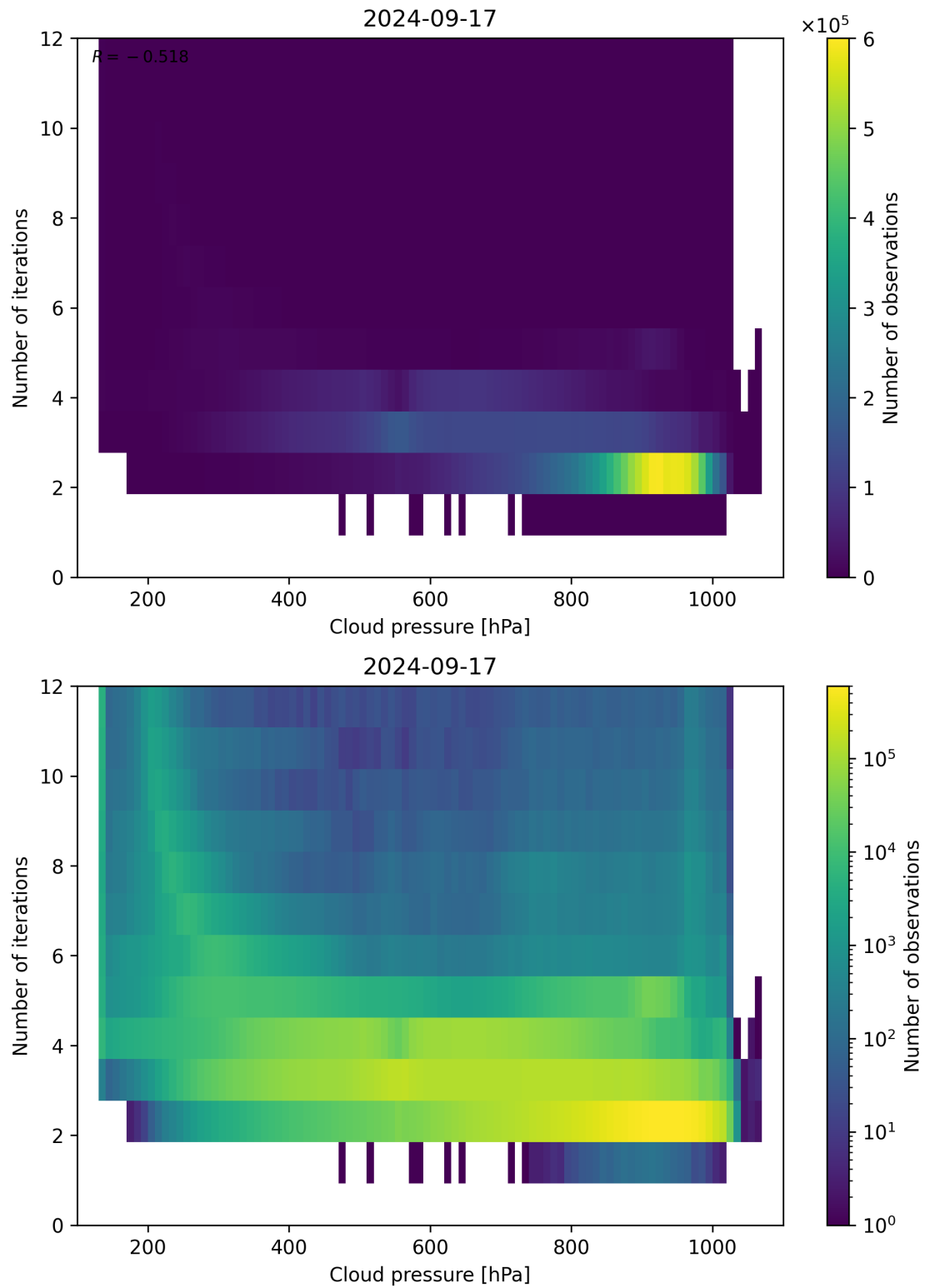
Figure 89: Scatter density plot of “Cloud pressure” against “Number of iterations” for 2024-09-17 to 2024-09-18.
