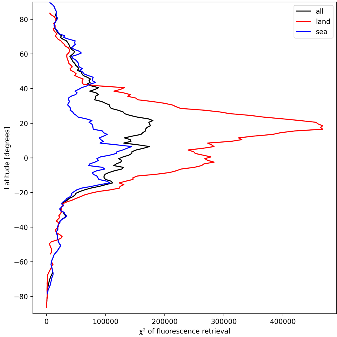
Figure 25: Zonal average of “ \chi^2 of fluorescence retrieval” for 2024-09-17 to 2024-09-18.
