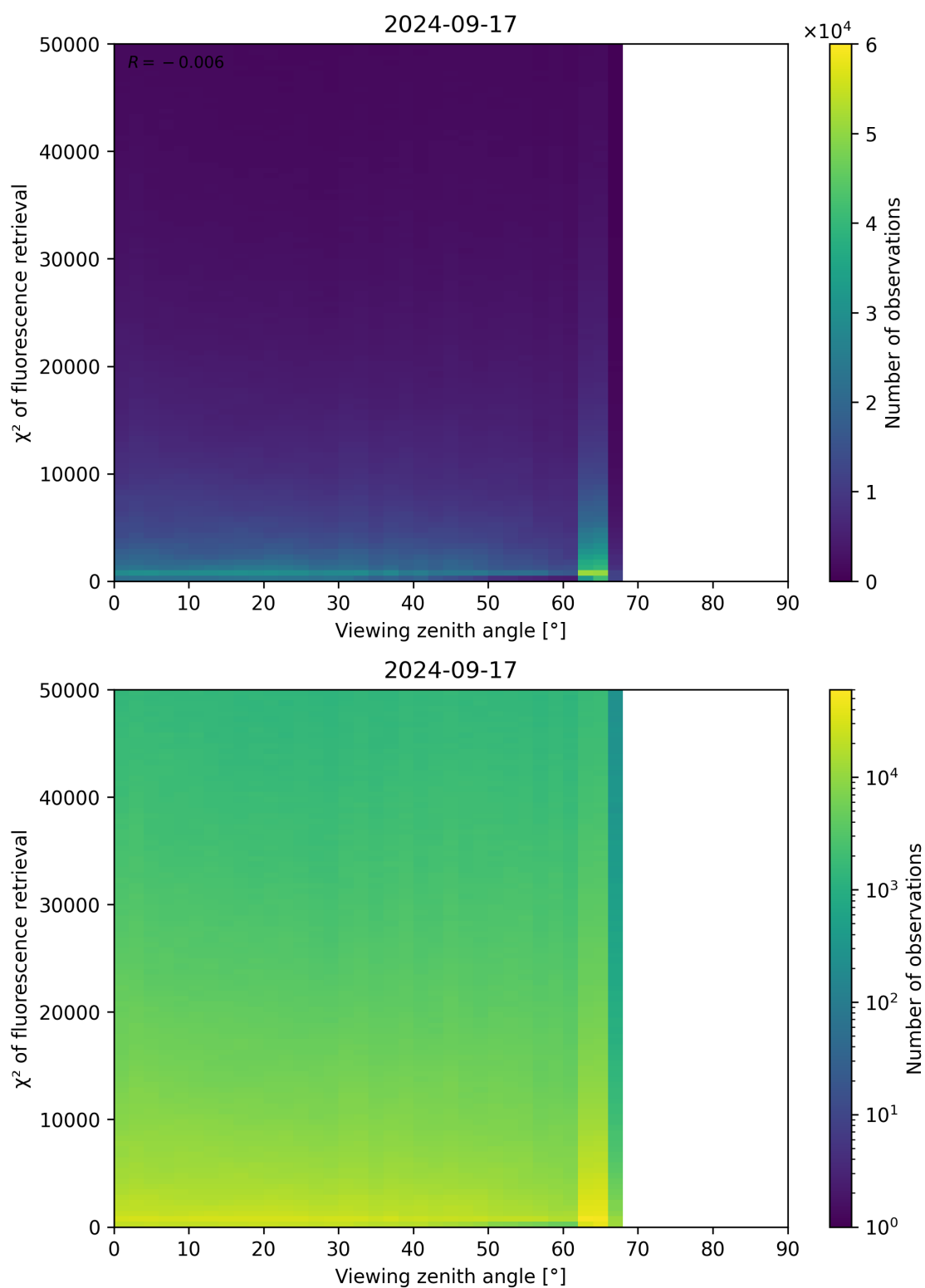
Figure 131: Scatter density plot of “Viewing zenith angle” against “ \chi^2 of fluorescence retrieval” for 2024-09-17 to 2024-09-18.
