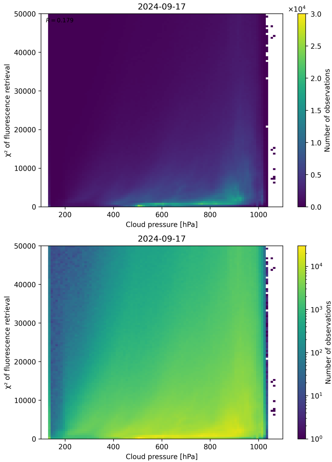
Figure 86: Scatter density plot of “Cloud pressure” against “ \chi^2 of fluorescence retrieval” for 2024-09-17 to 2024-09-18.
