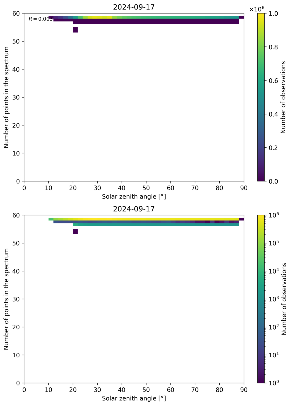
Figure 126: Scatter density plot of “Solar zenith angle” against “Number of points in the spectrum” for 2024-09-17 to 2024-09-18.
