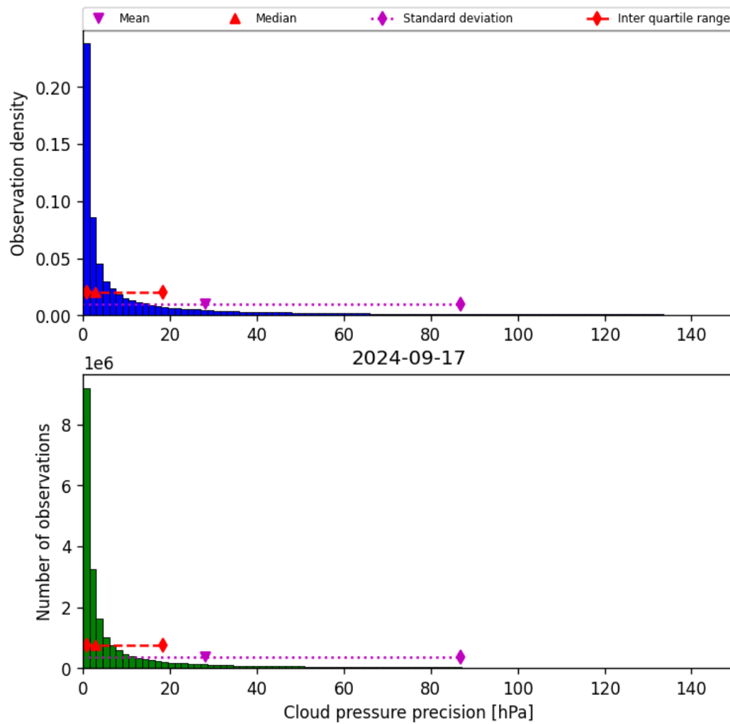
Figure 31: Histogram of “Cloud pressure precision” for 2024-09-17 to 2024-09-18
