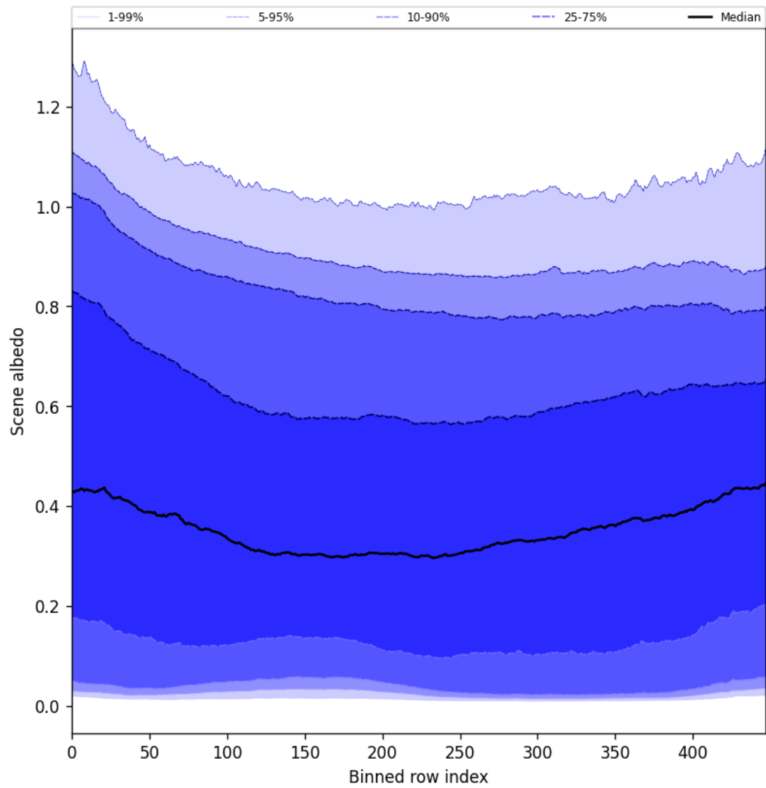
Figure 51: Along track statistics of “Scene albedo” for 2024-09-17 to 2024-09-18
