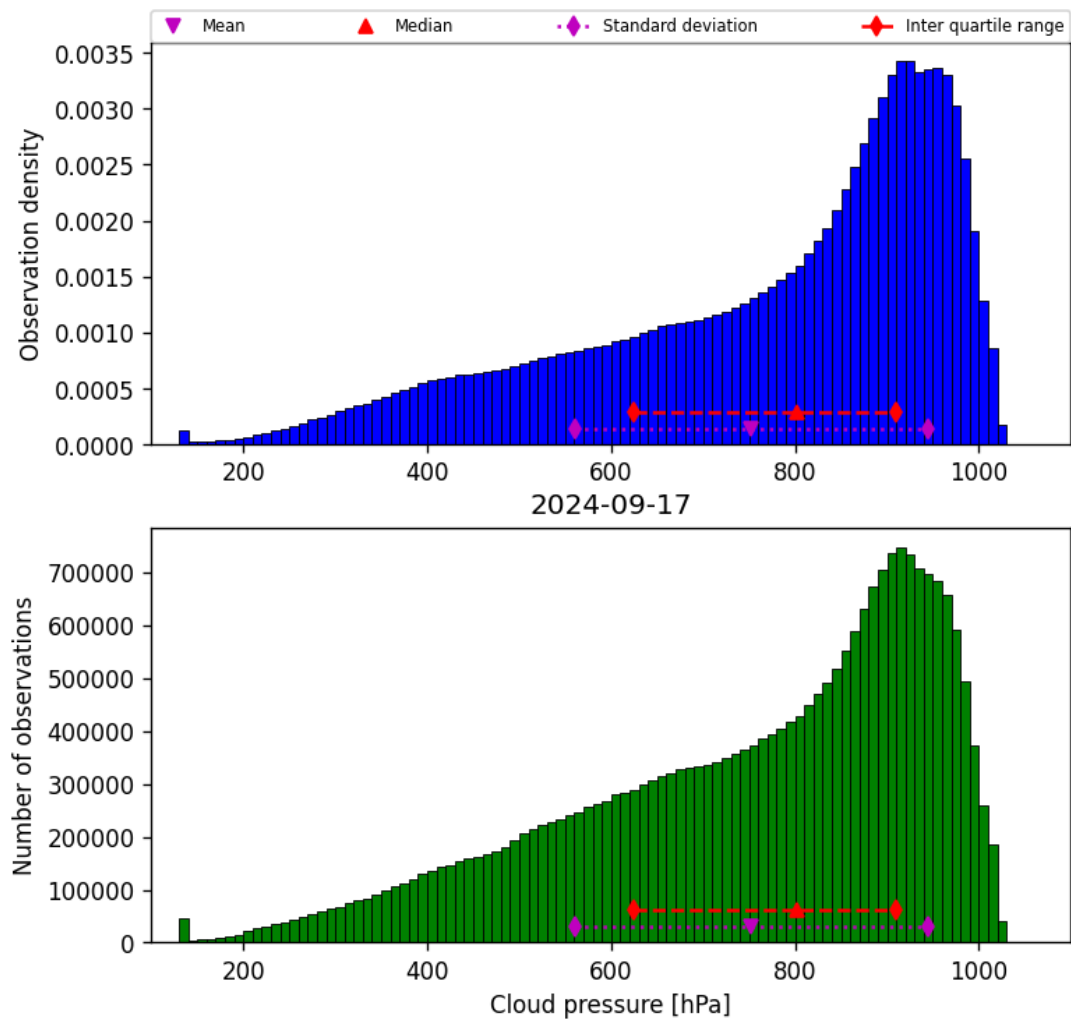
Figure 30: Histogram of “Cloud pressure” for 2024-09-17 to 2024-09-18
