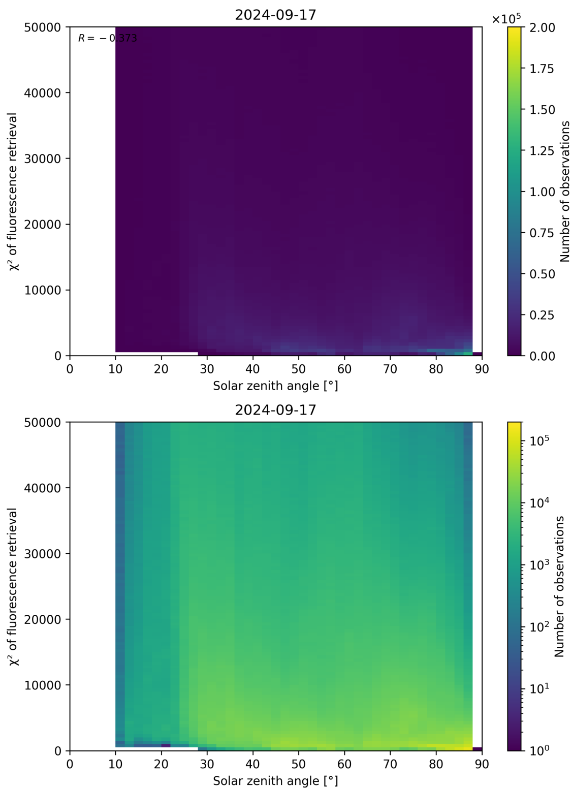
Figure 120: Scatter density plot of “Solar zenith angle” against “ \chi^2 of fluorescence retrieval” for 2024-09-17 to 2024-09-18.
