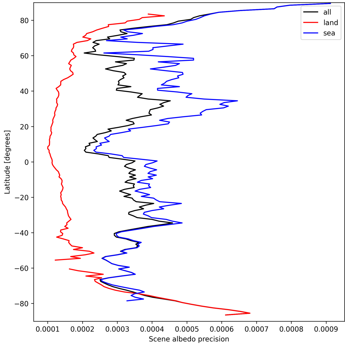
Figure 18: Zonal average of “Scene albedo precision” for 2024-09-17 to 2024-09-18.
