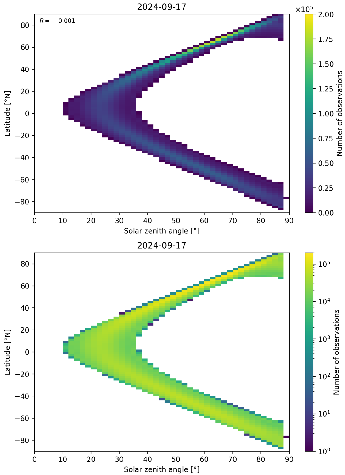
Figure 124: Scatter density plot of “Solar zenith angle” against “Latitude” for 2024-09-17 to 2024-09-18.
