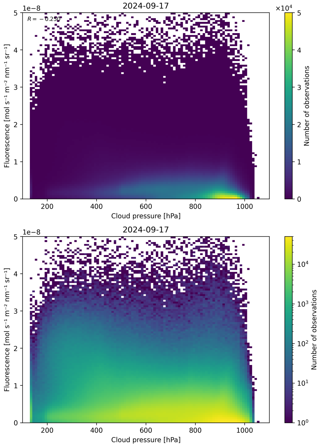
Figure 88: Scatter density plot of “Cloud pressure” against “Fluorescence” for 2024-09-17 to 2024-09-18.
