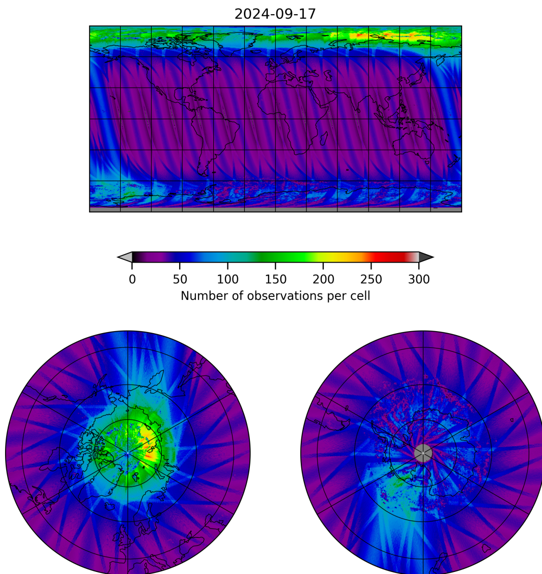
Figure 11: Map of the number of observations for 2024-09-17 to 2024-09-18
