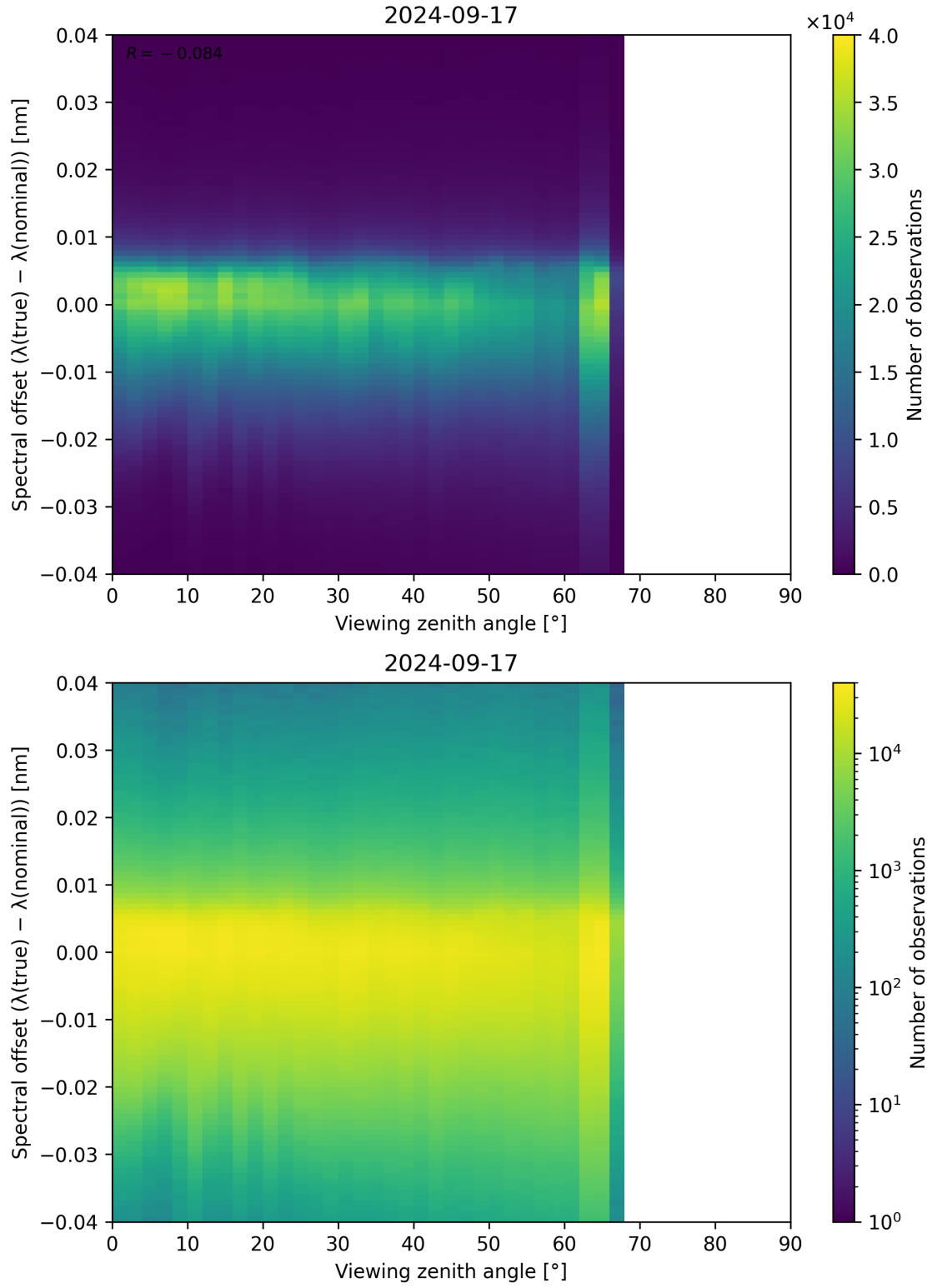
Figure 140: Scatter density plot of “Viewing zenith angle” against “Spectral offset ( \lambda_{\text{true}} - \lambda_{\text{nominal}} )” for 2024-09-17 to 2024-09-18.
