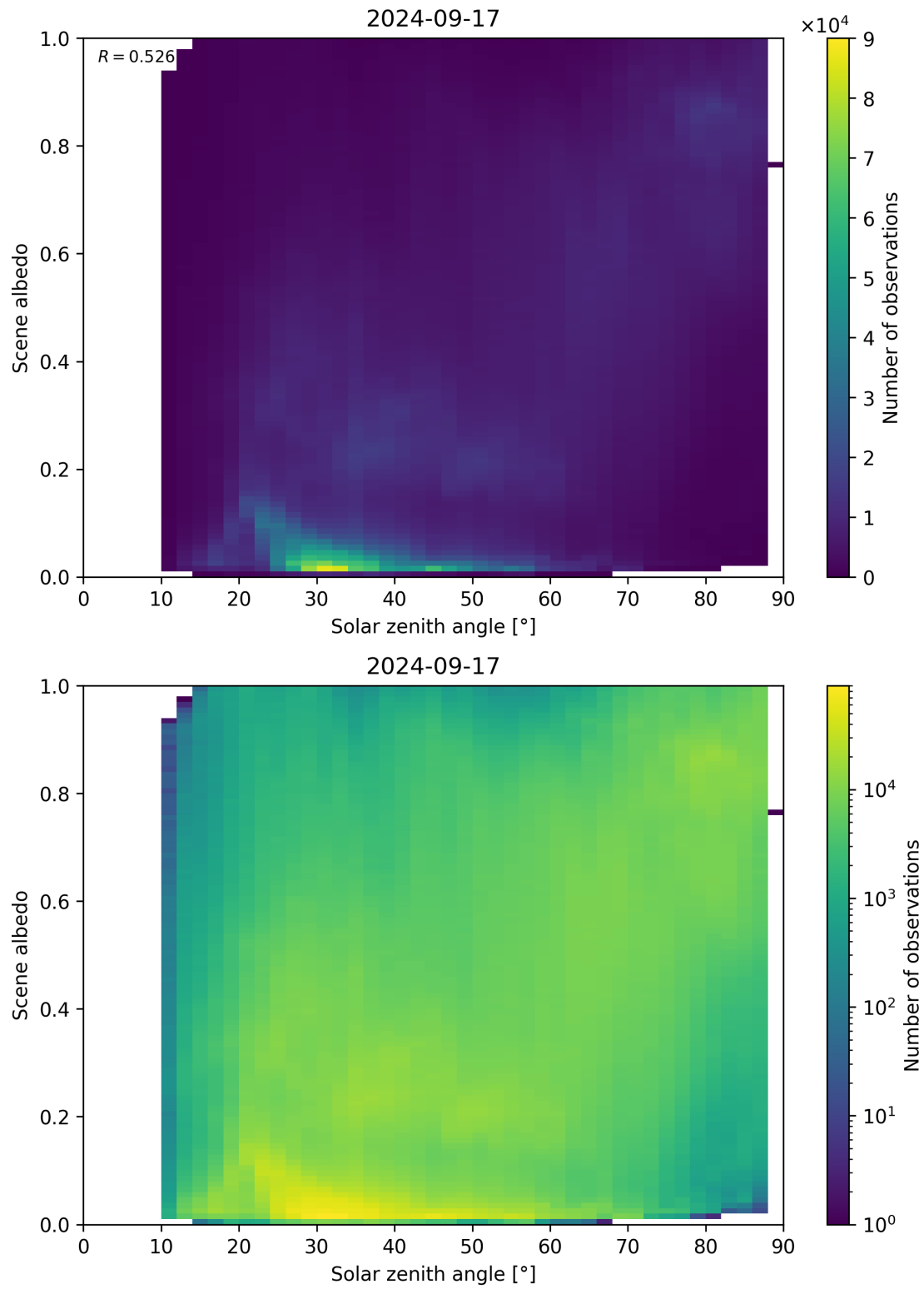
Figure 127: Scatter density plot of “Solar zenith angle” against “Scene albedo” for 2024-09-17 to 2024-09-18.
