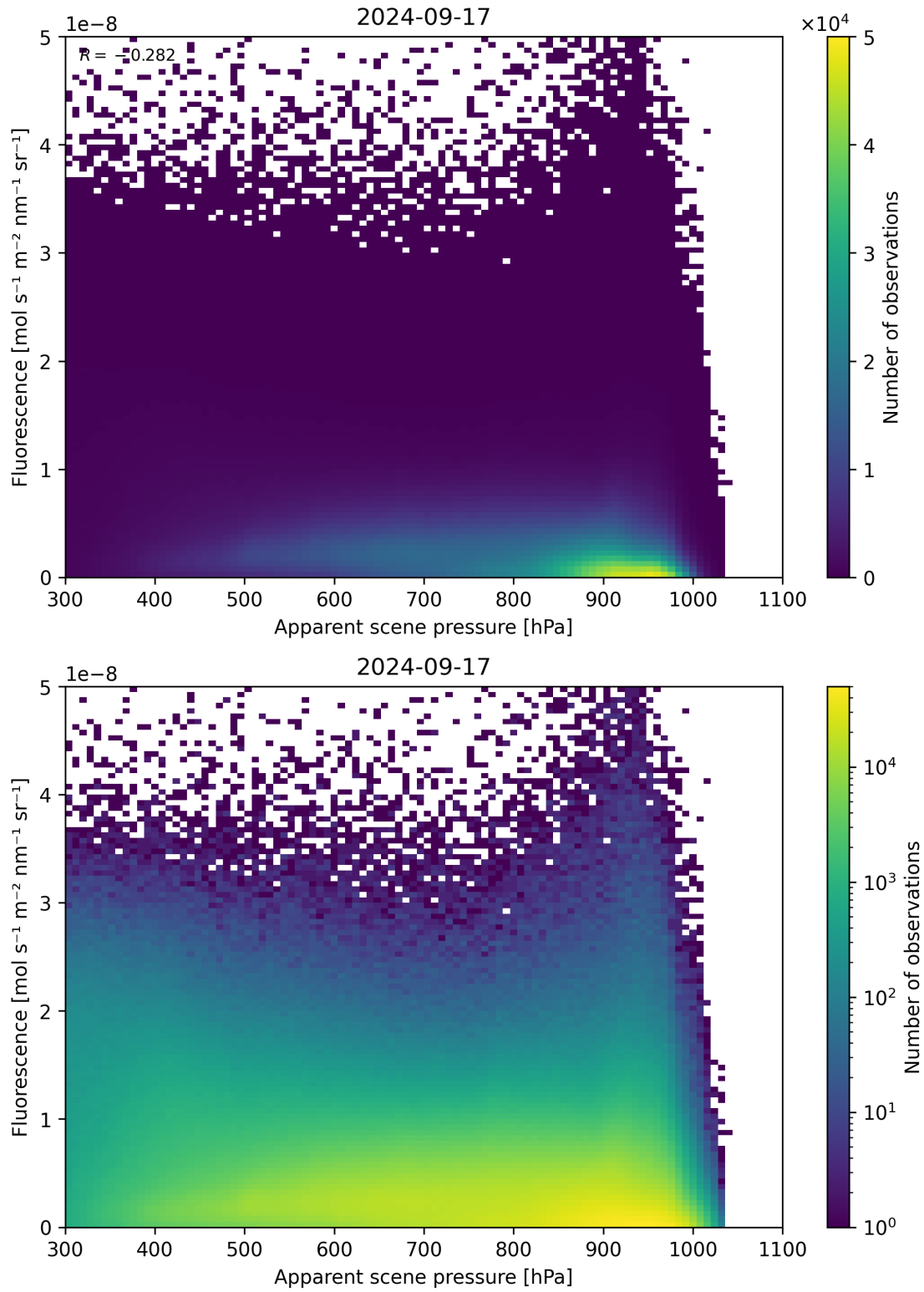
Figure 65: Scatter density plot of “Apparent scene pressure” against “Fluorescence” for 2024-09-17 to 2024-09-18.
