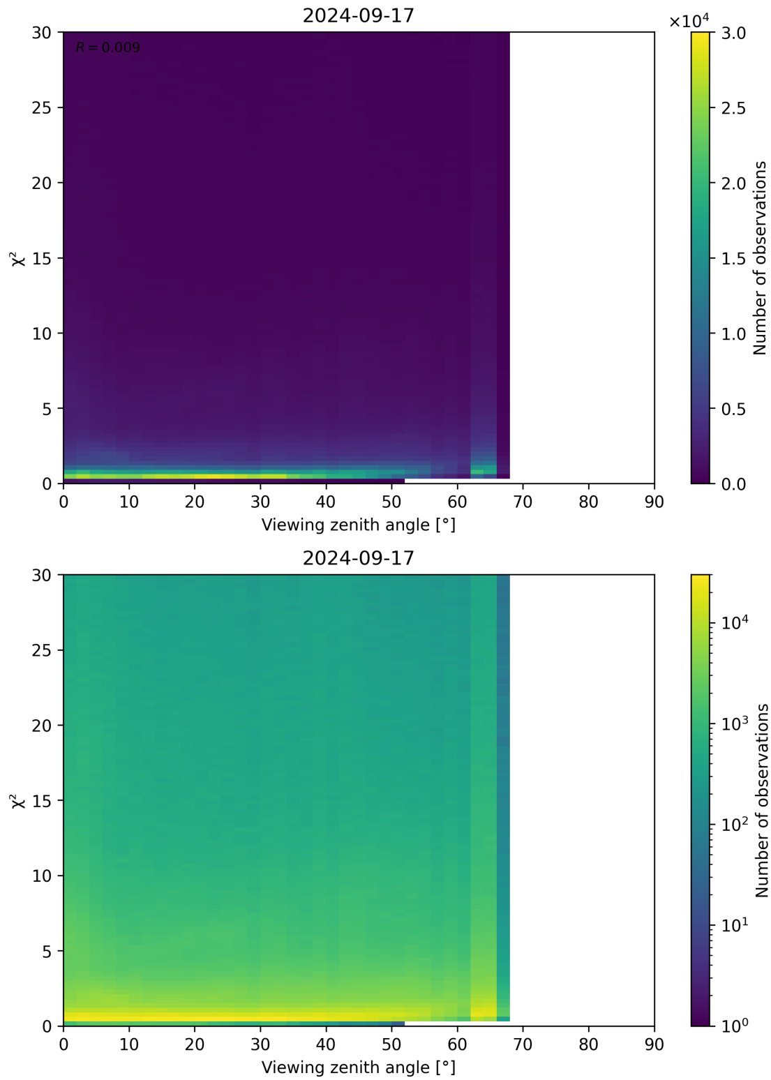
Figure 130: Scatter density plot of “Viewing zenith angle” against “ \chi^2 ” for 2024-09-17 to 2024-09-18.
