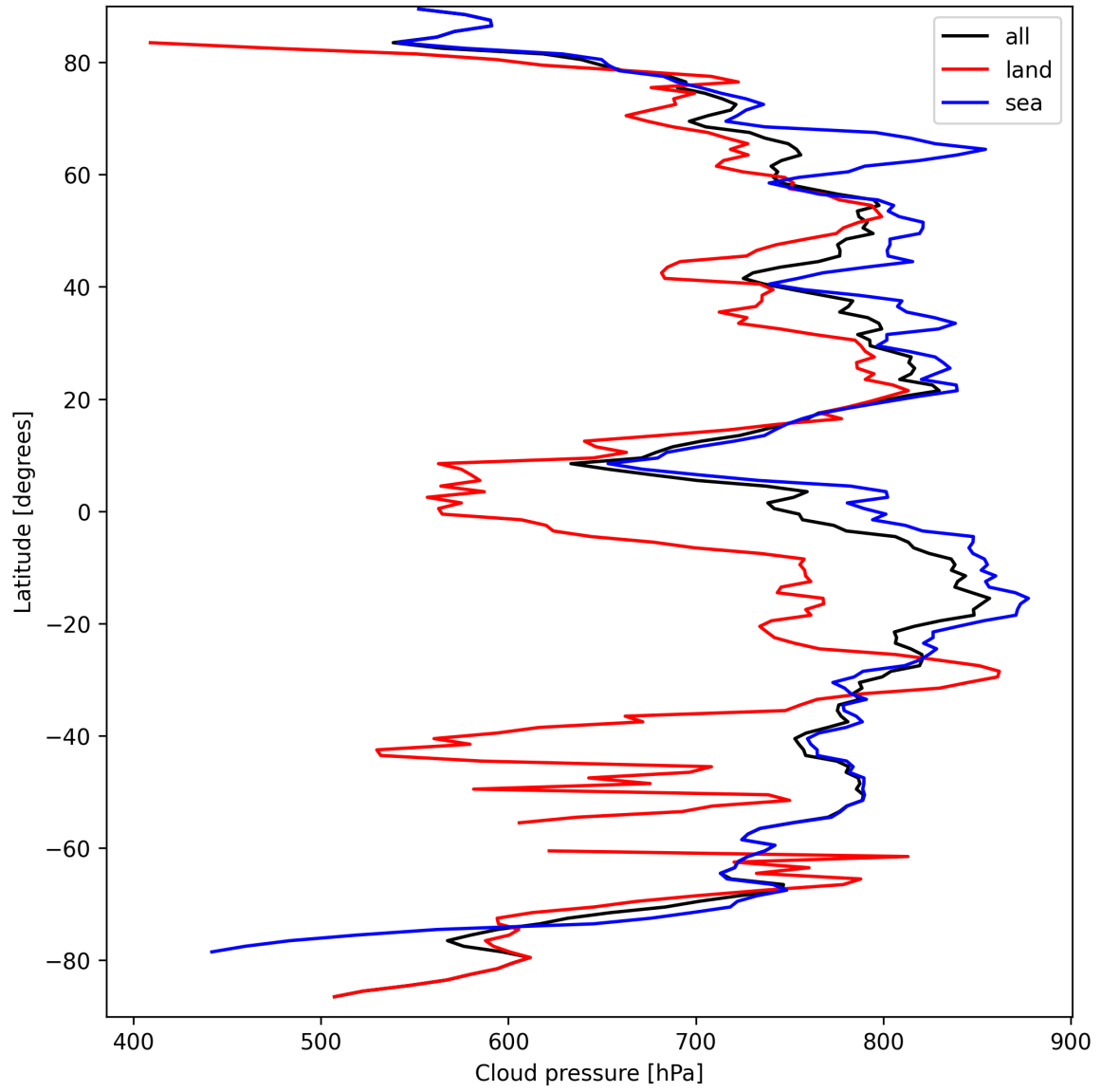
Figure 13: Zonal average of “Cloud pressure” for 2024-09-17 to 2024-09-18.
