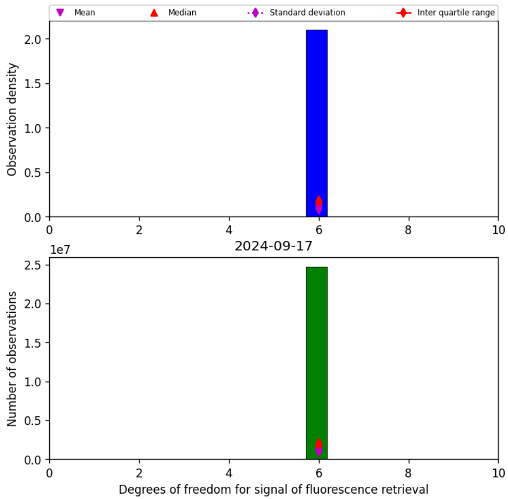
Figure 43: Histogram of “Degrees of freedom for signal of fluorescence retrieval” for 2024-09-17 to 2024-09-18
