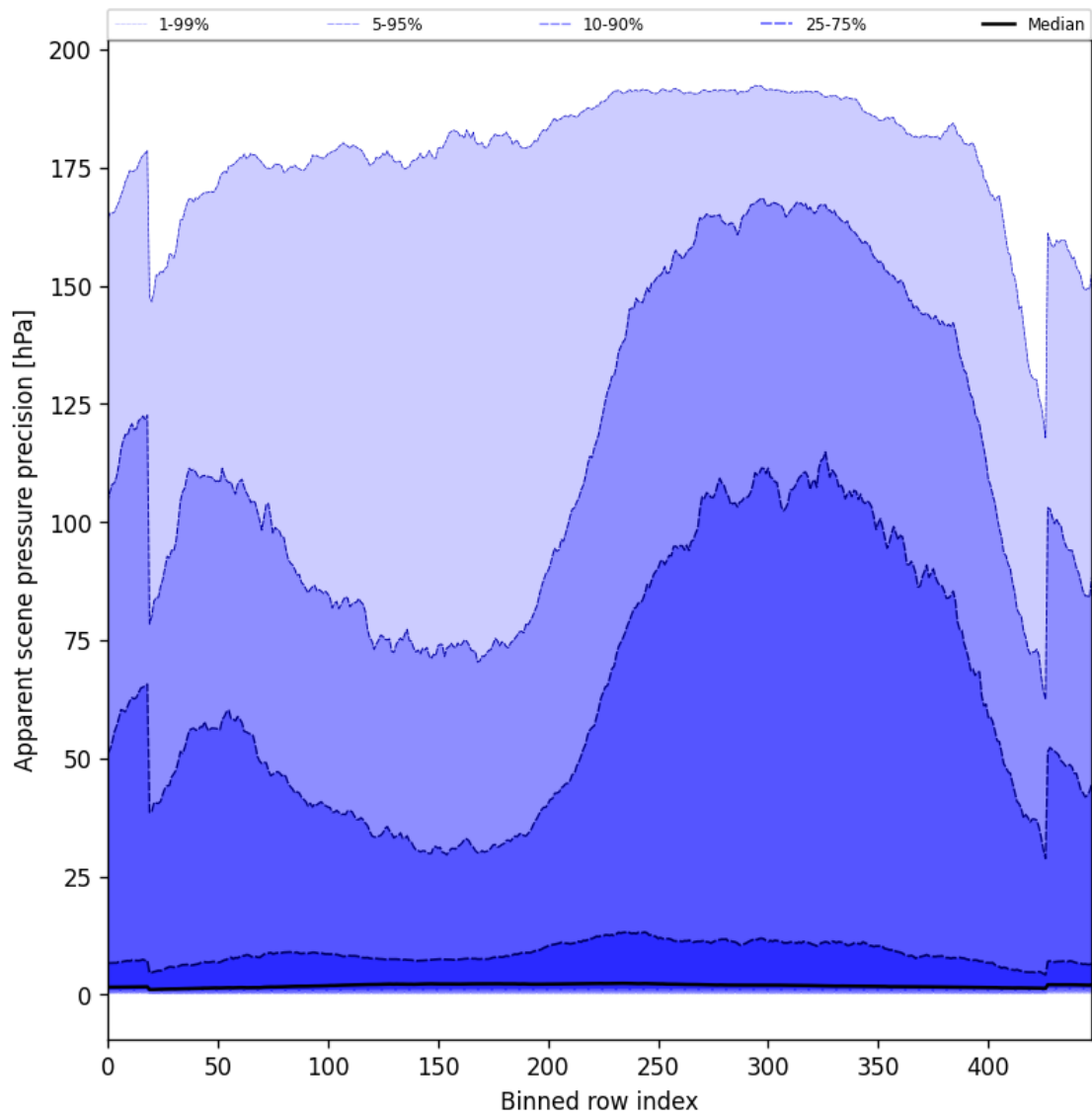
Figure 54: Along track statistics of “Apparent scene pressure precision” for 2024-09-17 to 2024-09-18
