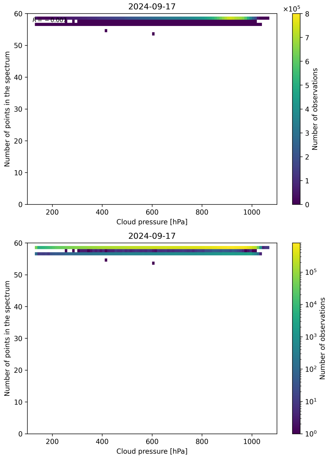
Figure 90: Scatter density plot of “Cloud pressure” against “Number of points in the spectrum” for 2024-09-17 to 2024-09-18.
