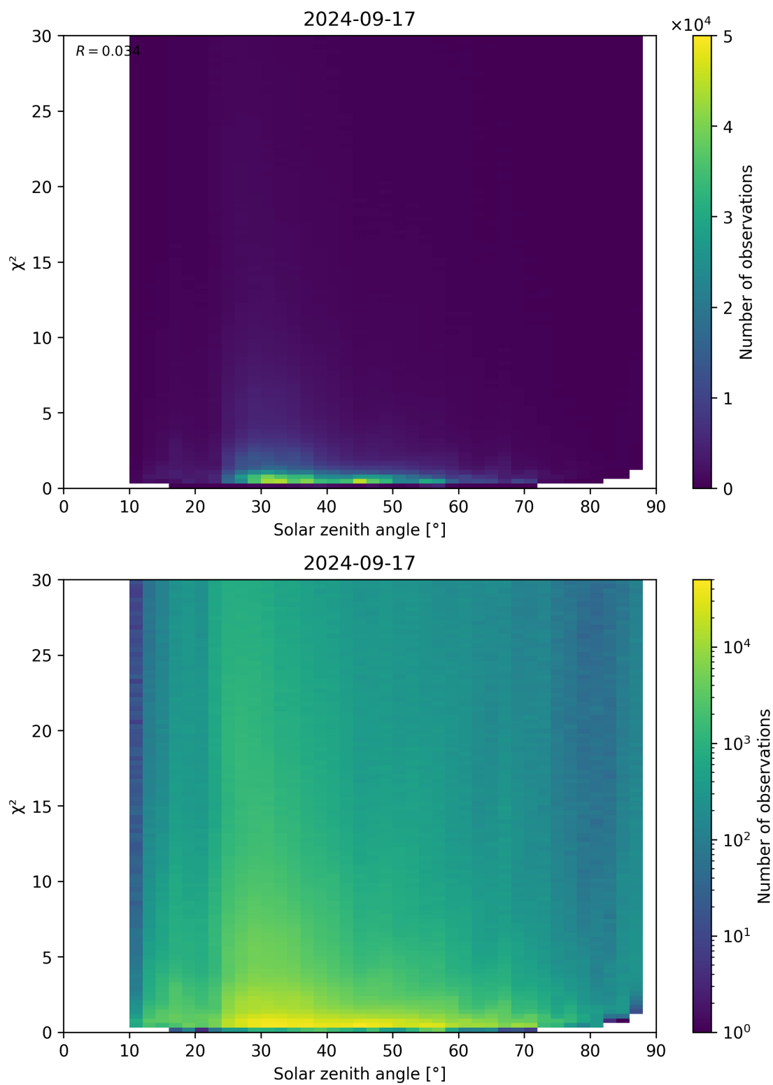
Figure 119: Scatter density plot of “Solar zenith angle” against “ \chi^2 ” for 2024-09-17 to 2024-09-18.
