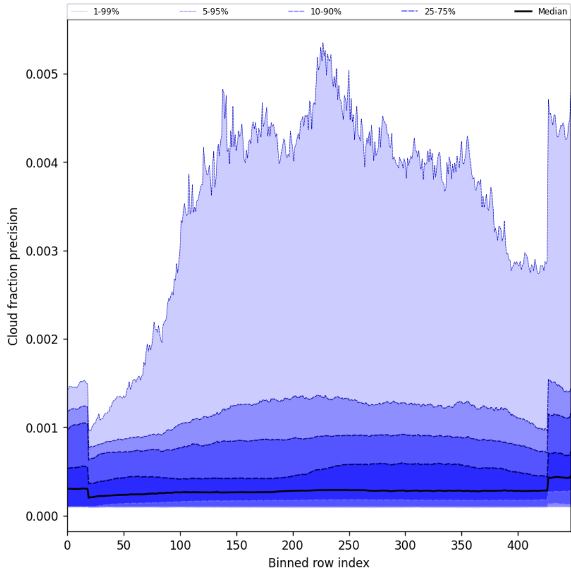
Figure 50: Along track statistics of “Cloud fraction precision” for 2024-09-17 to 2024-09-18
