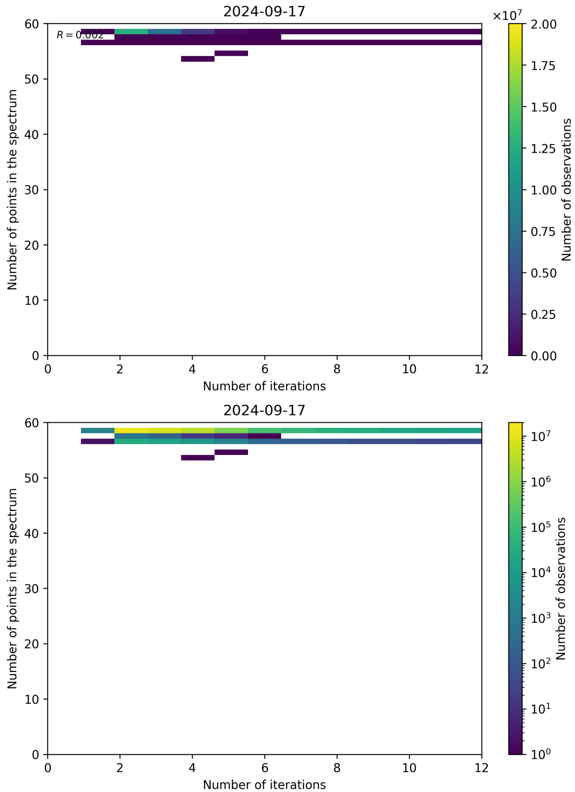
Figure 108: Scatter density plot of “Number of iterations” against “Number of points in the spectrum” for 2024-09-17 to 2024-09-18.
