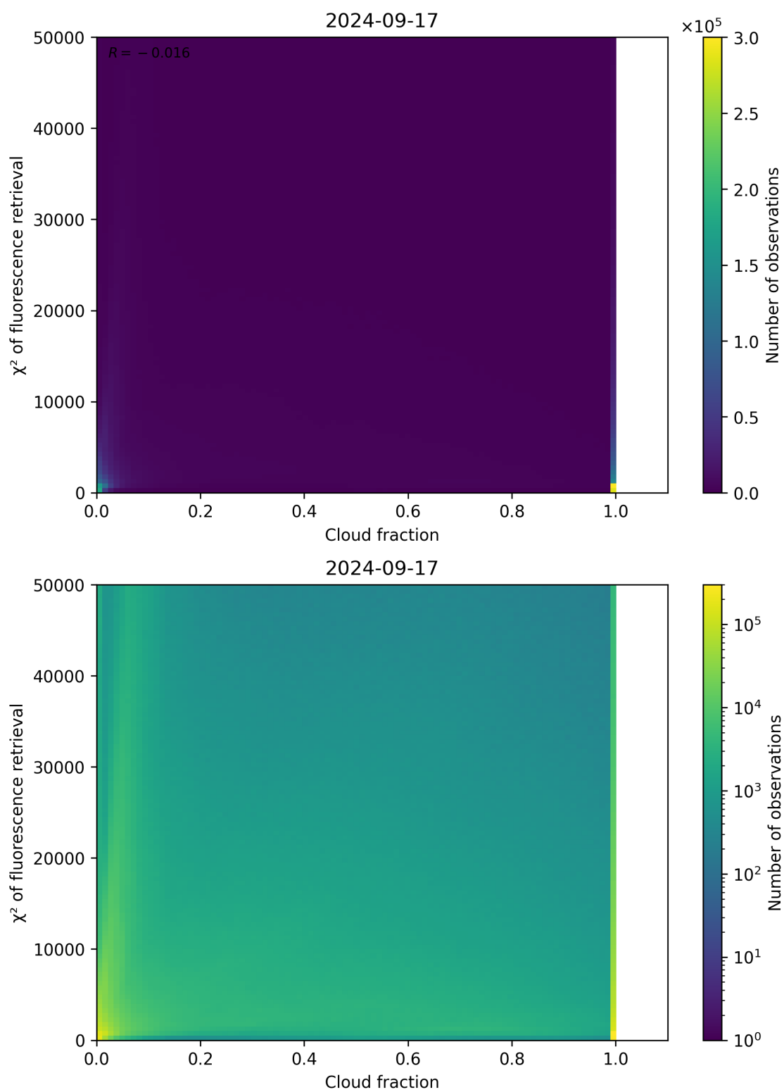
Figure 78: Scatter density plot of “Cloud fraction” against “ \chi^2 of fluorescence retrieval” for 2024-09-17 to 2024-09-18.
