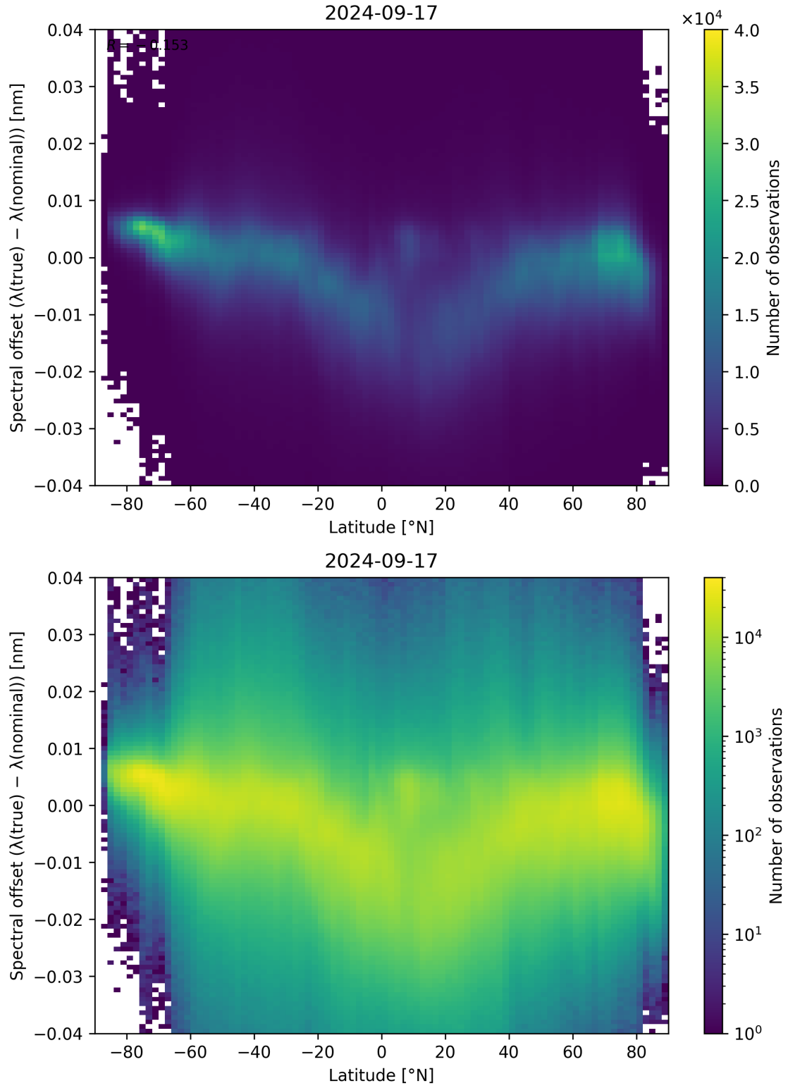
Figure 105: Scatter density plot of “Latitude” against “Spectral offset ( \lambda_{\text{true}} - \lambda_{\text{nominal}} )” for 2024-09-17 to 2024-09-18.
