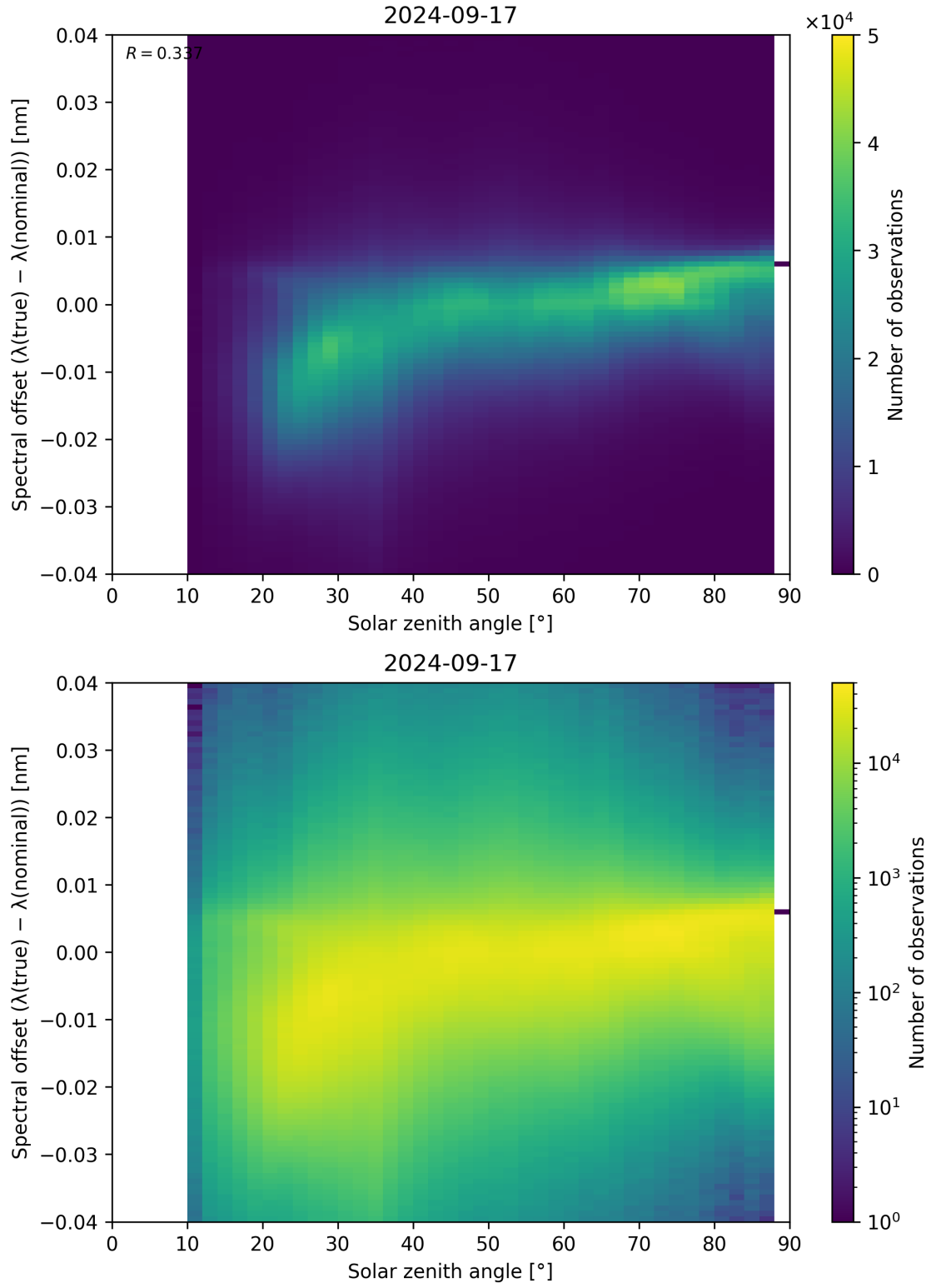
Figure 128: Scatter density plot of “Solar zenith angle” against “Spectral offset ( \lambda_{\text{true}} - \lambda_{\text{nominal}} )” for 2024-09-17 to 2024-09-18.
