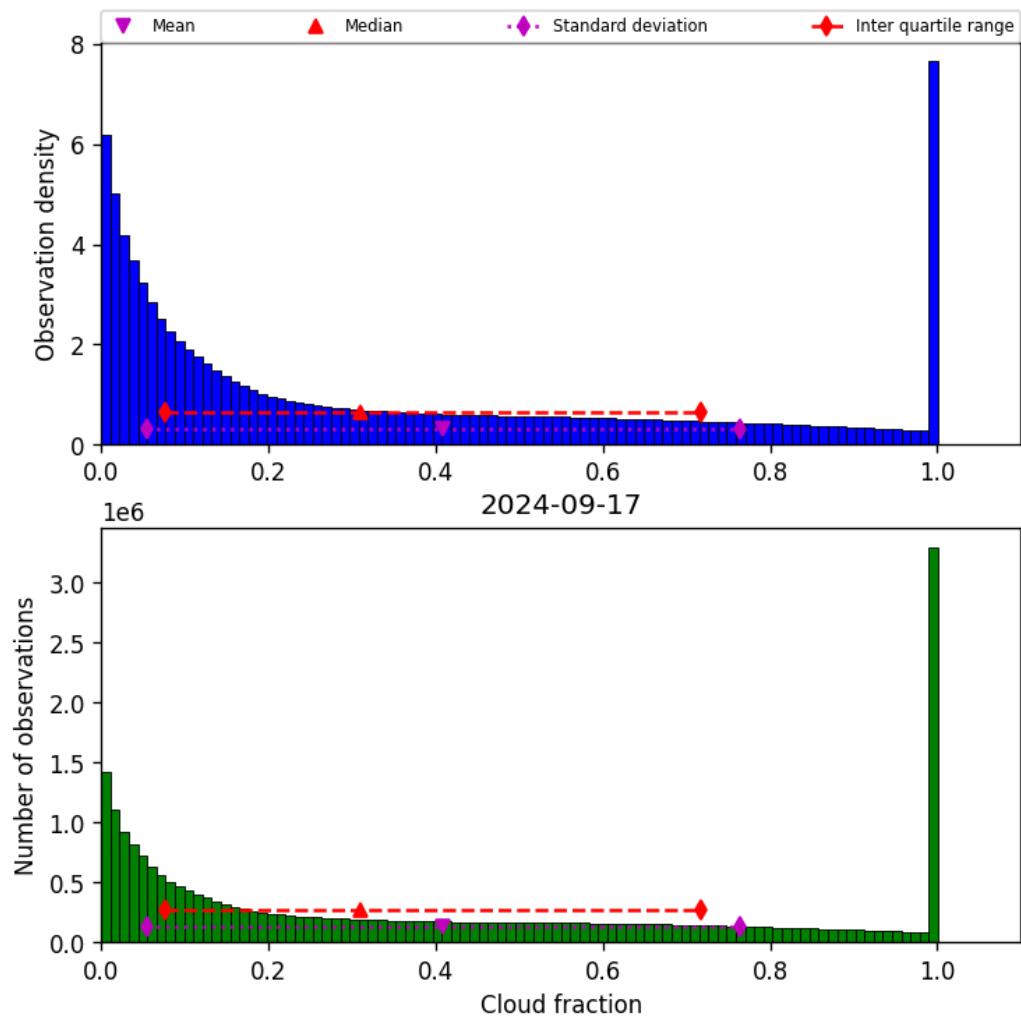
Figure 32: Histogram of “Cloud fraction” for 2024-09-17 to 2024-09-18
