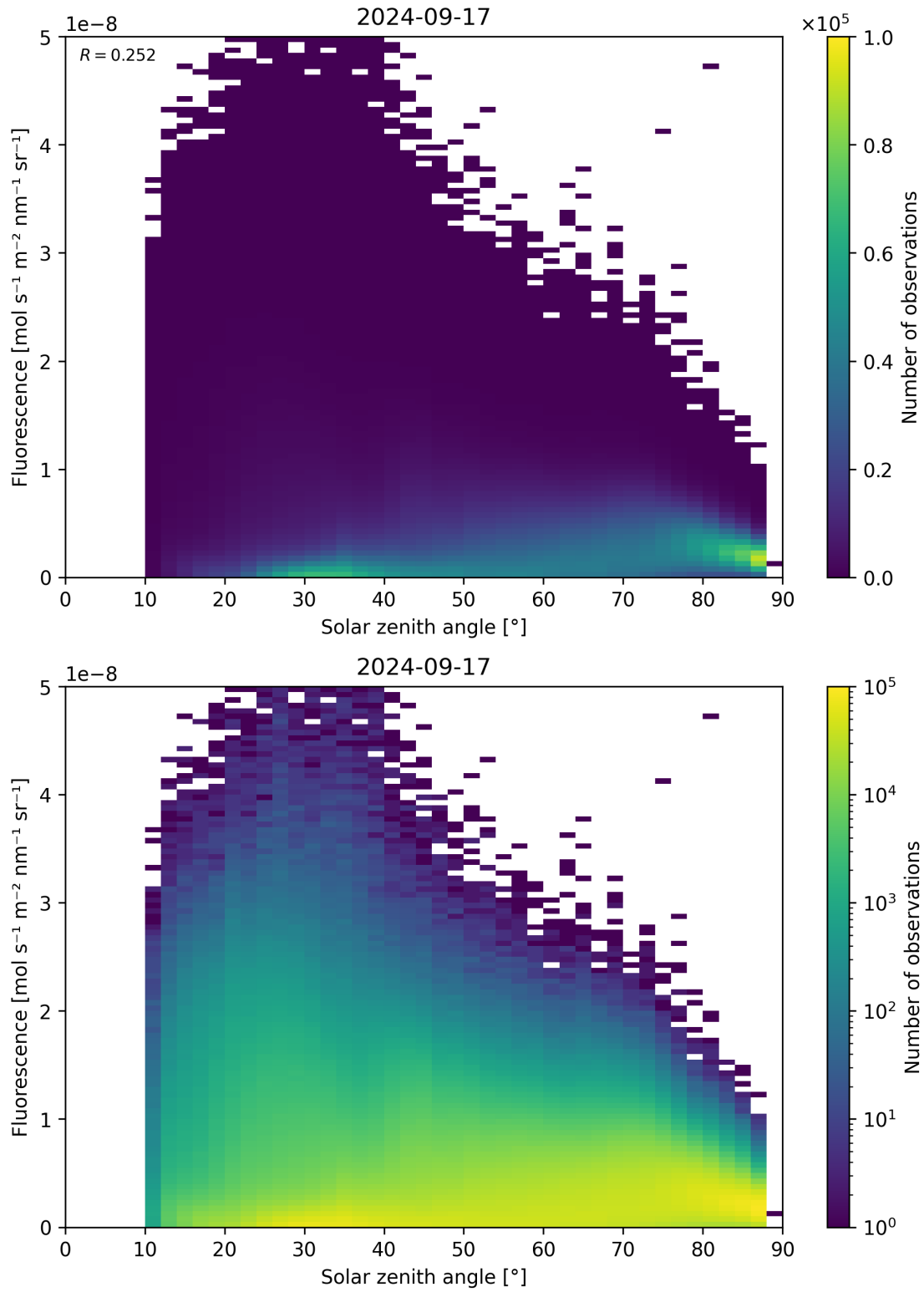
Figure 123: Scatter density plot of “Solar zenith angle” against “Fluorescence” for 2024-09-17 to 2024-09-18.
