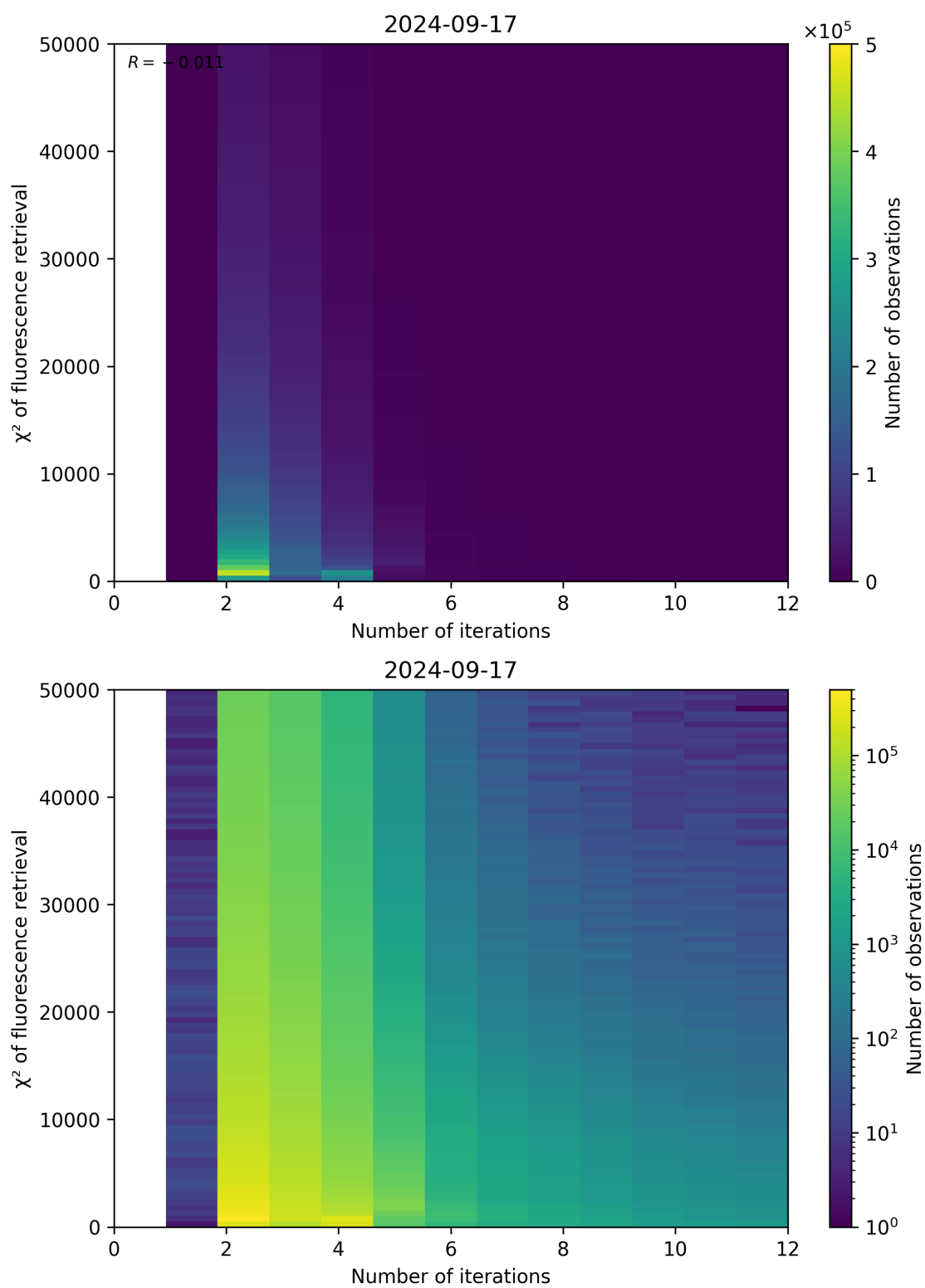
Figure 106: Scatter density plot of “Number of iterations” against “ \chi^2 of fluorescence retrieval” for 2024-09-17 to 2024-09-18.
