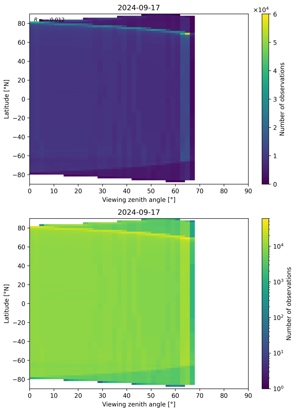
Figure 135: Scatter density plot of “Viewing zenith angle” against “Latitude” for 2024-09-17 to 2024-09-18.
