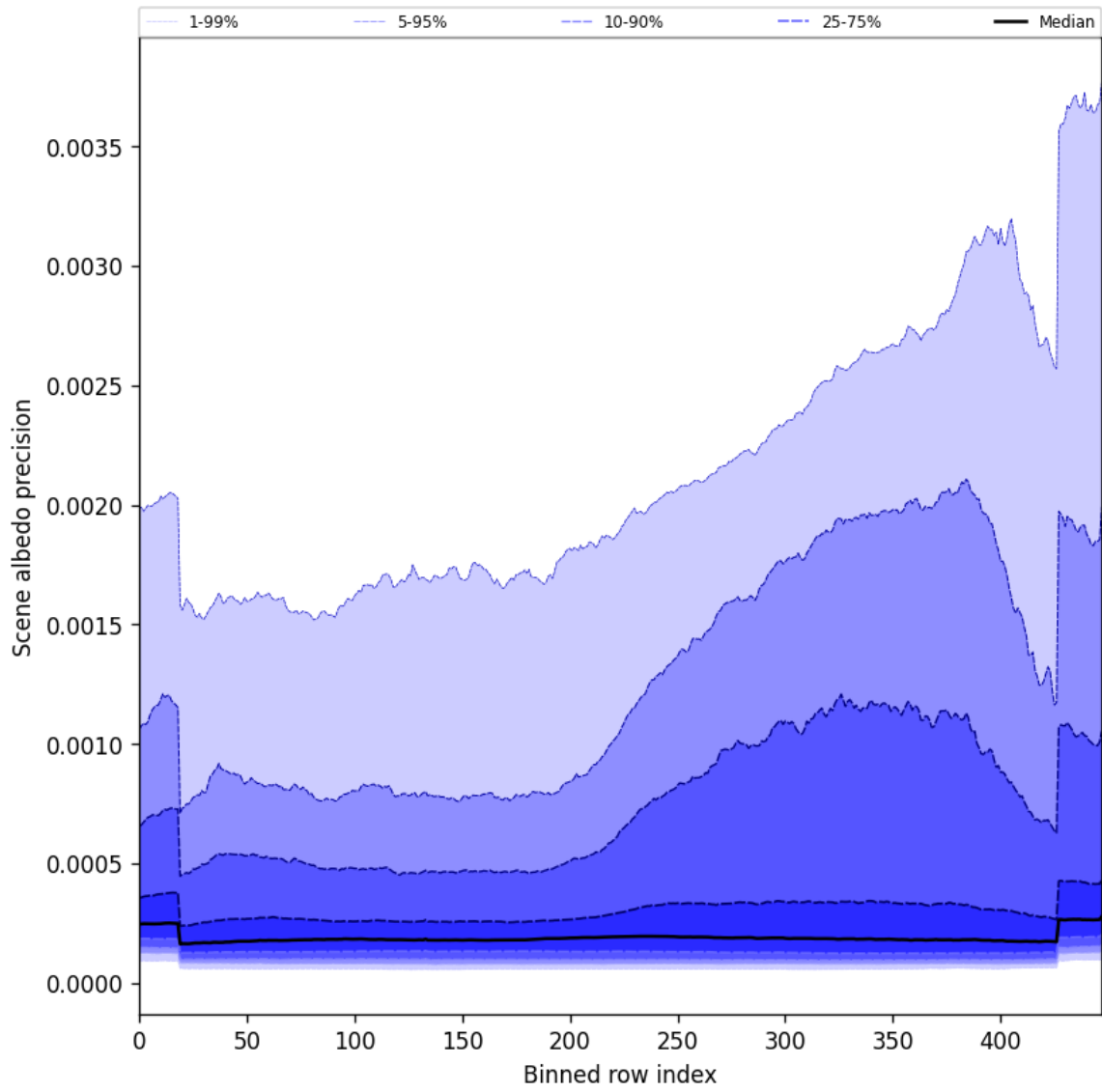
Figure 52: Along track statistics of “Scene albedo precision” for 2024-09-17 to 2024-09-18
