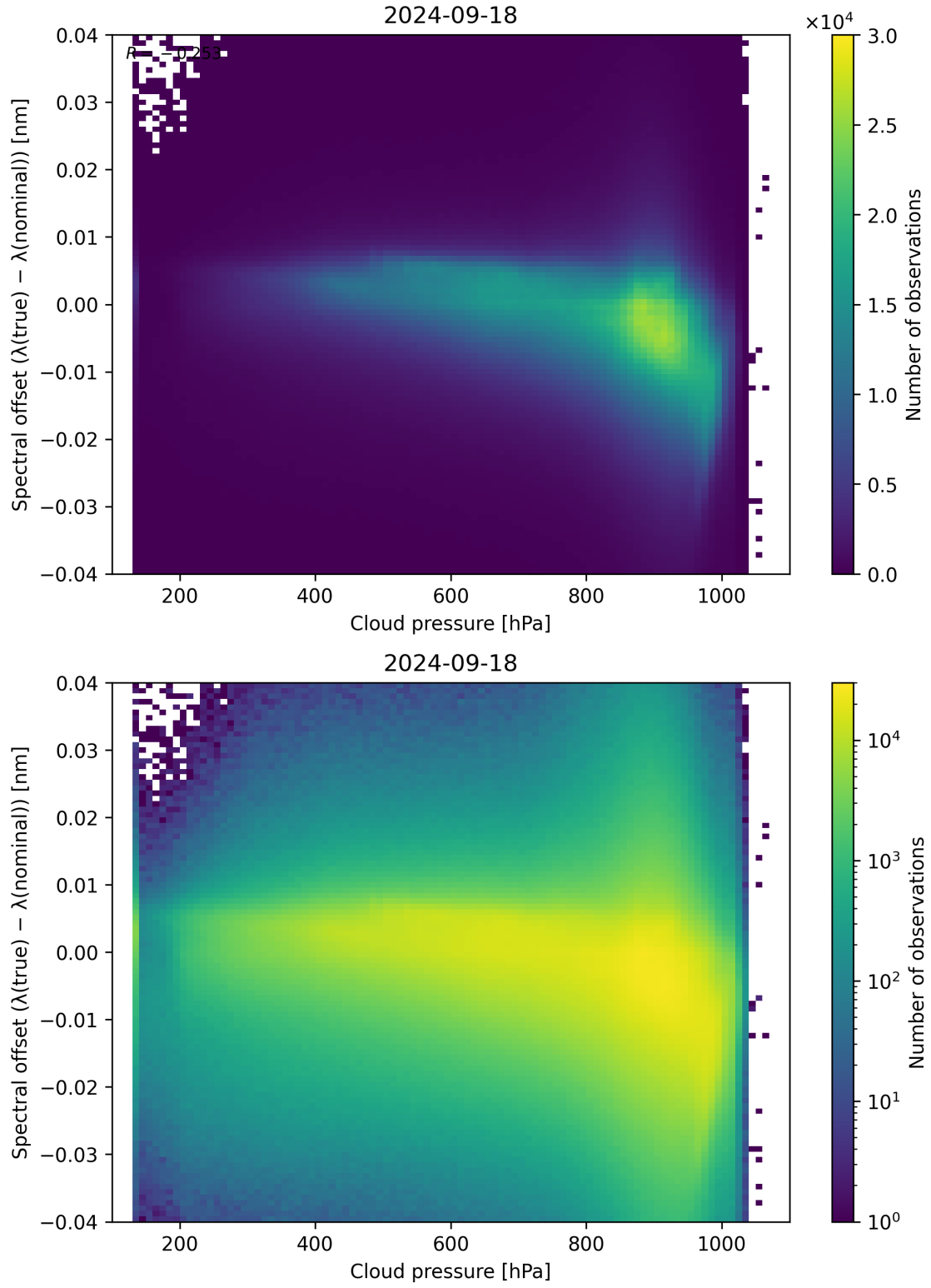
Figure 92: Scatter density plot of “Cloud pressure” against “Spectral offset ( \lambda_{\text{true}} - \lambda_{\text{nominal}} )” for 2024-09-17 to 2024-09-19.
