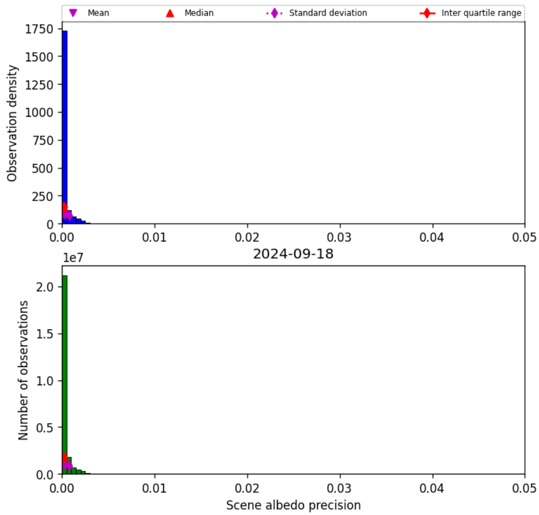
Figure 35: Histogram of “Scene albedo precision” for 2024-09-17 to 2024-09-19
