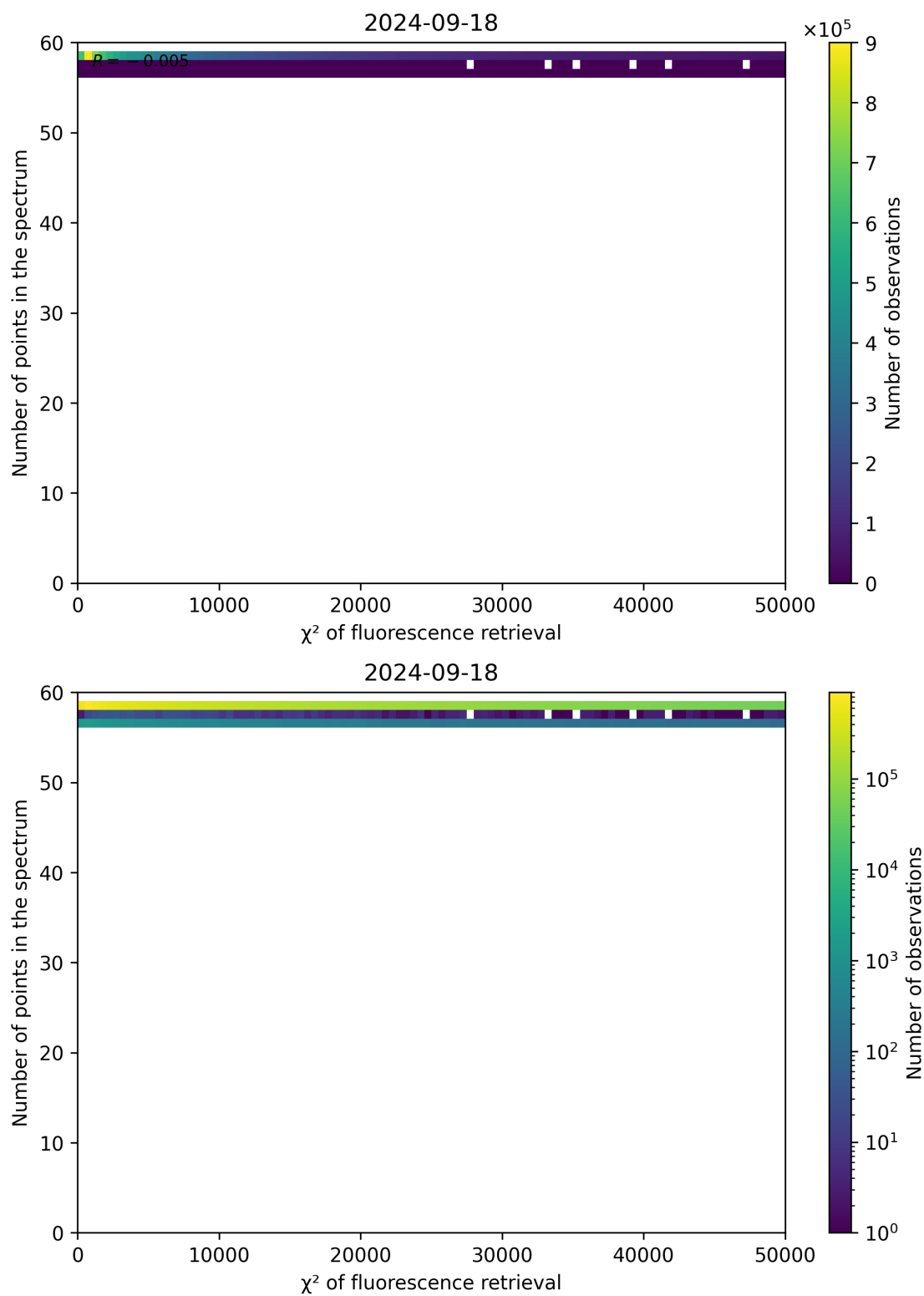
Figure 71: Scatter density plot of " \chi^2 of fluorescence retrieval" against "Number of points in the spectrum" for 2024-09-17 to 2024-09-19.
