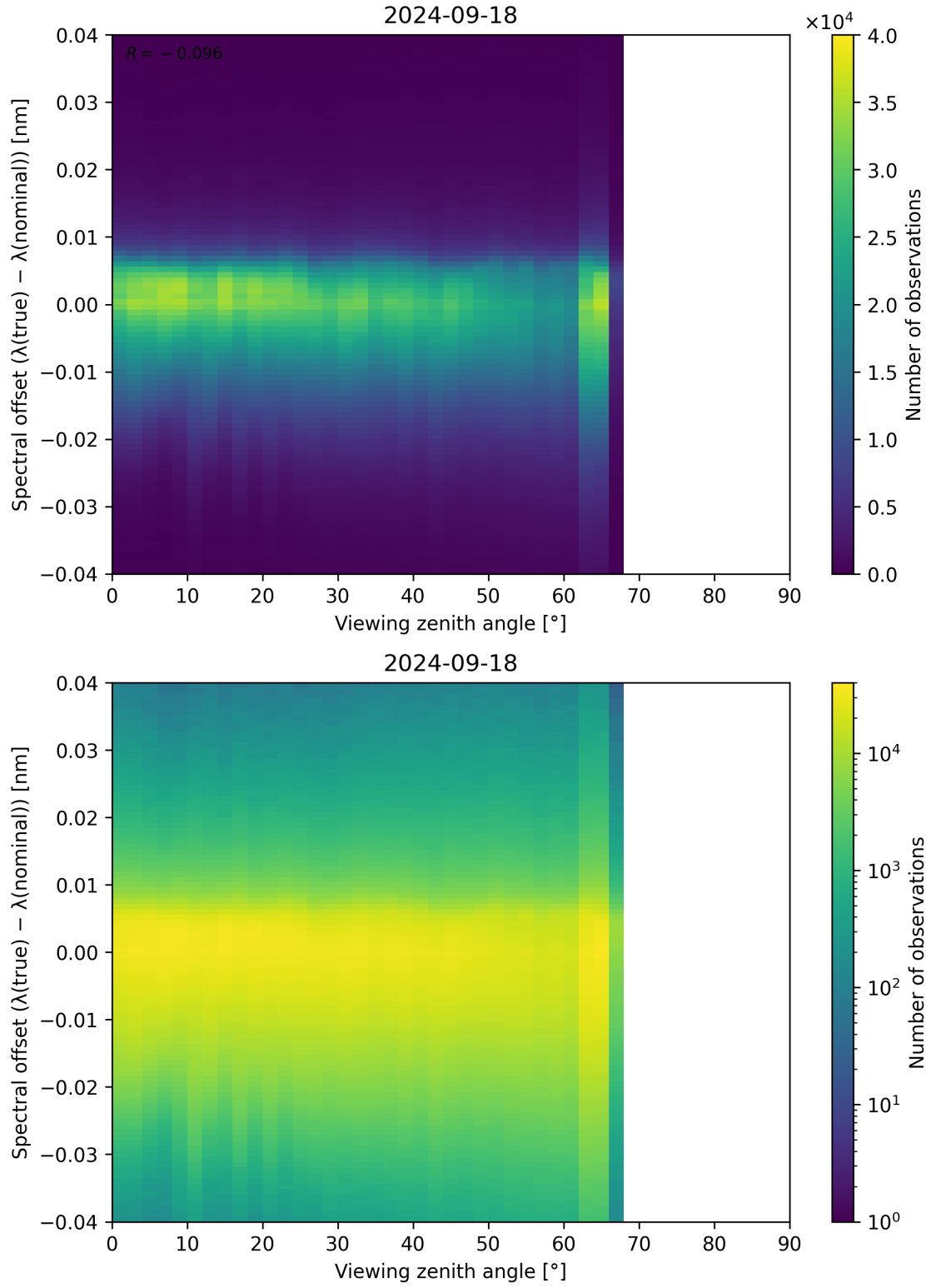
Figure 140: Scatter density plot of “Viewing zenith angle” against “Spectral offset ( \lambda_{\text{true}} - \lambda_{\text{nominal}} )” for 2024-09-17 to 2024-09-19.
