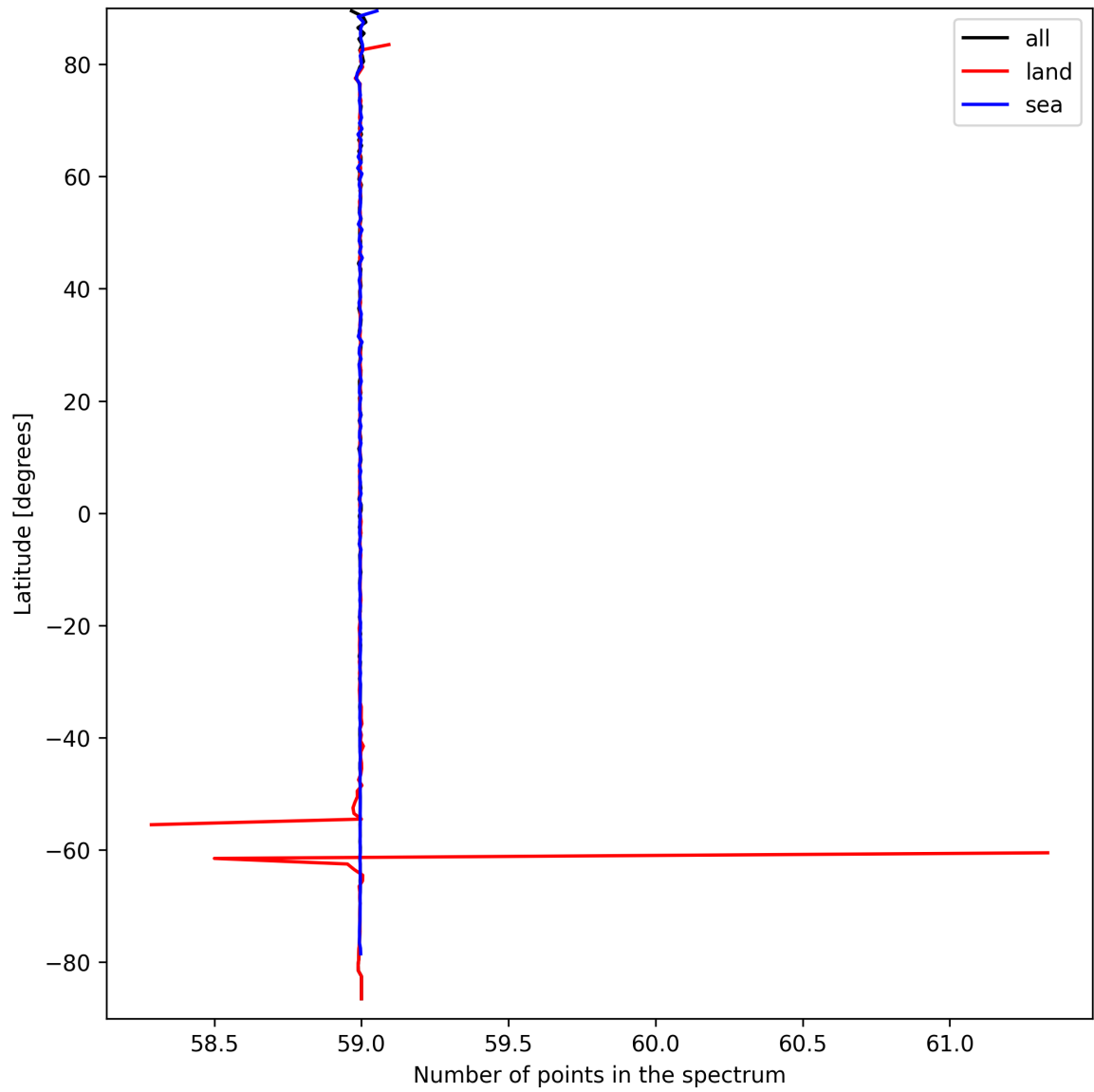
Figure 27: Zonal average of “Number of points in the spectrum” for 2024-09-17 to 2024-09-19.
