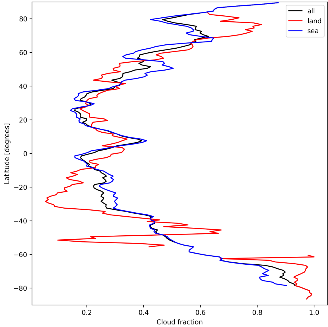
Figure 15: Zonal average of “Cloud fraction” for 2024-09-17 to 2024-09-19.
