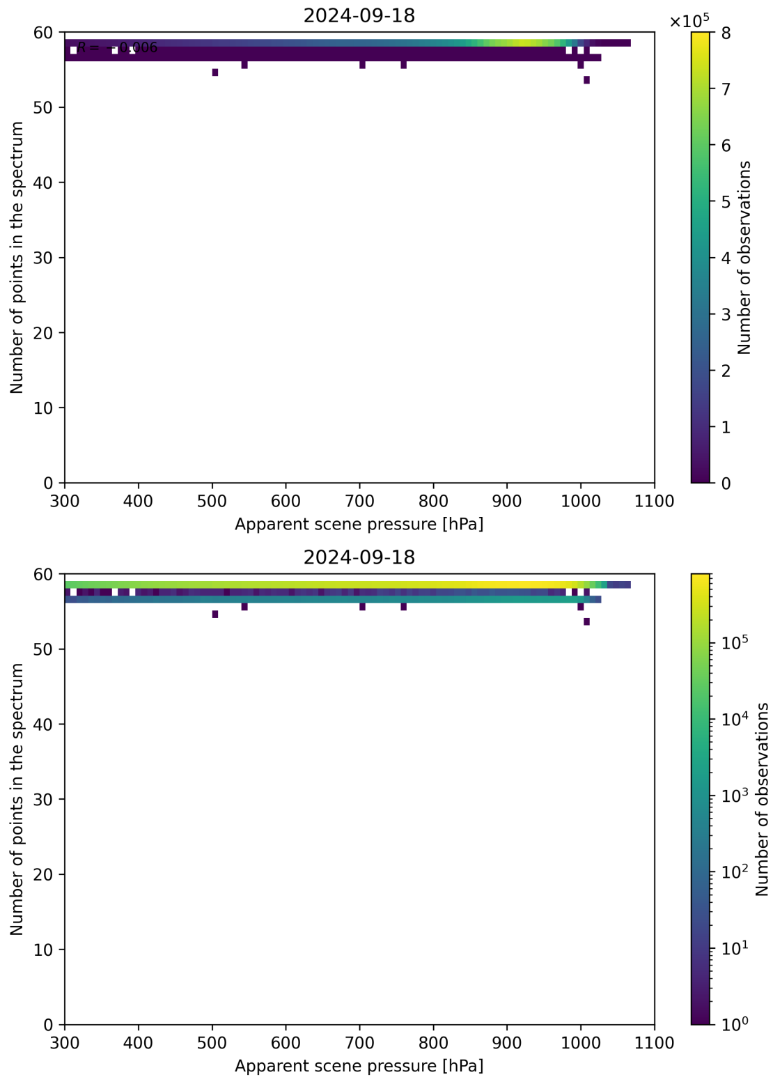
Figure 67: Scatter density plot of “Apparent scene pressure” against “Number of points in the spectrum” for 2024-09-17 to 2024-09-19.
