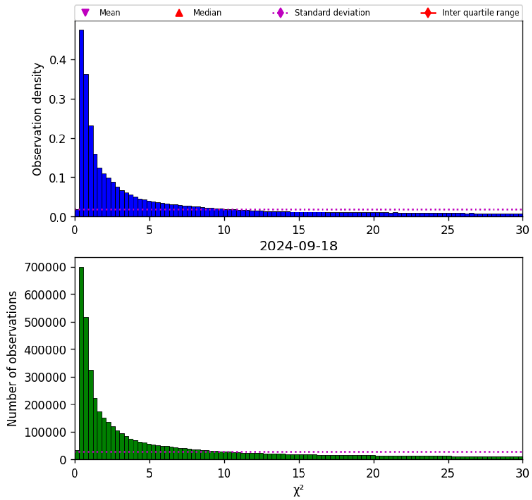
Figure 38: Histogram of “ \chi^2 ” for 2024-09-17 to 2024-09-19
