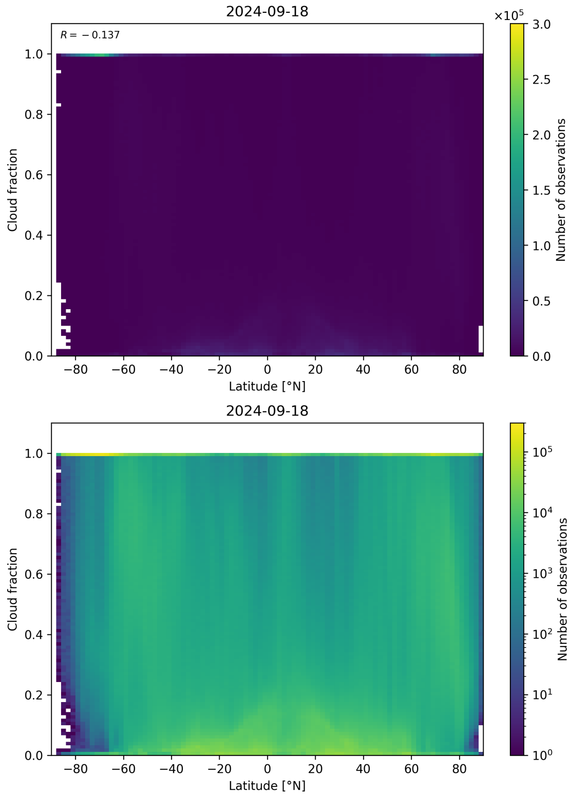
Figure 99: Scatter density plot of “Latitude” against “Cloud fraction” for 2024-09-17 to 2024-09-19.
