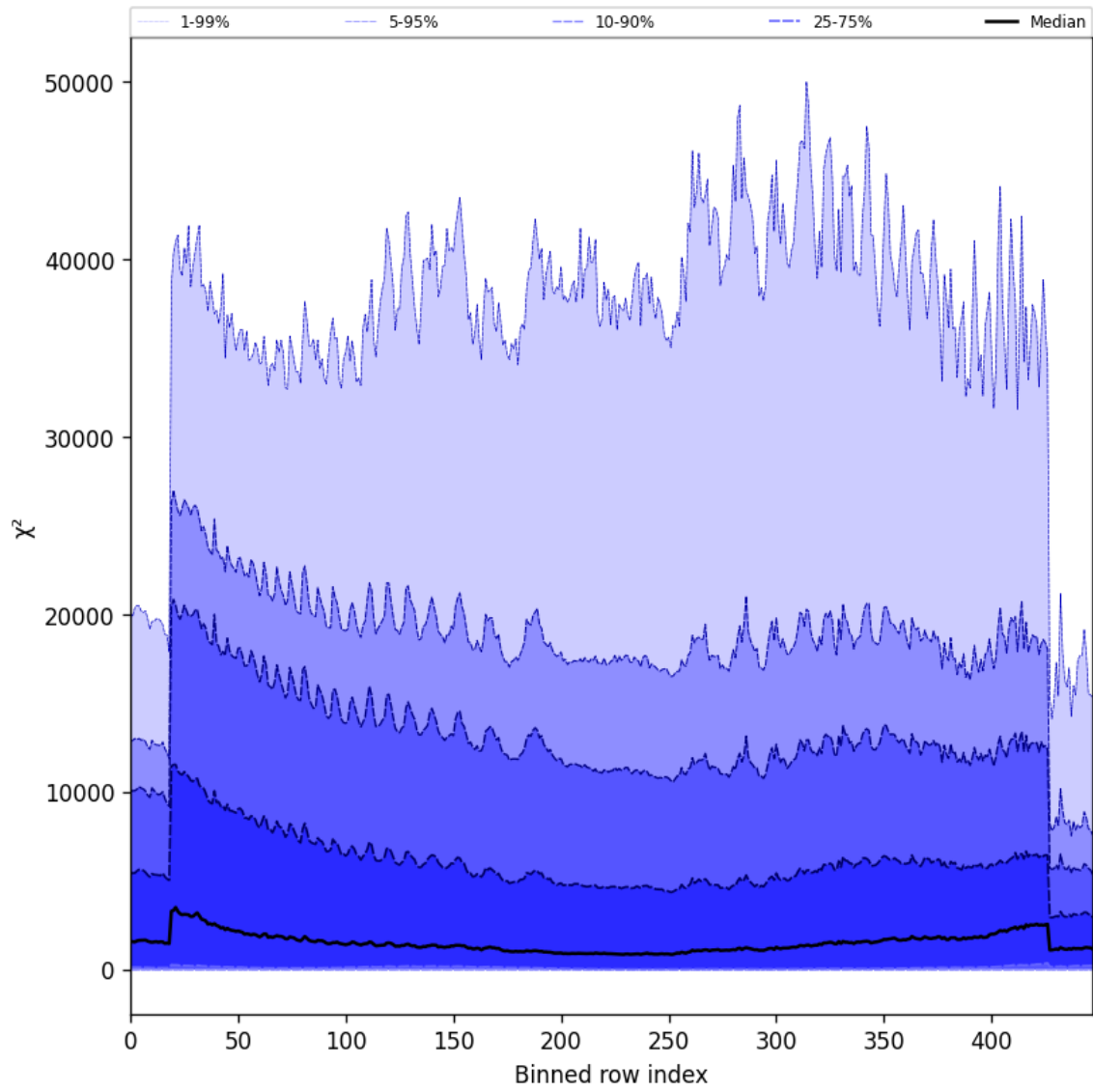
Figure 55: Along track statistics of “ \chi^2 ” for 2024-09-17 to 2024-09-19
