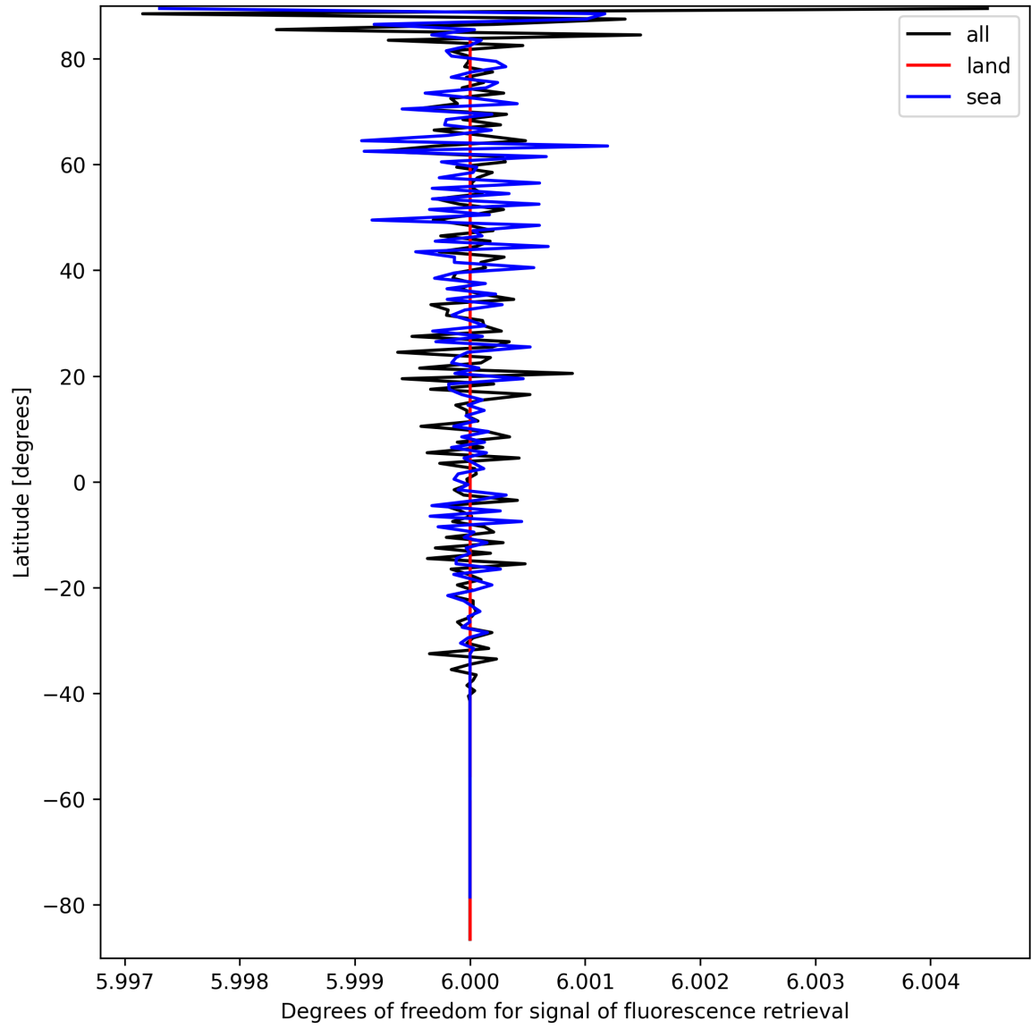
Figure 26: Zonal average of “Degrees of freedom for signal of fluorescence retrieval” for 2024-09-17 to 2024-09-19.
