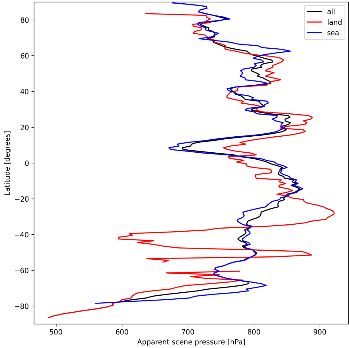
Figure 19: Zonal average of “Apparent scene pressure” for 2024-09-17 to 2024-09-19.
