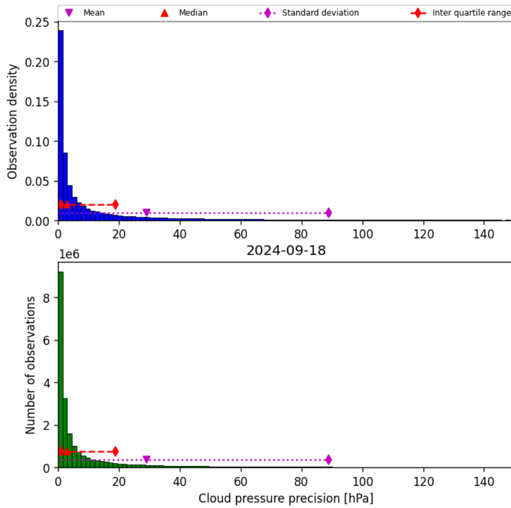
Figure 31: Histogram of “Cloud pressure precision” for 2024-09-17 to 2024-09-19
