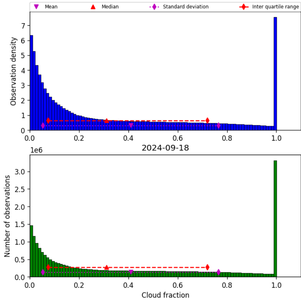
Figure 32: Histogram of “Cloud fraction” for 2024-09-17 to 2024-09-19
