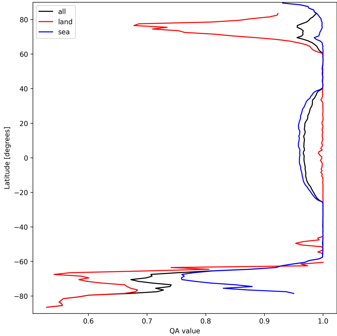
Figure 12: Zonal average of "QA value" for 2024-09-17 to 2024-09-19.
