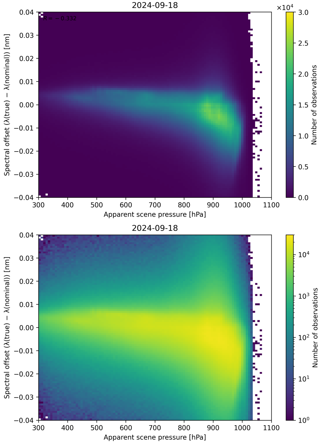
Figure 68: Scatter density plot of “Apparent scene pressure” against “Spectral offset ( \lambda_{\text{true}} - \lambda_{\text{nominal}} )” for 2024-09-17 to 2024-09-19.
