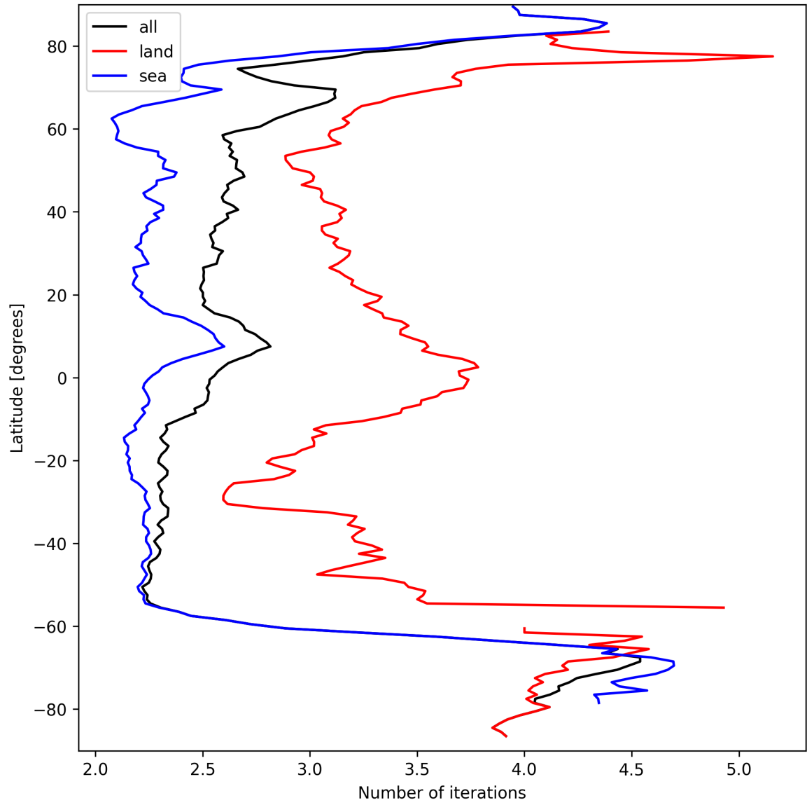
Figure 22: Zonal average of “Number of iterations” for 2024-09-17 to 2024-09-19.
