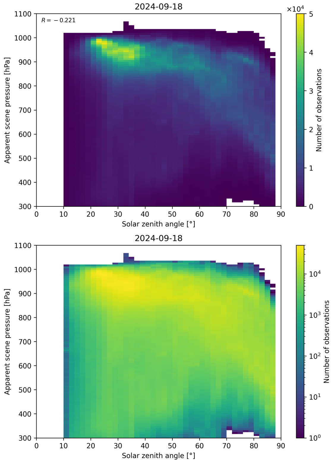
Figure 118: Scatter density plot of “Solar zenith angle” against “Apparent scene pressure” for 2024-09-17 to 2024-09-19.
