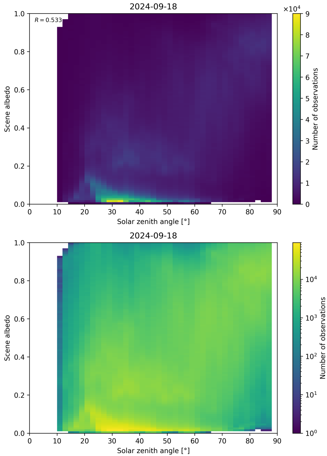
Figure 127: Scatter density plot of “Solar zenith angle” against “Scene albedo” for 2024-09-17 to 2024-09-19.
