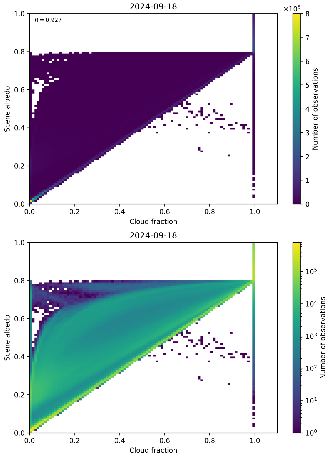
Figure 82: Scatter density plot of “Cloud fraction” against “Scene albedo” for 2024-09-17 to 2024-09-19.
