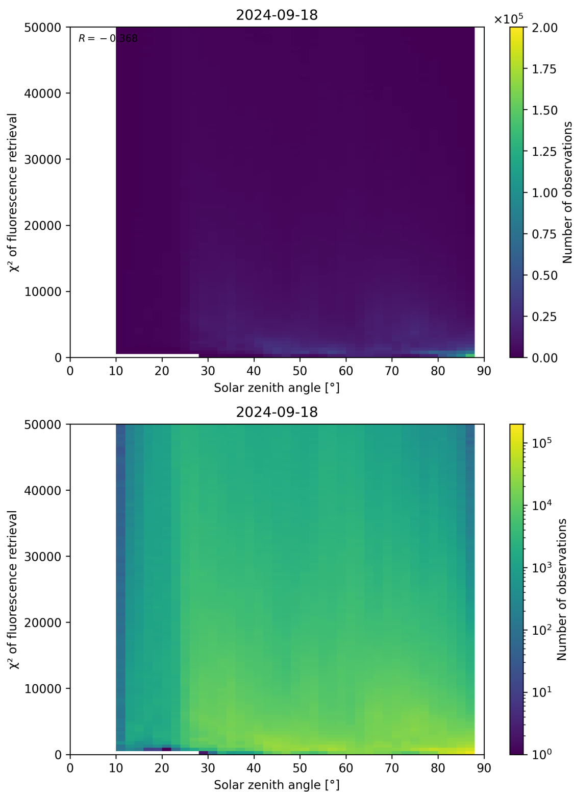
Figure 120: Scatter density plot of “Solar zenith angle” against “ \chi^2 of fluorescence retrieval” for 2024-09-17 to 2024-09-19.
