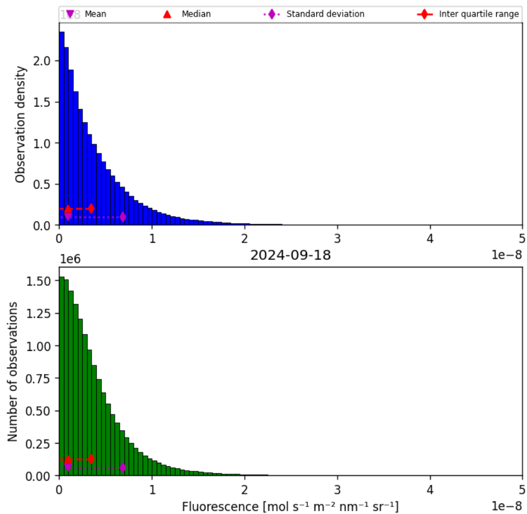
Figure 40: Histogram of “Fluorescence” for 2024-09-17 to 2024-09-19
