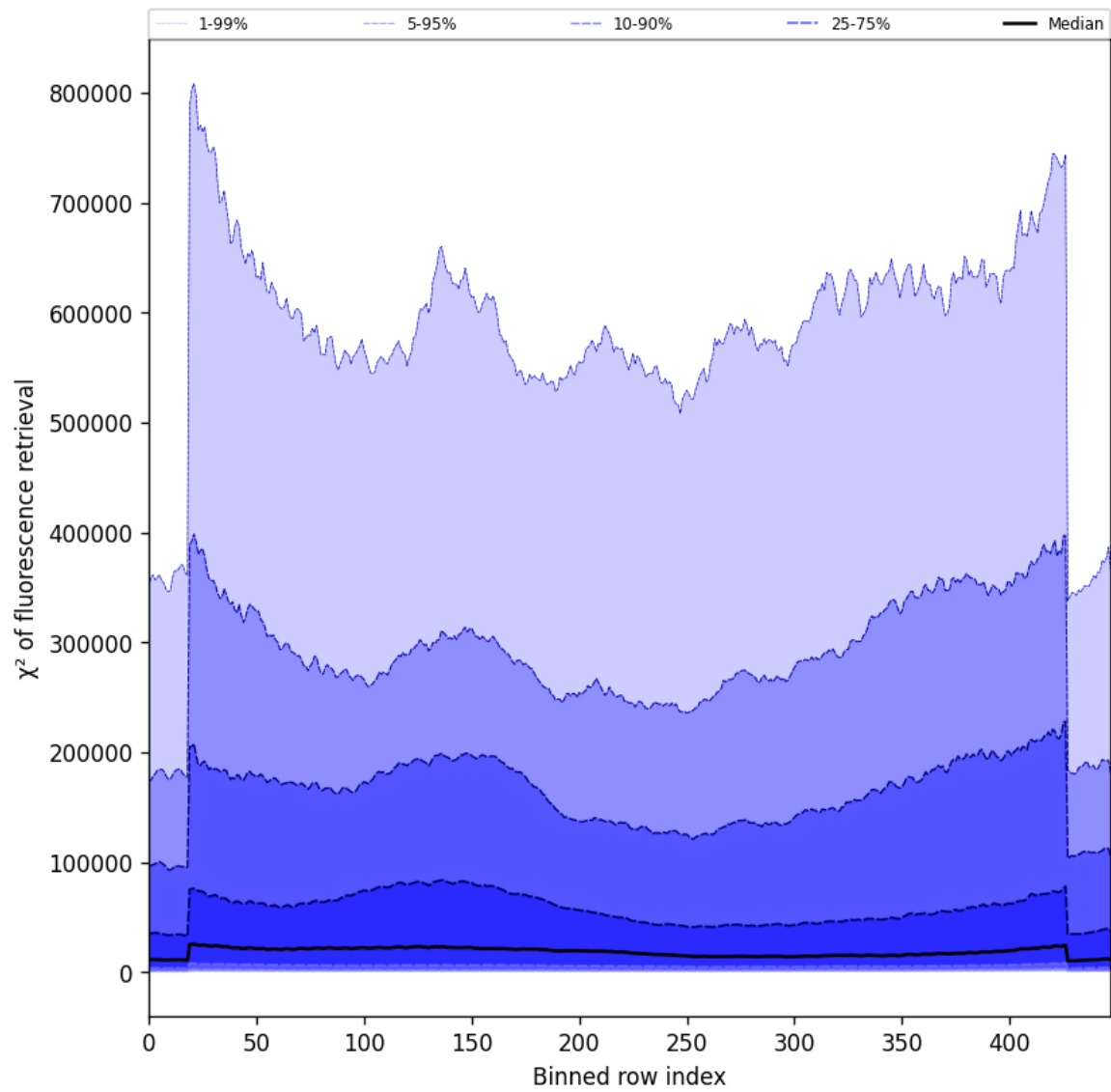
Figure 59: Along track statistics of “ \chi^2 of fluorescence retrieval” for 2024-09-17 to 2024-09-19
