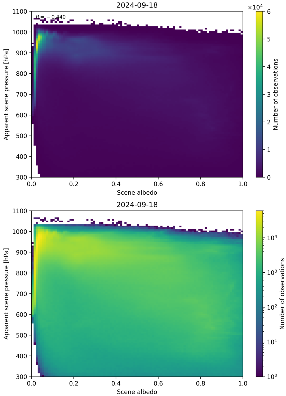
Figure 111: Scatter density plot of “Scene albedo” against “Apparent scene pressure” for 2024-09-17 to 2024-09-19.
