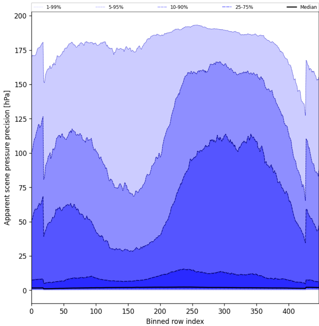
Figure 54: Along track statistics of “Apparent scene pressure precision” for 2024-09-17 to 2024-09-19
