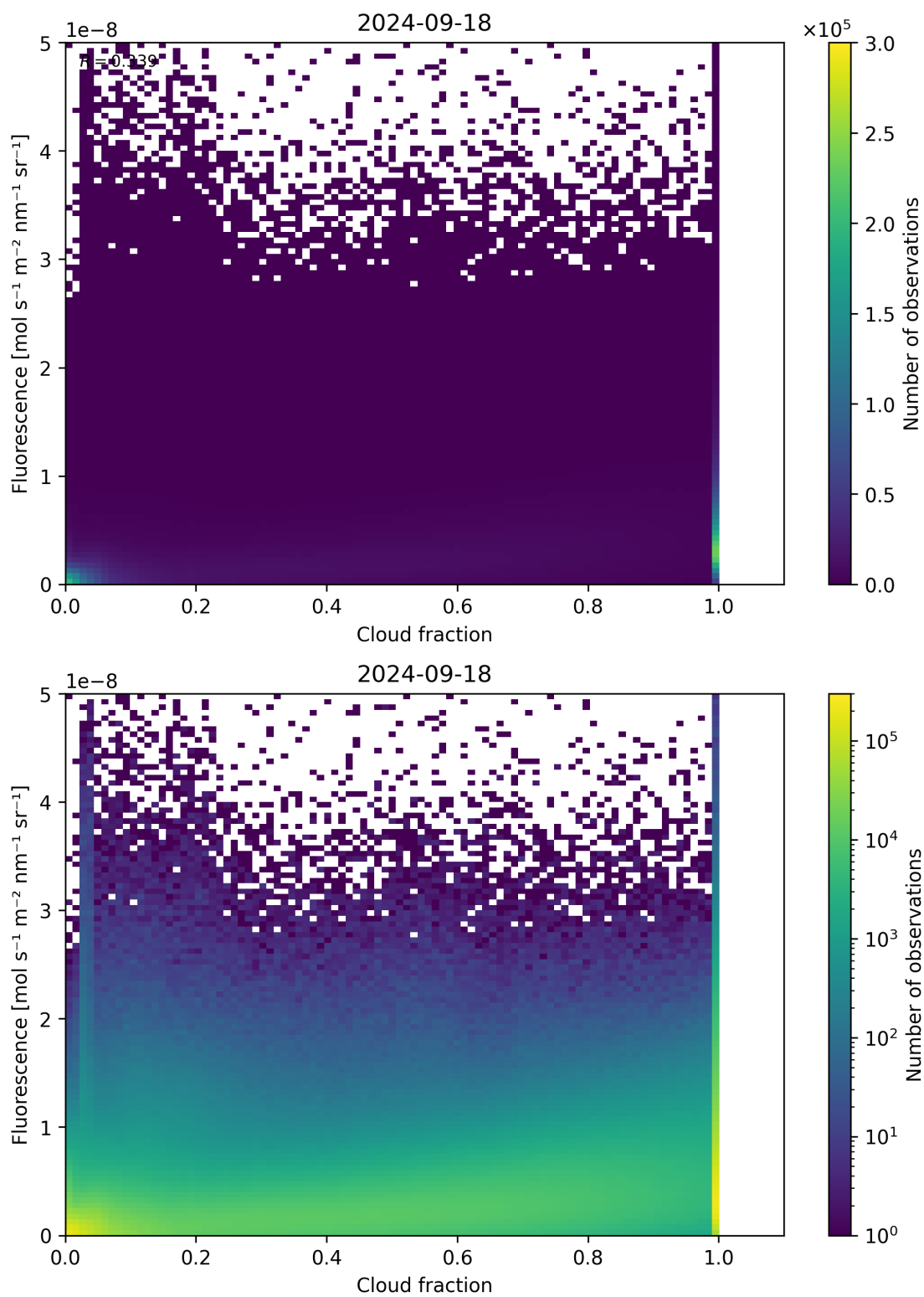
Figure 79: Scatter density plot of “Cloud fraction” against “Fluorescence” for 2024-09-17 to 2024-09-19.
