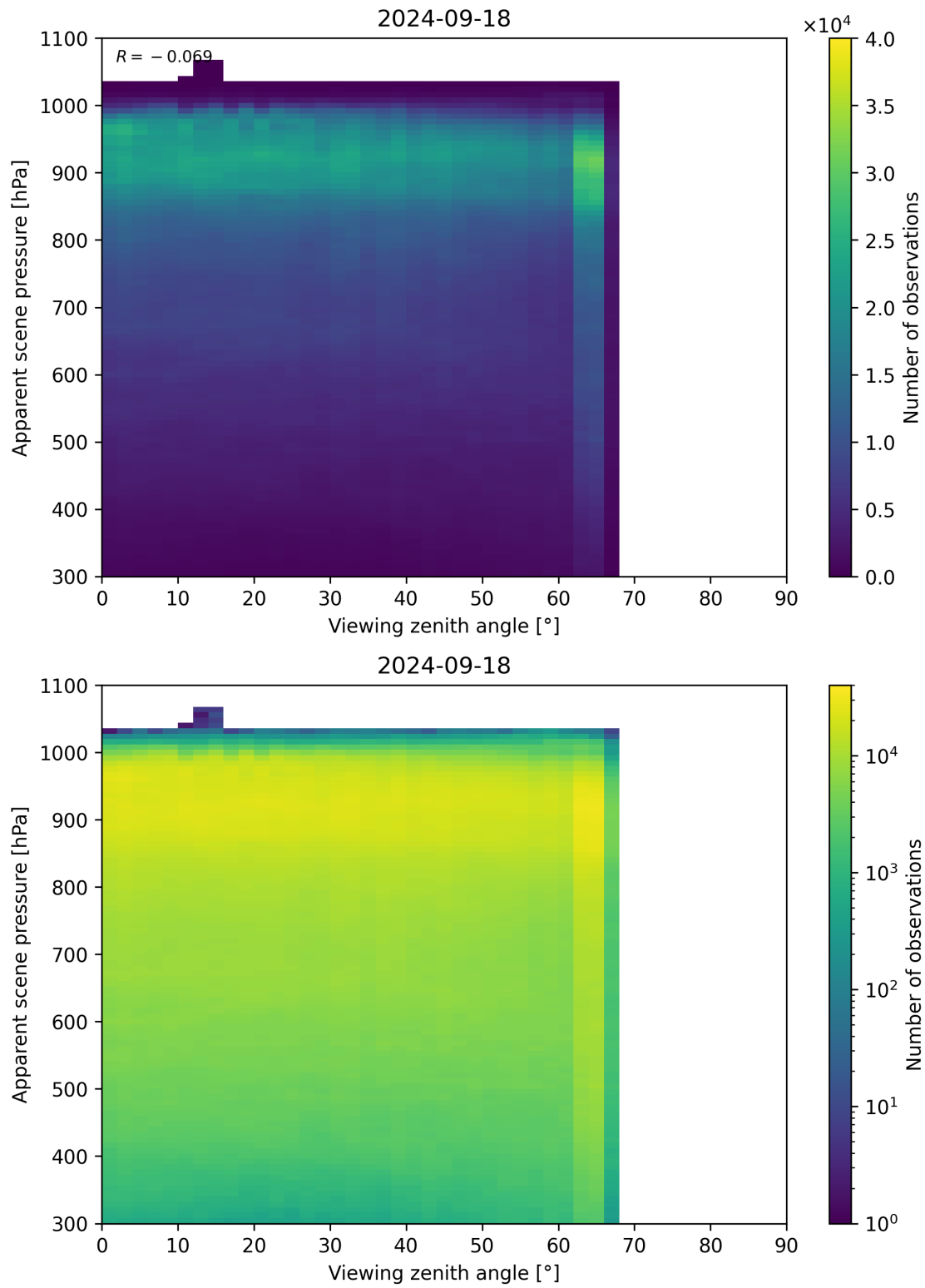
Figure 129: Scatter density plot of “Viewing zenith angle” against “Apparent scene pressure” for 2024-09-17 to 2024-09-19.
