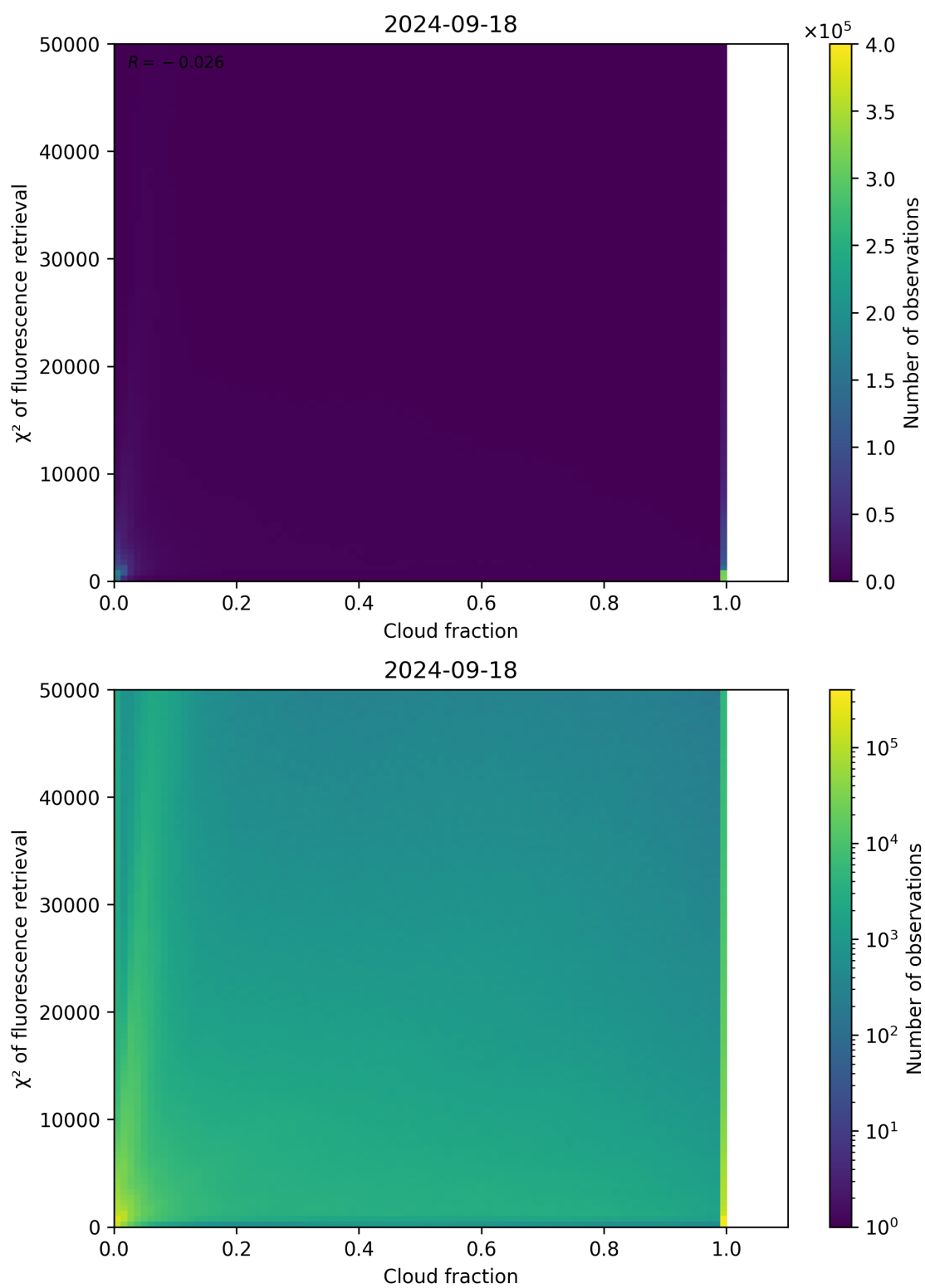
Figure 78: Scatter density plot of “Cloud fraction” against “ \chi^2 of fluorescence retrieval” for 2024-09-17 to 2024-09-19.
