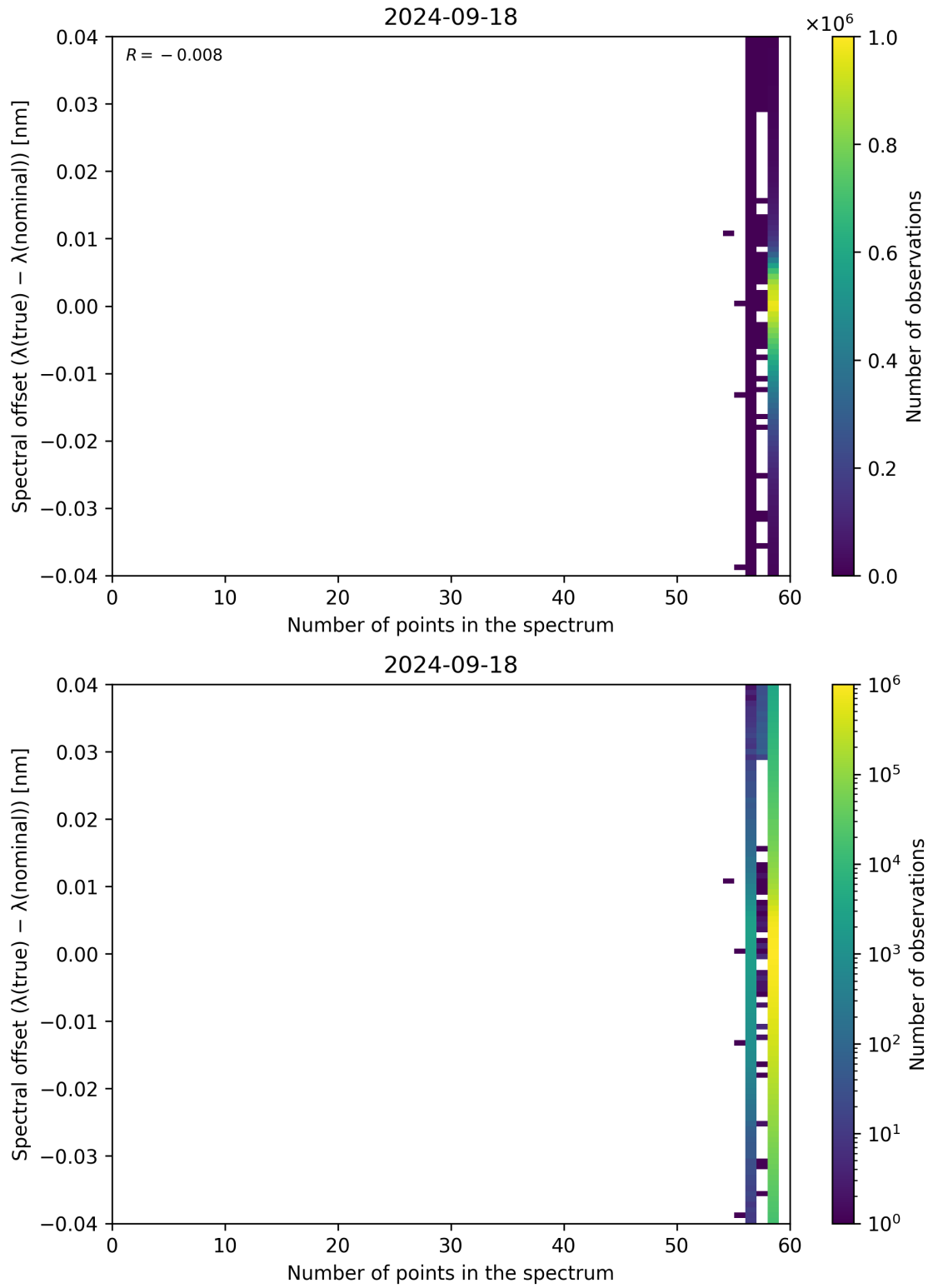
Figure 110: Scatter density plot of “Number of points in the spectrum” against “Spectral offset ( \lambda_{\text{true}} - \lambda_{\text{nominal}} )” for 2024-09-17 to 2024-09-19.
