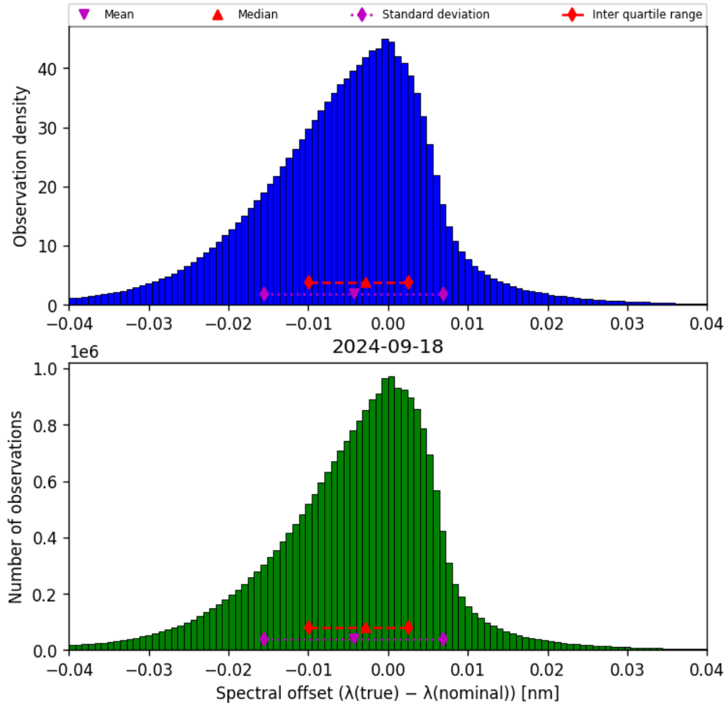
Figure 45: Histogram of “Spectral offset ( \lambda_{\text{true}} - \lambda_{\text{nominal}} )” for 2024-09-17 to 2024-09-19
