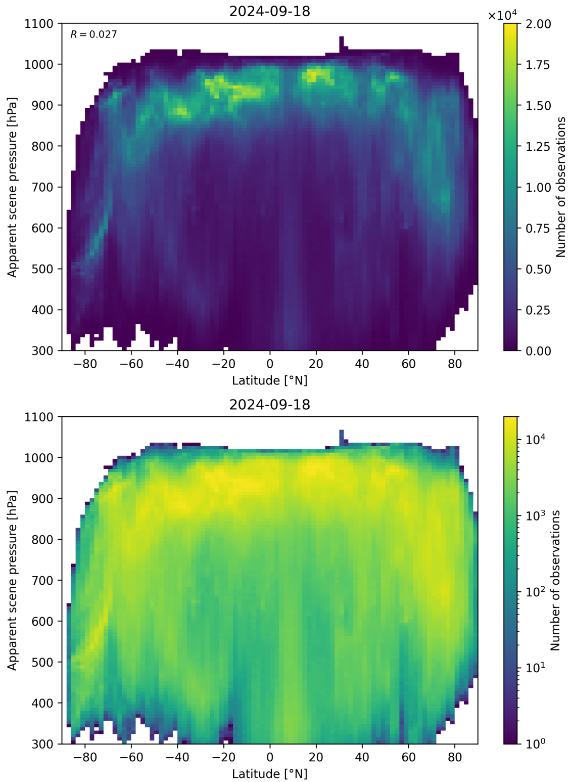
Figure 96: Scatter density plot of “Latitude” against “Apparent scene pressure” for 2024-09-17 to 2024-09-19.
