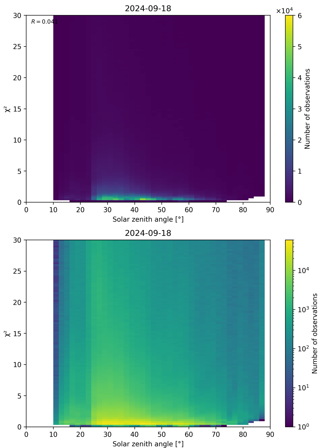
Figure 119: Scatter density plot of “Solar zenith angle” against “ \chi^2 ” for 2024-09-17 to 2024-09-19.
