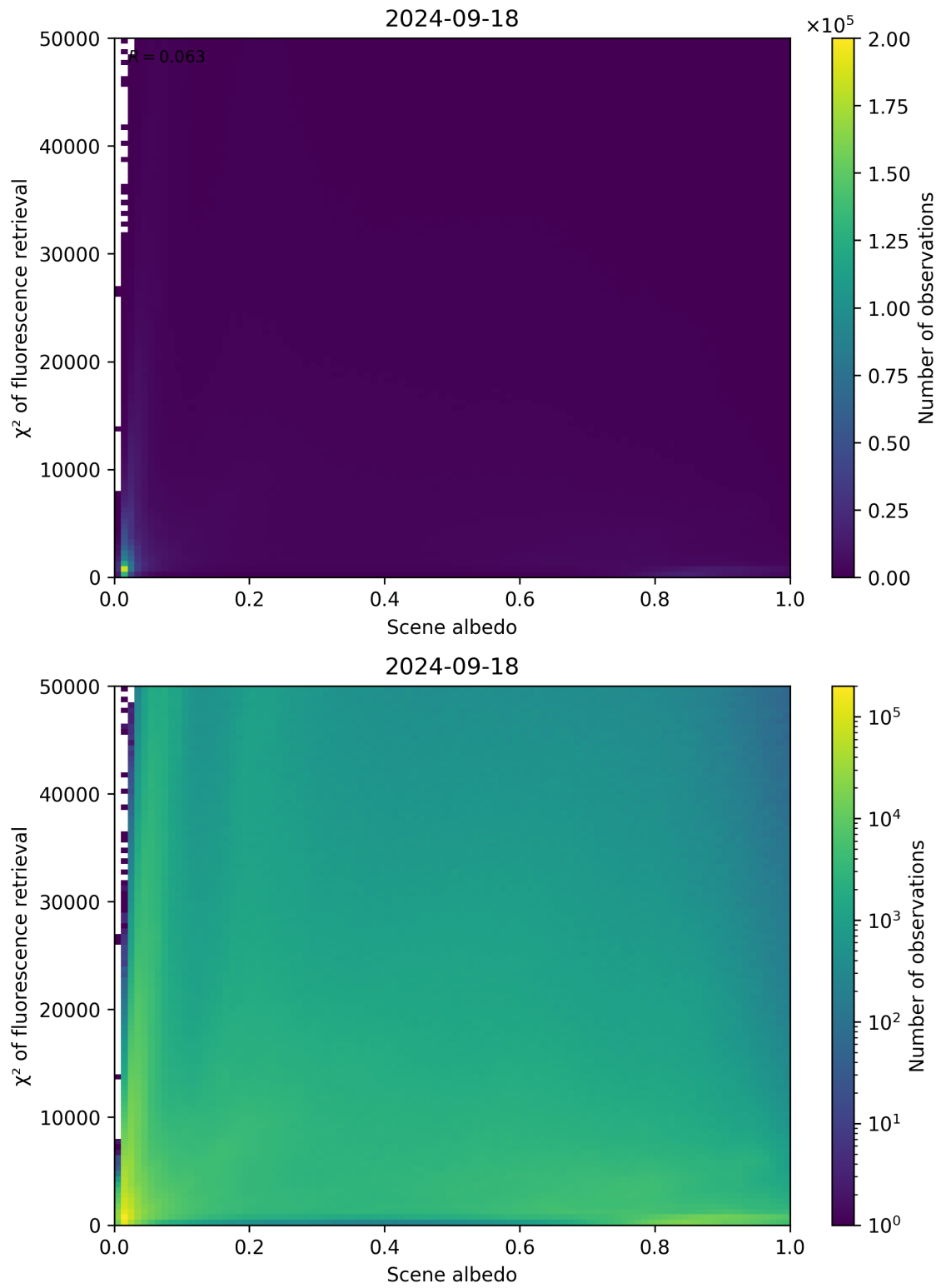
Figure 113: Scatter density plot of “Scene albedo” against “ \chi^2 of fluorescence retrieval” for 2024-09-17 to 2024-09-19.
