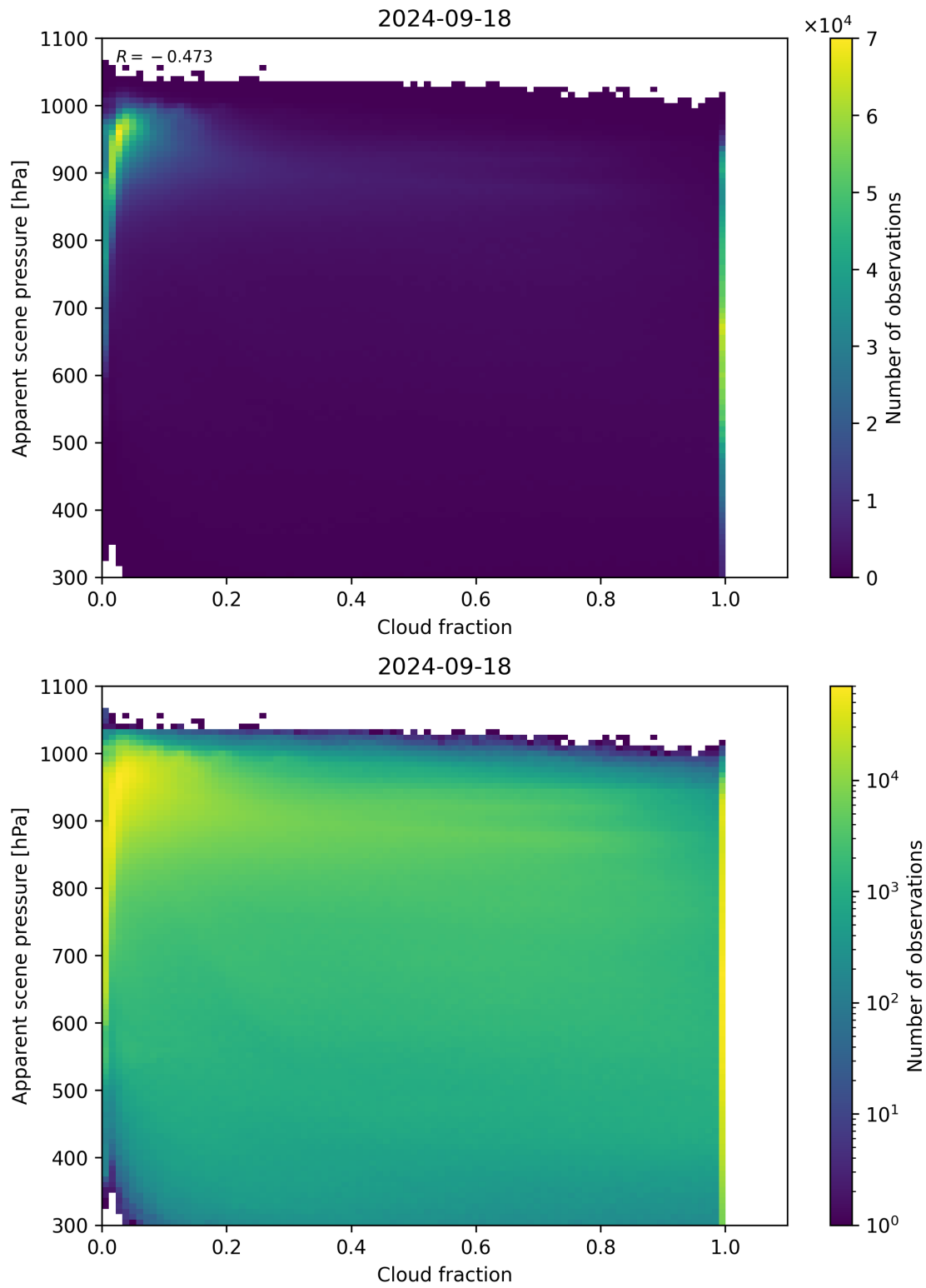
Figure 76: Scatter density plot of “Cloud fraction” against “Apparent scene pressure” for 2024-09-17 to 2024-09-19.
