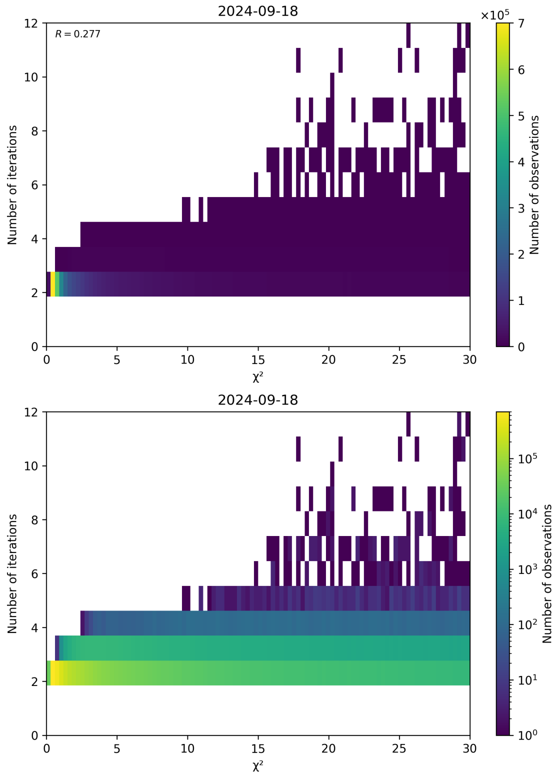
Figure 73: Scatter density plot of “ \chi^2 ” against “Number of iterations” for 2024-09-17 to 2024-09-19.
