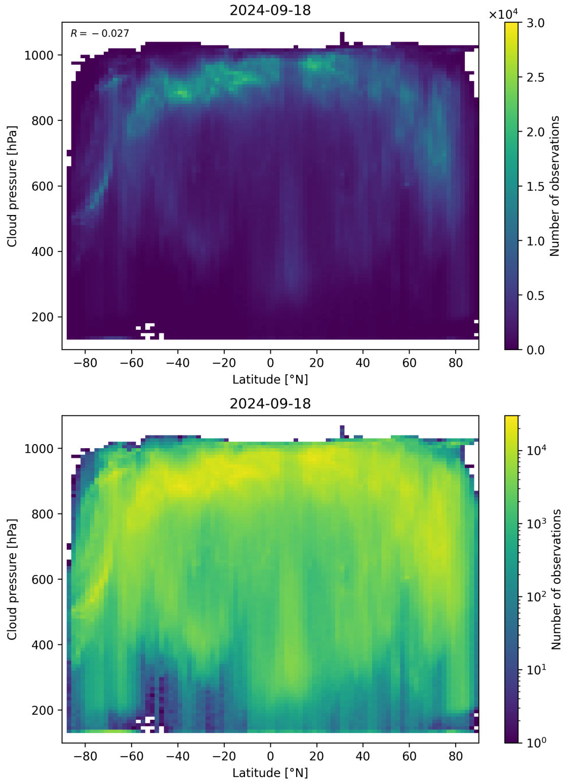
Figure 100: Scatter density plot of “Latitude” against “Cloud pressure” for 2024-09-17 to 2024-09-19.
