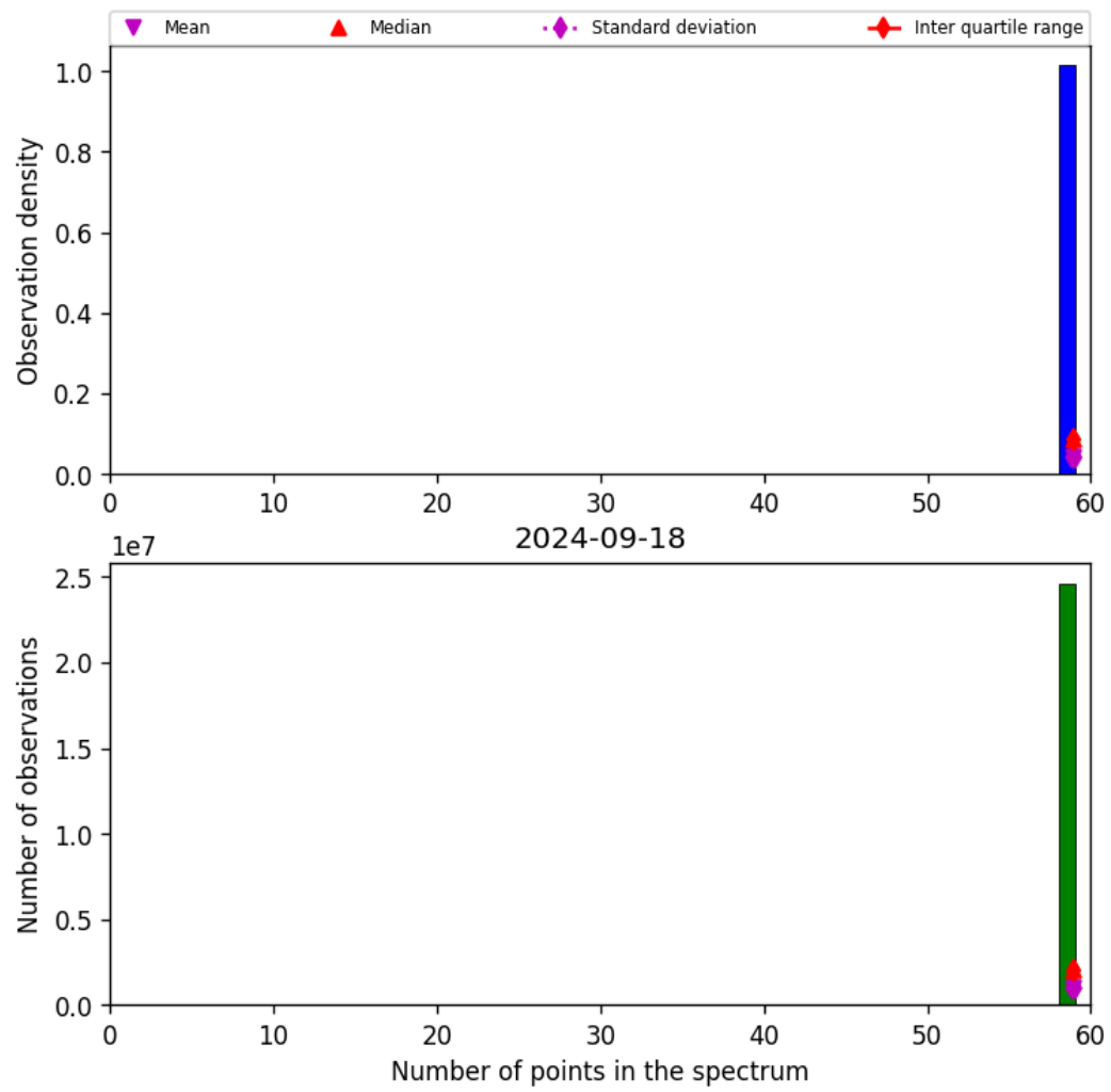
Figure 44: Histogram of “Number of points in the spectrum” for 2024-09-17 to 2024-09-19
