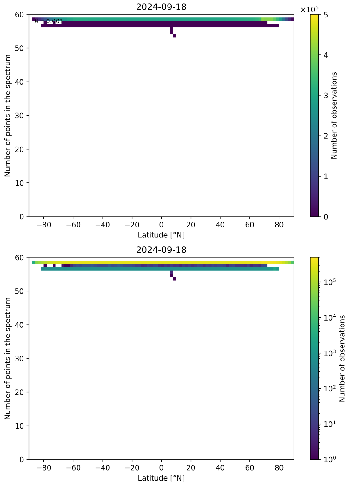
Figure 103: Scatter density plot of “Latitude” against “Number of points in the spectrum” for 2024-09-17 to 2024-09-19.
