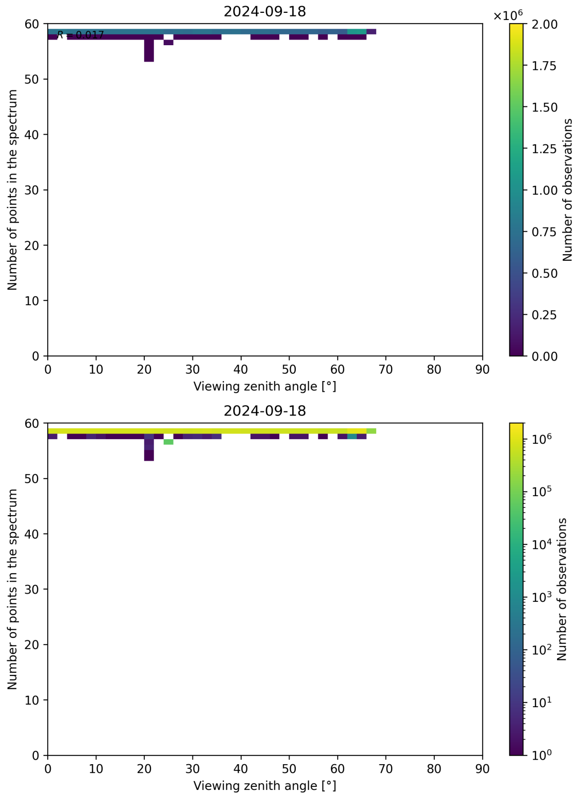
Figure 137: Scatter density plot of “Viewing zenith angle” against “Number of points in the spectrum” for 2024-09-17 to 2024-09-19.
