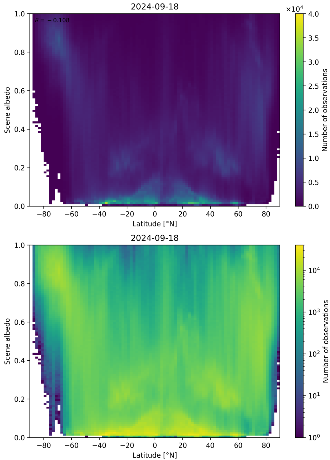
Figure 104: Scatter density plot of “Latitude” against “Scene albedo” for 2024-09-17 to 2024-09-19.
