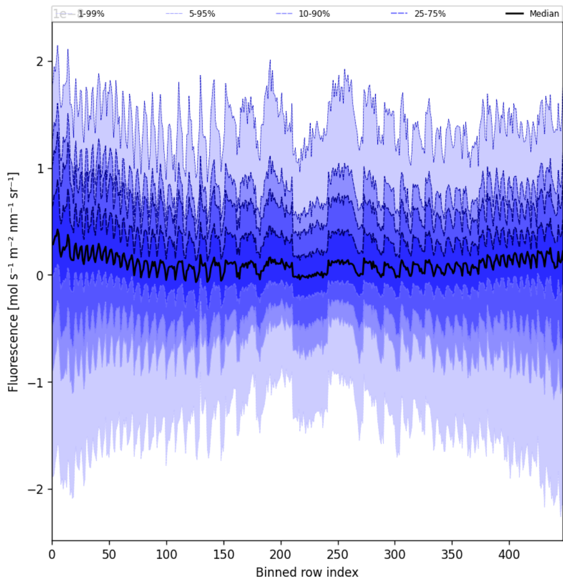
Figure 57: Along track statistics of “Fluorescence” for 2024-09-17 to 2024-09-19
