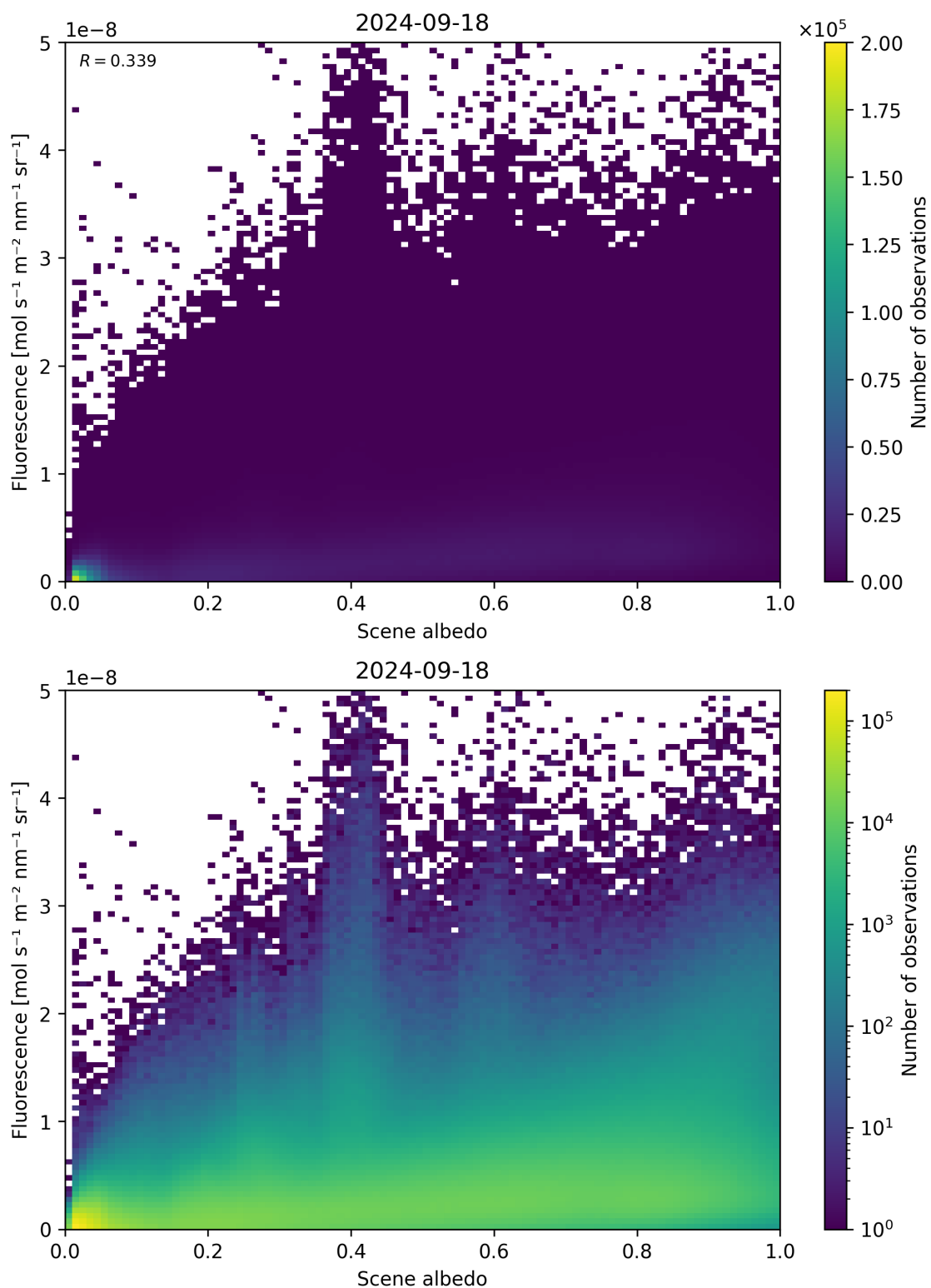
Figure 114: Scatter density plot of “Scene albedo” against “Fluorescence” for 2024-09-17 to 2024-09-19.
