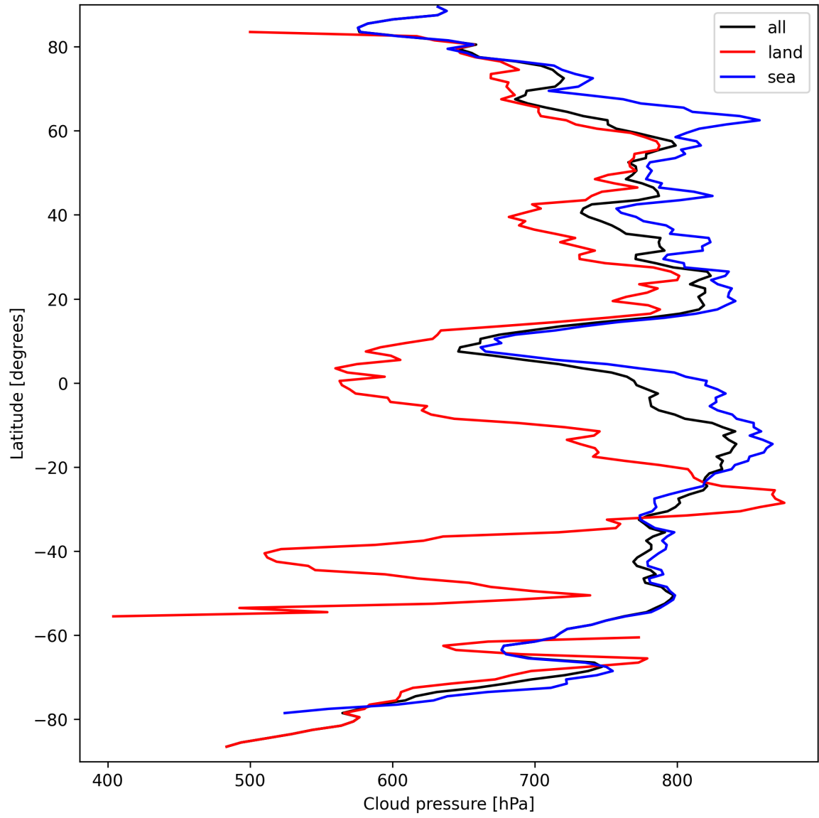
Figure 13: Zonal average of “Cloud pressure” for 2024-09-17 to 2024-09-19.
