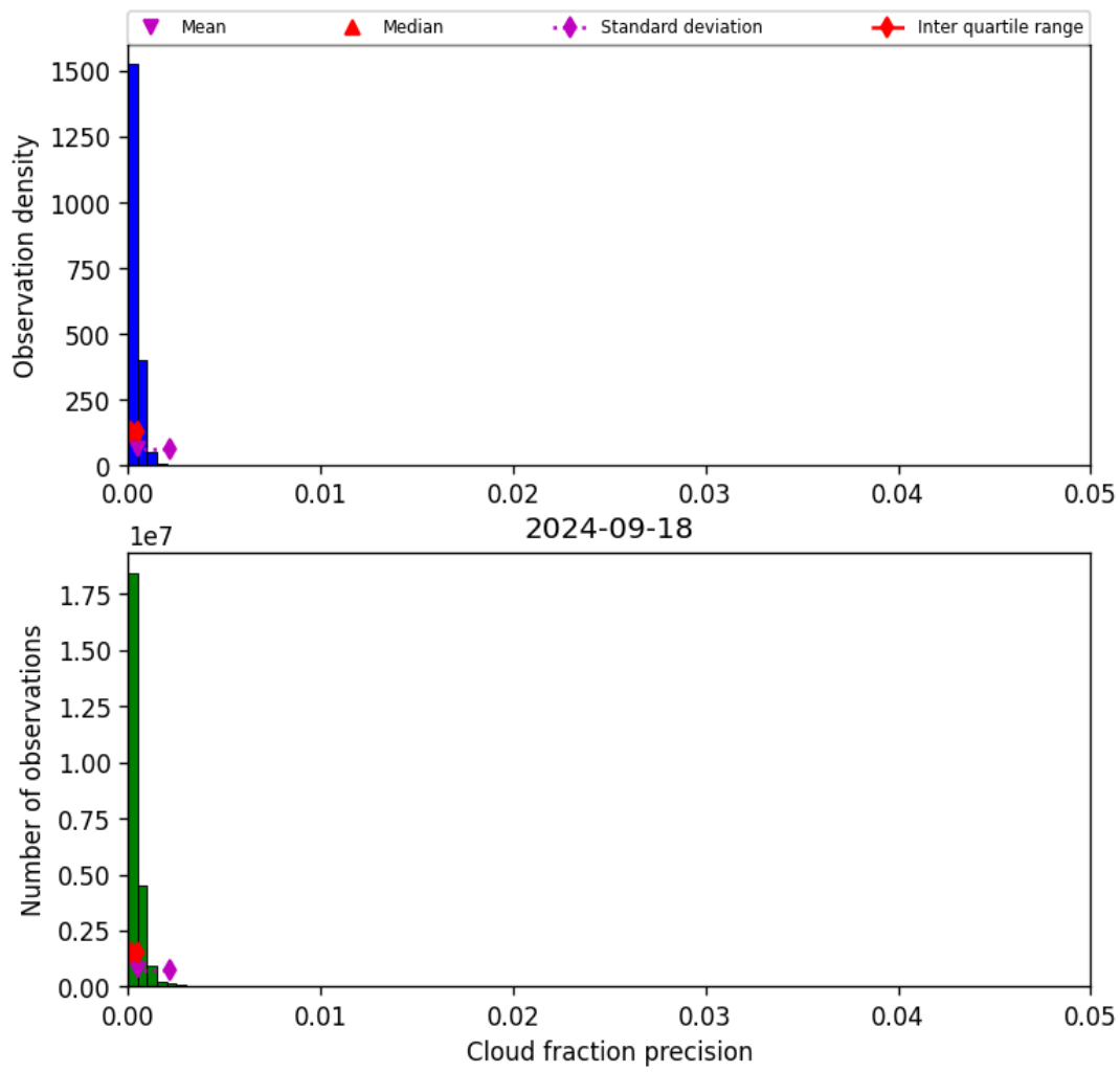
Figure 33: Histogram of “Cloud fraction precision” for 2024-09-17 to 2024-09-19
