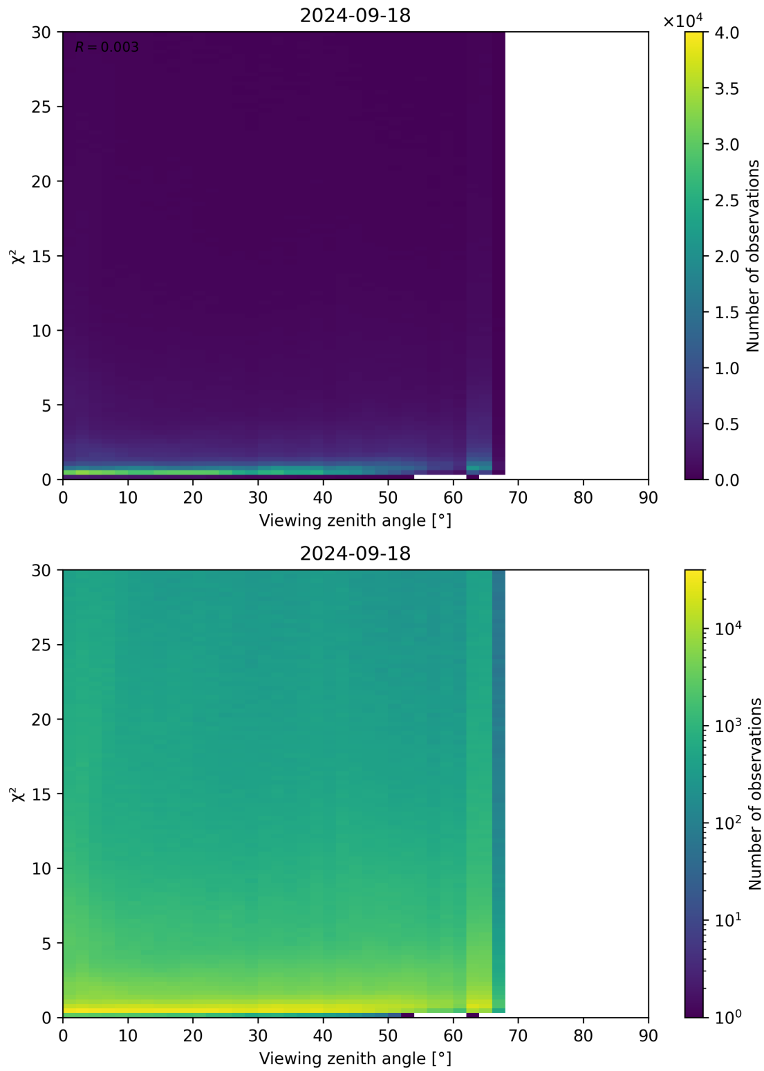
Figure 130: Scatter density plot of “Viewing zenith angle” against “ \chi^2 ” for 2024-09-17 to 2024-09-19.
