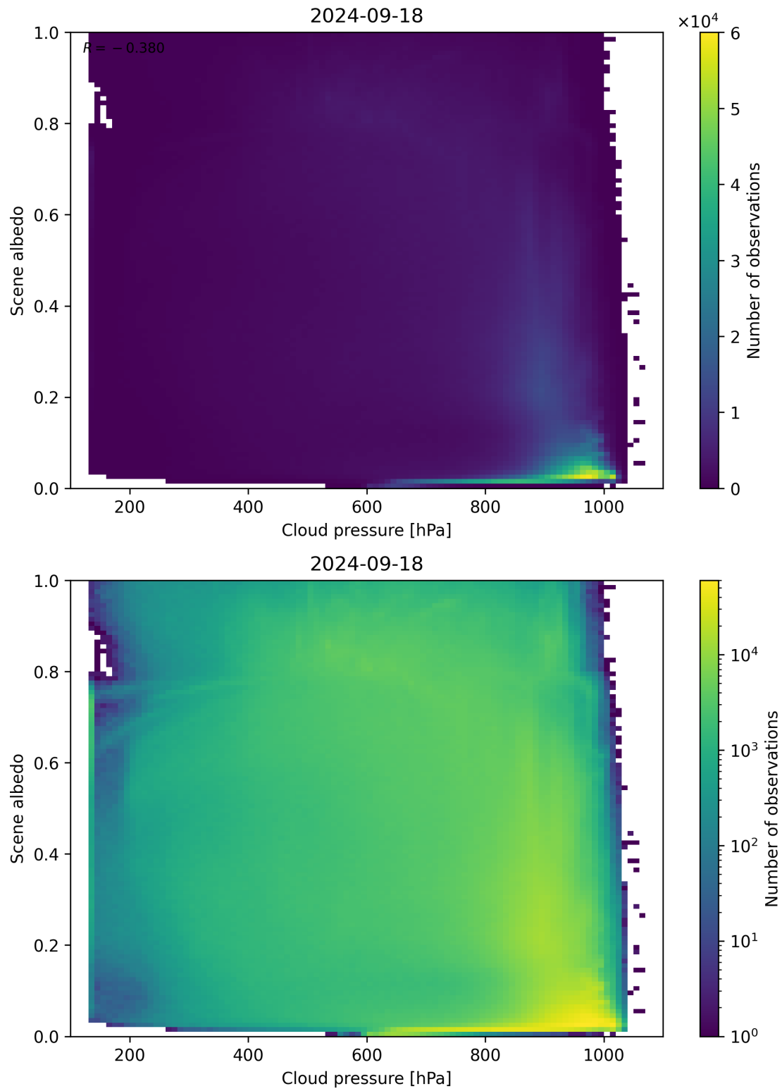
Figure 91: Scatter density plot of “Cloud pressure” against “Scene albedo” for 2024-09-17 to 2024-09-19.
