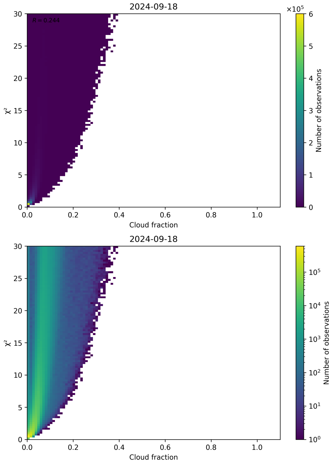
Figure 77: Scatter density plot of “Cloud fraction” against “ \chi^2 ” for 2024-09-17 to 2024-09-19.
