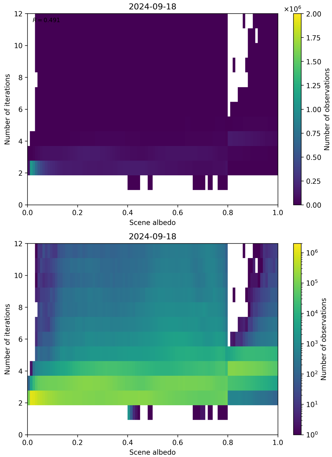
Figure 115: Scatter density plot of “Scene albedo” against “Number of iterations” for 2024-09-17 to 2024-09-19.
