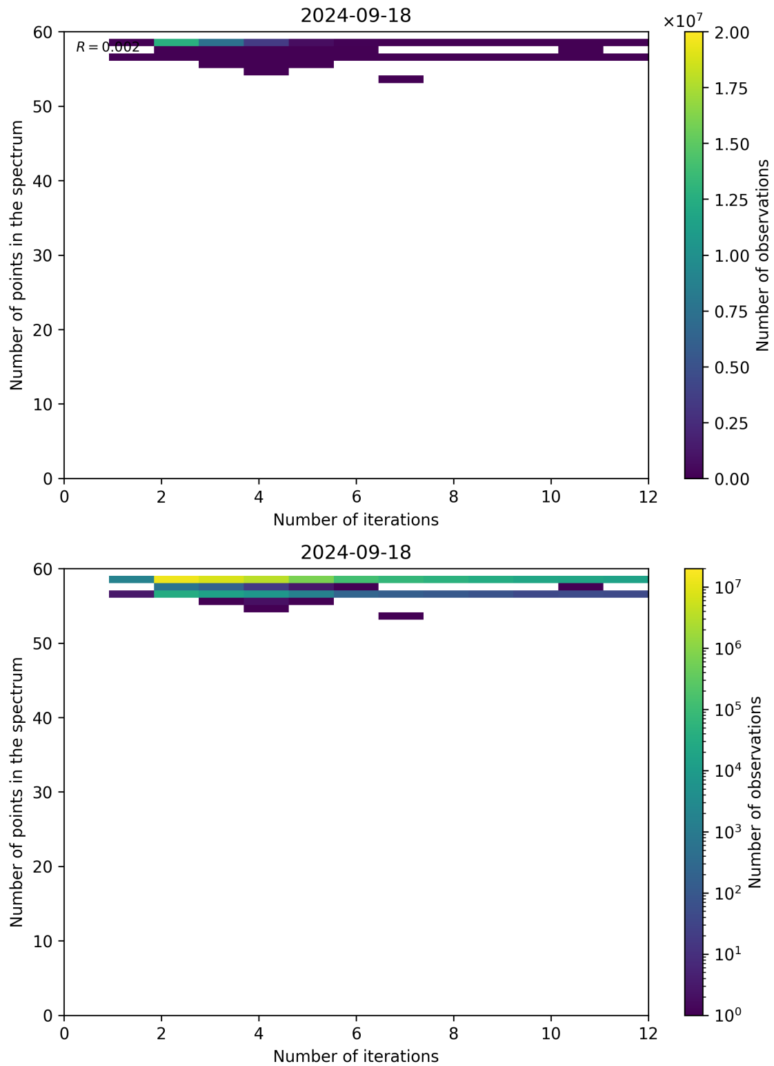
Figure 108: Scatter density plot of “Number of iterations” against “Number of points in the spectrum” for 2024-09-17 to 2024-09-19.
