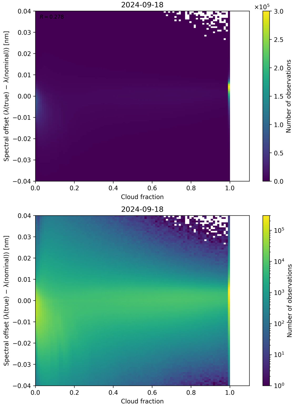
Figure 83: Scatter density plot of “Cloud fraction” against “Spectral offset ( \lambda_{\text{true}} - \lambda_{\text{nominal}} )” for 2024-09-17 to 2024-09-19.
