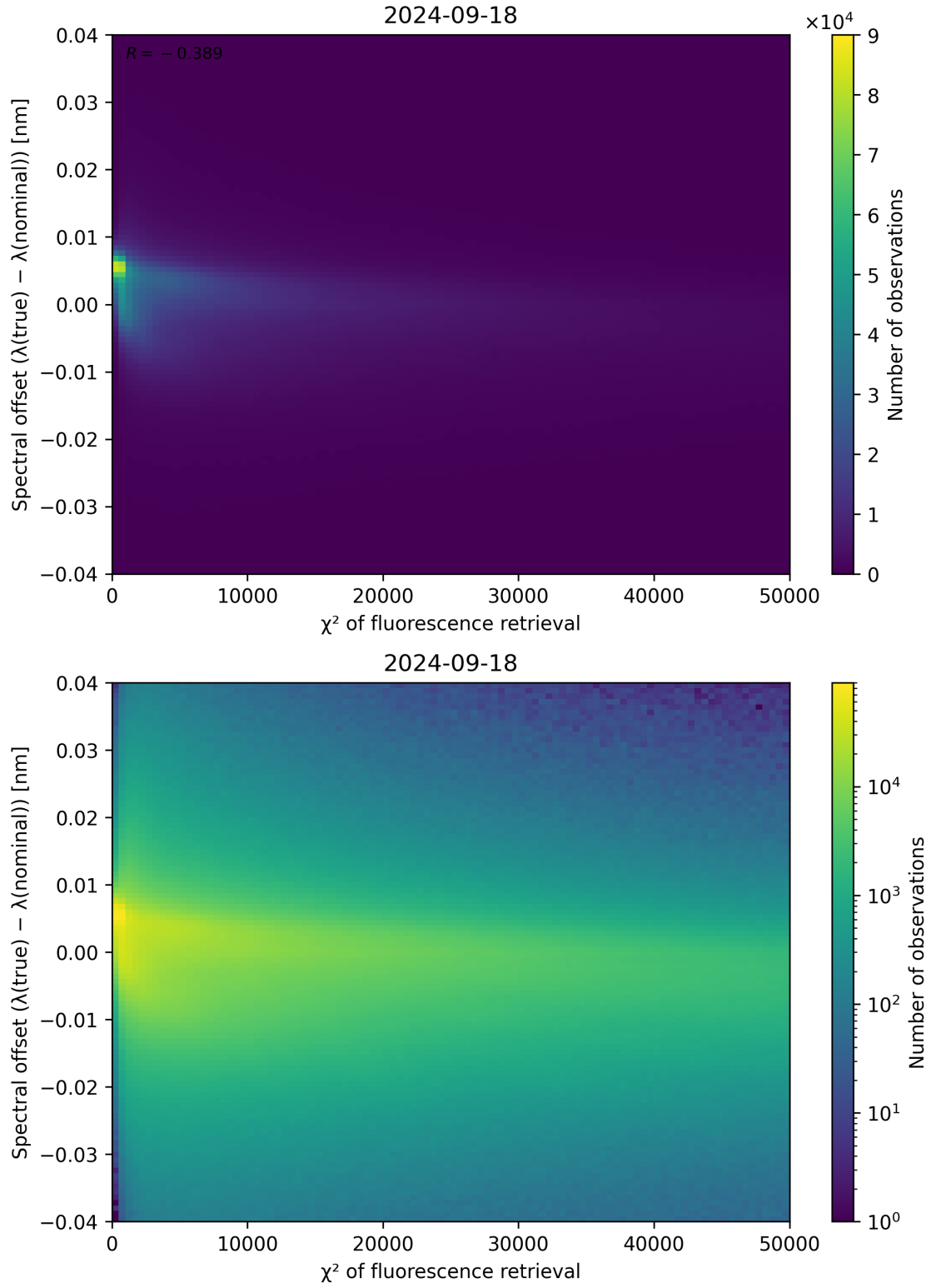
Figure 72: Scatter density plot of “ \chi^2 of fluorescence retrieval” against “Spectral offset ( \lambda_{\text{true}} - \lambda_{\text{nominal}} )” for 2024-09-17 to 2024-09-19.
