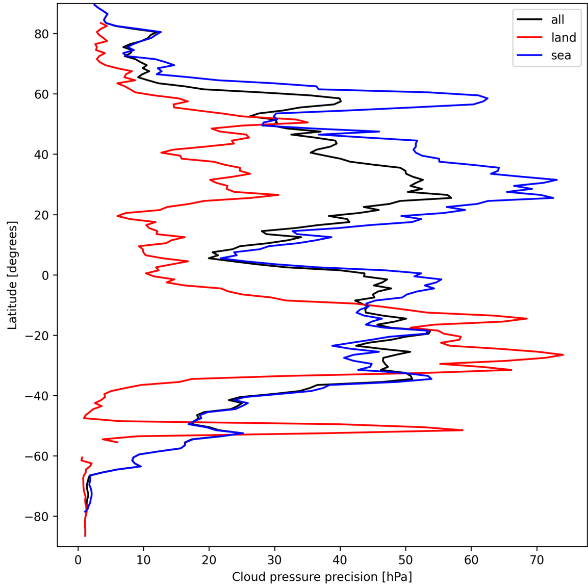
Figure 14: Zonal average of “Cloud pressure precision” for 2024-09-17 to 2024-09-19.
