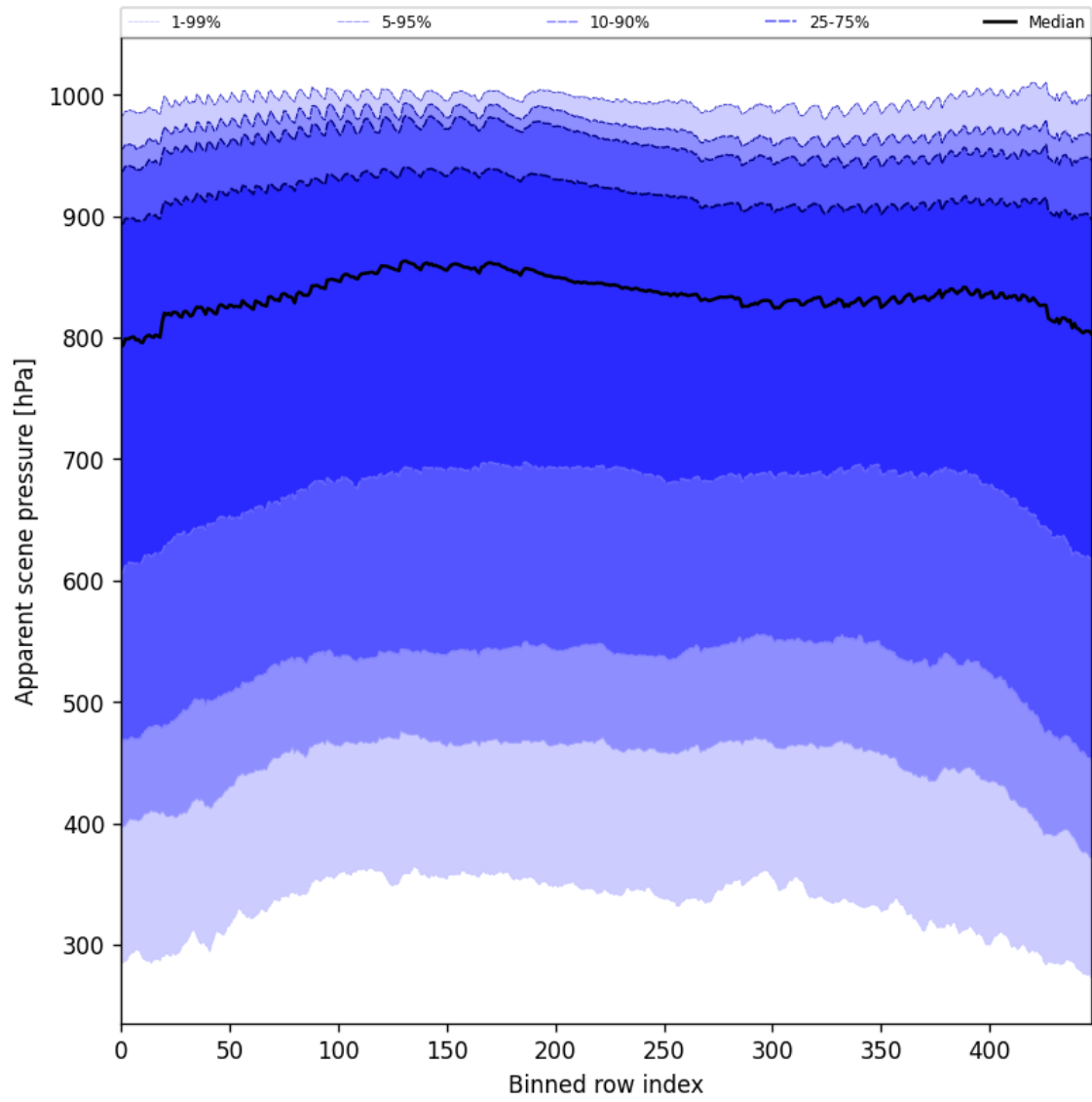
Figure 53: Along track statistics of “Apparent scene pressure” for 2024-09-17 to 2024-09-19
