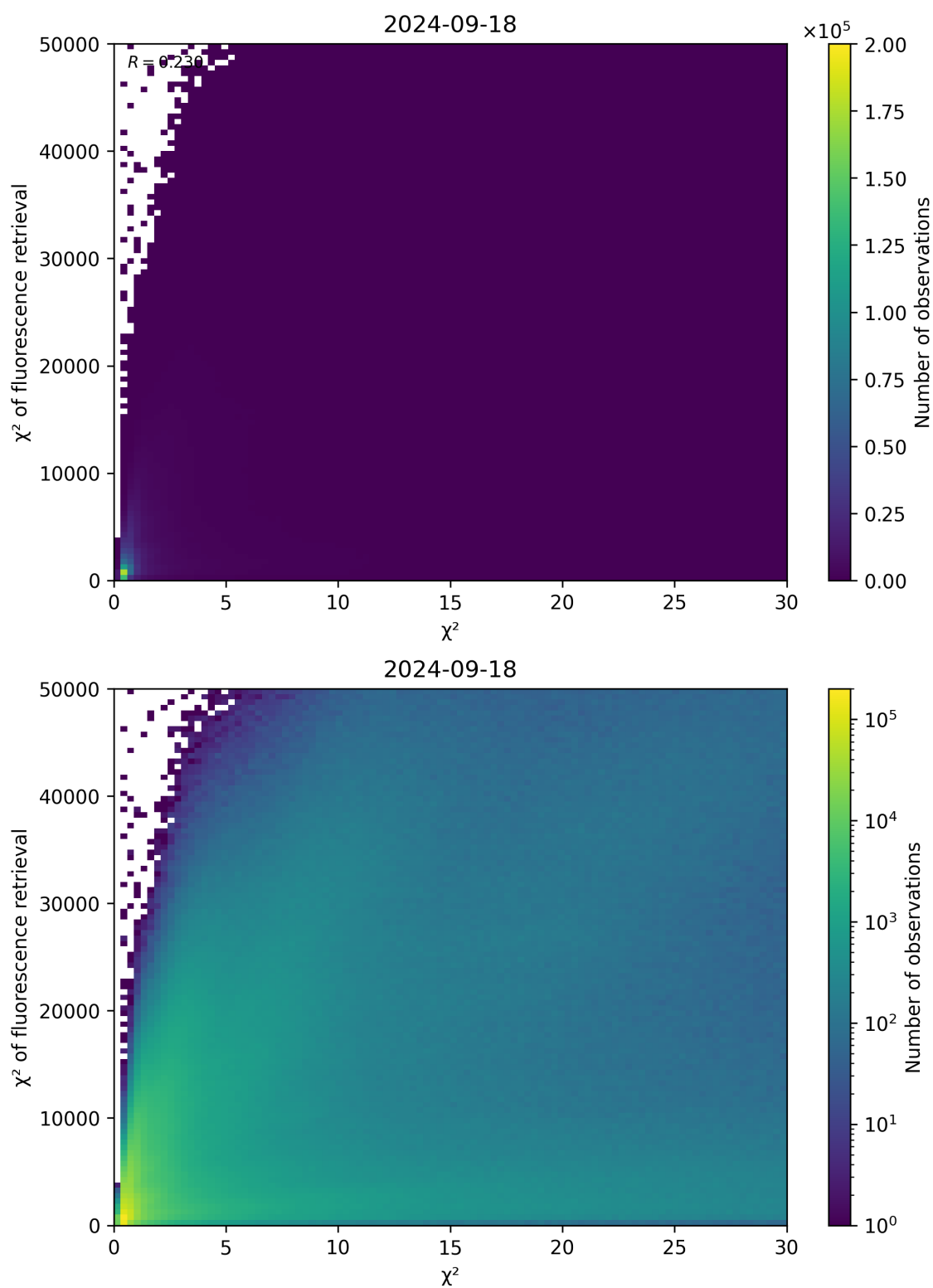
Figure 69: Scatter density plot of “ \chi^2 ” against “ \chi^2 of fluorescence retrieval” for 2024-09-17 to 2024-09-19.
