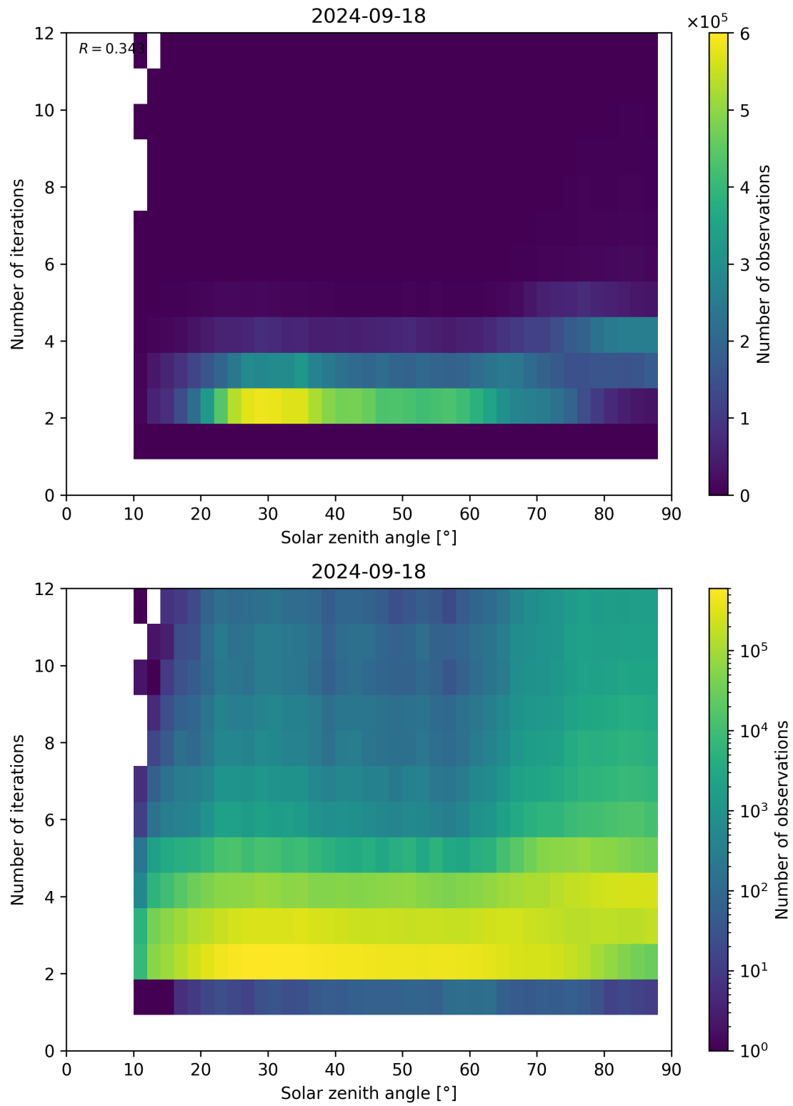
Figure 125: Scatter density plot of “Solar zenith angle” against “Number of iterations” for 2024-09-17 to 2024-09-19.
