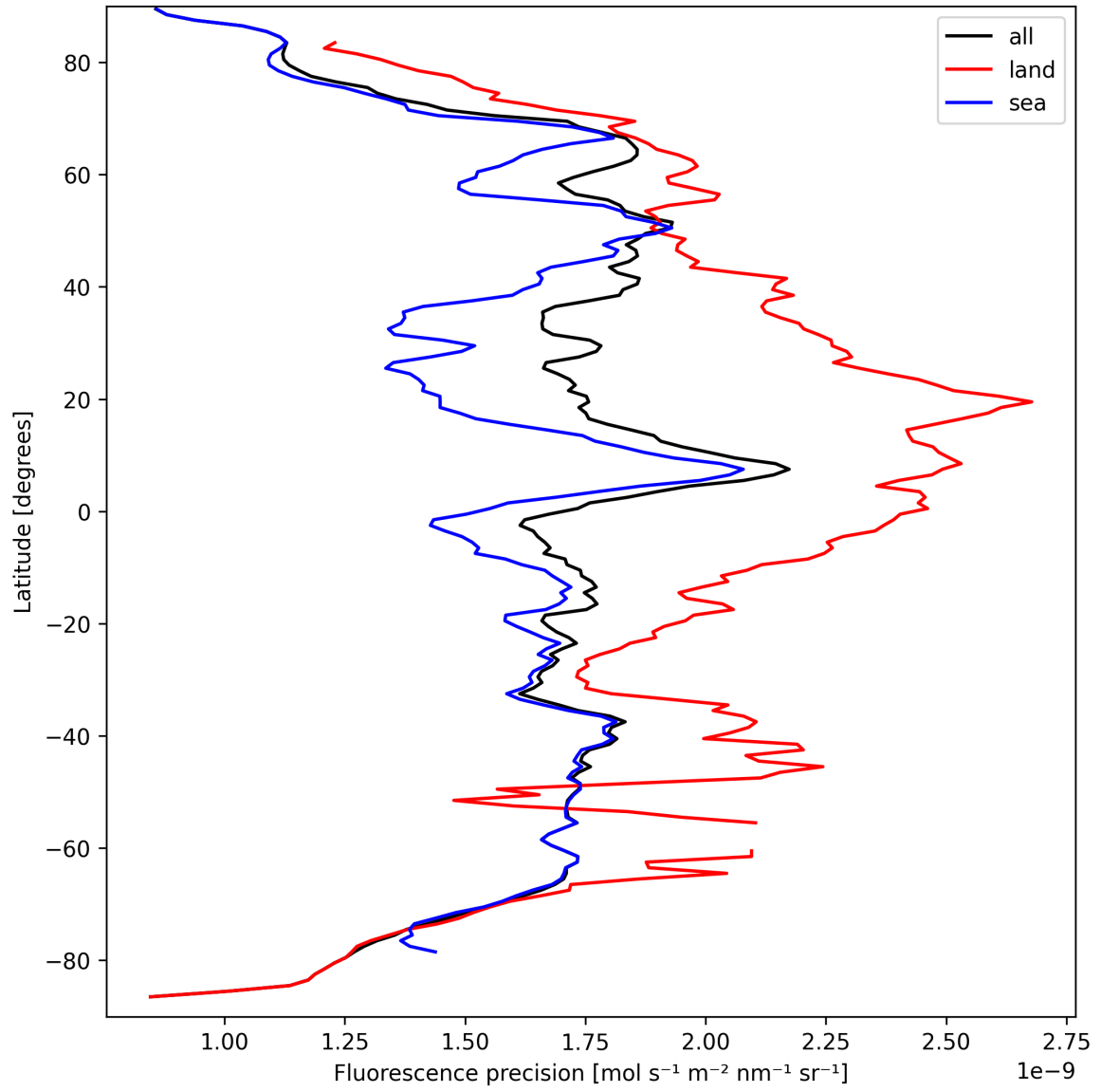
Figure 24: Zonal average of “Fluorescence precision” for 2024-09-17 to 2024-09-19.
