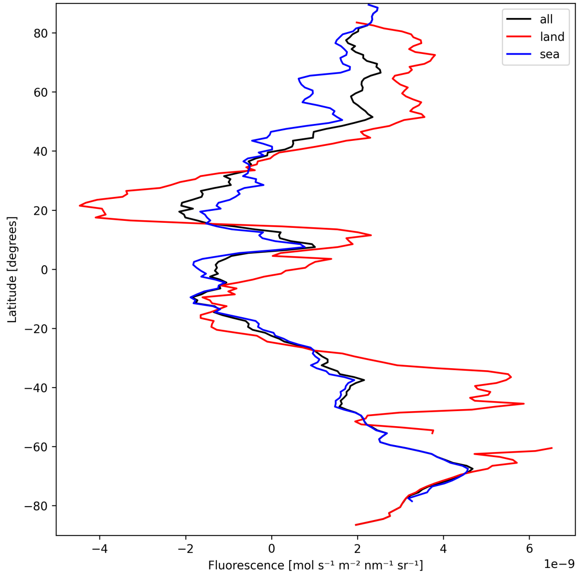
Figure 23: Zonal average of “Fluorescence” for 2024-09-17 to 2024-09-19.
