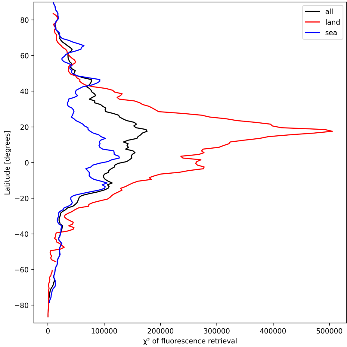
Figure 25: Zonal average of “ \chi^2 of fluorescence retrieval” for 2024-09-17 to 2024-09-19.
