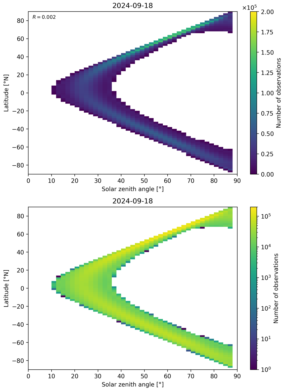
Figure 124: Scatter density plot of “Solar zenith angle” against “Latitude” for 2024-09-17 to 2024-09-19.
