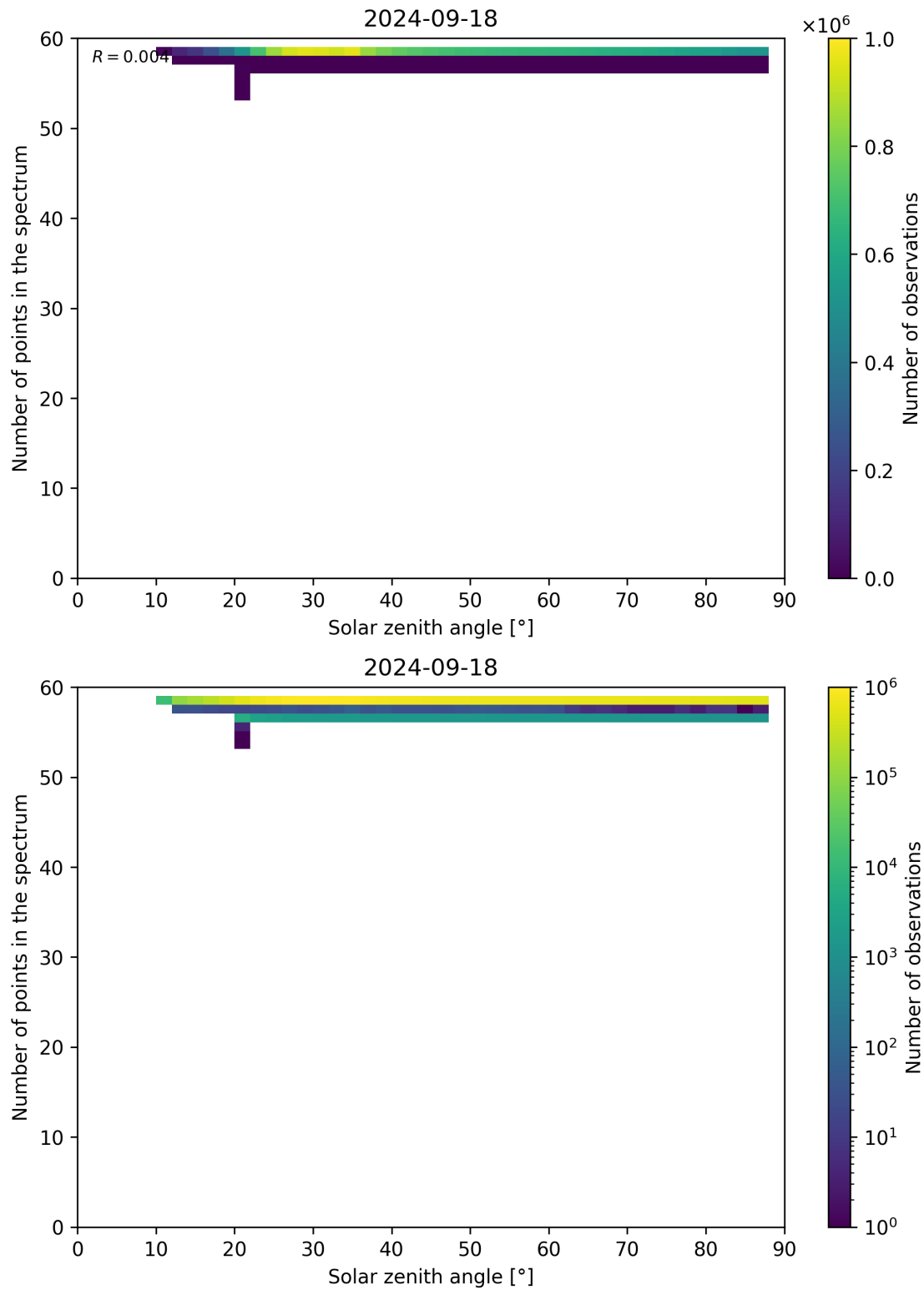
Figure 126: Scatter density plot of “Solar zenith angle” against “Number of points in the spectrum” for 2024-09-17 to 2024-09-19.
