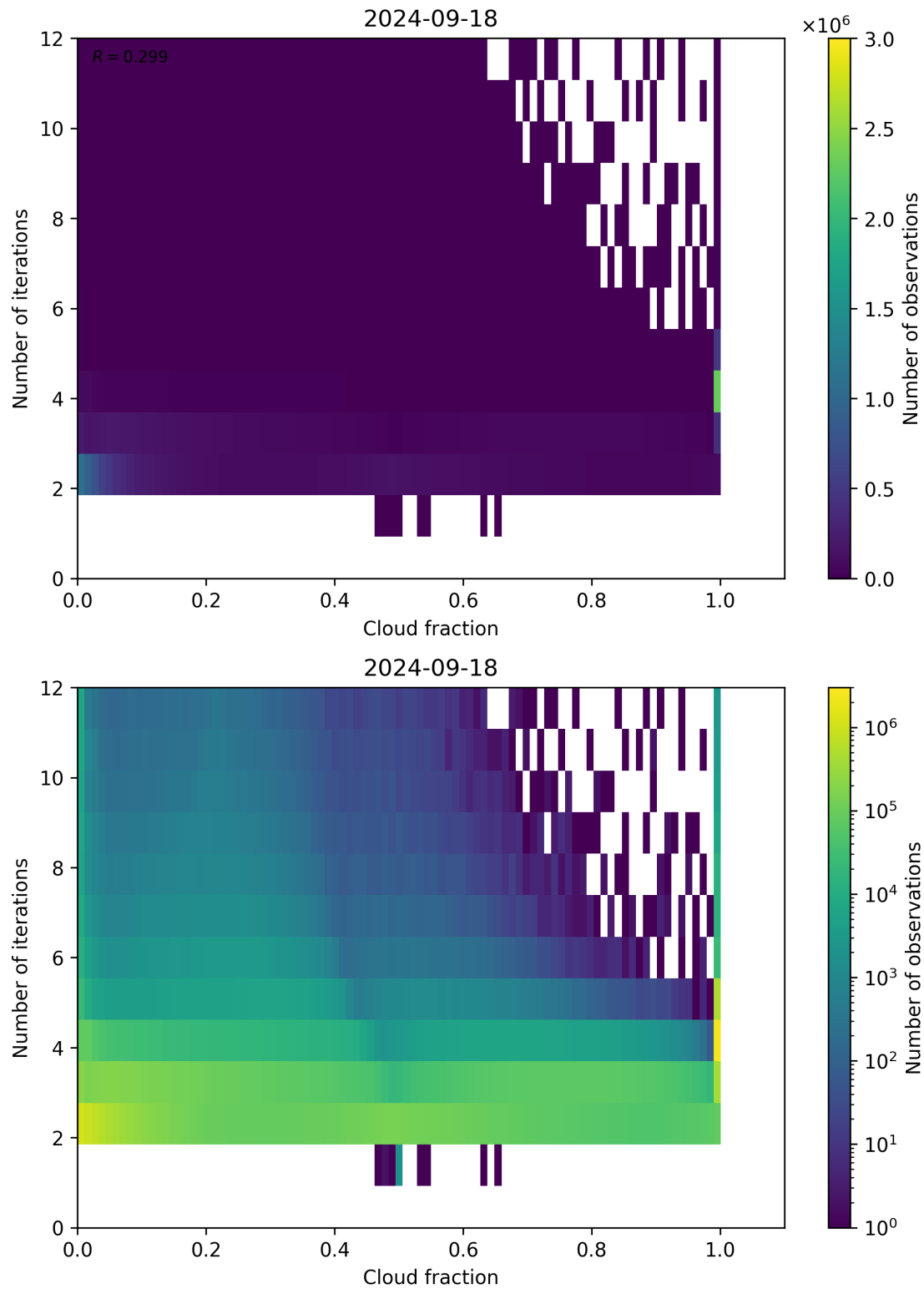
Figure 80: Scatter density plot of “Cloud fraction” against “Number of iterations” for 2024-09-17 to 2024-09-19.
