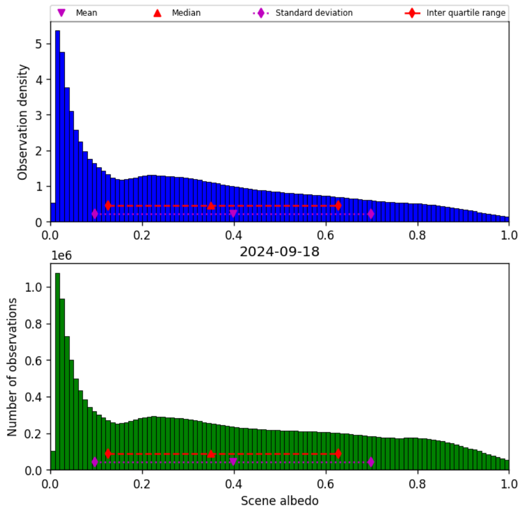
Figure 34: Histogram of “Scene albedo” for 2024-09-17 to 2024-09-19
