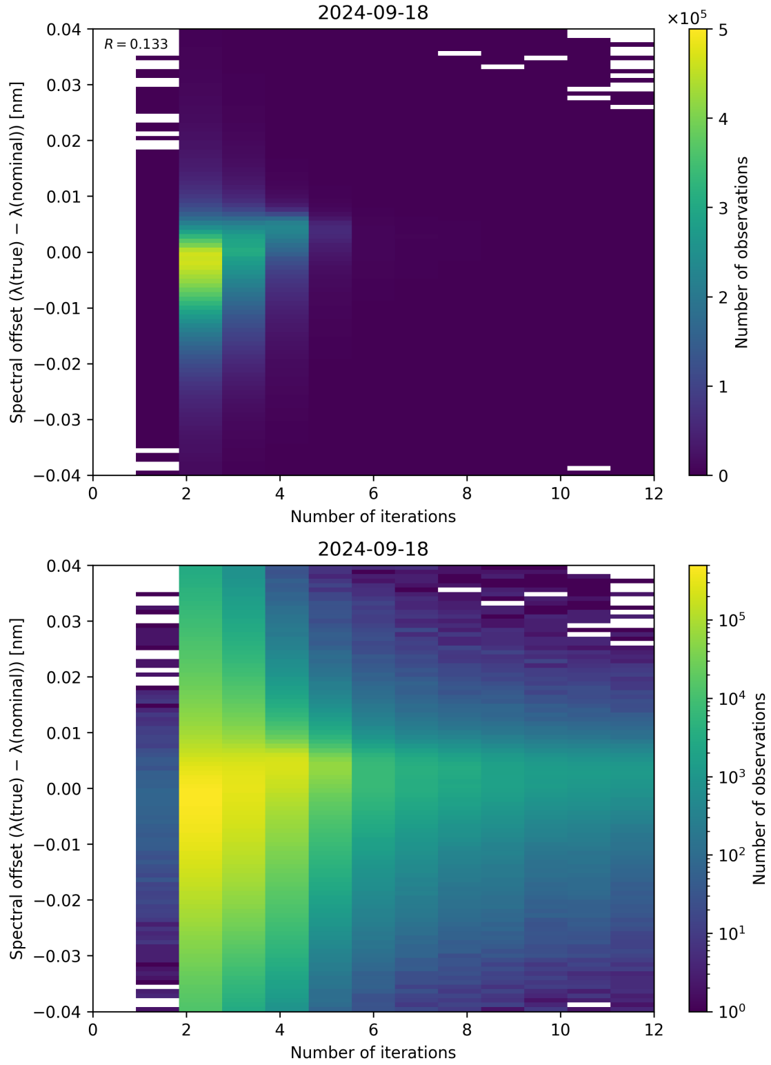
Figure 109: Scatter density plot of “Number of iterations” against “Spectral offset ( \lambda_{\text{true}} - \lambda_{\text{nominal}} )” for 2024-09-17 to 2024-09-19.
