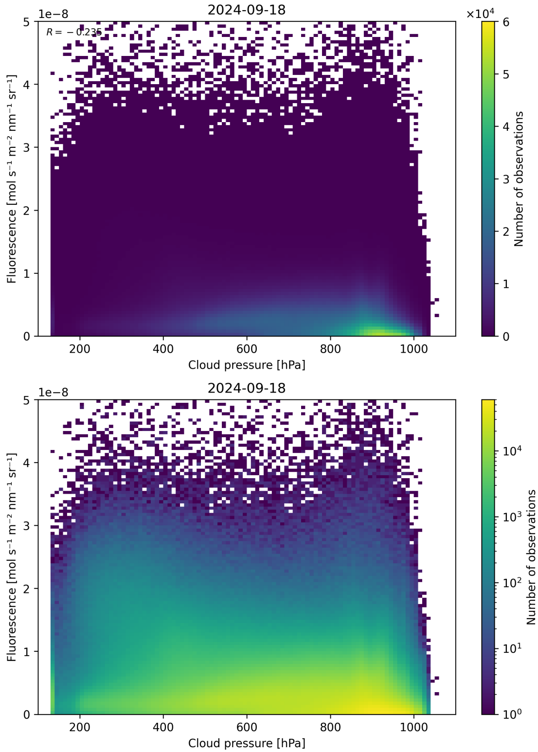
Figure 88: Scatter density plot of “Cloud pressure” against “Fluorescence” for 2024-09-17 to 2024-09-19.
