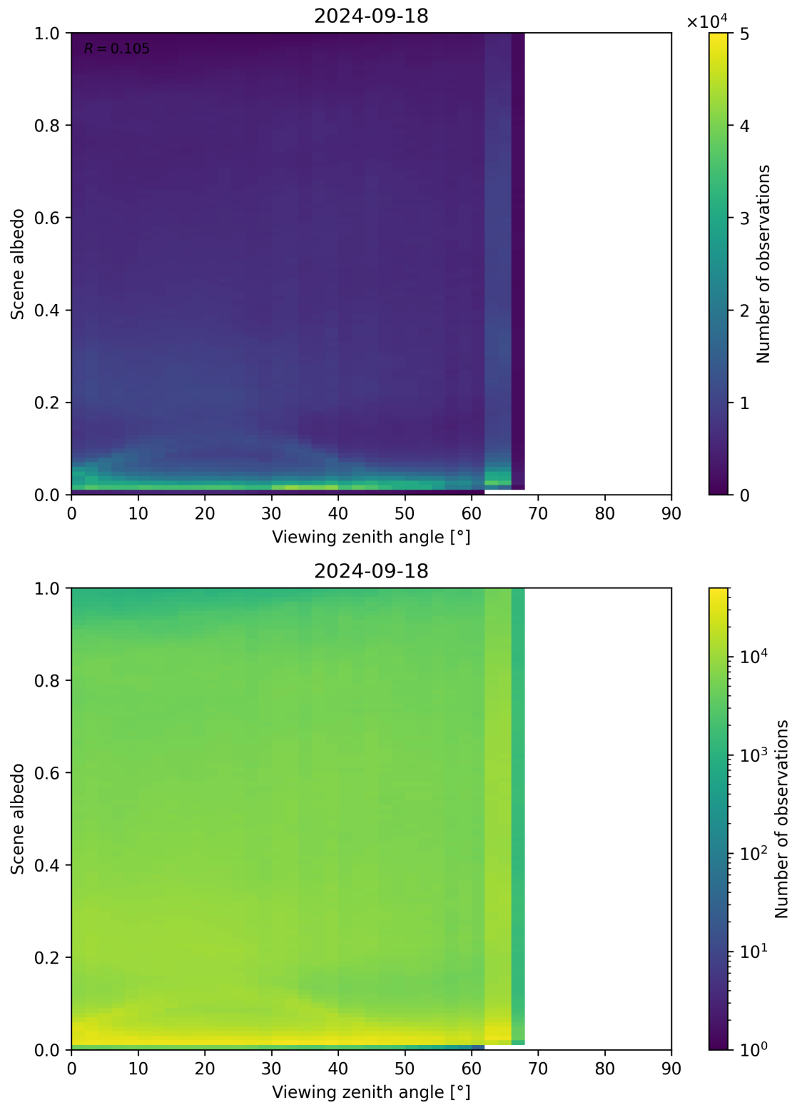
Figure 138: Scatter density plot of “Viewing zenith angle” against “Scene albedo” for 2024-09-17 to 2024-09-19.
