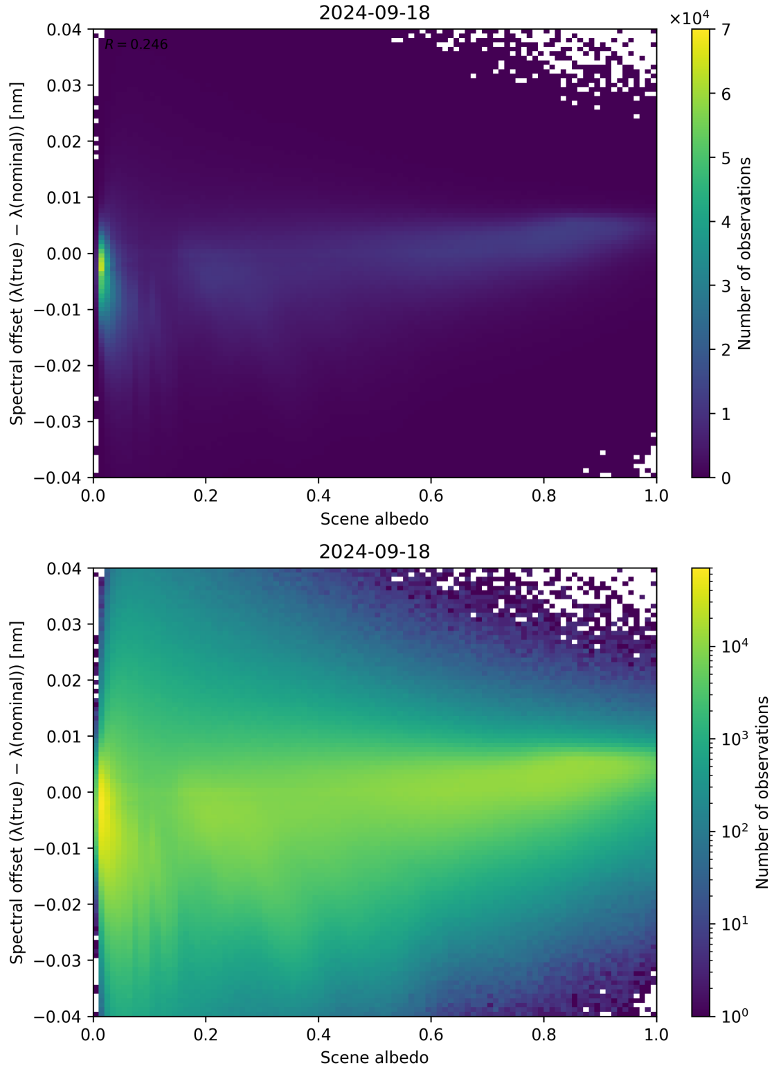
Figure 117: Scatter density plot of “Scene albedo” against “Spectral offset ( \lambda_{\text{true}} - \lambda_{\text{nominal}} )” for 2024-09-17 to 2024-09-19.
