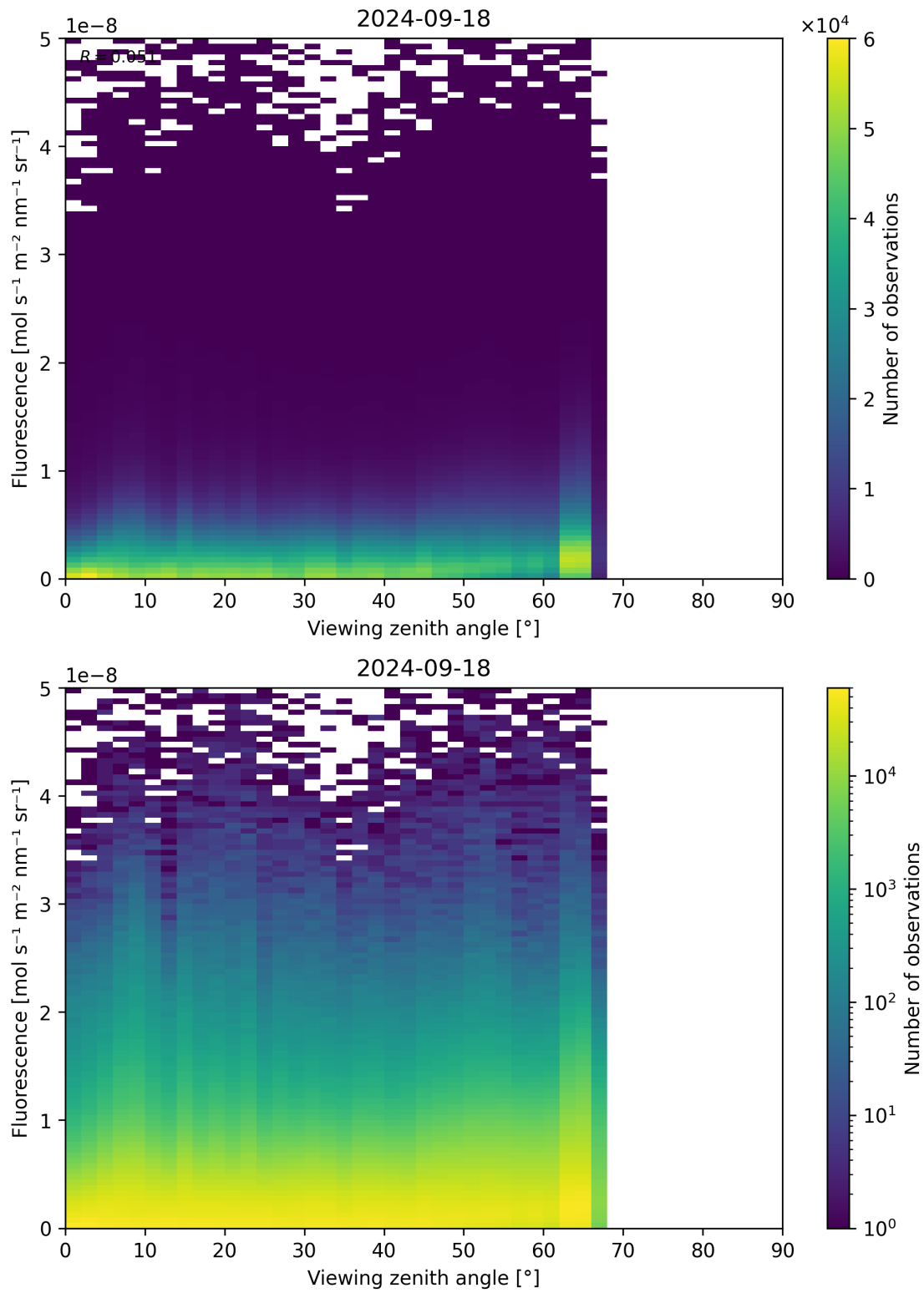
Figure 134: Scatter density plot of “Viewing zenith angle” against “Fluorescence” for 2024-09-17 to 2024-09-19.
