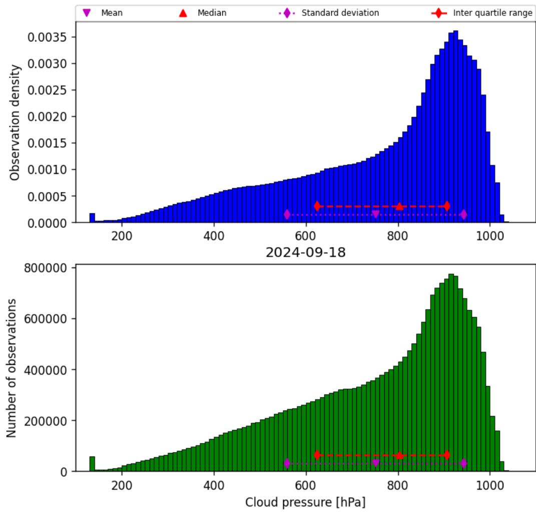
Figure 30: Histogram of “Cloud pressure” for 2024-09-17 to 2024-09-19
