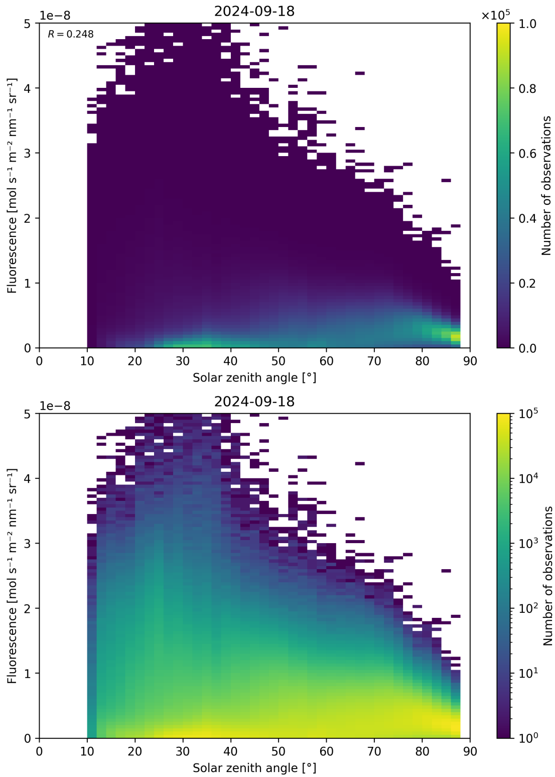
Figure 123: Scatter density plot of “Solar zenith angle” against “Fluorescence” for 2024-09-17 to 2024-09-19.
