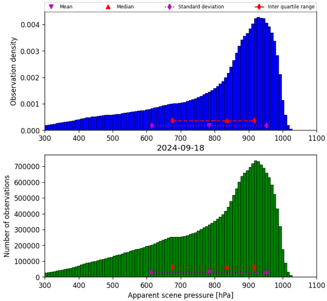
Figure 36: Histogram of “Apparent scene pressure” for 2024-09-17 to 2024-09-19
