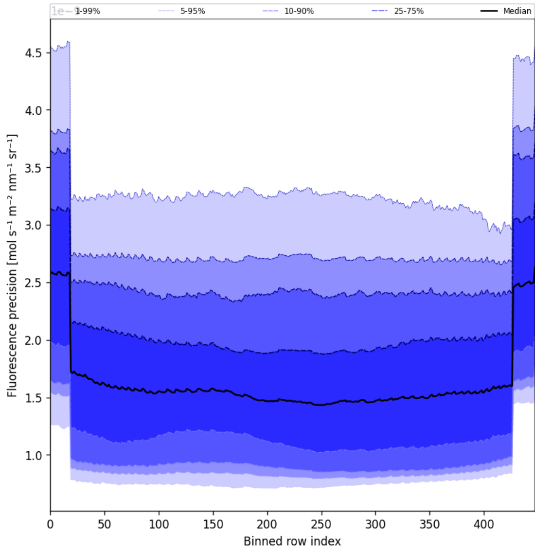
Figure 58: Along track statistics of “Fluorescence precision” for 2024-09-17 to 2024-09-19
