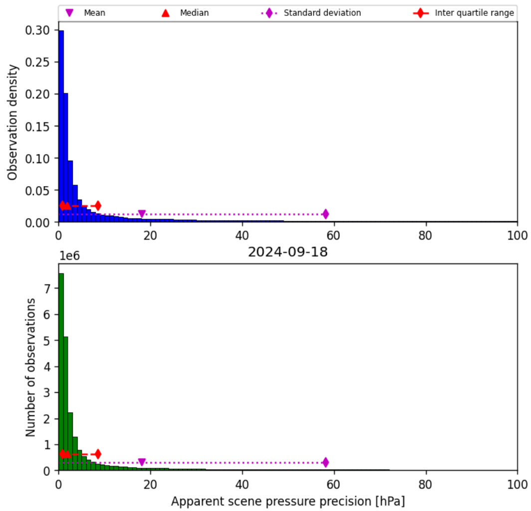
Figure 37: Histogram of “Apparent scene pressure precision” for 2024-09-17 to 2024-09-19
