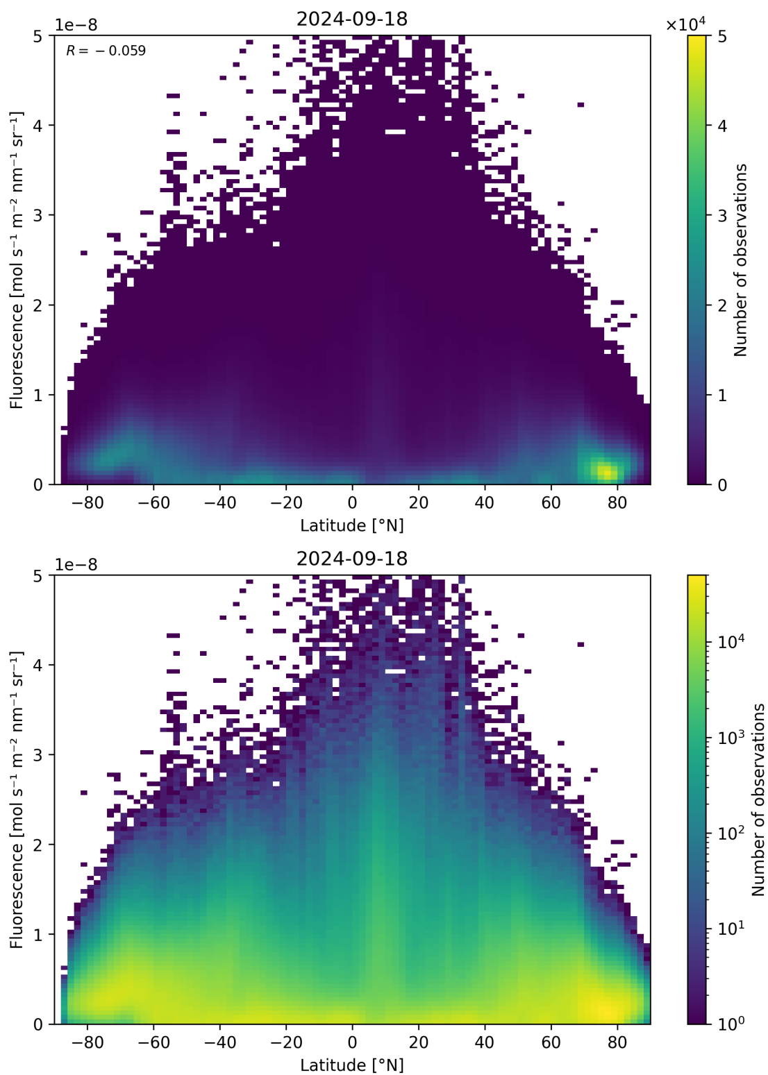
Figure 101: Scatter density plot of “Latitude” against “Fluorescence” for 2024-09-17 to 2024-09-19.
