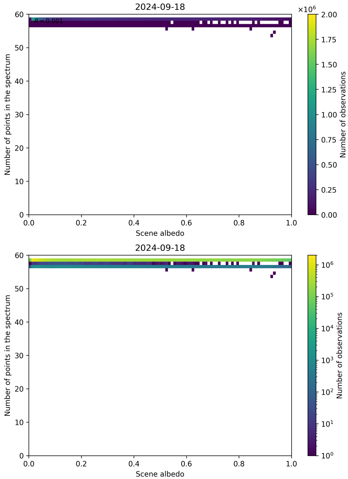
Figure 116: Scatter density plot of “Scene albedo” against “Number of points in the spectrum” for 2024-09-17 to 2024-09-19.
