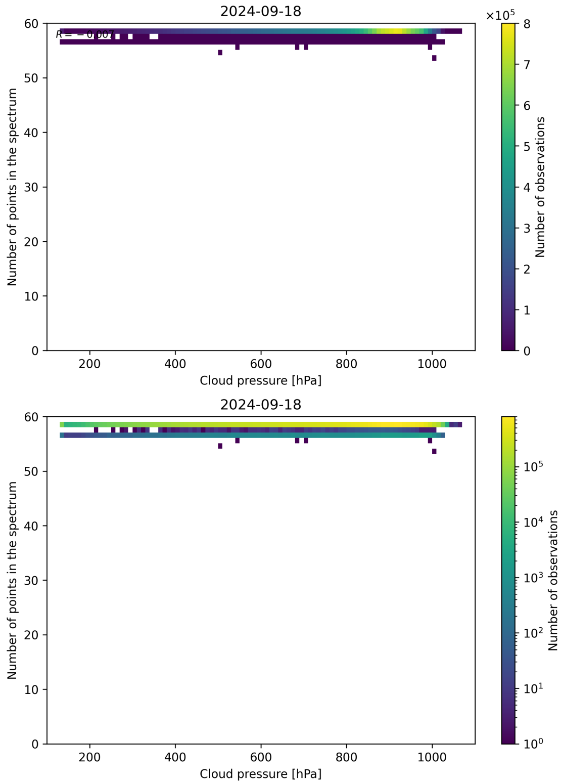
Figure 90: Scatter density plot of “Cloud pressure” against “Number of points in the spectrum” for 2024-09-17 to 2024-09-19.
