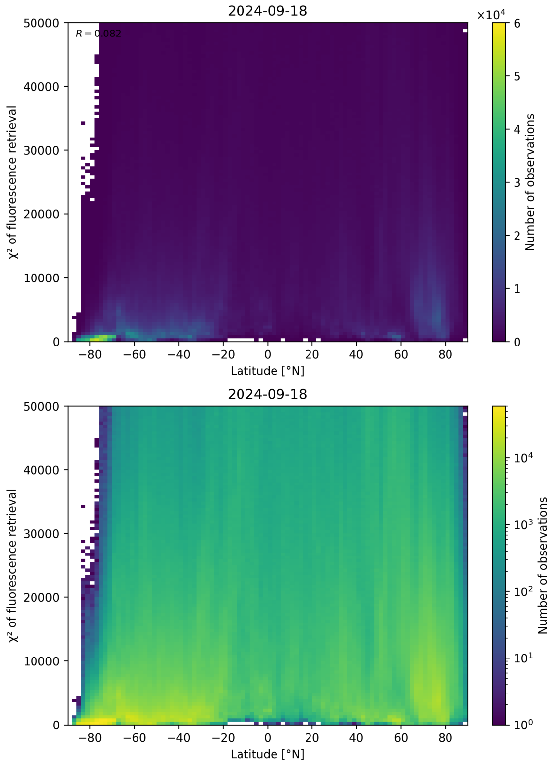
Figure 98: Scatter density plot of “Latitude” against “ \chi^2 of fluorescence retrieval” for 2024-09-17 to 2024-09-19.
