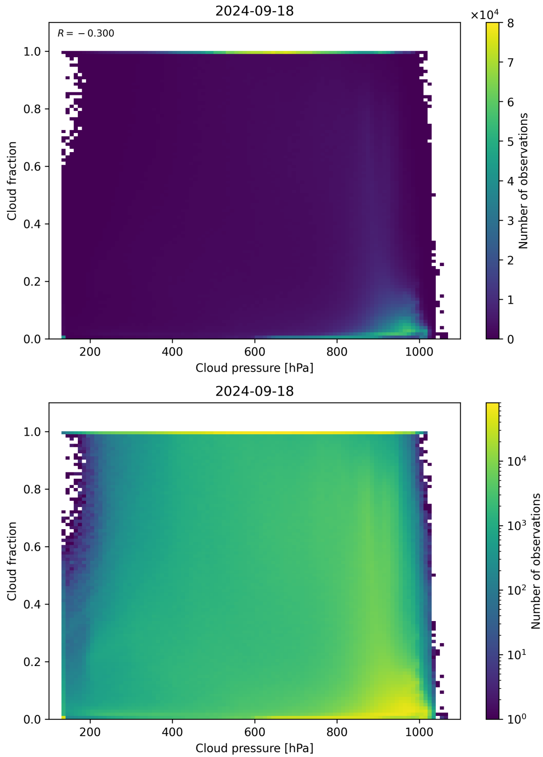
Figure 87: Scatter density plot of “Cloud pressure” against “Cloud fraction” for 2024-09-17 to 2024-09-19.
