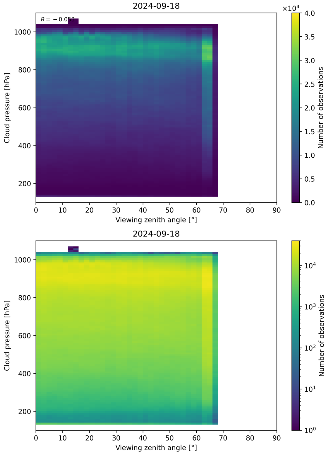
Figure 133: Scatter density plot of “Viewing zenith angle” against “Cloud pressure” for 2024-09-17 to 2024-09-19.
