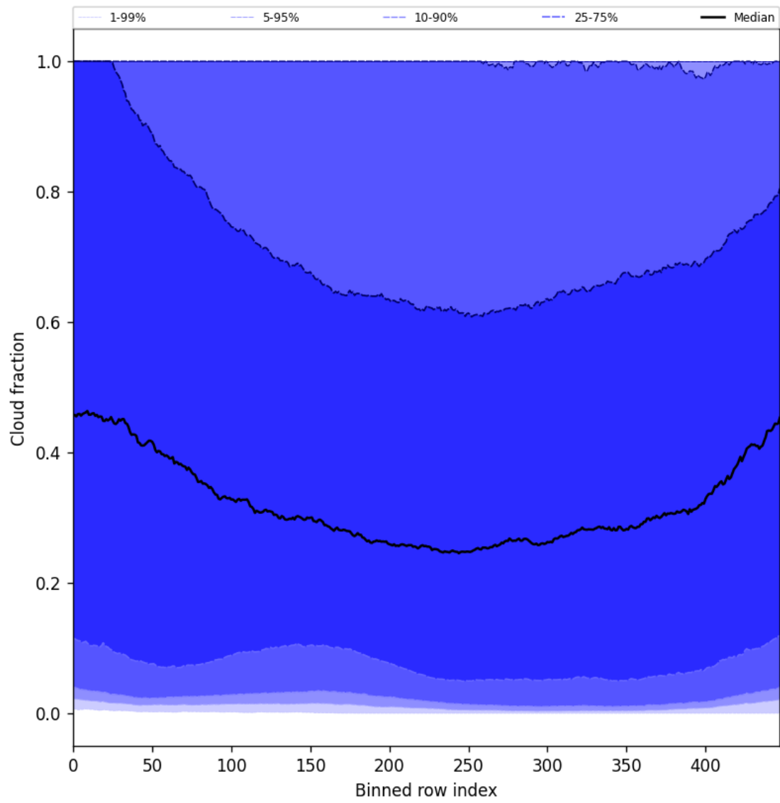
Figure 49: Along track statistics of “Cloud fraction” for 2024-09-17 to 2024-09-19
