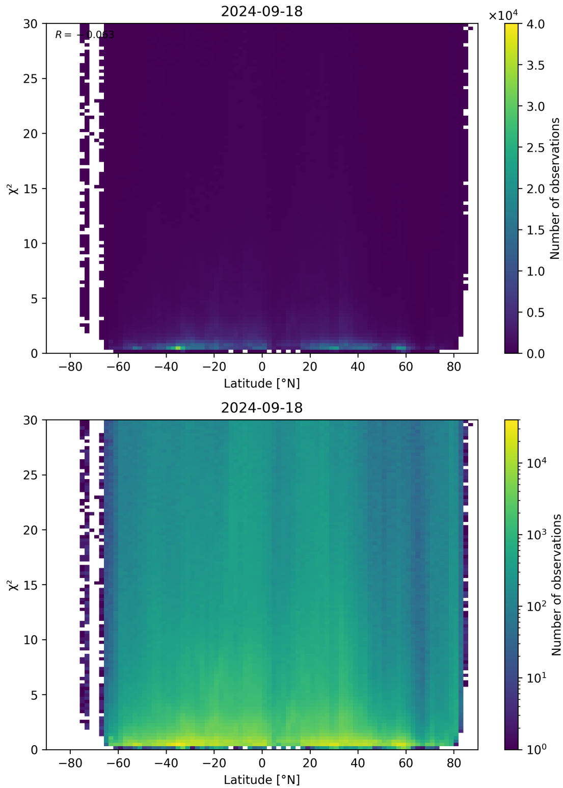
Figure 97: Scatter density plot of “Latitude” against “ \chi^2 ” for 2024-09-17 to 2024-09-19.
