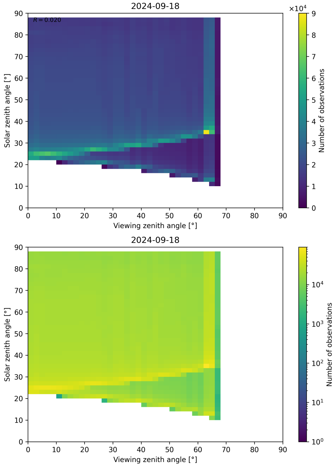
Figure 139: Scatter density plot of “Viewing zenith angle” against “Solar zenith angle” for 2024-09-17 to 2024-09-19.
