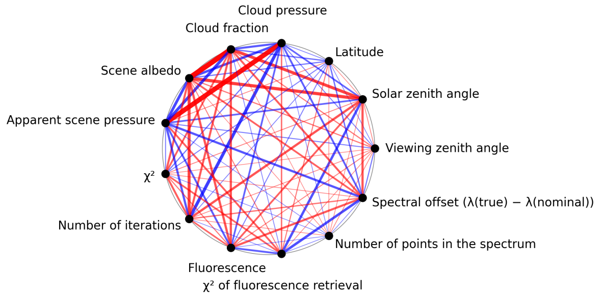
Figure 1: Map of correlation graph for 2024-09-17 to 2024-09-19.
