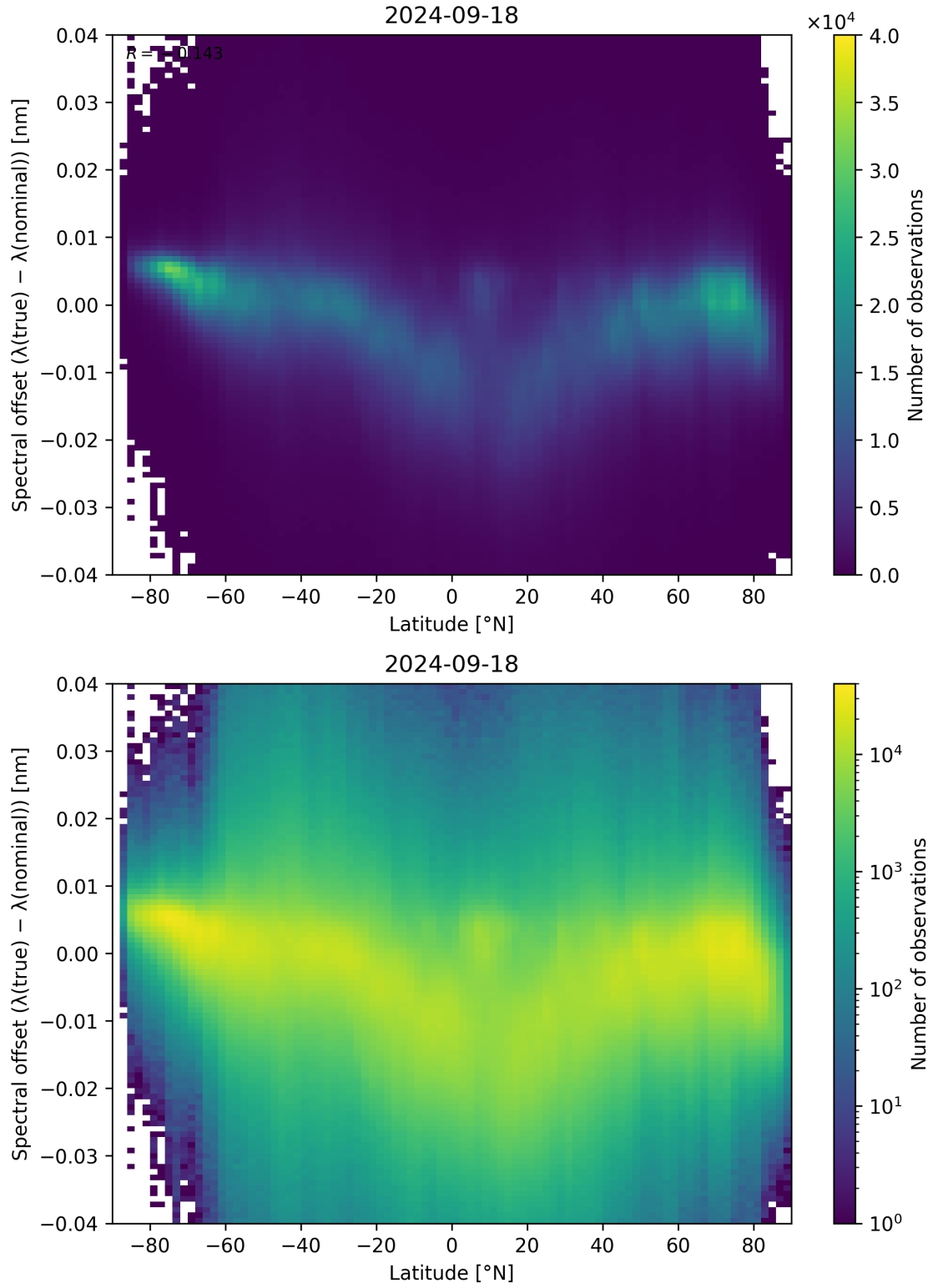
Figure 105: Scatter density plot of “Latitude” against “Spectral offset ( \lambda_{\text{true}} - \lambda_{\text{nominal}} )” for 2024-09-17 to 2024-09-19.
