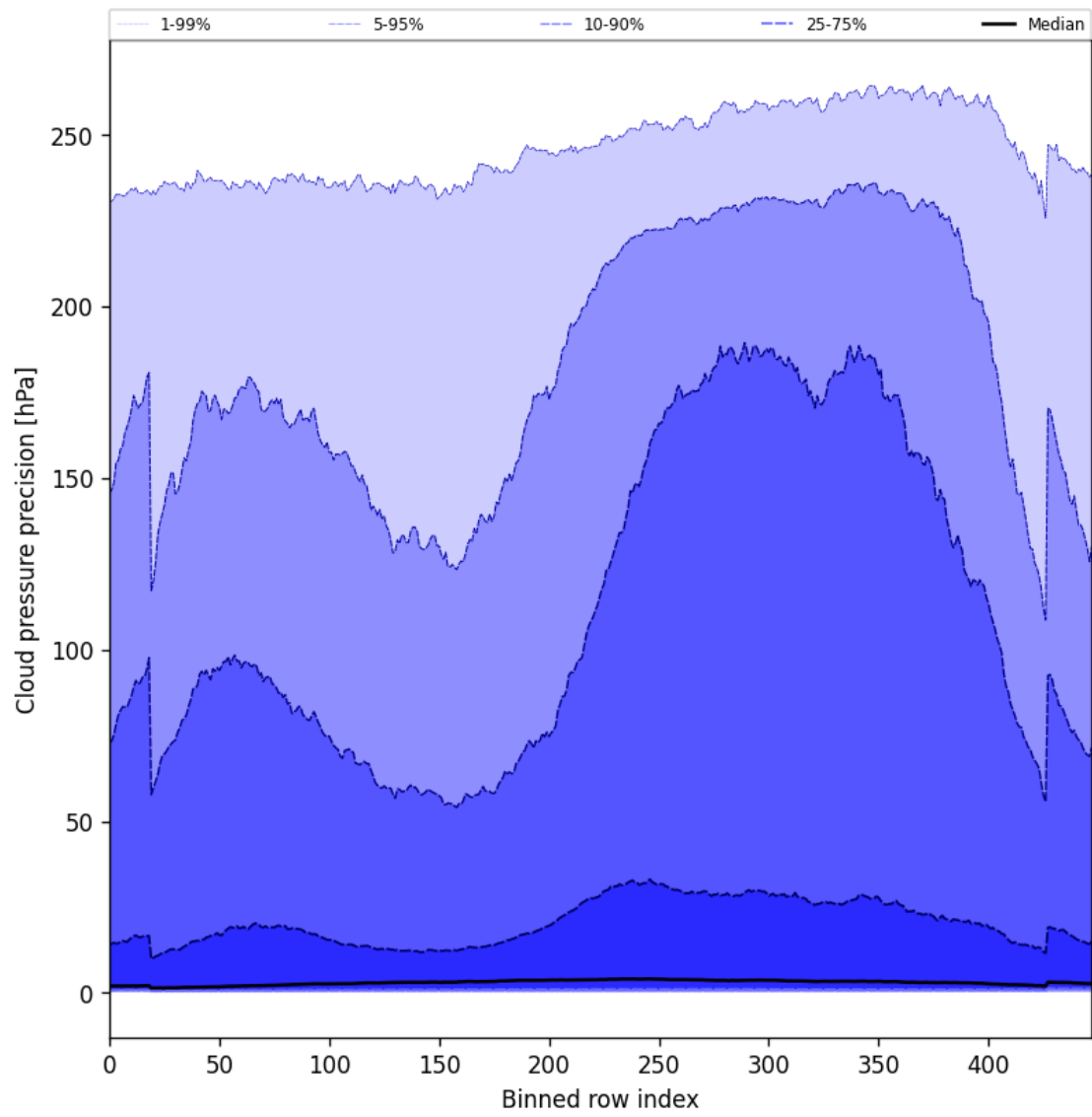
Figure 48: Along track statistics of “Cloud pressure precision” for 2024-09-17 to 2024-09-19
