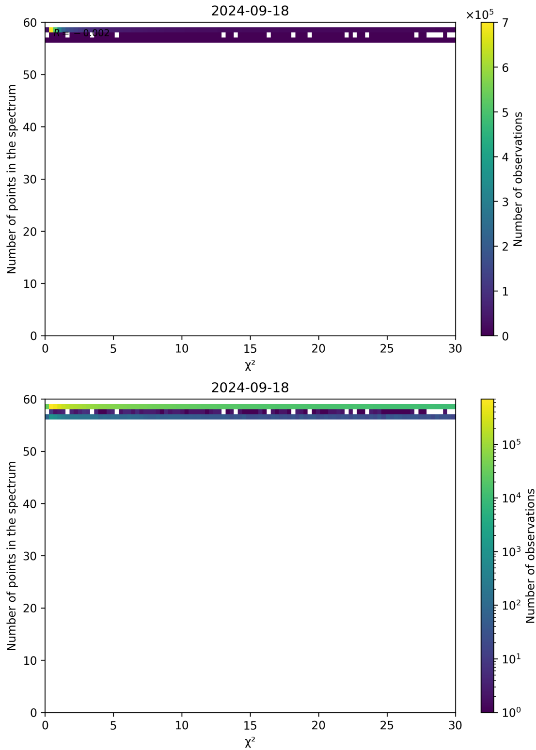
Figure 74: Scatter density plot of “ \chi^2 ” against “Number of points in the spectrum” for 2024-09-17 to 2024-09-19.
