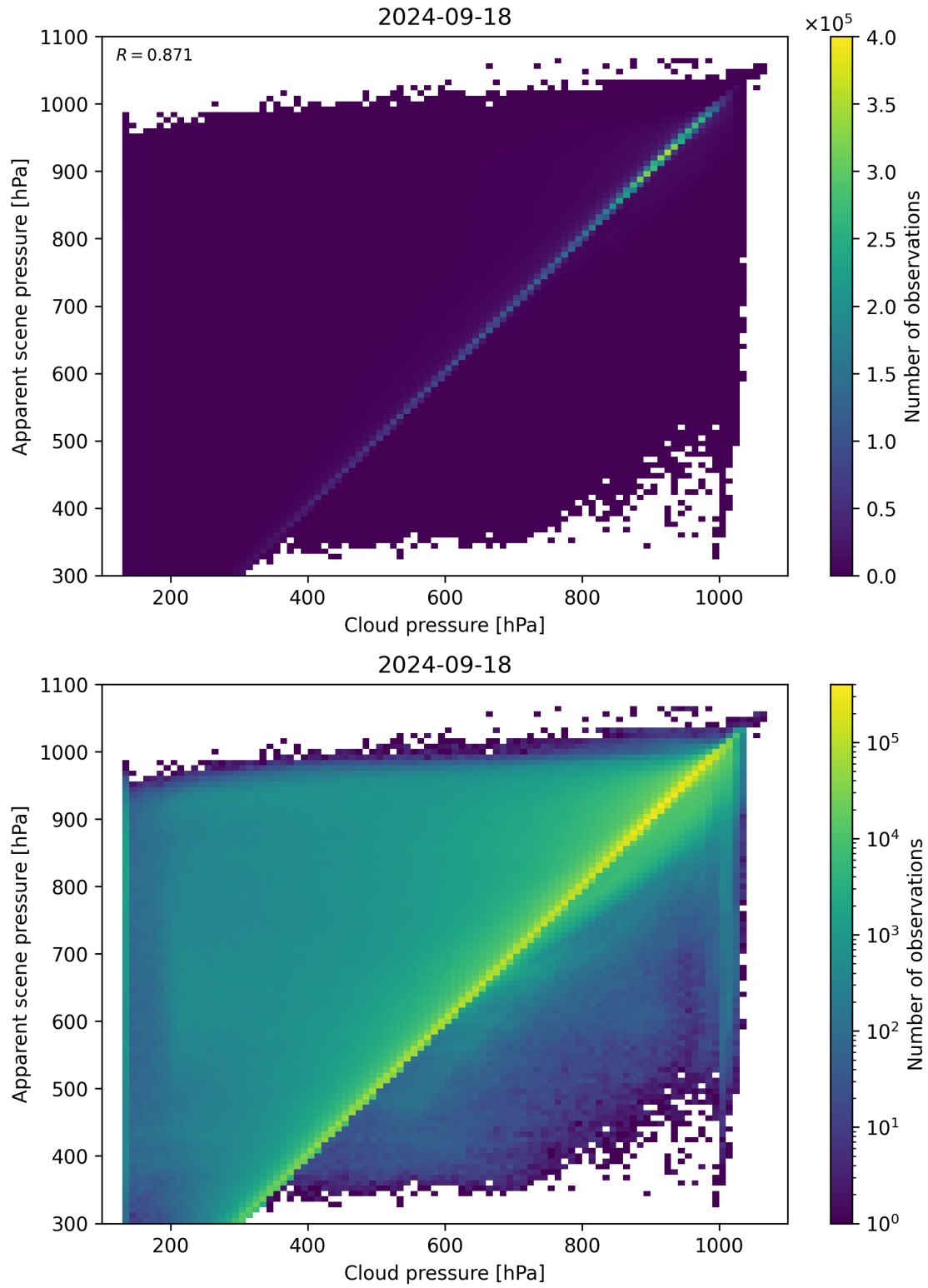
Figure 84: Scatter density plot of “Cloud pressure” against “Apparent scene pressure” for 2024-09-17 to 2024-09-19.
