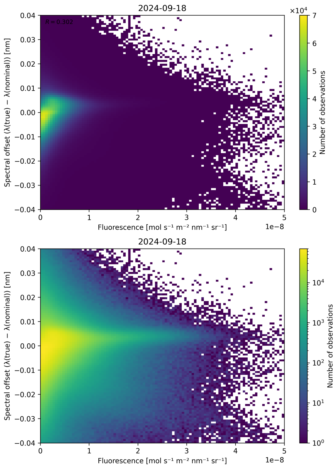
Figure 95: Scatter density plot of “Fluorescence” against “Spectral offset ( \lambda_{\text{true}} - \lambda_{\text{nominal}} )” for 2024-09-17 to 2024-09-19.
