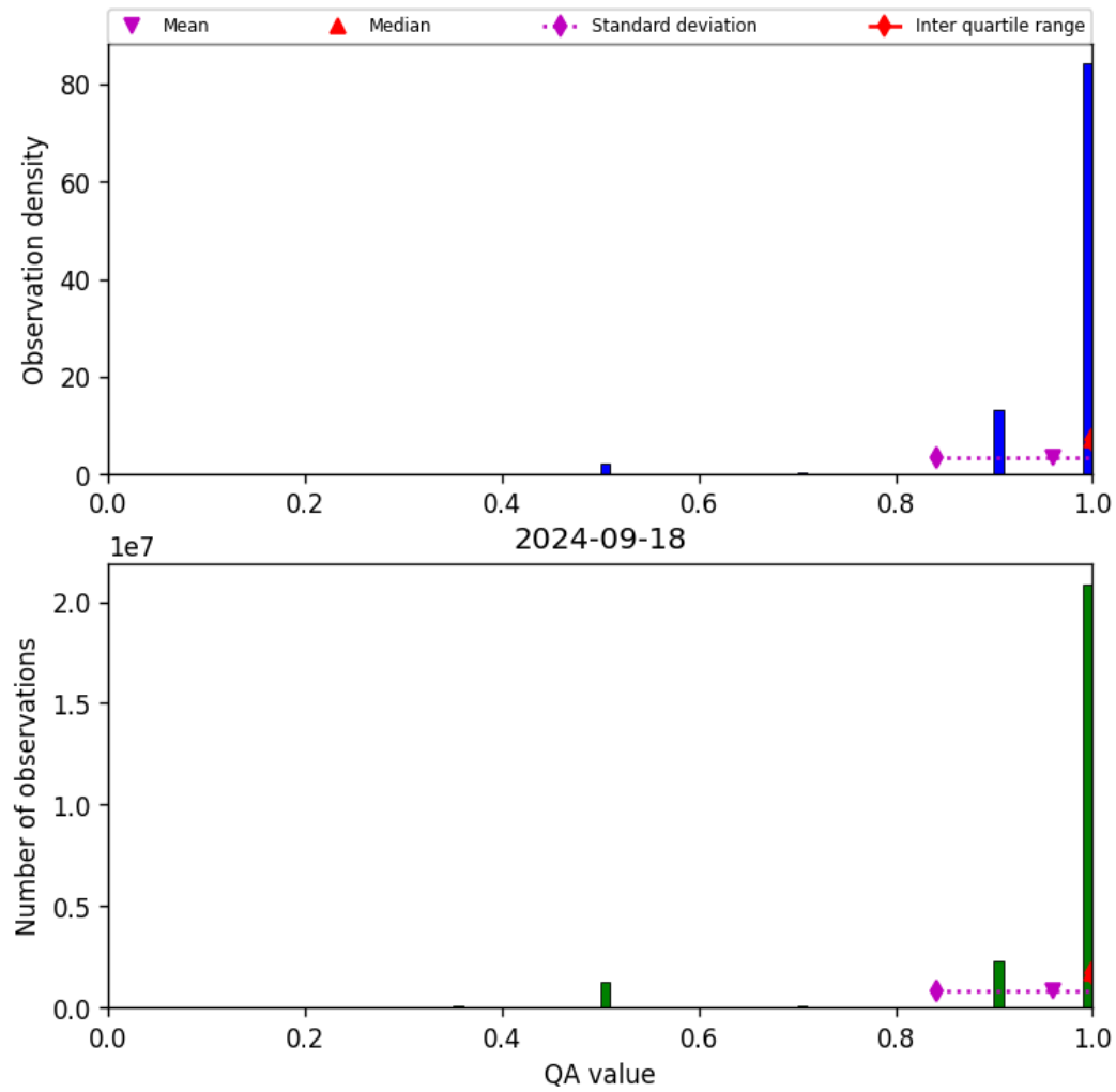
Figure 29: Histogram of “QA value” for 2024-09-17 to 2024-09-19
