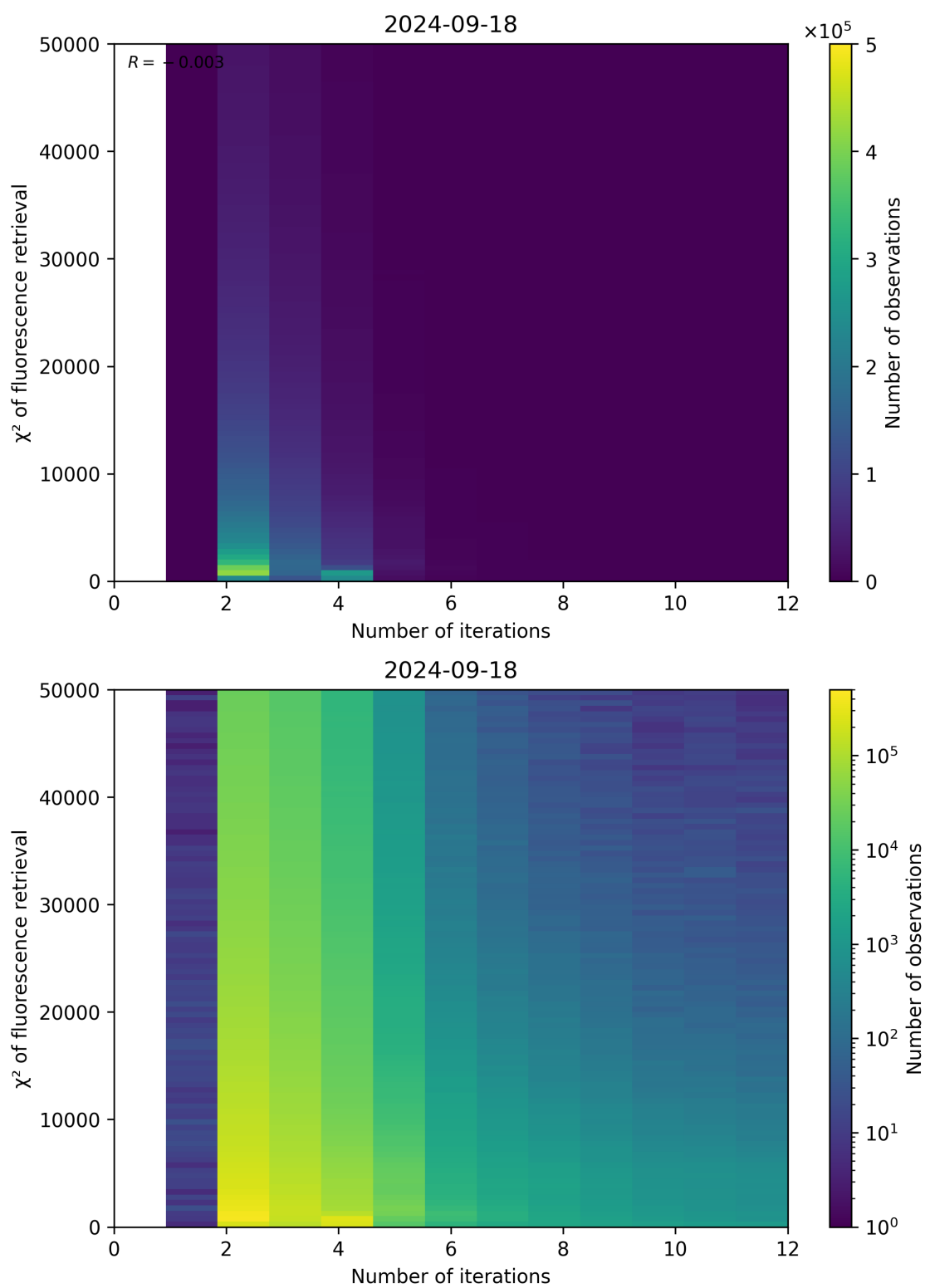
Figure 106: Scatter density plot of “Number of iterations” against “ \chi^2 of fluorescence retrieval” for 2024-09-17 to 2024-09-19.
