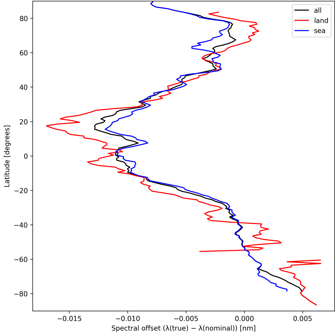
Figure 28: Zonal average of “Spectral offset ( \lambda_{\text{true}} - \lambda_{\text{nominal}} )” for 2024-09-17 to 2024-09-19.
