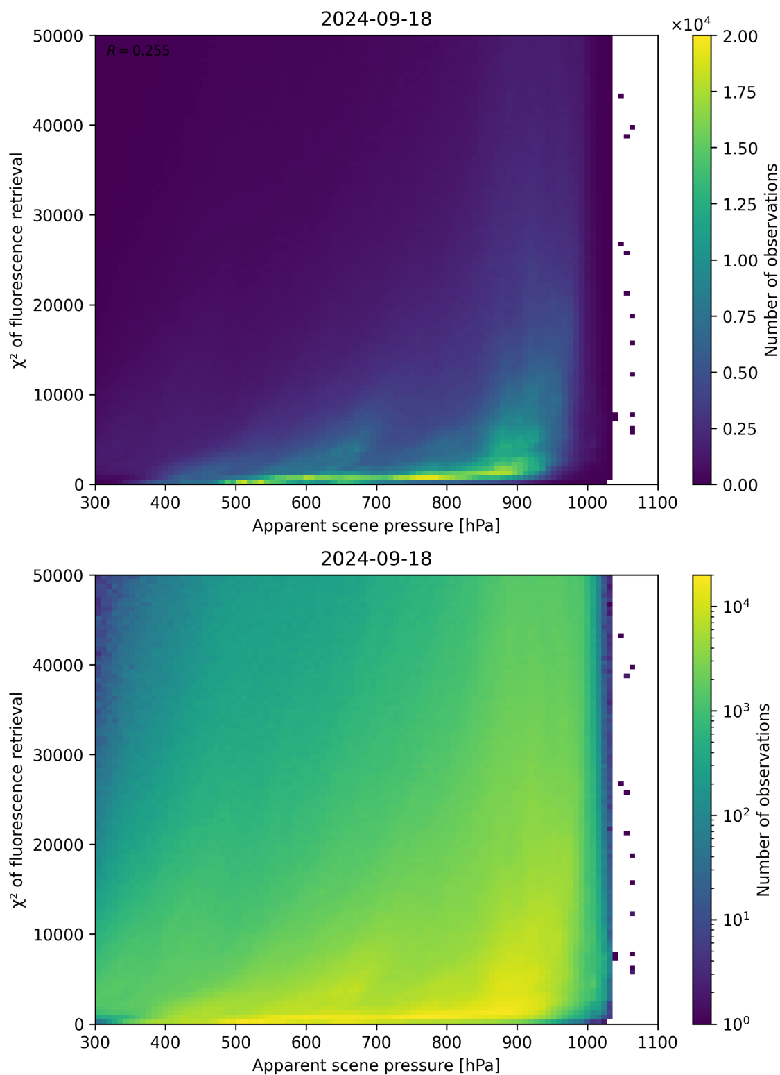
Figure 64: Scatter density plot of “Apparent scene pressure” against “ \chi^2 of fluorescence retrieval” for 2024-09-17 to 2024-09-19.
