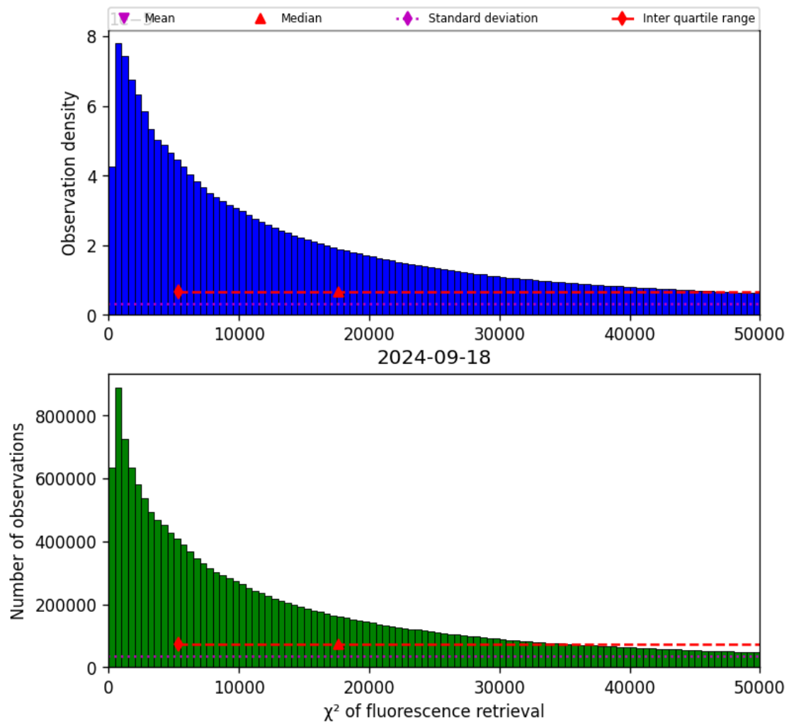
Figure 42: Histogram of “ \chi^2 of fluorescence retrieval” for 2024-09-17 to 2024-09-19
