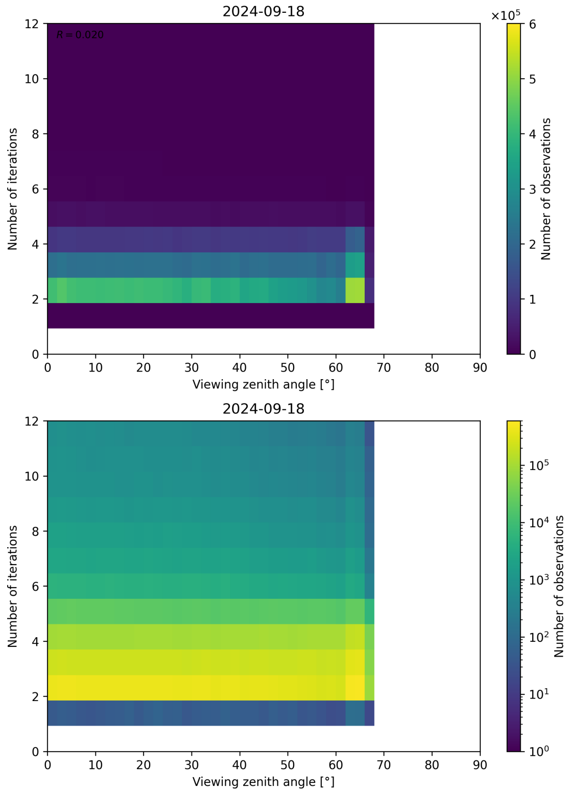
Figure 136: Scatter density plot of “Viewing zenith angle” against “Number of iterations” for 2024-09-17 to 2024-09-19.
