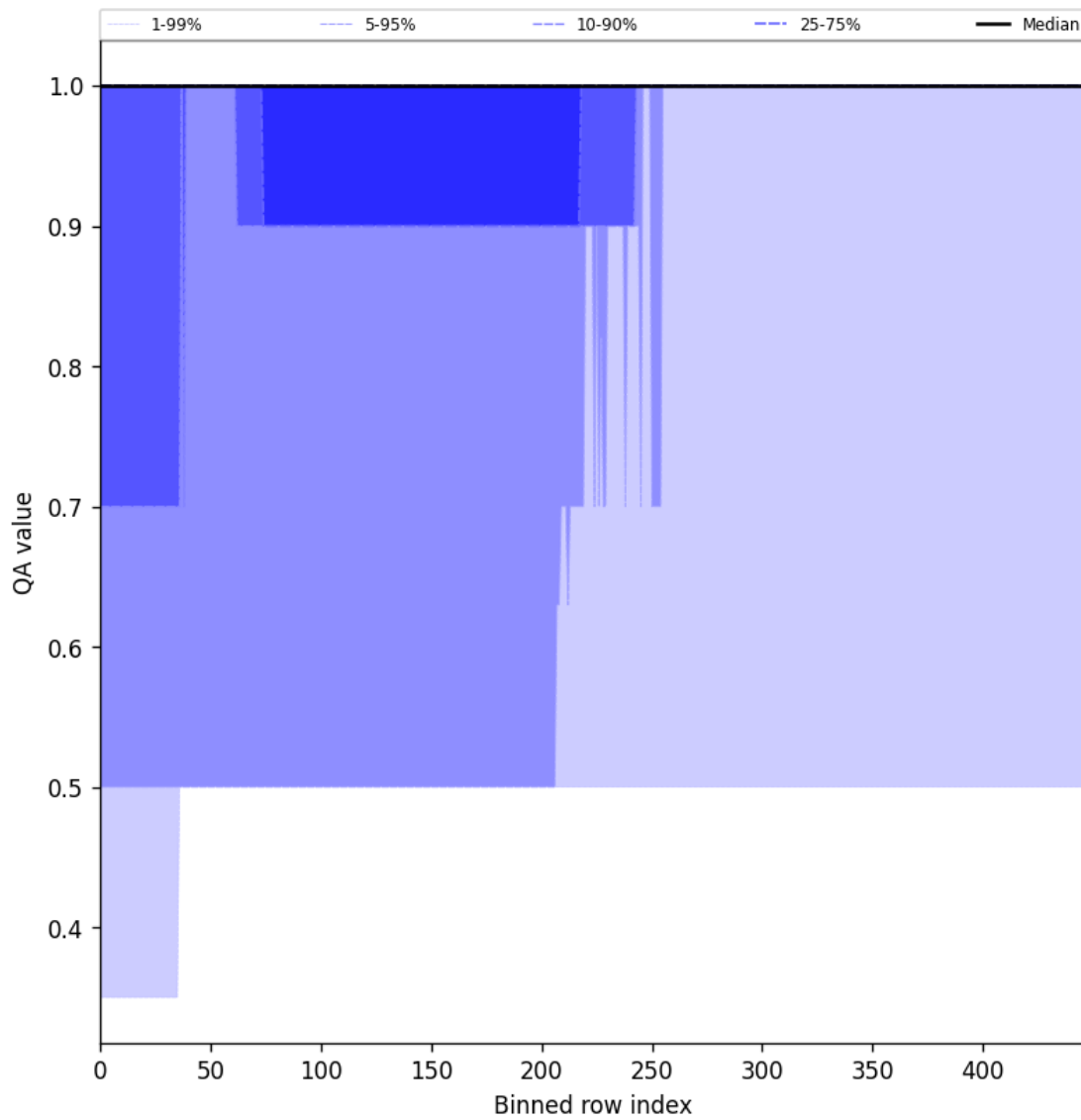
Figure 46: Along track statistics of “QA value” for 2024-09-17 to 2024-09-19
