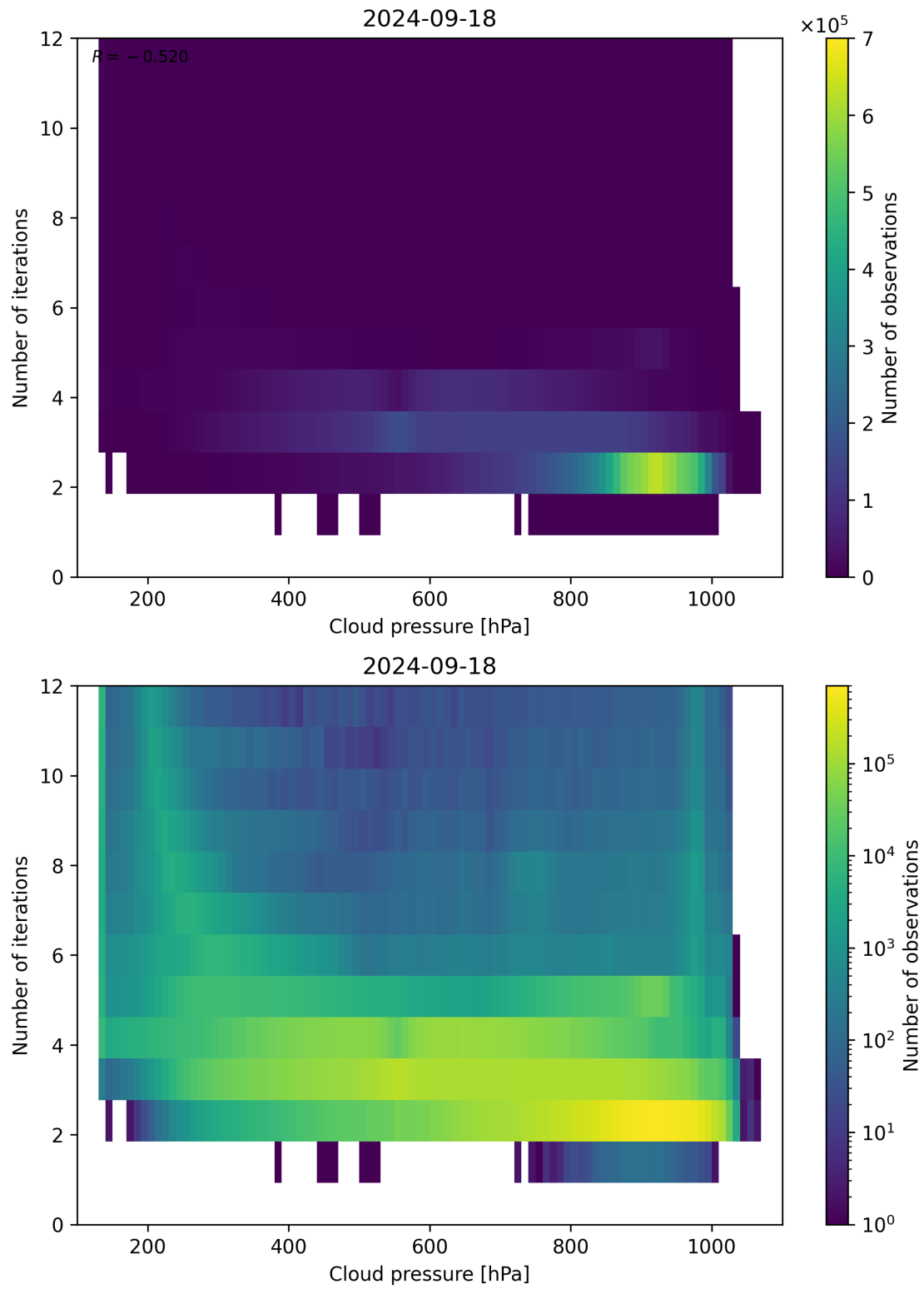
Figure 89: Scatter density plot of “Cloud pressure” against “Number of iterations” for 2024-09-17 to 2024-09-19.
