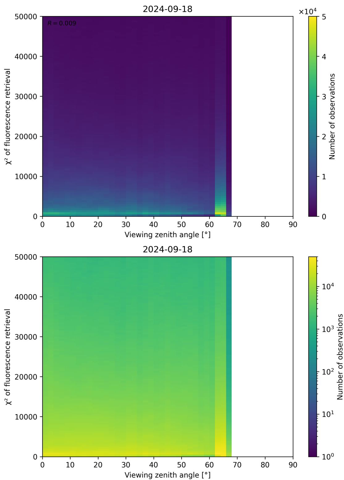
Figure 131: Scatter density plot of “Viewing zenith angle” against “ \chi^2 of fluorescence retrieval” for 2024-09-17 to 2024-09-19.
