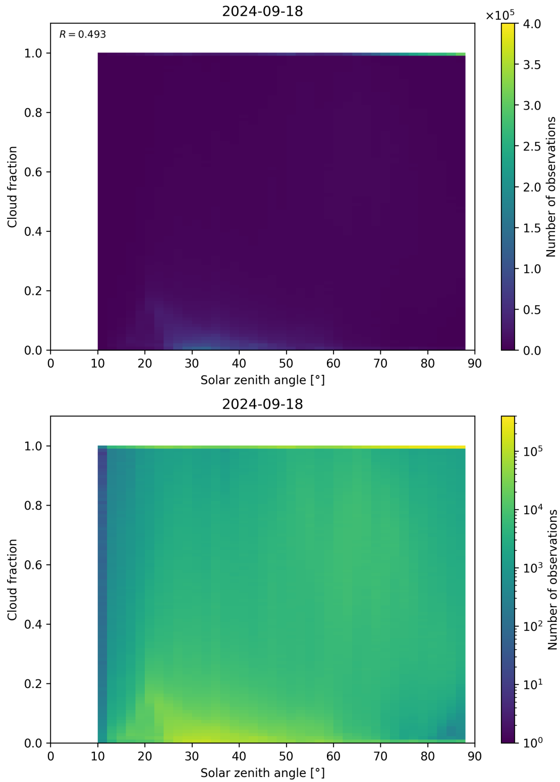
Figure 121: Scatter density plot of “Solar zenith angle” against “Cloud fraction” for 2024-09-17 to 2024-09-19.
