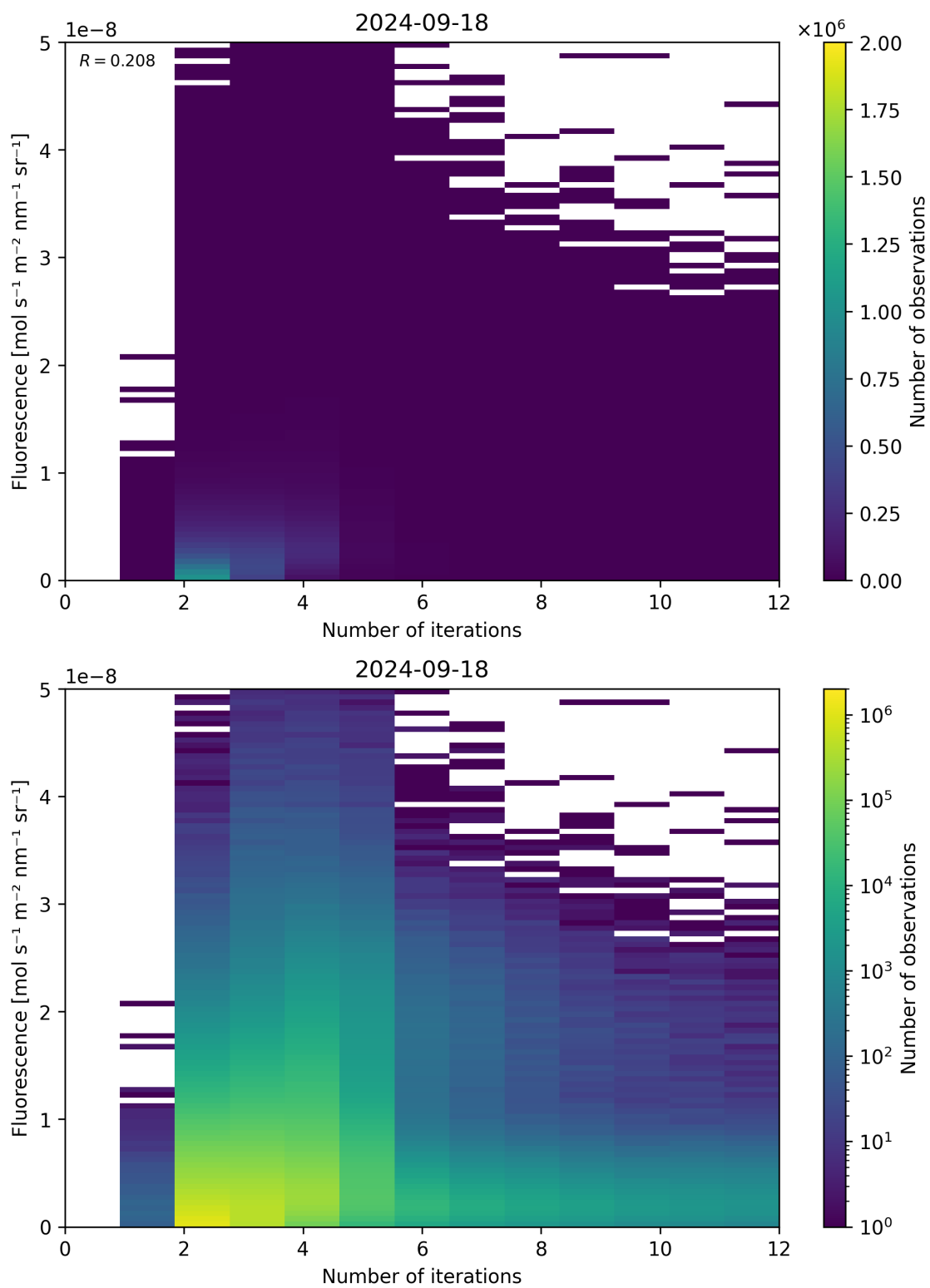
Figure 107: Scatter density plot of “Number of iterations” against “Fluorescence” for 2024-09-17 to 2024-09-19.
