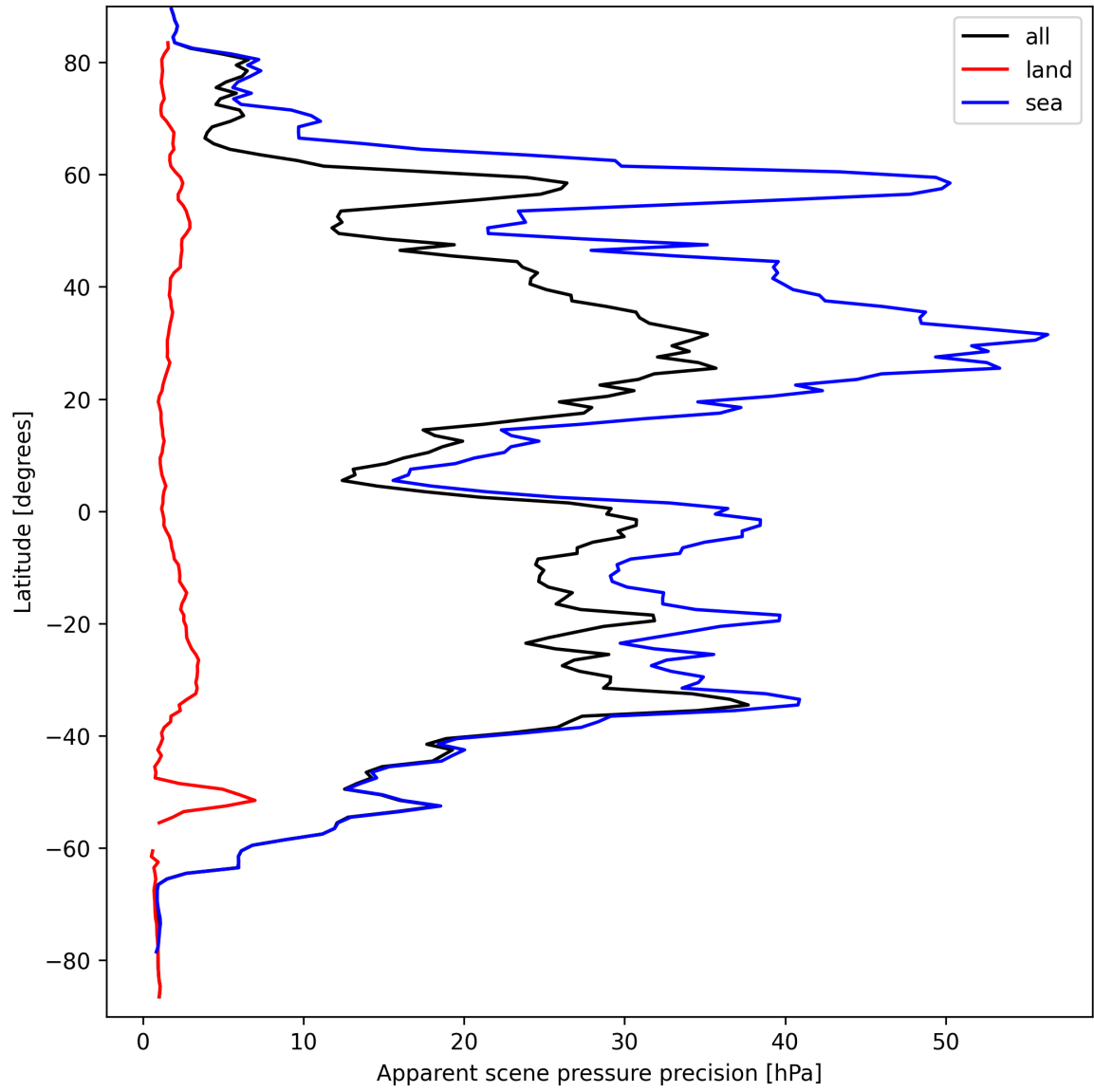
Figure 20: Zonal average of “Apparent scene pressure precision” for 2024-09-17 to 2024-09-19.
