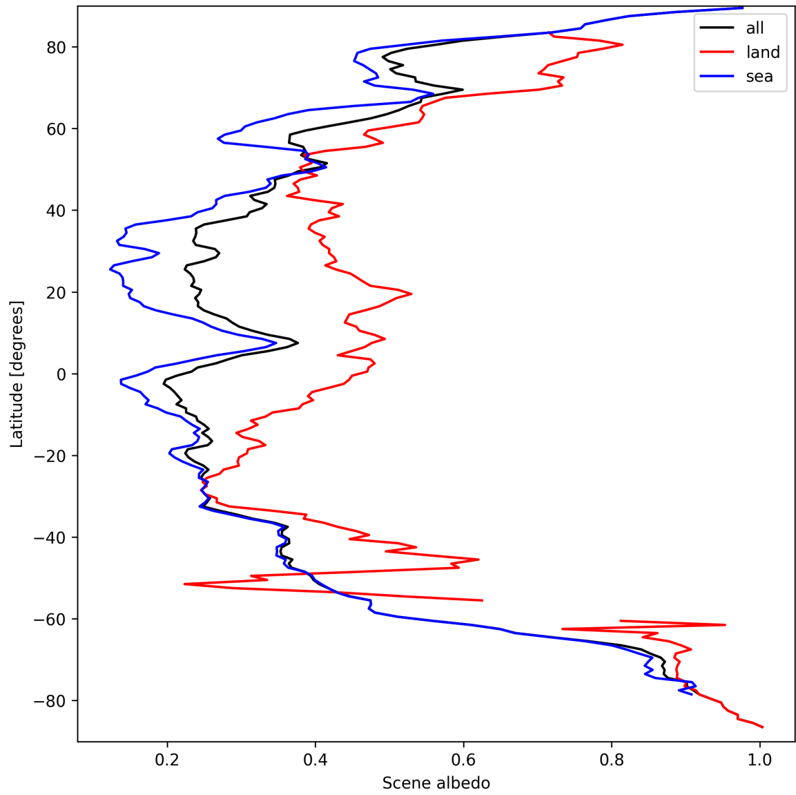
Figure 17: Zonal average of “Scene albedo” for 2024-09-17 to 2024-09-19.
