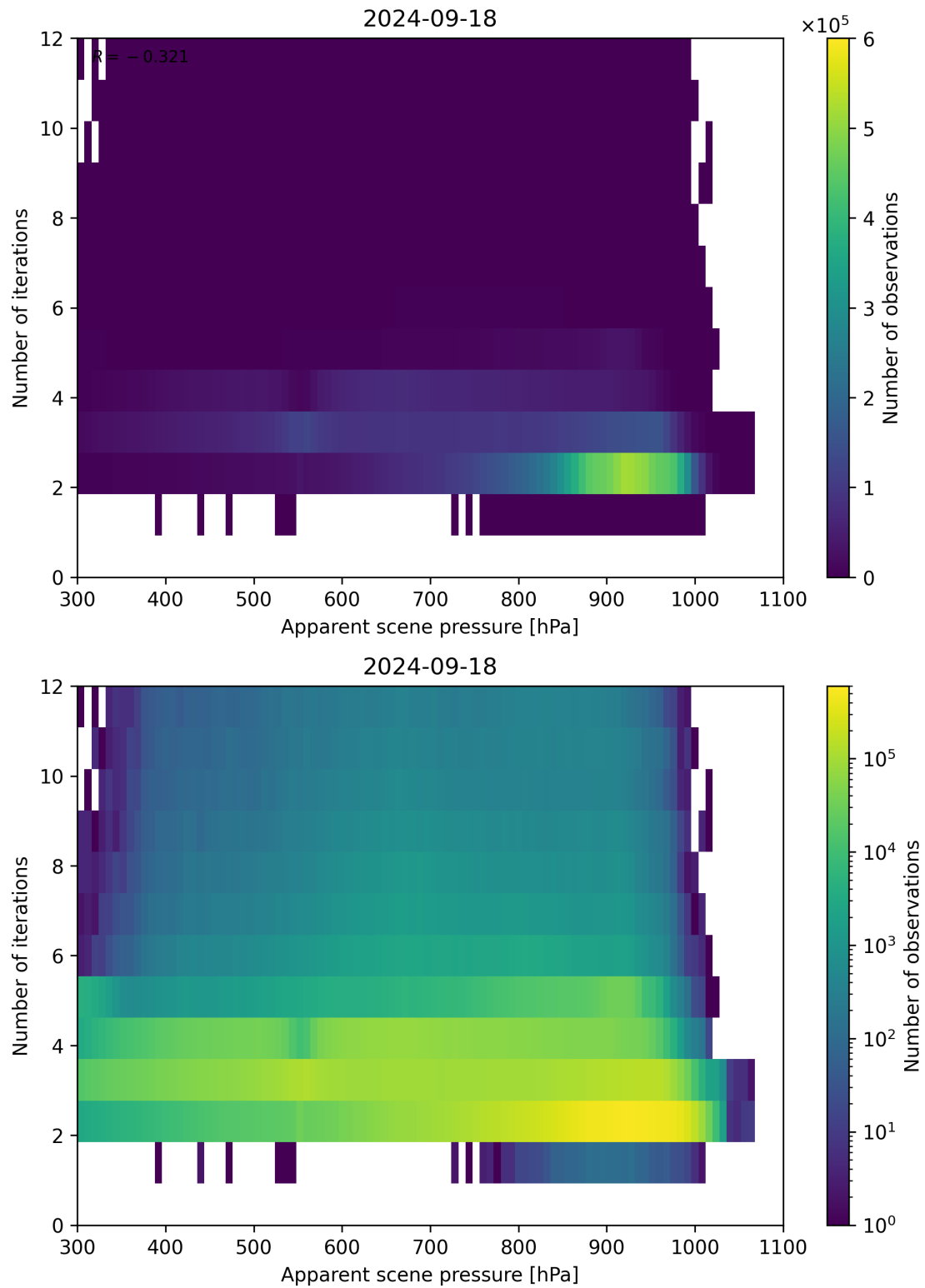
Figure 66: Scatter density plot of “Apparent scene pressure” against “Number of iterations” for 2024-09-17 to 2024-09-19.
