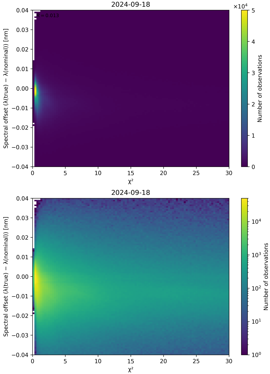
Figure 75: Scatter density plot of “ \chi^2 ” against “Spectral offset ( \lambda_{\text{true}} - \lambda_{\text{nominal}} )” for 2024-09-17 to 2024-09-19.
