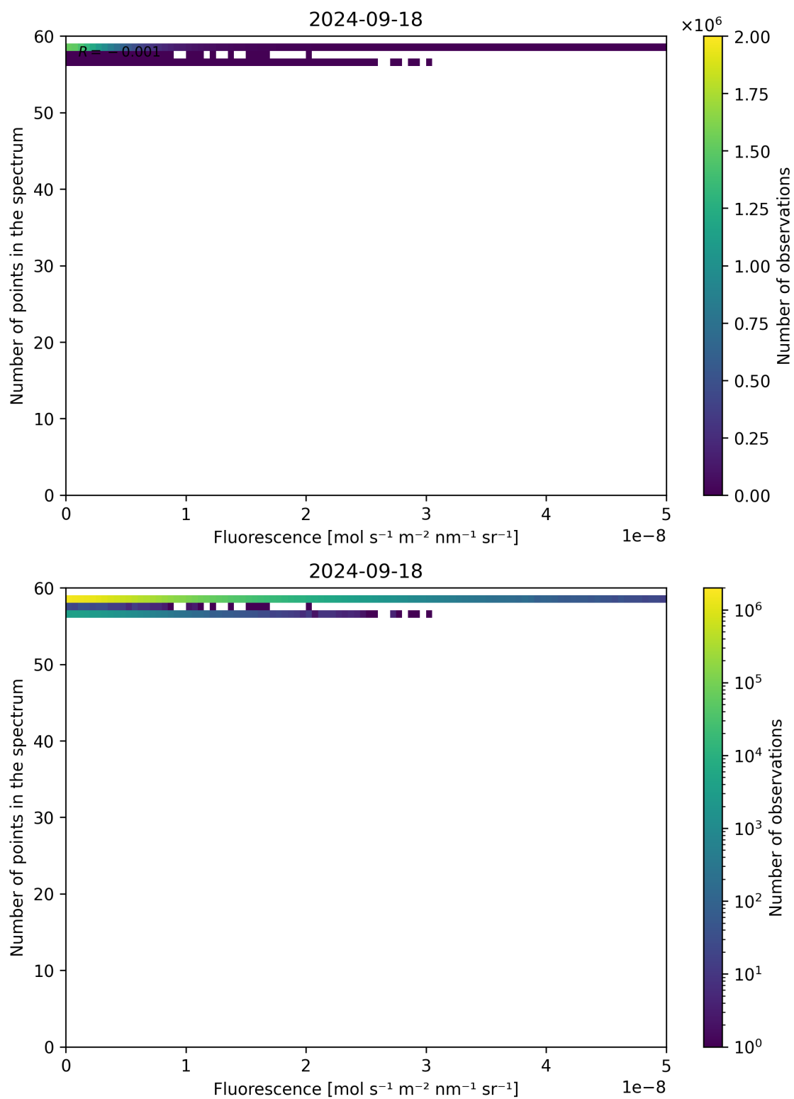
Figure 94: Scatter density plot of “Fluorescence” against “Number of points in the spectrum” for 2024-09-17 to 2024-09-19.
