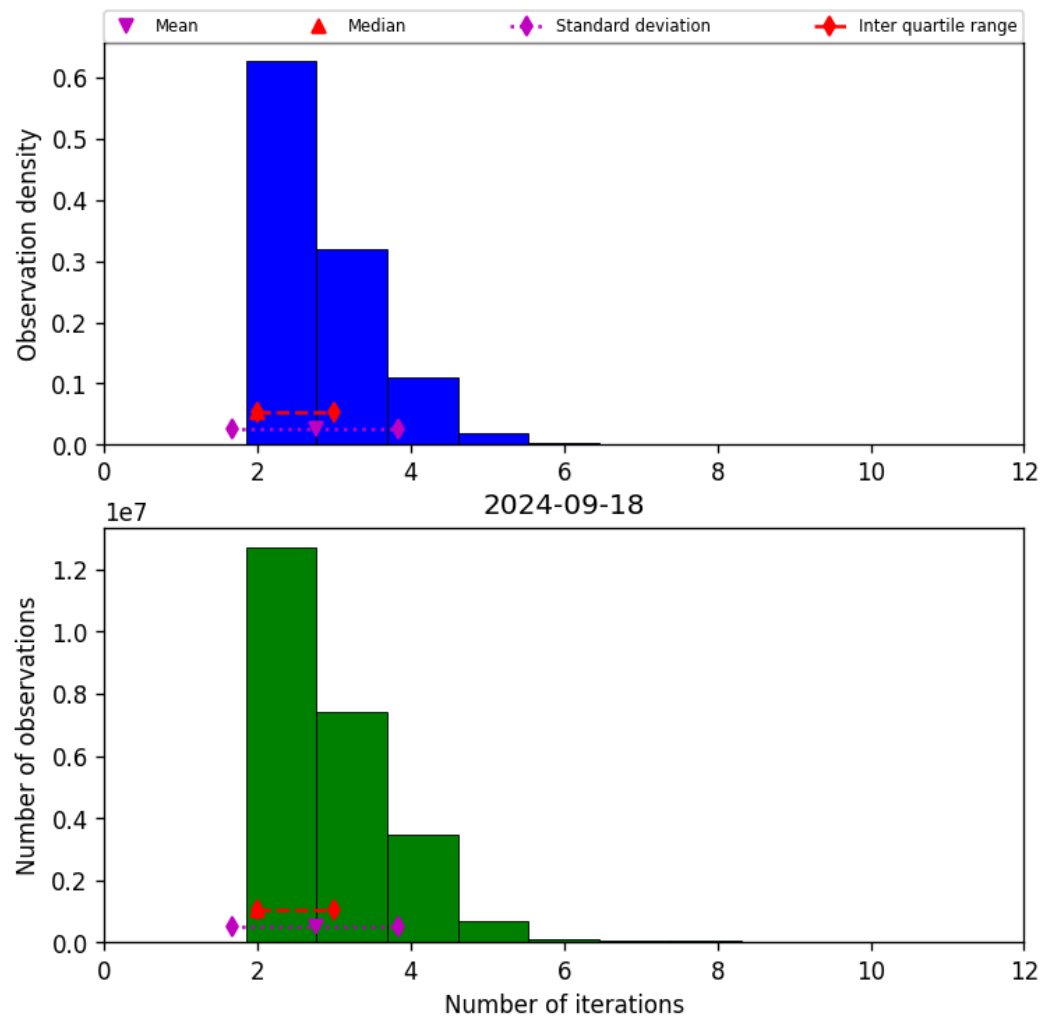
Figure 39: Histogram of “Number of iterations” for 2024-09-17 to 2024-09-19
