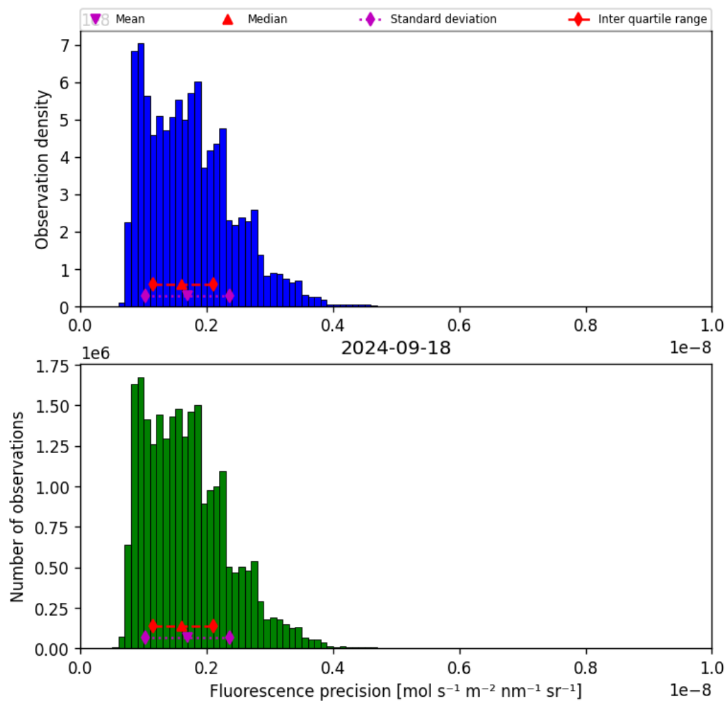
Figure 41: Histogram of “Fluorescence precision” for 2024-09-17 to 2024-09-19
