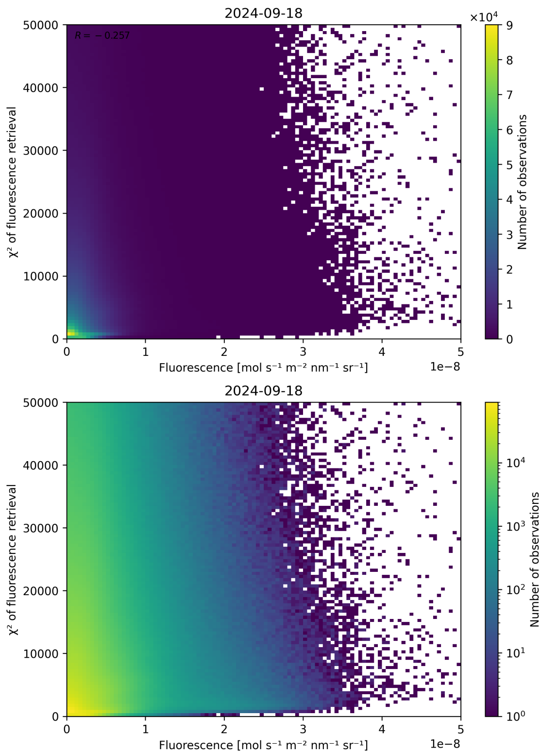
Figure 93: Scatter density plot of “Fluorescence” against “ \chi^2 of fluorescence retrieval” for 2024-09-17 to 2024-09-19.
