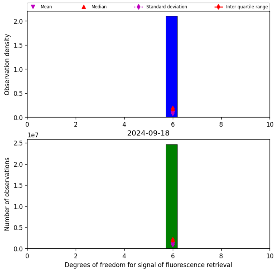
Figure 43: Histogram of “Degrees of freedom for signal of fluorescence retrieval” for 2024-09-17 to 2024-09-19
