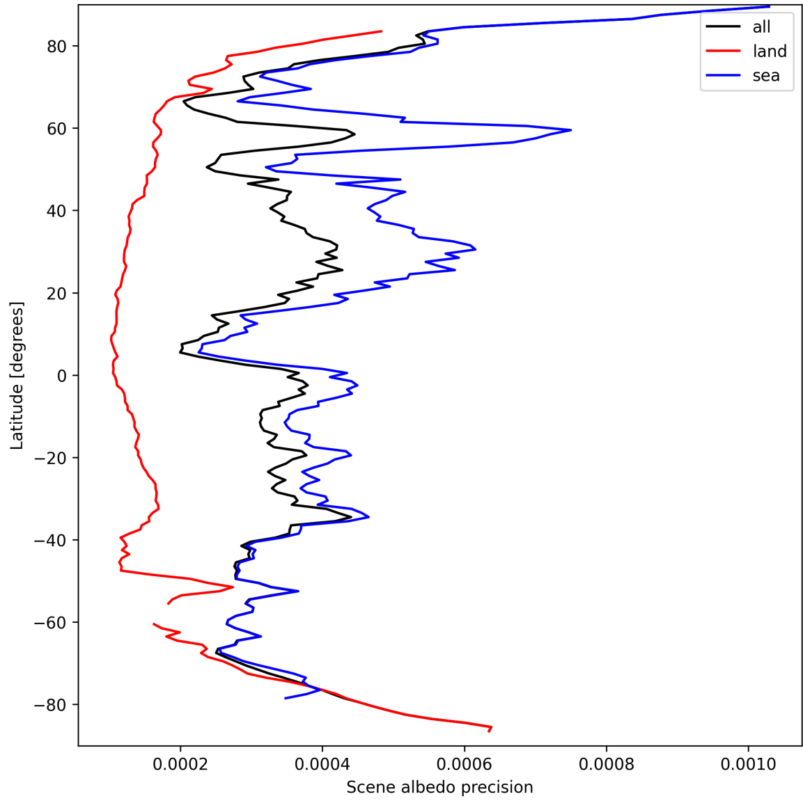
Figure 18: Zonal average of “Scene albedo precision” for 2024-09-17 to 2024-09-19.
