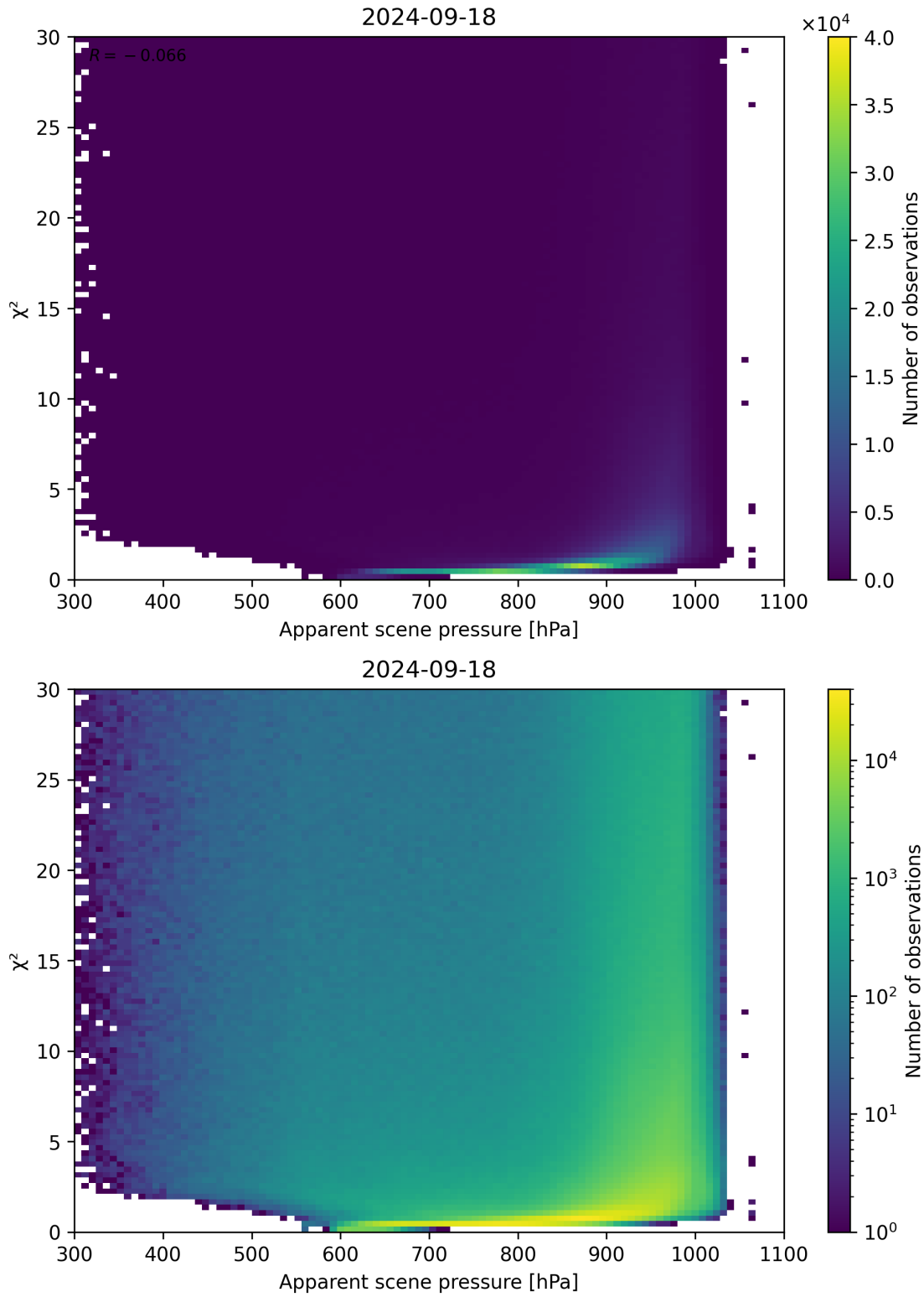
Figure 63: Scatter density plot of “Apparent scene pressure” against “ \chi^2 ” for 2024-09-17 to 2024-09-19.
