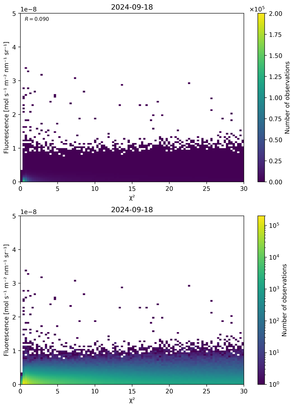
Figure 70: Scatter density plot of “ \chi^2 ” against “Fluorescence” for 2024-09-17 to 2024-09-19.
