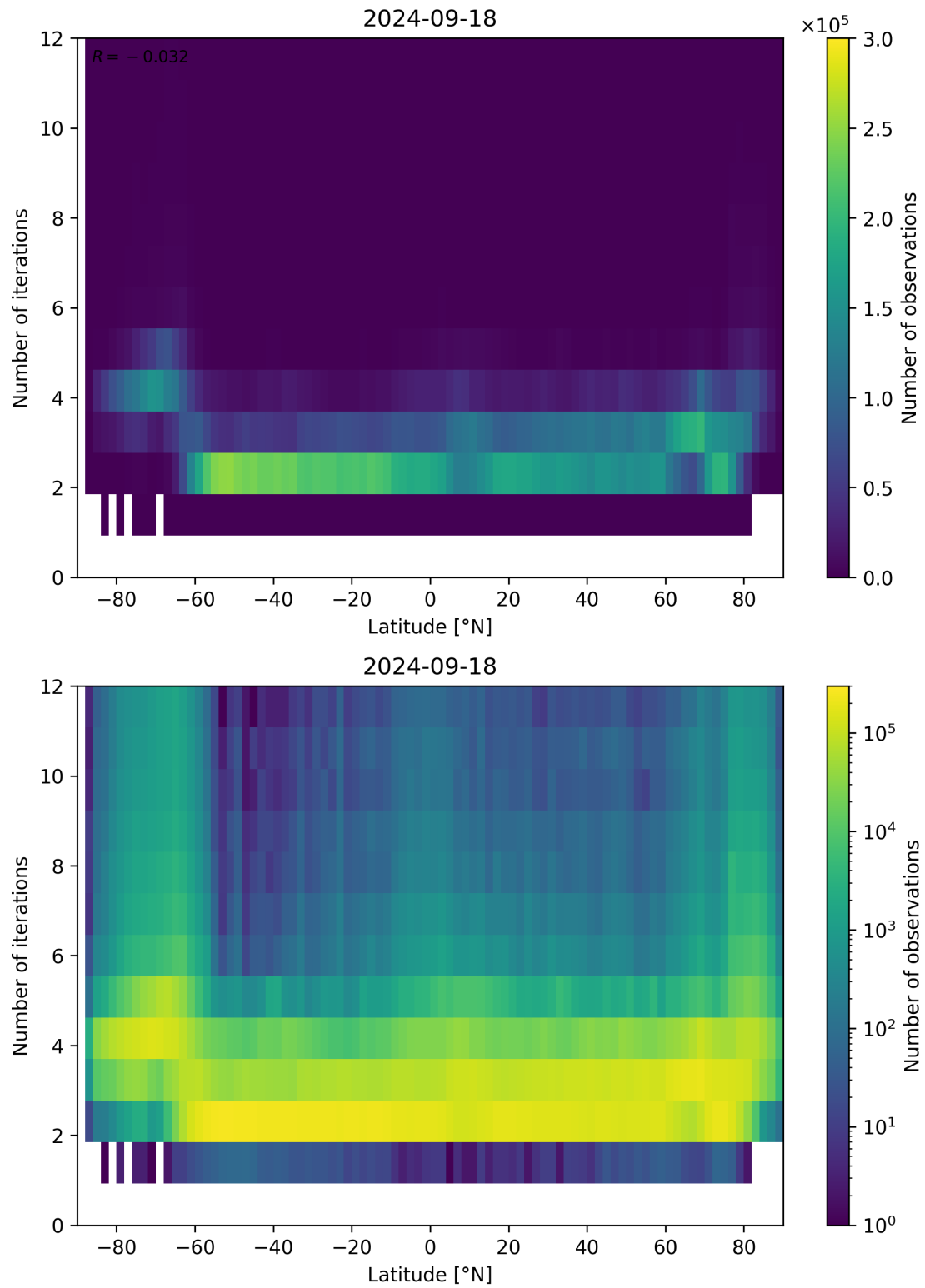
Figure 102: Scatter density plot of “Latitude” against “Number of iterations” for 2024-09-17 to 2024-09-19.
