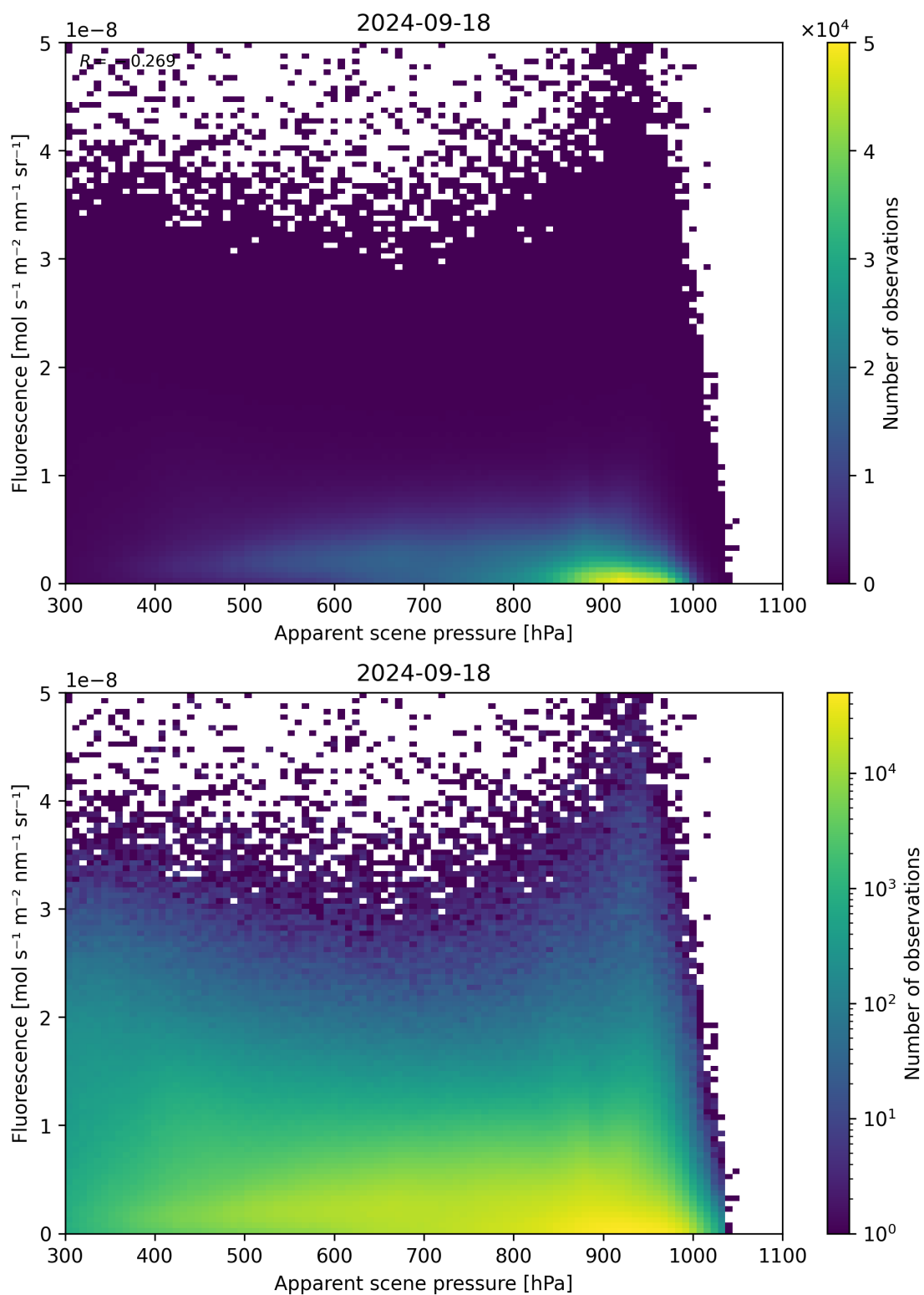
Figure 65: Scatter density plot of “Apparent scene pressure” against “Fluorescence” for 2024-09-17 to 2024-09-19.
