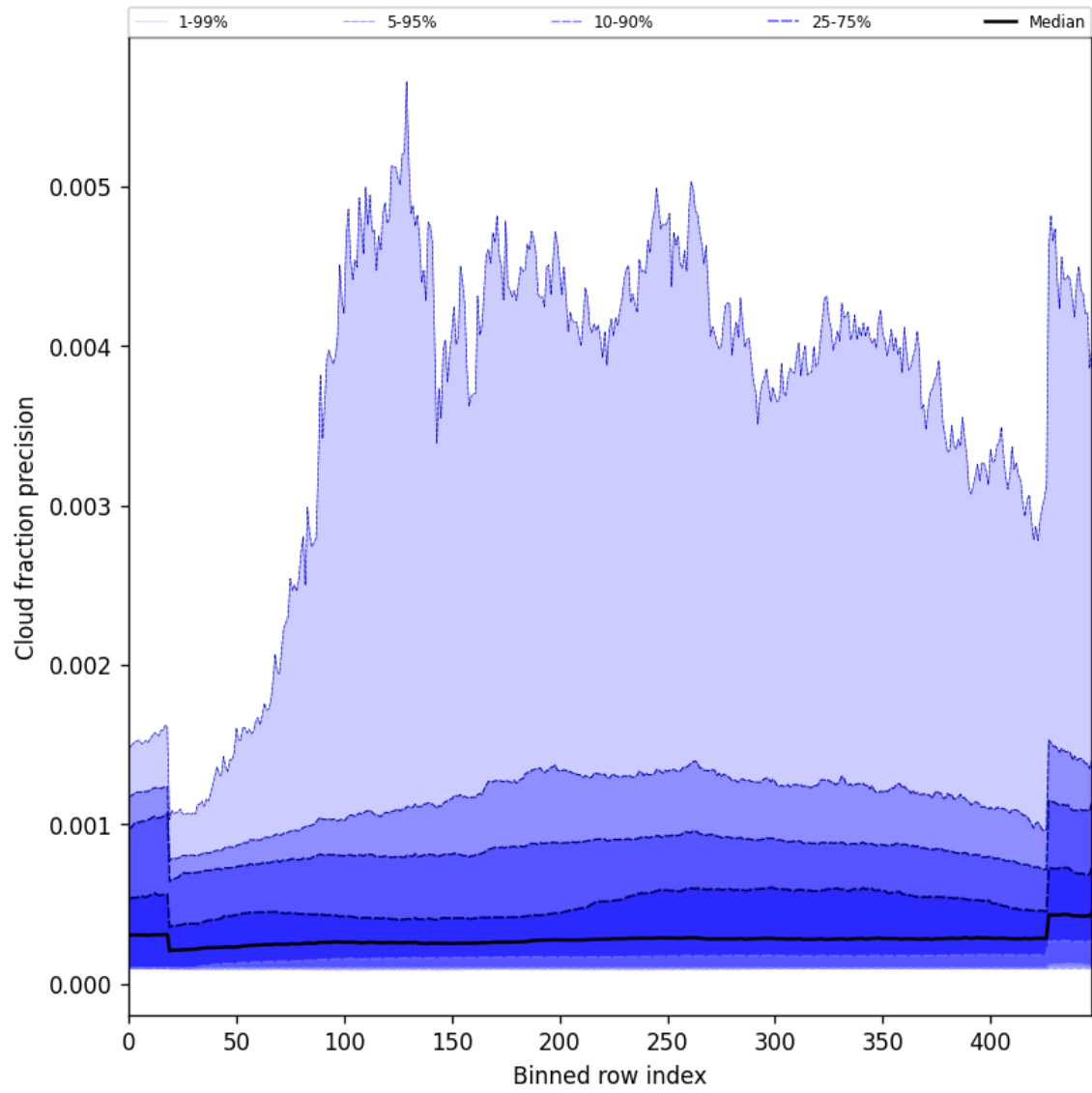
Figure 50: Along track statistics of “Cloud fraction precision” for 2024-09-17 to 2024-09-19
