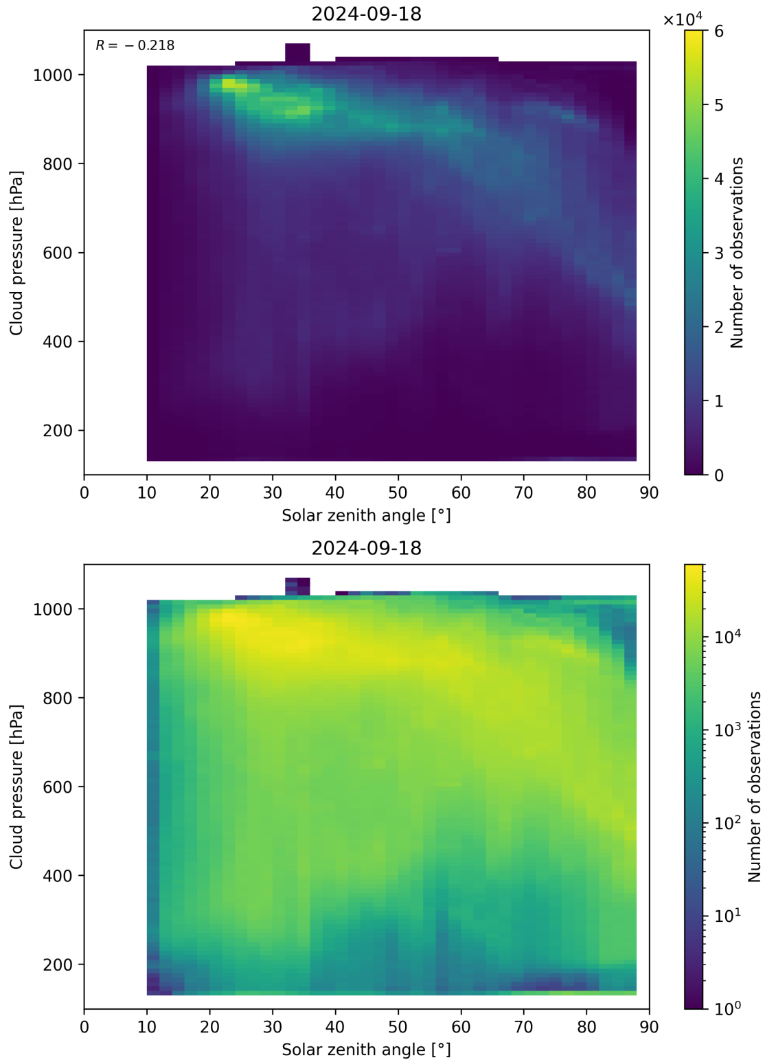
Figure 122: Scatter density plot of “Solar zenith angle” against “Cloud pressure” for 2024-09-17 to 2024-09-19.
