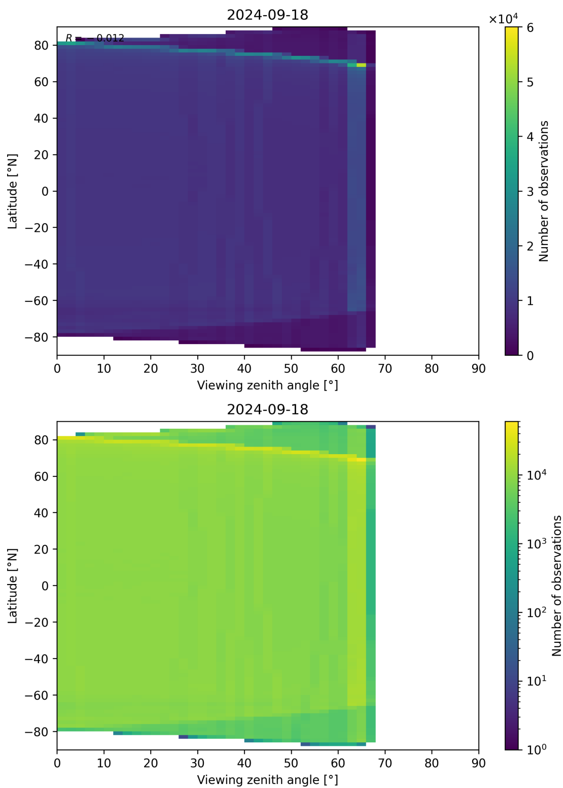
Figure 135: Scatter density plot of “Viewing zenith angle” against “Latitude” for 2024-09-17 to 2024-09-19.
