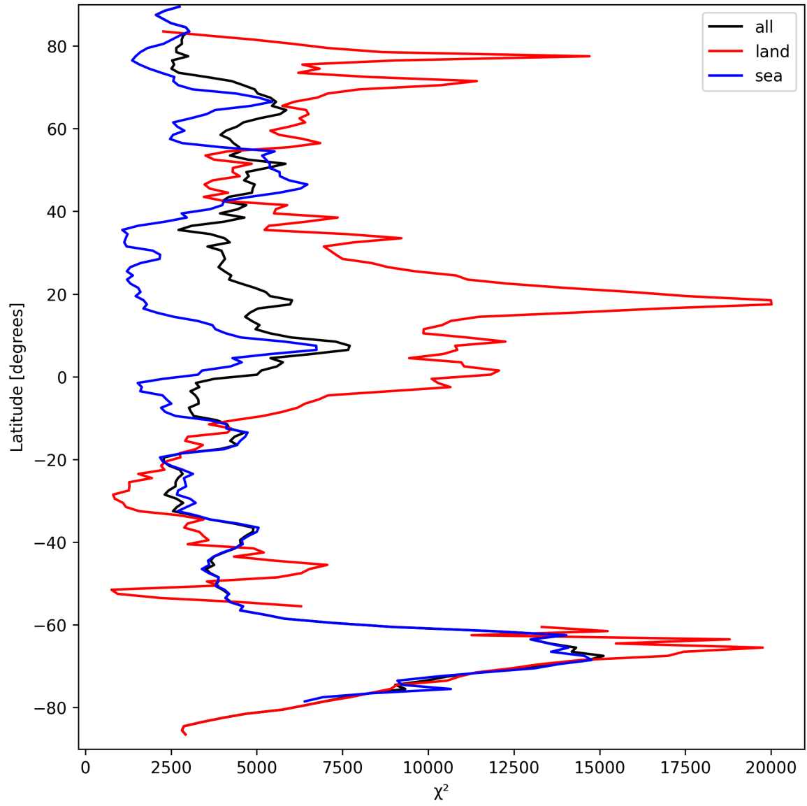
Figure 21: Zonal average of “ \chi^2 ” for 2024-09-17 to 2024-09-19.
