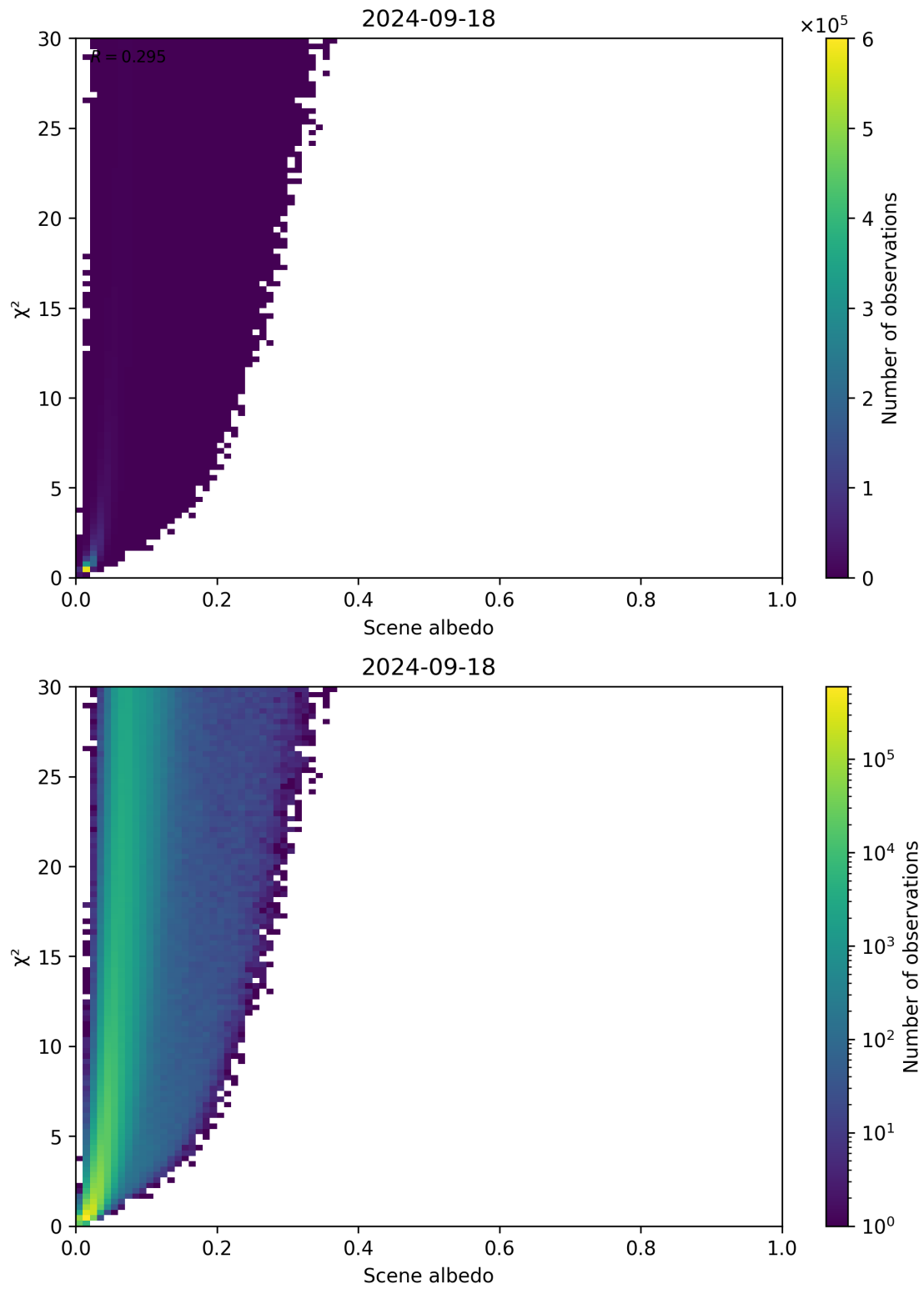
Figure 112: Scatter density plot of “Scene albedo” against “ \chi^2 ” for 2024-09-17 to 2024-09-19.
