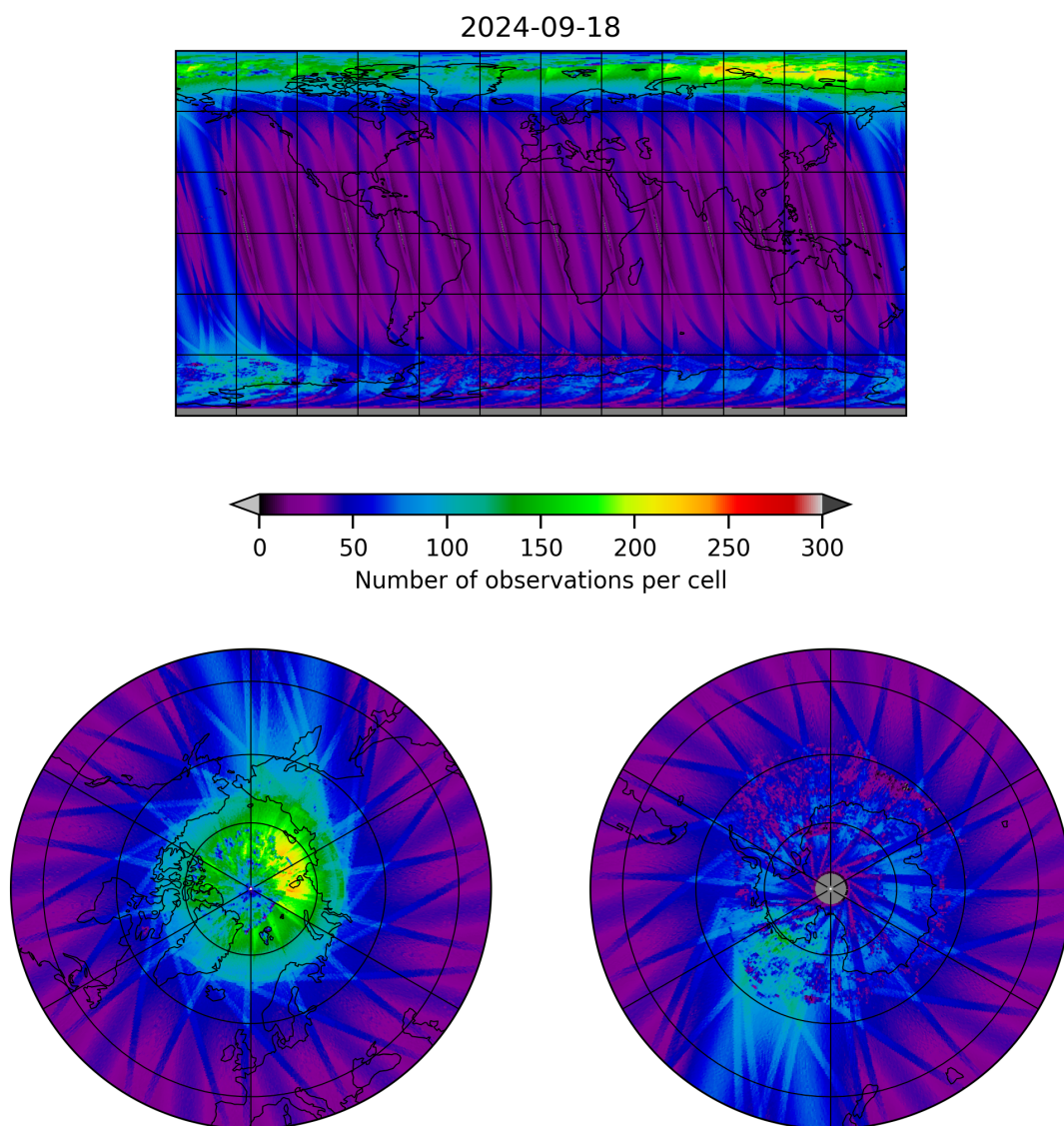
Figure 11: Map of the number of observations for 2024-09-17 to 2024-09-19
