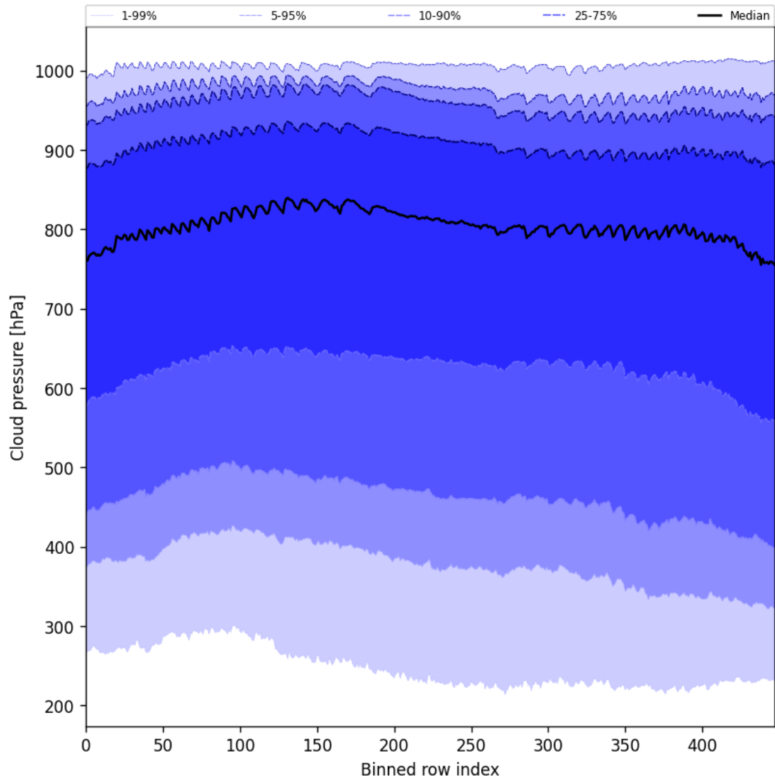
Figure 47: Along track statistics of “Cloud pressure” for 2024-09-17 to 2024-09-19
