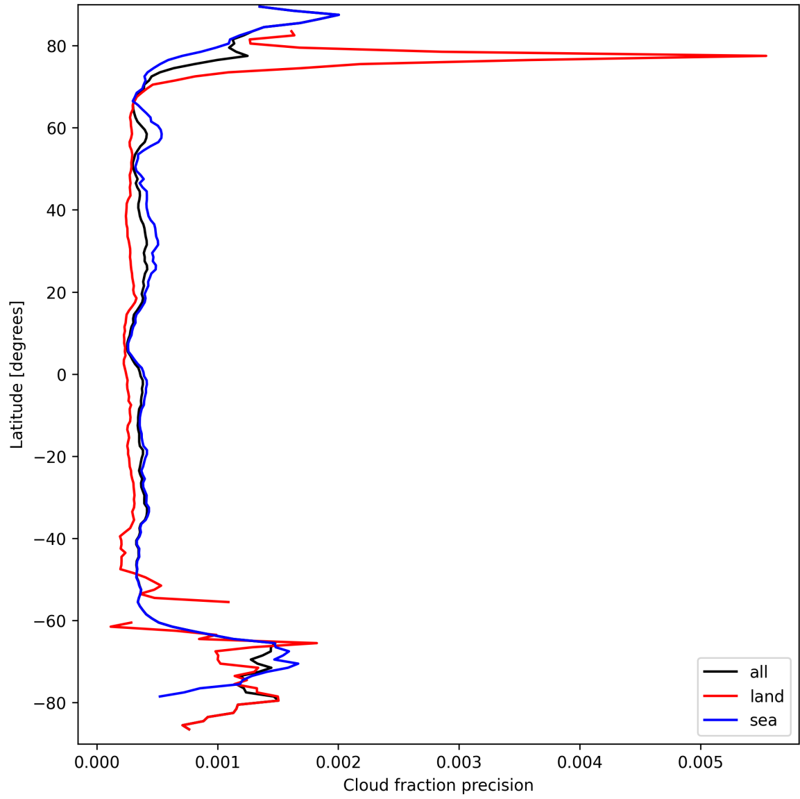
Figure 16: Zonal average of “Cloud fraction precision” for 2024-09-17 to 2024-09-19.
