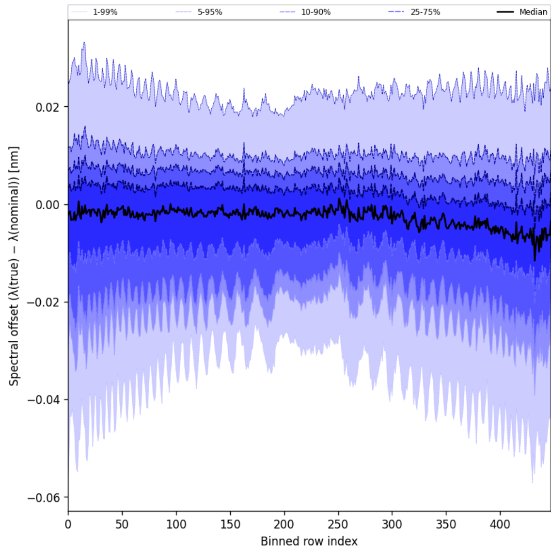
Figure 62: Along track statistics of “Spectral offset ( \lambda_{\text{true}} - \lambda_{\text{nominal}} )” for 2024-09-17 to 2024-09-19
