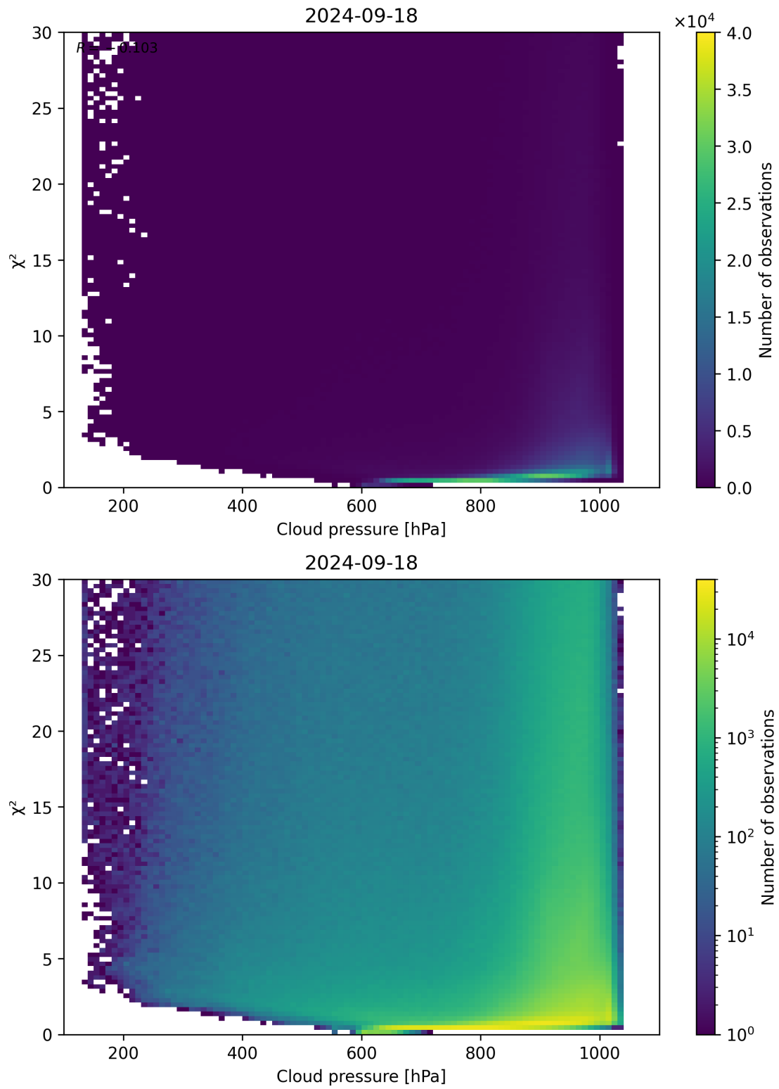
Figure 85: Scatter density plot of “Cloud pressure” against “ \chi^2 ” for 2024-09-17 to 2024-09-19.
