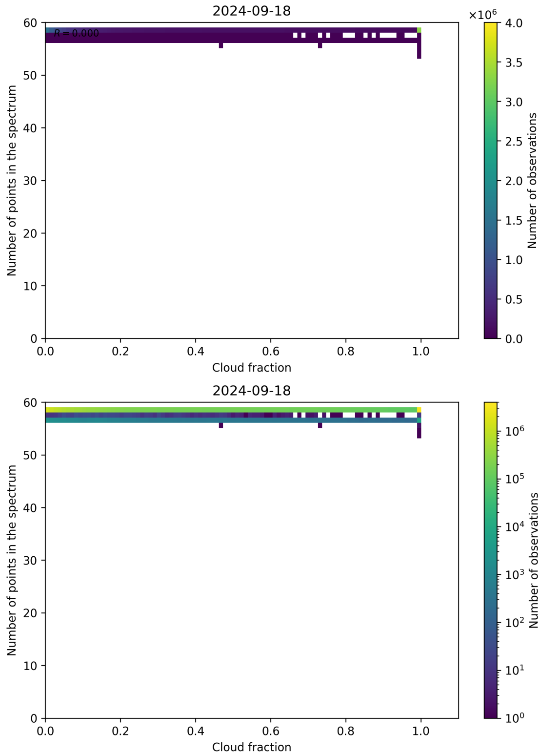
Figure 81: Scatter density plot of “Cloud fraction” against “Number of points in the spectrum” for 2024-09-17 to 2024-09-19.
