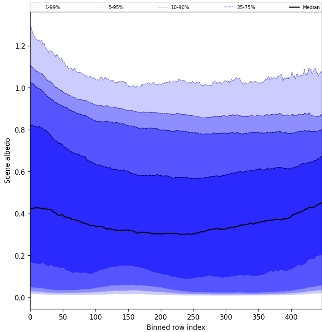
Figure 51: Along track statistics of “Scene albedo” for 2024-09-17 to 2024-09-19
