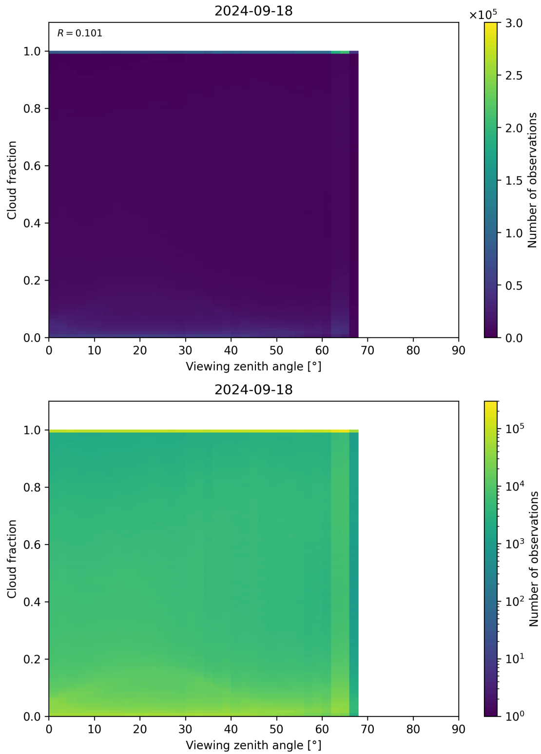
Figure 132: Scatter density plot of “Viewing zenith angle” against “Cloud fraction” for 2024-09-17 to 2024-09-19.
