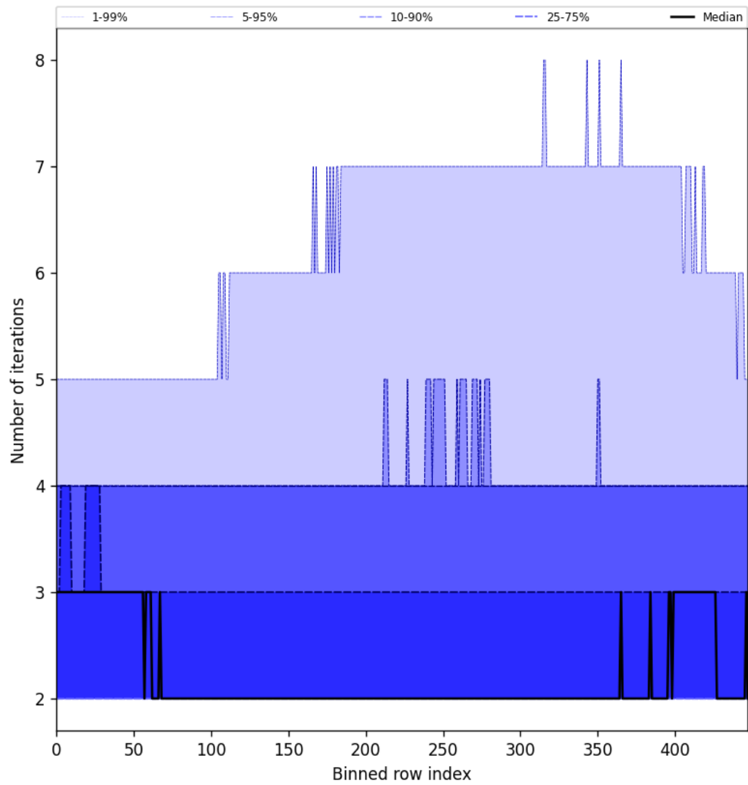
Figure 56: Along track statistics of “Number of iterations” for 2024-09-17 to 2024-09-19
