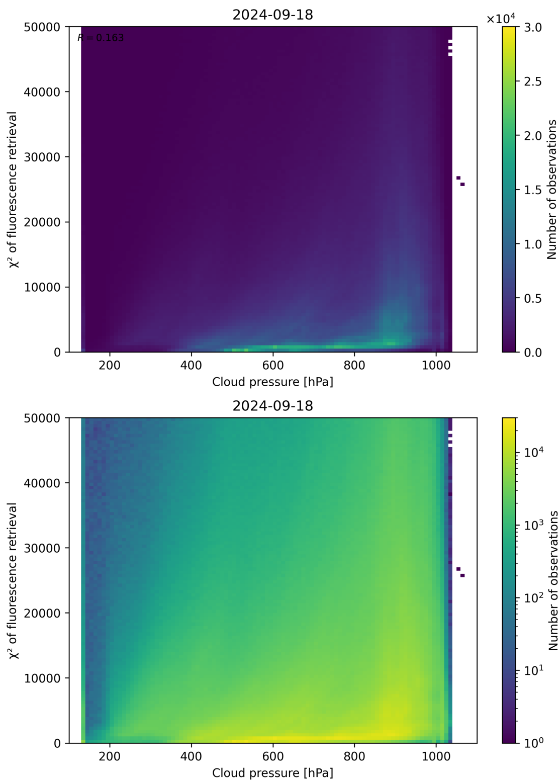
Figure 86: Scatter density plot of “Cloud pressure” against “ \chi^2 of fluorescence retrieval” for 2024-09-17 to 2024-09-19.
