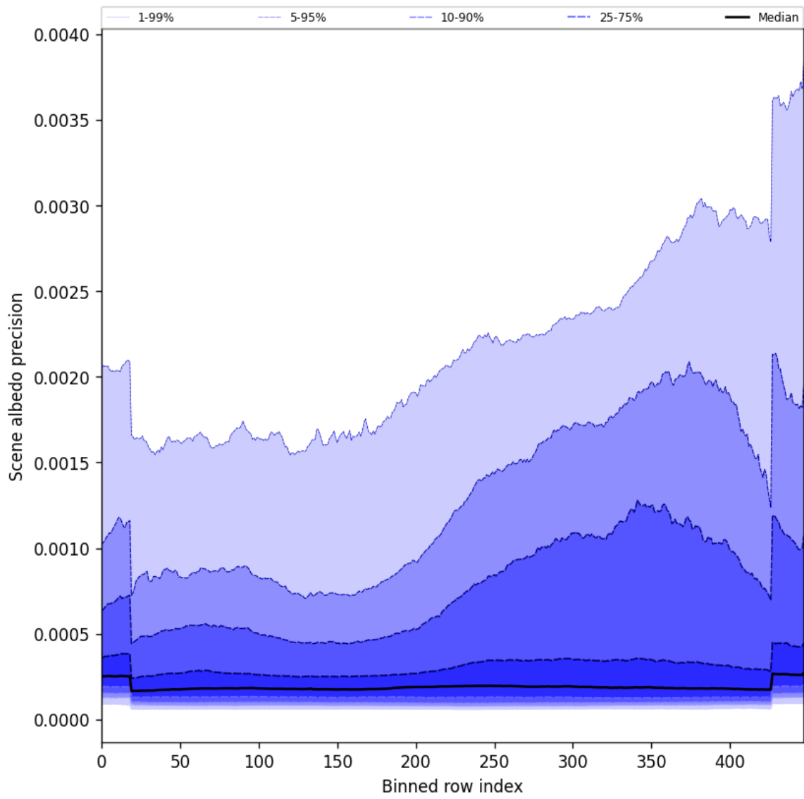
Figure 52: Along track statistics of “Scene albedo precision” for 2024-09-17 to 2024-09-19
