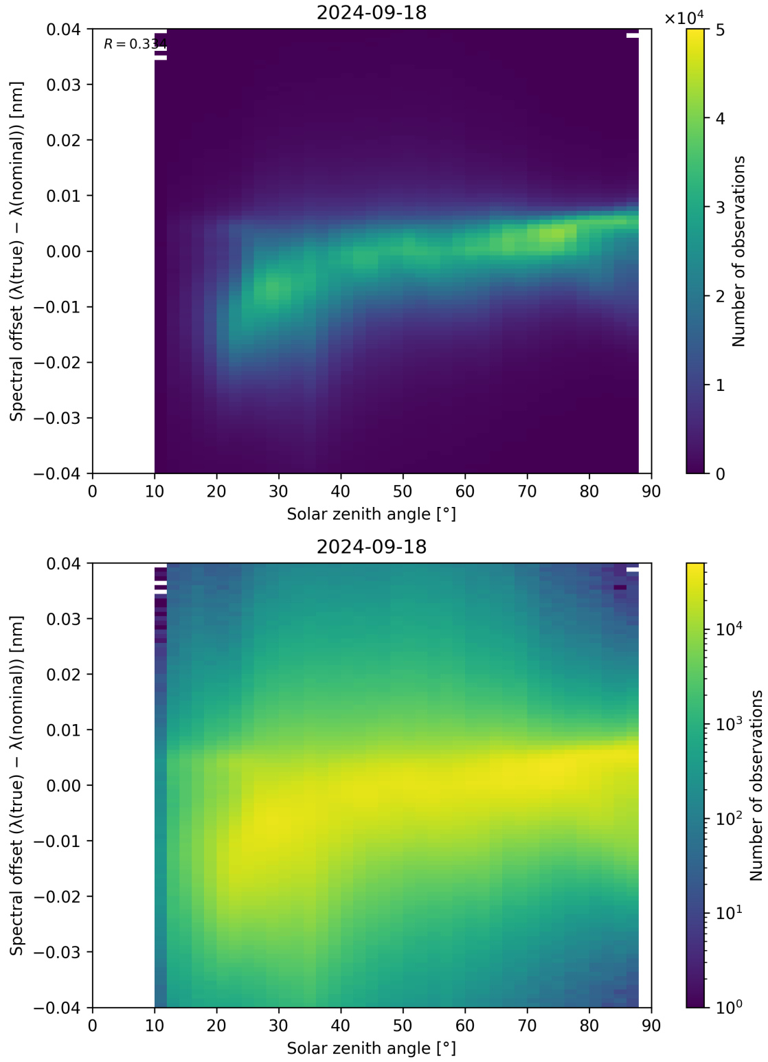
Figure 128: Scatter density plot of “Solar zenith angle” against “Spectral offset ( \lambda_{\text{true}} - \lambda_{\text{nominal}} )” for 2024-09-17 to 2024-09-19.
