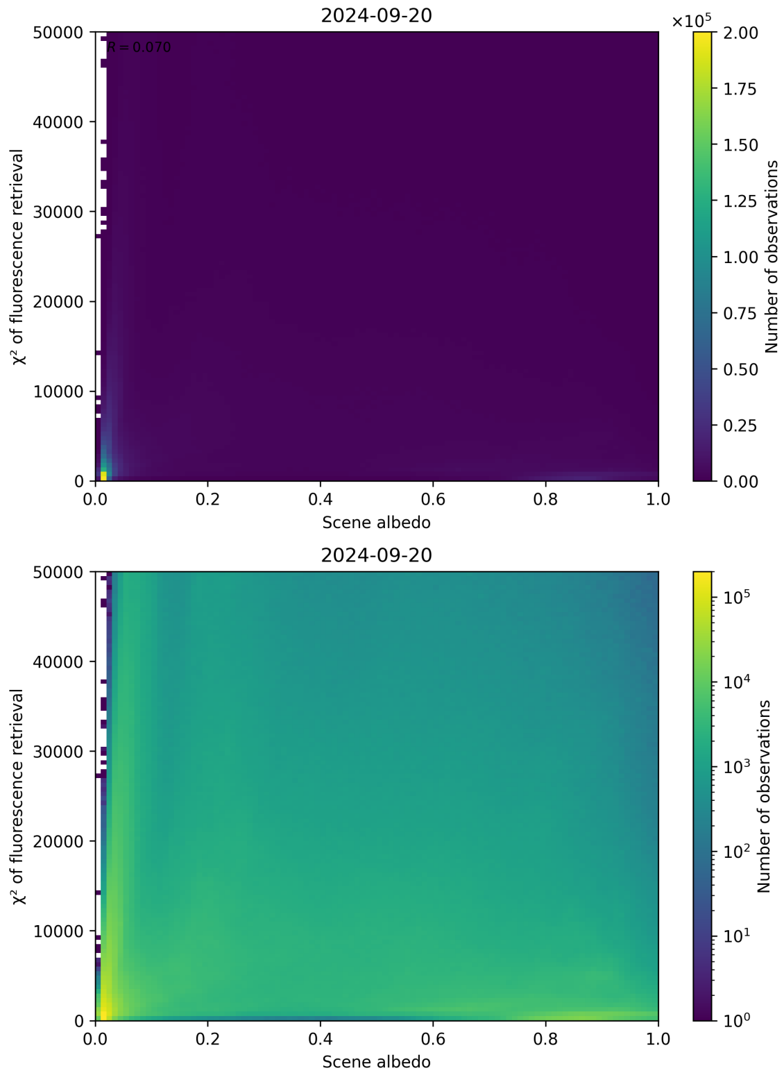
Figure 113: Scatter density plot of “Scene albedo” against “ \chi^2 of fluorescence retrieval” for 2024-09-19 to 2024-09-21.
