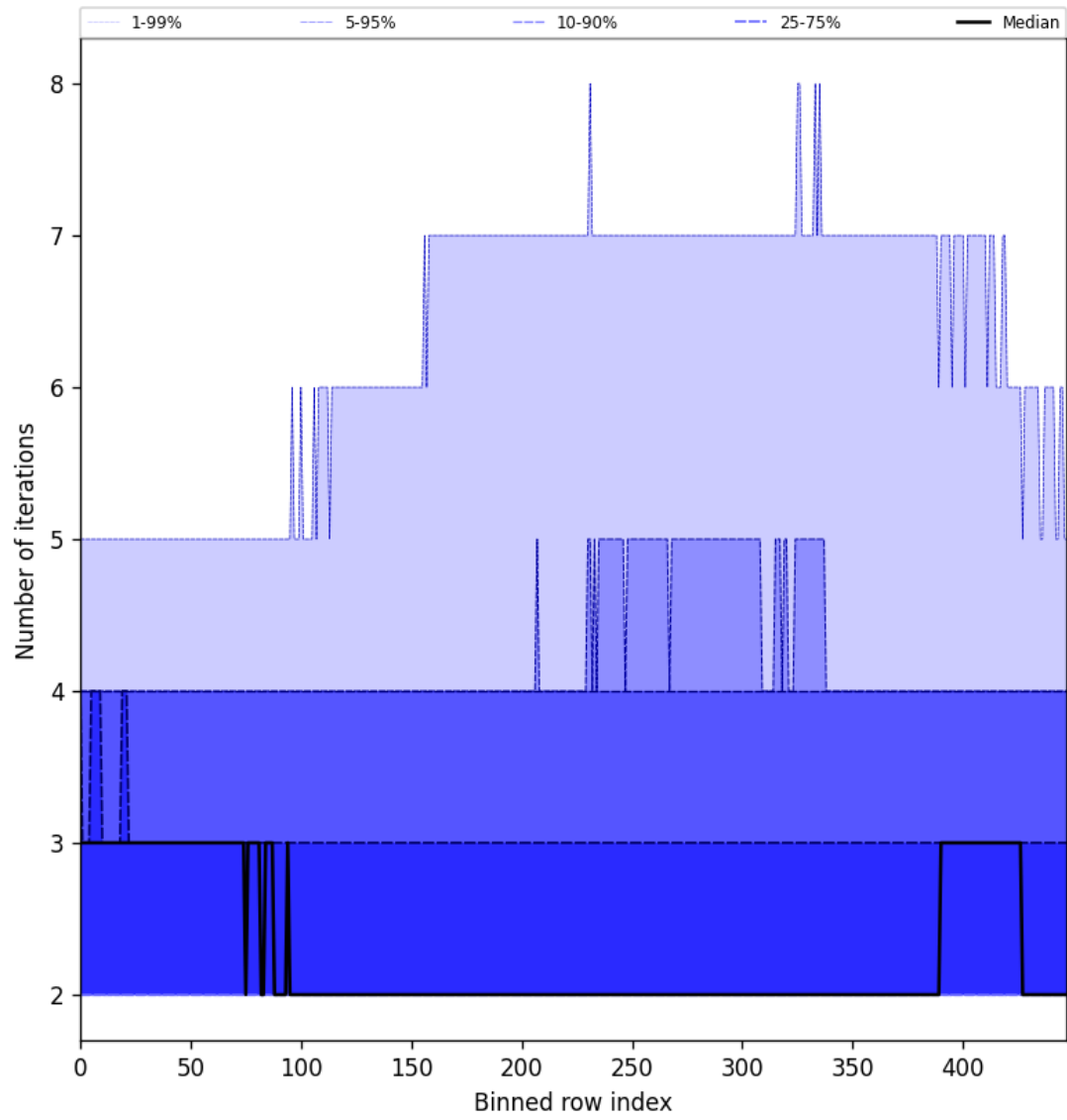
Figure 56: Along track statistics of “Number of iterations” for 2024-09-19 to 2024-09-21
