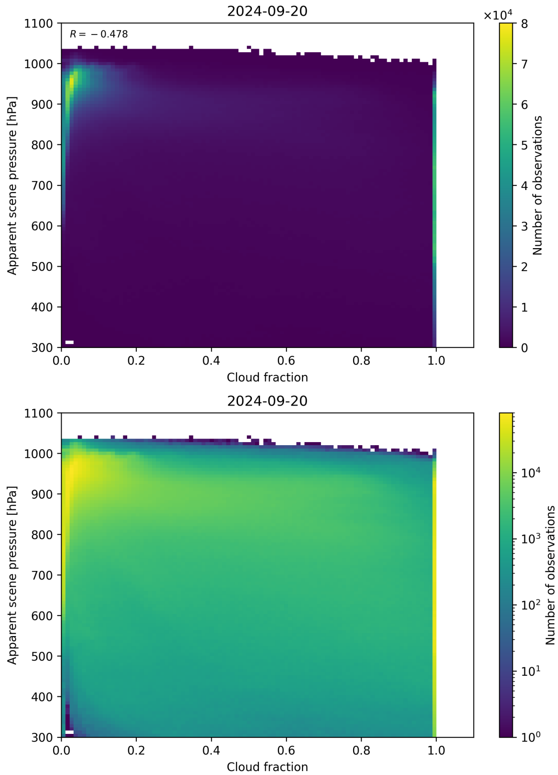
Figure 76: Scatter density plot of “Cloud fraction” against “Apparent scene pressure” for 2024-09-19 to 2024-09-21.
