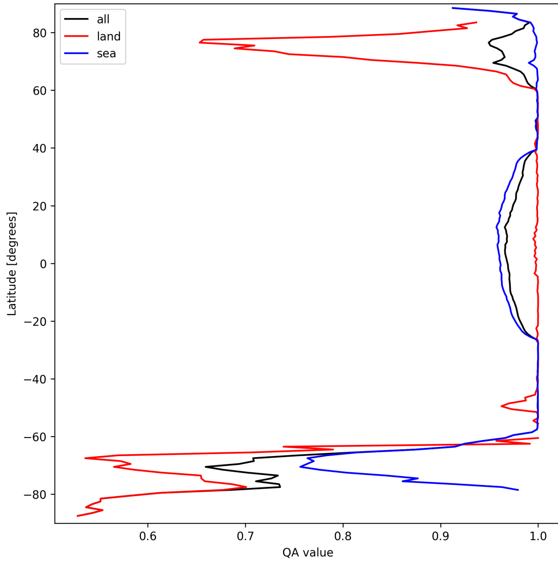
Figure 12: Zonal average of “QA value” for 2024-09-19 to 2024-09-21.
