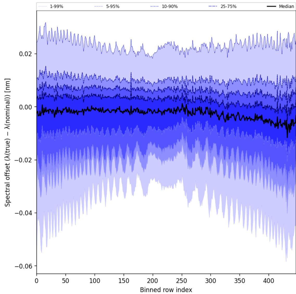
Figure 62: Along track statistics of “Spectral offset ( \lambda_{\text{true}} - \lambda_{\text{nominal}} )” for 2024-09-19 to 2024-09-21
