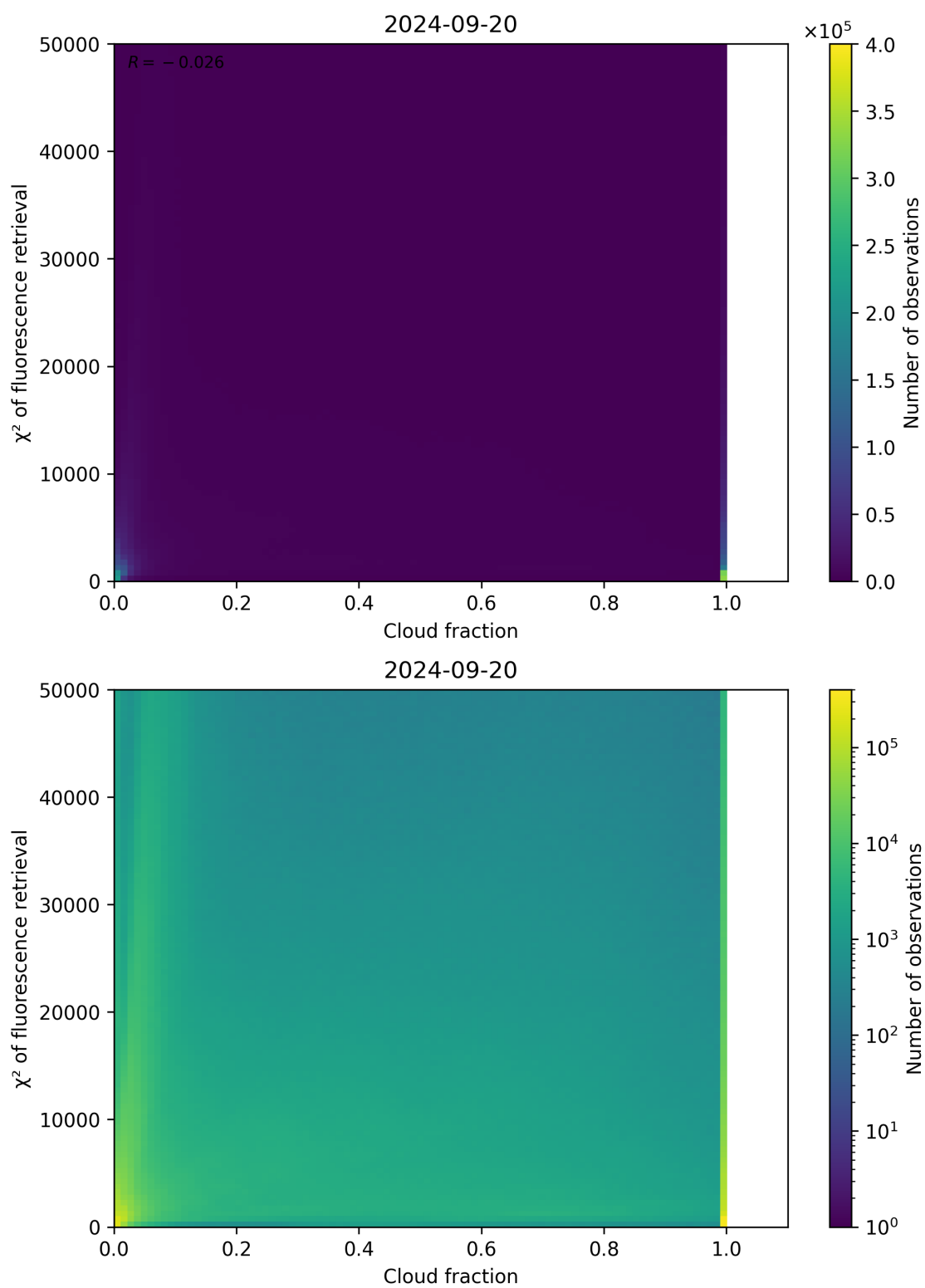
Figure 78: Scatter density plot of “Cloud fraction” against “ \chi^2 of fluorescence retrieval” for 2024-09-19 to 2024-09-21.
