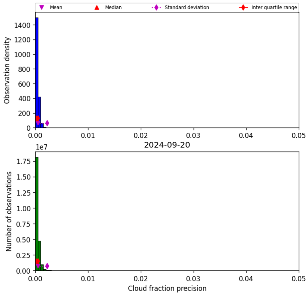
Figure 33: Histogram of “Cloud fraction precision” for 2024-09-19 to 2024-09-21
