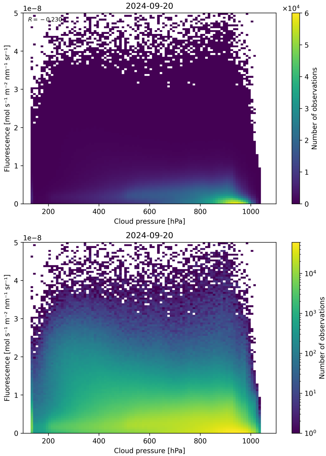
Figure 88: Scatter density plot of “Cloud pressure” against “Fluorescence” for 2024-09-19 to 2024-09-21.
