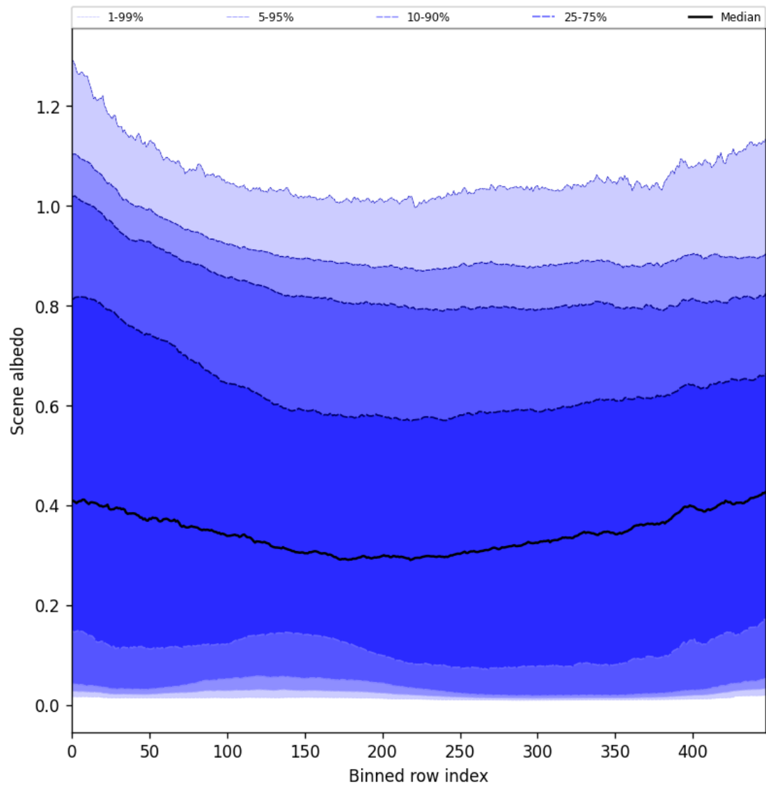
Figure 51: Along track statistics of "Scene albedo" for 2024-09-19 to 2024-09-21
