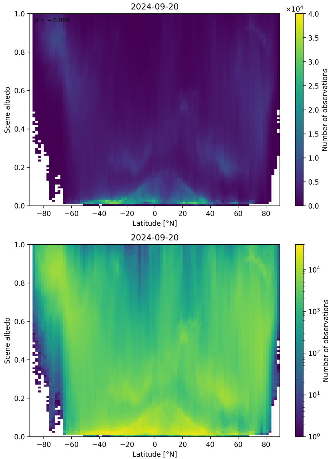
Figure 104: Scatter density plot of “Latitude” against “Scene albedo” for 2024-09-19 to 2024-09-21.
