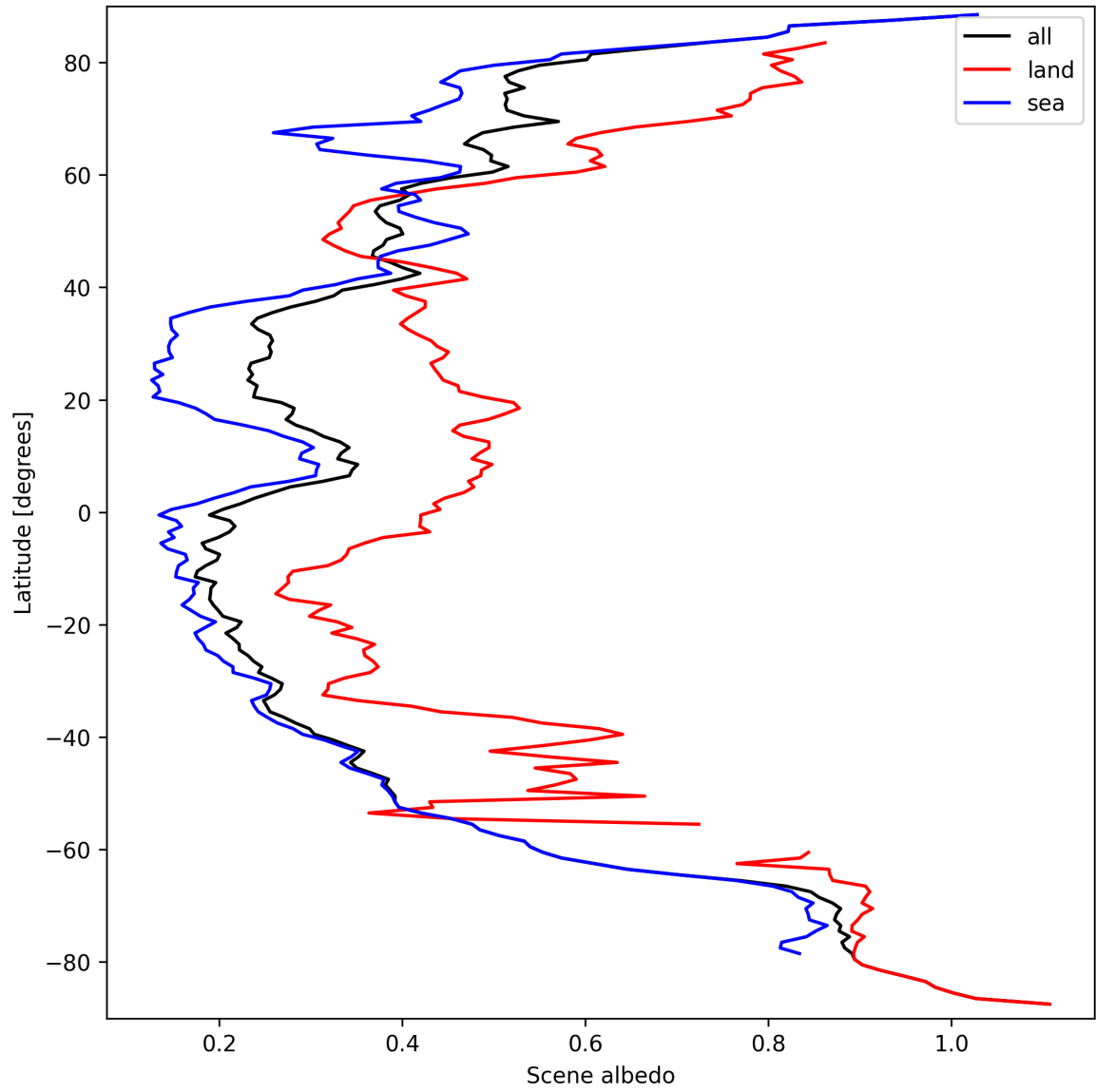
Figure 17: Zonal average of “Scene albedo” for 2024-09-19 to 2024-09-21.
