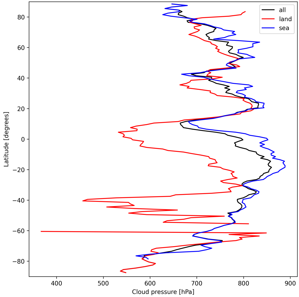
Figure 13: Zonal average of “Cloud pressure” for 2024-09-19 to 2024-09-21.
