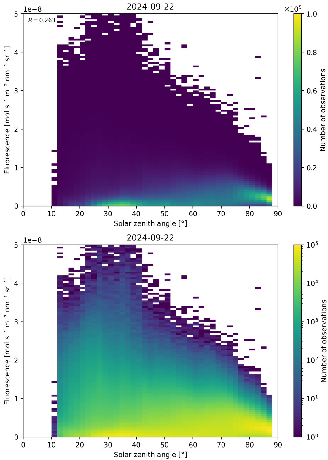
Figure 123: Scatter density plot of “Solar zenith angle” against “Fluorescence” for 2024-09-22 to 2024-09-23.
