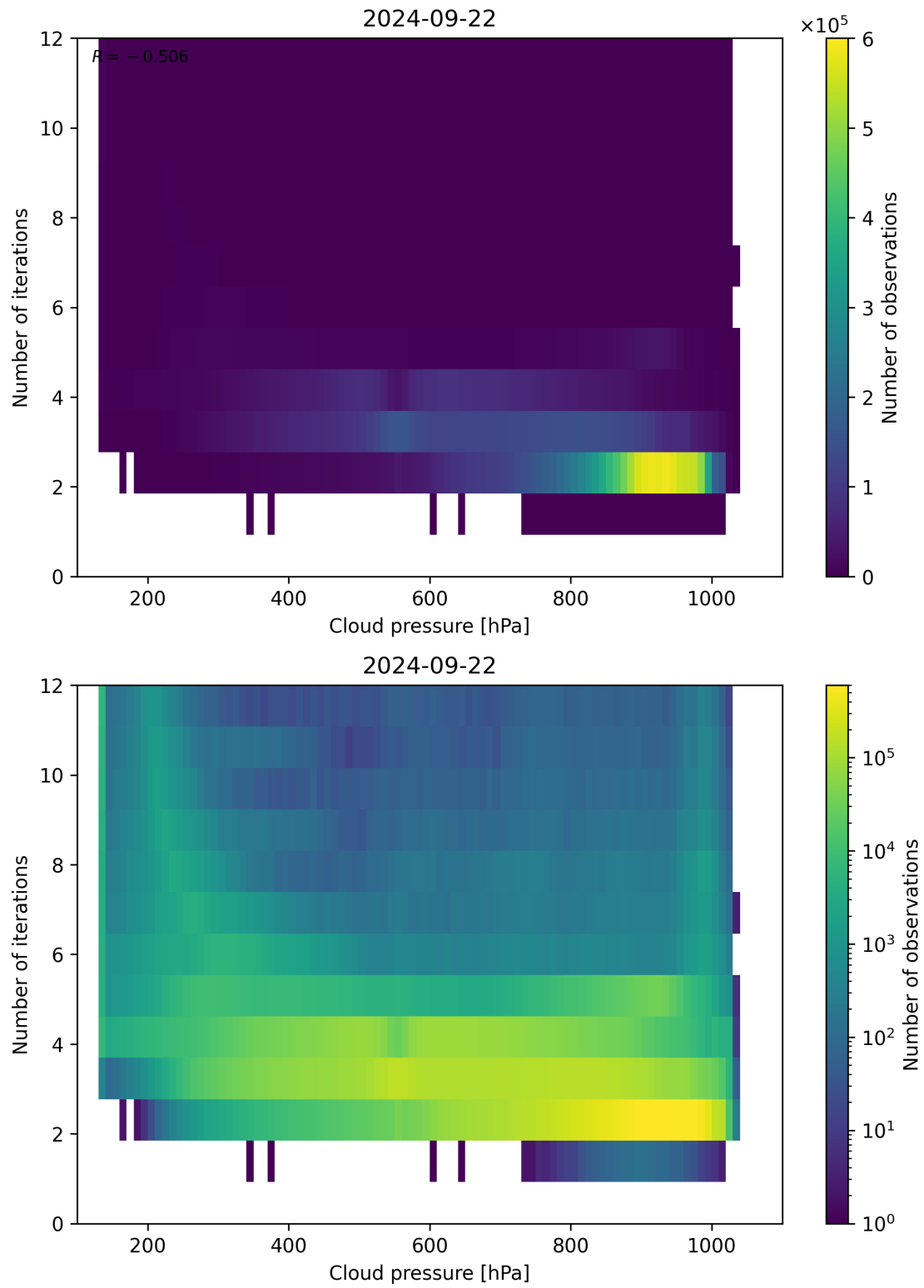
Figure 89: Scatter density plot of “Cloud pressure” against “Number of iterations” for 2024-09-22 to 2024-09-23.
