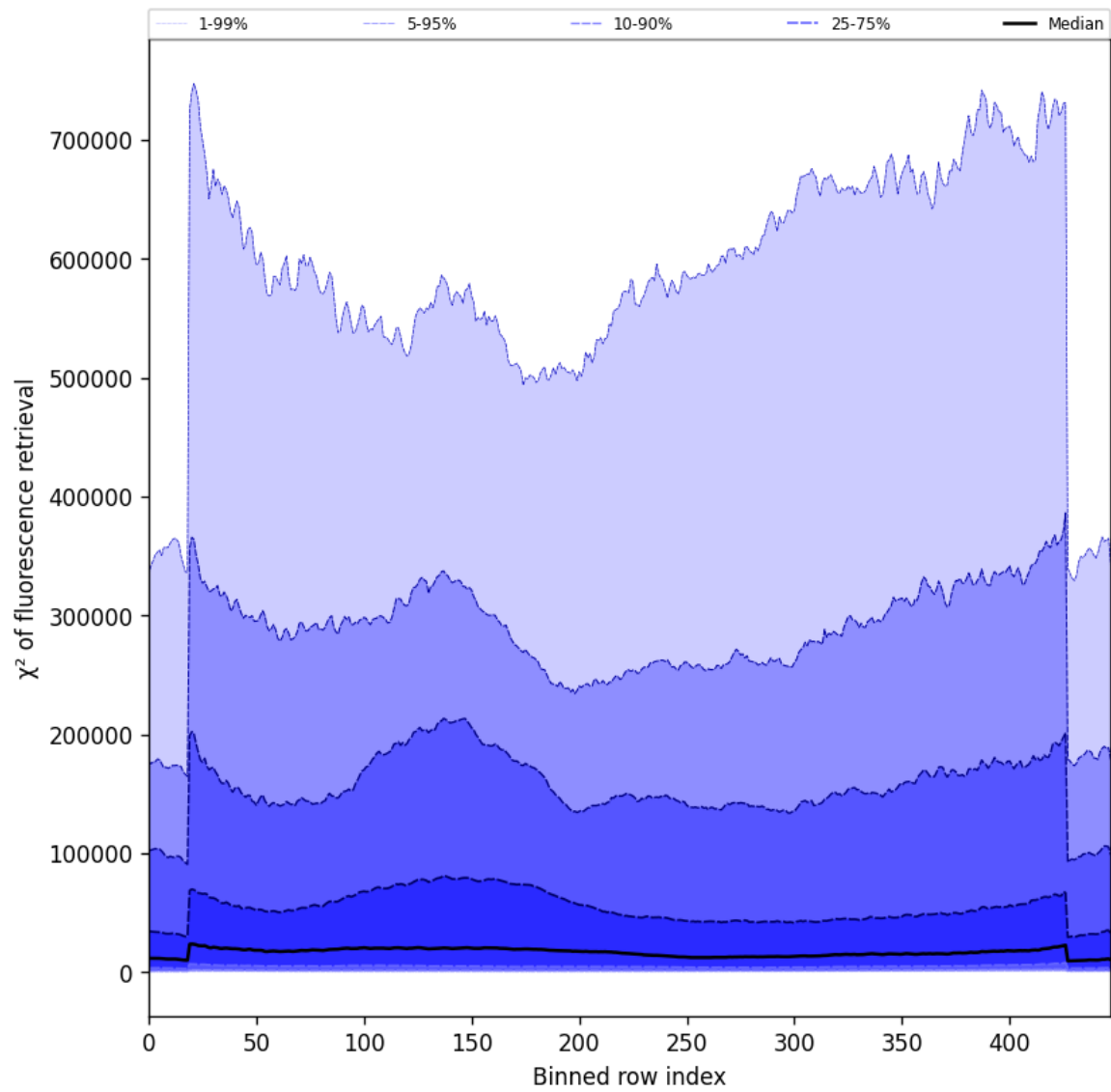
Figure 59: Along track statistics of “ \chi^2 of fluorescence retrieval” for 2024-09-22 to 2024-09-23
