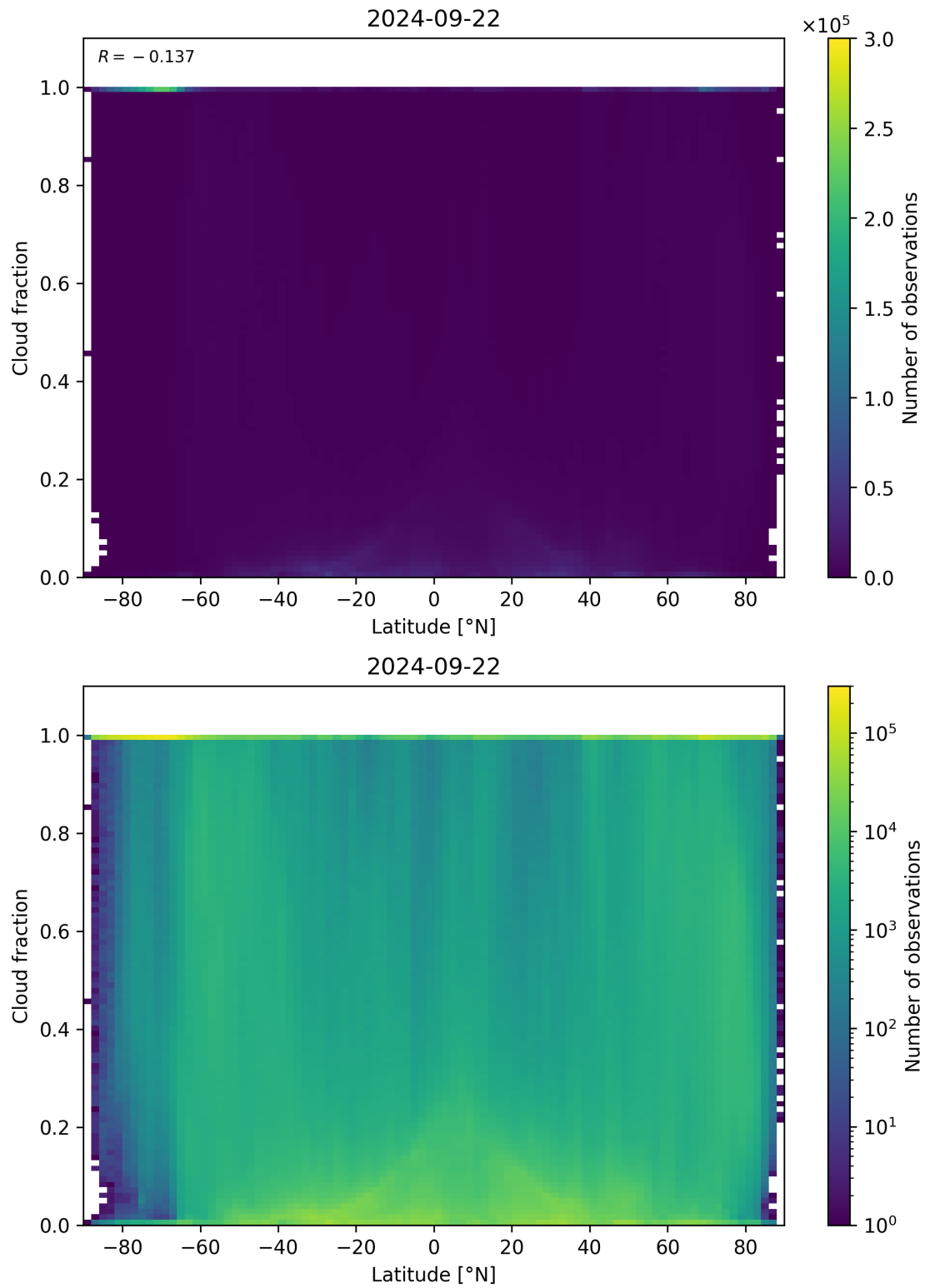
Figure 99: Scatter density plot of “Latitude” against “Cloud fraction” for 2024-09-22 to 2024-09-23.
