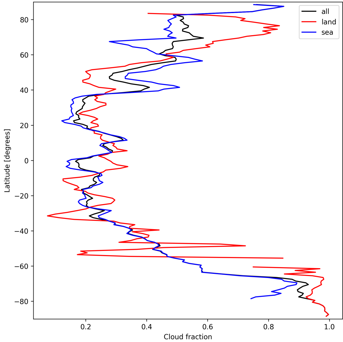
Figure 15: Zonal average of “Cloud fraction” for 2024-09-22 to 2024-09-23.
