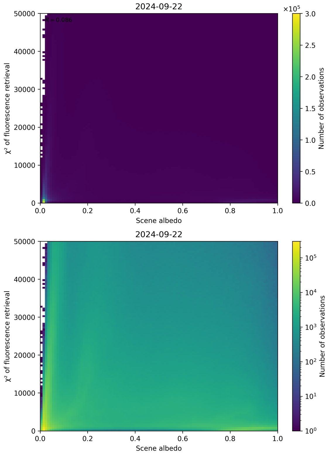
Figure 113: Scatter density plot of “Scene albedo” against “ \chi^2 of fluorescence retrieval” for 2024-09-22 to 2024-09-23.
