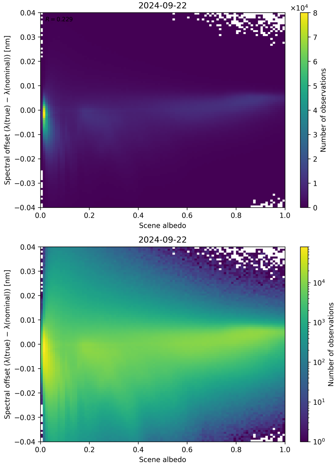
Figure 117: Scatter density plot of “Scene albedo” against “Spectral offset ( \lambda_{\text{true}} - \lambda_{\text{nominal}} )” for 2024-09-22 to 2024-09-23.
