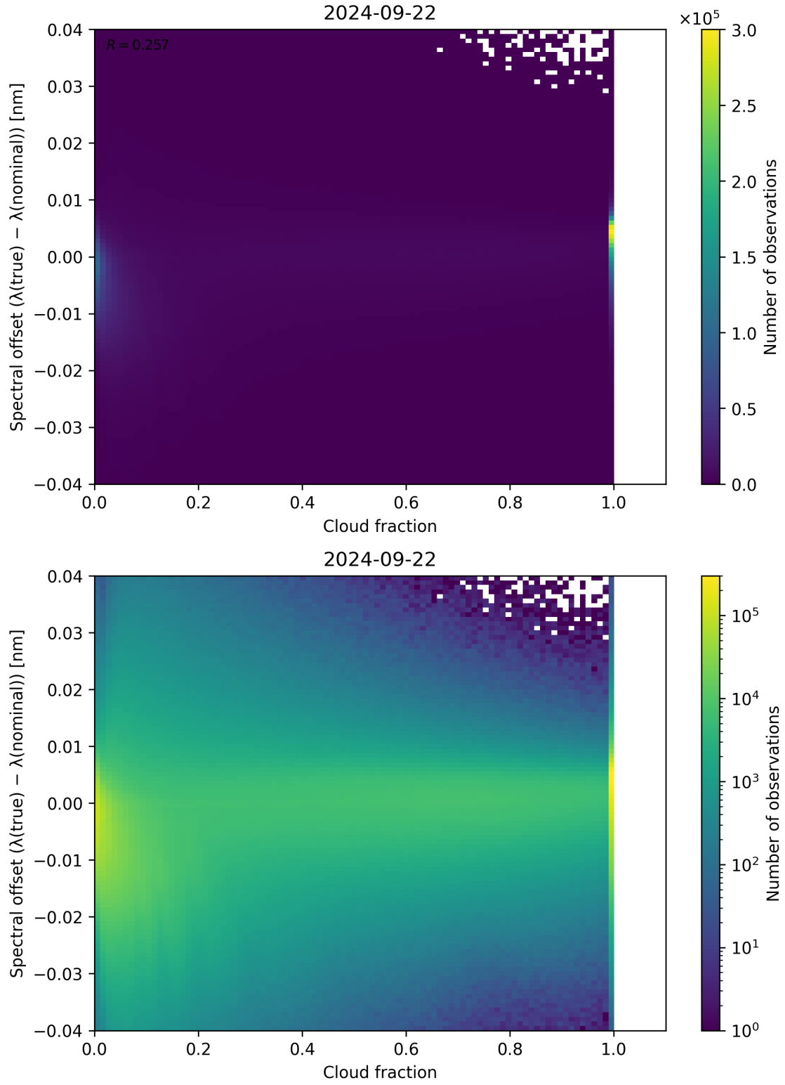
Figure 83: Scatter density plot of “Cloud fraction” against “Spectral offset ( \lambda_{\text{true}} - \lambda_{\text{nominal}} )” for 2024-09-22 to 2024-09-23.
