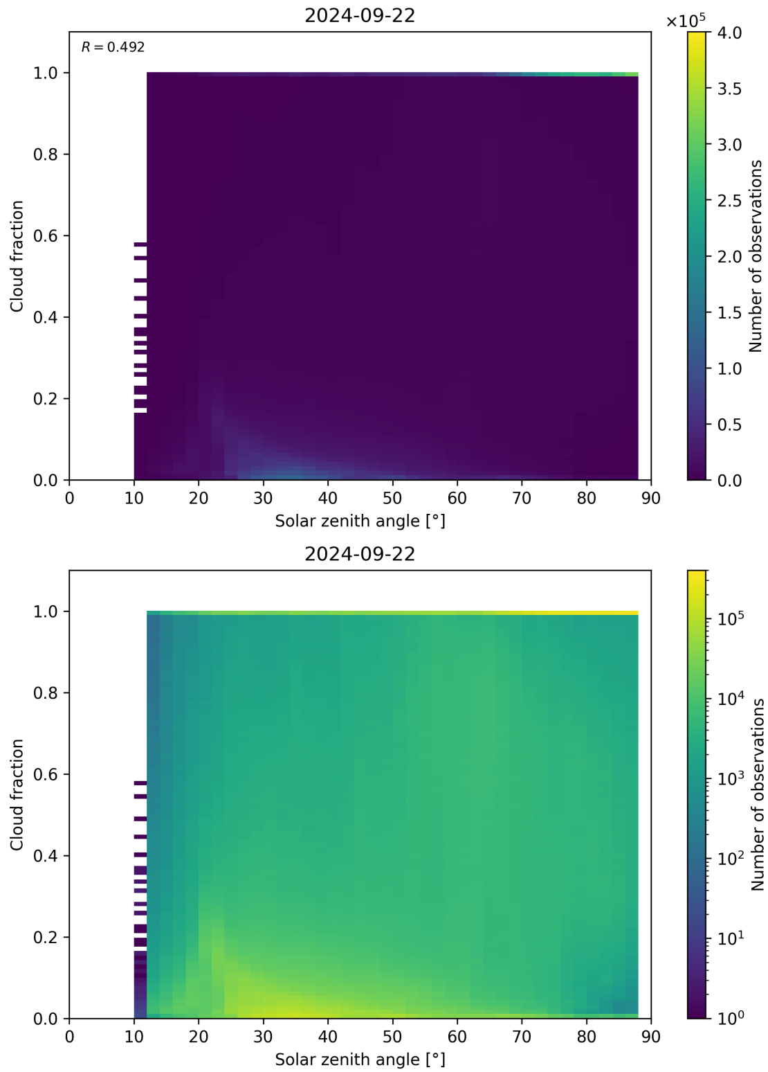
Figure 121: Scatter density plot of “Solar zenith angle” against “Cloud fraction” for 2024-09-22 to 2024-09-23.
