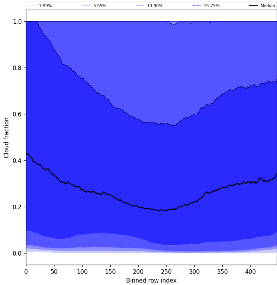
Figure 49: Along track statistics of “Cloud fraction” for 2024-09-22 to 2024-09-23
