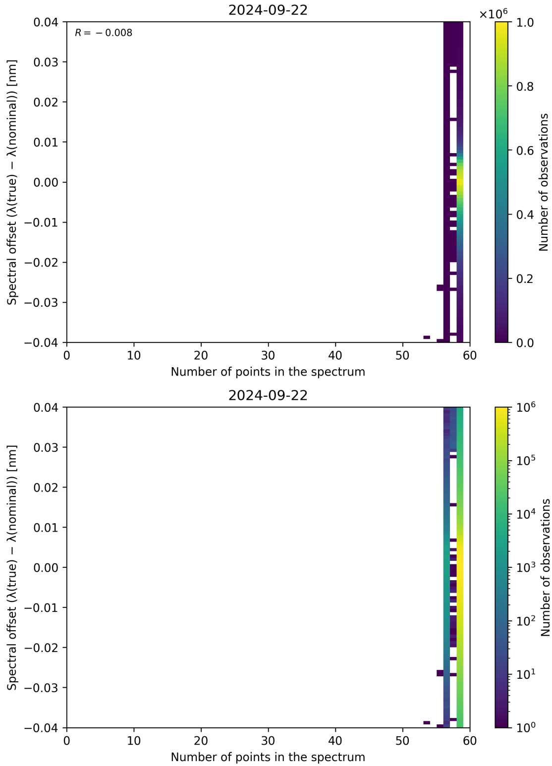
Figure 110: Scatter density plot of “Number of points in the spectrum” against “Spectral offset ( \lambda_{\text{true}} - \lambda_{\text{nominal}} )” for 2024-09-22 to 2024-09-23.
