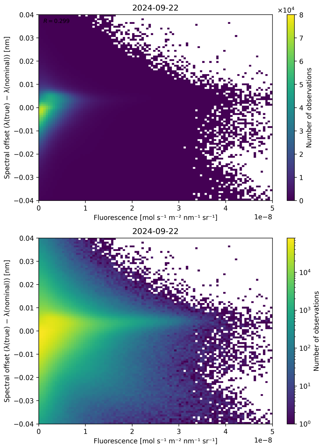
Figure 95: Scatter density plot of “Fluorescence” against “Spectral offset ( \lambda_{\text{true}} - \lambda_{\text{nominal}} )” for 2024-09-22 to 2024-09-23.
