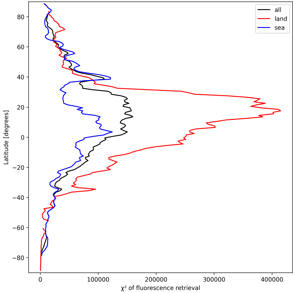
Figure 25: Zonal average of “ \chi^2 of fluorescence retrieval” for 2024-09-22 to 2024-09-23.
