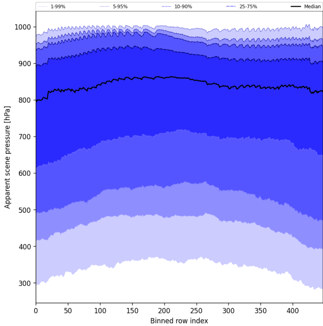
Figure 53: Along track statistics of “Apparent scene pressure” for 2024-09-22 to 2024-09-23
