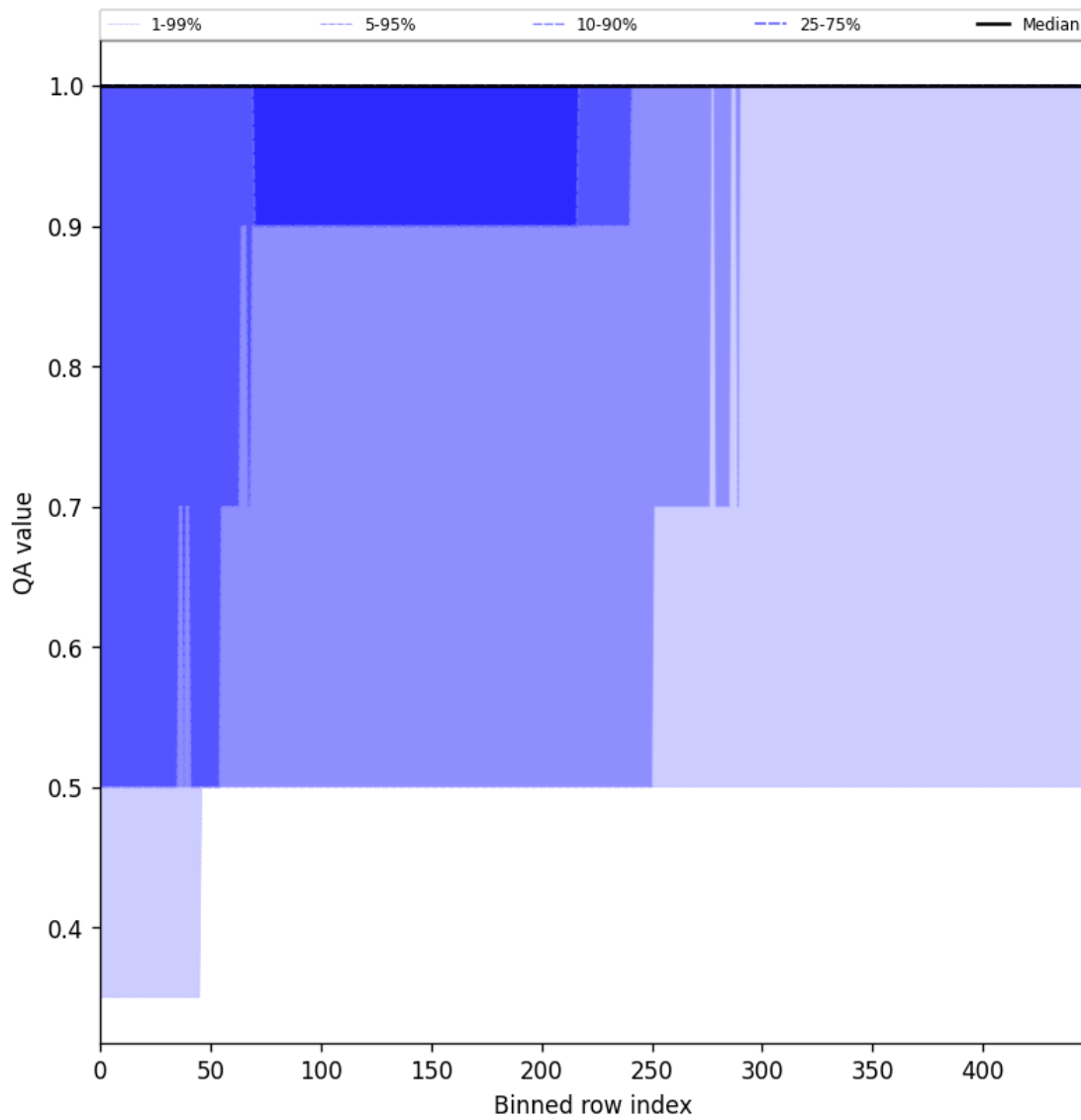
Figure 46: Along track statistics of “QA value” for 2024-09-22 to 2024-09-23
