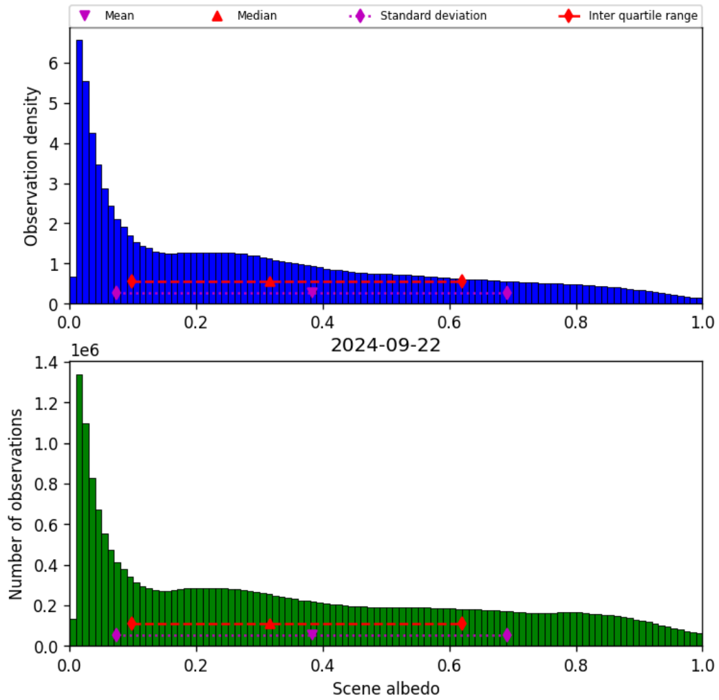
Figure 34: Histogram of “Scene albedo” for 2024-09-22 to 2024-09-23
