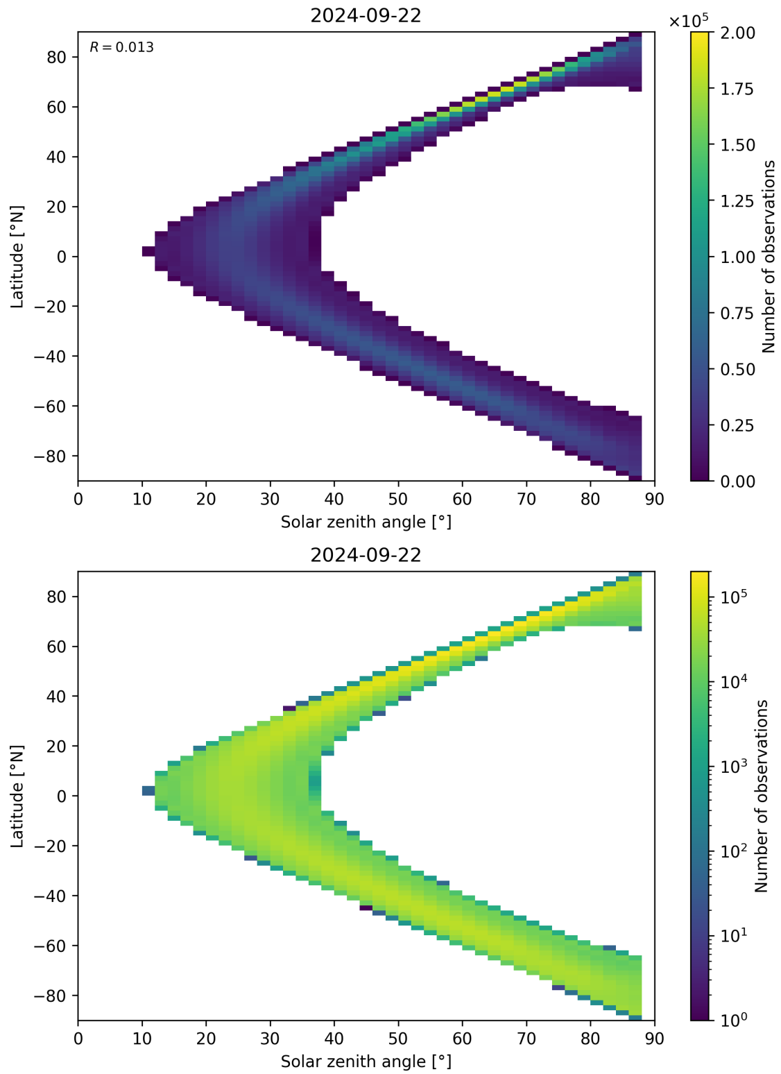
Figure 124: Scatter density plot of “Solar zenith angle” against “Latitude” for 2024-09-22 to 2024-09-23.
