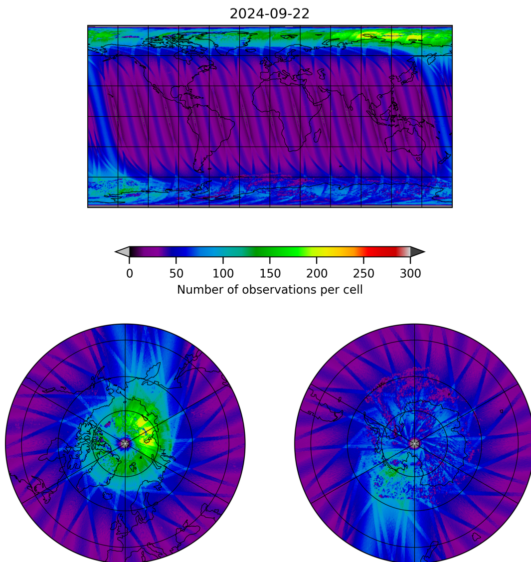
Figure 11: Map of the number of observations for 2024-09-22 to 2024-09-23
