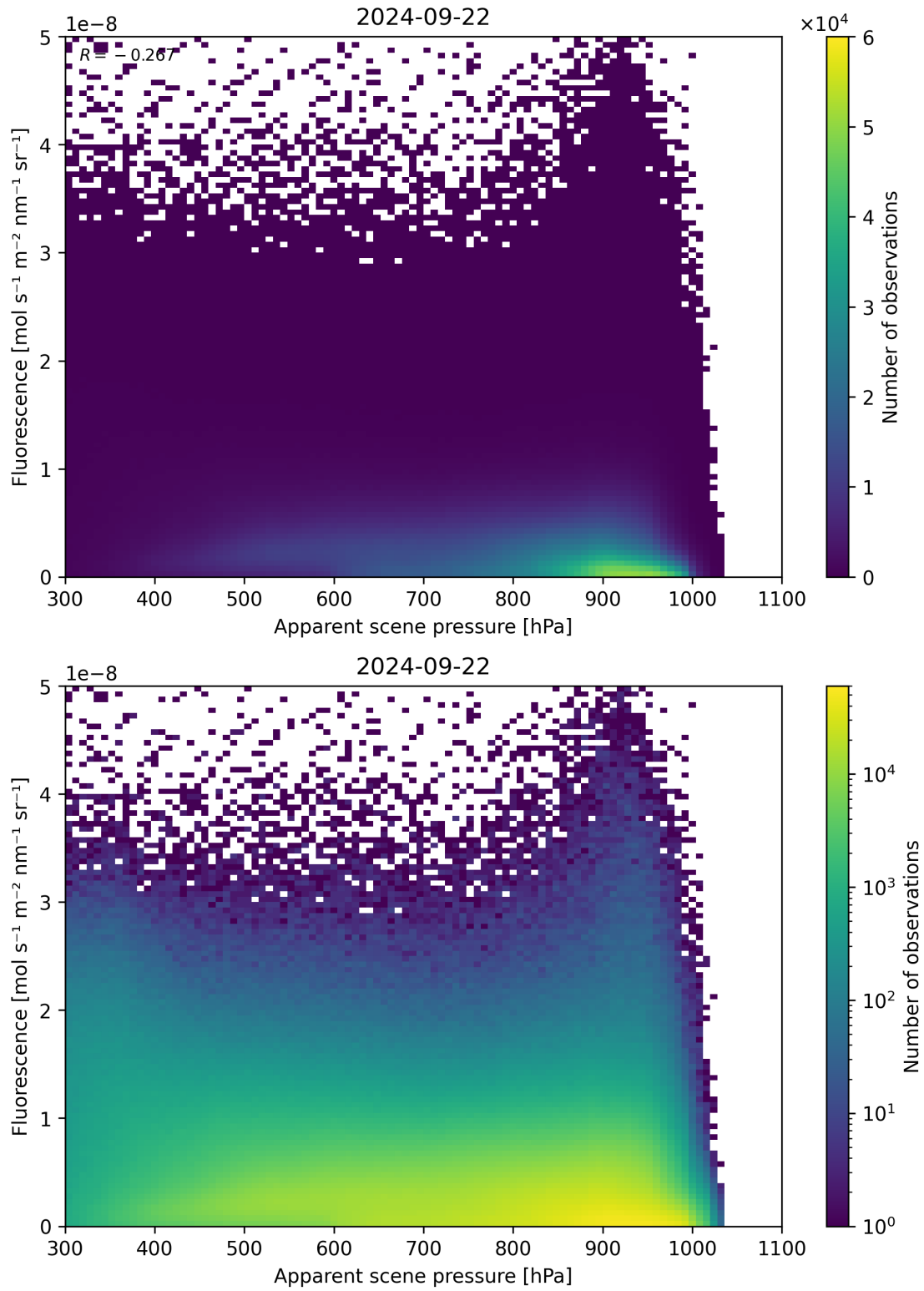
Figure 65: Scatter density plot of “Apparent scene pressure” against “Fluorescence” for 2024-09-22 to 2024-09-23.
