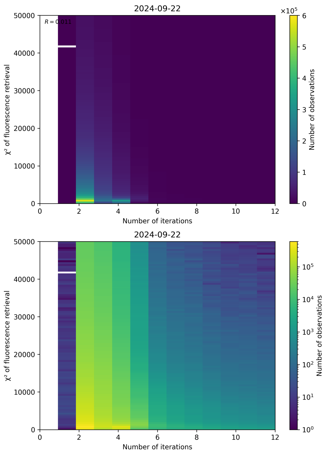
Figure 106: Scatter density plot of “Number of iterations” against “ \chi^2 of fluorescence retrieval” for 2024-09-22 to 2024-09-23.
