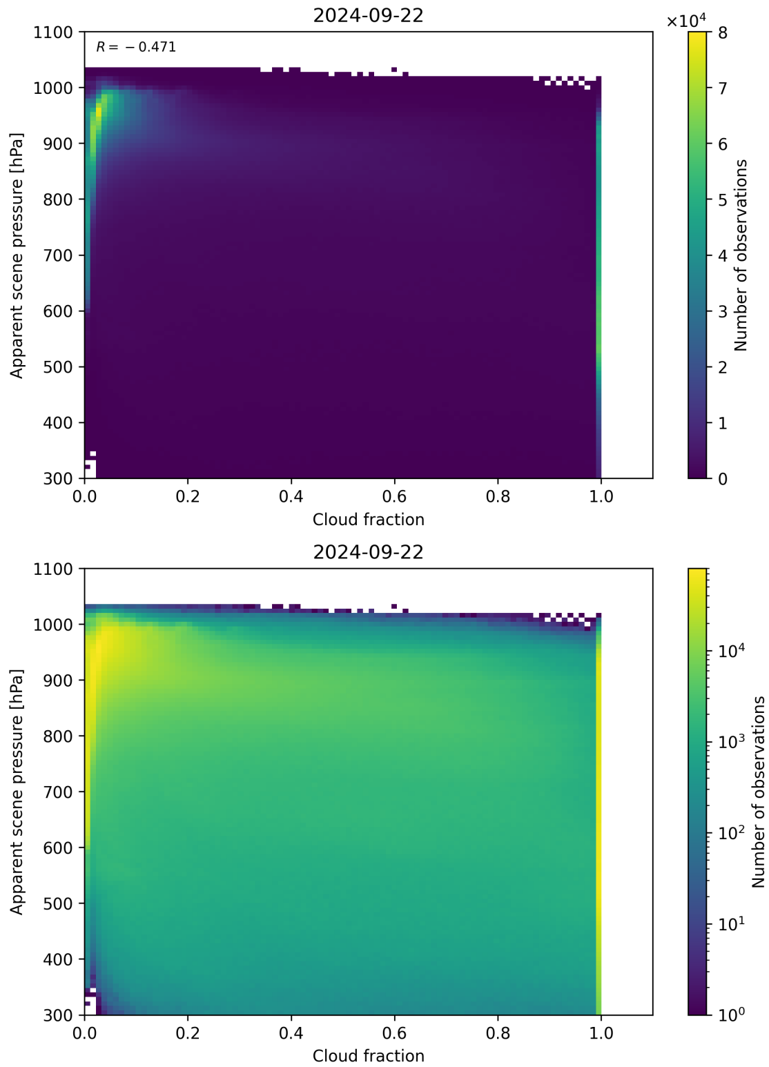
Figure 76: Scatter density plot of “Cloud fraction” against “Apparent scene pressure” for 2024-09-22 to 2024-09-23.
