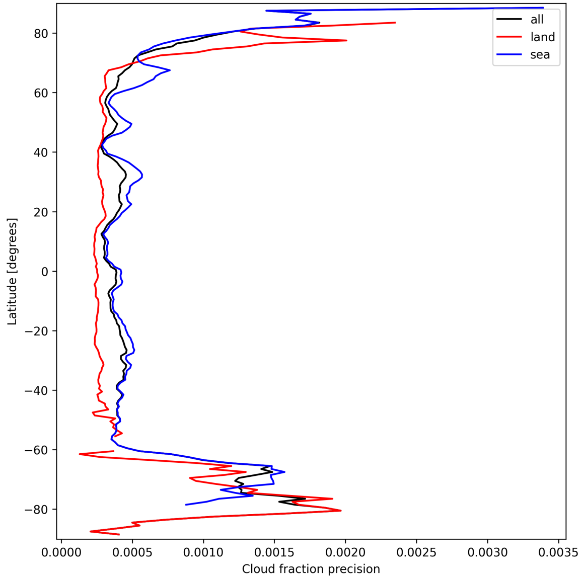
Figure 16: Zonal average of “Cloud fraction precision” for 2024-09-22 to 2024-09-23.
