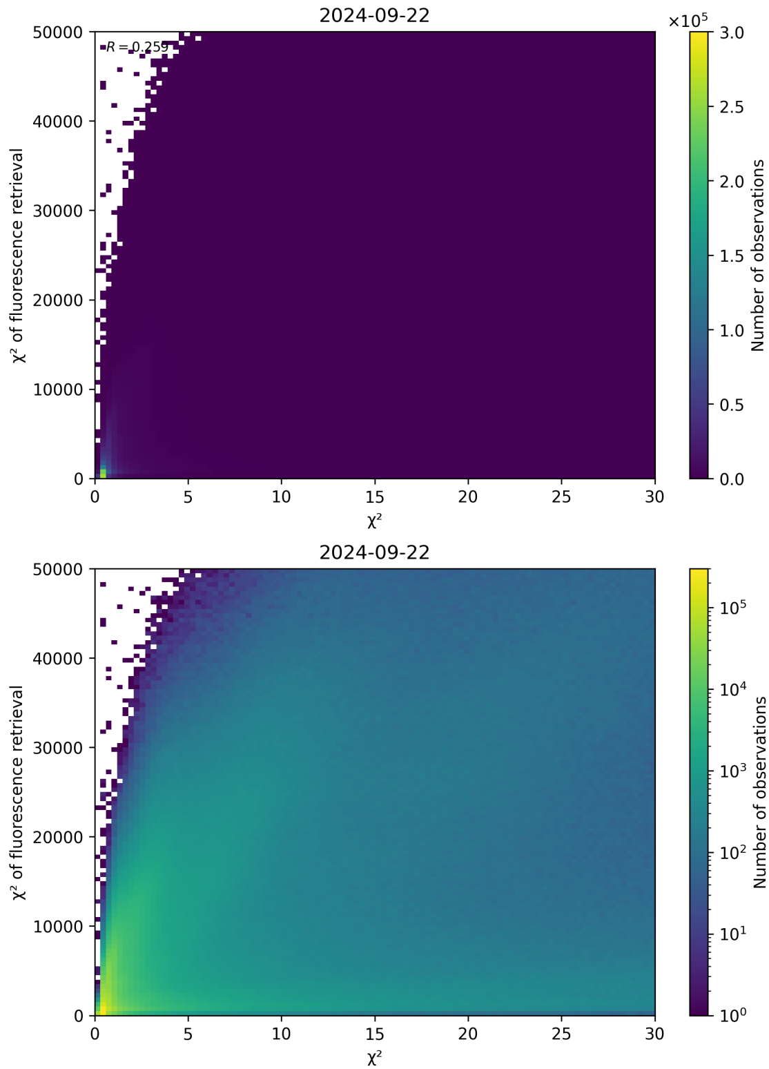
Figure 69: Scatter density plot of “ \chi^2 ” against “ \chi^2 of fluorescence retrieval” for 2024-09-22 to 2024-09-23.
