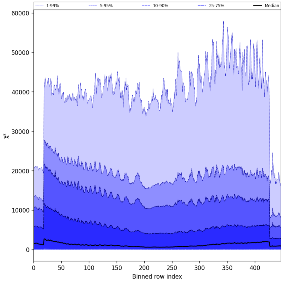
Figure 55: Along track statistics of “ \chi^2 ” for 2024-09-22 to 2024-09-23
