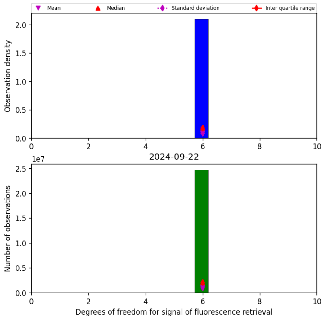
Figure 43: Histogram of “Degrees of freedom for signal of fluorescence retrieval” for 2024-09-22 to 2024-09-23
