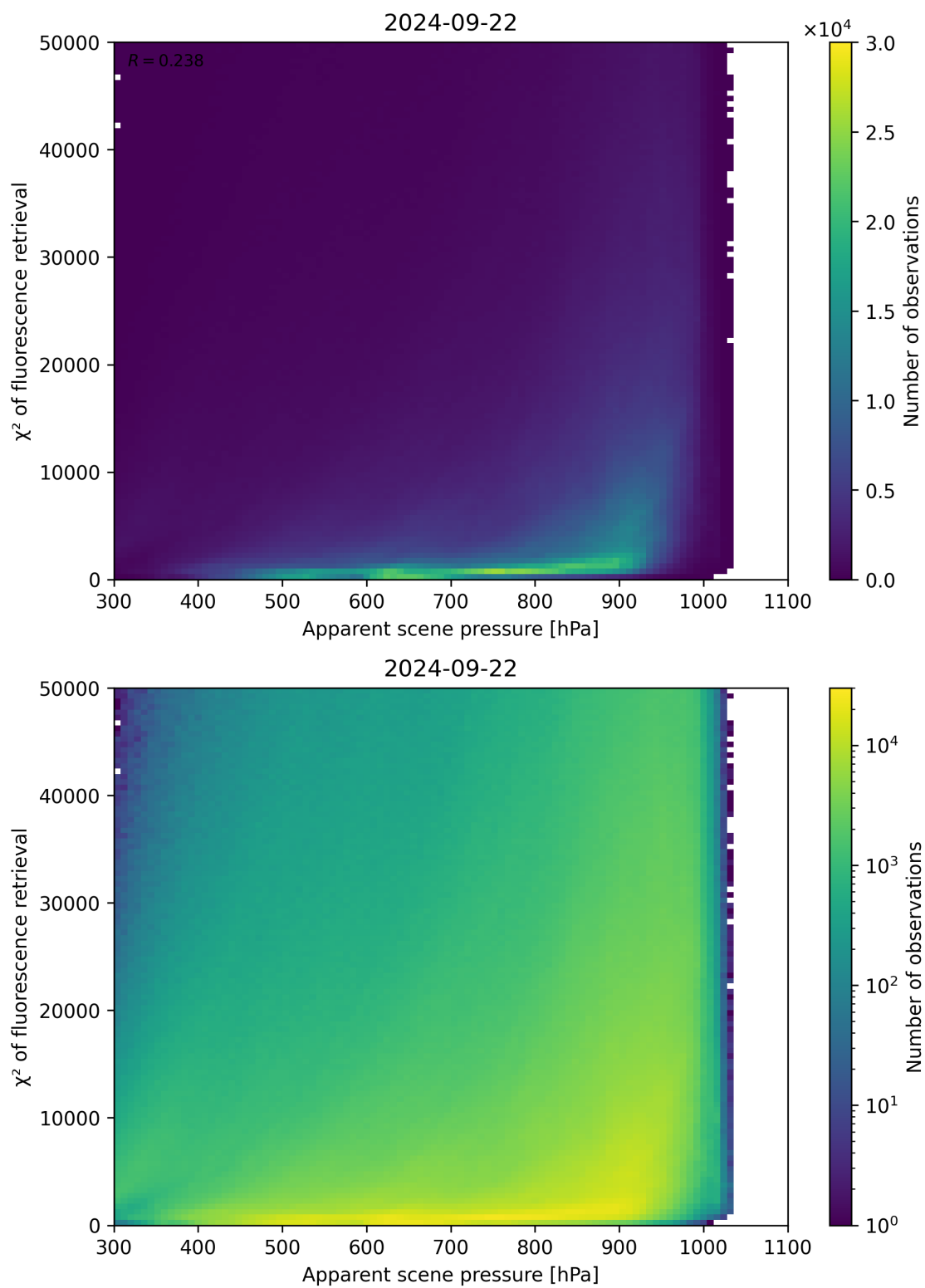
Figure 64: Scatter density plot of “Apparent scene pressure” against “ \chi^2 of fluorescence retrieval” for 2024-09-22 to 2024-09-23.
