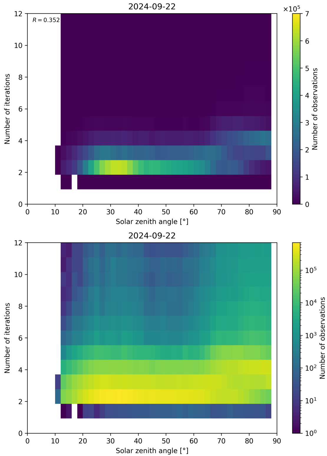
Figure 125: Scatter density plot of “Solar zenith angle” against “Number of iterations” for 2024-09-22 to 2024-09-23.
