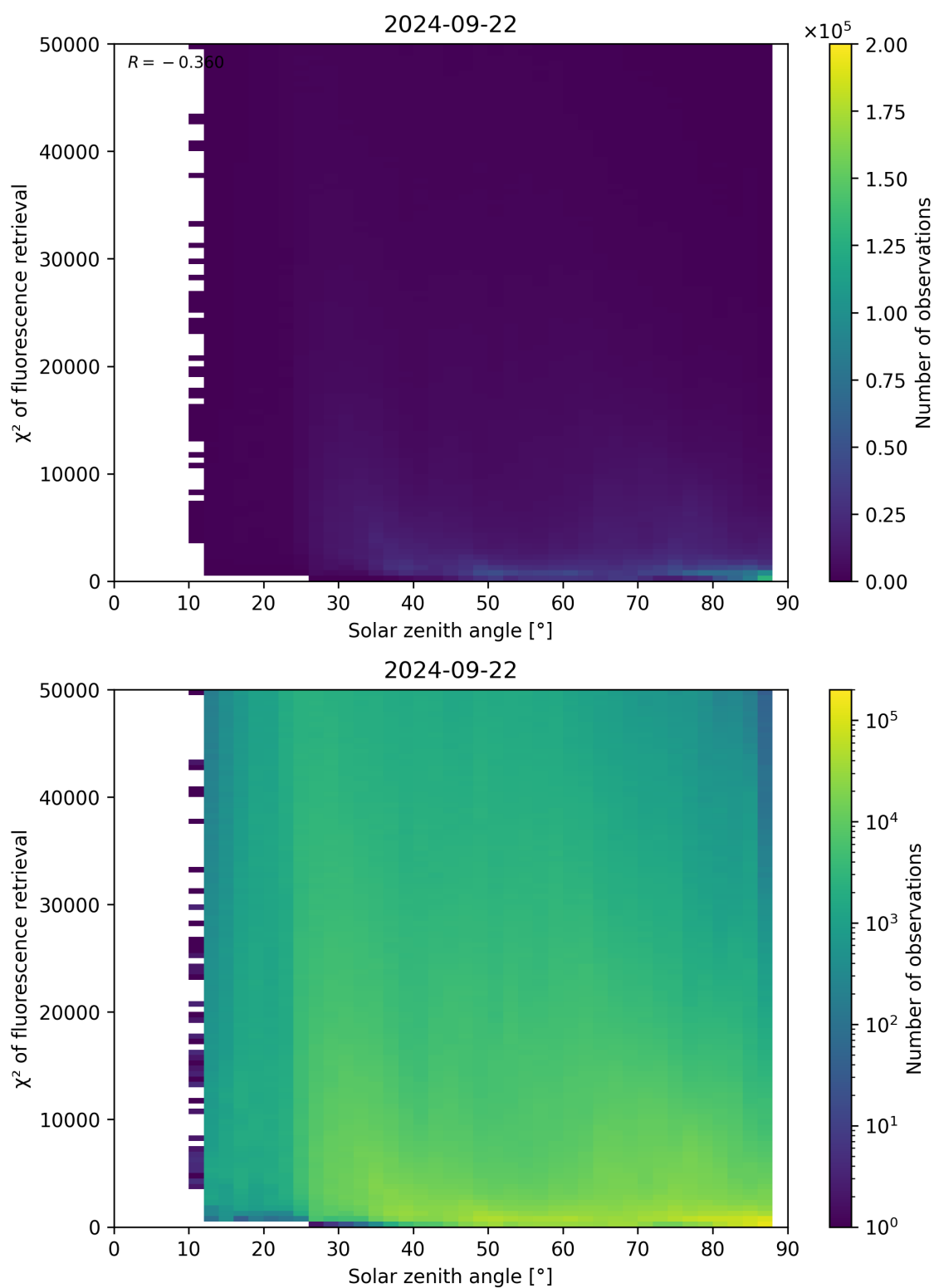
Figure 120: Scatter density plot of “Solar zenith angle” against “ \chi^2 of fluorescence retrieval” for 2024-09-22 to 2024-09-23.
