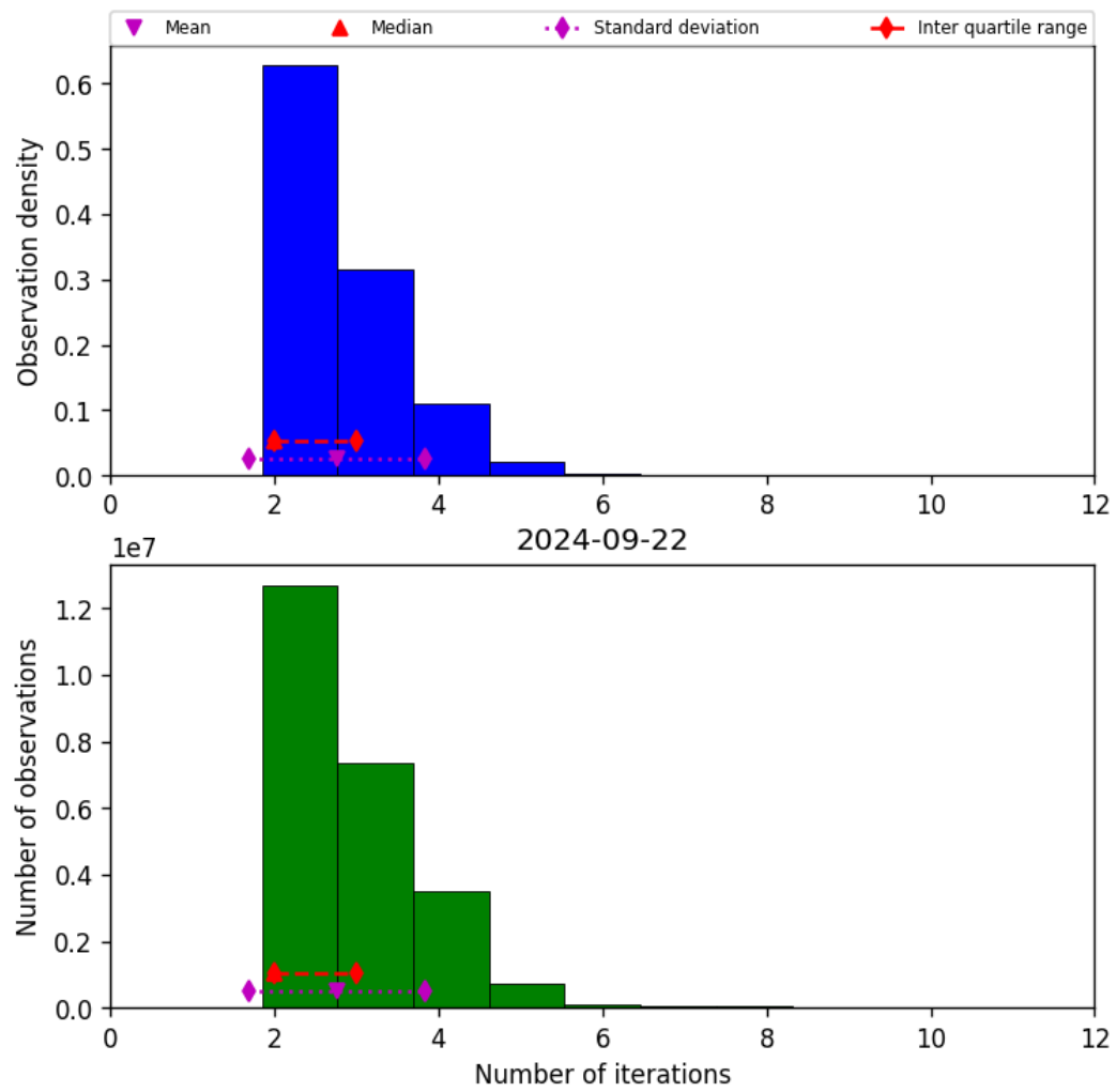
Figure 39: Histogram of “Number of iterations” for 2024-09-22 to 2024-09-23
