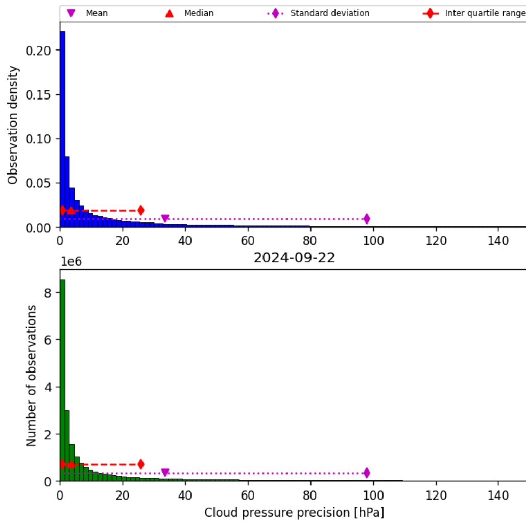
Figure 31: Histogram of “Cloud pressure precision” for 2024-09-22 to 2024-09-23
