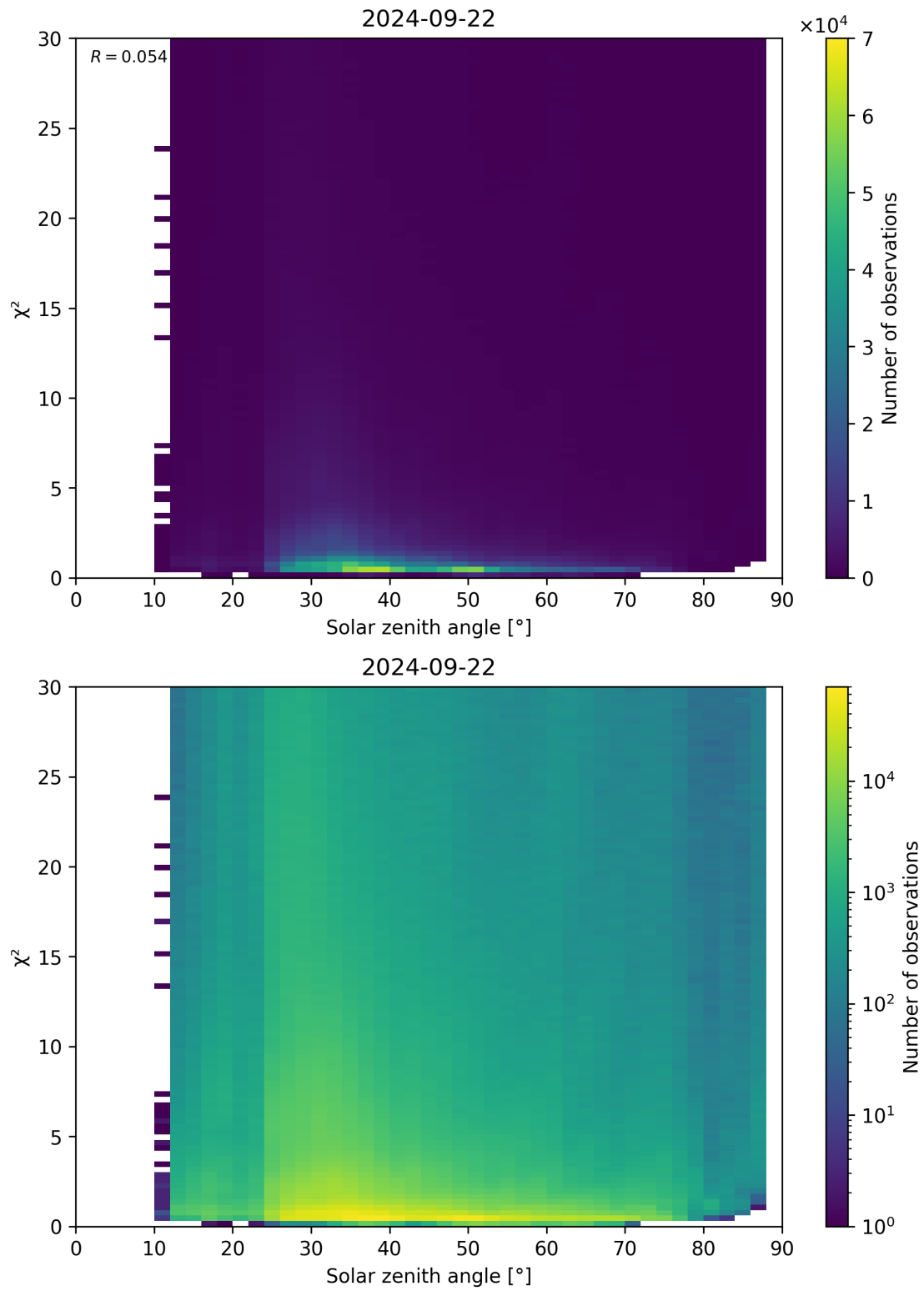
Figure 119: Scatter density plot of “Solar zenith angle” against “ \chi^2 ” for 2024-09-22 to 2024-09-23.
