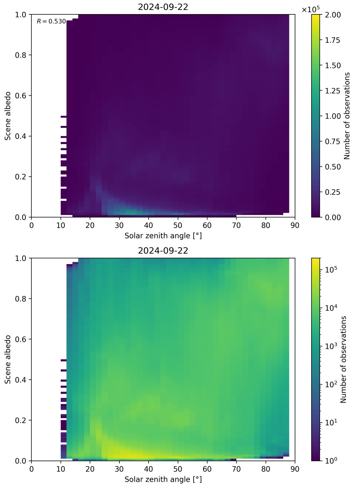
Figure 127: Scatter density plot of “Solar zenith angle” against “Scene albedo” for 2024-09-22 to 2024-09-23.
