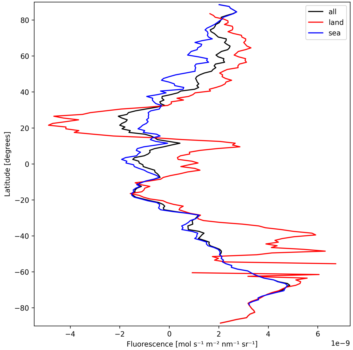
Figure 23: Zonal average of “Fluorescence” for 2024-09-22 to 2024-09-23.
