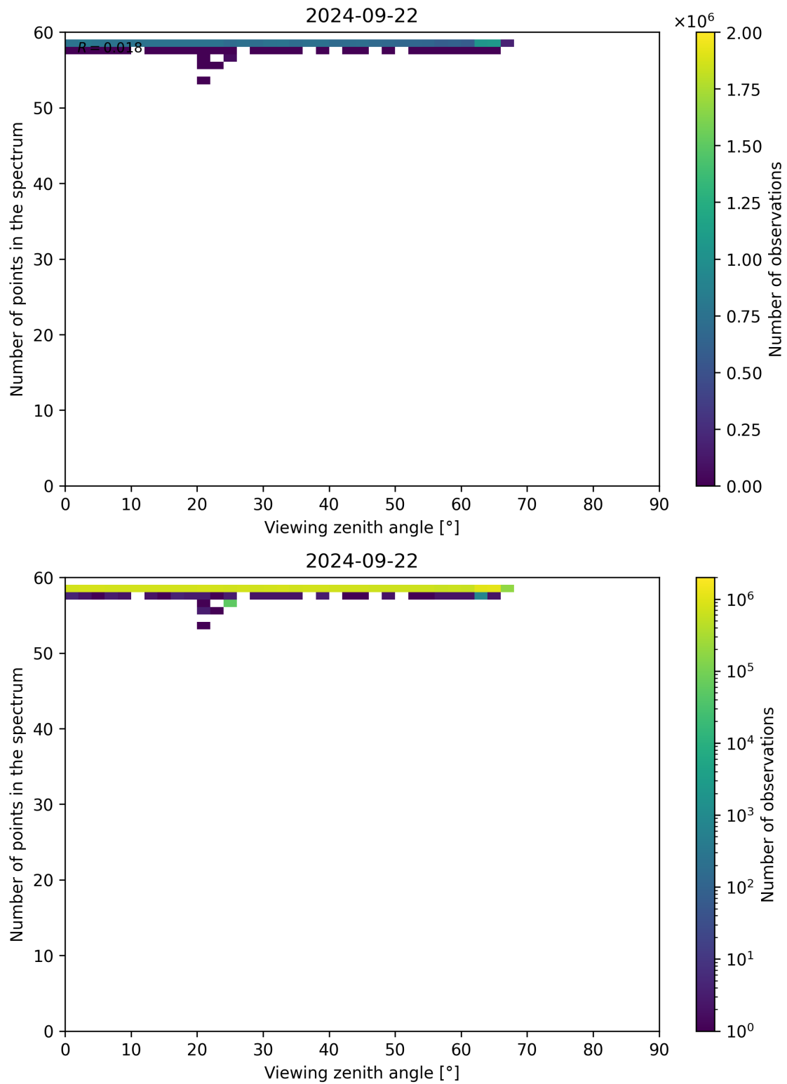
Figure 137: Scatter density plot of “Viewing zenith angle” against “Number of points in the spectrum” for 2024-09-22 to 2024-09-23.
