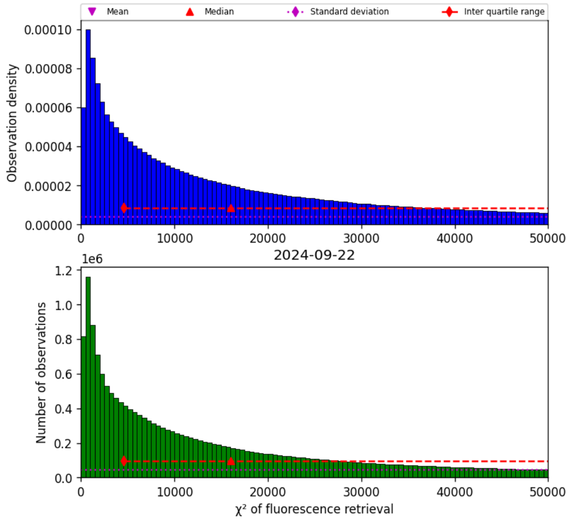
Figure 42: Histogram of “ \chi^2 of fluorescence retrieval” for 2024-09-22 to 2024-09-23
