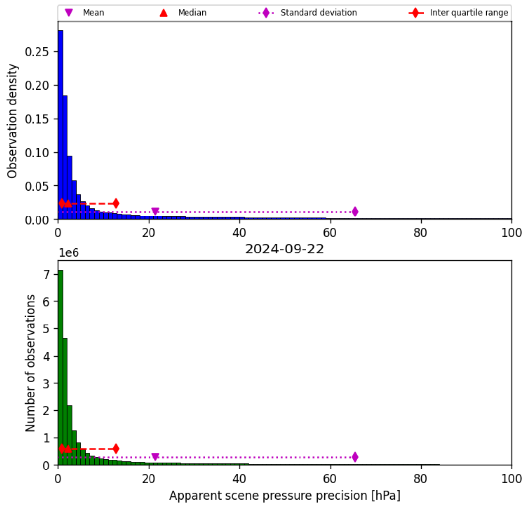
Figure 37: Histogram of “Apparent scene pressure precision” for 2024-09-22 to 2024-09-23
