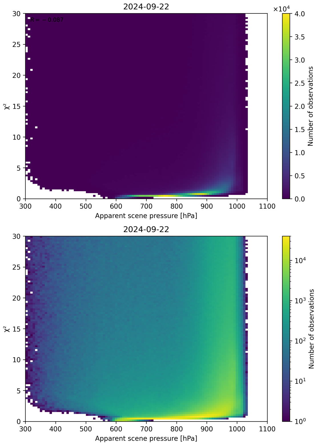
Figure 63: Scatter density plot of “Apparent scene pressure” against “ \chi^2 ” for 2024-09-22 to 2024-09-23.
