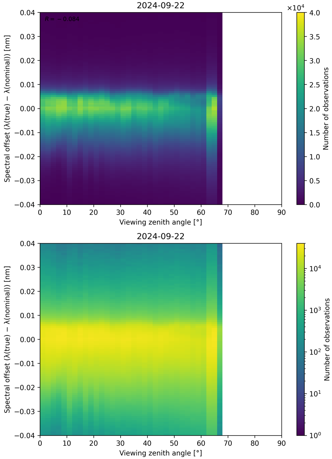
Figure 140: Scatter density plot of “Viewing zenith angle” against “Spectral offset ( \lambda_{\text{true}} - \lambda_{\text{nominal}} )” for 2024-09-22 to 2024-09-23.
