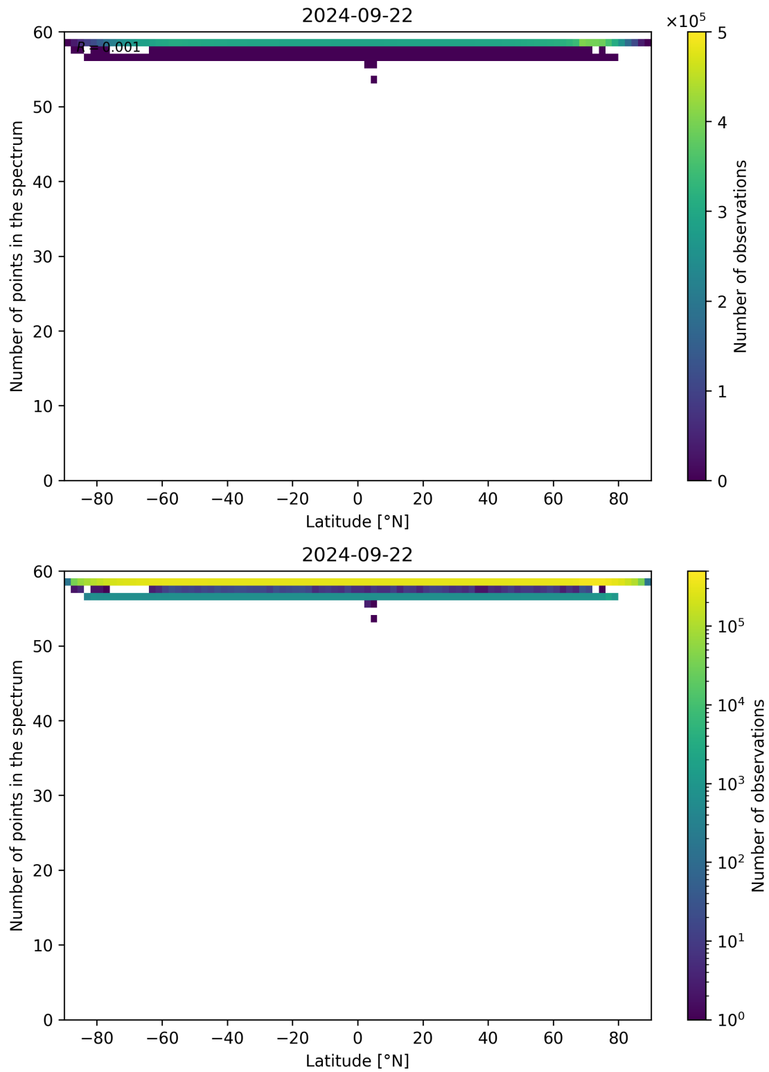
Figure 103: Scatter density plot of “Latitude” against “Number of points in the spectrum” for 2024-09-22 to 2024-09-23.
