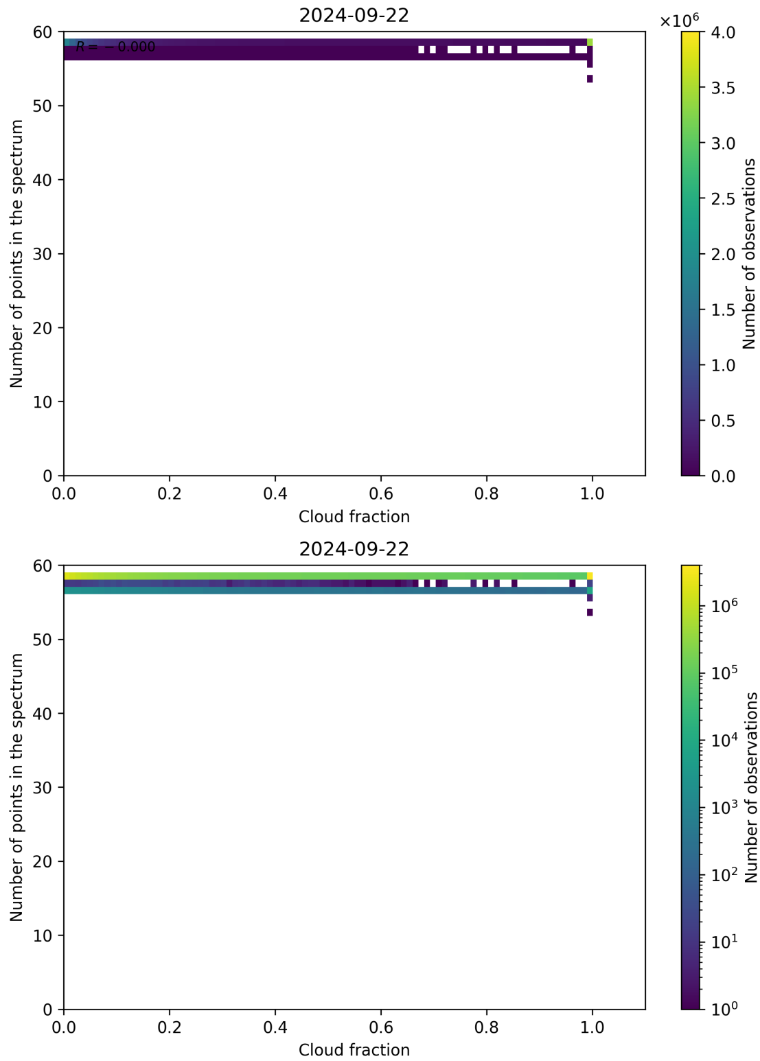
Figure 81: Scatter density plot of “Cloud fraction” against “Number of points in the spectrum” for 2024-09-22 to 2024-09-23.
