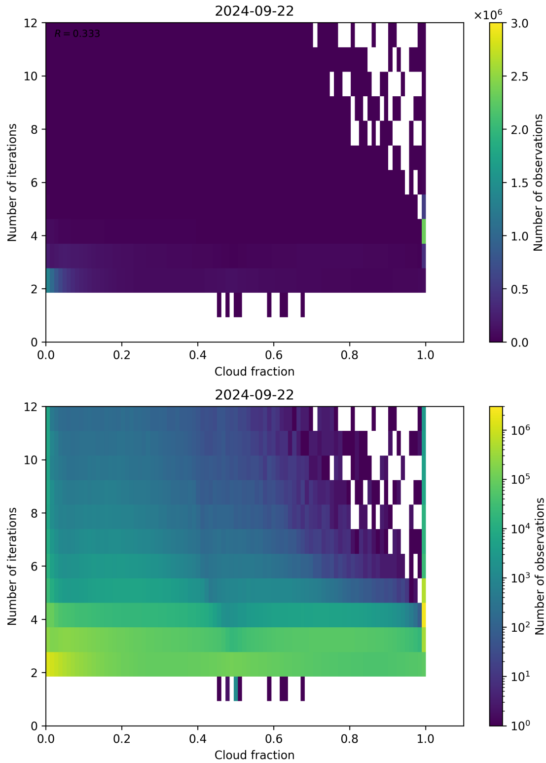
Figure 80: Scatter density plot of “Cloud fraction” against “Number of iterations” for 2024-09-22 to 2024-09-23.
