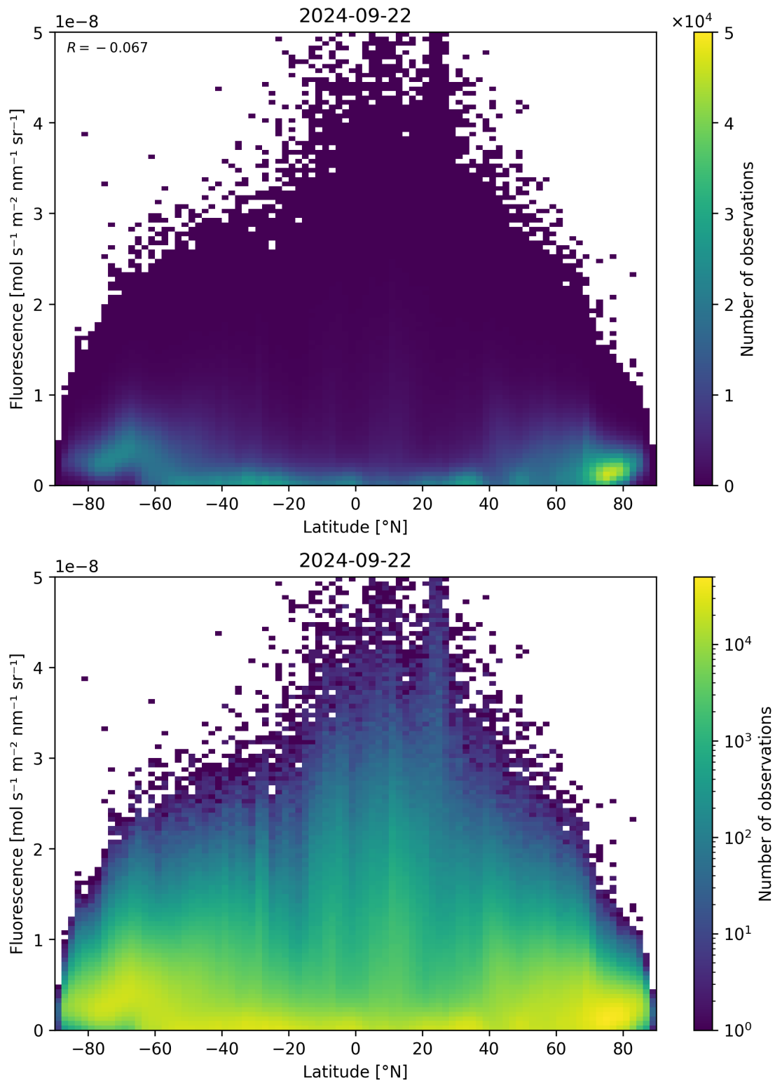
Figure 101: Scatter density plot of “Latitude” against “Fluorescence” for 2024-09-22 to 2024-09-23.
