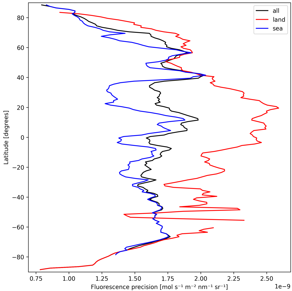
Figure 24: Zonal average of “Fluorescence precision” for 2024-09-22 to 2024-09-23.
