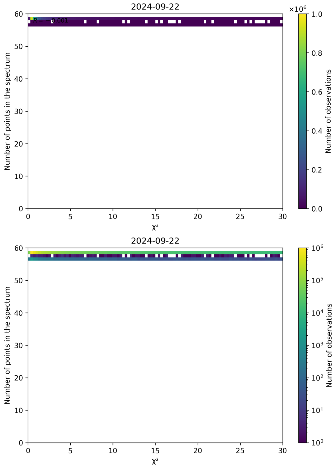
Figure 74: Scatter density plot of " \chi^2 " against "Number of points in the spectrum" for 2024-09-22 to 2024-09-23.
