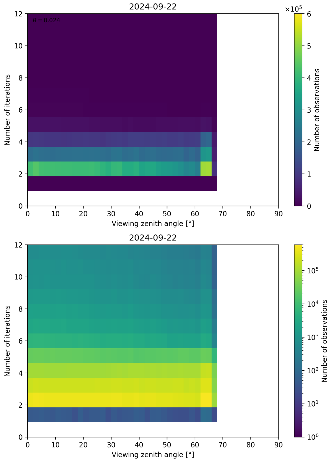
Figure 136: Scatter density plot of “Viewing zenith angle” against “Number of iterations” for 2024-09-22 to 2024-09-23.
