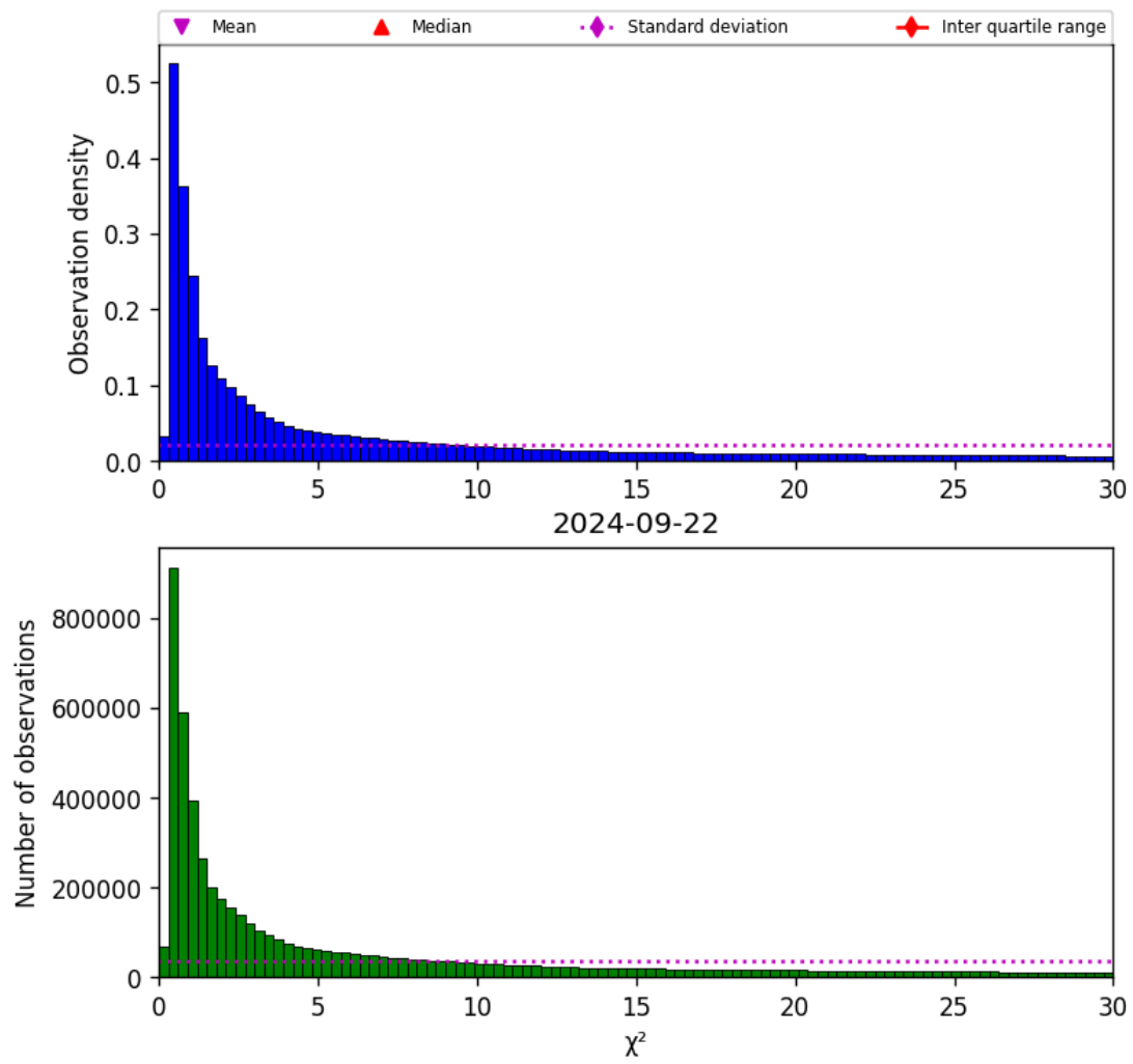
Figure 38: Histogram of " \chi^2 " for 2024-09-22 to 2024-09-23
