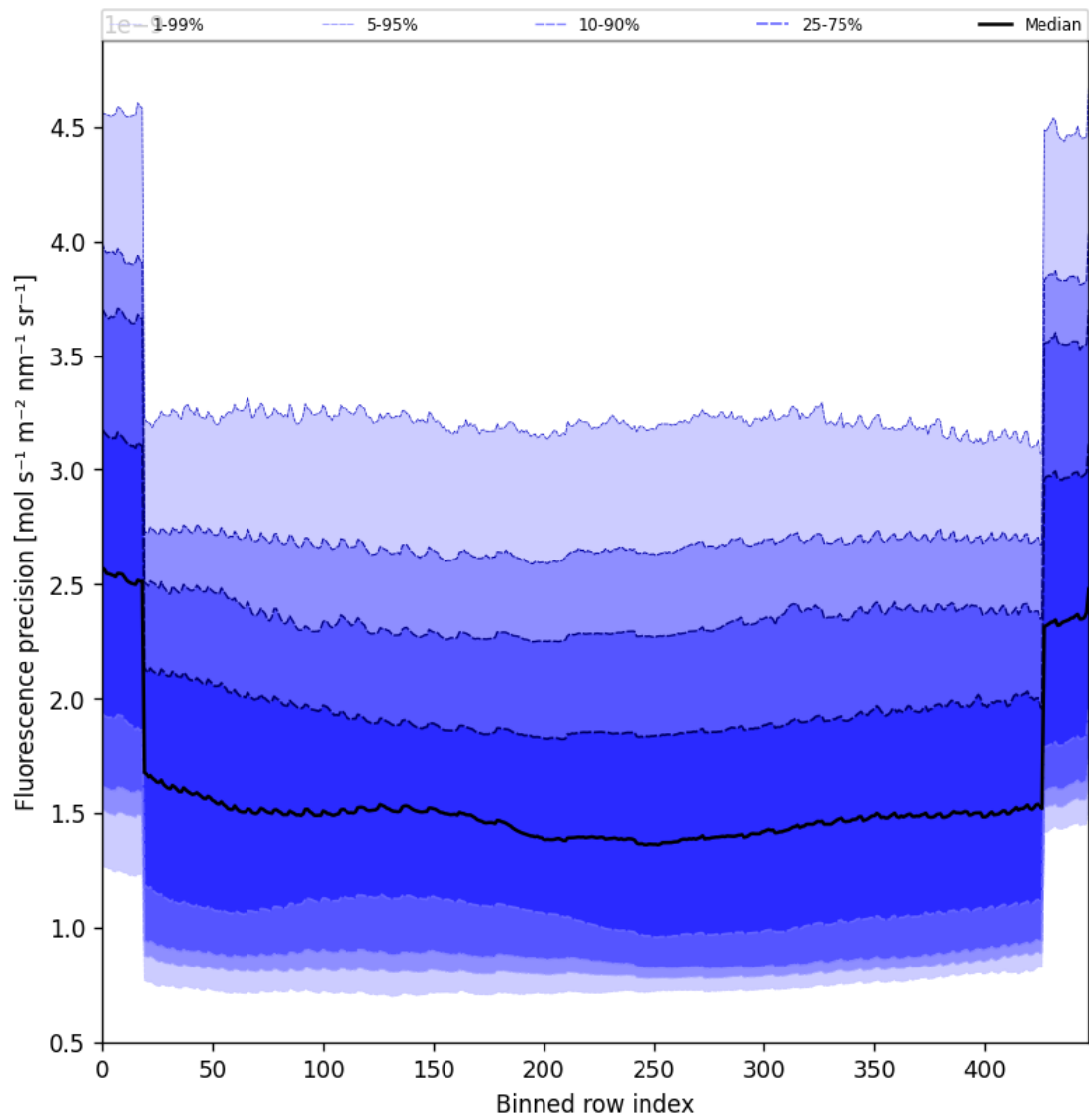
Figure 58: Along track statistics of “Fluorescence precision” for 2024-09-22 to 2024-09-23
