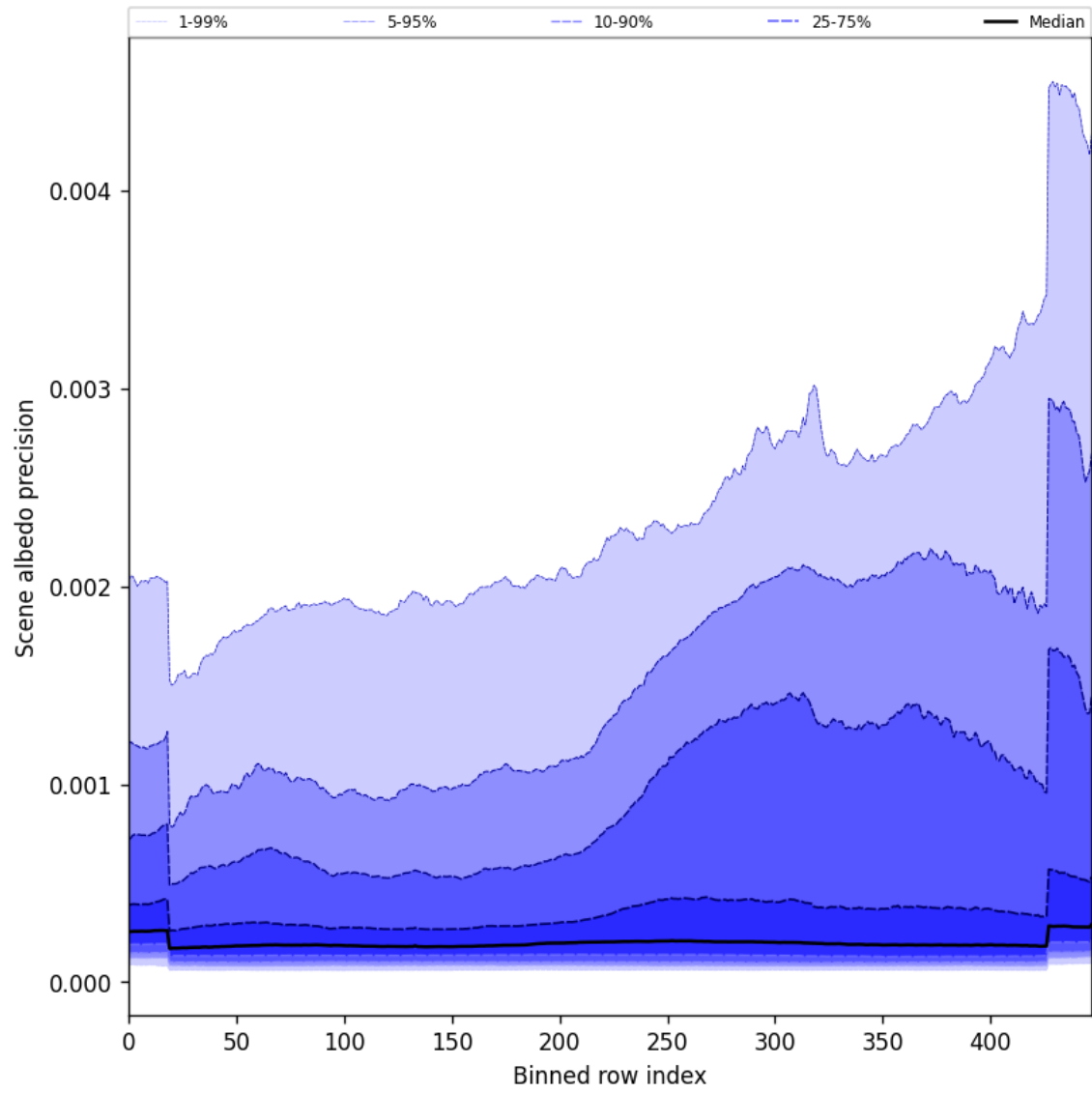
Figure 52: Along track statistics of “Scene albedo precision” for 2024-09-22 to 2024-09-23
