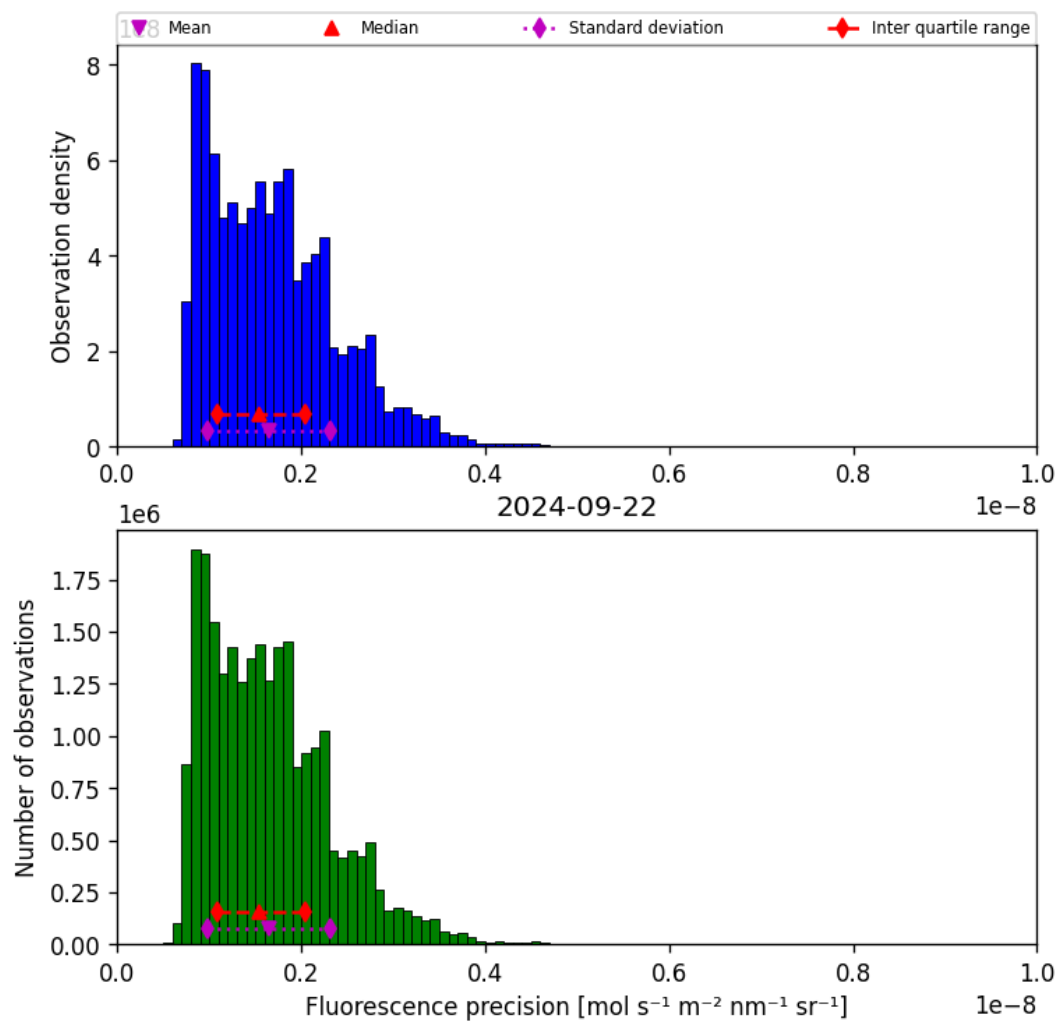
Figure 41: Histogram of “Fluorescence precision” for 2024-09-22 to 2024-09-23
