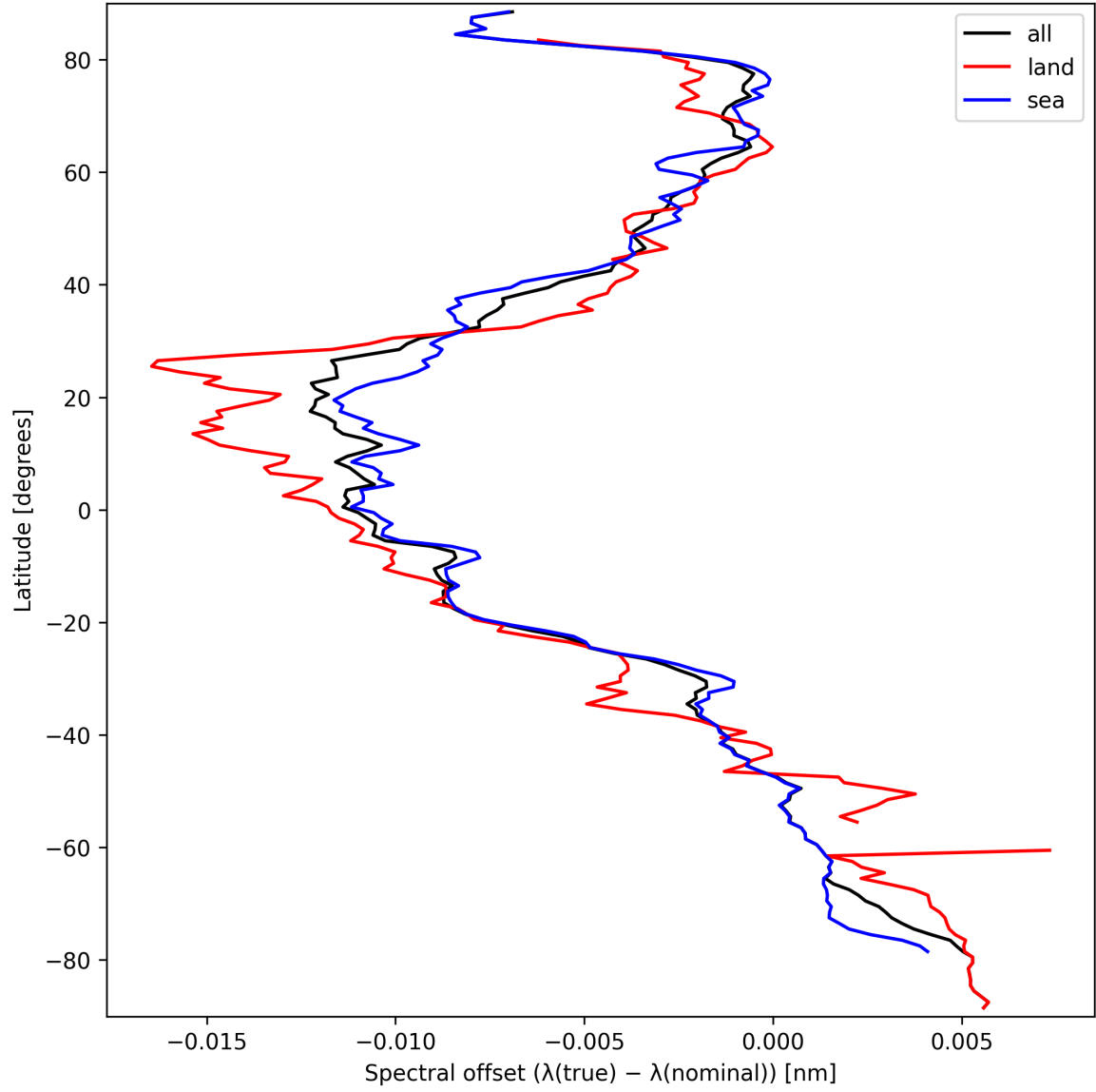
Figure 28: Zonal average of “Spectral offset ( \lambda_{\text{true}} - \lambda_{\text{nominal}} )” for 2024-09-22 to 2024-09-23.
