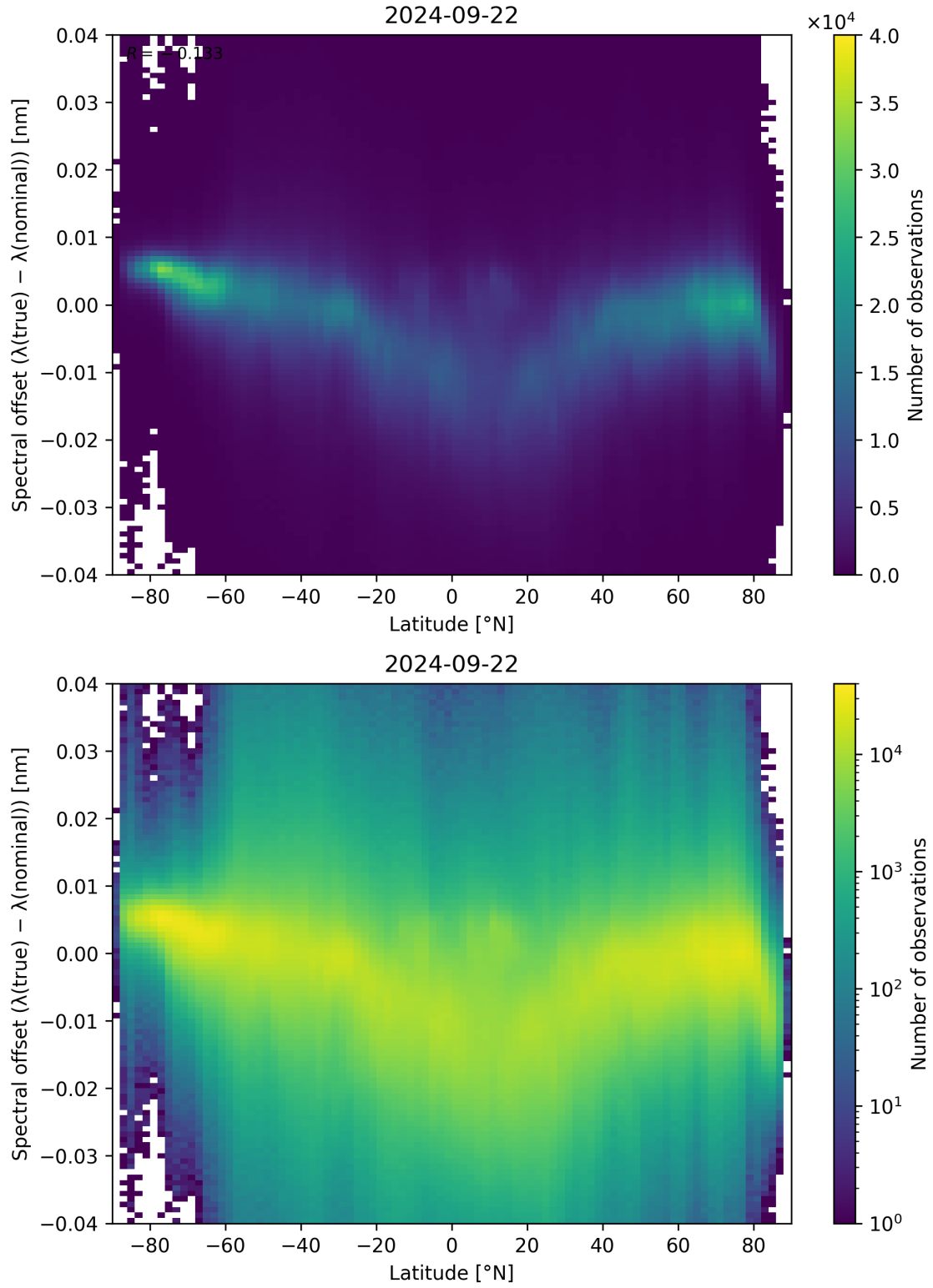
Figure 105: Scatter density plot of “Latitude” against “Spectral offset ( \lambda_{\text{true}} - \lambda_{\text{nominal}} )” for 2024-09-22 to 2024-09-23.
