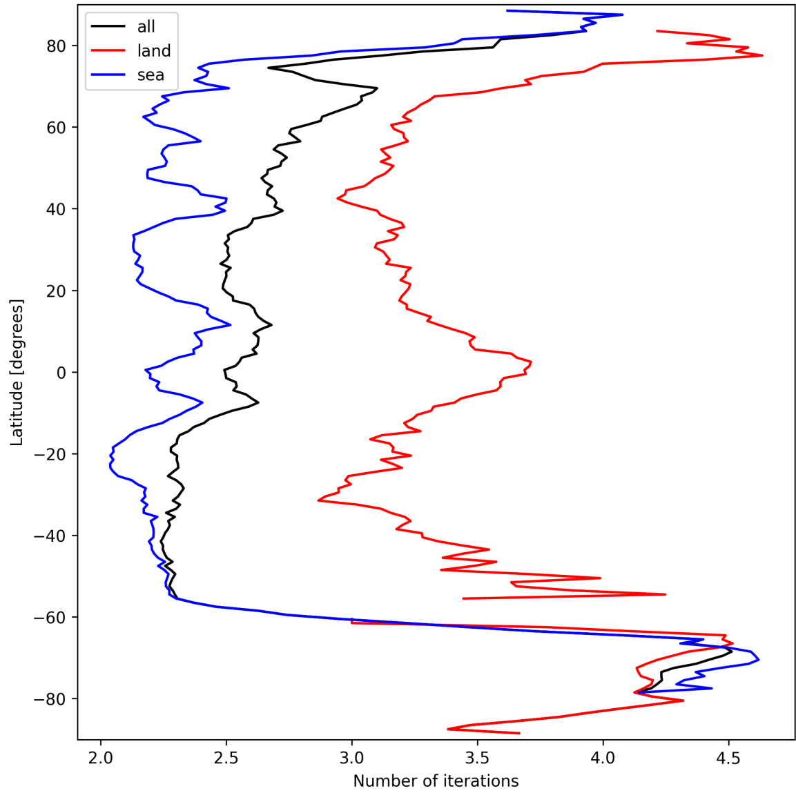
Figure 22: Zonal average of “Number of iterations” for 2024-09-22 to 2024-09-23.
