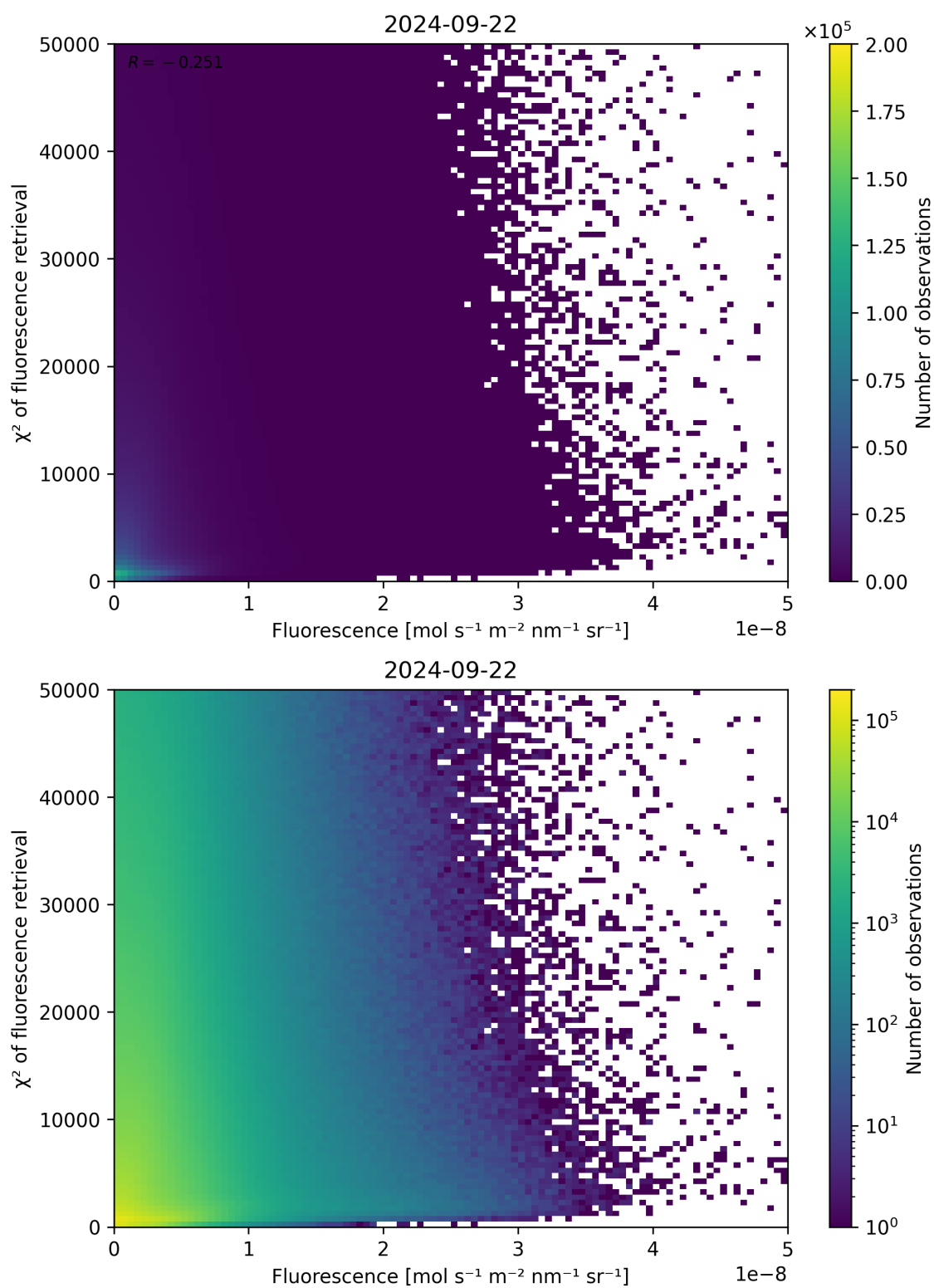
Figure 93: Scatter density plot of “Fluorescence” against “ \chi^2 of fluorescence retrieval” for 2024-09-22 to 2024-09-23.
