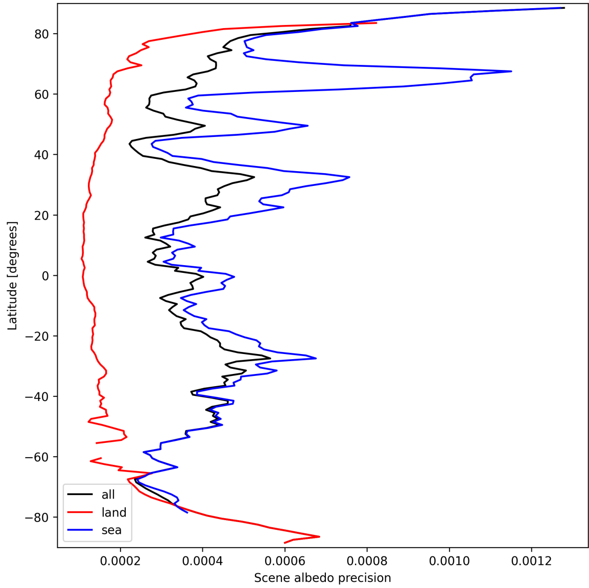
Figure 18: Zonal average of “Scene albedo precision” for 2024-09-22 to 2024-09-23.
