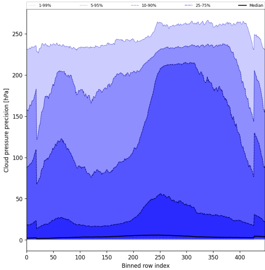
Figure 48: Along track statistics of “Cloud pressure precision” for 2024-09-22 to 2024-09-23
