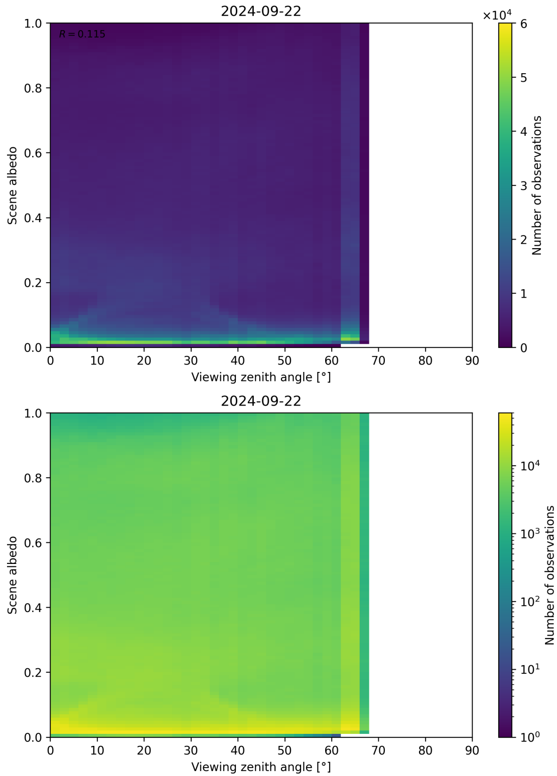
Figure 138: Scatter density plot of “Viewing zenith angle” against “Scene albedo” for 2024-09-22 to 2024-09-23.
