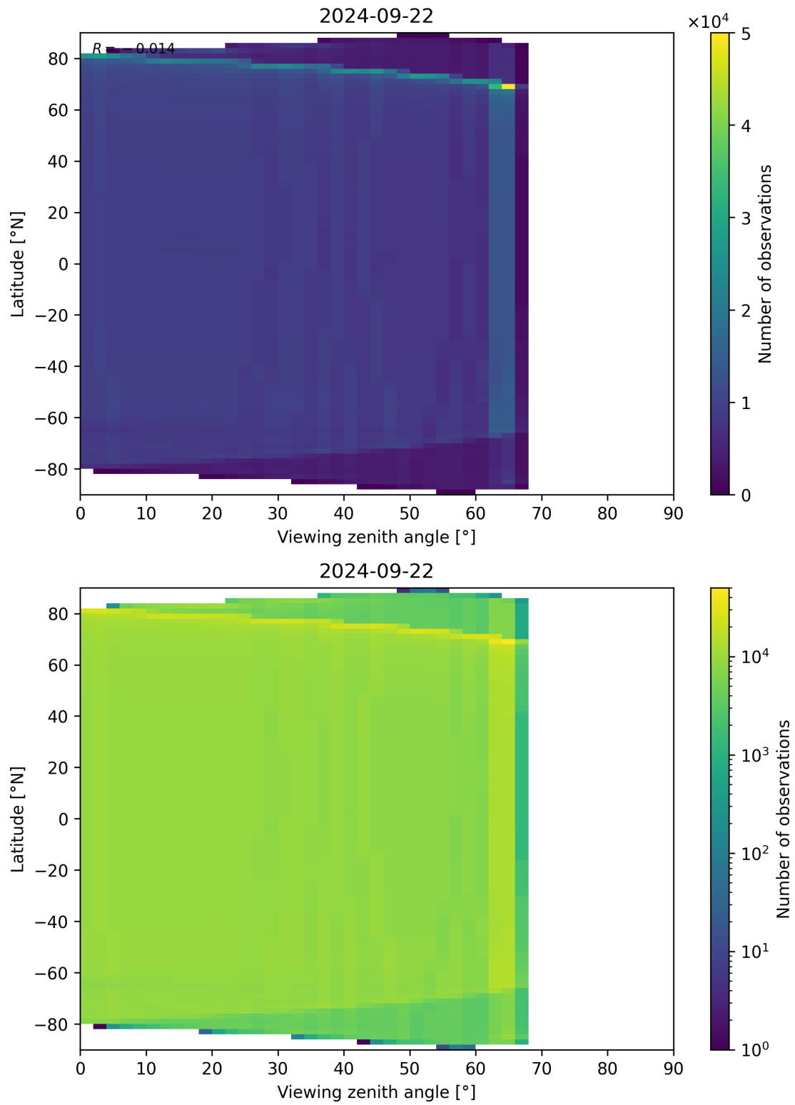
Figure 135: Scatter density plot of “Viewing zenith angle” against “Latitude” for 2024-09-22 to 2024-09-23.
