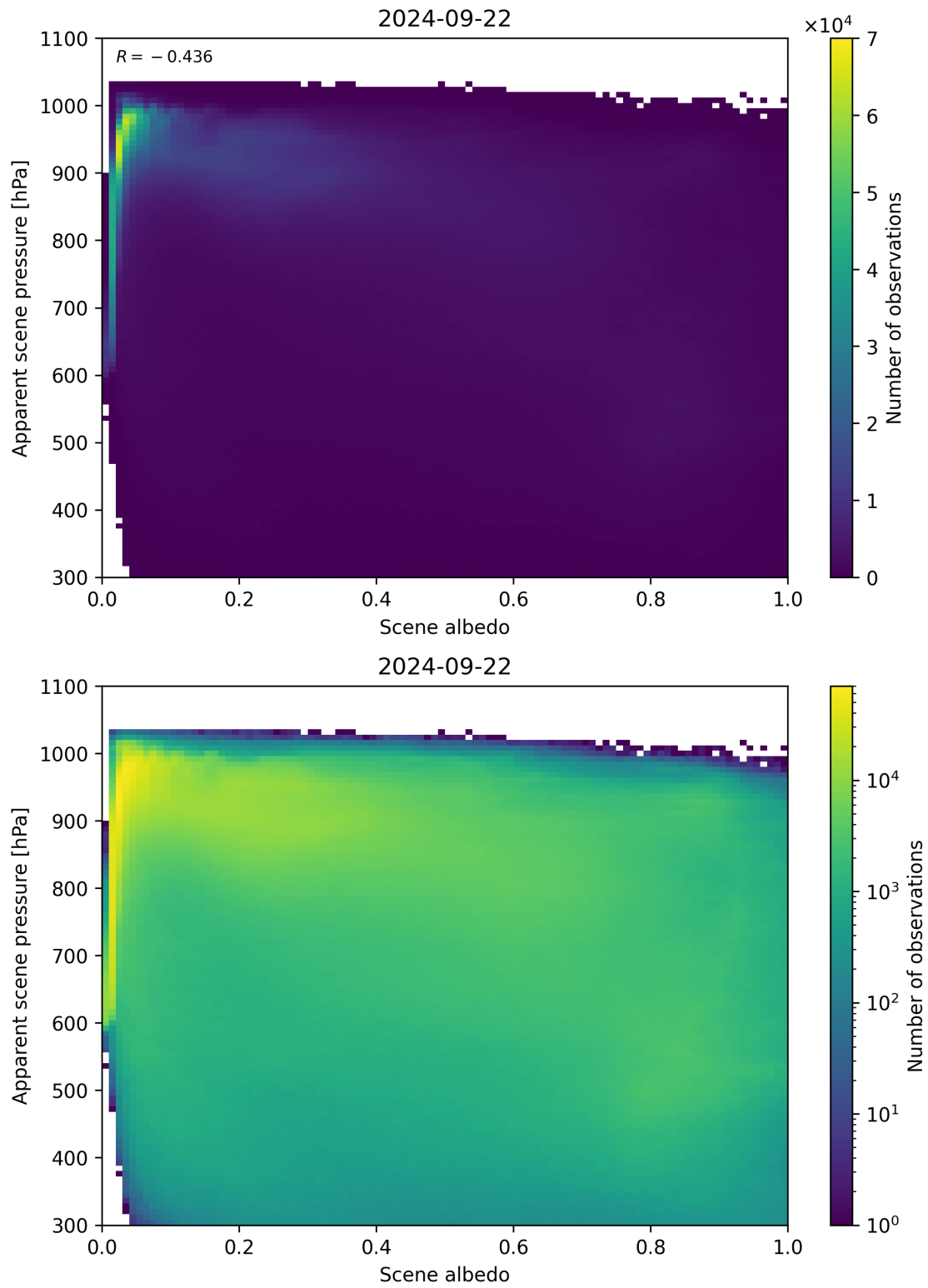
Figure 111: Scatter density plot of “Scene albedo” against “Apparent scene pressure” for 2024-09-22 to 2024-09-23.
