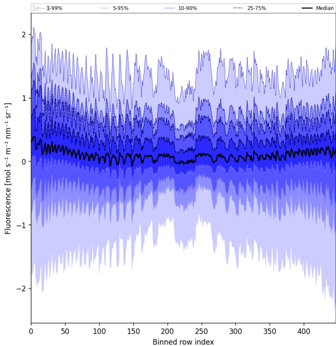
Figure 57: Along track statistics of “Fluorescence” for 2024-09-22 to 2024-09-23
