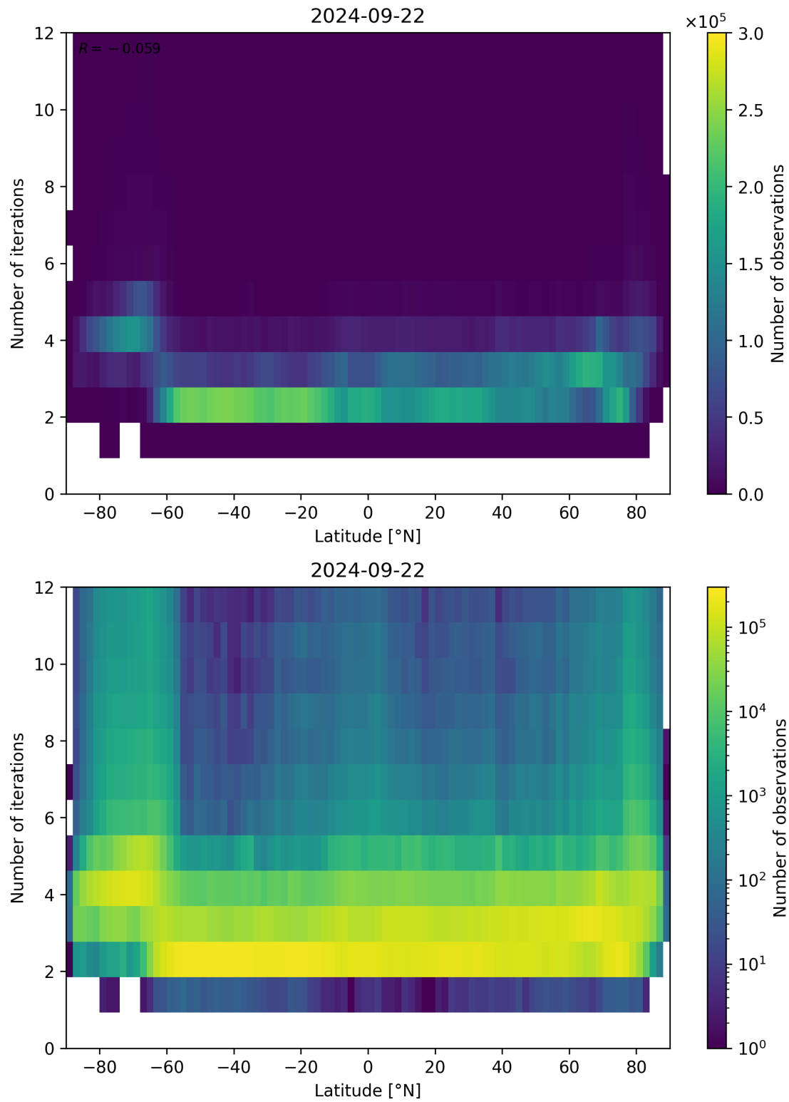
Figure 102: Scatter density plot of “Latitude” against “Number of iterations” for 2024-09-22 to 2024-09-23.
