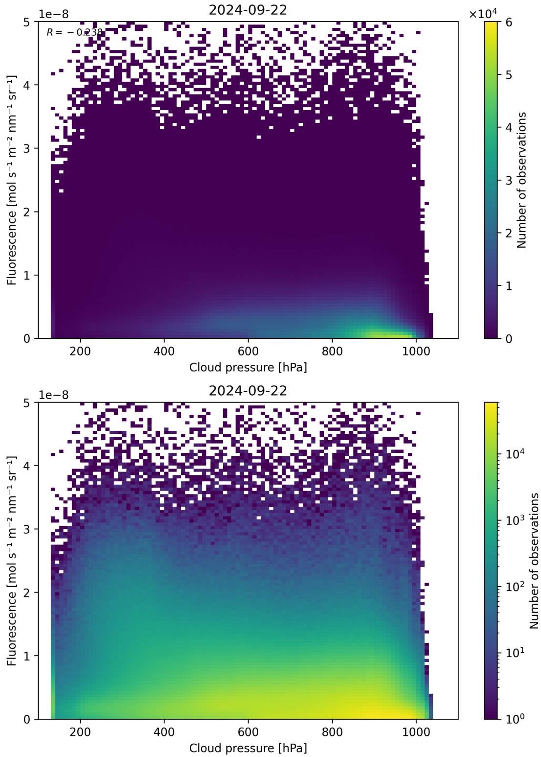
Figure 88: Scatter density plot of “Cloud pressure” against “Fluorescence” for 2024-09-22 to 2024-09-23.
