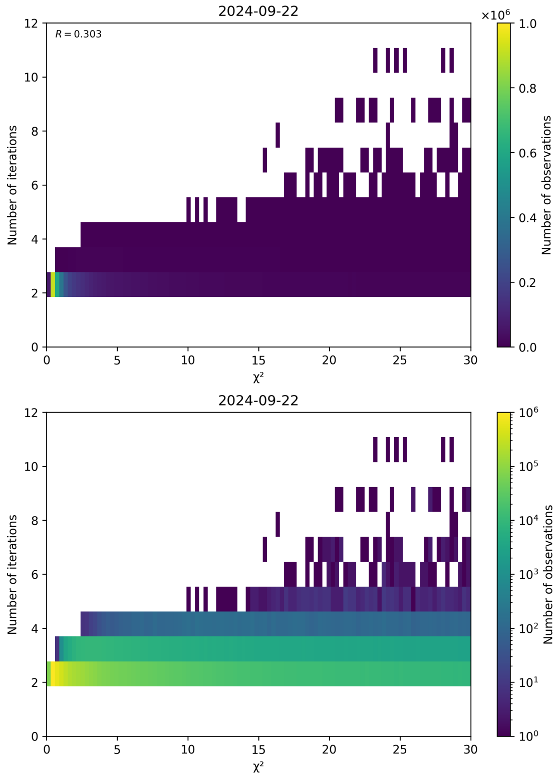
Figure 73: Scatter density plot of “ \chi^2 ” against “Number of iterations” for 2024-09-22 to 2024-09-23.
