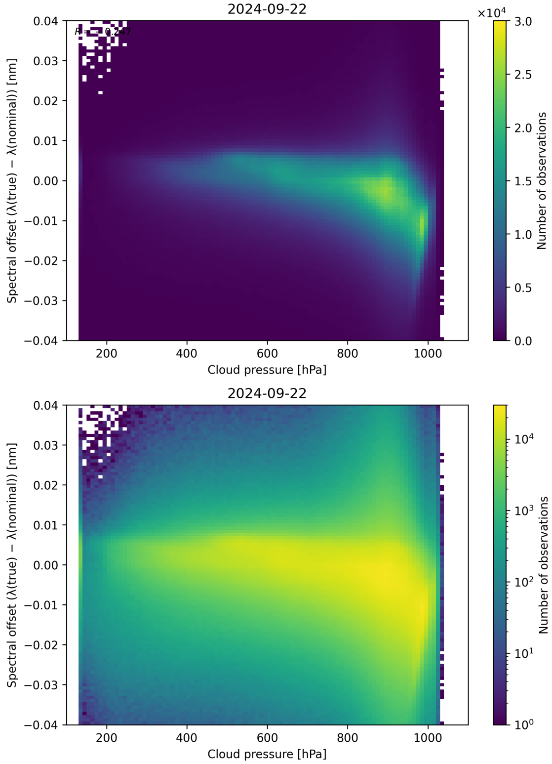
Figure 92: Scatter density plot of “Cloud pressure” against “Spectral offset ( \lambda_{\text{true}} - \lambda_{\text{nominal}} )” for 2024-09-22 to 2024-09-23.
