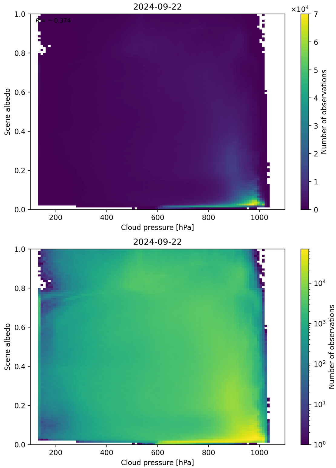
Figure 91: Scatter density plot of “Cloud pressure” against “Scene albedo” for 2024-09-22 to 2024-09-23.
