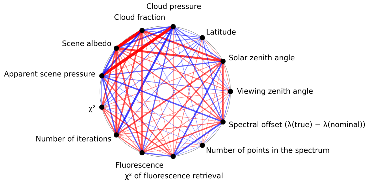
Figure 1: Map of correlation graph for 2024-09-22 to 2024-09-23.
