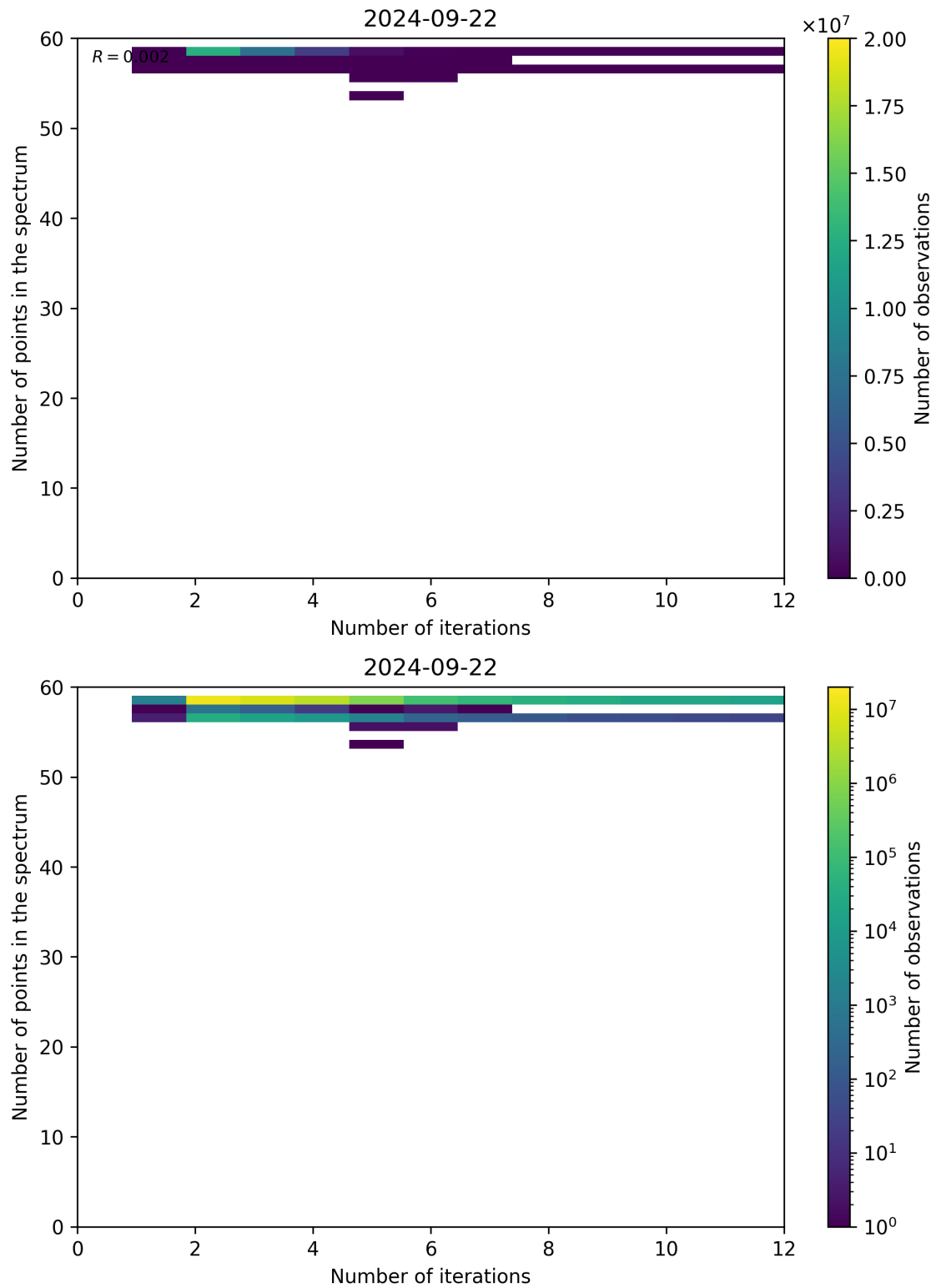
Figure 108: Scatter density plot of “Number of iterations” against “Number of points in the spectrum” for 2024-09-22 to 2024-09-23.
