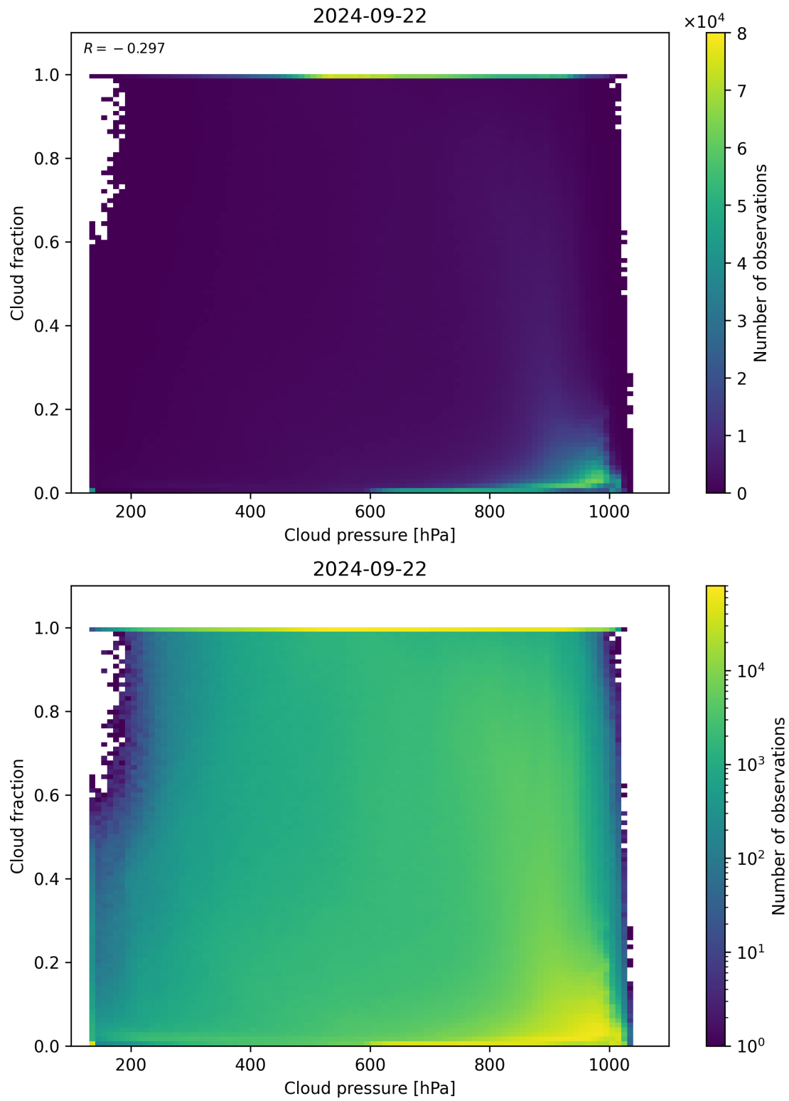
Figure 87: Scatter density plot of “Cloud pressure” against “Cloud fraction” for 2024-09-22 to 2024-09-23.
