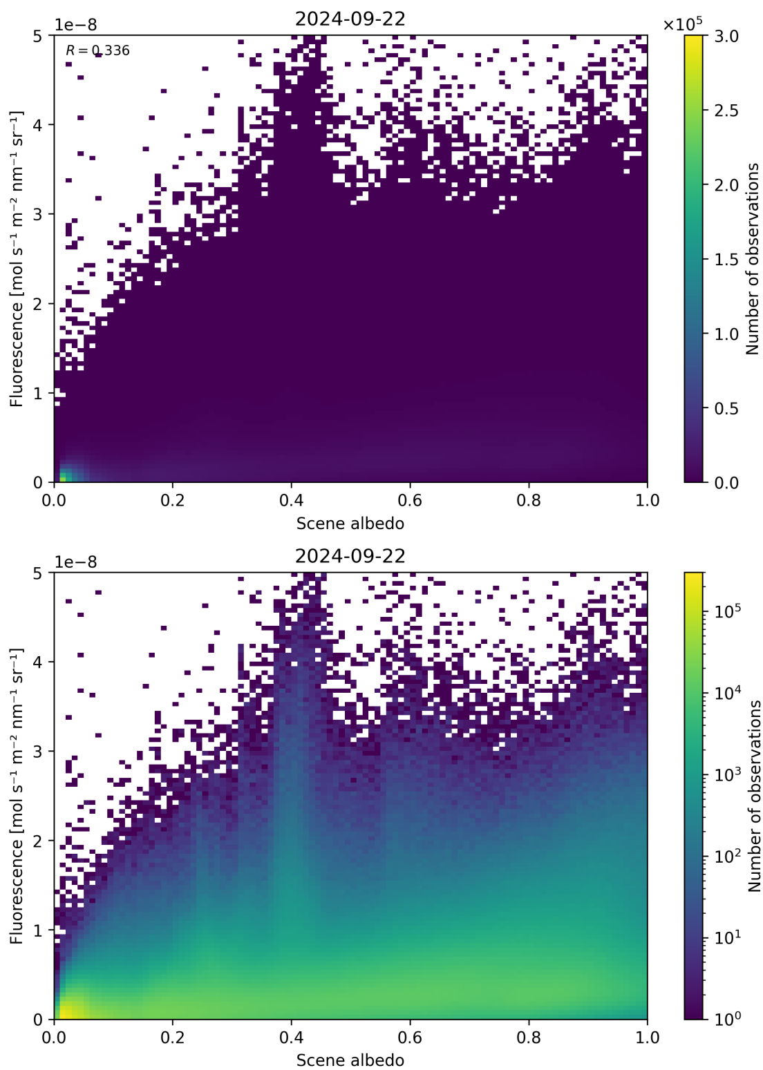
Figure 114: Scatter density plot of “Scene albedo” against “Fluorescence” for 2024-09-22 to 2024-09-23.
