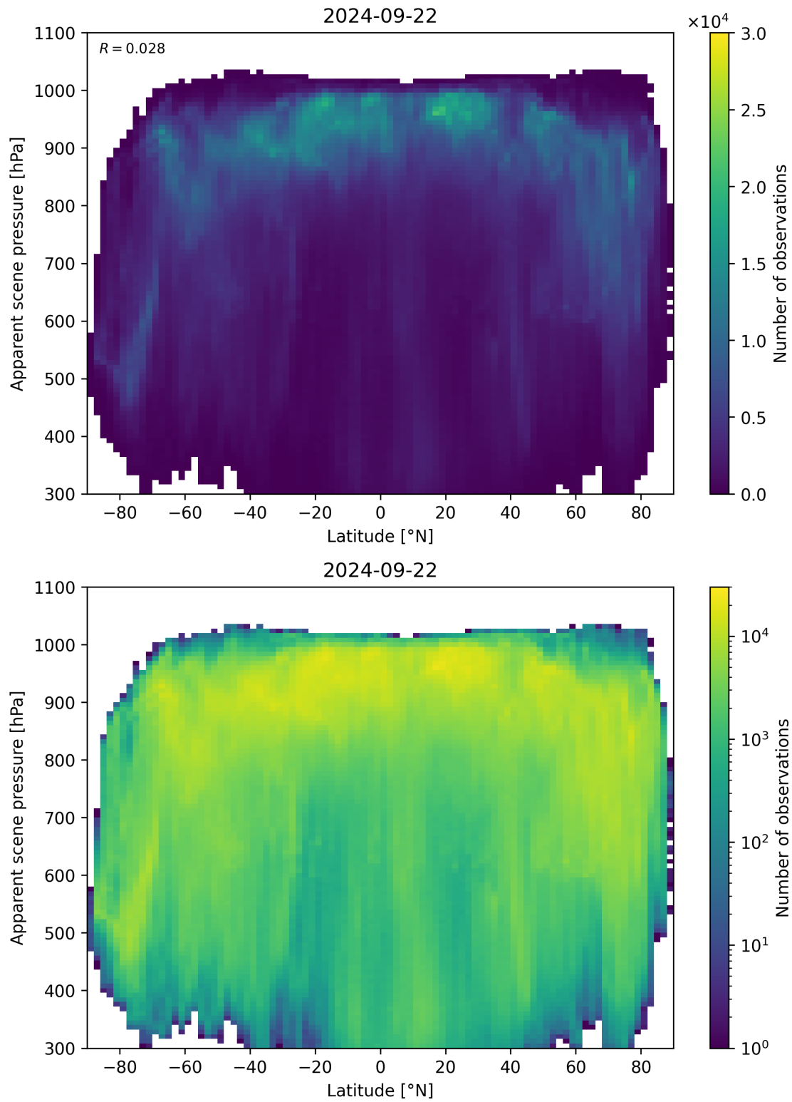
Figure 96: Scatter density plot of “Latitude” against “Apparent scene pressure” for 2024-09-22 to 2024-09-23.
