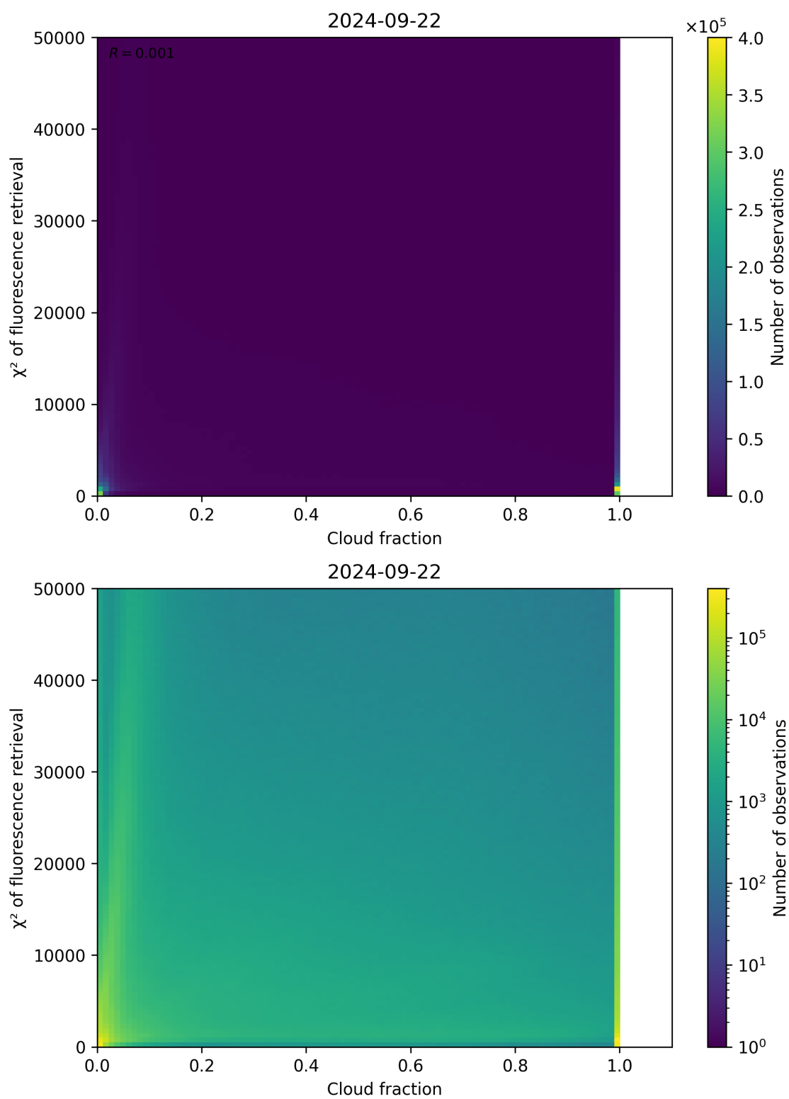
Figure 78: Scatter density plot of “Cloud fraction” against “ \chi^2 of fluorescence retrieval” for 2024-09-22 to 2024-09-23.
