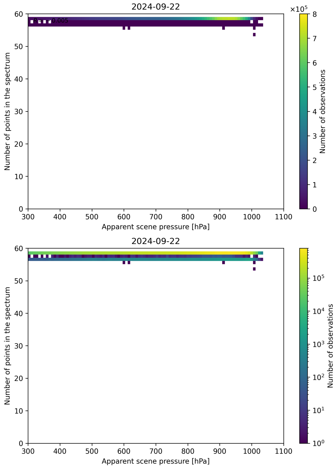
Figure 67: Scatter density plot of “Apparent scene pressure” against “Number of points in the spectrum” for 2024-09-22 to 2024-09-23.
