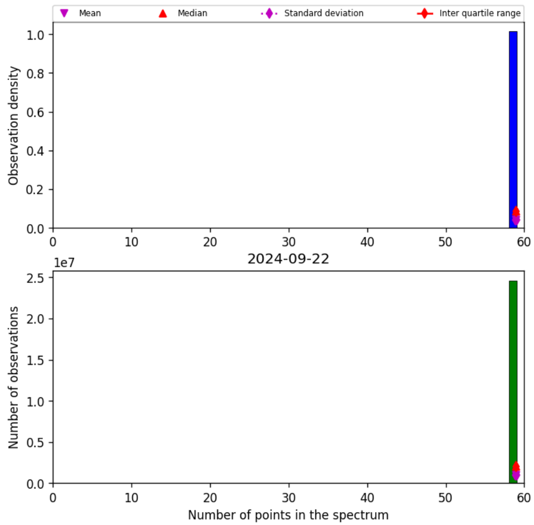
Figure 44: Histogram of “Number of points in the spectrum” for 2024-09-22 to 2024-09-23
