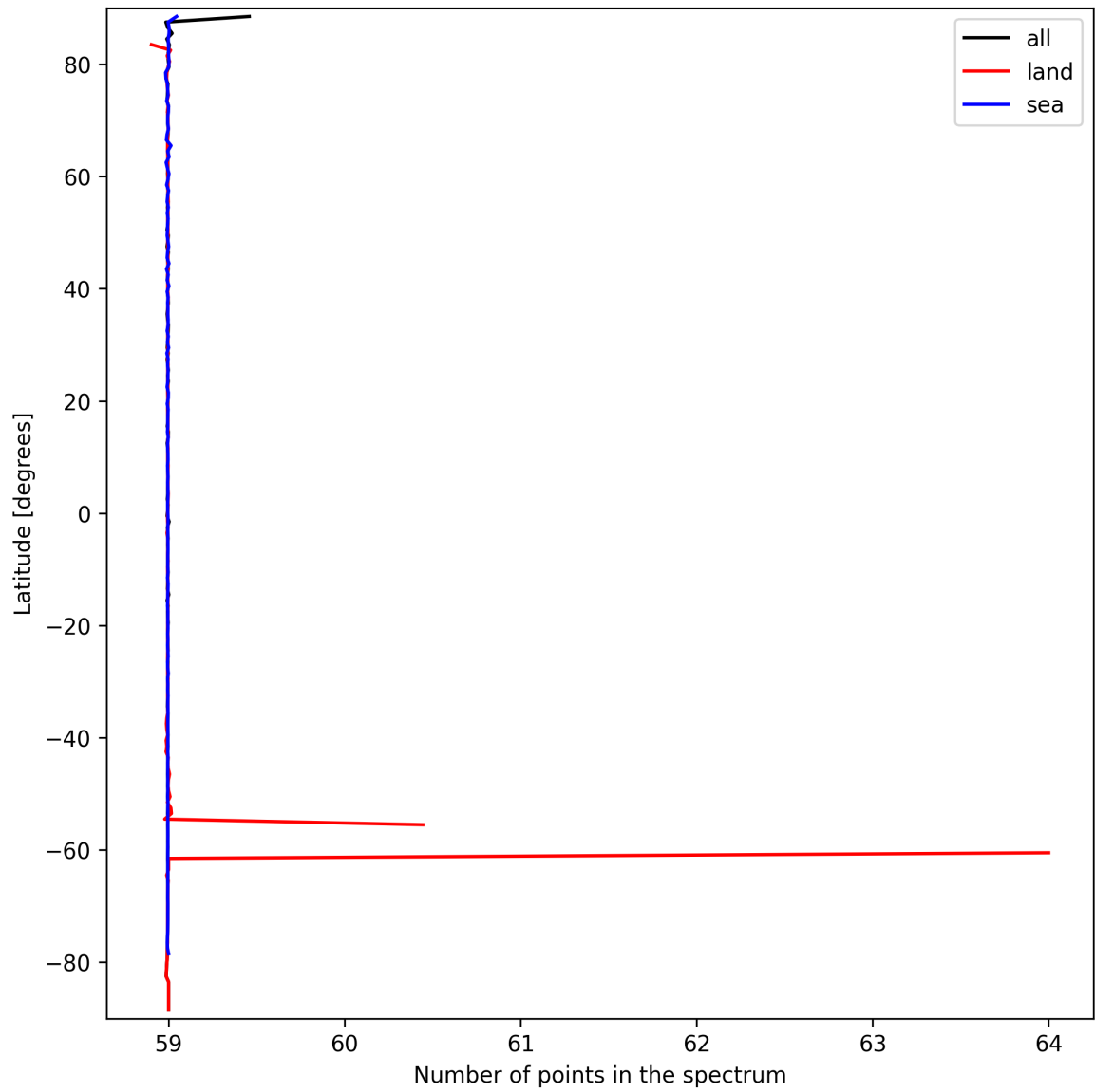
Figure 27: Zonal average of “Number of points in the spectrum” for 2024-09-22 to 2024-09-23.
