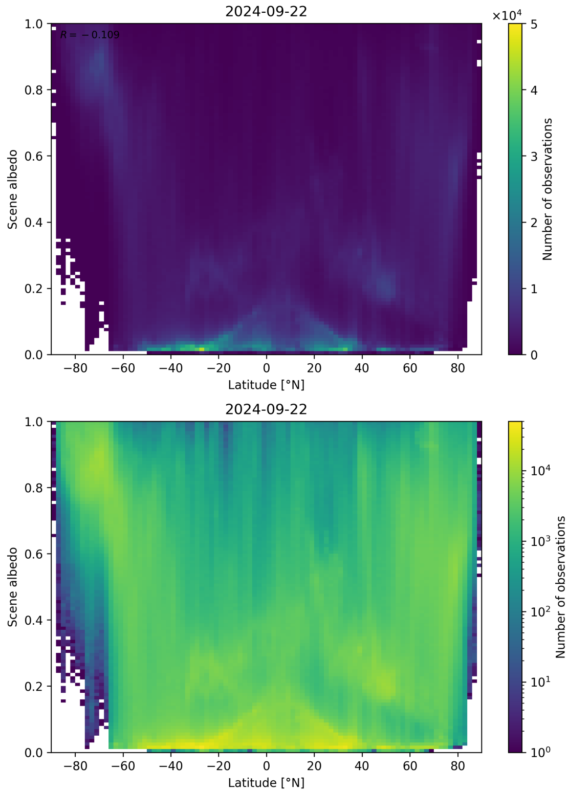
Figure 104: Scatter density plot of “Latitude” against “Scene albedo” for 2024-09-22 to 2024-09-23.
