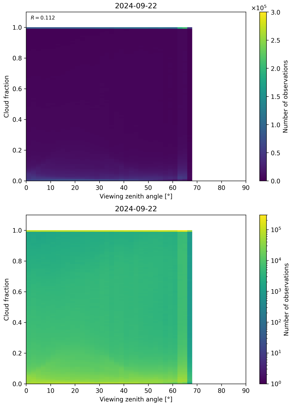
Figure 132: Scatter density plot of “Viewing zenith angle” against “Cloud fraction” for 2024-09-22 to 2024-09-23.
