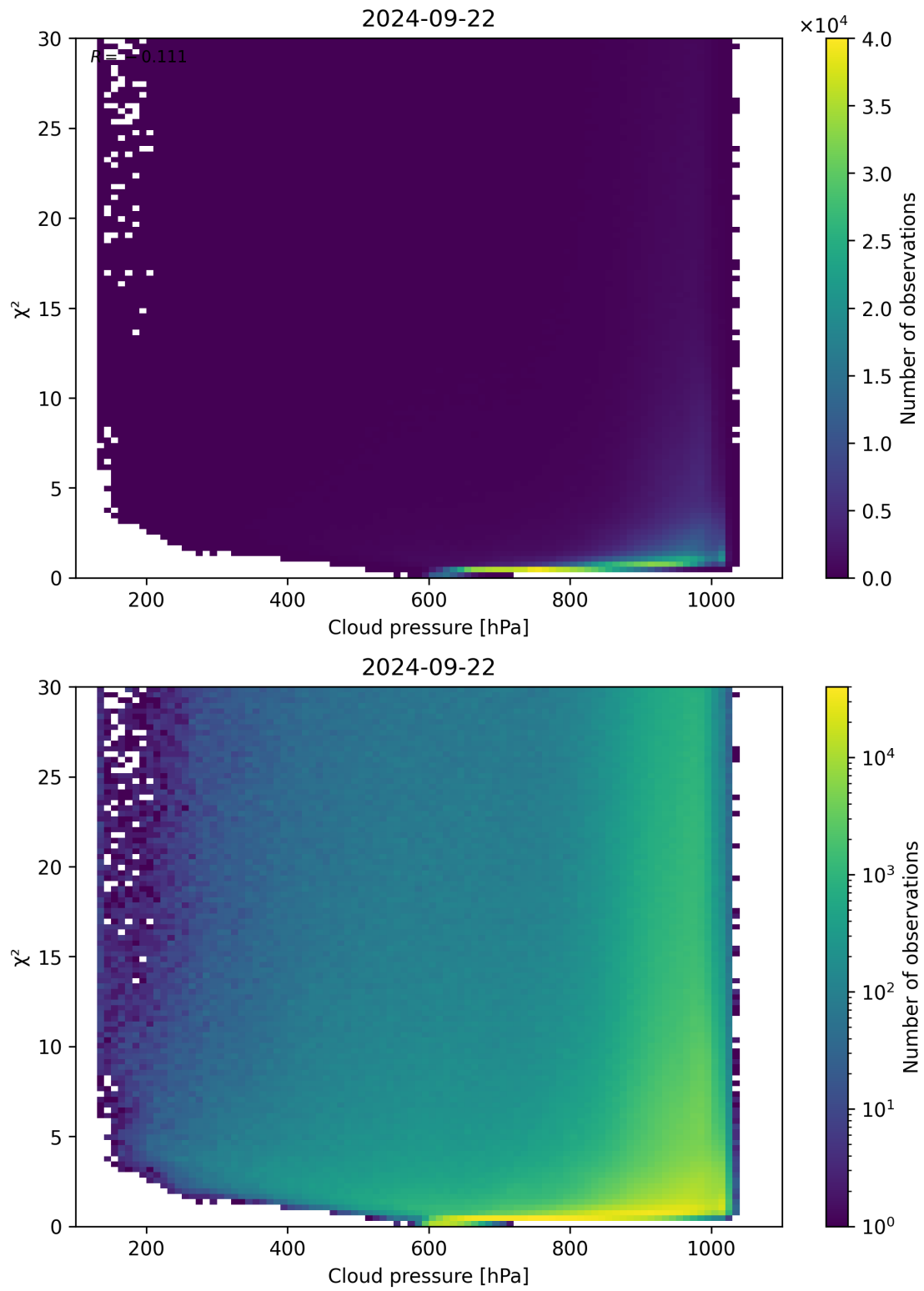
Figure 85: Scatter density plot of “Cloud pressure” against “ \chi^2 ” for 2024-09-22 to 2024-09-23.
