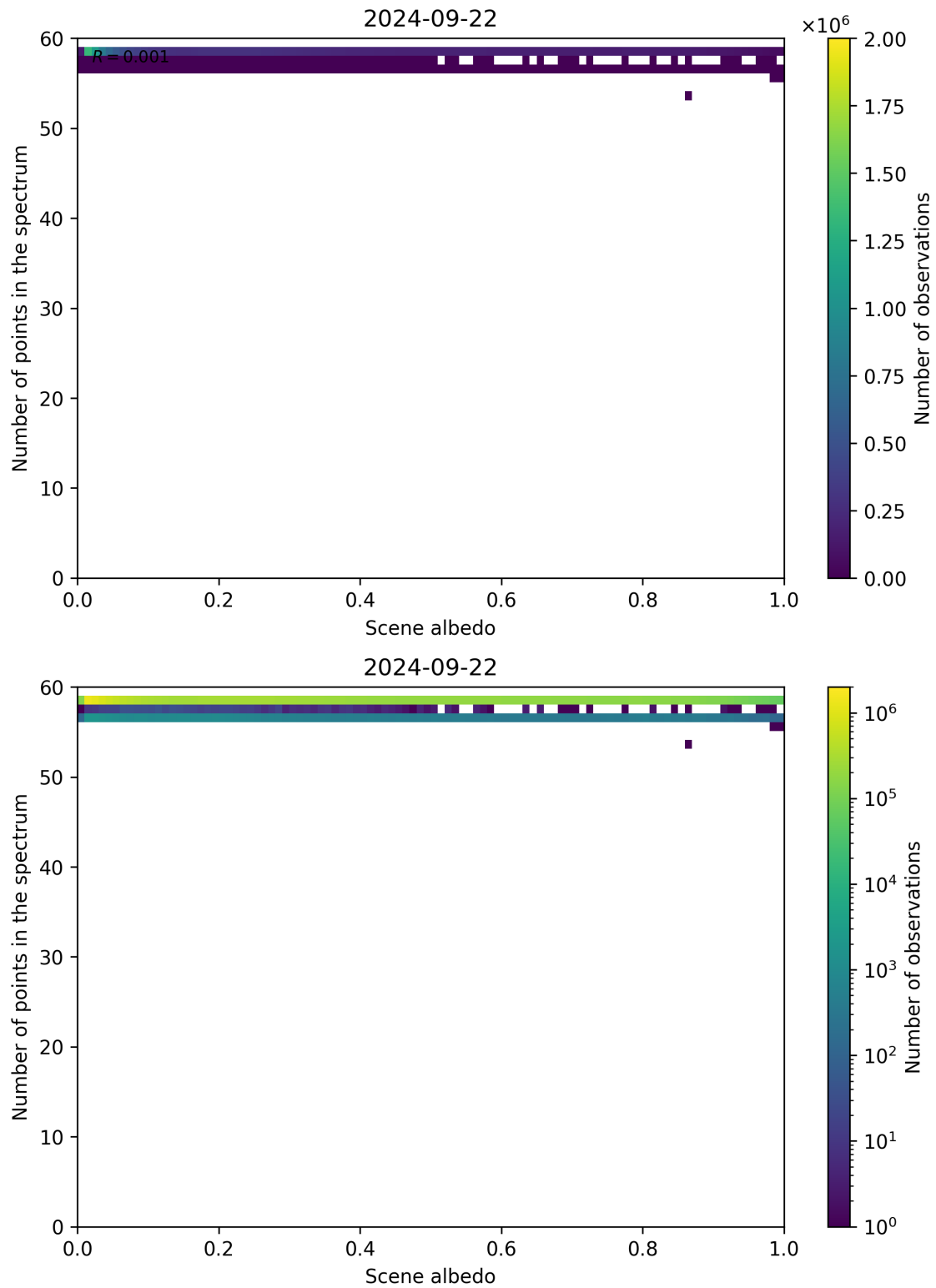
Figure 116: Scatter density plot of “Scene albedo” against “Number of points in the spectrum” for 2024-09-22 to 2024-09-23.
