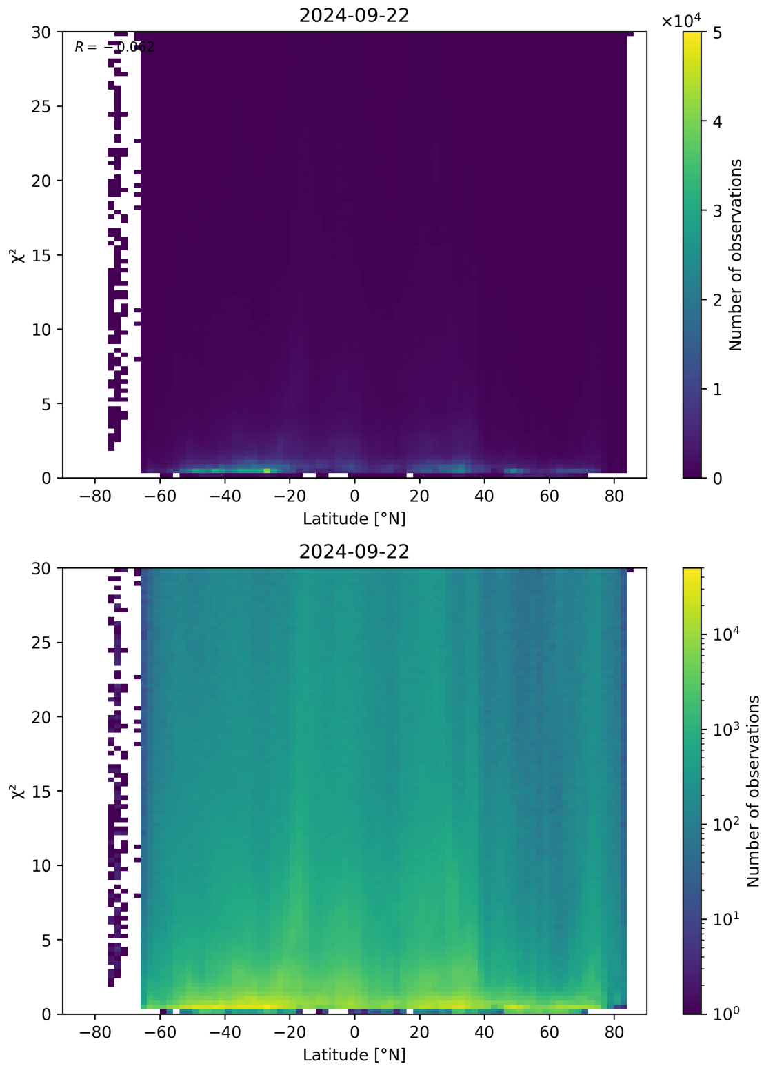
Figure 97: Scatter density plot of “Latitude” against “ \chi^2 ” for 2024-09-22 to 2024-09-23.
