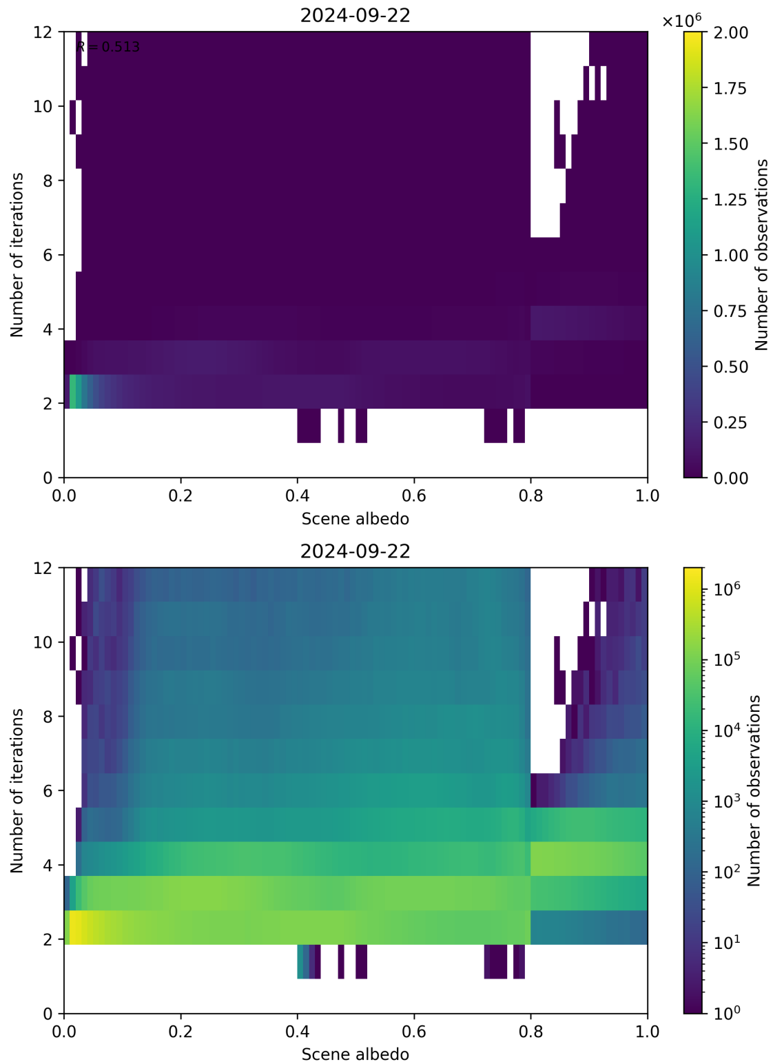
Figure 115: Scatter density plot of “Scene albedo” against “Number of iterations” for 2024-09-22 to 2024-09-23.
