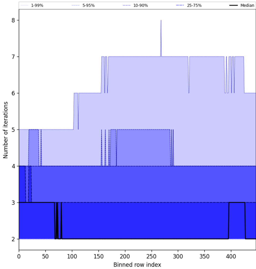
Figure 56: Along track statistics of “Number of iterations” for 2024-09-22 to 2024-09-23
