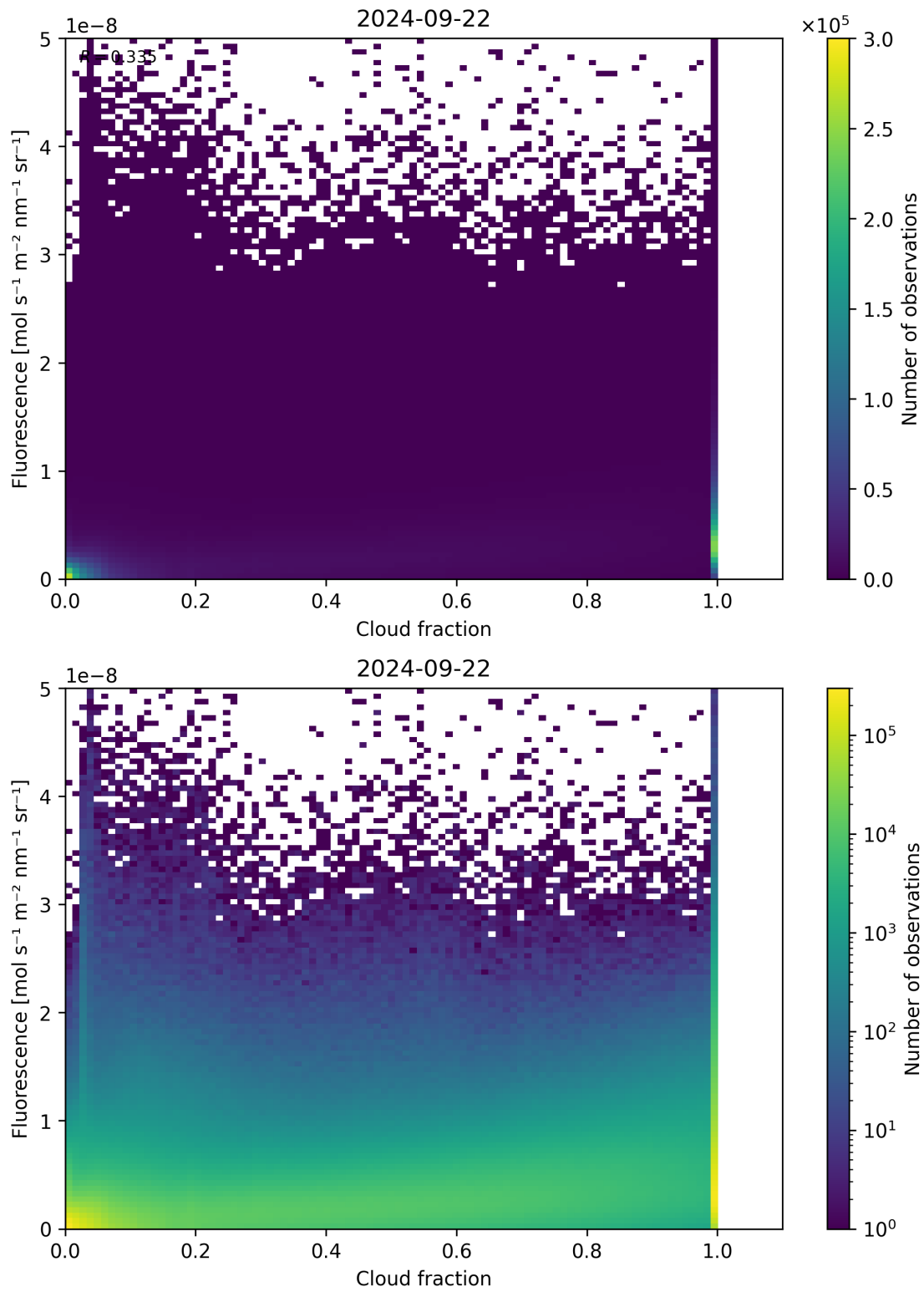
Figure 79: Scatter density plot of “Cloud fraction” against “Fluorescence” for 2024-09-22 to 2024-09-23.
