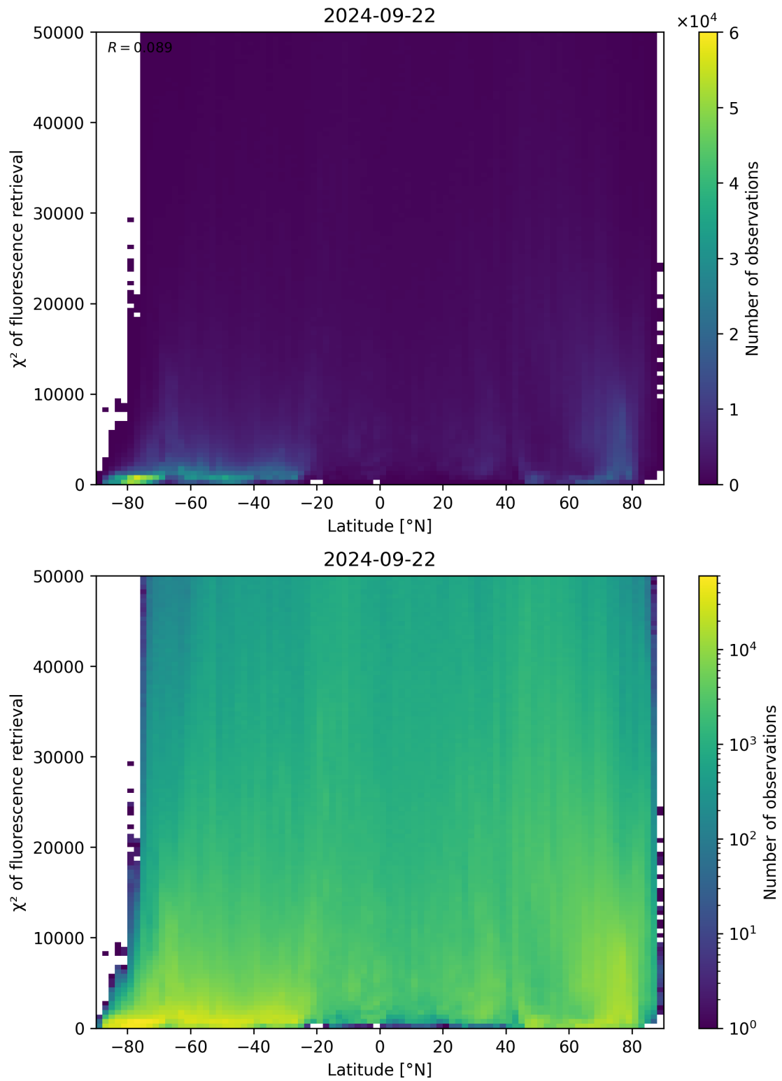
Figure 98: Scatter density plot of “Latitude” against “ \chi^2 of fluorescence retrieval” for 2024-09-22 to 2024-09-23.
