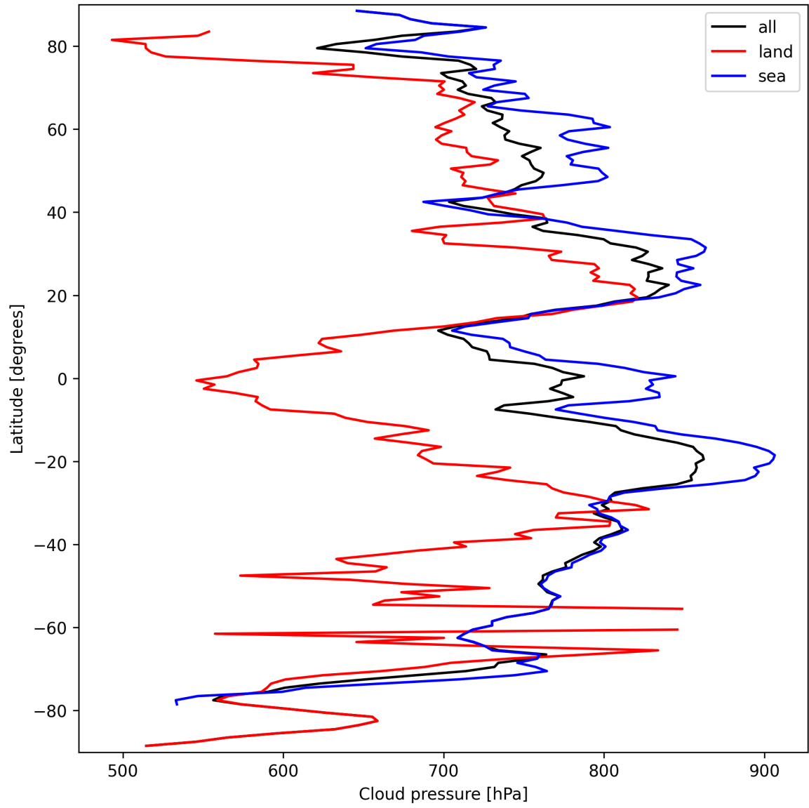
Figure 13: Zonal average of “Cloud pressure” for 2024-09-22 to 2024-09-23.
