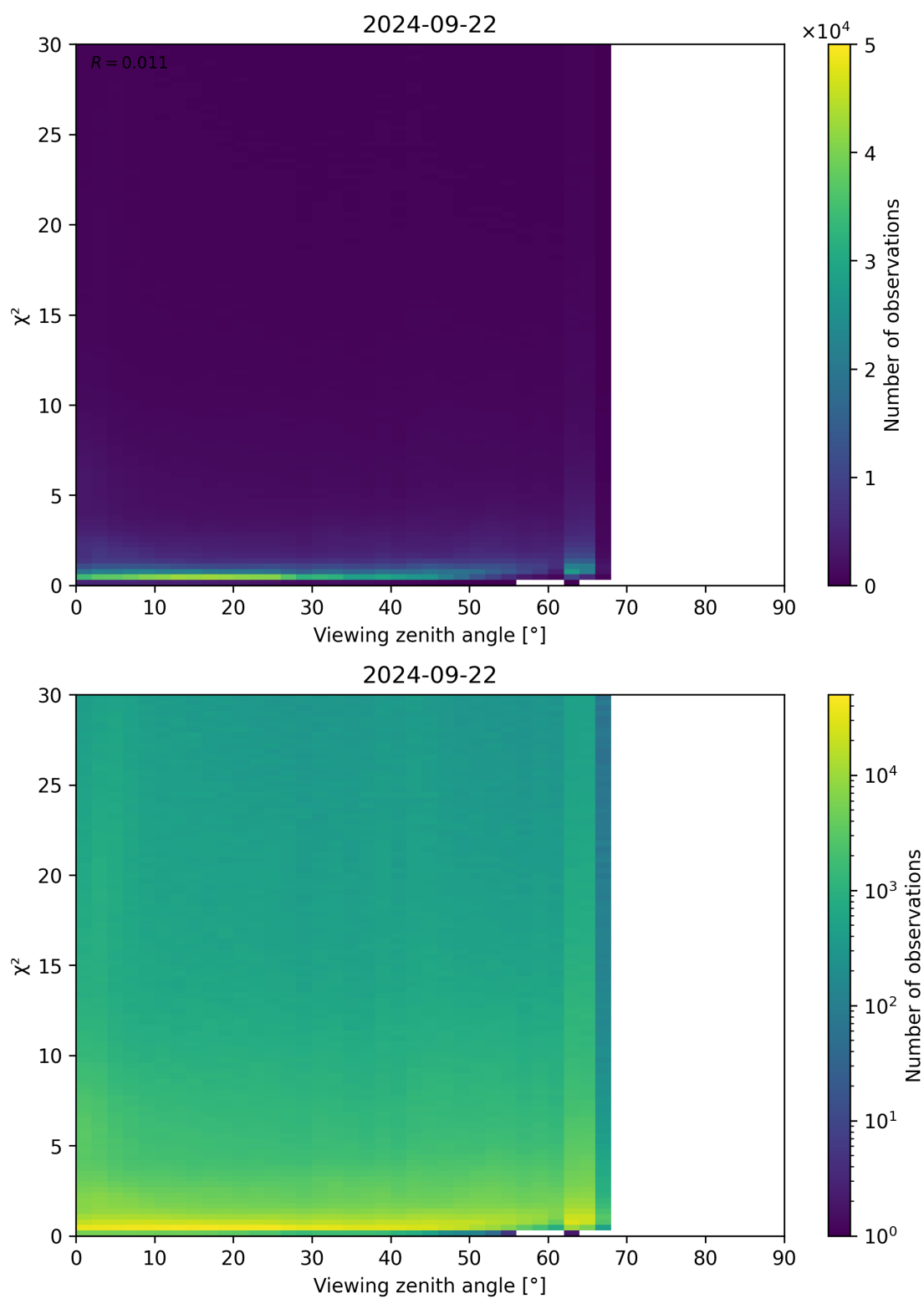
Figure 130: Scatter density plot of “Viewing zenith angle” against “ \chi^2 ” for 2024-09-22 to 2024-09-23.
