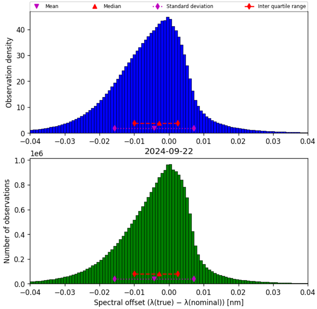
Figure 45: Histogram of “Spectral offset ( \lambda_{\text{true}} - \lambda_{\text{nominal}} )” for 2024-09-22 to 2024-09-23
