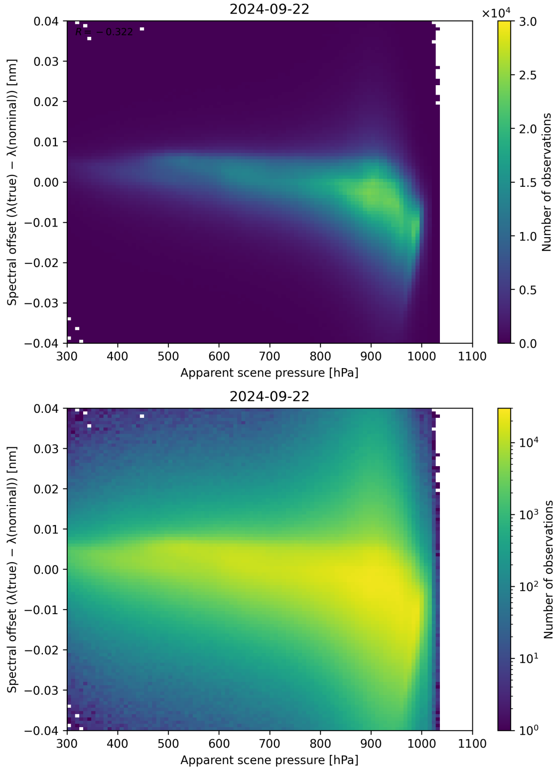
Figure 68: Scatter density plot of “Apparent scene pressure” against “Spectral offset ( \lambda_{\text{true}} - \lambda_{\text{nominal}} )” for 2024-09-22 to 2024-09-23.
