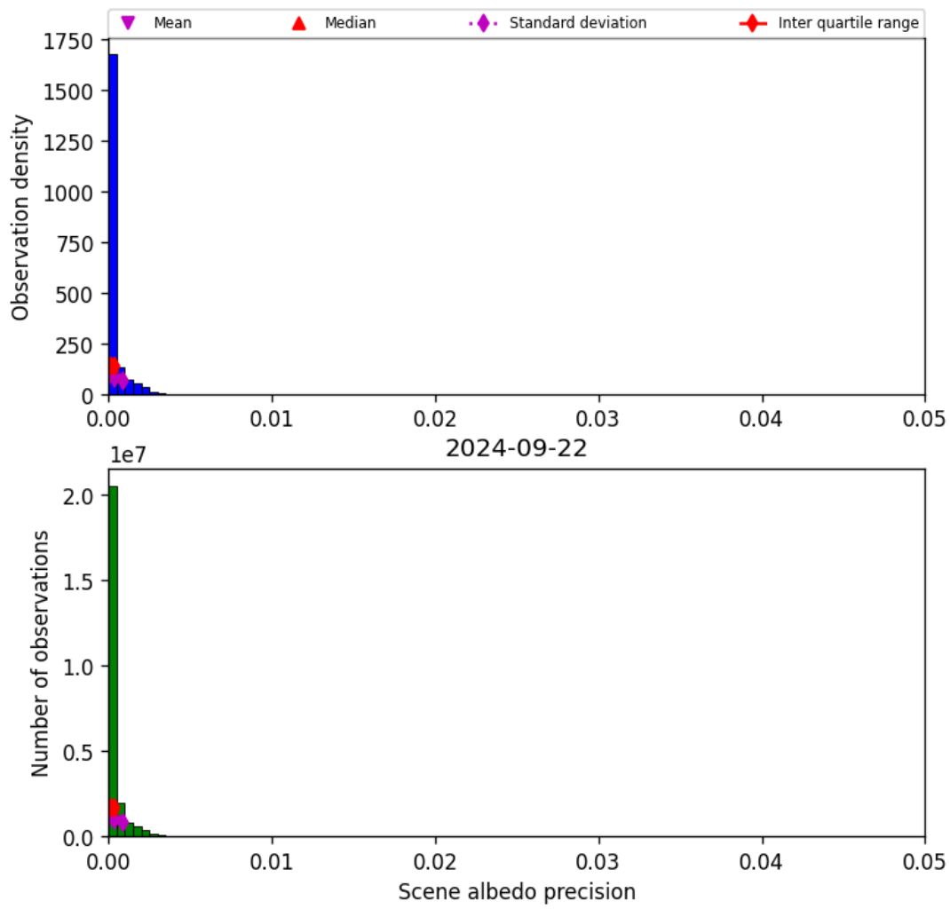
Figure 35: Histogram of “Scene albedo precision” for 2024-09-22 to 2024-09-23
