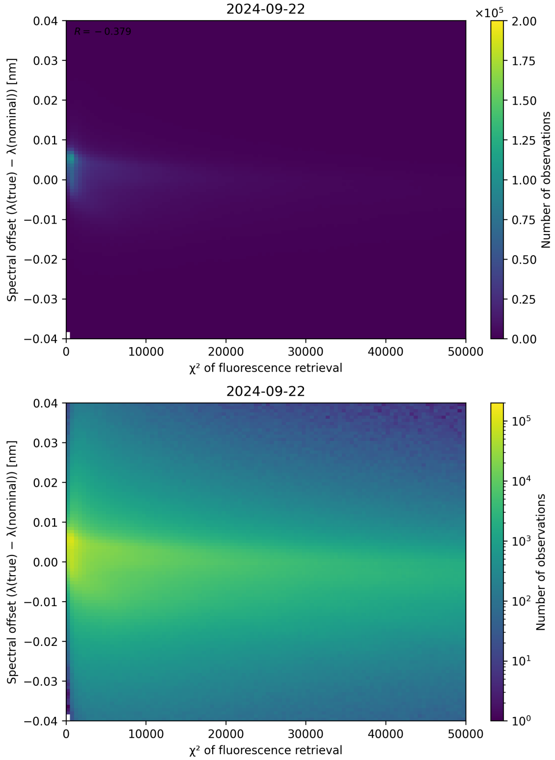
Figure 72: Scatter density plot of “ \chi^2 of fluorescence retrieval” against “Spectral offset ( \lambda_{\text{true}} - \lambda_{\text{nominal}} )” for 2024-09-22 to 2024-09-23.
