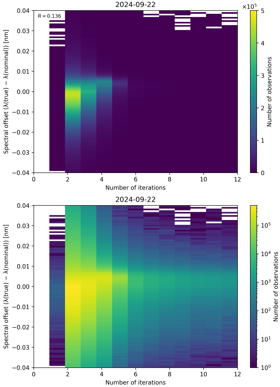
Figure 109: Scatter density plot of “Number of iterations” against “Spectral offset ( \lambda_{\text{true}} - \lambda_{\text{nominal}} )” for 2024-09-22 to 2024-09-23.
