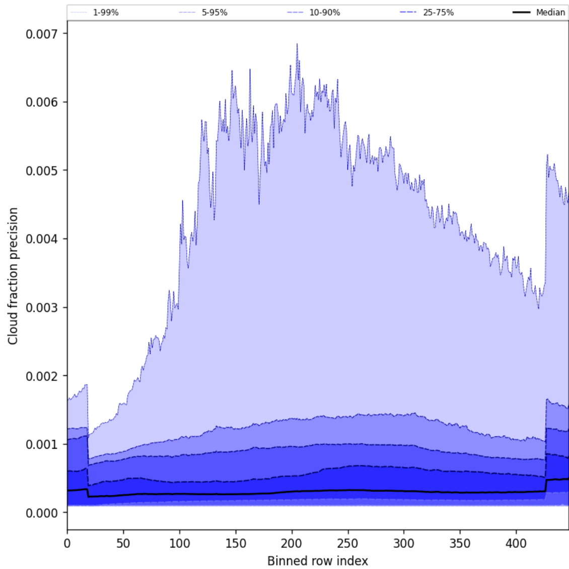
Figure 50: Along track statistics of “Cloud fraction precision” for 2024-09-22 to 2024-09-23
