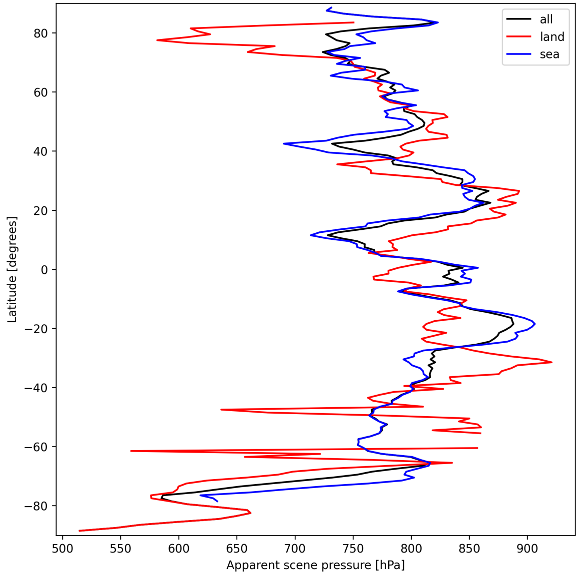
Figure 19: Zonal average of “Apparent scene pressure” for 2024-09-22 to 2024-09-23.
