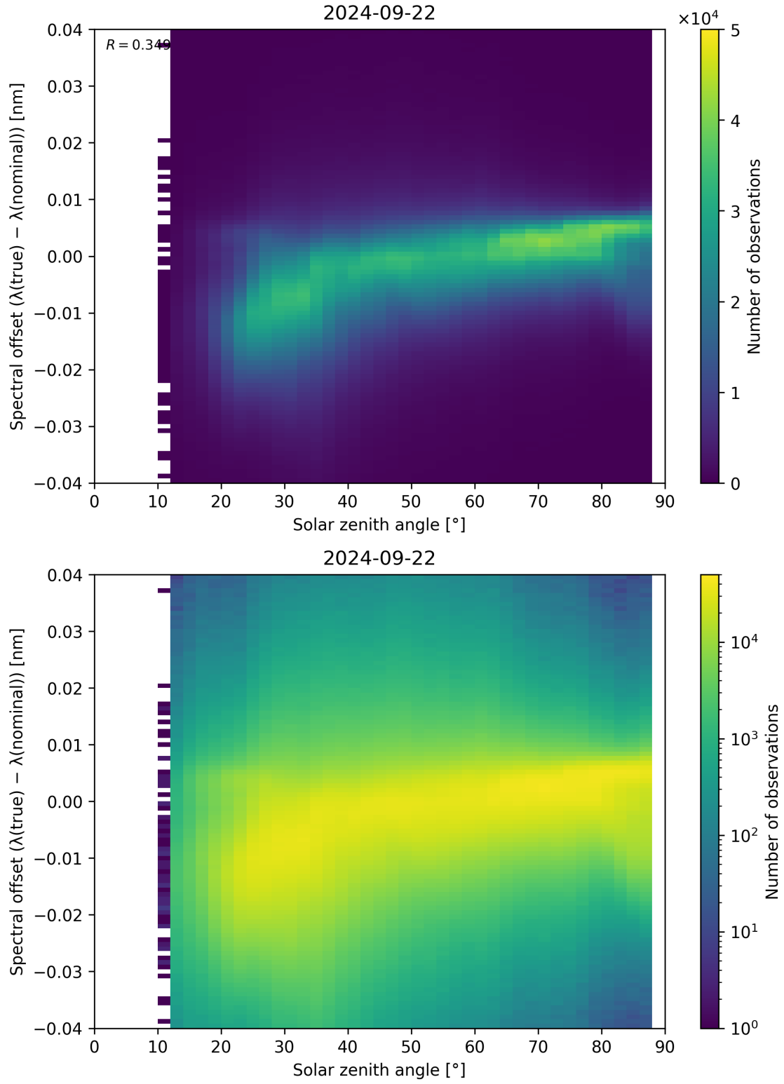
Figure 128: Scatter density plot of “Solar zenith angle” against “Spectral offset ( \lambda_{\text{true}} - \lambda_{\text{nominal}} )” for 2024-09-22 to 2024-09-23.
