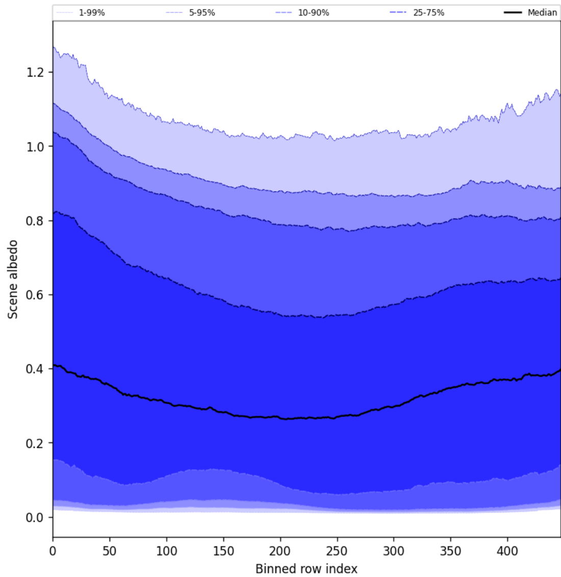
Figure 51: Along track statistics of “Scene albedo” for 2024-09-22 to 2024-09-23
