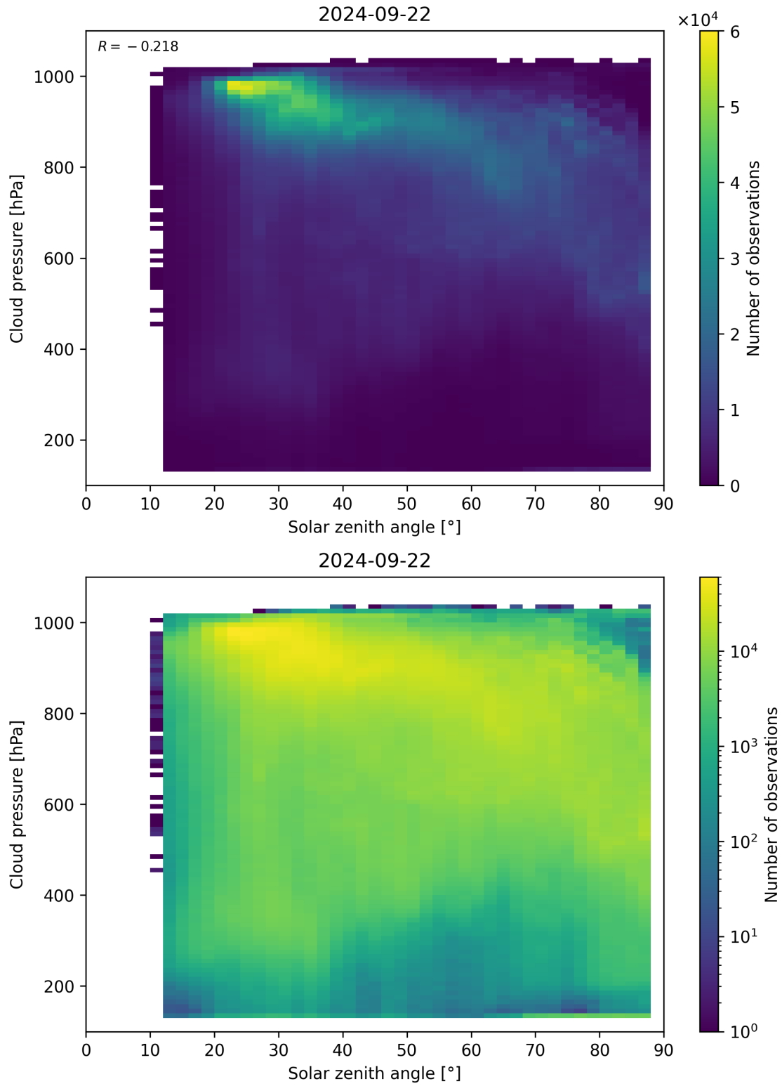
Figure 122: Scatter density plot of “Solar zenith angle” against “Cloud pressure” for 2024-09-22 to 2024-09-23.
