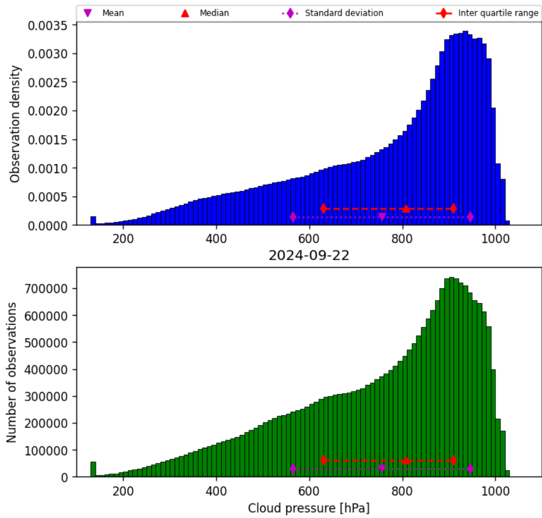
Figure 30: Histogram of “Cloud pressure” for 2024-09-22 to 2024-09-23
