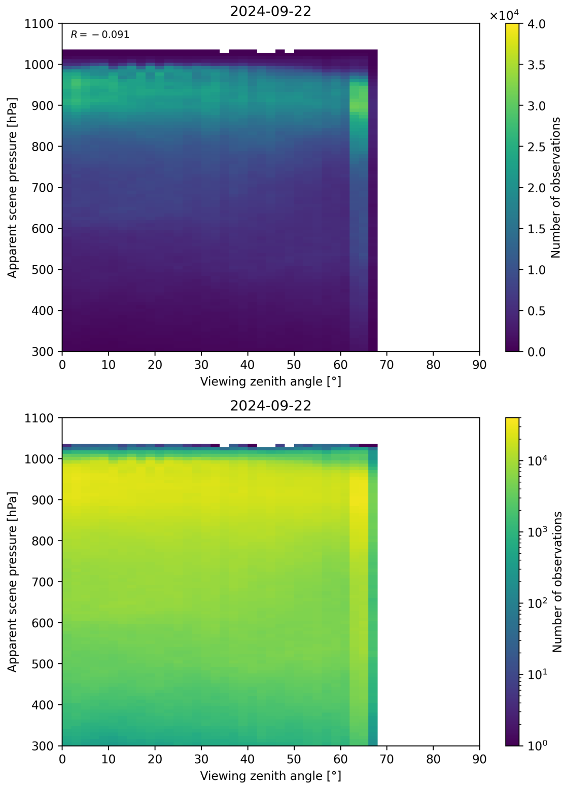
Figure 129: Scatter density plot of “Viewing zenith angle” against “Apparent scene pressure” for 2024-09-22 to 2024-09-23.
