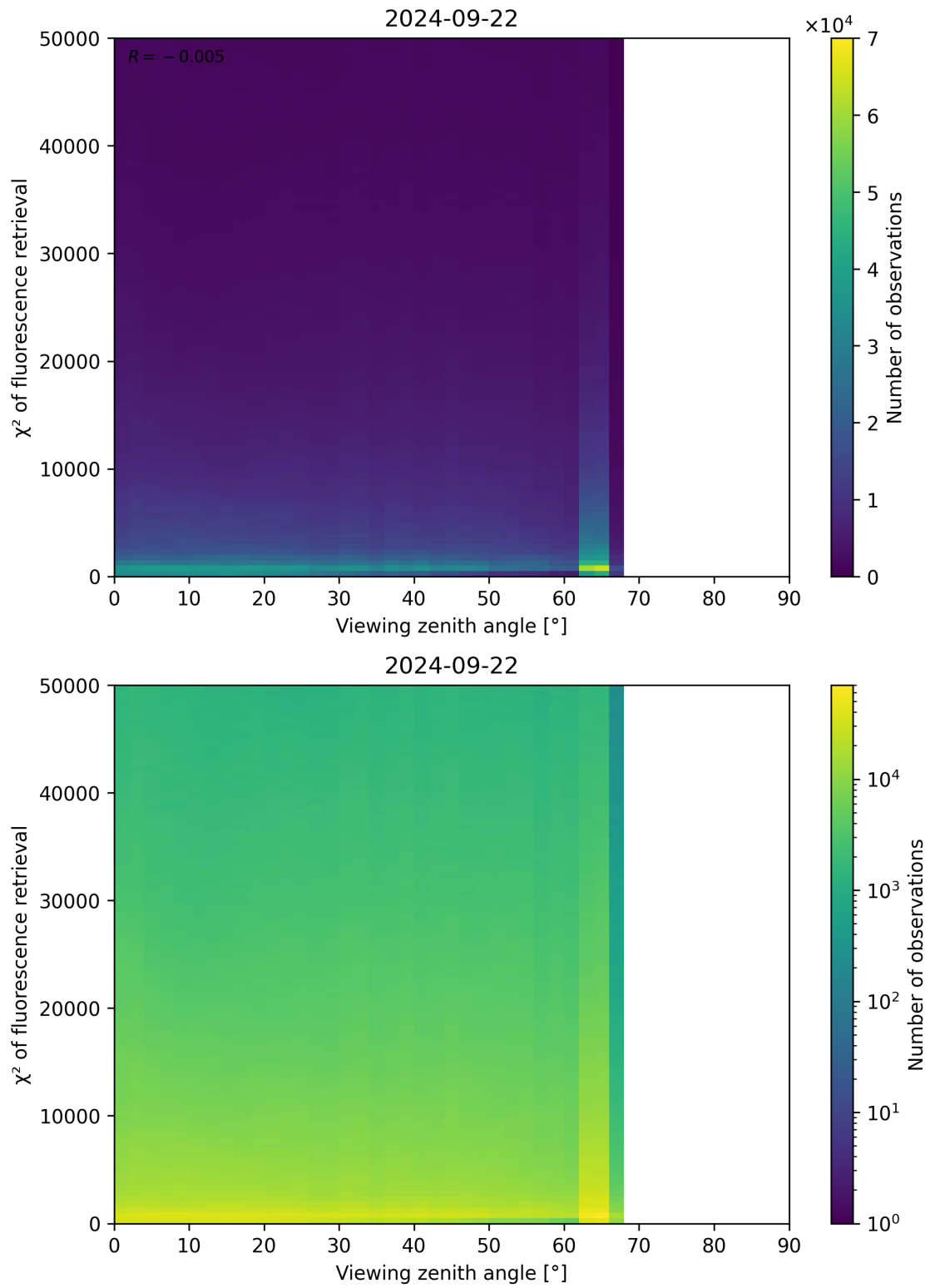
Figure 131: Scatter density plot of “Viewing zenith angle” against “ \chi^2 of fluorescence retrieval” for 2024-09-22 to 2024-09-23.
