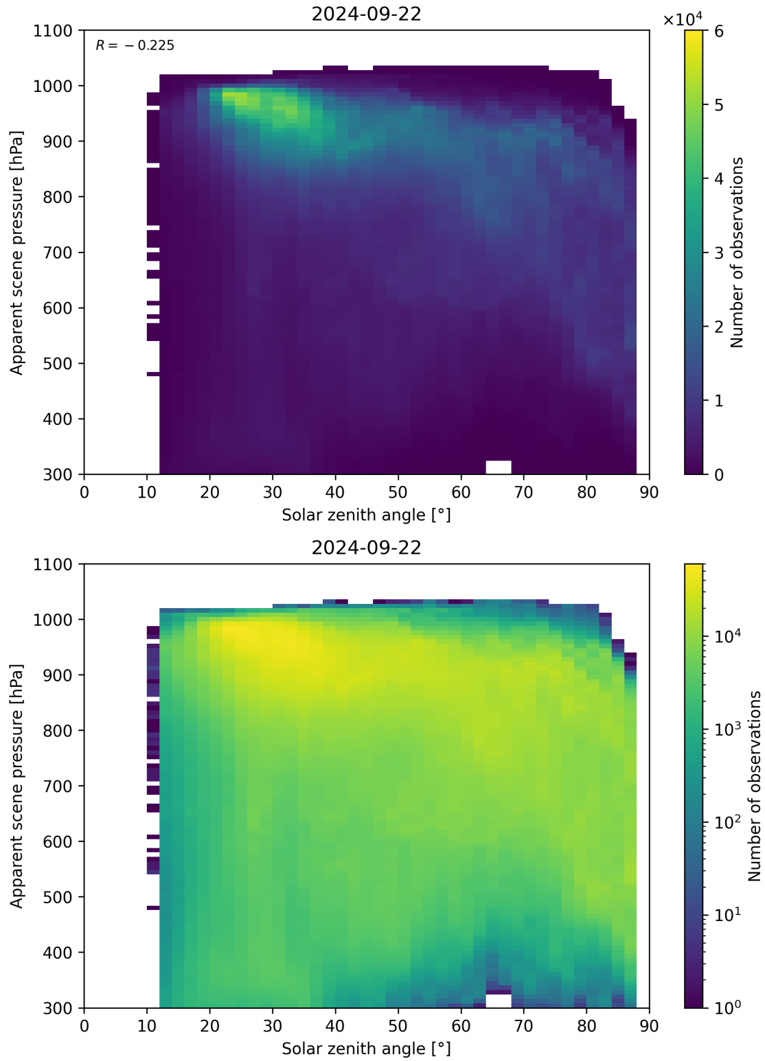
Figure 118: Scatter density plot of “Solar zenith angle” against “Apparent scene pressure” for 2024-09-22 to 2024-09-23.
