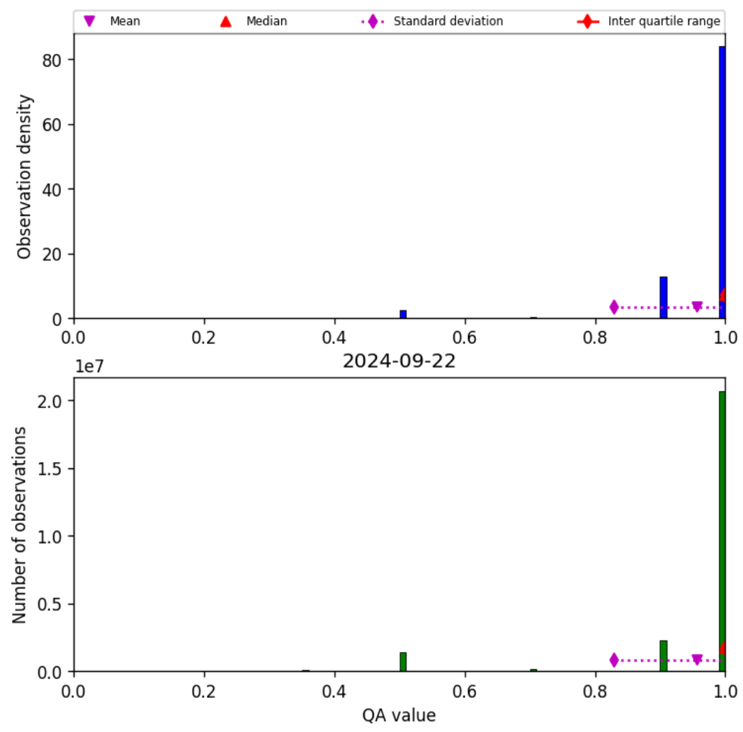
Figure 29: Histogram of “QA value” for 2024-09-22 to 2024-09-23
