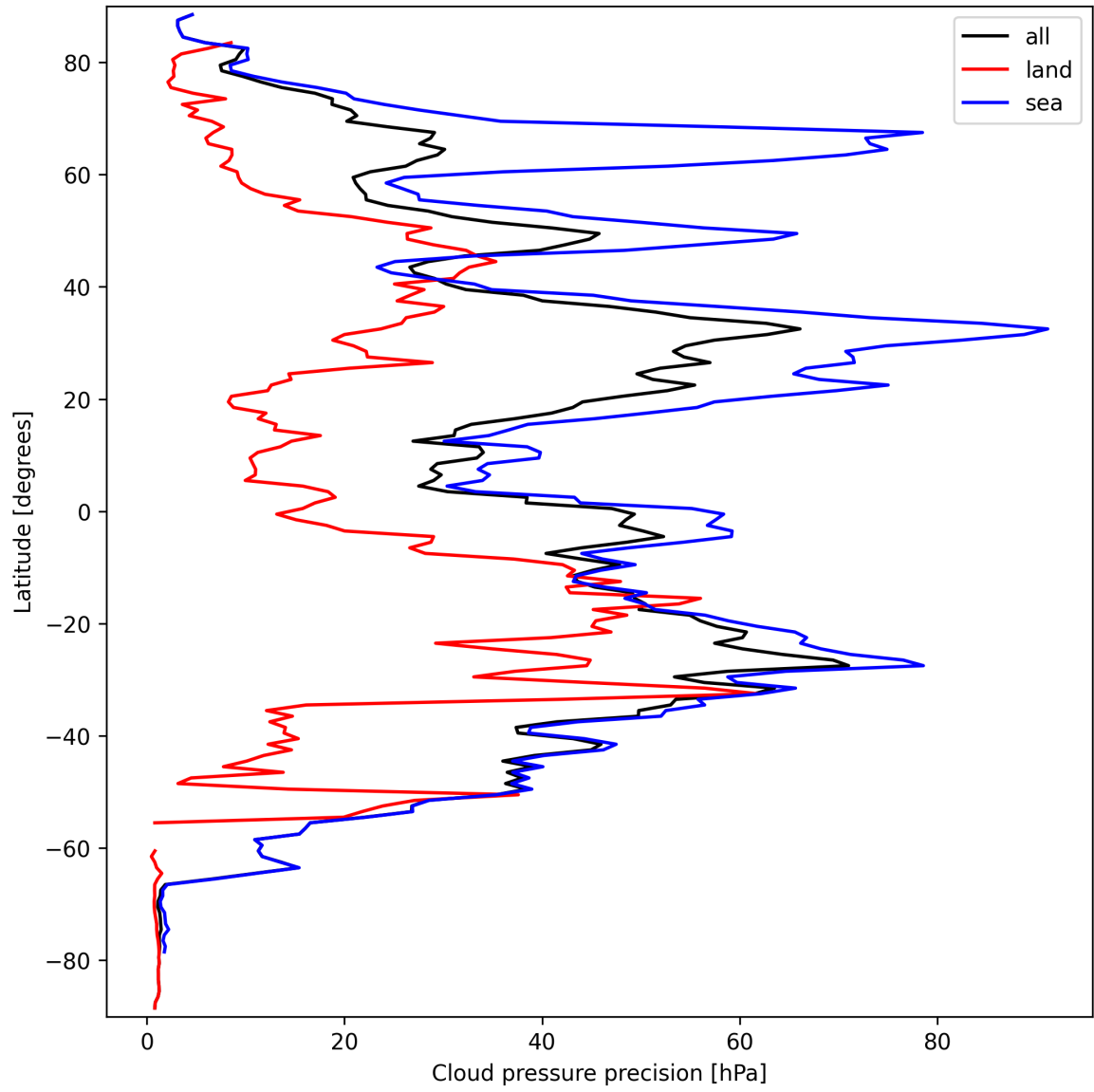
Figure 14: Zonal average of "Cloud pressure precision" for 2024-09-22 to 2024-09-23.
