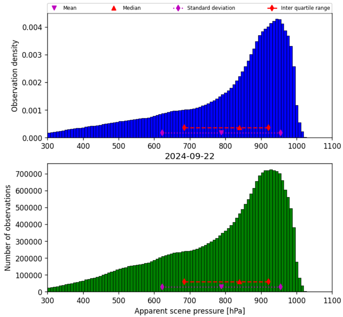
Figure 36: Histogram of “Apparent scene pressure” for 2024-09-22 to 2024-09-23
