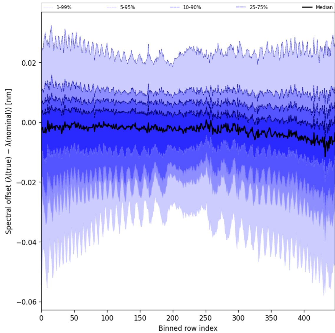
Figure 62: Along track statistics of “Spectral offset ( \lambda_{\text{true}} - \lambda_{\text{nominal}} )” for 2024-09-22 to 2024-09-23
