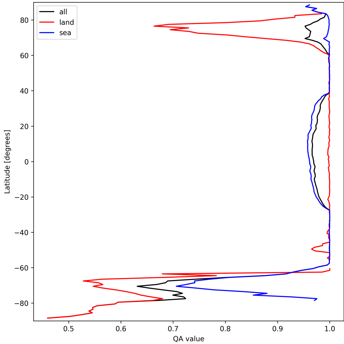
Figure 12: Zonal average of "QA value" for 2024-09-22 to 2024-09-23.
