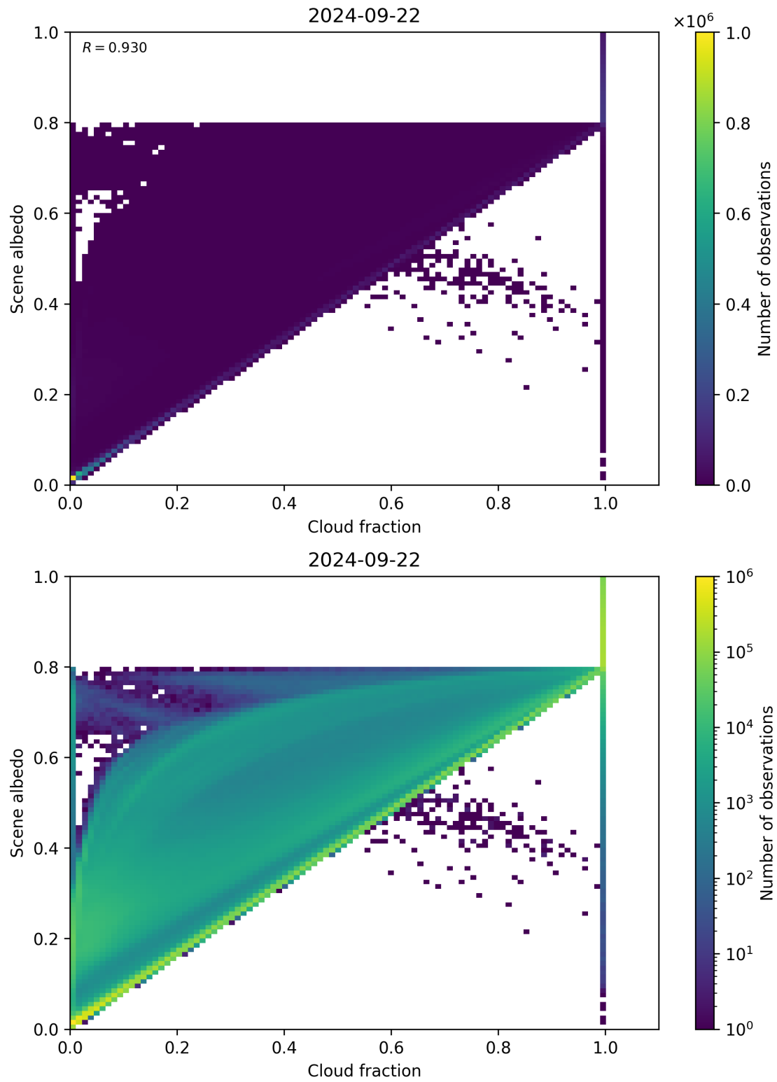
Figure 82: Scatter density plot of “Cloud fraction” against “Scene albedo” for 2024-09-22 to 2024-09-23.
