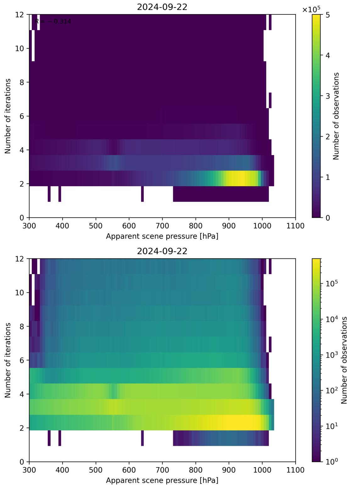
Figure 66: Scatter density plot of “Apparent scene pressure” against “Number of iterations” for 2024-09-22 to 2024-09-23.
