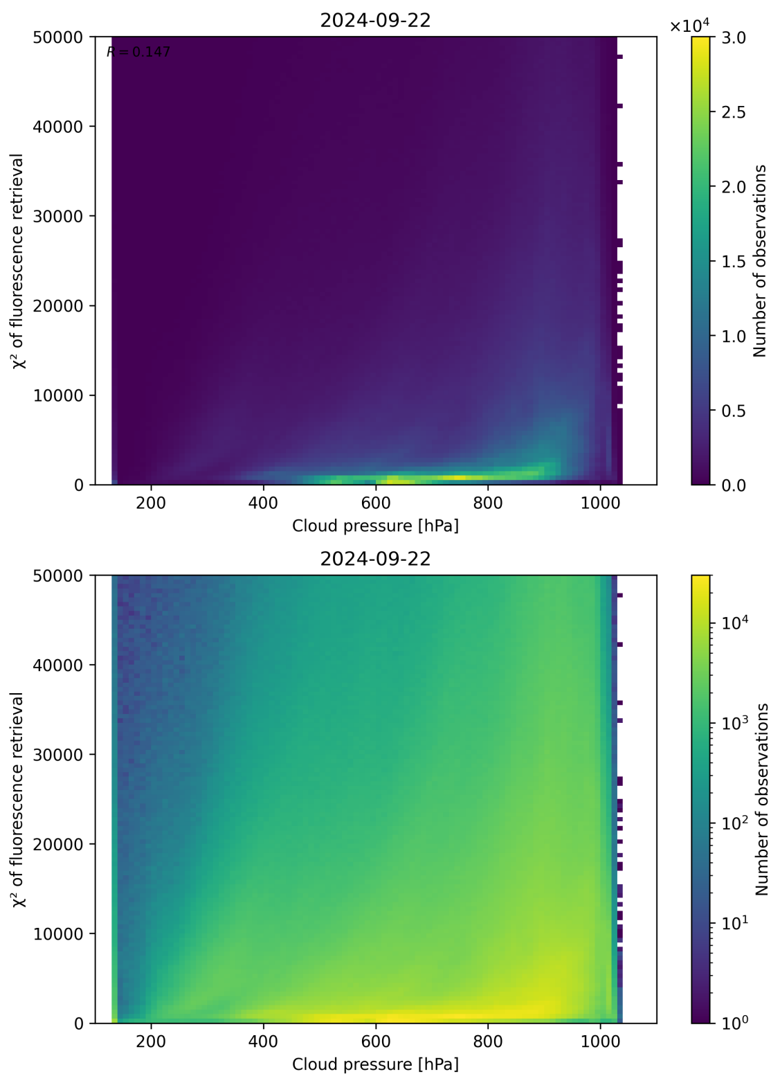
Figure 86: Scatter density plot of “Cloud pressure” against “ \chi^2 of fluorescence retrieval” for 2024-09-22 to 2024-09-23.
