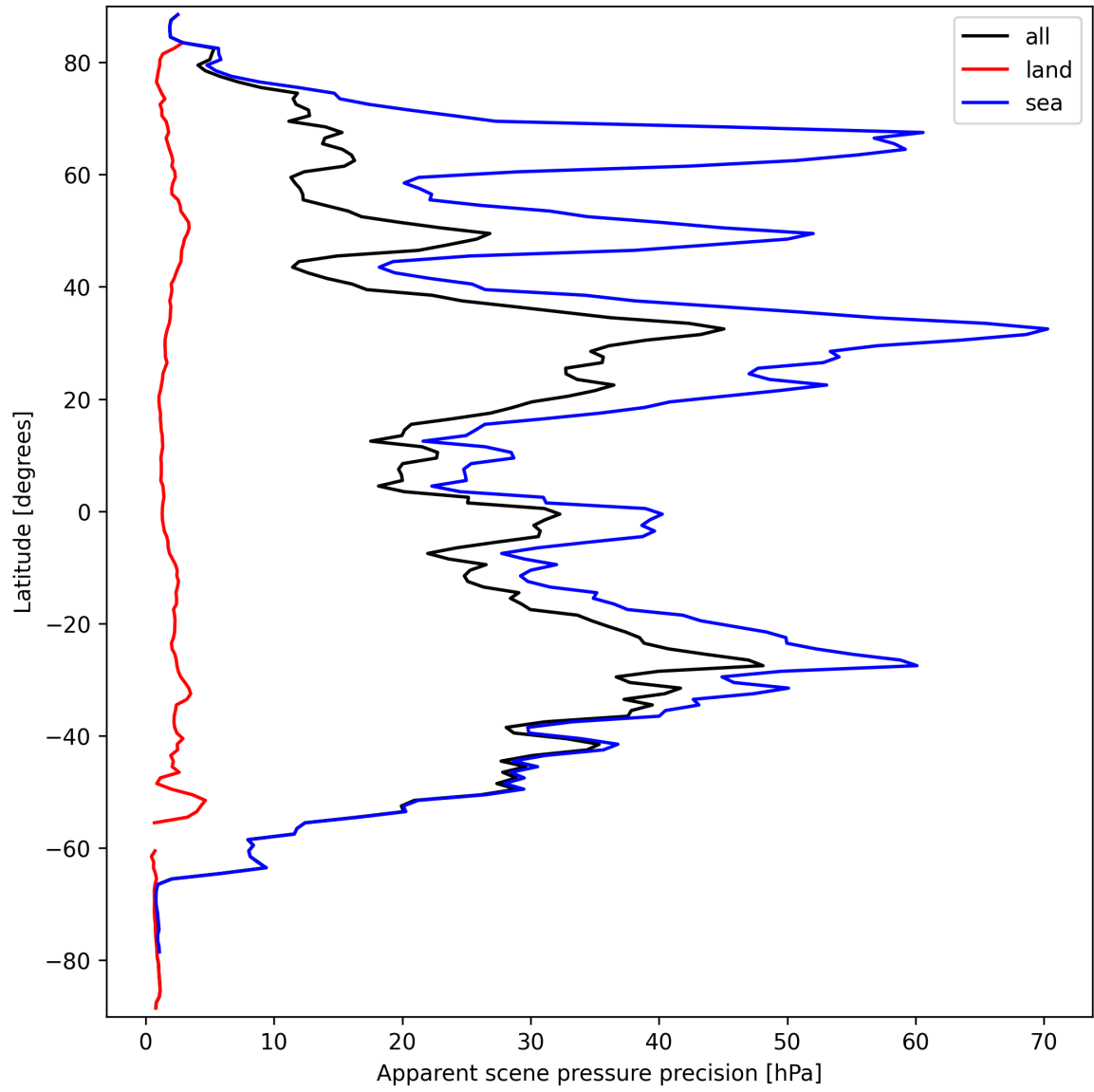
Figure 20: Zonal average of “Apparent scene pressure precision” for 2024-09-22 to 2024-09-23.
