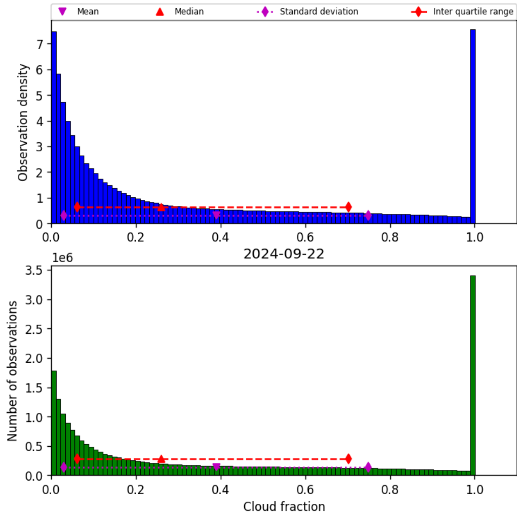
Figure 32: Histogram of “Cloud fraction” for 2024-09-22 to 2024-09-23
