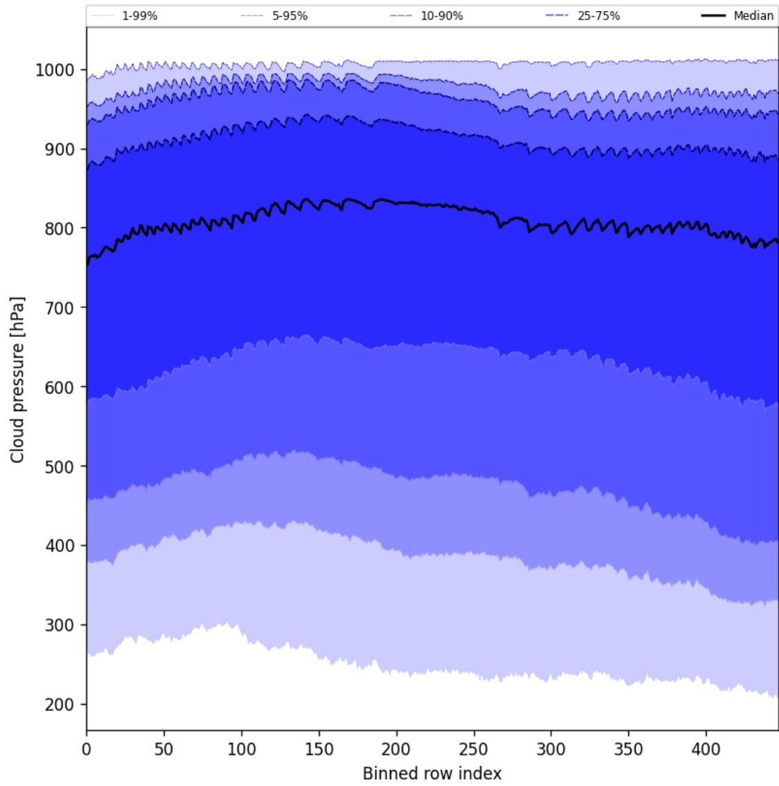
Figure 47: Along track statistics of “Cloud pressure” for 2024-09-22 to 2024-09-23
