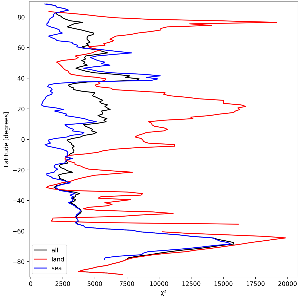
Figure 21: Zonal average of “ \chi^2 ” for 2024-09-22 to 2024-09-23.
