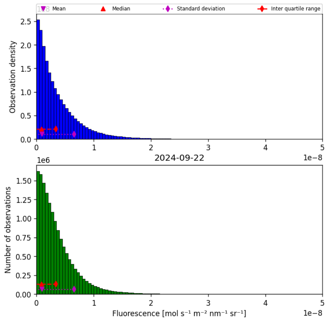
Figure 40: Histogram of “Fluorescence” for 2024-09-22 to 2024-09-23
