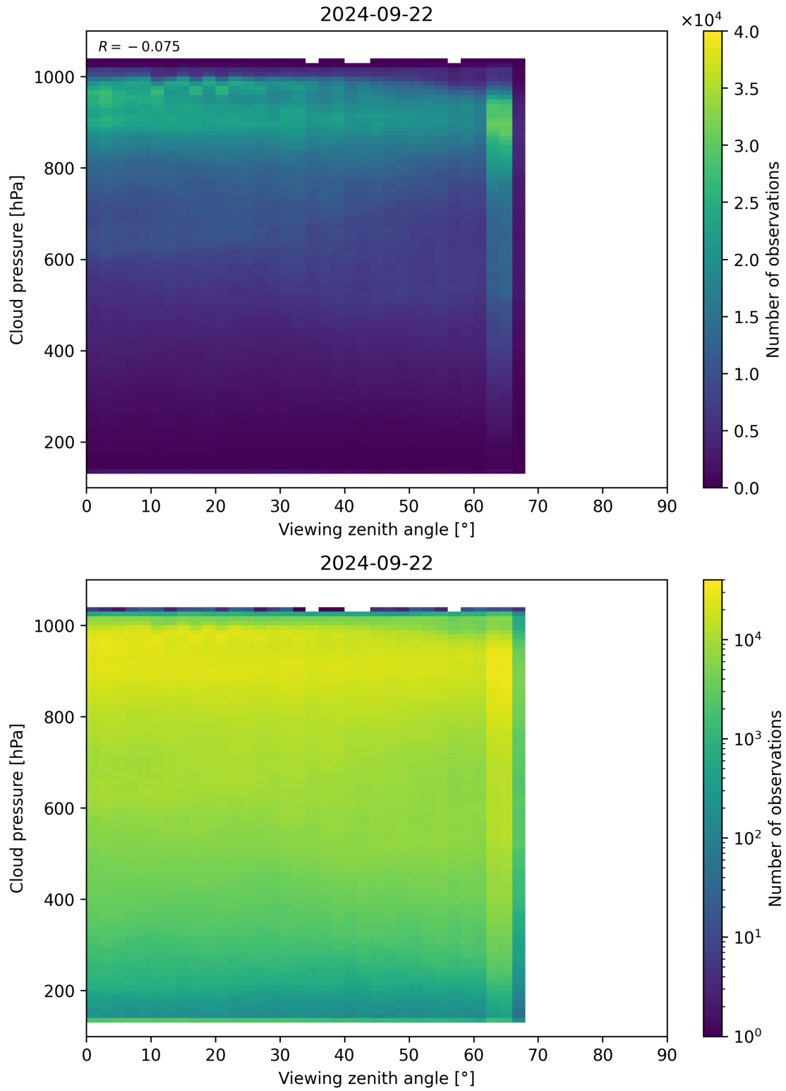
Figure 133: Scatter density plot of “Viewing zenith angle” against “Cloud pressure” for 2024-09-22 to 2024-09-23.
