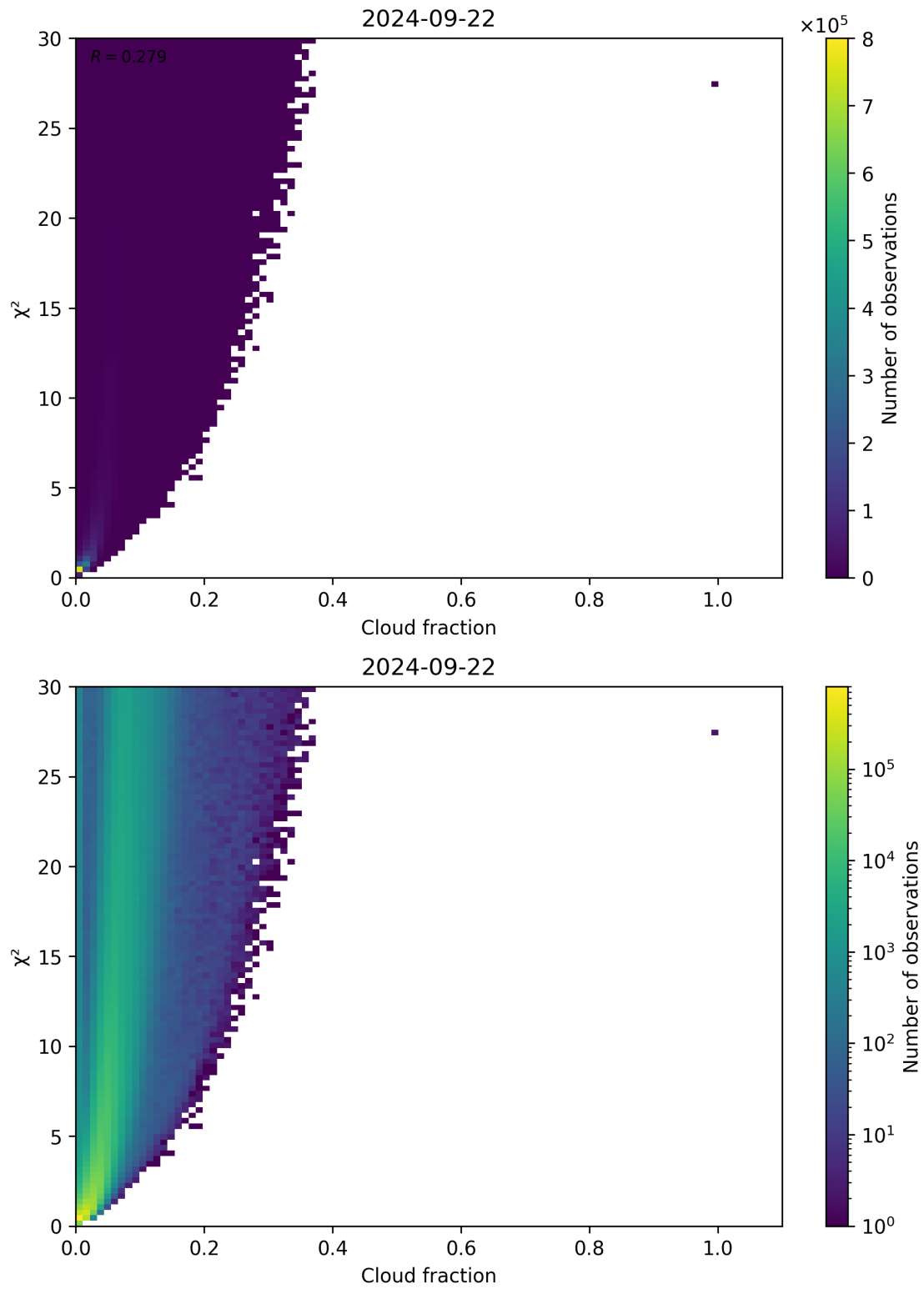
Figure 77: Scatter density plot of “Cloud fraction” against “ \chi^2 ” for 2024-09-22 to 2024-09-23.
