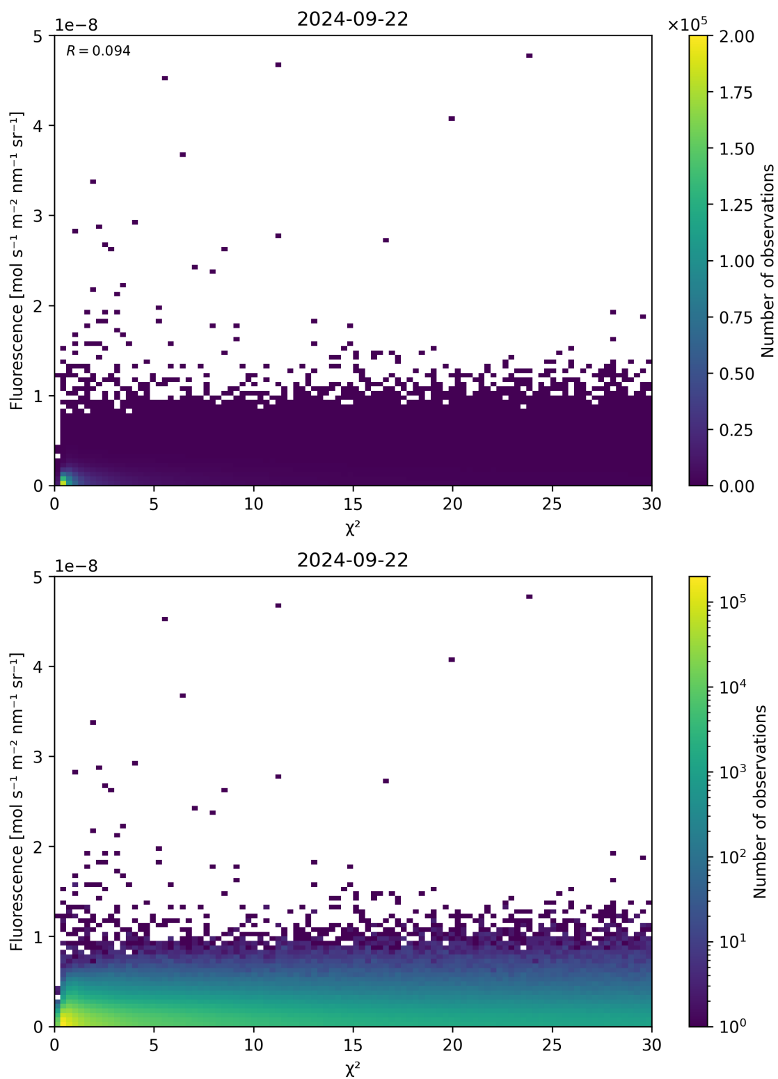
Figure 70: Scatter density plot of “ \chi^2 ” against “Fluorescence” for 2024-09-22 to 2024-09-23.
