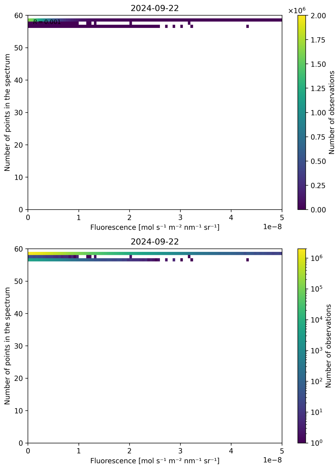
Figure 94: Scatter density plot of “Fluorescence” against “Number of points in the spectrum” for 2024-09-22 to 2024-09-23.
