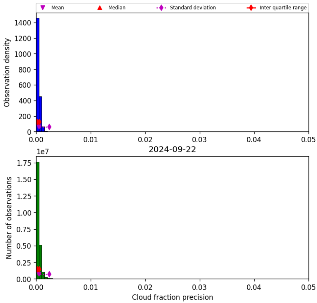
Figure 33: Histogram of “Cloud fraction precision” for 2024-09-22 to 2024-09-23
