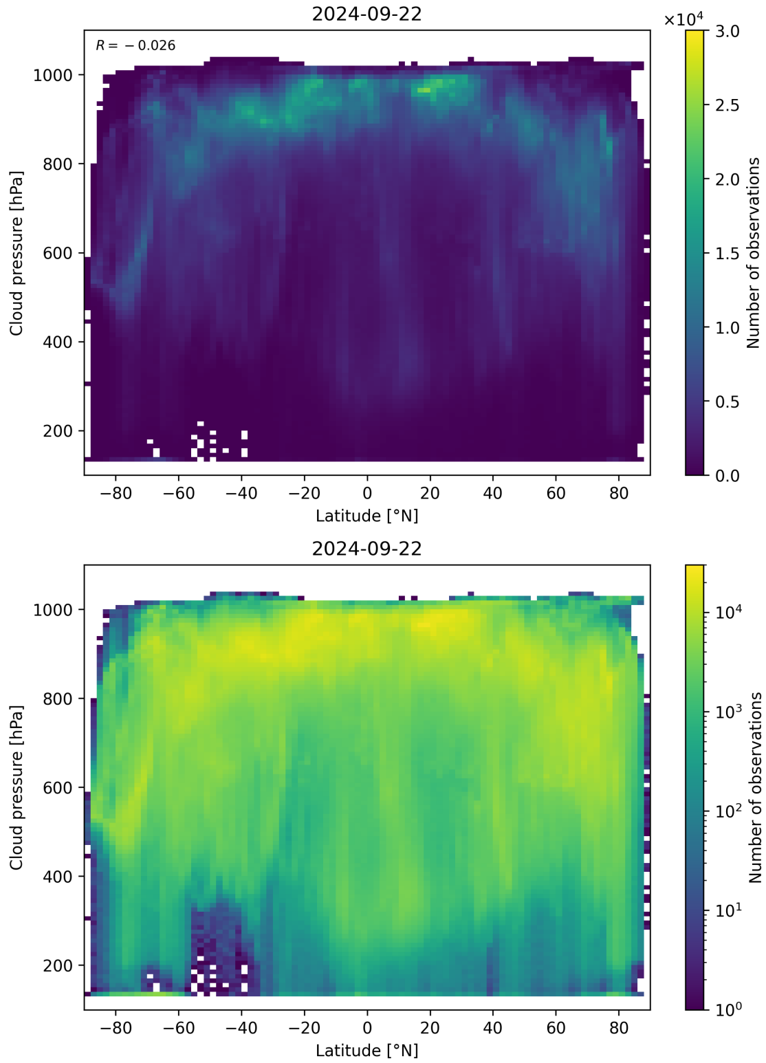
Figure 100: Scatter density plot of “Latitude” against “Cloud pressure” for 2024-09-22 to 2024-09-23.
