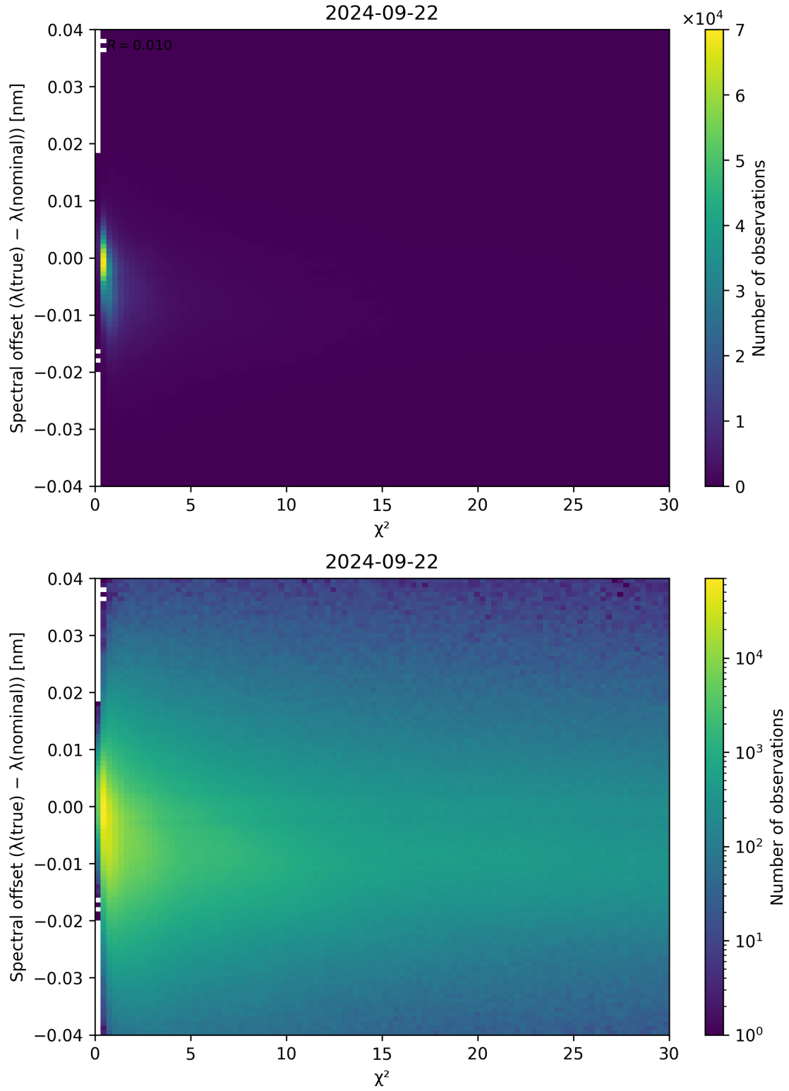
Figure 75: Scatter density plot of “ \chi^2 ” against “Spectral offset ( \lambda_{\text{true}} - \lambda_{\text{nominal}} )” for 2024-09-22 to 2024-09-23.
