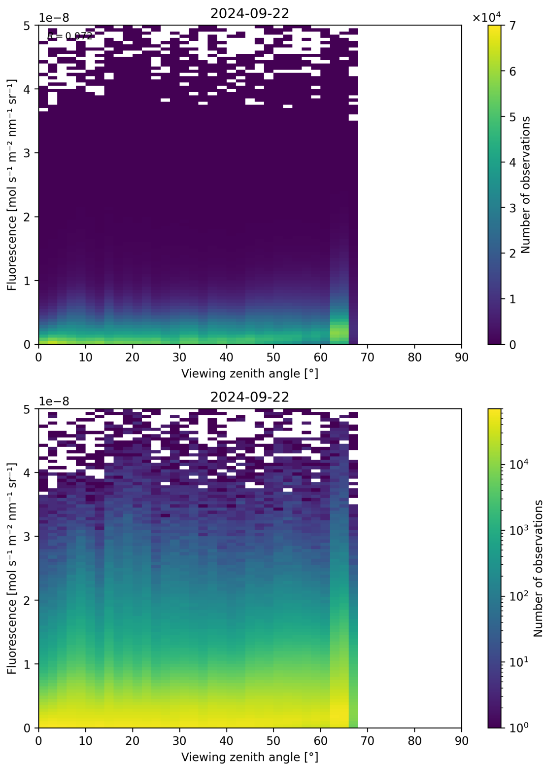
Figure 134: Scatter density plot of “Viewing zenith angle” against “Fluorescence” for 2024-09-22 to 2024-09-23.
