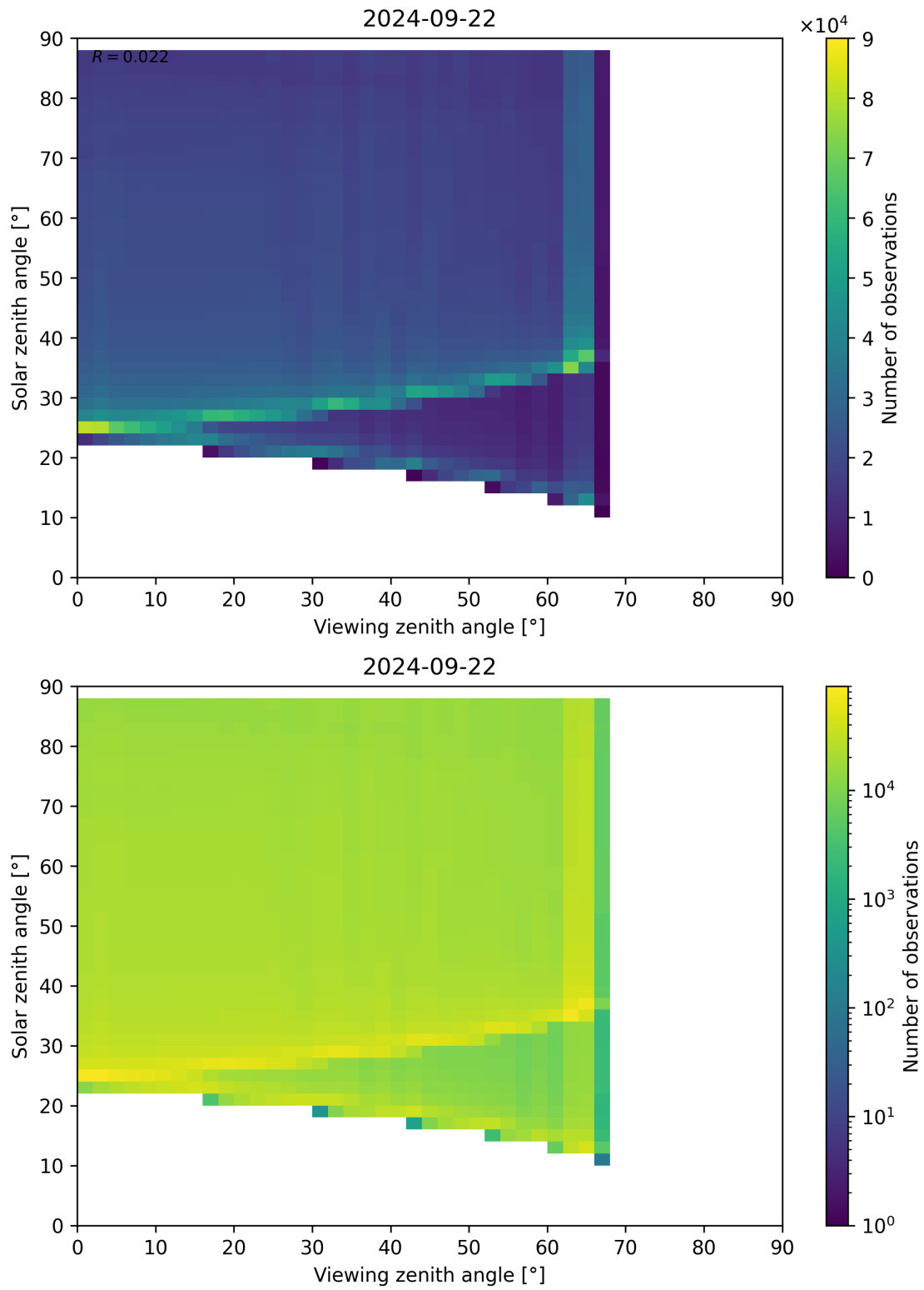
Figure 139: Scatter density plot of “Viewing zenith angle” against “Solar zenith angle” for 2024-09-22 to 2024-09-23.
