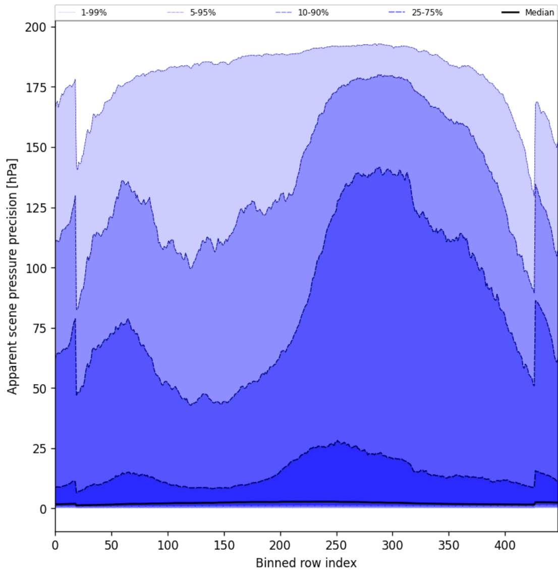
Figure 54: Along track statistics of “Apparent scene pressure precision” for 2024-09-22 to 2024-09-23
