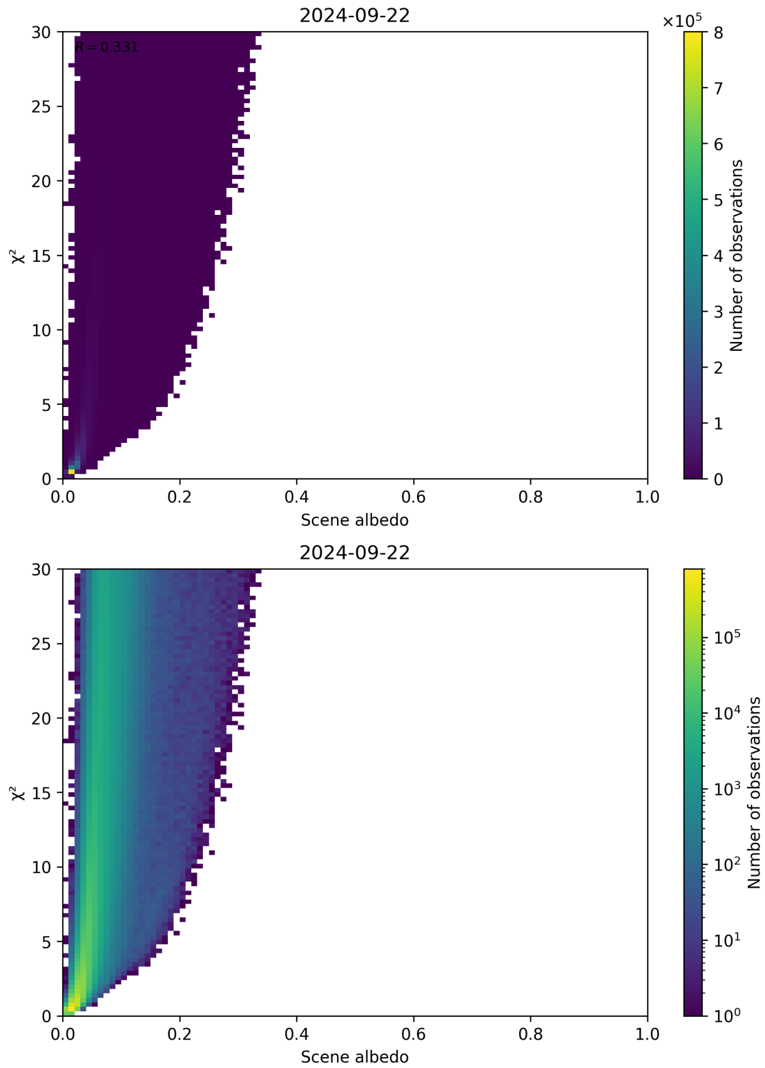
Figure 112: Scatter density plot of “Scene albedo” against “ \chi^2 ” for 2024-09-22 to 2024-09-23.
