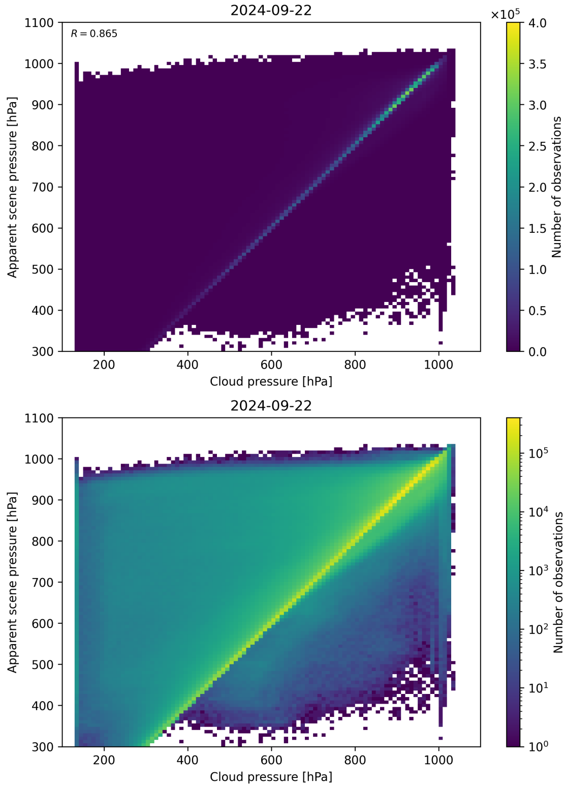
Figure 84: Scatter density plot of “Cloud pressure” against “Apparent scene pressure” for 2024-09-22 to 2024-09-23.
