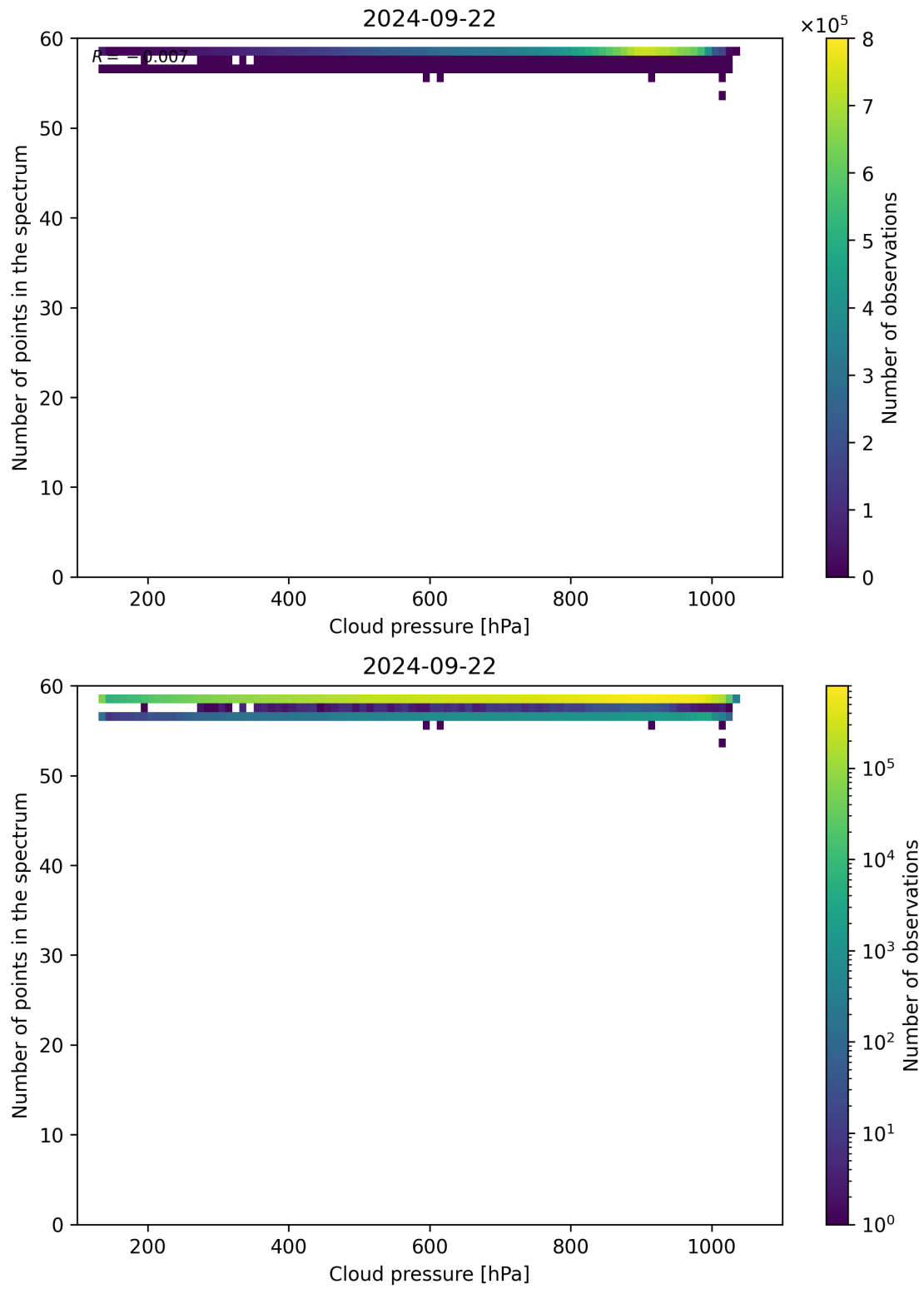
Figure 90: Scatter density plot of “Cloud pressure” against “Number of points in the spectrum” for 2024-09-22 to 2024-09-23.
