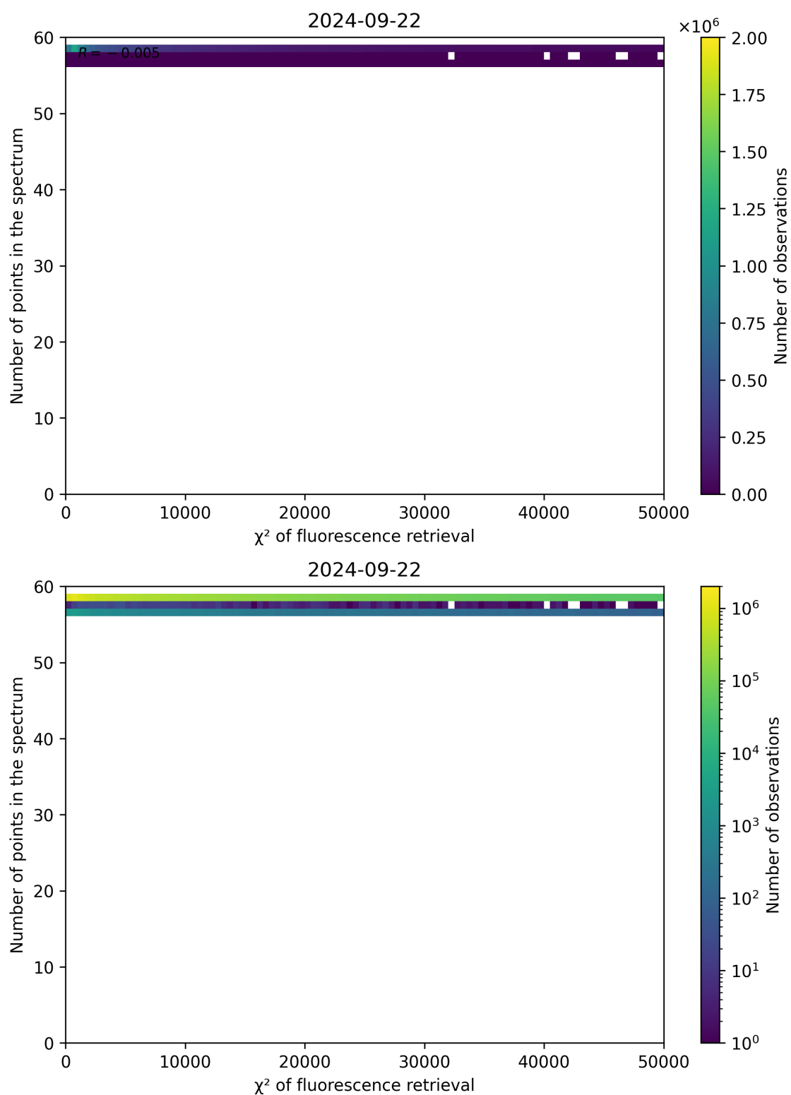
Figure 71: Scatter density plot of “ \chi^2 of fluorescence retrieval” against “Number of points in the spectrum” for 2024-09-22 to 2024-09-23.
