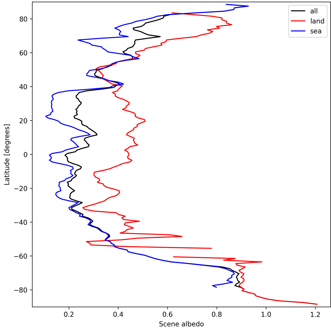
Figure 17: Zonal average of “Scene albedo” for 2024-09-22 to 2024-09-23.
