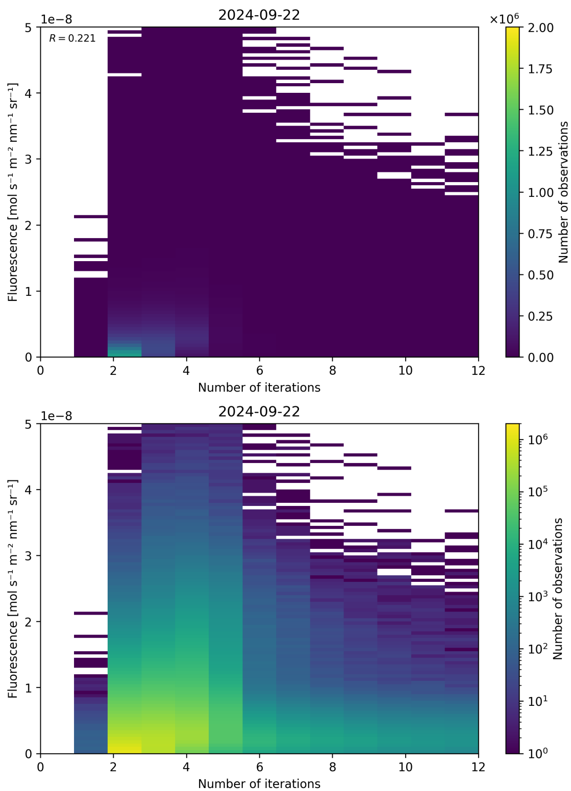
Figure 107: Scatter density plot of “Number of iterations” against “Fluorescence” for 2024-09-22 to 2024-09-23.
