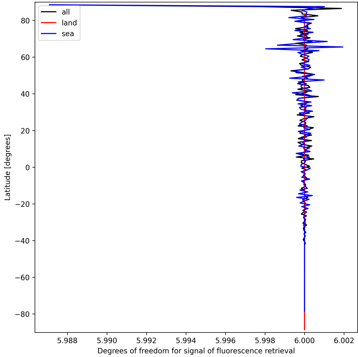
Figure 26: Zonal average of “Degrees of freedom for signal of fluorescence retrieval” for 2024-09-22 to 2024-09-23.
