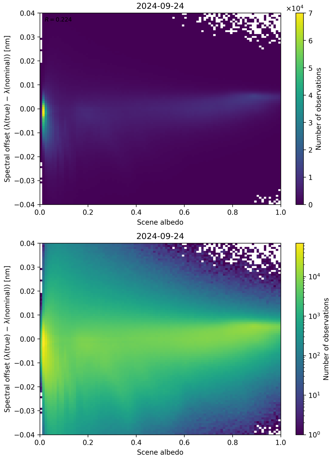
Figure 117: Scatter density plot of “Scene albedo” against “Spectral offset ( \lambda_{\text{true}} - \lambda_{\text{nominal}} )” for 2024-09-23 to 2024-09-25.
