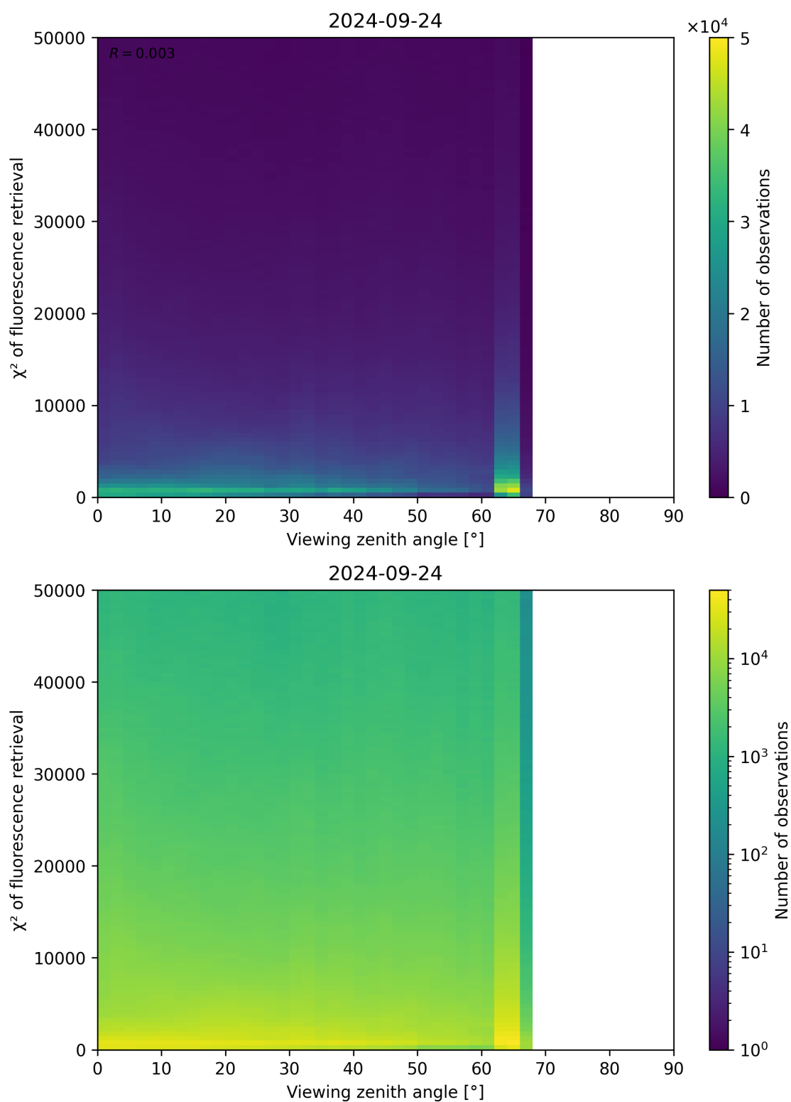
Figure 131: Scatter density plot of “Viewing zenith angle” against “ \chi^2 of fluorescence retrieval” for 2024-09-23 to 2024-09-25.
