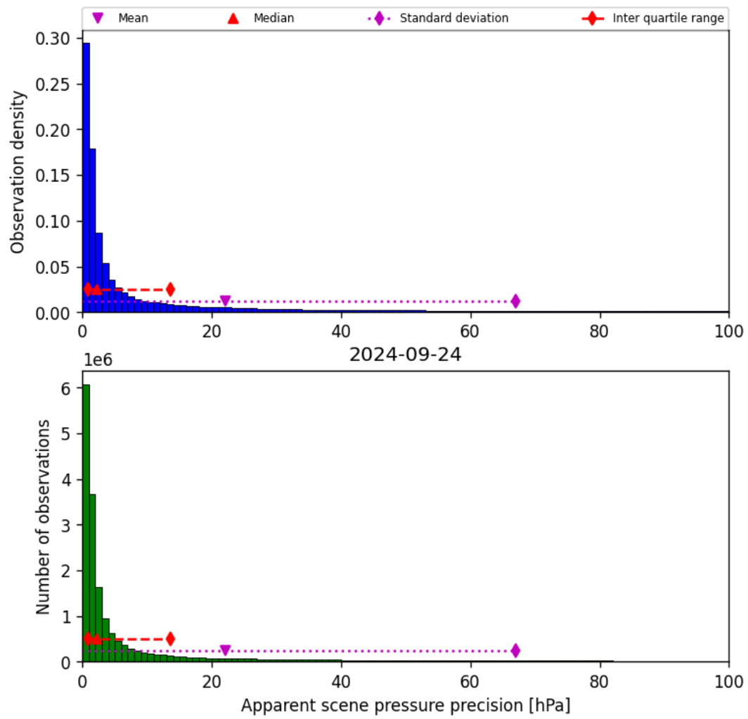
Figure 37: Histogram of “Apparent scene pressure precision” for 2024-09-23 to 2024-09-25
