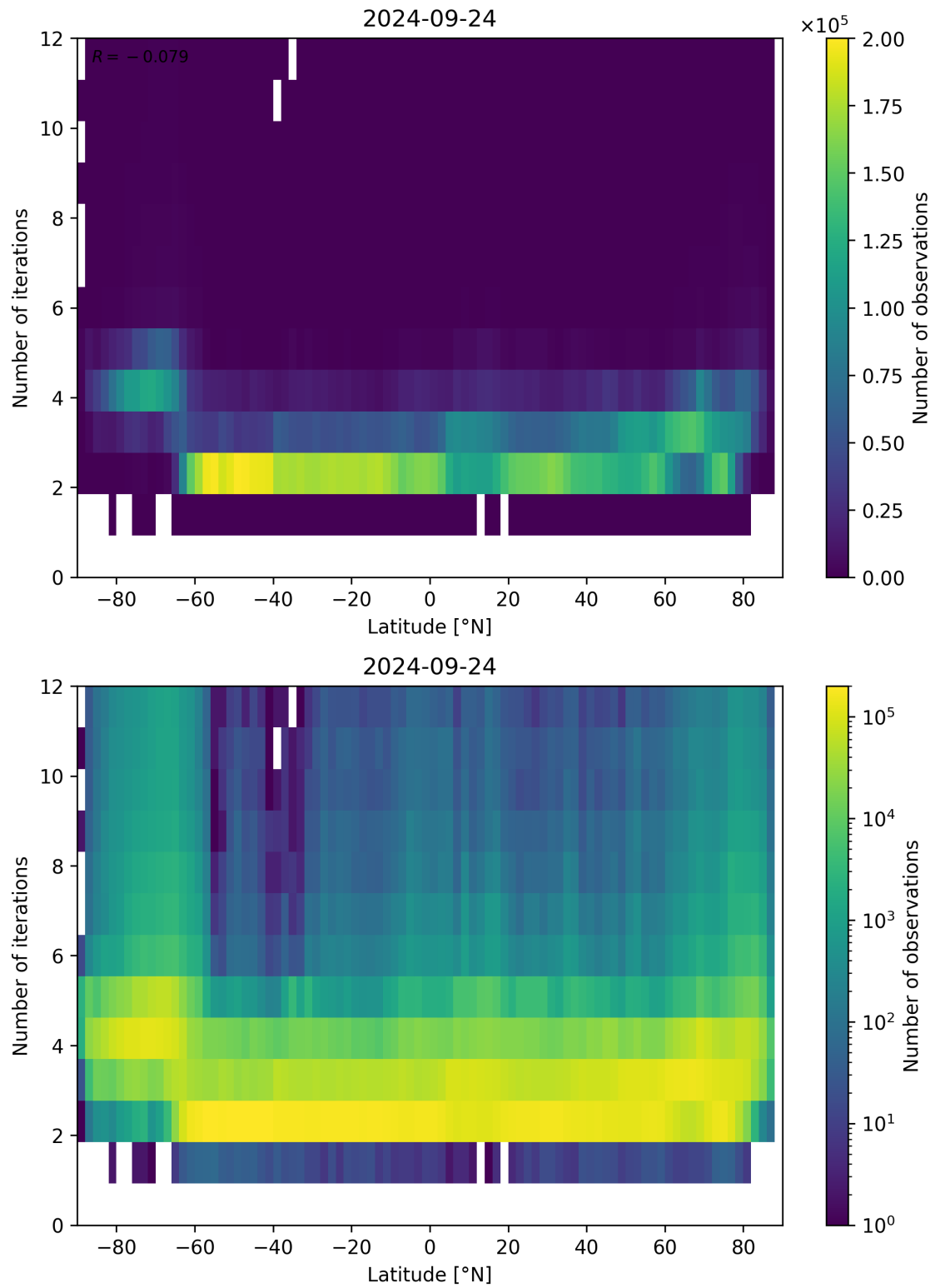
Figure 102: Scatter density plot of “Latitude” against “Number of iterations” for 2024-09-23 to 2024-09-25.
