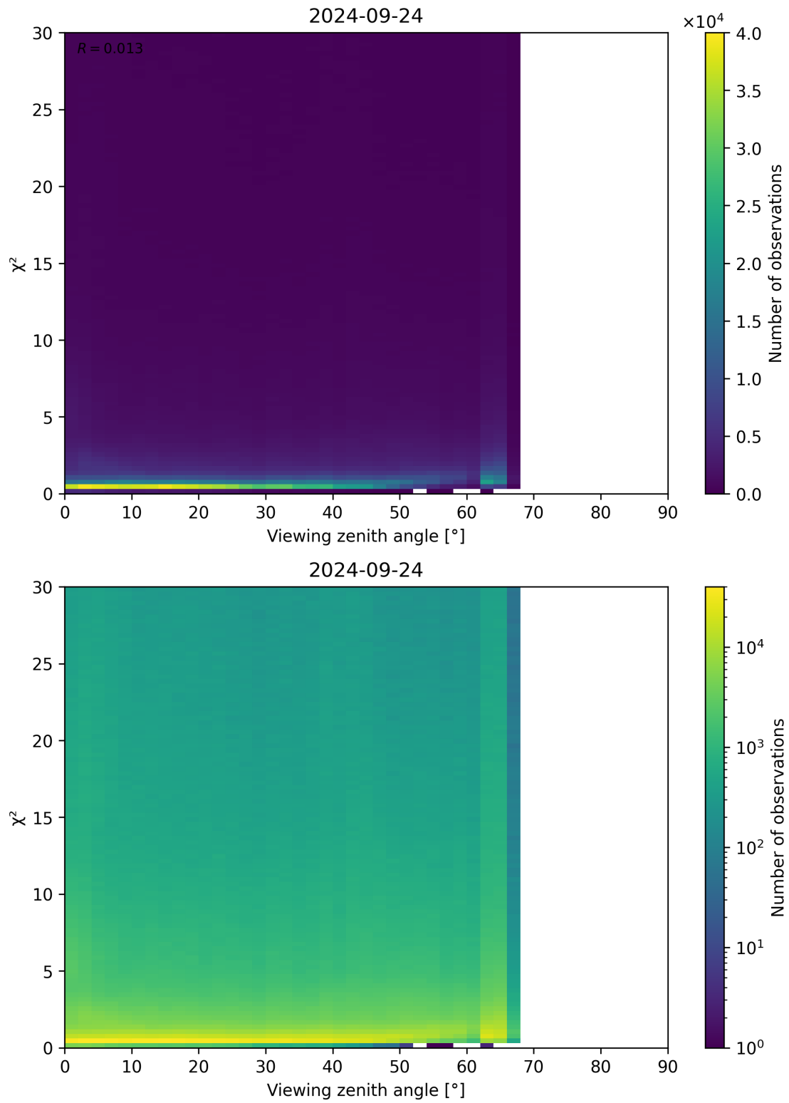
Figure 130: Scatter density plot of “Viewing zenith angle” against “ \chi^2 ” for 2024-09-23 to 2024-09-25.
