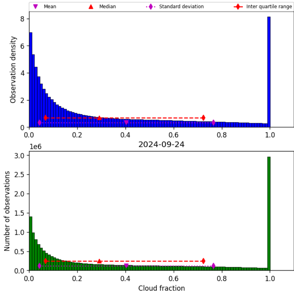
Figure 32: Histogram of “Cloud fraction” for 2024-09-23 to 2024-09-25
