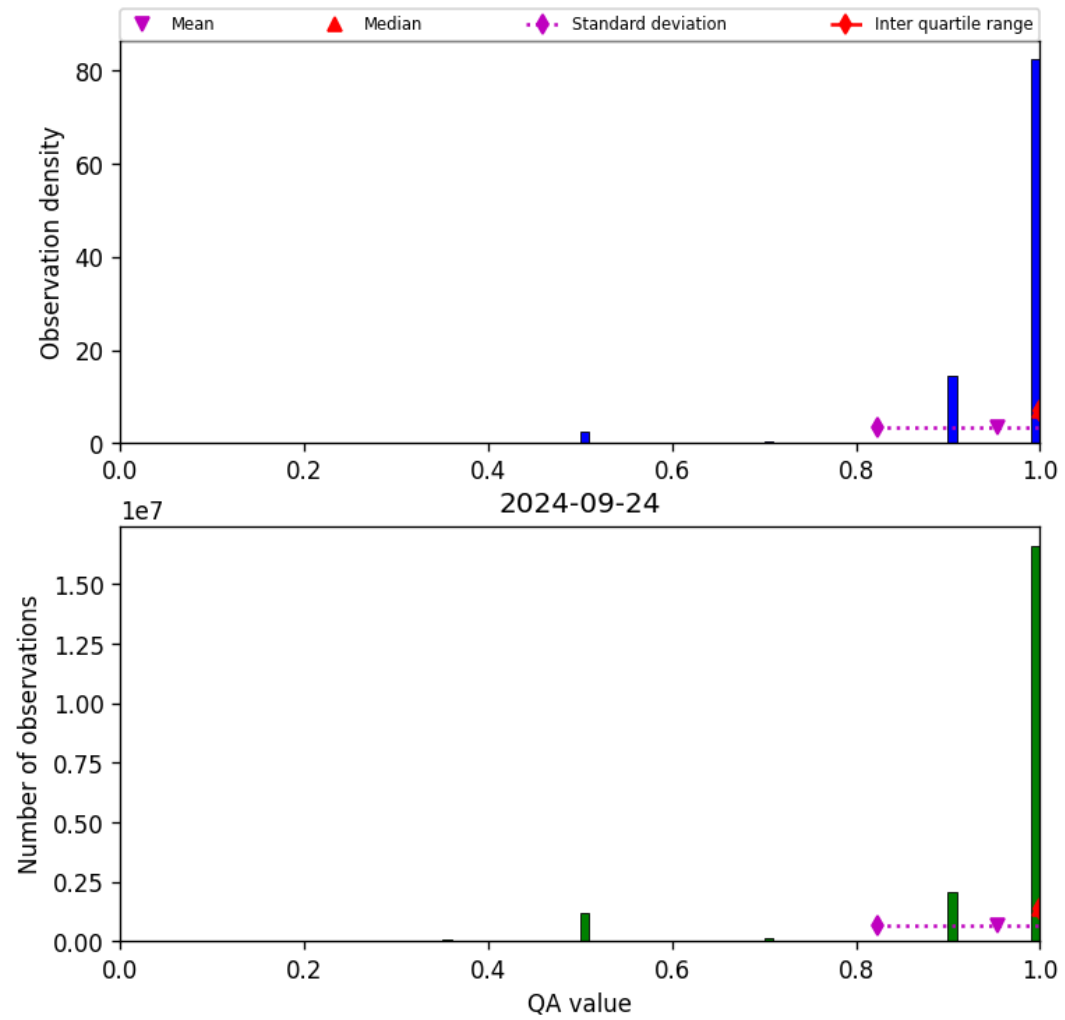
Figure 29: Histogram of “QA value” for 2024-09-23 to 2024-09-25
