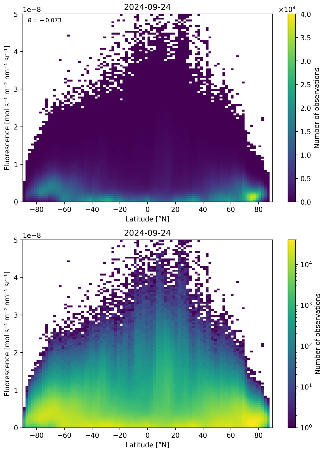
Figure 101: Scatter density plot of “Latitude” against “Fluorescence” for 2024-09-23 to 2024-09-25.
