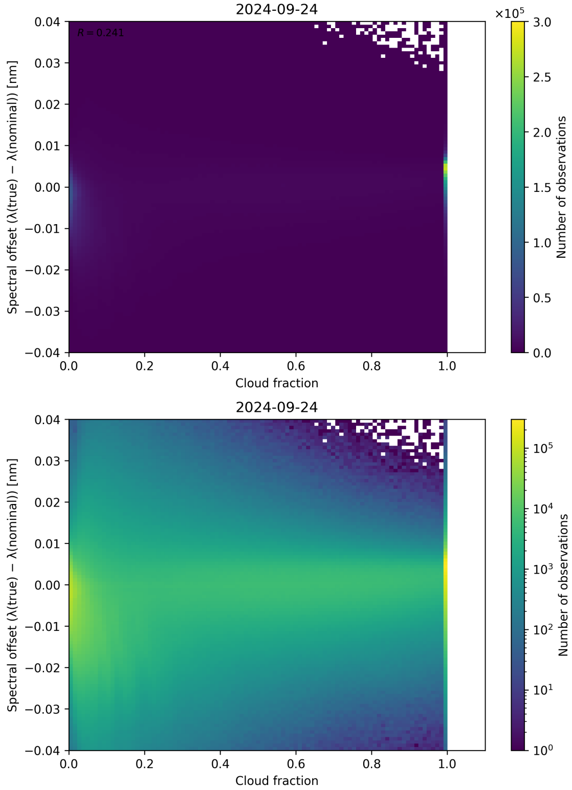
Figure 83: Scatter density plot of “Cloud fraction” against “Spectral offset ( \lambda_{\text{true}} - \lambda_{\text{nominal}} )” for 2024-09-23 to 2024-09-25.
