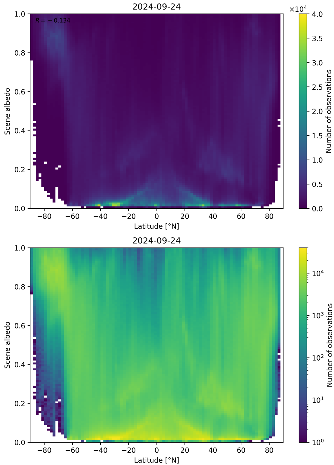
Figure 104: Scatter density plot of “Latitude” against “Scene albedo” for 2024-09-23 to 2024-09-25.
