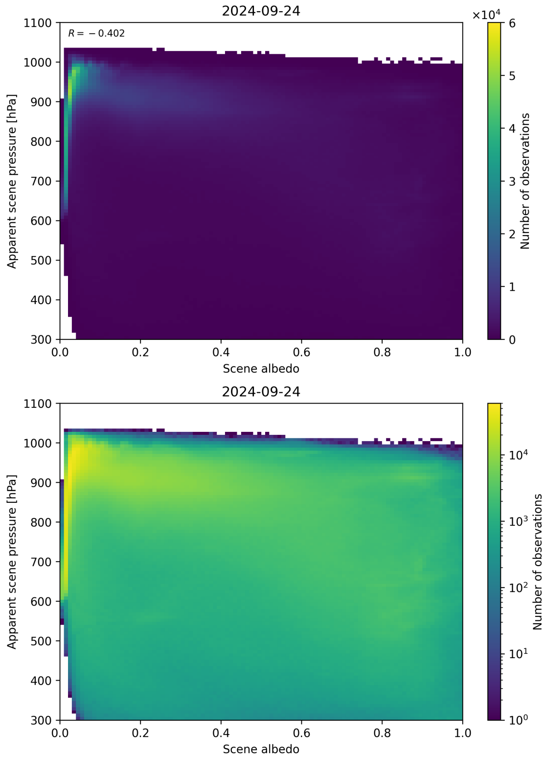
Figure 111: Scatter density plot of “Scene albedo” against “Apparent scene pressure” for 2024-09-23 to 2024-09-25.
