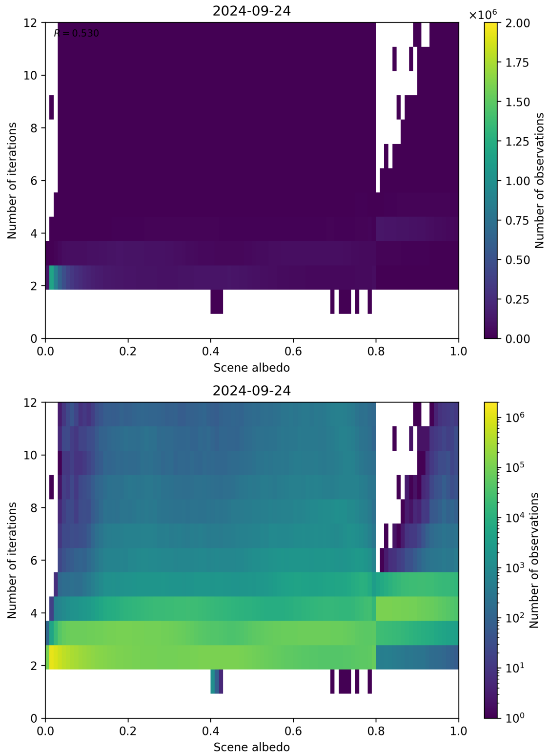
Figure 115: Scatter density plot of “Scene albedo” against “Number of iterations” for 2024-09-23 to 2024-09-25.
