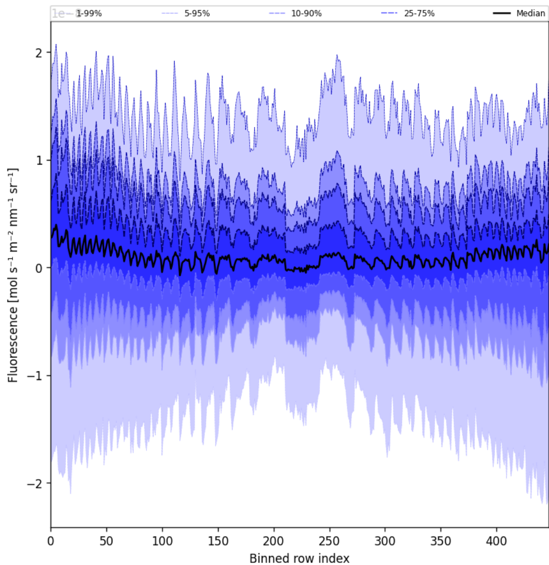
Figure 57: Along track statistics of “Fluorescence” for 2024-09-23 to 2024-09-25
