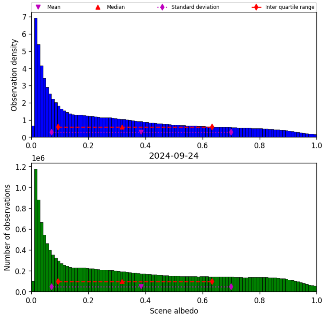
Figure 34: Histogram of “Scene albedo” for 2024-09-23 to 2024-09-25
