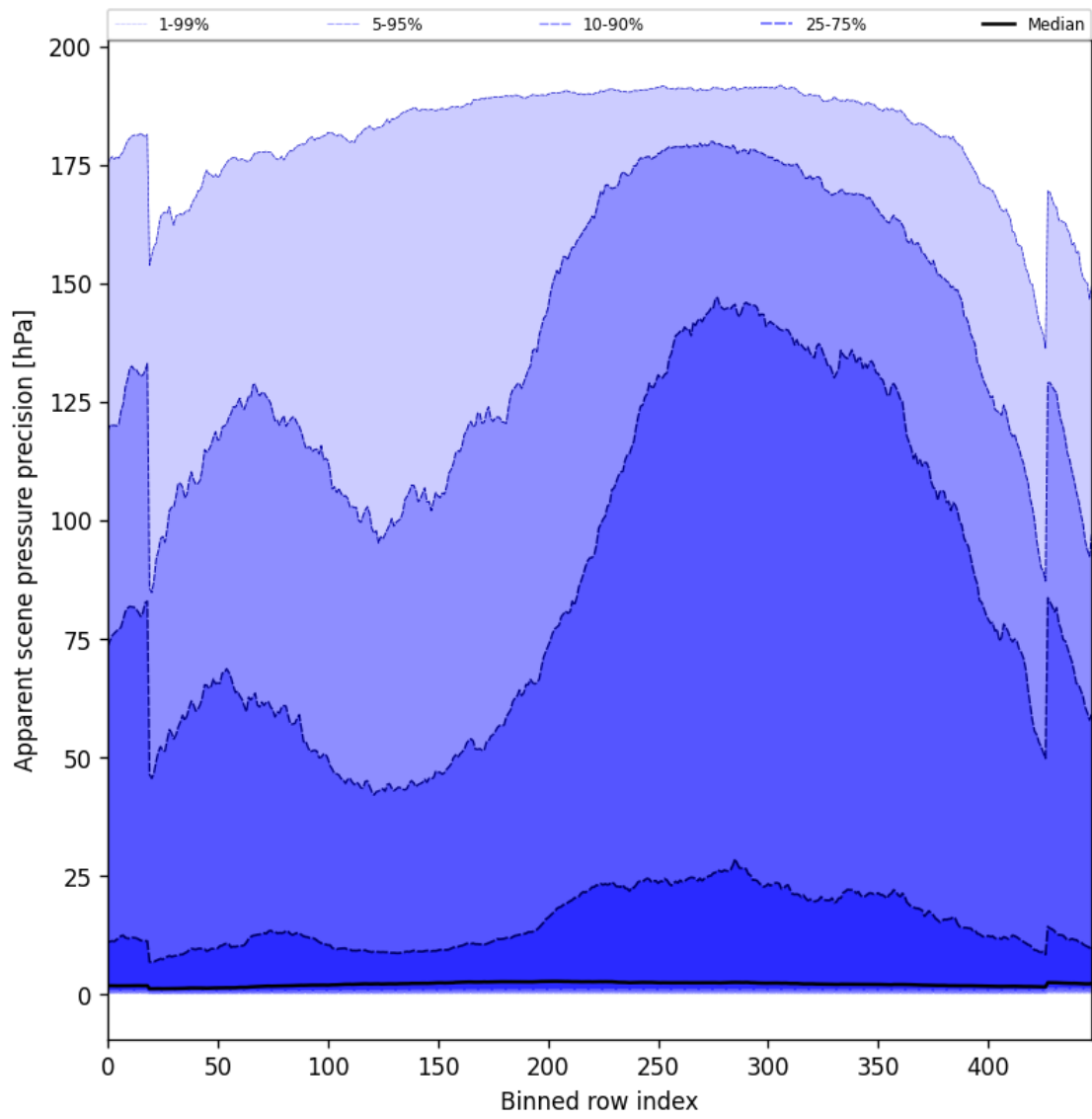
Figure 54: Along track statistics of “Apparent scene pressure precision” for 2024-09-23 to 2024-09-25
