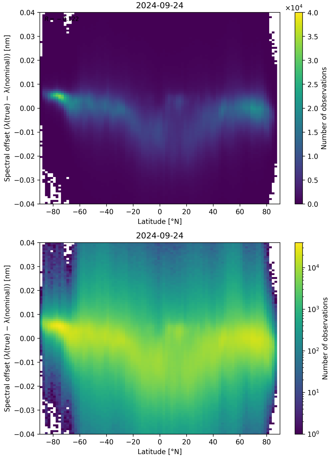
Figure 105: Scatter density plot of “Latitude” against “Spectral offset ( \lambda_{\text{true}} - \lambda_{\text{nominal}} )” for 2024-09-23 to 2024-09-25.
