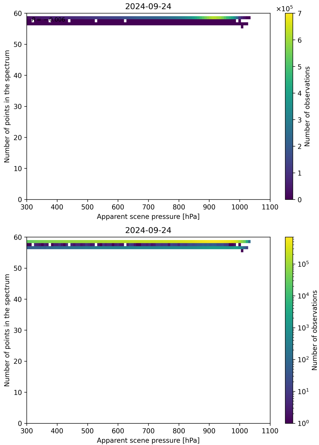
Figure 67: Scatter density plot of “Apparent scene pressure” against “Number of points in the spectrum” for 2024-09-23 to 2024-09-25.
