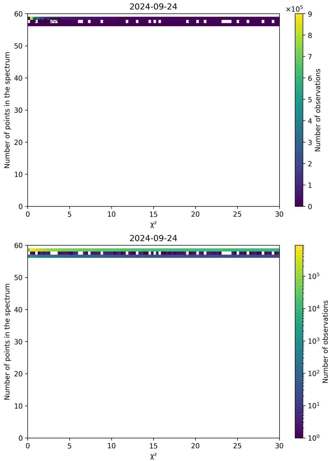
Figure 74: Scatter density plot of “ \chi^2 ” against “Number of points in the spectrum” for 2024-09-23 to 2024-09-25.
