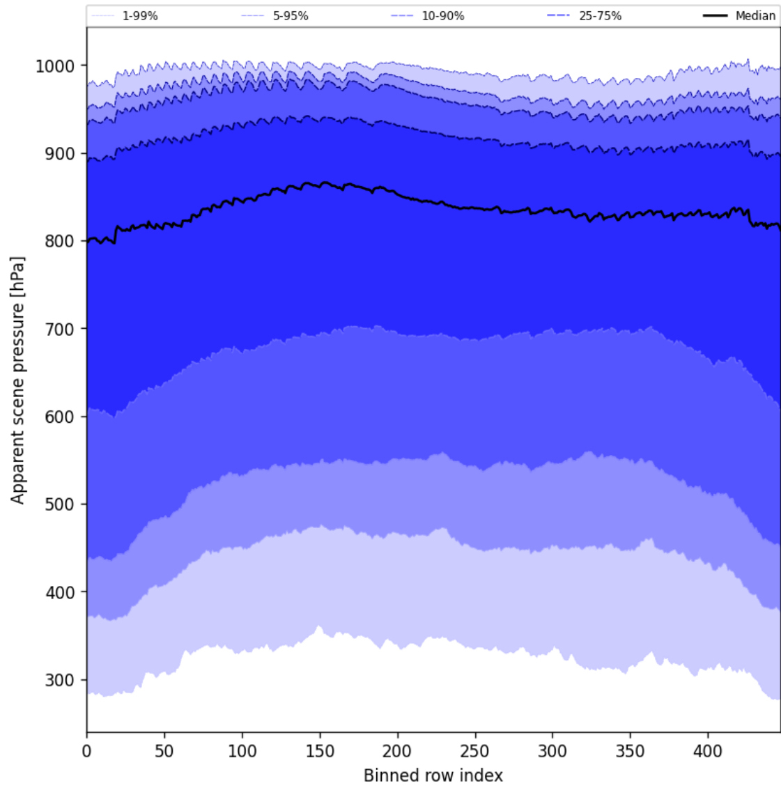
Figure 53: Along track statistics of “Apparent scene pressure” for 2024-09-23 to 2024-09-25
