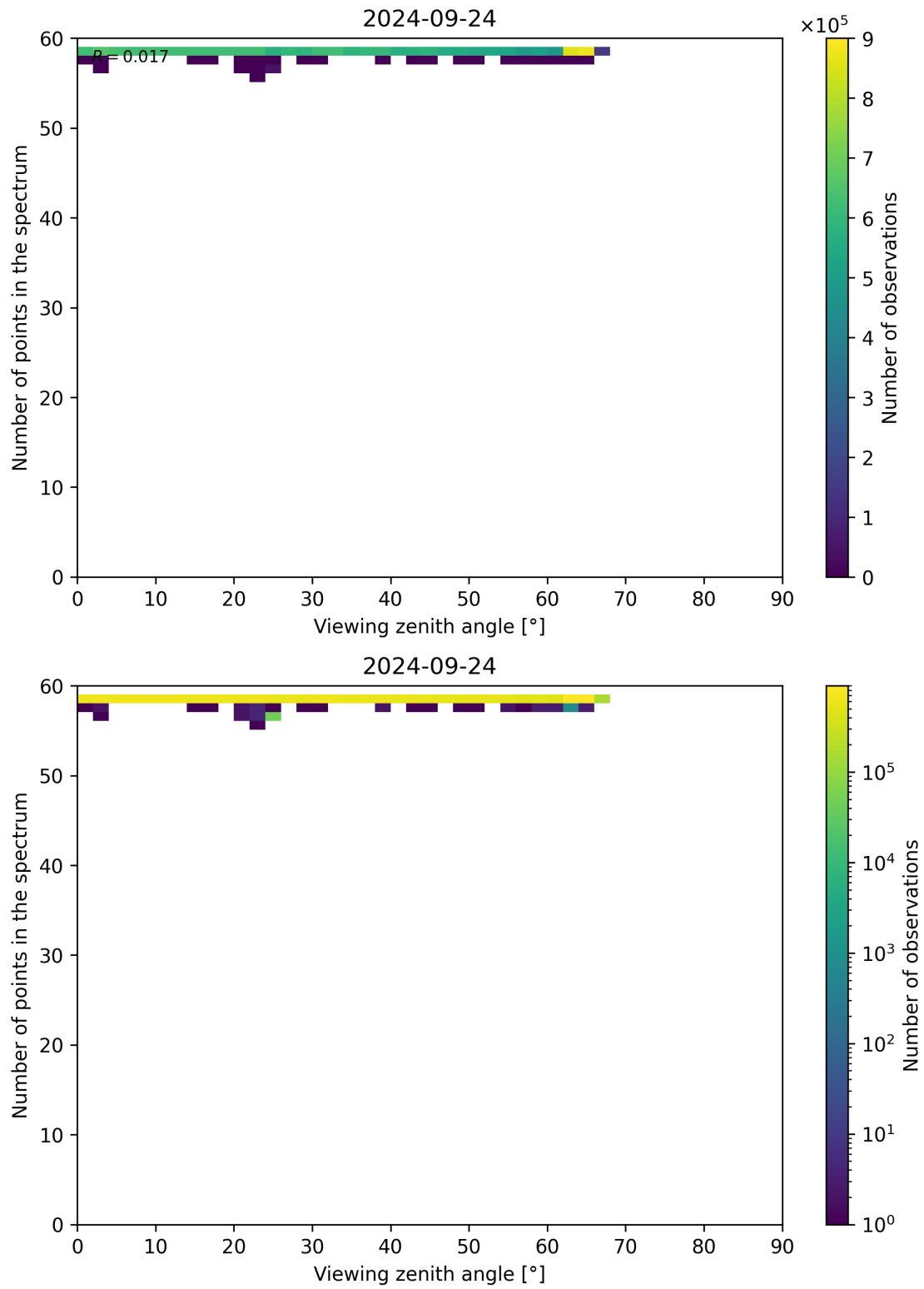
Figure 137: Scatter density plot of “Viewing zenith angle” against “Number of points in the spectrum” for 2024-09-23 to 2024-09-25.
