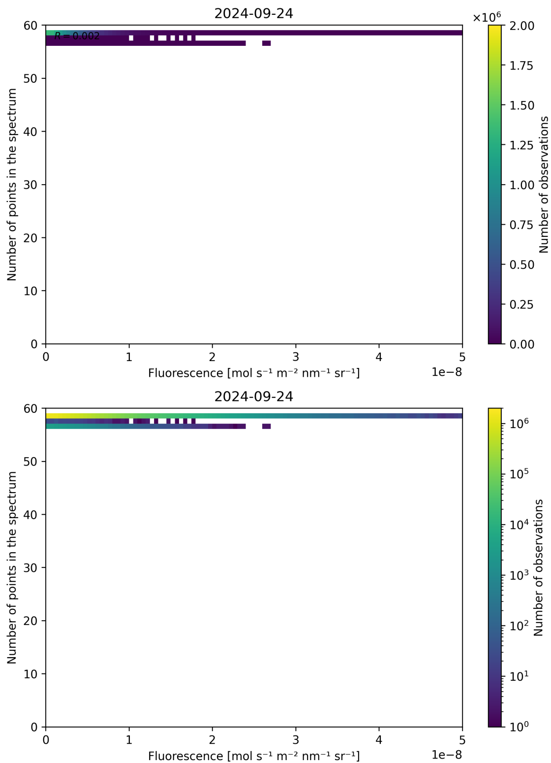
Figure 94: Scatter density plot of “Fluorescence” against “Number of points in the spectrum” for 2024-09-23 to 2024-09-25.
