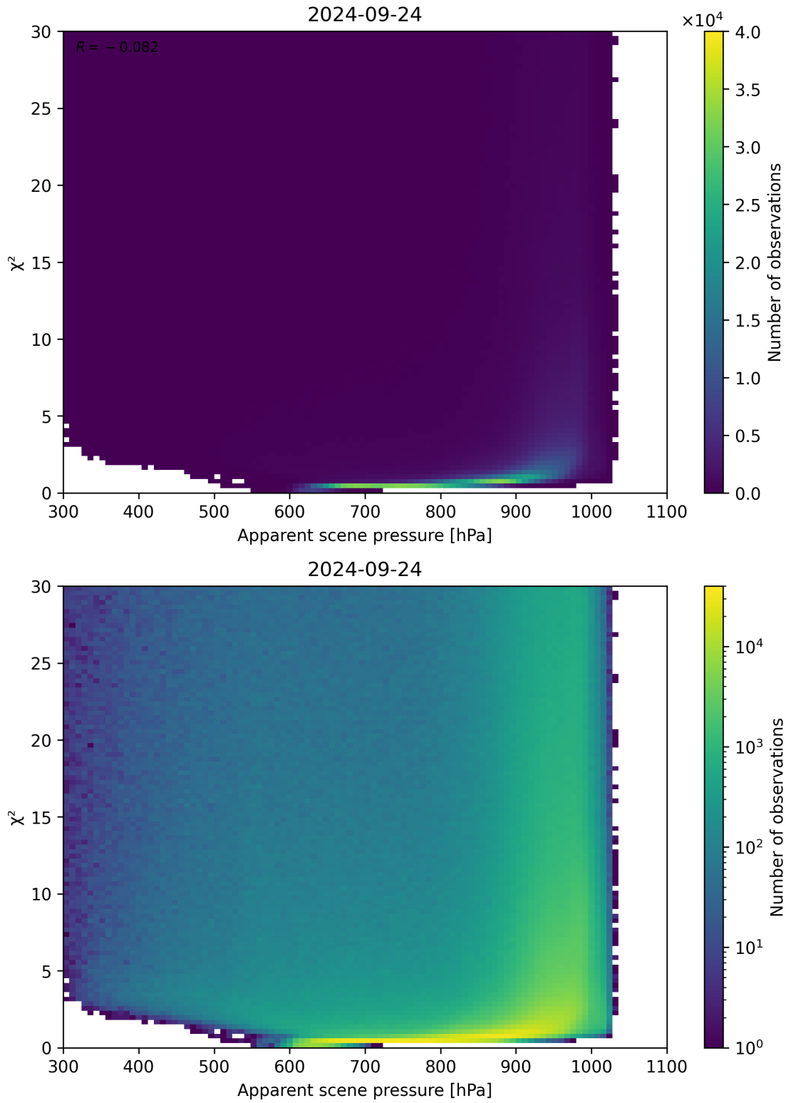
Figure 63: Scatter density plot of “Apparent scene pressure” against “ \chi^2 ” for 2024-09-23 to 2024-09-25.
