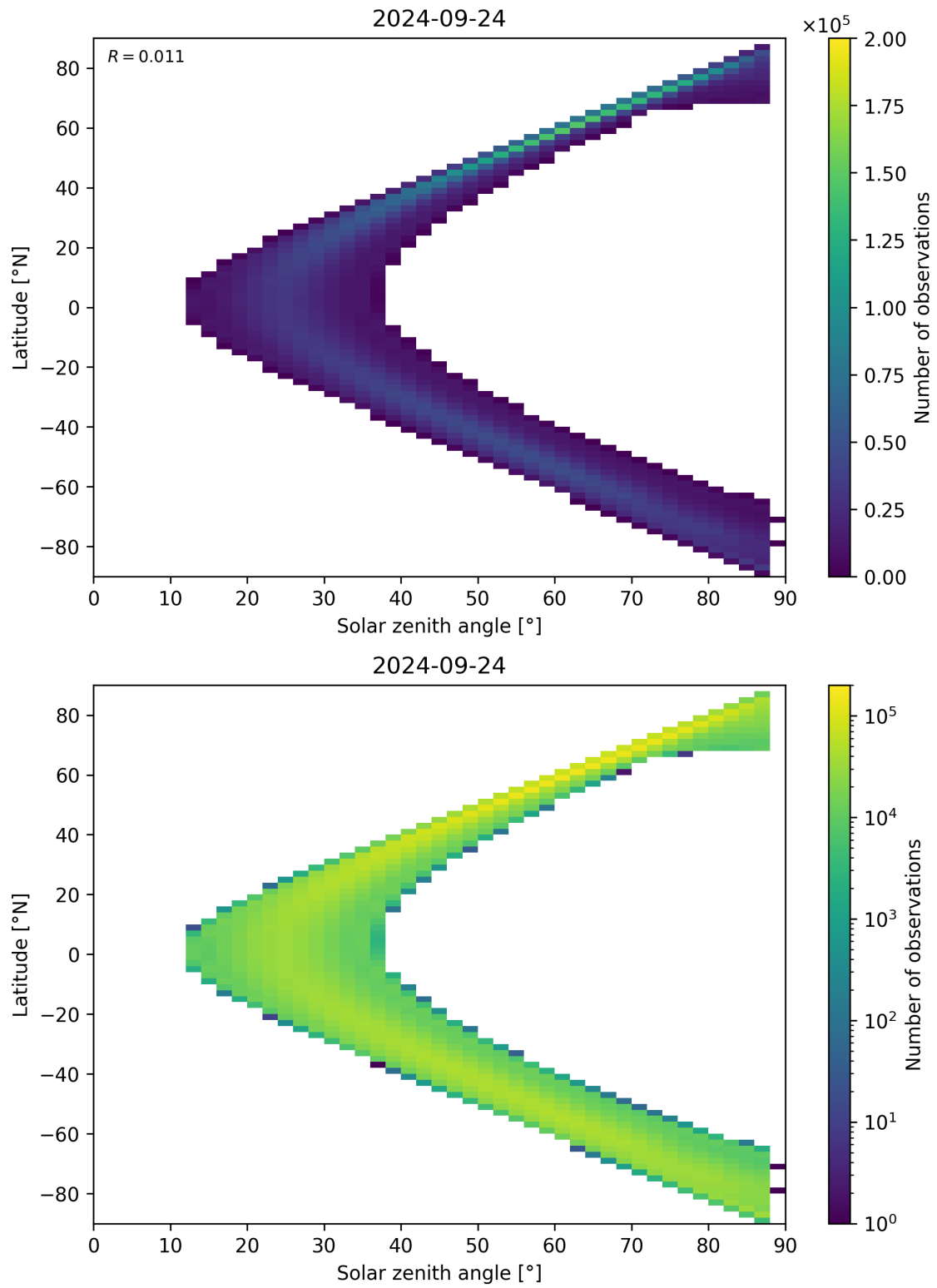
Figure 124: Scatter density plot of “Solar zenith angle” against “Latitude” for 2024-09-23 to 2024-09-25.
