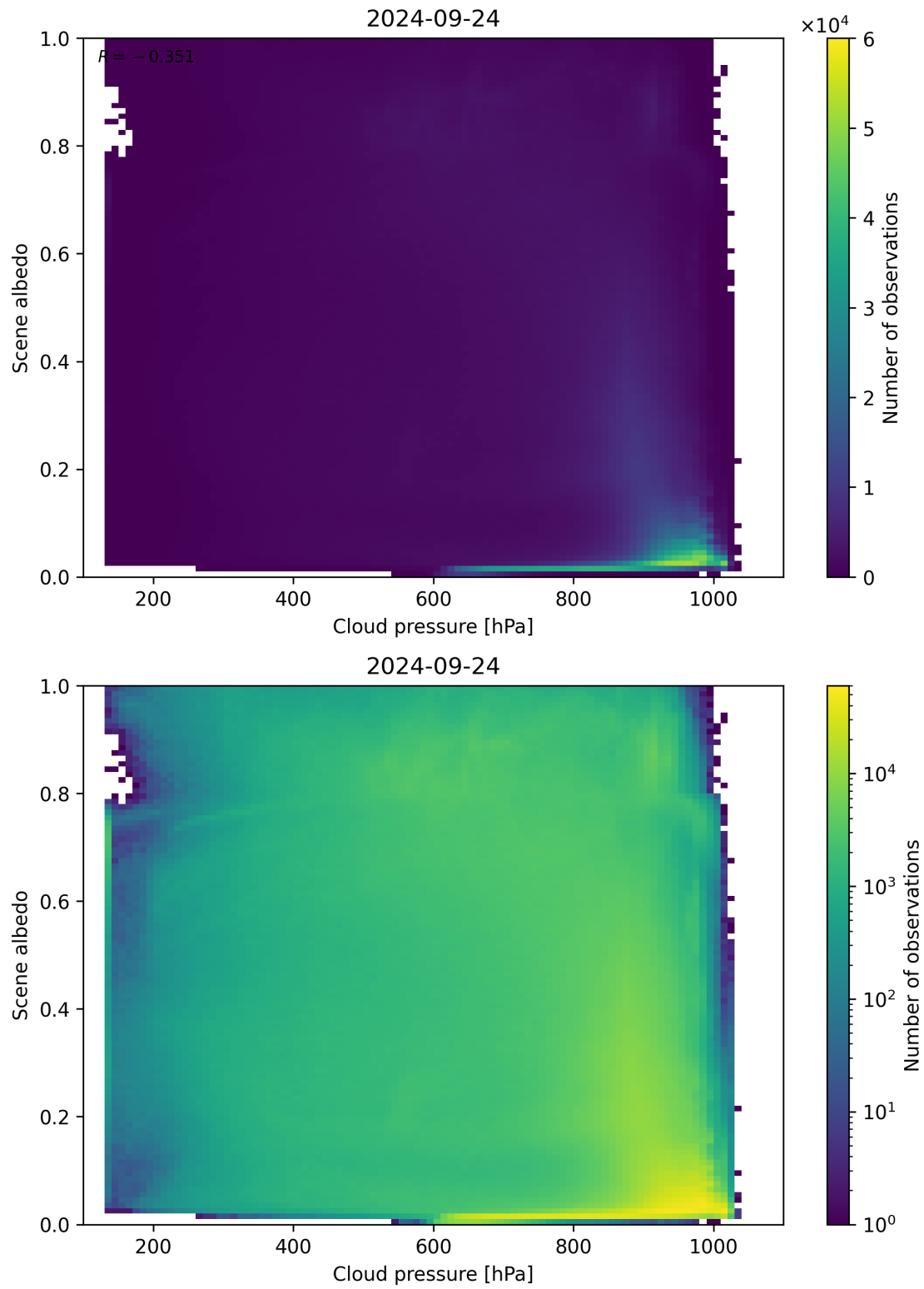
Figure 91: Scatter density plot of “Cloud pressure” against “Scene albedo” for 2024-09-23 to 2024-09-25.
