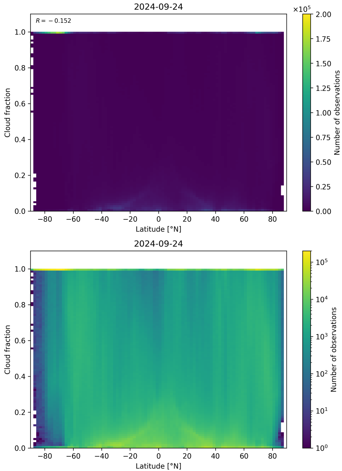
Figure 99: Scatter density plot of “Latitude” against “Cloud fraction” for 2024-09-23 to 2024-09-25.
