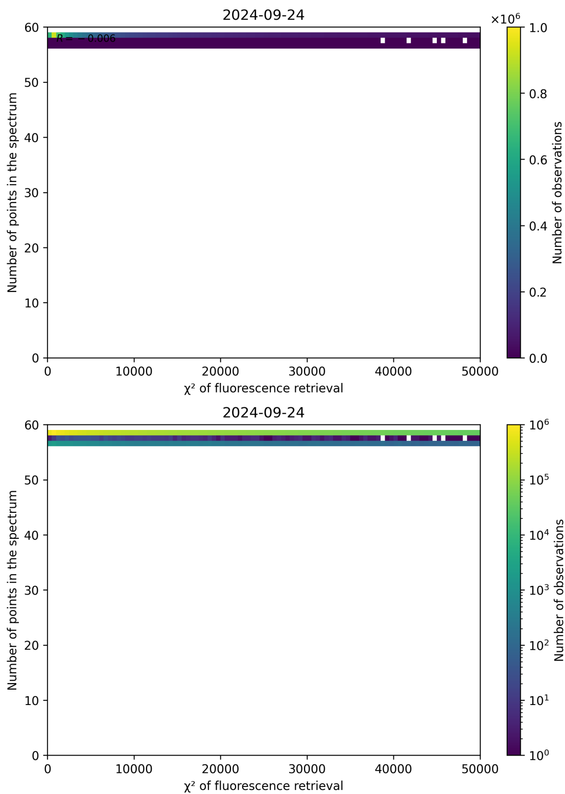
Figure 71: Scatter density plot of “ \chi^2 of fluorescence retrieval” against “Number of points in the spectrum” for 2024-09-23 to 2024-09-25.
