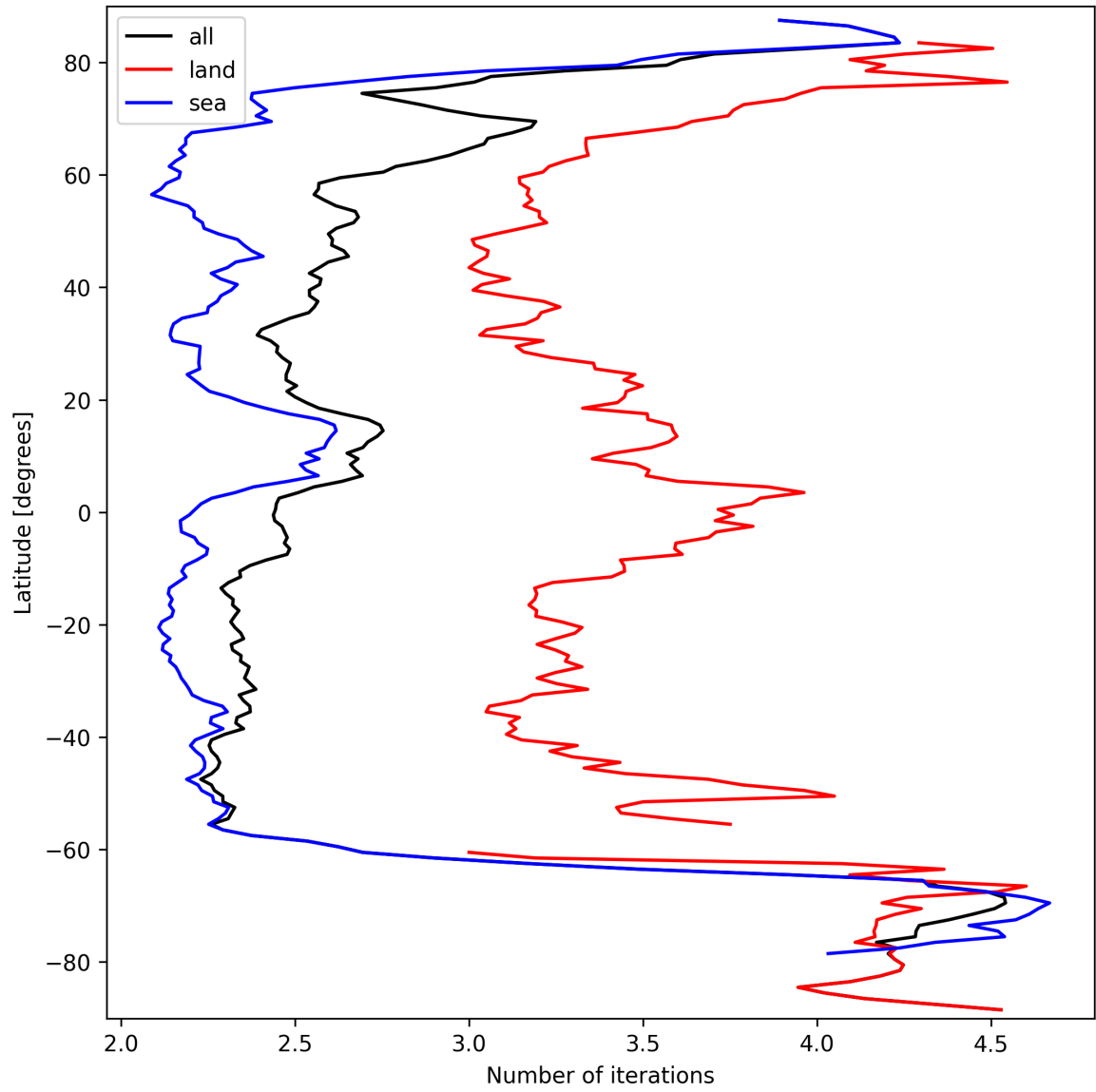
Figure 22: Zonal average of “Number of iterations” for 2024-09-23 to 2024-09-25.
