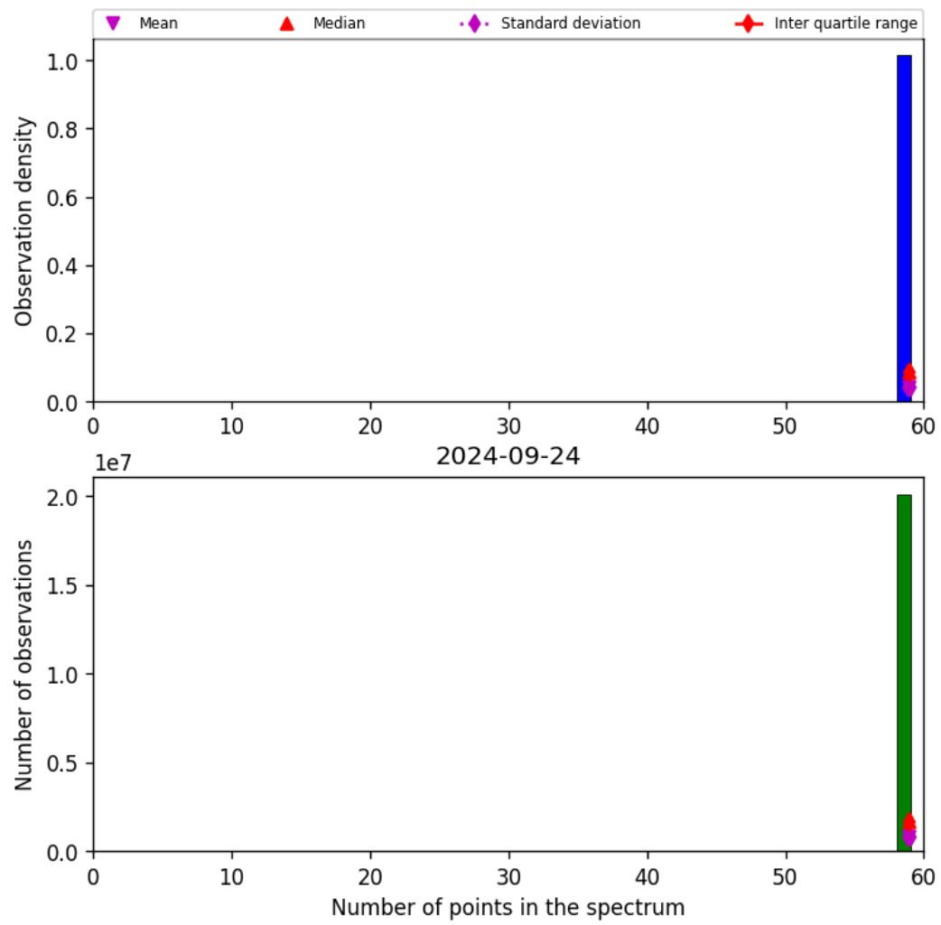
Figure 44: Histogram of “Number of points in the spectrum” for 2024-09-23 to 2024-09-25
