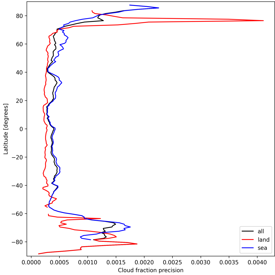
Figure 16: Zonal average of “Cloud fraction precision” for 2024-09-23 to 2024-09-25.
