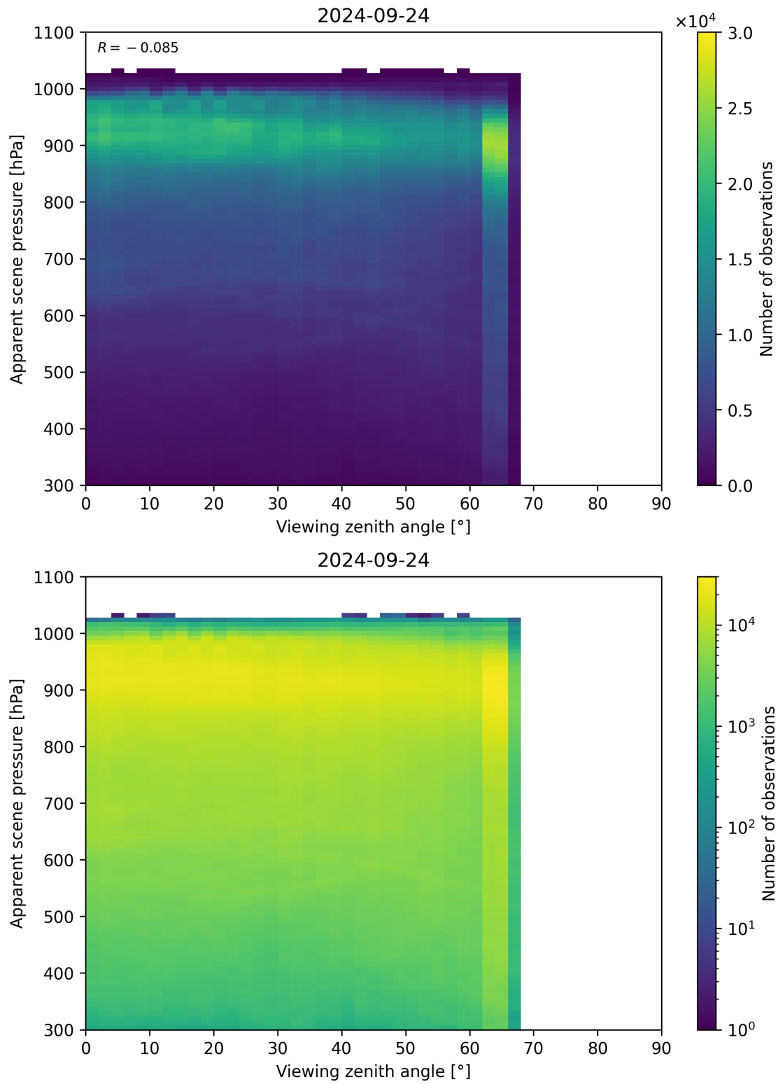
Figure 129: Scatter density plot of “Viewing zenith angle” against “Apparent scene pressure” for 2024-09-23 to 2024-09-25.
