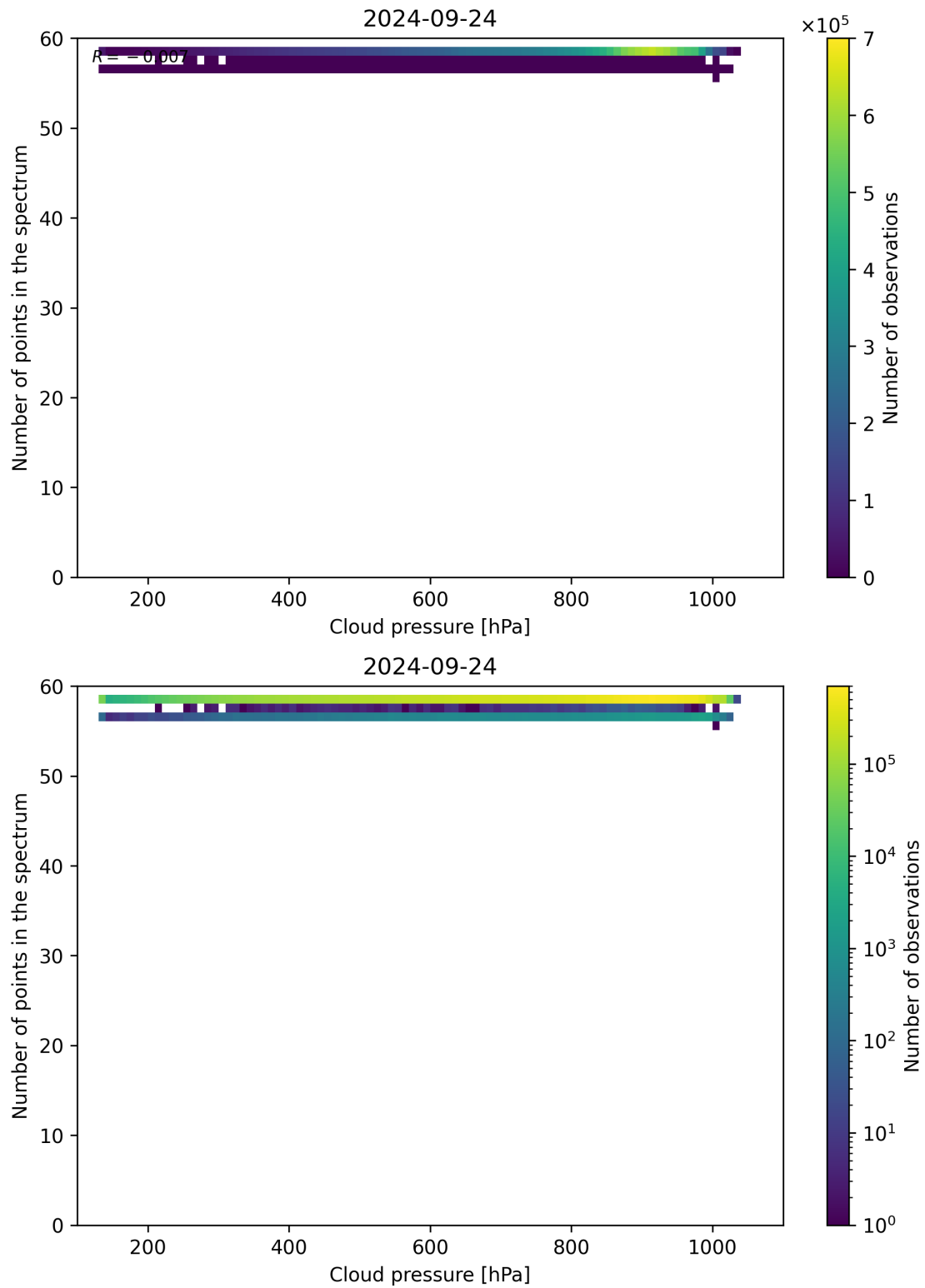
Figure 90: Scatter density plot of “Cloud pressure” against “Number of points in the spectrum” for 2024-09-23 to 2024-09-25.
