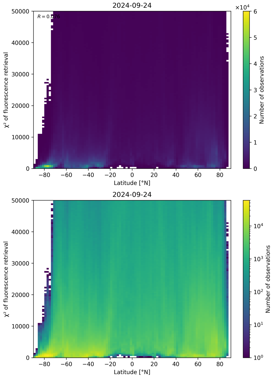
Figure 98: Scatter density plot of “Latitude” against “ \chi^2 of fluorescence retrieval” for 2024-09-23 to 2024-09-25.
