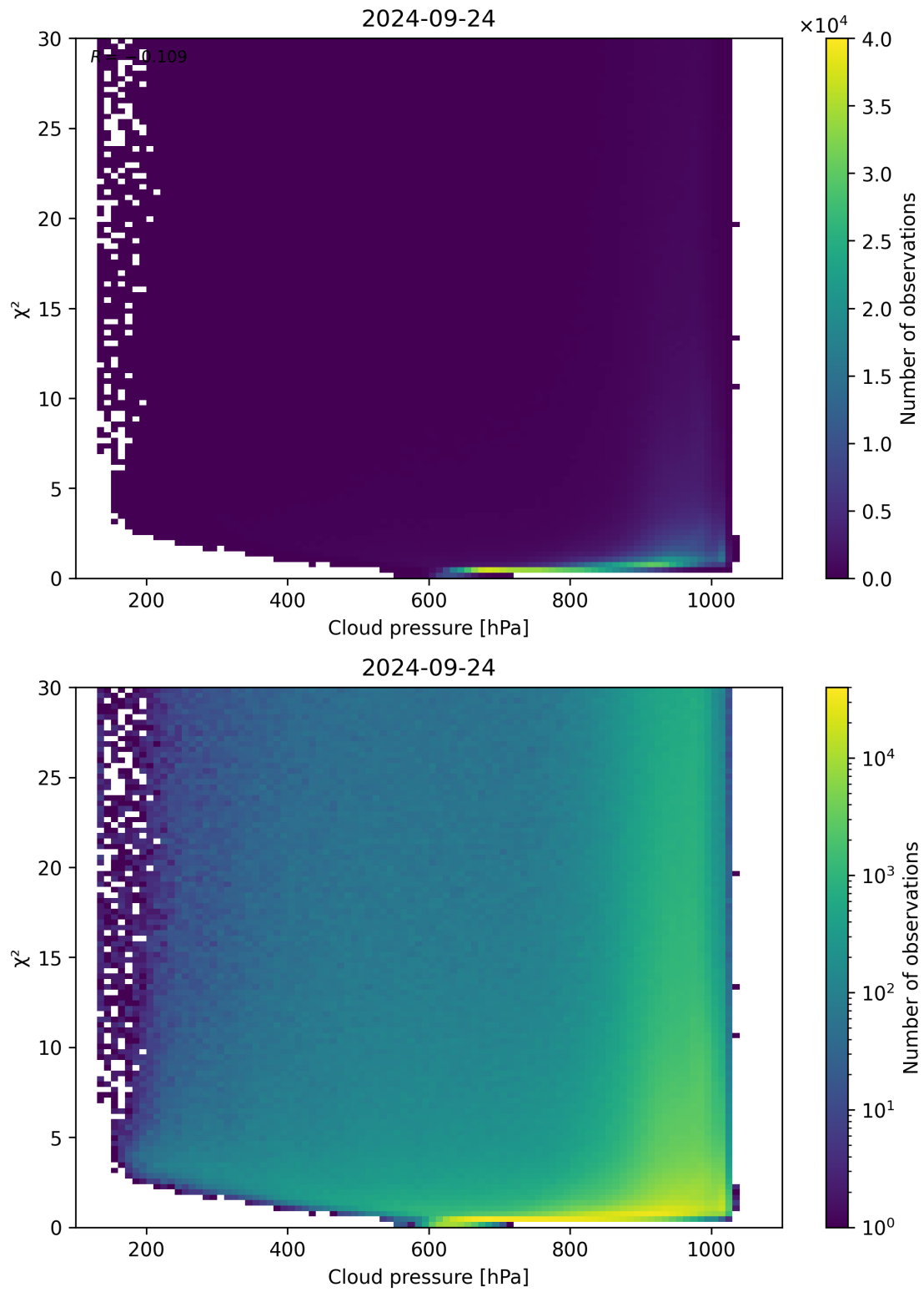
Figure 85: Scatter density plot of “Cloud pressure” against “ \chi^2 ” for 2024-09-23 to 2024-09-25.
