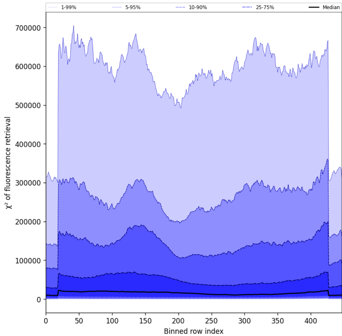
Figure 59: Along track statistics of “ \chi^2 of fluorescence retrieval” for 2024-09-23 to 2024-09-25
