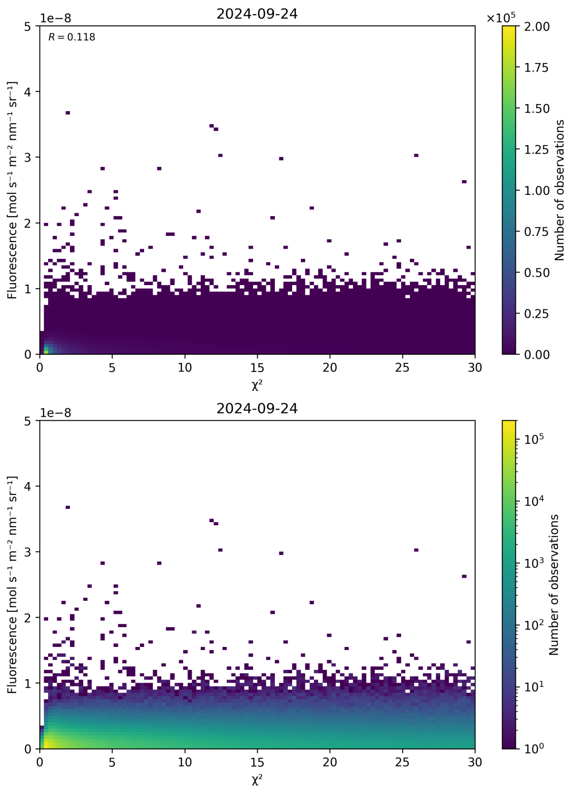
Figure 70: Scatter density plot of “ \chi^2 ” against “Fluorescence” for 2024-09-23 to 2024-09-25.
