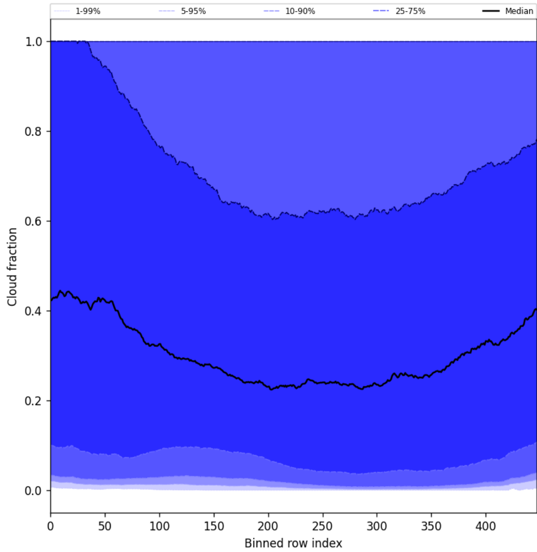
Figure 49: Along track statistics of “Cloud fraction” for 2024-09-23 to 2024-09-25
