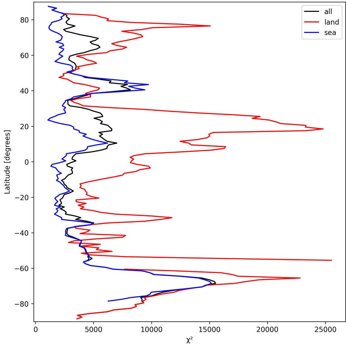
Figure 21: Zonal average of “ \chi^2 ” for 2024-09-23 to 2024-09-25.
