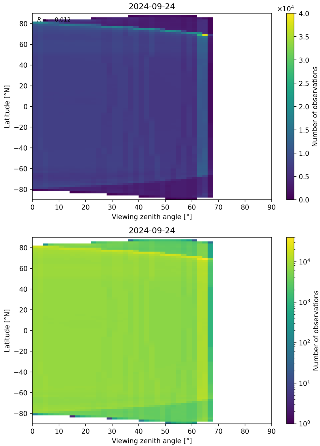
Figure 135: Scatter density plot of “Viewing zenith angle” against “Latitude” for 2024-09-23 to 2024-09-25.
