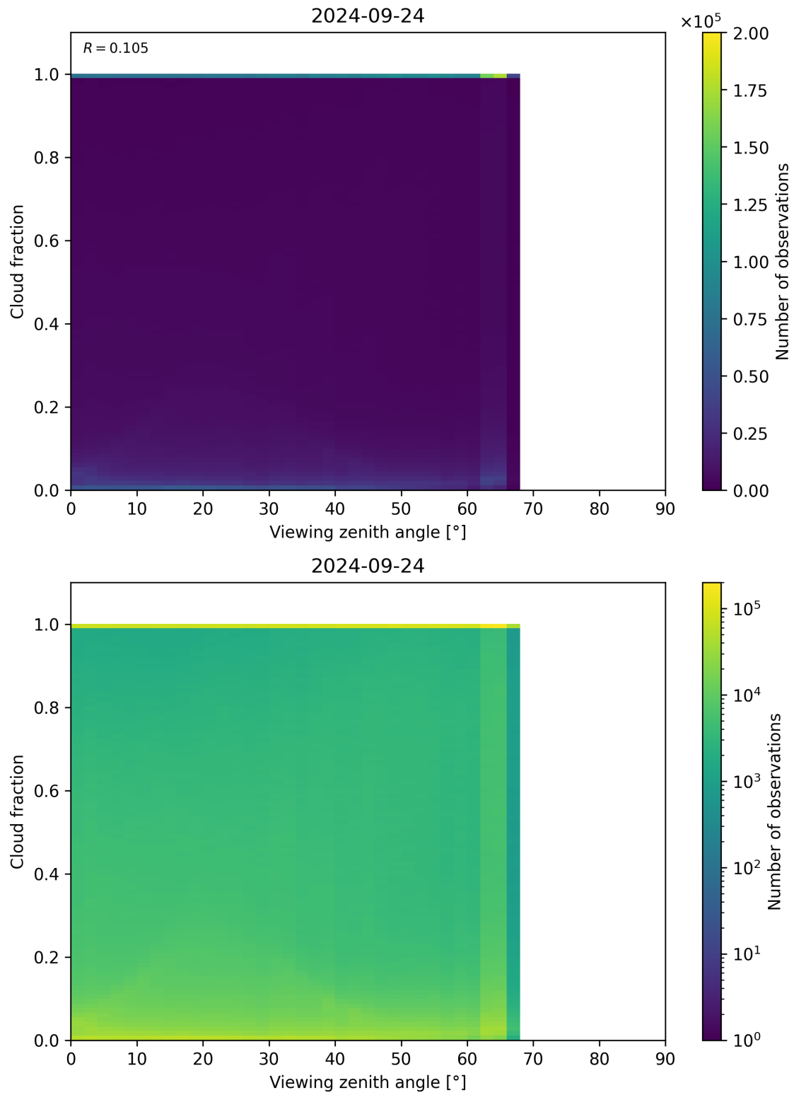
Figure 132: Scatter density plot of “Viewing zenith angle” against “Cloud fraction” for 2024-09-23 to 2024-09-25.
