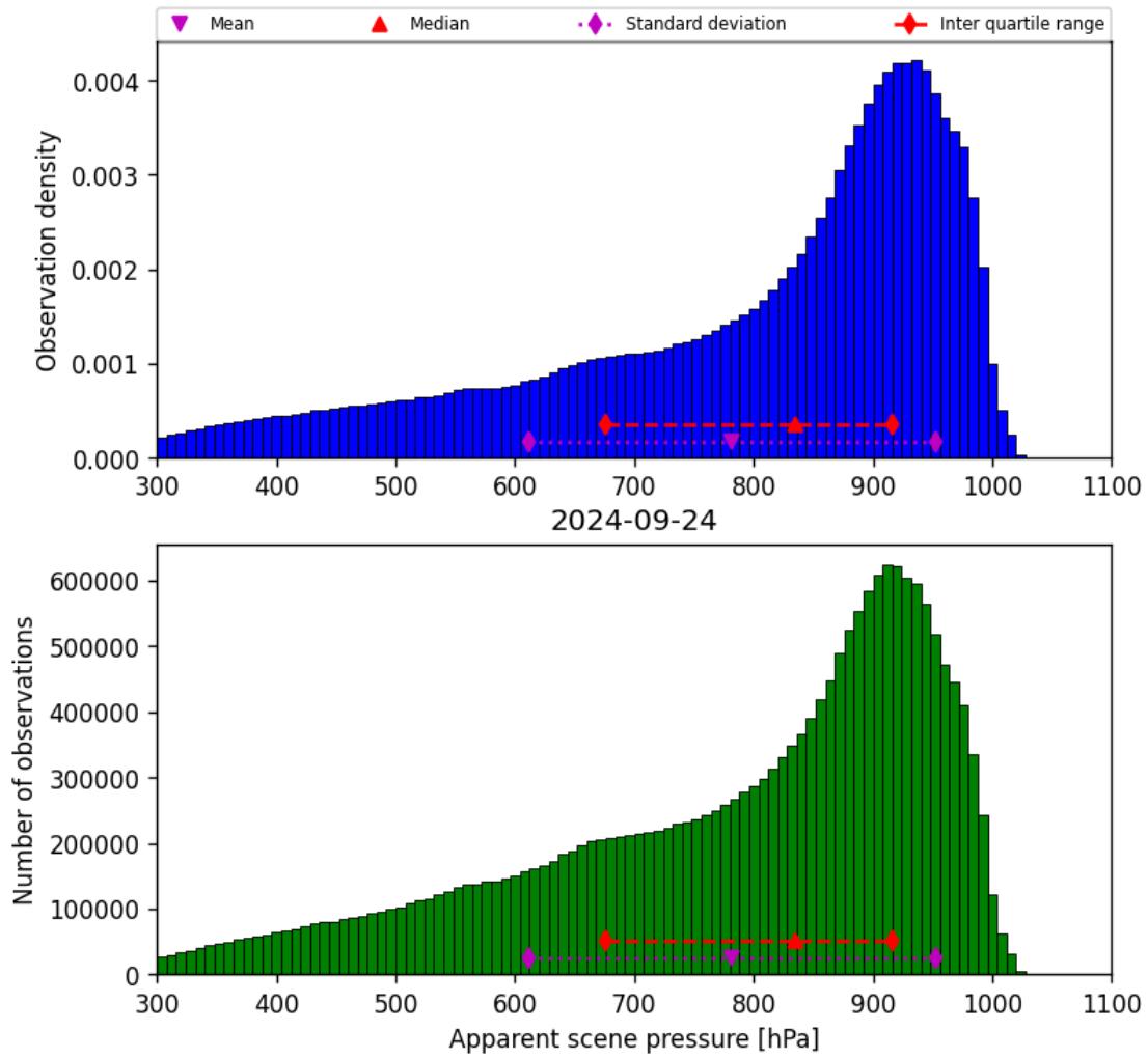
Figure 36: Histogram of “Apparent scene pressure” for 2024-09-23 to 2024-09-25
