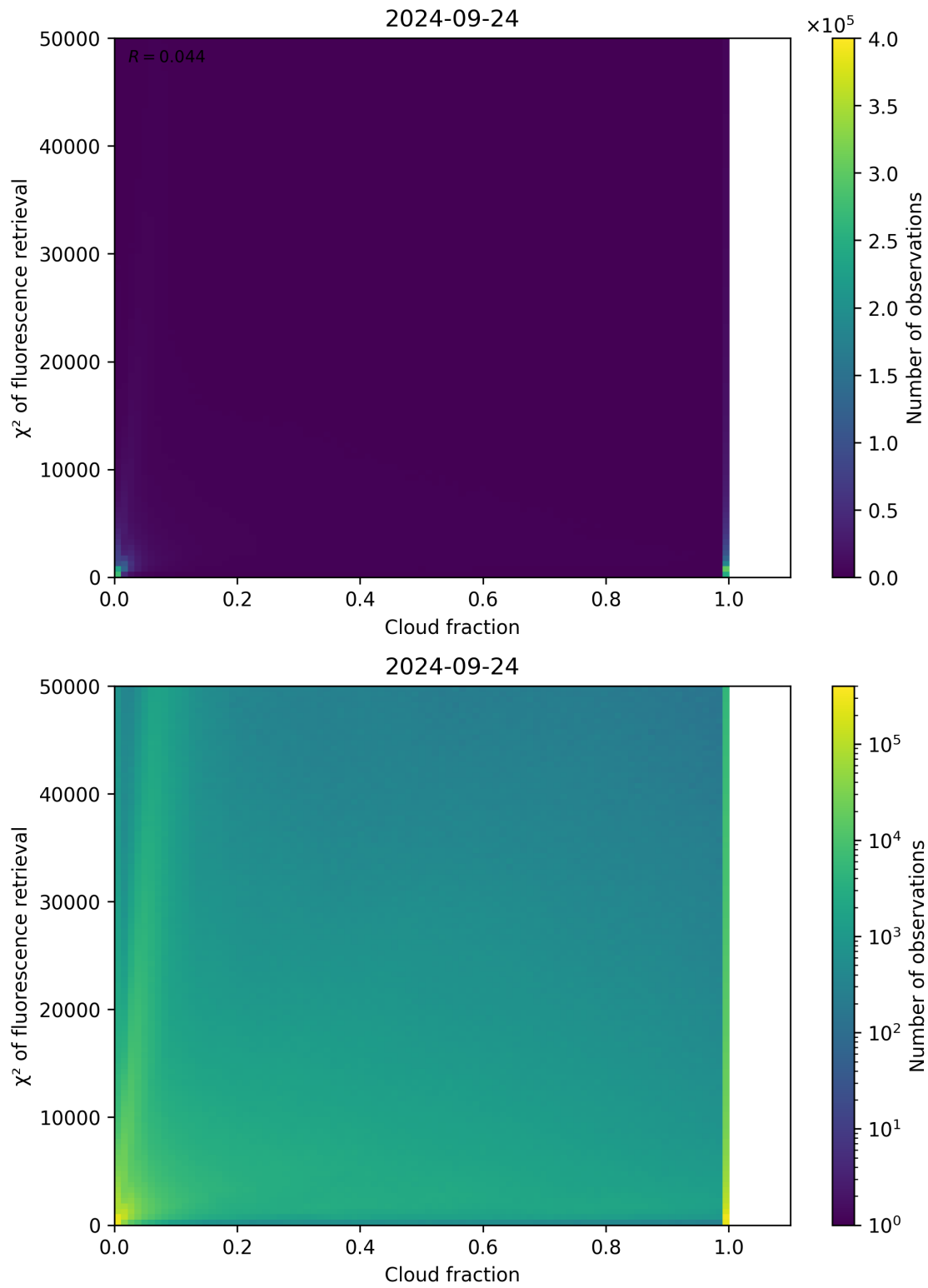
Figure 78: Scatter density plot of “Cloud fraction” against “ \chi^2 of fluorescence retrieval” for 2024-09-23 to 2024-09-25.
