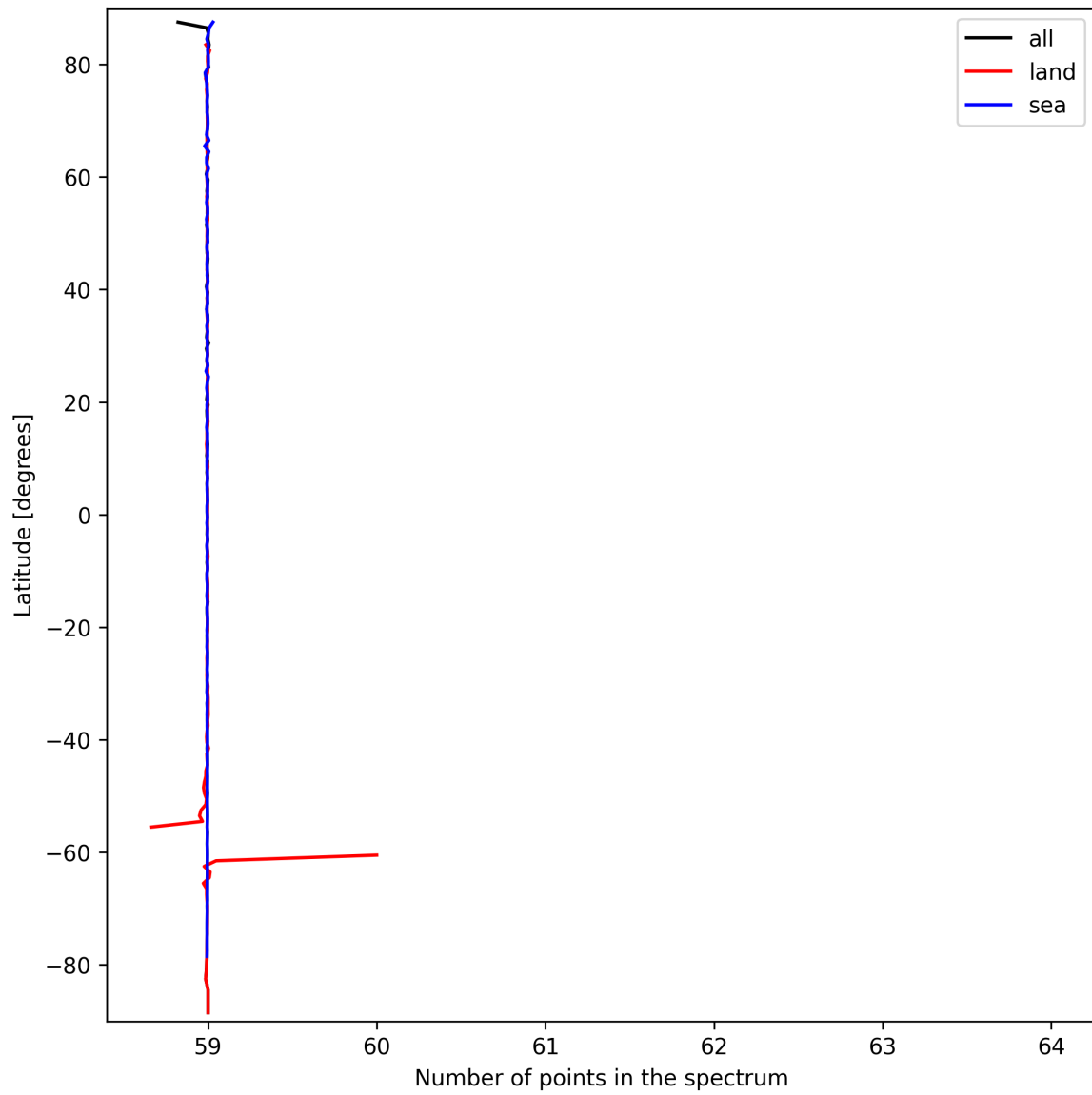
Figure 27: Zonal average of “Number of points in the spectrum” for 2024-09-23 to 2024-09-25.
