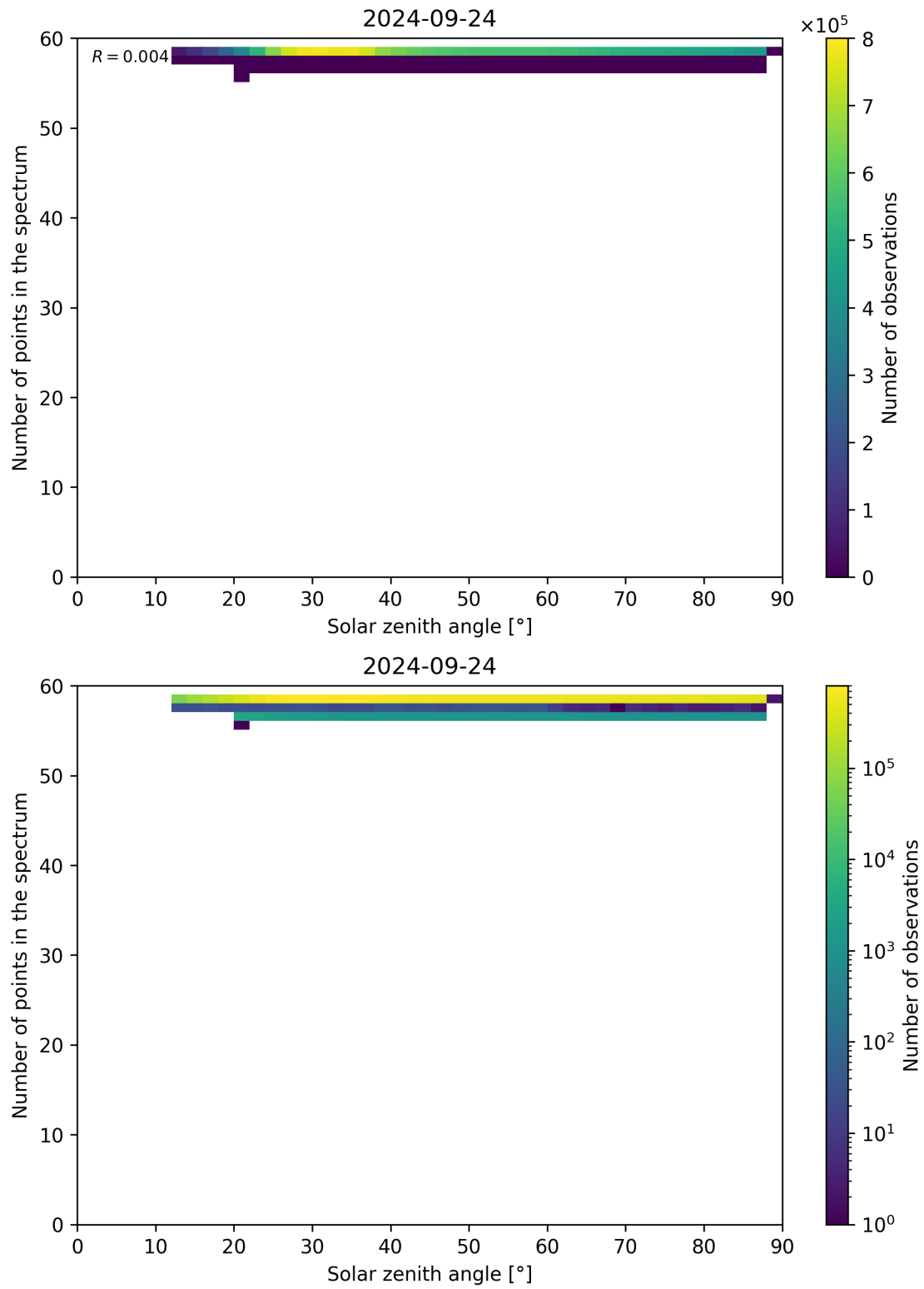
Figure 126: Scatter density plot of “Solar zenith angle” against “Number of points in the spectrum” for 2024-09-23 to 2024-09-25.
