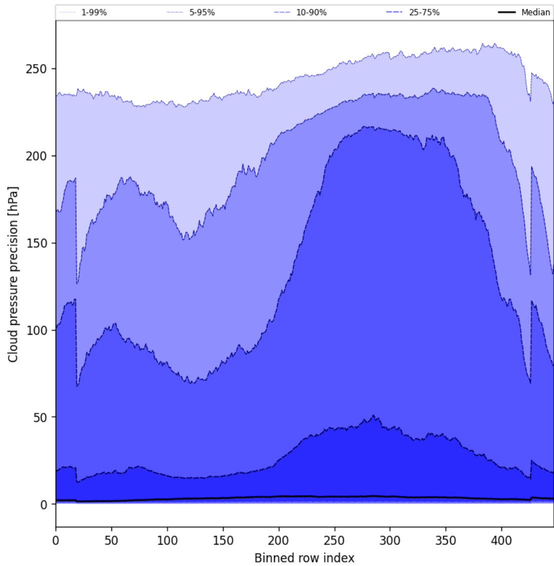
Figure 48: Along track statistics of “Cloud pressure precision” for 2024-09-23 to 2024-09-25
