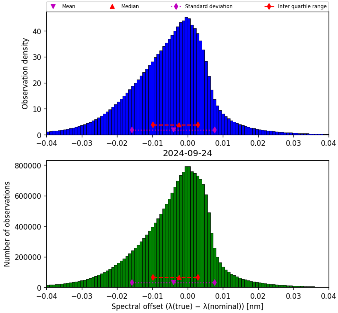
Figure 45: Histogram of “Spectral offset ( \lambda_{\text{true}} - \lambda_{\text{nominal}} )” for 2024-09-23 to 2024-09-25
