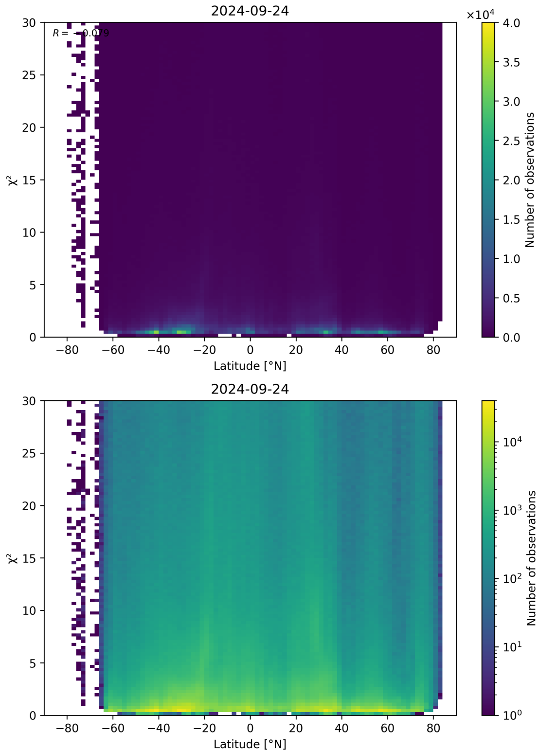
Figure 97: Scatter density plot of “Latitude” against “ \chi^2 ” for 2024-09-23 to 2024-09-25.
