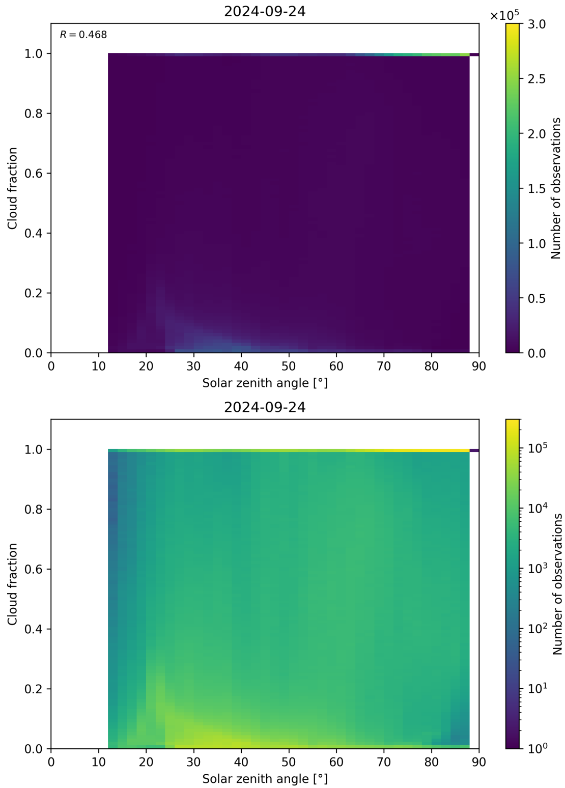
Figure 121: Scatter density plot of “Solar zenith angle” against “Cloud fraction” for 2024-09-23 to 2024-09-25.
