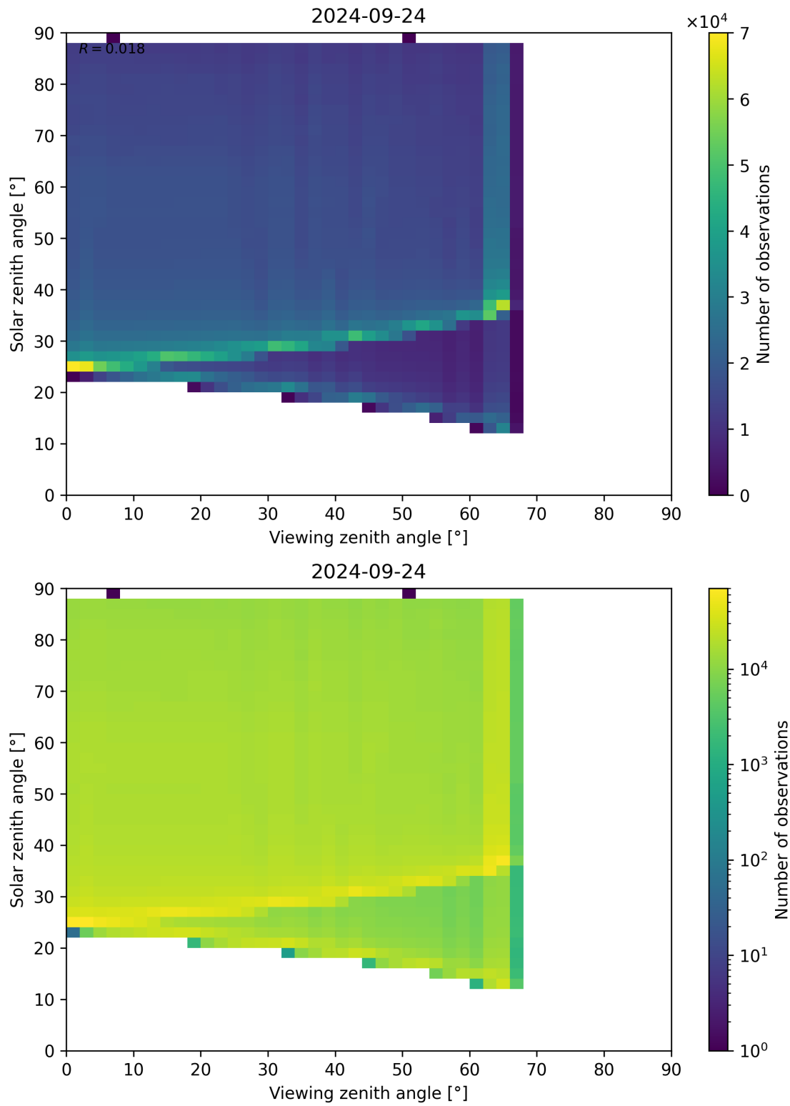
Figure 139: Scatter density plot of “Viewing zenith angle” against “Solar zenith angle” for 2024-09-23 to 2024-09-25.
