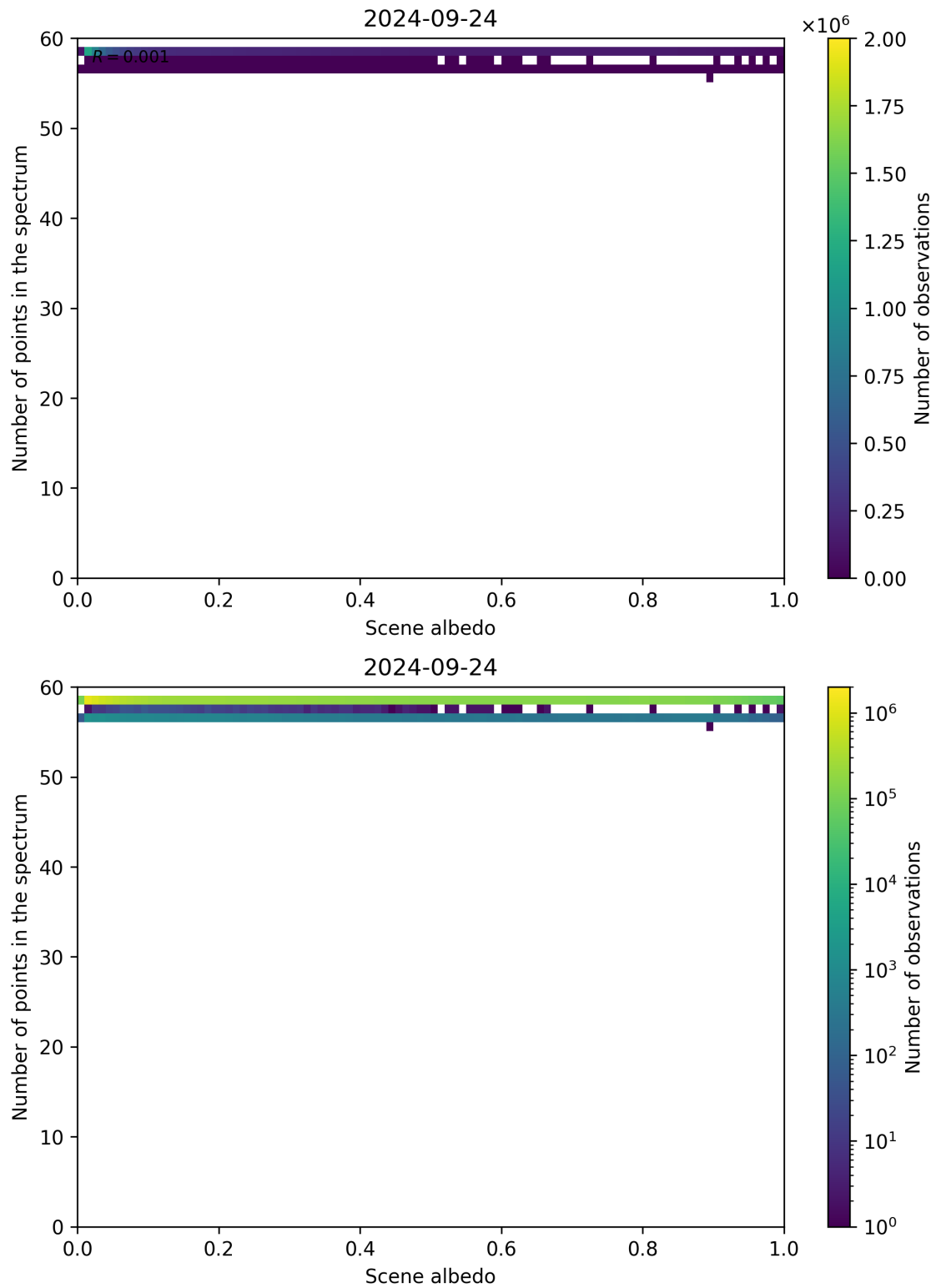
Figure 116: Scatter density plot of “Scene albedo” against “Number of points in the spectrum” for 2024-09-23 to 2024-09-25.
