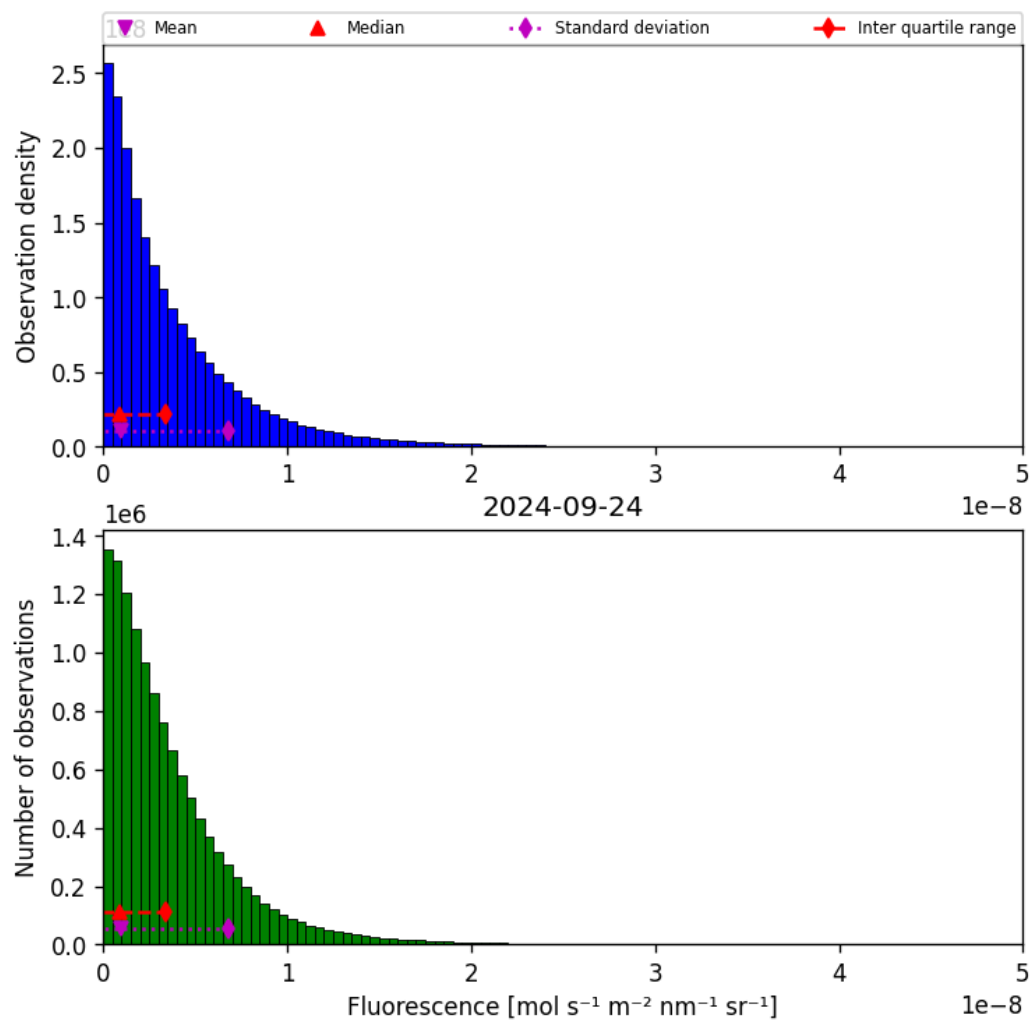
Figure 40: Histogram of “Fluorescence” for 2024-09-23 to 2024-09-25
