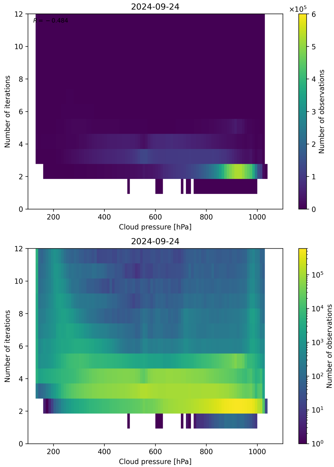
Figure 89: Scatter density plot of “Cloud pressure” against “Number of iterations” for 2024-09-23 to 2024-09-25.
