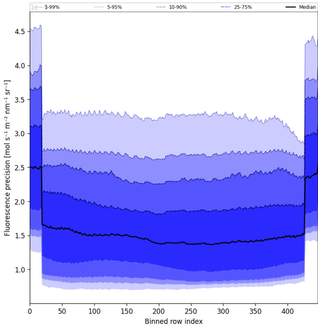
Figure 58: Along track statistics of “Fluorescence precision” for 2024-09-23 to 2024-09-25
