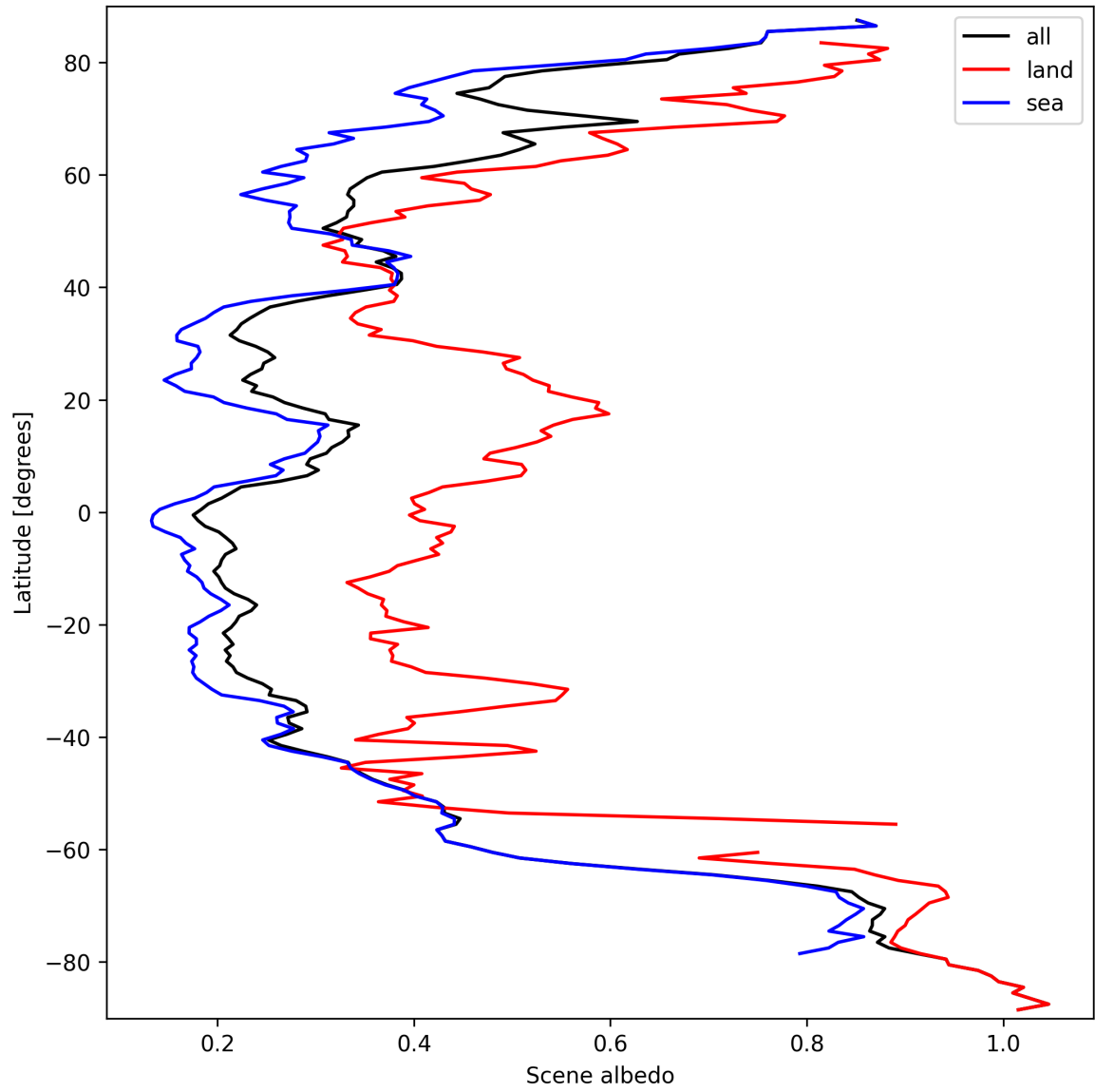
Figure 17: Zonal average of “Scene albedo” for 2024-09-23 to 2024-09-25.
