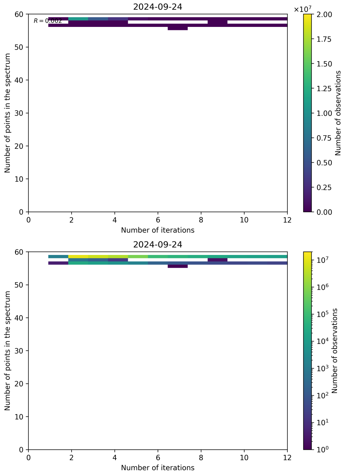
Figure 108: Scatter density plot of “Number of iterations” against “Number of points in the spectrum” for 2024-09-23 to 2024-09-25.
