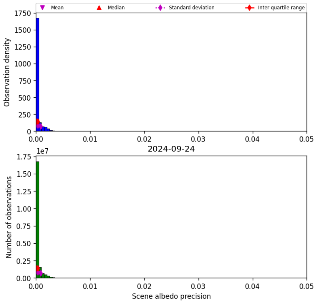
Figure 35: Histogram of “Scene albedo precision” for 2024-09-23 to 2024-09-25
