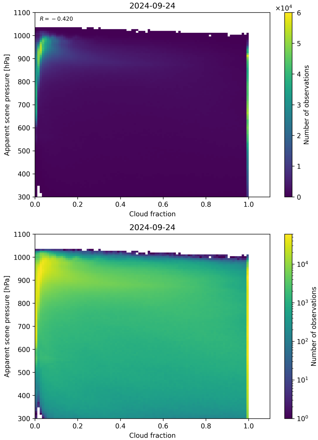
Figure 76: Scatter density plot of “Cloud fraction” against “Apparent scene pressure” for 2024-09-23 to 2024-09-25.
