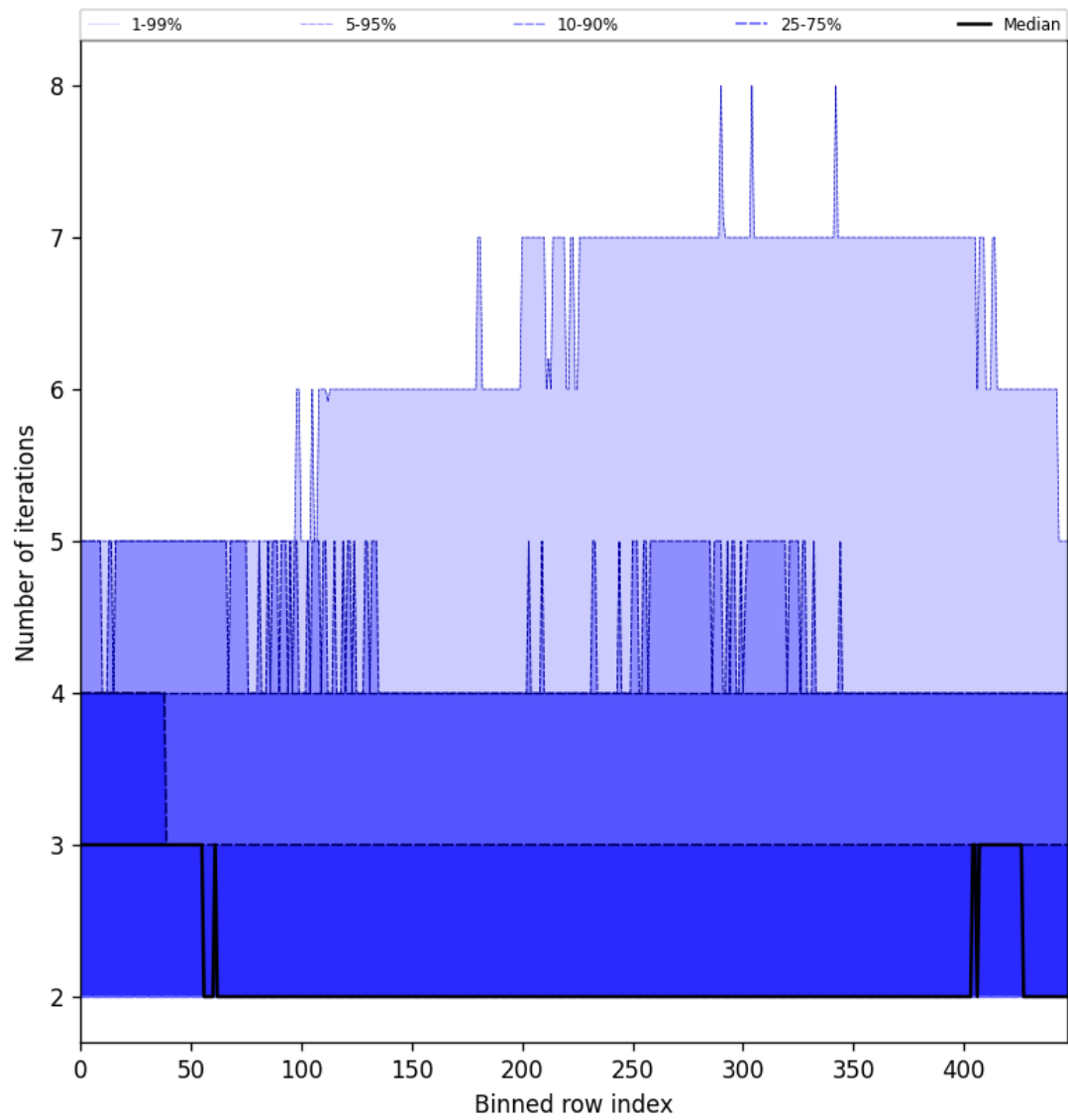
Figure 56: Along track statistics of “Number of iterations” for 2024-09-23 to 2024-09-25
