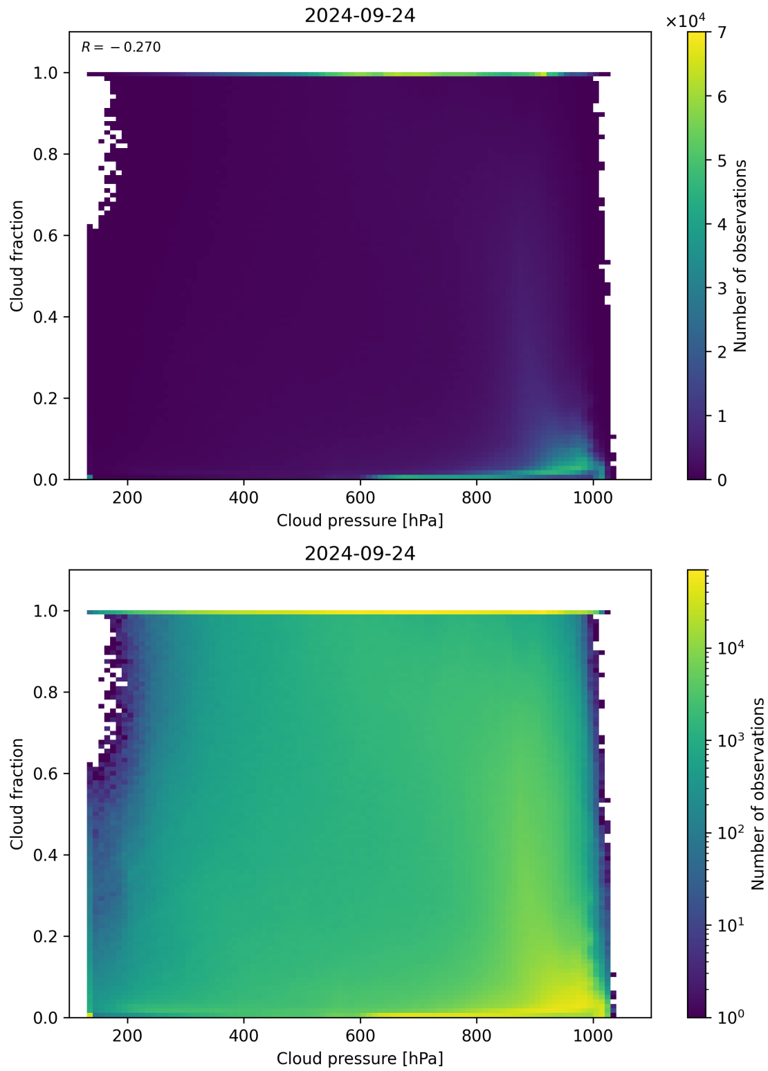
Figure 87: Scatter density plot of “Cloud pressure” against “Cloud fraction” for 2024-09-23 to 2024-09-25.
