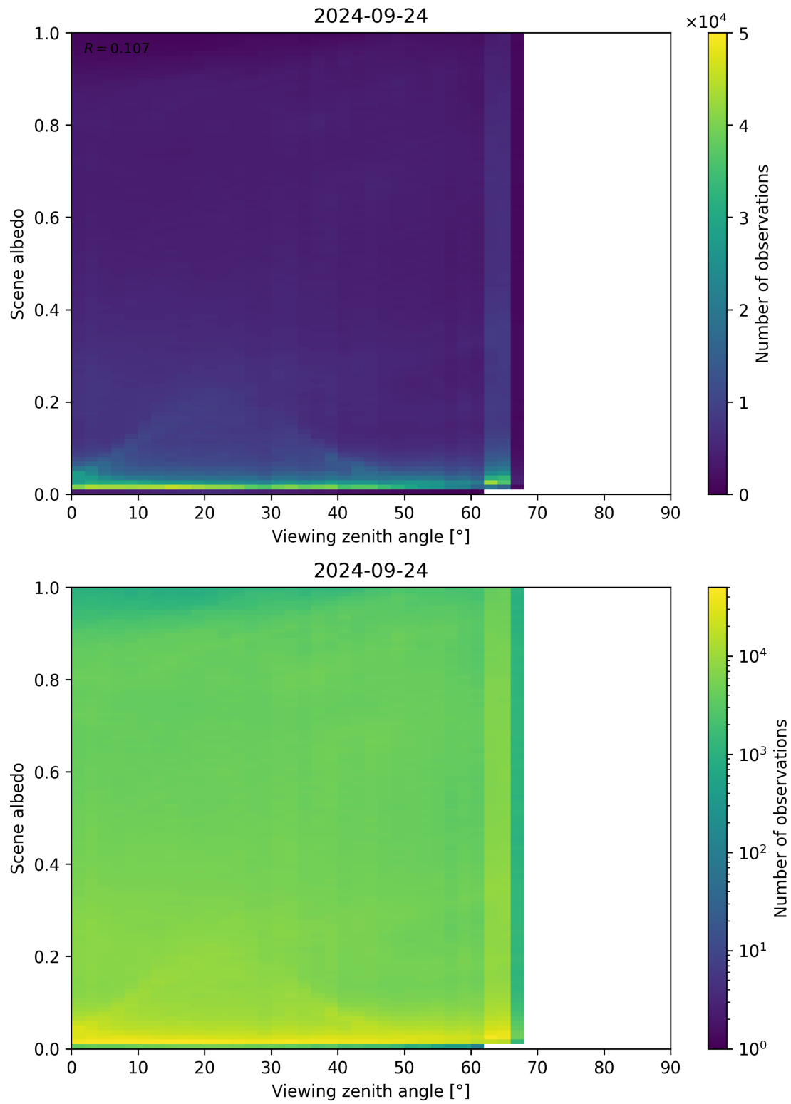
Figure 138: Scatter density plot of “Viewing zenith angle” against “Scene albedo” for 2024-09-23 to 2024-09-25.
