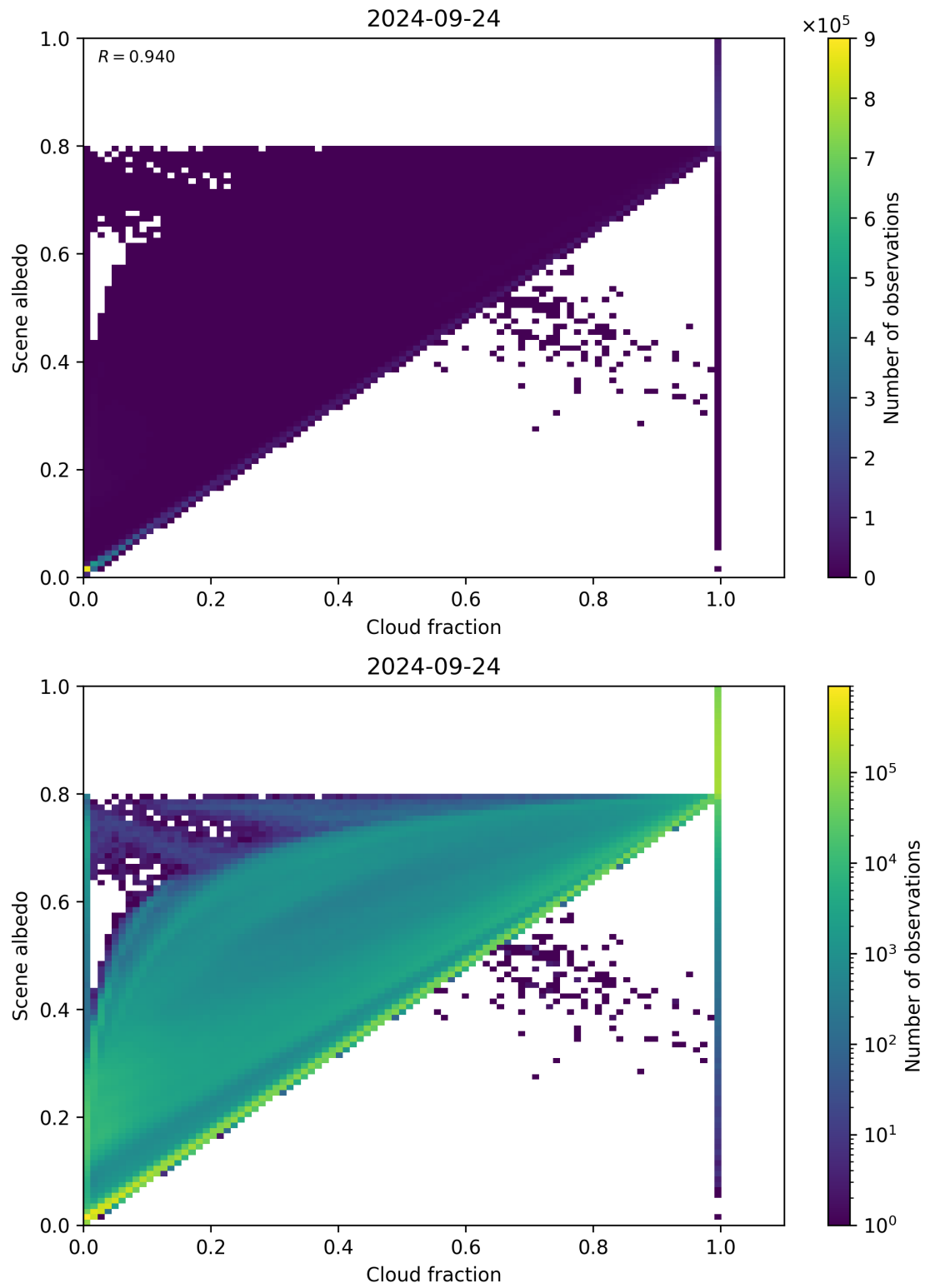
Figure 82: Scatter density plot of “Cloud fraction” against “Scene albedo” for 2024-09-23 to 2024-09-25.
