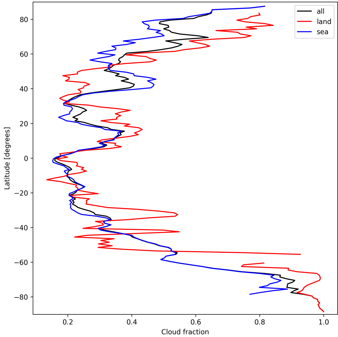
Figure 15: Zonal average of “Cloud fraction” for 2024-09-23 to 2024-09-25.
