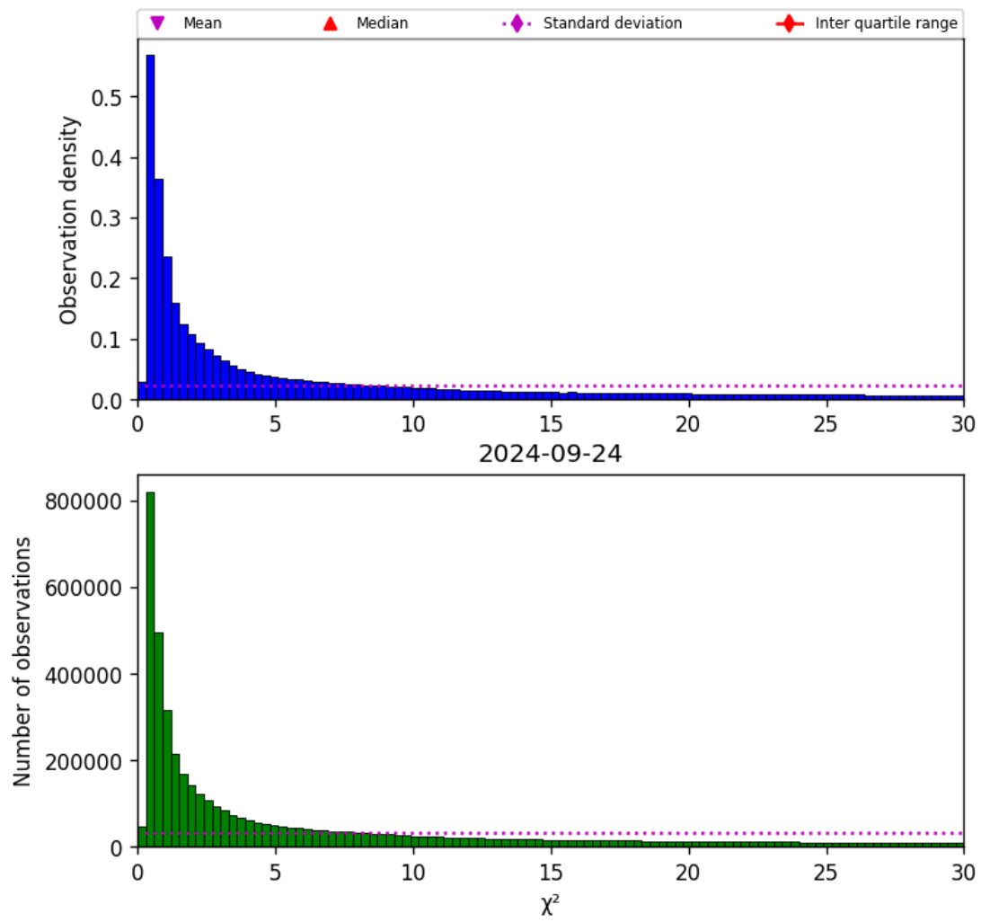
Figure 38: Histogram of " \chi^2 " for 2024-09-23 to 2024-09-25
