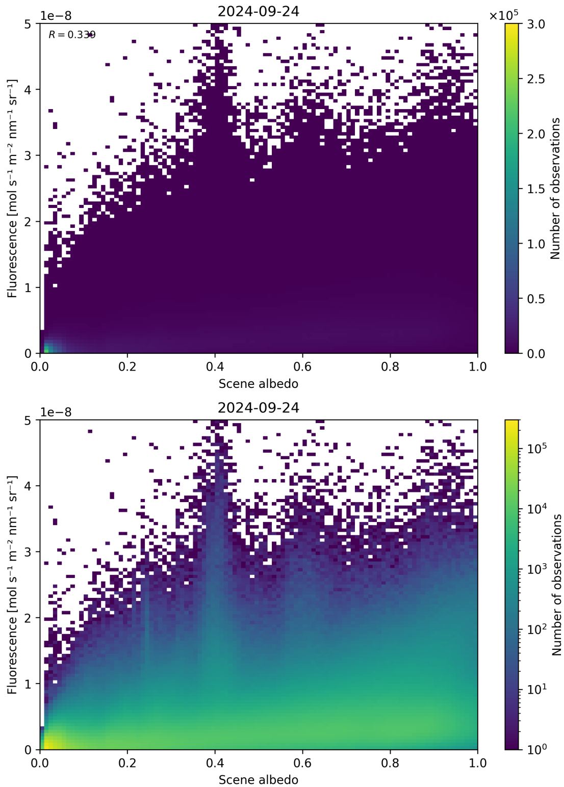
Figure 114: Scatter density plot of “Scene albedo” against “Fluorescence” for 2024-09-23 to 2024-09-25.
