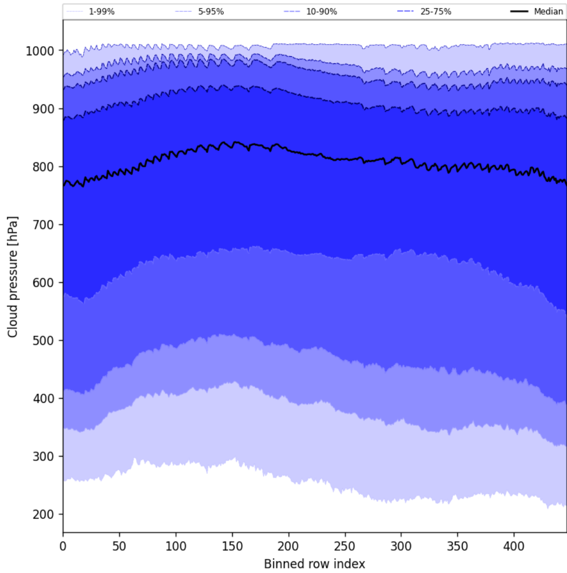
Figure 47: Along track statistics of “Cloud pressure” for 2024-09-23 to 2024-09-25
