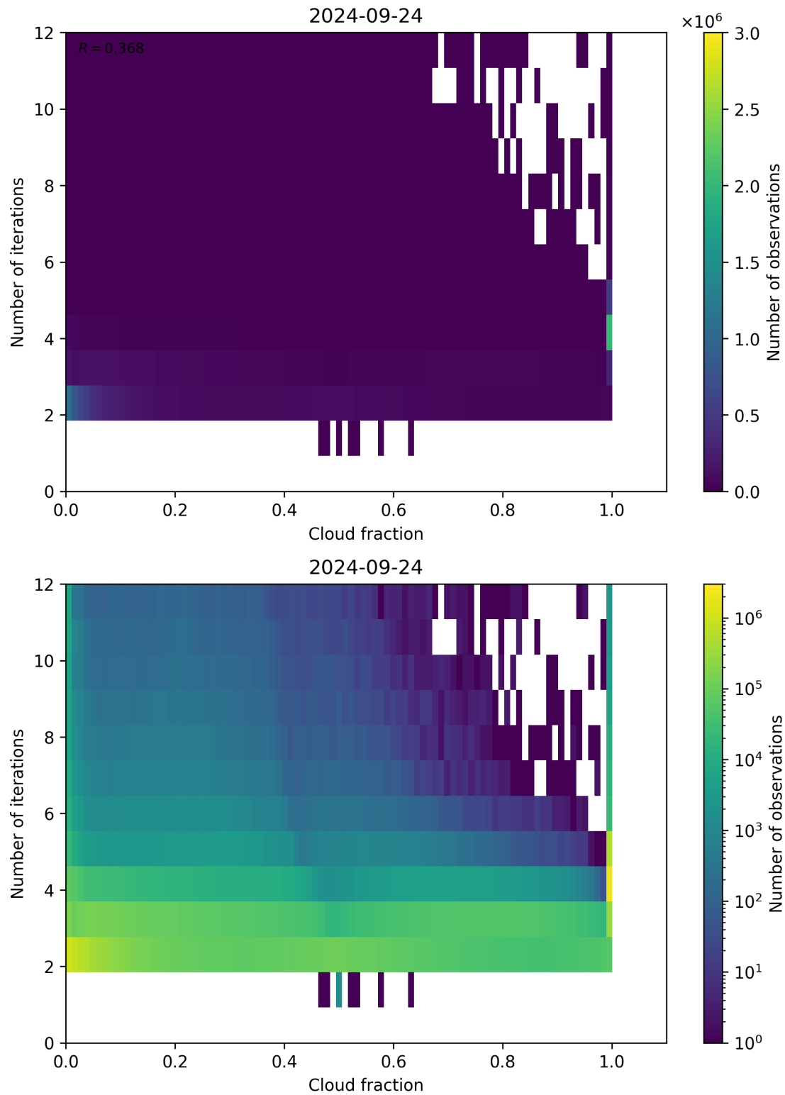
Figure 80: Scatter density plot of “Cloud fraction” against “Number of iterations” for 2024-09-23 to 2024-09-25.
