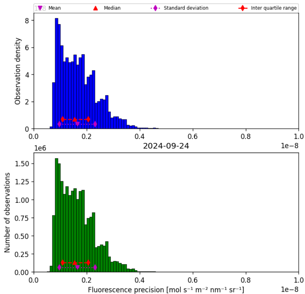
Figure 41: Histogram of “Fluorescence precision” for 2024-09-23 to 2024-09-25
