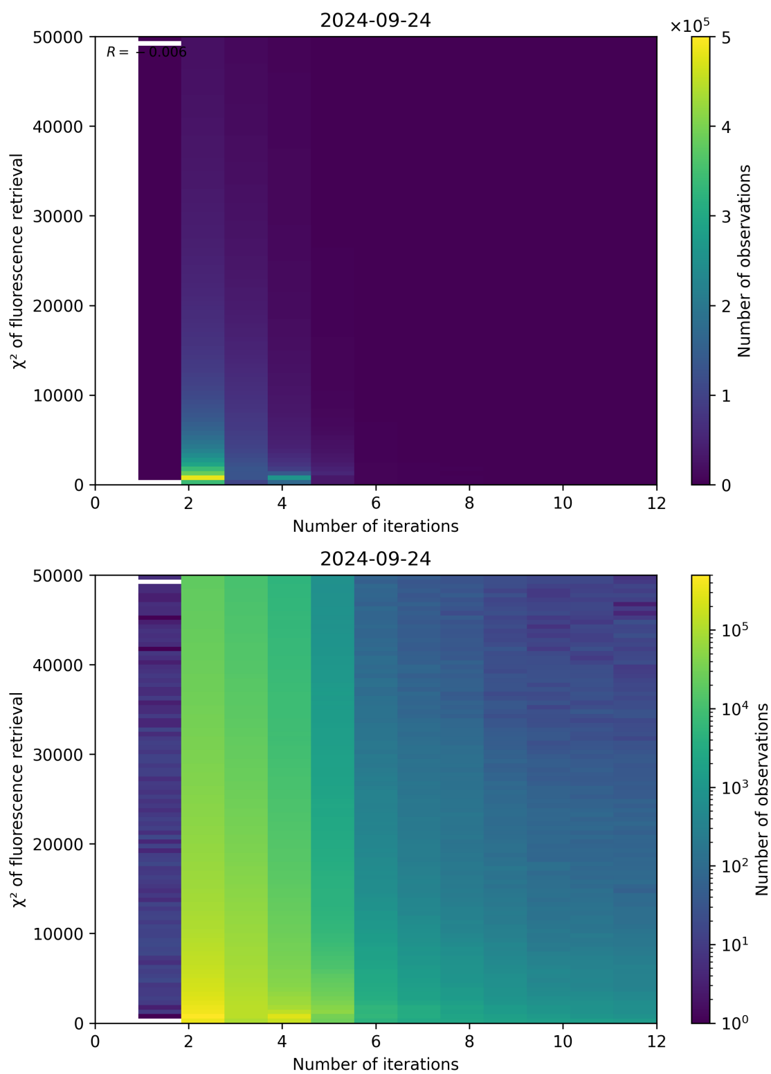
Figure 106: Scatter density plot of “Number of iterations” against “ \chi^2 of fluorescence retrieval” for 2024-09-23 to 2024-09-25.
