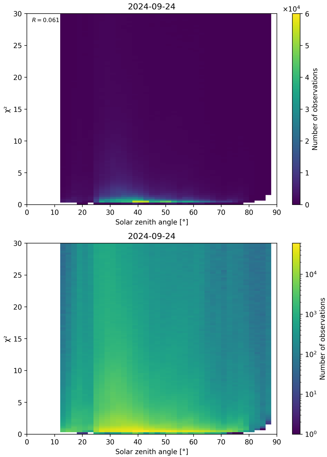
Figure 119: Scatter density plot of “Solar zenith angle” against “ \chi^2 ” for 2024-09-23 to 2024-09-25.
