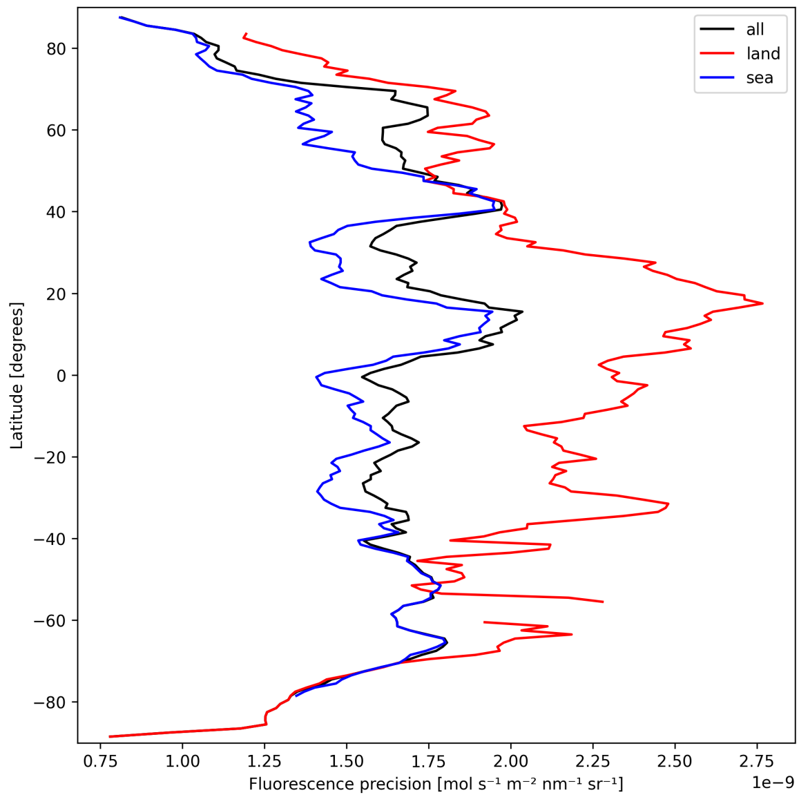
Figure 24: Zonal average of “Fluorescence precision” for 2024-09-23 to 2024-09-25.
