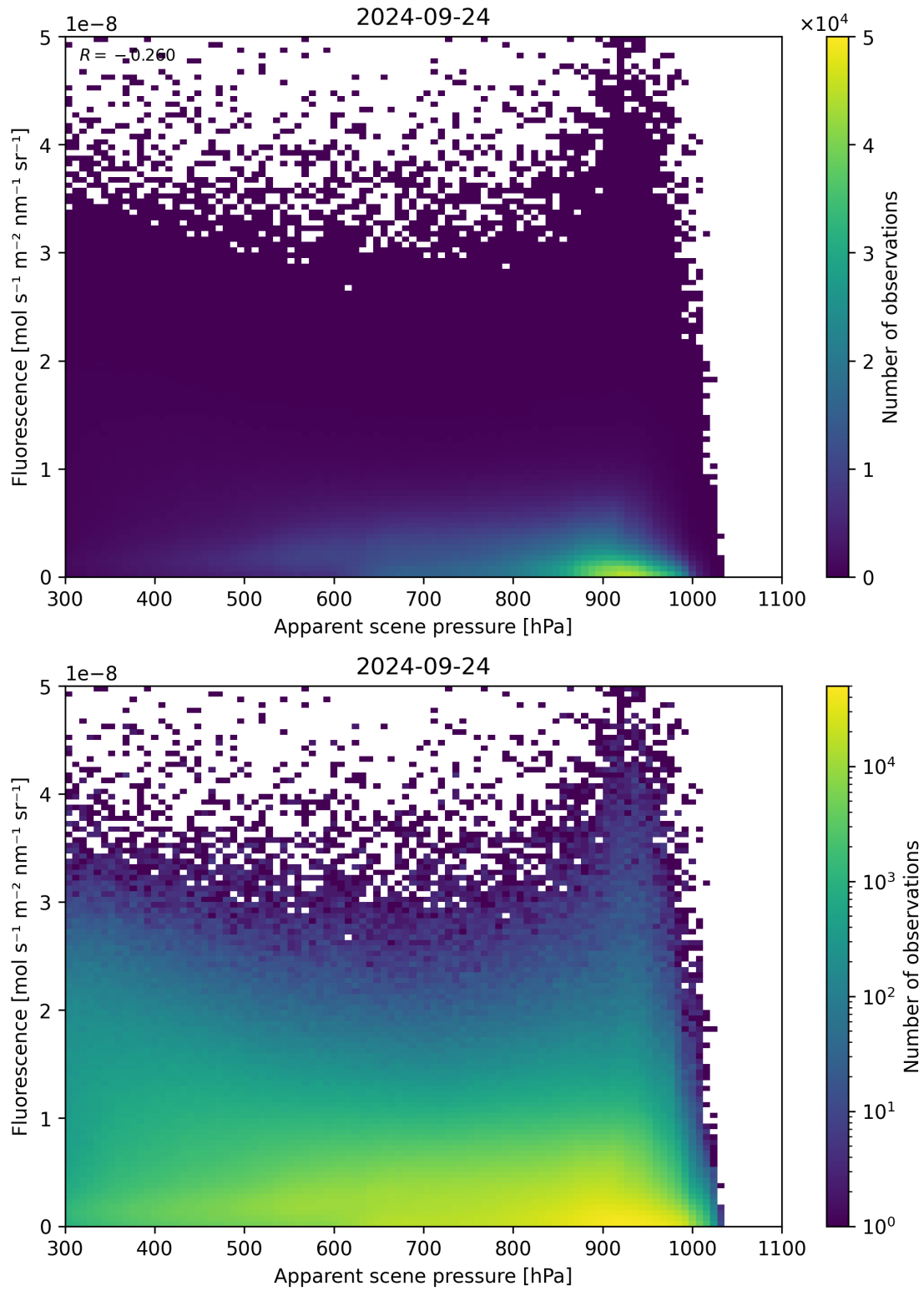
Figure 65: Scatter density plot of “Apparent scene pressure” against “Fluorescence” for 2024-09-23 to 2024-09-25.
