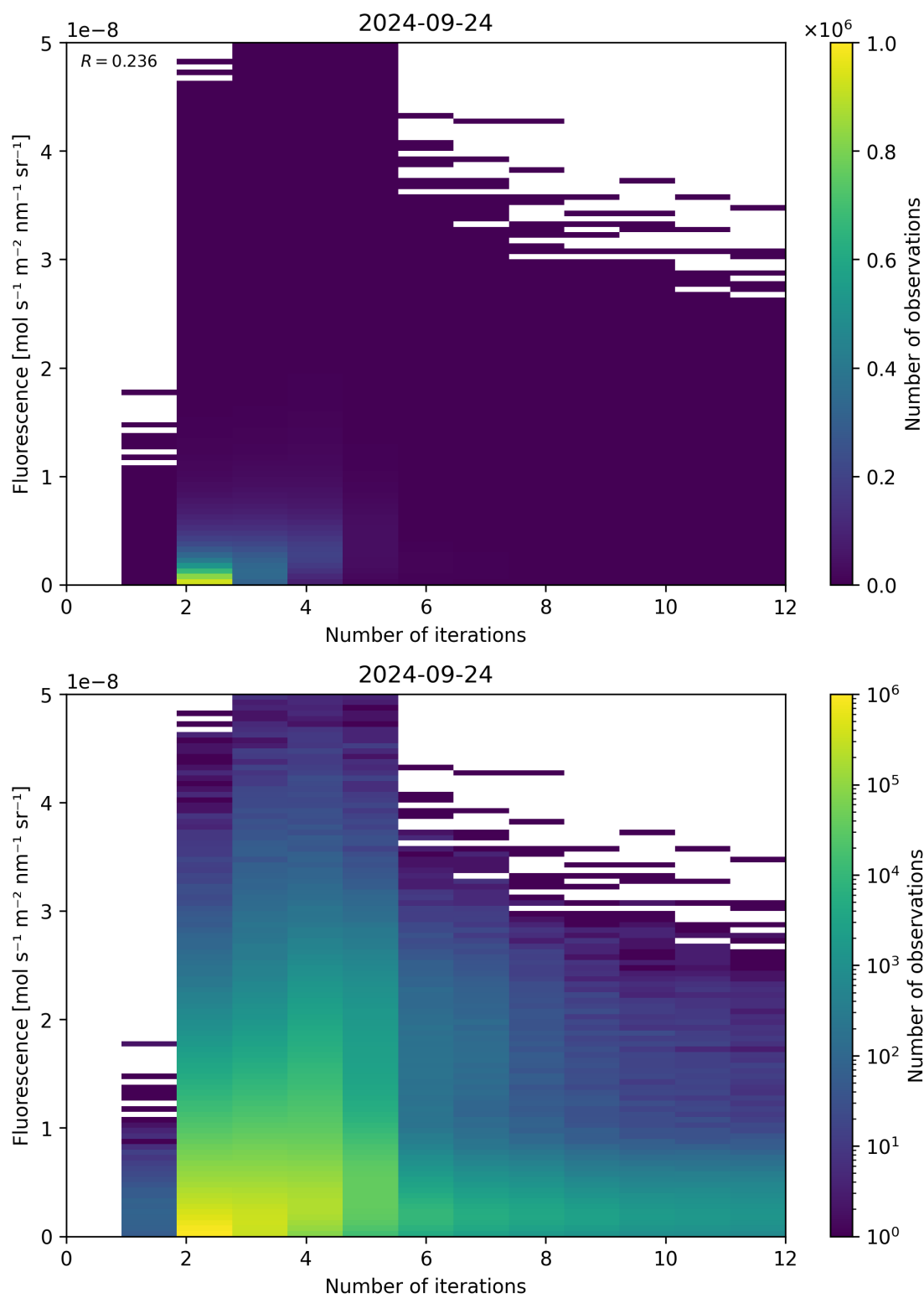
Figure 107: Scatter density plot of “Number of iterations” against “Fluorescence” for 2024-09-23 to 2024-09-25.
