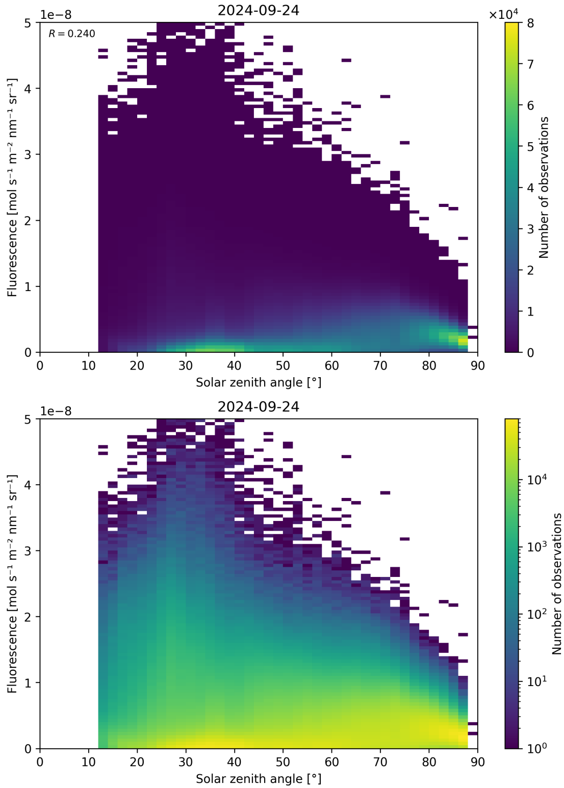
Figure 123: Scatter density plot of “Solar zenith angle” against “Fluorescence” for 2024-09-23 to 2024-09-25.
