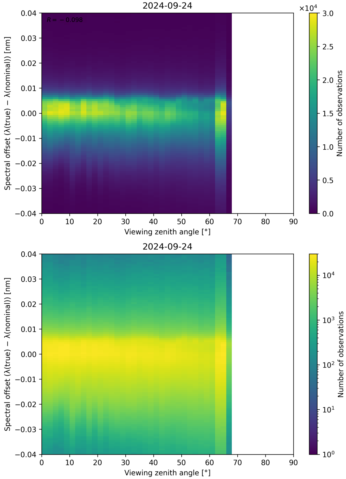
Figure 140: Scatter density plot of “Viewing zenith angle” against “Spectral offset ( \lambda_{\text{true}} - \lambda_{\text{nominal}} )” for 2024-09-23 to 2024-09-25.
