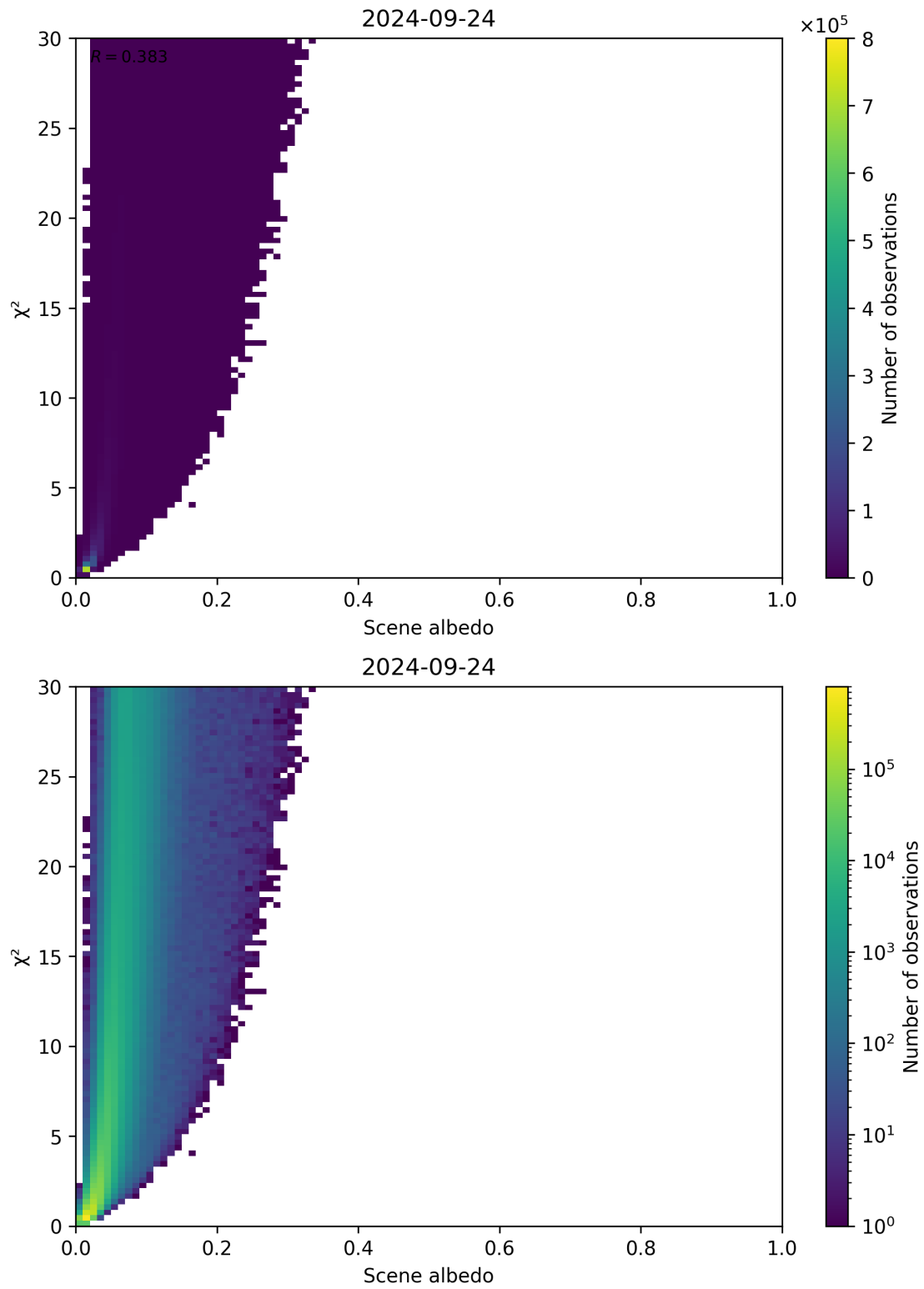
Figure 112: Scatter density plot of “Scene albedo” against “ \chi^2 ” for 2024-09-23 to 2024-09-25.
