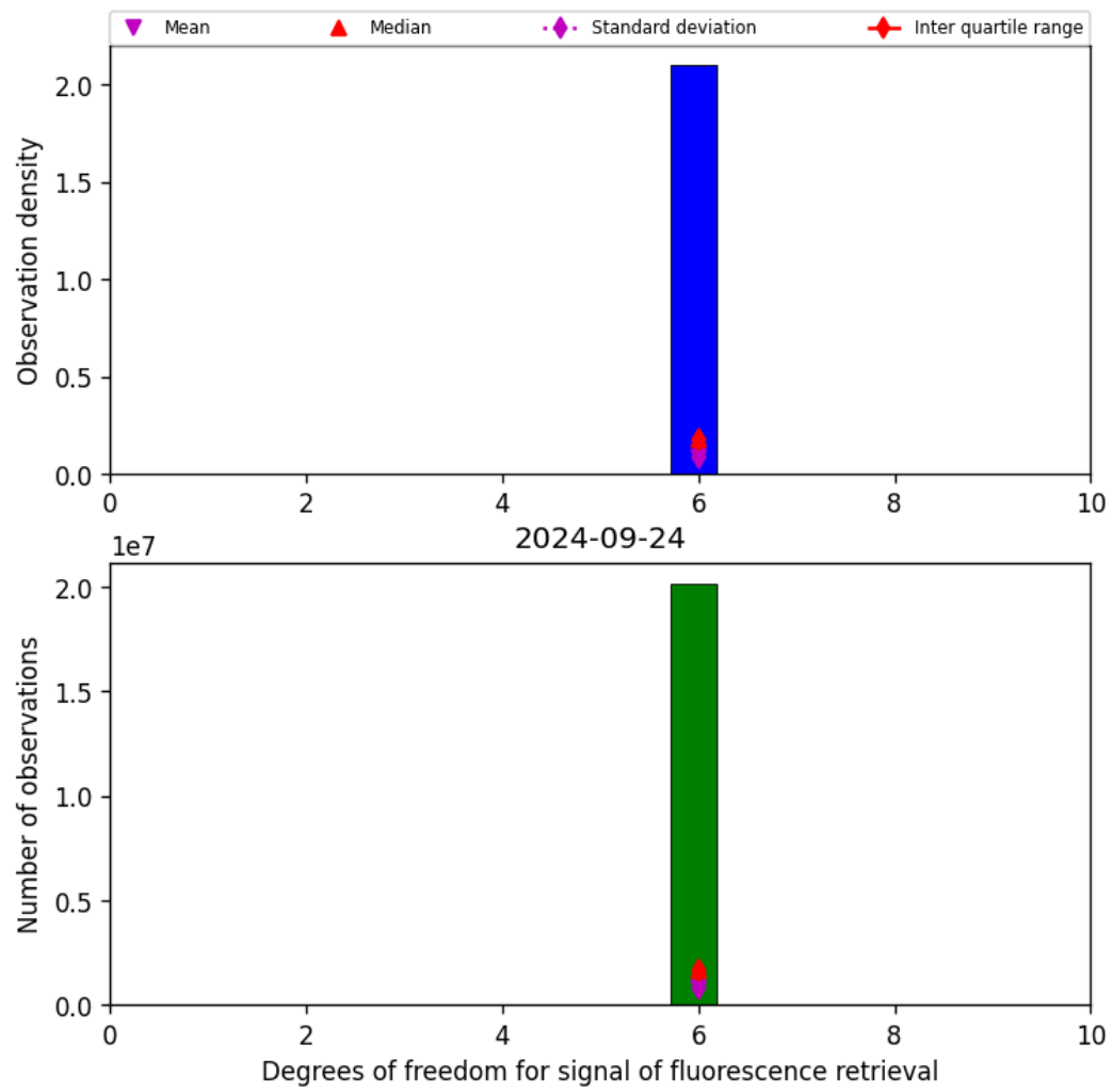
Figure 43: Histogram of "Degrees of freedom for signal of fluorescence retrieval" for 2024-09-23 to 2024-09-25
