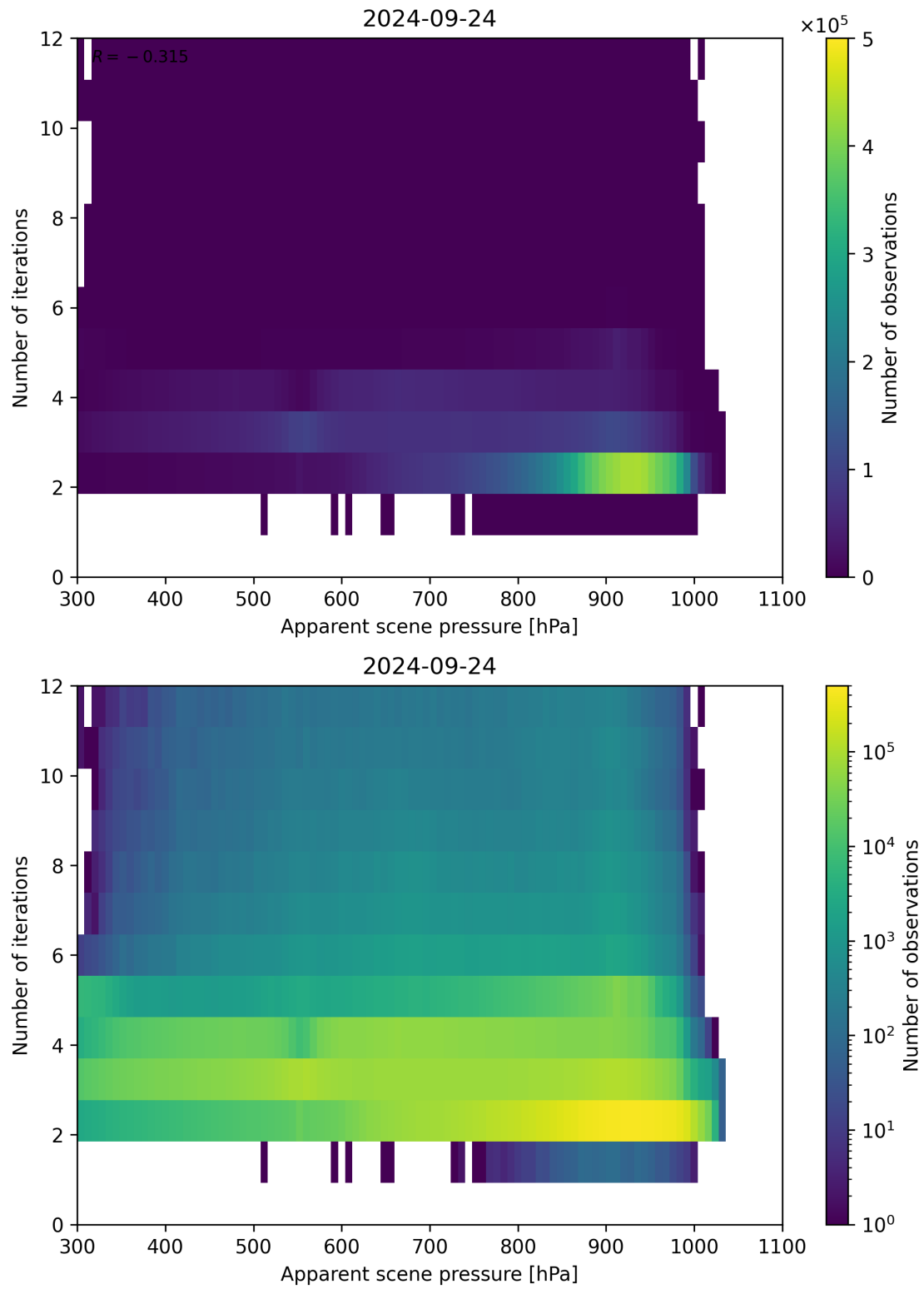
Figure 66: Scatter density plot of “Apparent scene pressure” against “Number of iterations” for 2024-09-23 to 2024-09-25.
