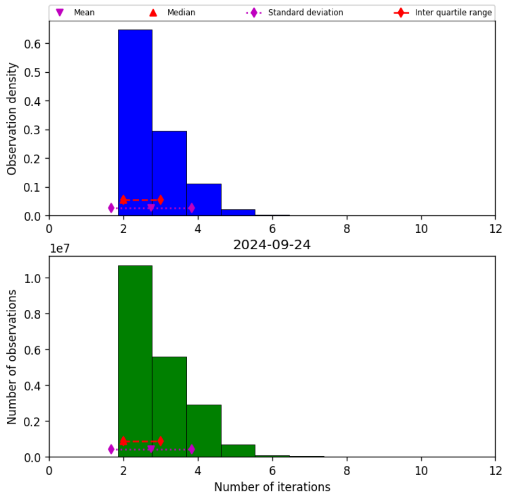
Figure 39: Histogram of “Number of iterations” for 2024-09-23 to 2024-09-25
