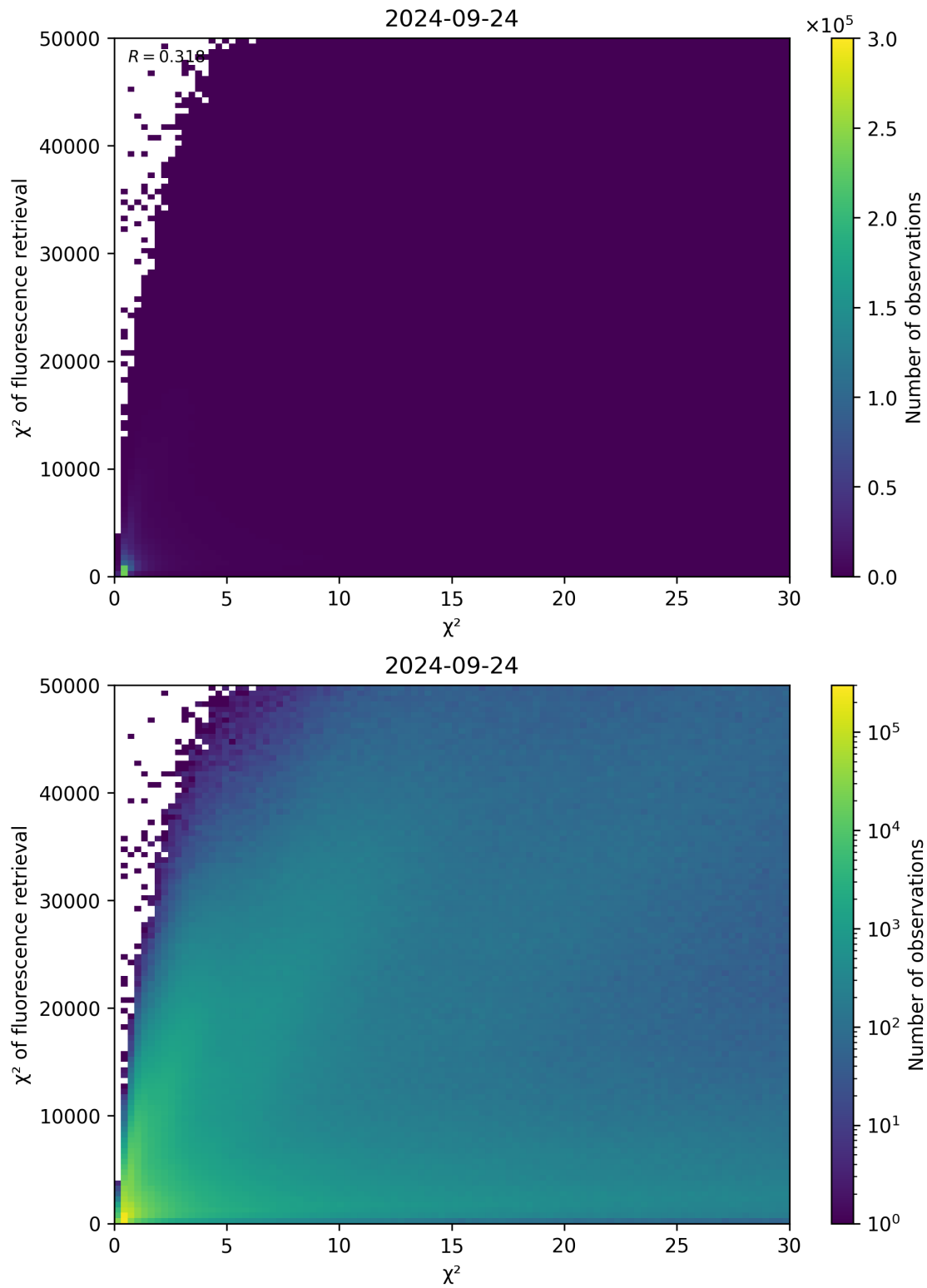
Figure 69: Scatter density plot of “ \chi^2 ” against “ \chi^2 of fluorescence retrieval” for 2024-09-23 to 2024-09-25.
