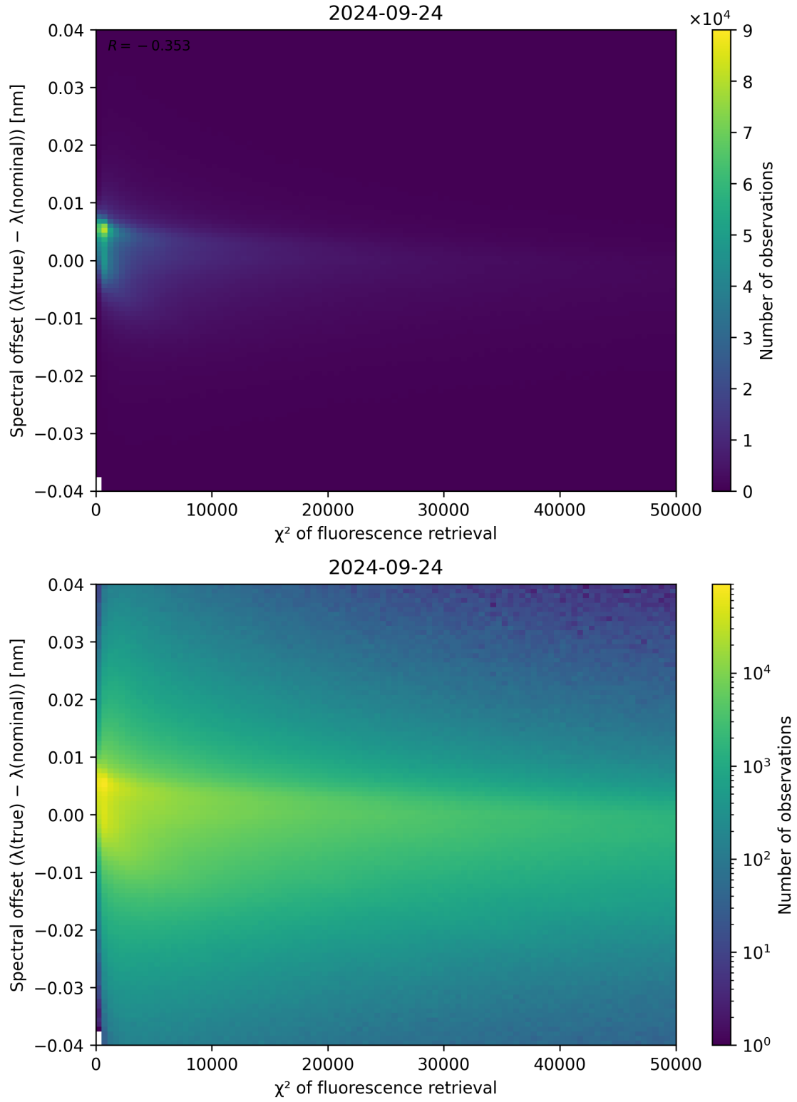
Figure 72: Scatter density plot of “ \chi^2 of fluorescence retrieval” against “Spectral offset ( \lambda_{\text{true}} - \lambda_{\text{nominal}} )” for 2024-09-23 to 2024-09-25.
