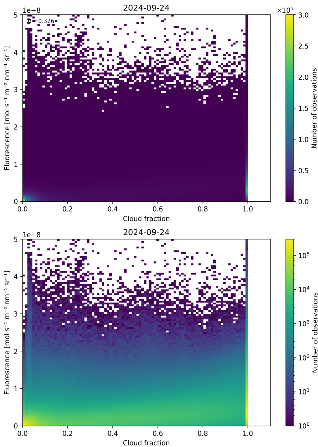
Figure 79: Scatter density plot of “Cloud fraction” against “Fluorescence” for 2024-09-23 to 2024-09-25.
