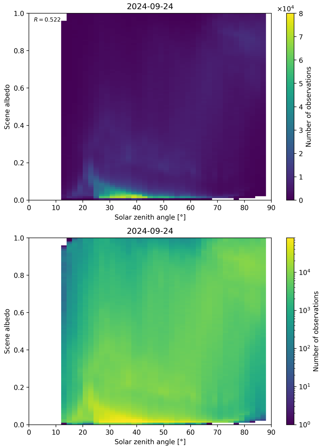
Figure 127: Scatter density plot of “Solar zenith angle” against “Scene albedo” for 2024-09-23 to 2024-09-25.
