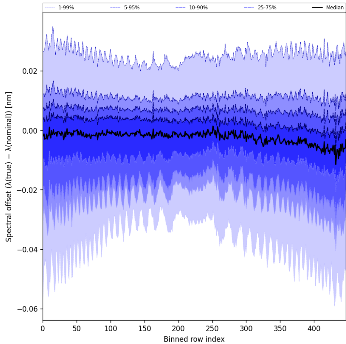
Figure 62: Along track statistics of “Spectral offset ( \lambda_{\text{true}} - \lambda_{\text{nominal}} )” for 2024-09-23 to 2024-09-25
