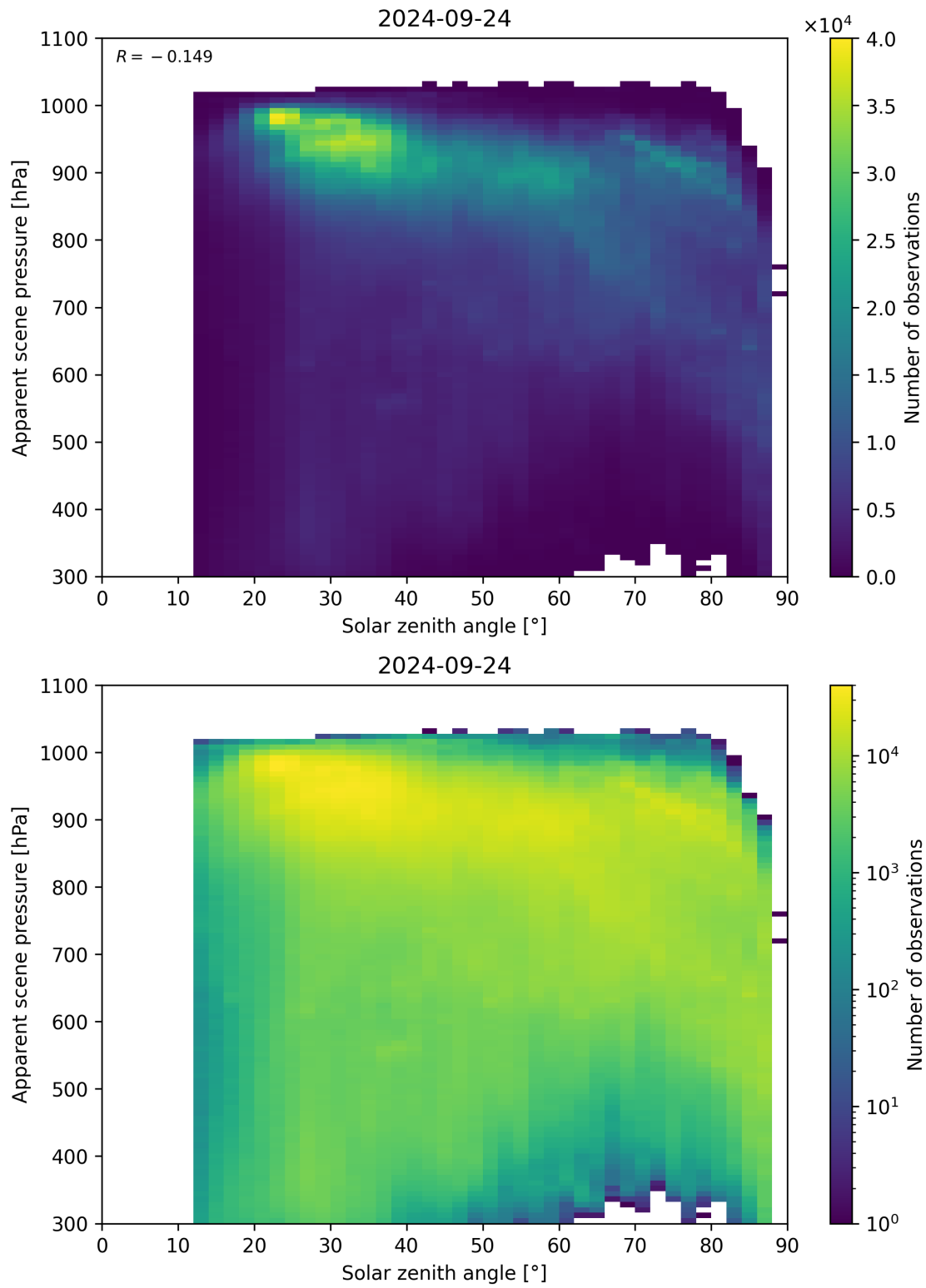
Figure 118: Scatter density plot of “Solar zenith angle” against “Apparent scene pressure” for 2024-09-23 to 2024-09-25.
