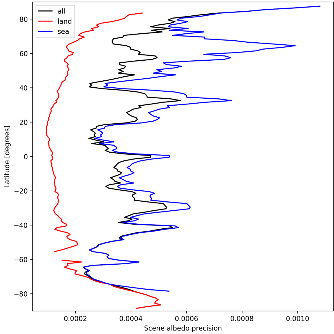
Figure 18: Zonal average of “Scene albedo precision” for 2024-09-23 to 2024-09-25.
