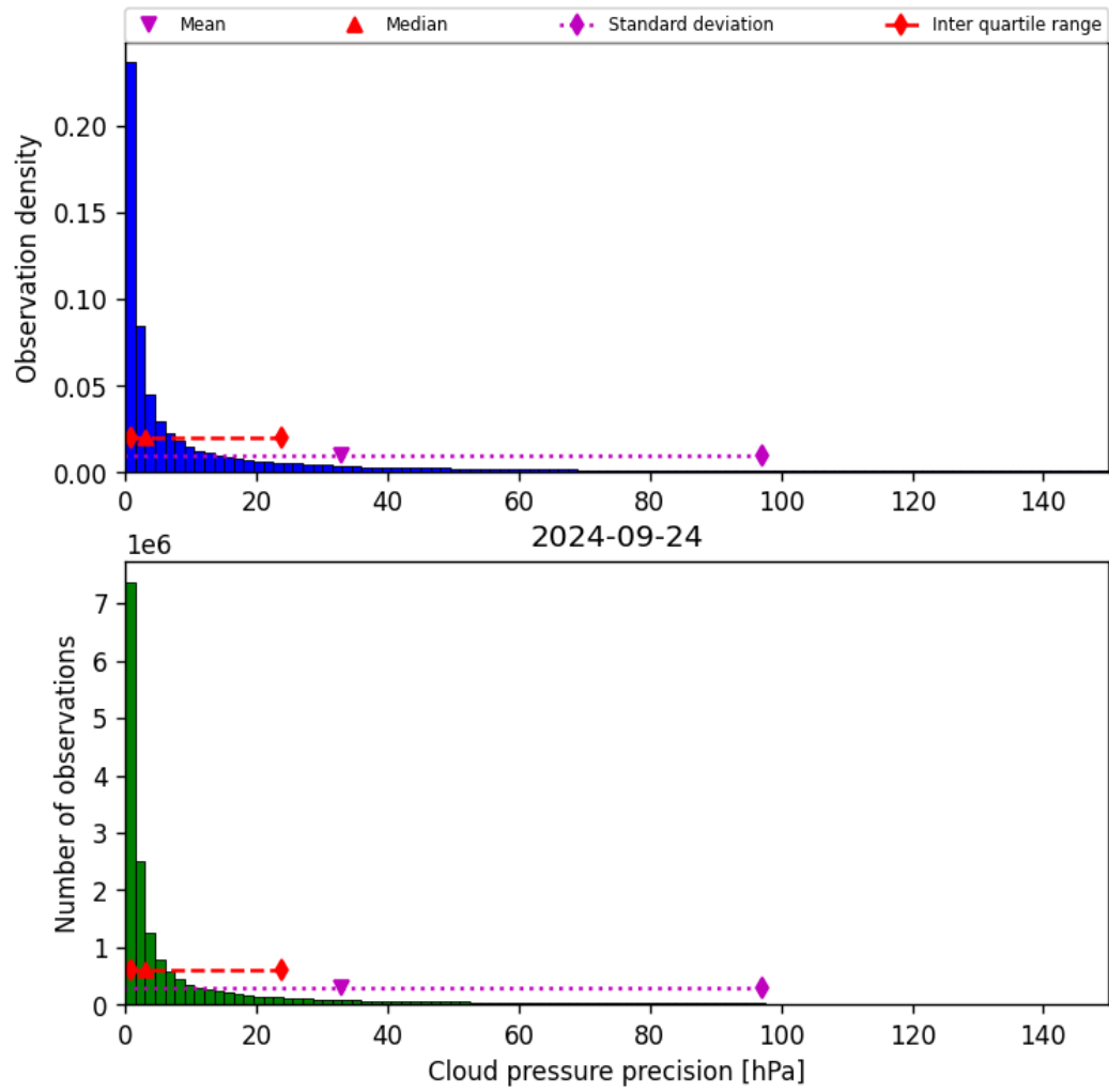
Figure 31: Histogram of “Cloud pressure precision” for 2024-09-23 to 2024-09-25
