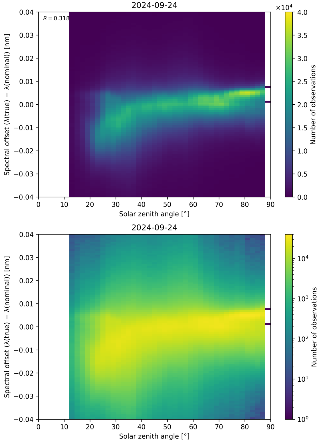
Figure 128: Scatter density plot of “Solar zenith angle” against “Spectral offset ( \lambda_{\text{true}} - \lambda_{\text{nominal}} )” for 2024-09-23 to 2024-09-25.
