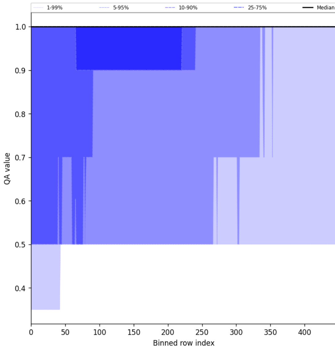
Figure 46: Along track statistics of “QA value” for 2024-09-23 to 2024-09-25
