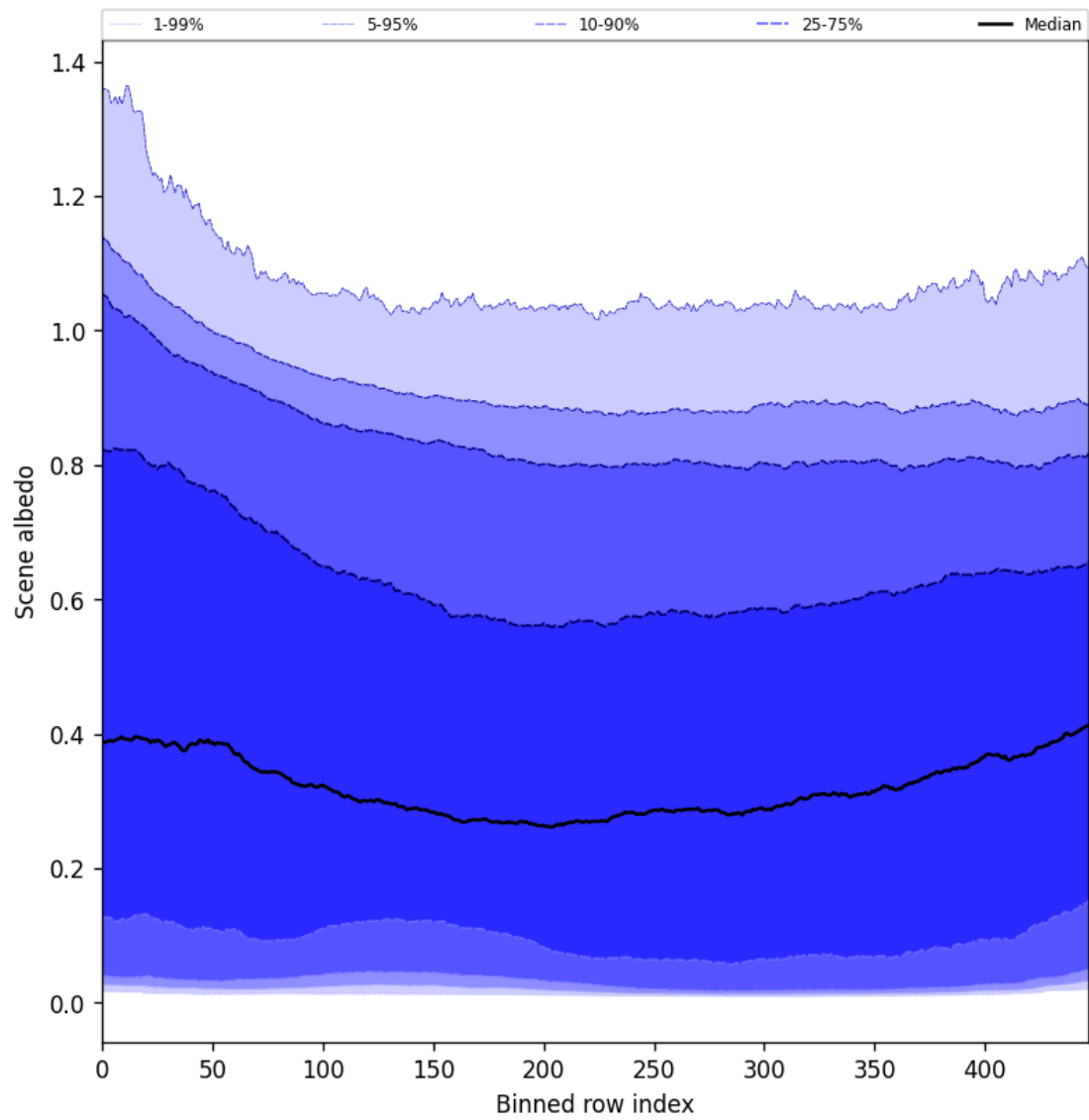
Figure 51: Along track statistics of “Scene albedo” for 2024-09-23 to 2024-09-25
