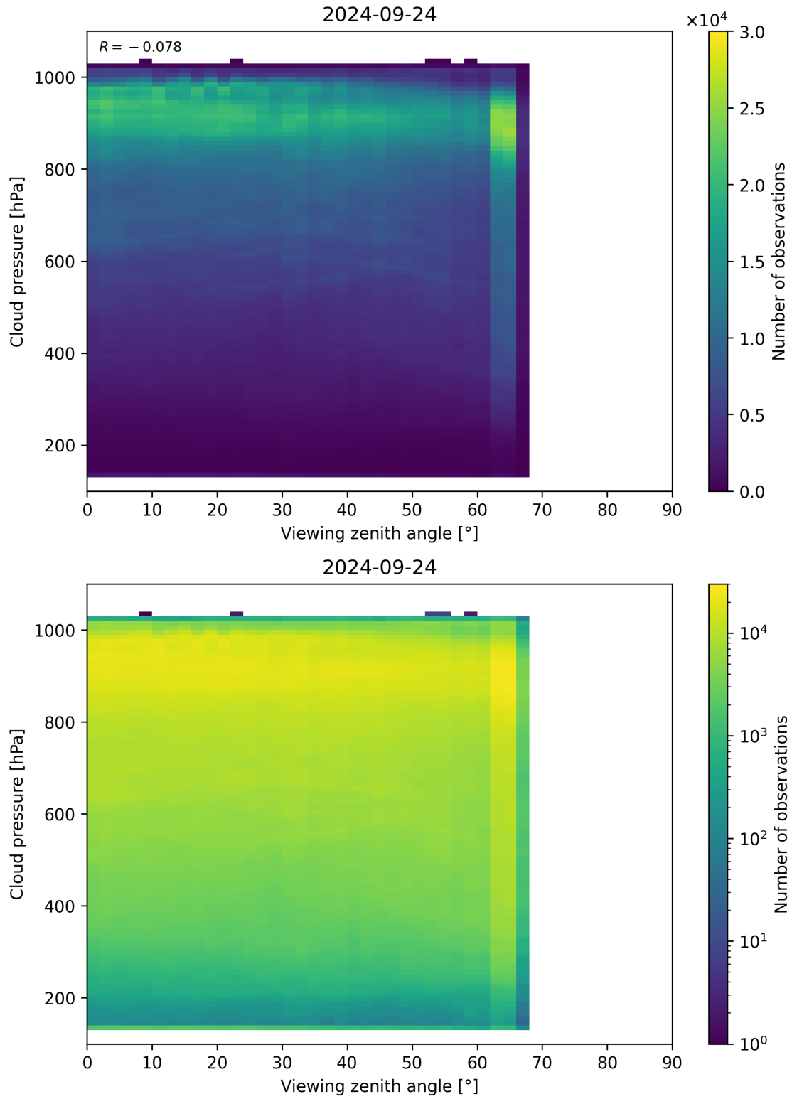
Figure 133: Scatter density plot of “Viewing zenith angle” against “Cloud pressure” for 2024-09-23 to 2024-09-25.
