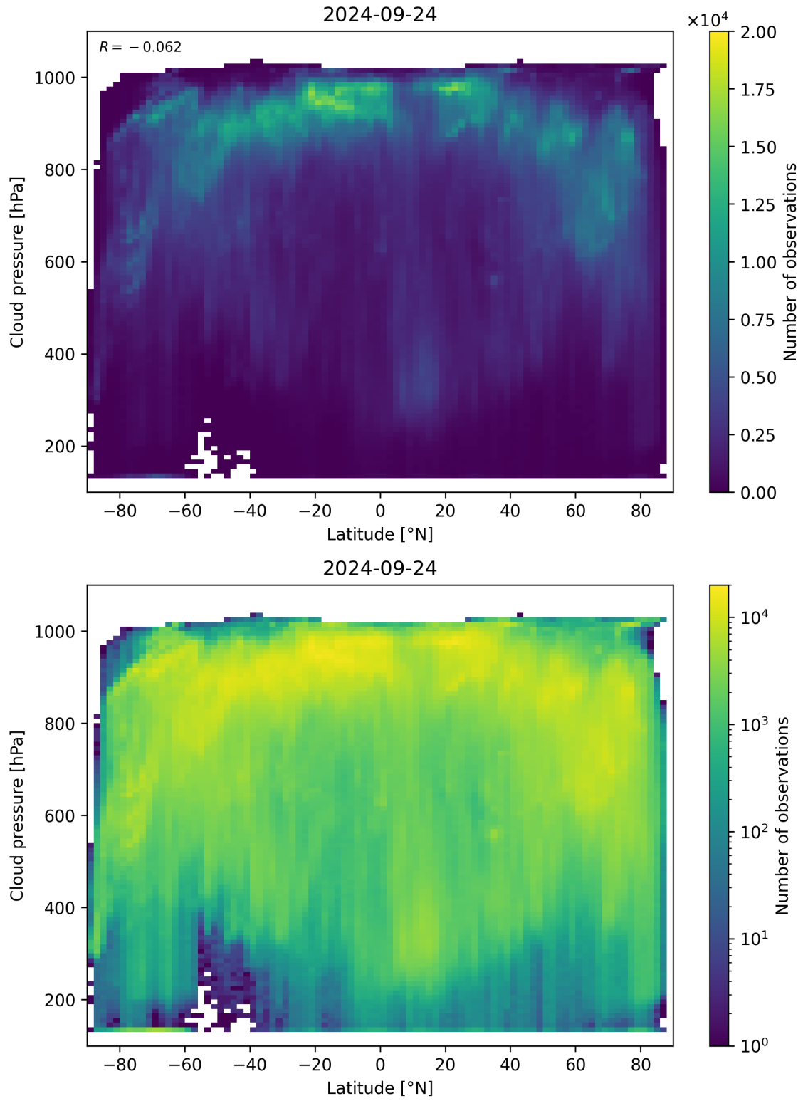
Figure 100: Scatter density plot of “Latitude” against “Cloud pressure” for 2024-09-23 to 2024-09-25.
