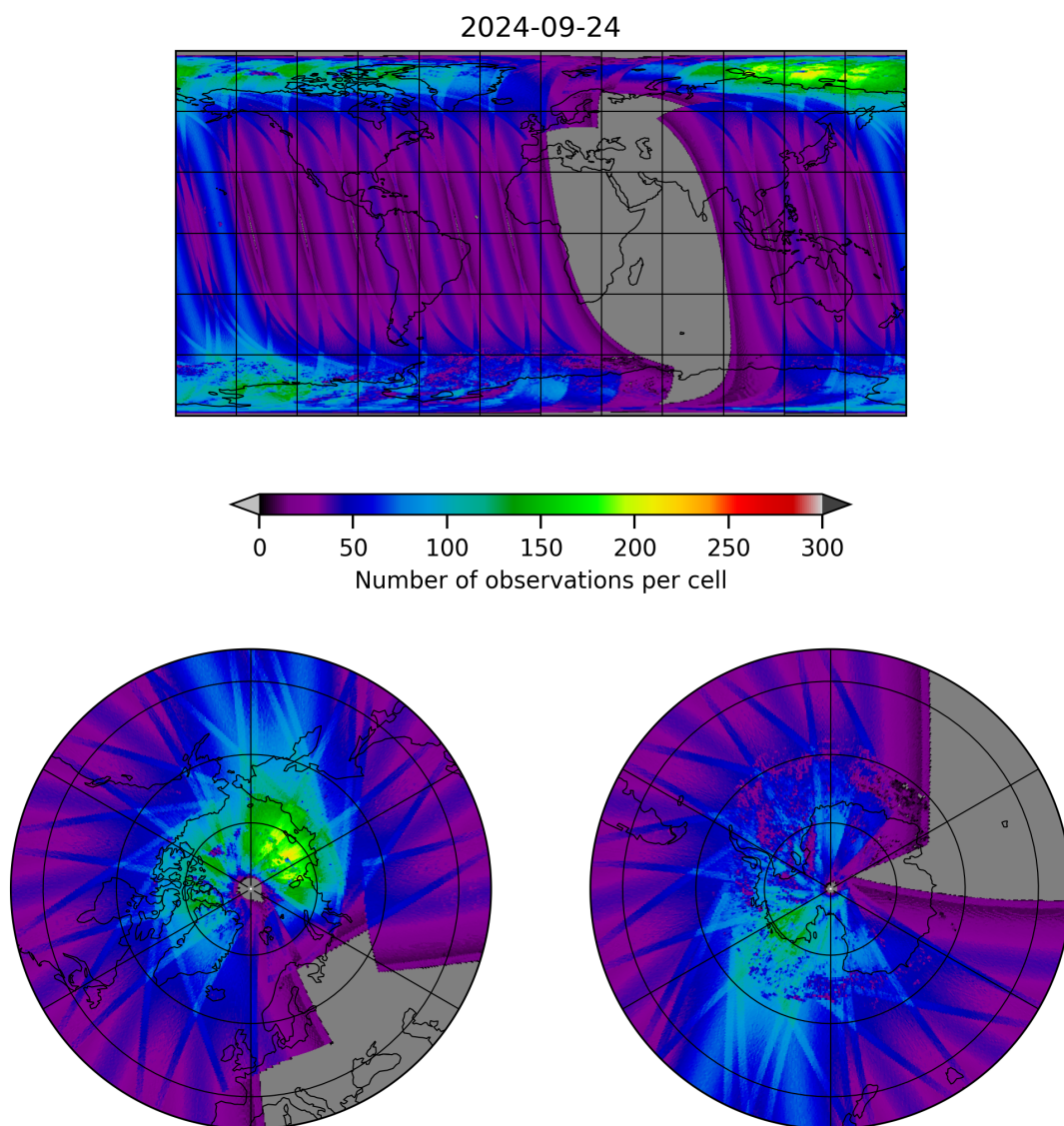
Figure 11: Map of the number of observations for 2024-09-23 to 2024-09-25
