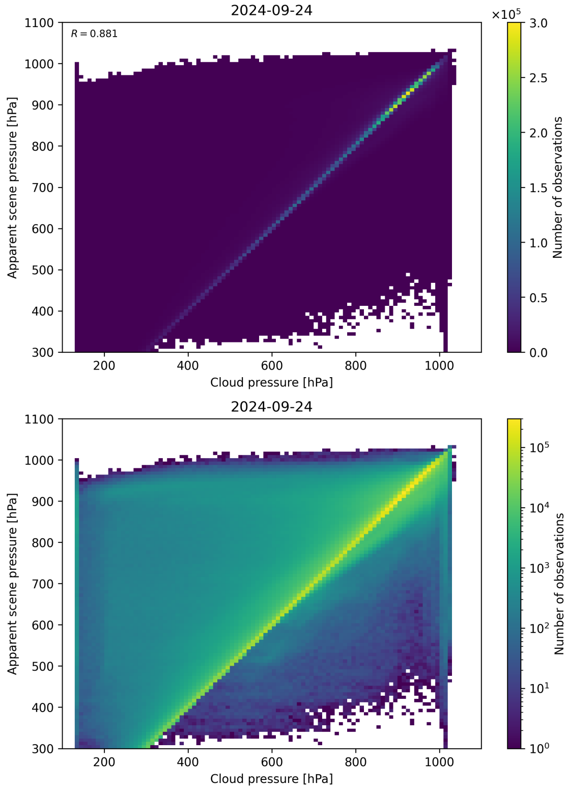
Figure 84: Scatter density plot of “Cloud pressure” against “Apparent scene pressure” for 2024-09-23 to 2024-09-25.
