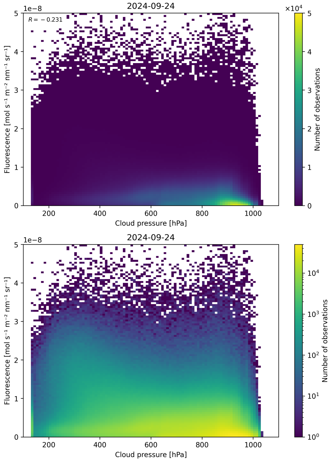
Figure 88: Scatter density plot of “Cloud pressure” against “Fluorescence” for 2024-09-23 to 2024-09-25.
