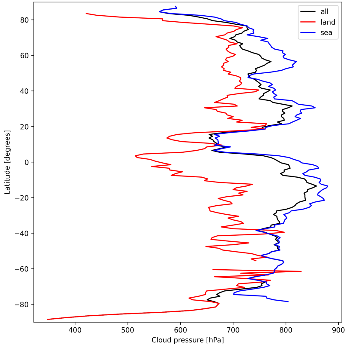
Figure 13: Zonal average of “Cloud pressure” for 2024-09-23 to 2024-09-25.
