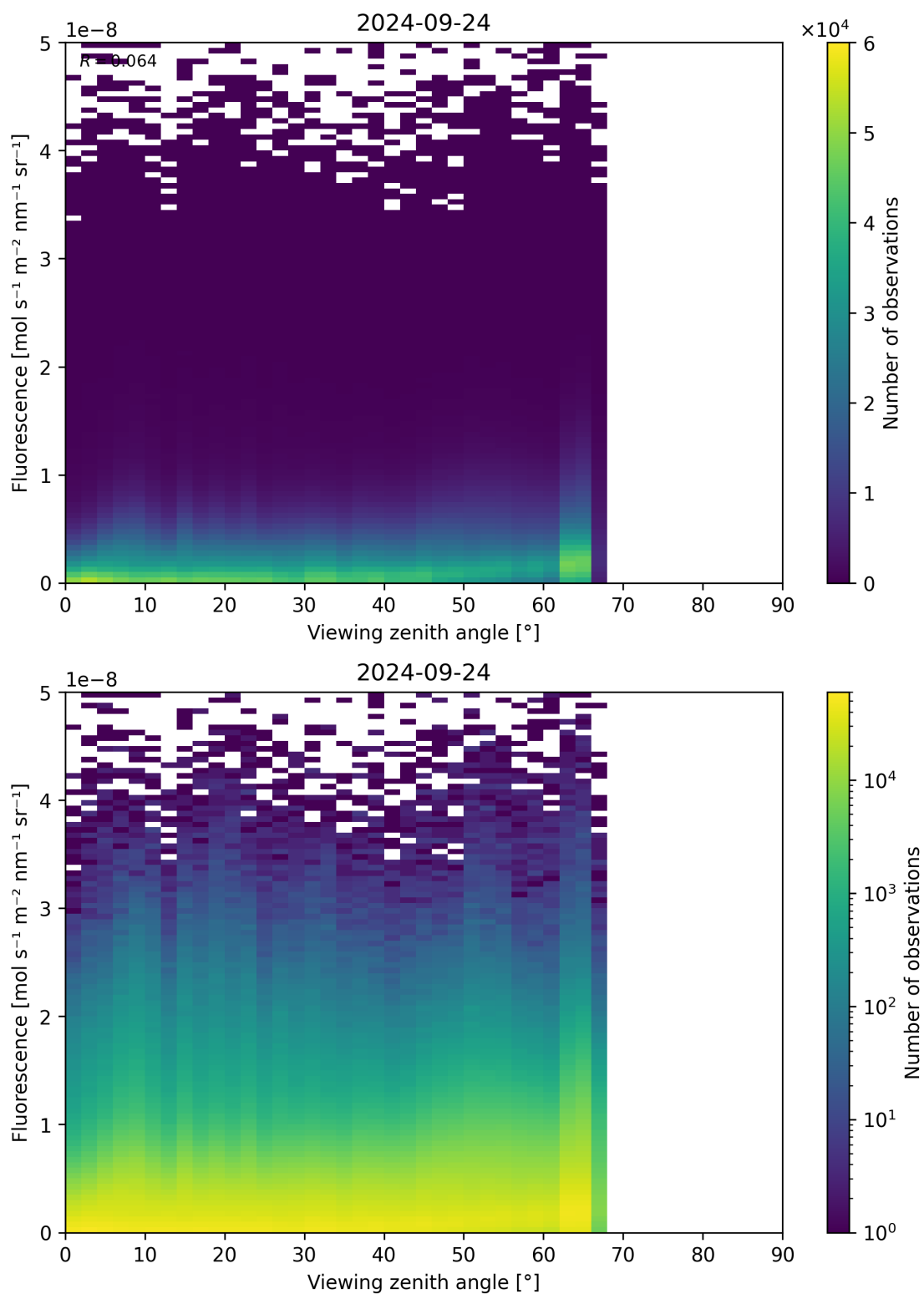
Figure 134: Scatter density plot of “Viewing zenith angle” against “Fluorescence” for 2024-09-23 to 2024-09-25.
