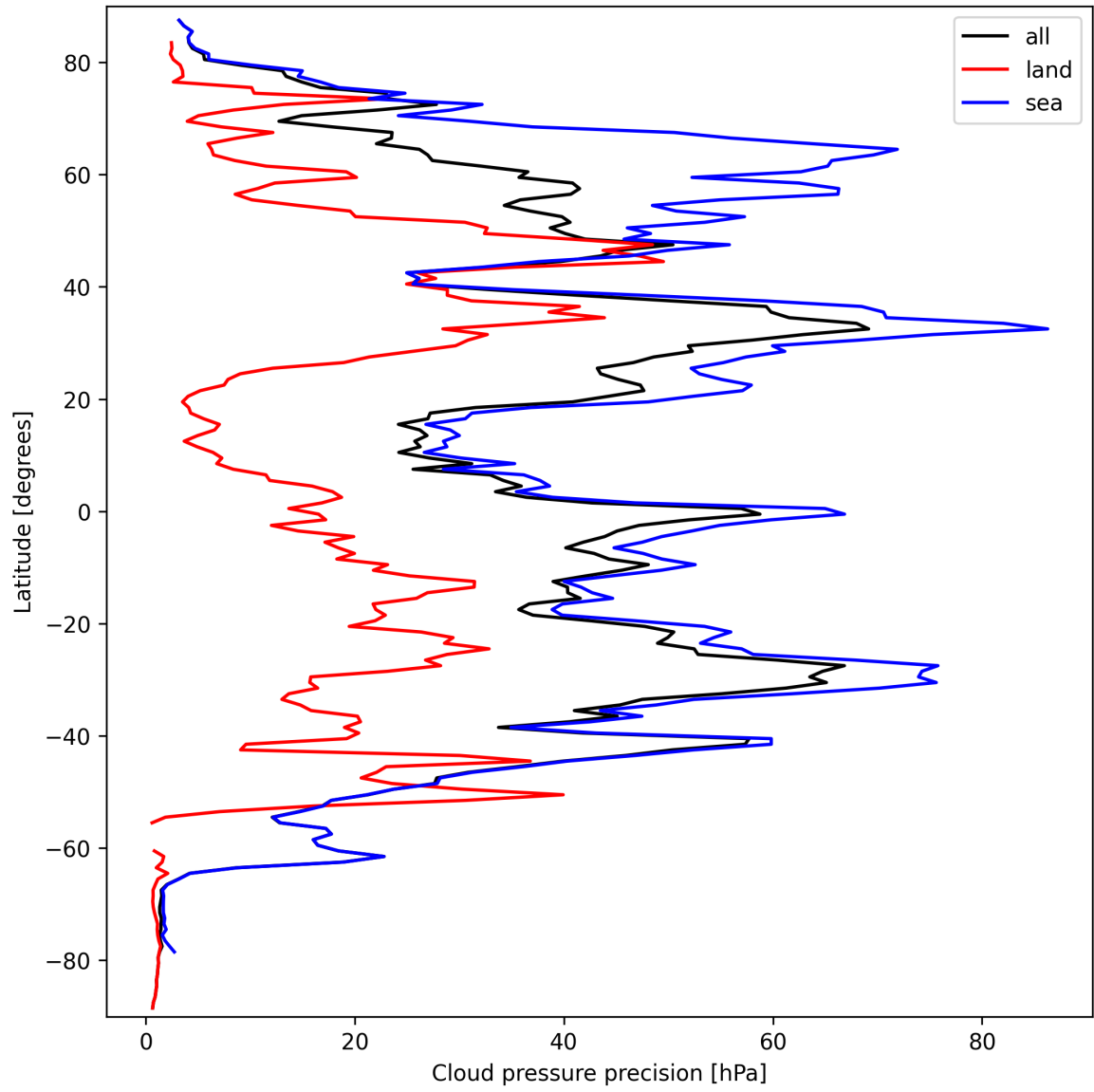
Figure 14: Zonal average of “Cloud pressure precision” for 2024-09-23 to 2024-09-25.
