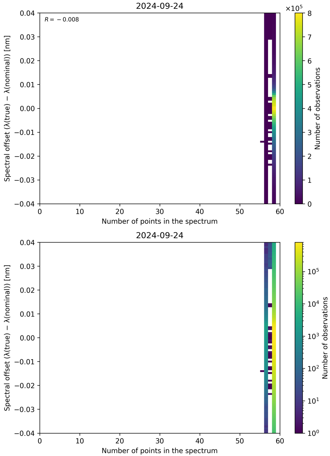
Figure 110: Scatter density plot of “Number of points in the spectrum” against “Spectral offset ( \lambda_{\text{true}} - \lambda_{\text{nominal}} )” for 2024-09-23 to 2024-09-25.
