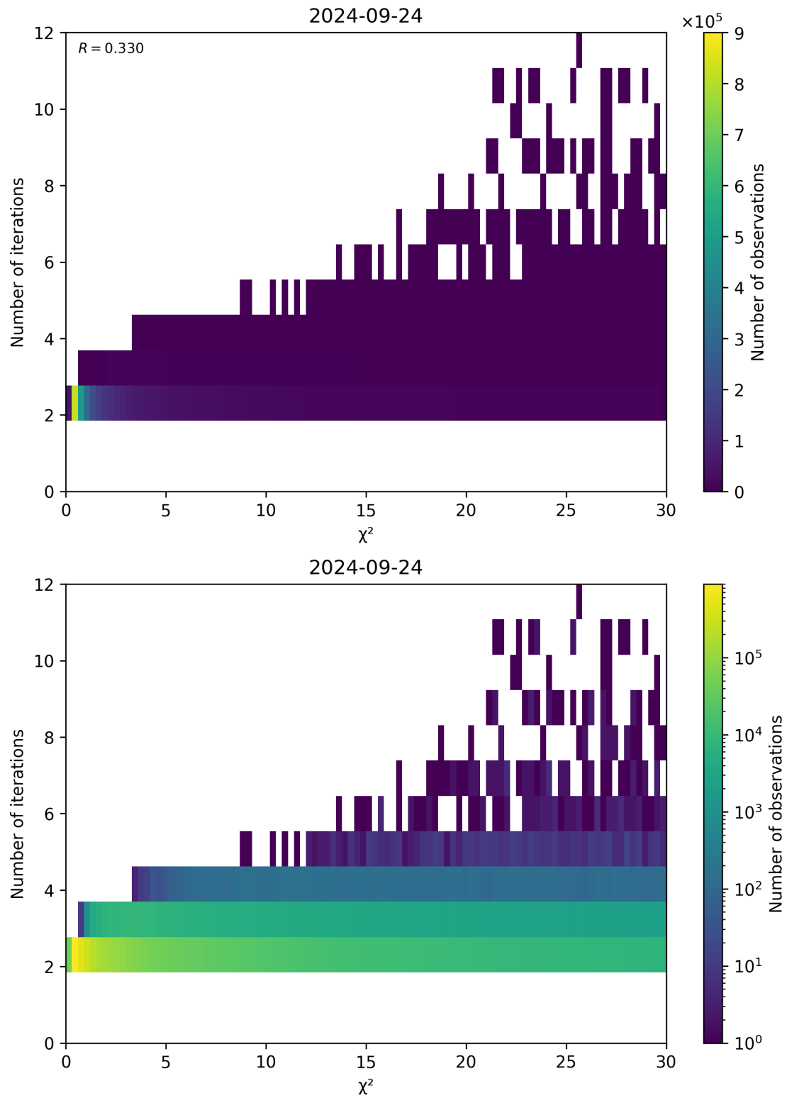
Figure 73: Scatter density plot of “ \chi^2 ” against “Number of iterations” for 2024-09-23 to 2024-09-25.
