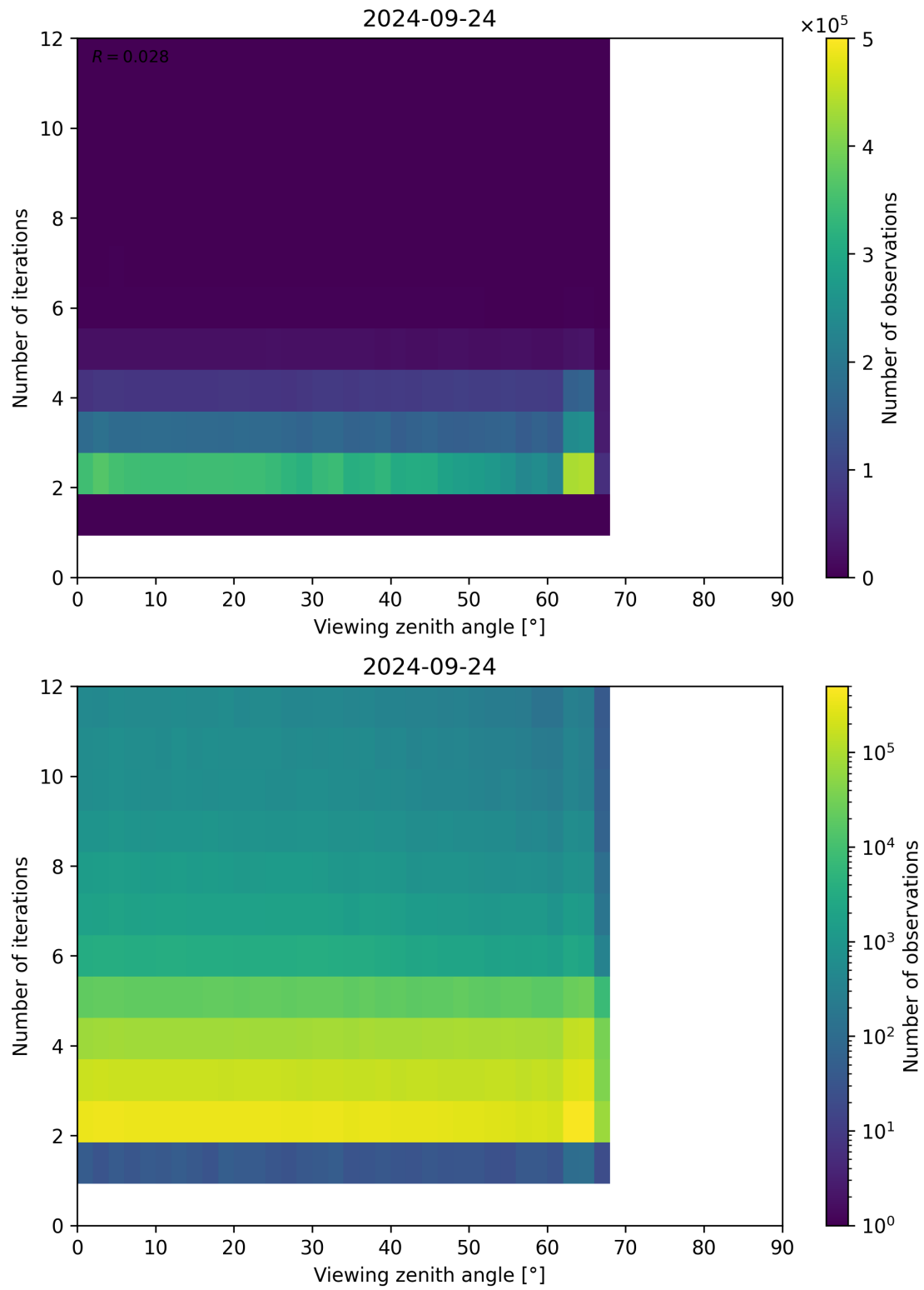
Figure 136: Scatter density plot of “Viewing zenith angle” against “Number of iterations” for 2024-09-23 to 2024-09-25.
