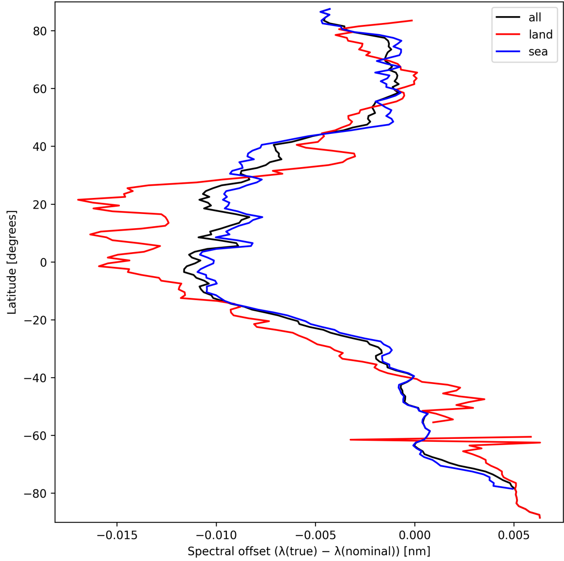
Figure 28: Zonal average of “Spectral offset ( \lambda_{\text{true}} - \lambda_{\text{nominal}} )” for 2024-09-23 to 2024-09-25.
