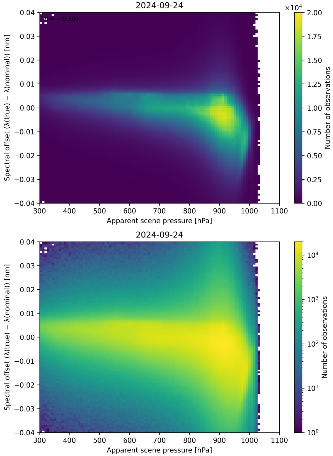
Figure 68: Scatter density plot of “Apparent scene pressure” against “Spectral offset ( \lambda_{\text{true}} - \lambda_{\text{nominal}} )” for 2024-09-23 to 2024-09-25.
