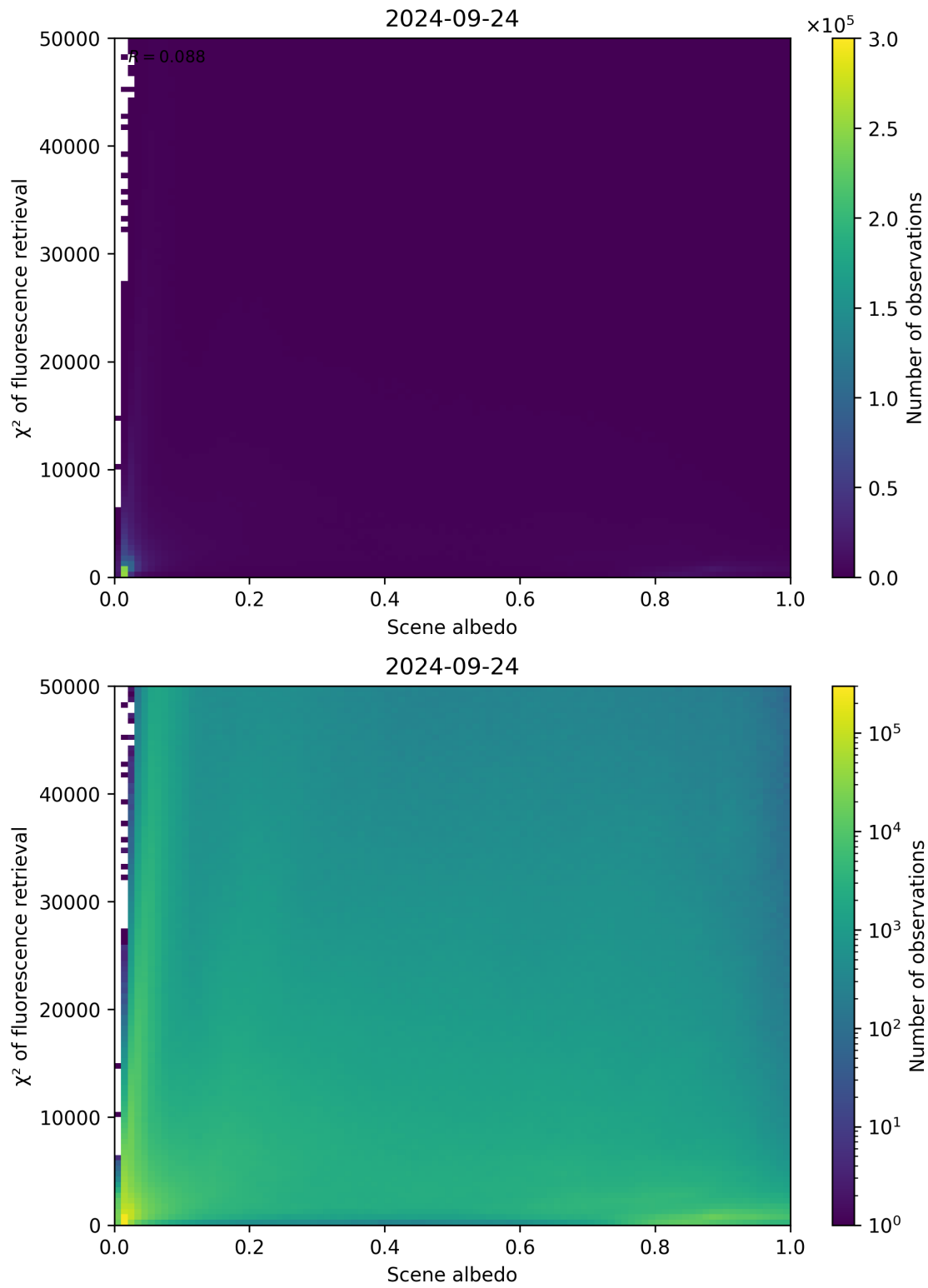
Figure 113: Scatter density plot of “Scene albedo” against “ \chi^2 of fluorescence retrieval” for 2024-09-23 to 2024-09-25.
