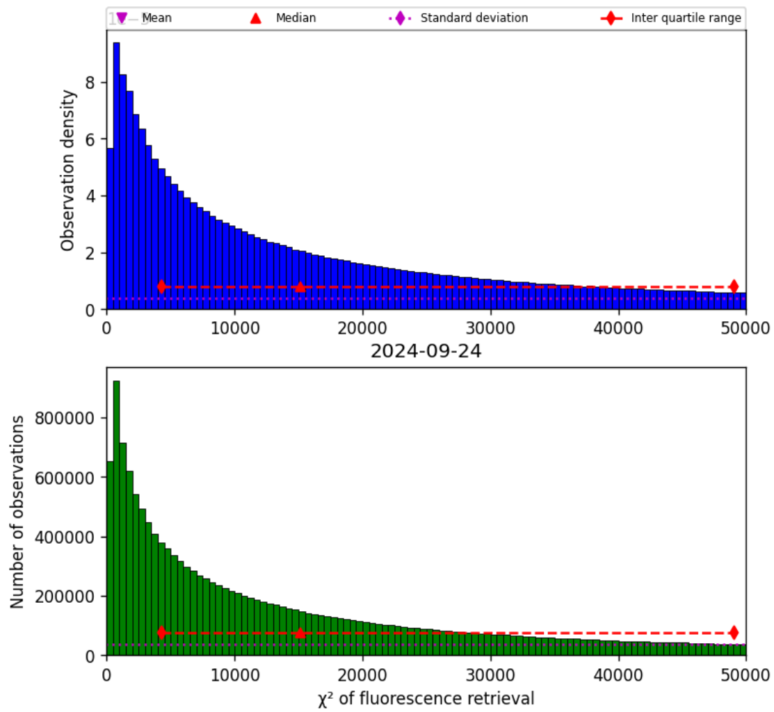
Figure 42: Histogram of “ \chi^2 of fluorescence retrieval” for 2024-09-23 to 2024-09-25
