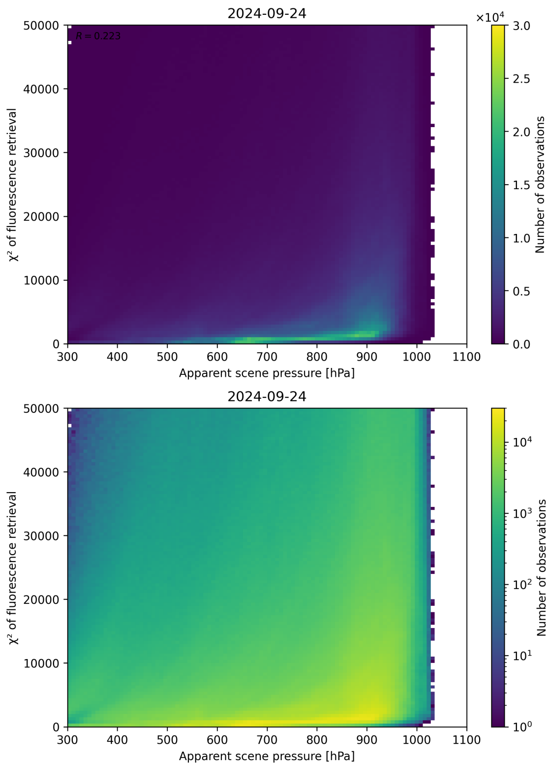
Figure 64: Scatter density plot of “Apparent scene pressure” against “ \chi^2 of fluorescence retrieval” for 2024-09-23 to 2024-09-25.
