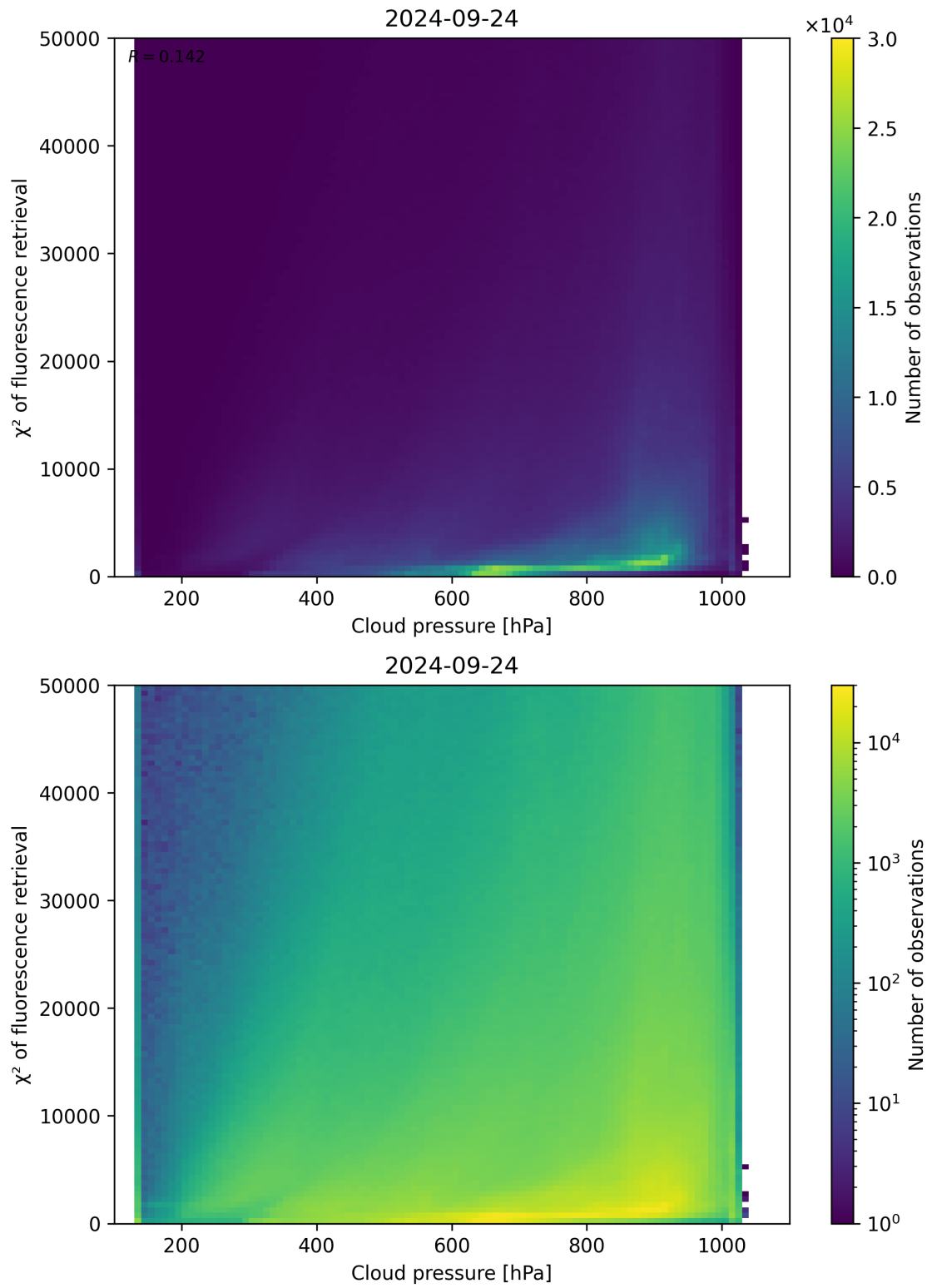
Figure 86: Scatter density plot of “Cloud pressure” against “ \chi^2 of fluorescence retrieval” for 2024-09-23 to 2024-09-25.
