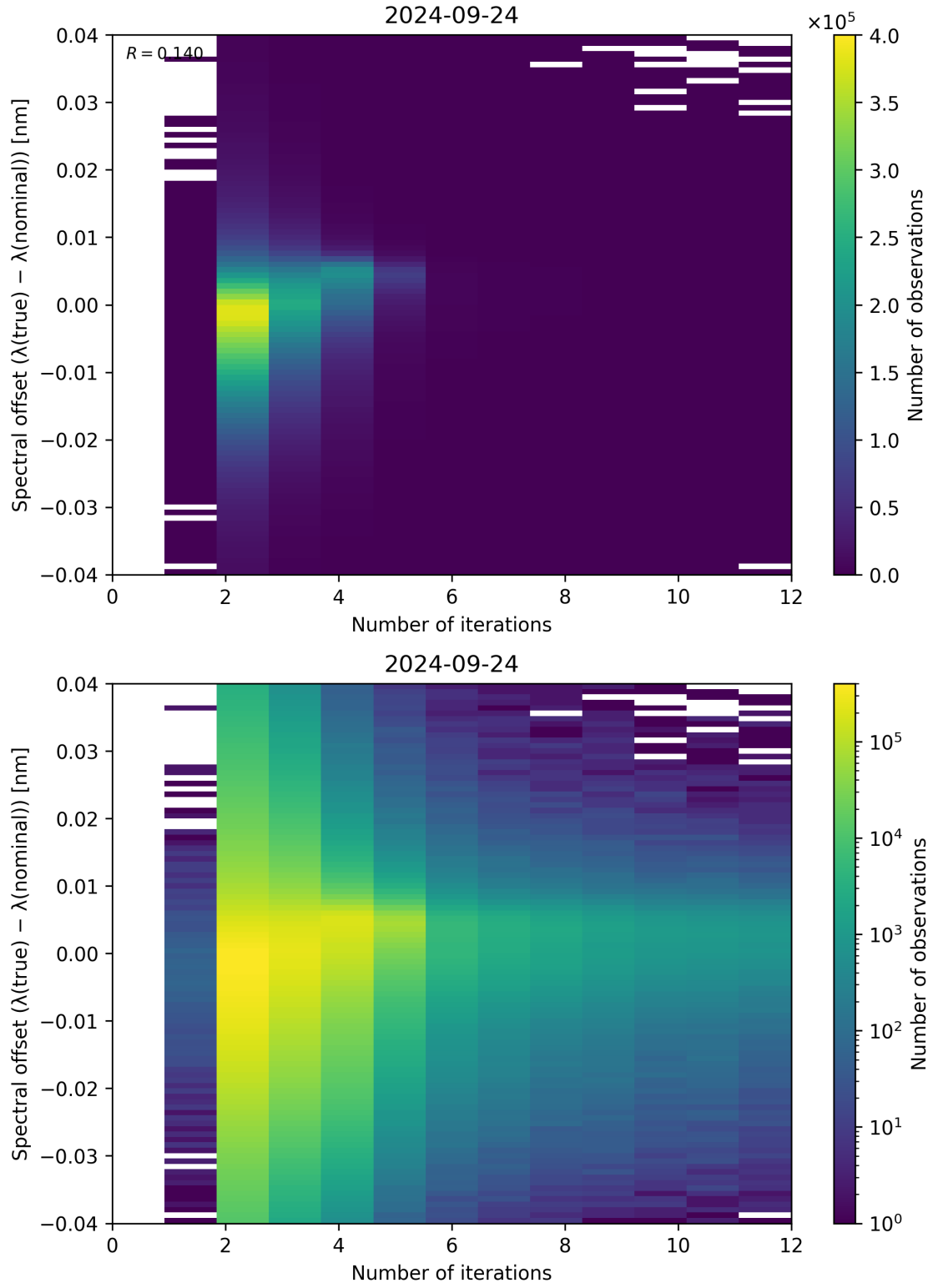
Figure 109: Scatter density plot of “Number of iterations” against “Spectral offset ( \lambda_{\text{true}} - \lambda_{\text{nominal}} )” for 2024-09-23 to 2024-09-25.
