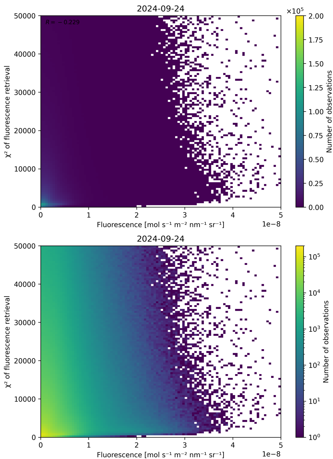
Figure 93: Scatter density plot of “Fluorescence” against “ \chi^2 of fluorescence retrieval” for 2024-09-23 to 2024-09-25.
