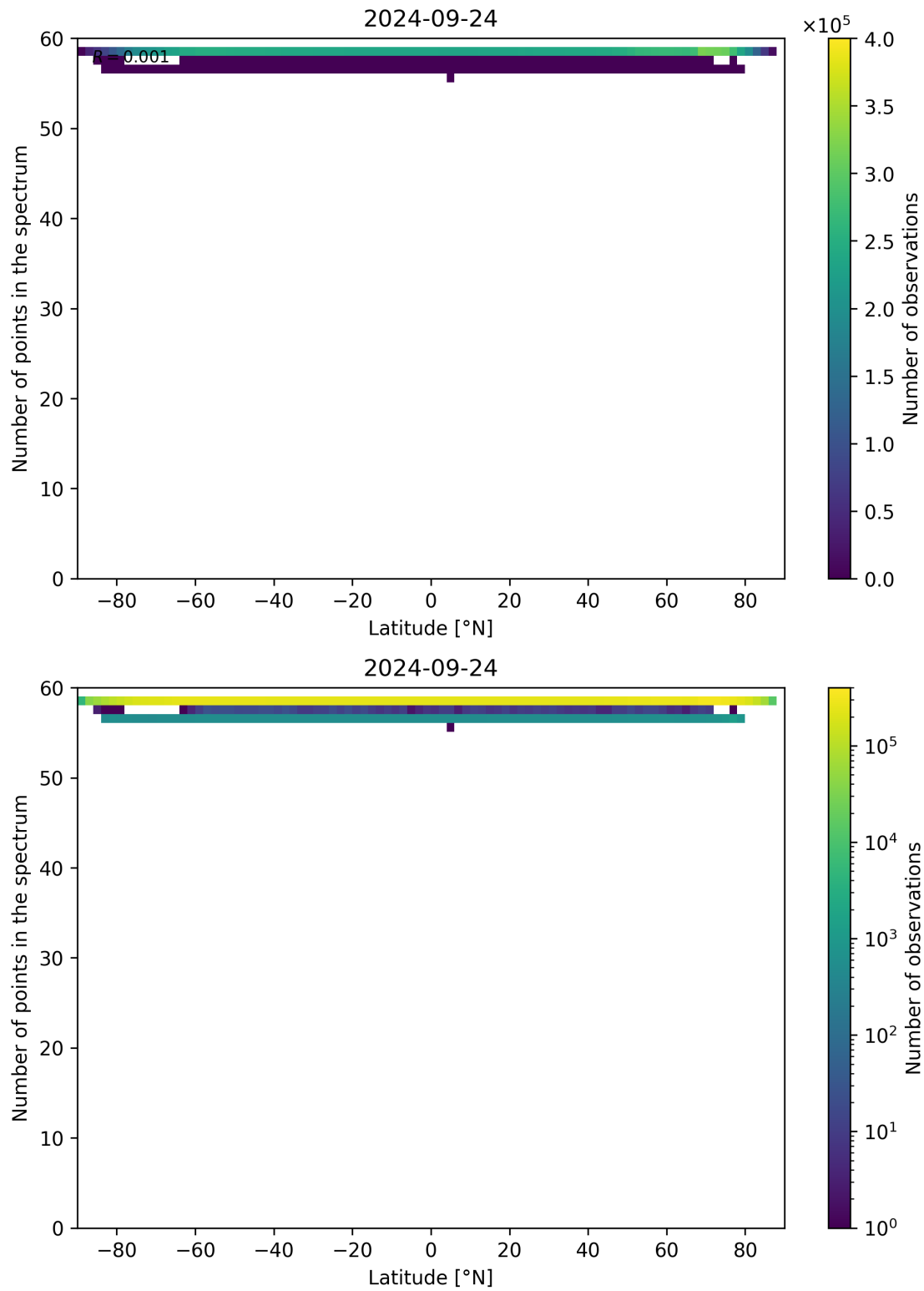
Figure 103: Scatter density plot of “Latitude” against “Number of points in the spectrum” for 2024-09-23 to 2024-09-25.
