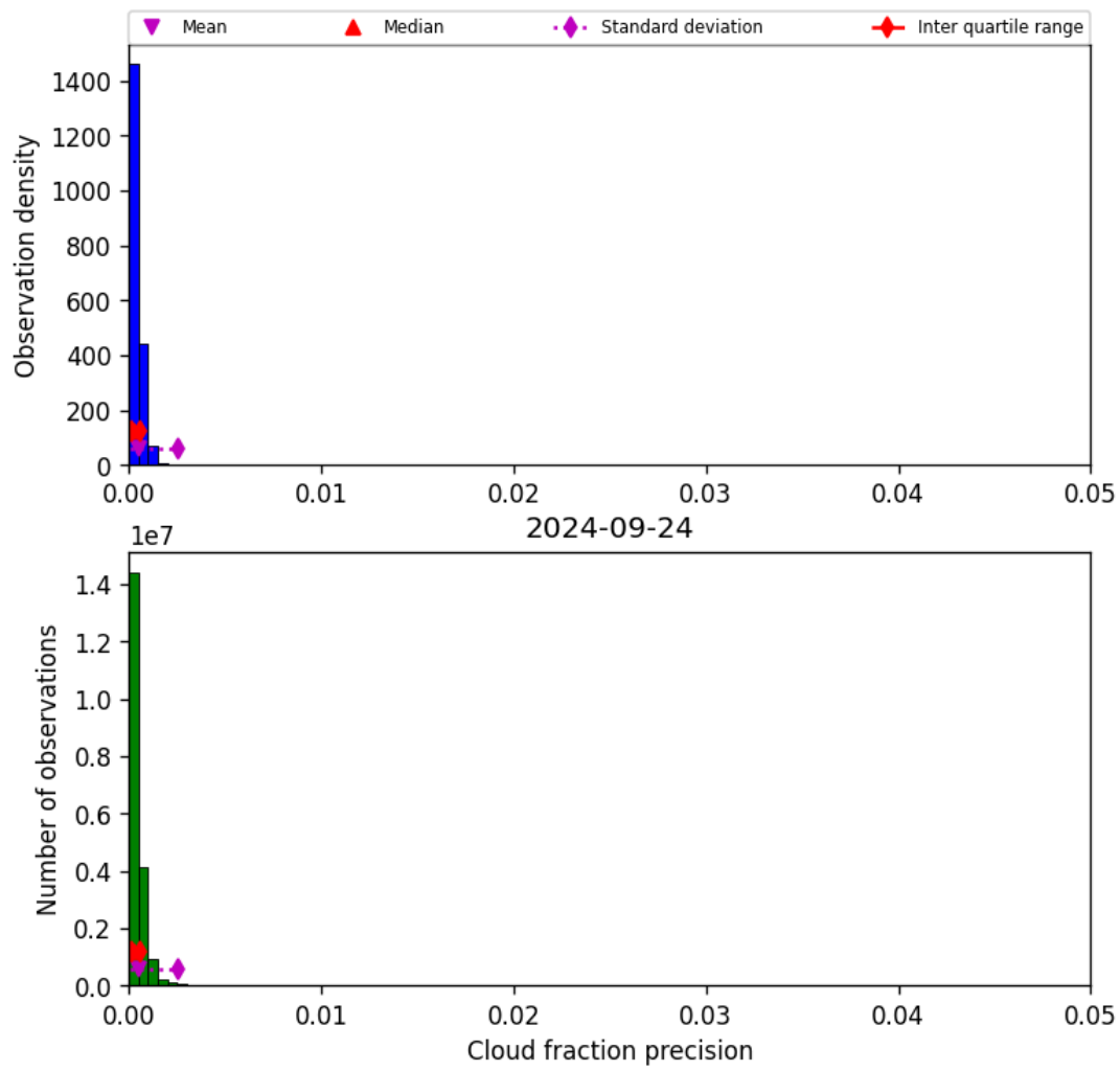
Figure 33: Histogram of “Cloud fraction precision” for 2024-09-23 to 2024-09-25
