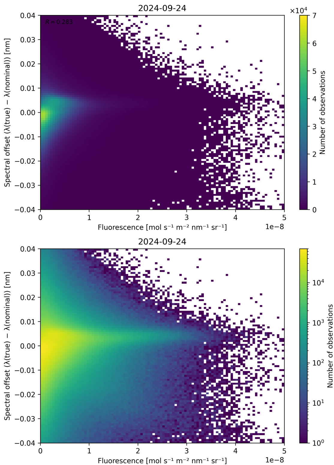
Figure 95: Scatter density plot of “Fluorescence” against “Spectral offset ( \lambda_{\text{true}} - \lambda_{\text{nominal}} )” for 2024-09-23 to 2024-09-25.
