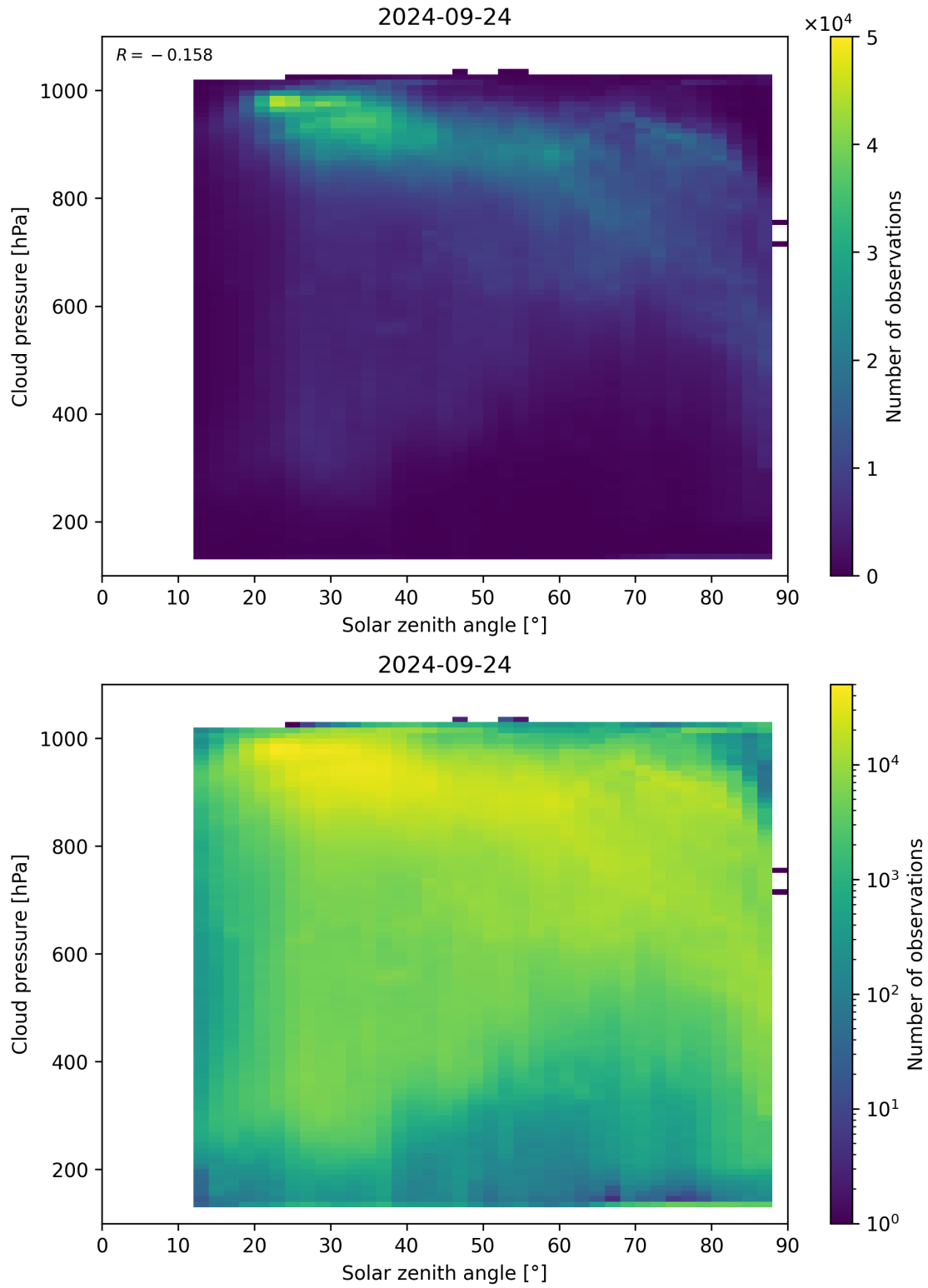
Figure 122: Scatter density plot of “Solar zenith angle” against “Cloud pressure” for 2024-09-23 to 2024-09-25.
