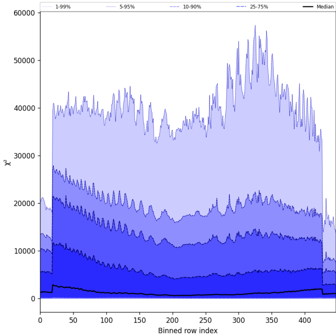
Figure 55: Along track statistics of “ \chi^2 ” for 2024-09-23 to 2024-09-25
