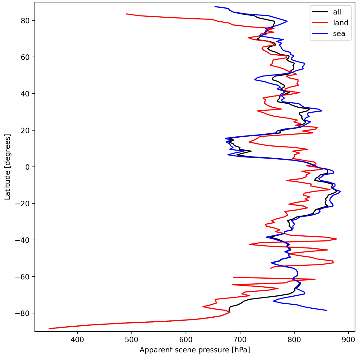
Figure 19: Zonal average of “Apparent scene pressure” for 2024-09-23 to 2024-09-25.
