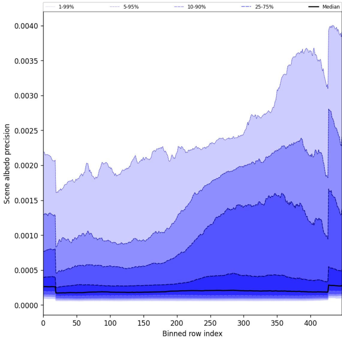
Figure 52: Along track statistics of “Scene albedo precision” for 2024-09-23 to 2024-09-25
