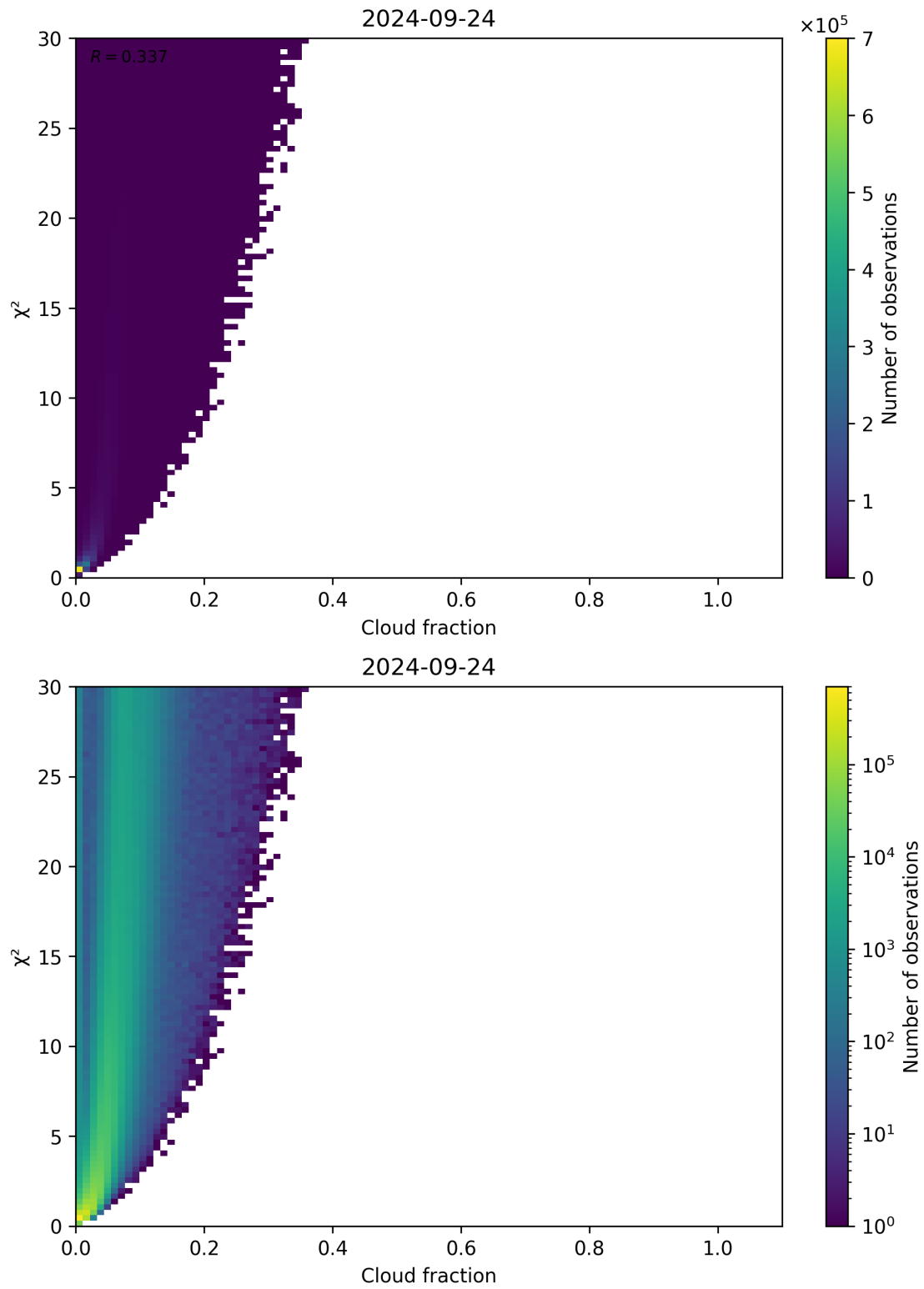
Figure 77: Scatter density plot of “Cloud fraction” against “ \chi^2 ” for 2024-09-23 to 2024-09-25.
