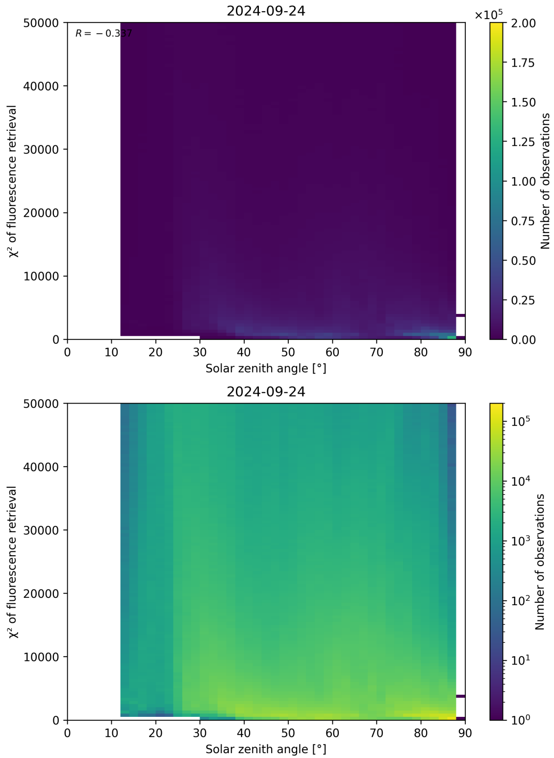
Figure 120: Scatter density plot of “Solar zenith angle” against “ \chi^2 of fluorescence retrieval” for 2024-09-23 to 2024-09-25.
