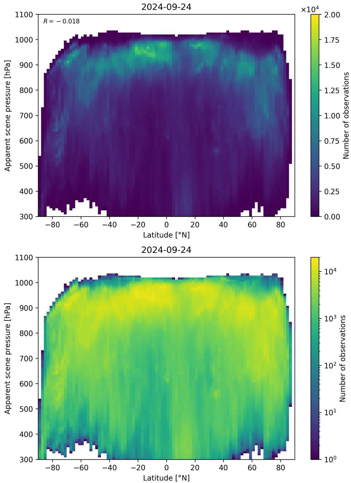
Figure 96: Scatter density plot of “Latitude” against “Apparent scene pressure” for 2024-09-23 to 2024-09-25.
