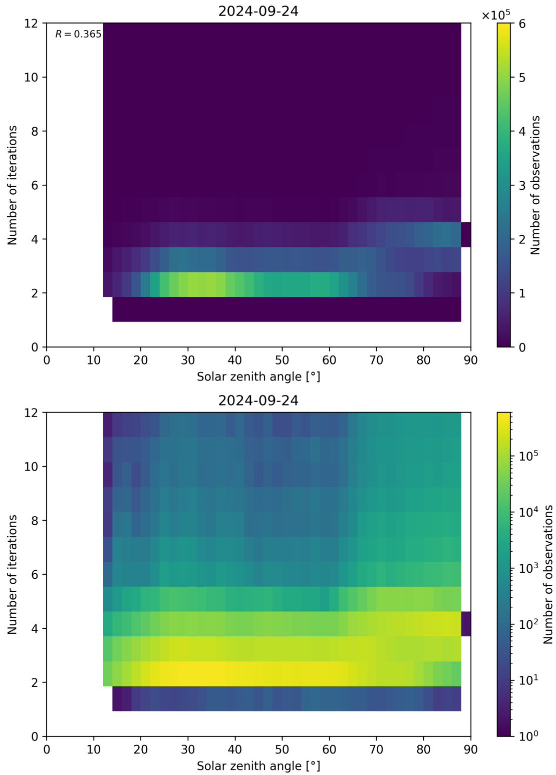
Figure 125: Scatter density plot of “Solar zenith angle” against “Number of iterations” for 2024-09-23 to 2024-09-25.
