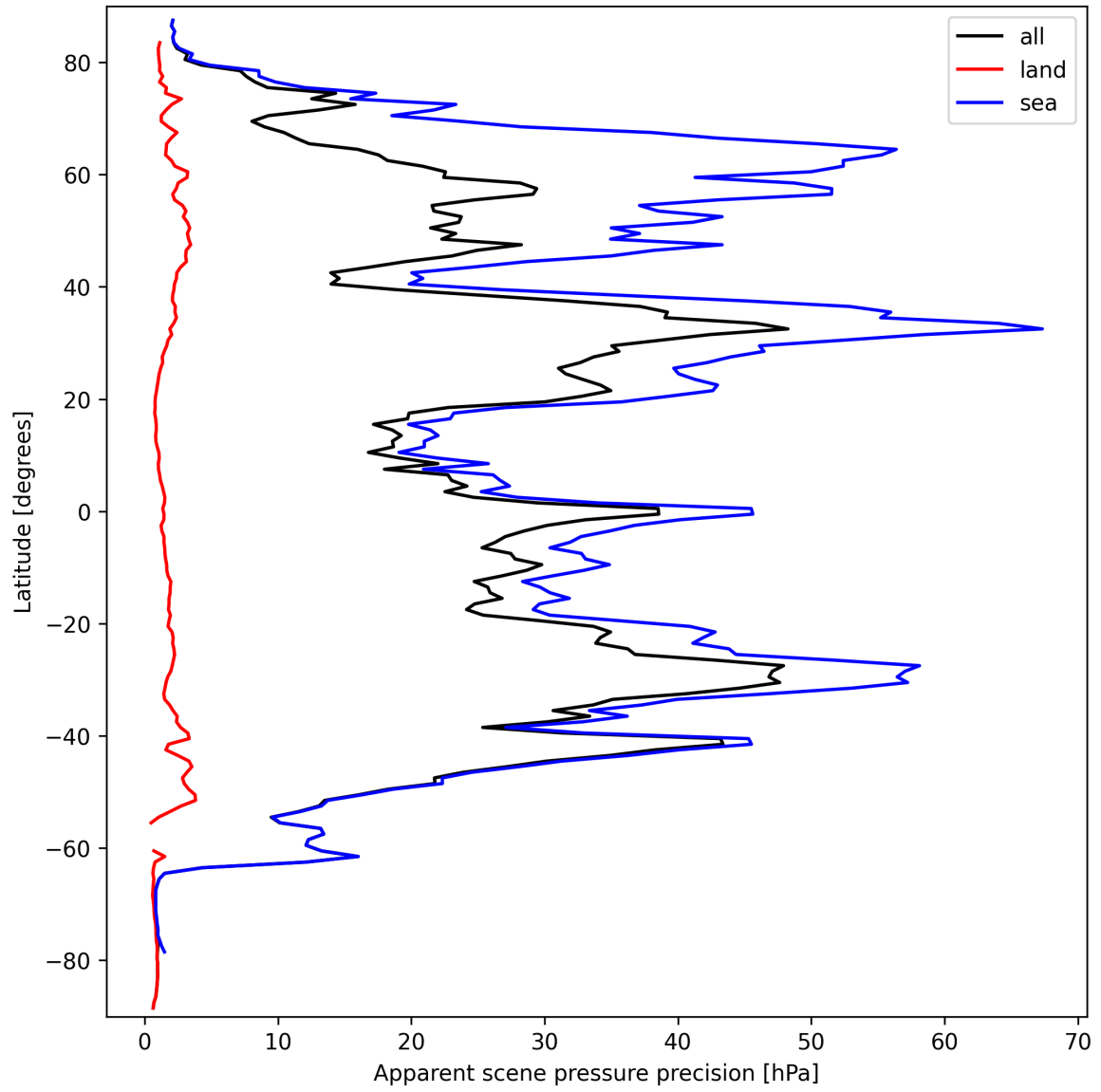
Figure 20: Zonal average of “Apparent scene pressure precision” for 2024-09-23 to 2024-09-25.
