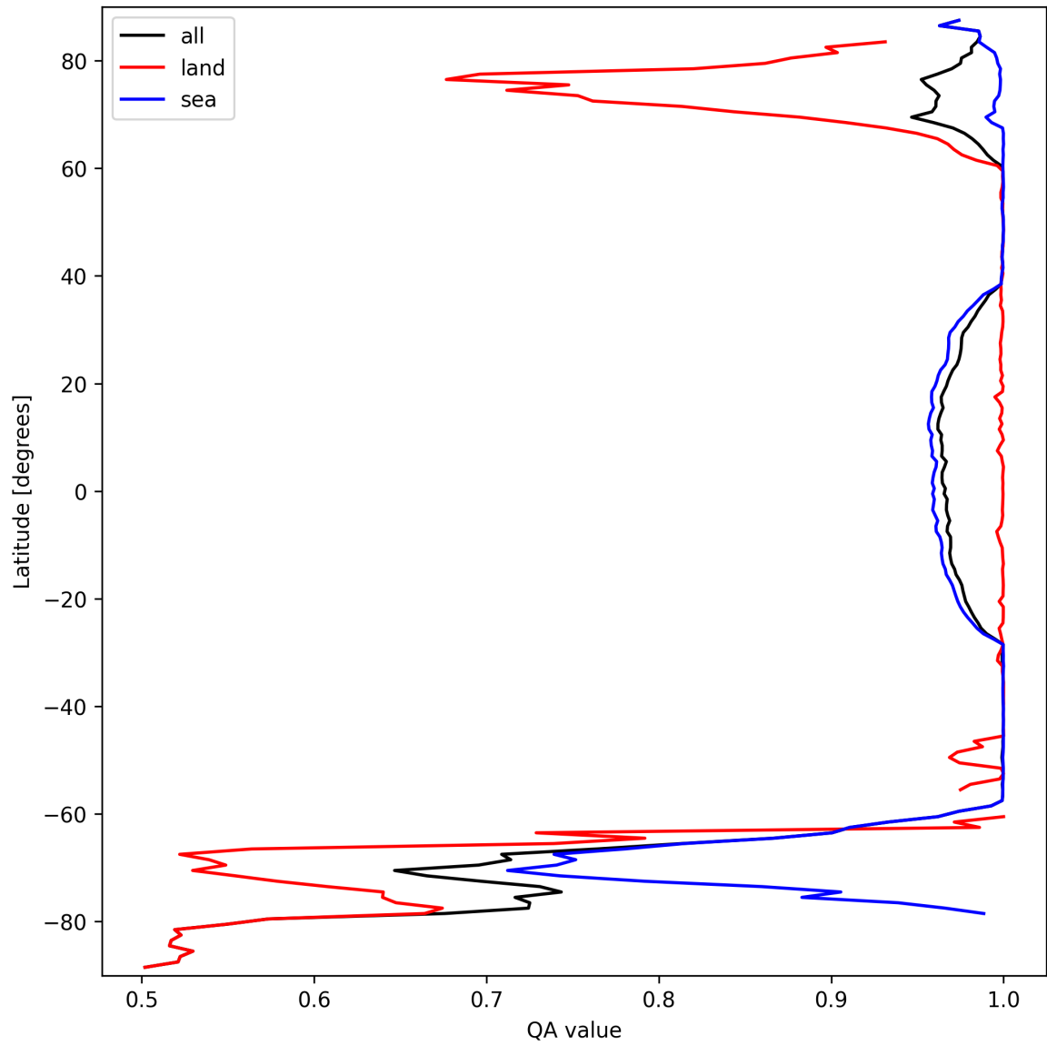
Figure 12: Zonal average of “QA value” for 2024-09-23 to 2024-09-25.
