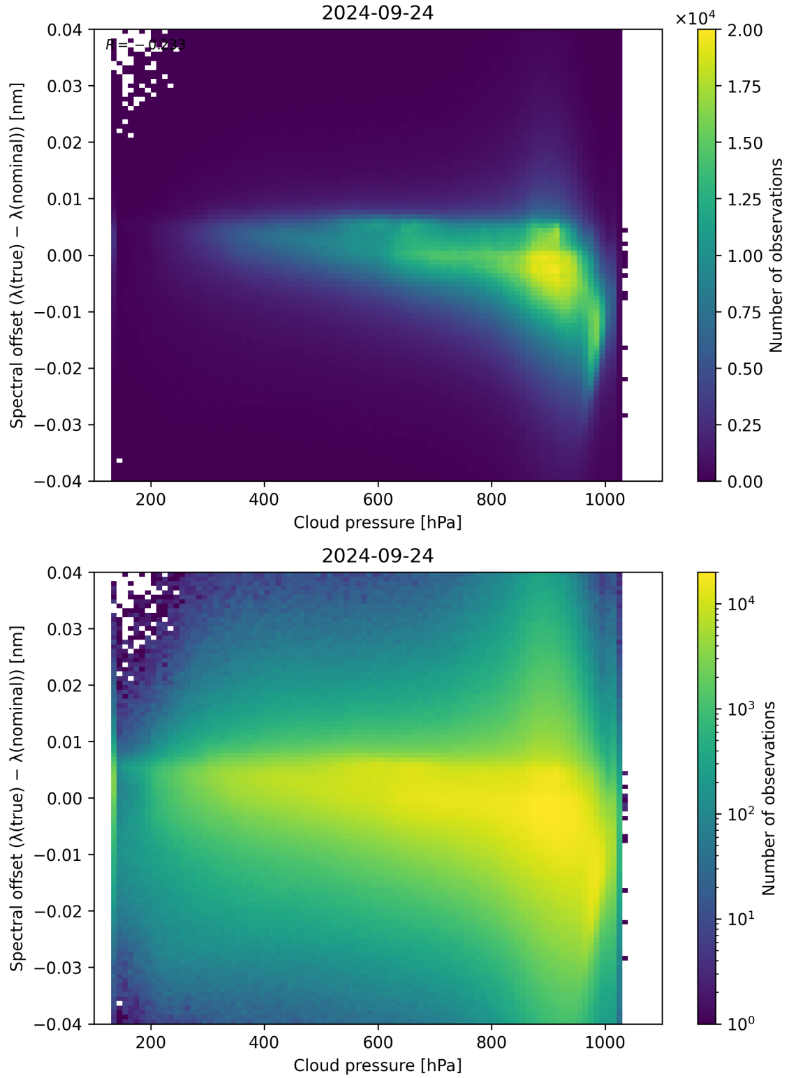
Figure 92: Scatter density plot of “Cloud pressure” against “Spectral offset ( \lambda_{\text{true}} - \lambda_{\text{nominal}} )” for 2024-09-23 to 2024-09-25.
