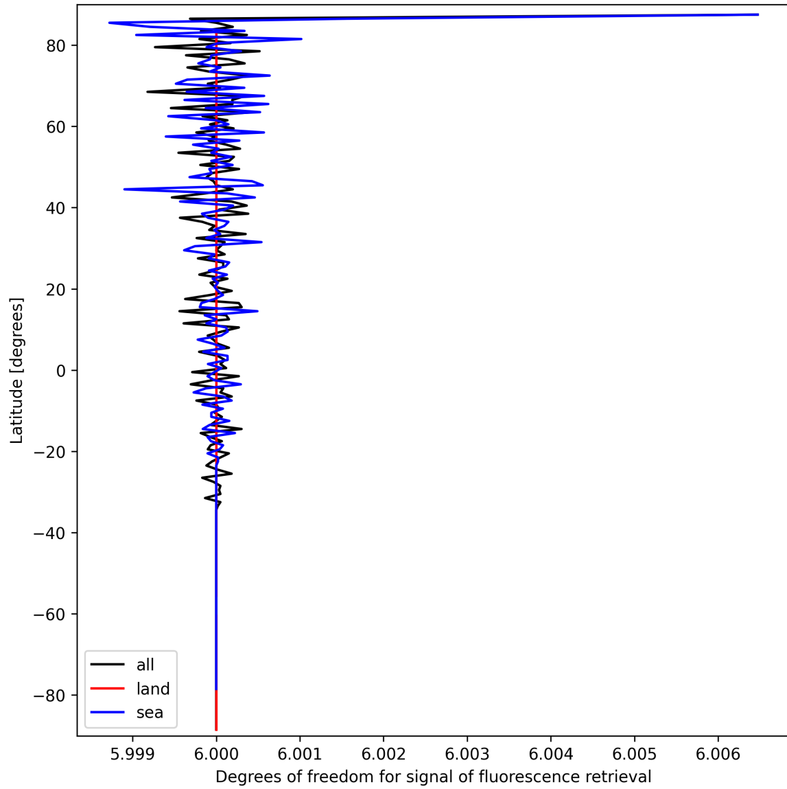
Figure 26: Zonal average of “Degrees of freedom for signal of fluorescence retrieval” for 2024-09-23 to 2024-09-25.
