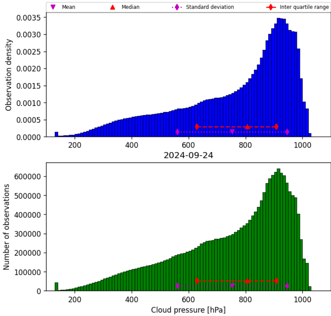
Figure 30: Histogram of “Cloud pressure” for 2024-09-23 to 2024-09-25
