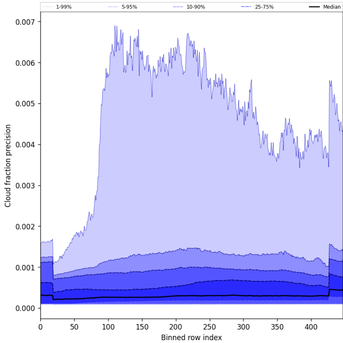
Figure 50: Along track statistics of “Cloud fraction precision” for 2024-09-23 to 2024-09-25
