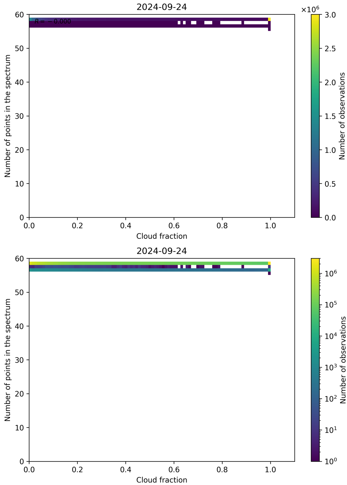
Figure 81: Scatter density plot of “Cloud fraction” against “Number of points in the spectrum” for 2024-09-23 to 2024-09-25.
