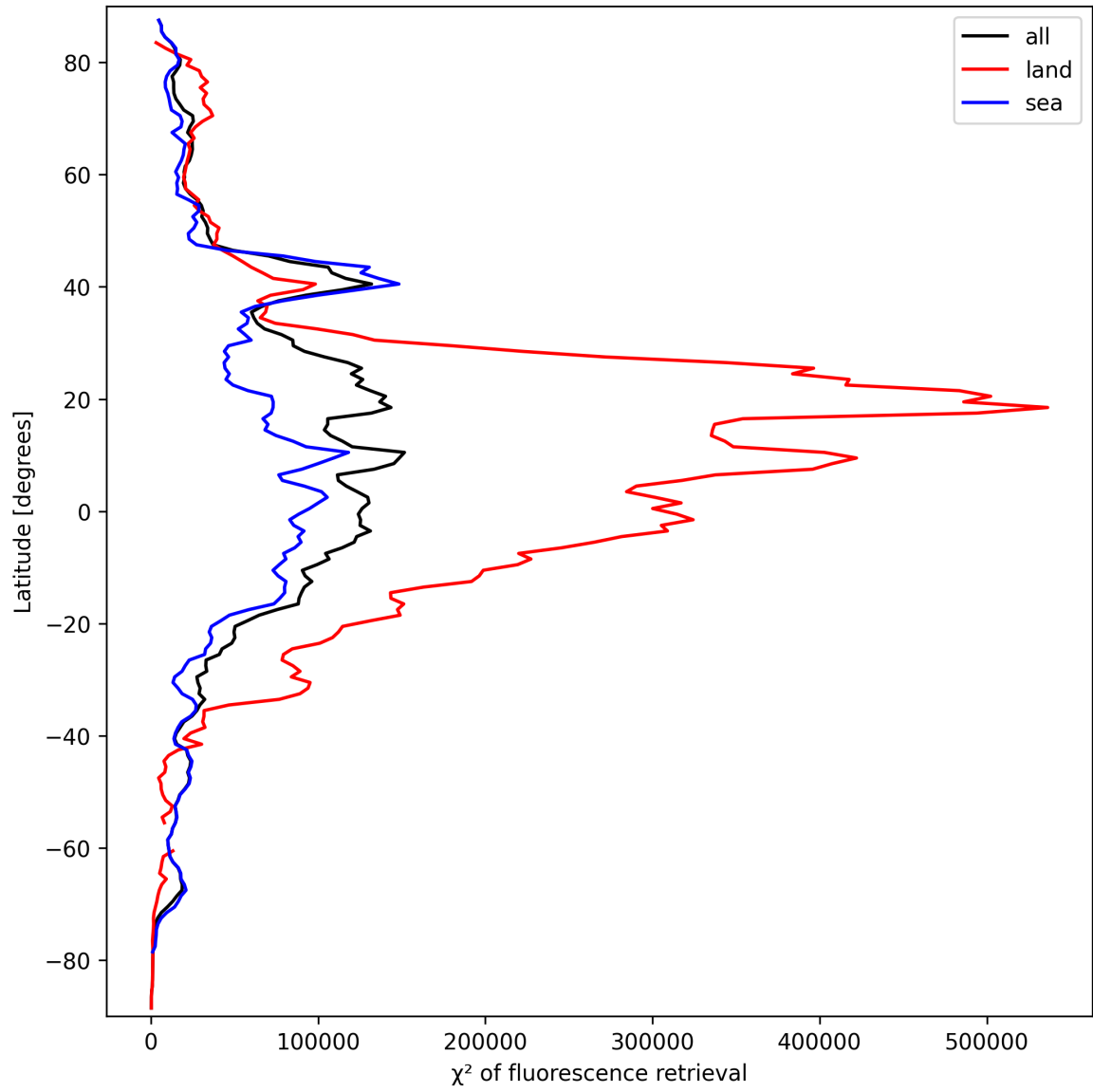
Figure 25: Zonal average of “ \chi^2 of fluorescence retrieval” for 2024-09-23 to 2024-09-25.
