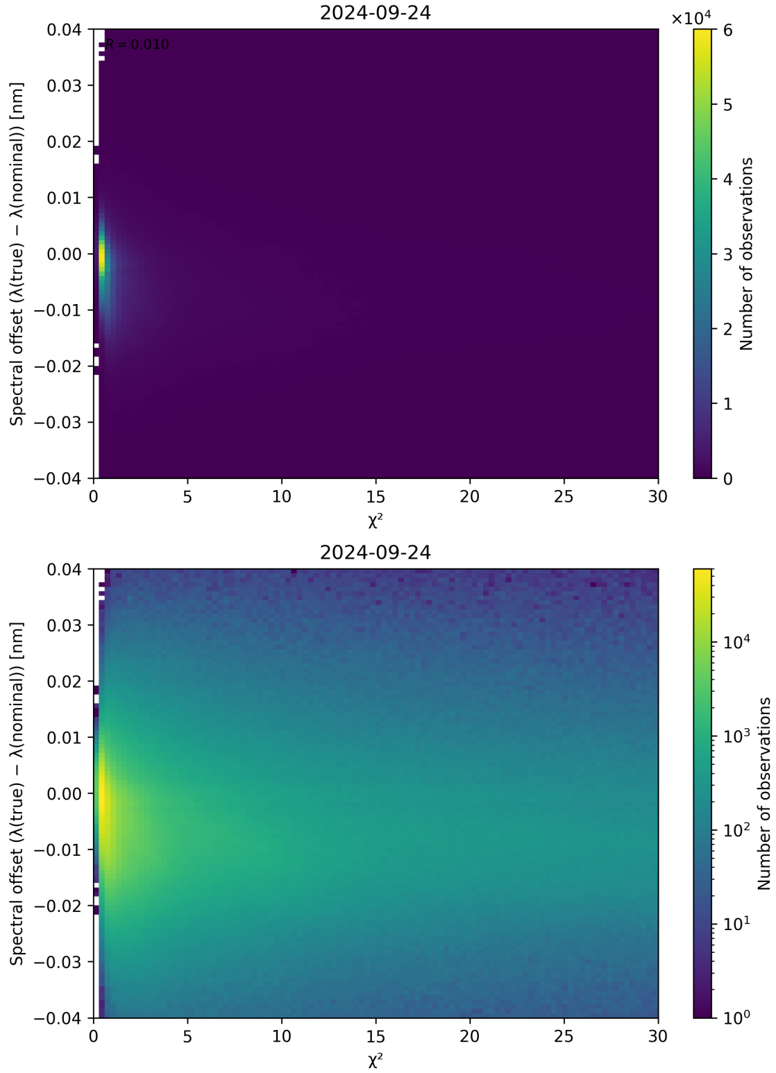
Figure 75: Scatter density plot of “ \chi^2 ” against “Spectral offset ( \lambda_{\text{true}} - \lambda_{\text{nominal}} )” for 2024-09-23 to 2024-09-25.
