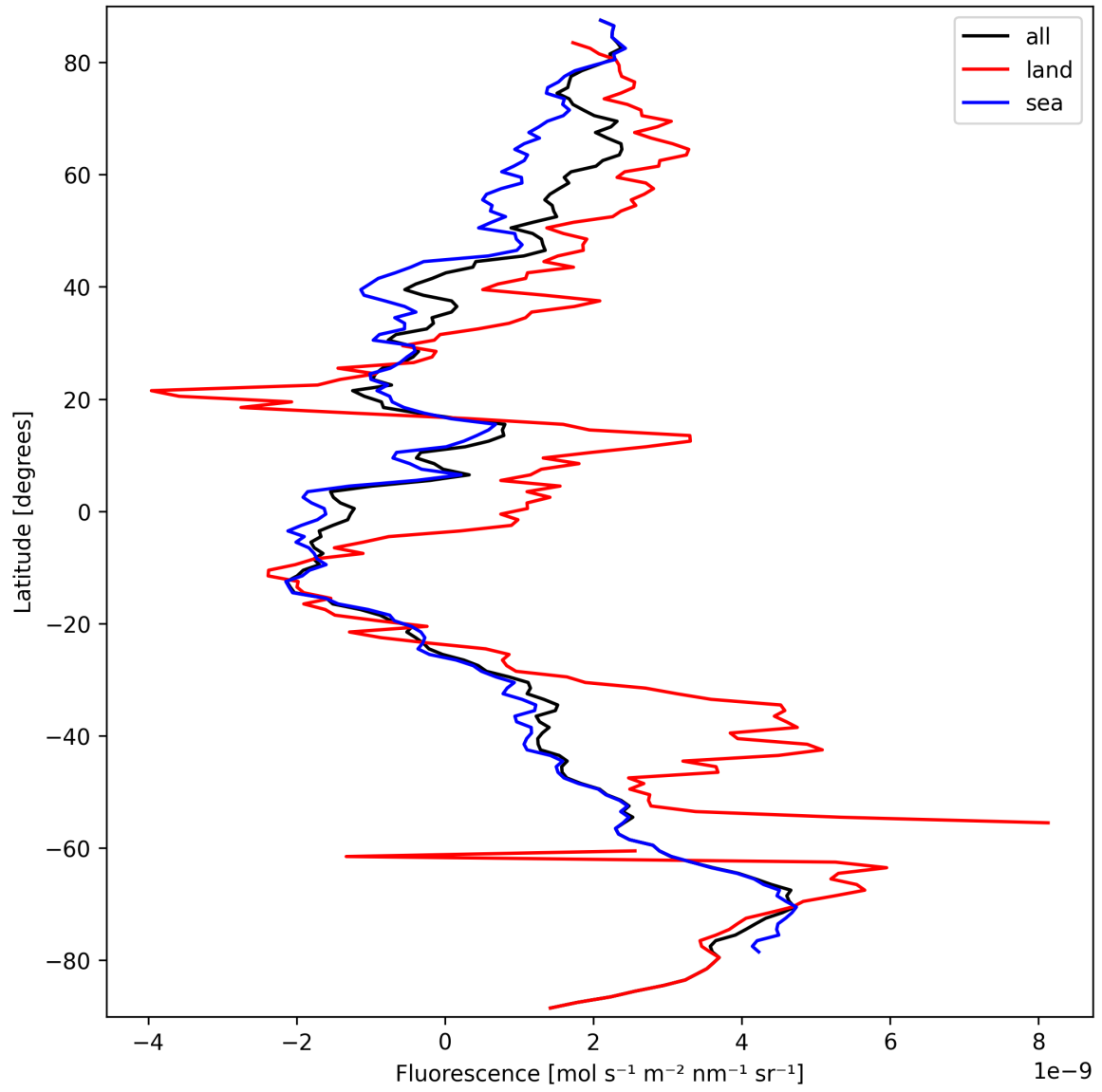
Figure 23: Zonal average of “Fluorescence” for 2024-09-23 to 2024-09-25.
