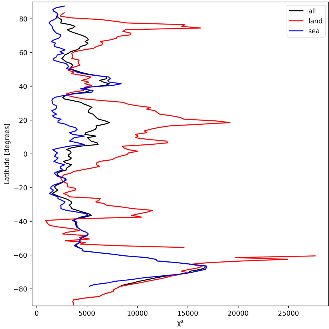
Figure 21: Zonal average of “ \chi^2 ” for 2024-09-24 to 2024-09-26.
