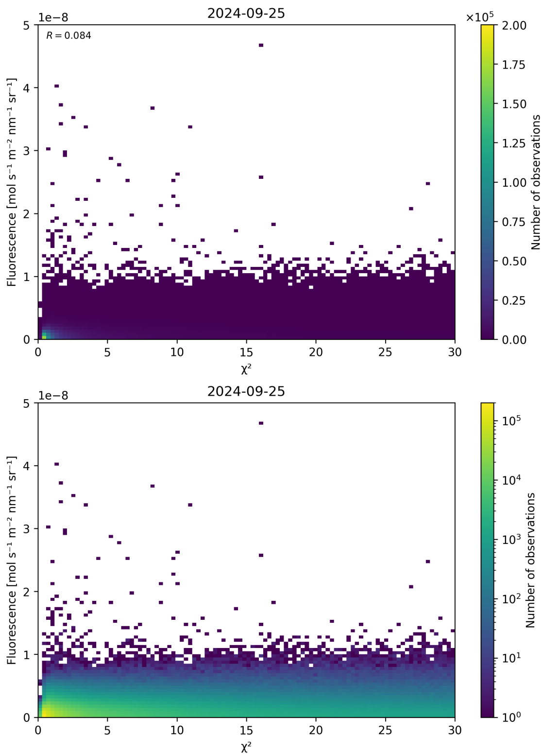
Figure 70: Scatter density plot of “ \chi^2 ” against “Fluorescence” for 2024-09-24 to 2024-09-26.
