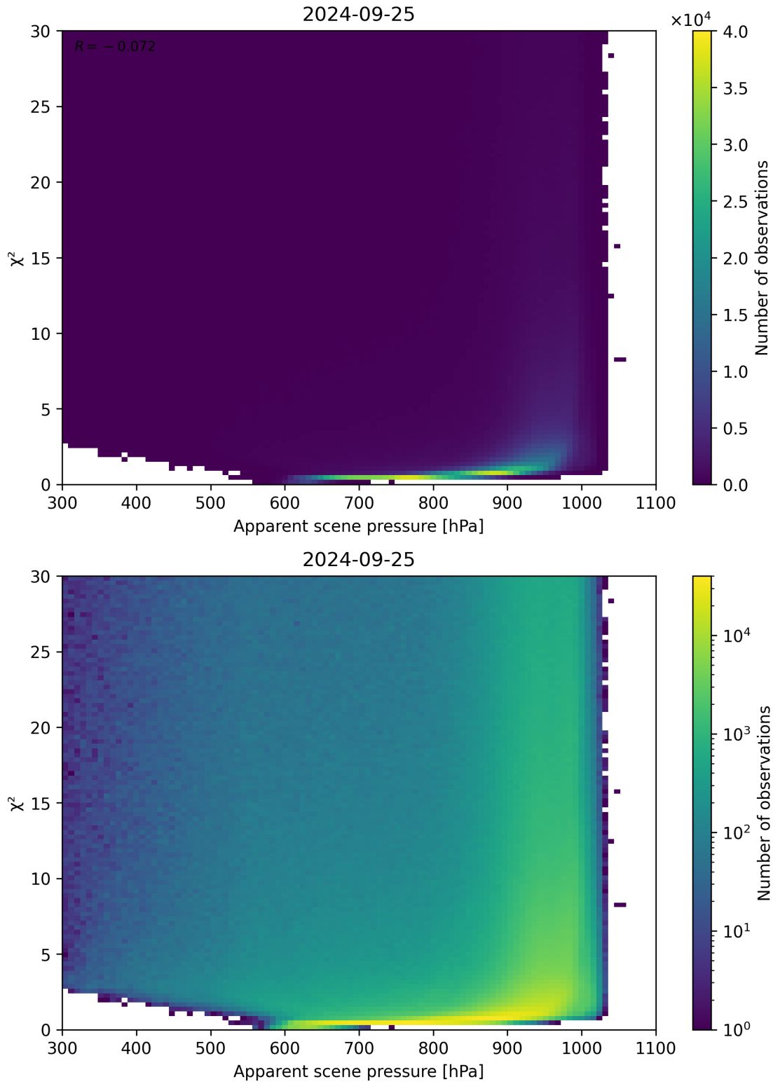
Figure 63: Scatter density plot of “Apparent scene pressure” against “ \chi^2 ” for 2024-09-24 to 2024-09-26.
