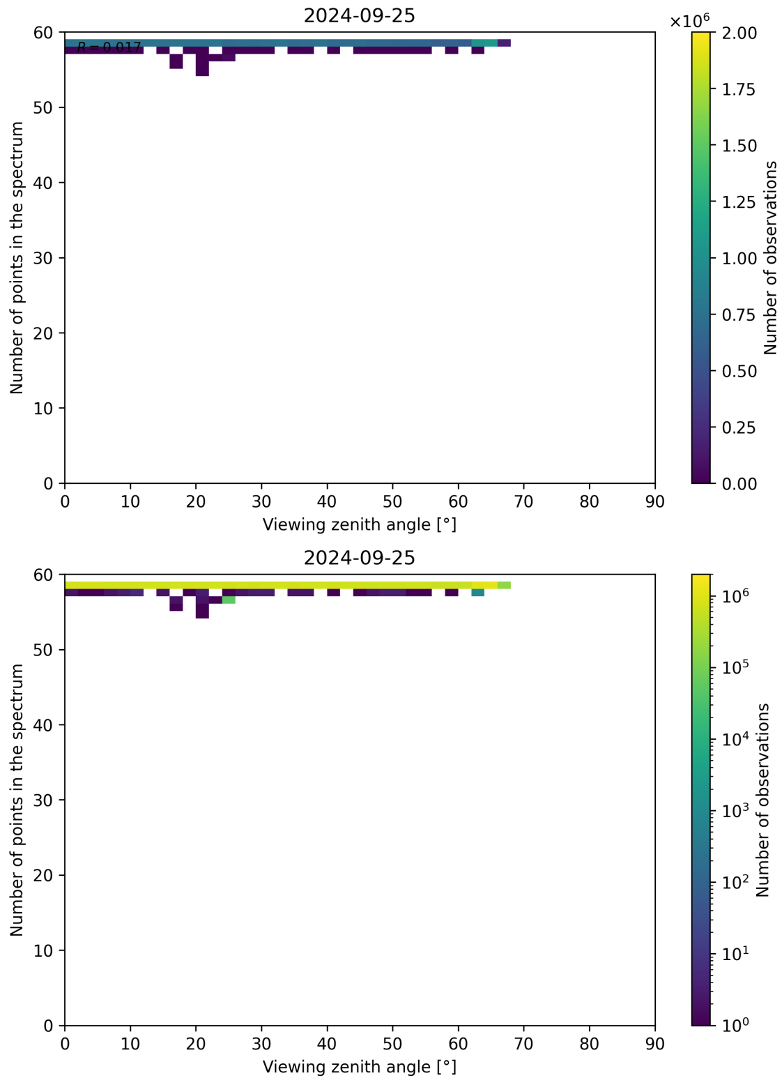
Figure 137: Scatter density plot of “Viewing zenith angle” against “Number of points in the spectrum” for 2024-09-24 to 2024-09-26.
