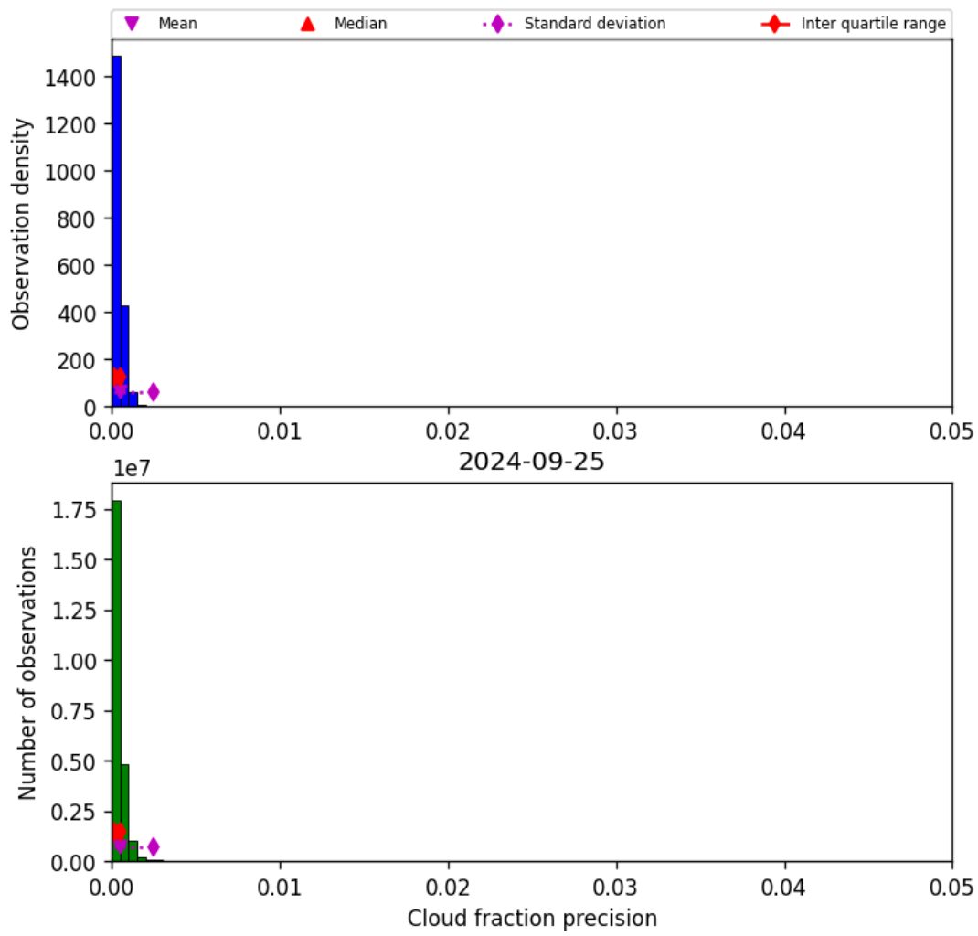
Figure 33: Histogram of “Cloud fraction precision” for 2024-09-24 to 2024-09-26
