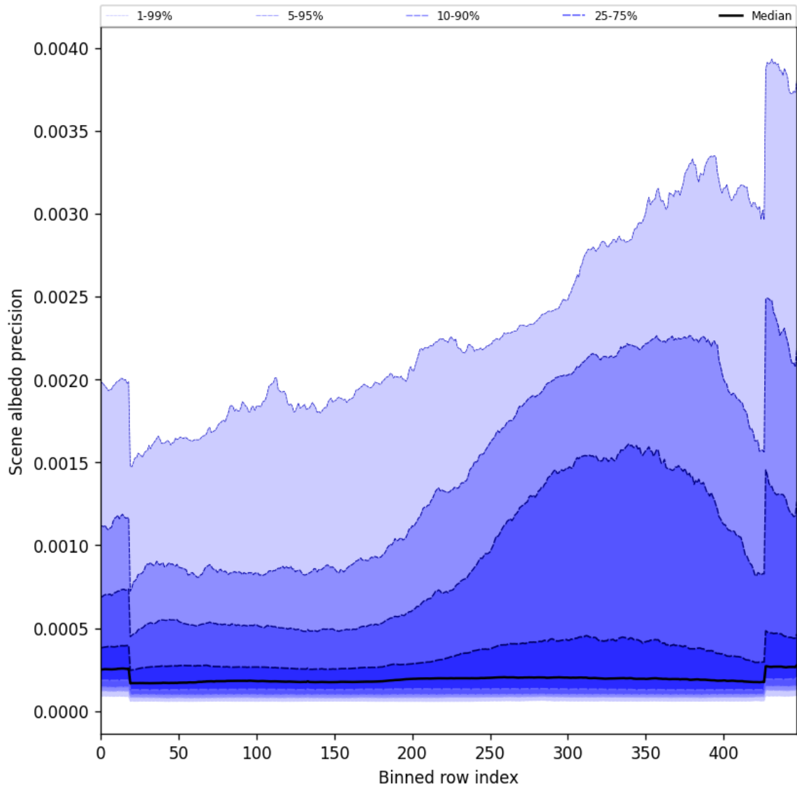
Figure 52: Along track statistics of “Scene albedo precision” for 2024-09-24 to 2024-09-26
