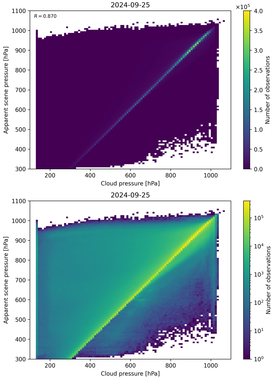
Figure 84: Scatter density plot of “Cloud pressure” against “Apparent scene pressure” for 2024-09-24 to 2024-09-26.
