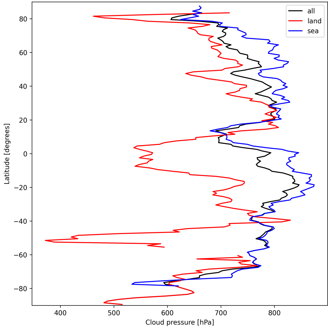
Figure 13: Zonal average of “Cloud pressure” for 2024-09-24 to 2024-09-26.
