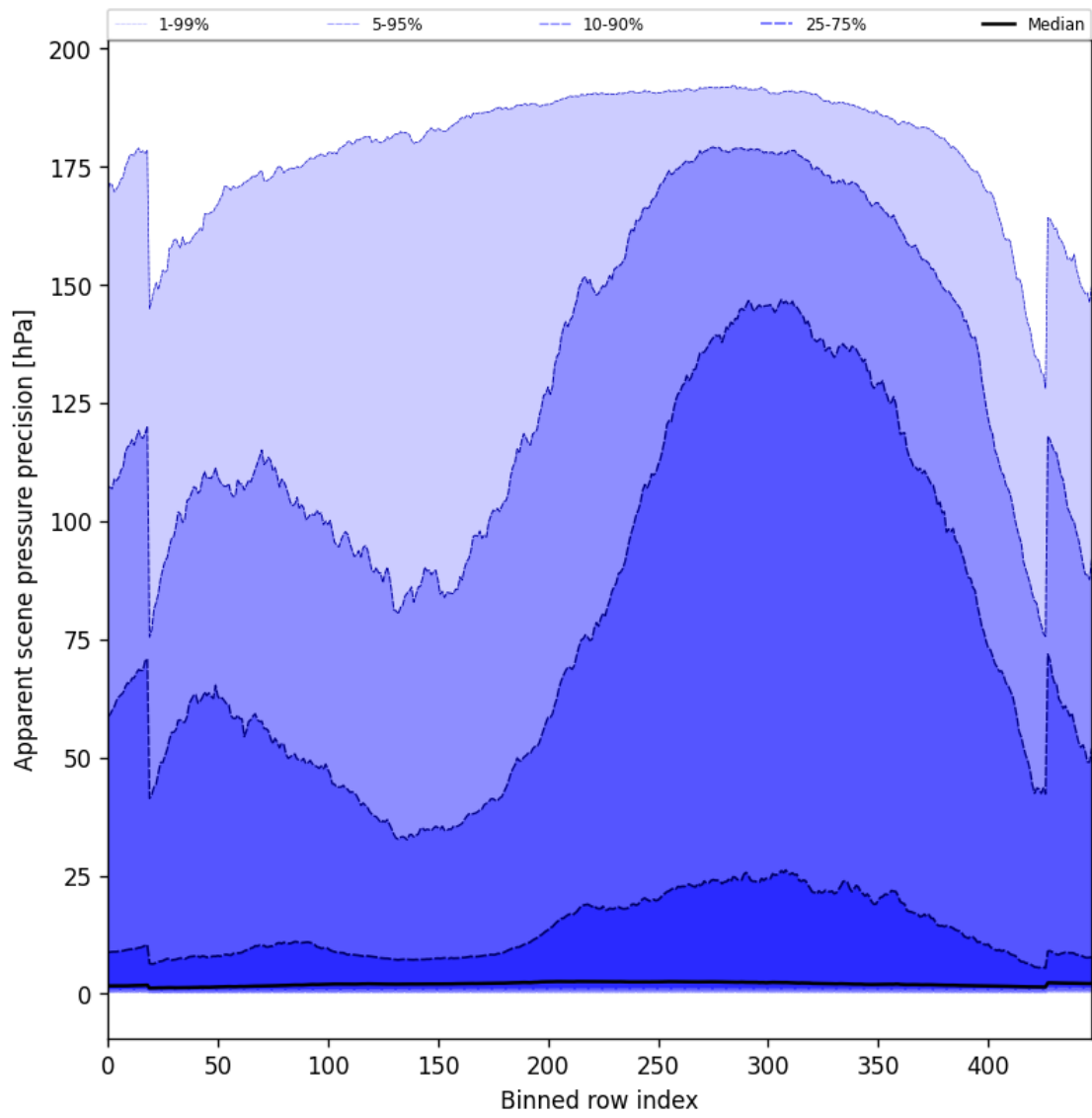
Figure 54: Along track statistics of “Apparent scene pressure precision” for 2024-09-24 to 2024-09-26
