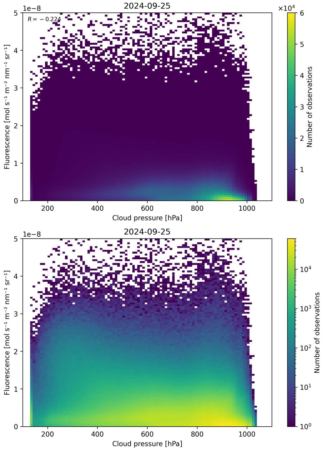
Figure 88: Scatter density plot of “Cloud pressure” against “Fluorescence” for 2024-09-24 to 2024-09-26.
