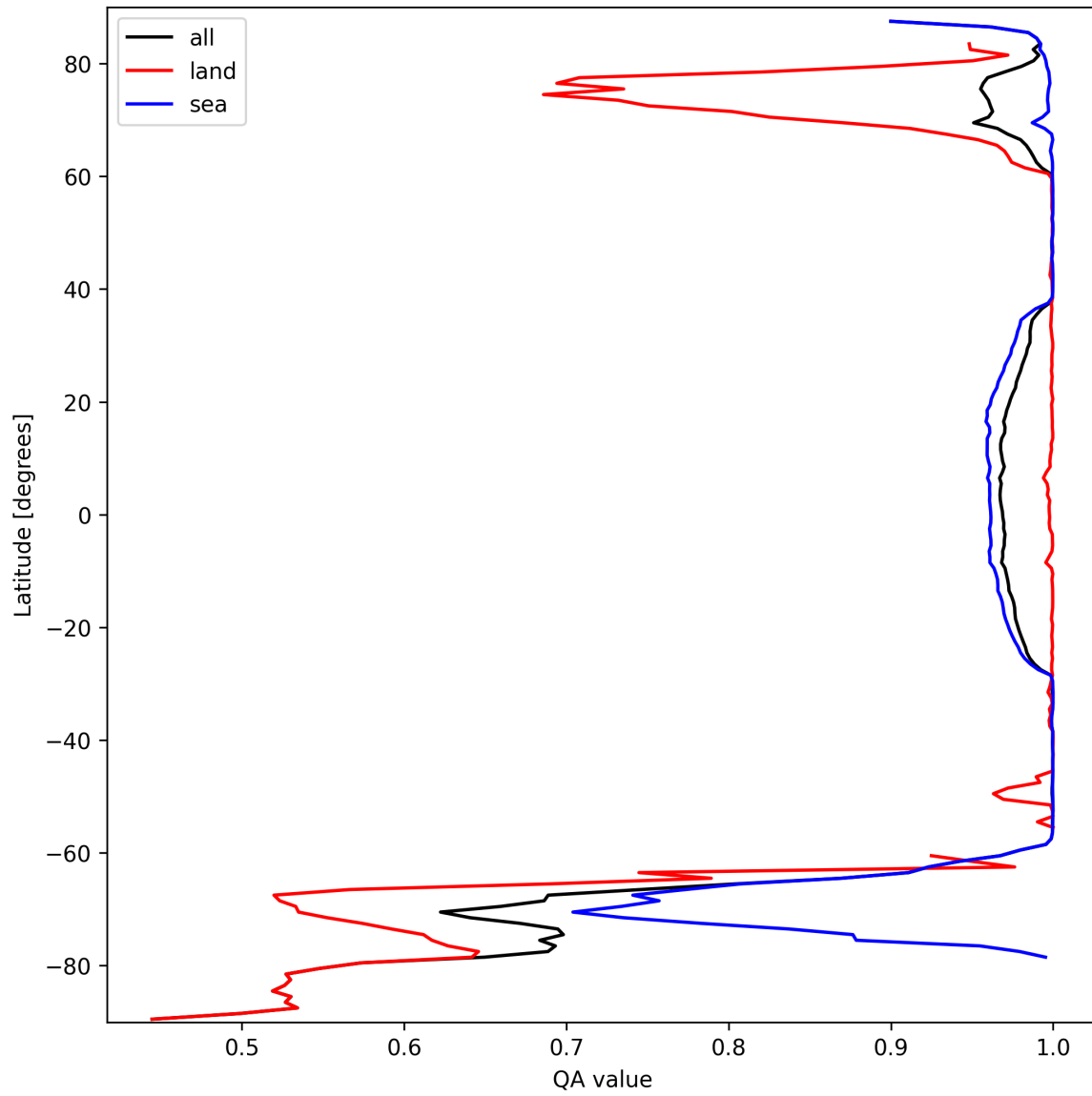
Figure 12: Zonal average of “QA value” for 2024-09-24 to 2024-09-26.
