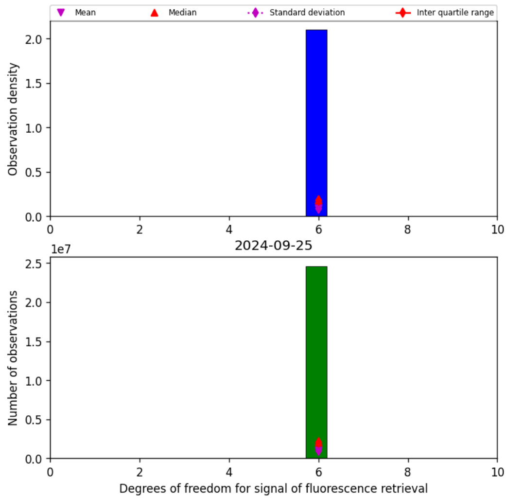
Figure 43: Histogram of "Degrees of freedom for signal of fluorescence retrieval" for 2024-09-24 to 2024-09-26
