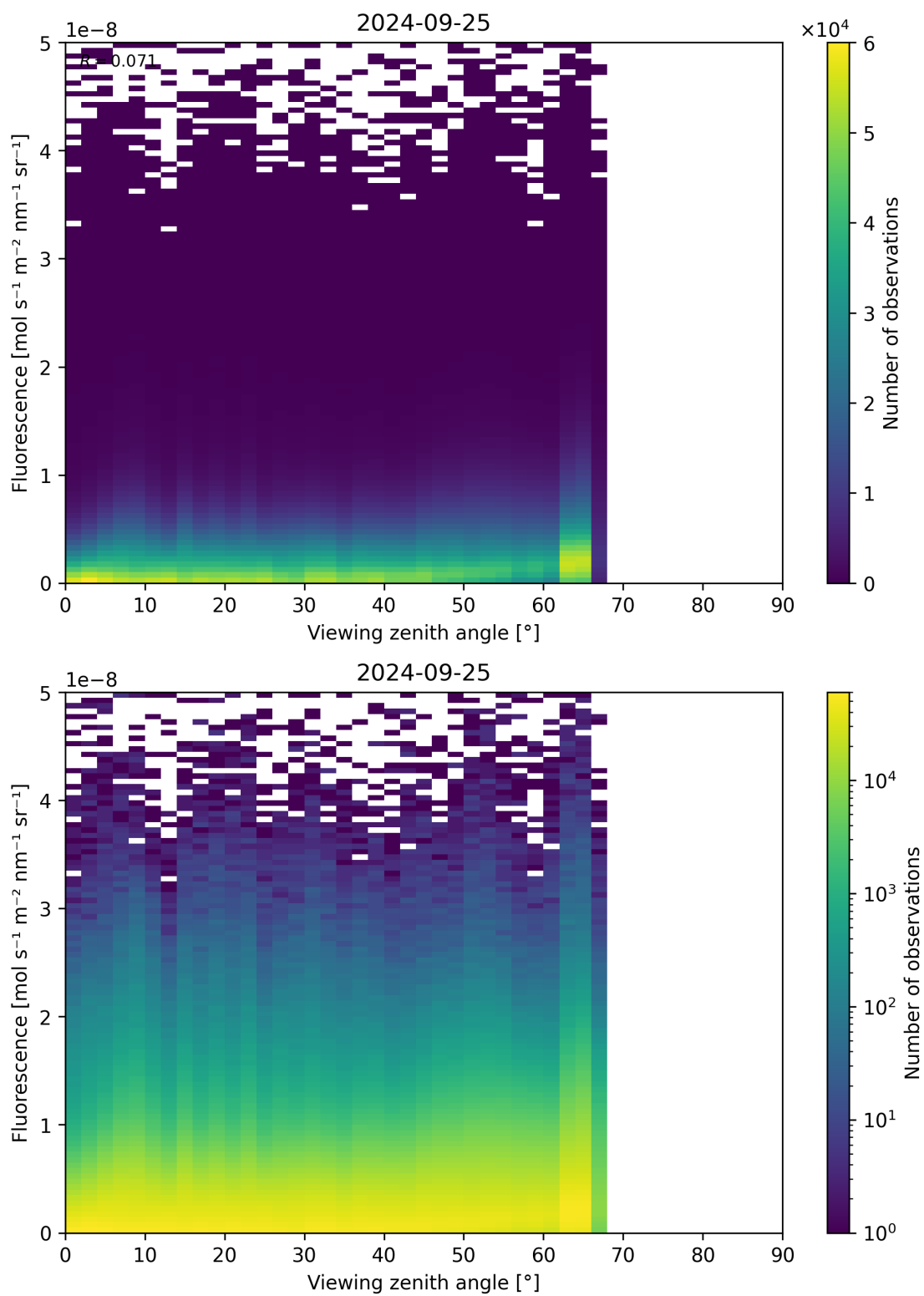
Figure 134: Scatter density plot of “Viewing zenith angle” against “Fluorescence” for 2024-09-24 to 2024-09-26.
