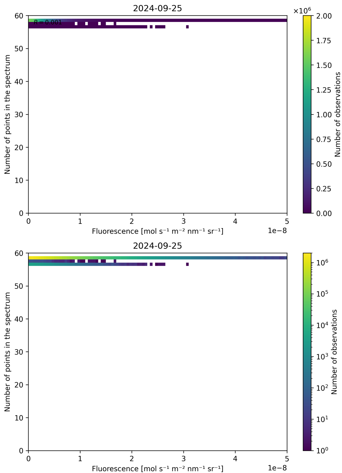
Figure 94: Scatter density plot of “Fluorescence” against “Number of points in the spectrum” for 2024-09-24 to 2024-09-26.
