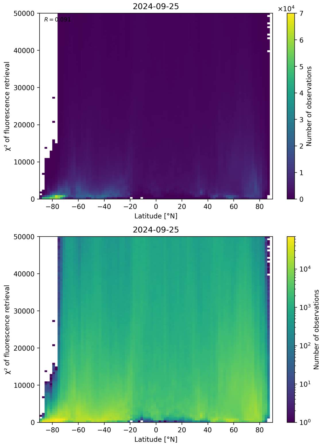
Figure 98: Scatter density plot of “Latitude” against “ \chi^2 of fluorescence retrieval” for 2024-09-24 to 2024-09-26.
