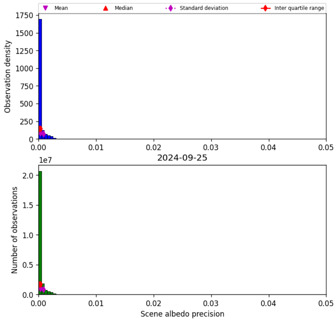
Figure 35: Histogram of “Scene albedo precision” for 2024-09-24 to 2024-09-26
