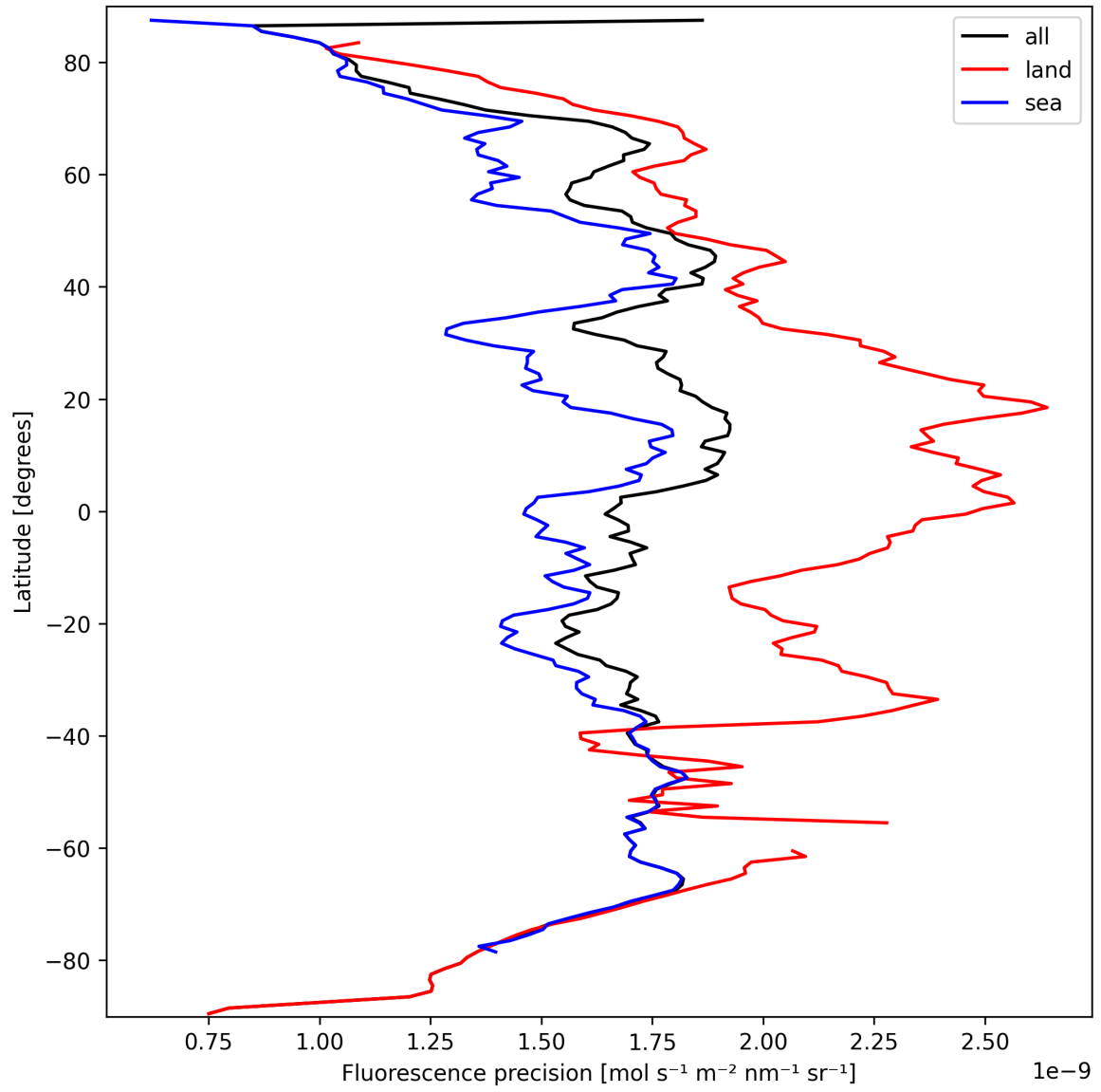
Figure 24: Zonal average of “Fluorescence precision” for 2024-09-24 to 2024-09-26.
