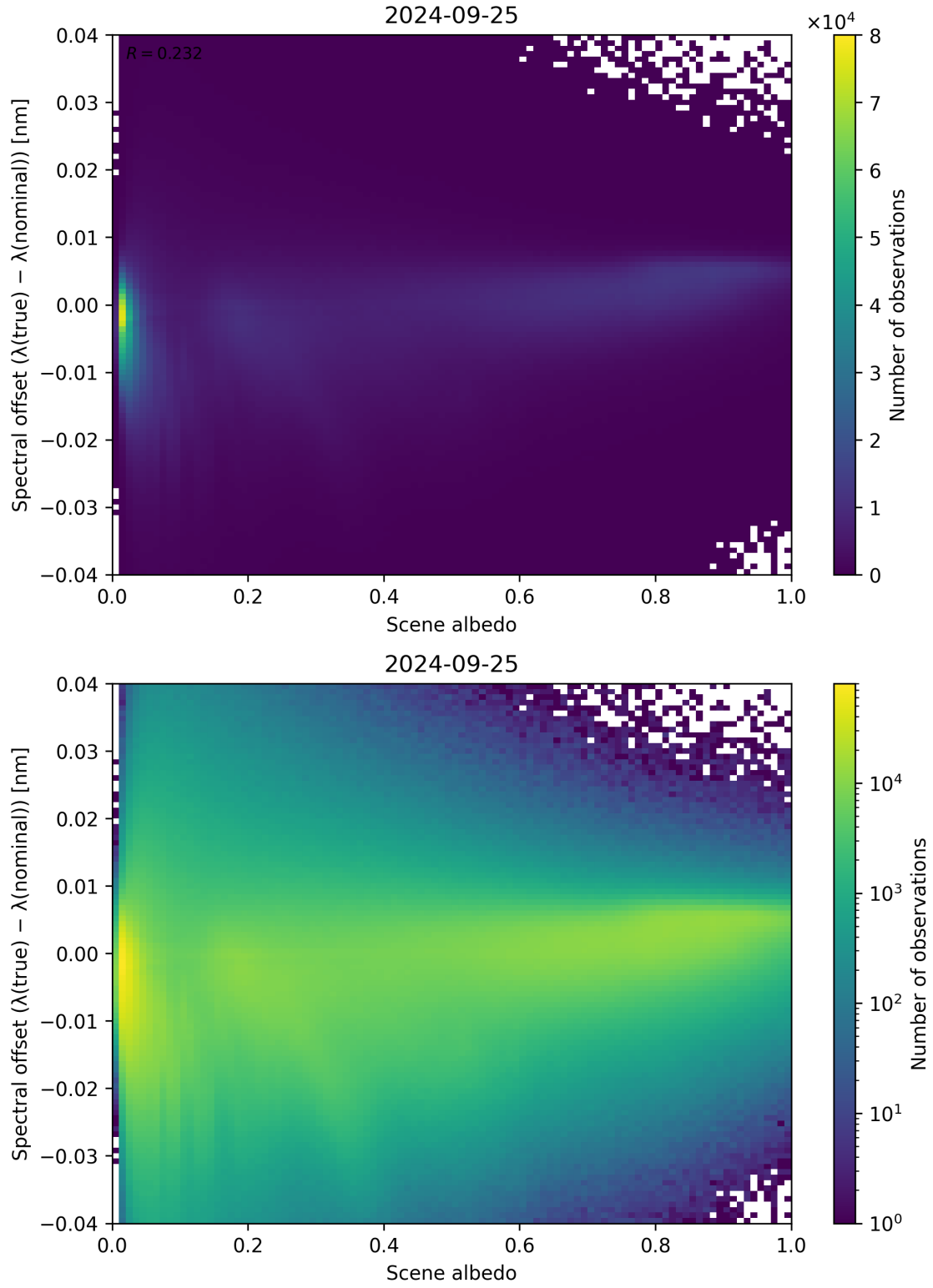
Figure 117: Scatter density plot of “Scene albedo” against “Spectral offset ( \lambda_{\text{true}} - \lambda_{\text{nominal}} )” for 2024-09-24 to 2024-09-26.
