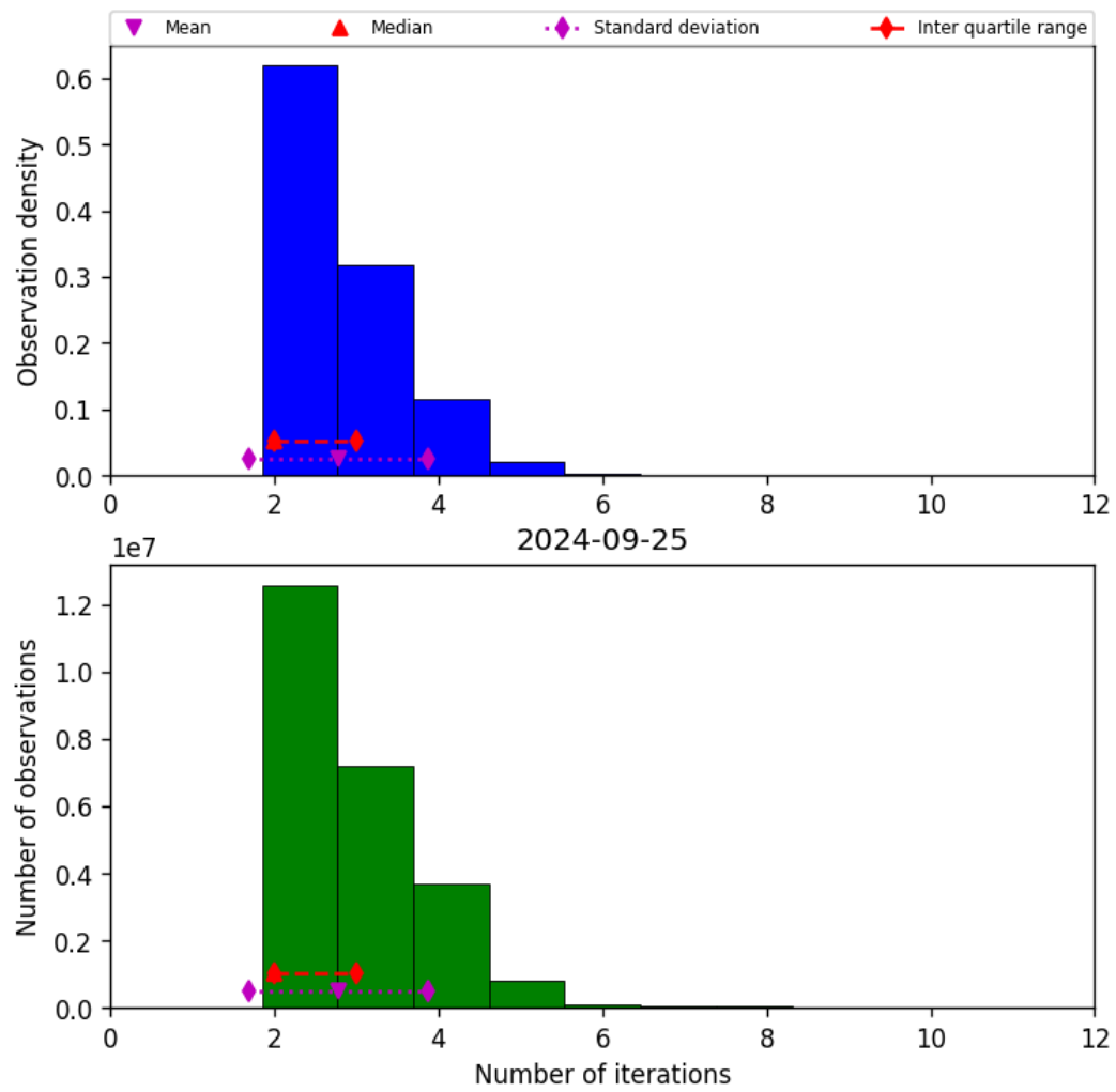
Figure 39: Histogram of “Number of iterations” for 2024-09-24 to 2024-09-26
