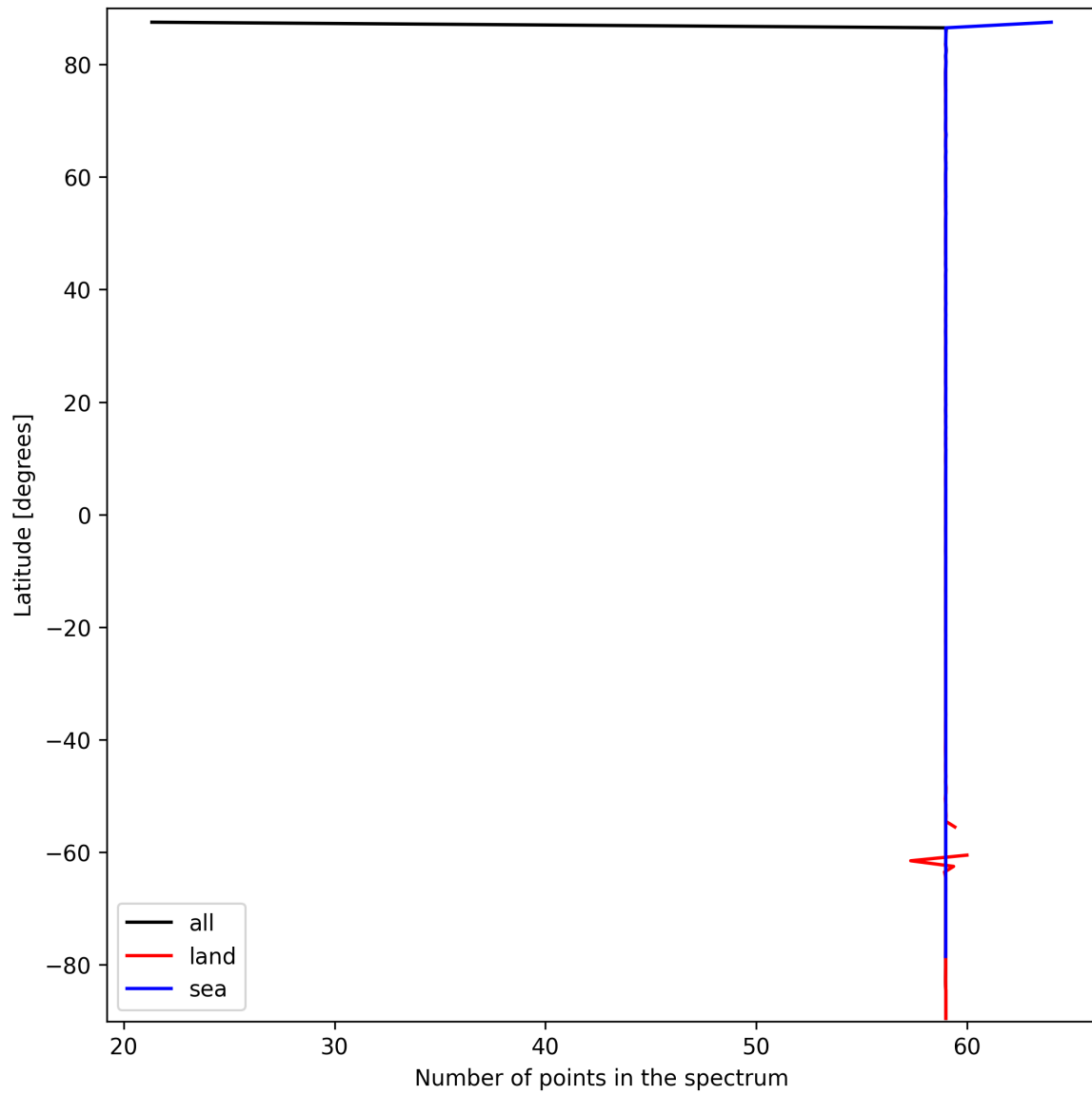
Figure 27: Zonal average of “Number of points in the spectrum” for 2024-09-24 to 2024-09-26.
