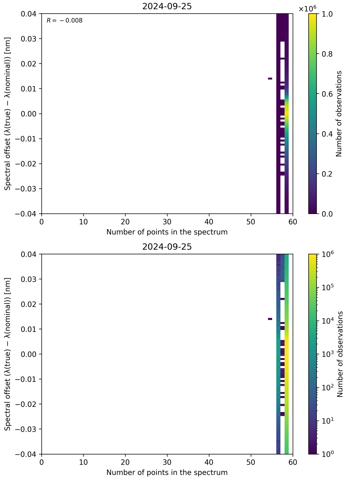
Figure 110: Scatter density plot of “Number of points in the spectrum” against “Spectral offset ( \lambda_{\text{true}} - \lambda_{\text{nominal}} )” for 2024-09-24 to 2024-09-26.
