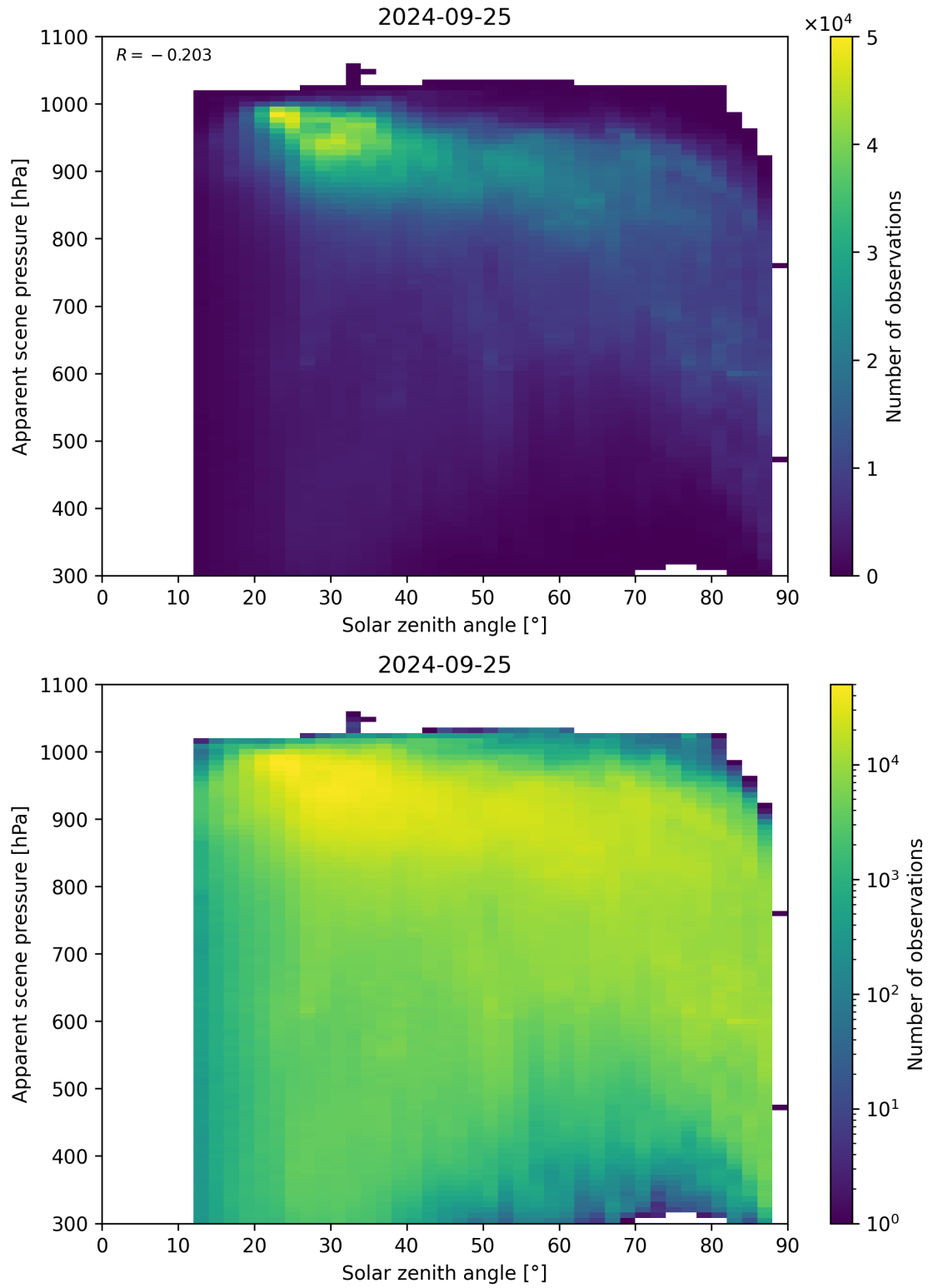
Figure 118: Scatter density plot of “Solar zenith angle” against “Apparent scene pressure” for 2024-09-24 to 2024-09-26.
