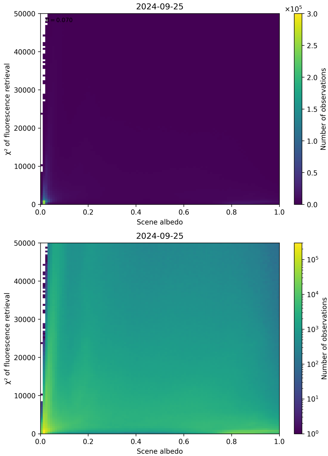
Figure 113: Scatter density plot of “Scene albedo” against “ \chi^2 of fluorescence retrieval” for 2024-09-24 to 2024-09-26.
