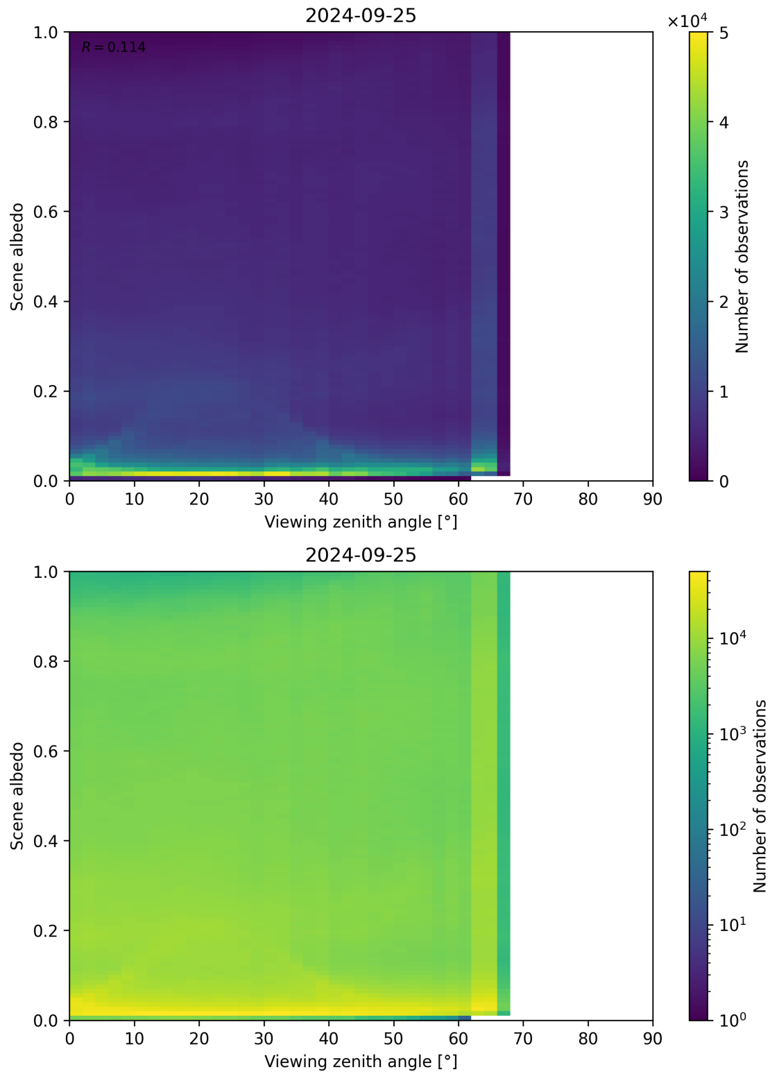
Figure 138: Scatter density plot of “Viewing zenith angle” against “Scene albedo” for 2024-09-24 to 2024-09-26.
