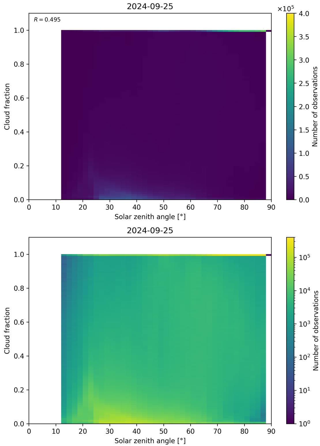
Figure 121: Scatter density plot of “Solar zenith angle” against “Cloud fraction” for 2024-09-24 to 2024-09-26.
