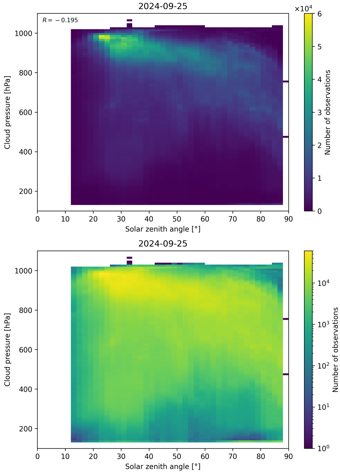
Figure 122: Scatter density plot of “Solar zenith angle” against “Cloud pressure” for 2024-09-24 to 2024-09-26.
