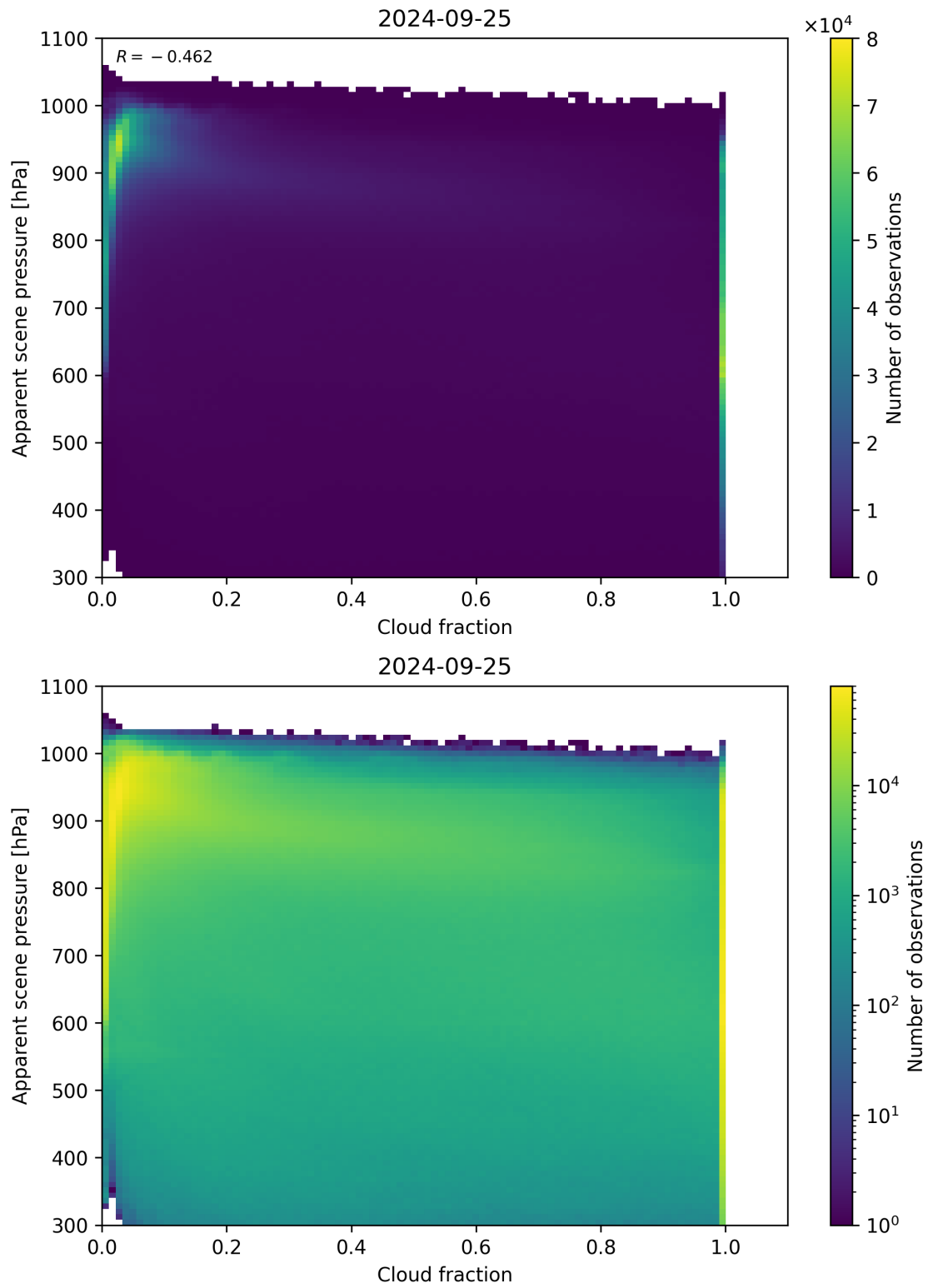
Figure 76: Scatter density plot of “Cloud fraction” against “Apparent scene pressure” for 2024-09-24 to 2024-09-26.
