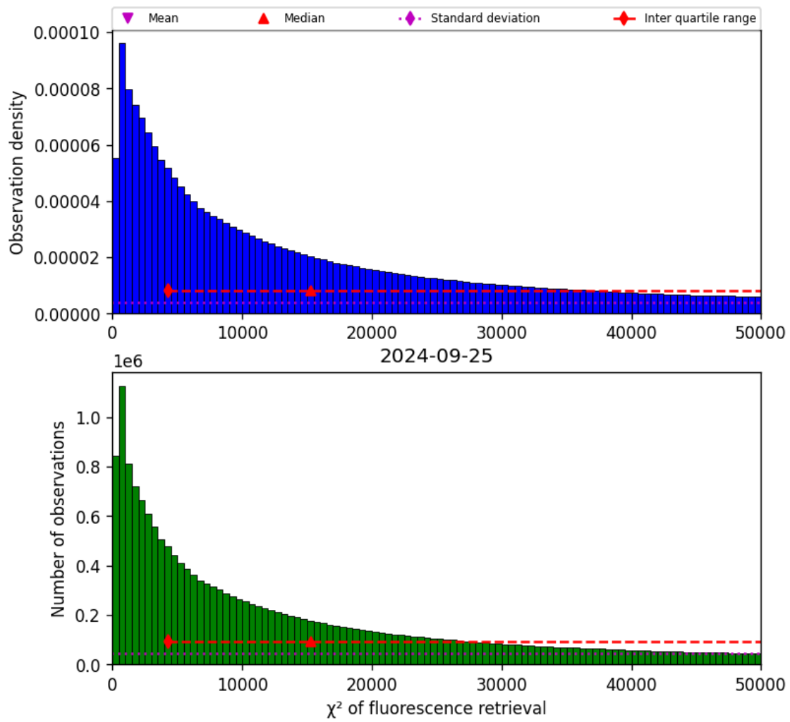
Figure 42: Histogram of “ \chi^2 of fluorescence retrieval” for 2024-09-24 to 2024-09-26
