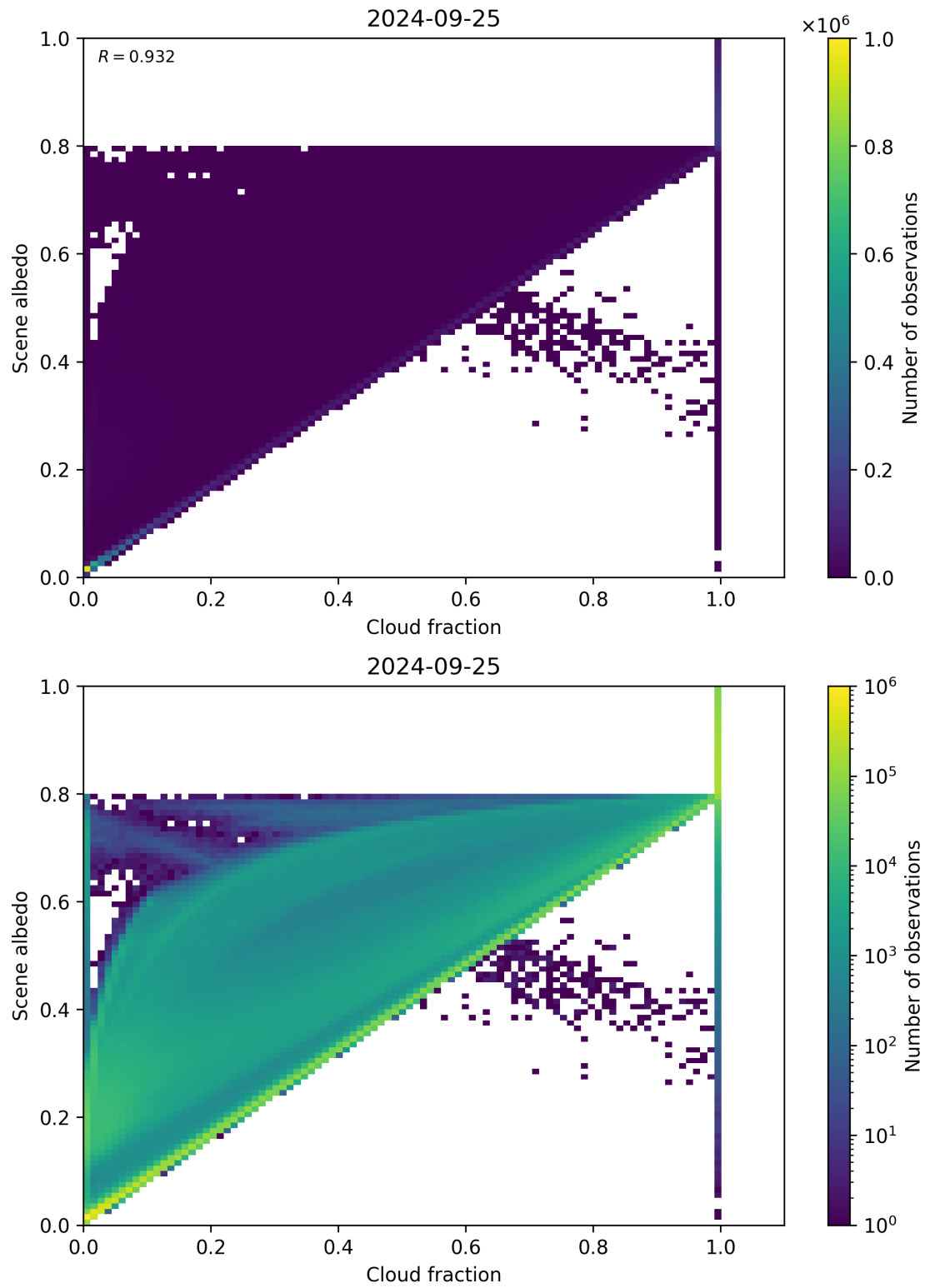
Figure 82: Scatter density plot of “Cloud fraction” against “Scene albedo” for 2024-09-24 to 2024-09-26.
