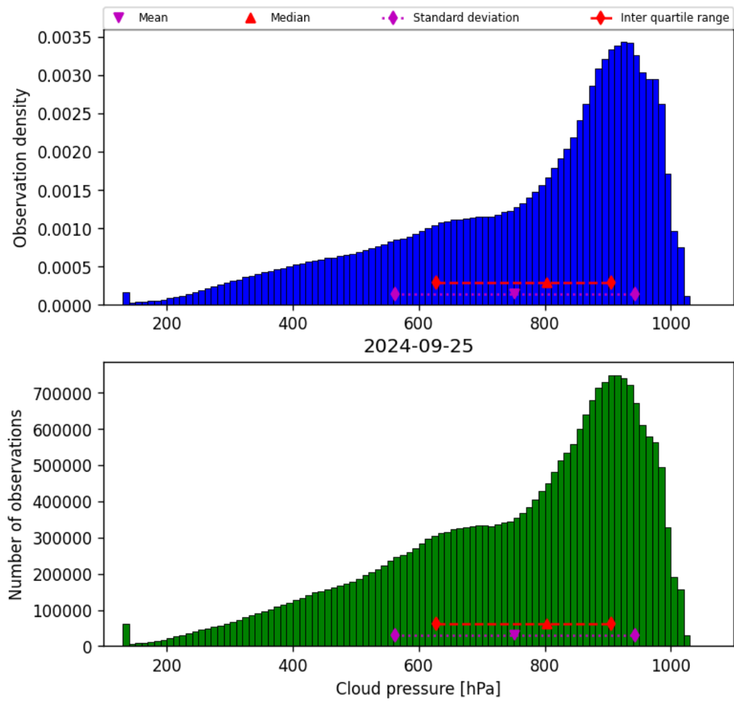
Figure 30: Histogram of “Cloud pressure” for 2024-09-24 to 2024-09-26
