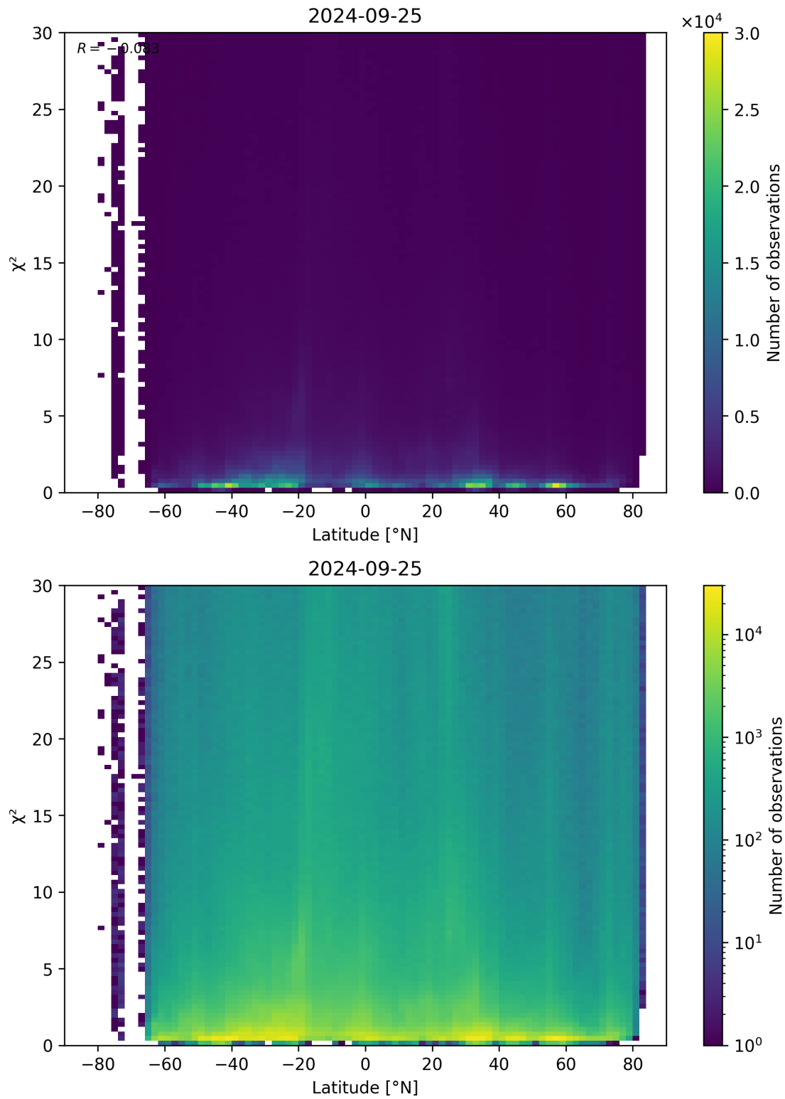
Figure 97: Scatter density plot of “Latitude” against “ \chi^2 ” for 2024-09-24 to 2024-09-26.
