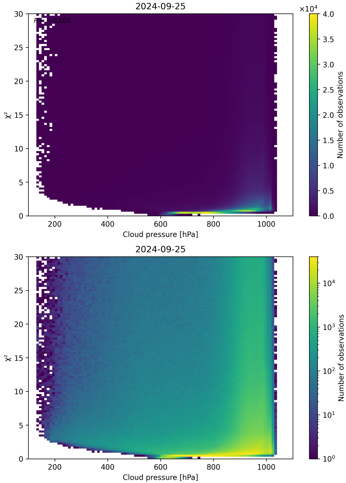
Figure 85: Scatter density plot of “Cloud pressure” against “ \chi^2 ” for 2024-09-24 to 2024-09-26.
