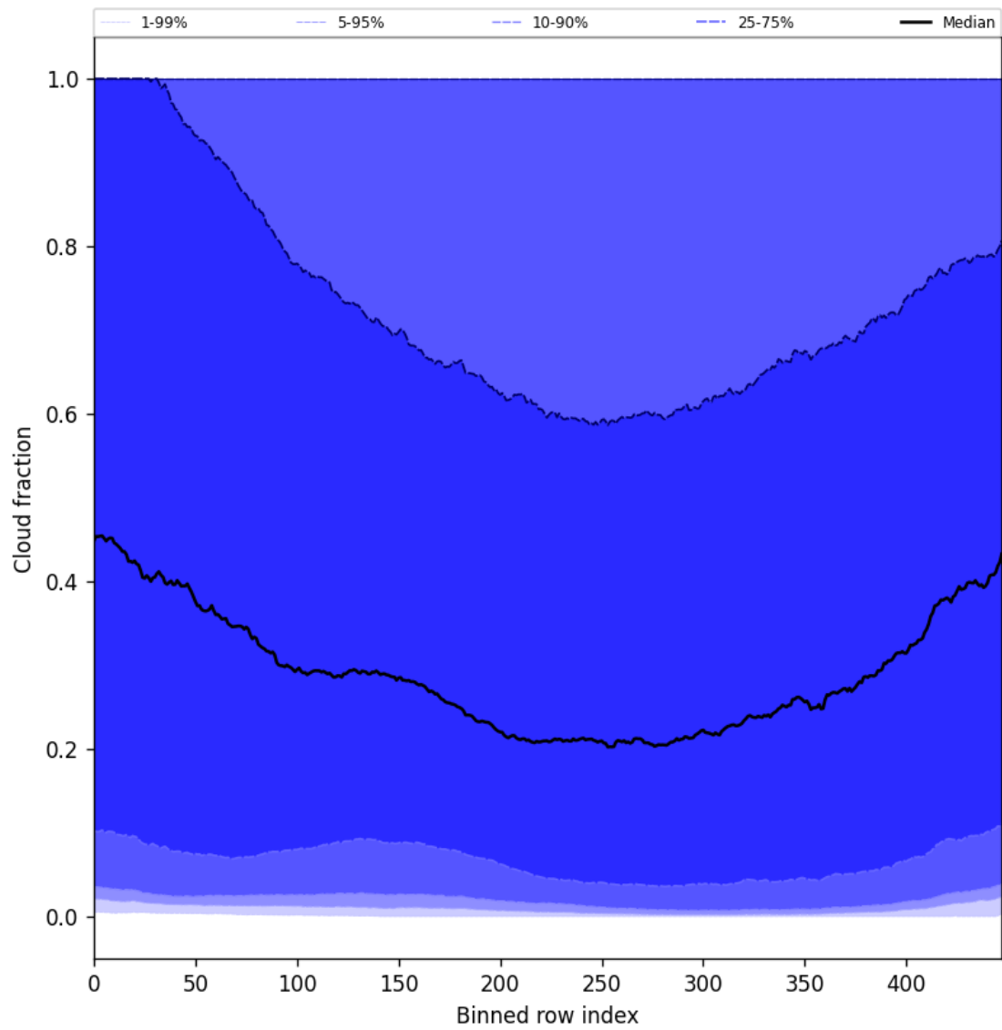
Figure 49: Along track statistics of “Cloud fraction” for 2024-09-24 to 2024-09-26
