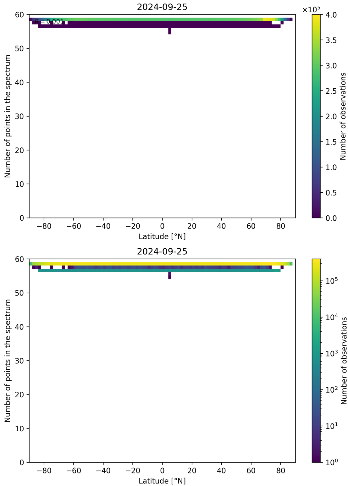
Figure 103: Scatter density plot of “Latitude” against “Number of points in the spectrum” for 2024-09-24 to 2024-09-26.
