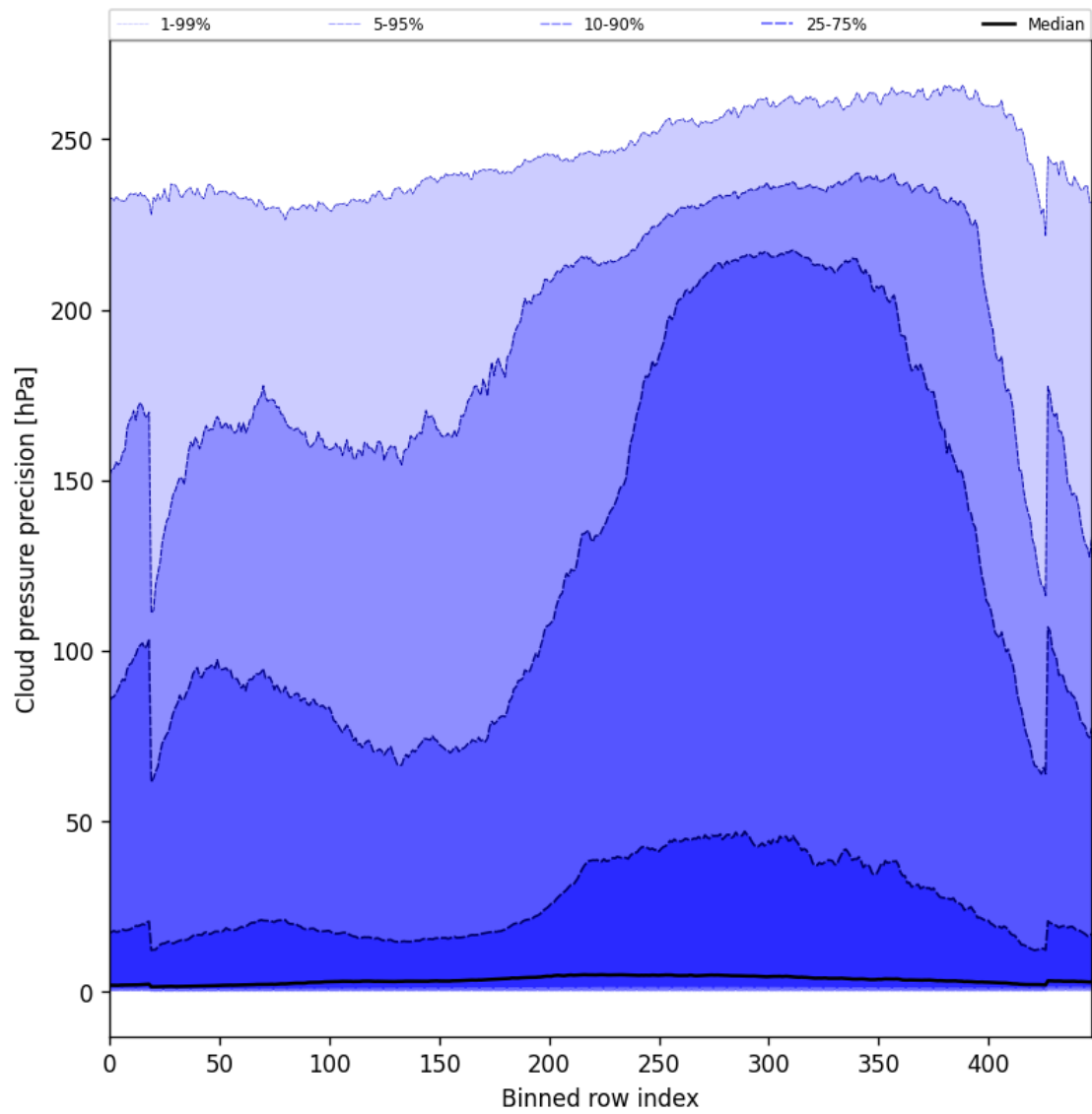
Figure 48: Along track statistics of “Cloud pressure precision” for 2024-09-24 to 2024-09-26
