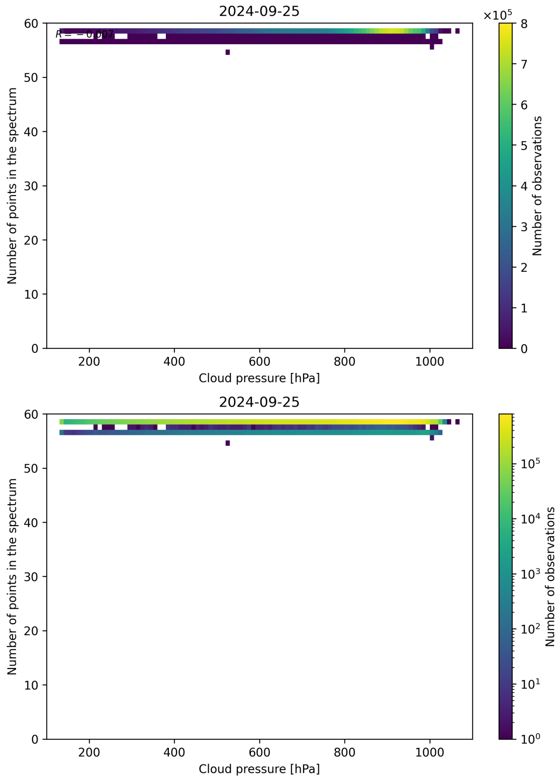
Figure 90: Scatter density plot of “Cloud pressure” against “Number of points in the spectrum” for 2024-09-24 to 2024-09-26.
