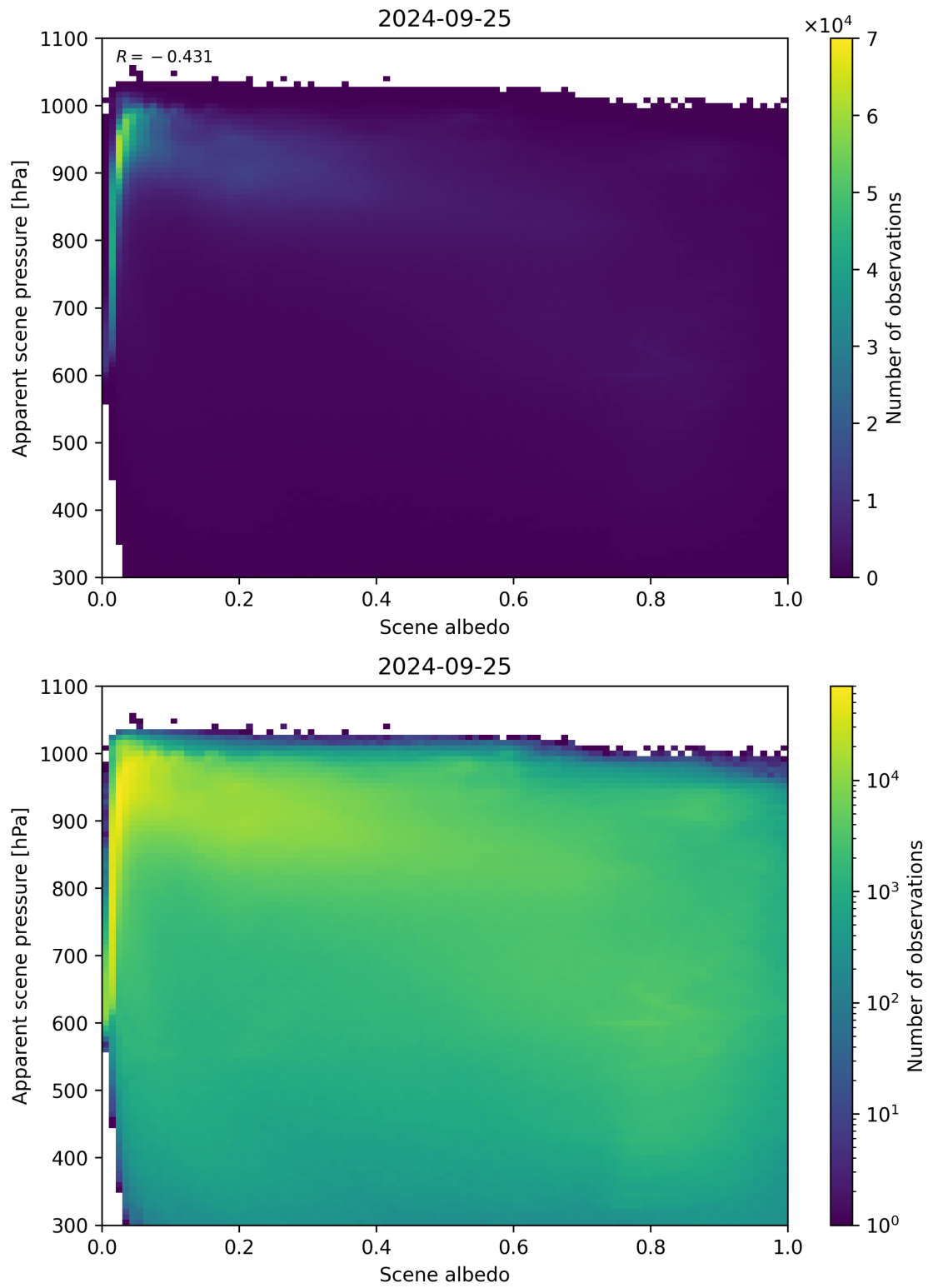
Figure 111: Scatter density plot of “Scene albedo” against “Apparent scene pressure” for 2024-09-24 to 2024-09-26.
