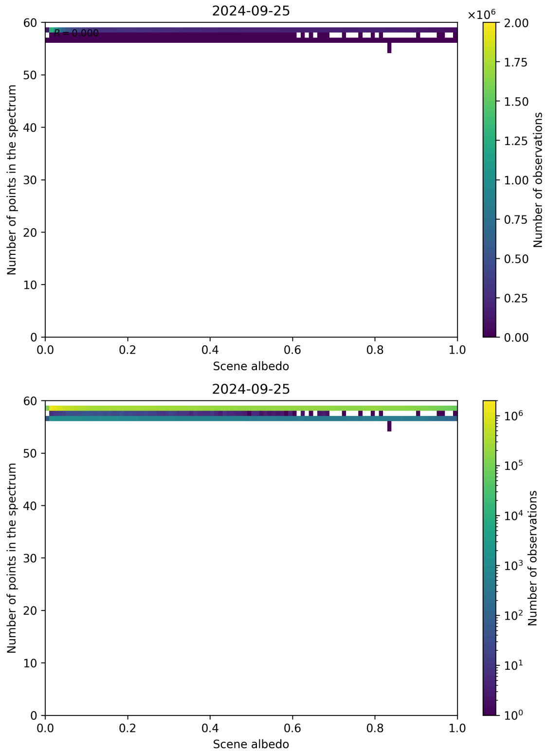
Figure 116: Scatter density plot of “Scene albedo” against “Number of points in the spectrum” for 2024-09-24 to 2024-09-26.
