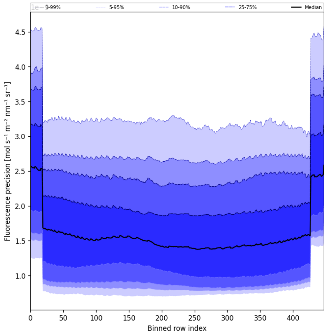
Figure 58: Along track statistics of “Fluorescence precision” for 2024-09-24 to 2024-09-26
