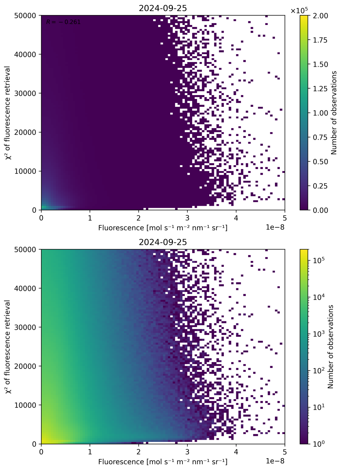
Figure 93: Scatter density plot of “Fluorescence” against “ \chi^2 of fluorescence retrieval” for 2024-09-24 to 2024-09-26.
