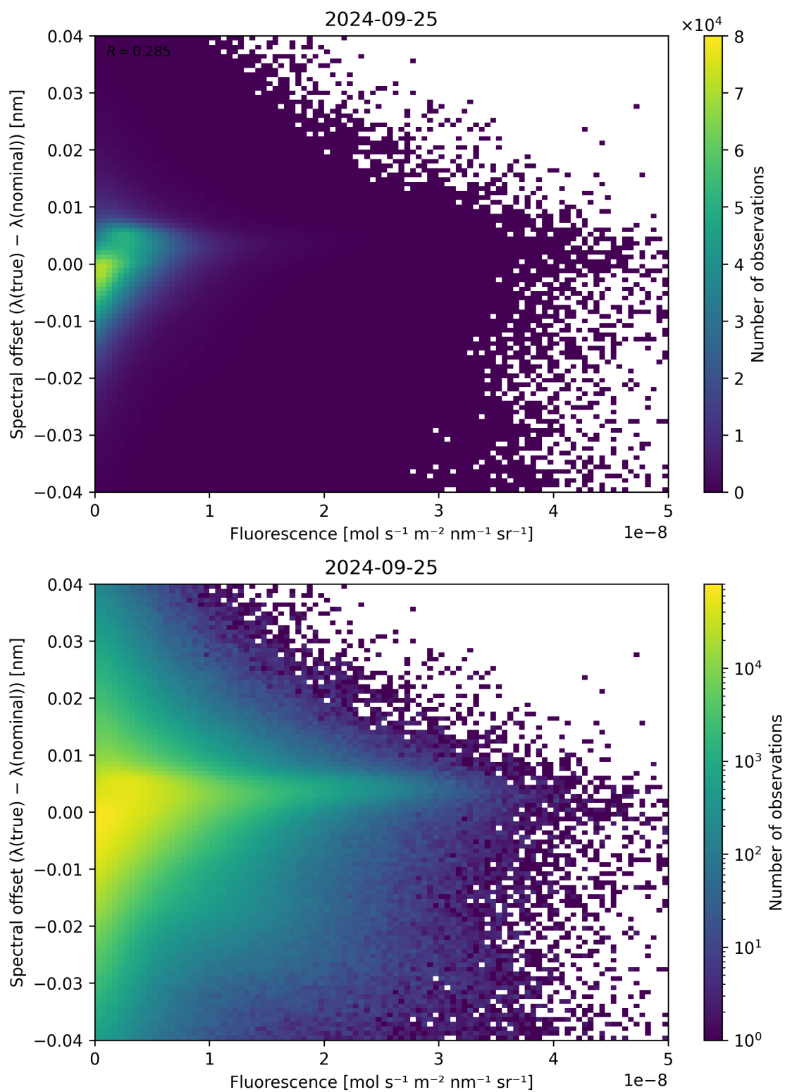
Figure 95: Scatter density plot of “Fluorescence” against “Spectral offset ( \lambda_{\text{true}} - \lambda_{\text{nominal}} )” for 2024-09-24 to 2024-09-26.
