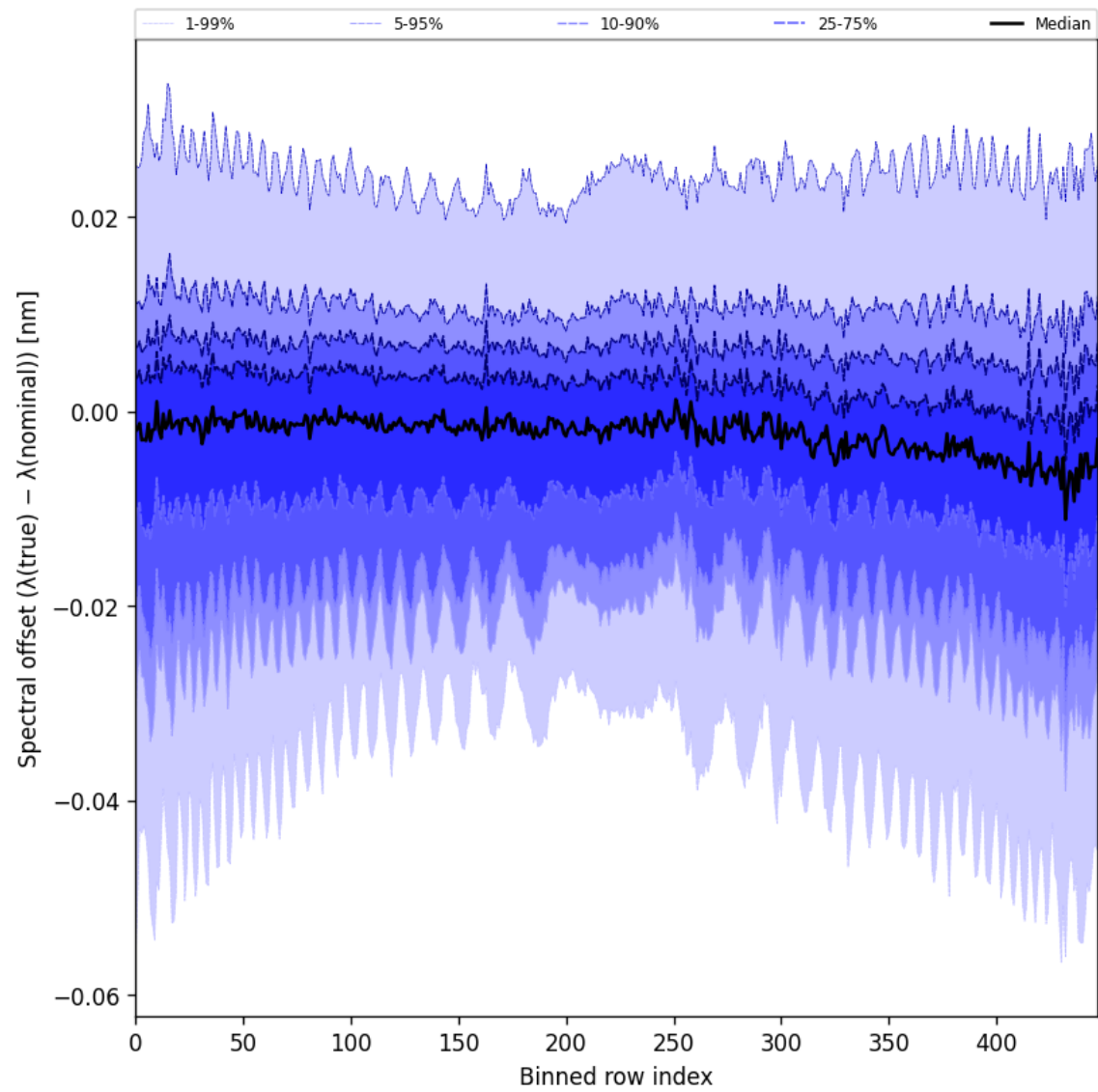
Figure 62: Along track statistics of “Spectral offset ( \lambda_{\text{true}} - \lambda_{\text{nominal}} )” for 2024-09-24 to 2024-09-26
