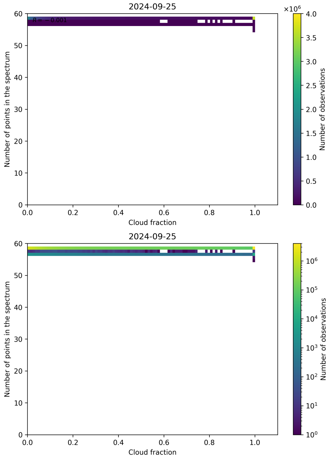
Figure 81: Scatter density plot of “Cloud fraction” against “Number of points in the spectrum” for 2024-09-24 to 2024-09-26.
