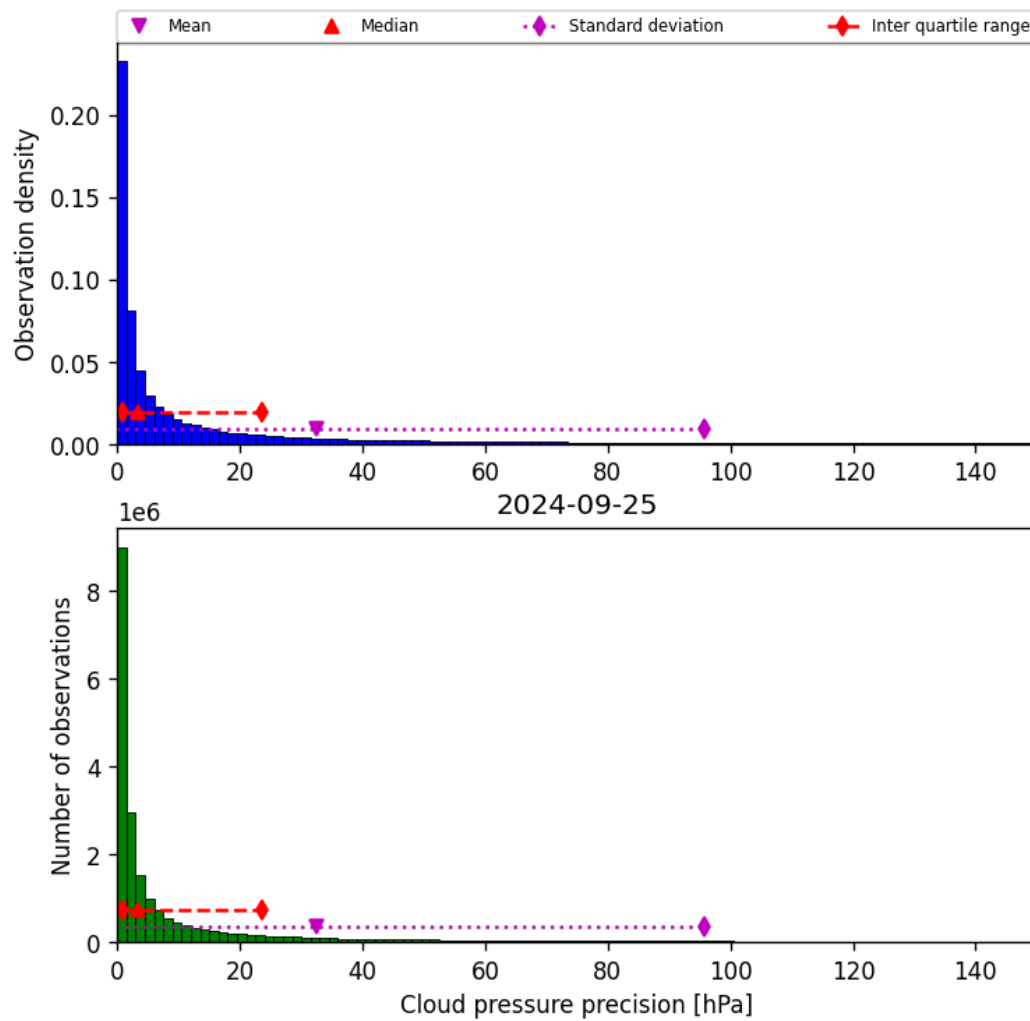
Figure 31: Histogram of “Cloud pressure precision” for 2024-09-24 to 2024-09-26
