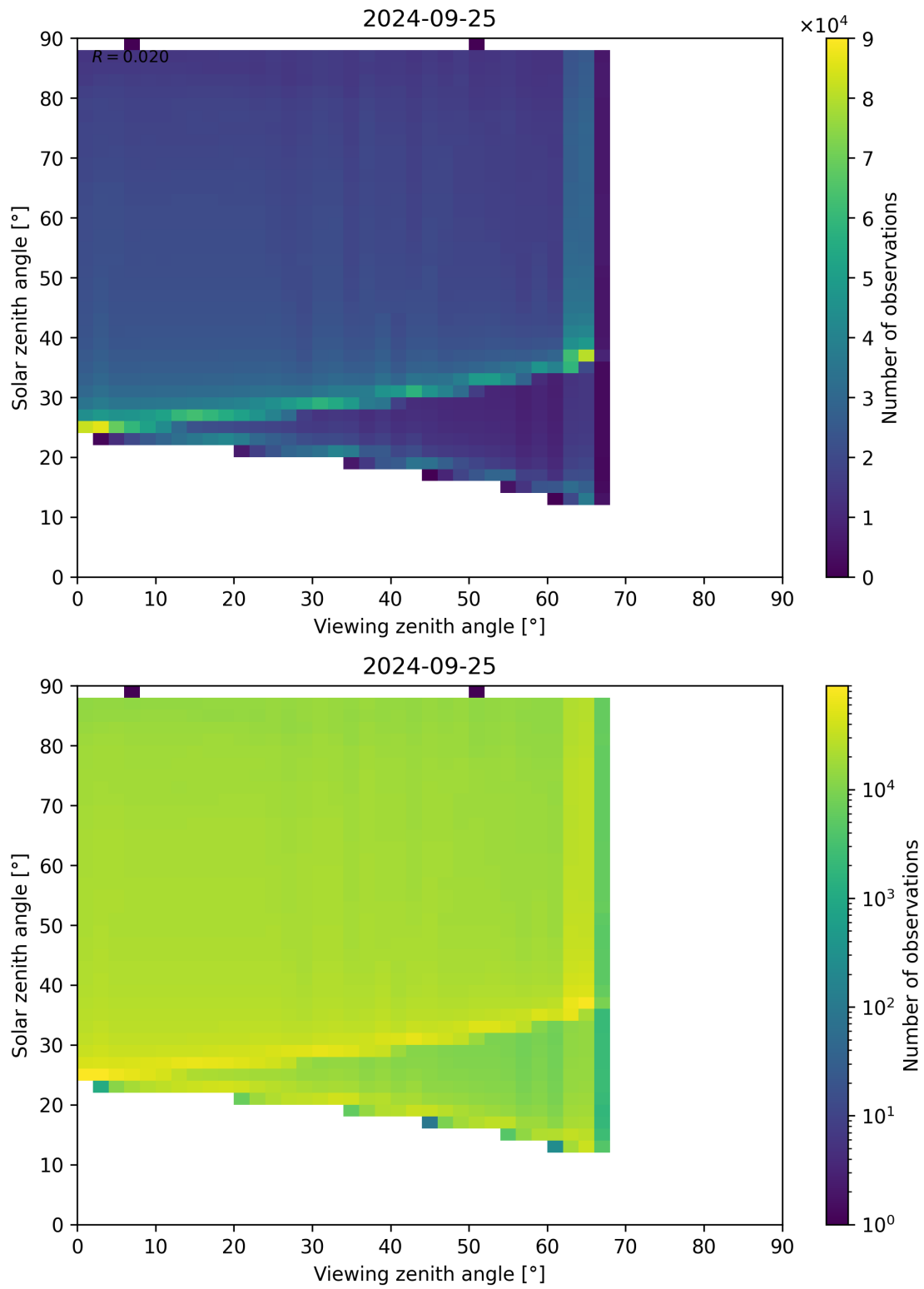
Figure 139: Scatter density plot of “Viewing zenith angle” against “Solar zenith angle” for 2024-09-24 to 2024-09-26.
