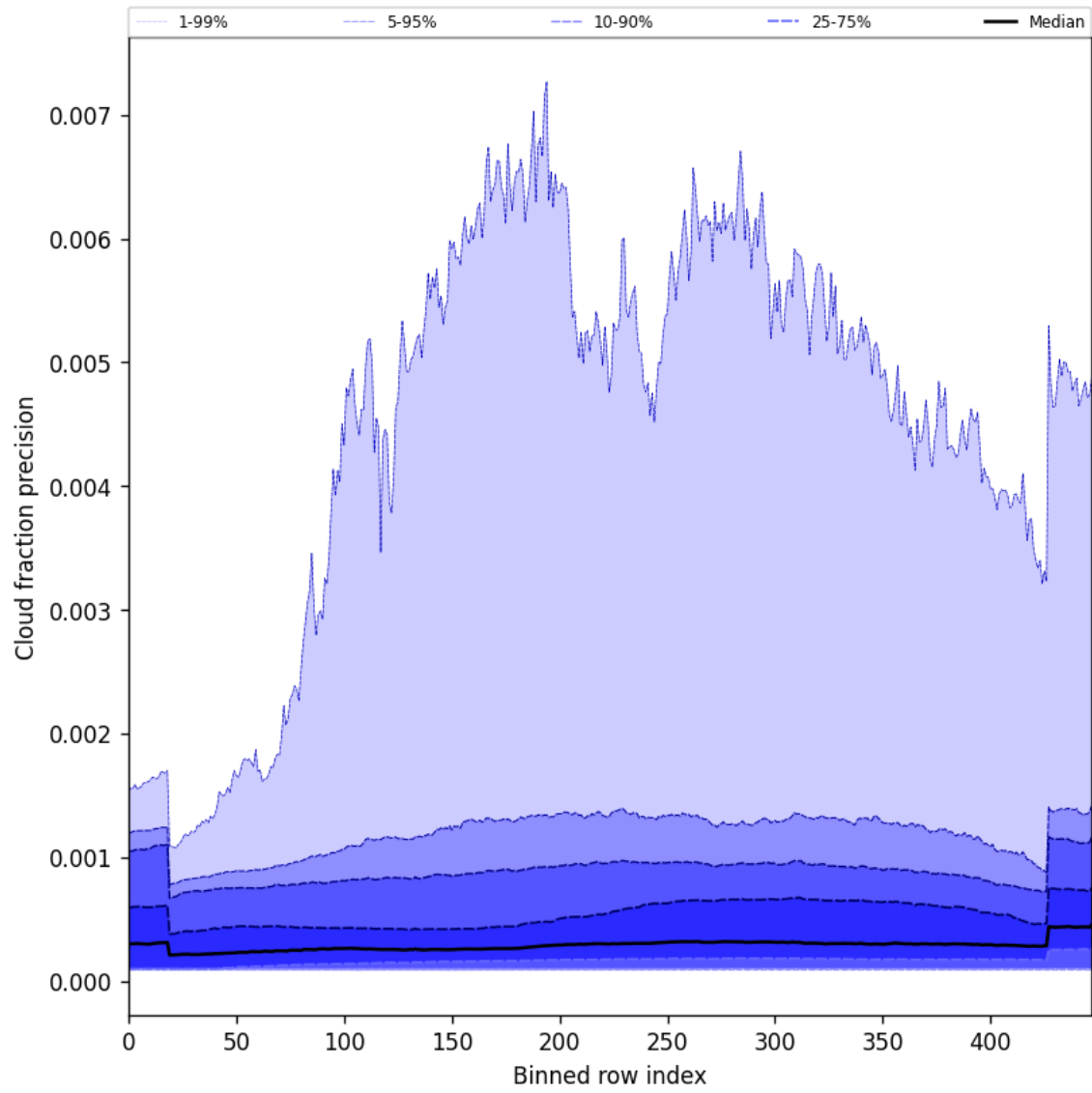
Figure 50: Along track statistics of “Cloud fraction precision” for 2024-09-24 to 2024-09-26
