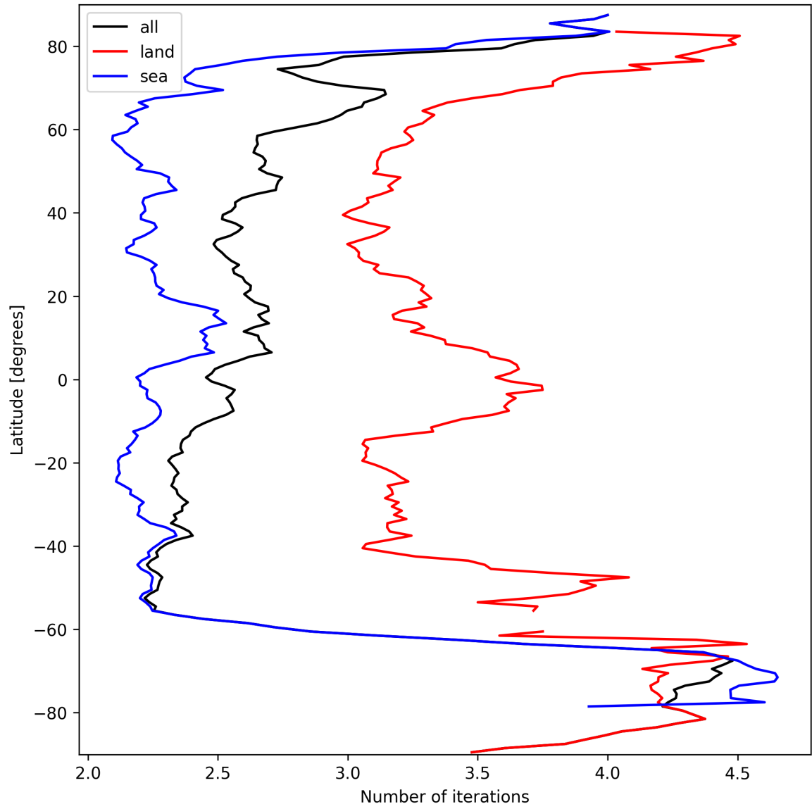
Figure 22: Zonal average of “Number of iterations” for 2024-09-24 to 2024-09-26.
