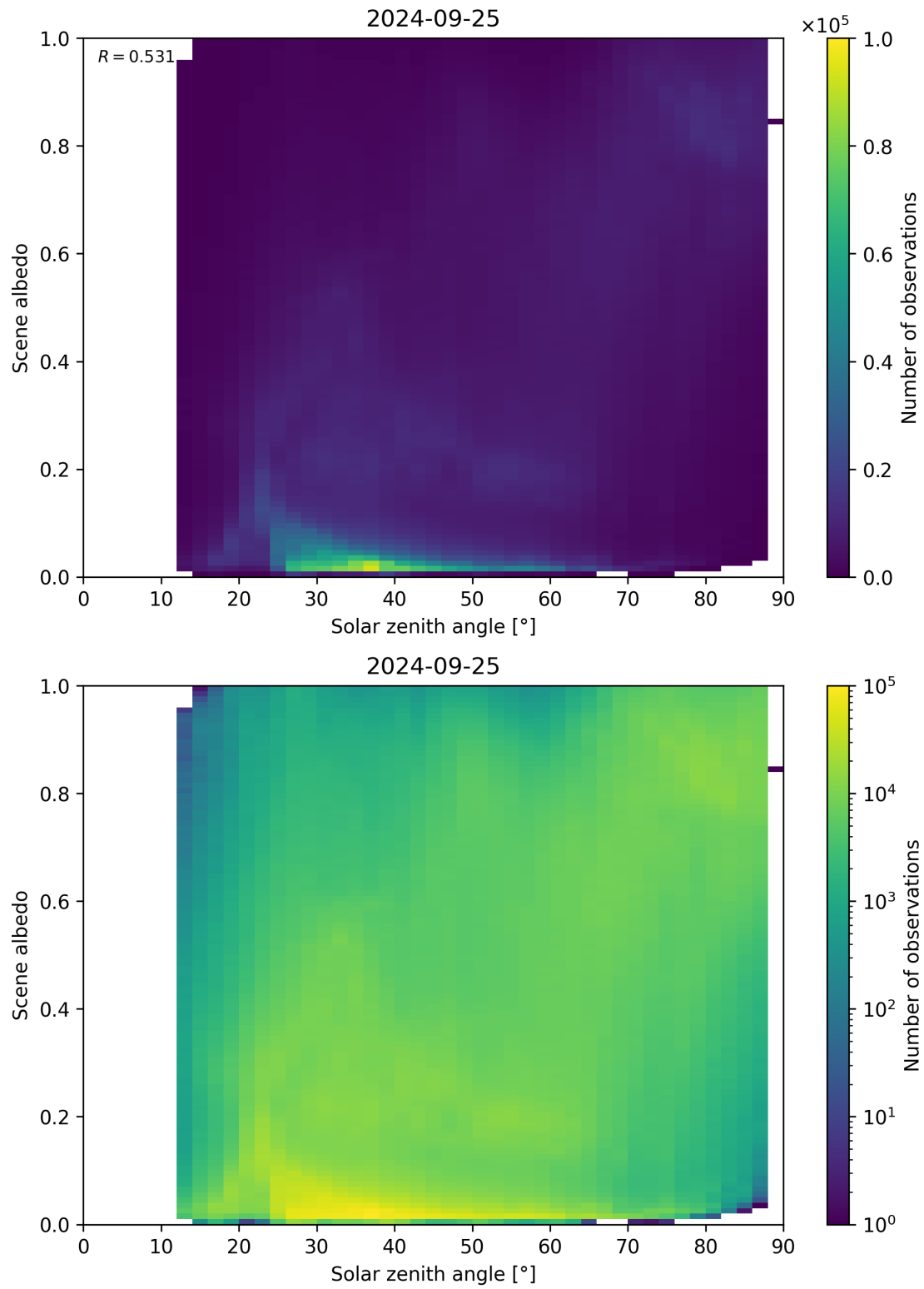
Figure 127: Scatter density plot of “Solar zenith angle” against “Scene albedo” for 2024-09-24 to 2024-09-26.
