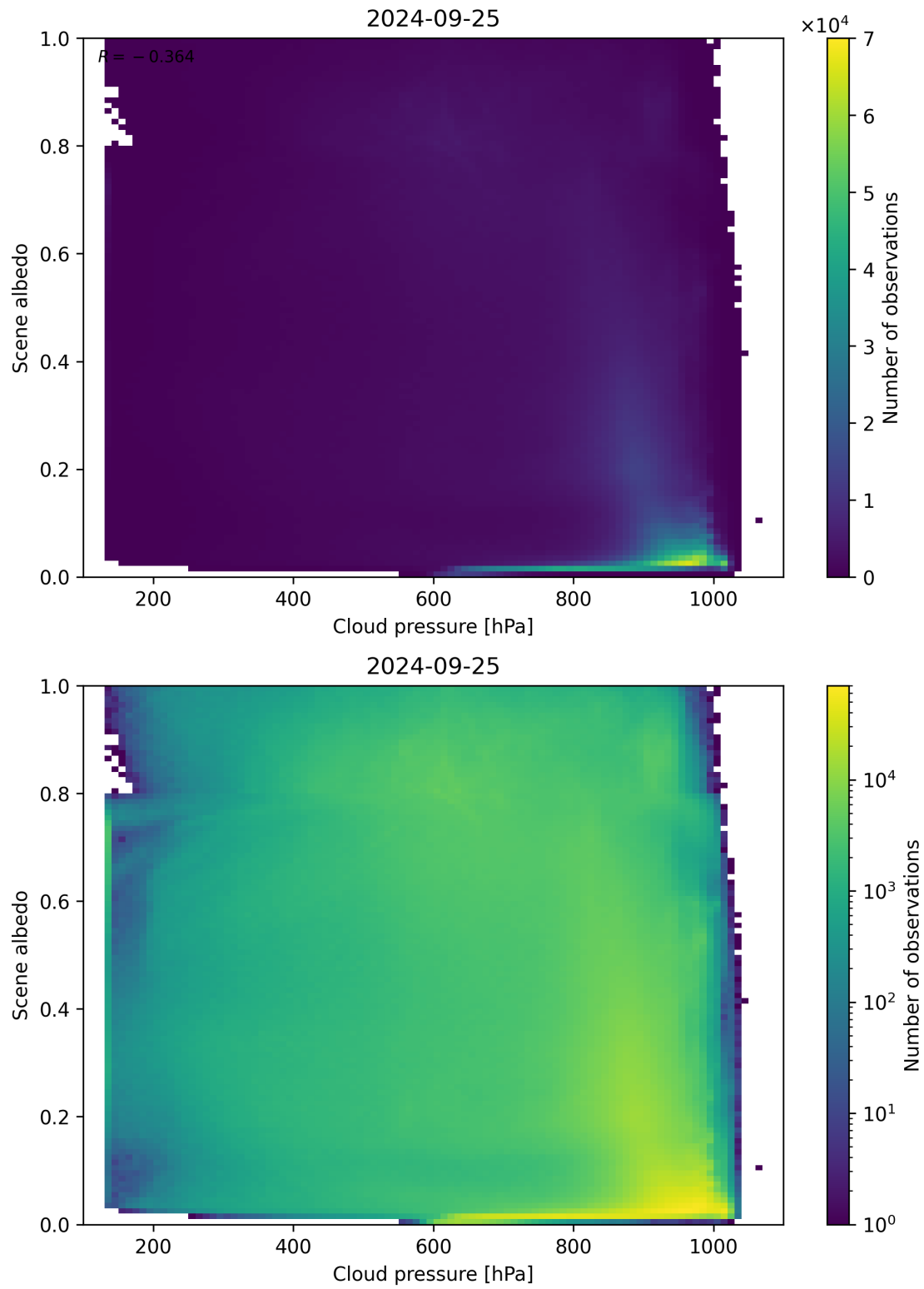
Figure 91: Scatter density plot of “Cloud pressure” against “Scene albedo” for 2024-09-24 to 2024-09-26.
