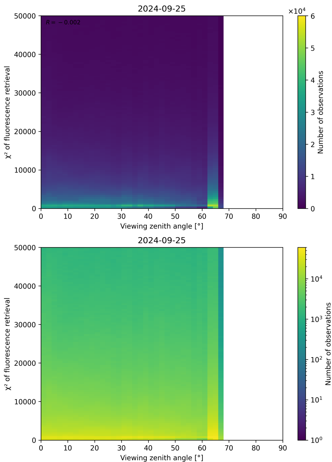
Figure 131: Scatter density plot of “Viewing zenith angle” against “ \chi^2 of fluorescence retrieval” for 2024-09-24 to 2024-09-26.
