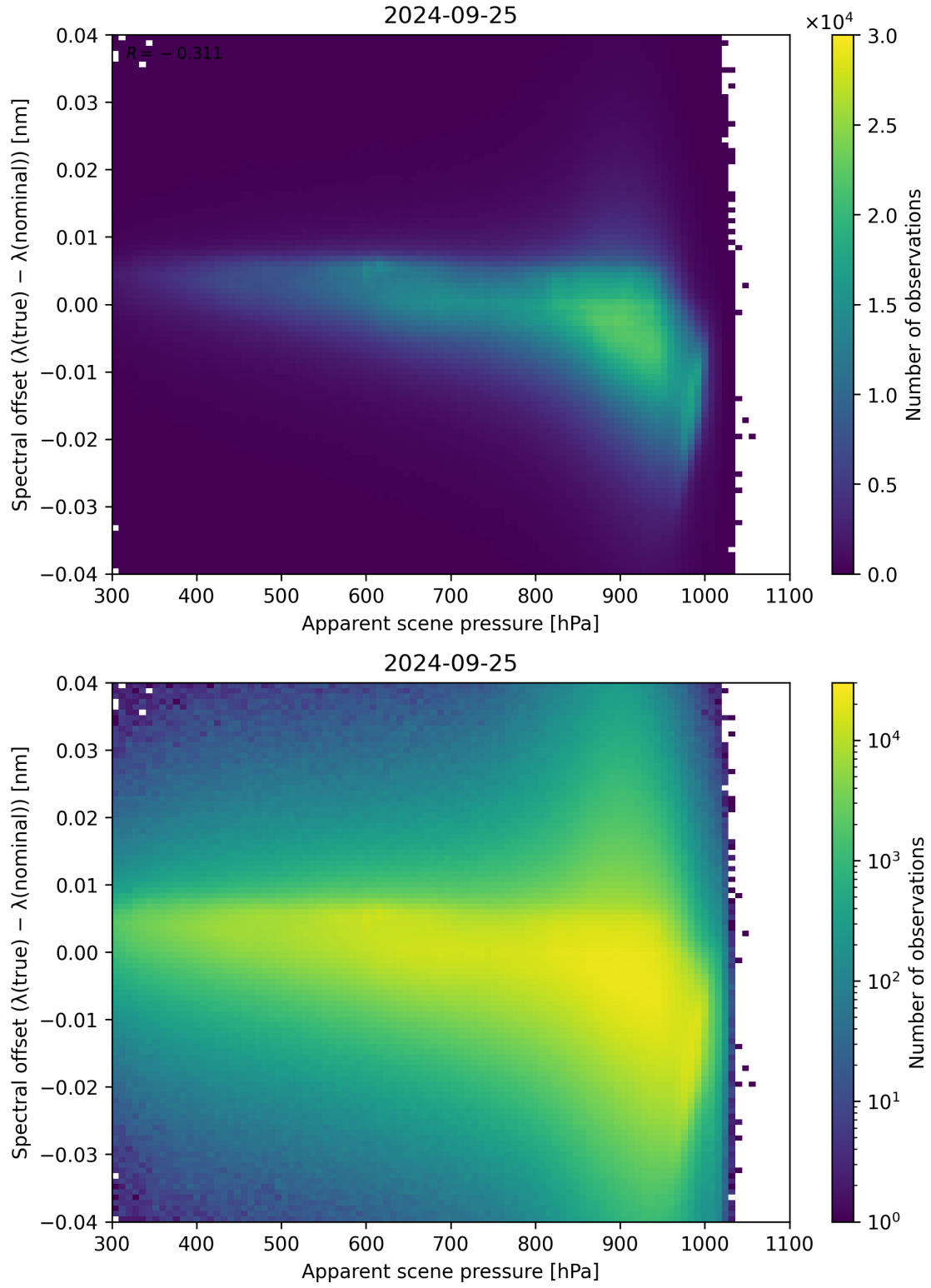
Figure 68: Scatter density plot of “Apparent scene pressure” against “Spectral offset ( \lambda_{\text{true}} - \lambda_{\text{nominal}} )” for 2024-09-24 to 2024-09-26.
