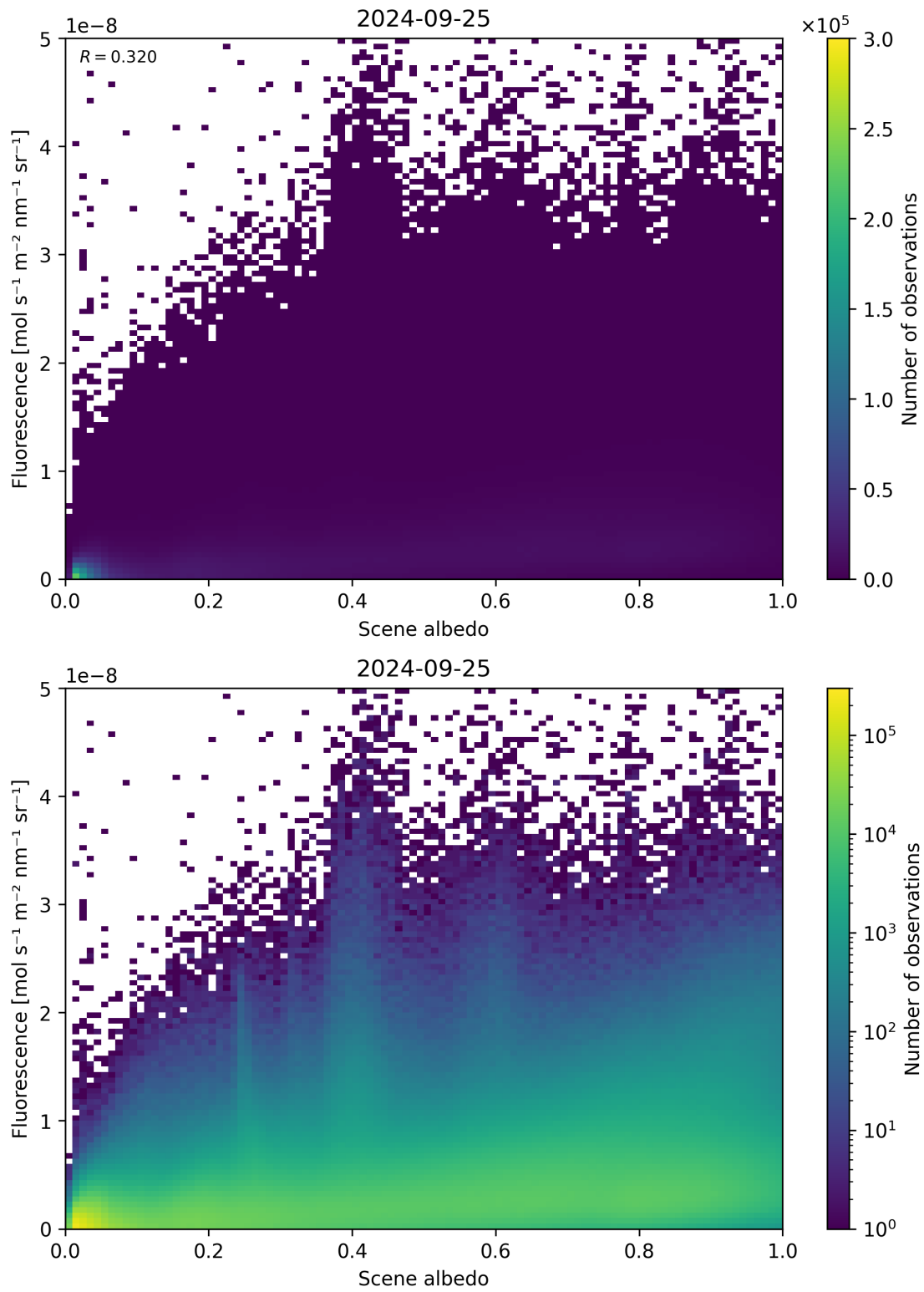
Figure 114: Scatter density plot of “Scene albedo” against “Fluorescence” for 2024-09-24 to 2024-09-26.
