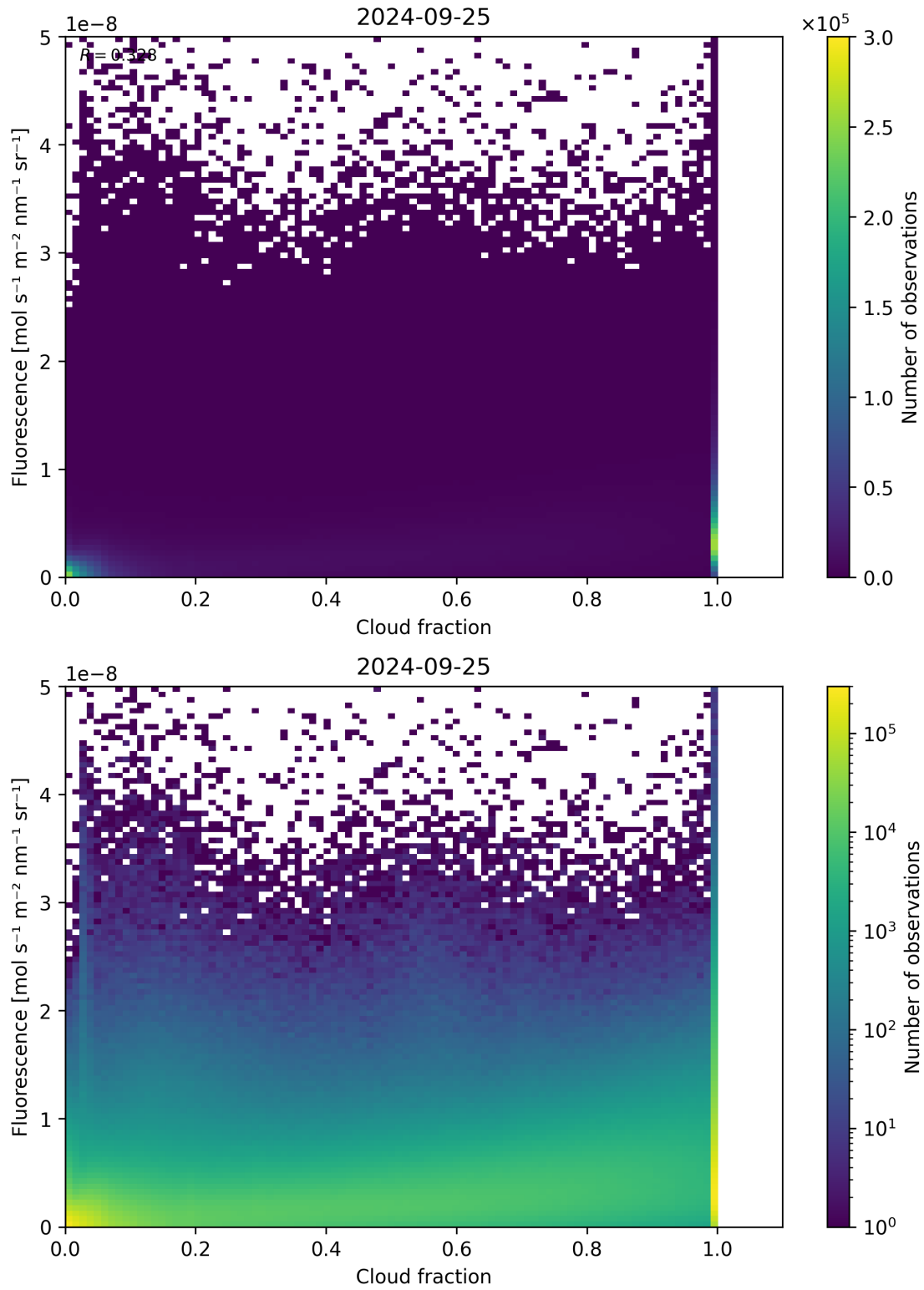
Figure 79: Scatter density plot of “Cloud fraction” against “Fluorescence” for 2024-09-24 to 2024-09-26.
