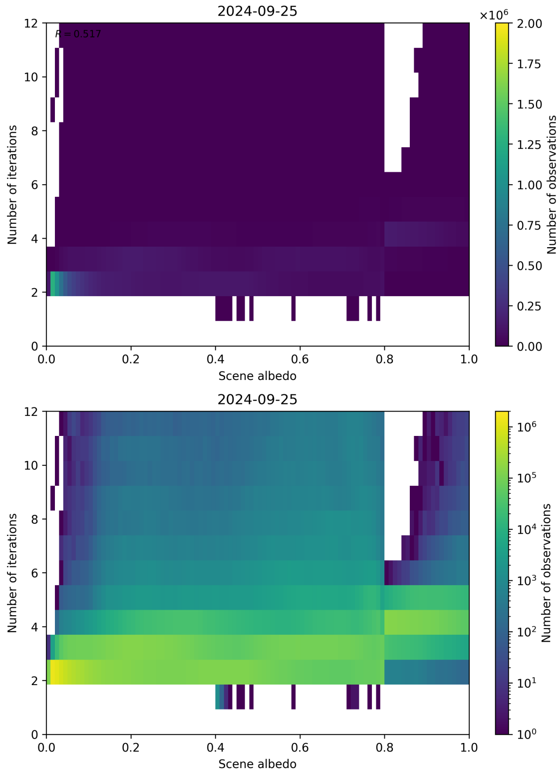
Figure 115: Scatter density plot of “Scene albedo” against “Number of iterations” for 2024-09-24 to 2024-09-26.
