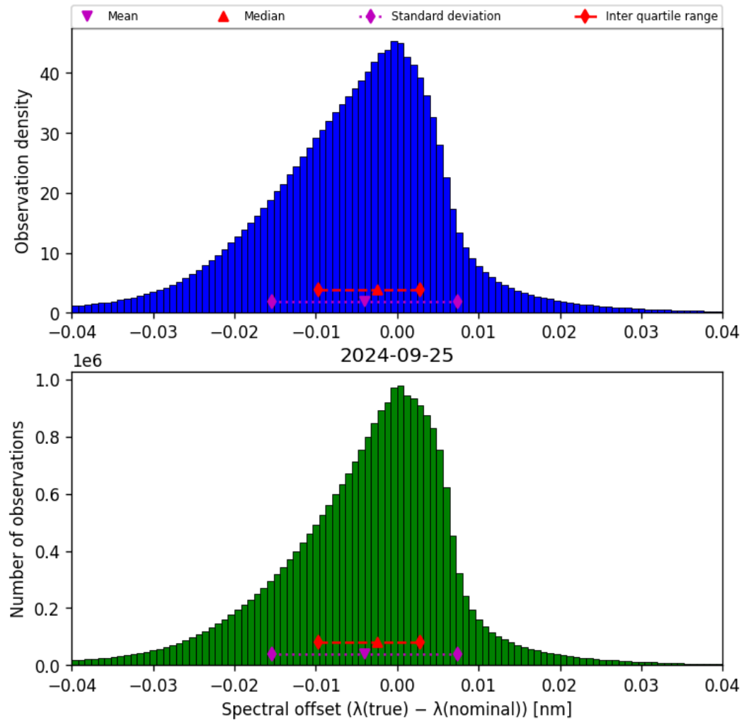
Figure 45: Histogram of “Spectral offset ( \lambda_{\text{true}} - \lambda_{\text{nominal}} )” for 2024-09-24 to 2024-09-26
