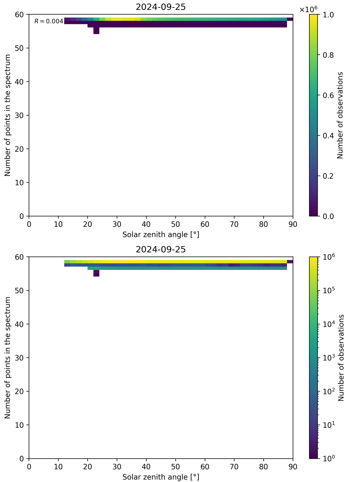
Figure 126: Scatter density plot of “Solar zenith angle” against “Number of points in the spectrum” for 2024-09-24 to 2024-09-26.
