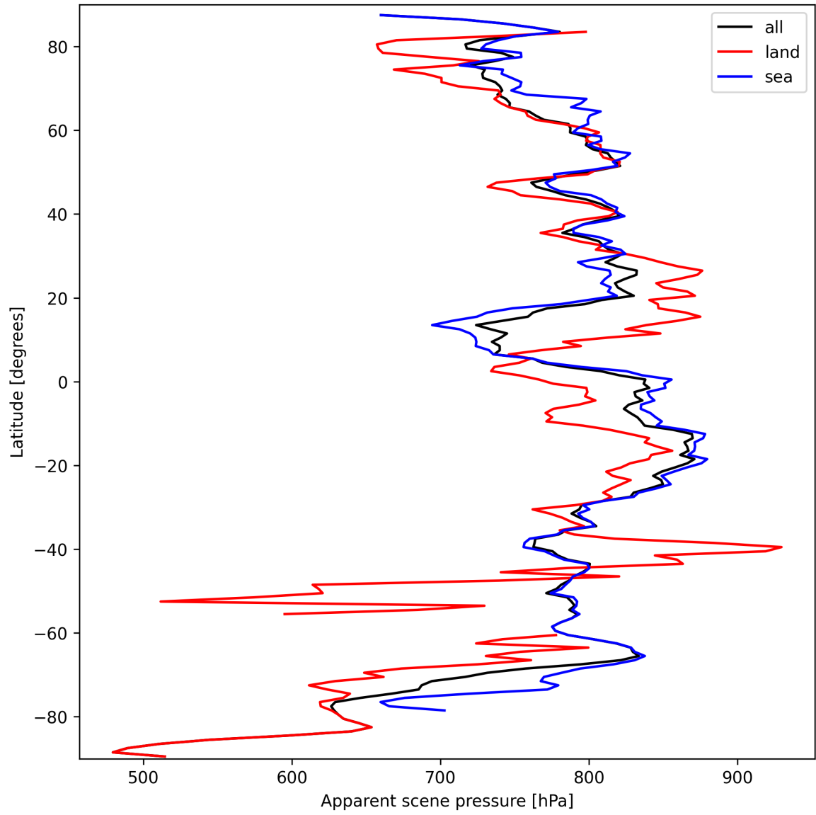
Figure 19: Zonal average of “Apparent scene pressure” for 2024-09-24 to 2024-09-26.
