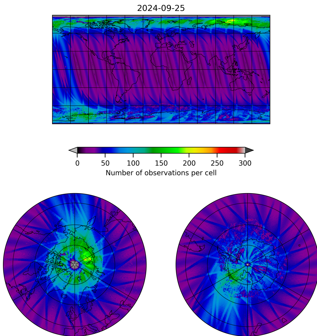
Figure 11: Map of the number of observations for 2024-09-24 to 2024-09-26
