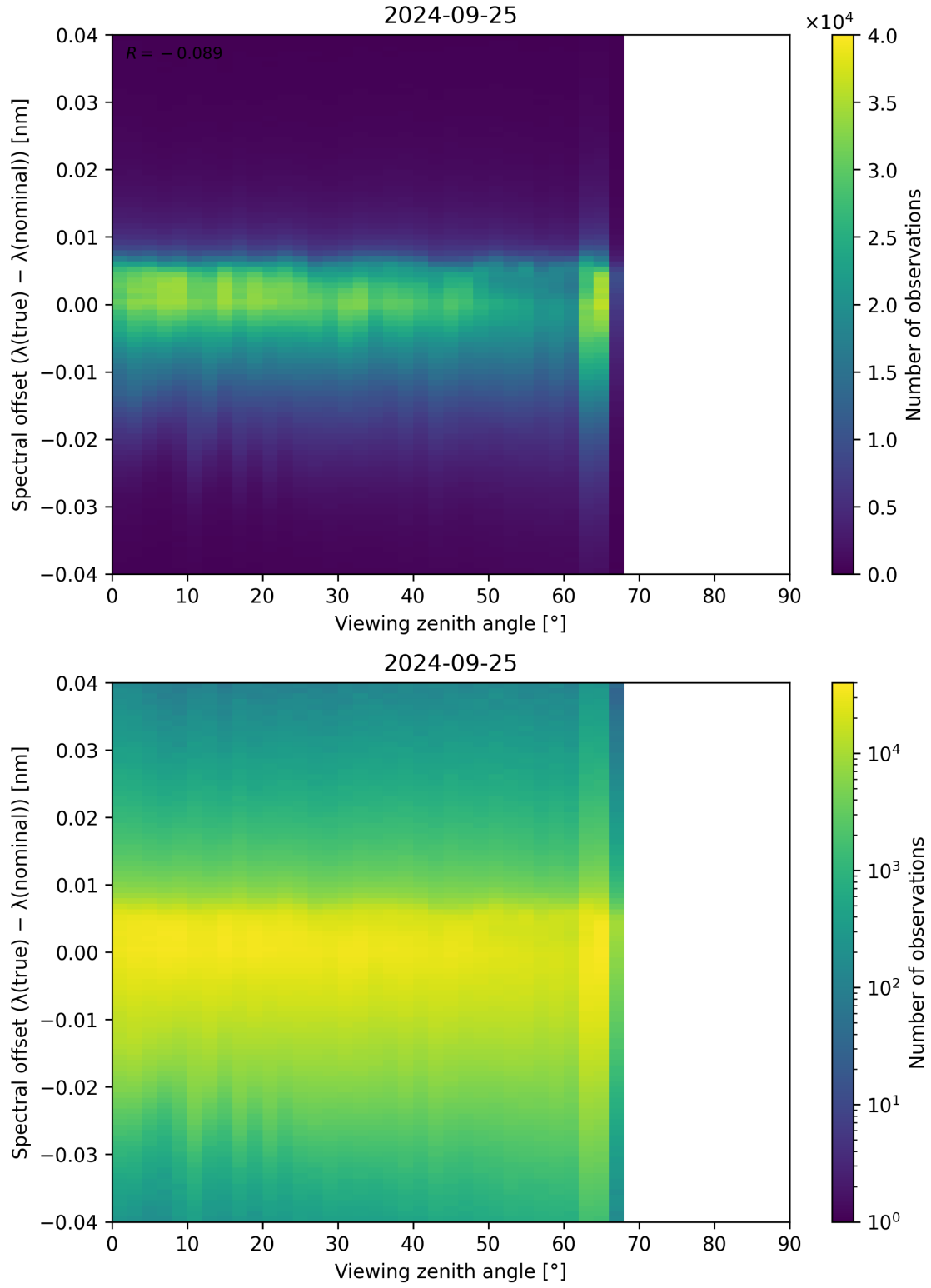
Figure 140: Scatter density plot of “Viewing zenith angle” against “Spectral offset ( \lambda_{\text{true}} - \lambda_{\text{nominal}} )” for 2024-09-24 to 2024-09-26.
