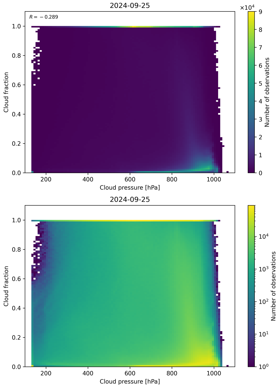
Figure 87: Scatter density plot of “Cloud pressure” against “Cloud fraction” for 2024-09-24 to 2024-09-26.
