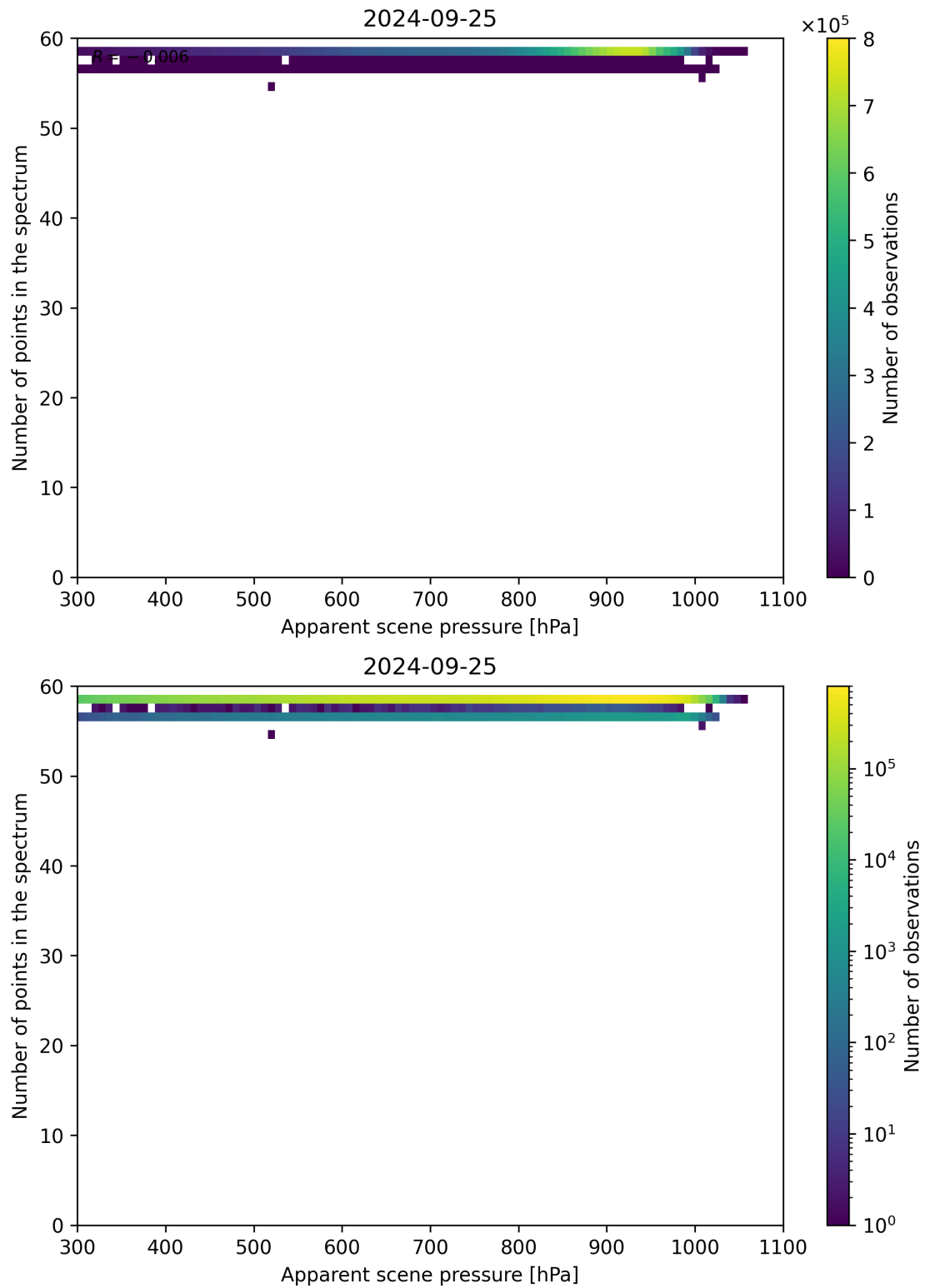
Figure 67: Scatter density plot of “Apparent scene pressure” against “Number of points in the spectrum” for 2024-09-24 to 2024-09-26.
