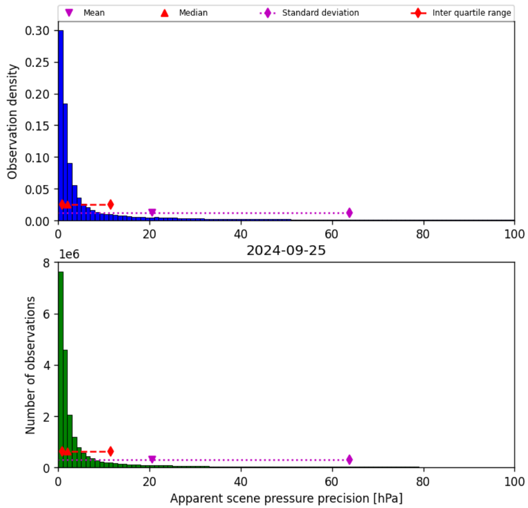
Figure 37: Histogram of “Apparent scene pressure precision” for 2024-09-24 to 2024-09-26
