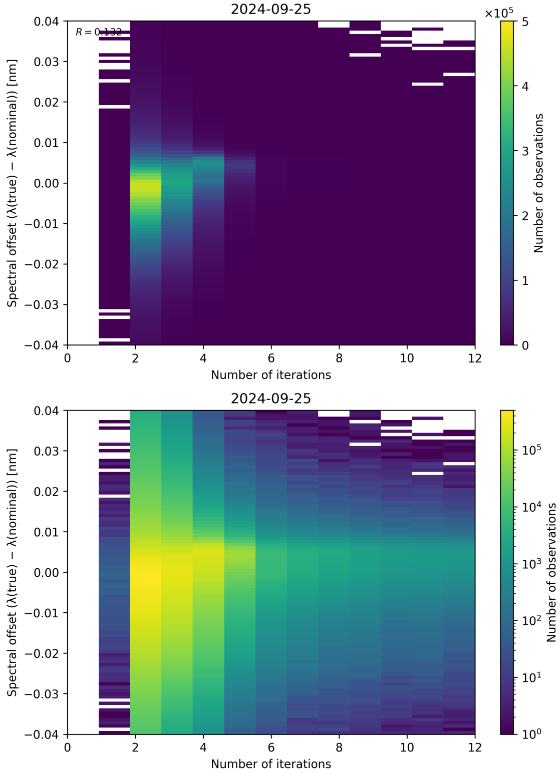
Figure 109: Scatter density plot of “Number of iterations” against “Spectral offset ( \lambda_{\text{true}} - \lambda_{\text{nominal}} )” for 2024-09-24 to 2024-09-26.
