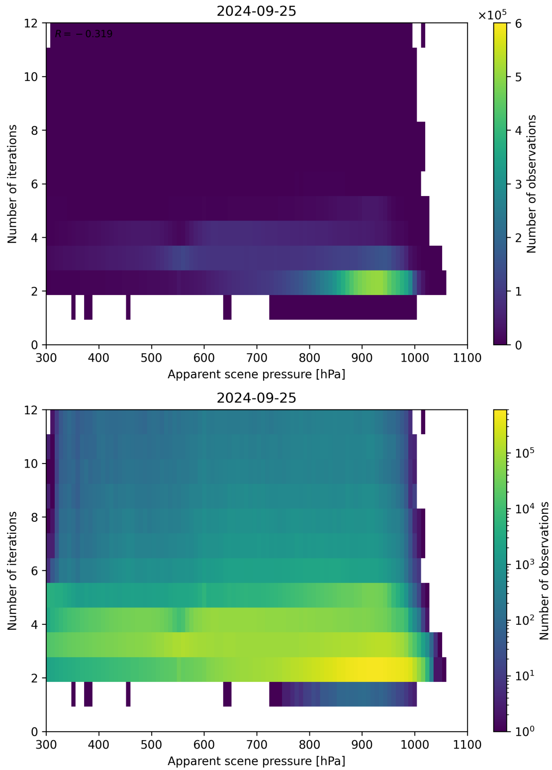
Figure 66: Scatter density plot of “Apparent scene pressure” against “Number of iterations” for 2024-09-24 to 2024-09-26.
