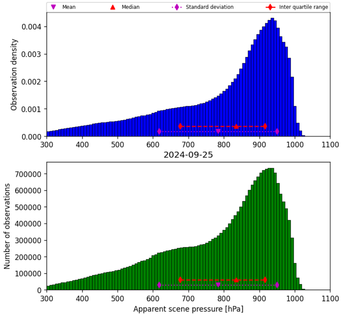
Figure 36: Histogram of “Apparent scene pressure” for 2024-09-24 to 2024-09-26
