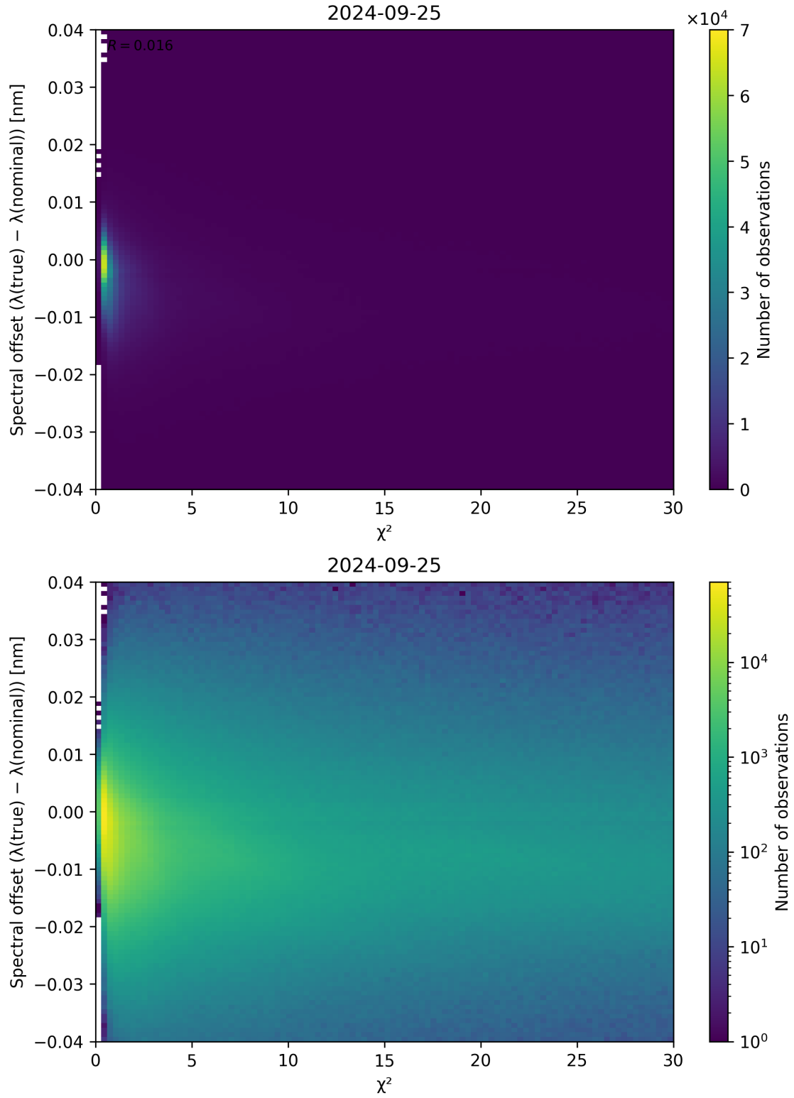
Figure 75: Scatter density plot of “ \chi^2 ” against “Spectral offset ( \lambda_{\text{true}} - \lambda_{\text{nominal}} )” for 2024-09-24 to 2024-09-26.
