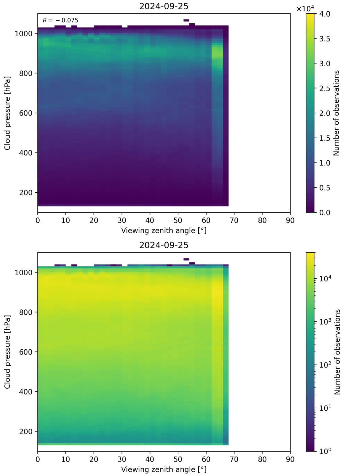
Figure 133: Scatter density plot of “Viewing zenith angle” against “Cloud pressure” for 2024-09-24 to 2024-09-26.
