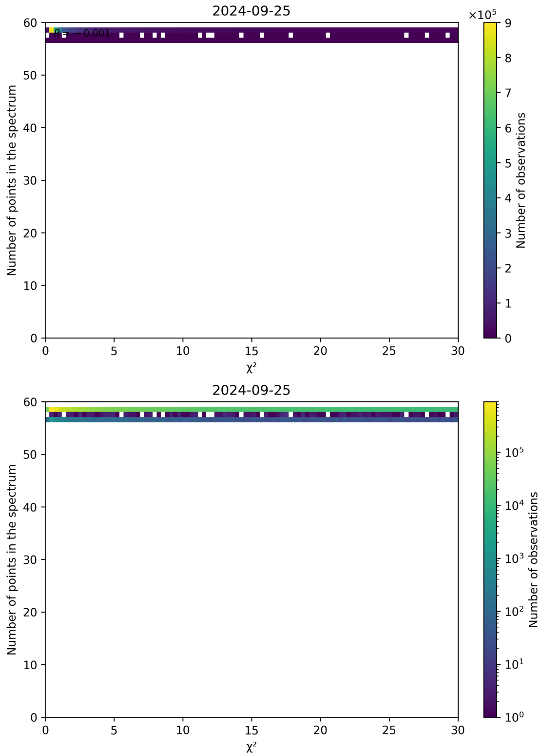
Figure 74: Scatter density plot of " \chi^2 " against "Number of points in the spectrum" for 2024-09-24 to 2024-09-26.
