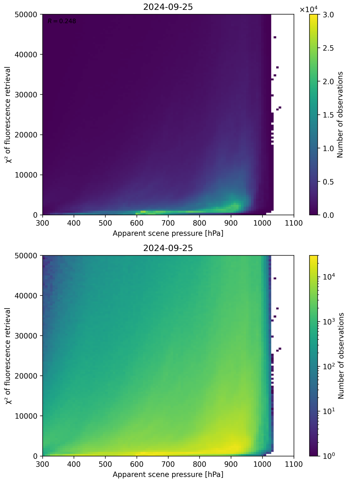
Figure 64: Scatter density plot of “Apparent scene pressure” against “ \chi^2 of fluorescence retrieval” for 2024-09-24 to 2024-09-26.
