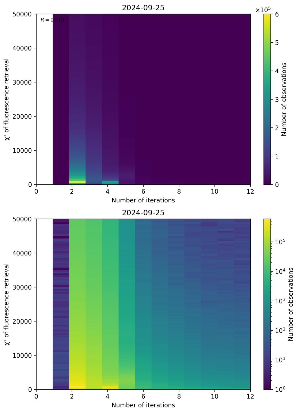
Figure 106: Scatter density plot of “Number of iterations” against “ \chi^2 of fluorescence retrieval” for 2024-09-24 to 2024-09-26.
