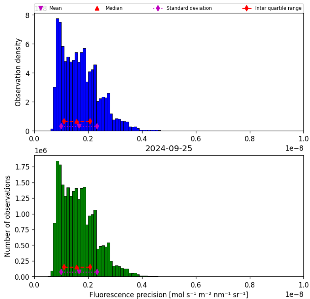
Figure 41: Histogram of “Fluorescence precision” for 2024-09-24 to 2024-09-26
