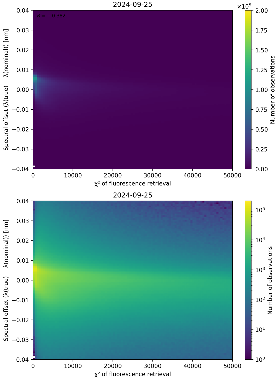
Figure 72: Scatter density plot of “ \chi^2 of fluorescence retrieval” against “Spectral offset ( \lambda_{\text{true}} - \lambda_{\text{nominal}} )” for 2024-09-24 to 2024-09-26.
