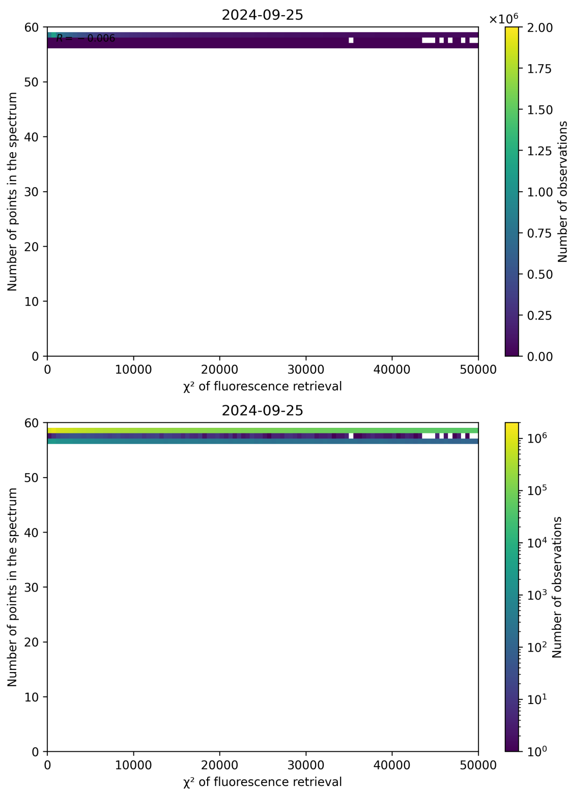
Figure 71: Scatter density plot of “ \chi^2 of fluorescence retrieval” against “Number of points in the spectrum” for 2024-09-24 to 2024-09-26.
