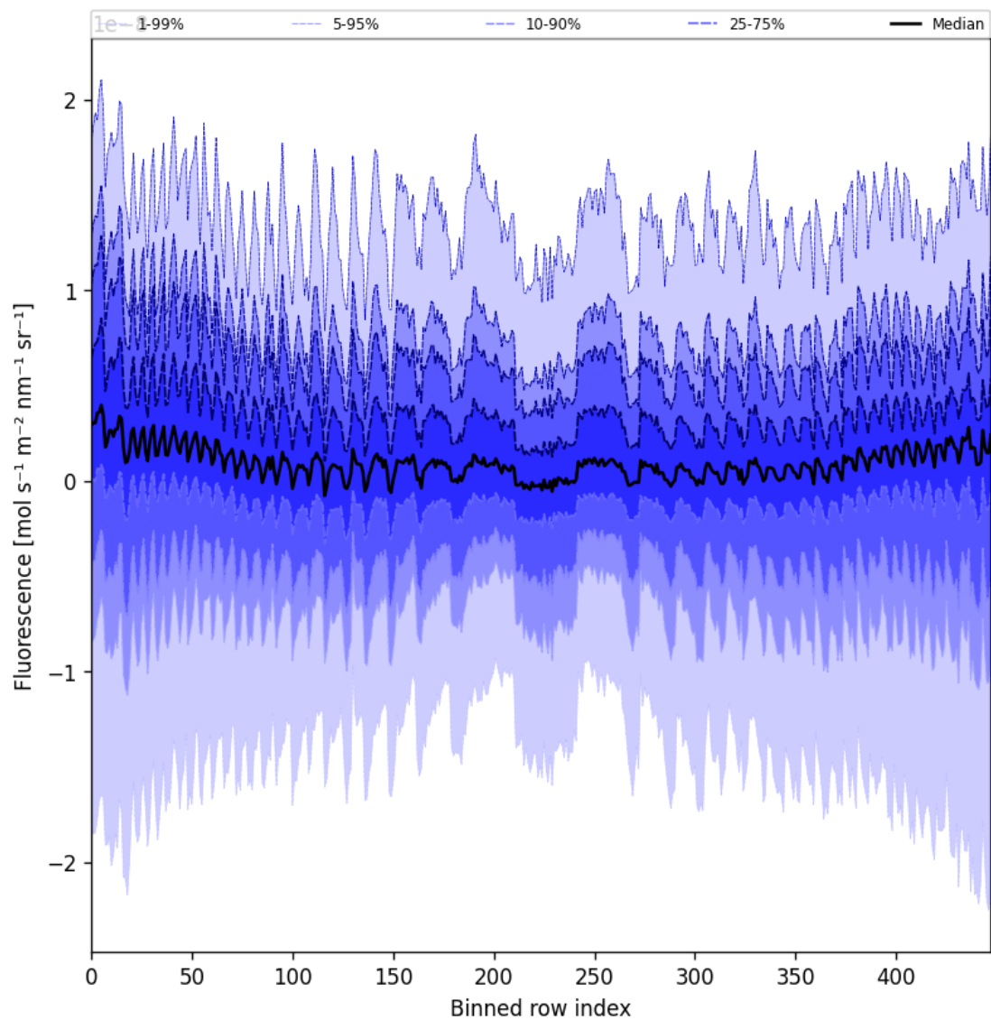
Figure 57: Along track statistics of “Fluorescence” for 2024-09-24 to 2024-09-26
