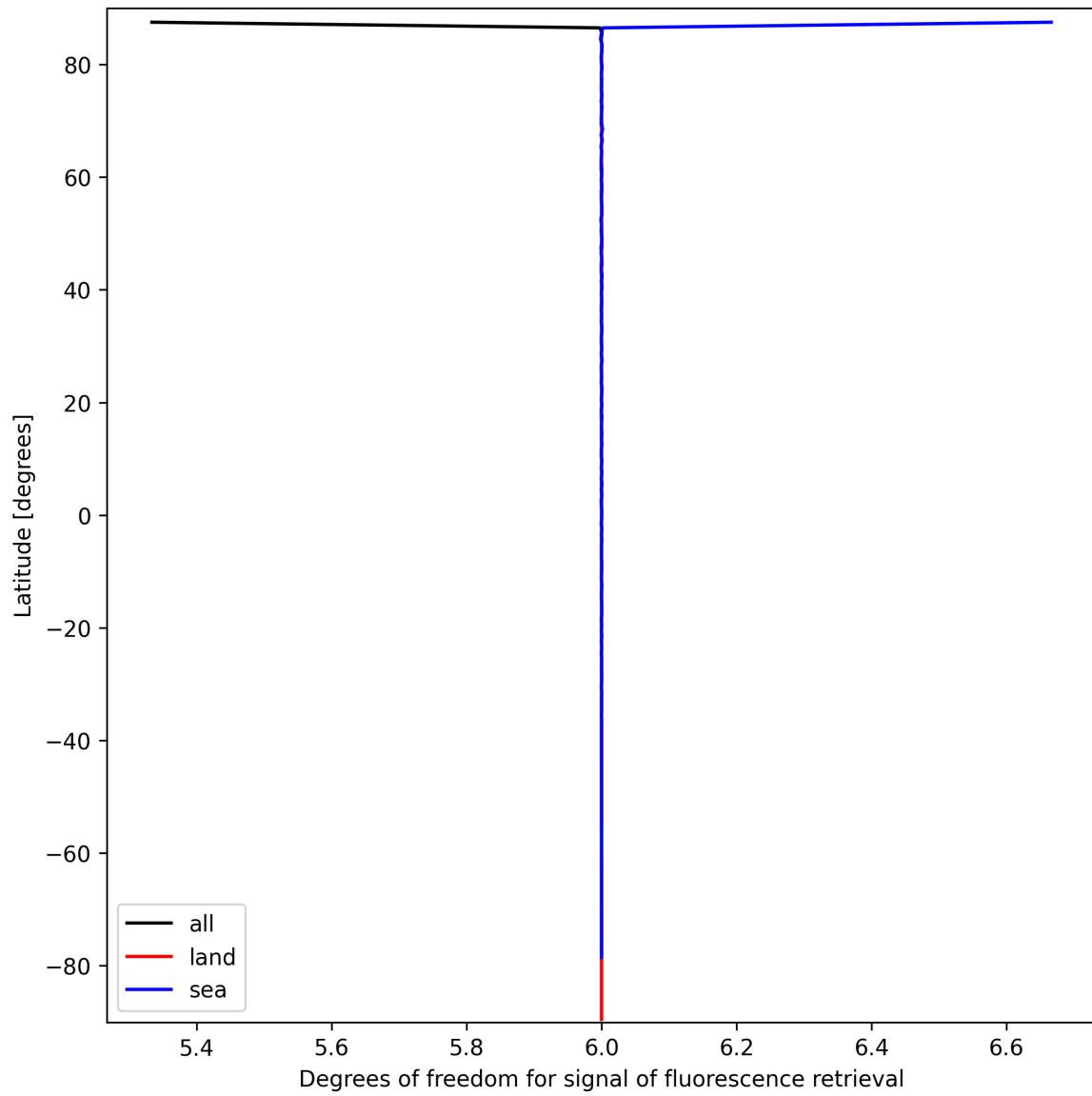
Figure 26: Zonal average of “Degrees of freedom for signal of fluorescence retrieval” for 2024-09-24 to 2024-09-26.
