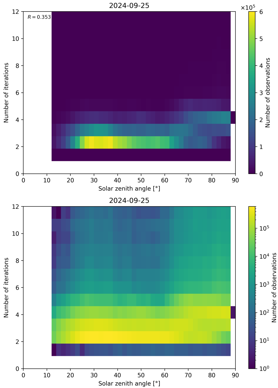
Figure 125: Scatter density plot of “Solar zenith angle” against “Number of iterations” for 2024-09-24 to 2024-09-26.
