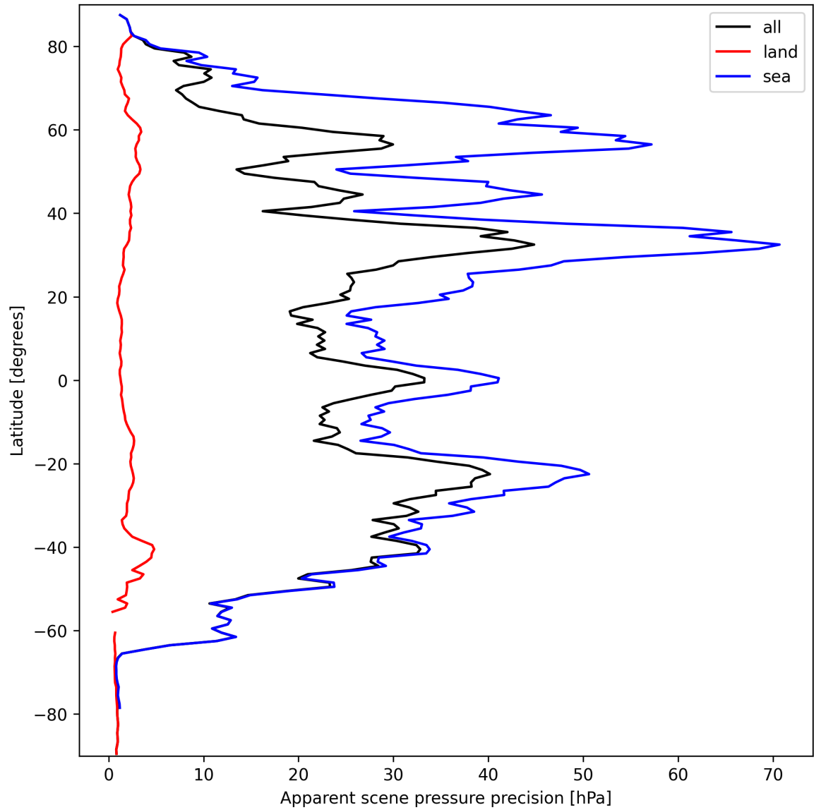
Figure 20: Zonal average of “Apparent scene pressure precision” for 2024-09-24 to 2024-09-26.
