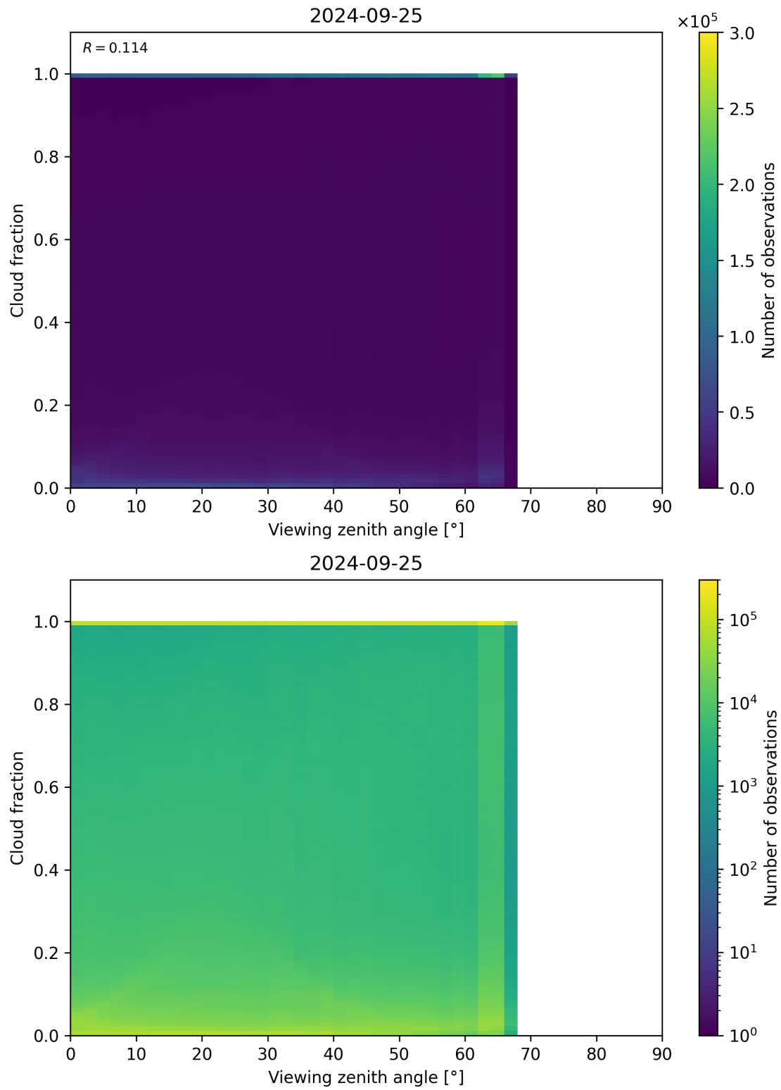
Figure 132: Scatter density plot of “Viewing zenith angle” against “Cloud fraction” for 2024-09-24 to 2024-09-26.
