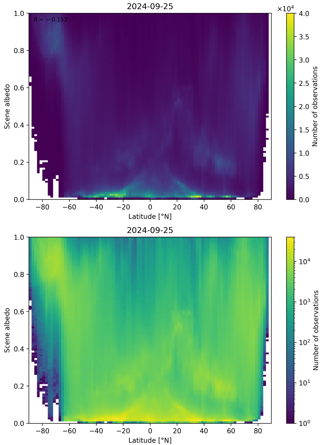
Figure 104: Scatter density plot of “Latitude” against “Scene albedo” for 2024-09-24 to 2024-09-26.
