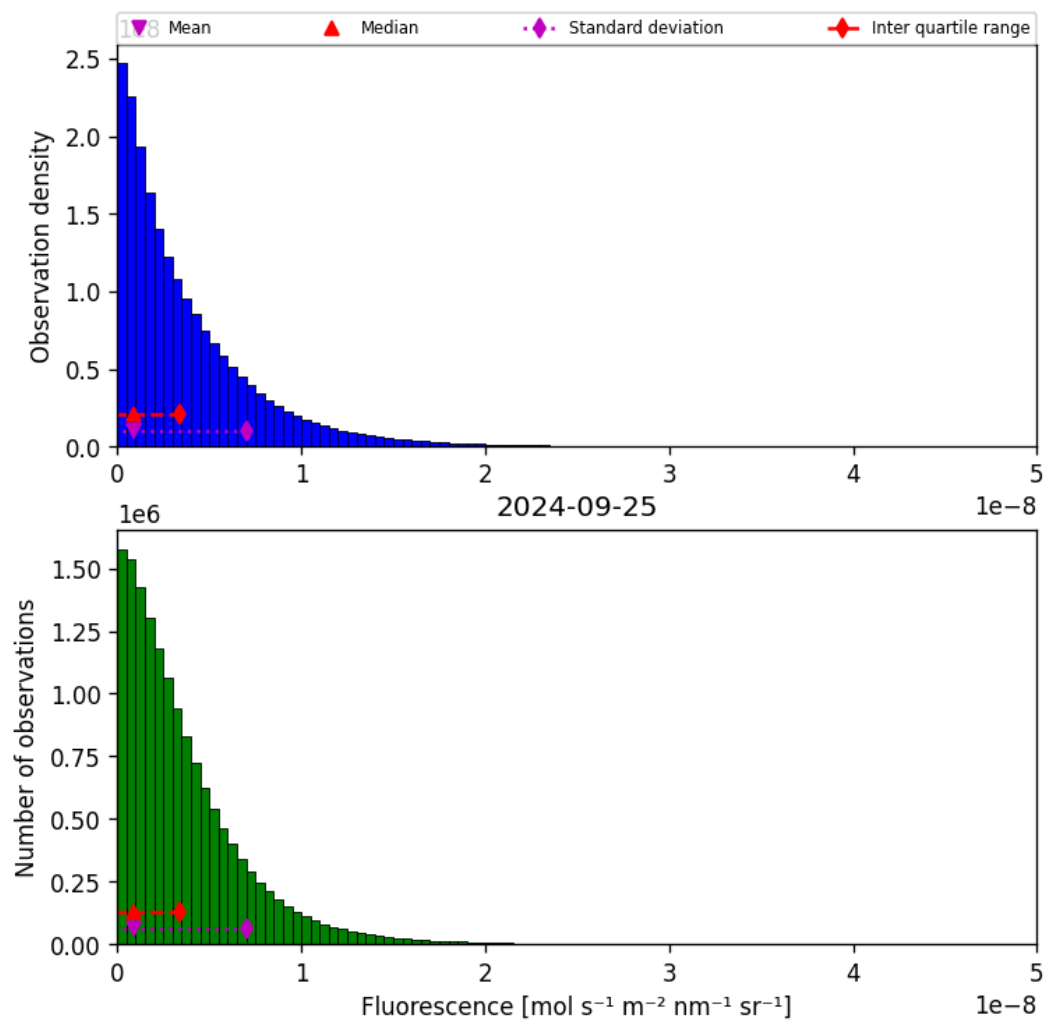
Figure 40: Histogram of “Fluorescence” for 2024-09-24 to 2024-09-26
