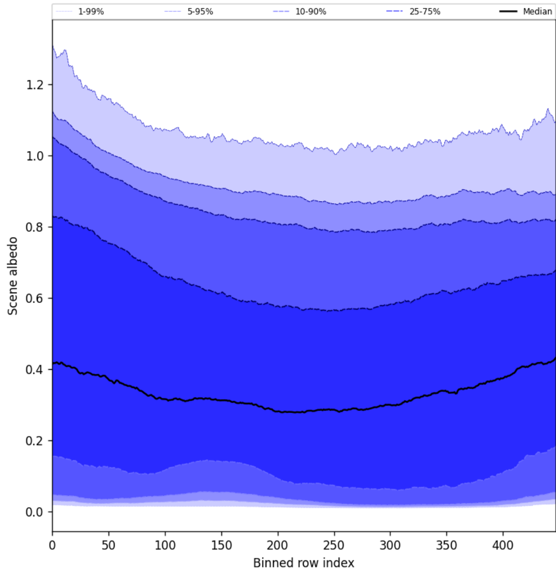
Figure 51: Along track statistics of “Scene albedo” for 2024-09-24 to 2024-09-26
