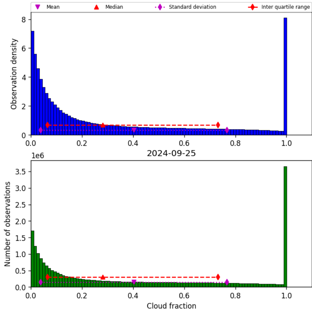
Figure 32: Histogram of “Cloud fraction” for 2024-09-24 to 2024-09-26
