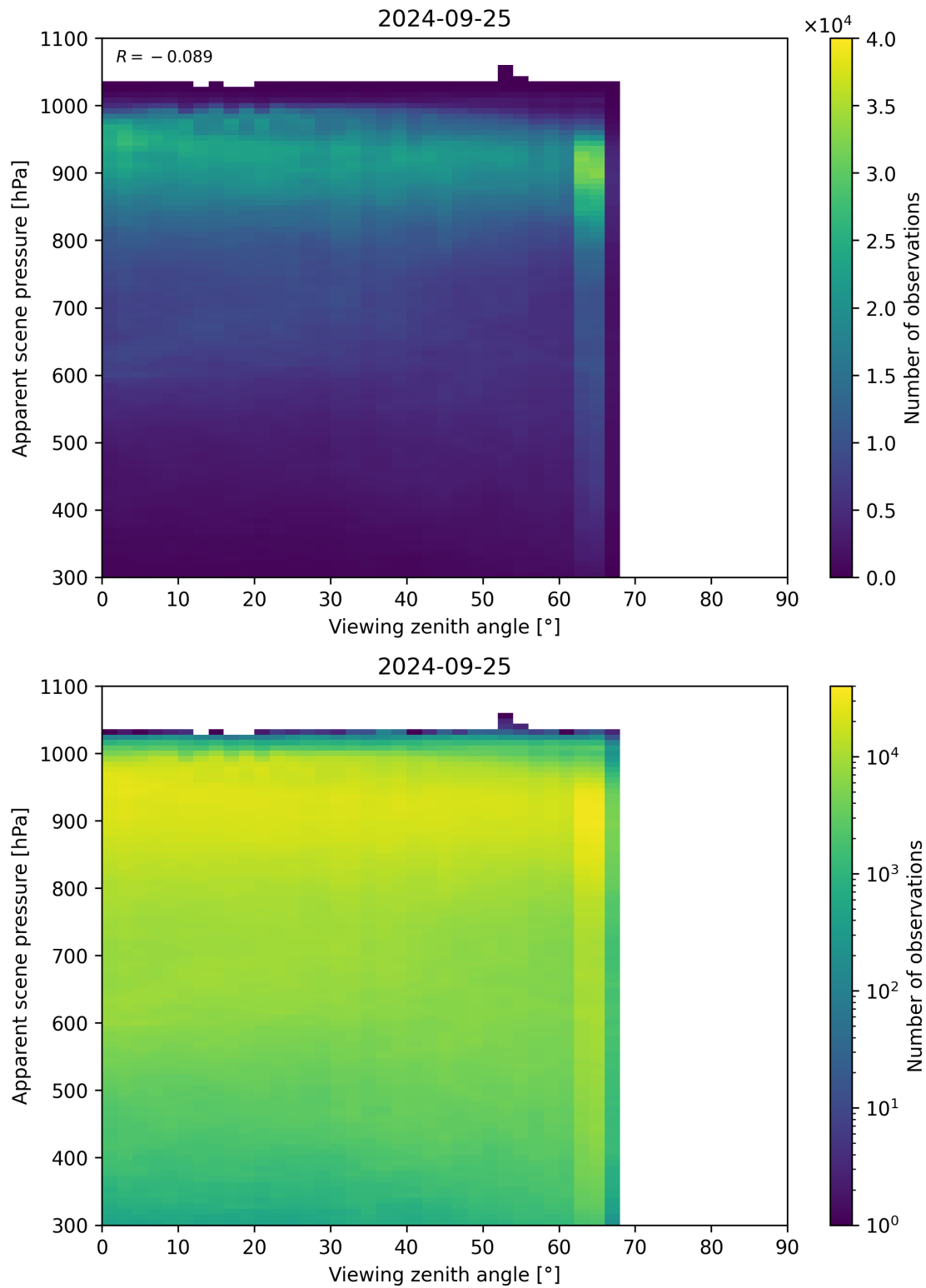
Figure 129: Scatter density plot of “Viewing zenith angle” against “Apparent scene pressure” for 2024-09-24 to 2024-09-26.
