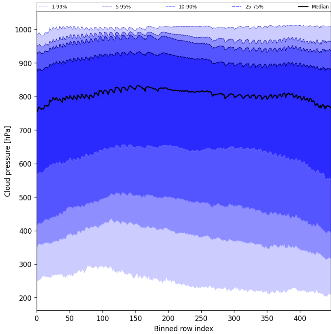
Figure 47: Along track statistics of “Cloud pressure” for 2024-09-24 to 2024-09-26
