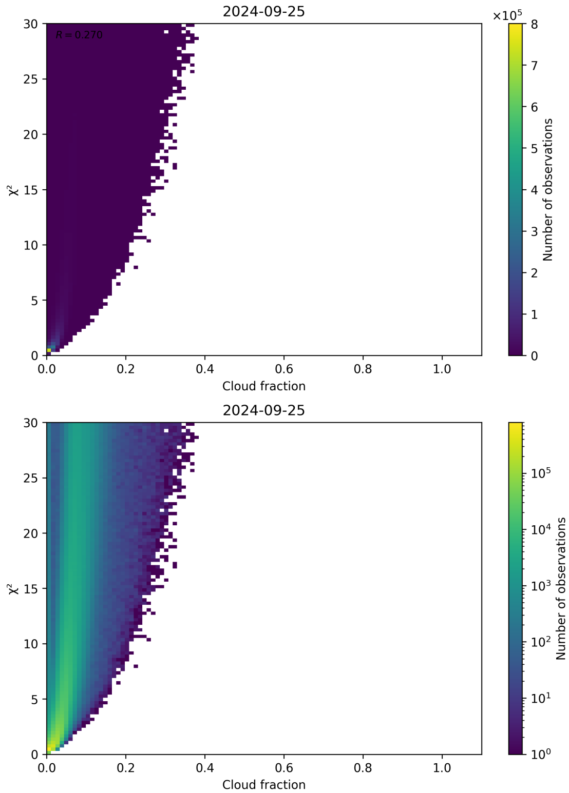
Figure 77: Scatter density plot of “Cloud fraction” against “ \chi^2 ” for 2024-09-24 to 2024-09-26.
