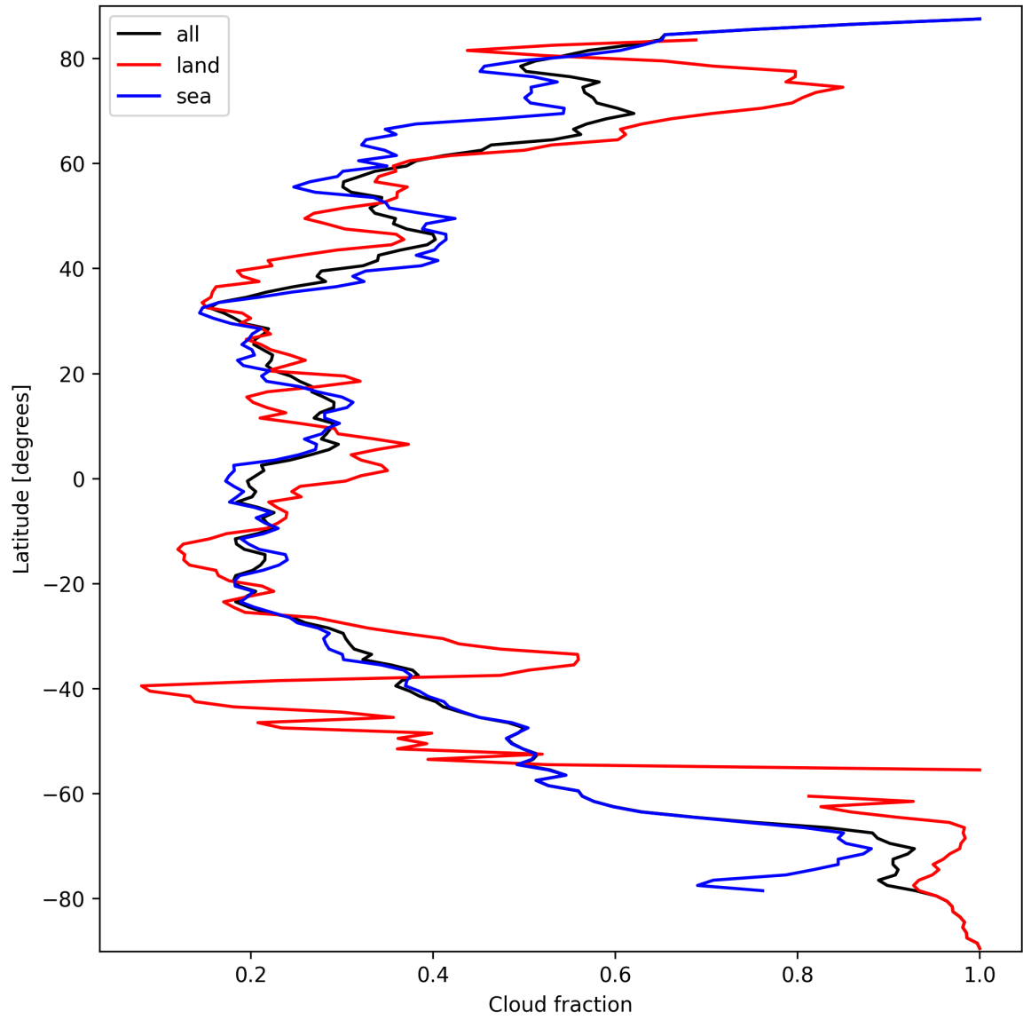
Figure 15: Zonal average of “Cloud fraction” for 2024-09-24 to 2024-09-26.
