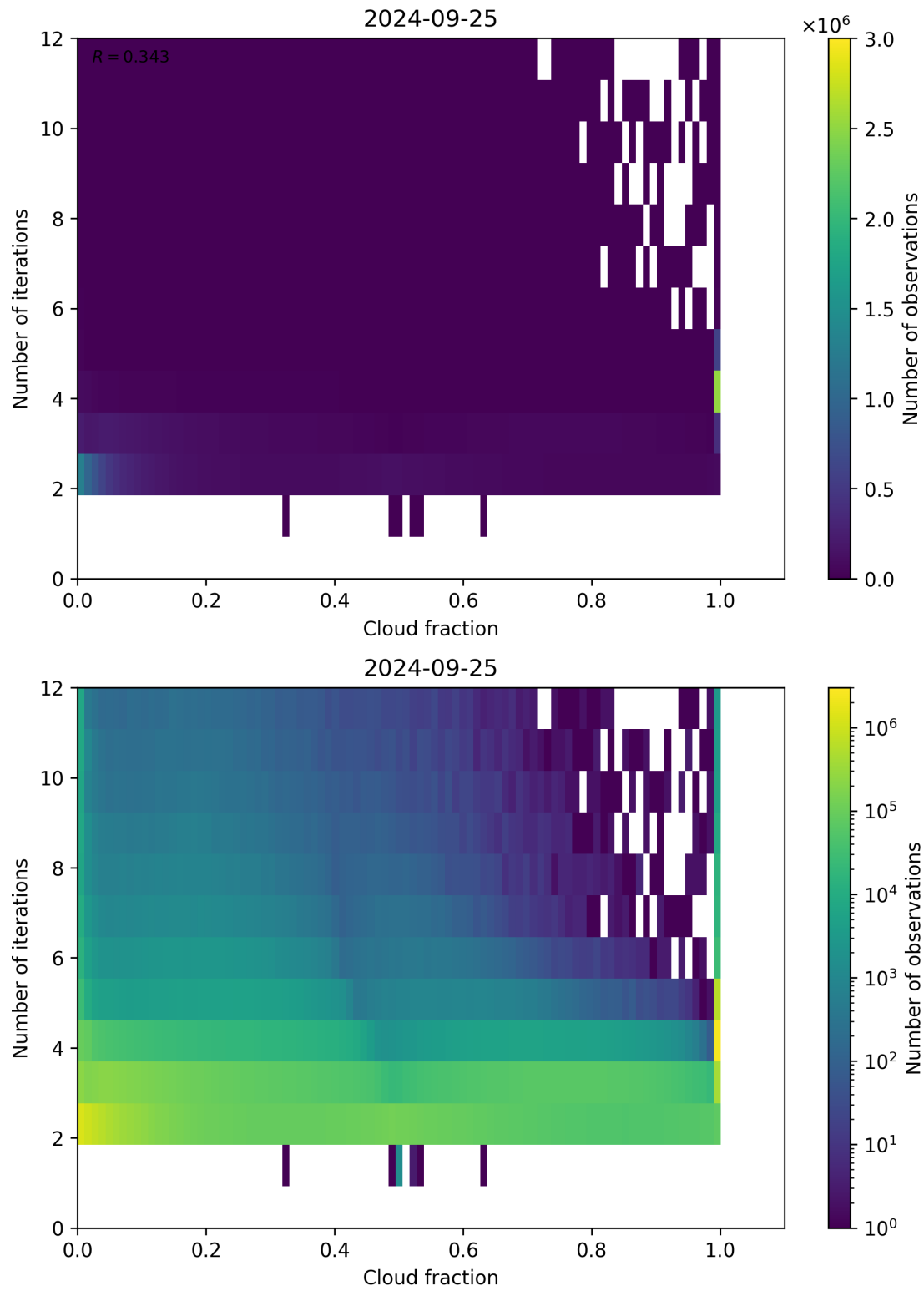
Figure 80: Scatter density plot of “Cloud fraction” against “Number of iterations” for 2024-09-24 to 2024-09-26.
