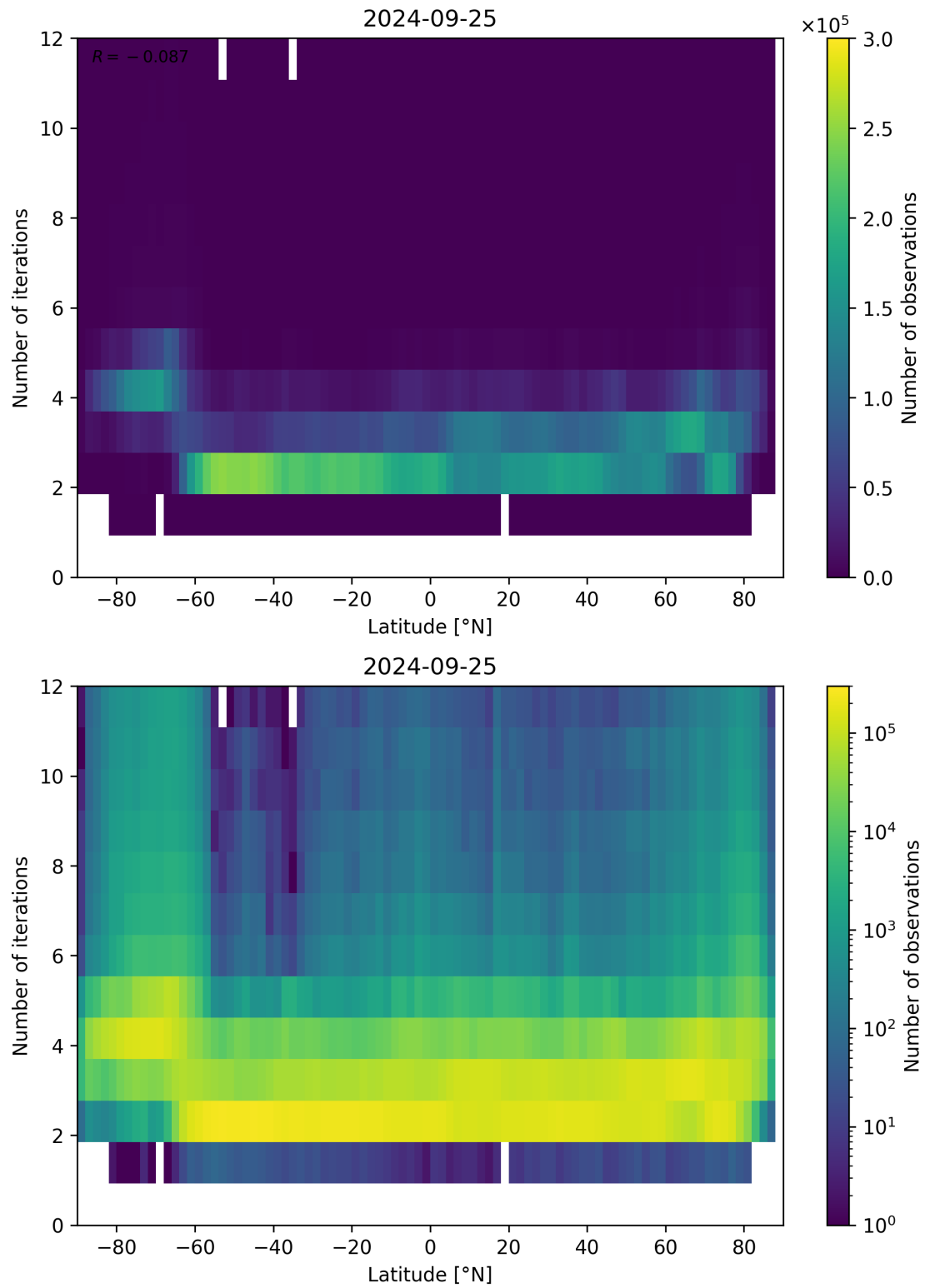
Figure 102: Scatter density plot of “Latitude” against “Number of iterations” for 2024-09-24 to 2024-09-26.
