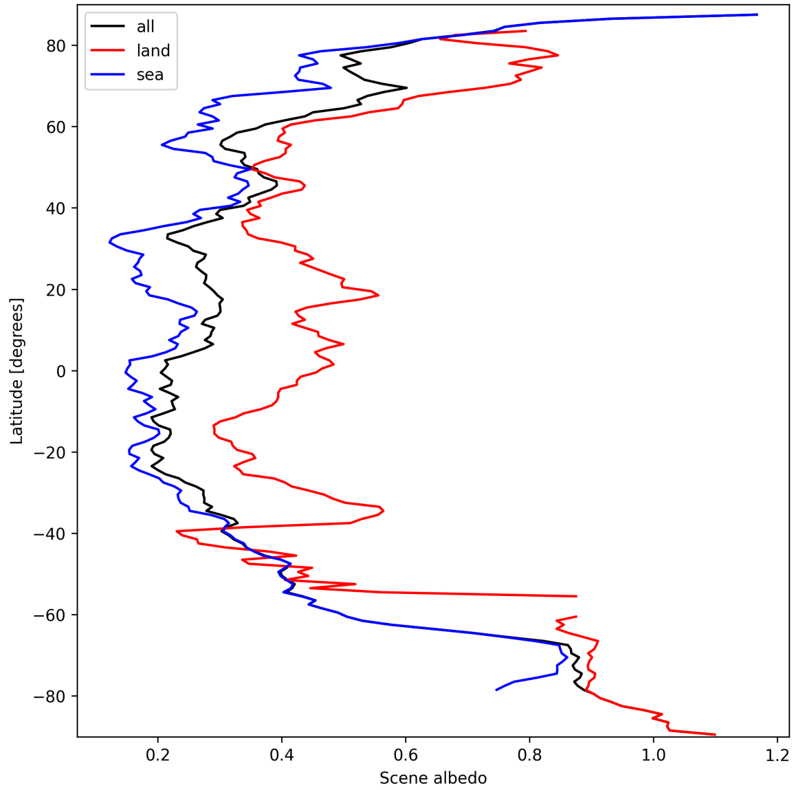
Figure 17: Zonal average of “Scene albedo” for 2024-09-24 to 2024-09-26.
