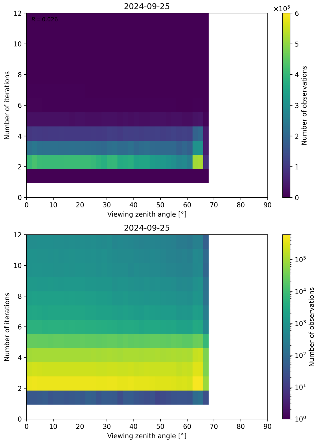
Figure 136: Scatter density plot of “Viewing zenith angle” against “Number of iterations” for 2024-09-24 to 2024-09-26.
