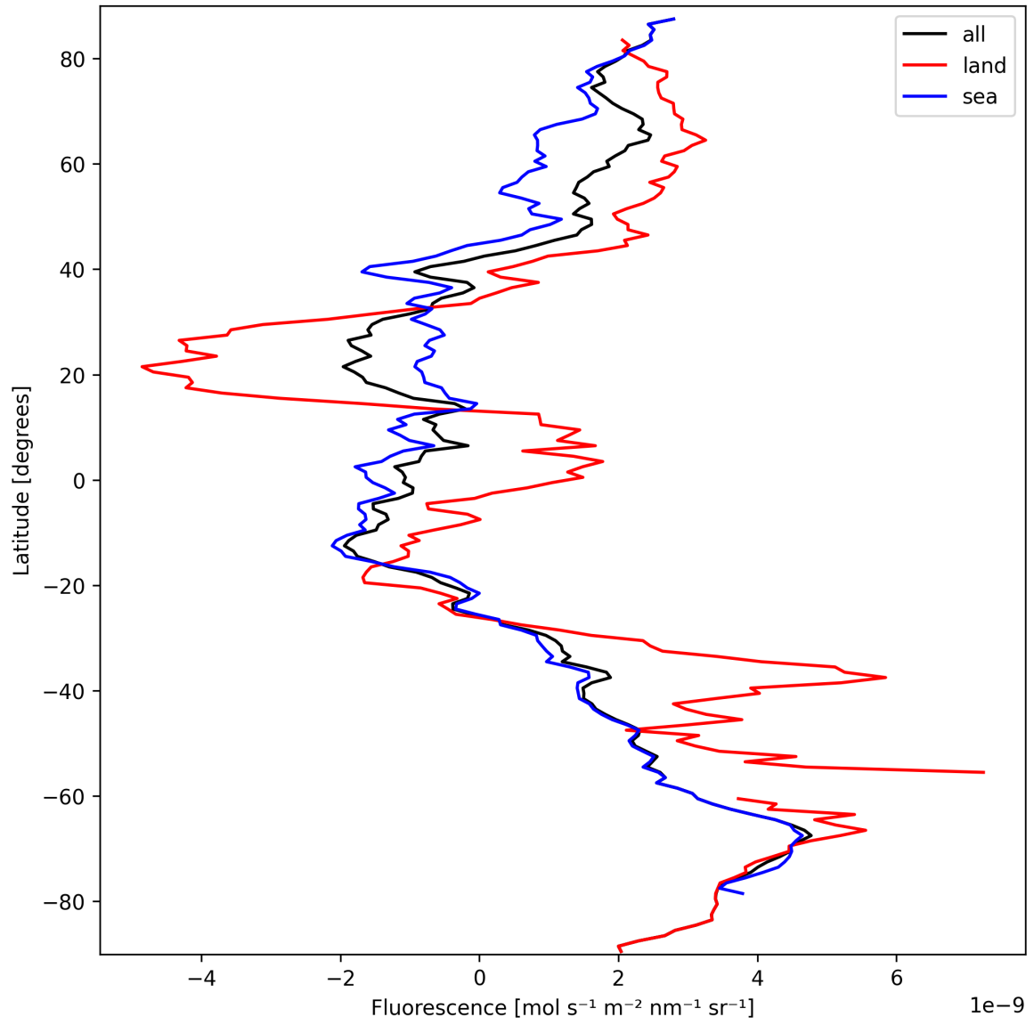
Figure 23: Zonal average of “Fluorescence” for 2024-09-24 to 2024-09-26.
