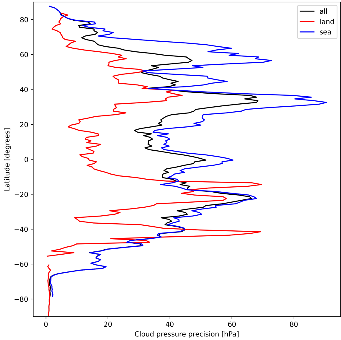
Figure 14: Zonal average of “Cloud pressure precision” for 2024-09-24 to 2024-09-26.
