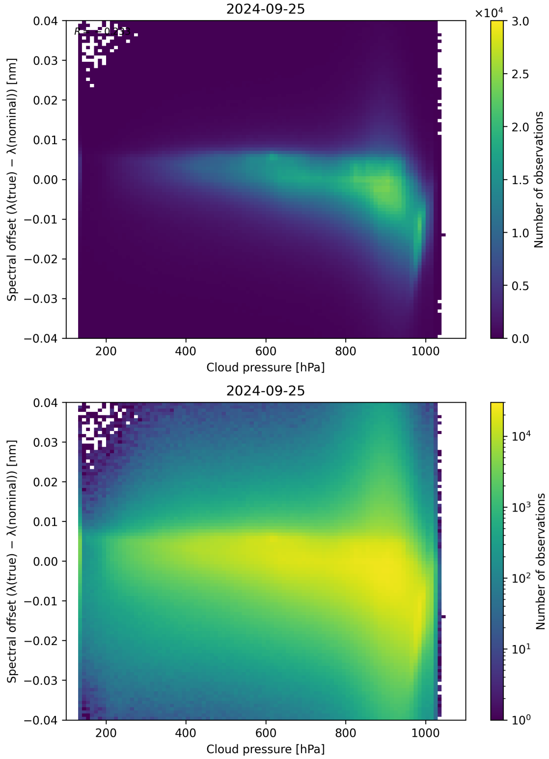
Figure 92: Scatter density plot of “Cloud pressure” against “Spectral offset ( \lambda_{\text{true}} - \lambda_{\text{nominal}} )” for 2024-09-24 to 2024-09-26.
