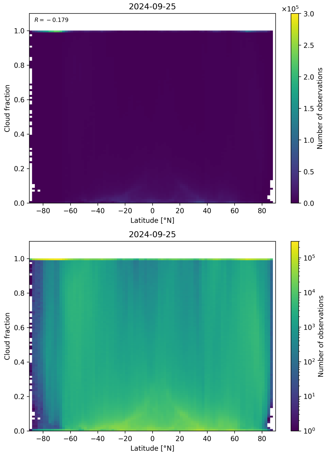
Figure 99: Scatter density plot of “Latitude” against “Cloud fraction” for 2024-09-24 to 2024-09-26.
