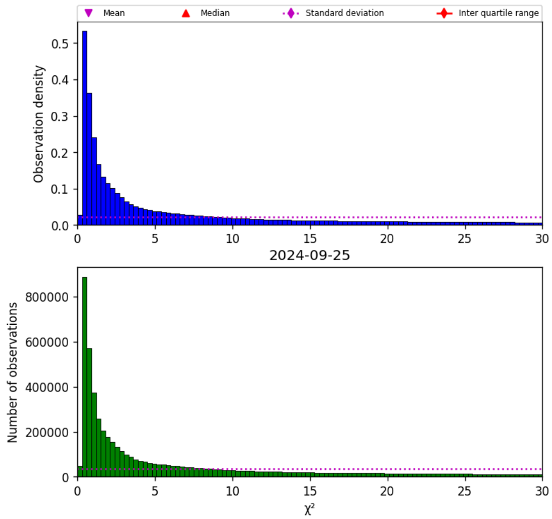
Figure 38: Histogram of “ \chi^2 ” for 2024-09-24 to 2024-09-26
