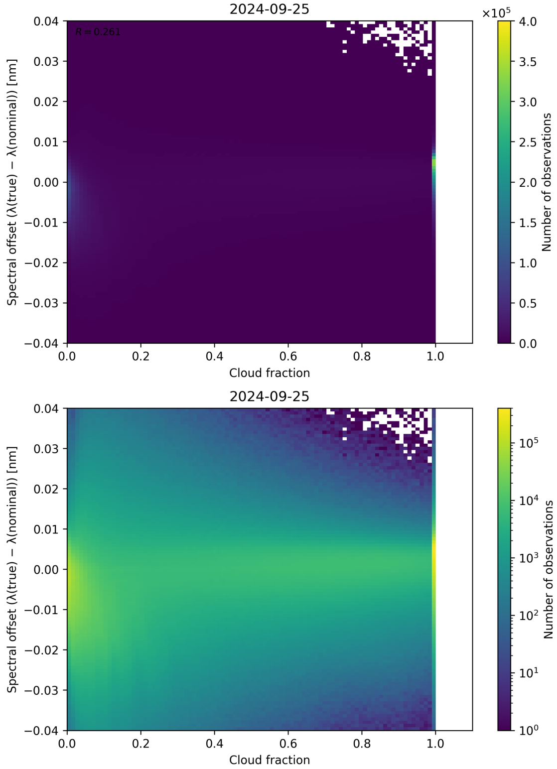
Figure 83: Scatter density plot of “Cloud fraction” against “Spectral offset ( \lambda_{\text{true}} - \lambda_{\text{nominal}} )” for 2024-09-24 to 2024-09-26.
