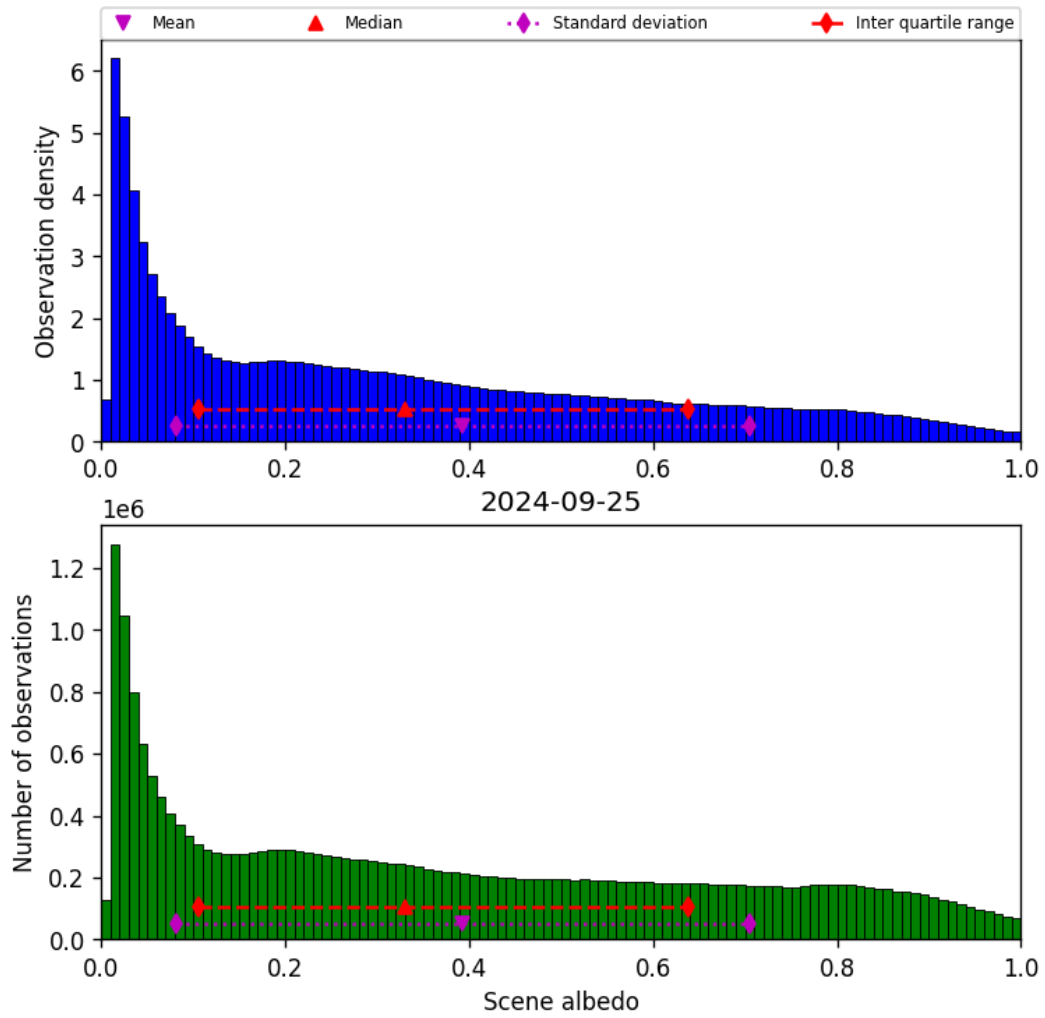
Figure 34: Histogram of “Scene albedo” for 2024-09-24 to 2024-09-26
