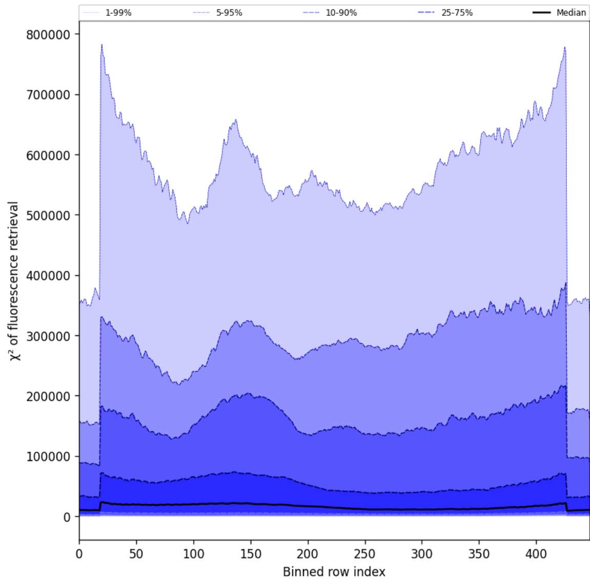
Figure 59: Along track statistics of “ \chi^2 of fluorescence retrieval” for 2024-09-24 to 2024-09-26
