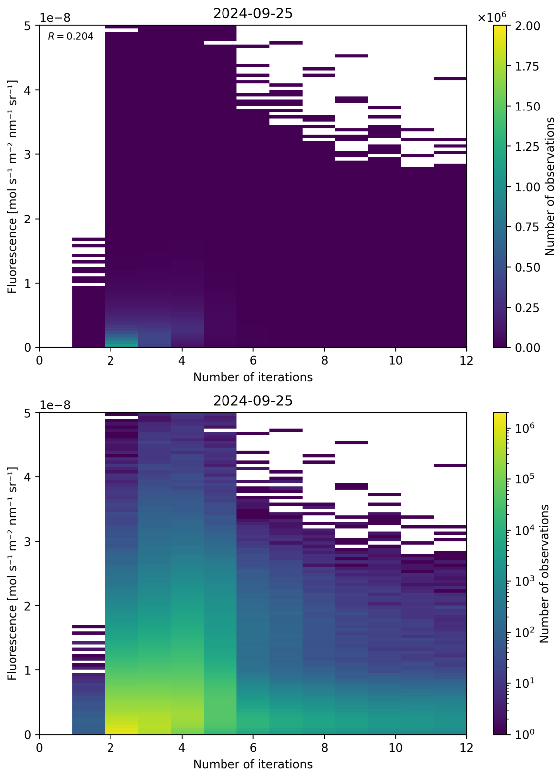
Figure 107: Scatter density plot of “Number of iterations” against “Fluorescence” for 2024-09-24 to 2024-09-26.
