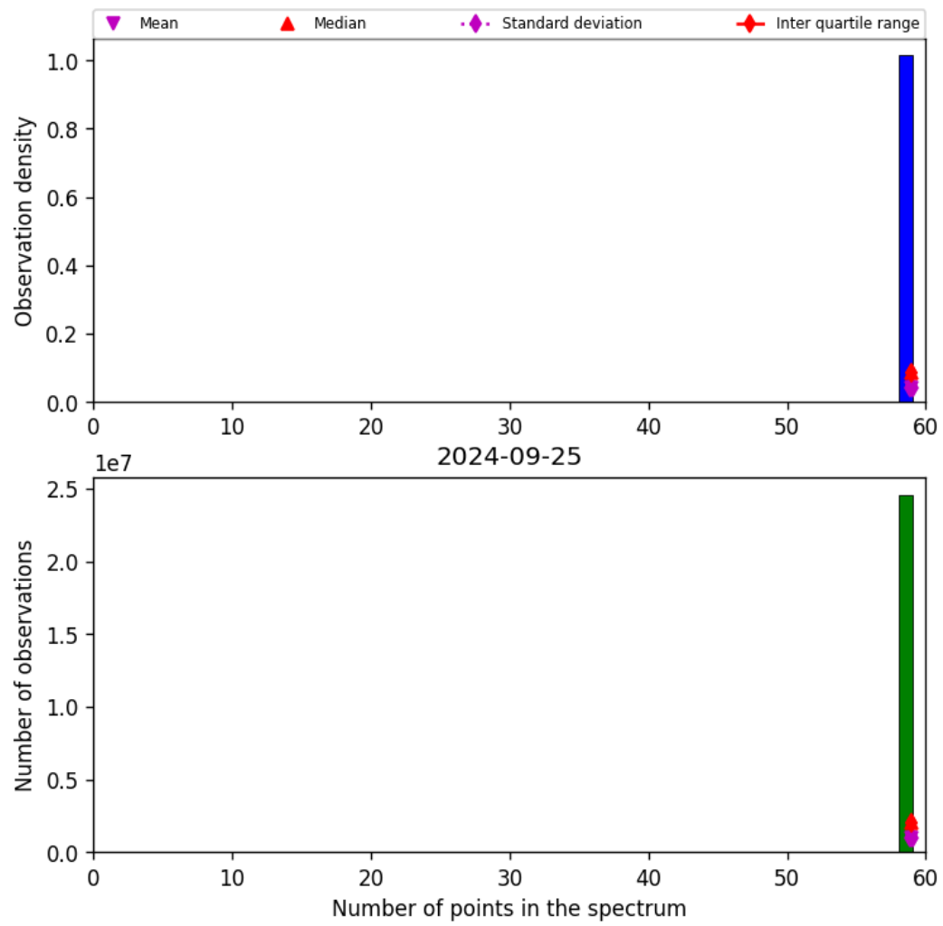
Figure 44: Histogram of “Number of points in the spectrum” for 2024-09-24 to 2024-09-26
