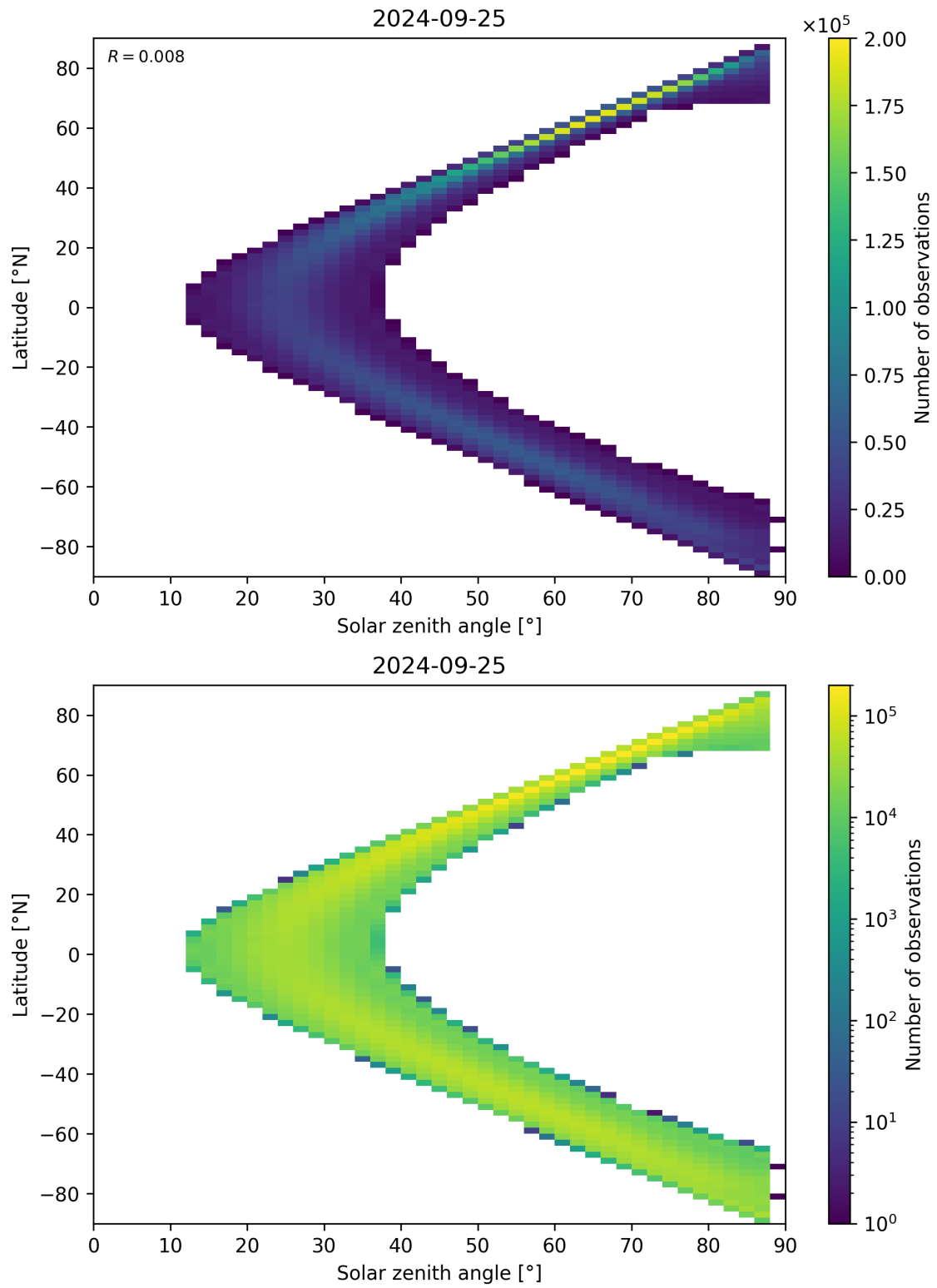
Figure 124: Scatter density plot of “Solar zenith angle” against “Latitude” for 2024-09-24 to 2024-09-26.
