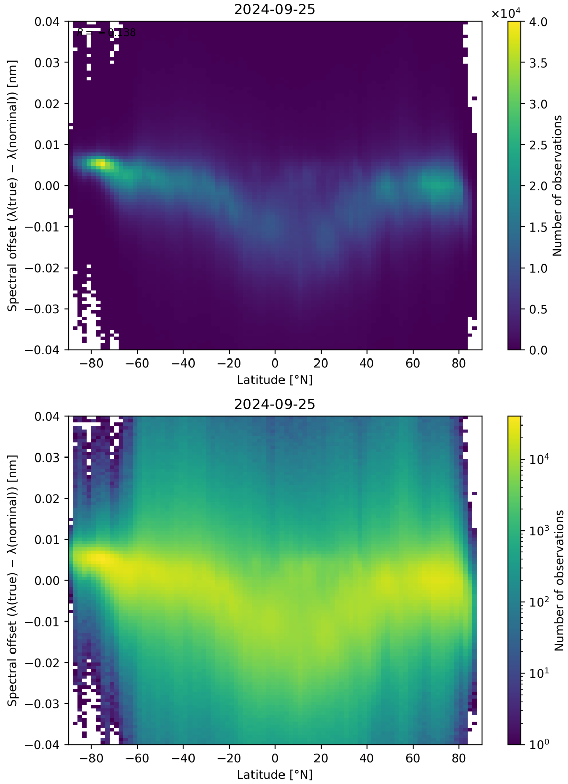
Figure 105: Scatter density plot of “Latitude” against “Spectral offset ( \lambda_{\text{true}} - \lambda_{\text{nominal}} )” for 2024-09-24 to 2024-09-26.
