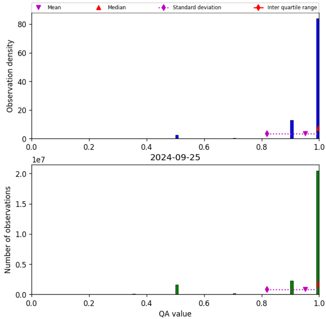
Figure 29: Histogram of “QA value” for 2024-09-24 to 2024-09-26
