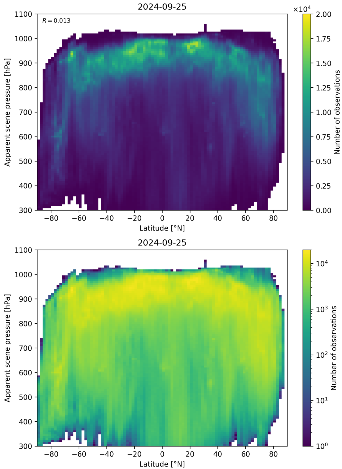
Figure 96: Scatter density plot of “Latitude” against “Apparent scene pressure” for 2024-09-24 to 2024-09-26.
