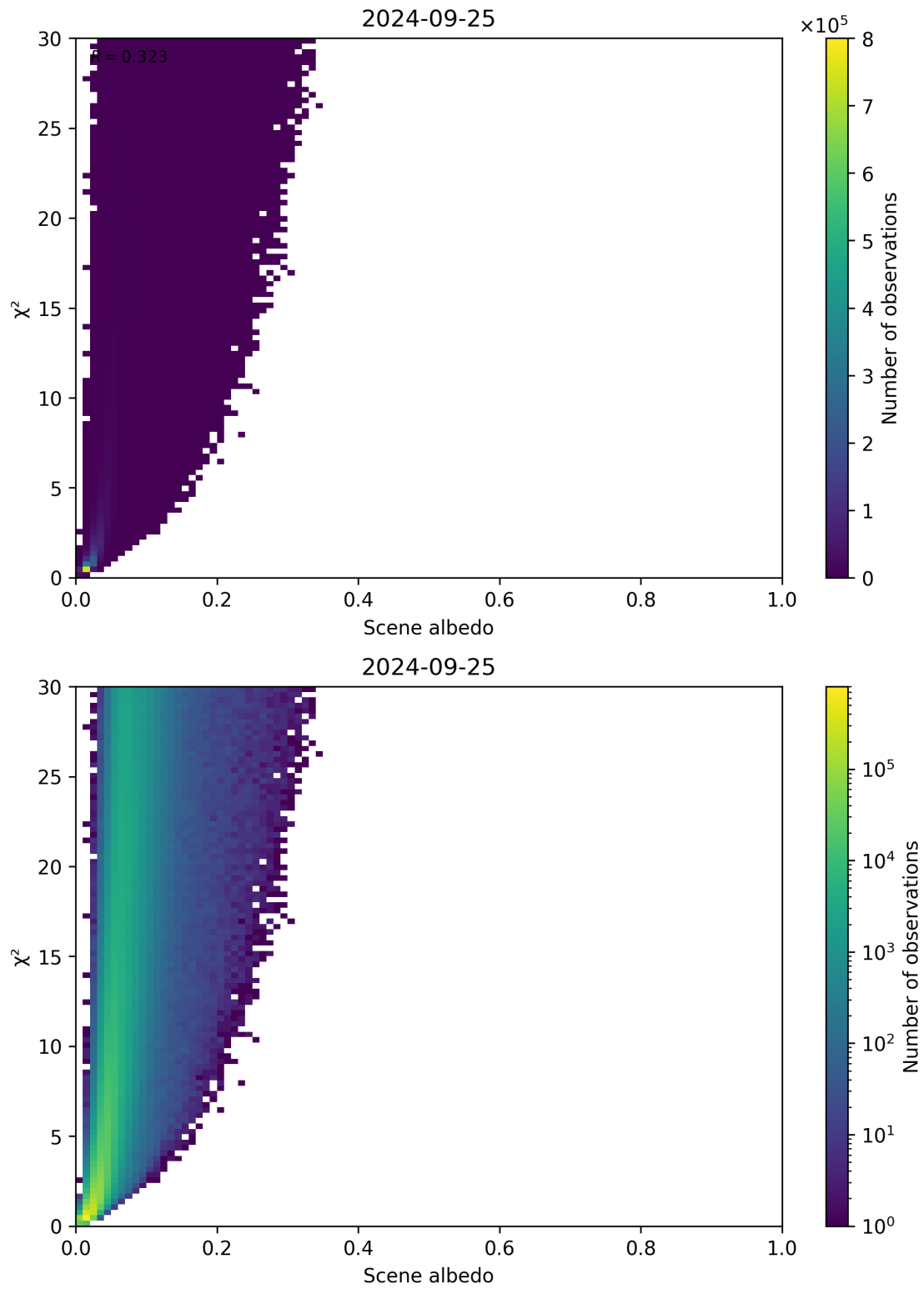
Figure 112: Scatter density plot of “Scene albedo” against “ \chi^2 ” for 2024-09-24 to 2024-09-26.
