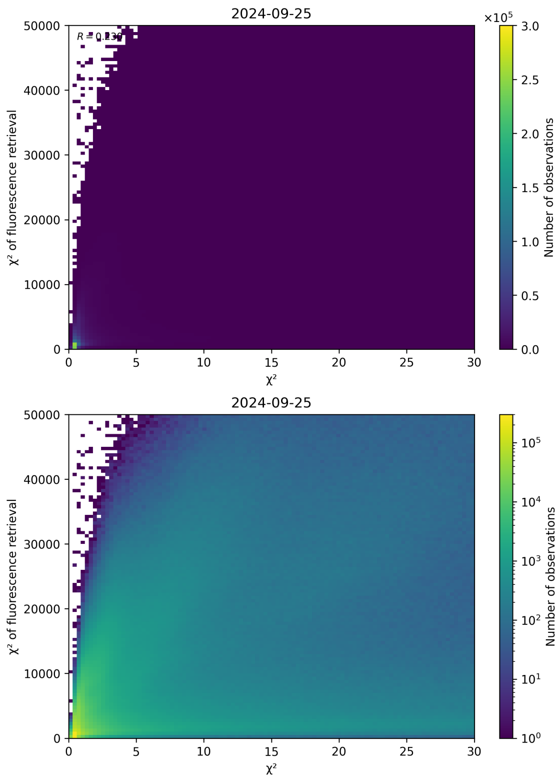
Figure 69: Scatter density plot of “ \chi^2 ” against “ \chi^2 of fluorescence retrieval” for 2024-09-24 to 2024-09-26.
