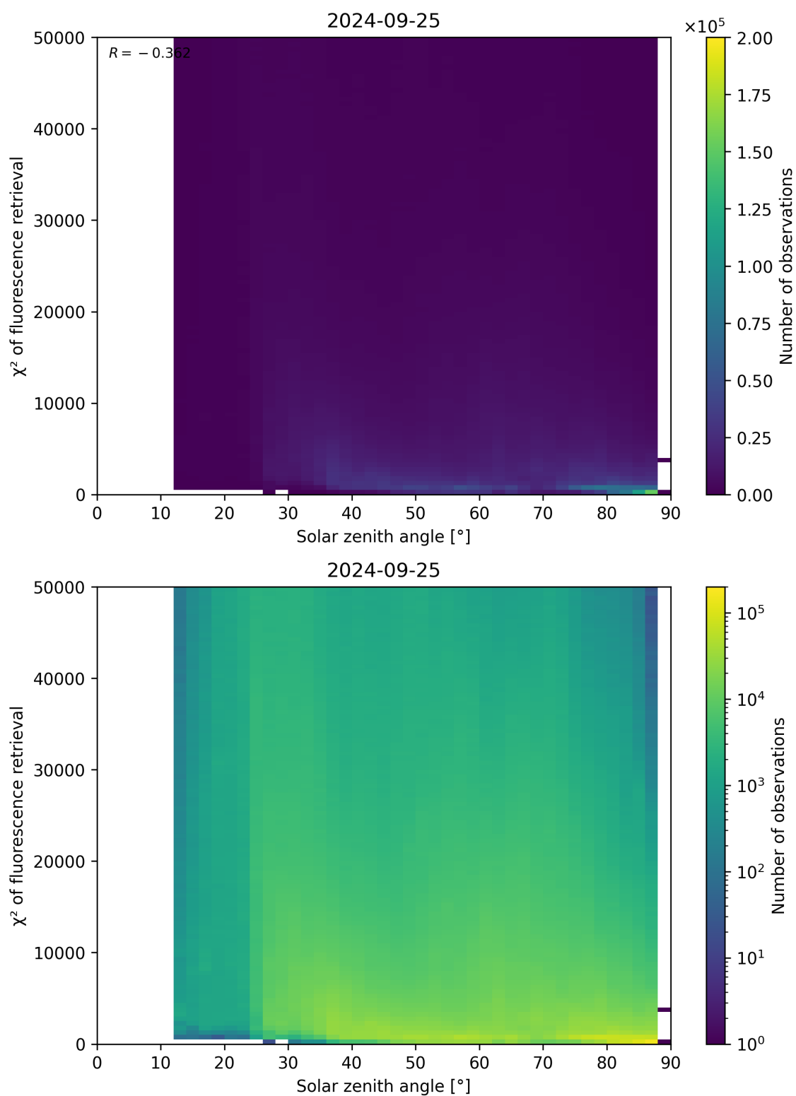
Figure 120: Scatter density plot of “Solar zenith angle” against “ \chi^2 of fluorescence retrieval” for 2024-09-24 to 2024-09-26.
