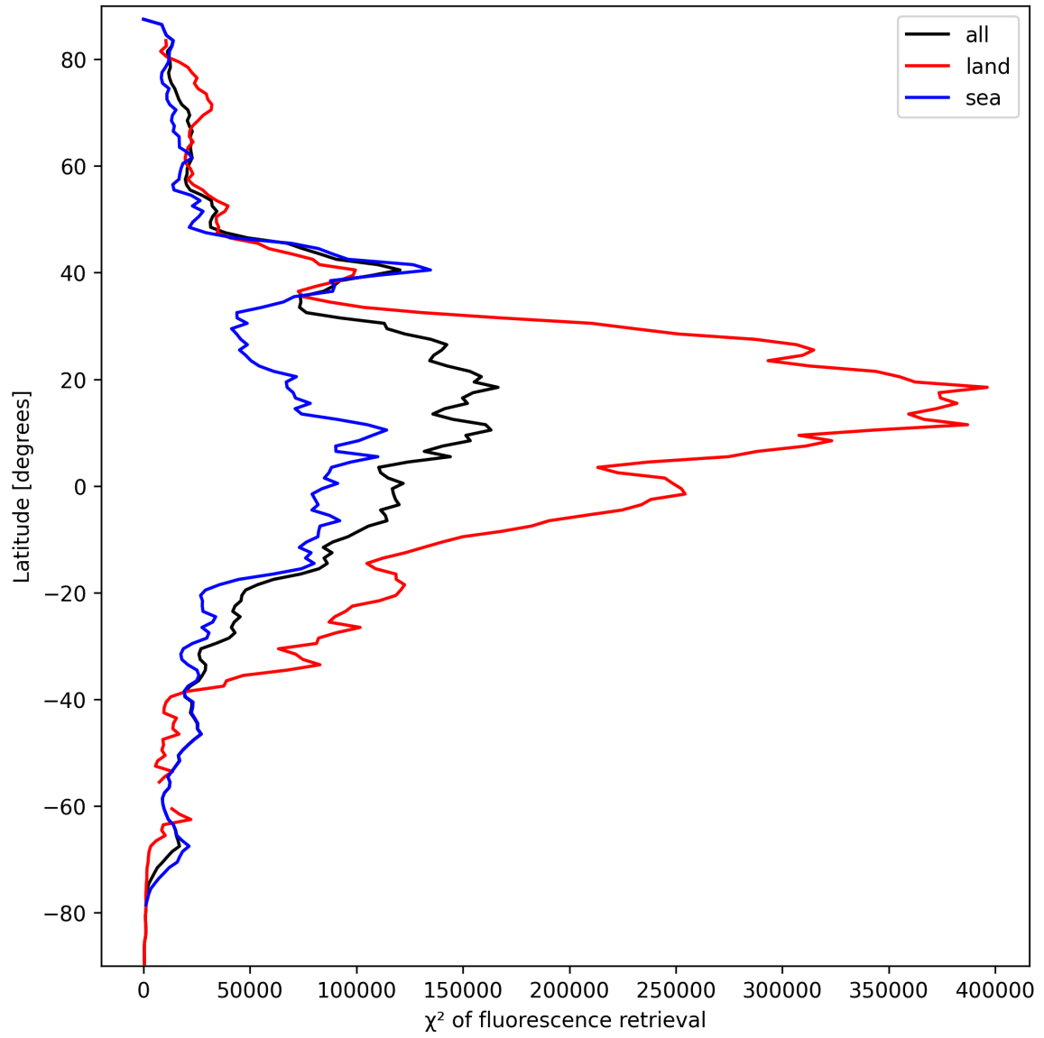
Figure 25: Zonal average of “ \chi^2 of fluorescence retrieval” for 2024-09-24 to 2024-09-26.
