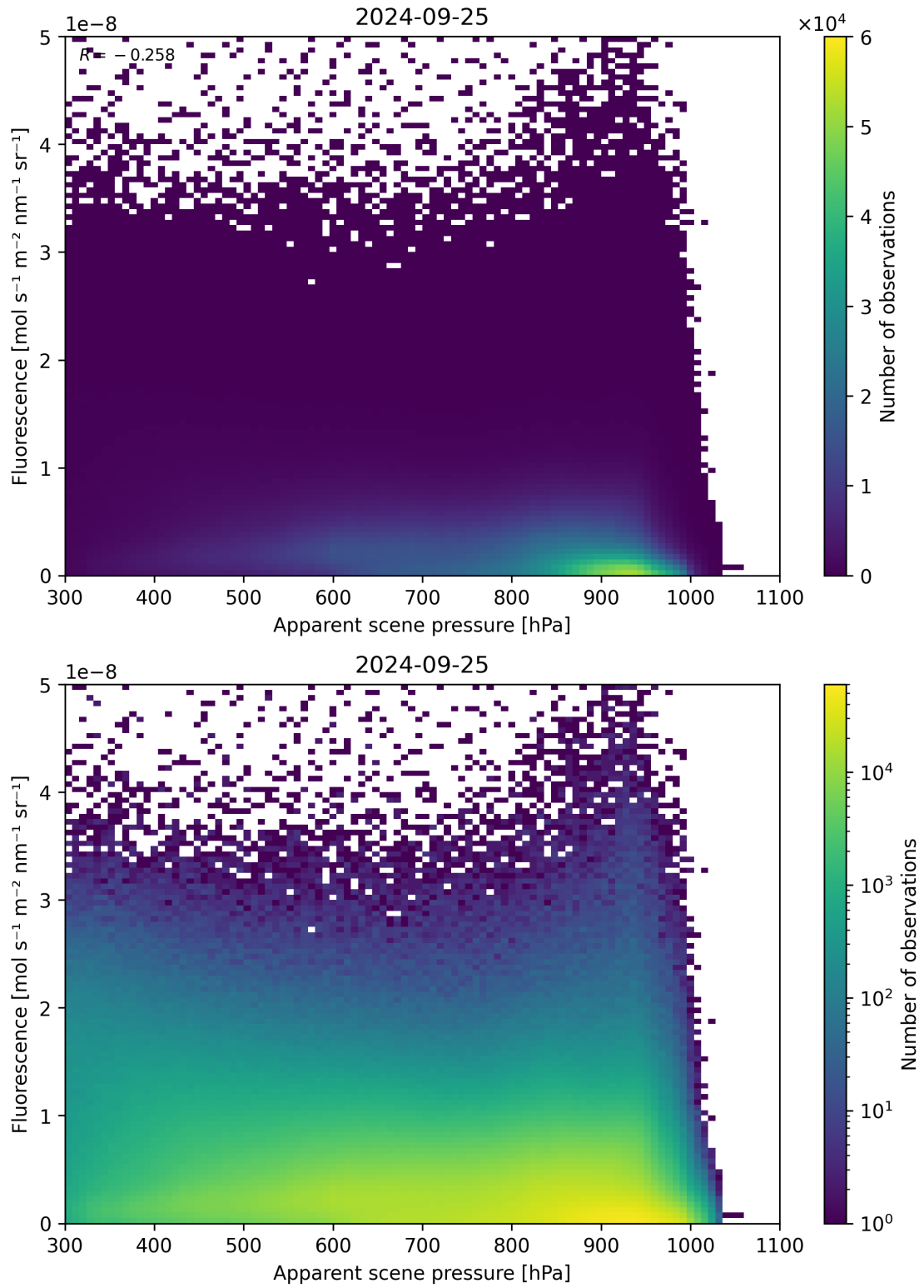
Figure 65: Scatter density plot of “Apparent scene pressure” against “Fluorescence” for 2024-09-24 to 2024-09-26.
