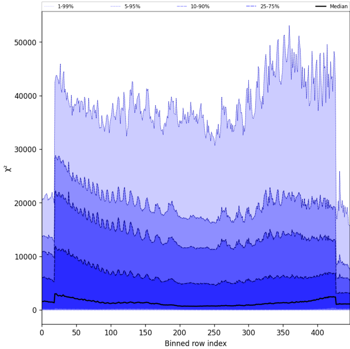
Figure 55: Along track statistics of “ \chi^2 ” for 2024-09-24 to 2024-09-26
