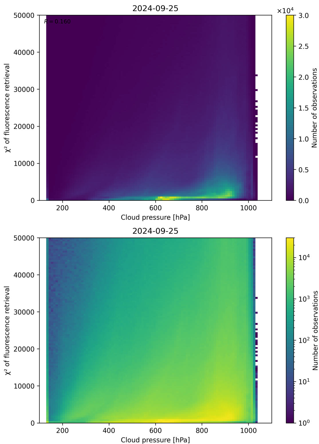
Figure 86: Scatter density plot of “Cloud pressure” against “ \chi^2 of fluorescence retrieval” for 2024-09-24 to 2024-09-26.
