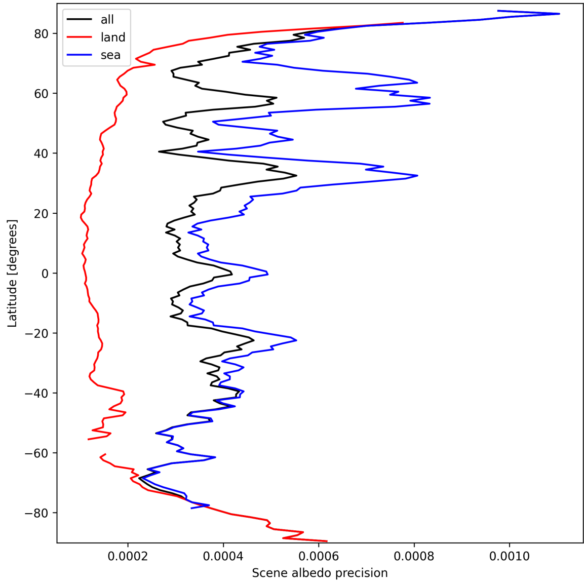
Figure 18: Zonal average of "Scene albedo precision" for 2024-09-24 to 2024-09-26.
