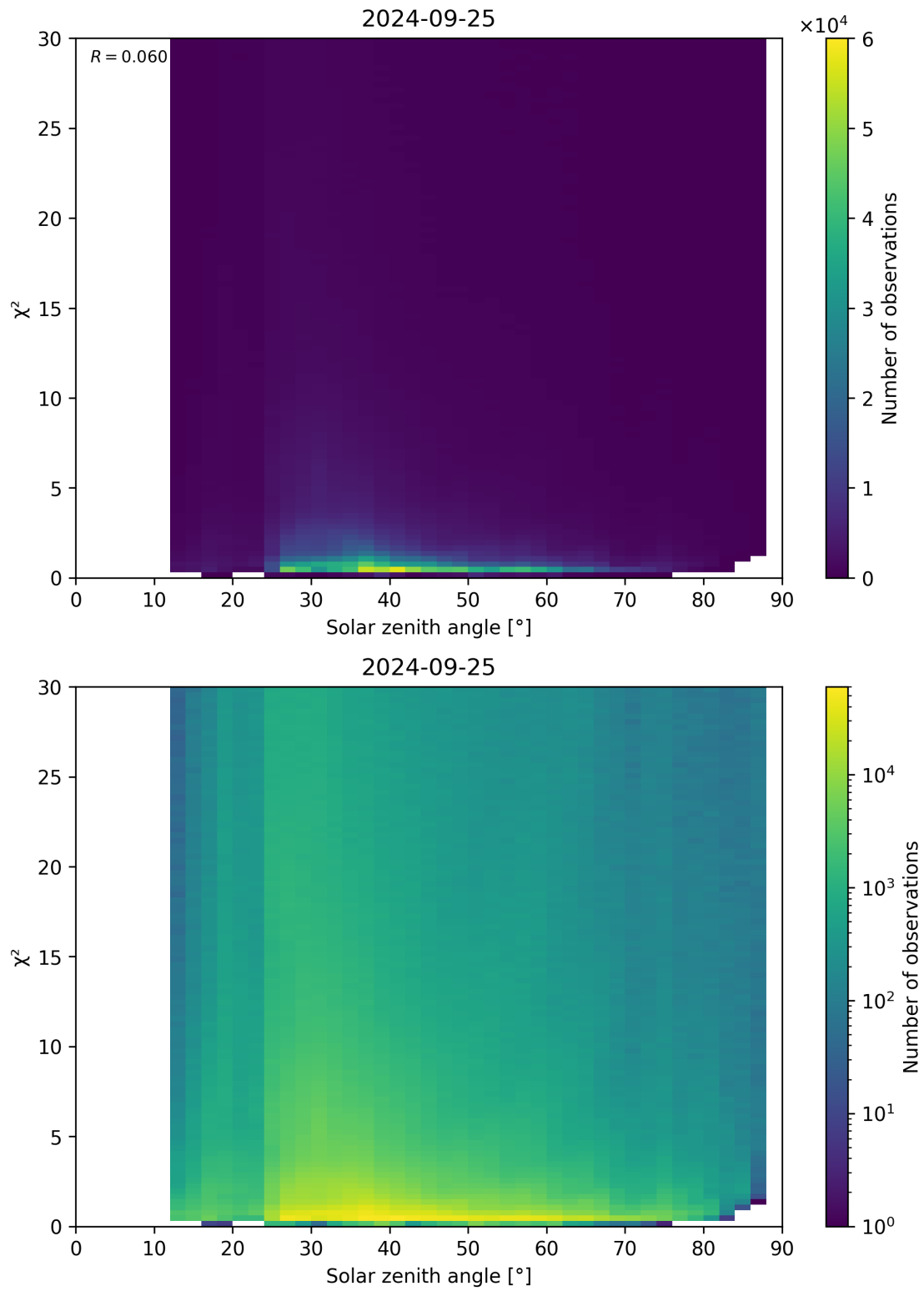
Figure 119: Scatter density plot of “Solar zenith angle” against “ \chi^2 ” for 2024-09-24 to 2024-09-26.
