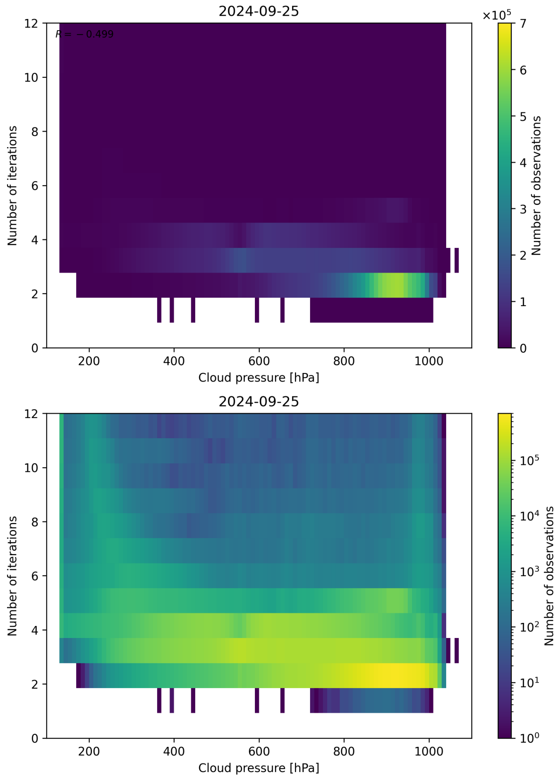
Figure 89: Scatter density plot of “Cloud pressure” against “Number of iterations” for 2024-09-24 to 2024-09-26.
