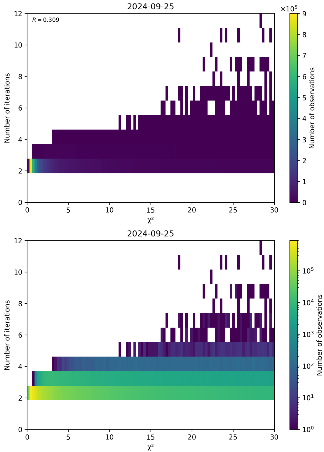
Figure 73: Scatter density plot of “ \chi^2 ” against “Number of iterations” for 2024-09-24 to 2024-09-26.
