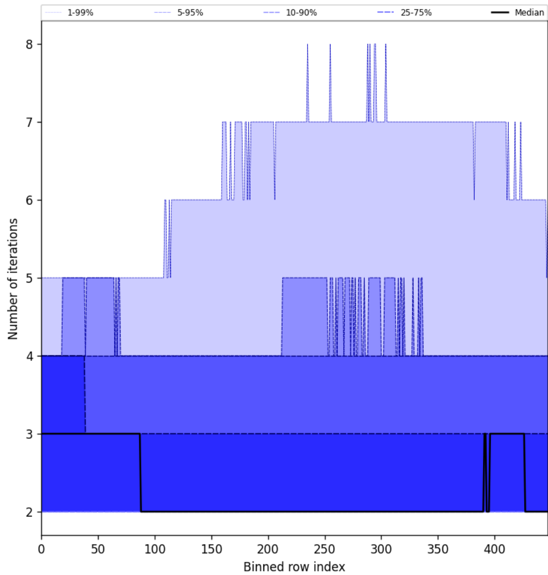
Figure 56: Along track statistics of “Number of iterations” for 2024-09-24 to 2024-09-26
