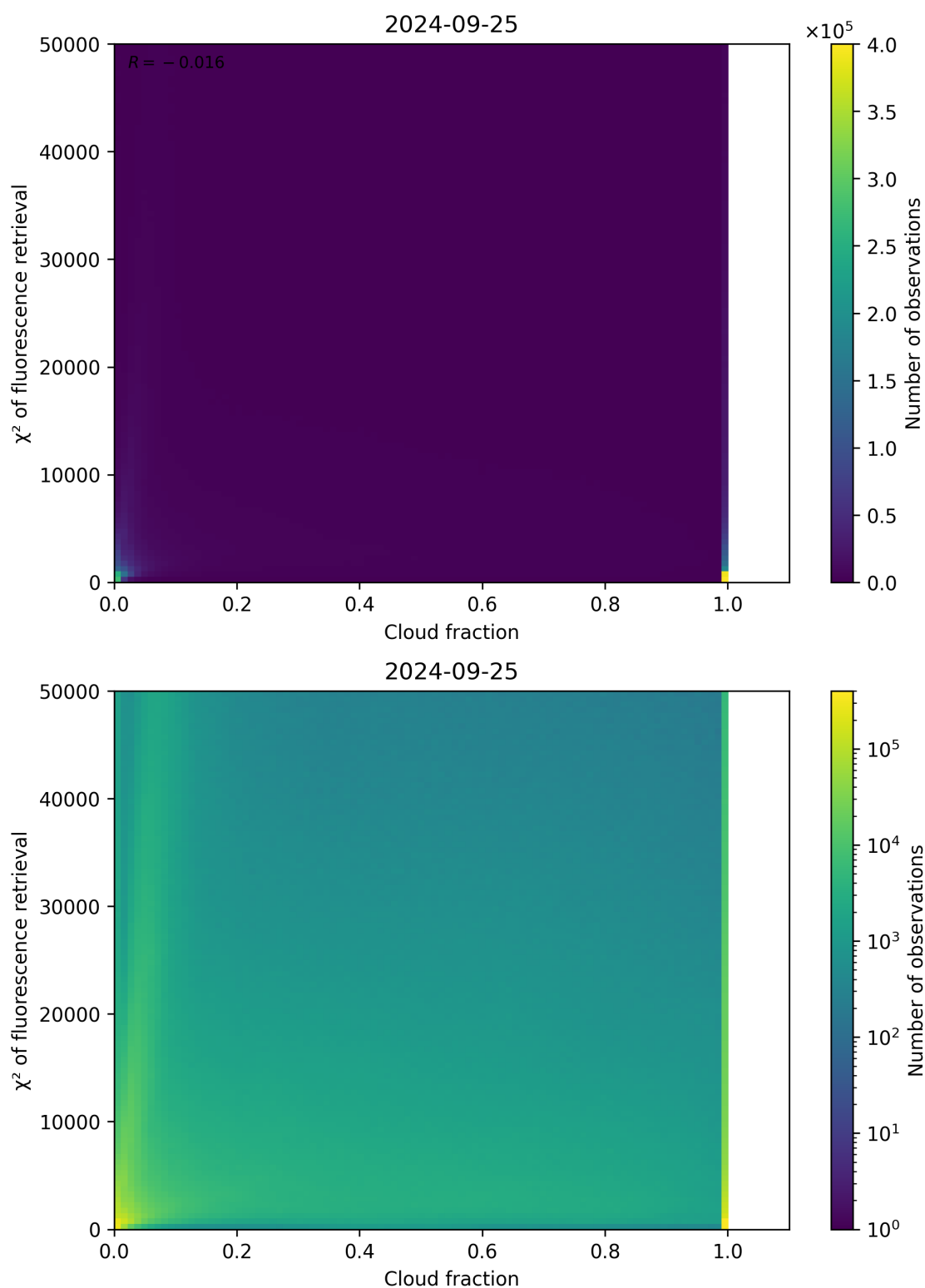
Figure 78: Scatter density plot of “Cloud fraction” against “ \chi^2 of fluorescence retrieval” for 2024-09-24 to 2024-09-26.
