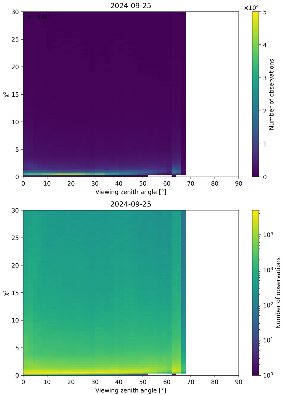
Figure 130: Scatter density plot of “Viewing zenith angle” against “ \chi^2 ” for 2024-09-24 to 2024-09-26.
