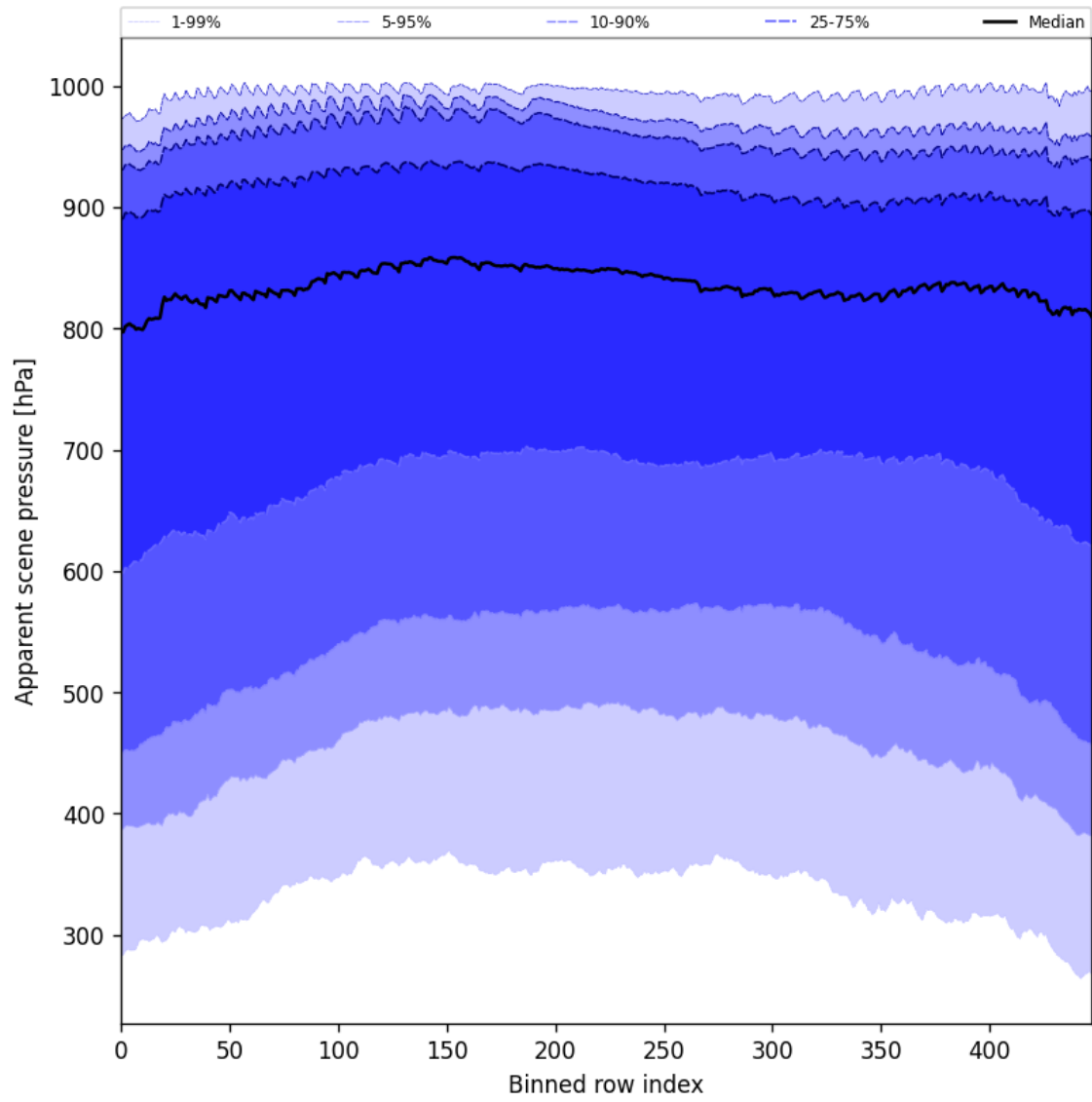
Figure 53: Along track statistics of “Apparent scene pressure” for 2024-09-24 to 2024-09-26
