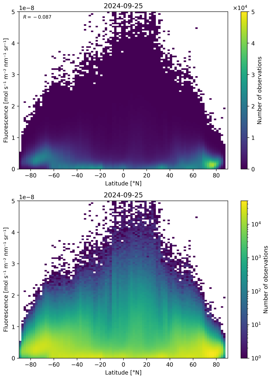
Figure 101: Scatter density plot of “Latitude” against “Fluorescence” for 2024-09-24 to 2024-09-26.
