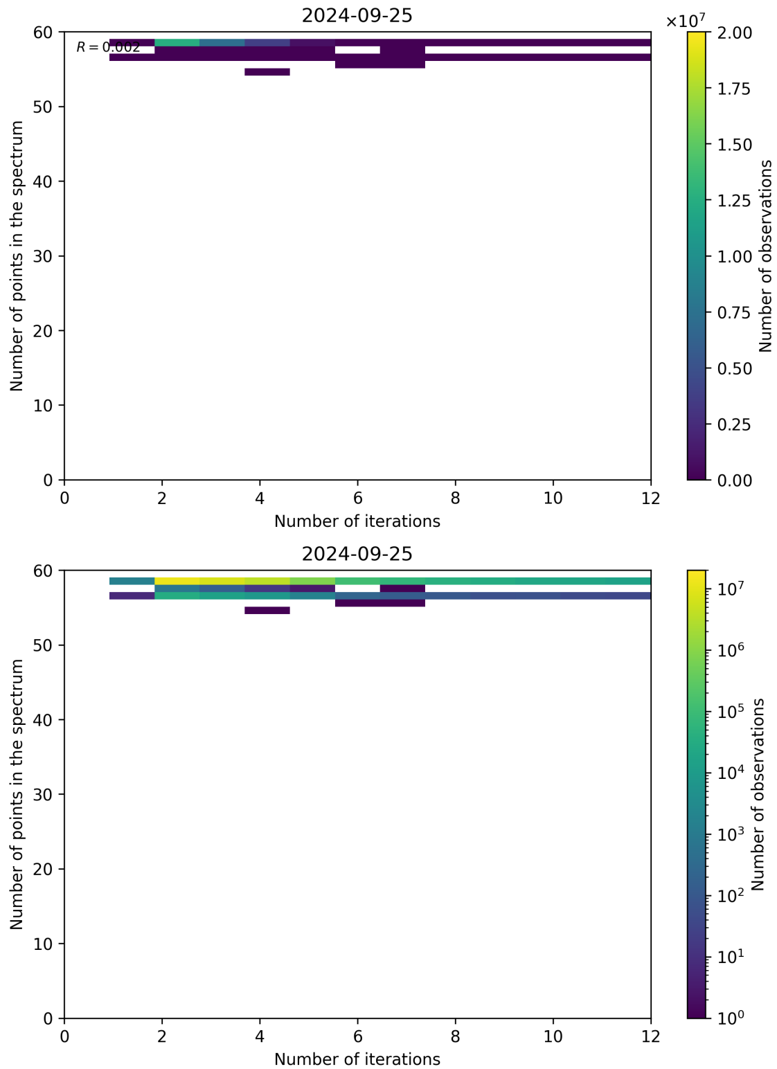
Figure 108: Scatter density plot of “Number of iterations” against “Number of points in the spectrum” for 2024-09-24 to 2024-09-26.
