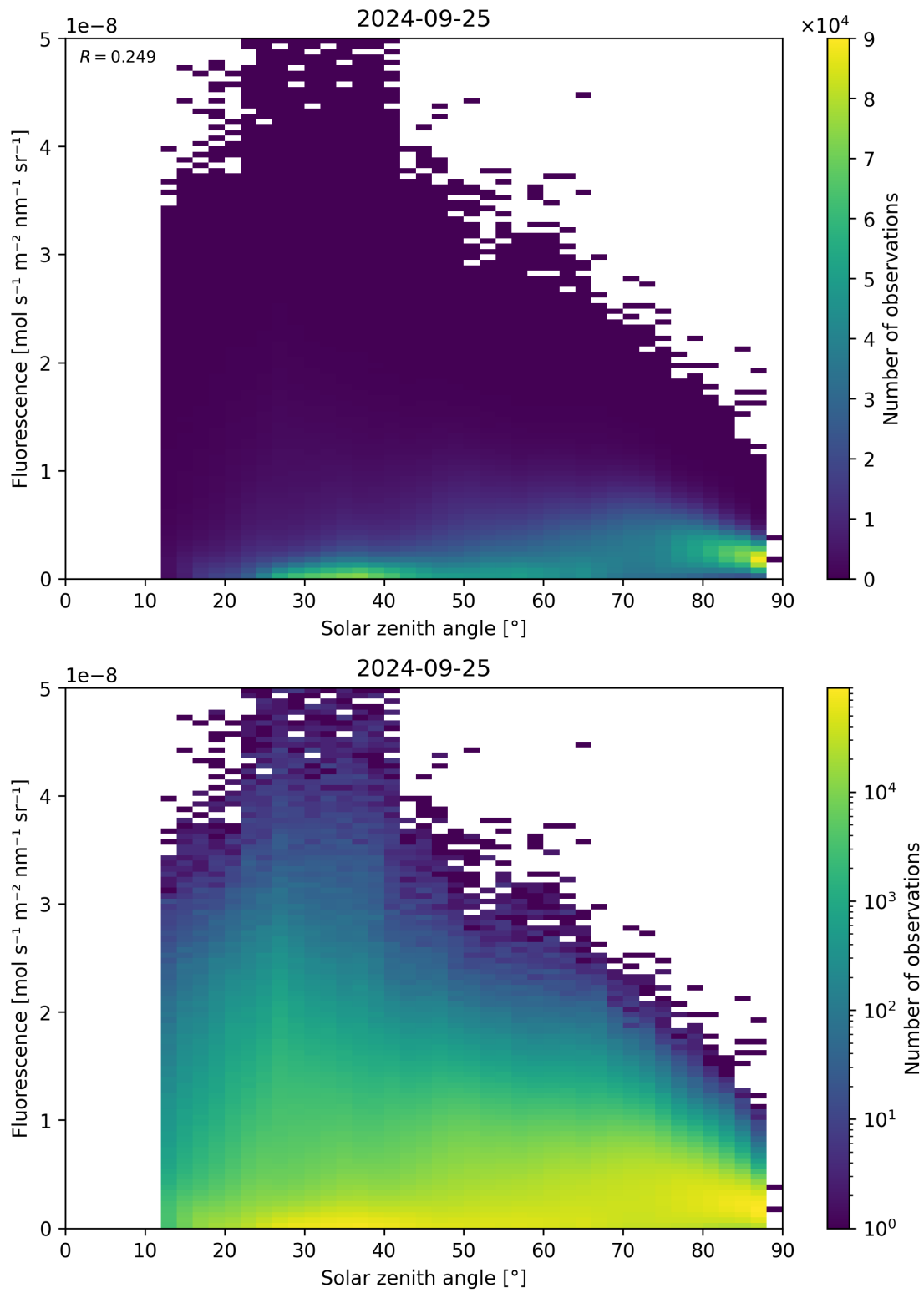
Figure 123: Scatter density plot of “Solar zenith angle” against “Fluorescence” for 2024-09-24 to 2024-09-26.
