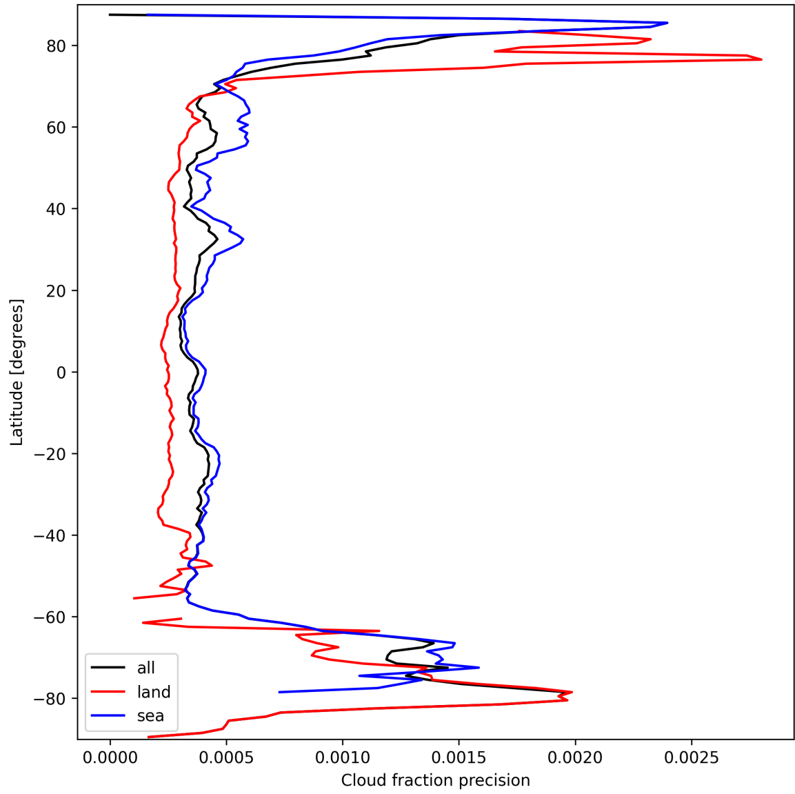
Figure 16: Zonal average of “Cloud fraction precision” for 2024-09-24 to 2024-09-26.
