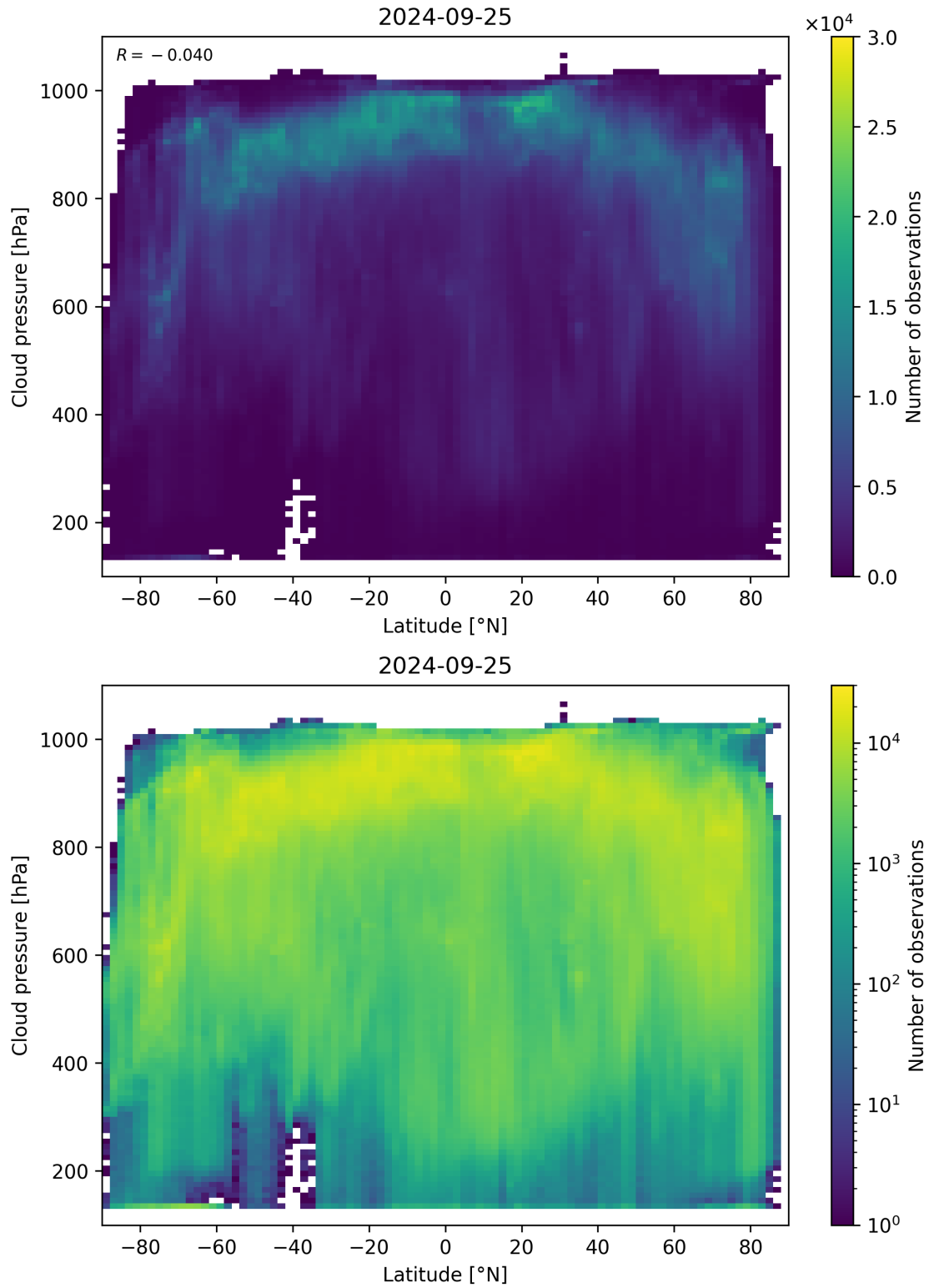
Figure 100: Scatter density plot of “Latitude” against “Cloud pressure” for 2024-09-24 to 2024-09-26.
