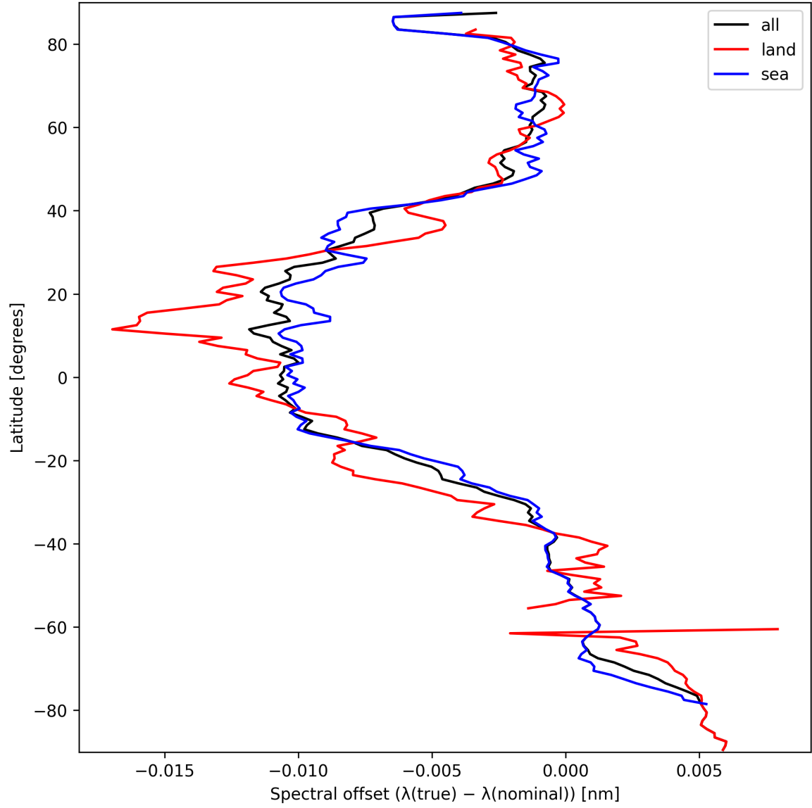
Figure 28: Zonal average of “Spectral offset ( \lambda_{\text{true}} - \lambda_{\text{nominal}} )” for 2024-09-24 to 2024-09-26.
