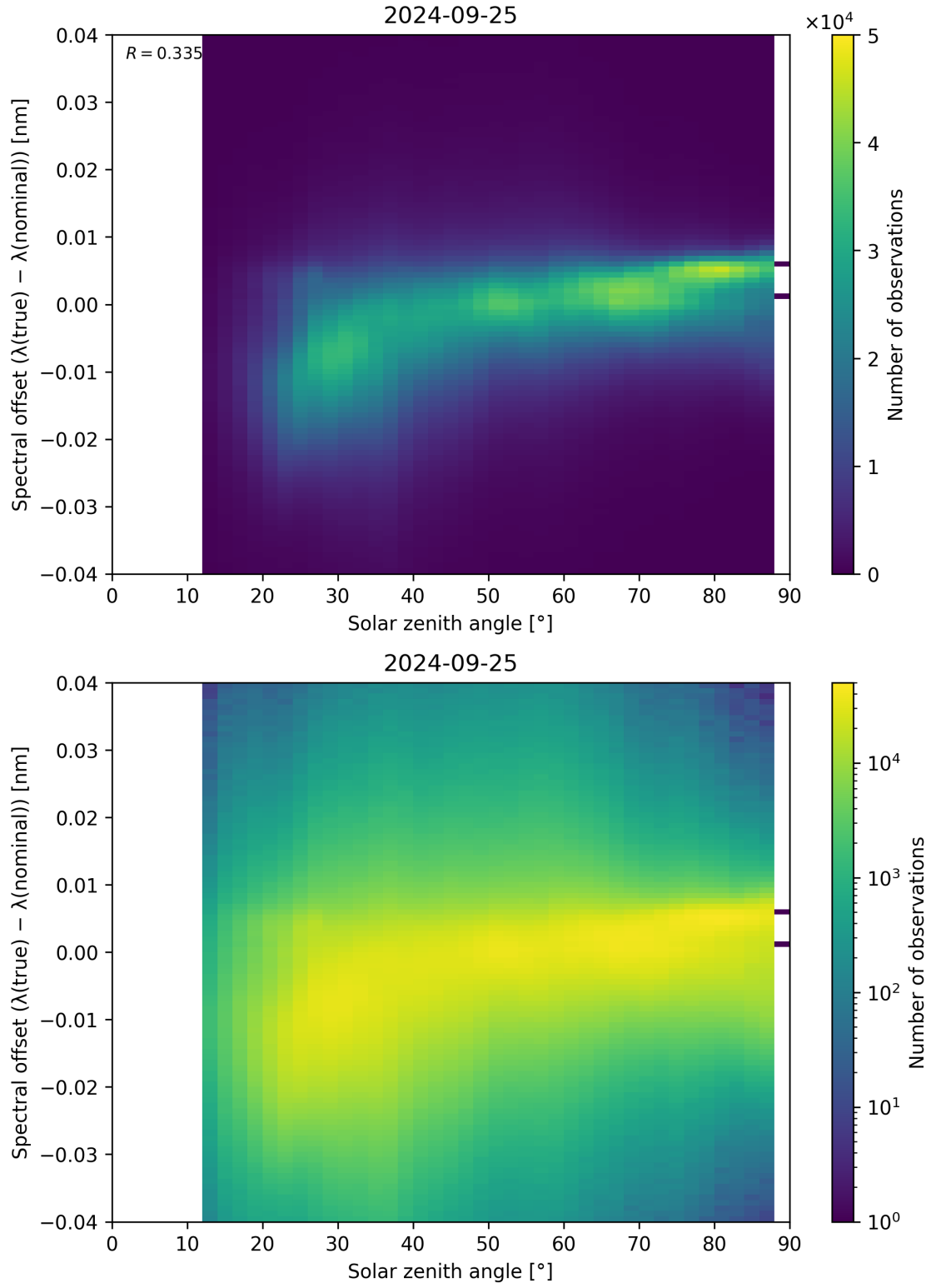
Figure 128: Scatter density plot of “Solar zenith angle” against “Spectral offset ( \lambda_{\text{true}} - \lambda_{\text{nominal}} )” for 2024-09-24 to 2024-09-26.
