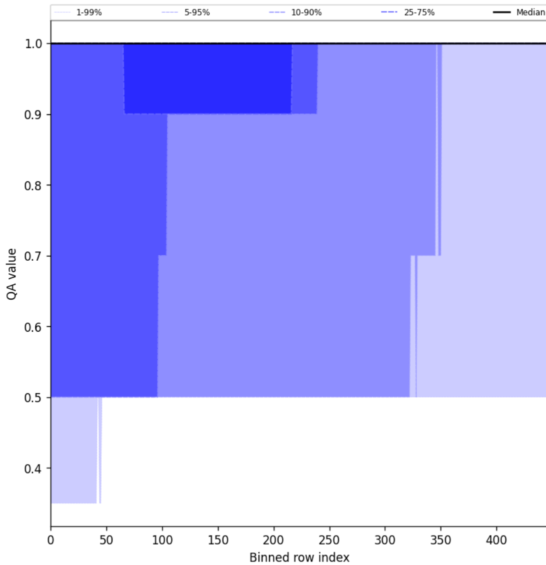
Figure 46: Along track statistics of “QA value” for 2024-09-24 to 2024-09-26
