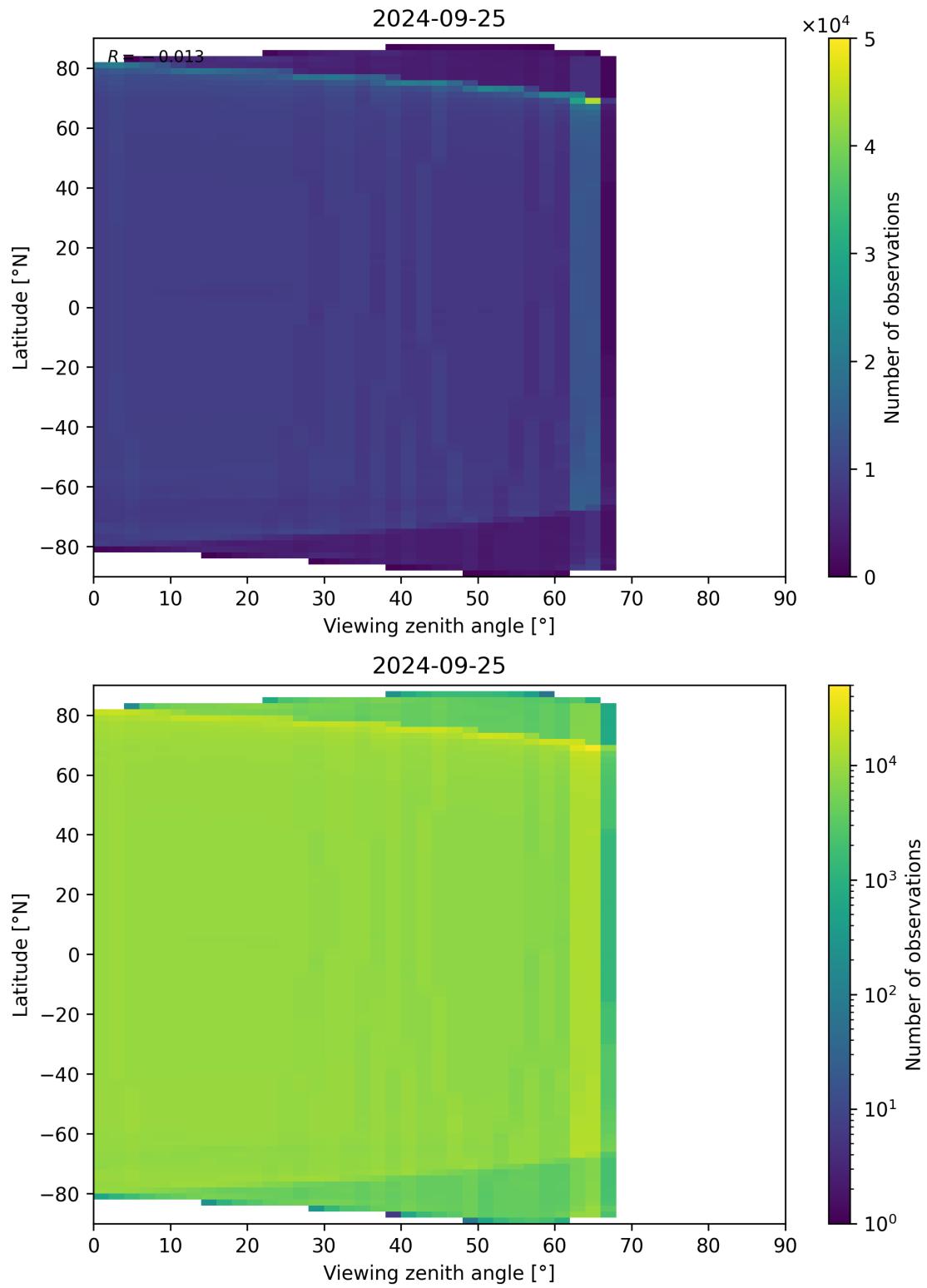
Figure 135: Scatter density plot of “Viewing zenith angle” against “Latitude” for 2024-09-24 to 2024-09-26.
