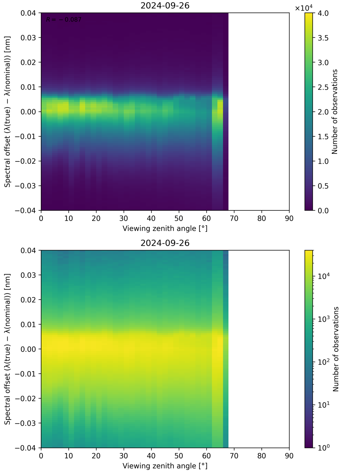
Figure 140: Scatter density plot of “Viewing zenith angle” against “Spectral offset ( \lambda_{\text{true}} - \lambda_{\text{nominal}} )” for 2024-09-25 to 2024-09-27.
