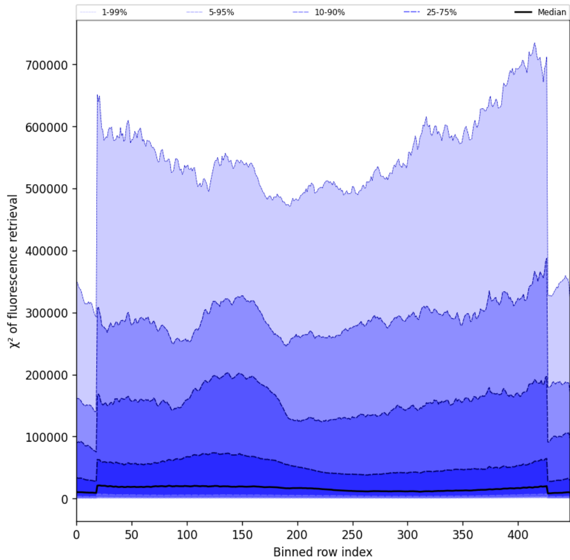
Figure 59: Along track statistics of “ \chi^2 of fluorescence retrieval” for 2024-09-25 to 2024-09-27
