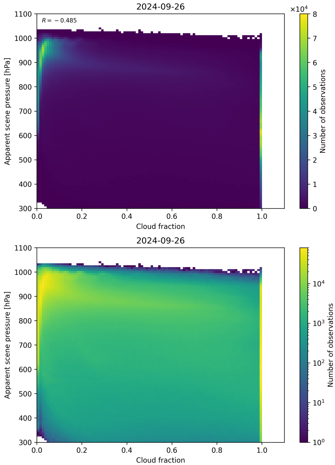
Figure 76: Scatter density plot of “Cloud fraction” against “Apparent scene pressure” for 2024-09-25 to 2024-09-27.
