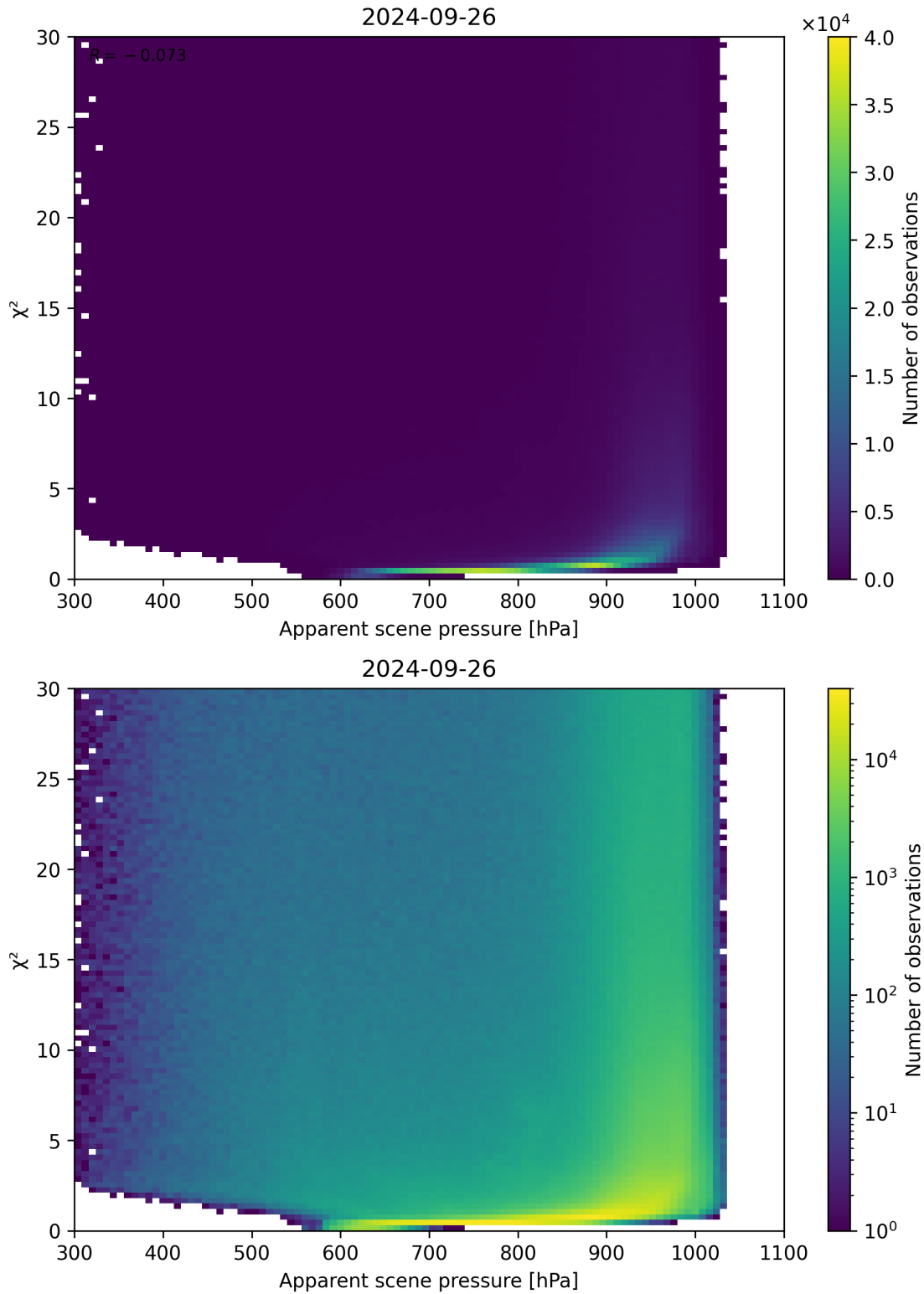
Figure 63: Scatter density plot of “Apparent scene pressure” against “ \chi^2 ” for 2024-09-25 to 2024-09-27.
