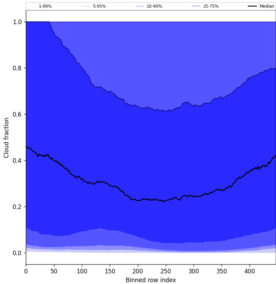
Figure 49: Along track statistics of “Cloud fraction” for 2024-09-25 to 2024-09-27
