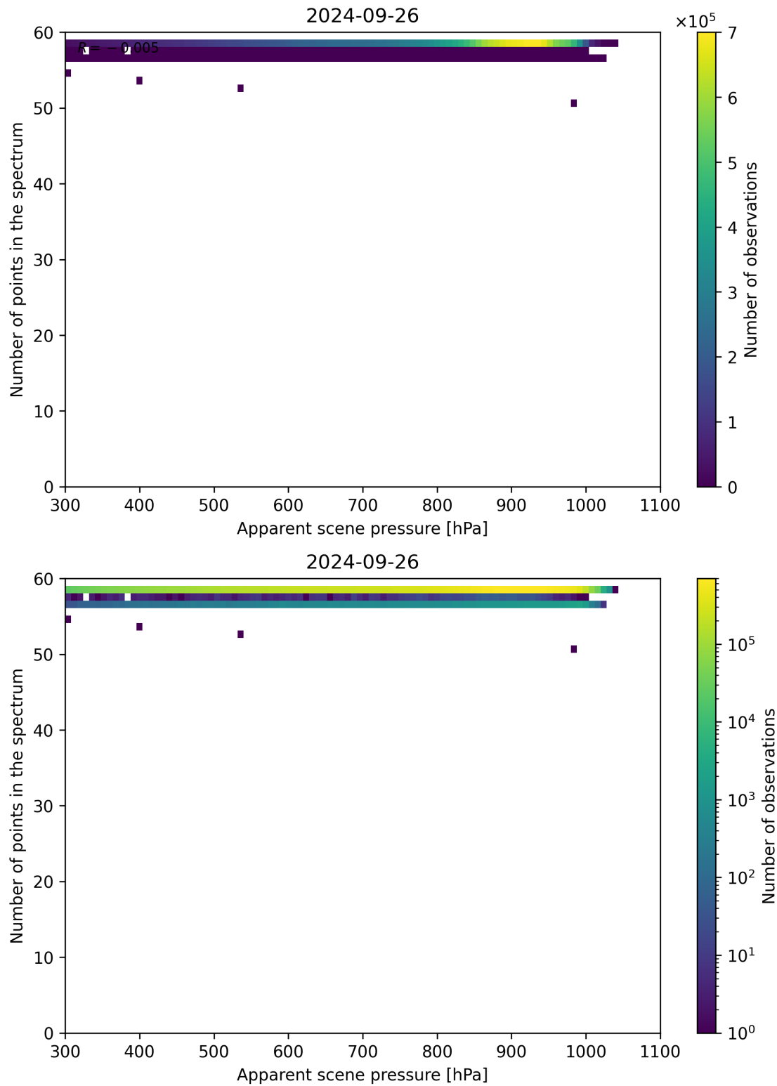
Figure 67: Scatter density plot of “Apparent scene pressure” against “Number of points in the spectrum” for 2024-09-25 to 2024-09-27.
