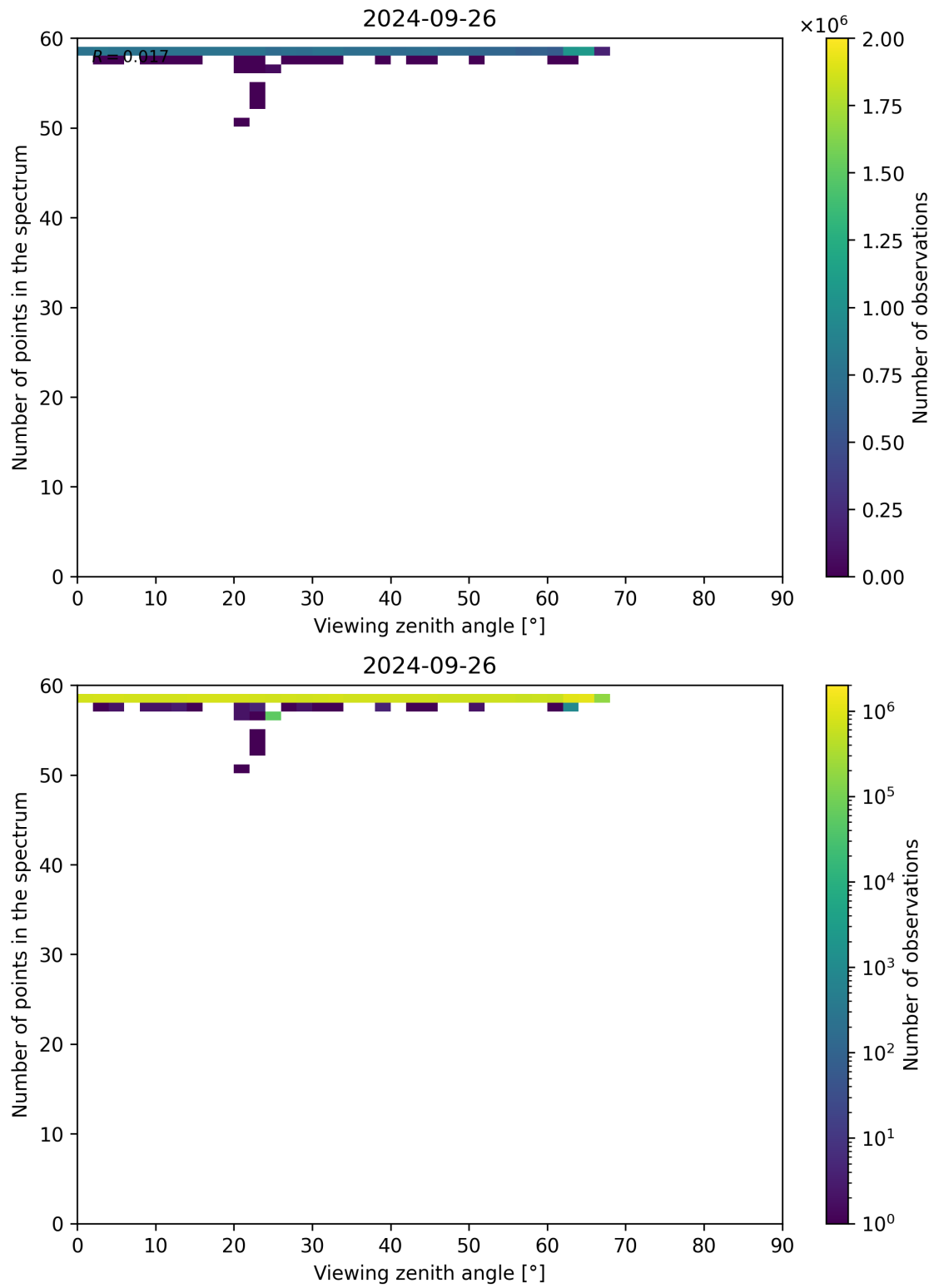
Figure 137: Scatter density plot of “Viewing zenith angle” against “Number of points in the spectrum” for 2024-09-25 to 2024-09-27.
