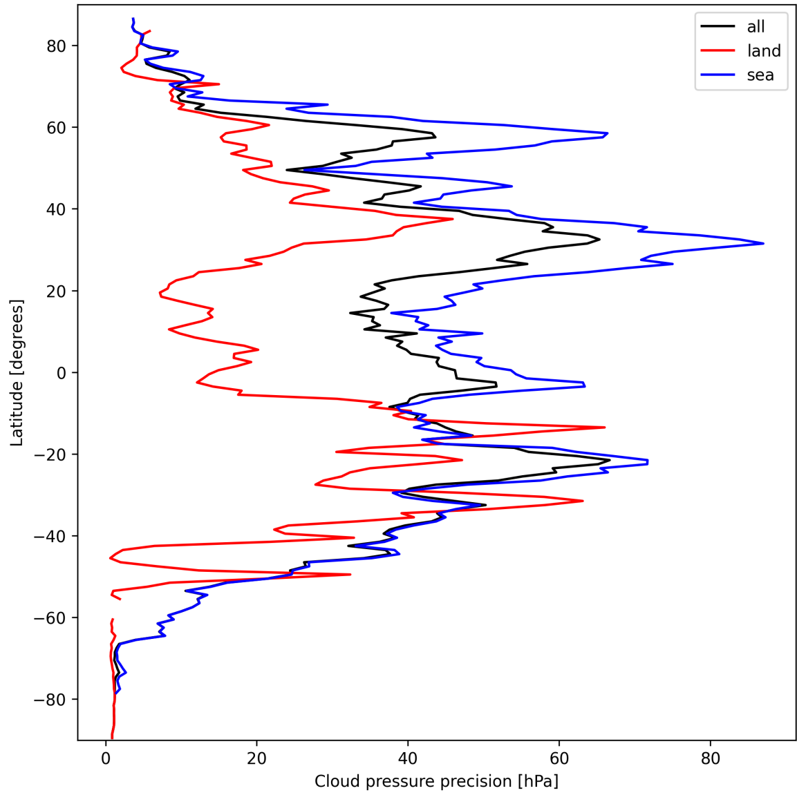
Figure 14: Zonal average of “Cloud pressure precision” for 2024-09-25 to 2024-09-27.
