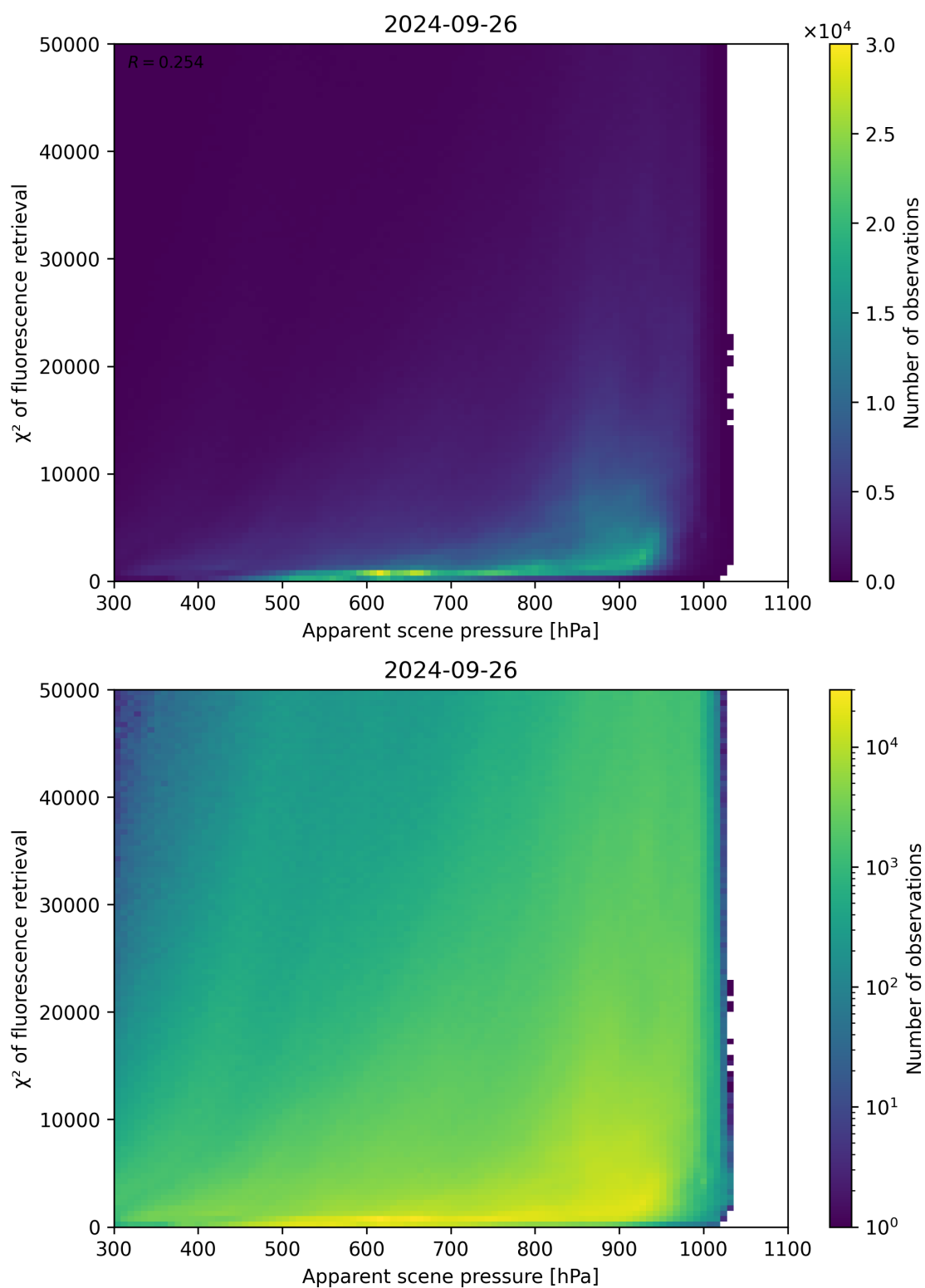
Figure 64: Scatter density plot of “Apparent scene pressure” against “ \chi^2 of fluorescence retrieval” for 2024-09-25 to 2024-09-27.
