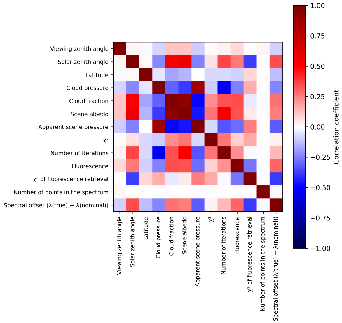
Figure 2: Map of correlation matrix for 2024-09-25 to 2024-09-27.
