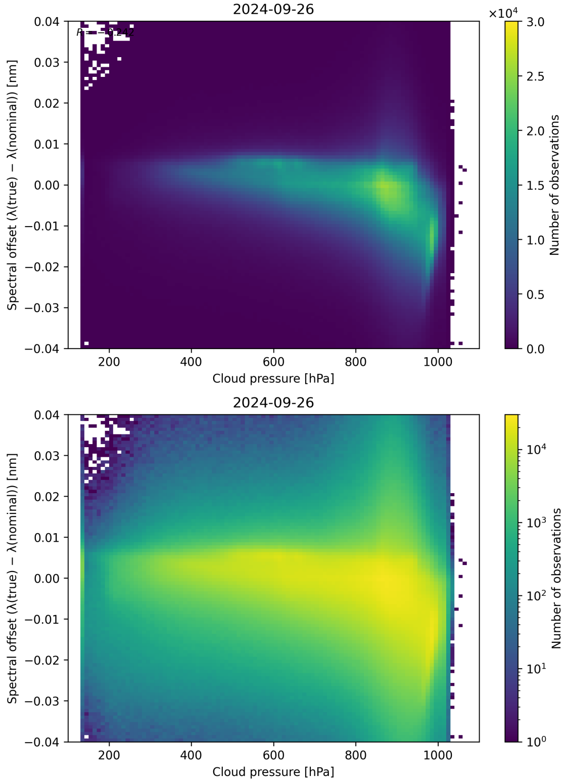
Figure 92: Scatter density plot of “Cloud pressure” against “Spectral offset ( \lambda_{\text{true}} - \lambda_{\text{nominal}} )” for 2024-09-25 to 2024-09-27.
