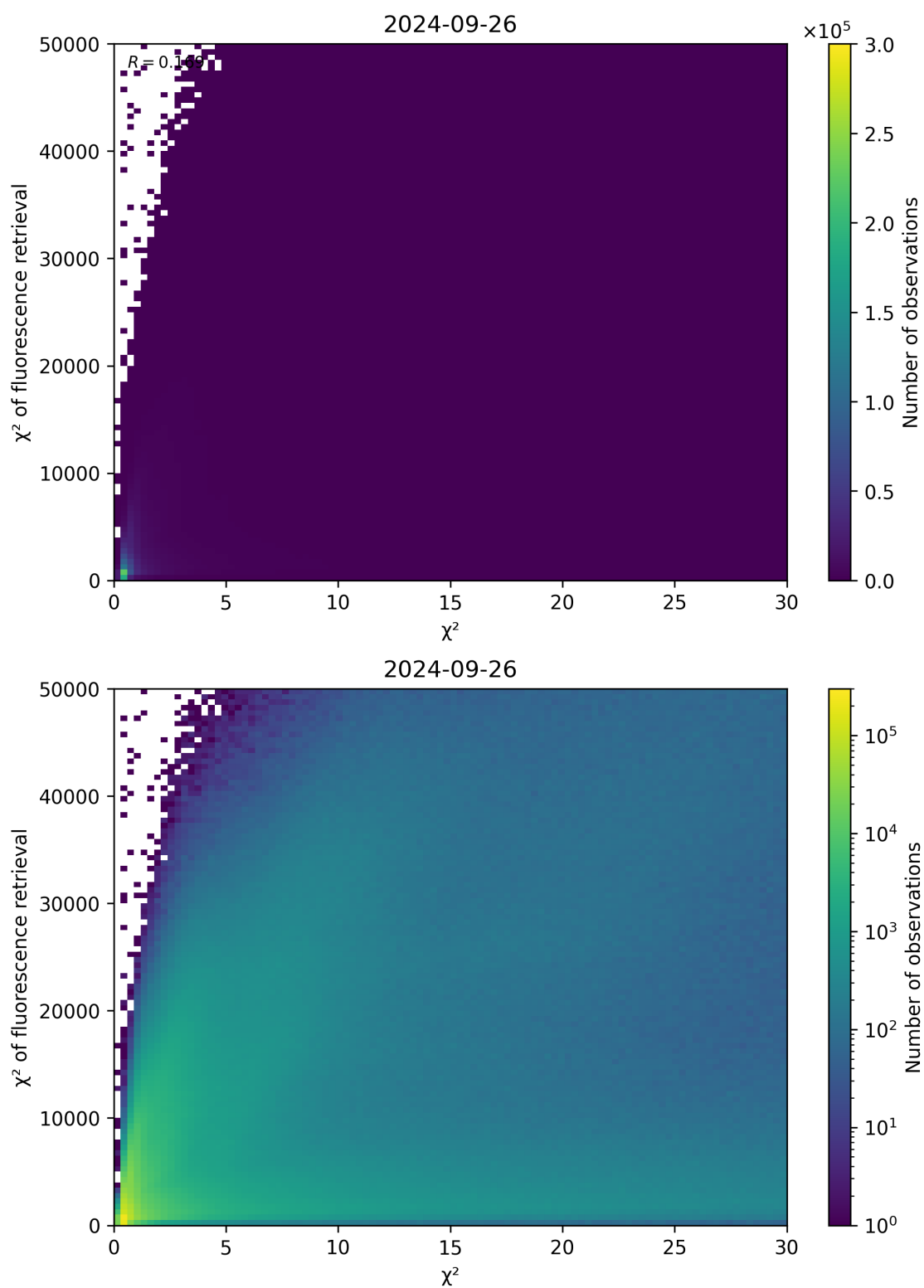
Figure 69: Scatter density plot of “ \chi^2 ” against “ \chi^2 of fluorescence retrieval” for 2024-09-25 to 2024-09-27.
