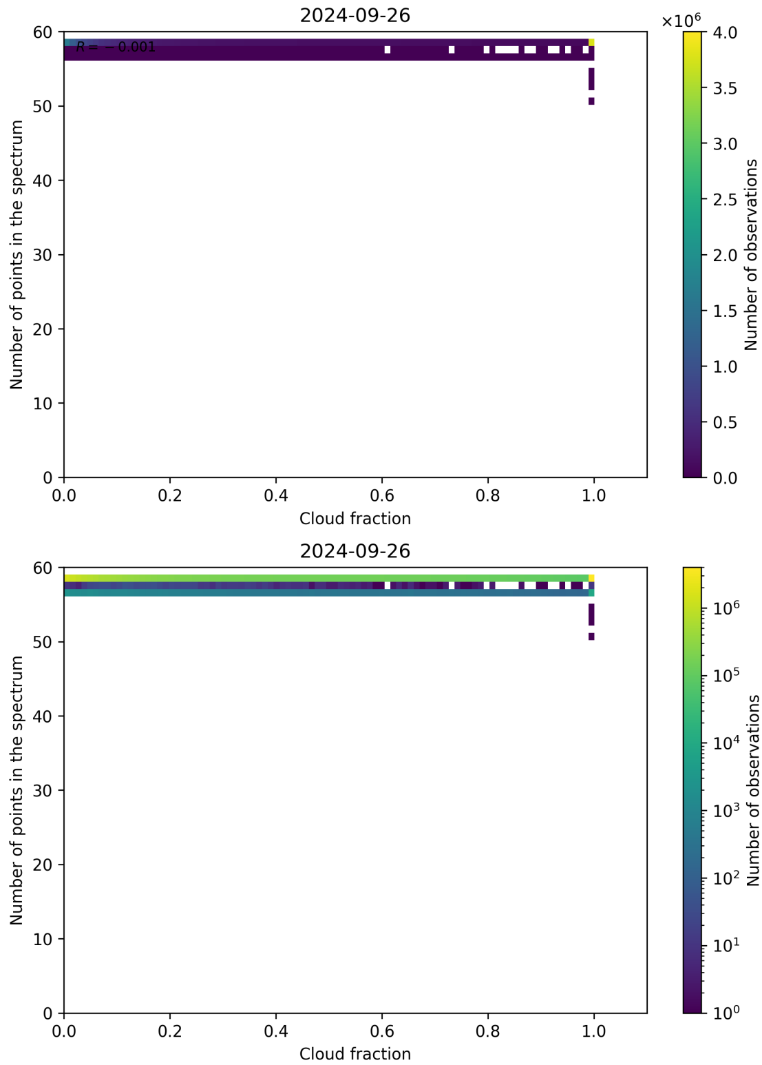
Figure 81: Scatter density plot of “Cloud fraction” against “Number of points in the spectrum” for 2024-09-25 to 2024-09-27.
