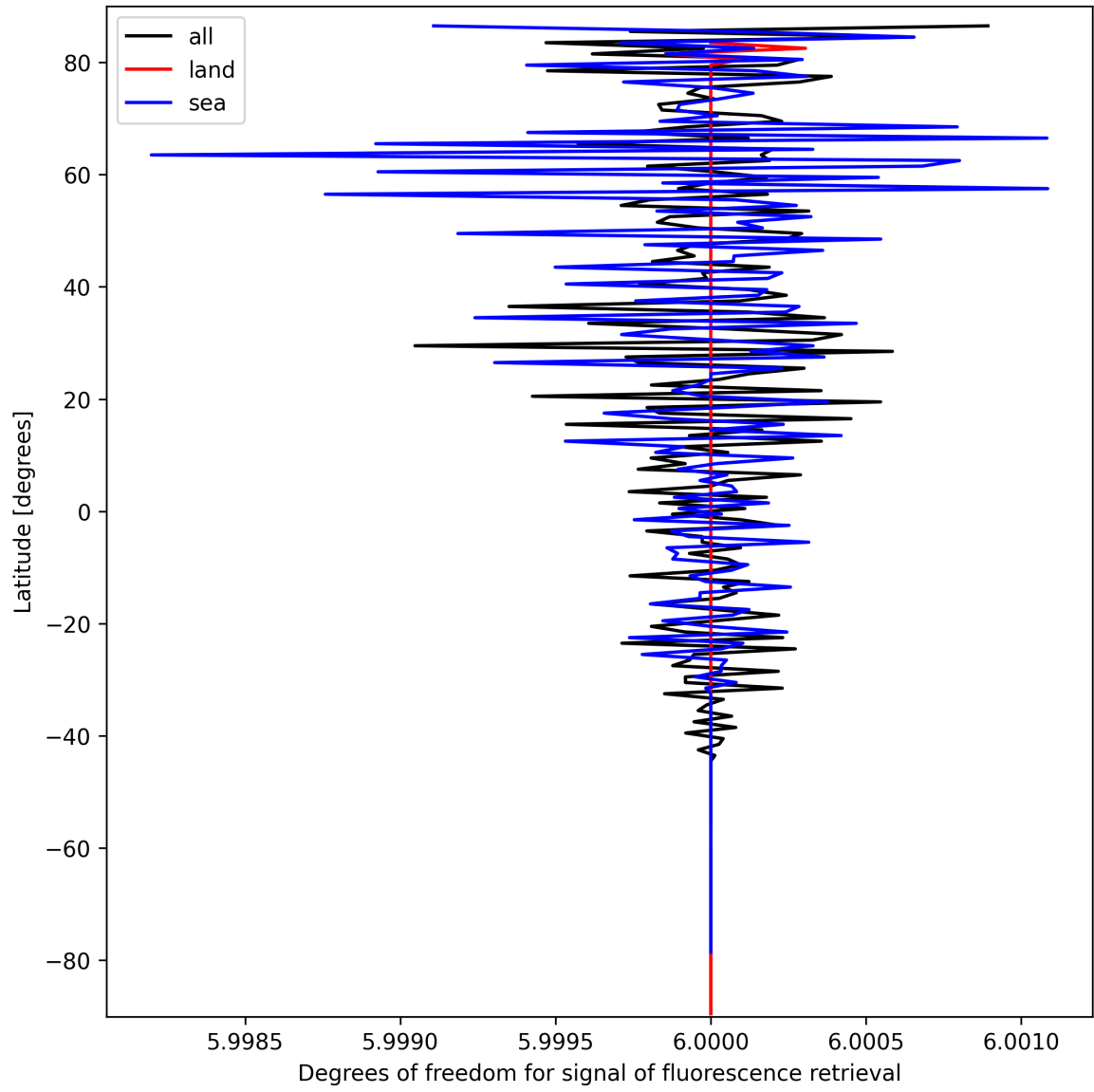
Figure 26: Zonal average of “Degrees of freedom for signal of fluorescence retrieval” for 2024-09-25 to 2024-09-27.
