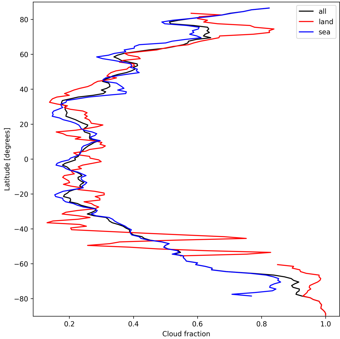
Figure 15: Zonal average of “Cloud fraction” for 2024-09-25 to 2024-09-27.
