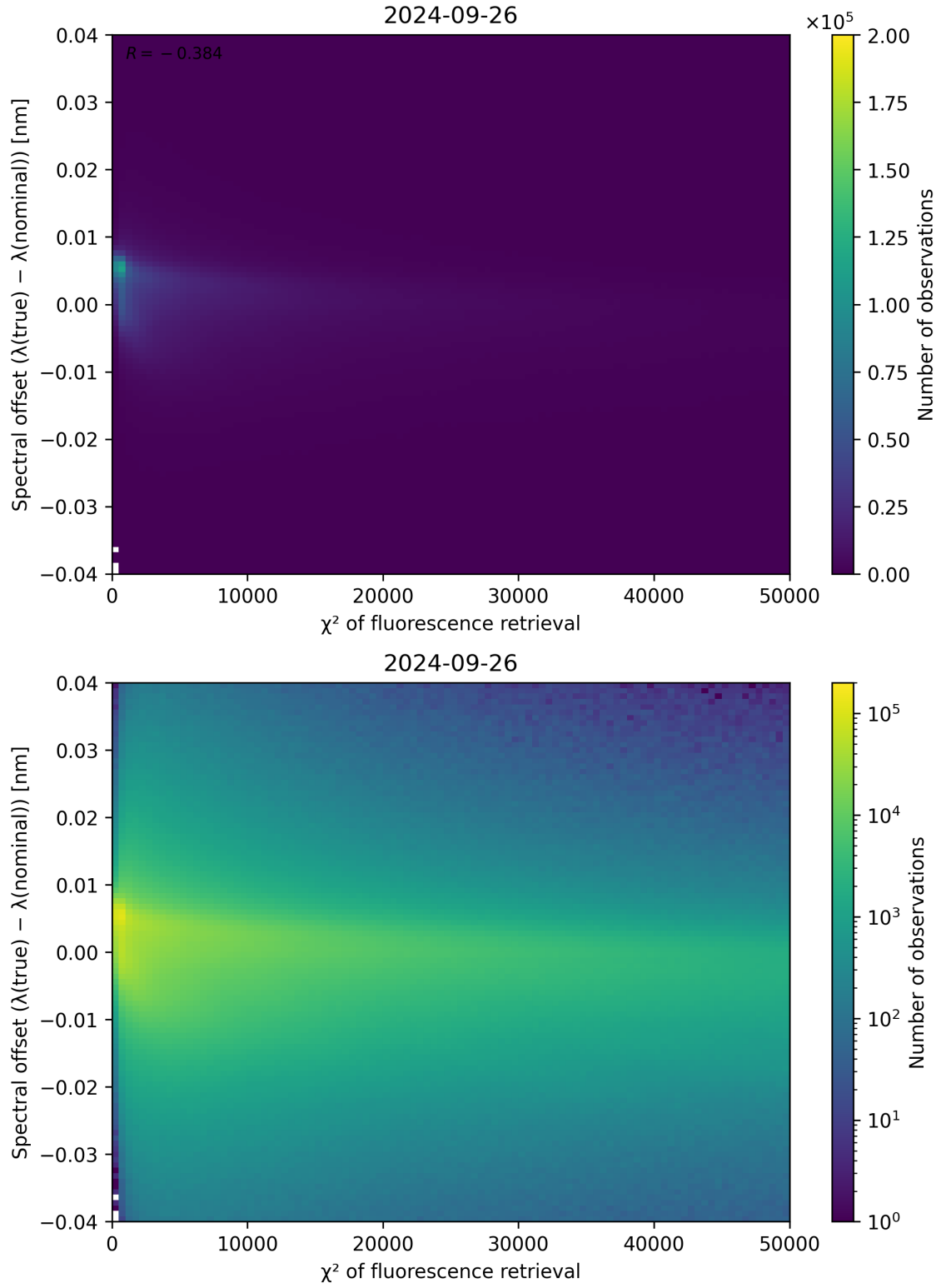
Figure 72: Scatter density plot of “ \chi^2 of fluorescence retrieval” against “Spectral offset ( \lambda_{\text{true}} - \lambda_{\text{nominal}} )” for 2024-09-25 to 2024-09-27.
