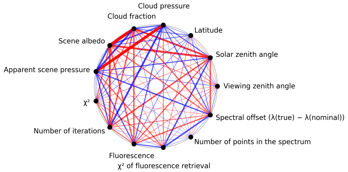
Figure 1: Map of correlation graph for 2024-09-25 to 2024-09-27.
