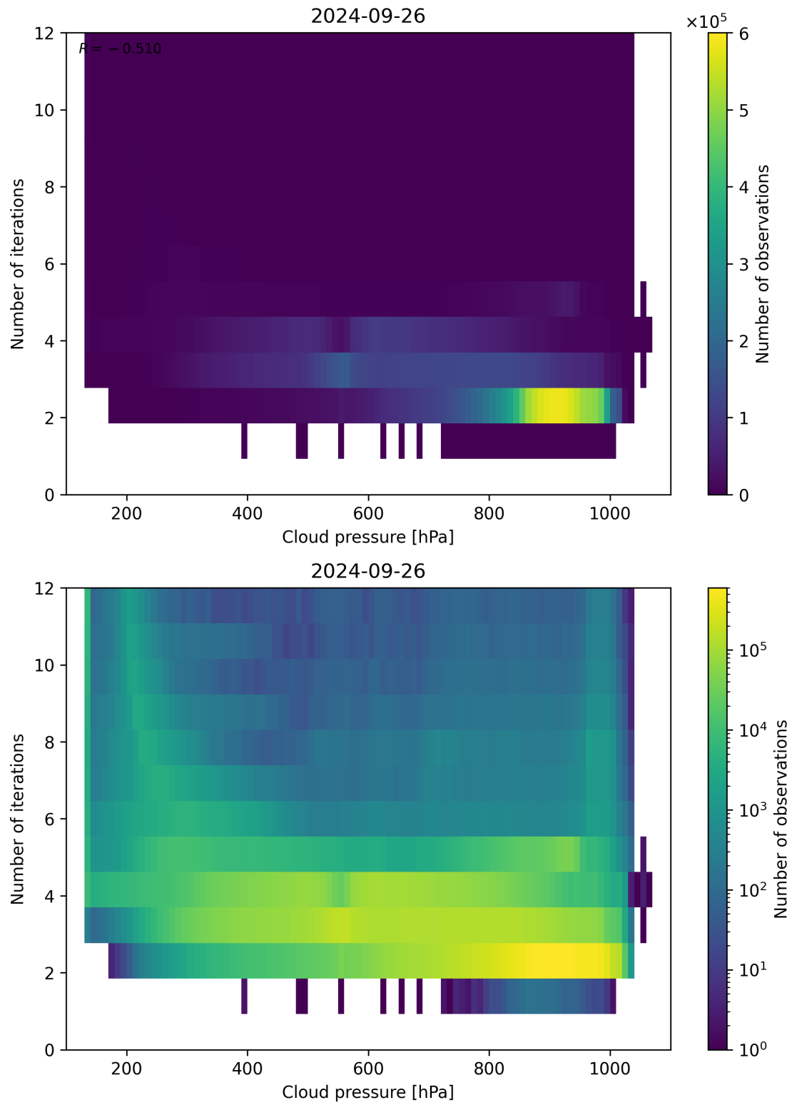
Figure 89: Scatter density plot of “Cloud pressure” against “Number of iterations” for 2024-09-25 to 2024-09-27.
