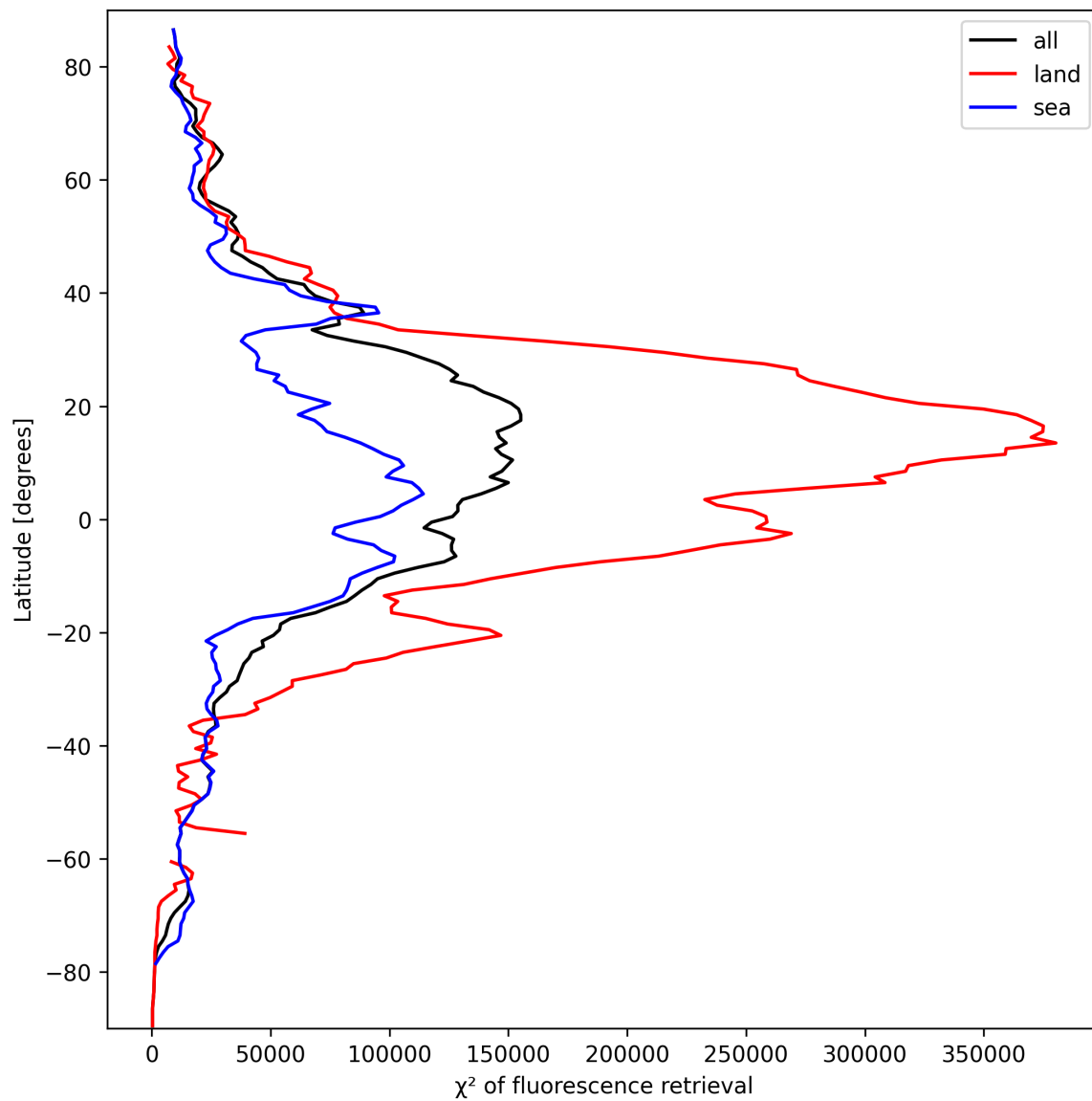
Figure 25: Zonal average of “ \chi^2 of fluorescence retrieval” for 2024-09-25 to 2024-09-27.
