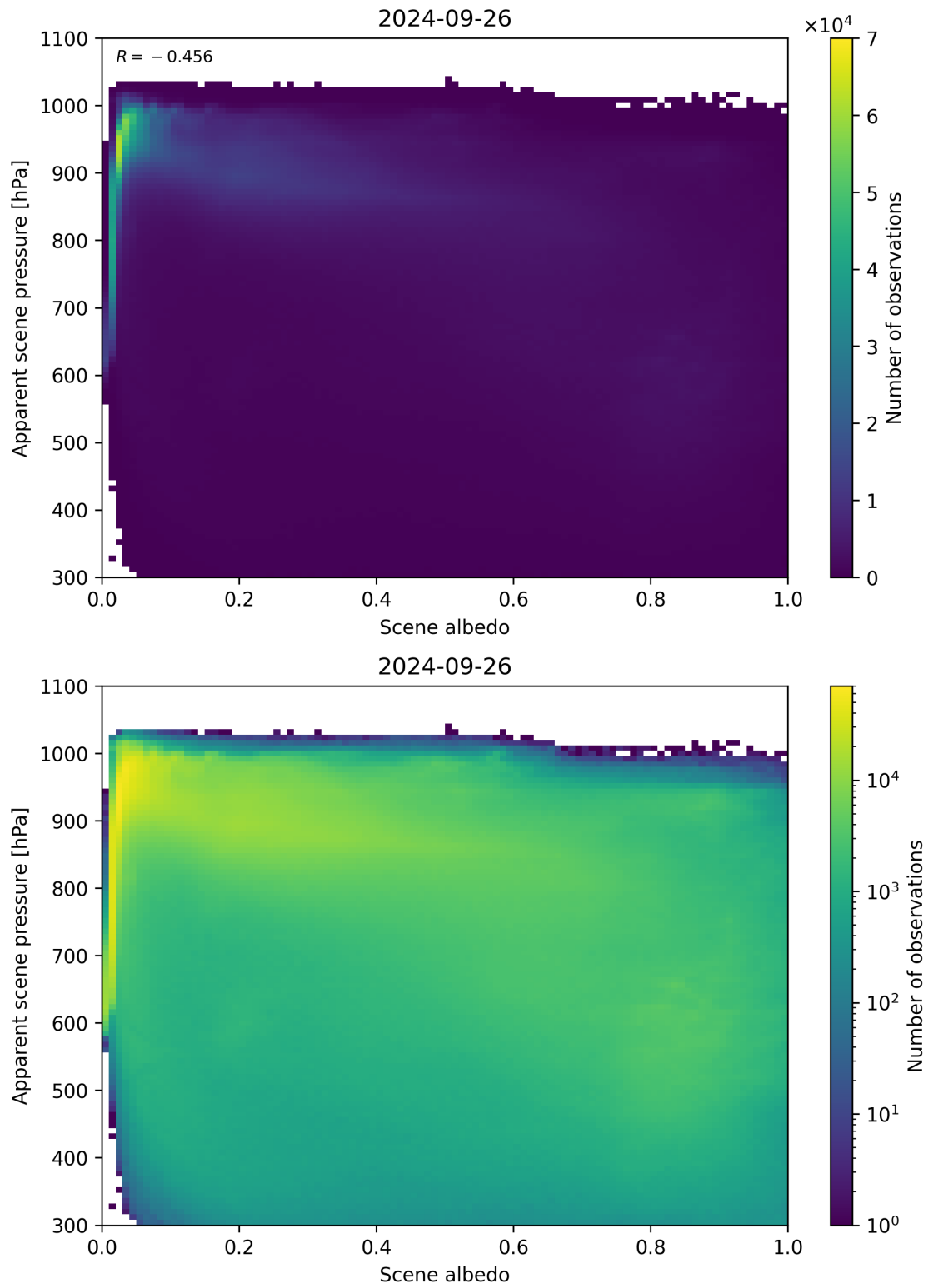
Figure 111: Scatter density plot of “Scene albedo” against “Apparent scene pressure” for 2024-09-25 to 2024-09-27.
