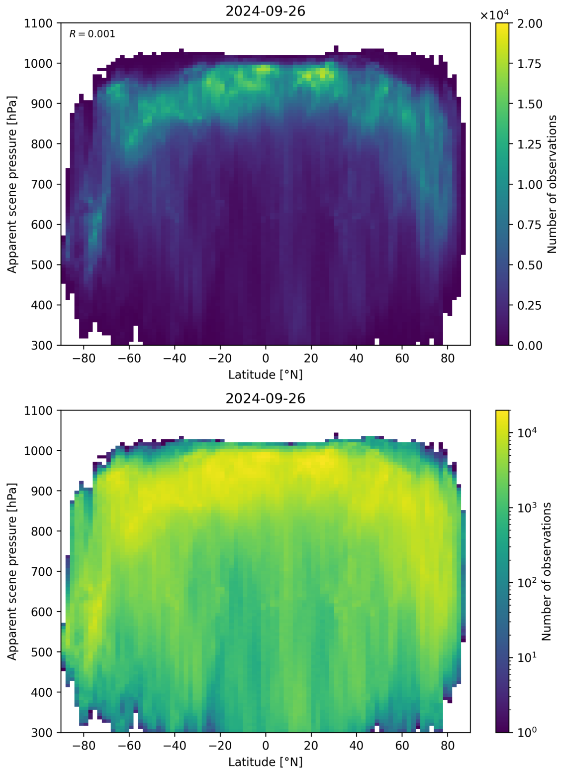
Figure 96: Scatter density plot of “Latitude” against “Apparent scene pressure” for 2024-09-25 to 2024-09-27.
