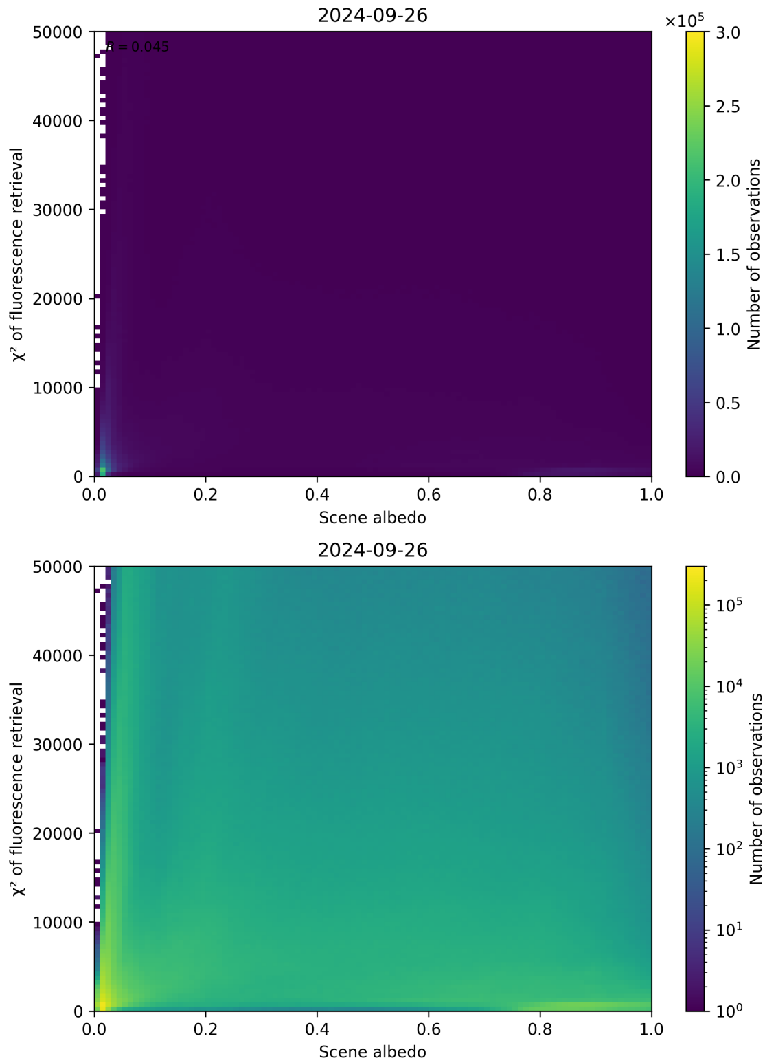
Figure 113: Scatter density plot of “Scene albedo” against “ \chi^2 of fluorescence retrieval” for 2024-09-25 to 2024-09-27.
