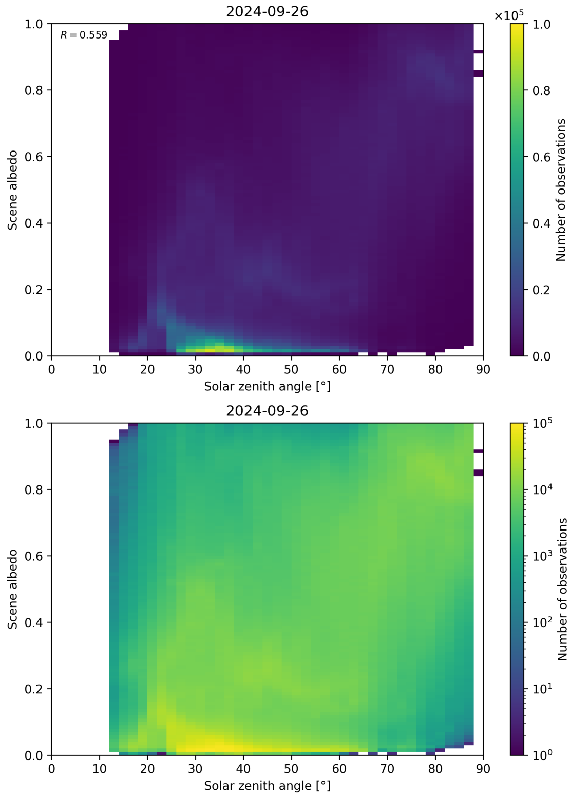
Figure 127: Scatter density plot of “Solar zenith angle” against “Scene albedo” for 2024-09-25 to 2024-09-27.
