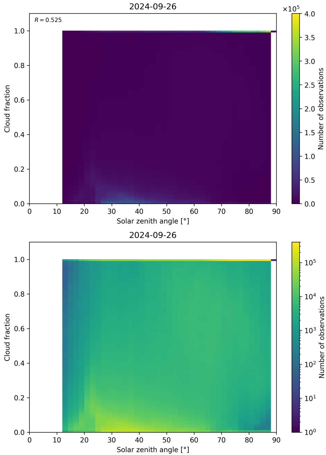
Figure 121: Scatter density plot of “Solar zenith angle” against “Cloud fraction” for 2024-09-25 to 2024-09-27.
