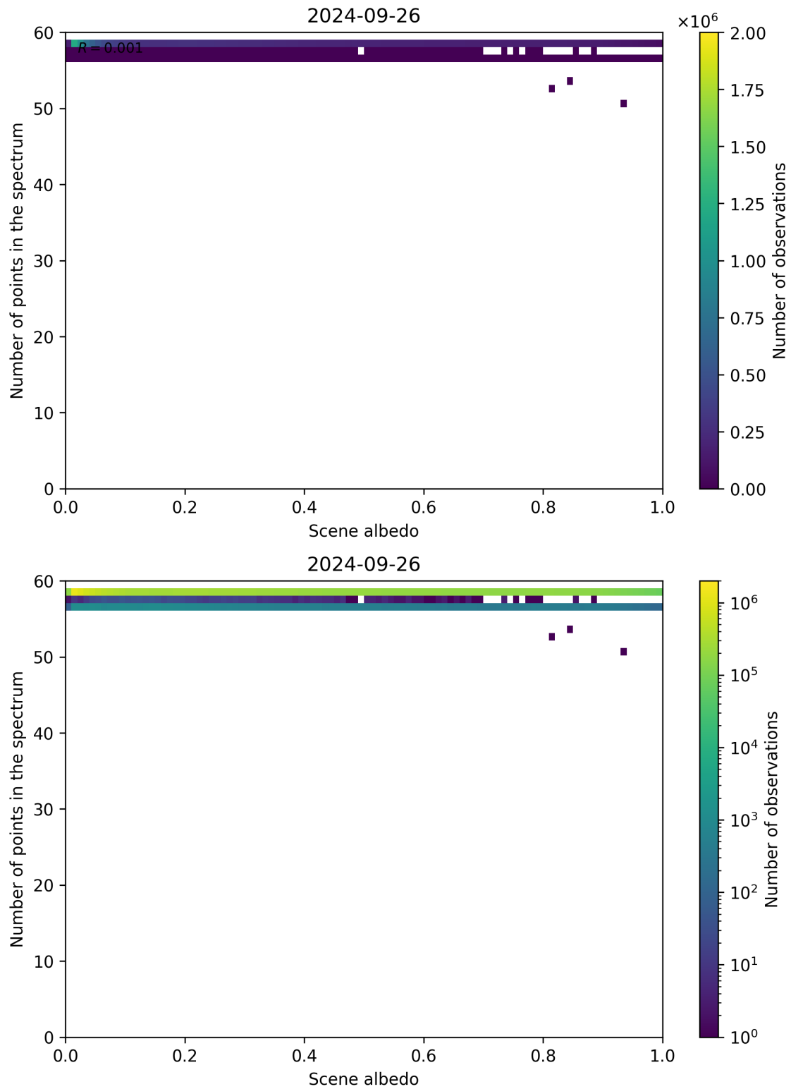
Figure 116: Scatter density plot of “Scene albedo” against “Number of points in the spectrum” for 2024-09-25 to 2024-09-27.
