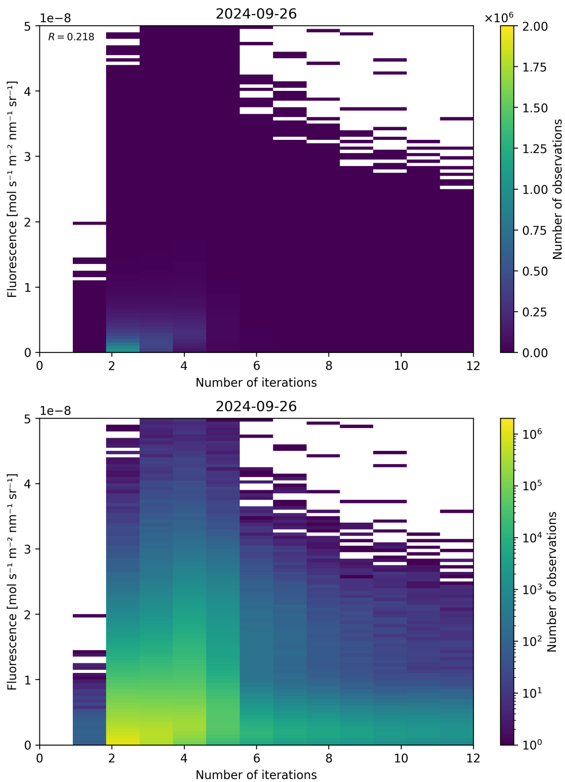
Figure 107: Scatter density plot of “Number of iterations” against “Fluorescence” for 2024-09-25 to 2024-09-27.
