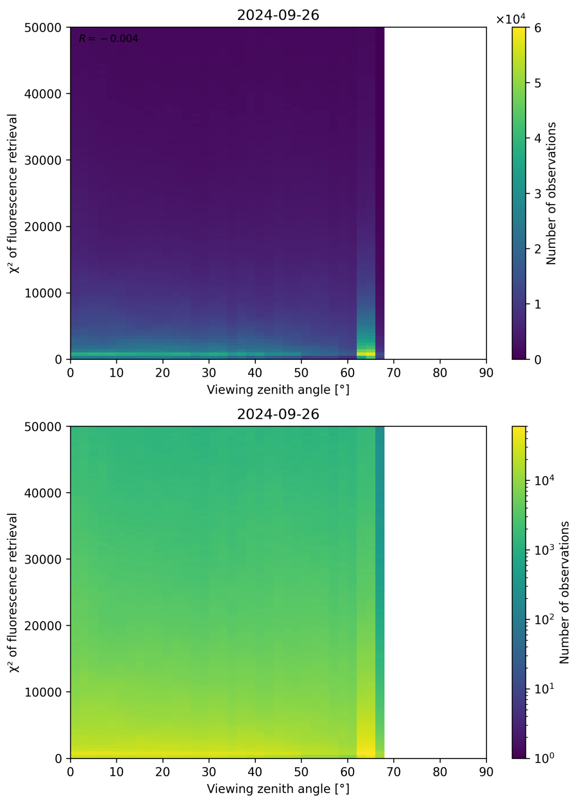
Figure 131: Scatter density plot of “Viewing zenith angle” against “ \chi^2 of fluorescence retrieval” for 2024-09-25 to 2024-09-27.
