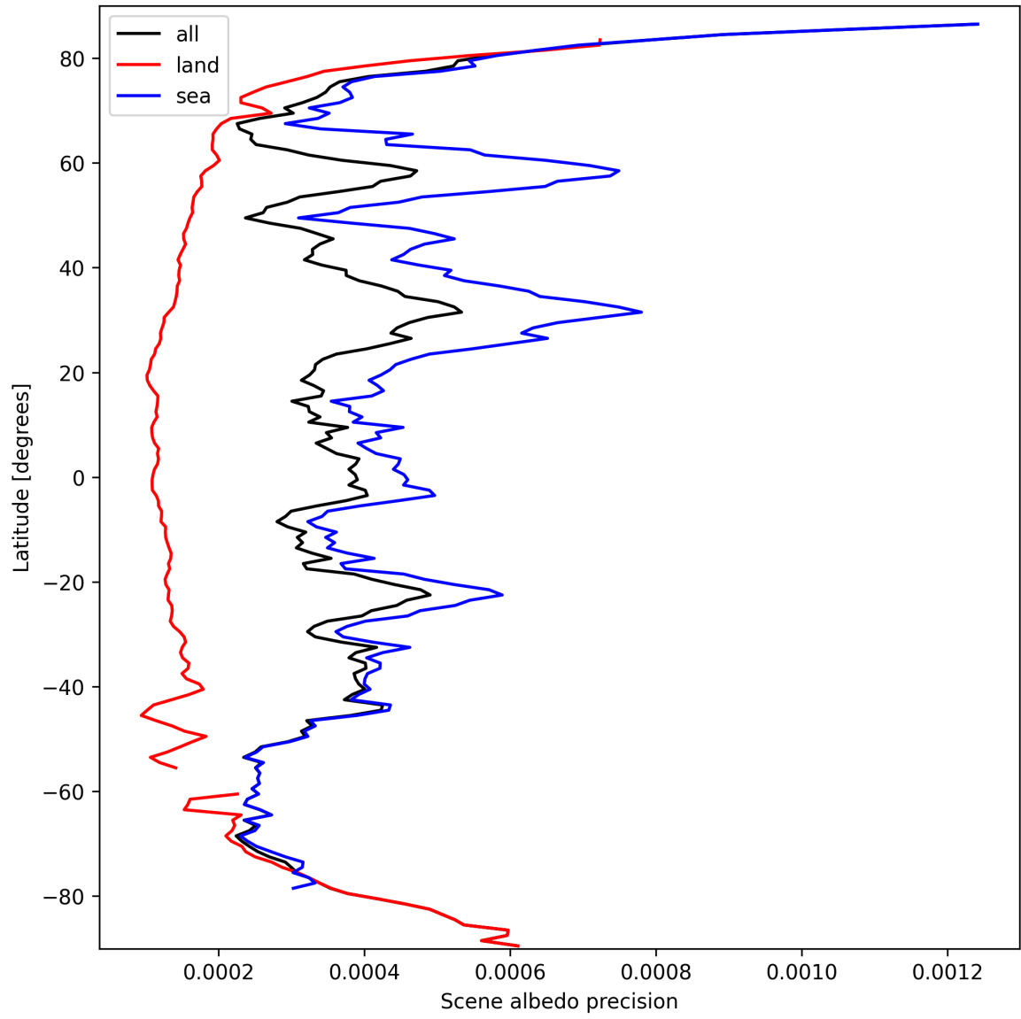
Figure 18: Zonal average of "Scene albedo precision" for 2024-09-25 to 2024-09-27.
