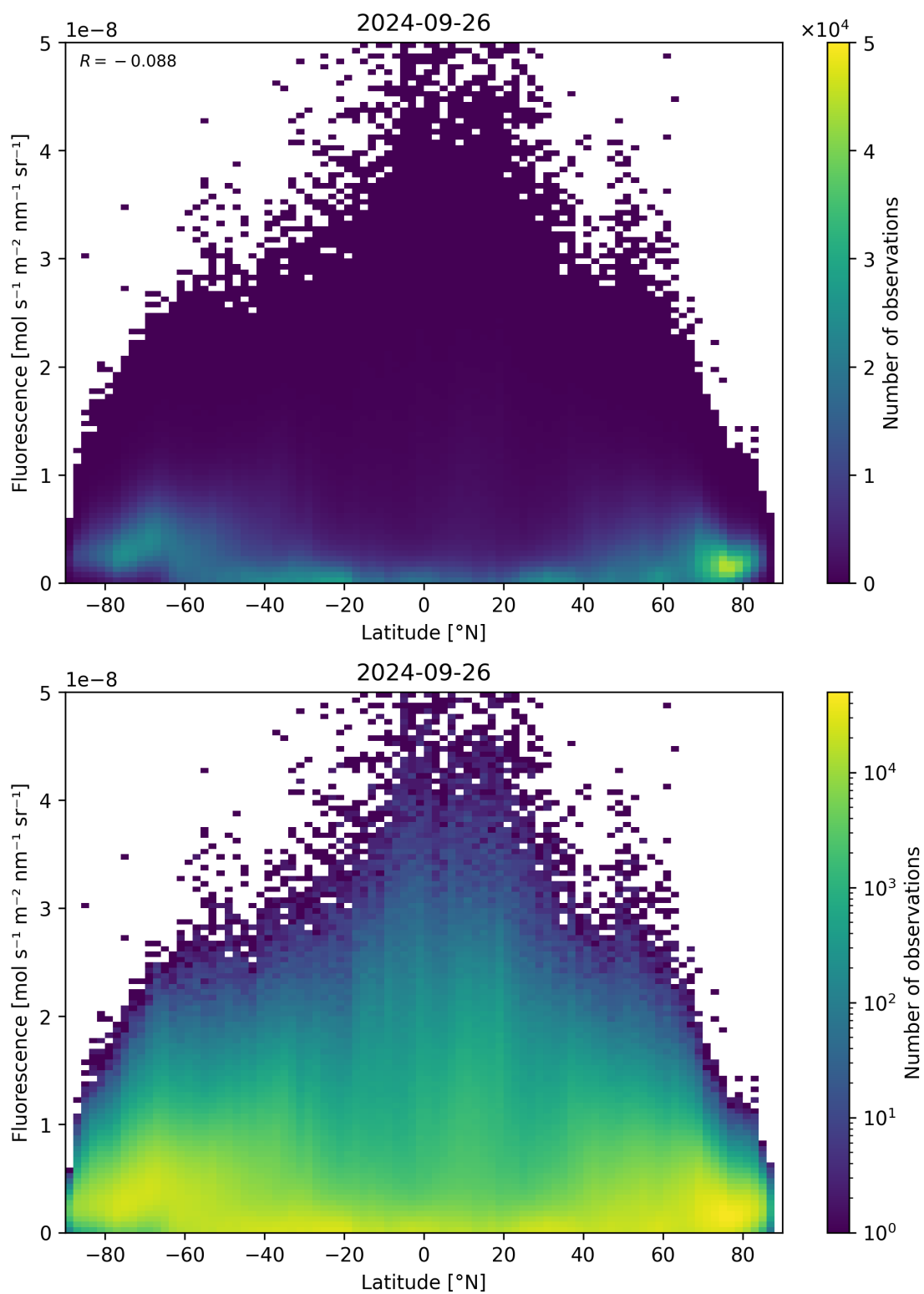
Figure 101: Scatter density plot of “Latitude” against “Fluorescence” for 2024-09-25 to 2024-09-27.
