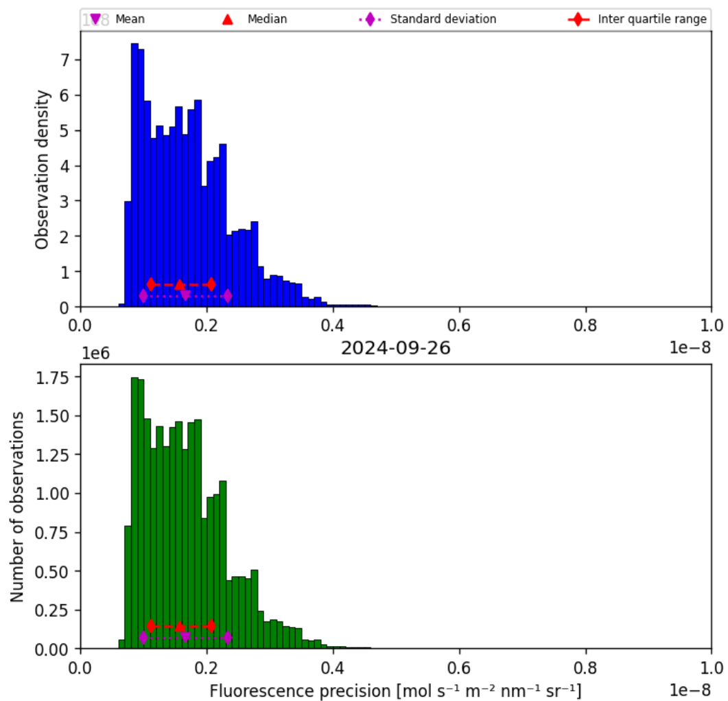
Figure 41: Histogram of “Fluorescence precision” for 2024-09-25 to 2024-09-27
