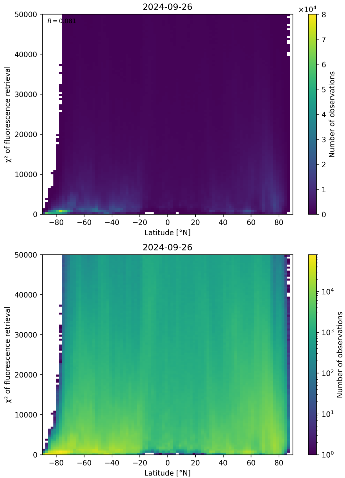
Figure 98: Scatter density plot of “Latitude” against “ \chi^2 of fluorescence retrieval” for 2024-09-25 to 2024-09-27.
