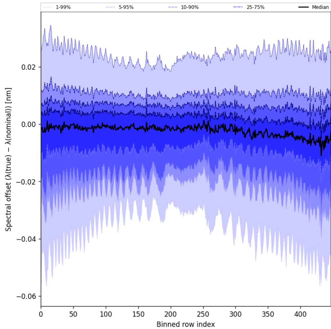
Figure 62: Along track statistics of “Spectral offset ( \lambda_{\text{true}} - \lambda_{\text{nominal}} )” for 2024-09-25 to 2024-09-27
