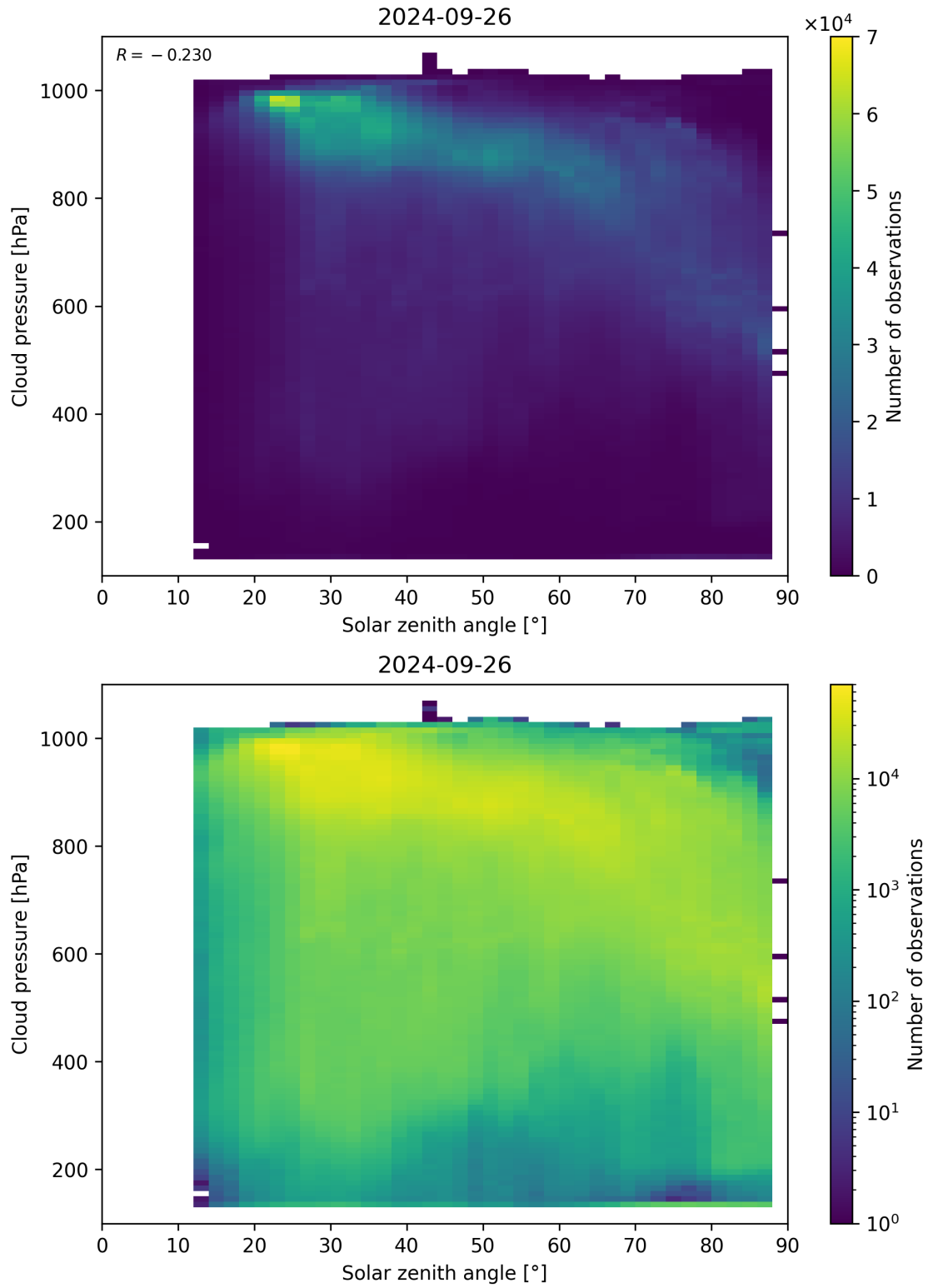
Figure 122: Scatter density plot of “Solar zenith angle” against “Cloud pressure” for 2024-09-25 to 2024-09-27.
