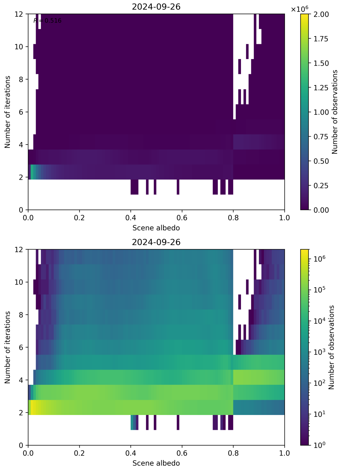
Figure 115: Scatter density plot of “Scene albedo” against “Number of iterations” for 2024-09-25 to 2024-09-27.
