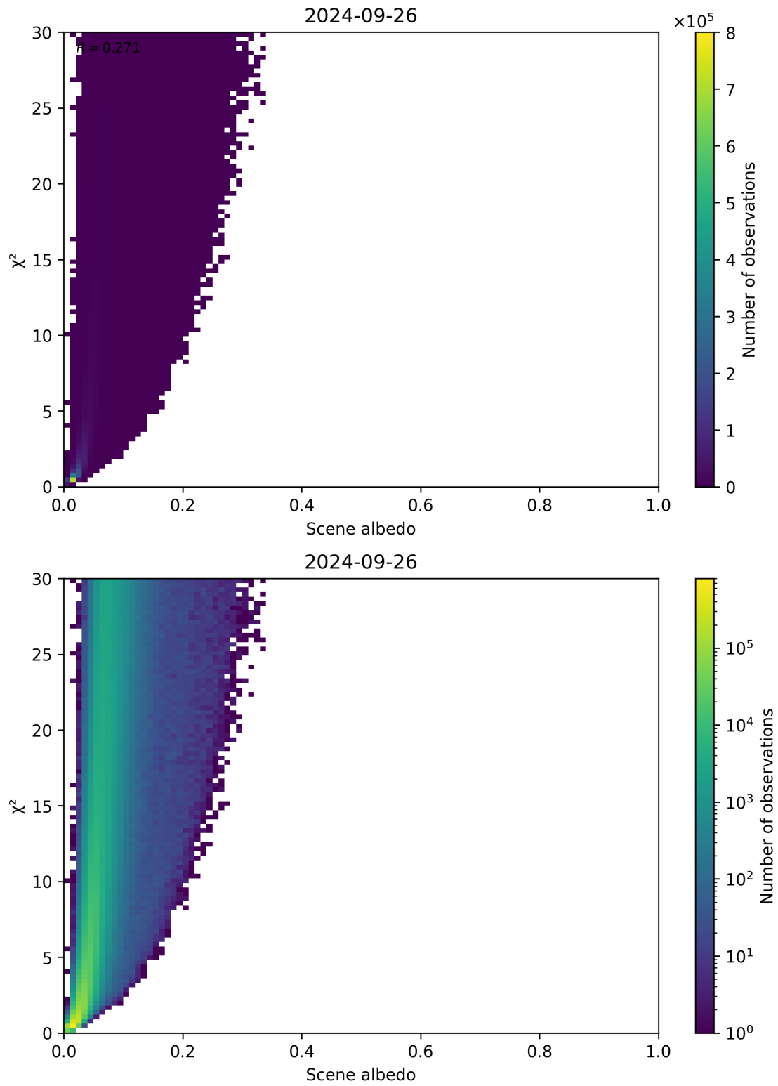
Figure 112: Scatter density plot of “Scene albedo” against “ \chi^2 ” for 2024-09-25 to 2024-09-27.
