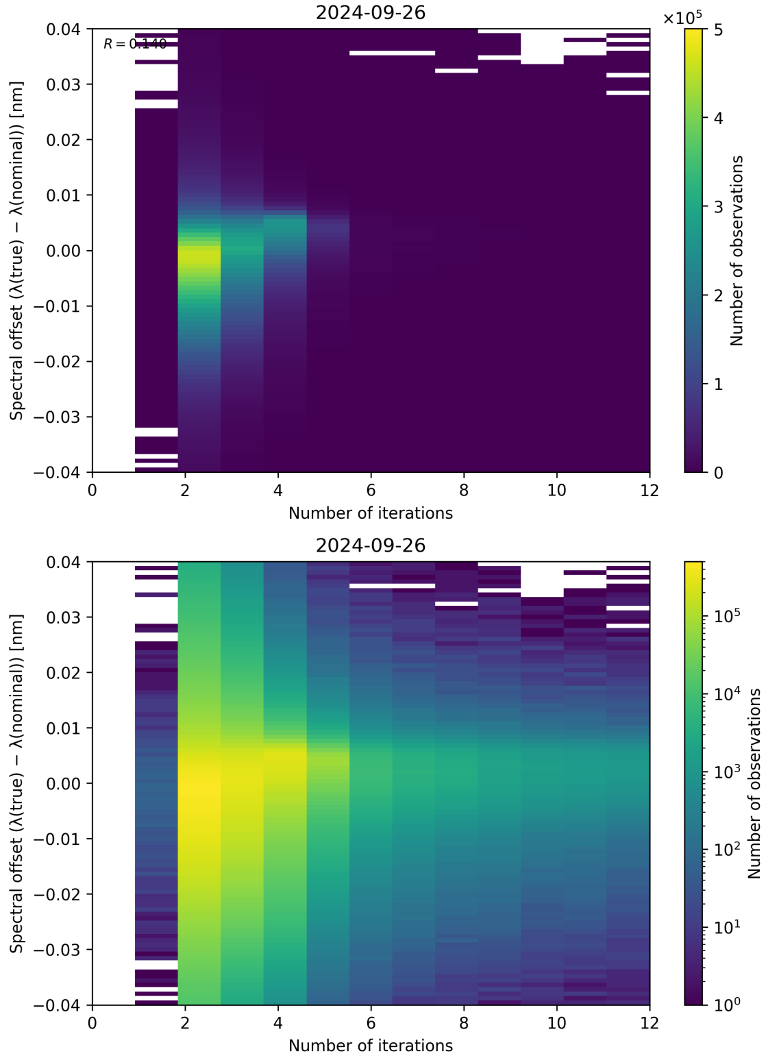
Figure 109: Scatter density plot of “Number of iterations” against “Spectral offset ( \lambda_{\text{true}} - \lambda_{\text{nominal}} )” for 2024-09-25 to 2024-09-27.
