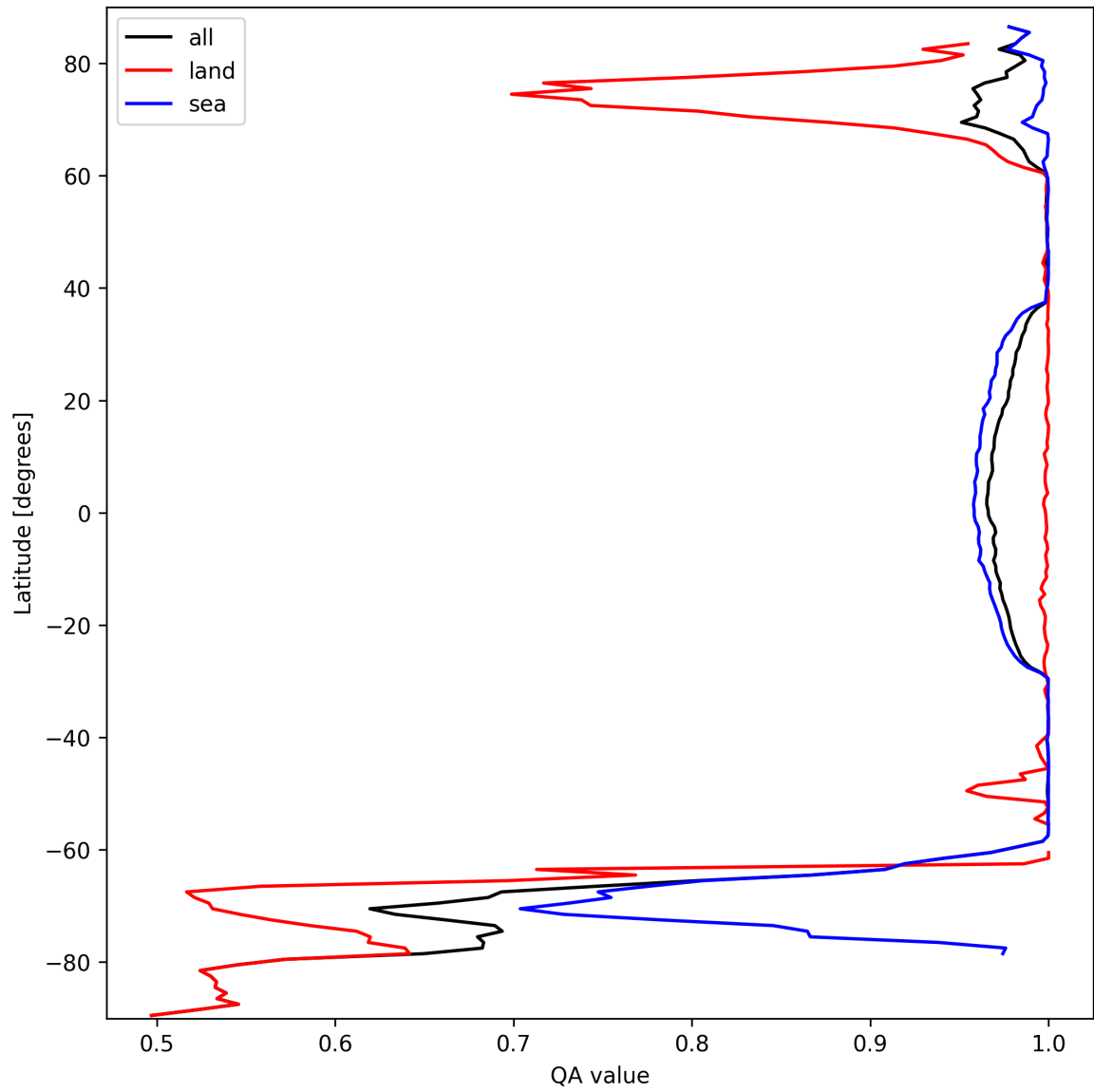
Figure 12: Zonal average of “QA value” for 2024-09-25 to 2024-09-27.
