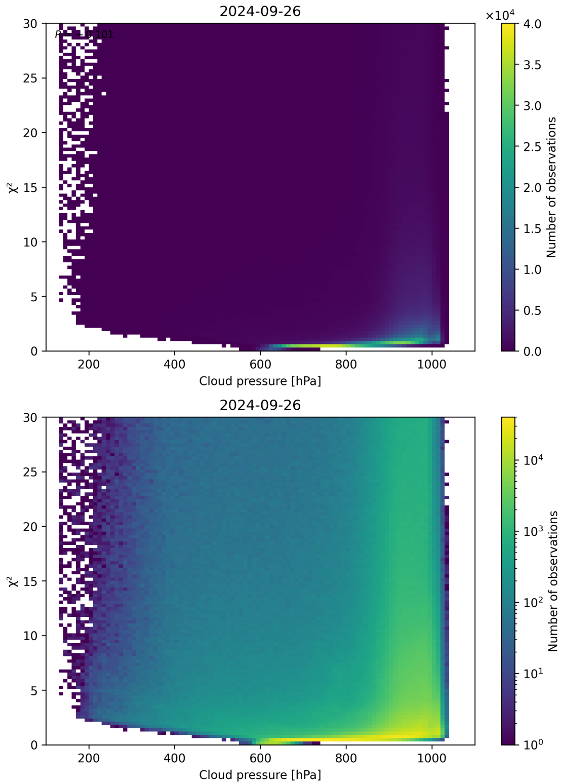
Figure 85: Scatter density plot of “Cloud pressure” against “ \chi^2 ” for 2024-09-25 to 2024-09-27.
