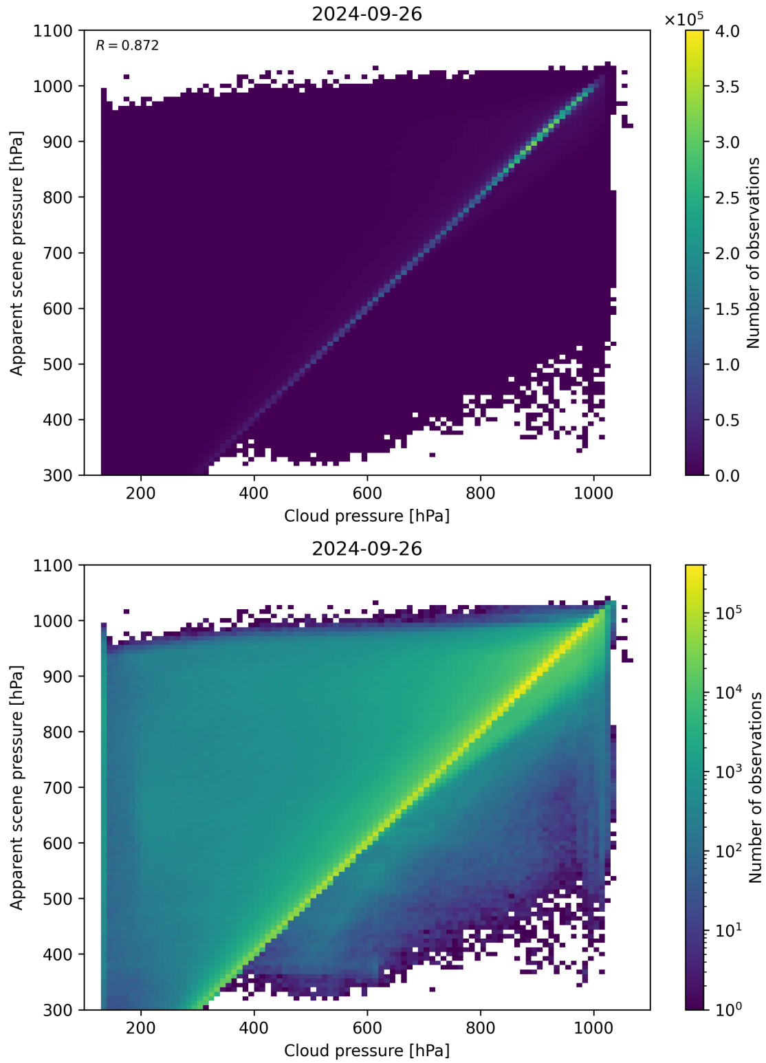
Figure 84: Scatter density plot of “Cloud pressure” against “Apparent scene pressure” for 2024-09-25 to 2024-09-27.
