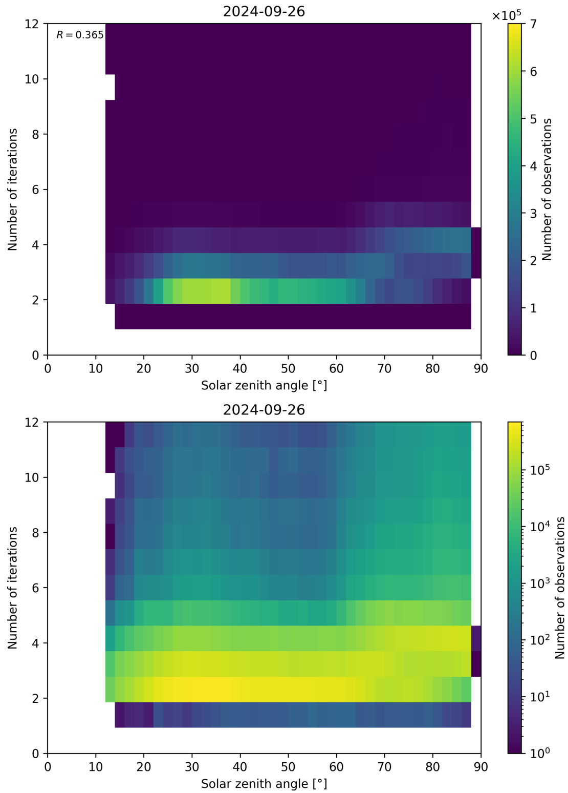
Figure 125: Scatter density plot of “Solar zenith angle” against “Number of iterations” for 2024-09-25 to 2024-09-27.
