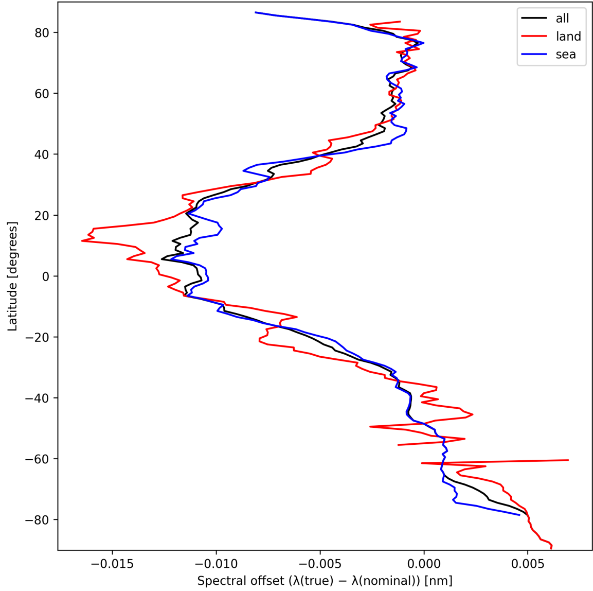
Figure 28: Zonal average of “Spectral offset ( \lambda_{\text{true}} - \lambda_{\text{nominal}} )” for 2024-09-25 to 2024-09-27.
