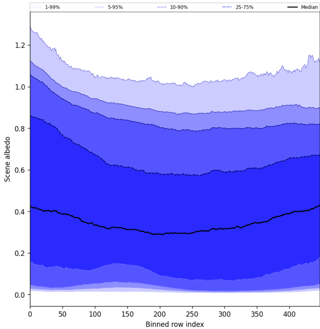
Figure 51: Along track statistics of “Scene albedo” for 2024-09-25 to 2024-09-27
