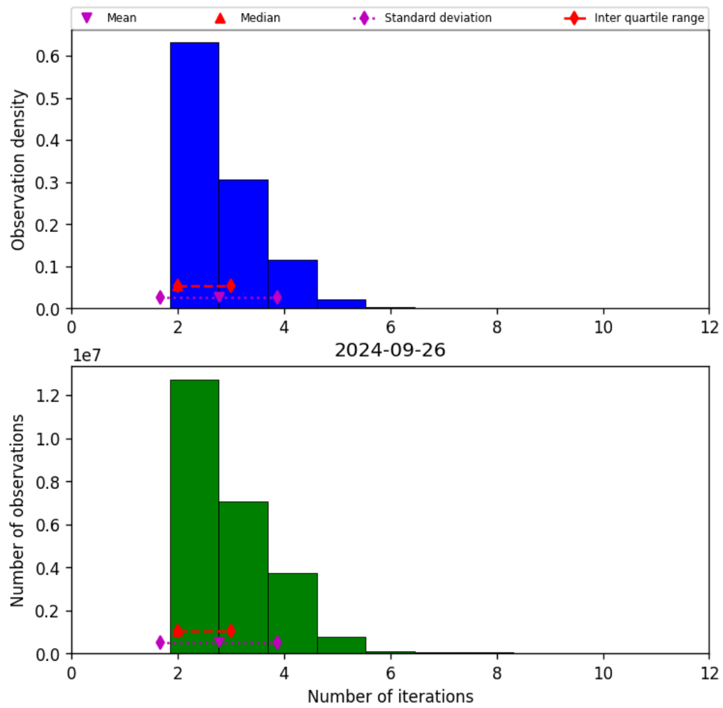
Figure 39: Histogram of “Number of iterations” for 2024-09-25 to 2024-09-27
