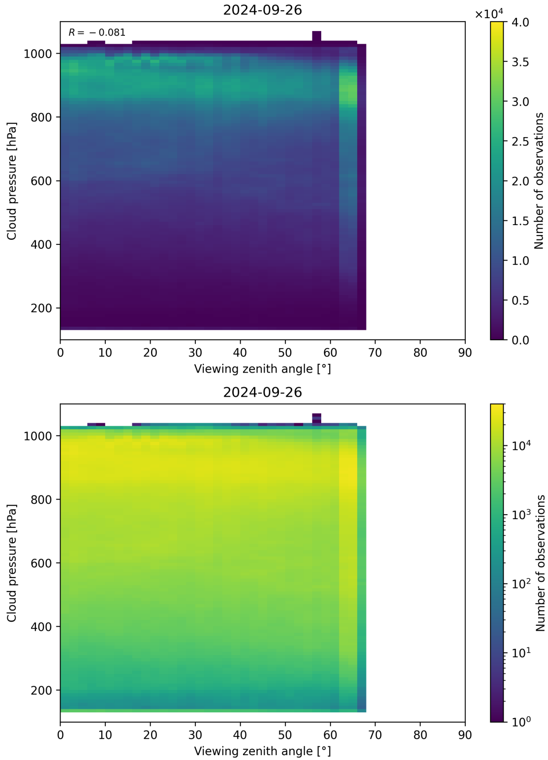
Figure 133: Scatter density plot of “Viewing zenith angle” against “Cloud pressure” for 2024-09-25 to 2024-09-27.
