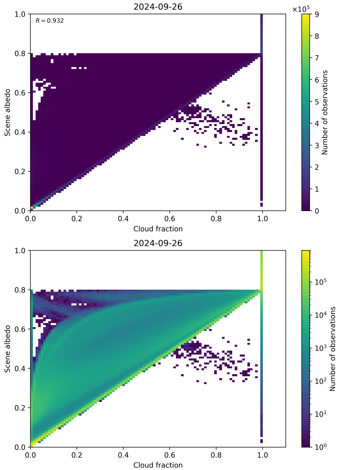
Figure 82: Scatter density plot of “Cloud fraction” against “Scene albedo” for 2024-09-25 to 2024-09-27.
