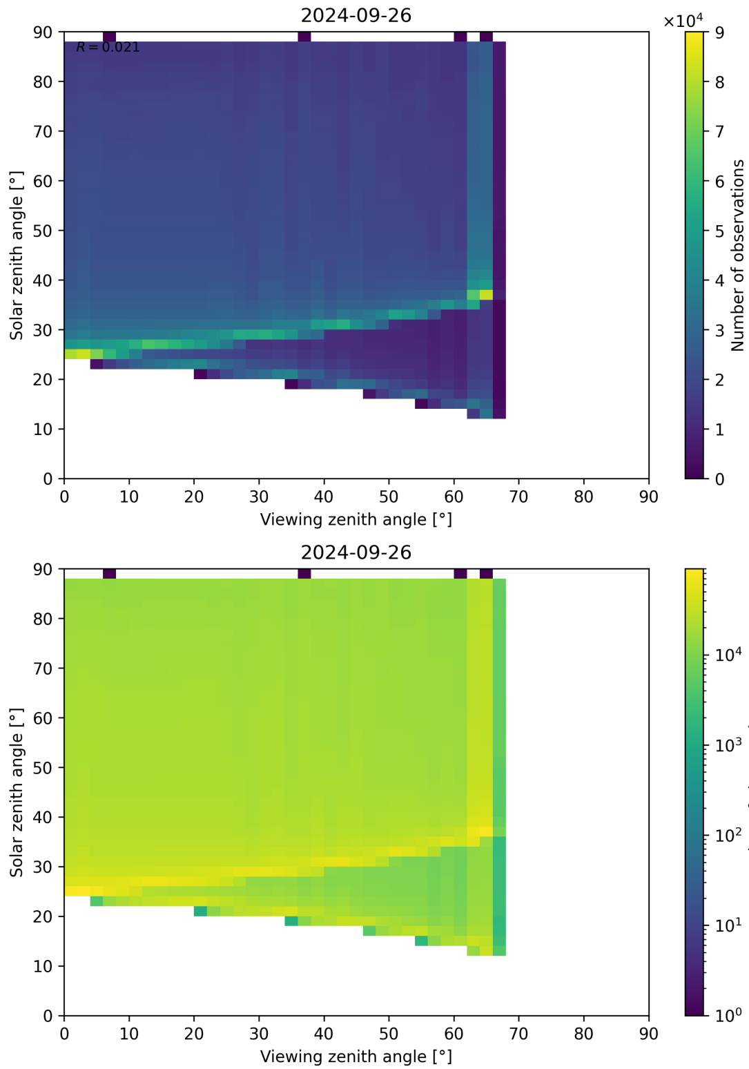
Figure 139: Scatter density plot of “Viewing zenith angle” against “Solar zenith angle” for 2024-09-25 to 2024-09-27.
