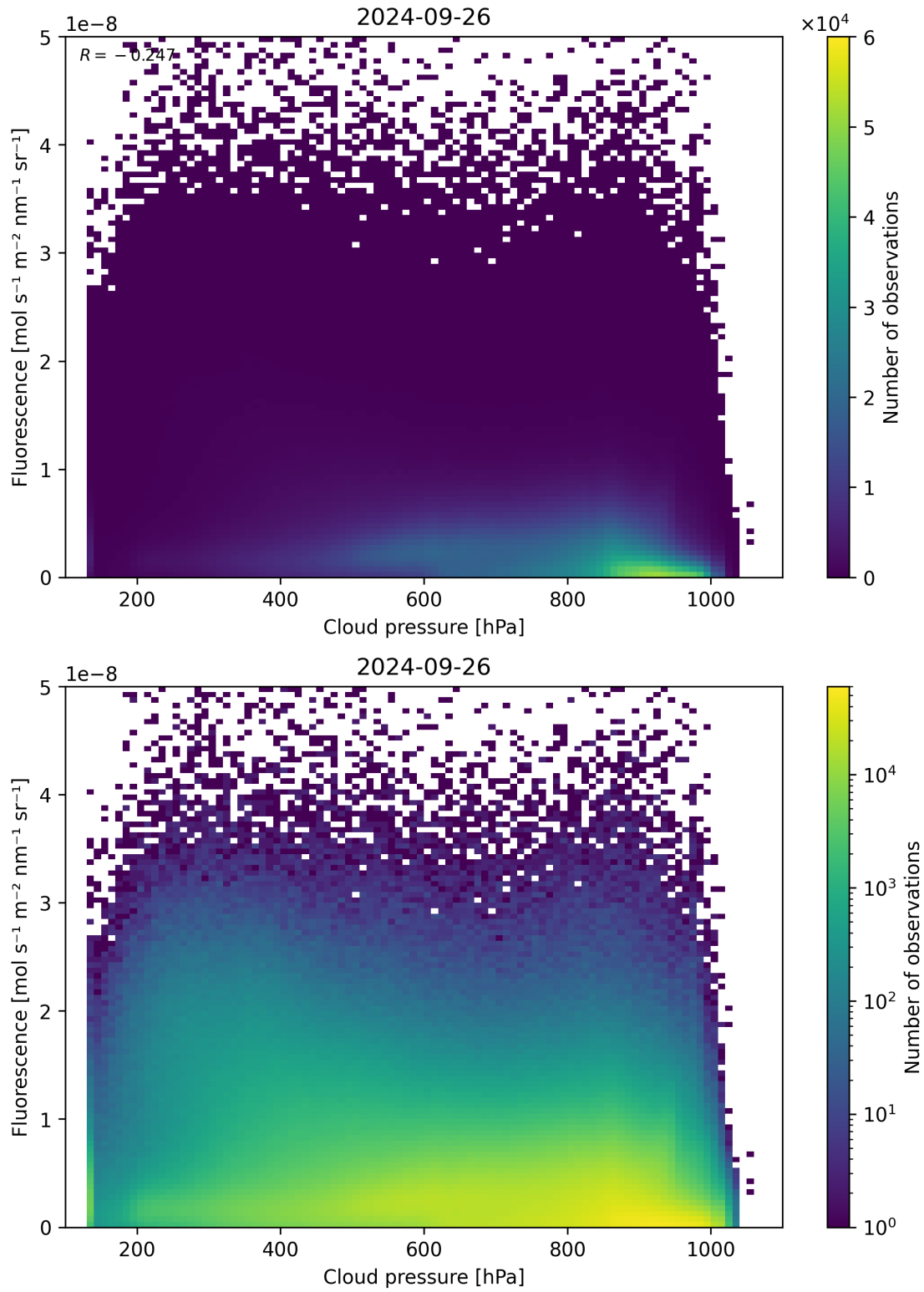
Figure 88: Scatter density plot of “Cloud pressure” against “Fluorescence” for 2024-09-25 to 2024-09-27.
