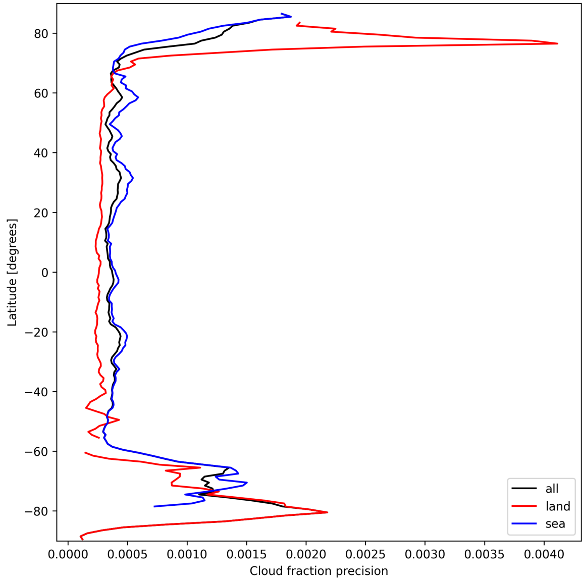
Figure 16: Zonal average of “Cloud fraction precision” for 2024-09-25 to 2024-09-27.
