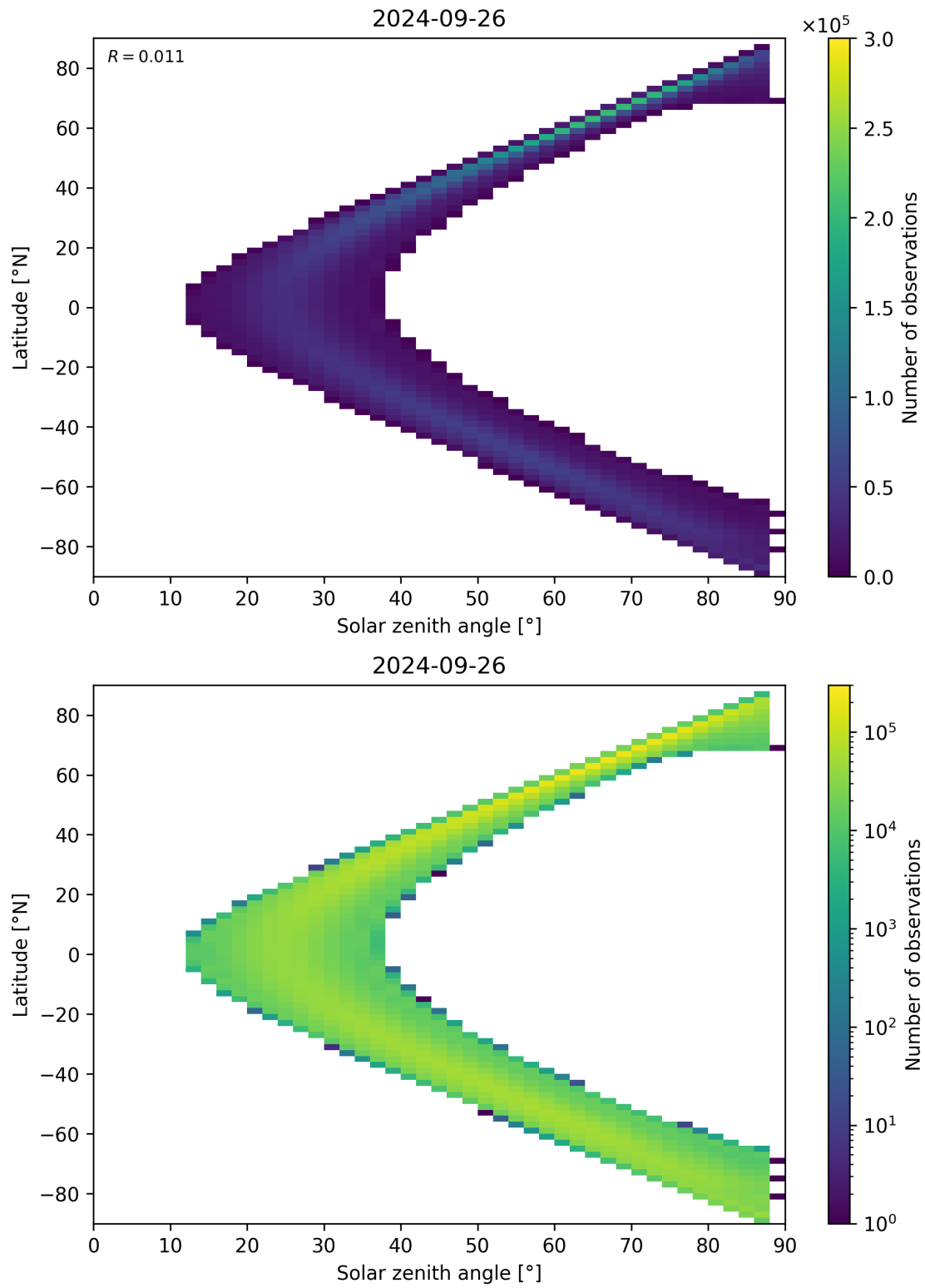
Figure 124: Scatter density plot of “Solar zenith angle” against “Latitude” for 2024-09-25 to 2024-09-27.
