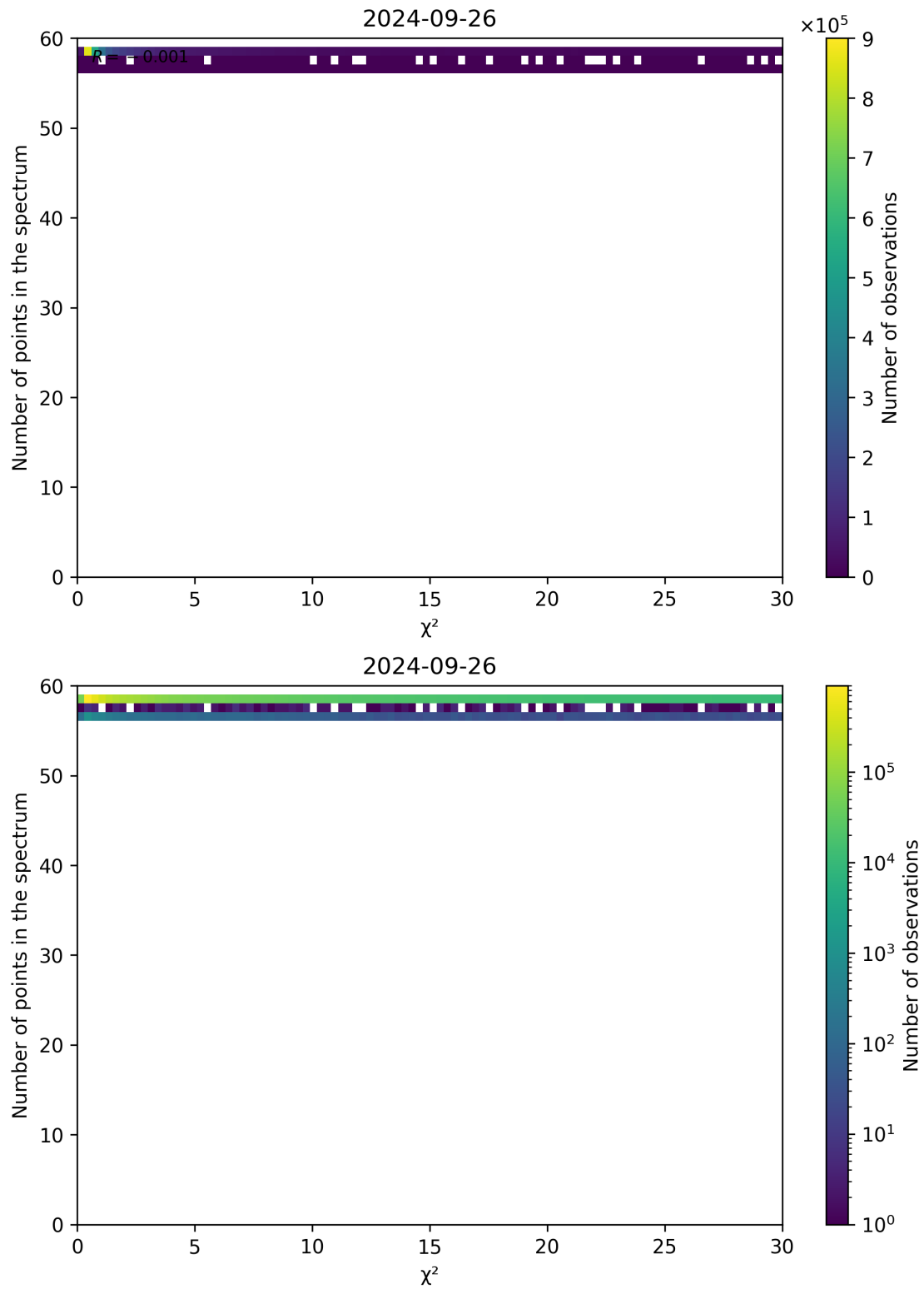
Figure 74: Scatter density plot of “ \chi^2 ” against “Number of points in the spectrum” for 2024-09-25 to 2024-09-27.
