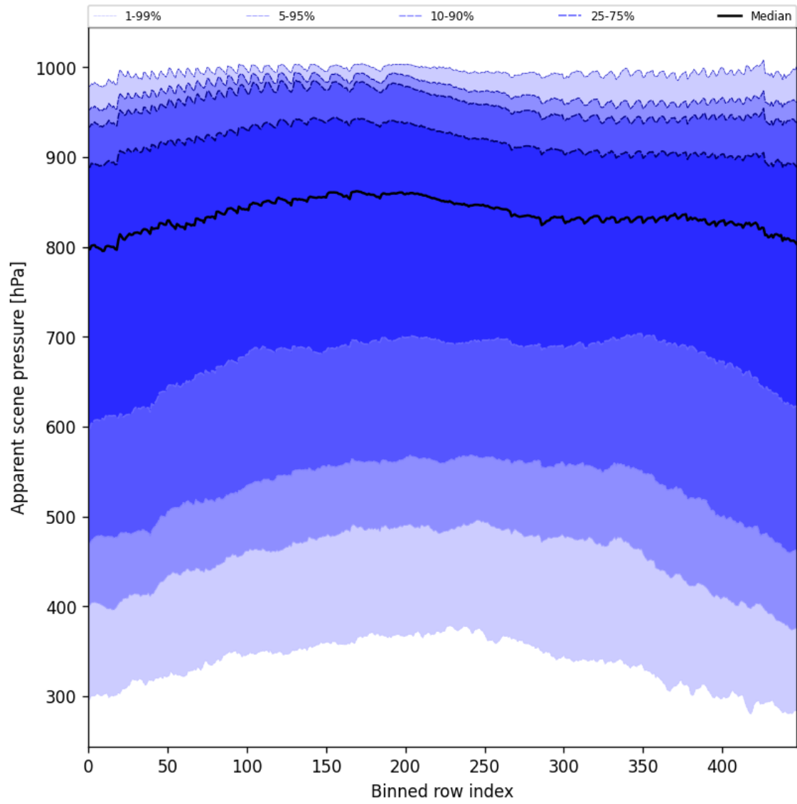
Figure 53: Along track statistics of “Apparent scene pressure” for 2024-09-25 to 2024-09-27
