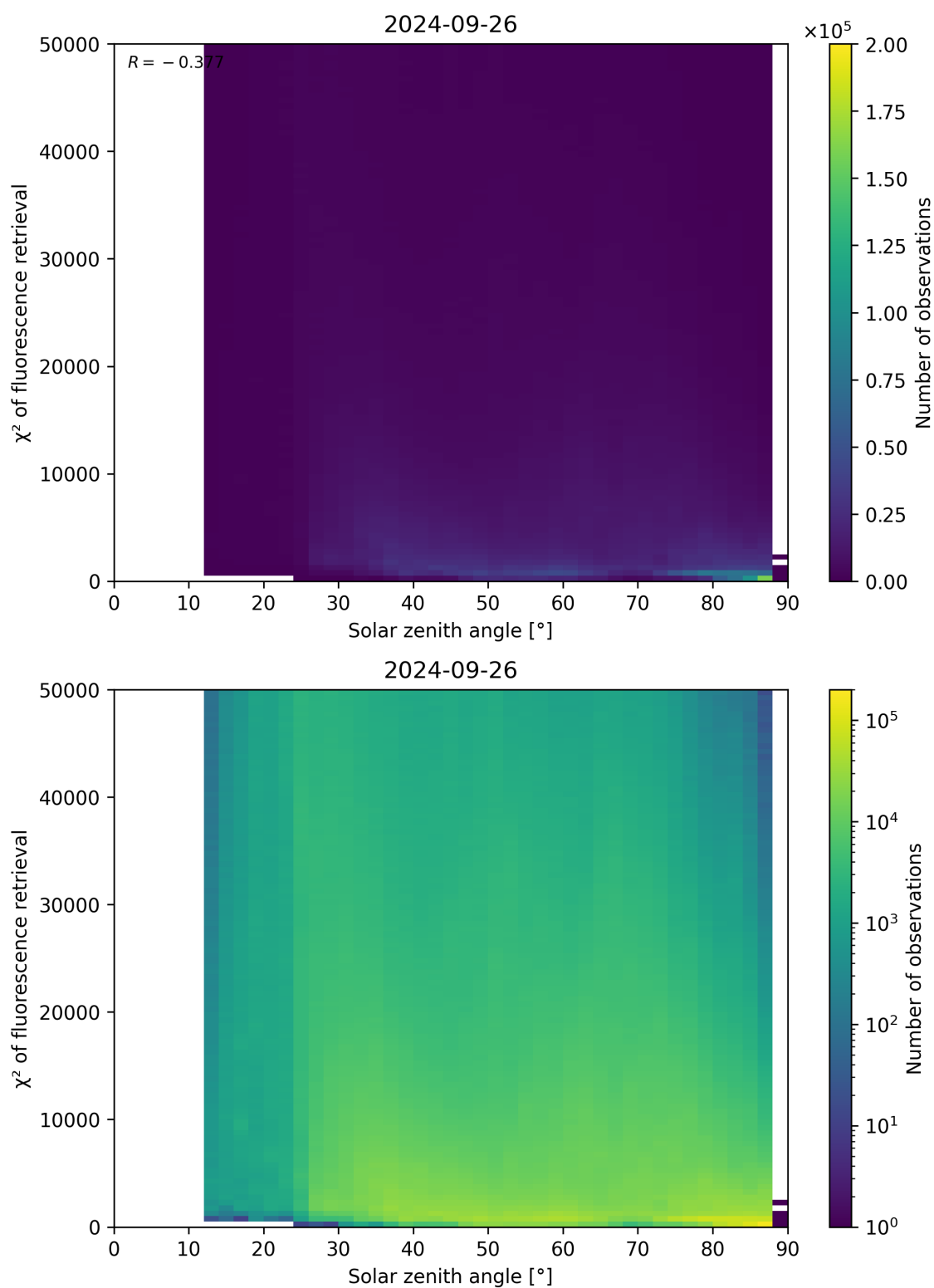
Figure 120: Scatter density plot of “Solar zenith angle” against “ \chi^2 of fluorescence retrieval” for 2024-09-25 to 2024-09-27.
