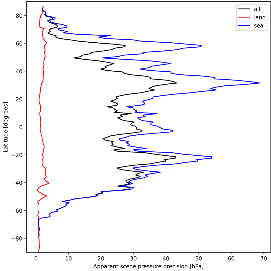
Figure 20: Zonal average of “Apparent scene pressure precision” for 2024-09-25 to 2024-09-27.
