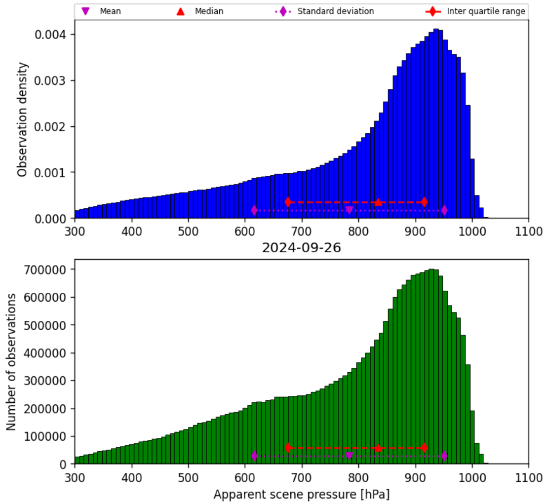
Figure 36: Histogram of “Apparent scene pressure” for 2024-09-25 to 2024-09-27
