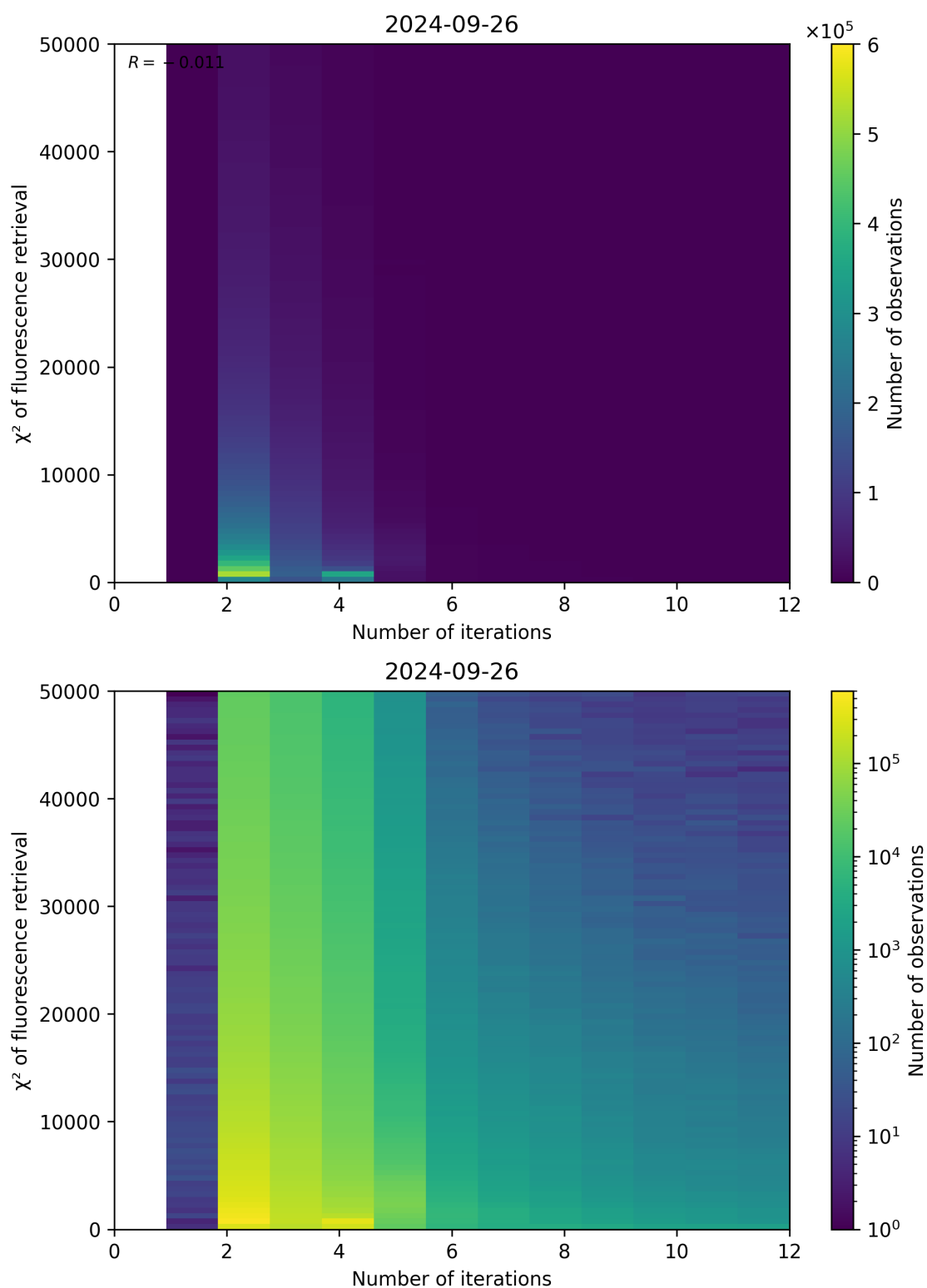
Figure 106: Scatter density plot of “Number of iterations” against “ \chi^2 of fluorescence retrieval” for 2024-09-25 to 2024-09-27.
