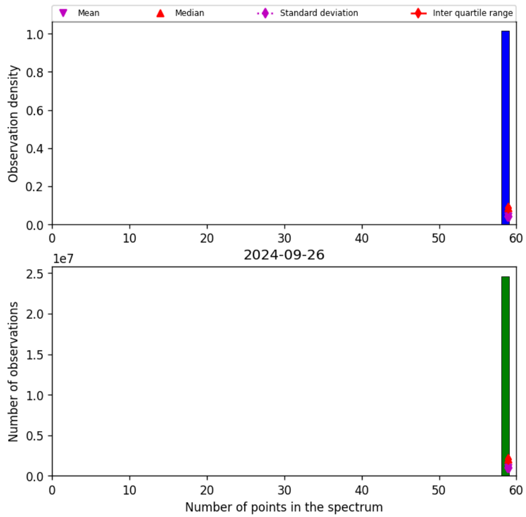
Figure 44: Histogram of “Number of points in the spectrum” for 2024-09-25 to 2024-09-27
