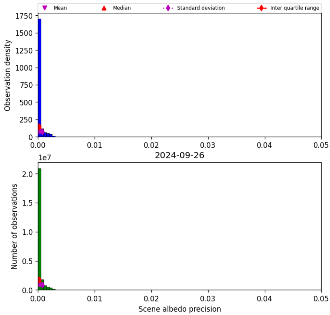
Figure 35: Histogram of “Scene albedo precision” for 2024-09-25 to 2024-09-27
