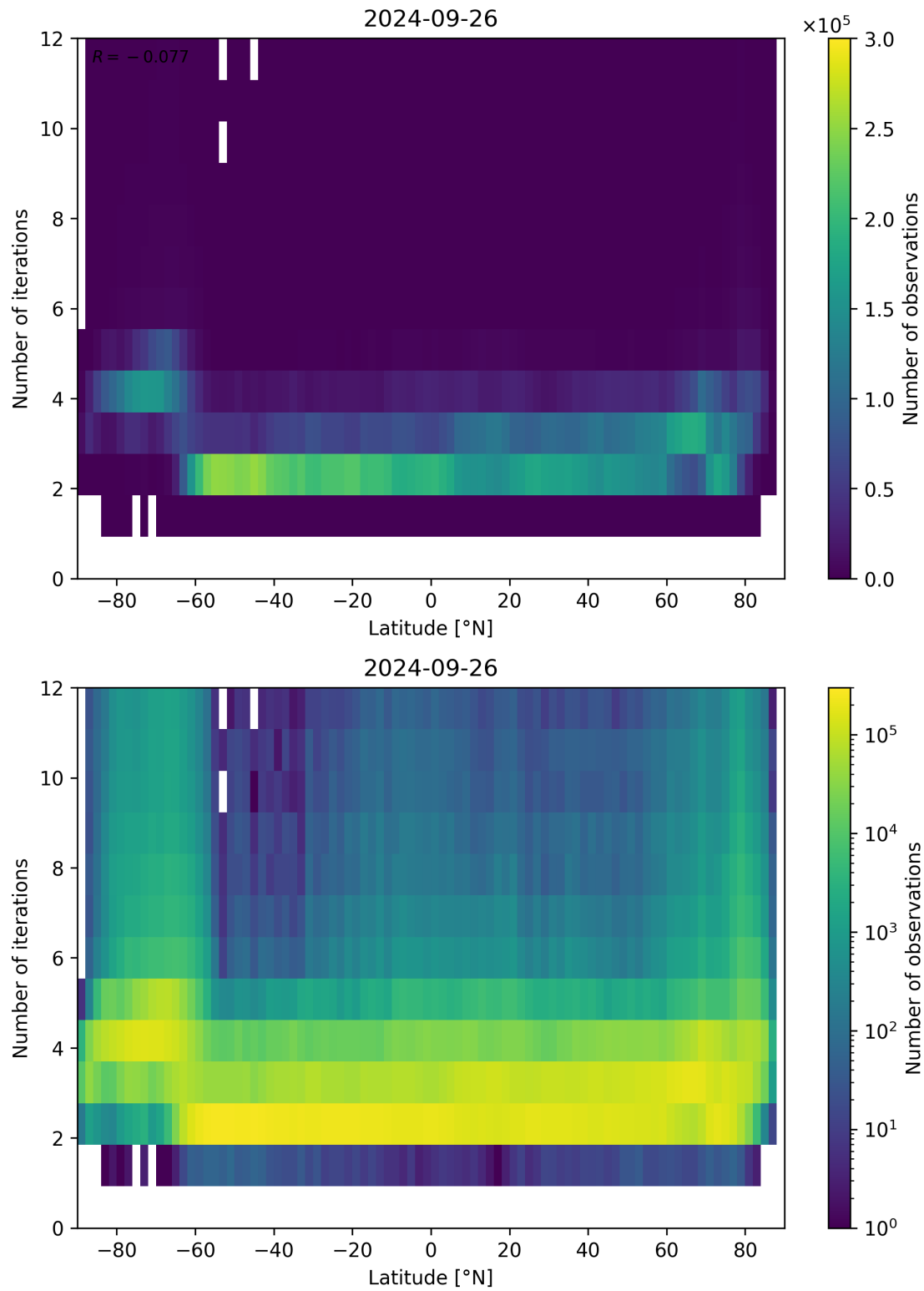
Figure 102: Scatter density plot of “Latitude” against “Number of iterations” for 2024-09-25 to 2024-09-27.
