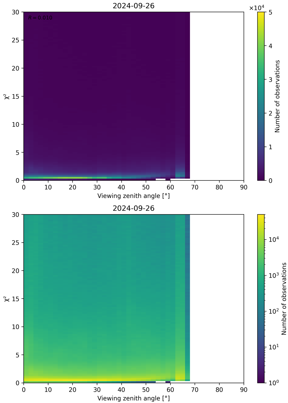
Figure 130: Scatter density plot of “Viewing zenith angle” against “ \chi^2 ” for 2024-09-25 to 2024-09-27.
