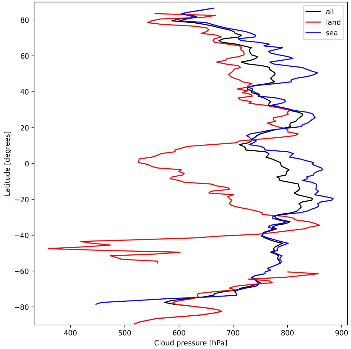
Figure 13: Zonal average of “Cloud pressure” for 2024-09-25 to 2024-09-27.
