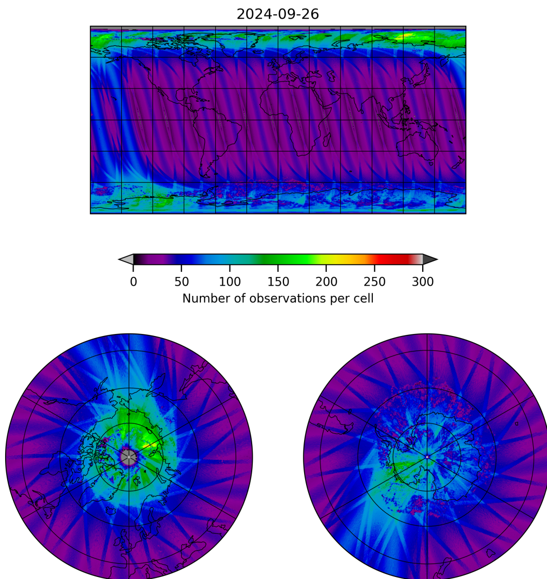
Figure 11: Map of the number of observations for 2024-09-25 to 2024-09-27
