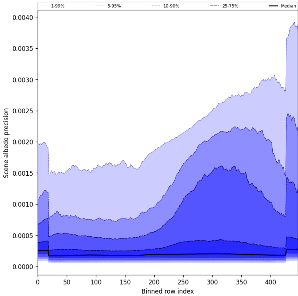
Figure 52: Along track statistics of “Scene albedo precision” for 2024-09-25 to 2024-09-27
