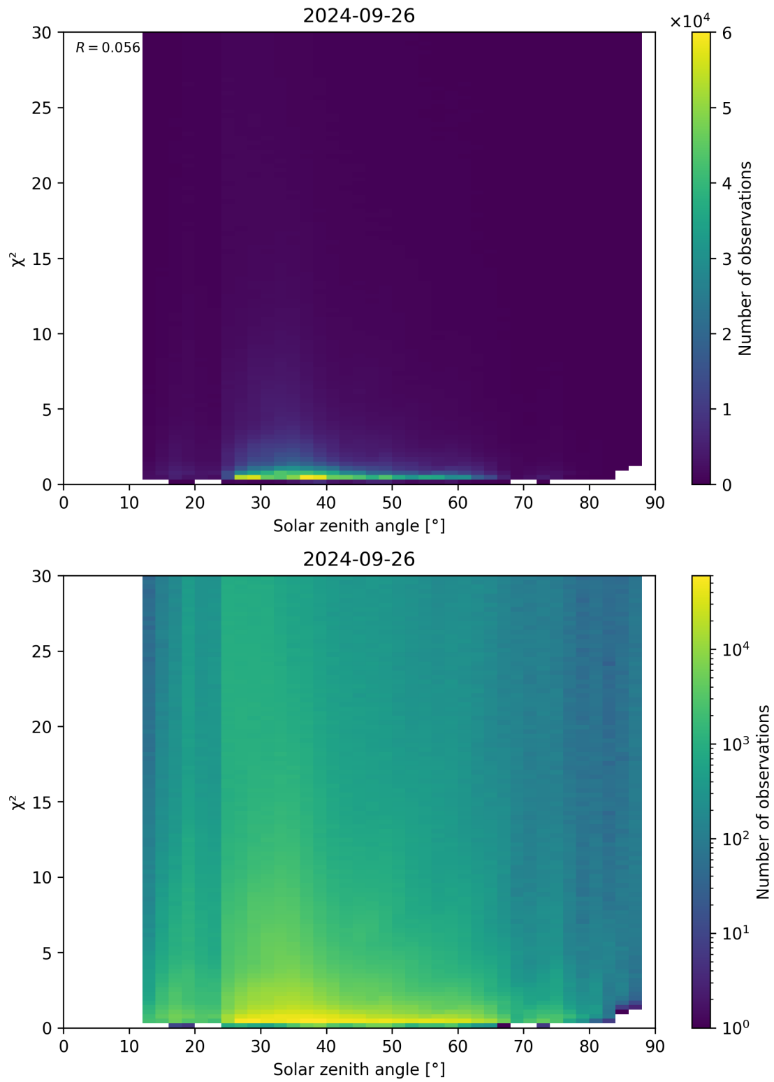
Figure 119: Scatter density plot of “Solar zenith angle” against “ \chi^2 ” for 2024-09-25 to 2024-09-27.
