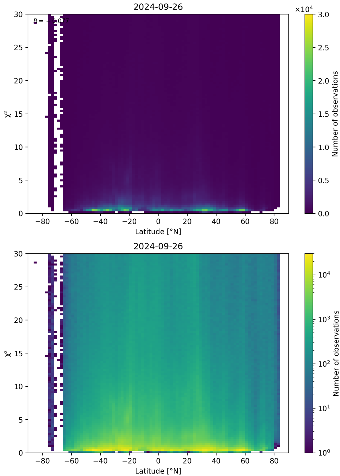
Figure 97: Scatter density plot of “Latitude” against “ \chi^2 ” for 2024-09-25 to 2024-09-27.
