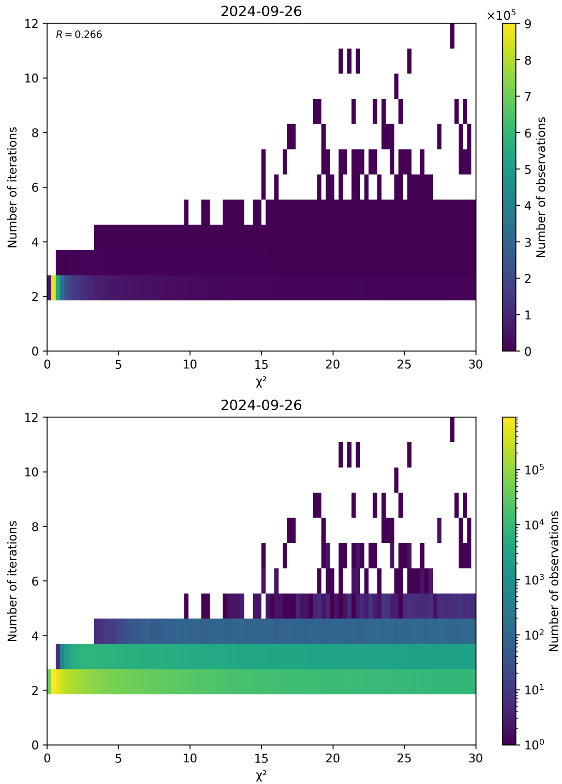
Figure 73: Scatter density plot of “ \chi^2 ” against “Number of iterations” for 2024-09-25 to 2024-09-27.
