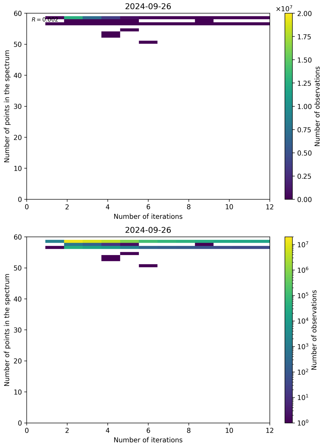
Figure 108: Scatter density plot of “Number of iterations” against “Number of points in the spectrum” for 2024-09-25 to 2024-09-27.
