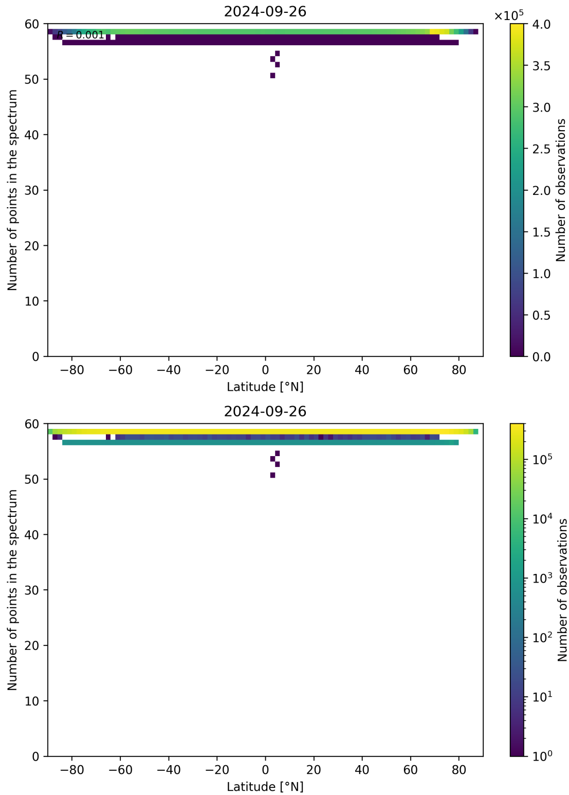
Figure 103: Scatter density plot of “Latitude” against “Number of points in the spectrum” for 2024-09-25 to 2024-09-27.
