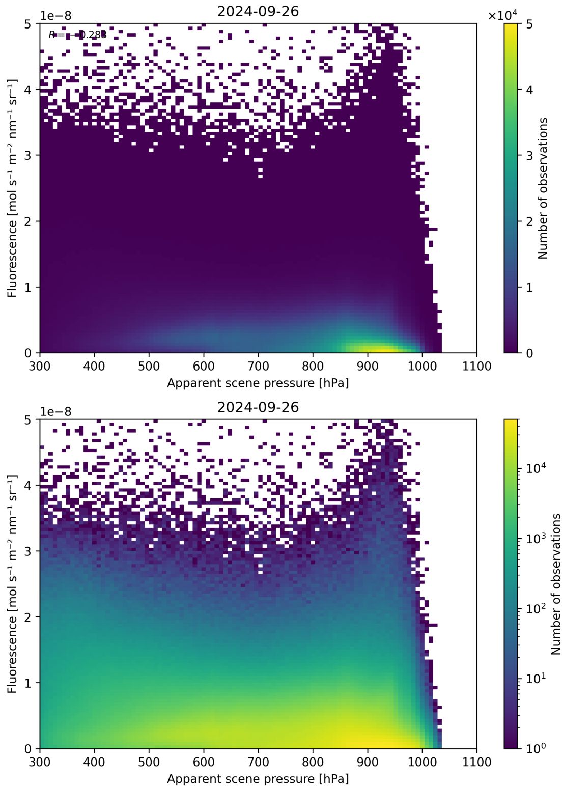
Figure 65: Scatter density plot of “Apparent scene pressure” against “Fluorescence” for 2024-09-25 to 2024-09-27.
