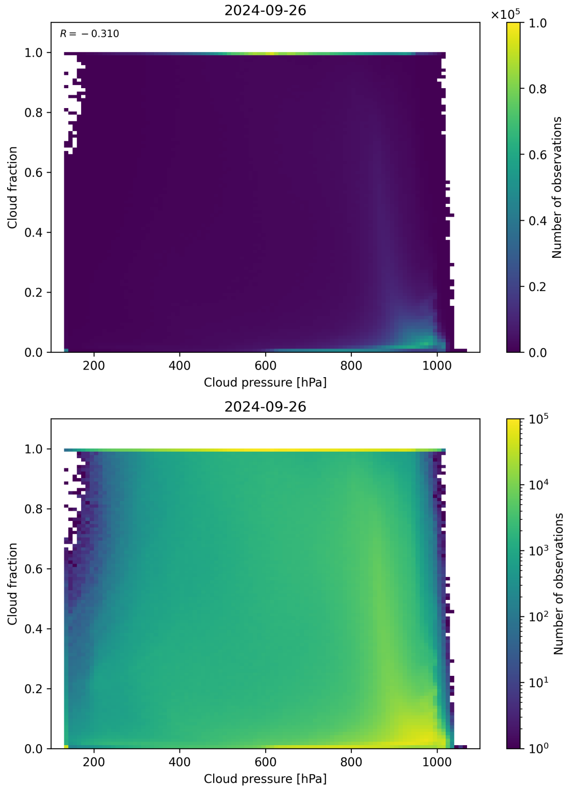
Figure 87: Scatter density plot of “Cloud pressure” against “Cloud fraction” for 2024-09-25 to 2024-09-27.
