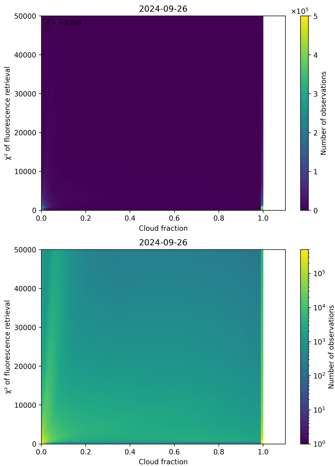
Figure 78: Scatter density plot of “Cloud fraction” against “ \chi^2 of fluorescence retrieval” for 2024-09-25 to 2024-09-27.
