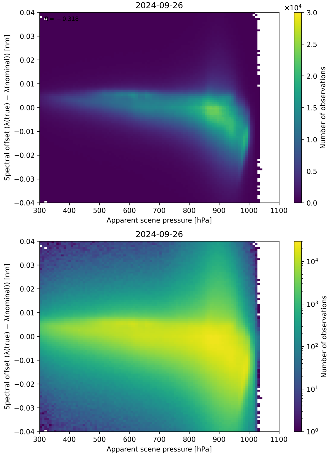
Figure 68: Scatter density plot of “Apparent scene pressure” against “Spectral offset ( \lambda_{\text{true}} - \lambda_{\text{nominal}} )” for 2024-09-25 to 2024-09-27.
