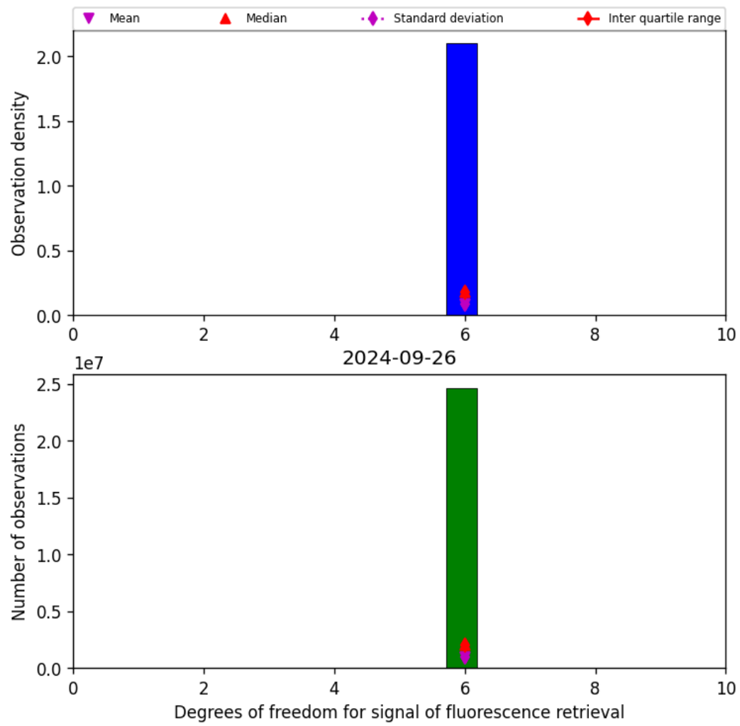
Figure 43: Histogram of "Degrees of freedom for signal of fluorescence retrieval" for 2024-09-25 to 2024-09-27
