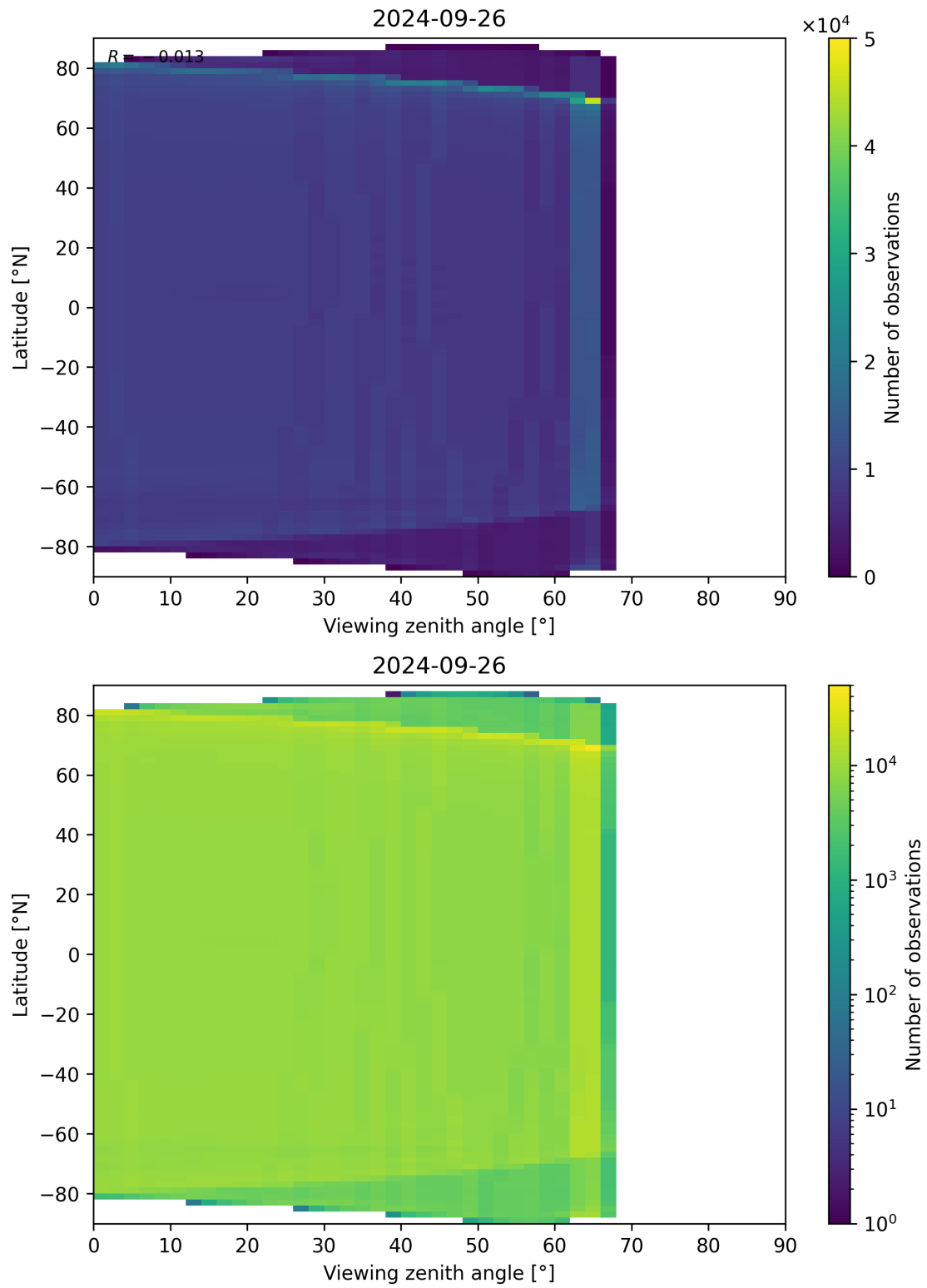
Figure 135: Scatter density plot of “Viewing zenith angle” against “Latitude” for 2024-09-25 to 2024-09-27.
