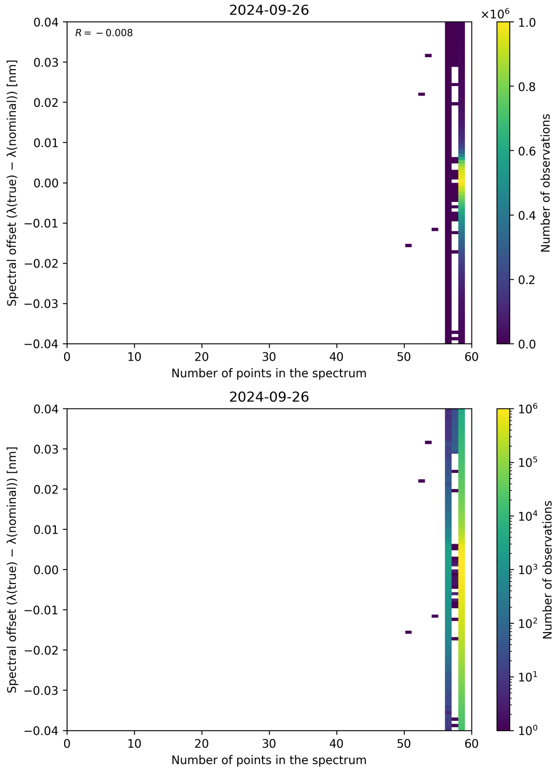
Figure 110: Scatter density plot of “Number of points in the spectrum” against “Spectral offset ( \lambda_{\text{true}} - \lambda_{\text{nominal}} )” for 2024-09-25 to 2024-09-27.
