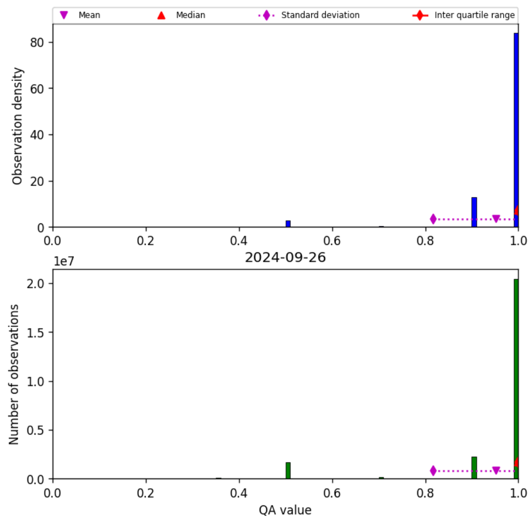
Figure 29: Histogram of “QA value” for 2024-09-25 to 2024-09-27
