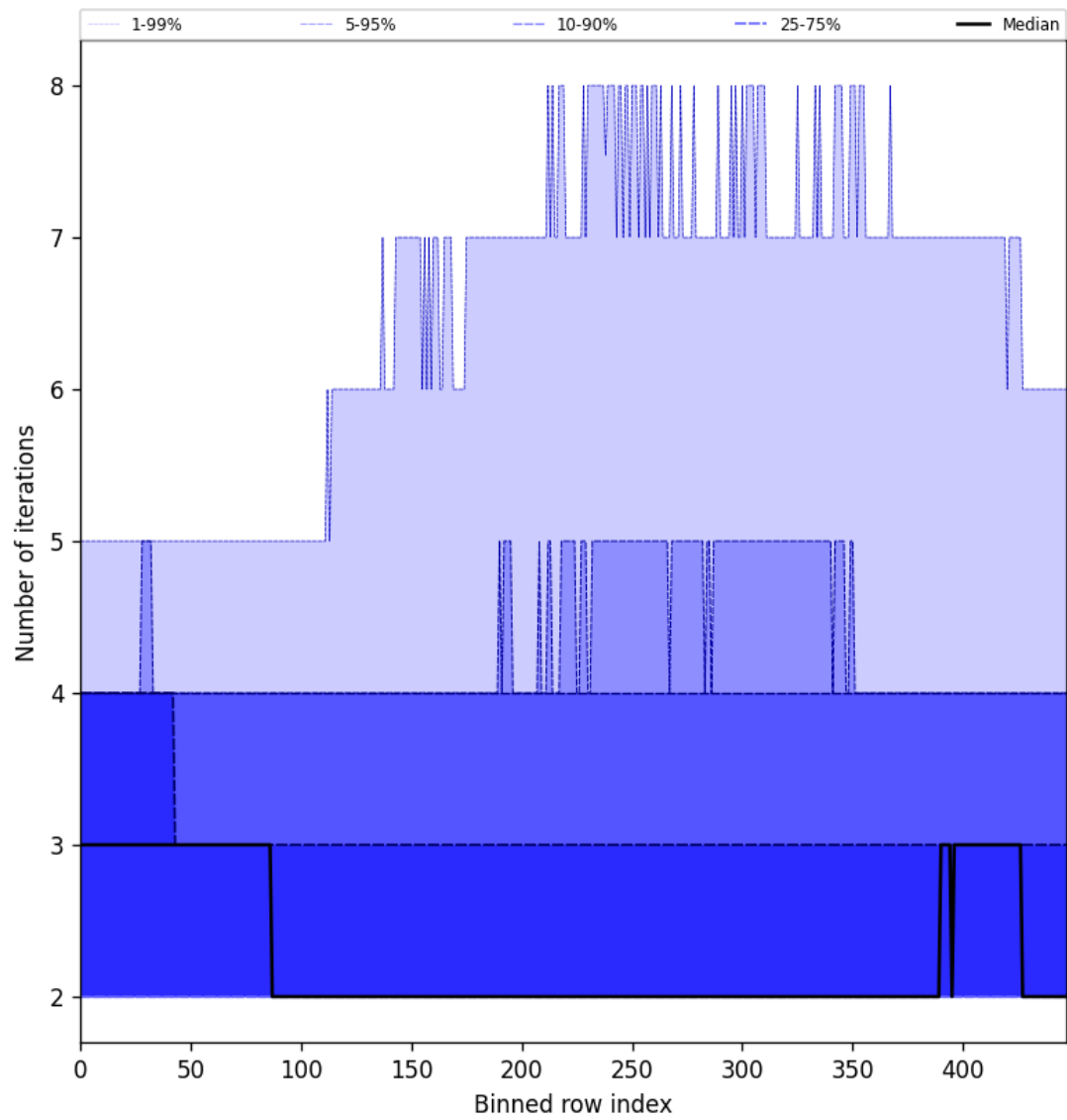
Figure 56: Along track statistics of “Number of iterations” for 2024-09-25 to 2024-09-27
