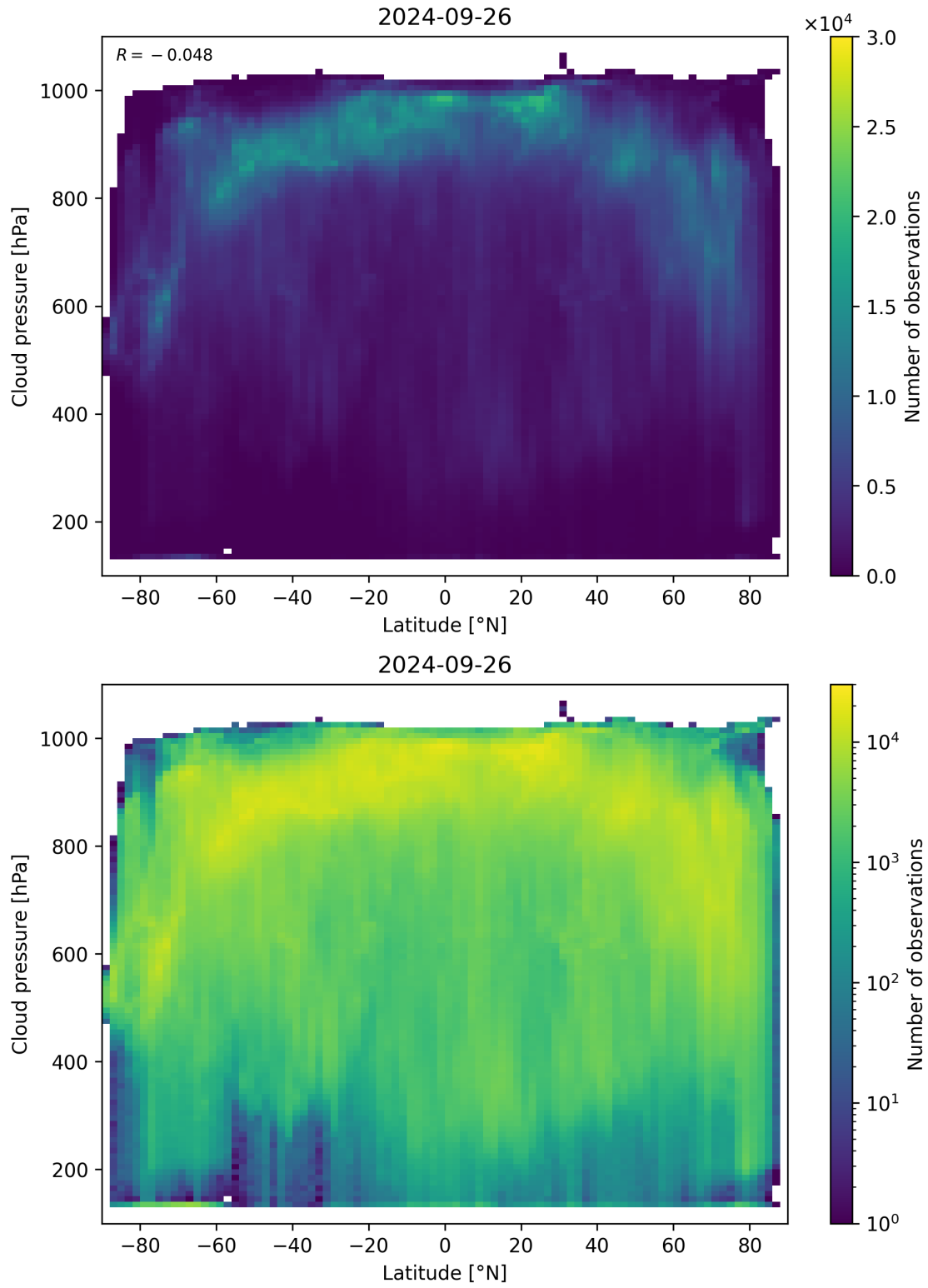
Figure 100: Scatter density plot of “Latitude” against “Cloud pressure” for 2024-09-25 to 2024-09-27.
