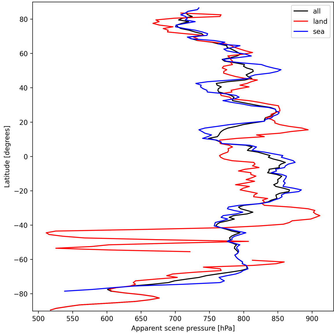
Figure 19: Zonal average of “Apparent scene pressure” for 2024-09-25 to 2024-09-27.
