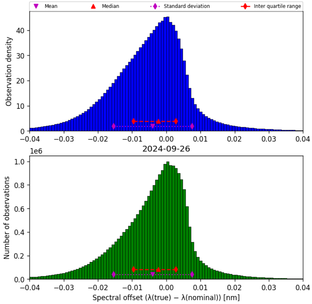
Figure 45: Histogram of “Spectral offset ( \lambda_{\text{true}} - \lambda_{\text{nominal}} )” for 2024-09-25 to 2024-09-27
