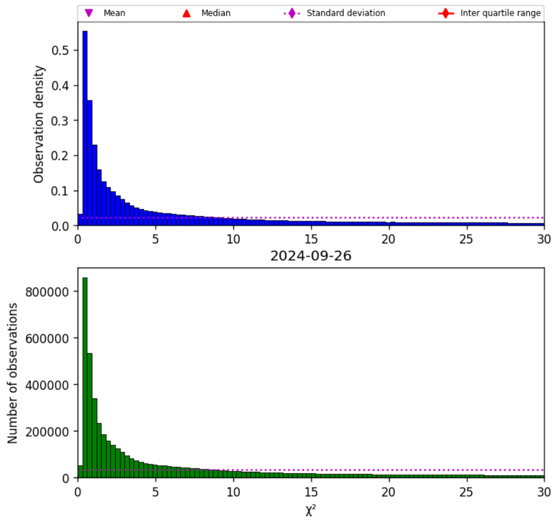
Figure 38: Histogram of “ \chi^2 ” for 2024-09-25 to 2024-09-27
