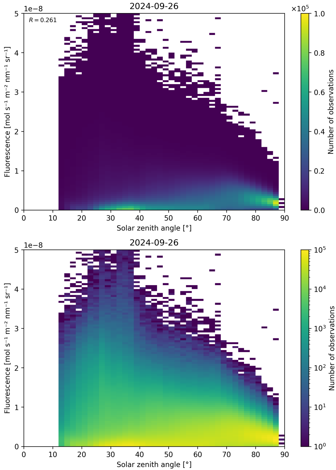
Figure 123: Scatter density plot of “Solar zenith angle” against “Fluorescence” for 2024-09-25 to 2024-09-27.
