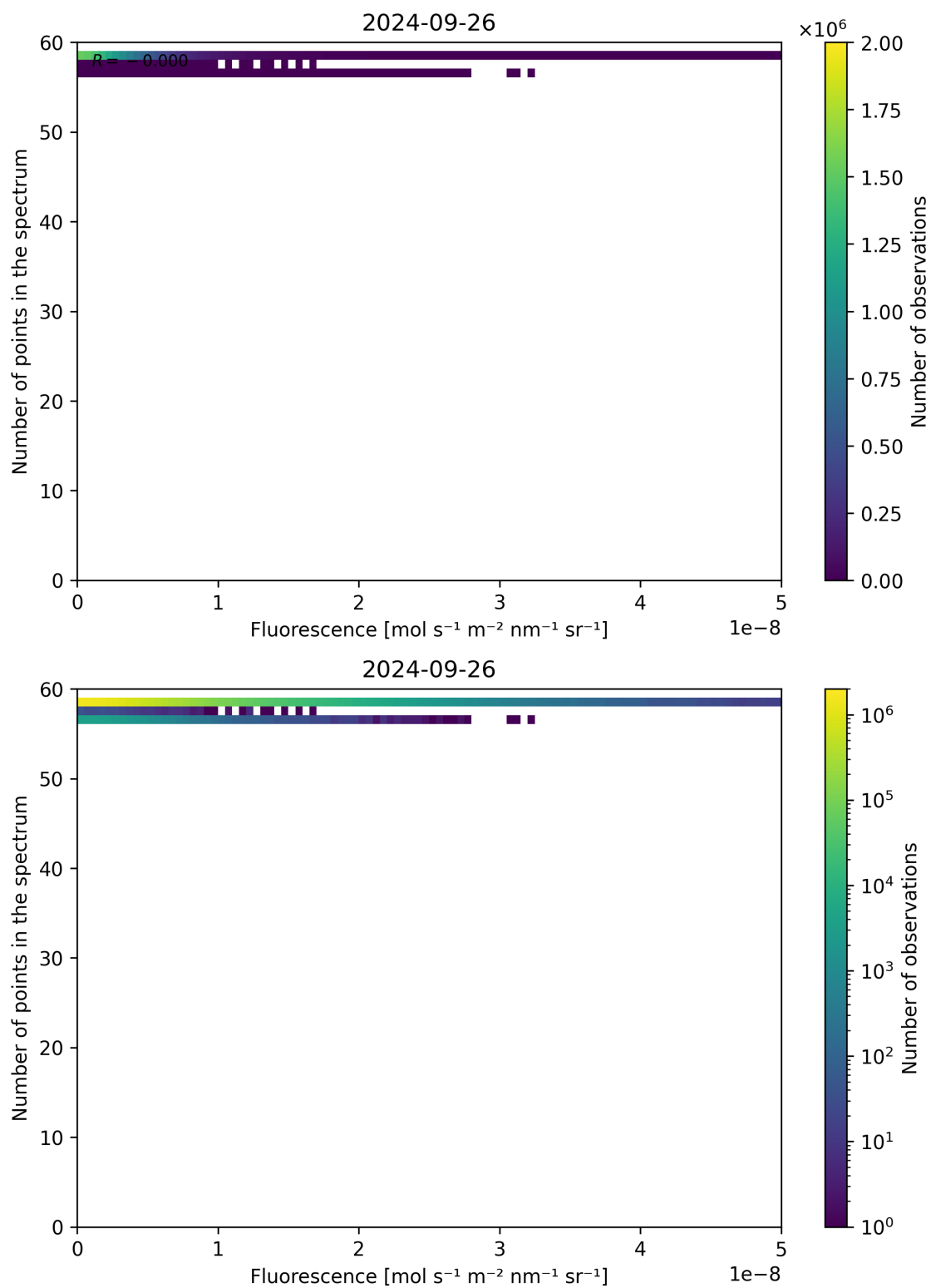
Figure 94: Scatter density plot of “Fluorescence” against “Number of points in the spectrum” for 2024-09-25 to 2024-09-27.
