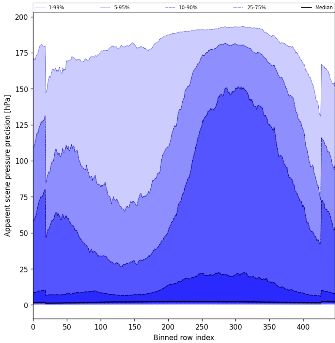
Figure 54: Along track statistics of “Apparent scene pressure precision” for 2024-09-25 to 2024-09-27
