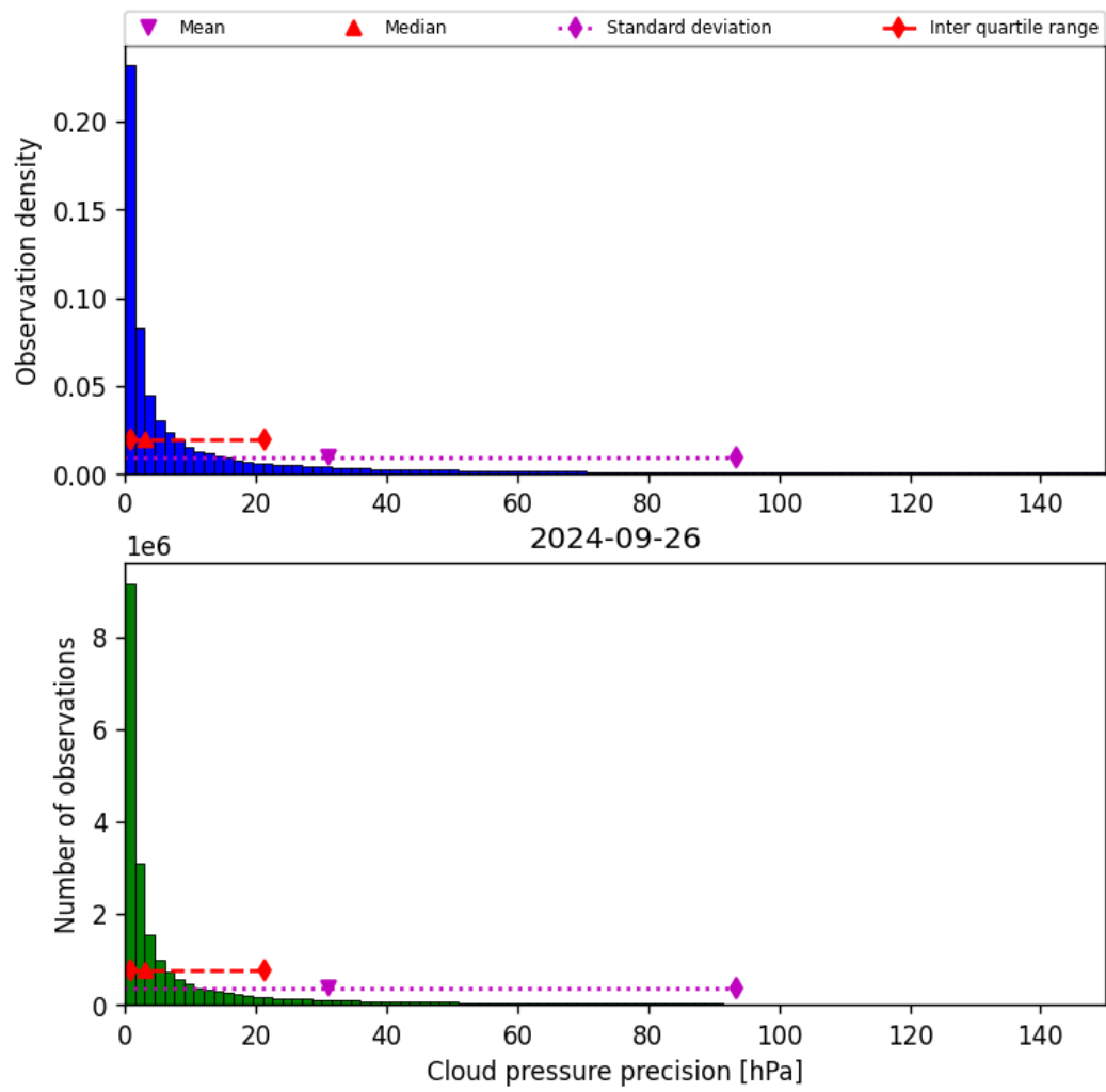
Figure 31: Histogram of “Cloud pressure precision” for 2024-09-25 to 2024-09-27
