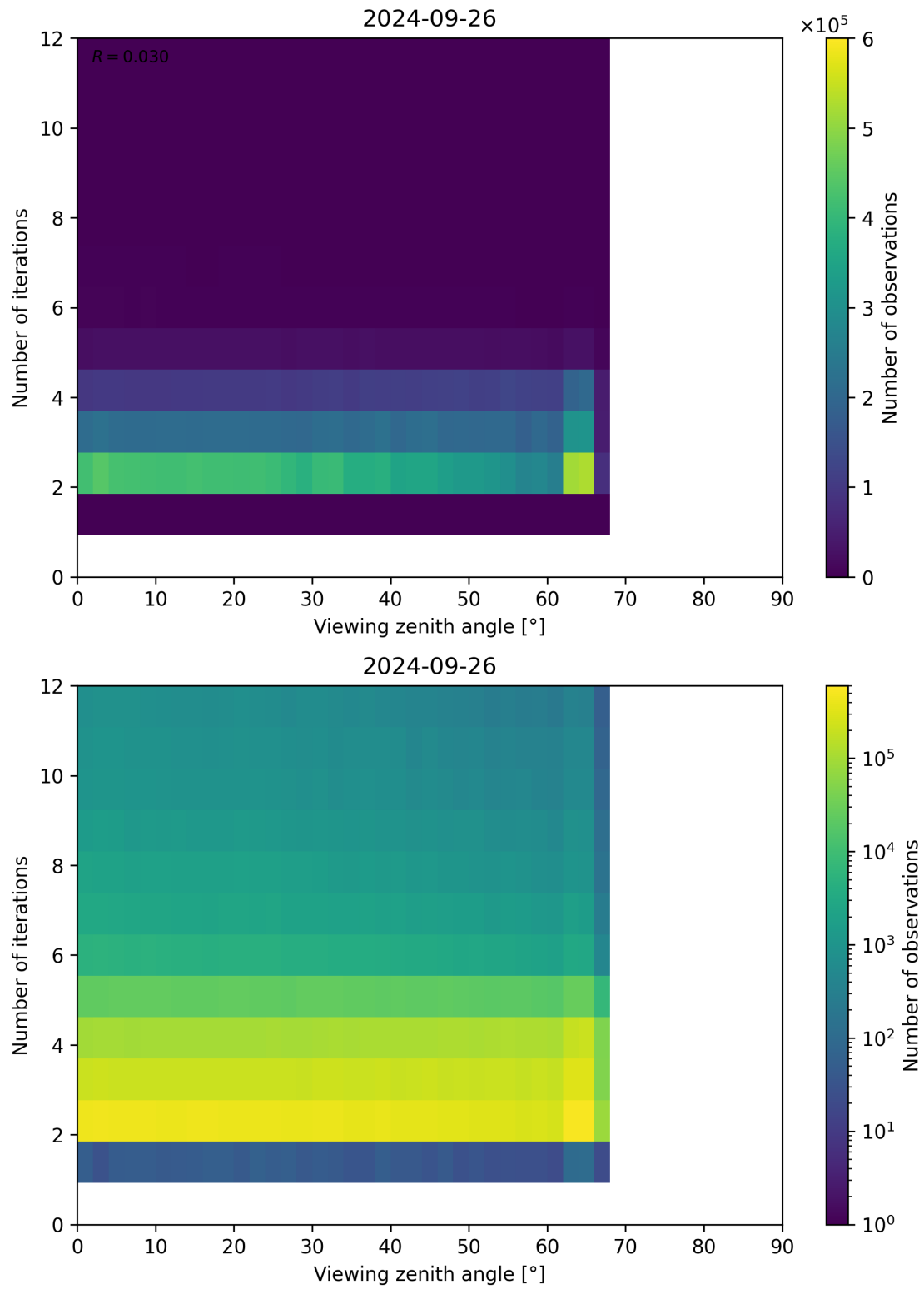
Figure 136: Scatter density plot of “Viewing zenith angle” against “Number of iterations” for 2024-09-25 to 2024-09-27.
