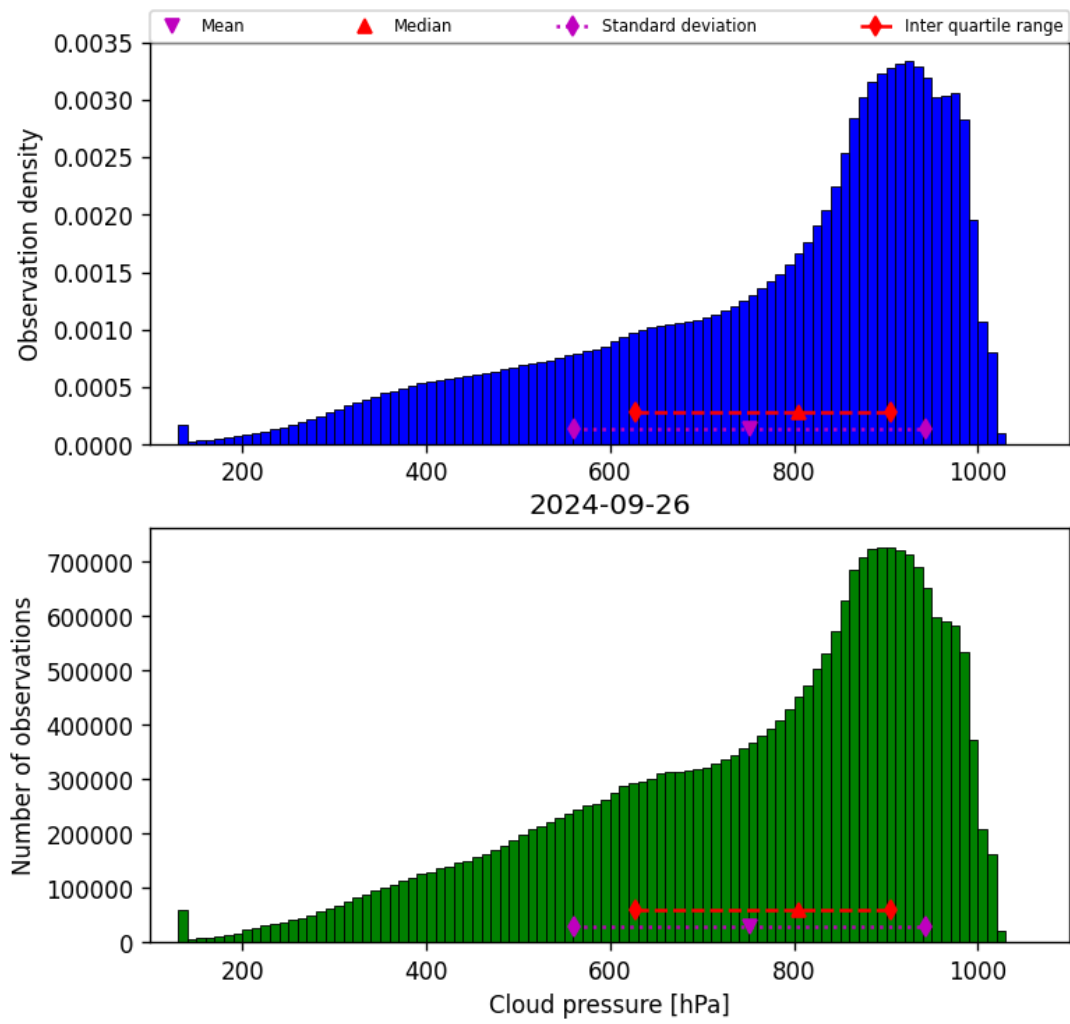
Figure 30: Histogram of “Cloud pressure” for 2024-09-25 to 2024-09-27
