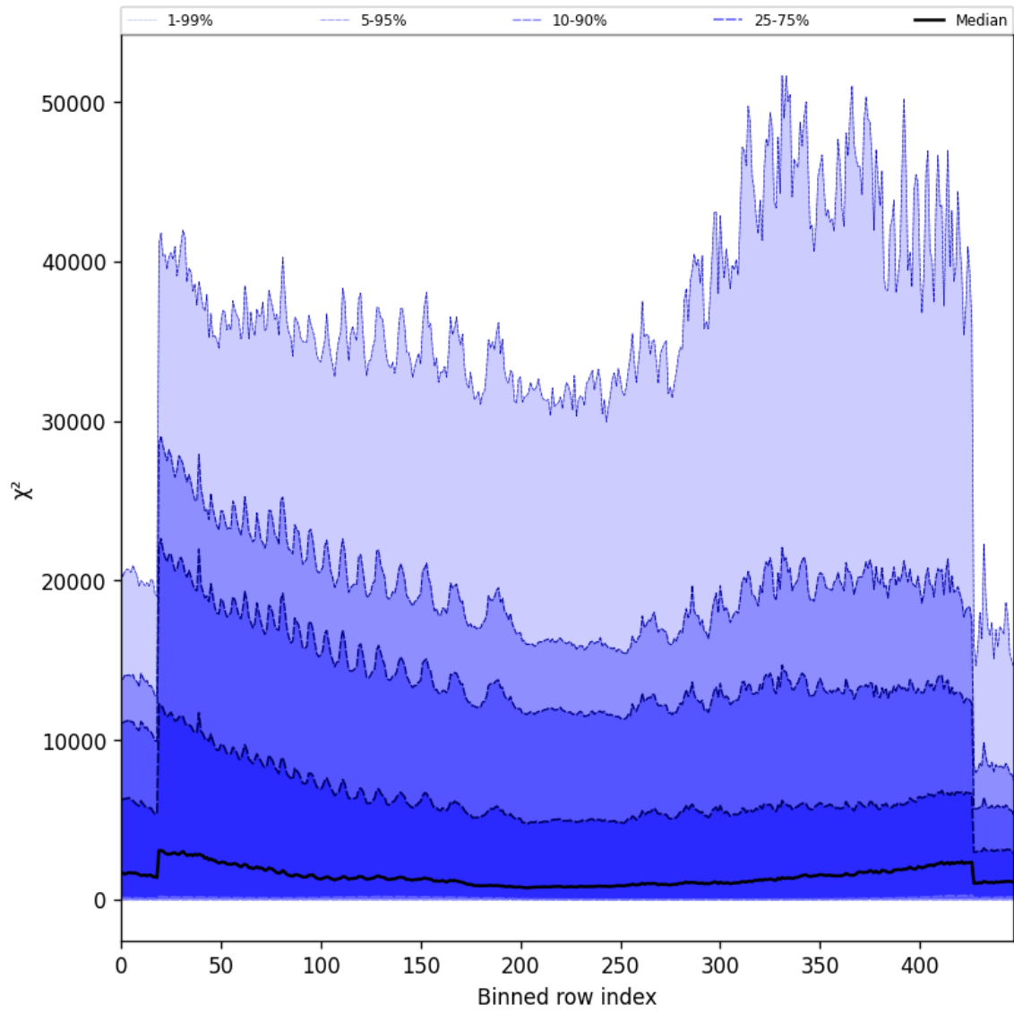
Figure 55: Along track statistics of “ \chi^2 ” for 2024-09-25 to 2024-09-27
