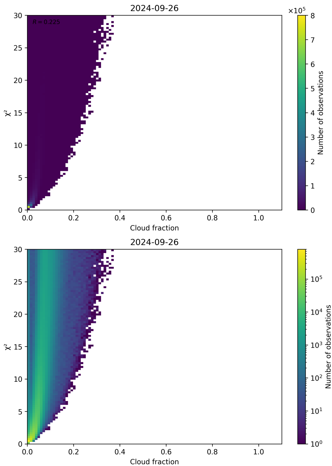
Figure 77: Scatter density plot of “Cloud fraction” against “ \chi^2 ” for 2024-09-25 to 2024-09-27.
