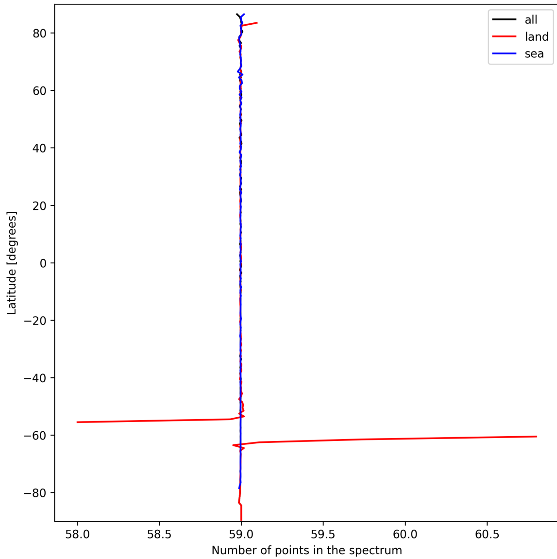
Figure 27: Zonal average of “Number of points in the spectrum” for 2024-09-25 to 2024-09-27.
