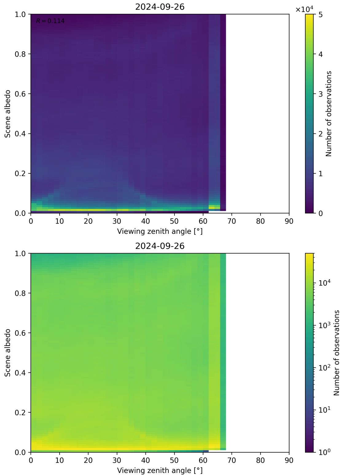
Figure 138: Scatter density plot of “Viewing zenith angle” against “Scene albedo” for 2024-09-25 to 2024-09-27.
