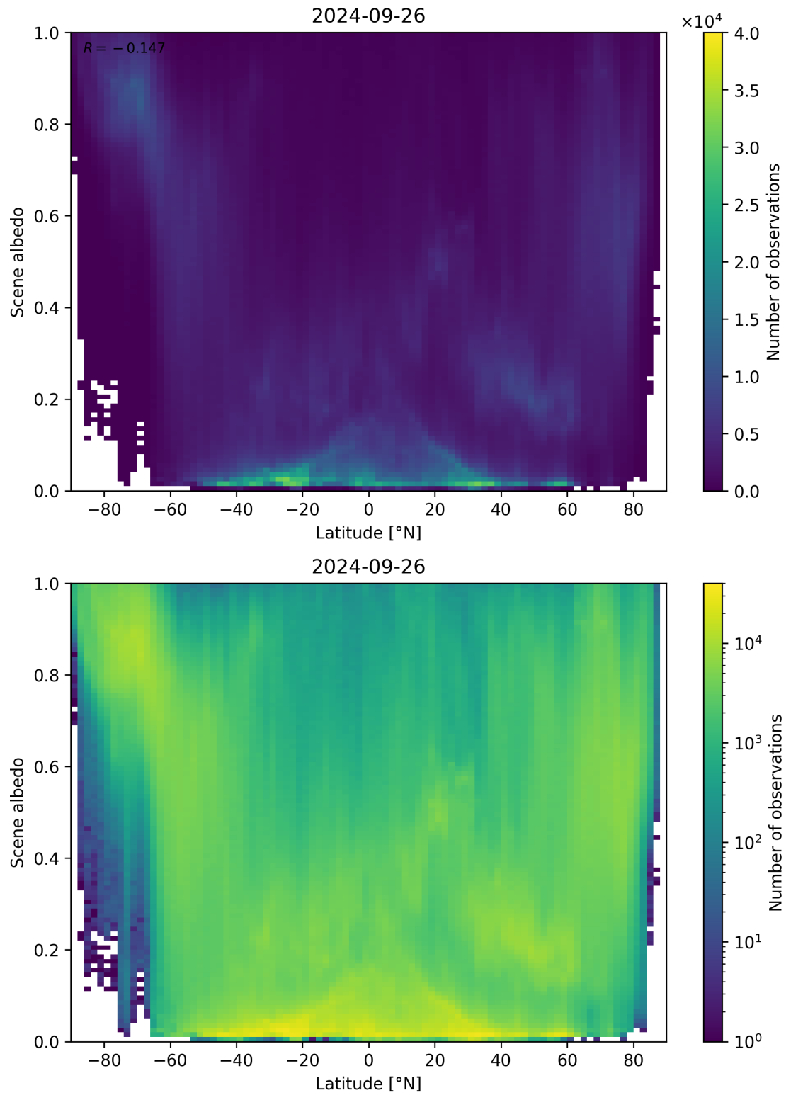
Figure 104: Scatter density plot of “Latitude” against “Scene albedo” for 2024-09-25 to 2024-09-27.
