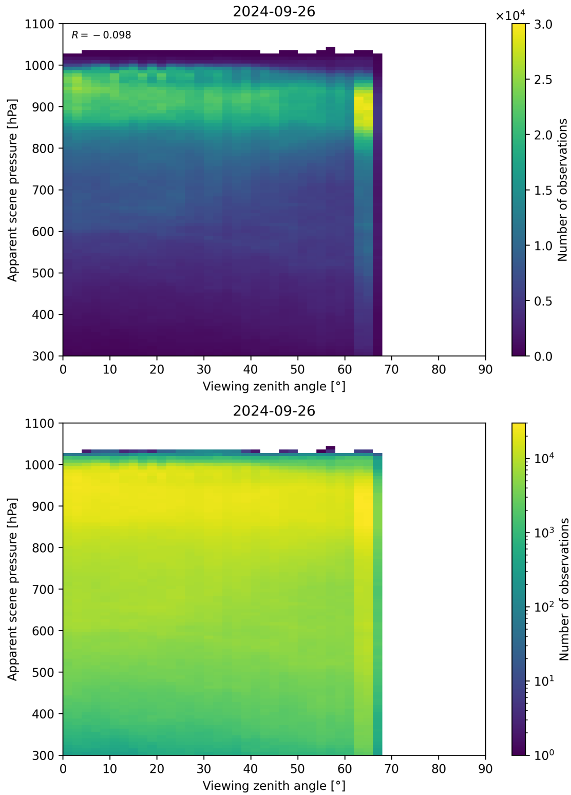
Figure 129: Scatter density plot of “Viewing zenith angle” against “Apparent scene pressure” for 2024-09-25 to 2024-09-27.
