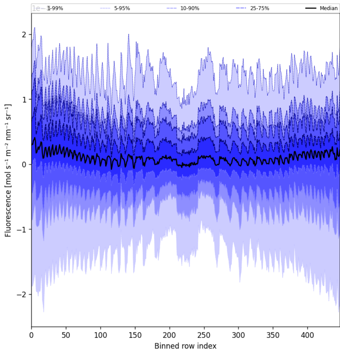
Figure 57: Along track statistics of “Fluorescence” for 2024-09-25 to 2024-09-27
