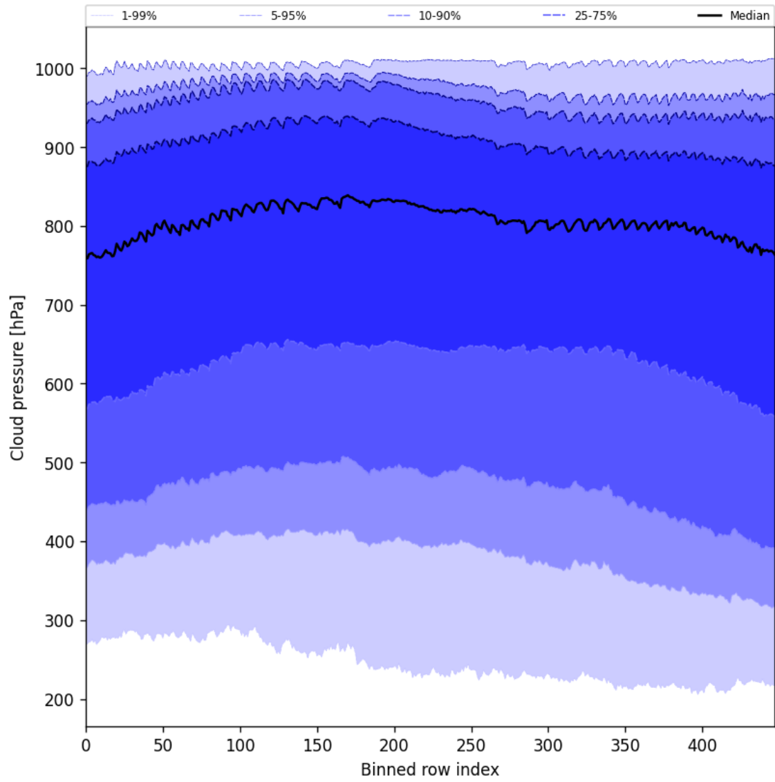
Figure 47: Along track statistics of “Cloud pressure” for 2024-09-25 to 2024-09-27
