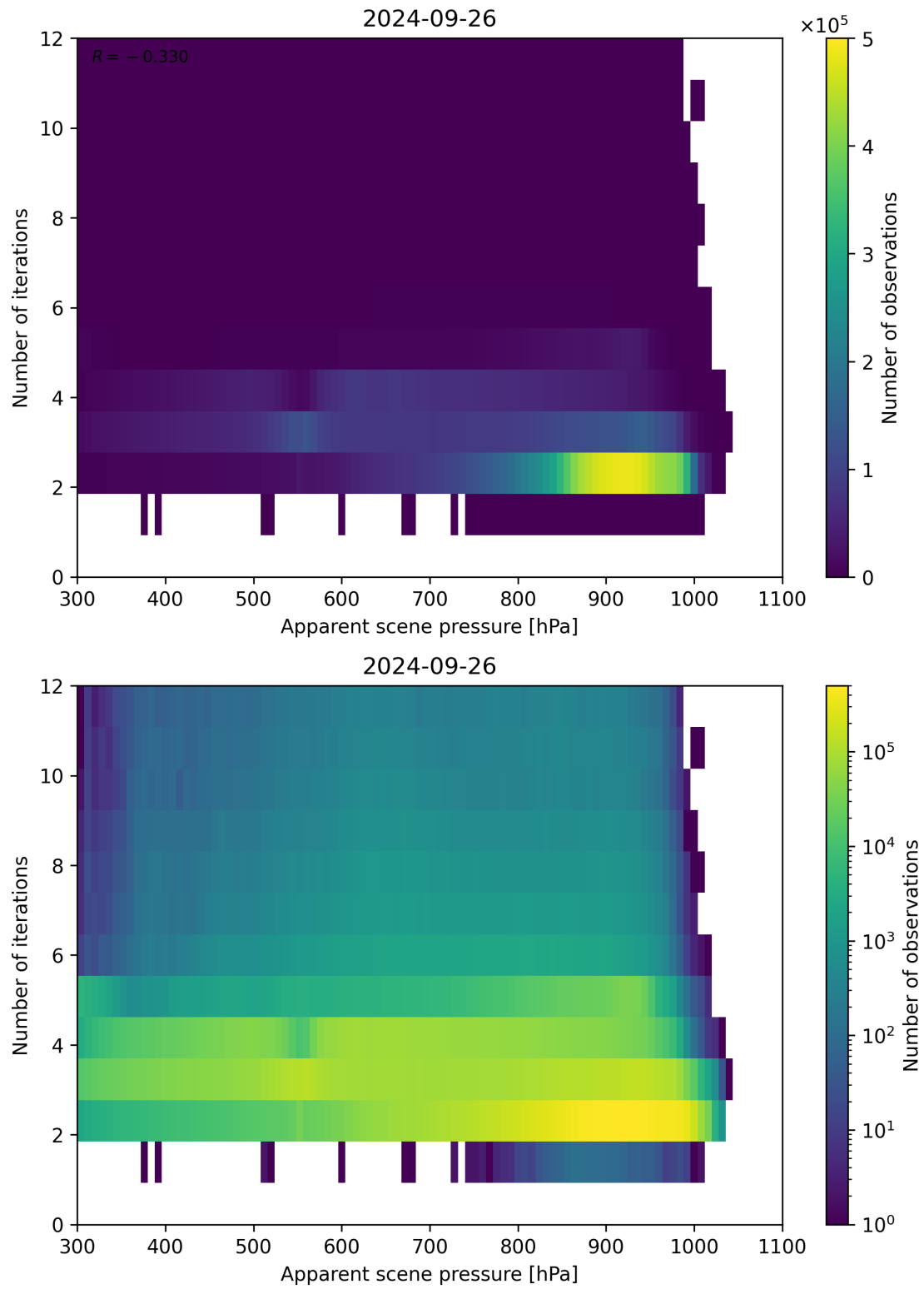
Figure 66: Scatter density plot of “Apparent scene pressure” against “Number of iterations” for 2024-09-25 to 2024-09-27.
