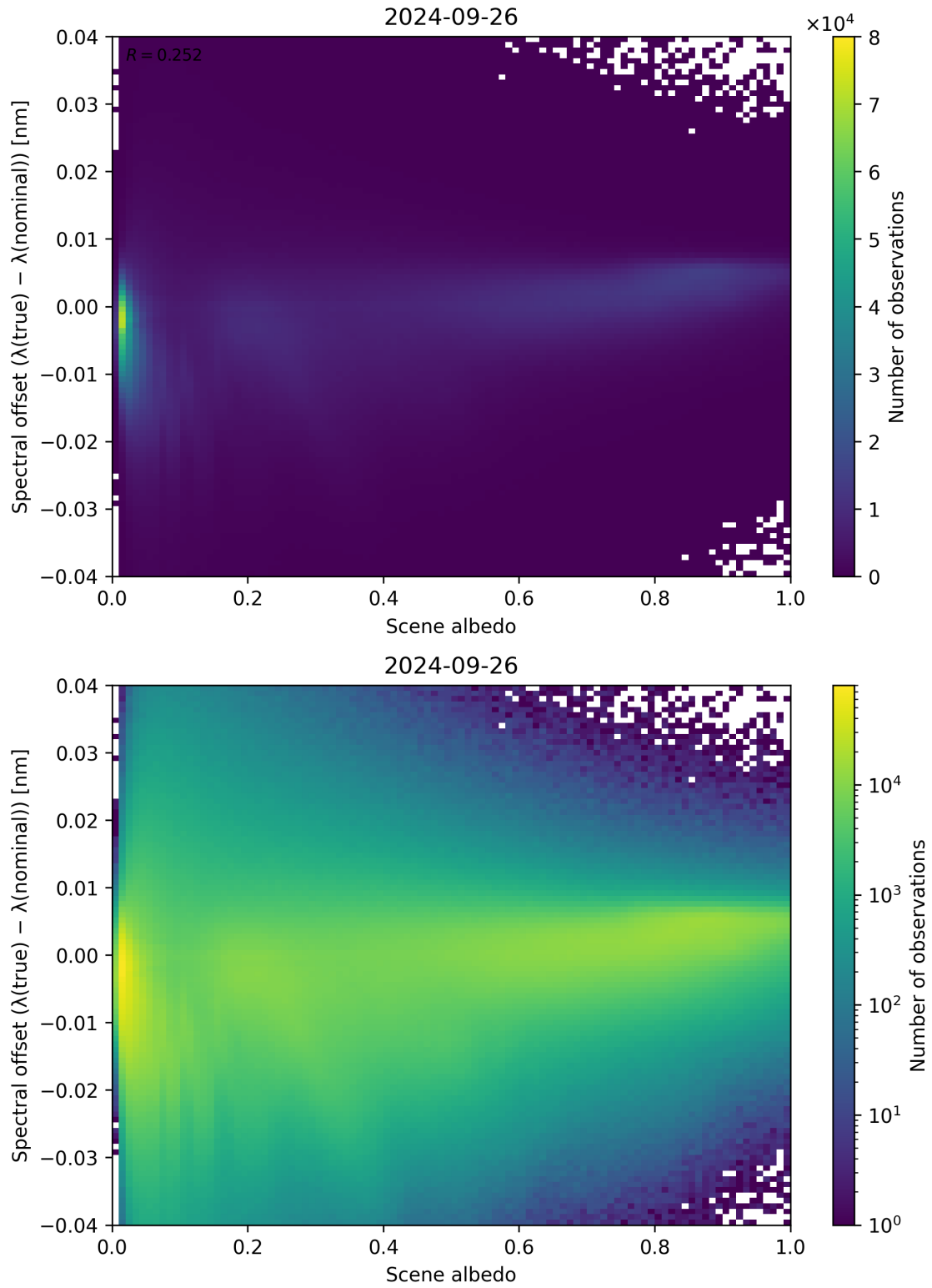
Figure 117: Scatter density plot of “Scene albedo” against “Spectral offset ( \lambda_{\text{true}} - \lambda_{\text{nominal}} )” for 2024-09-25 to 2024-09-27.
