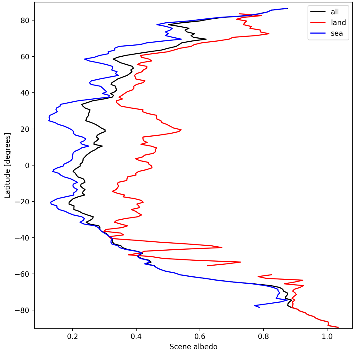
Figure 17: Zonal average of “Scene albedo” for 2024-09-25 to 2024-09-27.
