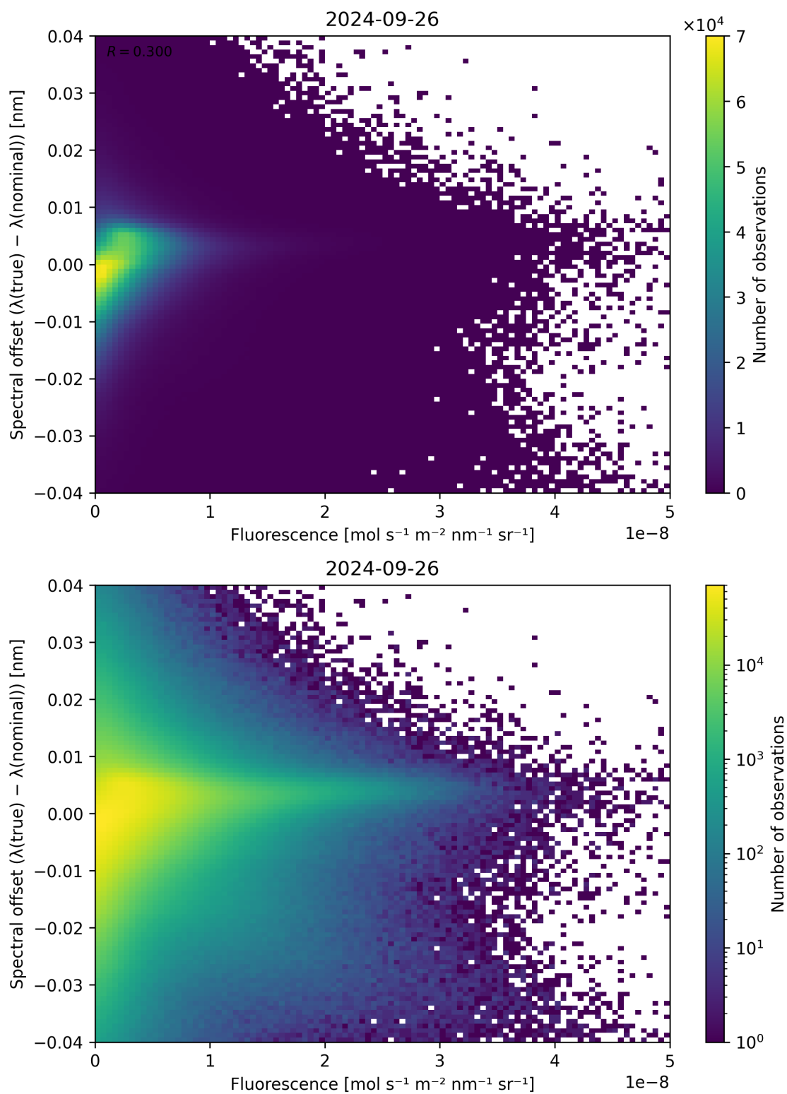
Figure 95: Scatter density plot of “Fluorescence” against “Spectral offset ( \lambda_{\text{true}} - \lambda_{\text{nominal}} )” for 2024-09-25 to 2024-09-27.
