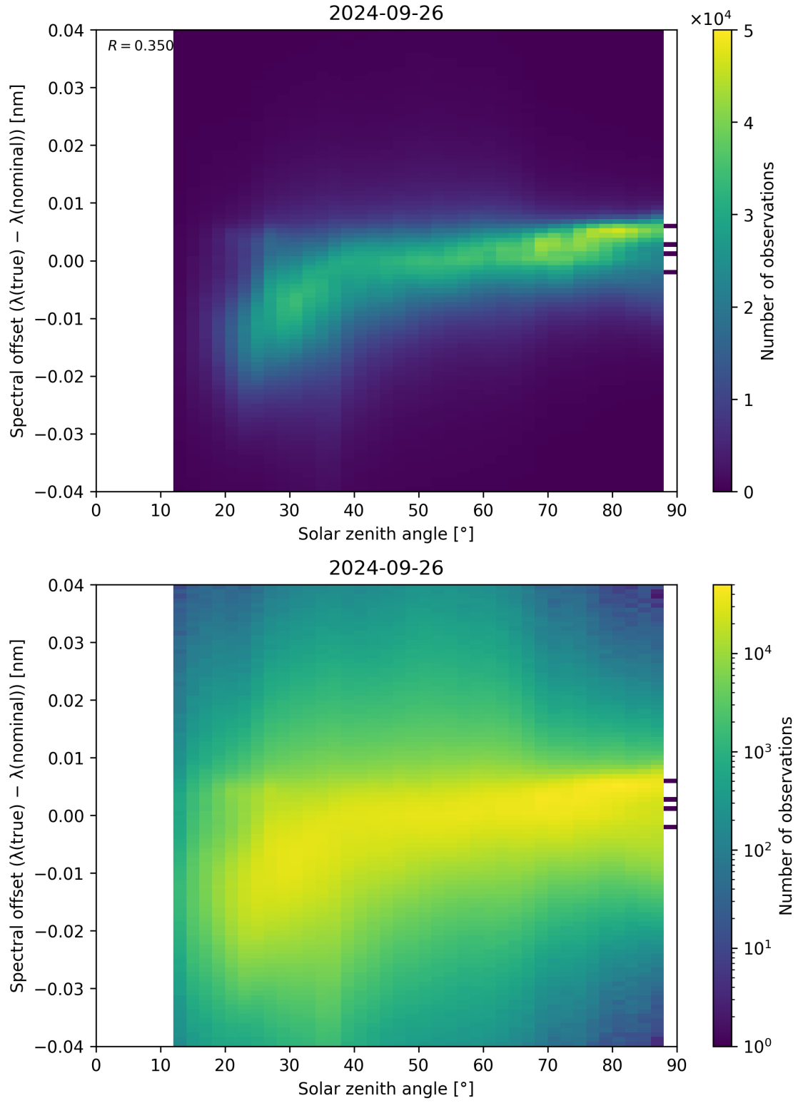
Figure 128: Scatter density plot of “Solar zenith angle” against “Spectral offset ( \lambda_{\text{true}} - \lambda_{\text{nominal}} )” for 2024-09-25 to 2024-09-27.
