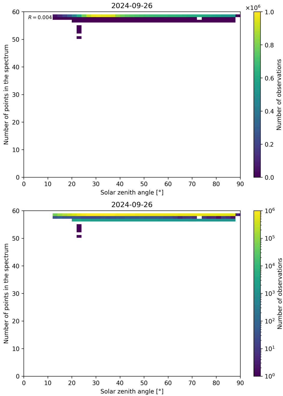
Figure 126: Scatter density plot of “Solar zenith angle” against “Number of points in the spectrum” for 2024-09-25 to 2024-09-27.
