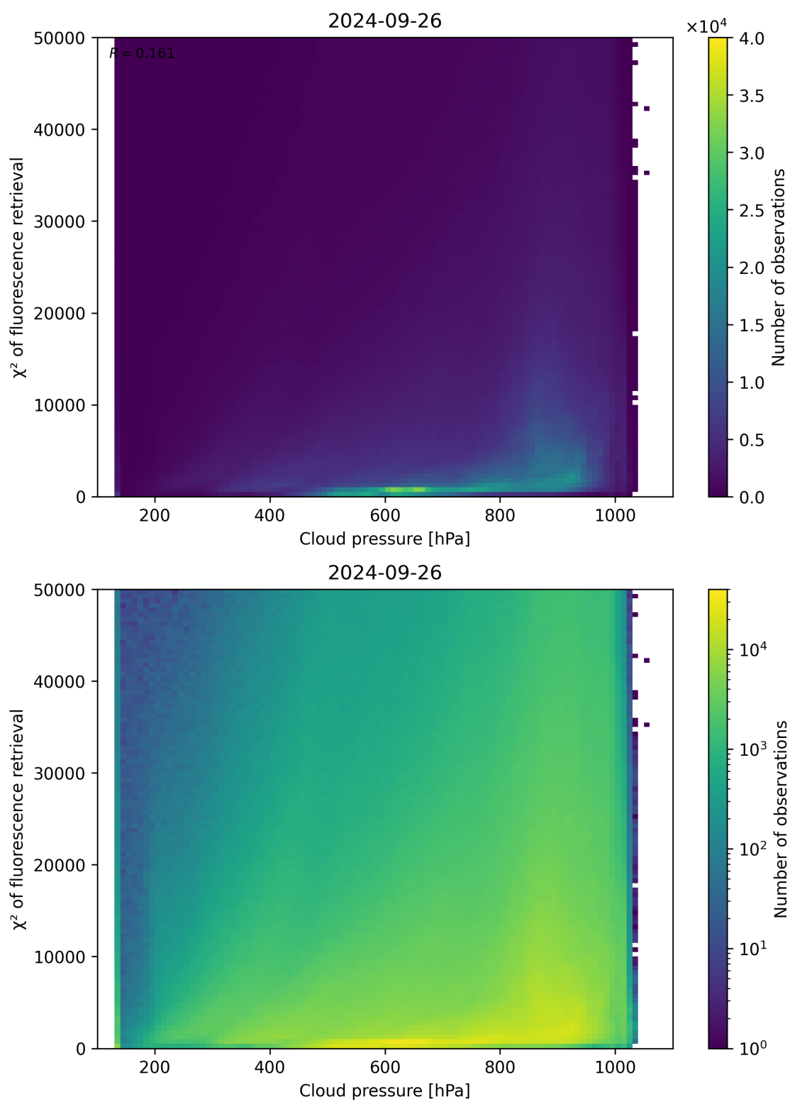
Figure 86: Scatter density plot of “Cloud pressure” against “ \chi^2 of fluorescence retrieval” for 2024-09-25 to 2024-09-27.
