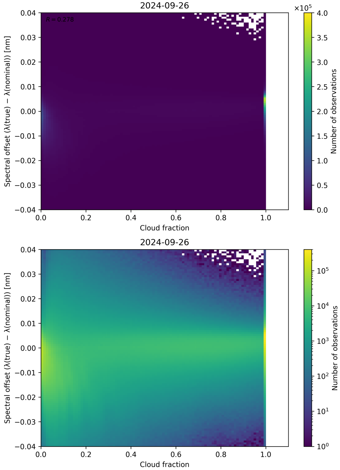
Figure 83: Scatter density plot of “Cloud fraction” against “Spectral offset ( \lambda_{\text{true}} - \lambda_{\text{nominal}} )” for 2024-09-25 to 2024-09-27.
