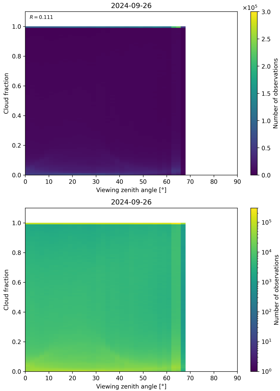
Figure 132: Scatter density plot of “Viewing zenith angle” against “Cloud fraction” for 2024-09-25 to 2024-09-27.
