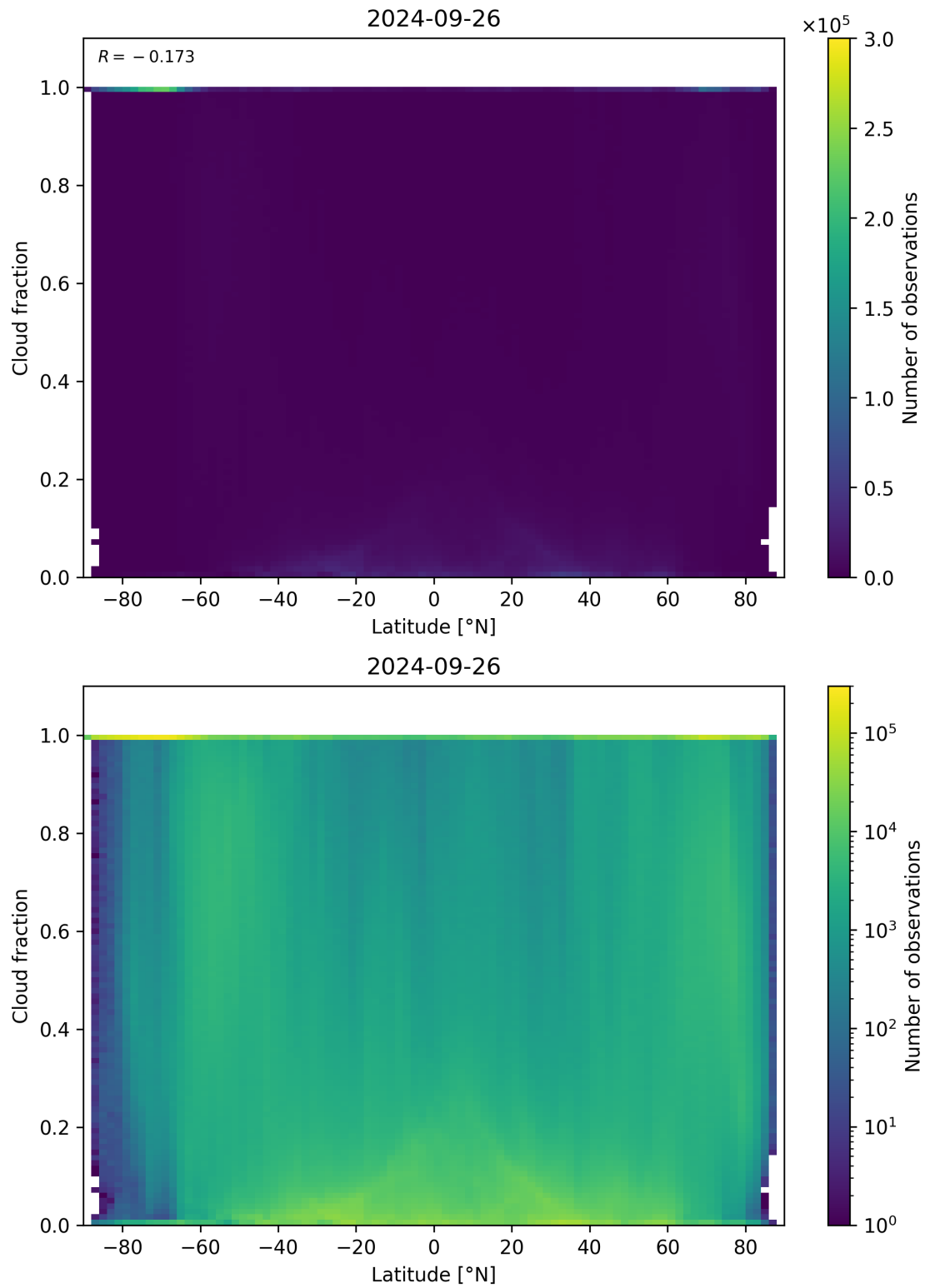
Figure 99: Scatter density plot of “Latitude” against “Cloud fraction” for 2024-09-25 to 2024-09-27.
