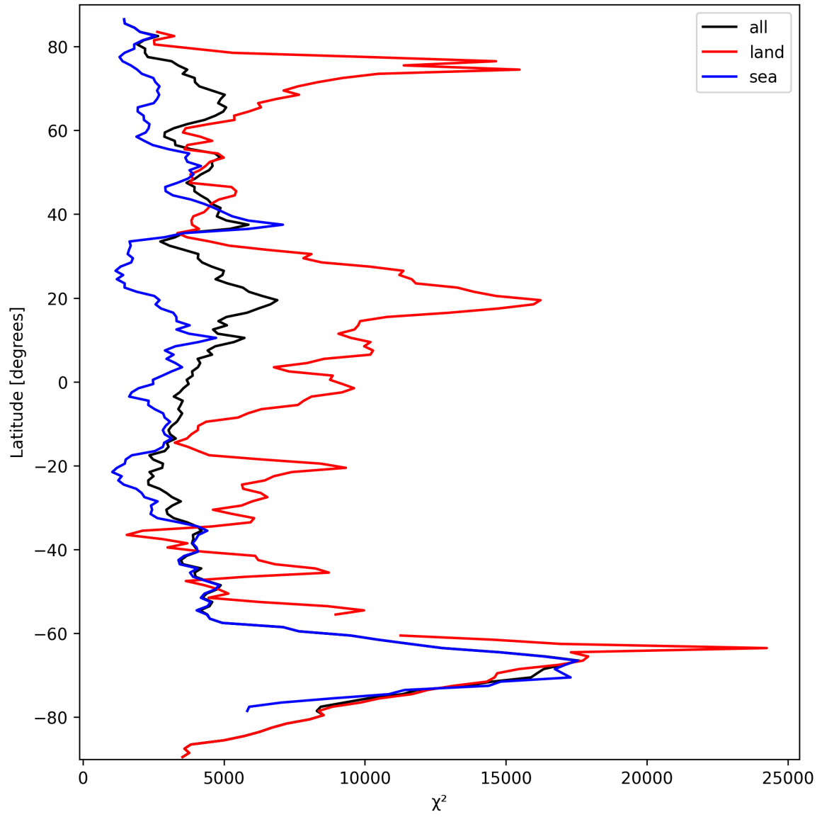
Figure 21: Zonal average of “ \chi^2 ” for 2024-09-25 to 2024-09-27.
