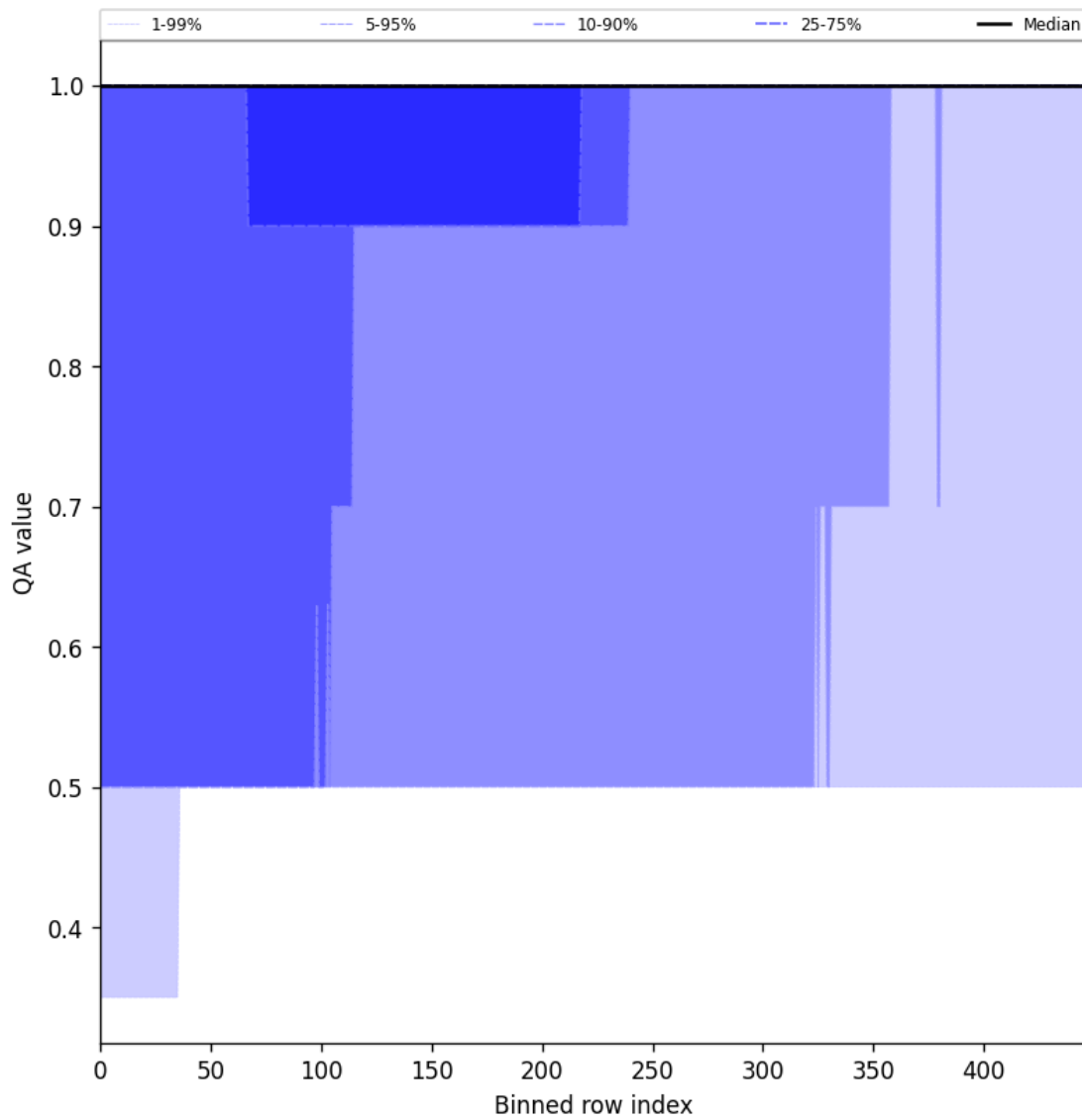
Figure 46: Along track statistics of “QA value” for 2024-09-25 to 2024-09-27
