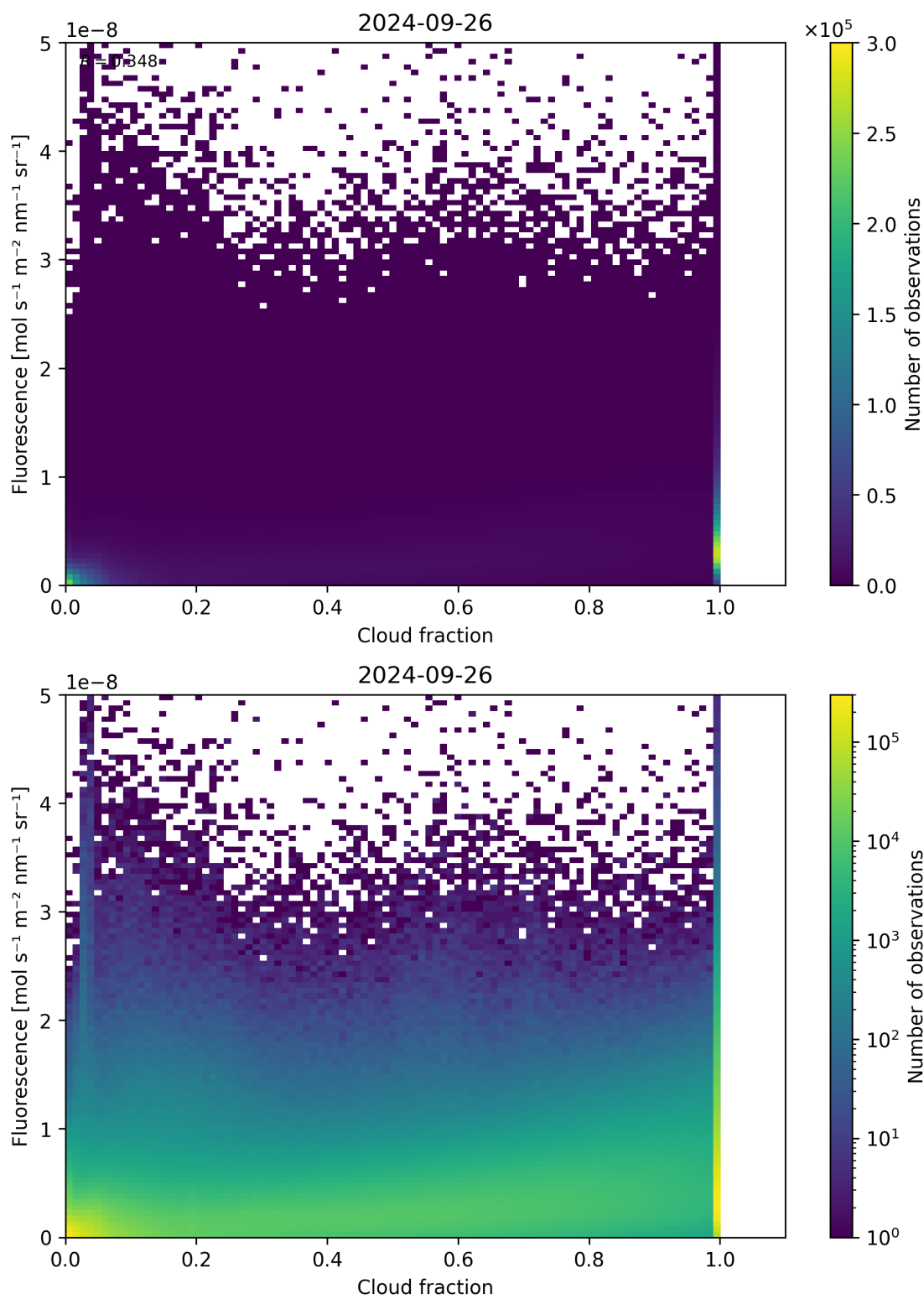
Figure 79: Scatter density plot of “Cloud fraction” against “Fluorescence” for 2024-09-25 to 2024-09-27.
