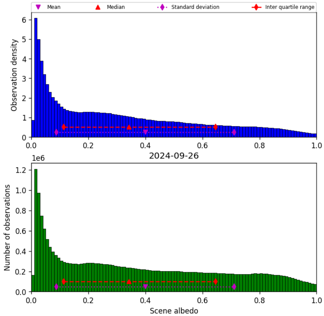
Figure 34: Histogram of “Scene albedo” for 2024-09-25 to 2024-09-27
