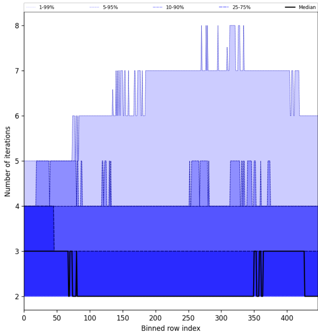
Figure 56: Along track statistics of “Number of iterations” for 2024-09-28 to 2024-09-30
