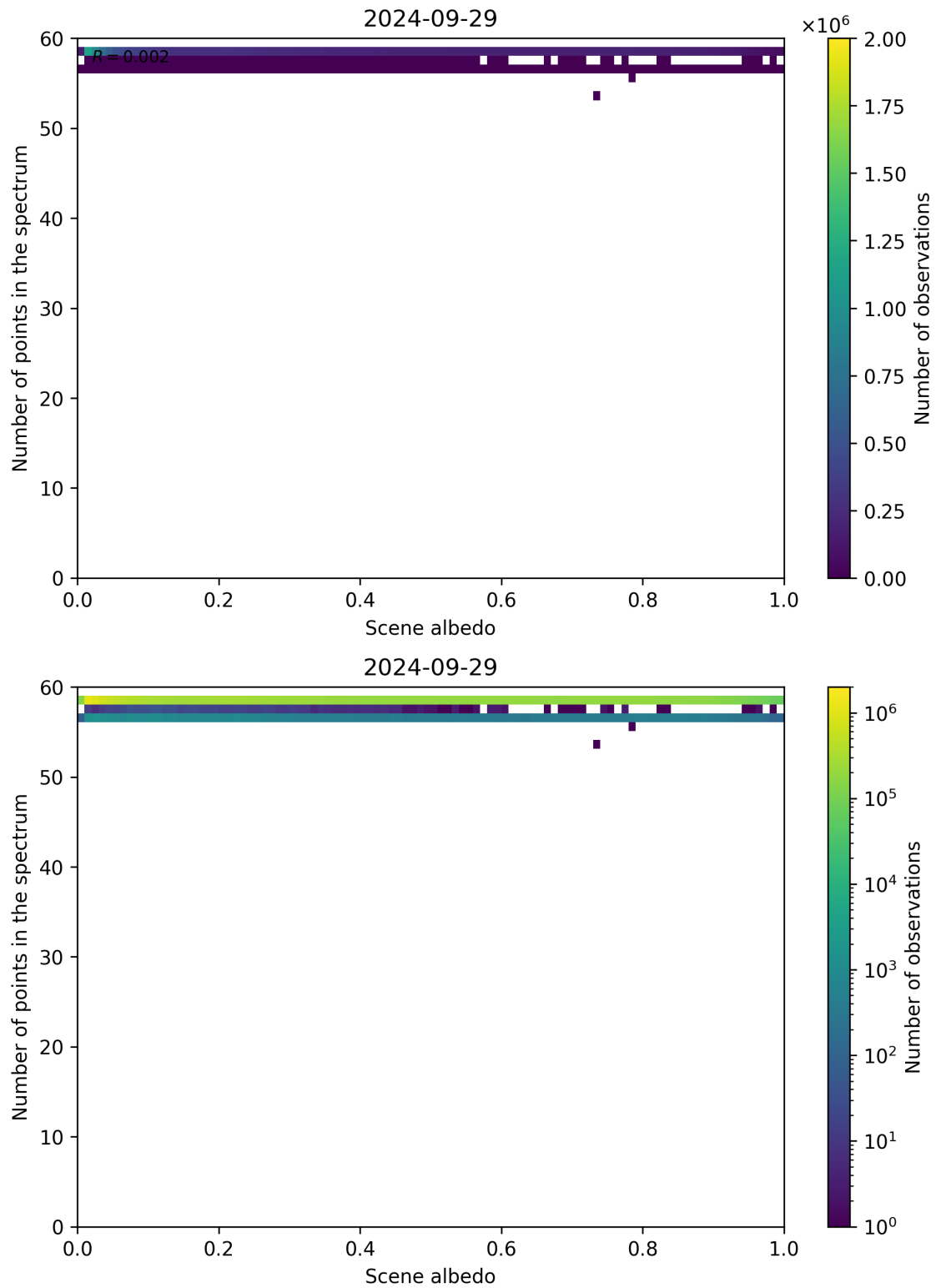
Figure 116: Scatter density plot of “Scene albedo” against “Number of points in the spectrum” for 2024-09-28 to 2024-09-30.
