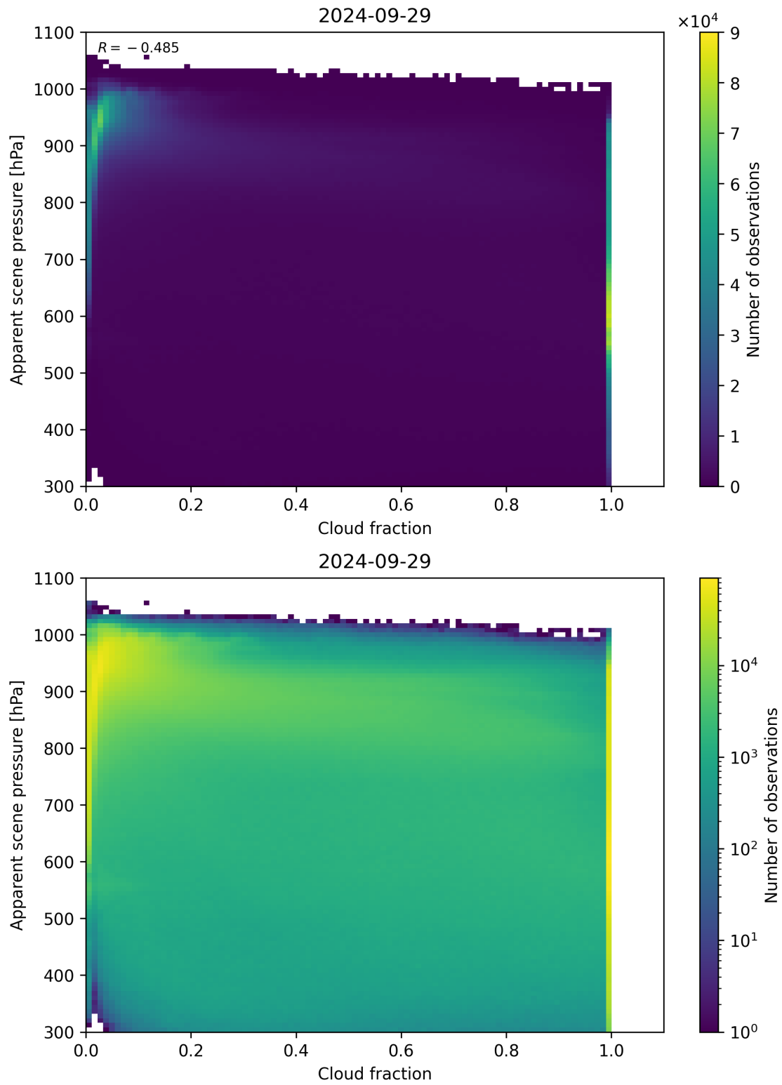
Figure 76: Scatter density plot of “Cloud fraction” against “Apparent scene pressure” for 2024-09-28 to 2024-09-30.
