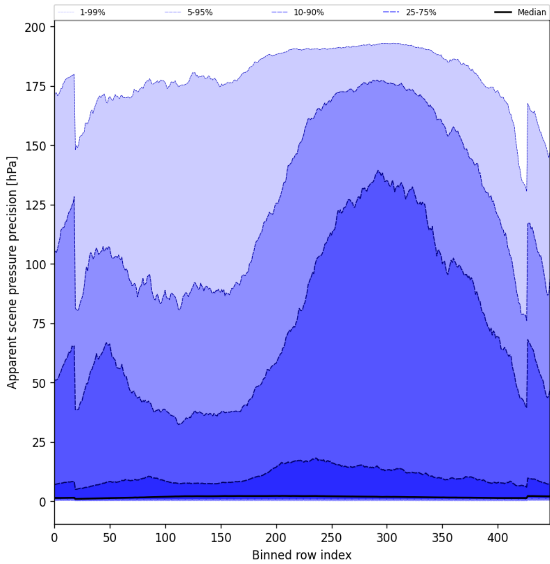
Figure 54: Along track statistics of “Apparent scene pressure precision” for 2024-09-28 to 2024-09-30
