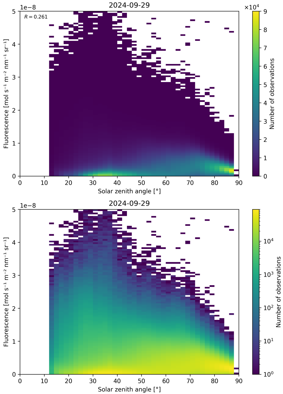
Figure 123: Scatter density plot of “Solar zenith angle” against “Fluorescence” for 2024-09-28 to 2024-09-30.
