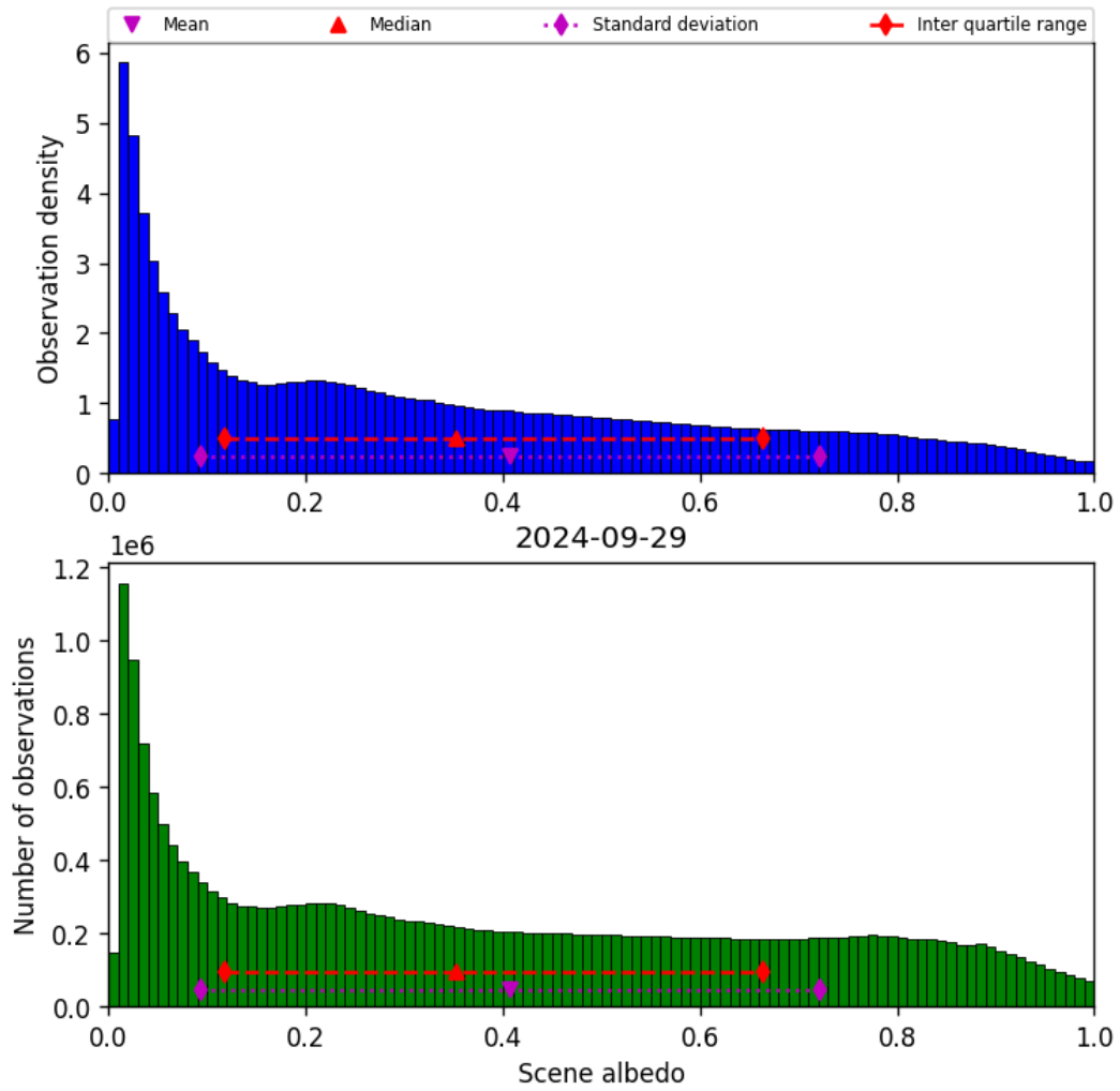
Figure 34: Histogram of “Scene albedo” for 2024-09-28 to 2024-09-30
