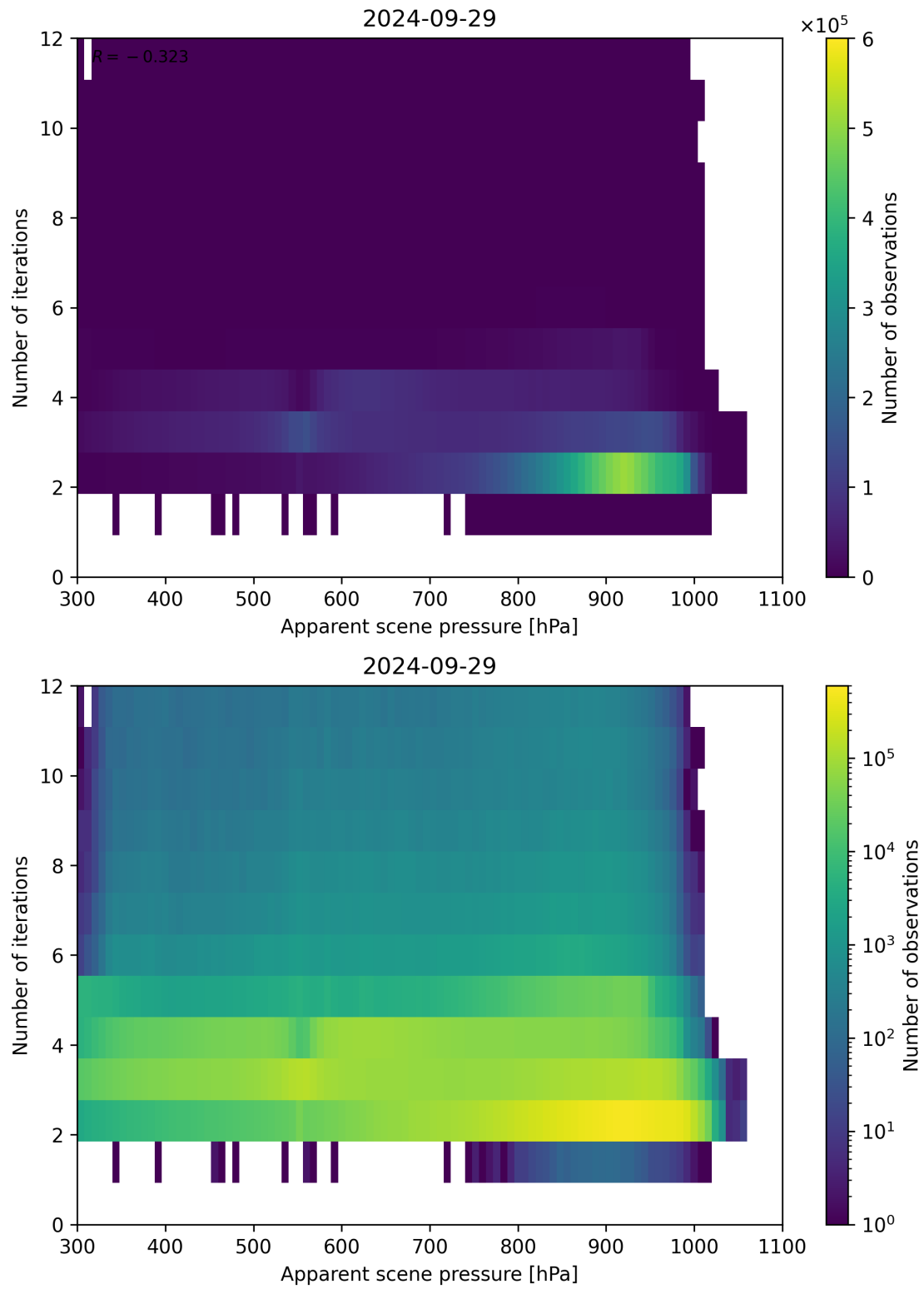
Figure 66: Scatter density plot of “Apparent scene pressure” against “Number of iterations” for 2024-09-28 to 2024-09-30.
