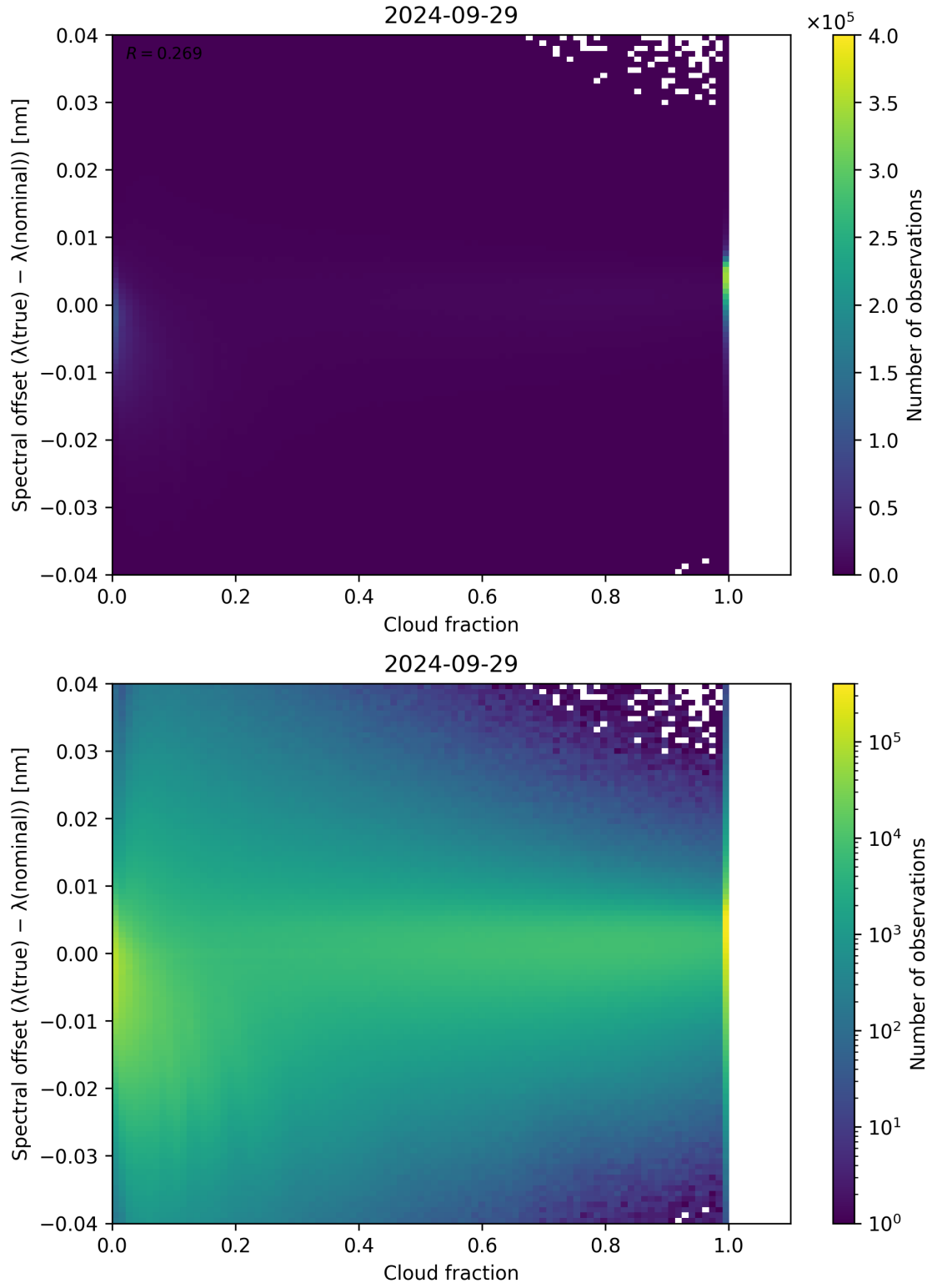
Figure 83: Scatter density plot of “Cloud fraction” against “Spectral offset ( \lambda_{\text{true}} - \lambda_{\text{nominal}} )” for 2024-09-28 to 2024-09-30.
