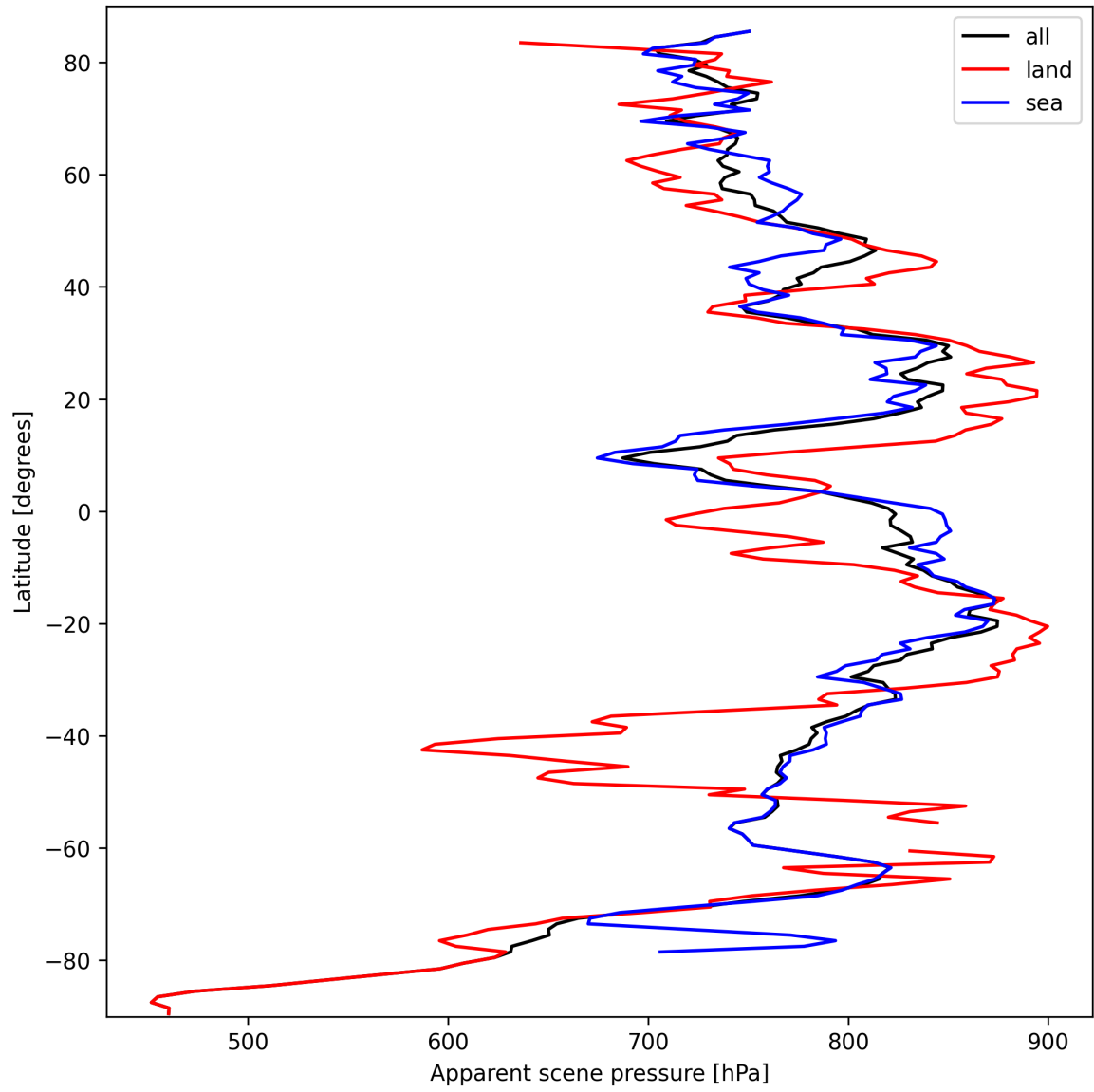
Figure 19: Zonal average of “Apparent scene pressure” for 2024-09-28 to 2024-09-30.
