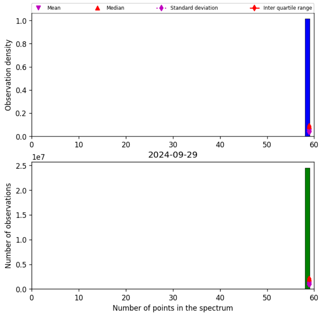
Figure 44: Histogram of “Number of points in the spectrum” for 2024-09-28 to 2024-09-30
