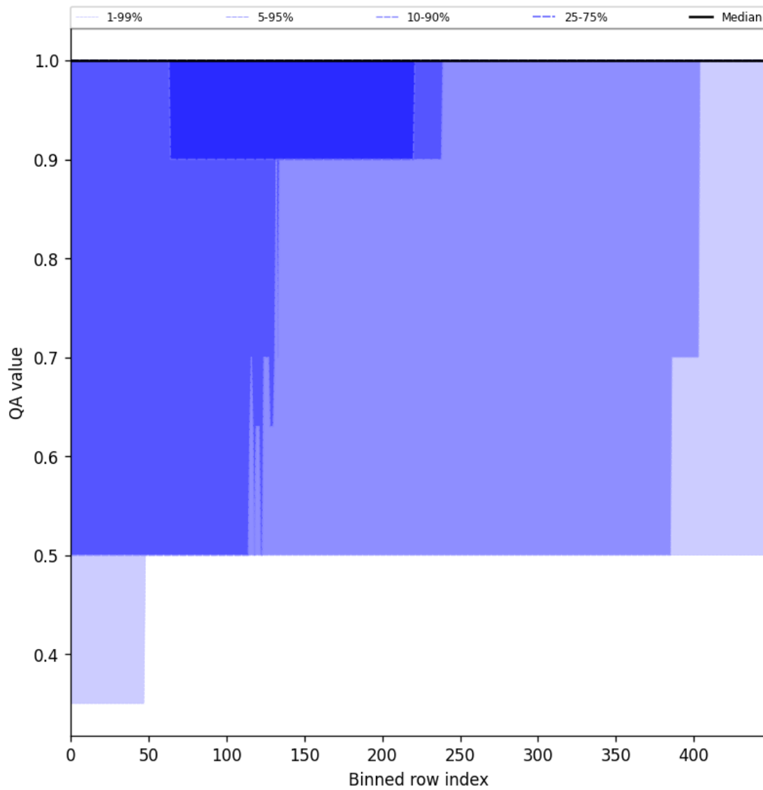
Figure 46: Along track statistics of “QA value” for 2024-09-28 to 2024-09-30
