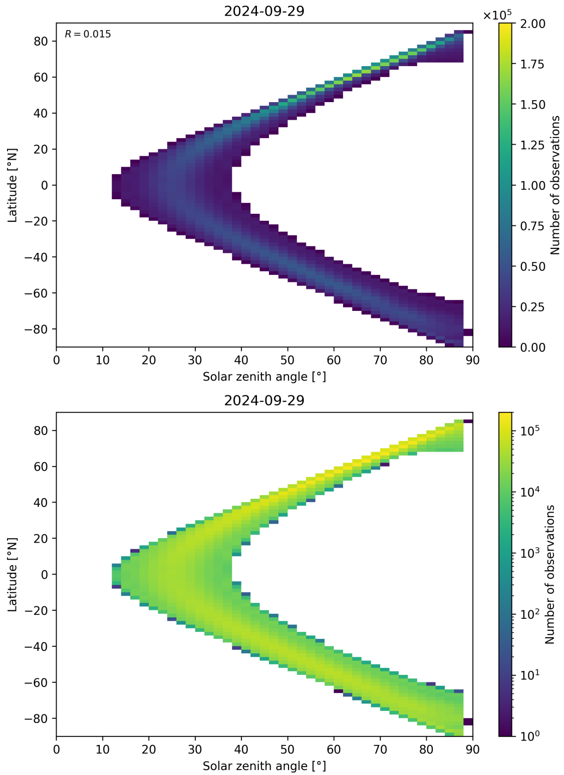
Figure 124: Scatter density plot of “Solar zenith angle” against “Latitude” for 2024-09-28 to 2024-09-30.
