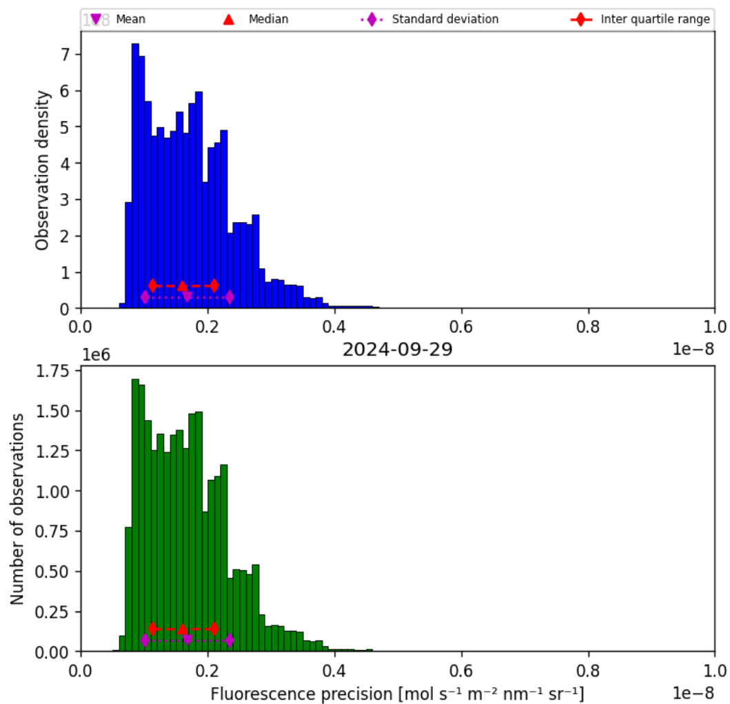
Figure 41: Histogram of “Fluorescence precision” for 2024-09-28 to 2024-09-30
