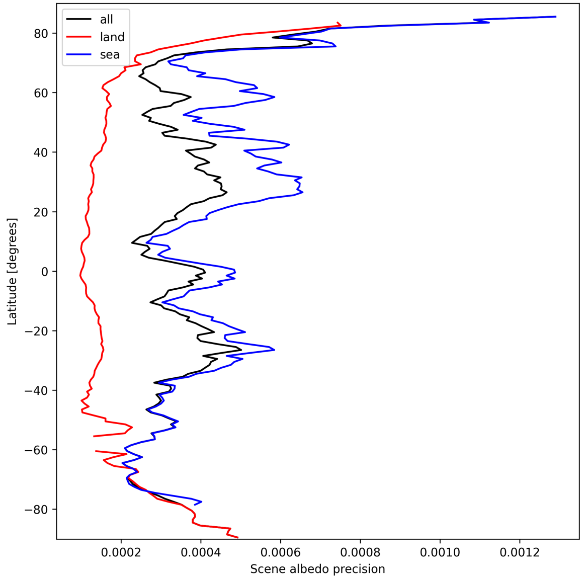
Figure 18: Zonal average of "Scene albedo precision" for 2024-09-28 to 2024-09-30.
