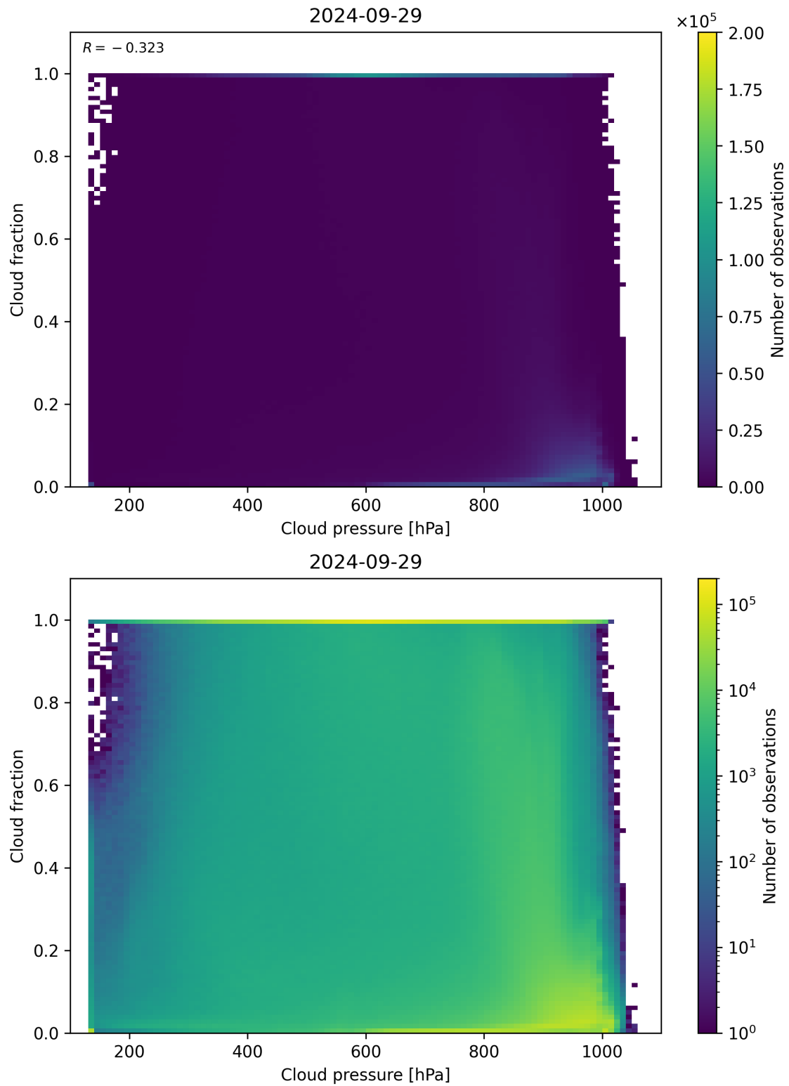
Figure 87: Scatter density plot of “Cloud pressure” against “Cloud fraction” for 2024-09-28 to 2024-09-30.
