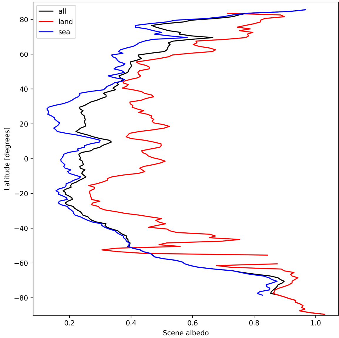
Figure 17: Zonal average of “Scene albedo” for 2024-09-28 to 2024-09-30.
