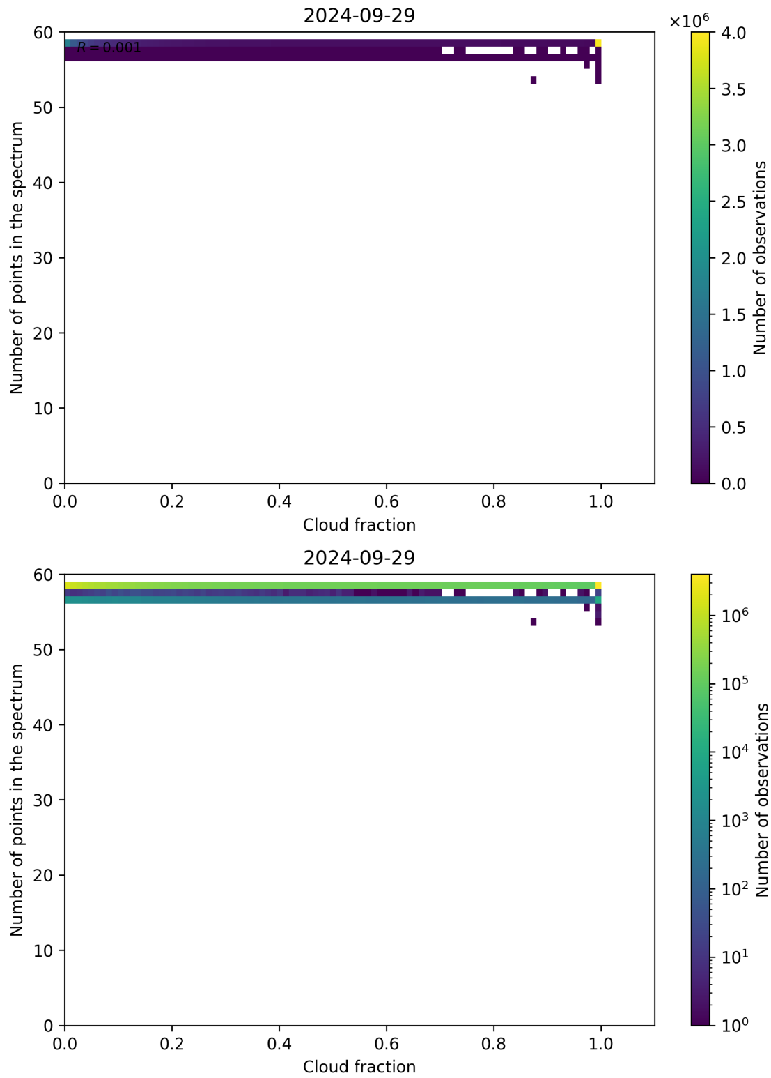
Figure 81: Scatter density plot of “Cloud fraction” against “Number of points in the spectrum” for 2024-09-28 to 2024-09-30.
