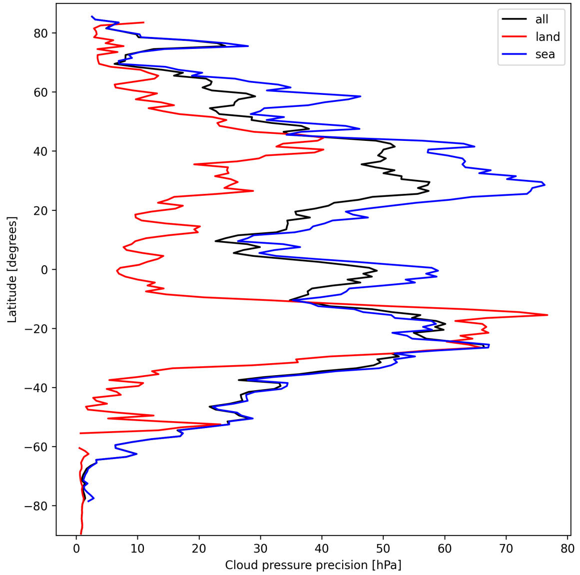
Figure 14: Zonal average of “Cloud pressure precision” for 2024-09-28 to 2024-09-30.
