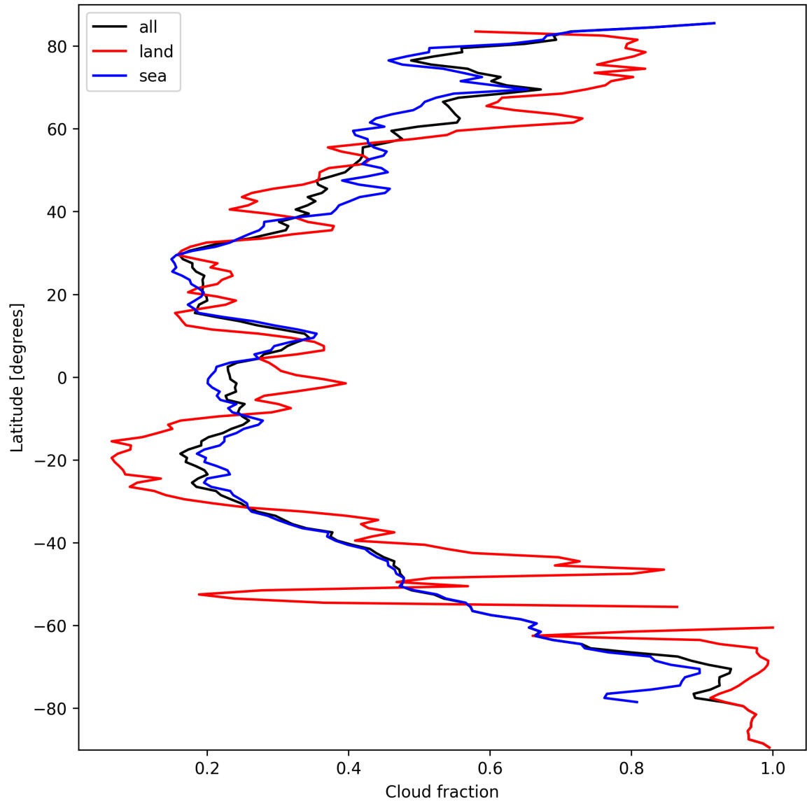
Figure 15: Zonal average of “Cloud fraction” for 2024-09-28 to 2024-09-30.
