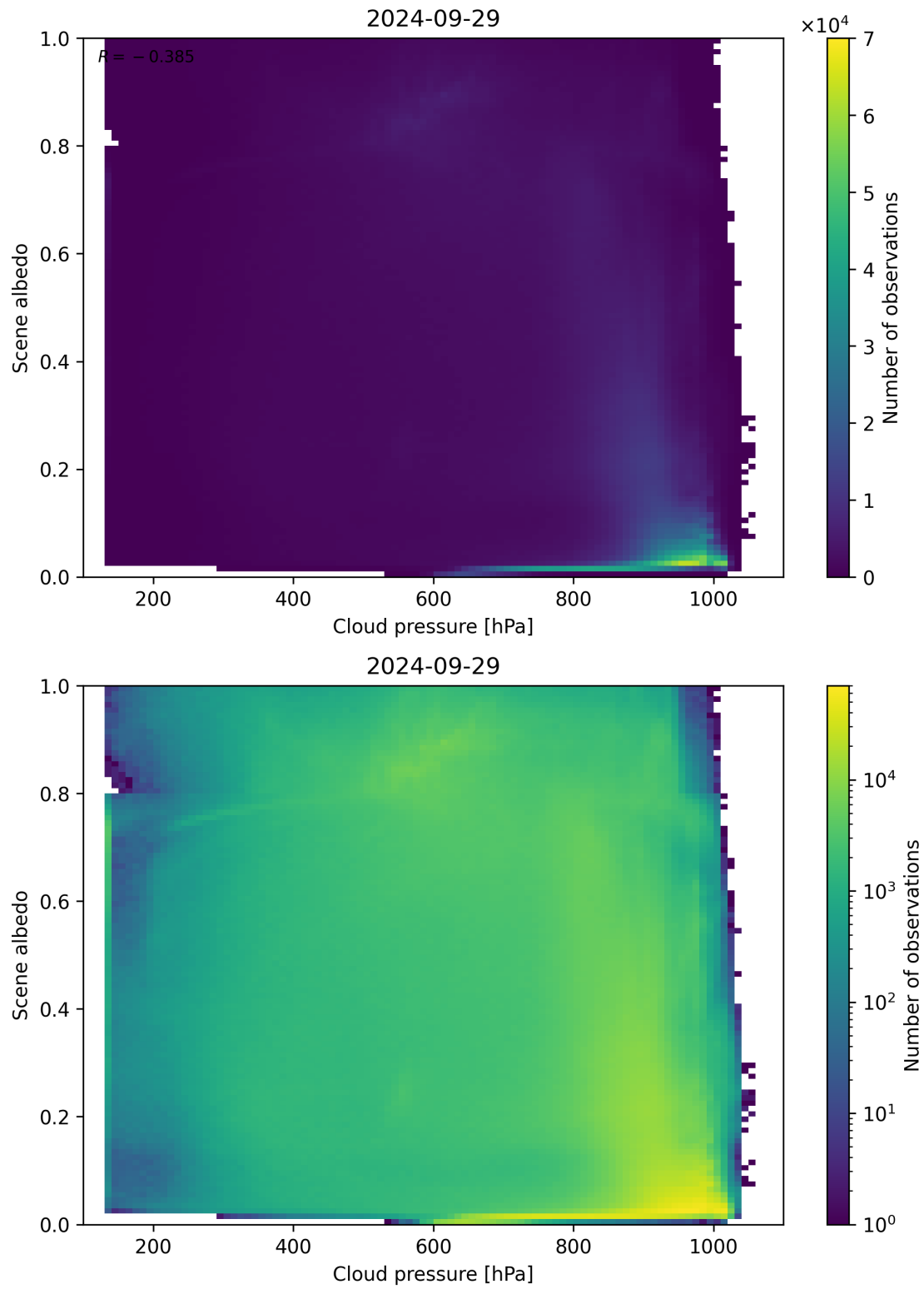
Figure 91: Scatter density plot of “Cloud pressure” against “Scene albedo” for 2024-09-28 to 2024-09-30.
