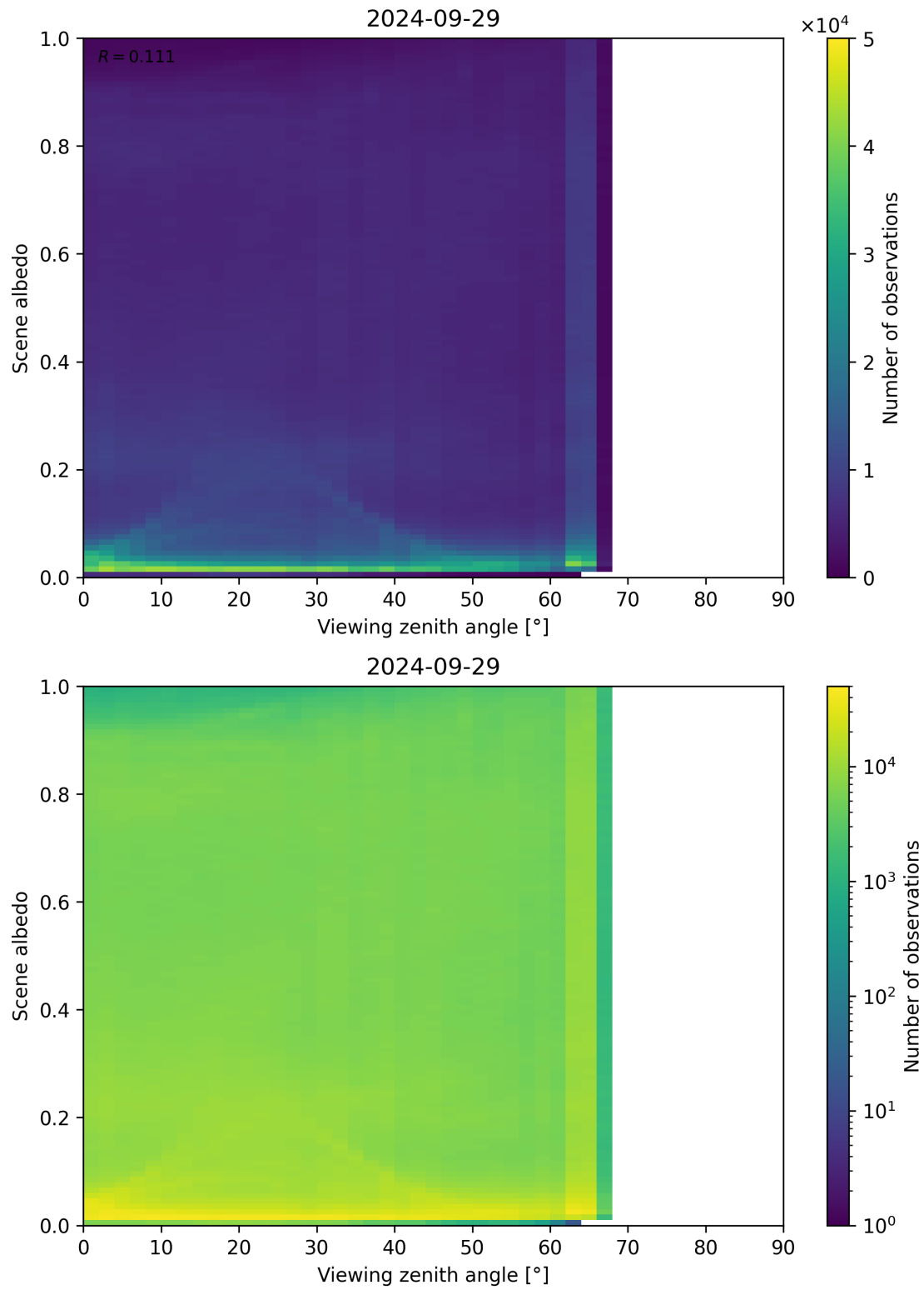
Figure 138: Scatter density plot of “Viewing zenith angle” against “Scene albedo” for 2024-09-28 to 2024-09-30.
