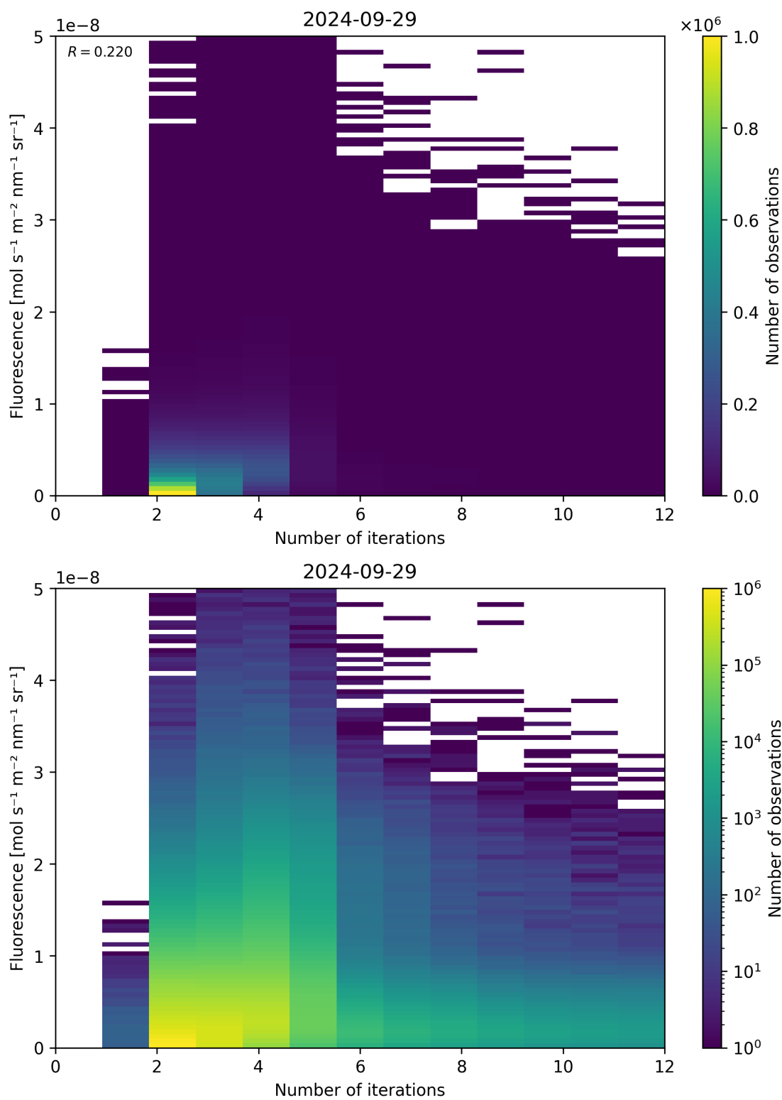
Figure 107: Scatter density plot of “Number of iterations” against “Fluorescence” for 2024-09-28 to 2024-09-30.
