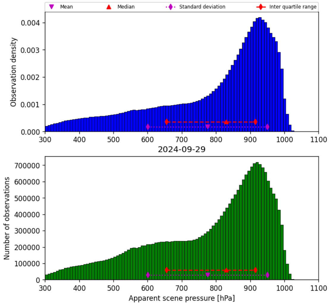
Figure 36: Histogram of “Apparent scene pressure” for 2024-09-28 to 2024-09-30
