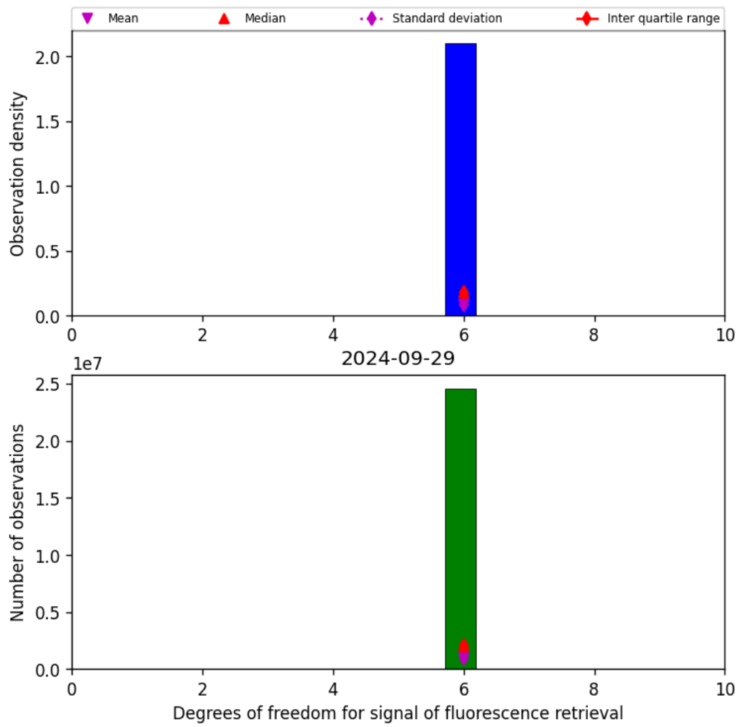
Figure 43: Histogram of “Degrees of freedom for signal of fluorescence retrieval” for 2024-09-28 to 2024-09-30
