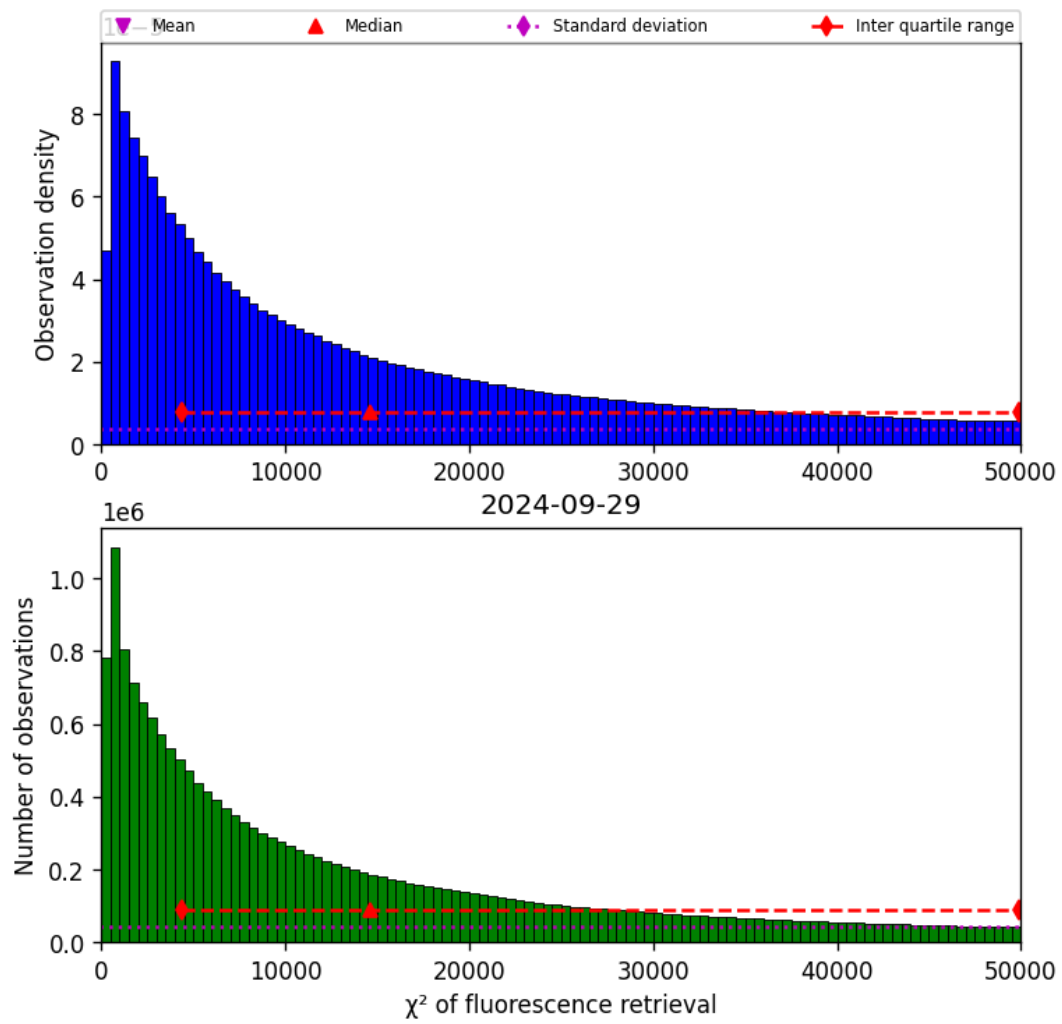
Figure 42: Histogram of “ \chi^2 of fluorescence retrieval” for 2024-09-28 to 2024-09-30
