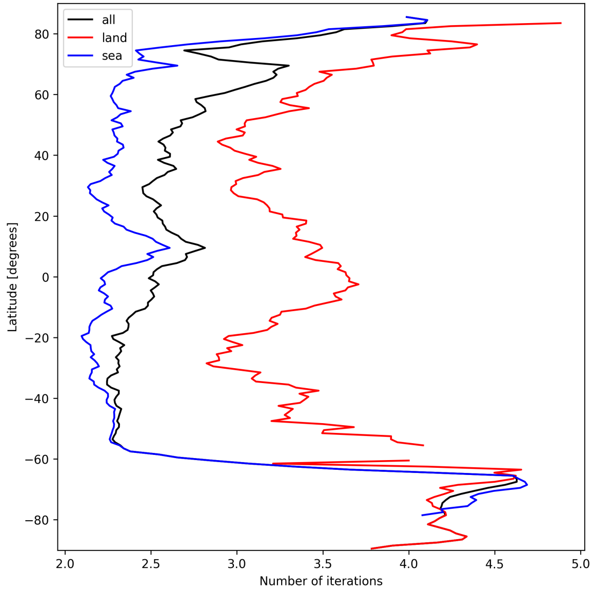
Figure 22: Zonal average of “Number of iterations” for 2024-09-28 to 2024-09-30.
