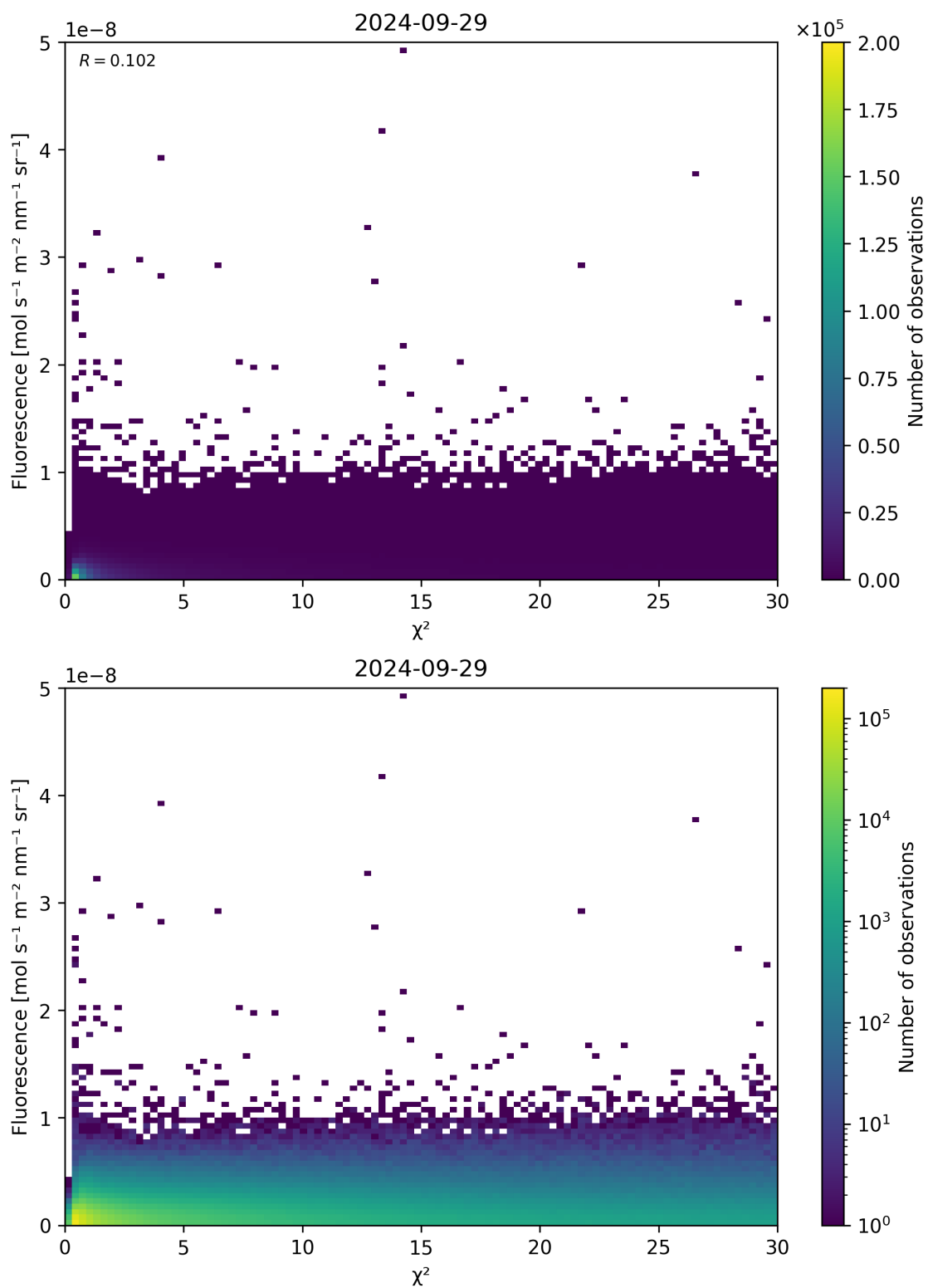
Figure 70: Scatter density plot of “ \chi^2 ” against “Fluorescence” for 2024-09-28 to 2024-09-30.
