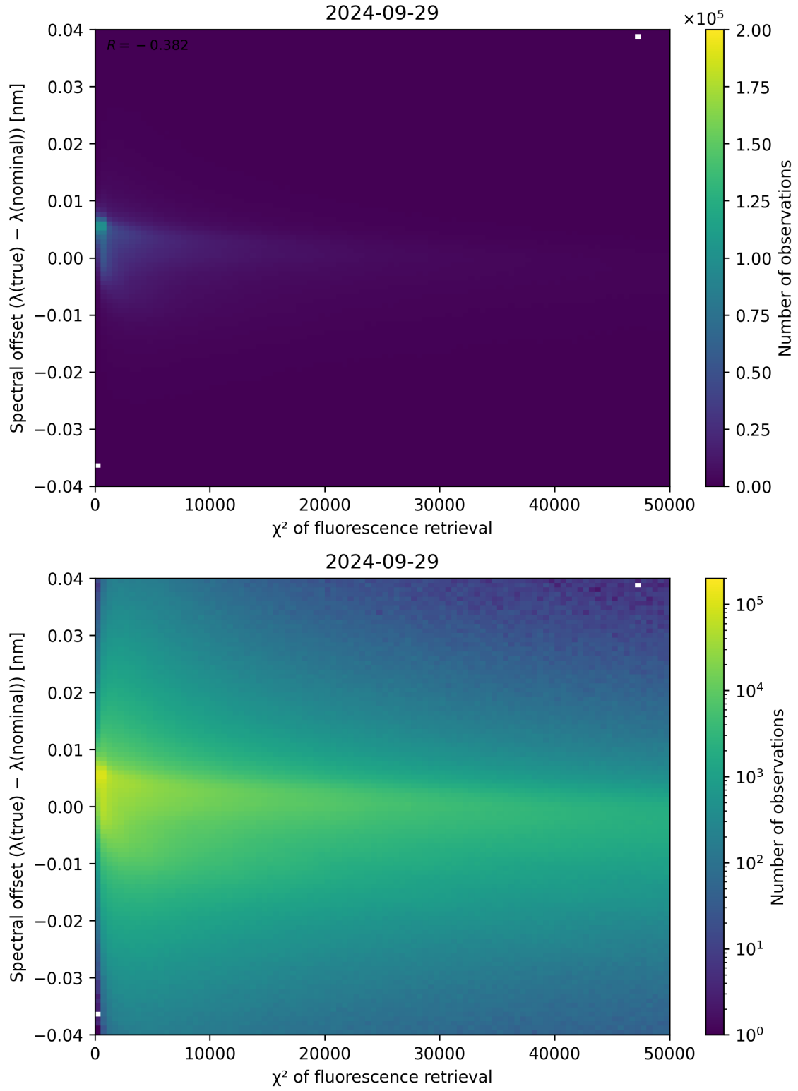
Figure 72: Scatter density plot of “ \chi^2 of fluorescence retrieval” against “Spectral offset ( \lambda_{\text{true}} - \lambda_{\text{nominal}} )” for 2024-09-28 to 2024-09-30.
