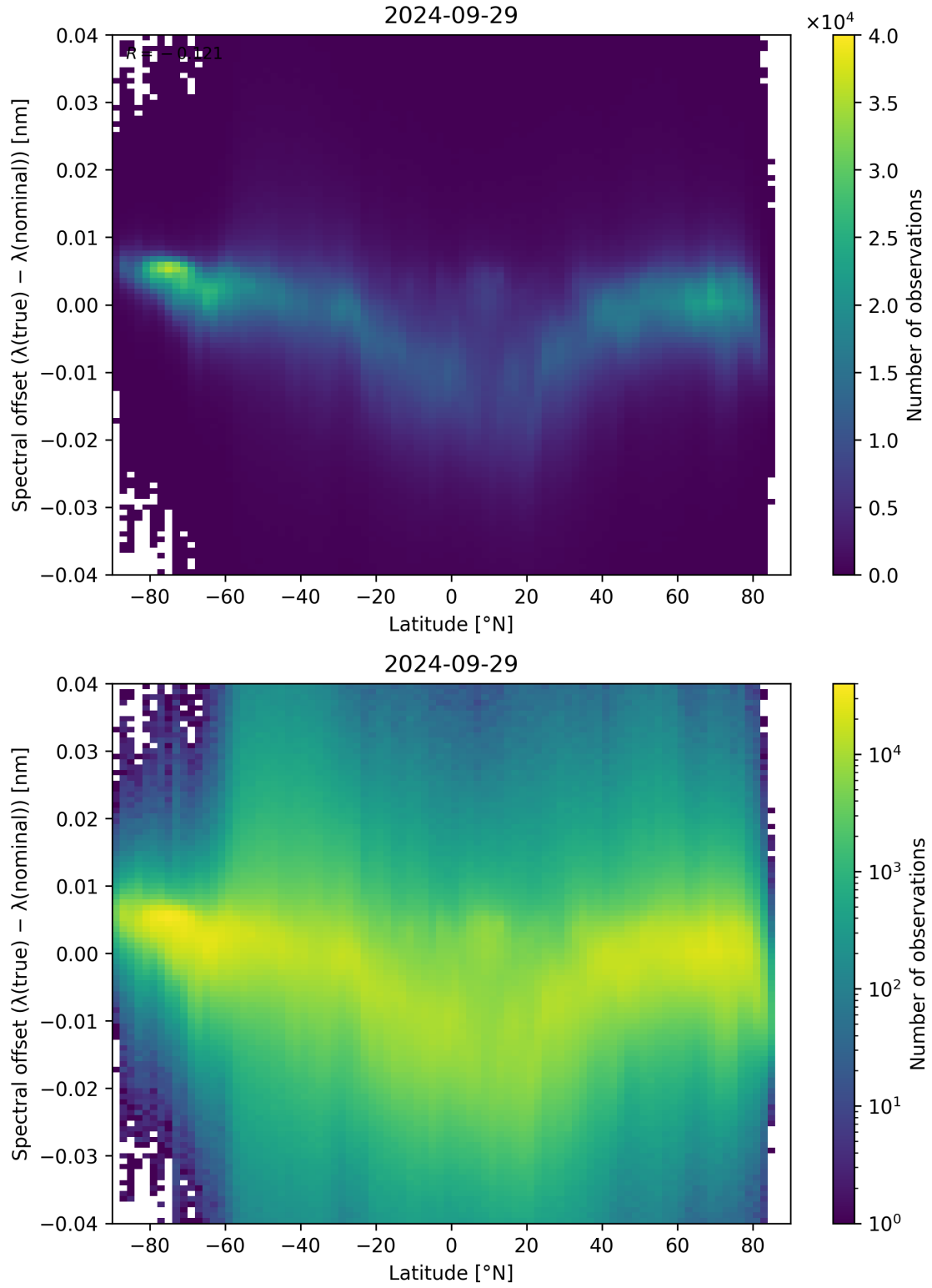
Figure 105: Scatter density plot of “Latitude” against “Spectral offset ( \lambda_{\text{true}} - \lambda_{\text{nominal}} )” for 2024-09-28 to 2024-09-30.
