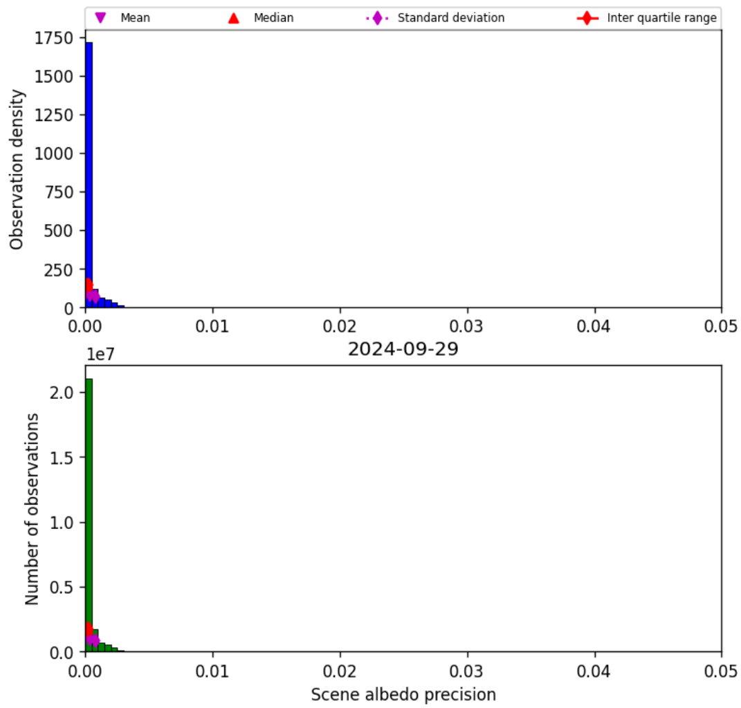
Figure 35: Histogram of “Scene albedo precision” for 2024-09-28 to 2024-09-30
