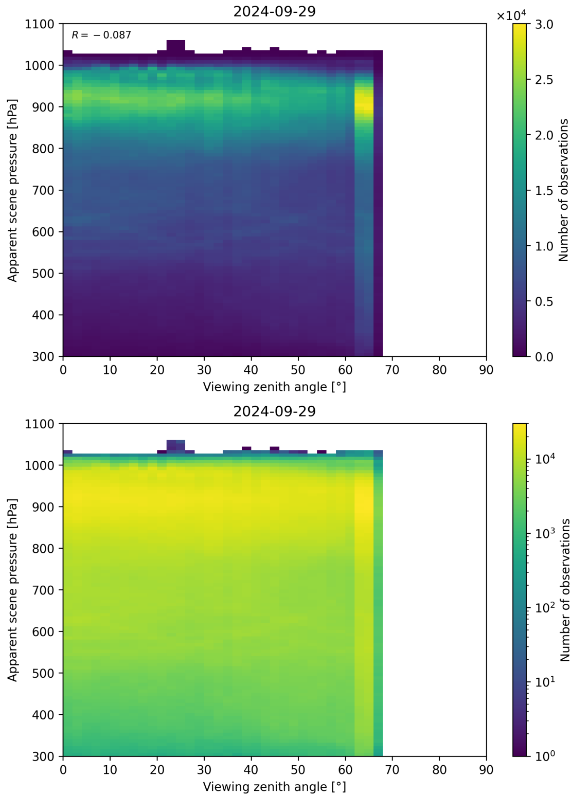
Figure 129: Scatter density plot of “Viewing zenith angle” against “Apparent scene pressure” for 2024-09-28 to 2024-09-30.
