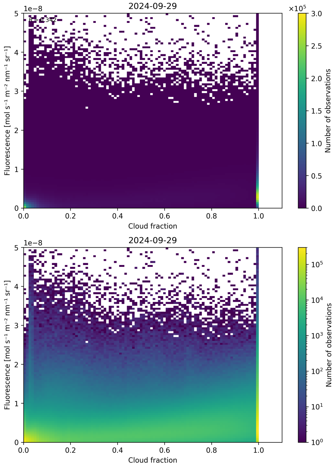
Figure 79: Scatter density plot of “Cloud fraction” against “Fluorescence” for 2024-09-28 to 2024-09-30.
