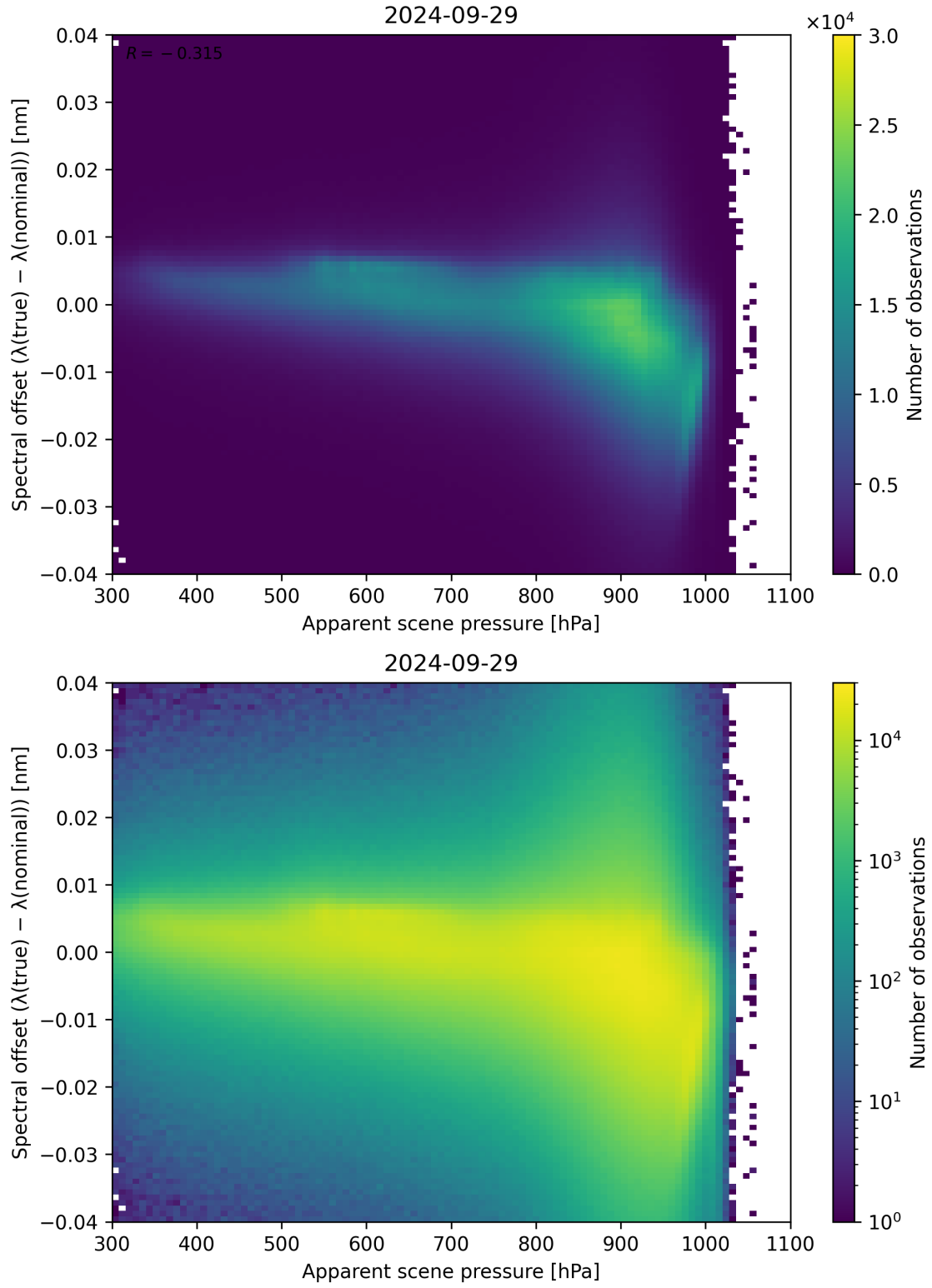
Figure 68: Scatter density plot of “Apparent scene pressure” against “Spectral offset ( \lambda_{\text{true}} - \lambda_{\text{nominal}} )” for 2024-09-28 to 2024-09-30.
