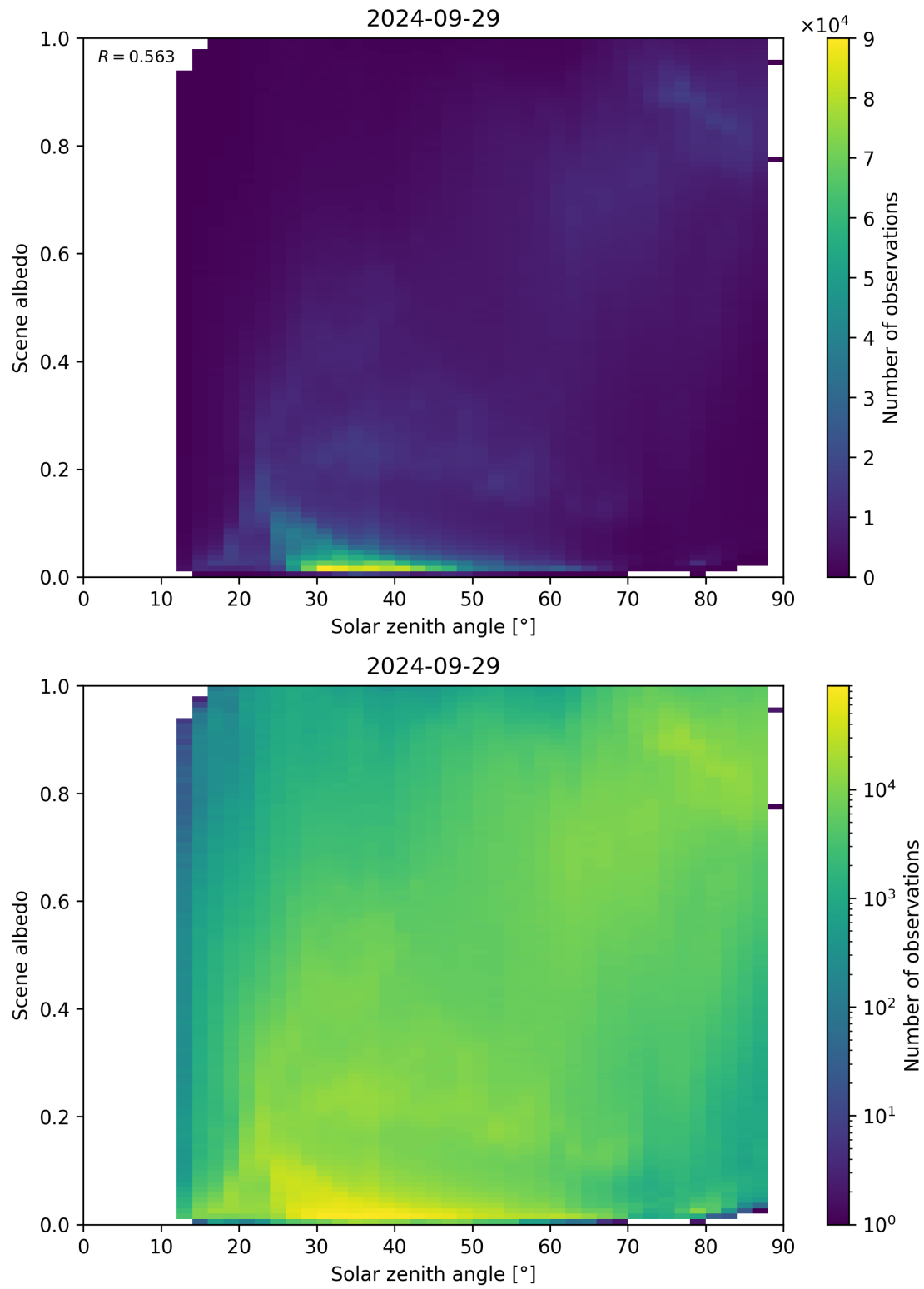
Figure 127: Scatter density plot of “Solar zenith angle” against “Scene albedo” for 2024-09-28 to 2024-09-30.
