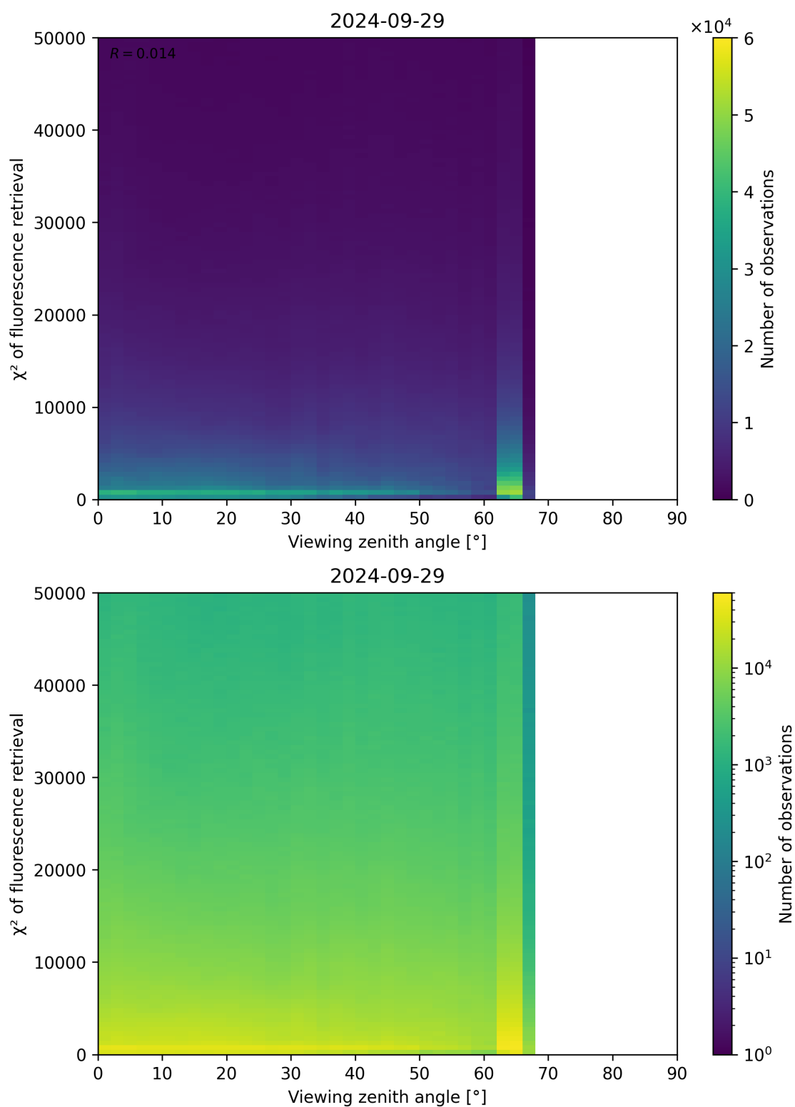
Figure 131: Scatter density plot of “Viewing zenith angle” against “ \chi^2 of fluorescence retrieval” for 2024-09-28 to 2024-09-30.
