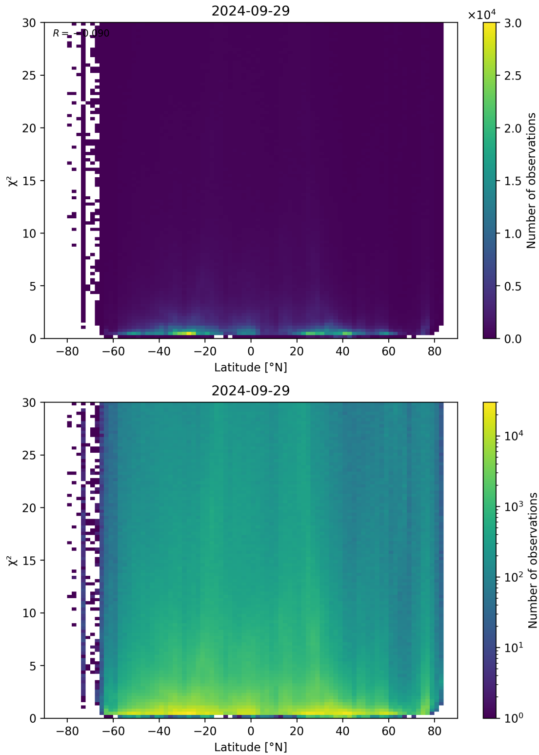
Figure 97: Scatter density plot of “Latitude” against “ \chi^2 ” for 2024-09-28 to 2024-09-30.
