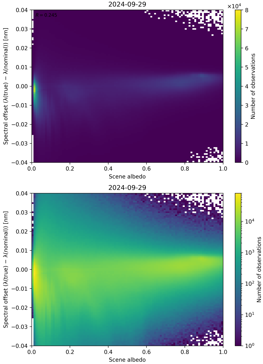
Figure 117: Scatter density plot of “Scene albedo” against “Spectral offset ( \lambda_{\text{true}} - \lambda_{\text{nominal}} )” for 2024-09-28 to 2024-09-30.
