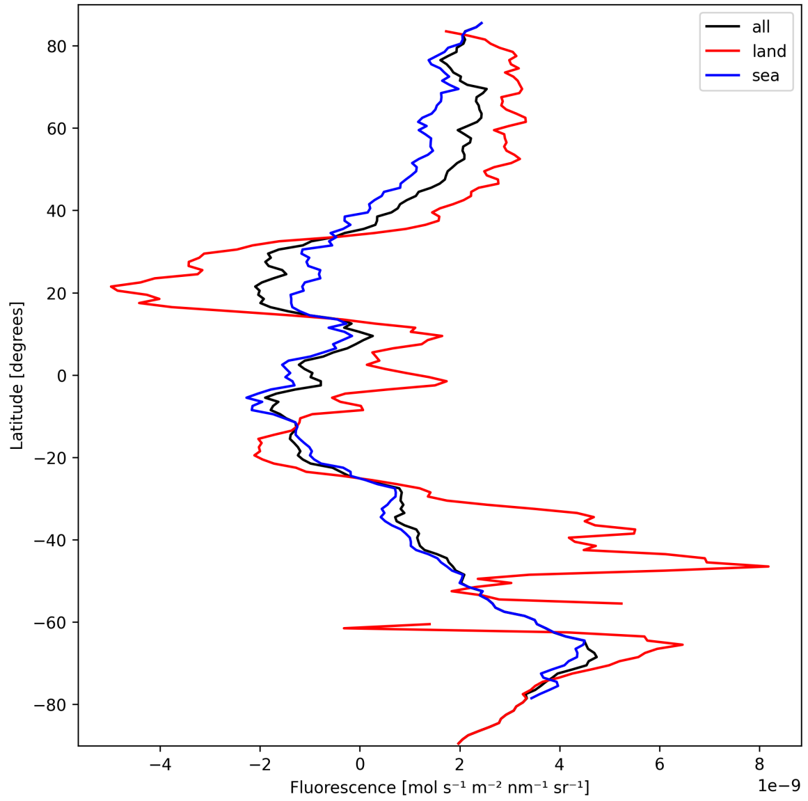
Figure 23: Zonal average of “Fluorescence” for 2024-09-28 to 2024-09-30.
