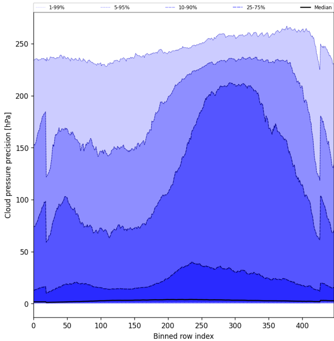
Figure 48: Along track statistics of “Cloud pressure precision” for 2024-09-28 to 2024-09-30
