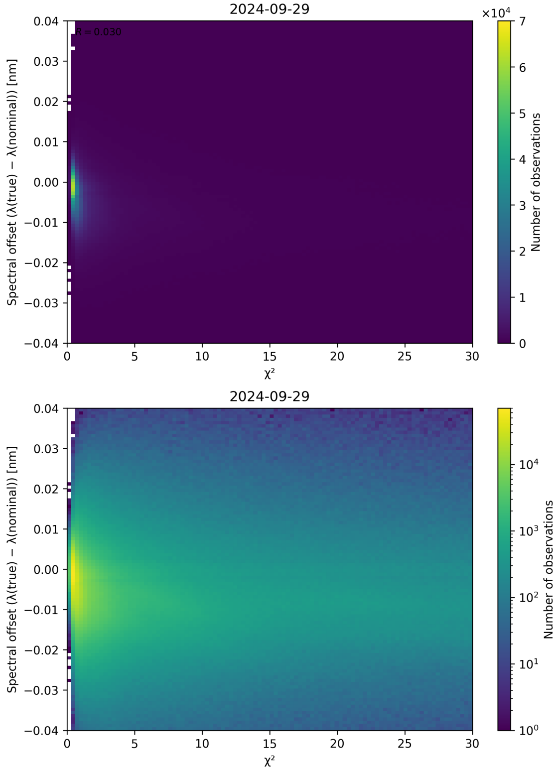
Figure 75: Scatter density plot of “ \chi^2 ” against “Spectral offset ( \lambda_{\text{true}} - \lambda_{\text{nominal}} )” for 2024-09-28 to 2024-09-30.
