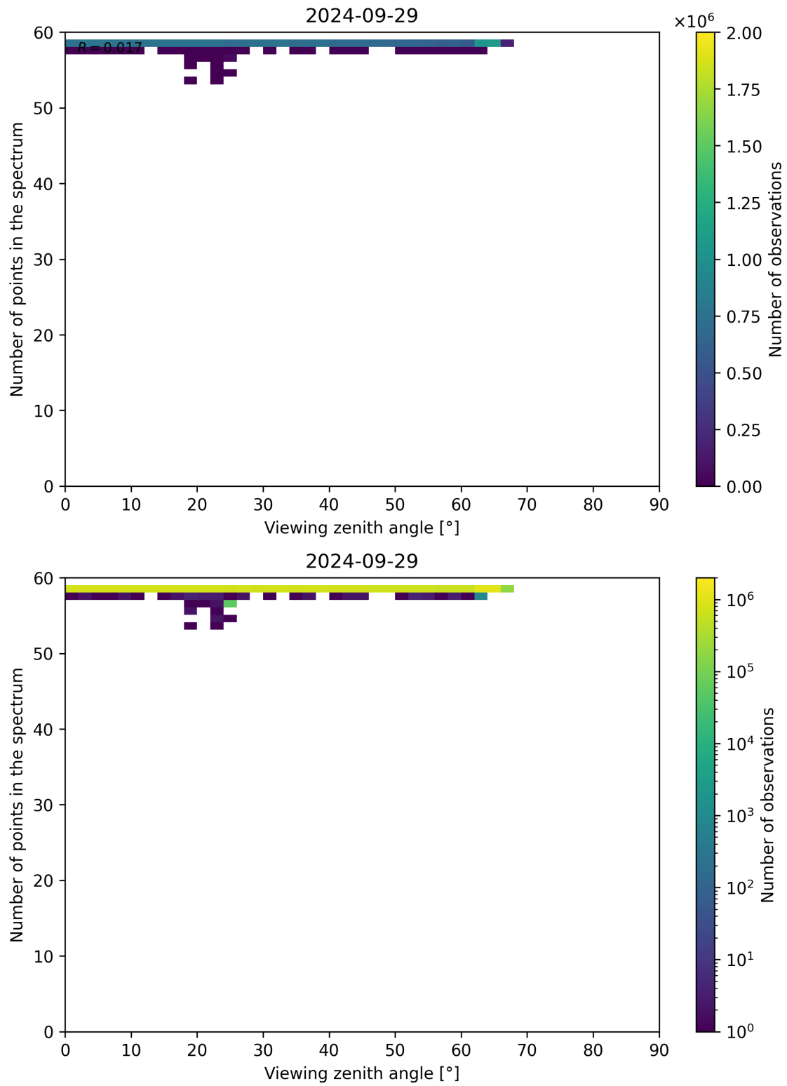
Figure 137: Scatter density plot of “Viewing zenith angle” against “Number of points in the spectrum” for 2024-09-28 to 2024-09-30.
