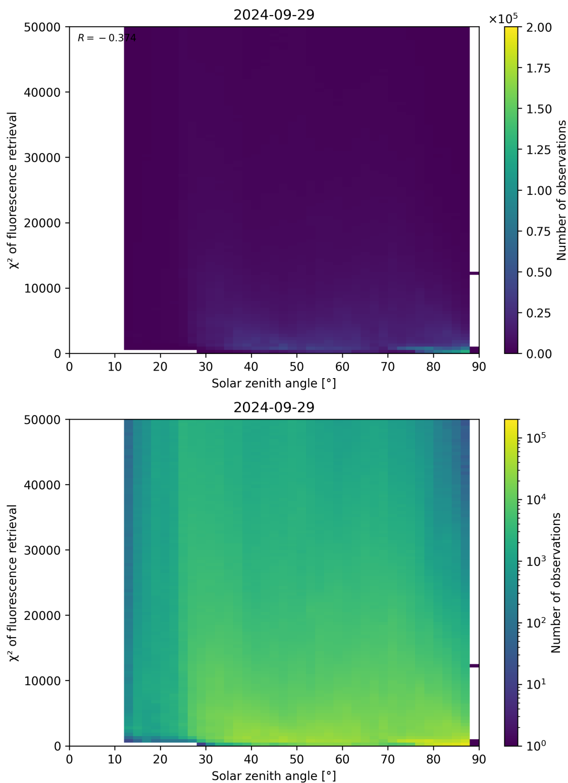
Figure 120: Scatter density plot of “Solar zenith angle” against “ \chi^2 of fluorescence retrieval” for 2024-09-28 to 2024-09-30.
