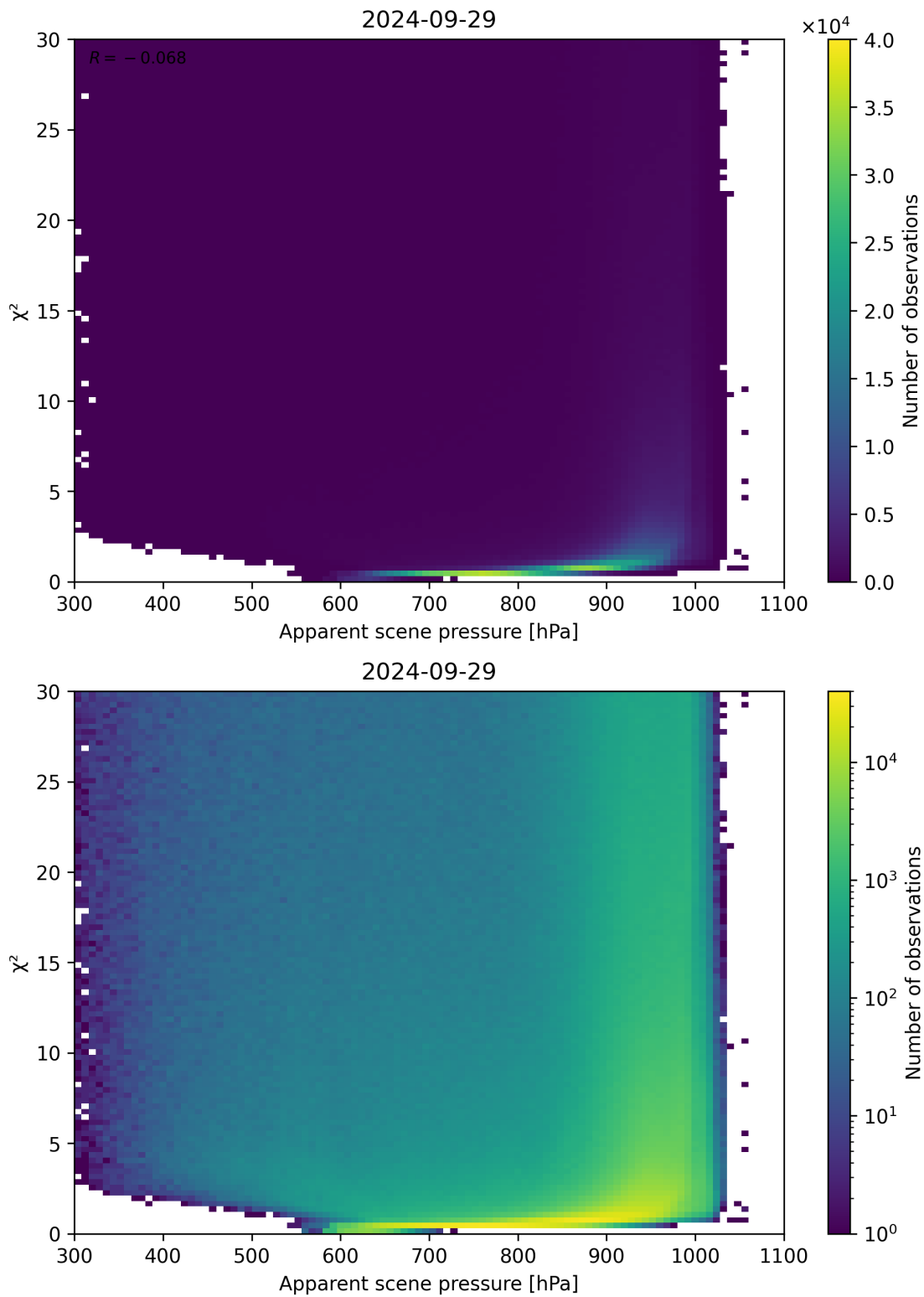
Figure 63: Scatter density plot of “Apparent scene pressure” against “ \chi^2 ” for 2024-09-28 to 2024-09-30.
