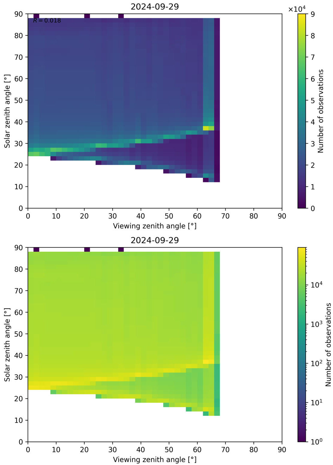
Figure 139: Scatter density plot of “Viewing zenith angle” against “Solar zenith angle” for 2024-09-28 to 2024-09-30.
