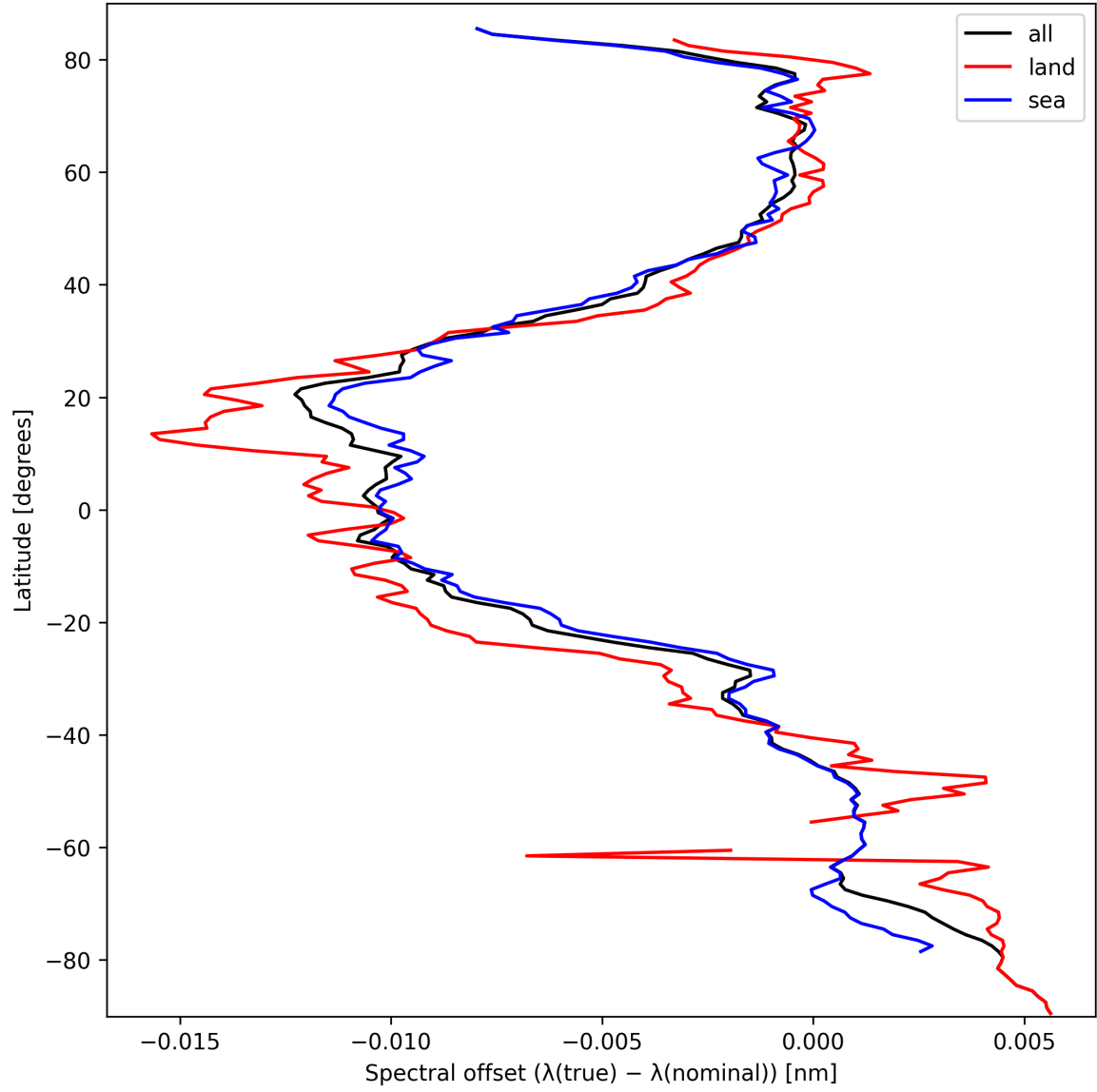
Figure 28: Zonal average of “Spectral offset ( \lambda_{\text{true}} - \lambda_{\text{nominal}} )” for 2024-09-28 to 2024-09-30.
