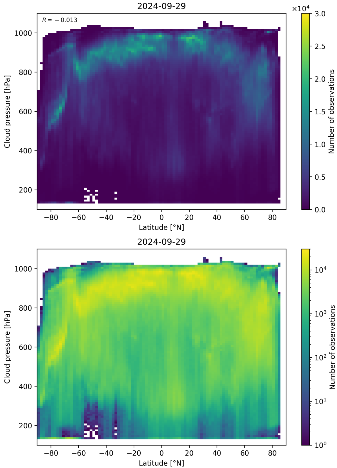
Figure 100: Scatter density plot of “Latitude” against “Cloud pressure” for 2024-09-28 to 2024-09-30.
