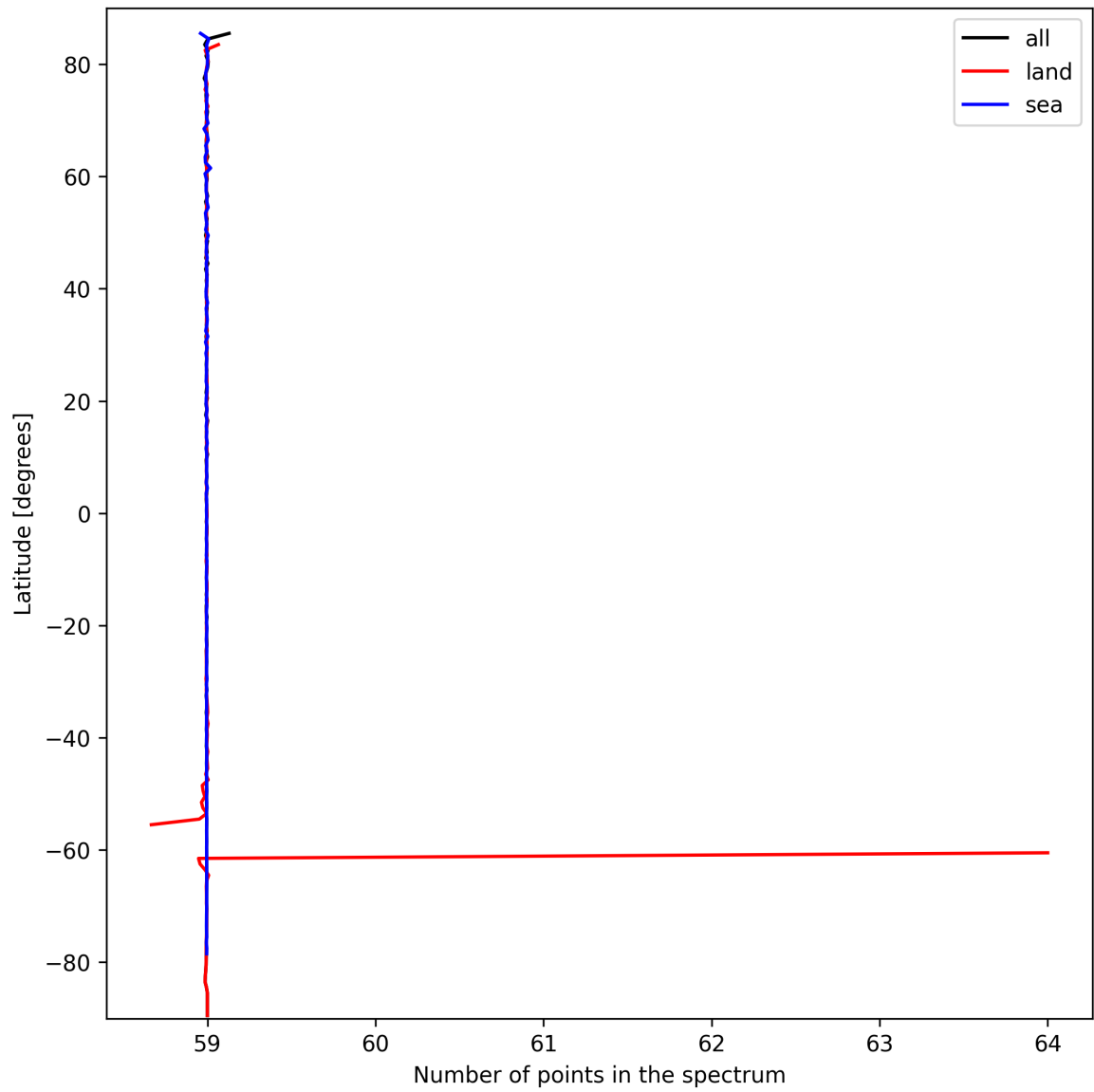
Figure 27: Zonal average of “Number of points in the spectrum” for 2024-09-28 to 2024-09-30.
