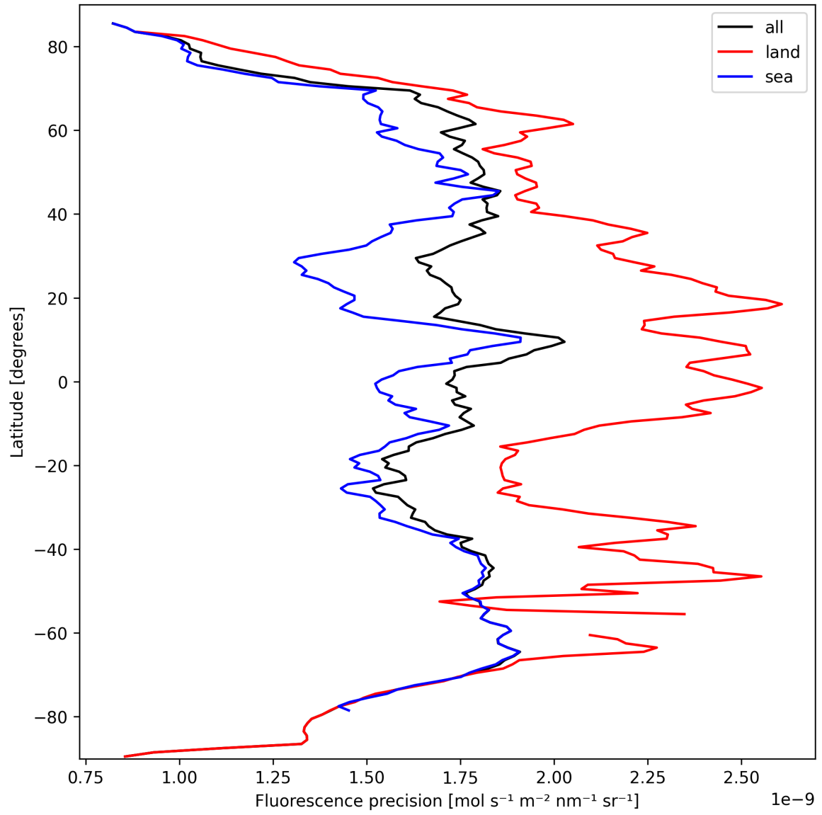
Figure 24: Zonal average of “Fluorescence precision” for 2024-09-28 to 2024-09-30.
