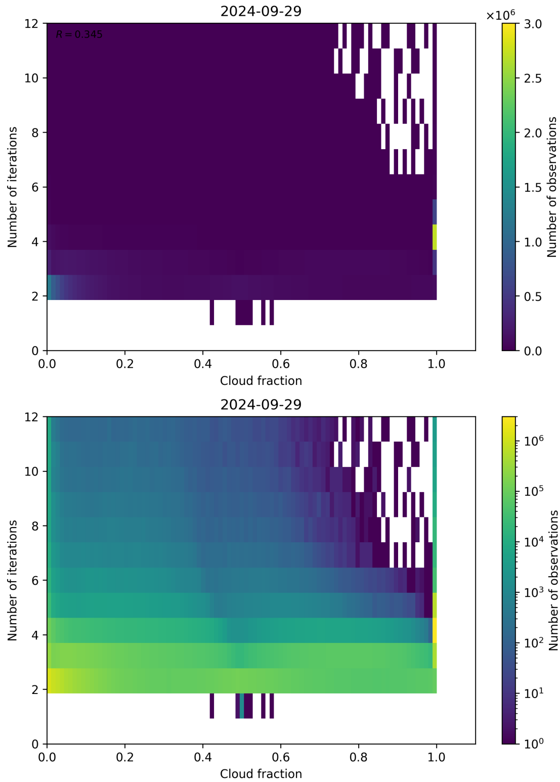
Figure 80: Scatter density plot of “Cloud fraction” against “Number of iterations” for 2024-09-28 to 2024-09-30.
