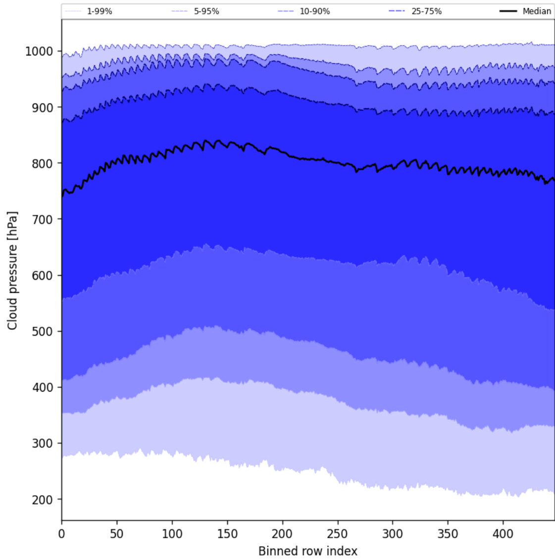
Figure 47: Along track statistics of “Cloud pressure” for 2024-09-28 to 2024-09-30
