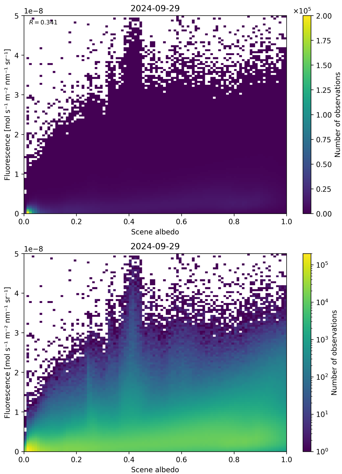
Figure 114: Scatter density plot of “Scene albedo” against “Fluorescence” for 2024-09-28 to 2024-09-30.
