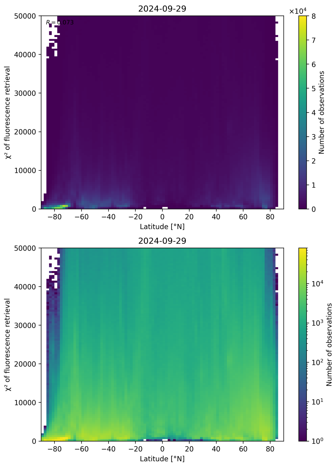
Figure 98: Scatter density plot of “Latitude” against “ \chi^2 of fluorescence retrieval” for 2024-09-28 to 2024-09-30.
