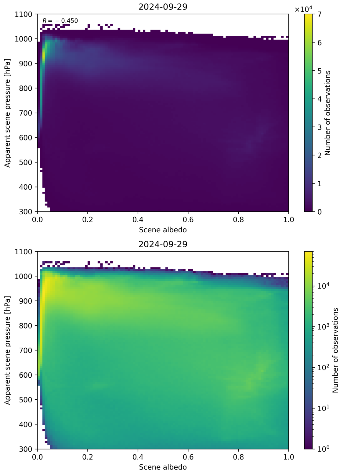
Figure 111: Scatter density plot of “Scene albedo” against “Apparent scene pressure” for 2024-09-28 to 2024-09-30.
