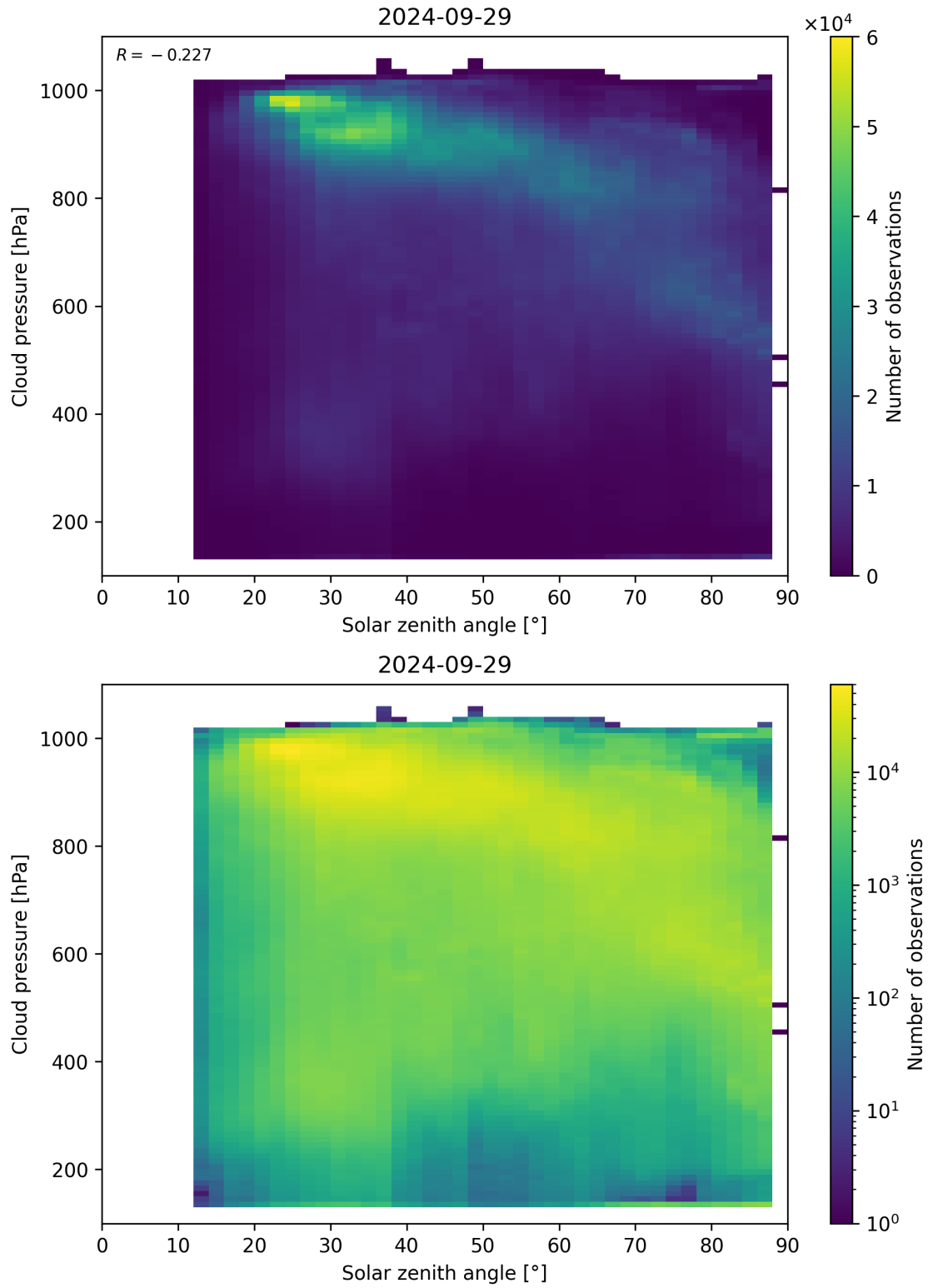
Figure 122: Scatter density plot of “Solar zenith angle” against “Cloud pressure” for 2024-09-28 to 2024-09-30.
