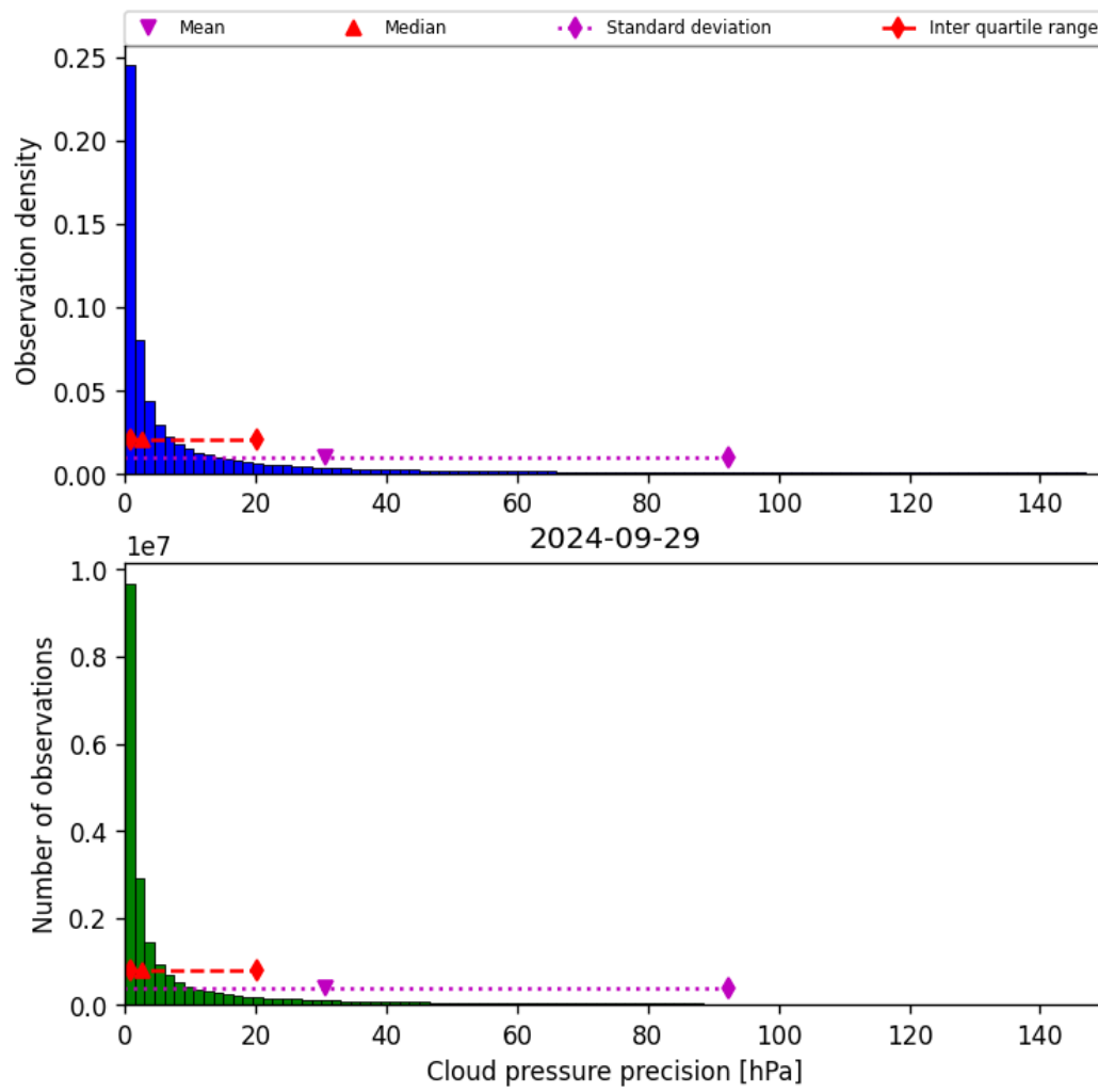
Figure 31: Histogram of “Cloud pressure precision” for 2024-09-28 to 2024-09-30
