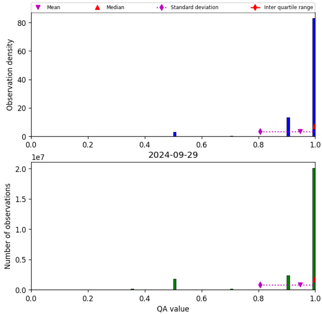
Figure 29: Histogram of “QA value” for 2024-09-28 to 2024-09-30
