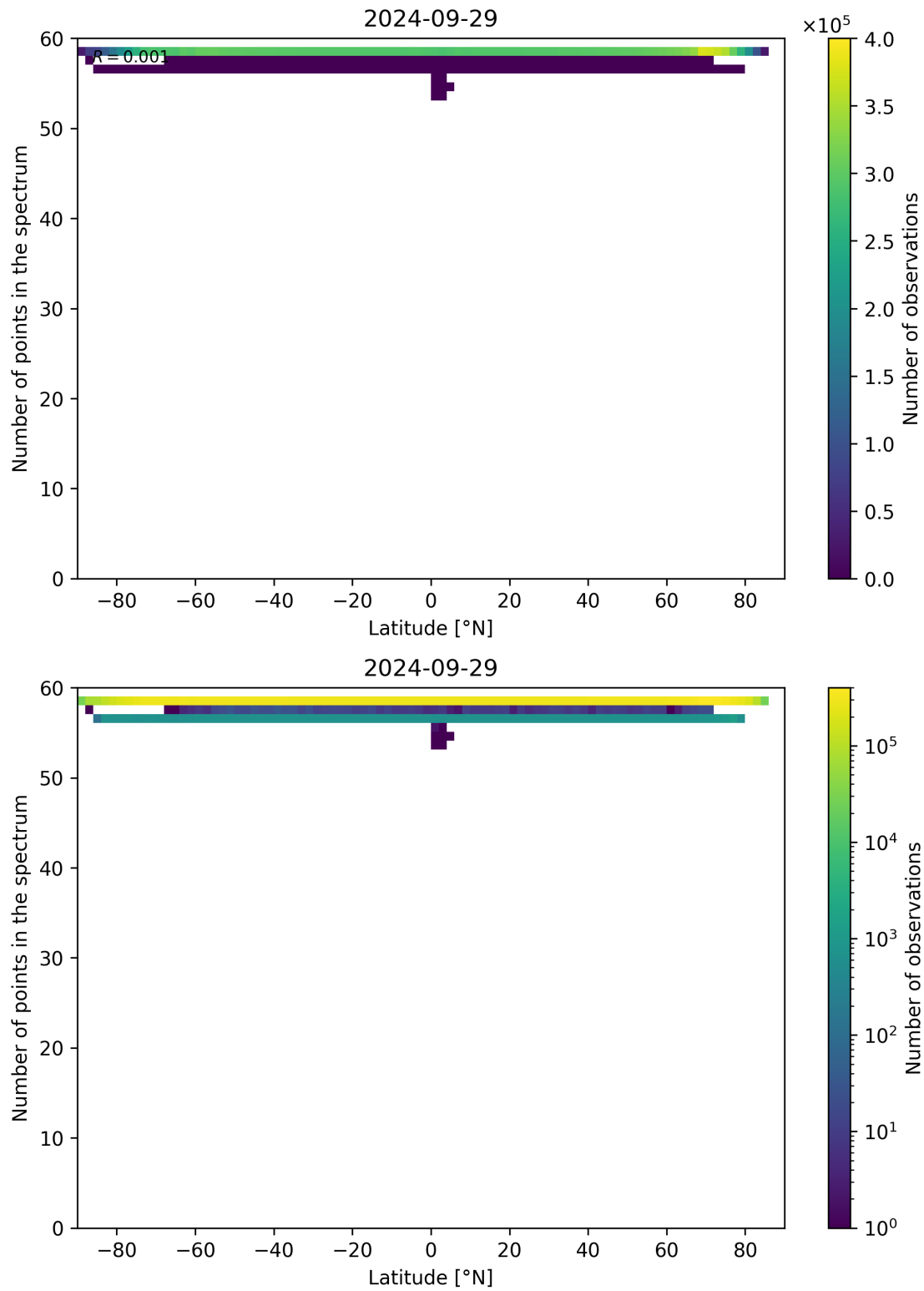
Figure 103: Scatter density plot of “Latitude” against “Number of points in the spectrum” for 2024-09-28 to 2024-09-30.
