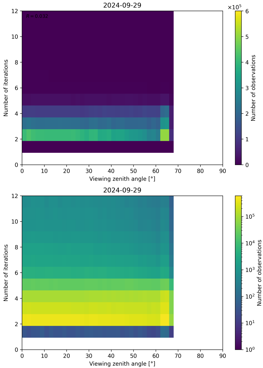
Figure 136: Scatter density plot of “Viewing zenith angle” against “Number of iterations” for 2024-09-28 to 2024-09-30.
