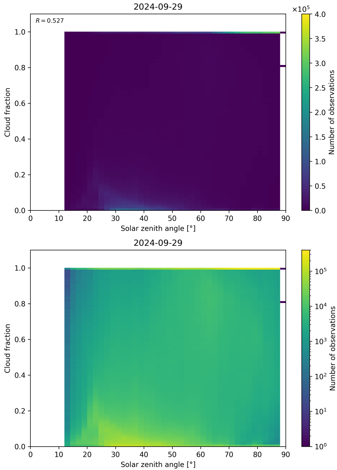
Figure 121: Scatter density plot of “Solar zenith angle” against “Cloud fraction” for 2024-09-28 to 2024-09-30.
