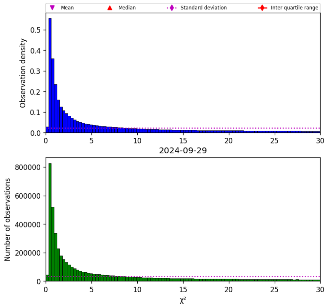
Figure 38: Histogram of “ \chi^2 ” for 2024-09-28 to 2024-09-30
