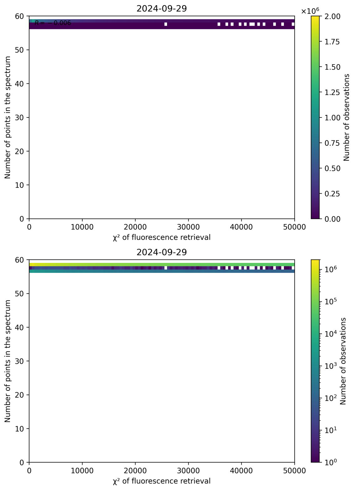
Figure 71: Scatter density plot of " \chi^2 of fluorescence retrieval" against "Number of points in the spectrum" for 2024-09-28 to 2024-09-30.
