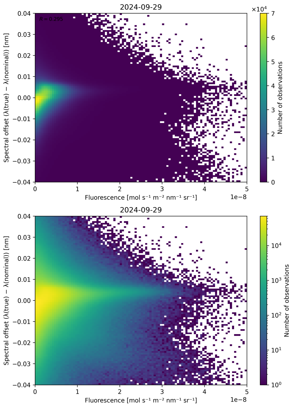
Figure 95: Scatter density plot of “Fluorescence” against “Spectral offset ( \lambda_{\text{true}} - \lambda_{\text{nominal}} )” for 2024-09-28 to 2024-09-30.
