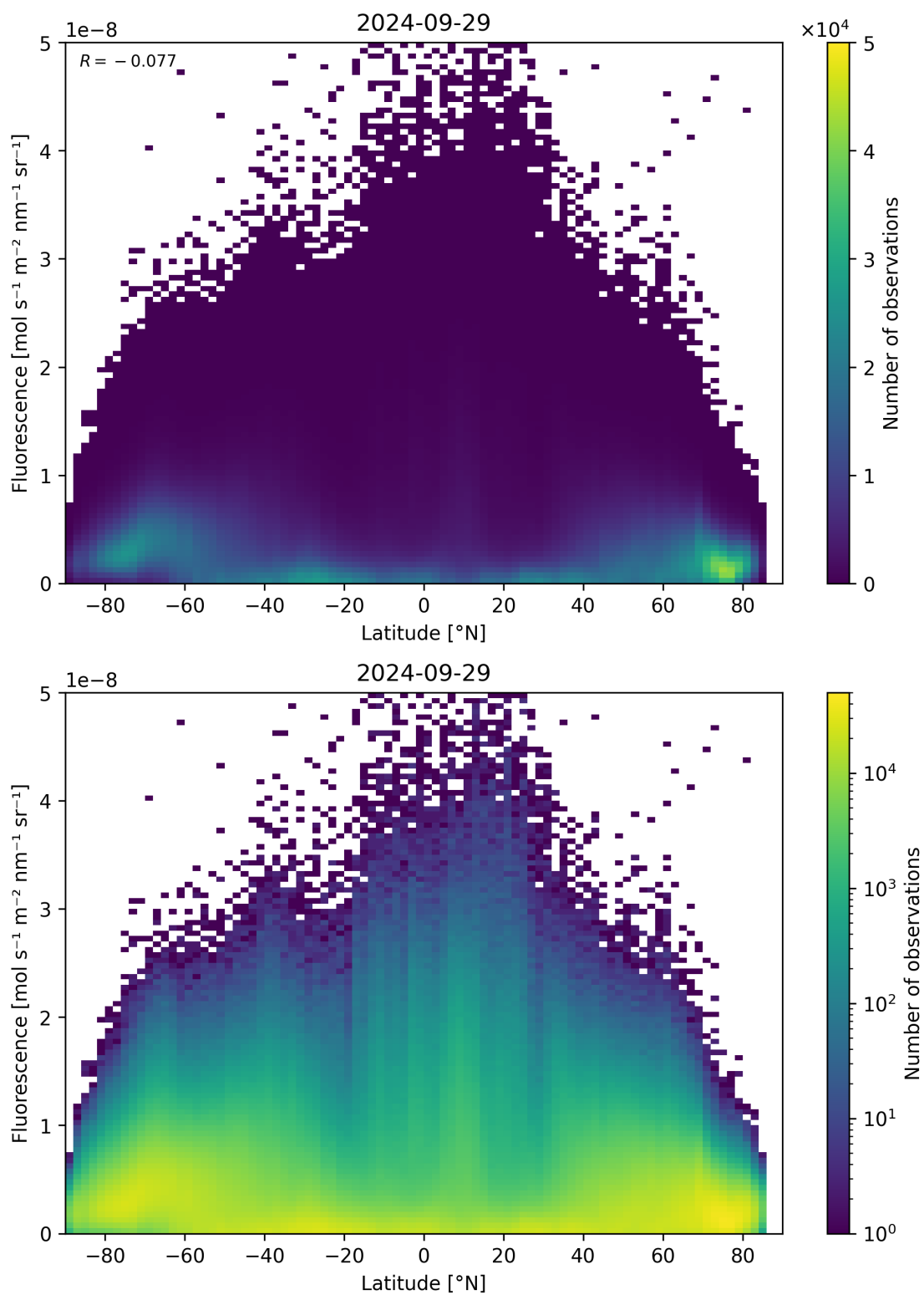
Figure 101: Scatter density plot of “Latitude” against “Fluorescence” for 2024-09-28 to 2024-09-30.
