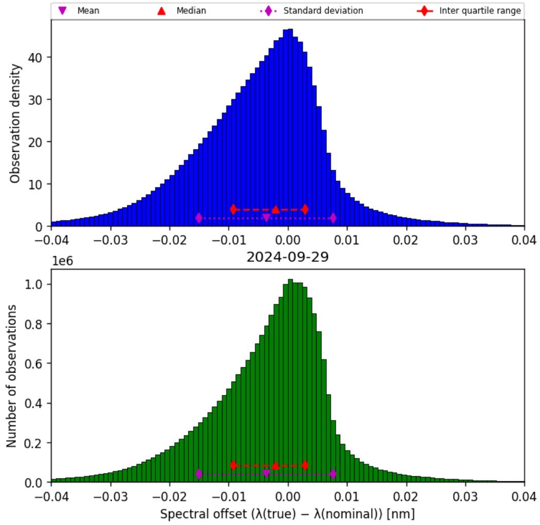
Figure 45: Histogram of “Spectral offset ( \lambda_{\text{true}} - \lambda_{\text{nominal}} )” for 2024-09-28 to 2024-09-30
