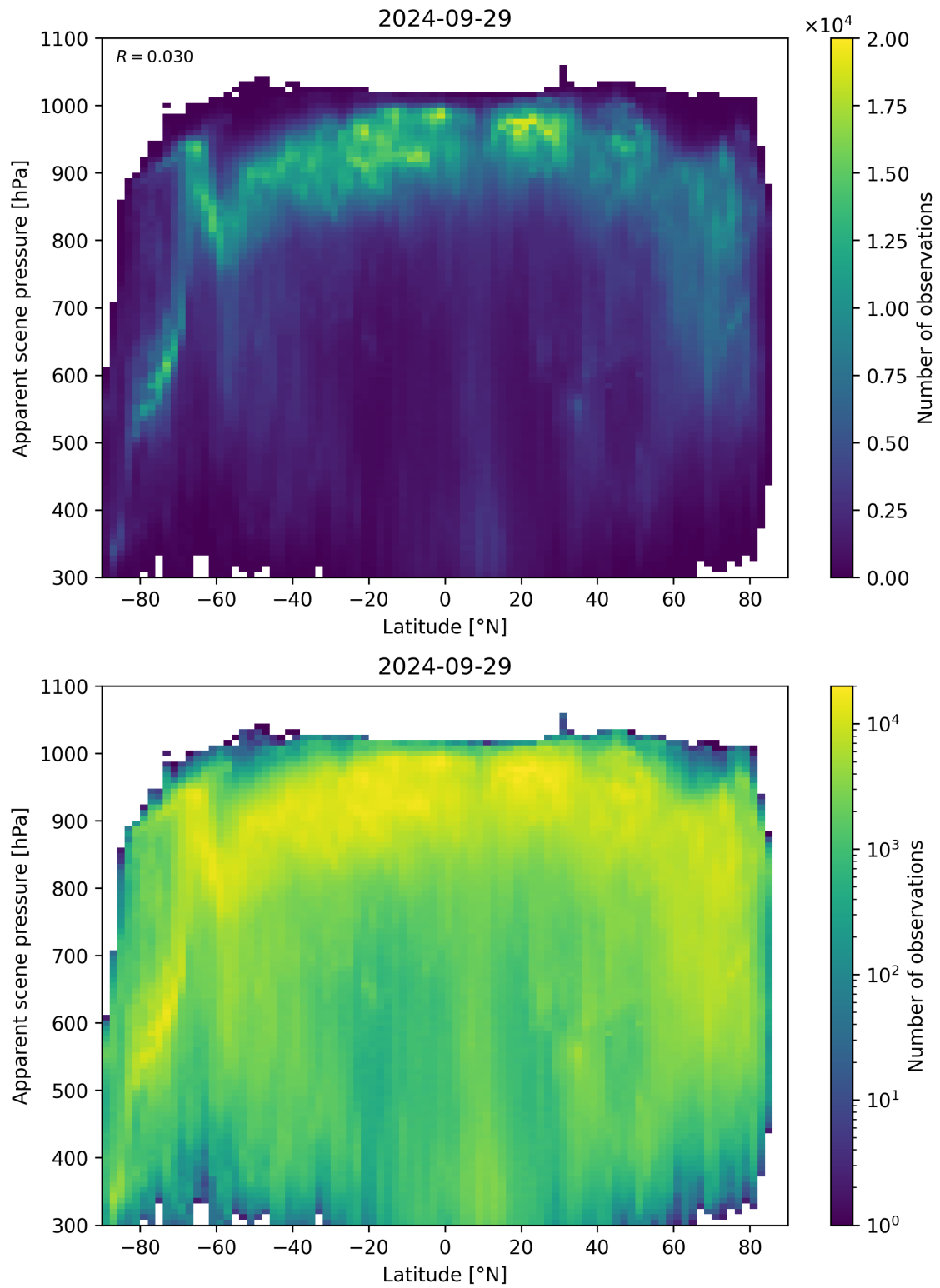
Figure 96: Scatter density plot of “Latitude” against “Apparent scene pressure” for 2024-09-28 to 2024-09-30.
