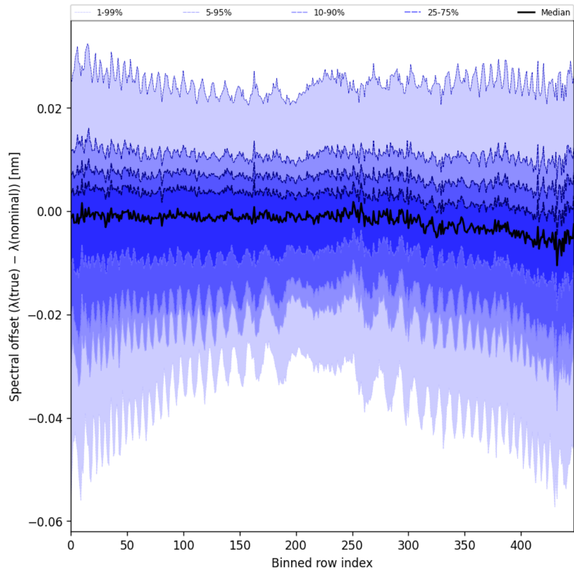
Figure 62: Along track statistics of “Spectral offset ( \lambda_{\text{true}} - \lambda_{\text{nominal}} )” for 2024-09-28 to 2024-09-30
