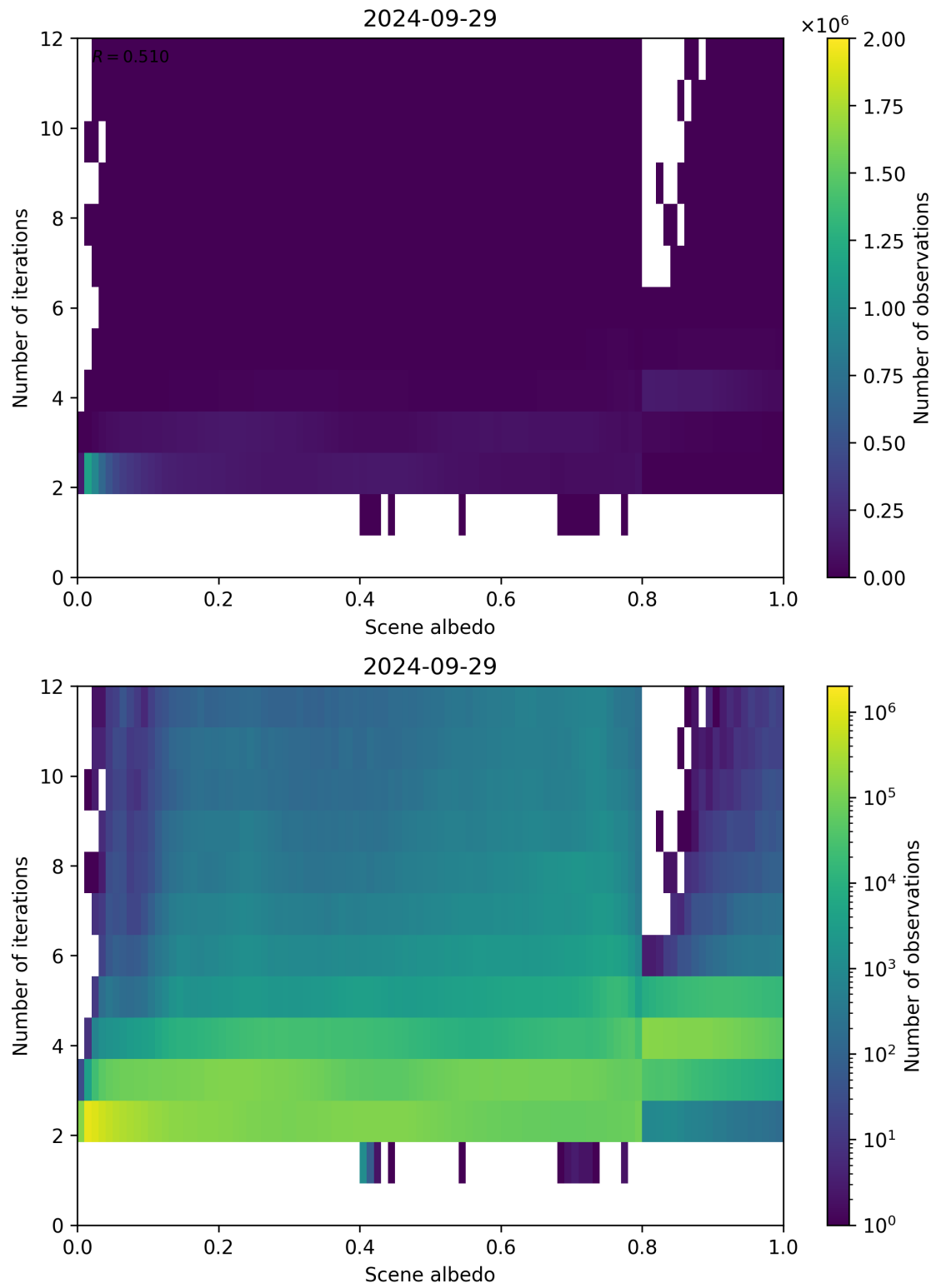
Figure 115: Scatter density plot of “Scene albedo” against “Number of iterations” for 2024-09-28 to 2024-09-30.
