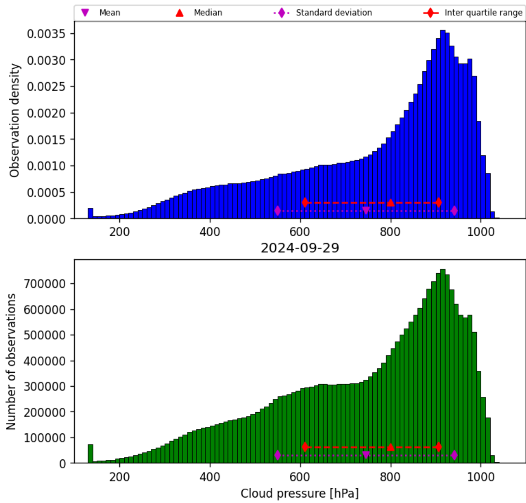
Figure 30: Histogram of “Cloud pressure” for 2024-09-28 to 2024-09-30
