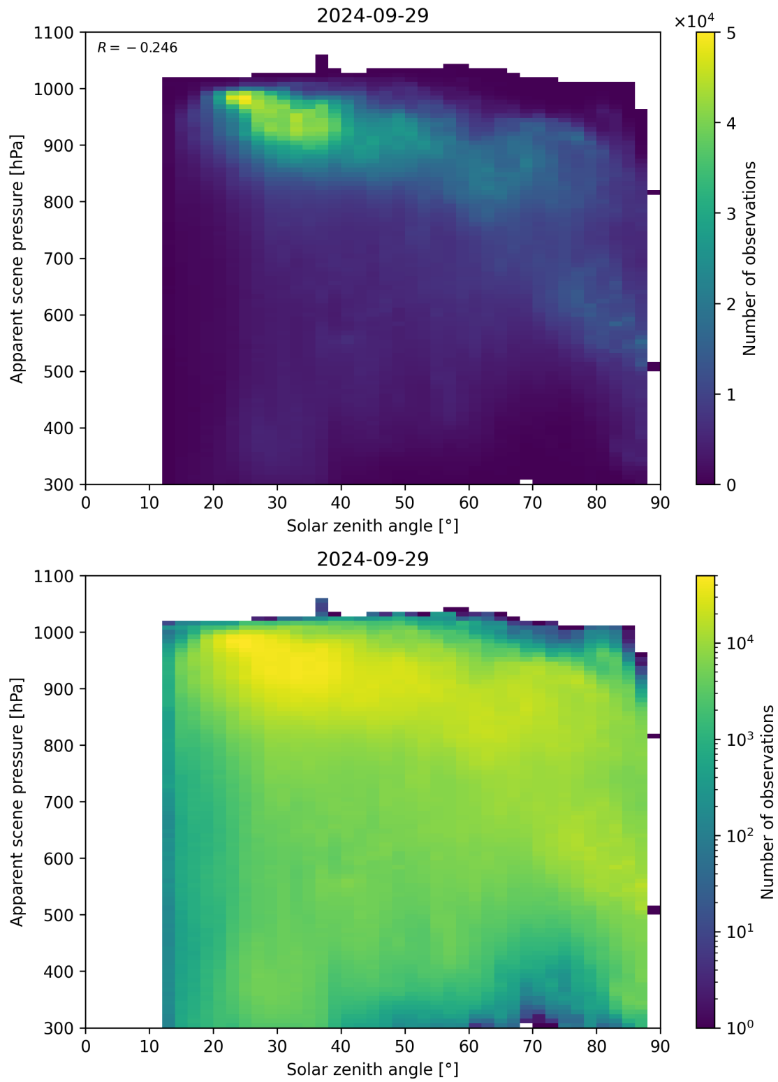
Figure 118: Scatter density plot of “Solar zenith angle” against “Apparent scene pressure” for 2024-09-28 to 2024-09-30.
