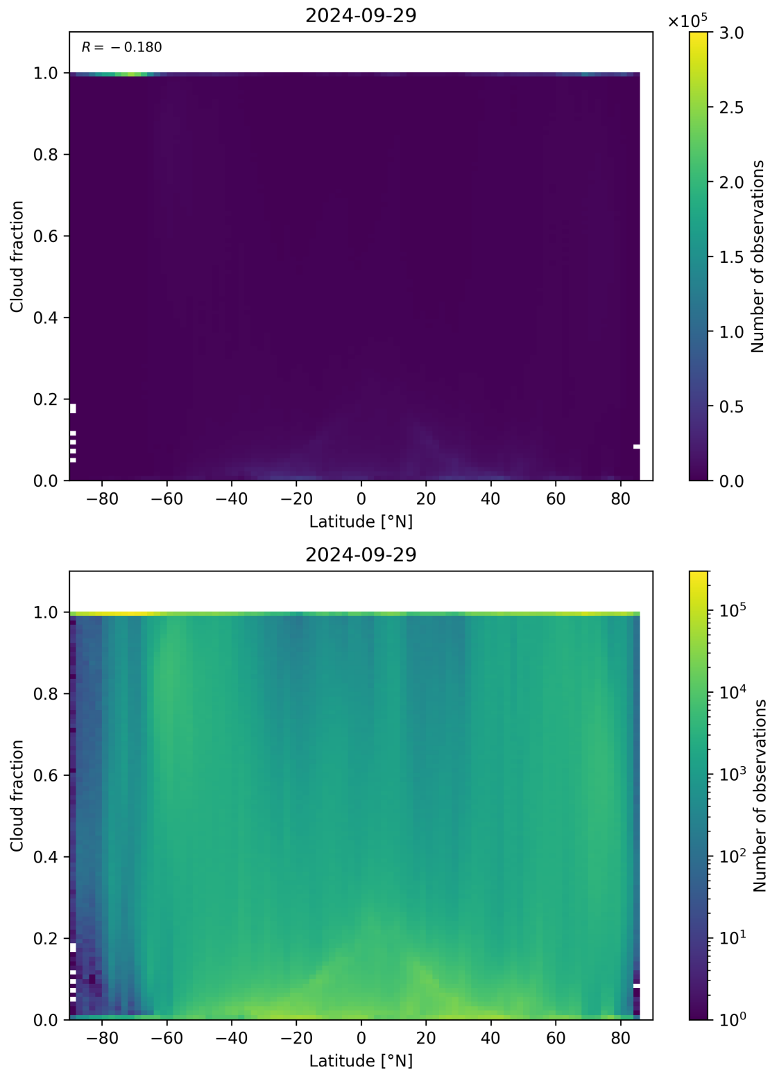
Figure 99: Scatter density plot of “Latitude” against “Cloud fraction” for 2024-09-28 to 2024-09-30.
