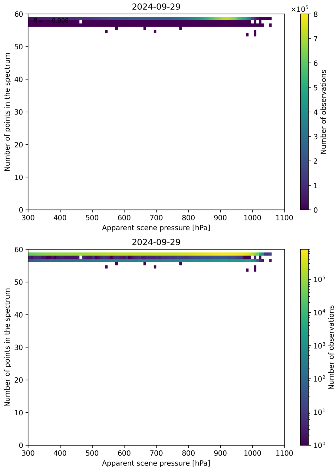
Figure 67: Scatter density plot of “Apparent scene pressure” against “Number of points in the spectrum” for 2024-09-28 to 2024-09-30.
