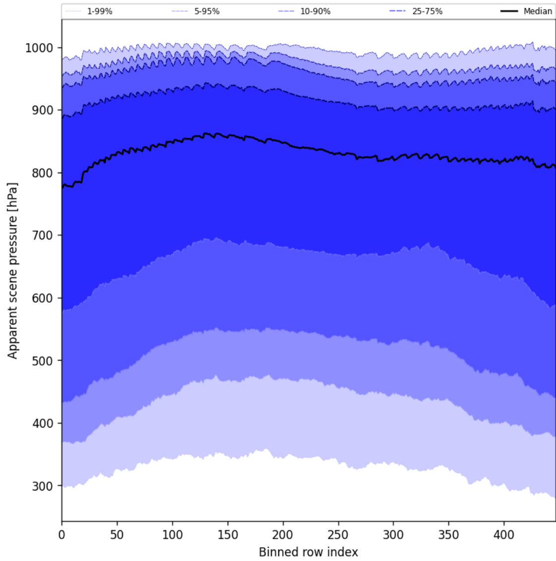
Figure 53: Along track statistics of “Apparent scene pressure” for 2024-09-28 to 2024-09-30
