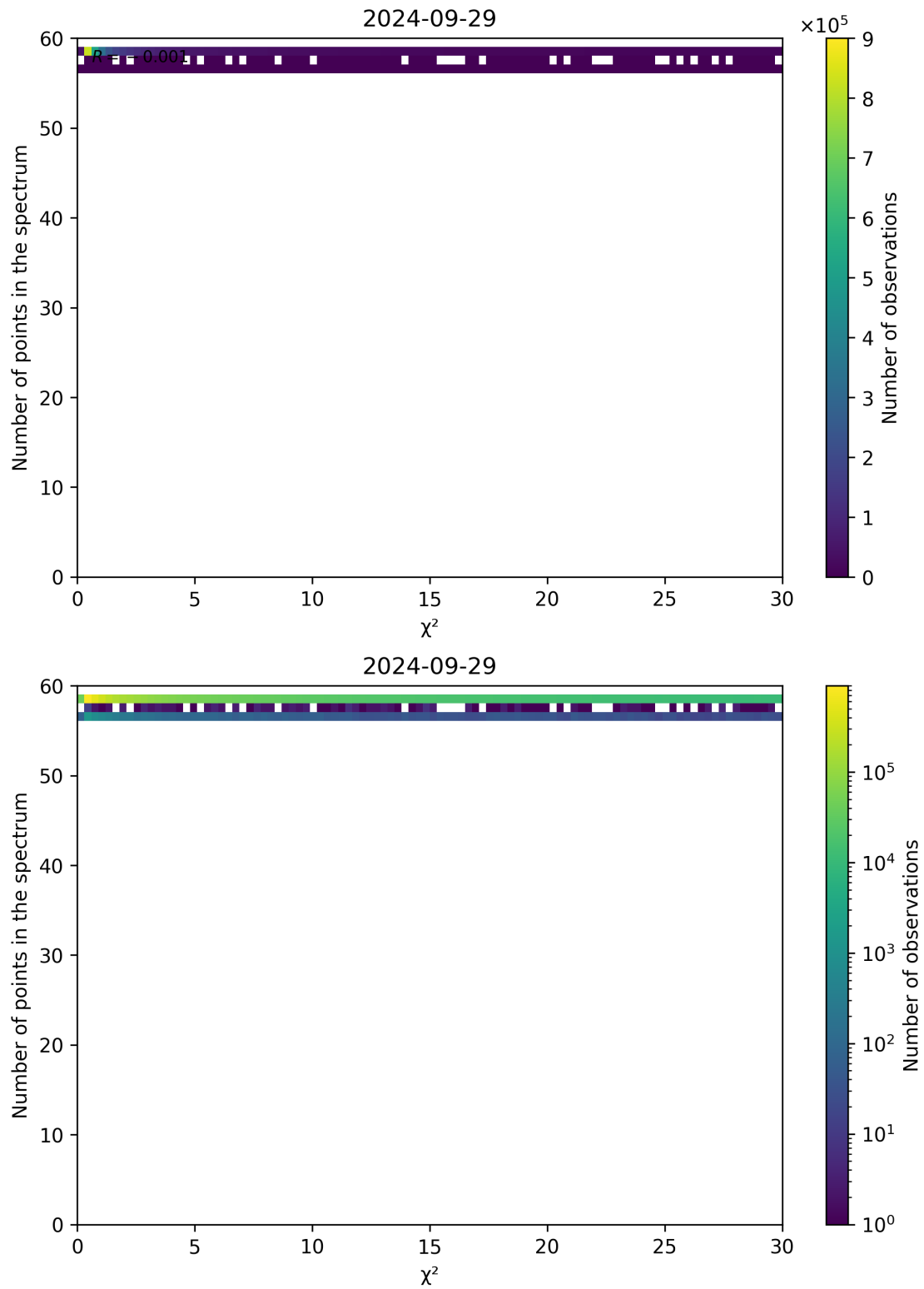
Figure 74: Scatter density plot of “ \chi^2 ” against “Number of points in the spectrum” for 2024-09-28 to 2024-09-30.
