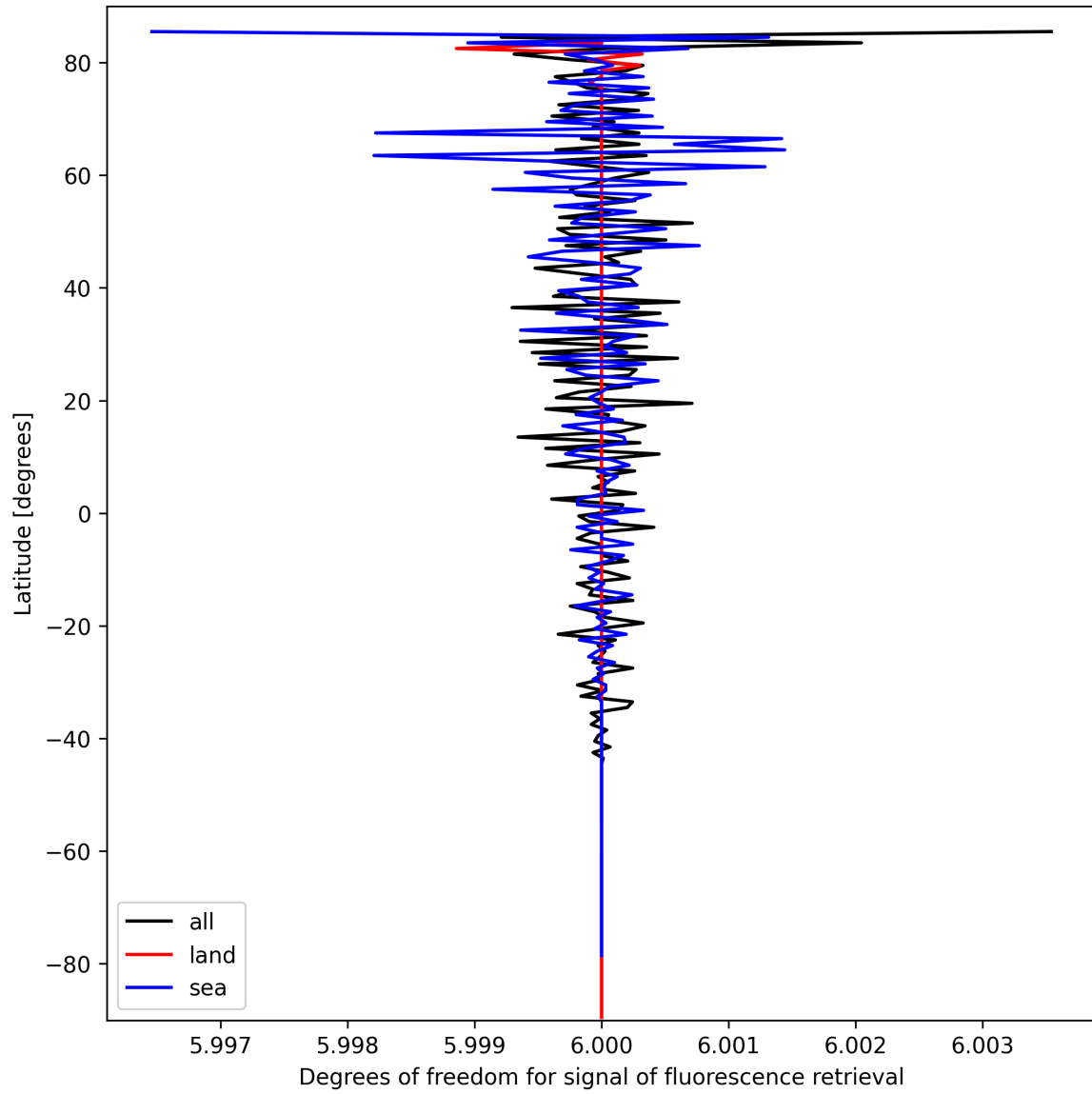
Figure 26: Zonal average of “Degrees of freedom for signal of fluorescence retrieval” for 2024-09-28 to 2024-09-30.
