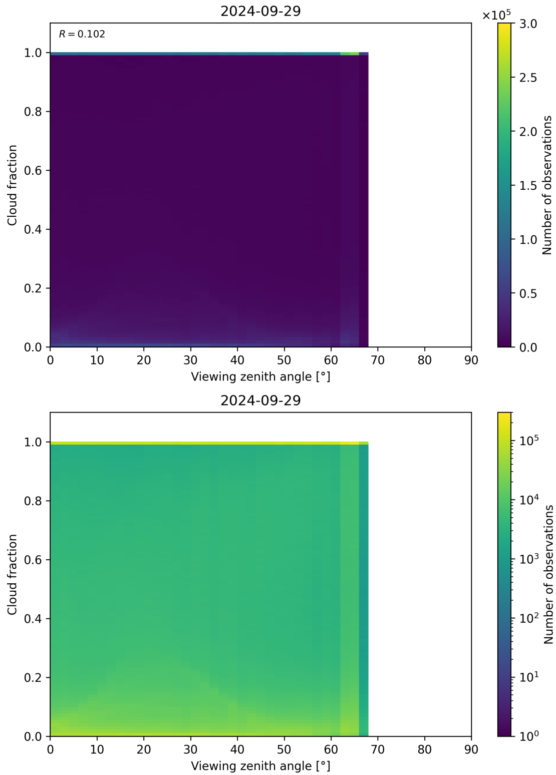
Figure 132: Scatter density plot of “Viewing zenith angle” against “Cloud fraction” for 2024-09-28 to 2024-09-30.
