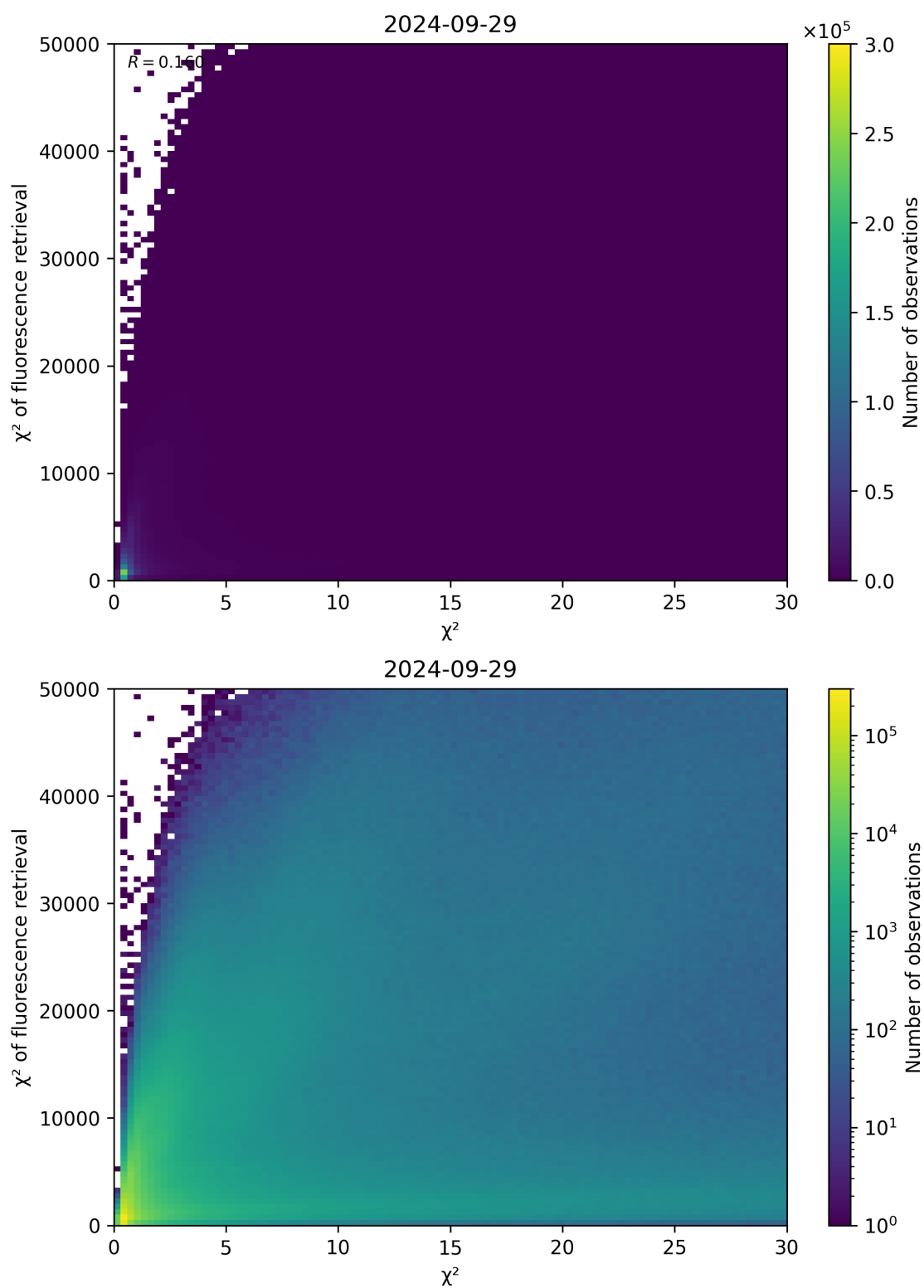
Figure 69: Scatter density plot of “ \chi^2 ” against “ \chi^2 of fluorescence retrieval” for 2024-09-28 to 2024-09-30.
