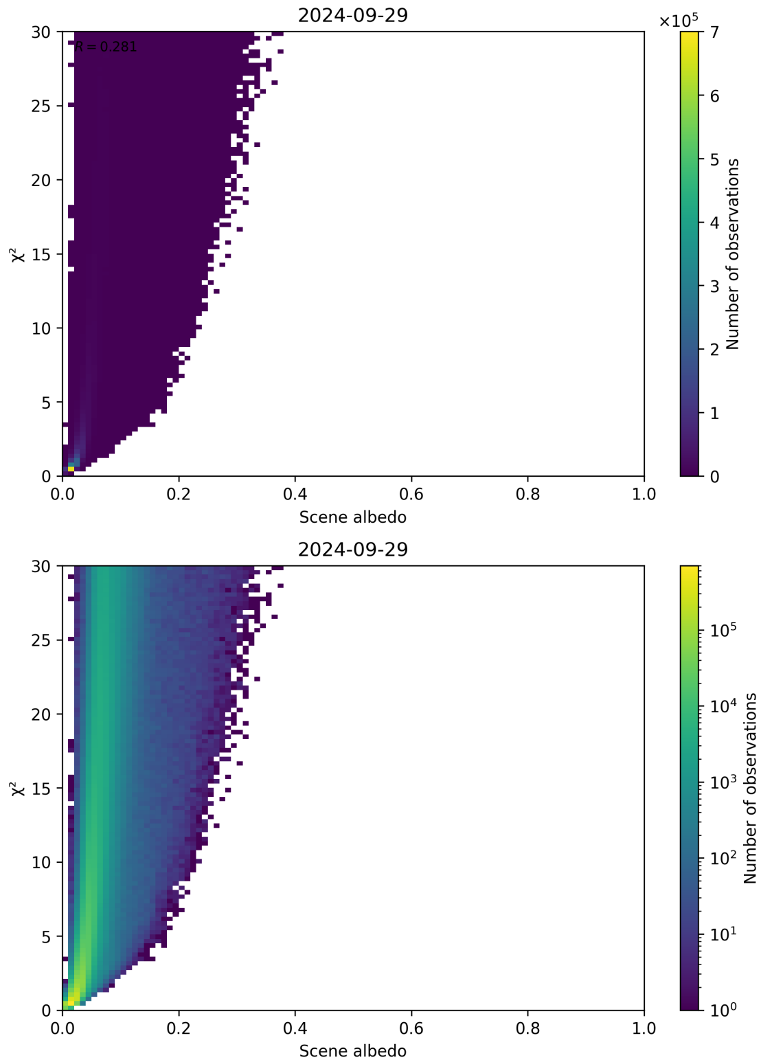
Figure 112: Scatter density plot of “Scene albedo” against “ \chi^2 ” for 2024-09-28 to 2024-09-30.
