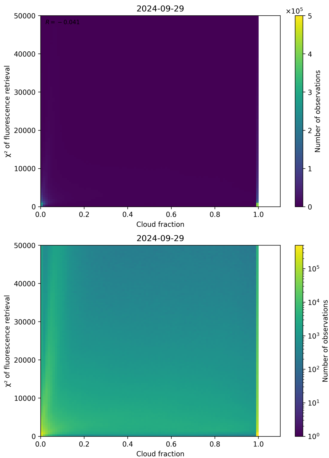
Figure 78: Scatter density plot of “Cloud fraction” against “ \chi^2 of fluorescence retrieval” for 2024-09-28 to 2024-09-30.
