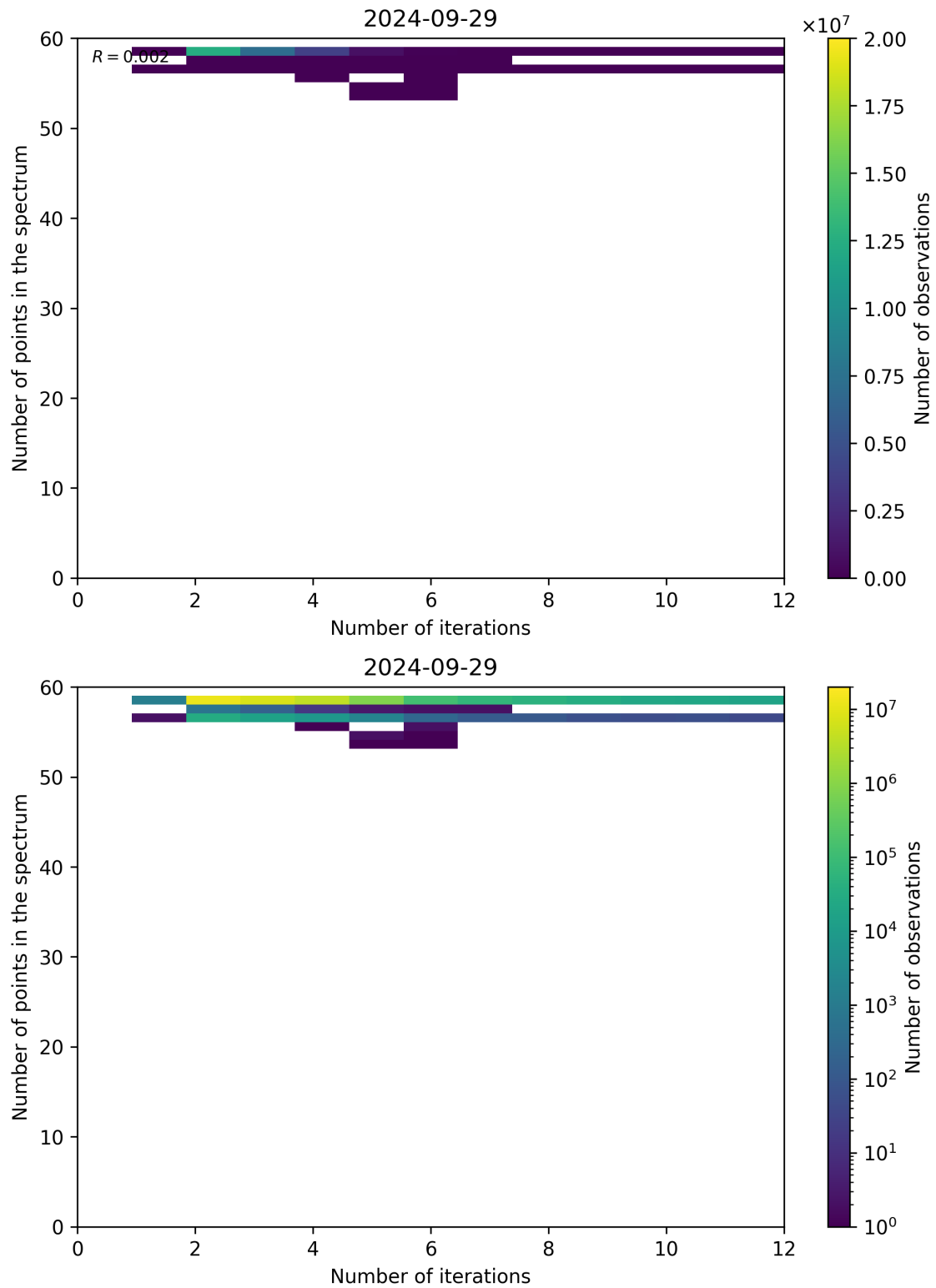
Figure 108: Scatter density plot of “Number of iterations” against “Number of points in the spectrum” for 2024-09-28 to 2024-09-30.
