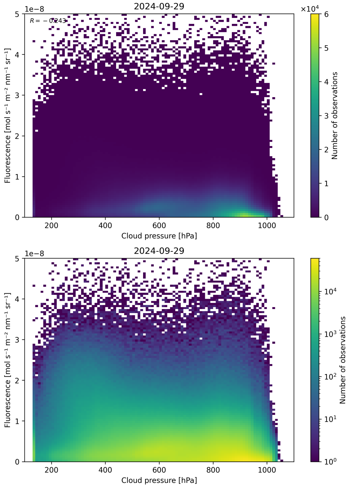
Figure 88: Scatter density plot of “Cloud pressure” against “Fluorescence” for 2024-09-28 to 2024-09-30.
