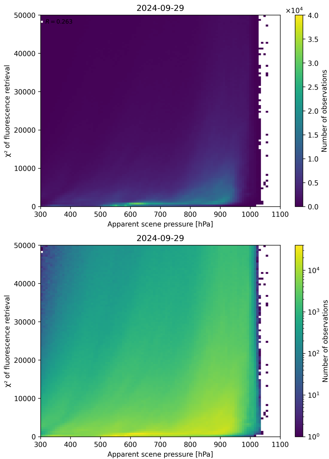
Figure 64: Scatter density plot of “Apparent scene pressure” against “ \chi^2 of fluorescence retrieval” for 2024-09-28 to 2024-09-30.
