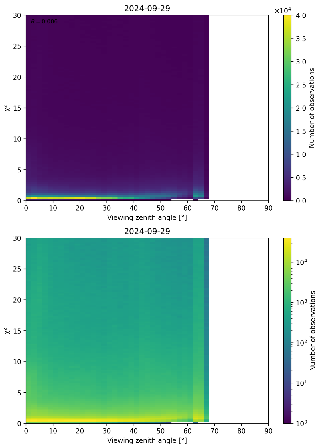
Figure 130: Scatter density plot of “Viewing zenith angle” against “ \chi^2 ” for 2024-09-28 to 2024-09-30.
