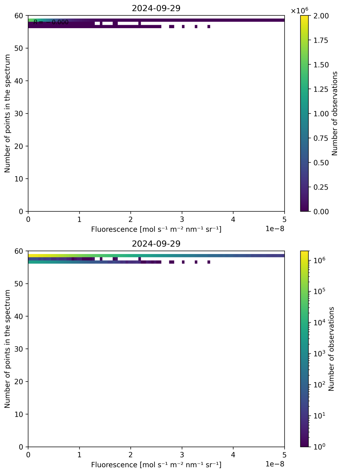
Figure 94: Scatter density plot of “Fluorescence” against “Number of points in the spectrum” for 2024-09-28 to 2024-09-30.
