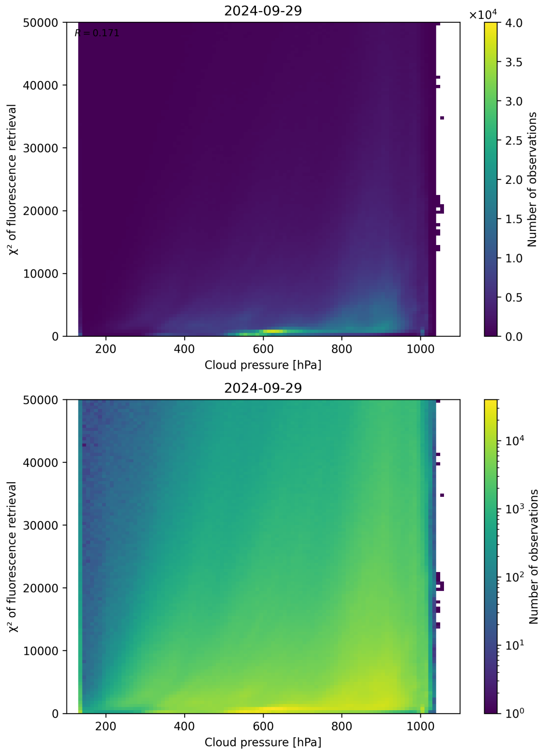
Figure 86: Scatter density plot of “Cloud pressure” against “ \chi^2 of fluorescence retrieval” for 2024-09-28 to 2024-09-30.
