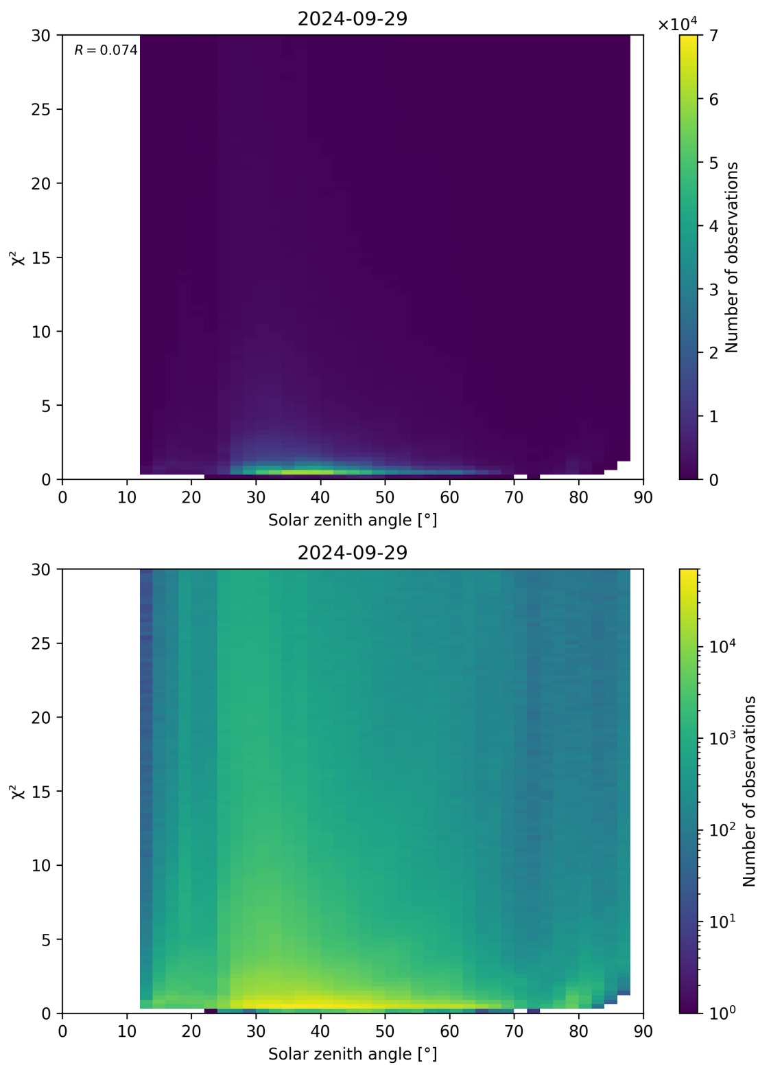
Figure 119: Scatter density plot of “Solar zenith angle” against “ \chi^2 ” for 2024-09-28 to 2024-09-30.
