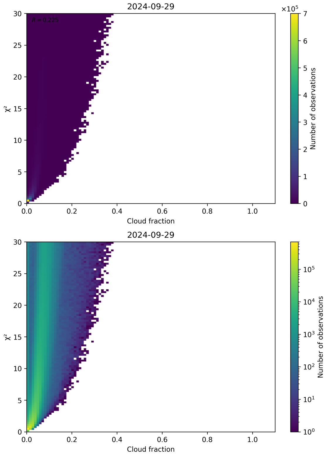
Figure 77: Scatter density plot of “Cloud fraction” against “ \chi^2 ” for 2024-09-28 to 2024-09-30.
