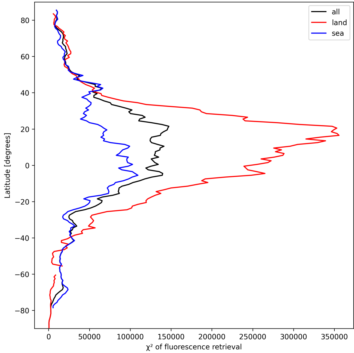
Figure 25: Zonal average of “ \chi^2 of fluorescence retrieval” for 2024-09-28 to 2024-09-30.
