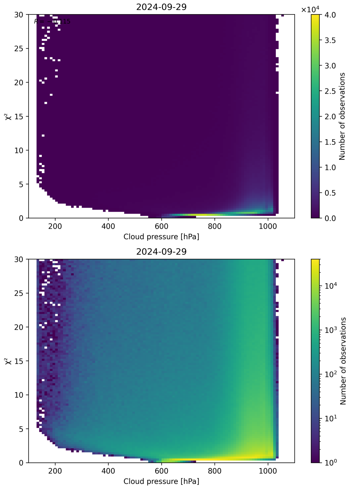
Figure 85: Scatter density plot of “Cloud pressure” against “ \chi^2 ” for 2024-09-28 to 2024-09-30.
