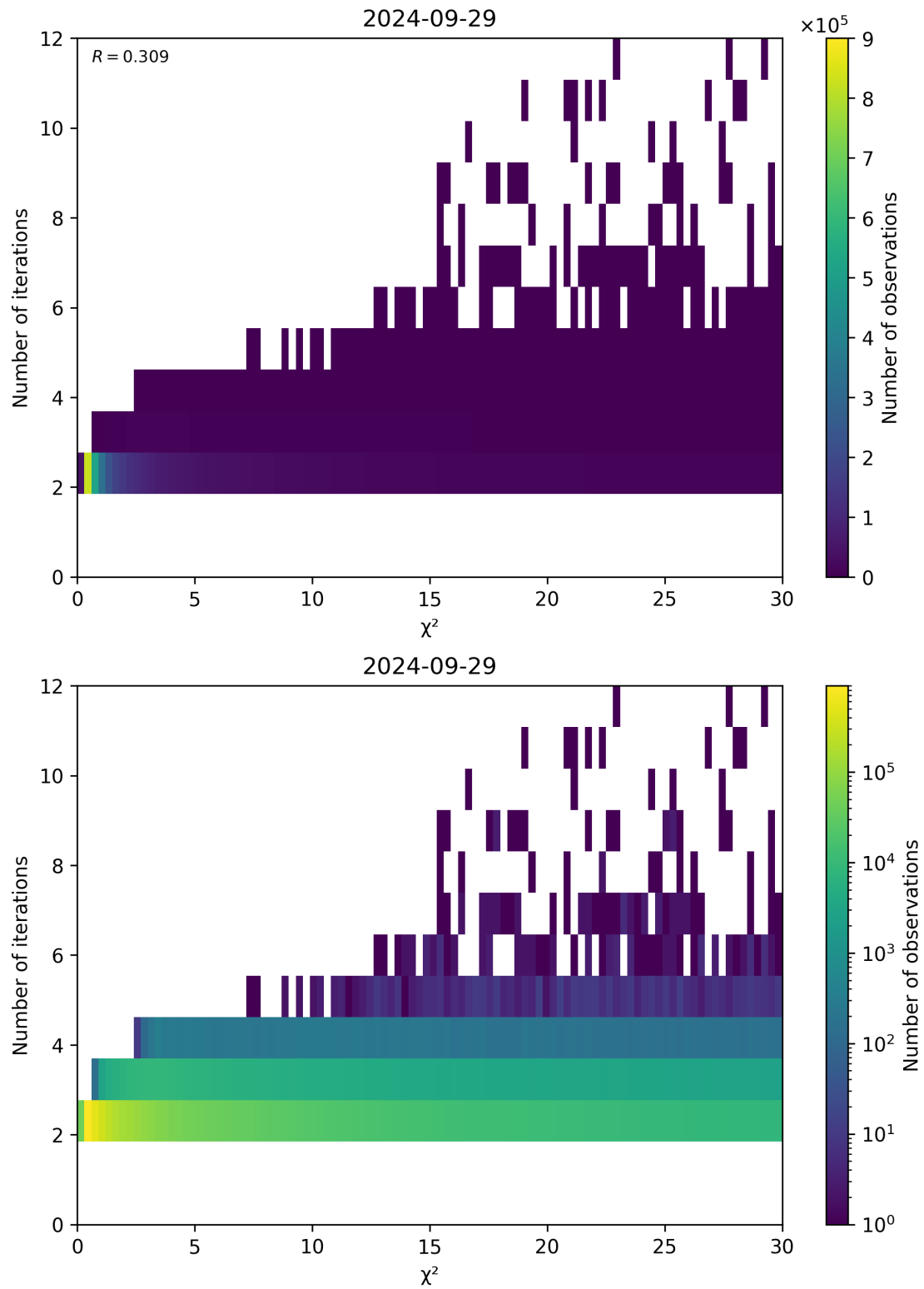
Figure 73: Scatter density plot of “ \chi^2 ” against “Number of iterations” for 2024-09-28 to 2024-09-30.
