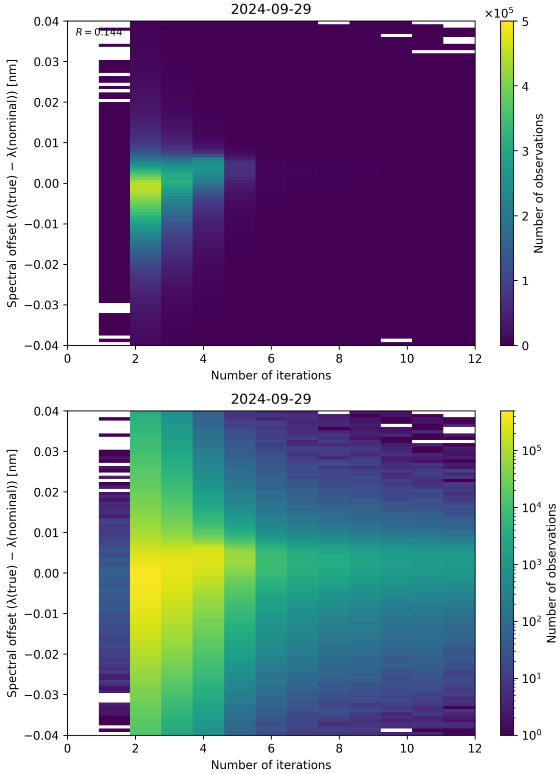
Figure 109: Scatter density plot of “Number of iterations” against “Spectral offset ( \lambda_{\text{true}} - \lambda_{\text{nominal}} )” for 2024-09-28 to 2024-09-30.
