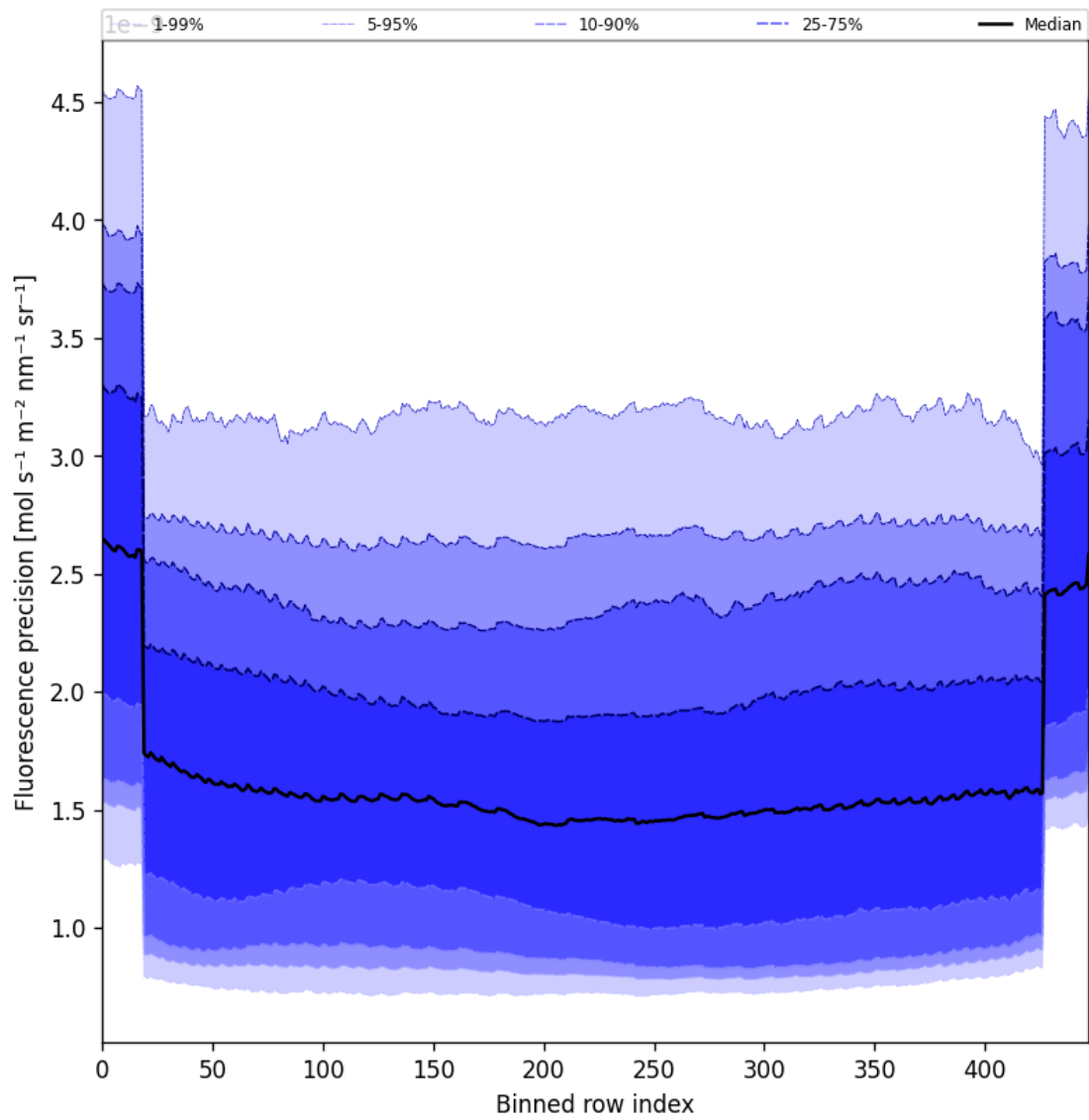
Figure 58: Along track statistics of “Fluorescence precision” for 2024-09-28 to 2024-09-30
