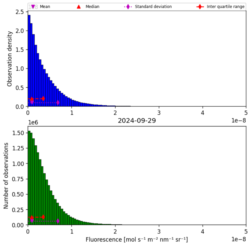
Figure 40: Histogram of “Fluorescence” for 2024-09-28 to 2024-09-30
