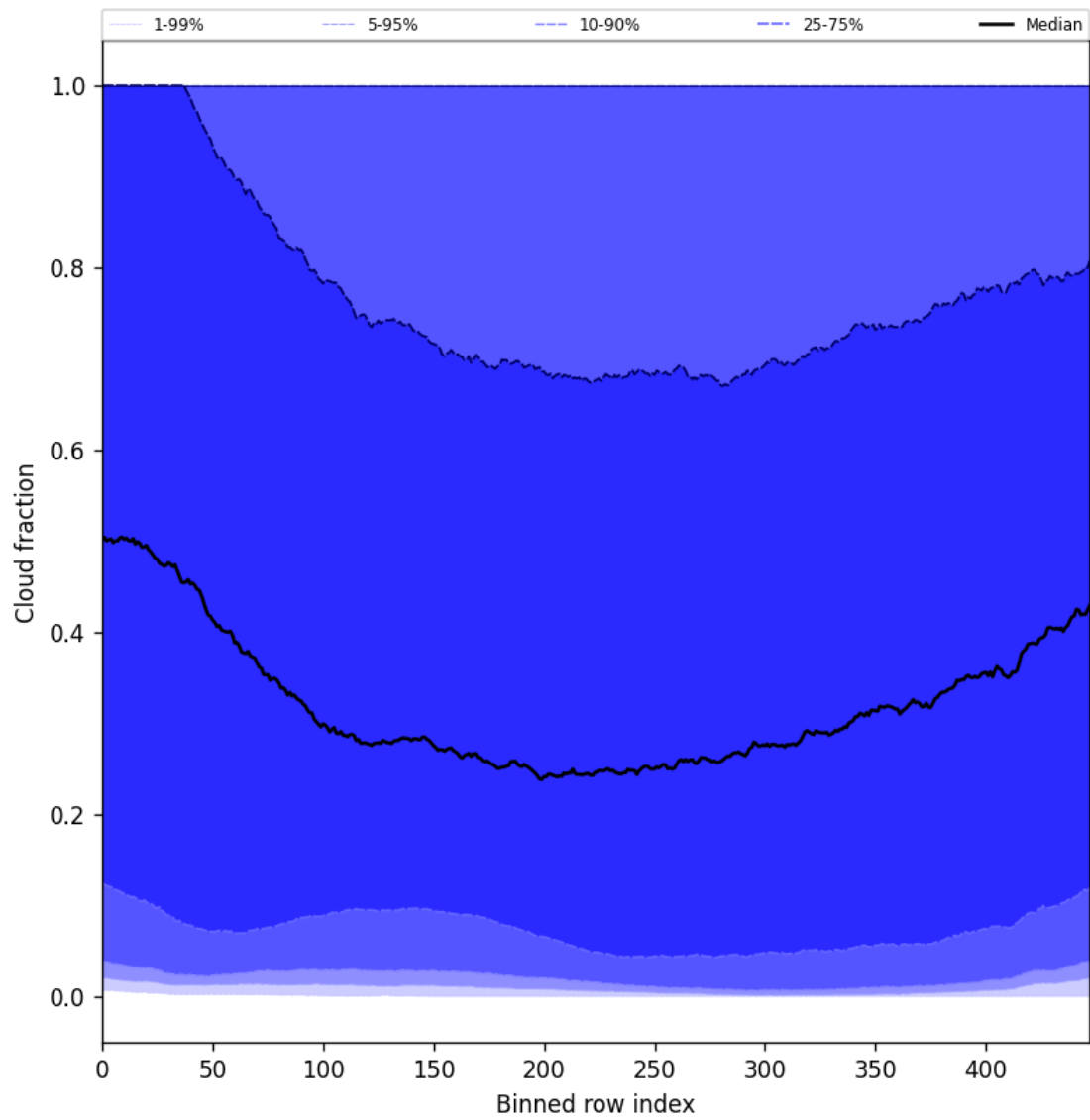
Figure 49: Along track statistics of “Cloud fraction” for 2024-09-28 to 2024-09-30
