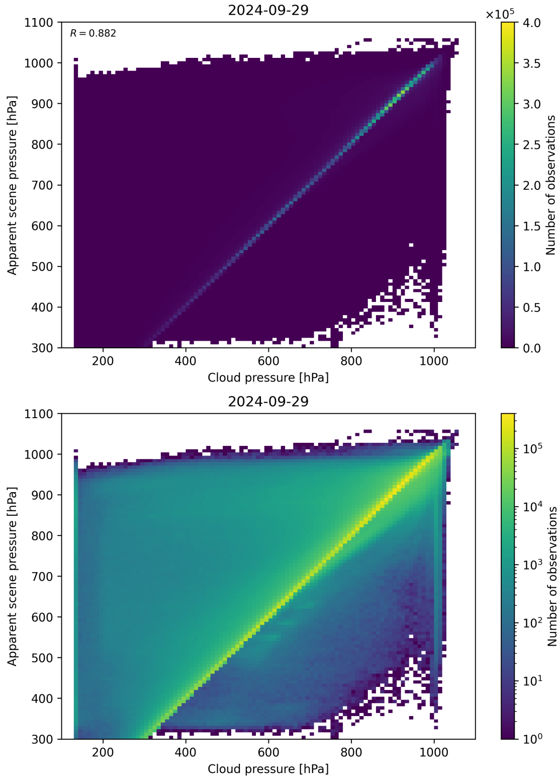
Figure 84: Scatter density plot of “Cloud pressure” against “Apparent scene pressure” for 2024-09-28 to 2024-09-30.
