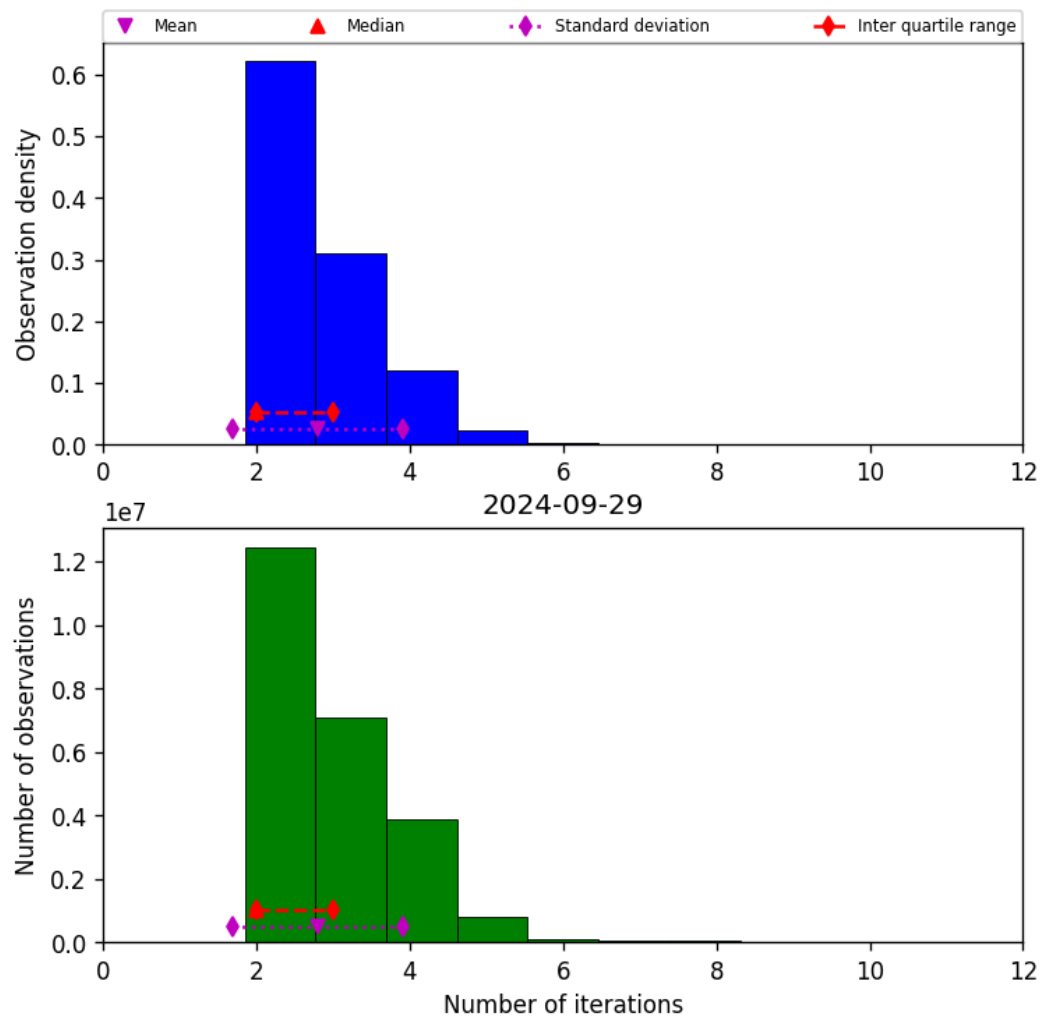
Figure 39: Histogram of “Number of iterations” for 2024-09-28 to 2024-09-30
