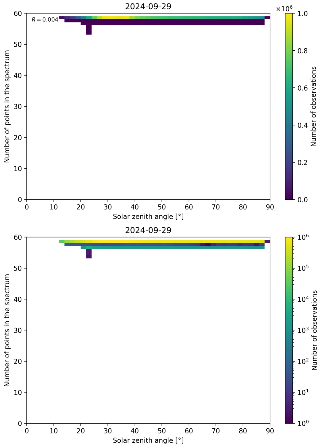
Figure 126: Scatter density plot of “Solar zenith angle” against “Number of points in the spectrum” for 2024-09-28 to 2024-09-30.
