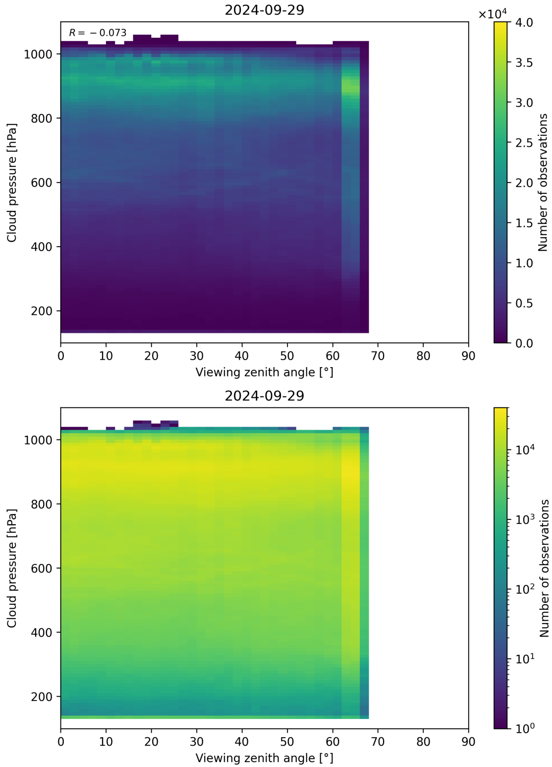
Figure 133: Scatter density plot of “Viewing zenith angle” against “Cloud pressure” for 2024-09-28 to 2024-09-30.
