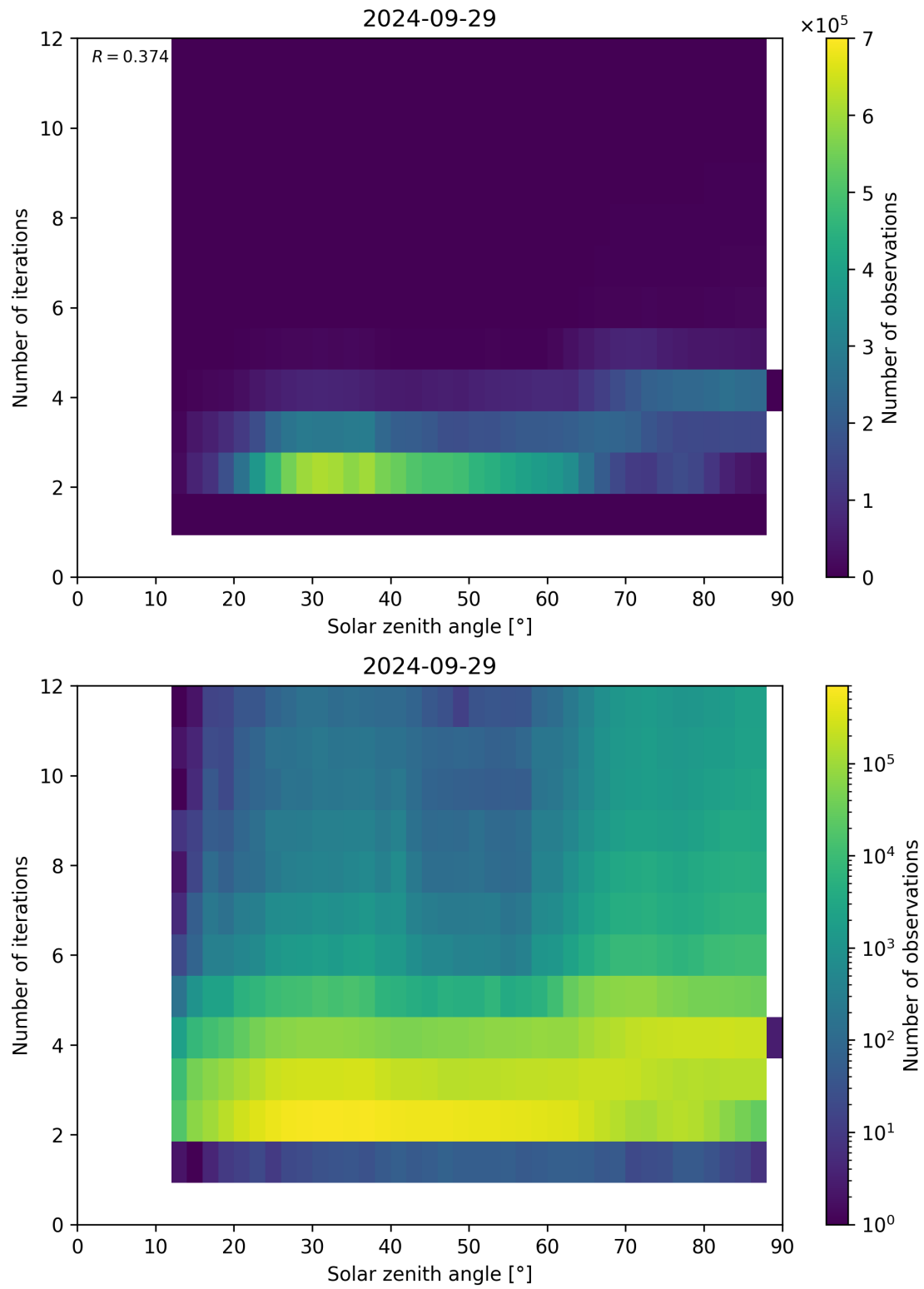
Figure 125: Scatter density plot of “Solar zenith angle” against “Number of iterations” for 2024-09-28 to 2024-09-30.
