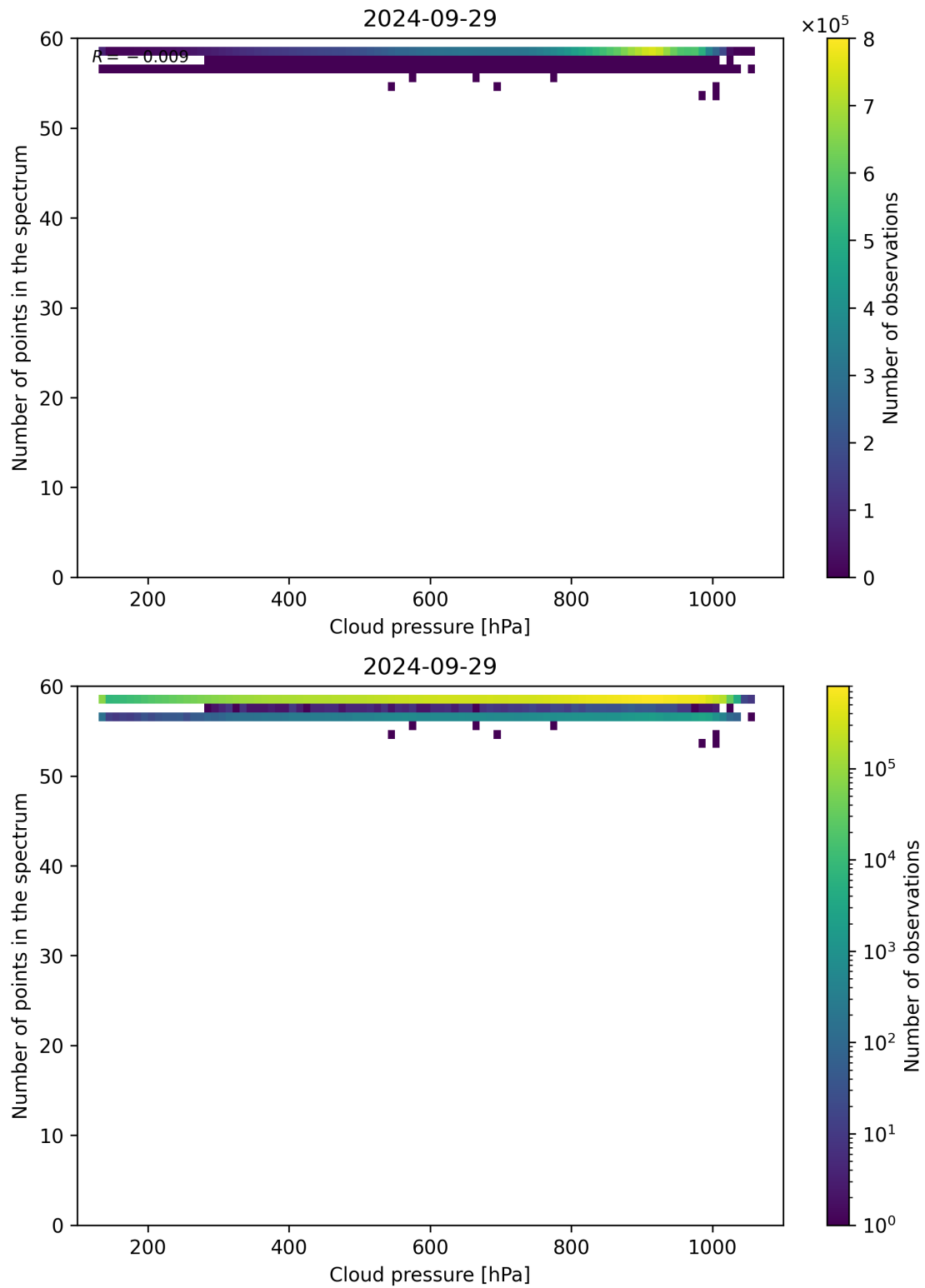
Figure 90: Scatter density plot of “Cloud pressure” against “Number of points in the spectrum” for 2024-09-28 to 2024-09-30.
