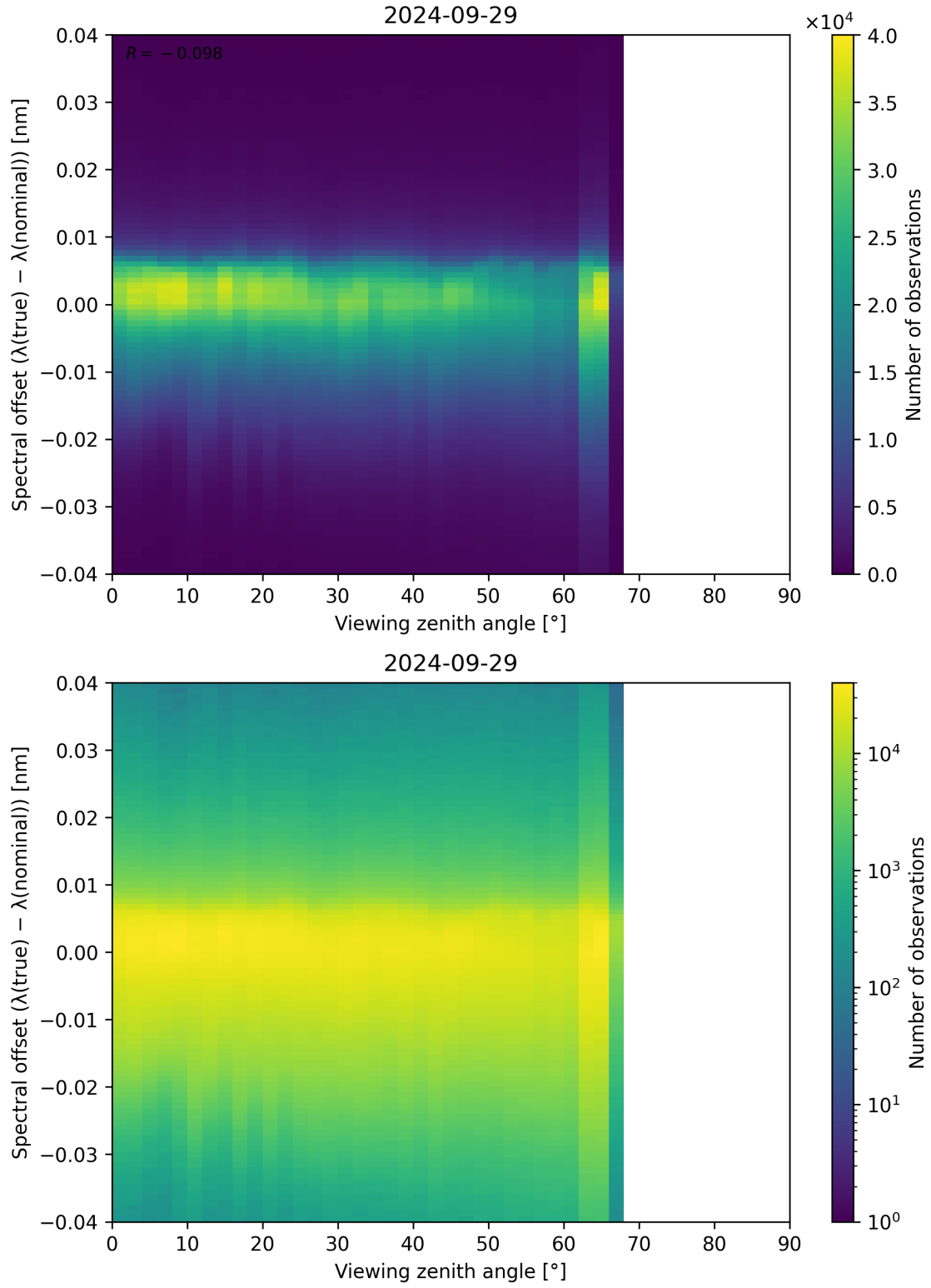
Figure 140: Scatter density plot of “Viewing zenith angle” against “Spectral offset ( \lambda_{\text{true}} - \lambda_{\text{nominal}} )” for 2024-09-28 to 2024-09-30.
