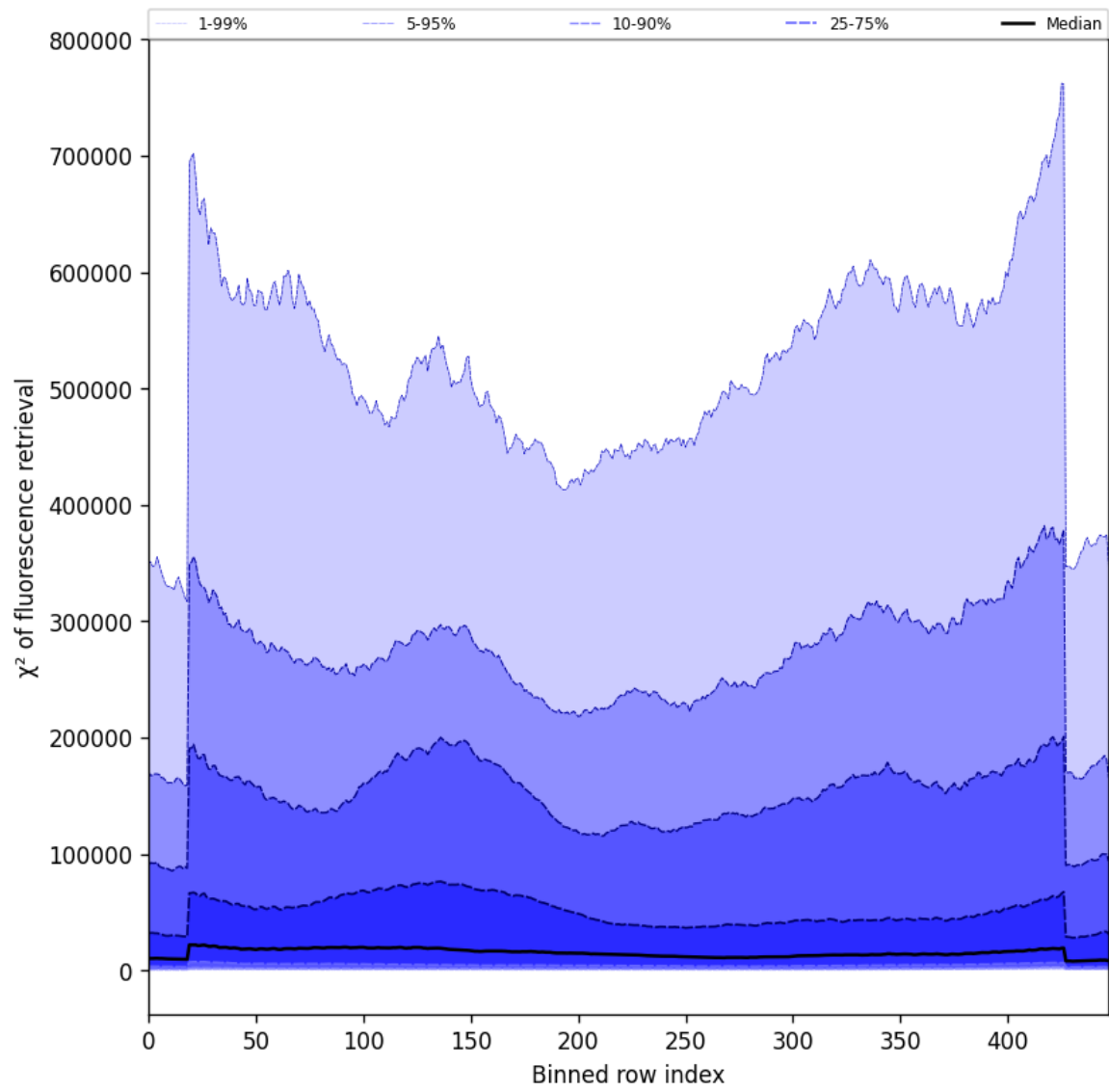
Figure 59: Along track statistics of “ \chi^2 of fluorescence retrieval” for 2024-09-28 to 2024-09-30
