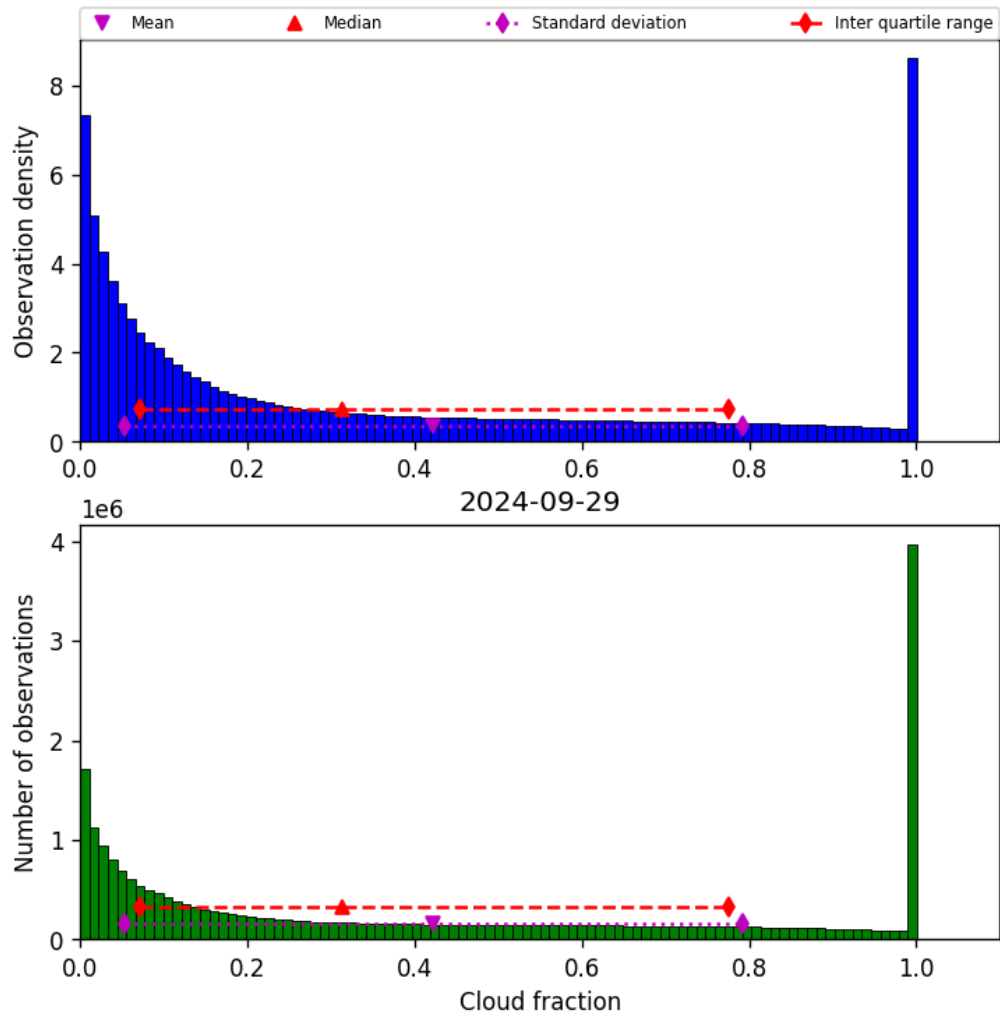
Figure 32: Histogram of “Cloud fraction” for 2024-09-28 to 2024-09-30
