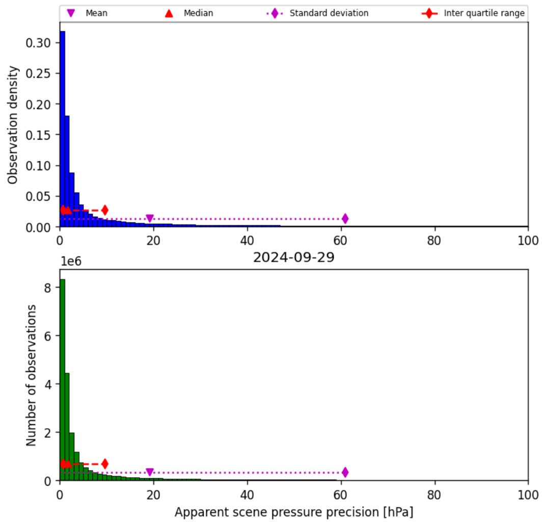
Figure 37: Histogram of “Apparent scene pressure precision” for 2024-09-28 to 2024-09-30
