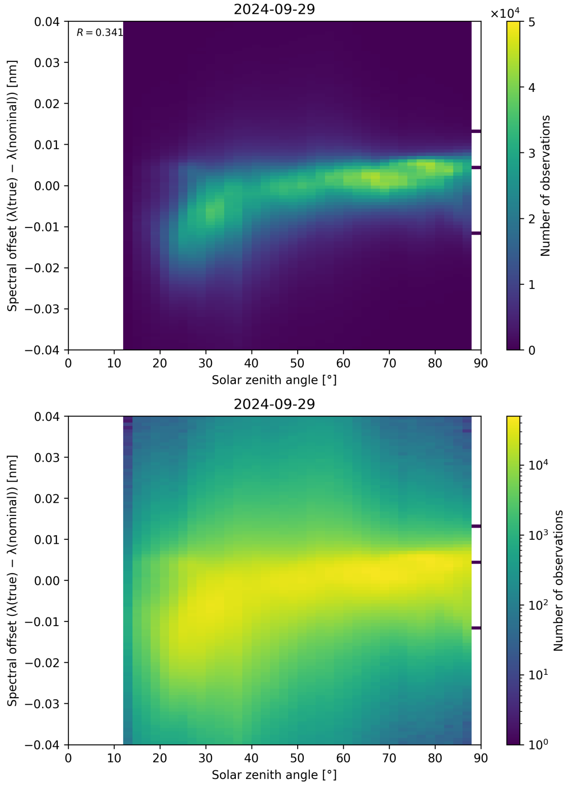
Figure 128: Scatter density plot of “Solar zenith angle” against “Spectral offset ( \lambda_{\text{true}} - \lambda_{\text{nominal}} )” for 2024-09-28 to 2024-09-30.
