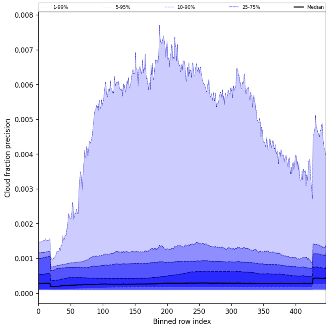
Figure 50: Along track statistics of “Cloud fraction precision” for 2024-09-28 to 2024-09-30
