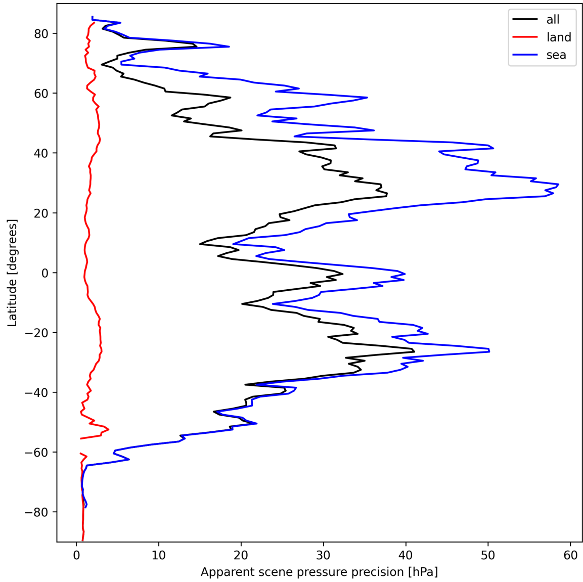
Figure 20: Zonal average of “Apparent scene pressure precision” for 2024-09-28 to 2024-09-30.
