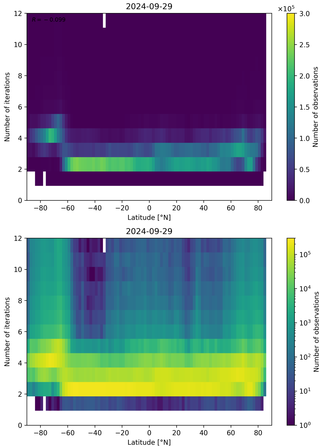
Figure 102: Scatter density plot of “Latitude” against “Number of iterations” for 2024-09-28 to 2024-09-30.
