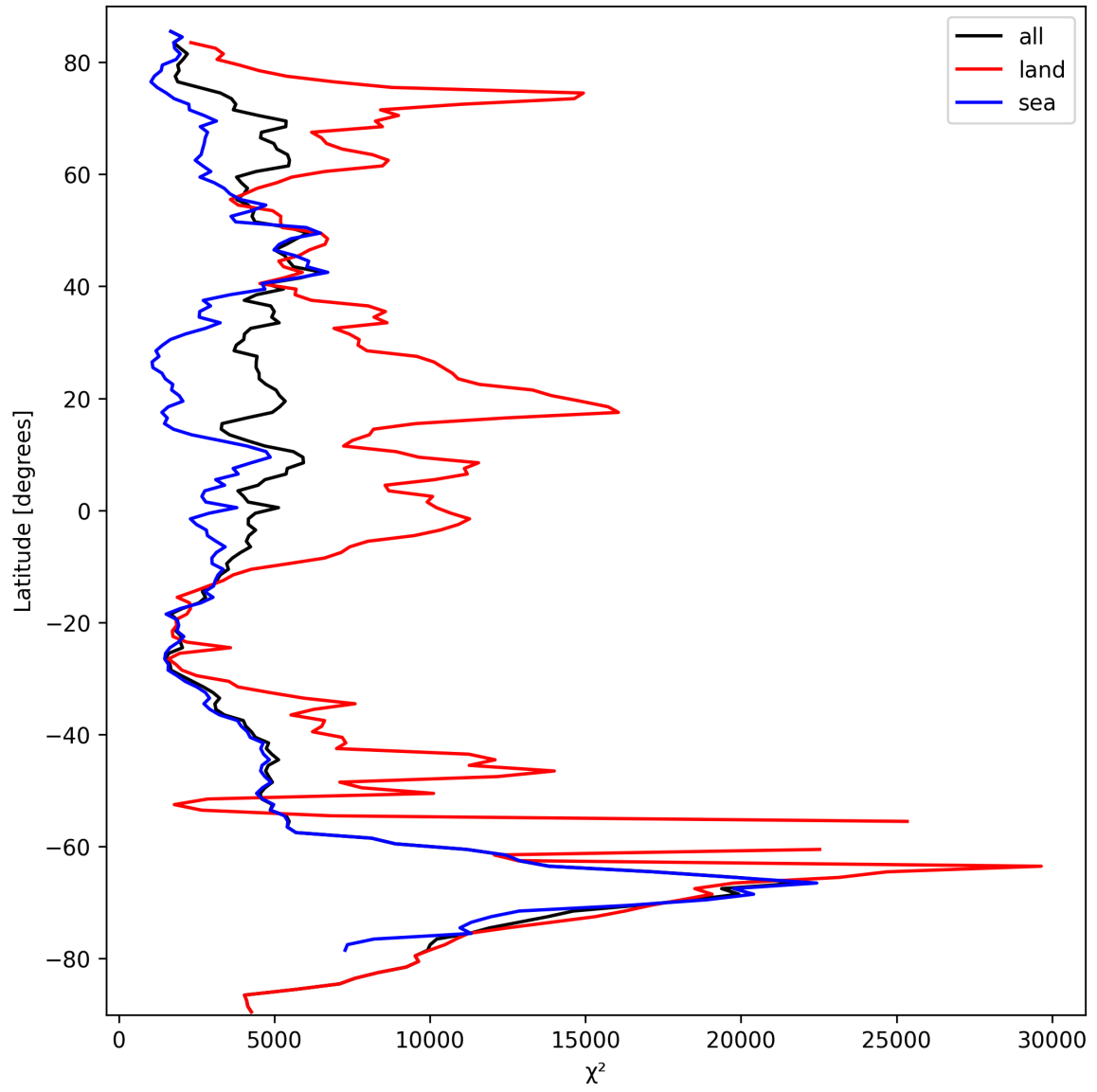
Figure 21: Zonal average of “ \chi^2 ” for 2024-09-28 to 2024-09-30.
