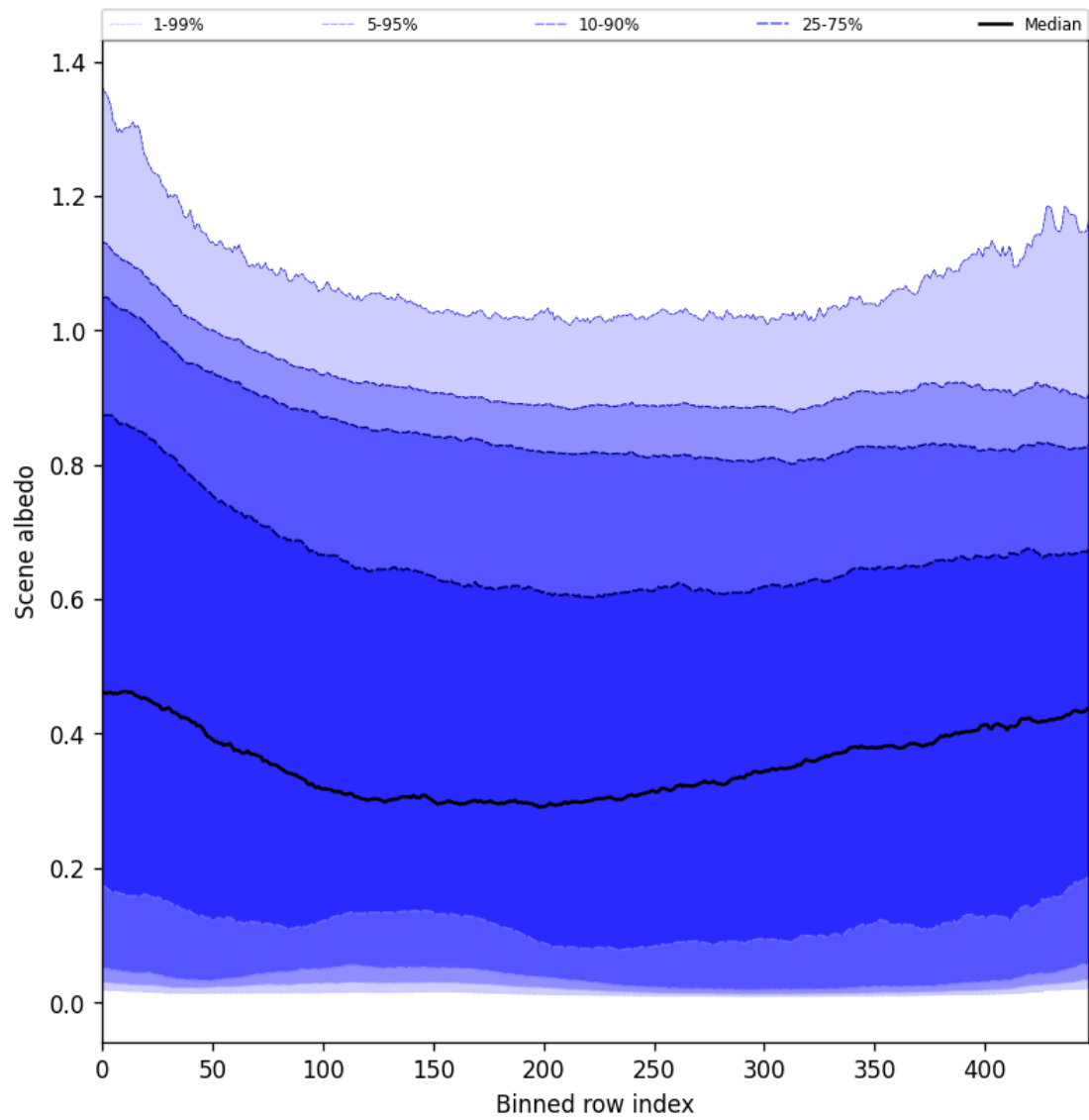
Figure 51: Along track statistics of “Scene albedo” for 2024-09-28 to 2024-09-30
