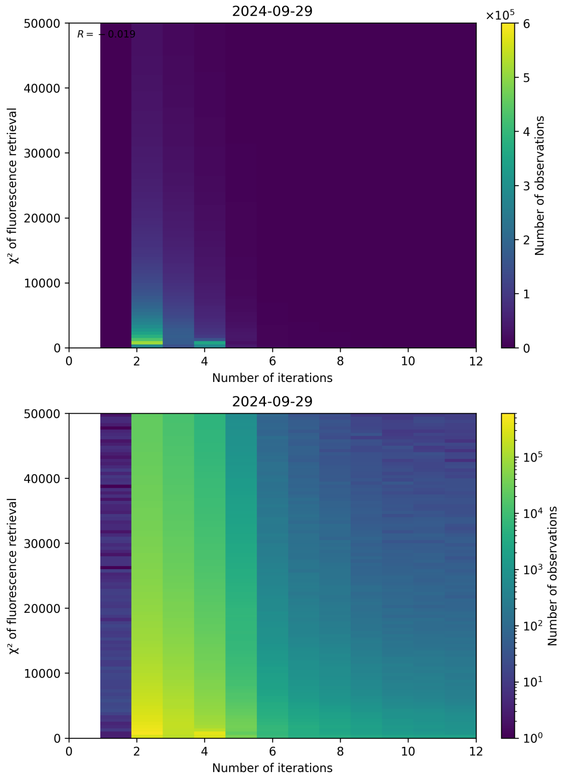
Figure 106: Scatter density plot of “Number of iterations” against “ \chi^2 of fluorescence retrieval” for 2024-09-28 to 2024-09-30.
