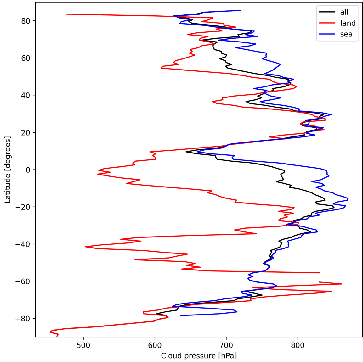
Figure 13: Zonal average of “Cloud pressure” for 2024-09-28 to 2024-09-30.
