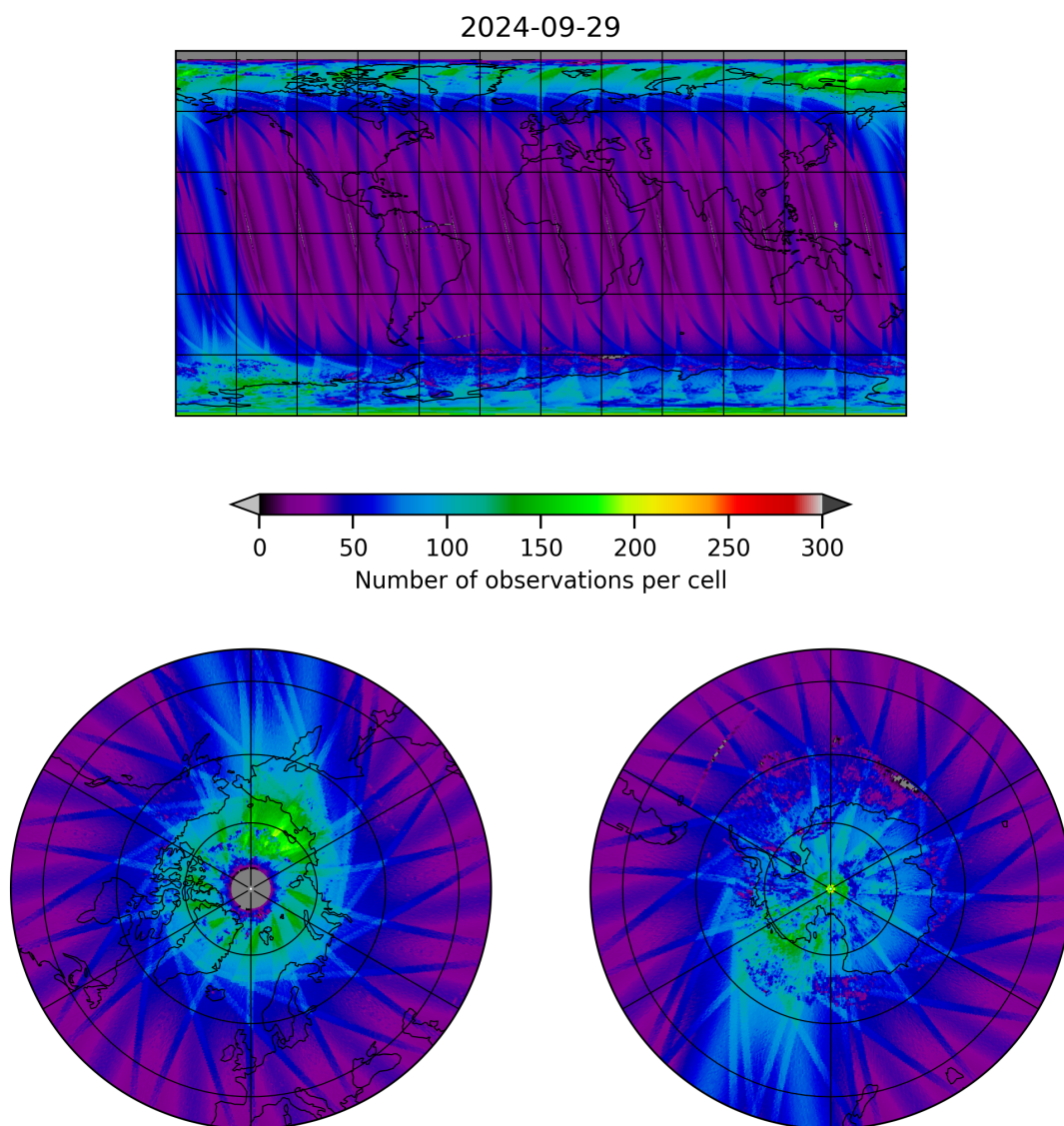
Figure 11: Map of the number of observations for 2024-09-28 to 2024-09-30
