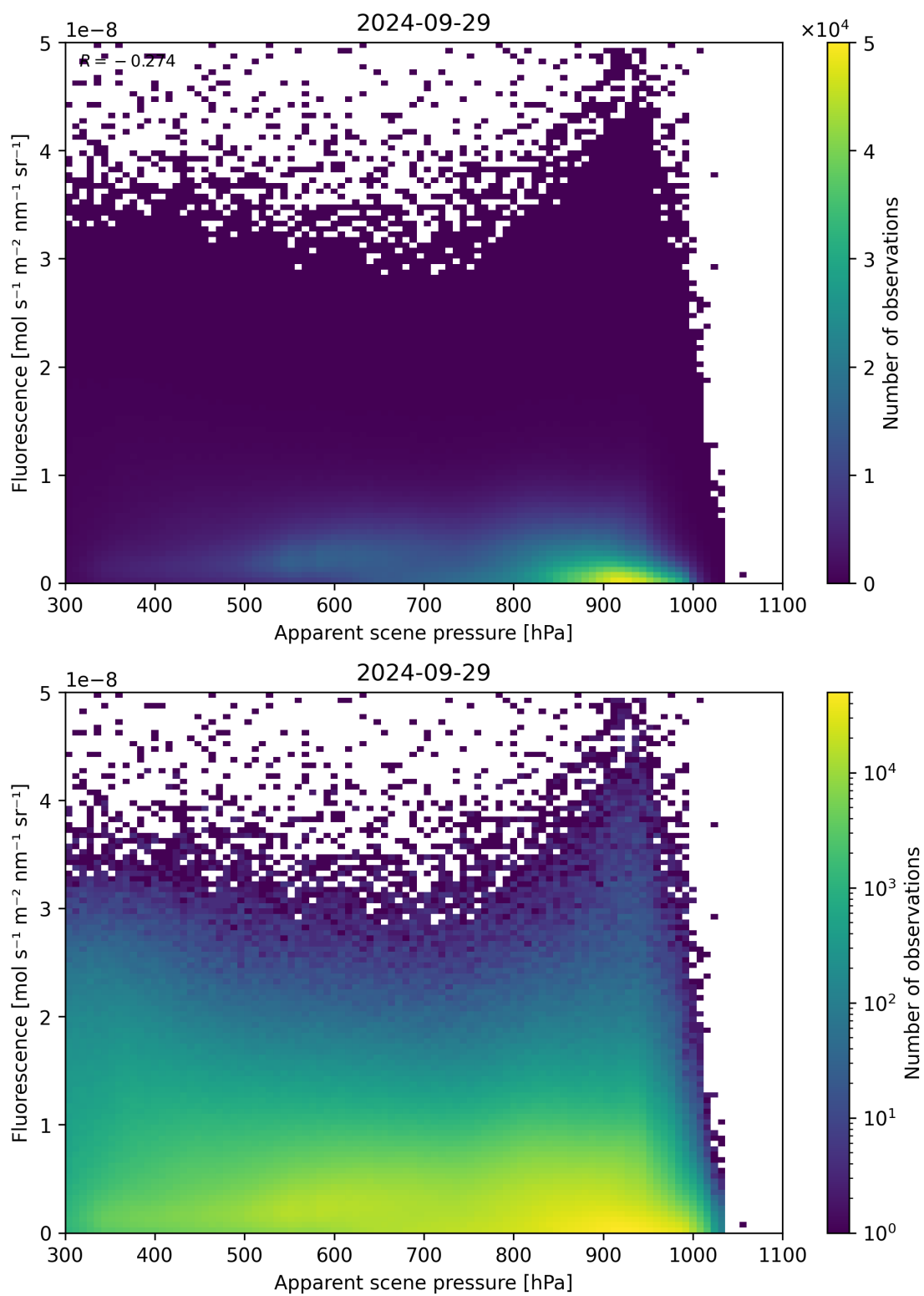
Figure 65: Scatter density plot of “Apparent scene pressure” against “Fluorescence” for 2024-09-28 to 2024-09-30.
