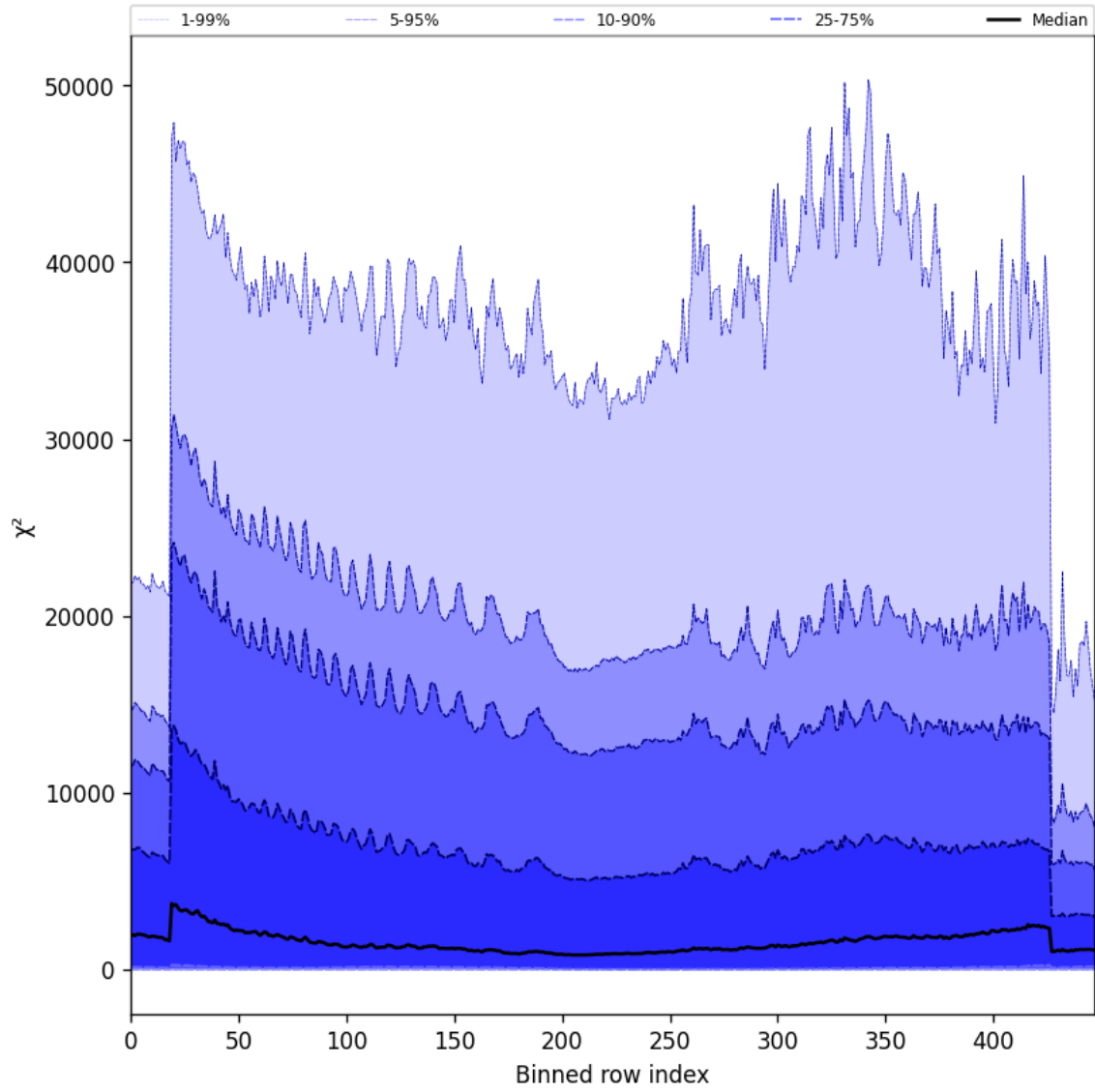
Figure 55: Along track statistics of “ \chi^2 ” for 2024-09-28 to 2024-09-30
