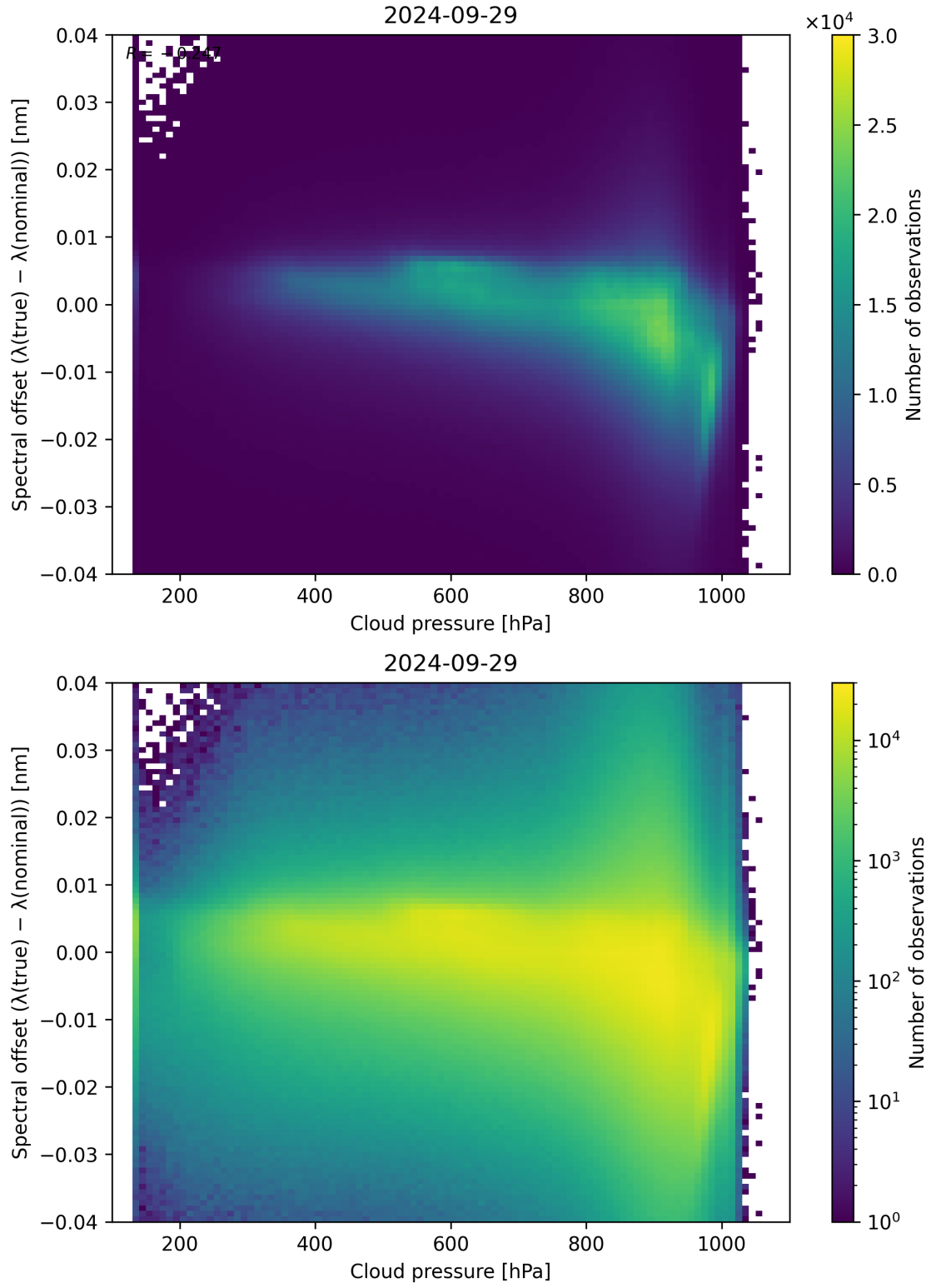
Figure 92: Scatter density plot of “Cloud pressure” against “Spectral offset ( \lambda_{\text{true}} - \lambda_{\text{nominal}} )” for 2024-09-28 to 2024-09-30.
