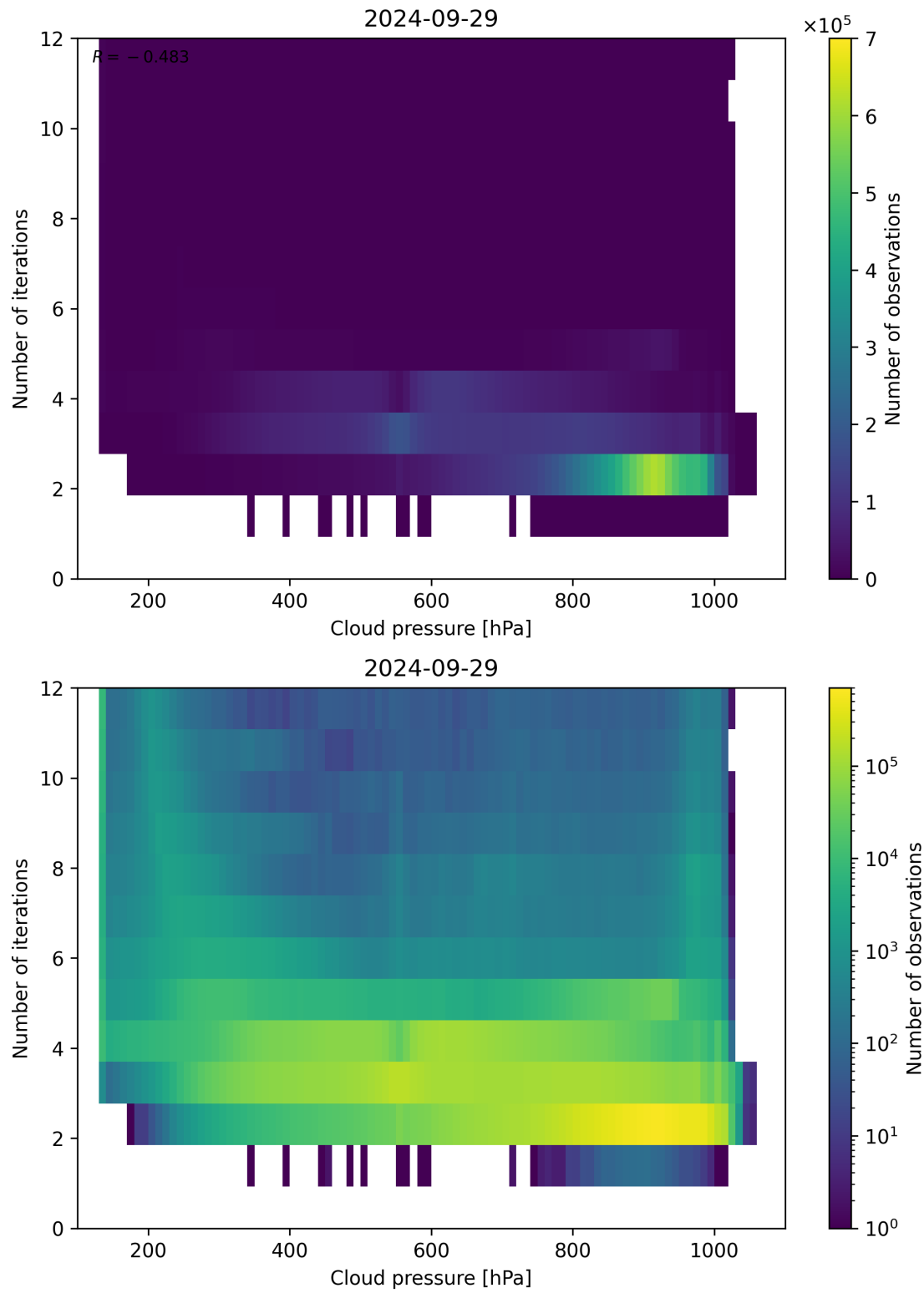
Figure 89: Scatter density plot of “Cloud pressure” against “Number of iterations” for 2024-09-28 to 2024-09-30.
