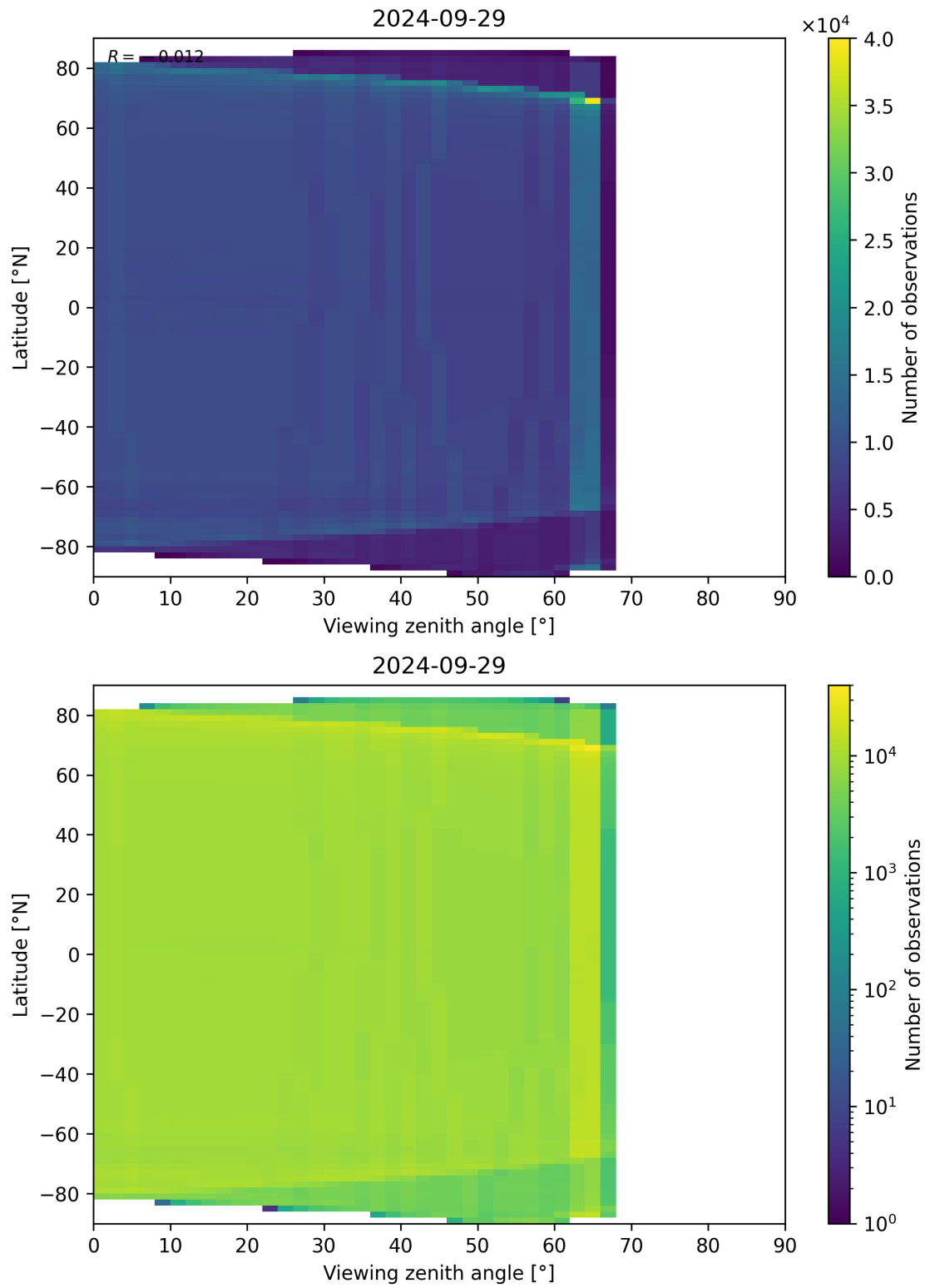
Figure 135: Scatter density plot of “Viewing zenith angle” against “Latitude” for 2024-09-28 to 2024-09-30.
