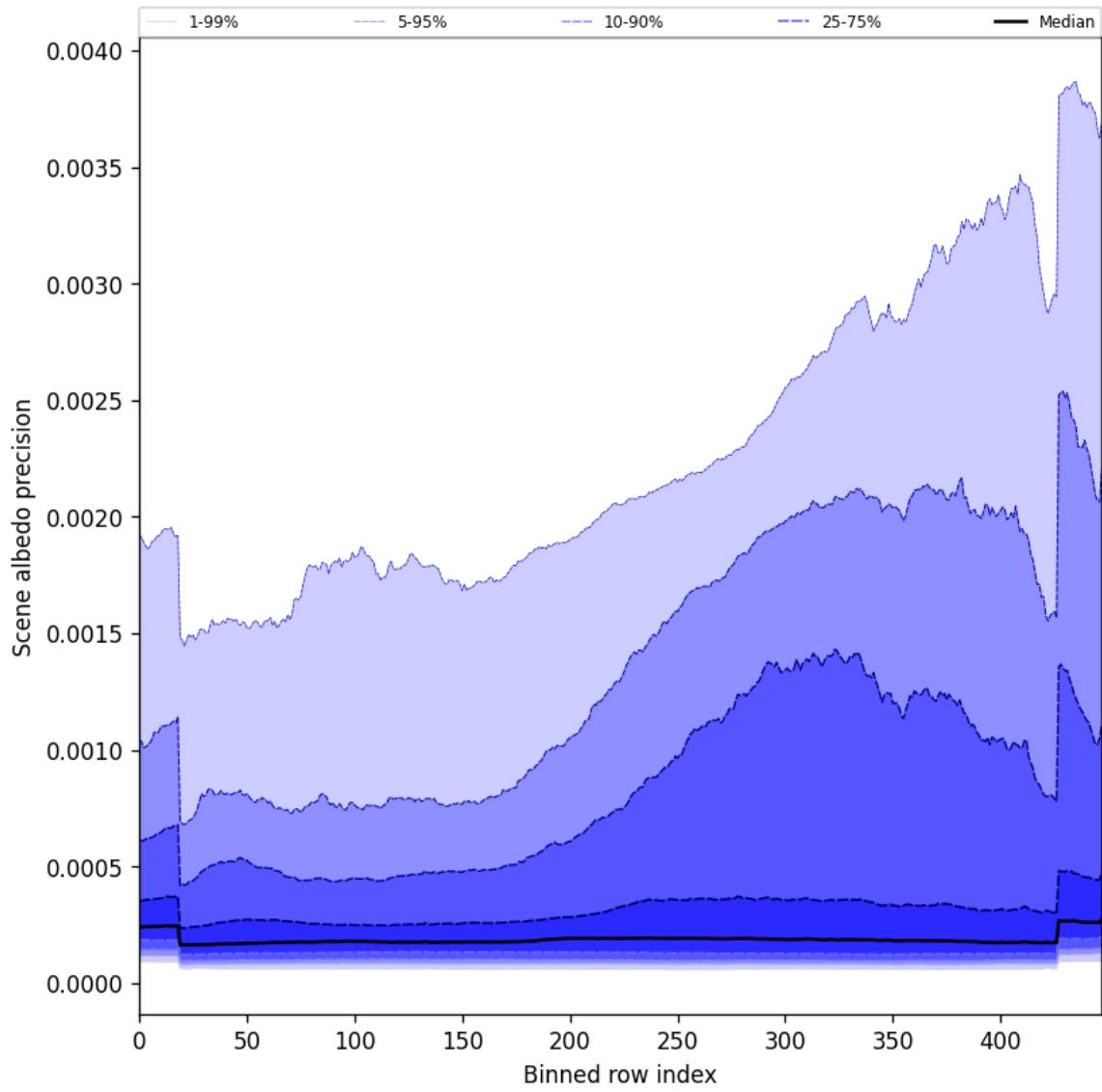
Figure 52: Along track statistics of “Scene albedo precision” for 2024-09-28 to 2024-09-30
