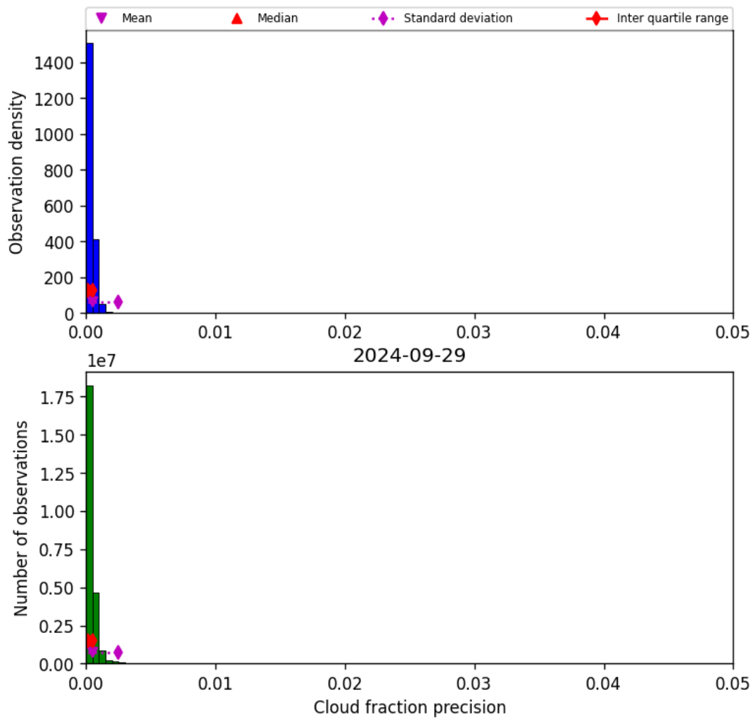
Figure 33: Histogram of “Cloud fraction precision” for 2024-09-28 to 2024-09-30
