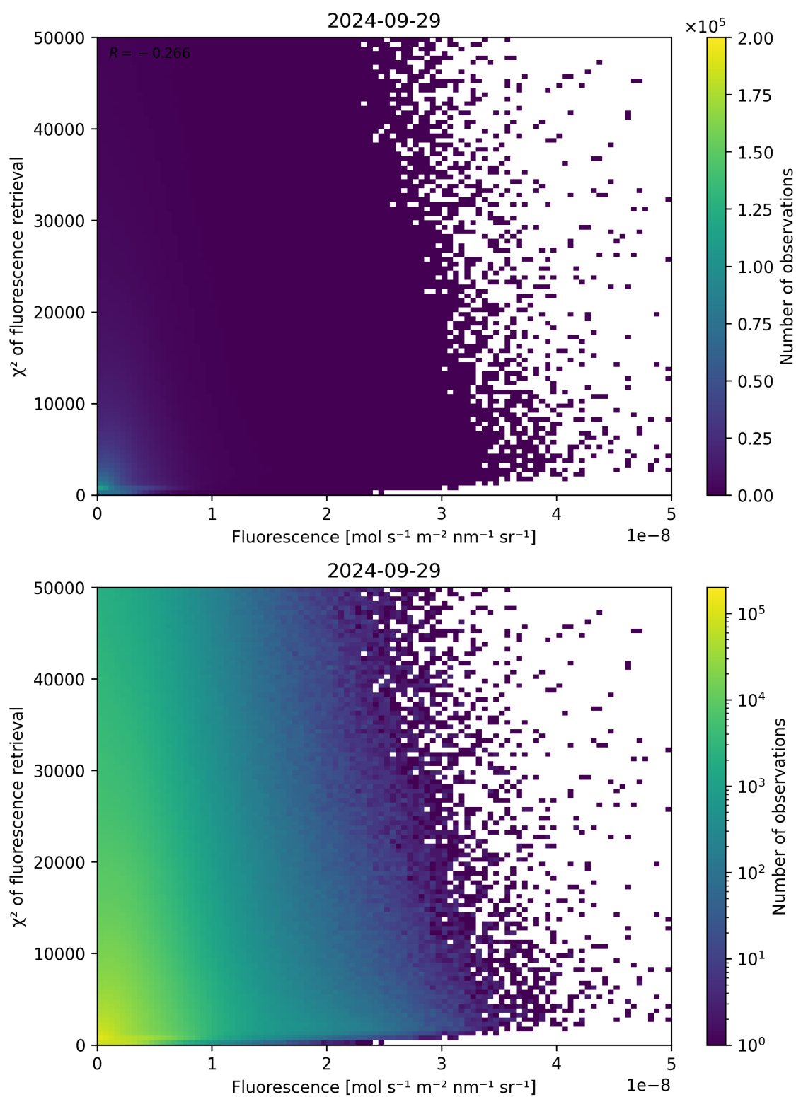
Figure 93: Scatter density plot of “Fluorescence” against “ \chi^2 of fluorescence retrieval” for 2024-09-28 to 2024-09-30.
