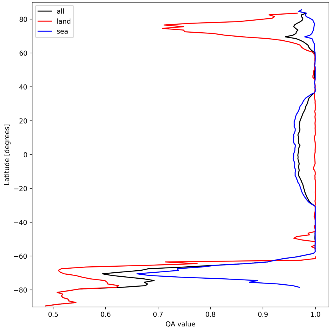
Figure 12: Zonal average of “QA value” for 2024-09-28 to 2024-09-30.
