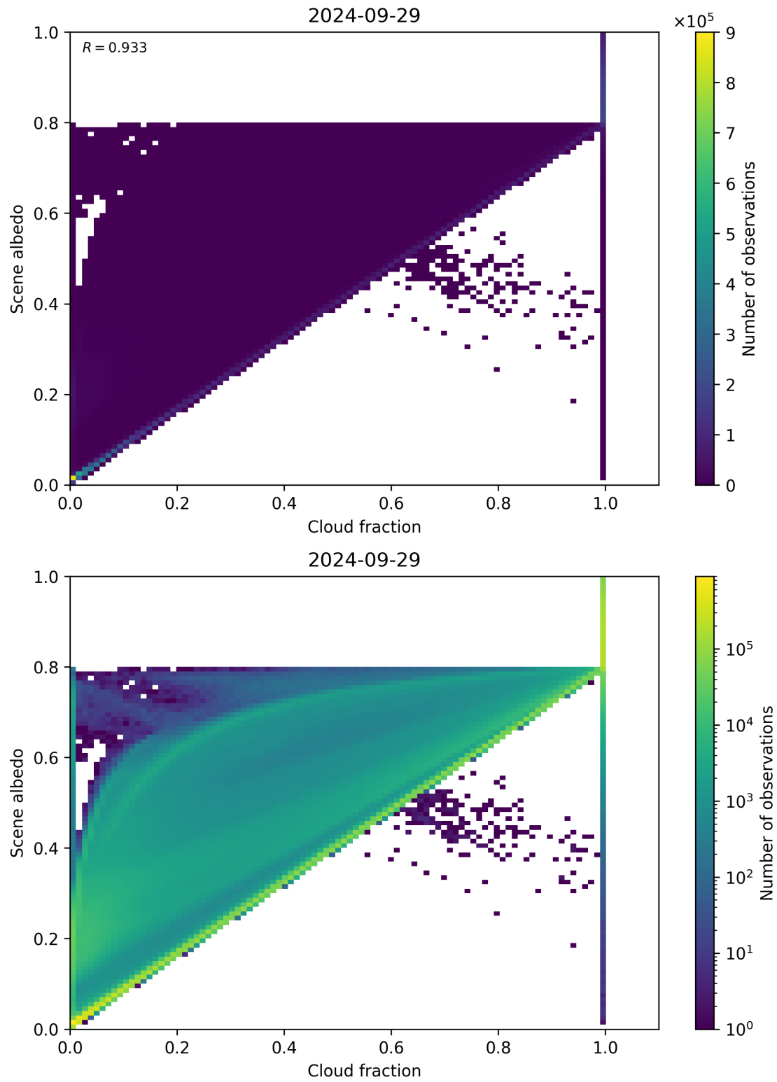
Figure 82: Scatter density plot of “Cloud fraction” against “Scene albedo” for 2024-09-28 to 2024-09-30.
