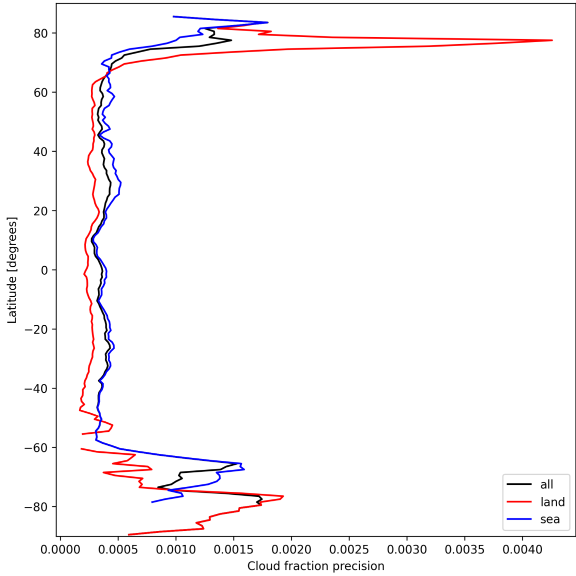
Figure 16: Zonal average of “Cloud fraction precision” for 2024-09-28 to 2024-09-30.
