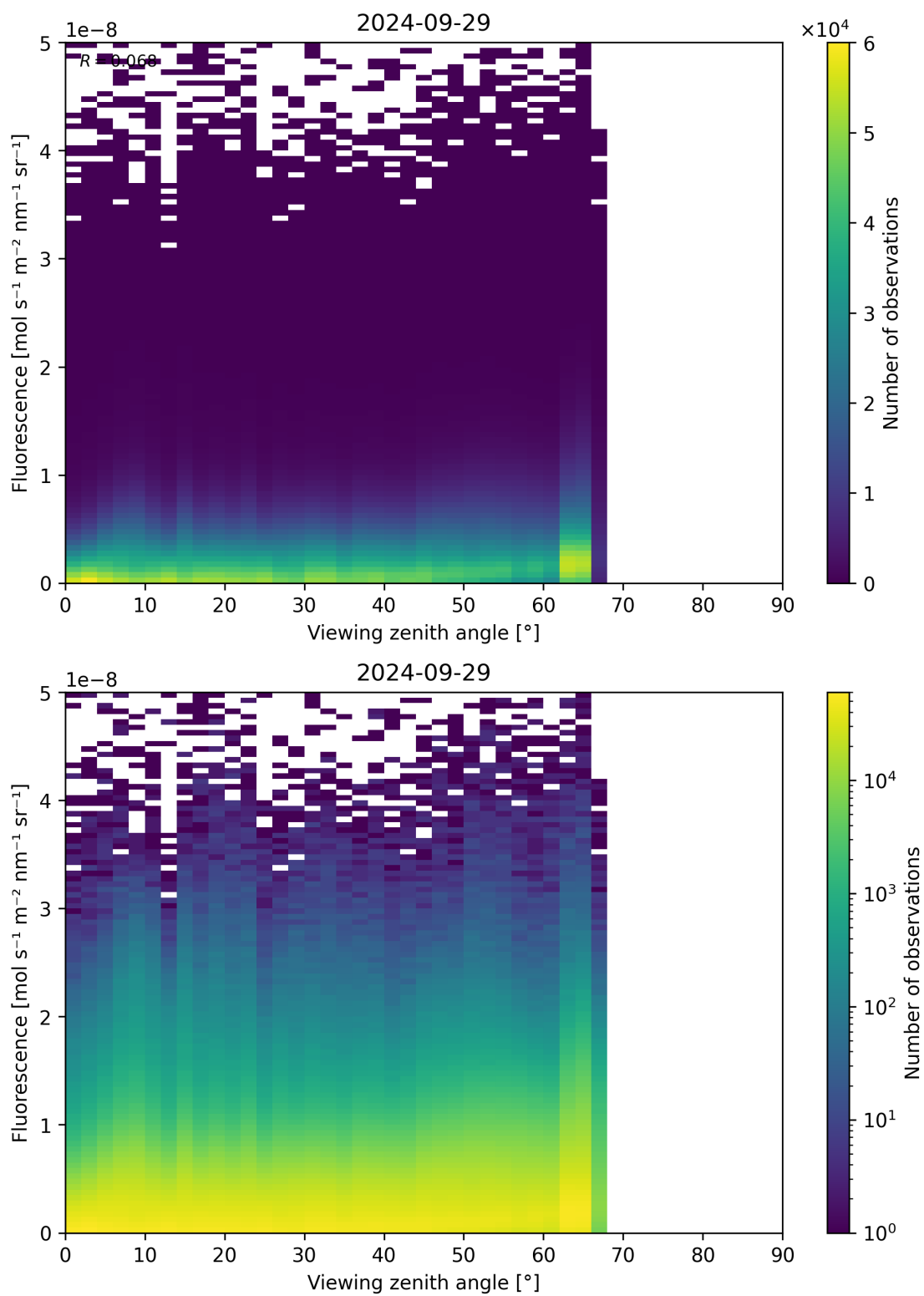
Figure 134: Scatter density plot of “Viewing zenith angle” against “Fluorescence” for 2024-09-28 to 2024-09-30.
