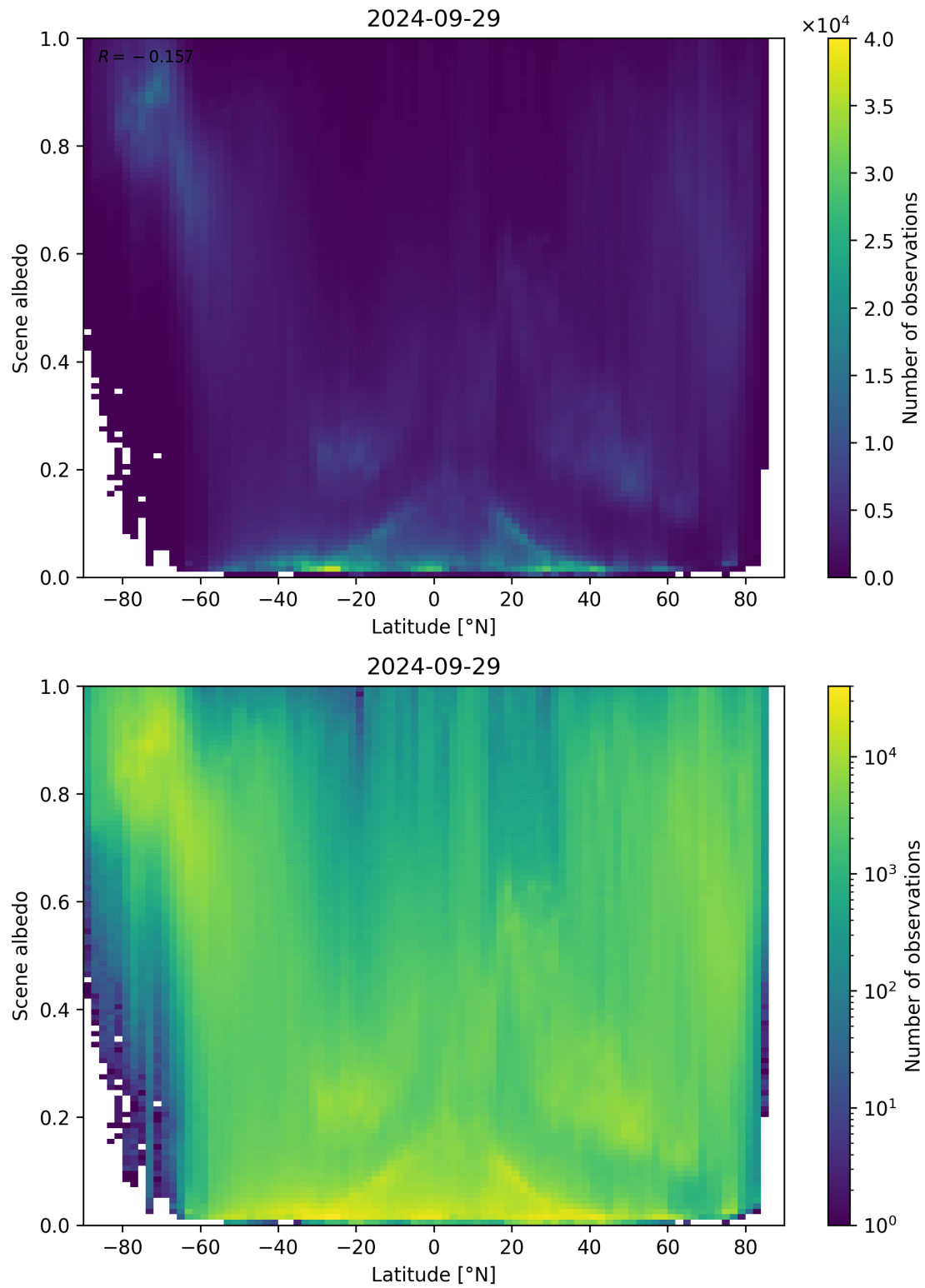
Figure 104: Scatter density plot of “Latitude” against “Scene albedo” for 2024-09-28 to 2024-09-30.
