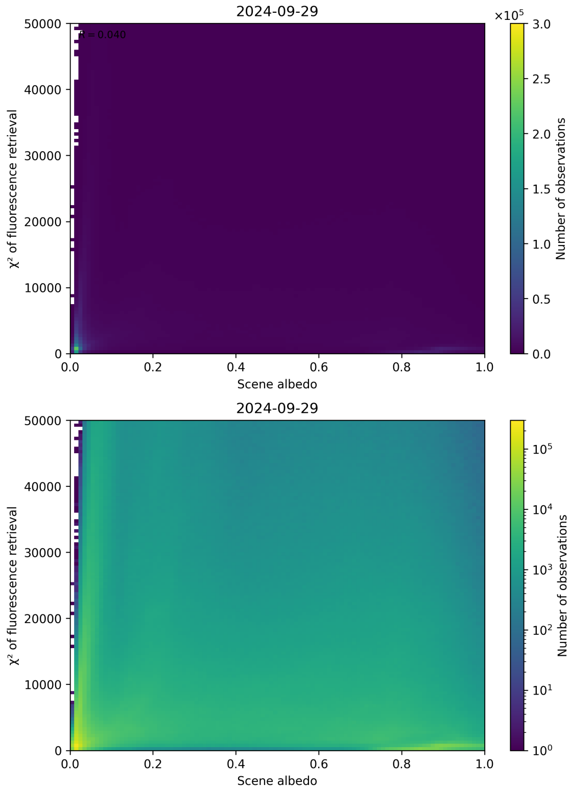
Figure 113: Scatter density plot of “Scene albedo” against “ \chi^2 of fluorescence retrieval” for 2024-09-28 to 2024-09-30.
