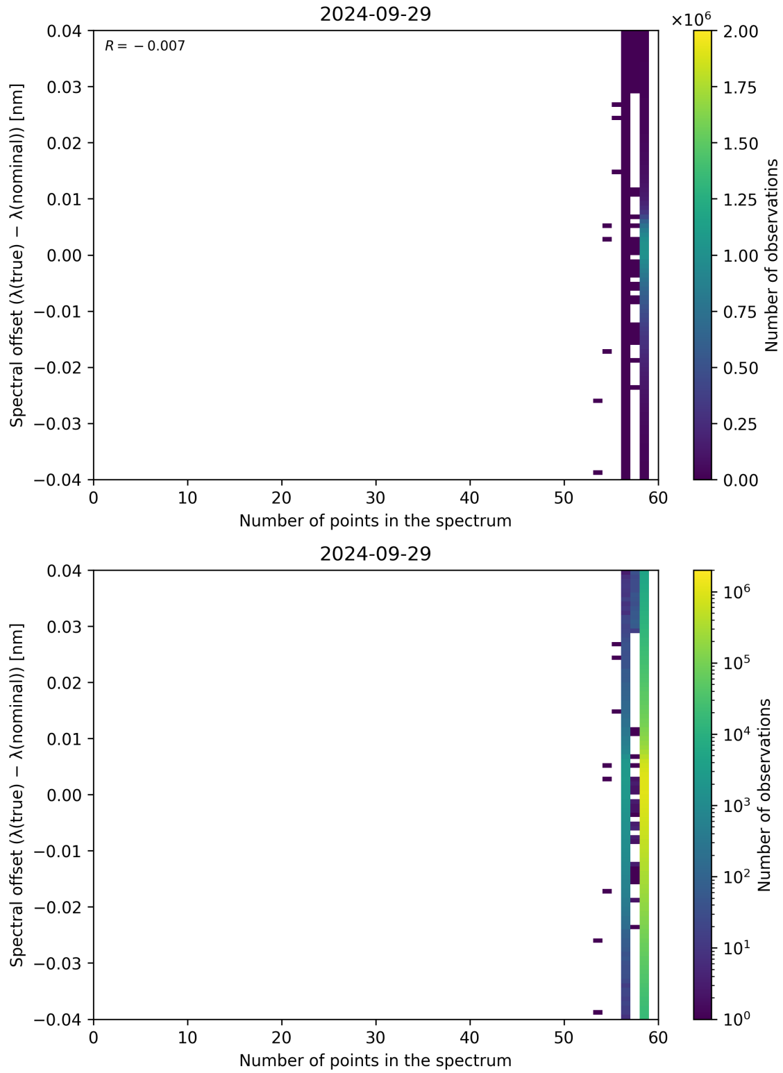
Figure 110: Scatter density plot of “Number of points in the spectrum” against “Spectral offset ( \lambda_{\text{true}} - \lambda_{\text{nominal}} )” for 2024-09-28 to 2024-09-30.
