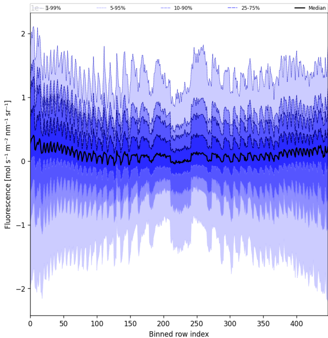
Figure 57: Along track statistics of “Fluorescence” for 2024-09-28 to 2024-09-30
