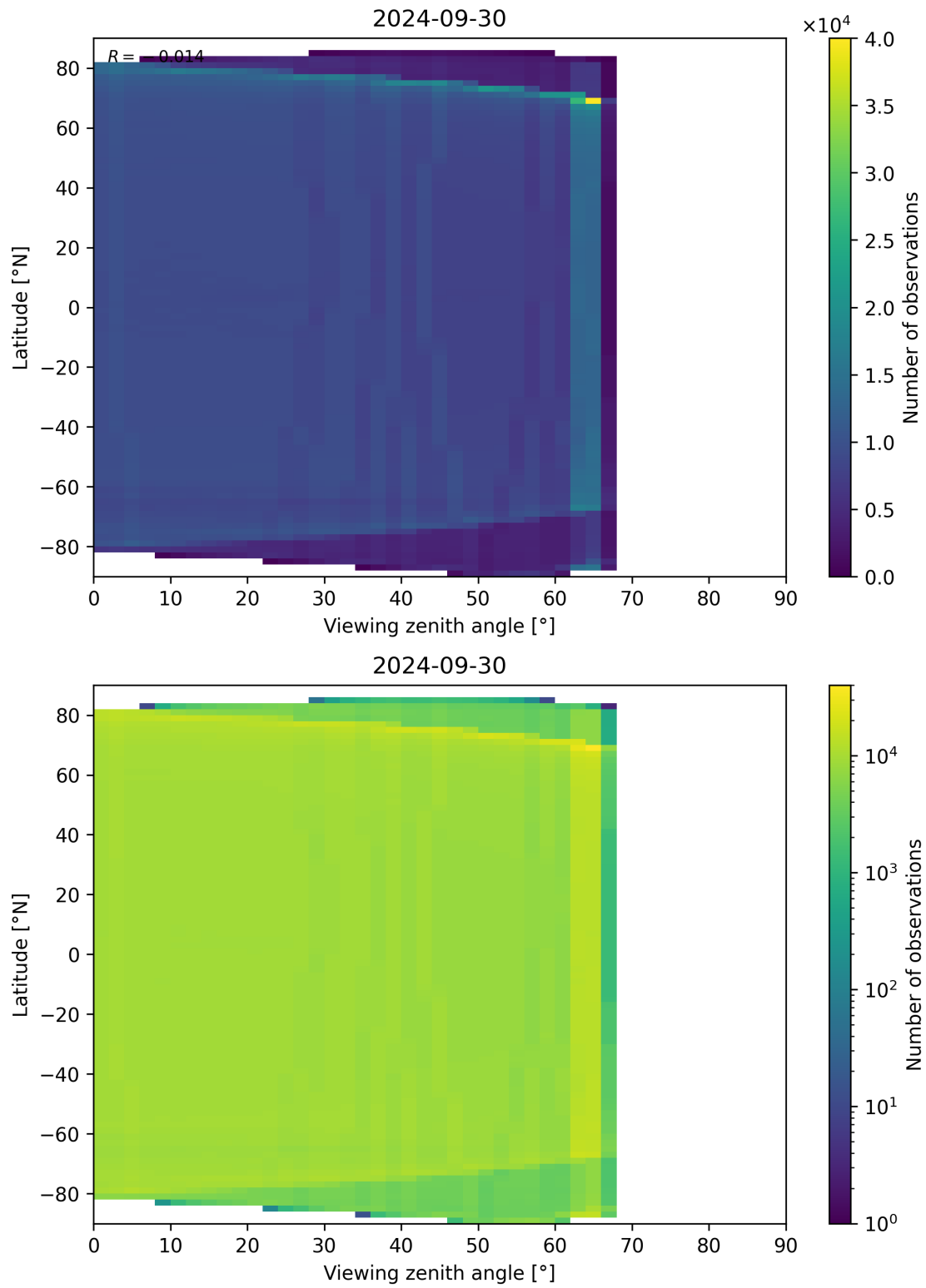
Figure 135: Scatter density plot of “Viewing zenith angle” against “Latitude” for 2024-09-29 to 2024-10-01.
