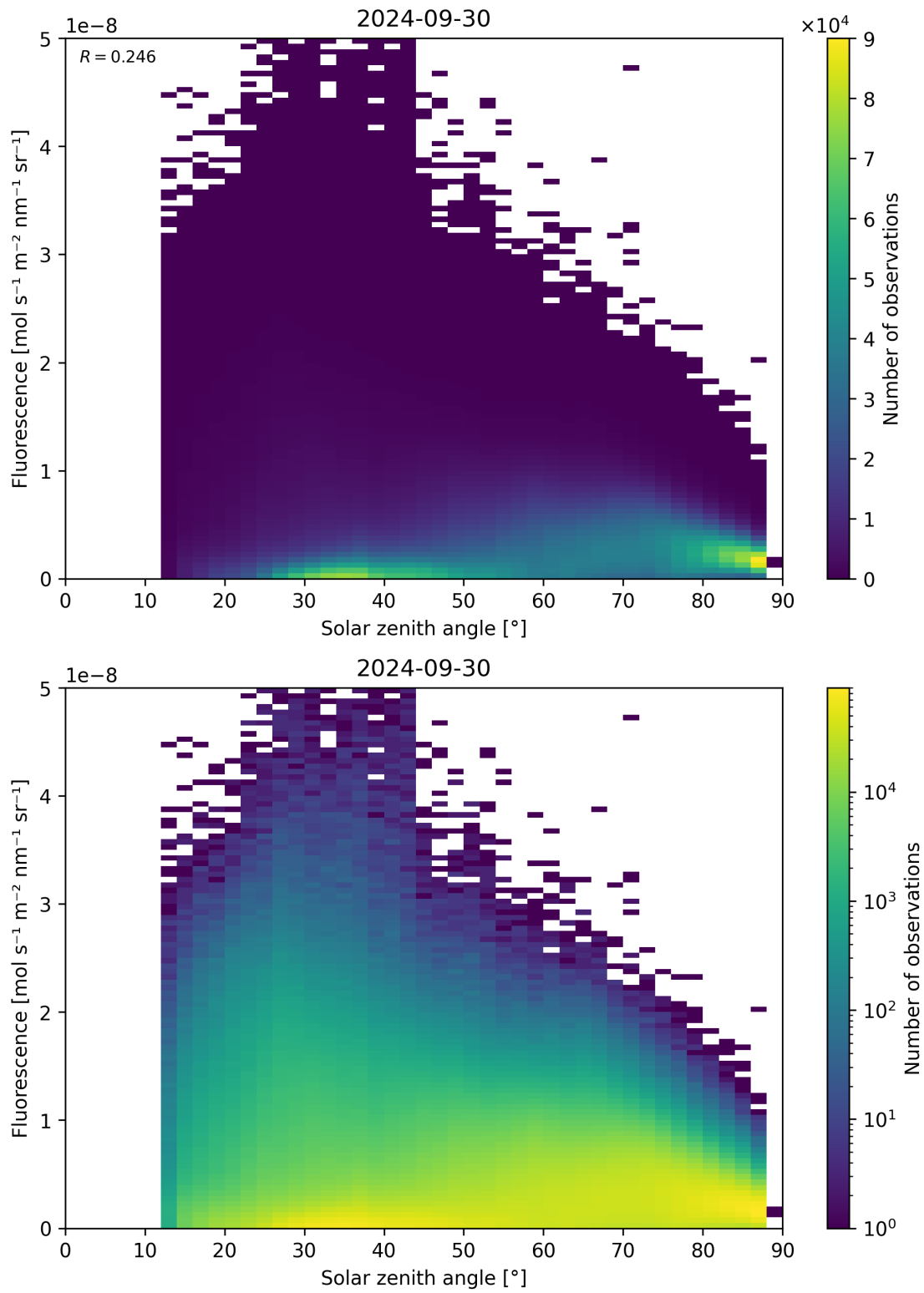
Figure 123: Scatter density plot of “Solar zenith angle” against “Fluorescence” for 2024-09-29 to 2024-10-01.
