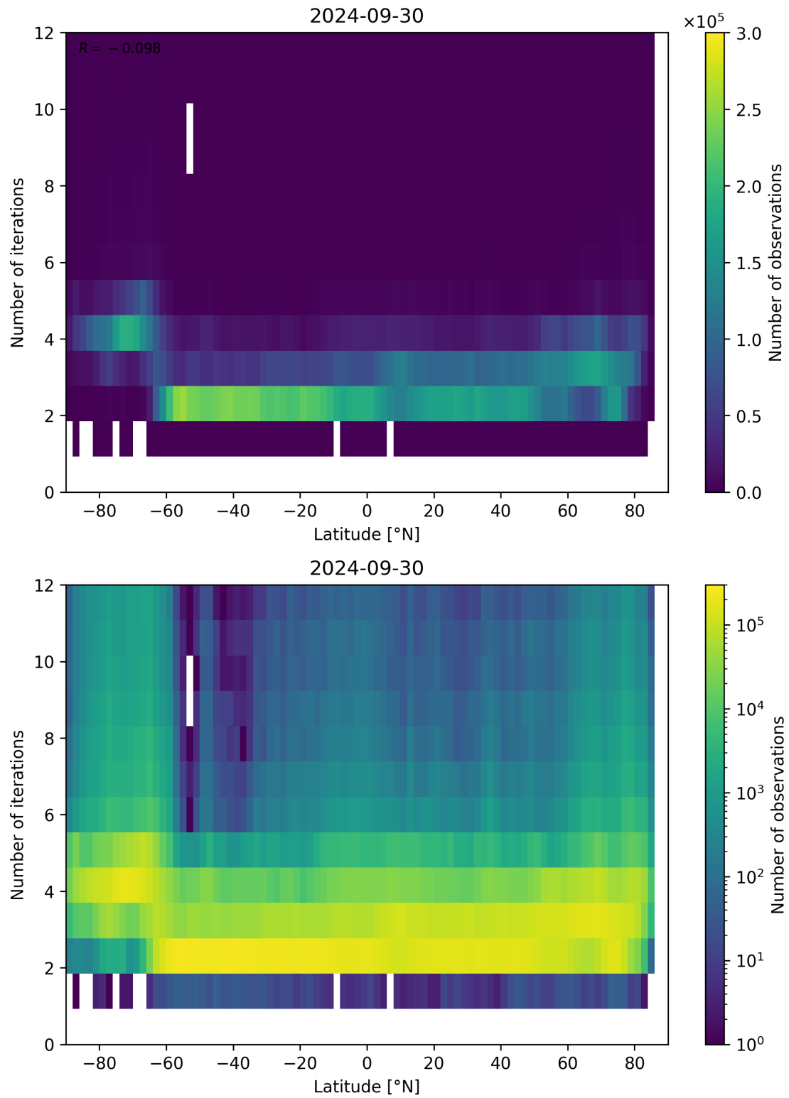
Figure 102: Scatter density plot of “Latitude” against “Number of iterations” for 2024-09-29 to 2024-10-01.
