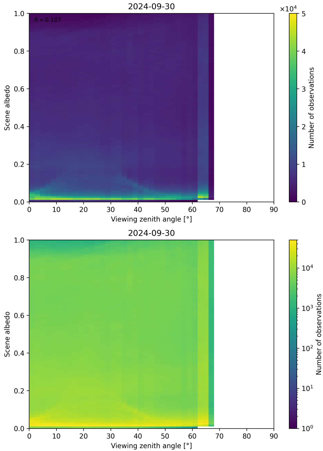
Figure 138: Scatter density plot of “Viewing zenith angle” against “Scene albedo” for 2024-09-29 to 2024-10-01.
