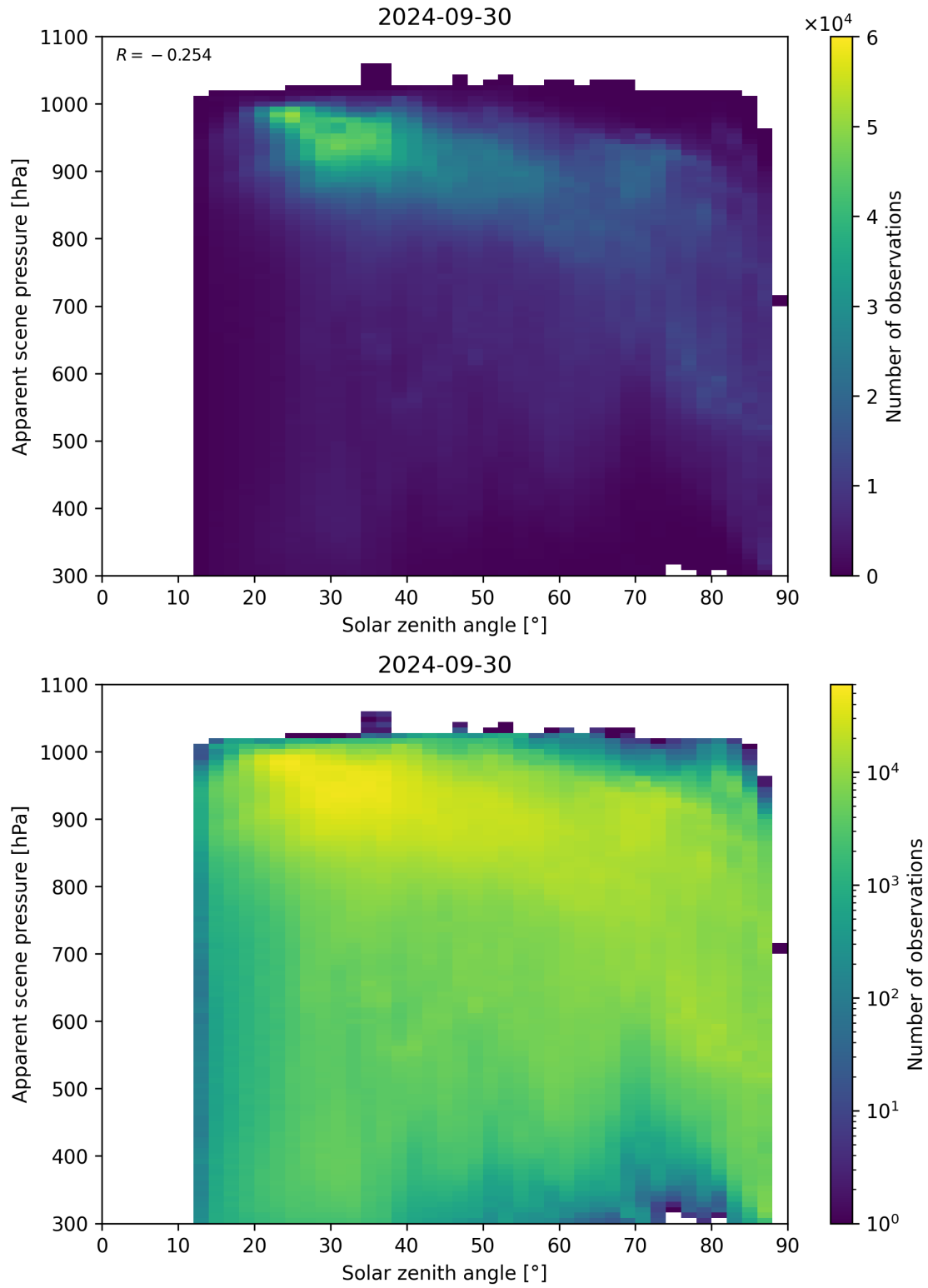
Figure 118: Scatter density plot of “Solar zenith angle” against “Apparent scene pressure” for 2024-09-29 to 2024-10-01.
