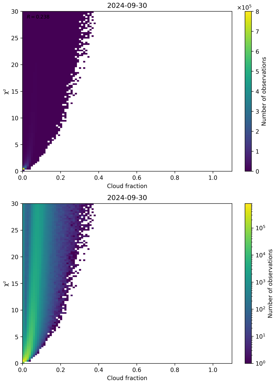
Figure 77: Scatter density plot of “Cloud fraction” against “ \chi^2 ” for 2024-09-29 to 2024-10-01.
