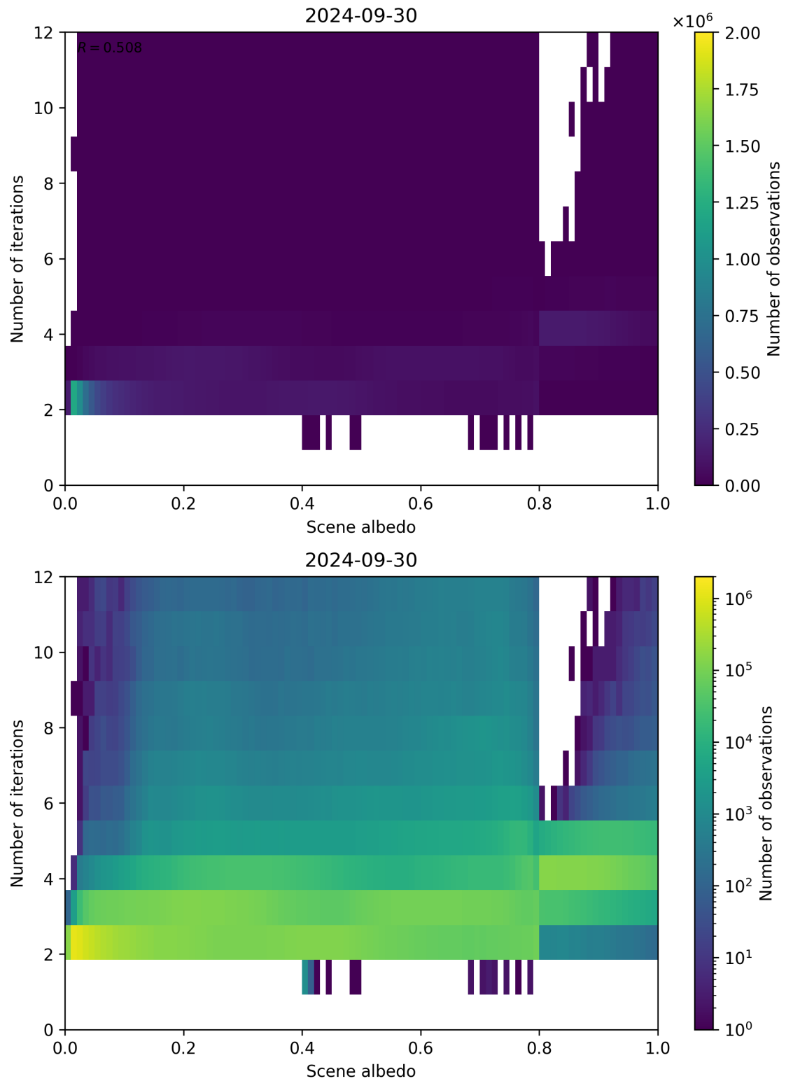
Figure 115: Scatter density plot of “Scene albedo” against “Number of iterations” for 2024-09-29 to 2024-10-01.
