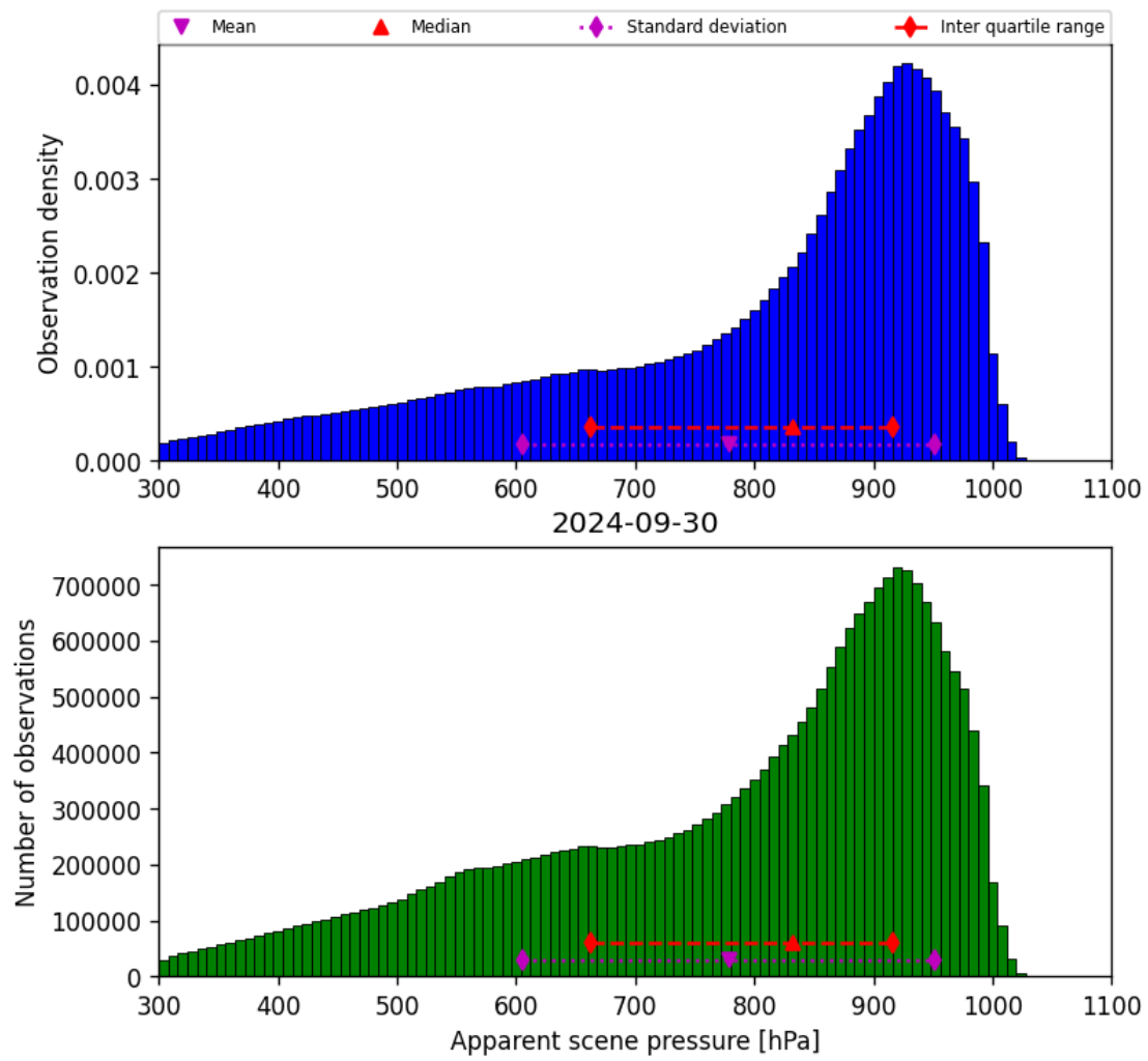
Figure 36: Histogram of “Apparent scene pressure” for 2024-09-29 to 2024-10-01
