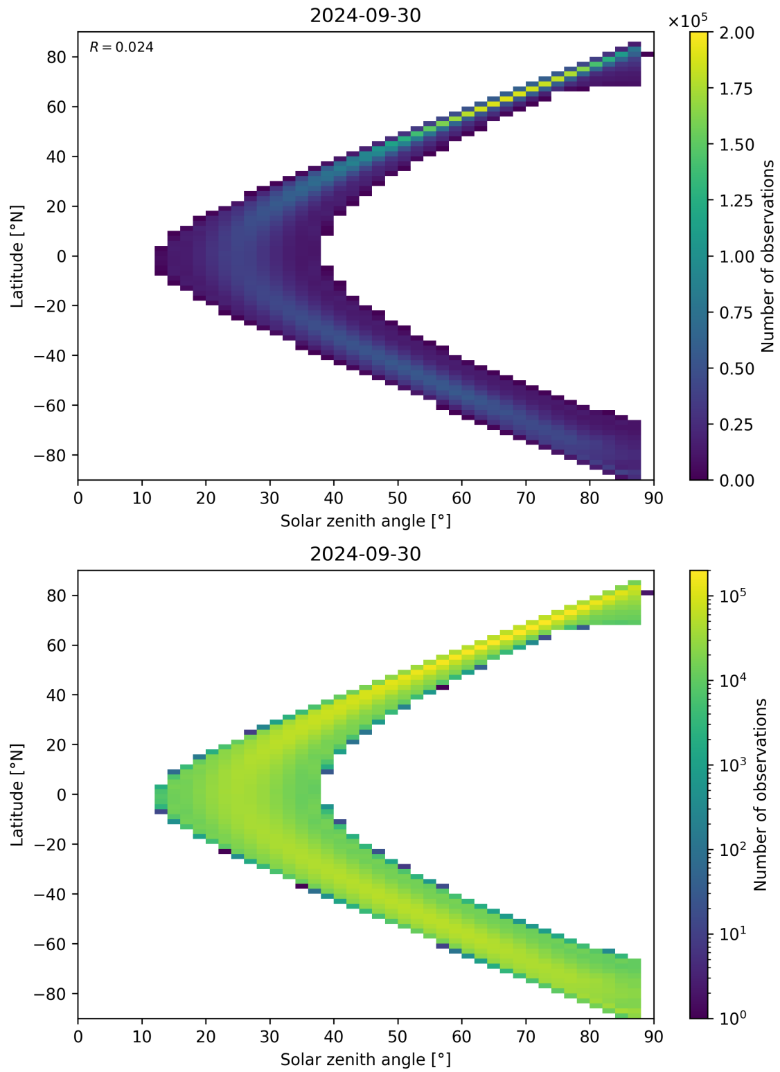
Figure 124: Scatter density plot of “Solar zenith angle” against “Latitude” for 2024-09-29 to 2024-10-01.
