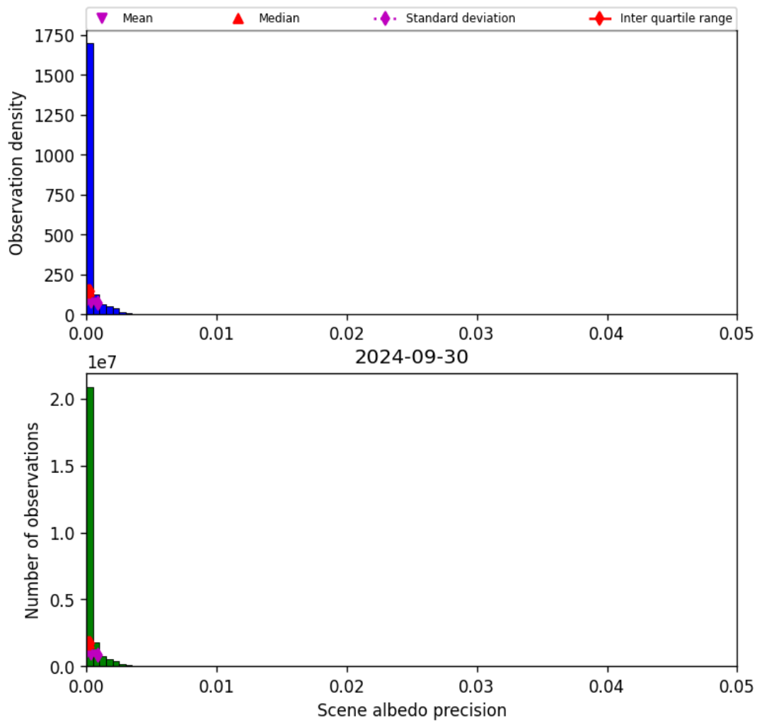
Figure 35: Histogram of “Scene albedo precision” for 2024-09-29 to 2024-10-01
