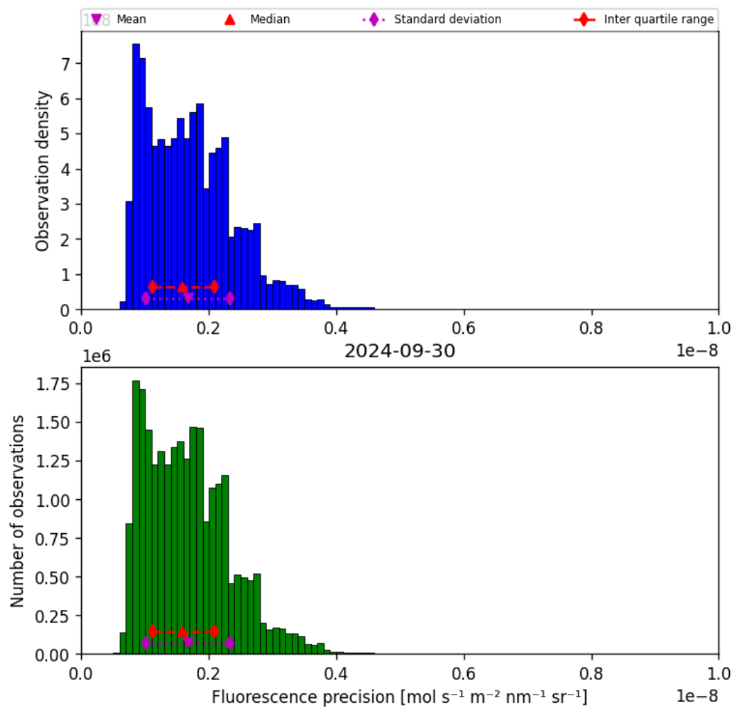
Figure 41: Histogram of “Fluorescence precision” for 2024-09-29 to 2024-10-01
