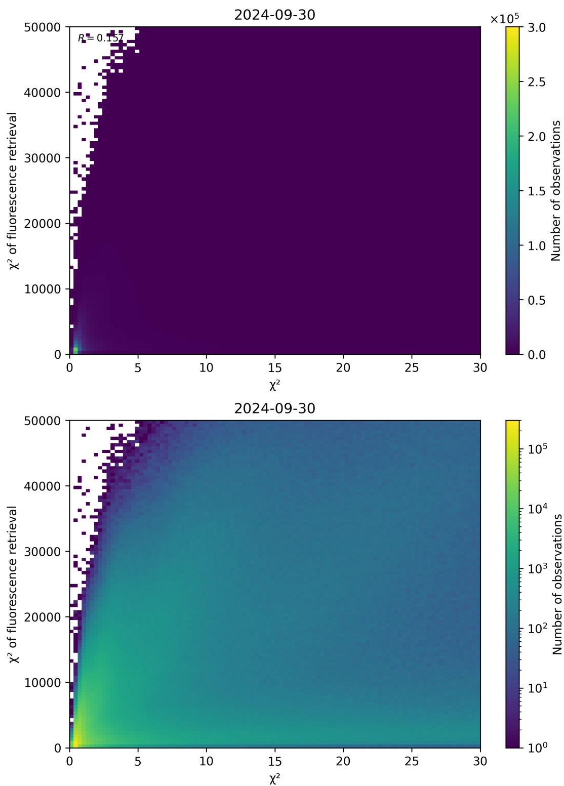
Figure 69: Scatter density plot of “ \chi^2 ” against “ \chi^2 of fluorescence retrieval” for 2024-09-29 to 2024-10-01.
