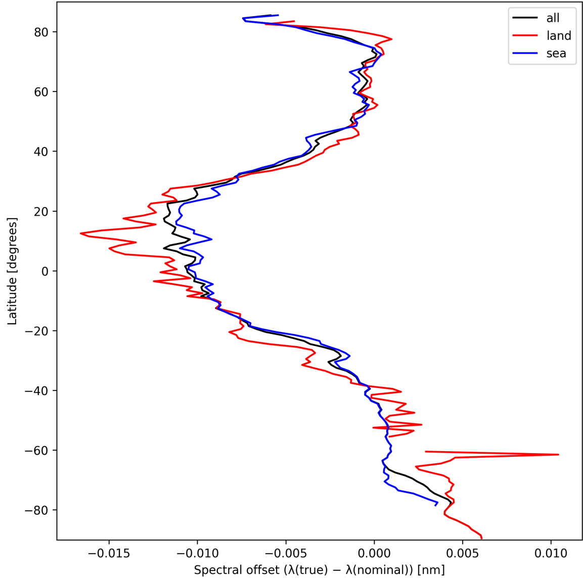
Figure 28: Zonal average of “Spectral offset ( \lambda_{\text{true}} - \lambda_{\text{nominal}} )” for 2024-09-29 to 2024-10-01.
