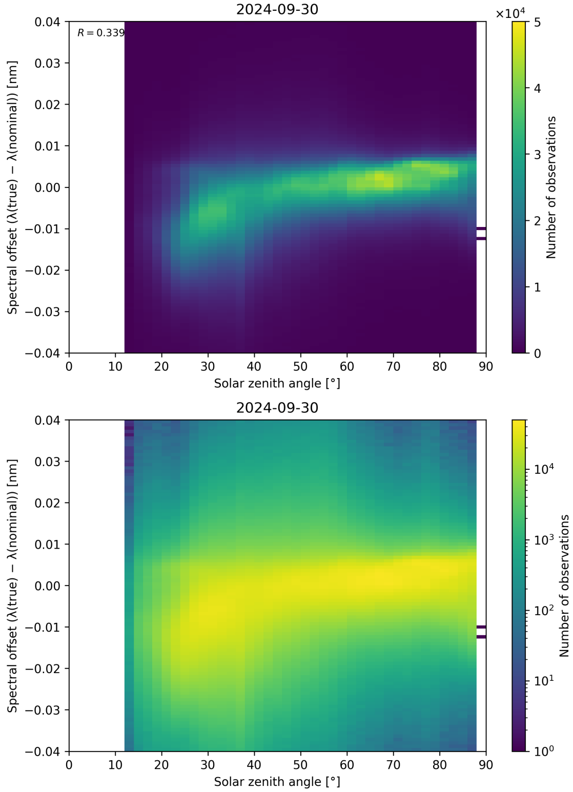
Figure 128: Scatter density plot of “Solar zenith angle” against “Spectral offset ( \lambda_{\text{true}} - \lambda_{\text{nominal}} )” for 2024-09-29 to 2024-10-01.
