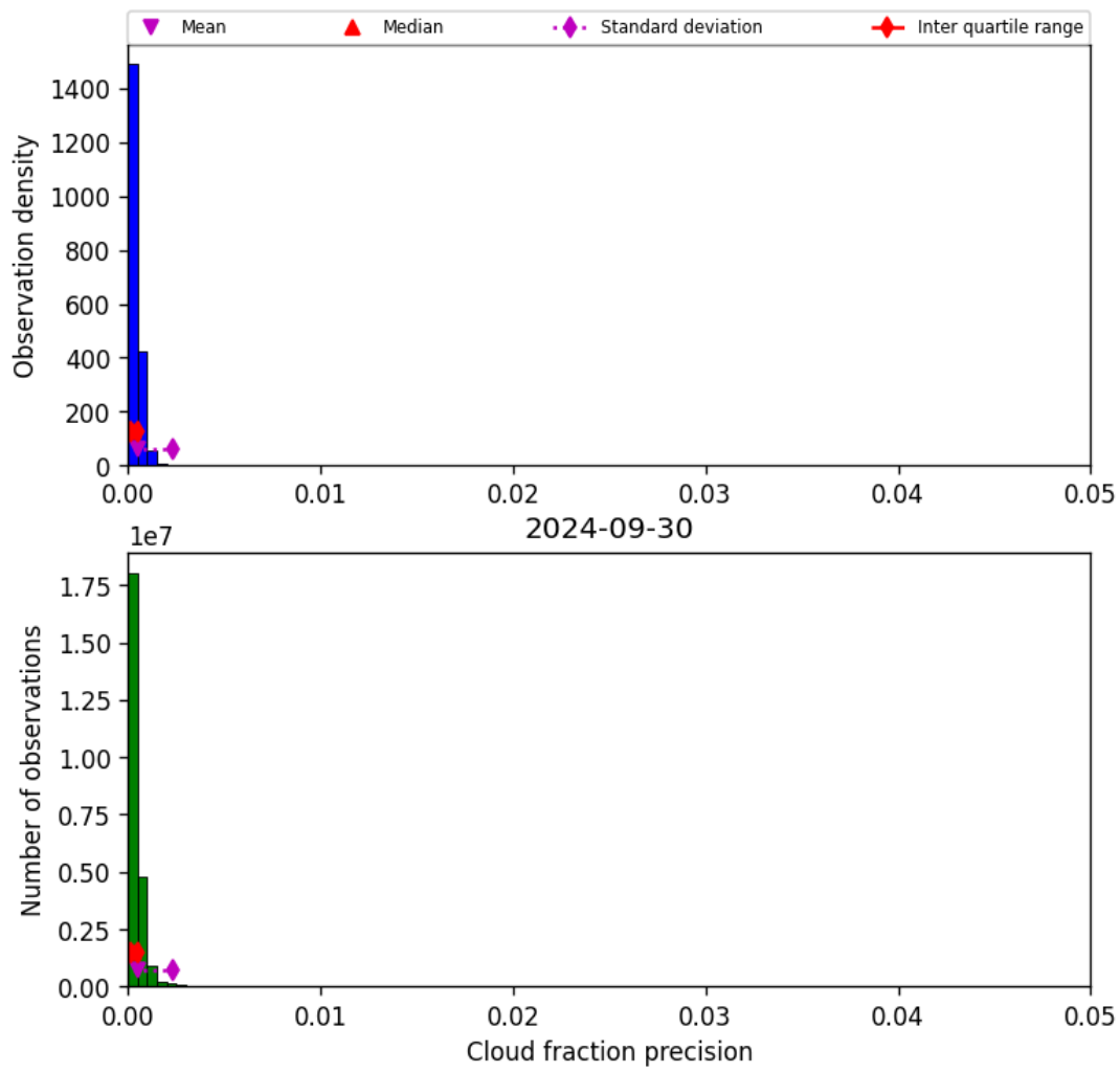
Figure 33: Histogram of “Cloud fraction precision” for 2024-09-29 to 2024-10-01
