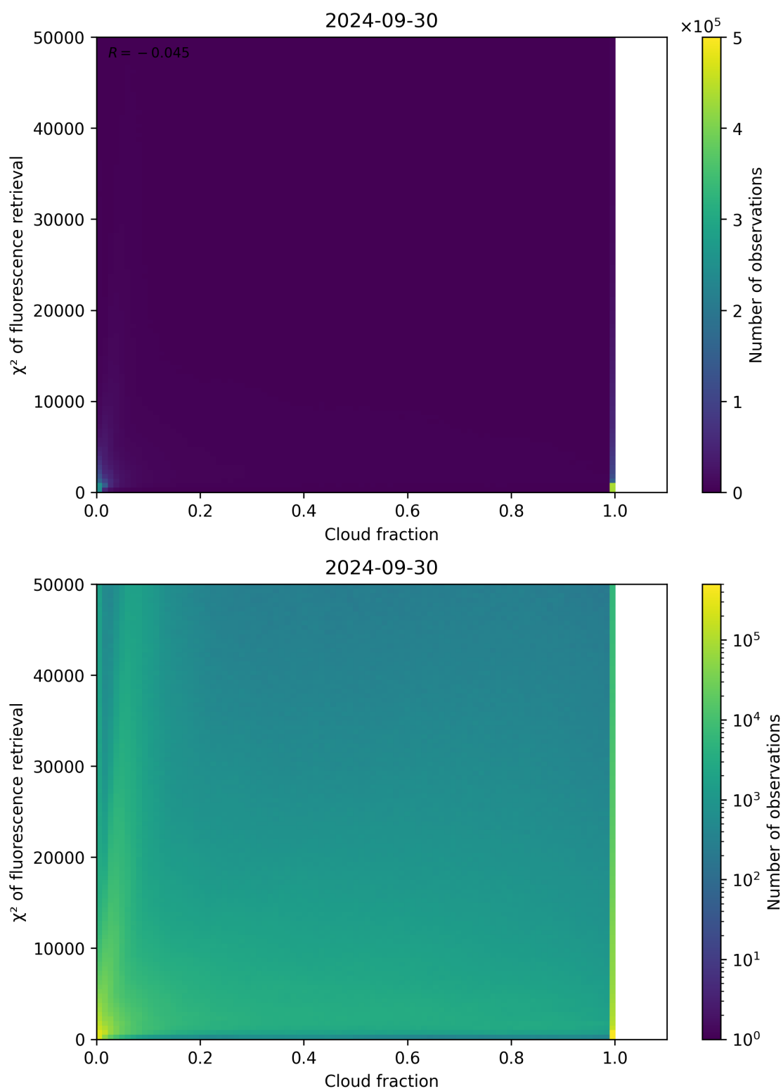
Figure 78: Scatter density plot of “Cloud fraction” against “ \chi^2 of fluorescence retrieval” for 2024-09-29 to 2024-10-01.
