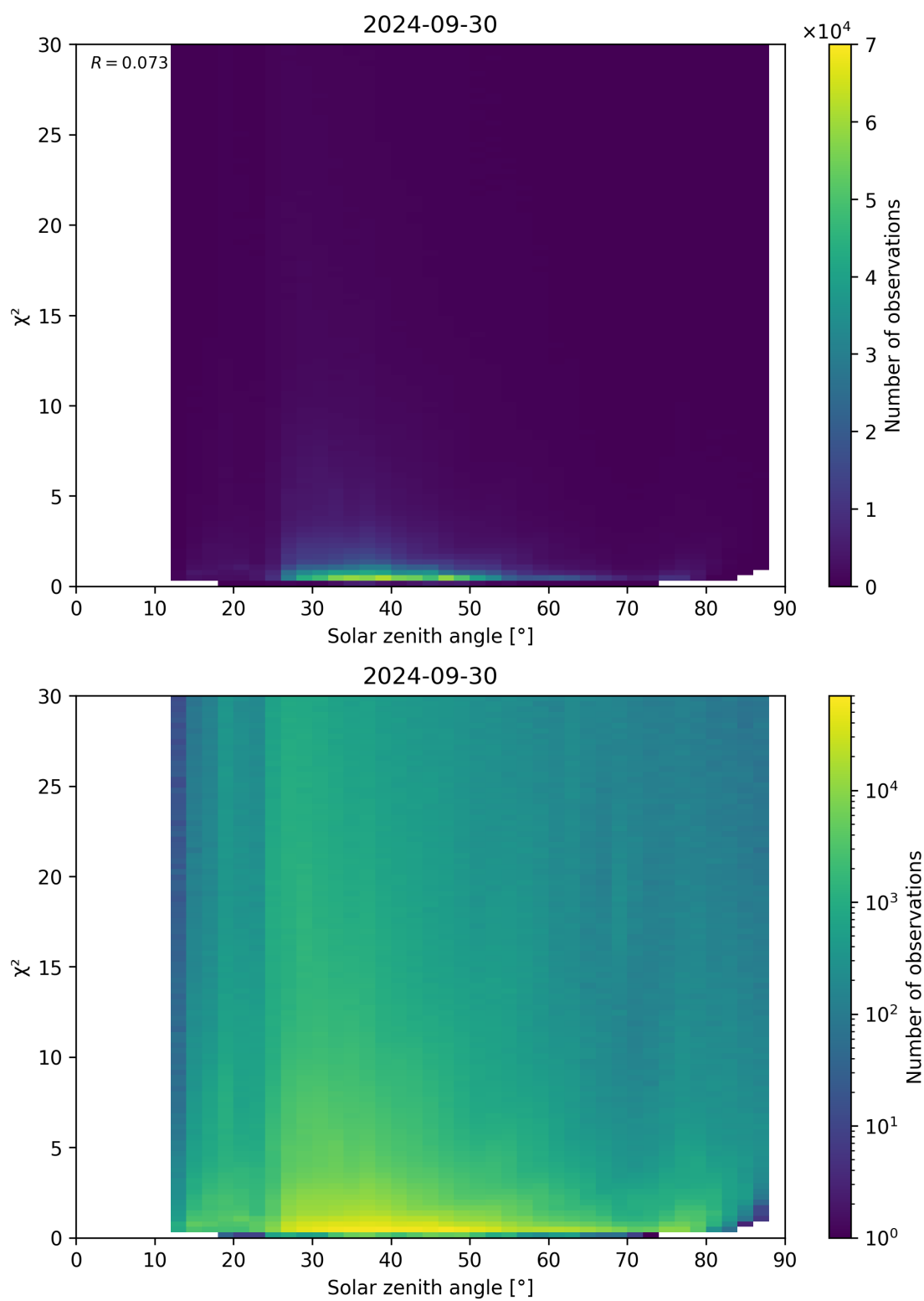
Figure 119: Scatter density plot of “Solar zenith angle” against “ \chi^2 ” for 2024-09-29 to 2024-10-01.
