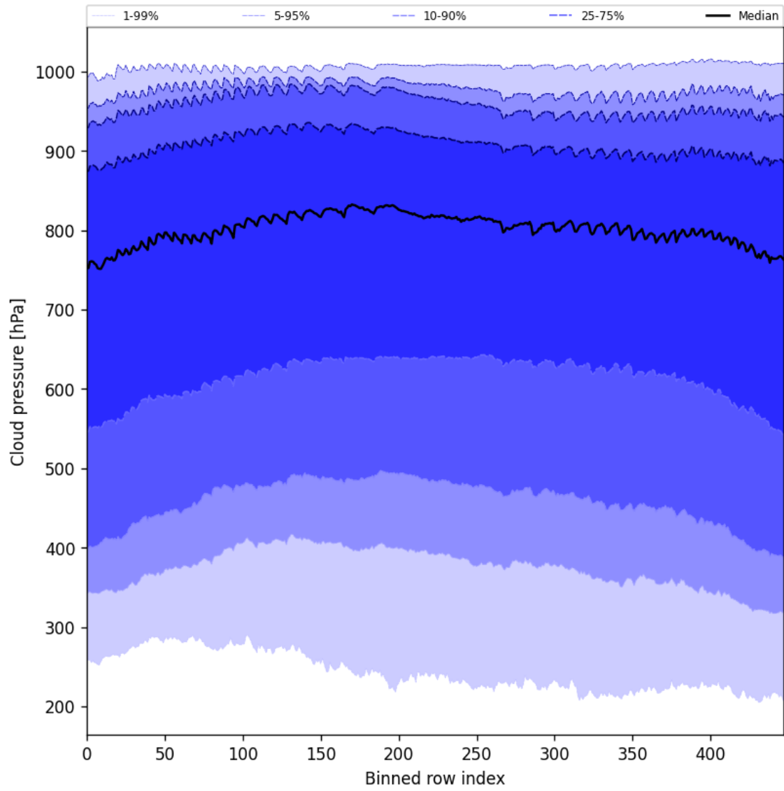
Figure 47: Along track statistics of “Cloud pressure” for 2024-09-29 to 2024-10-01
