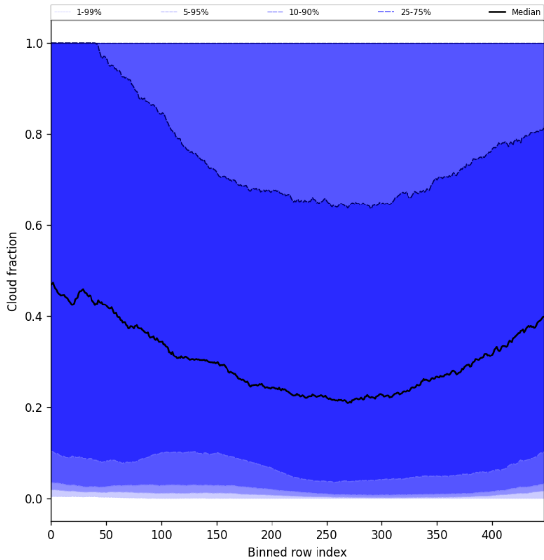
Figure 49: Along track statistics of “Cloud fraction” for 2024-09-29 to 2024-10-01
