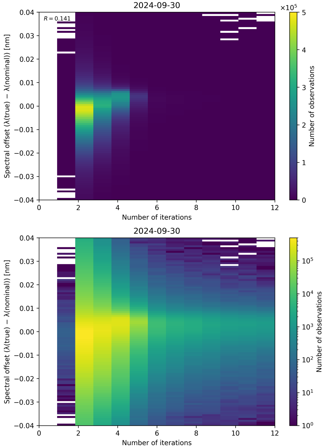
Figure 109: Scatter density plot of “Number of iterations” against “Spectral offset ( \lambda_{\text{true}} - \lambda_{\text{nominal}} )” for 2024-09-29 to 2024-10-01.
