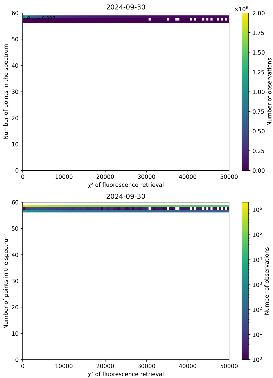
Figure 71: Scatter density plot of " \chi^2 of fluorescence retrieval" against "Number of points in the spectrum" for 2024-09-29 to 2024-10-01.
