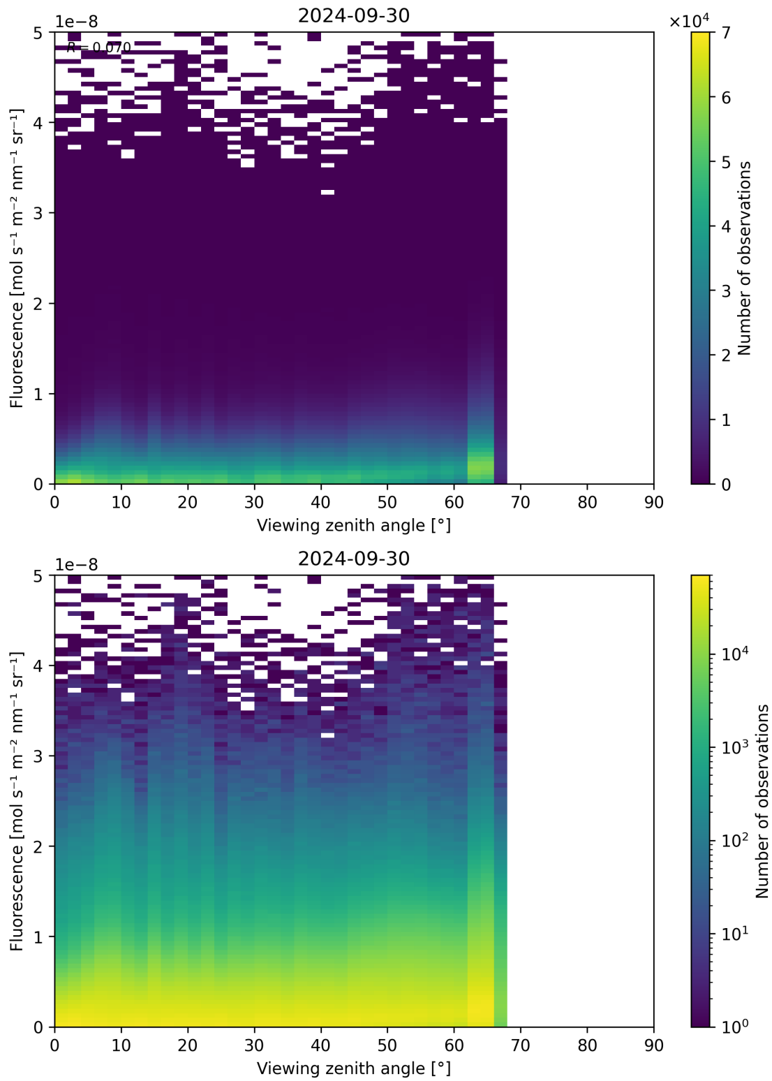
Figure 134: Scatter density plot of “Viewing zenith angle” against “Fluorescence” for 2024-09-29 to 2024-10-01.
