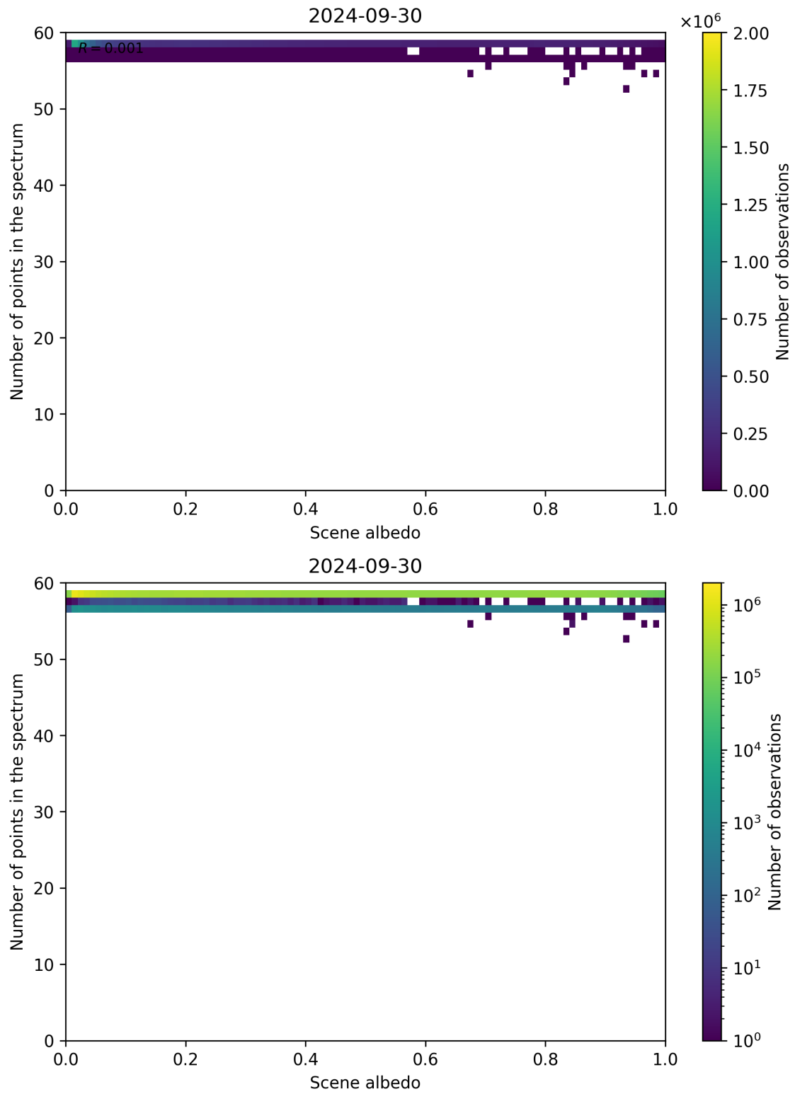
Figure 116: Scatter density plot of “Scene albedo” against “Number of points in the spectrum” for 2024-09-29 to 2024-10-01.
