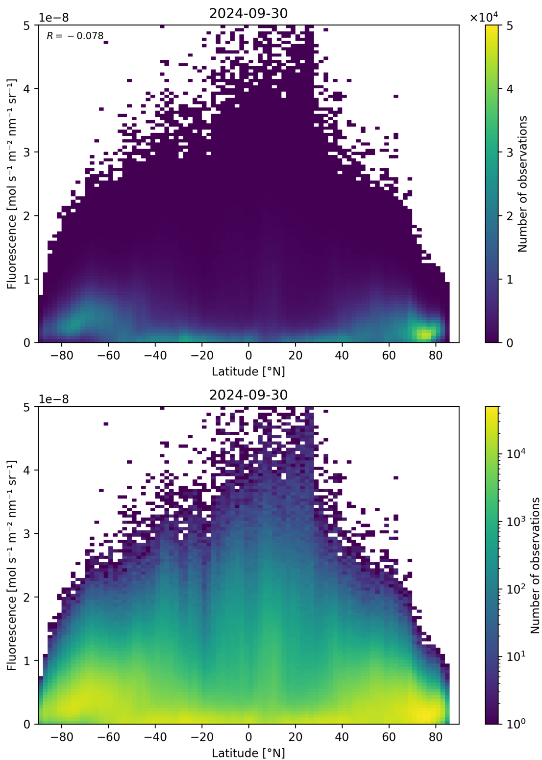
Figure 101: Scatter density plot of “Latitude” against “Fluorescence” for 2024-09-29 to 2024-10-01.
