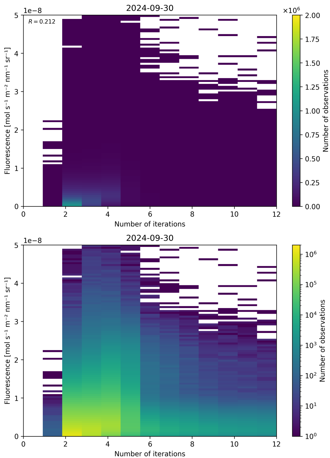
Figure 107: Scatter density plot of “Number of iterations” against “Fluorescence” for 2024-09-29 to 2024-10-01.
