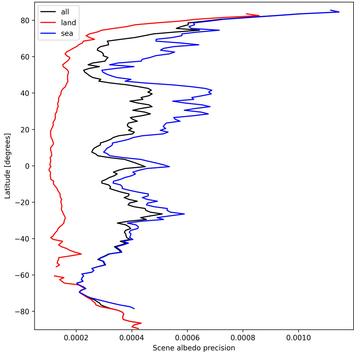
Figure 18: Zonal average of “Scene albedo precision” for 2024-09-29 to 2024-10-01.
