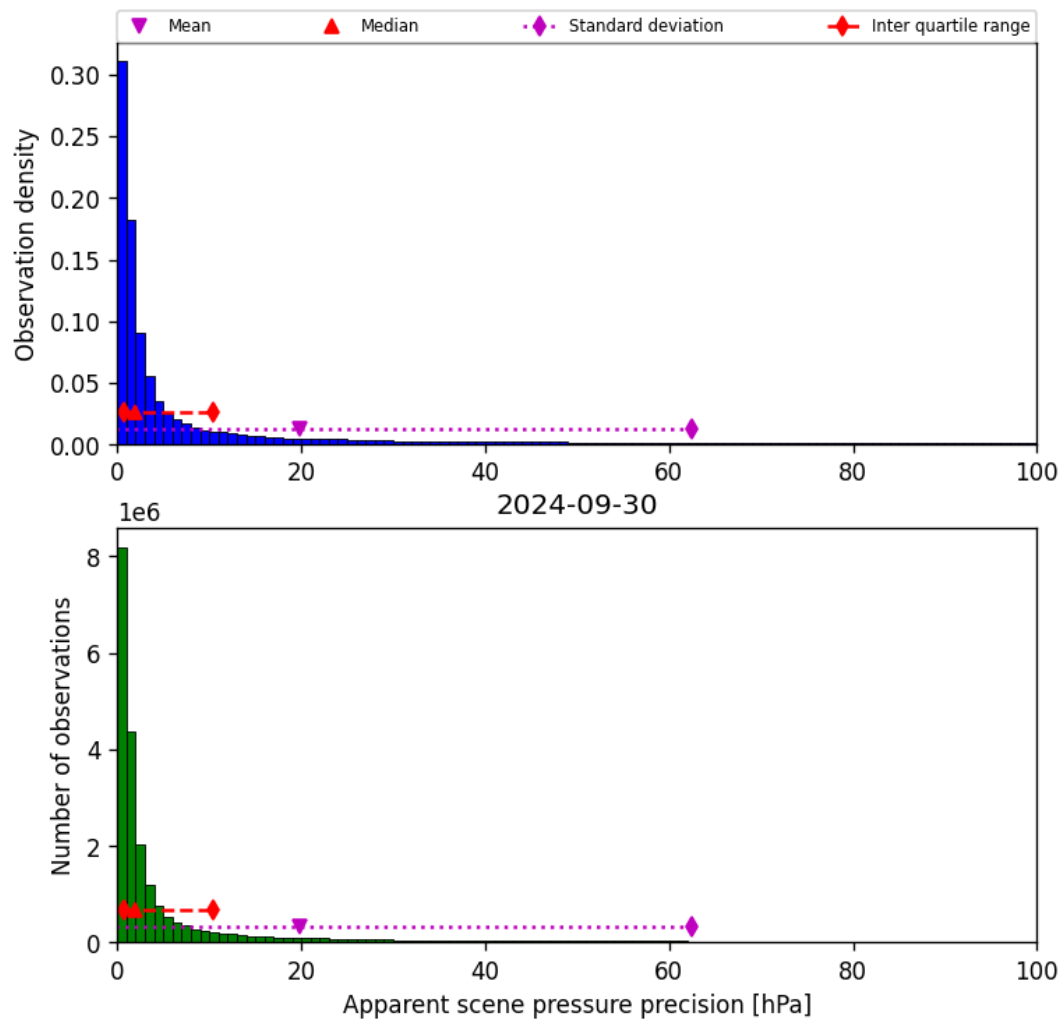
Figure 37: Histogram of “Apparent scene pressure precision” for 2024-09-29 to 2024-10-01
