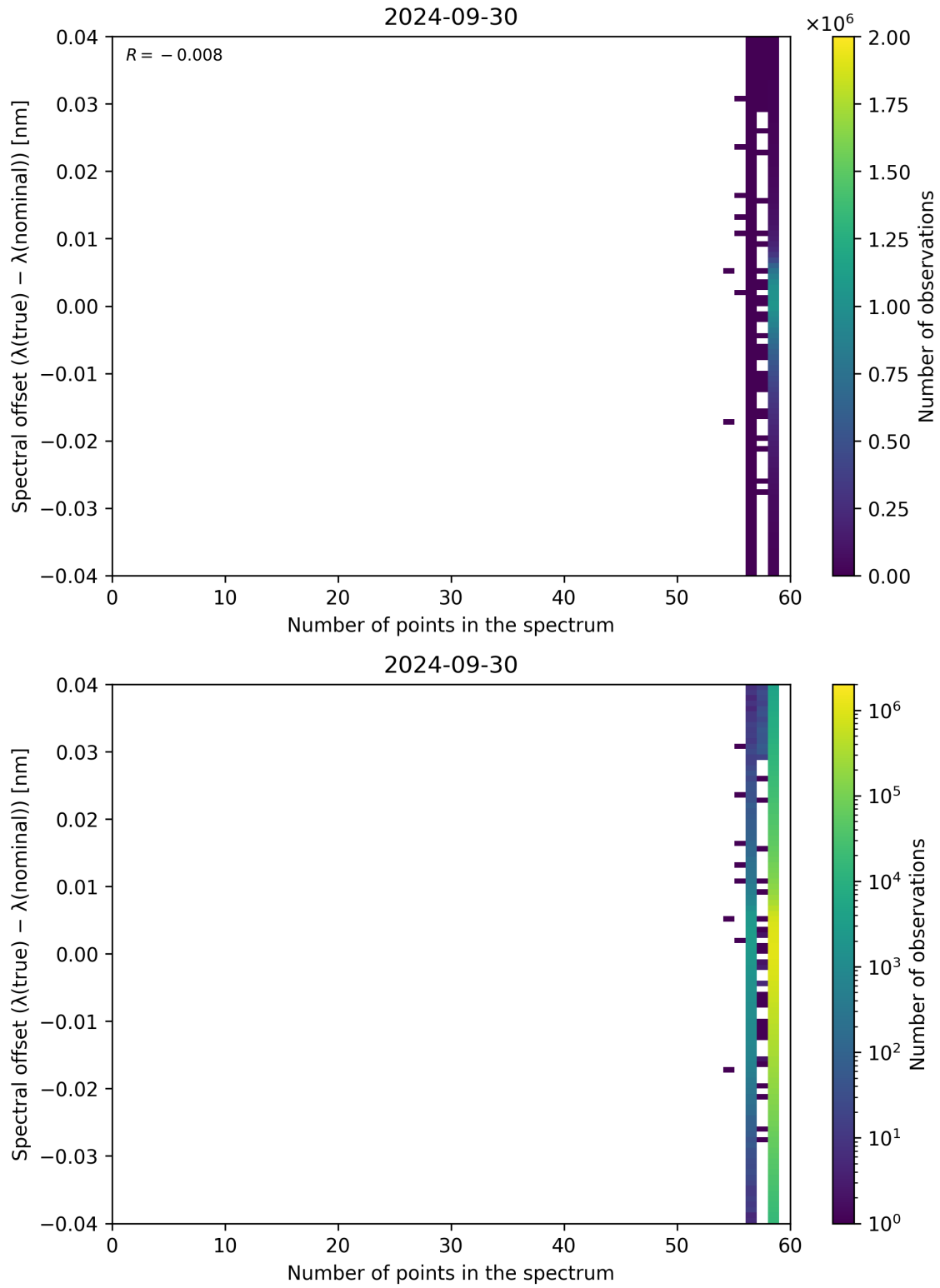
Figure 110: Scatter density plot of “Number of points in the spectrum” against “Spectral offset ( \lambda_{\text{true}} - \lambda_{\text{nominal}} )” for 2024-09-29 to 2024-10-01.
