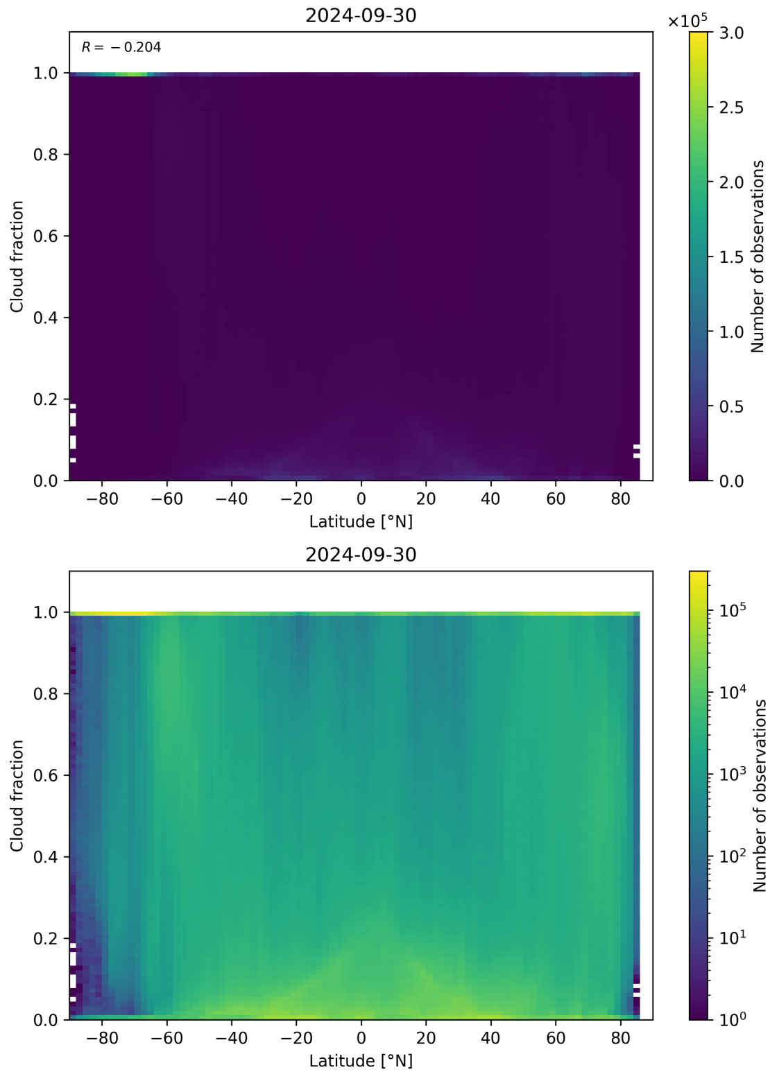
Figure 99: Scatter density plot of “Latitude” against “Cloud fraction” for 2024-09-29 to 2024-10-01.
