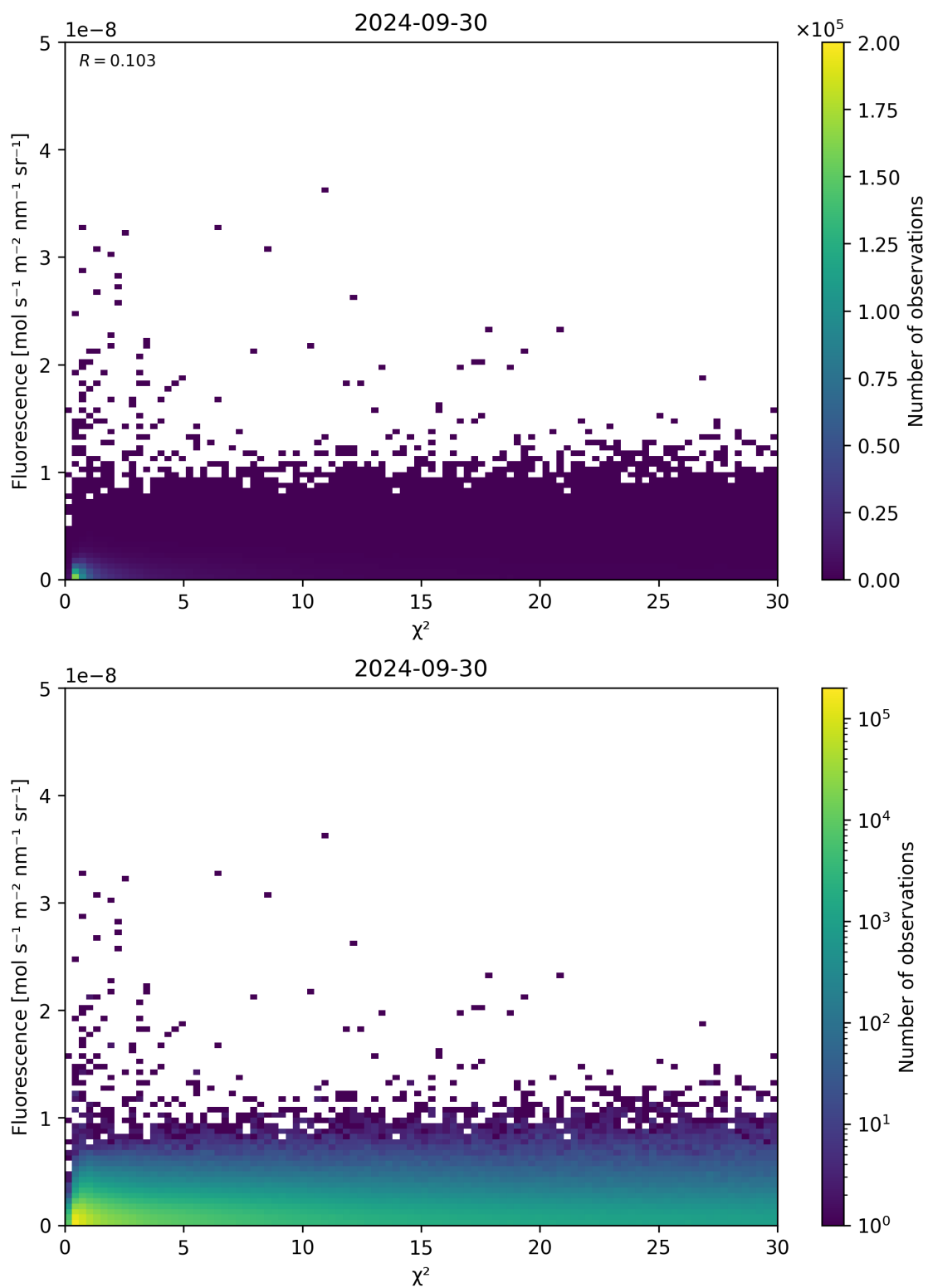
Figure 70: Scatter density plot of “ \chi^2 ” against “Fluorescence” for 2024-09-29 to 2024-10-01.
