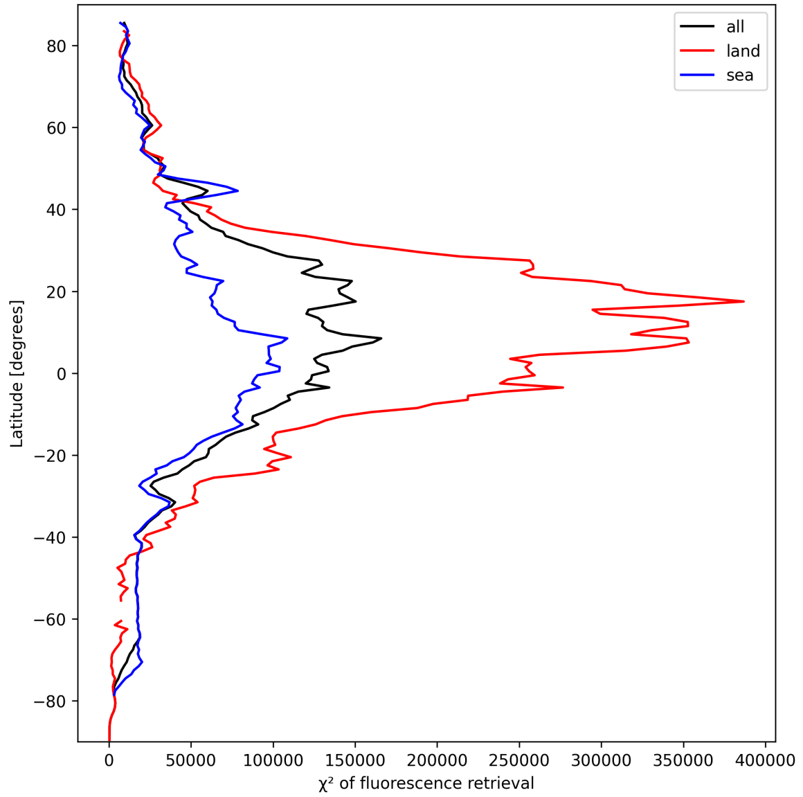
Figure 25: Zonal average of “ \chi^2 of fluorescence retrieval” for 2024-09-29 to 2024-10-01.
