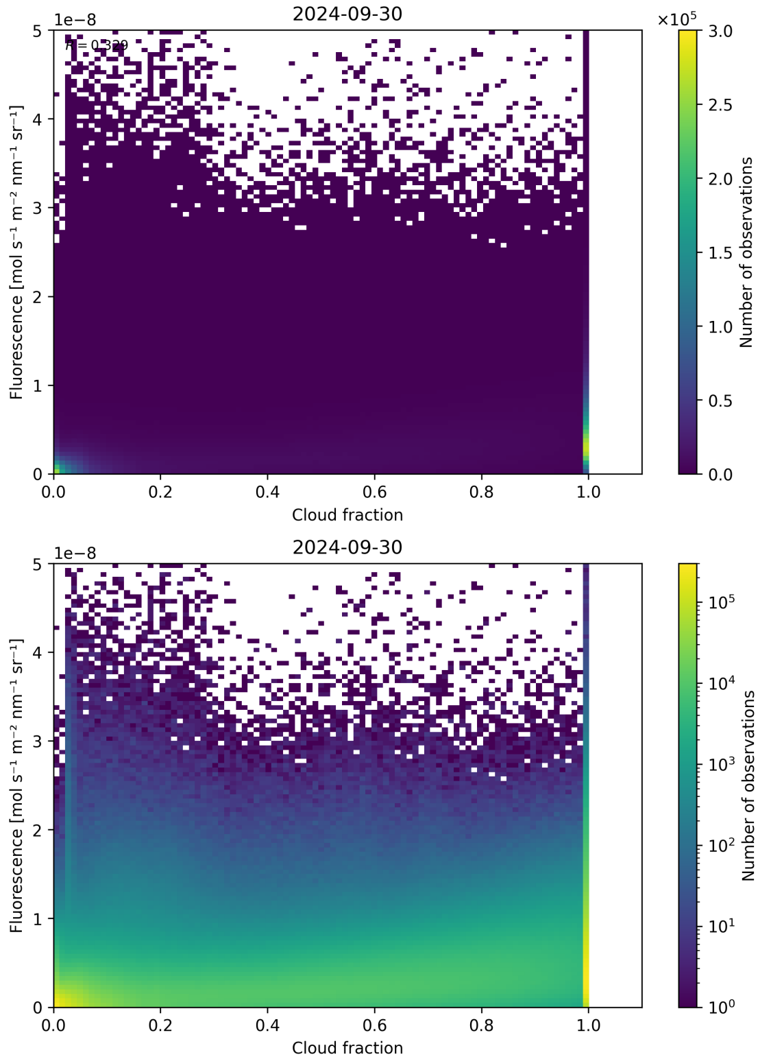
Figure 79: Scatter density plot of “Cloud fraction” against “Fluorescence” for 2024-09-29 to 2024-10-01.
