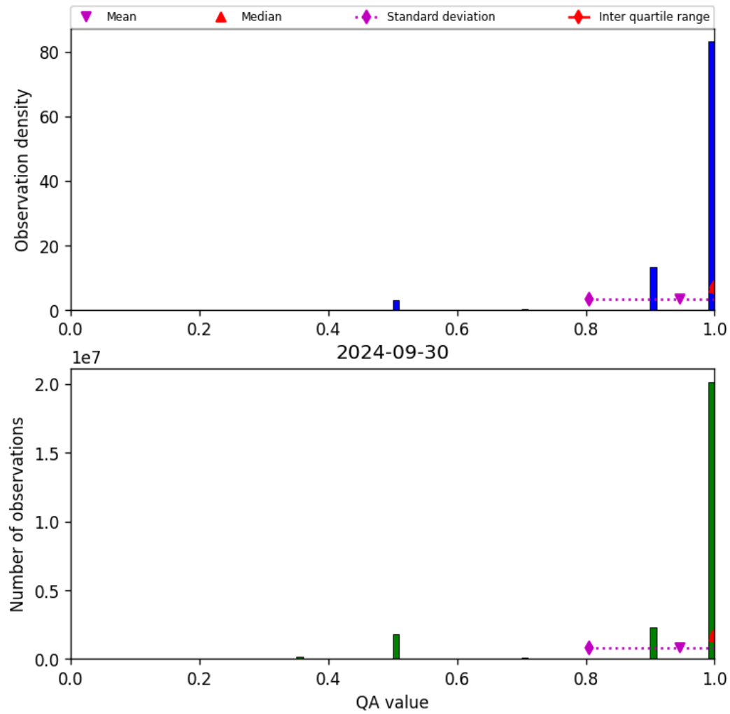
Figure 29: Histogram of “QA value” for 2024-09-29 to 2024-10-01
