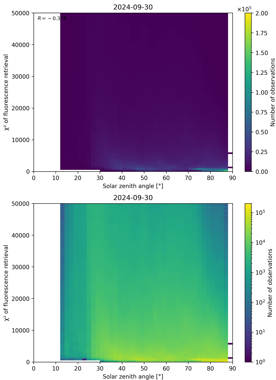
Figure 120: Scatter density plot of “Solar zenith angle” against “ \chi^2 of fluorescence retrieval” for 2024-09-29 to 2024-10-01.
