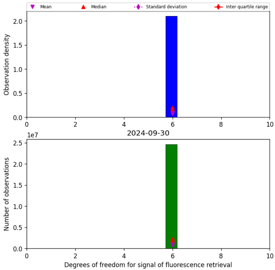
Figure 43: Histogram of "Degrees of freedom for signal of fluorescence retrieval" for 2024-09-29 to 2024-10-01
