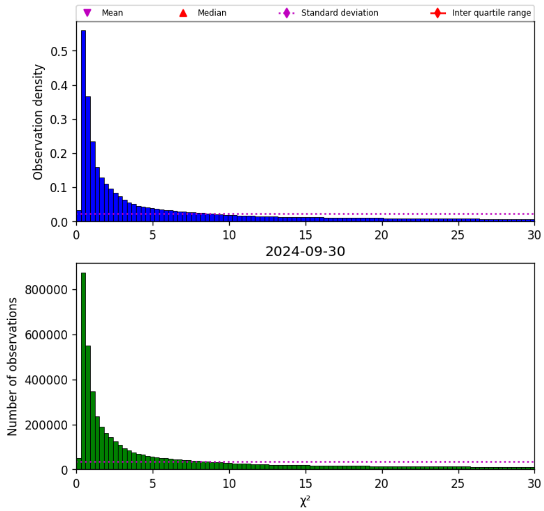
Figure 38: Histogram of “ \chi^2 ” for 2024-09-29 to 2024-10-01
