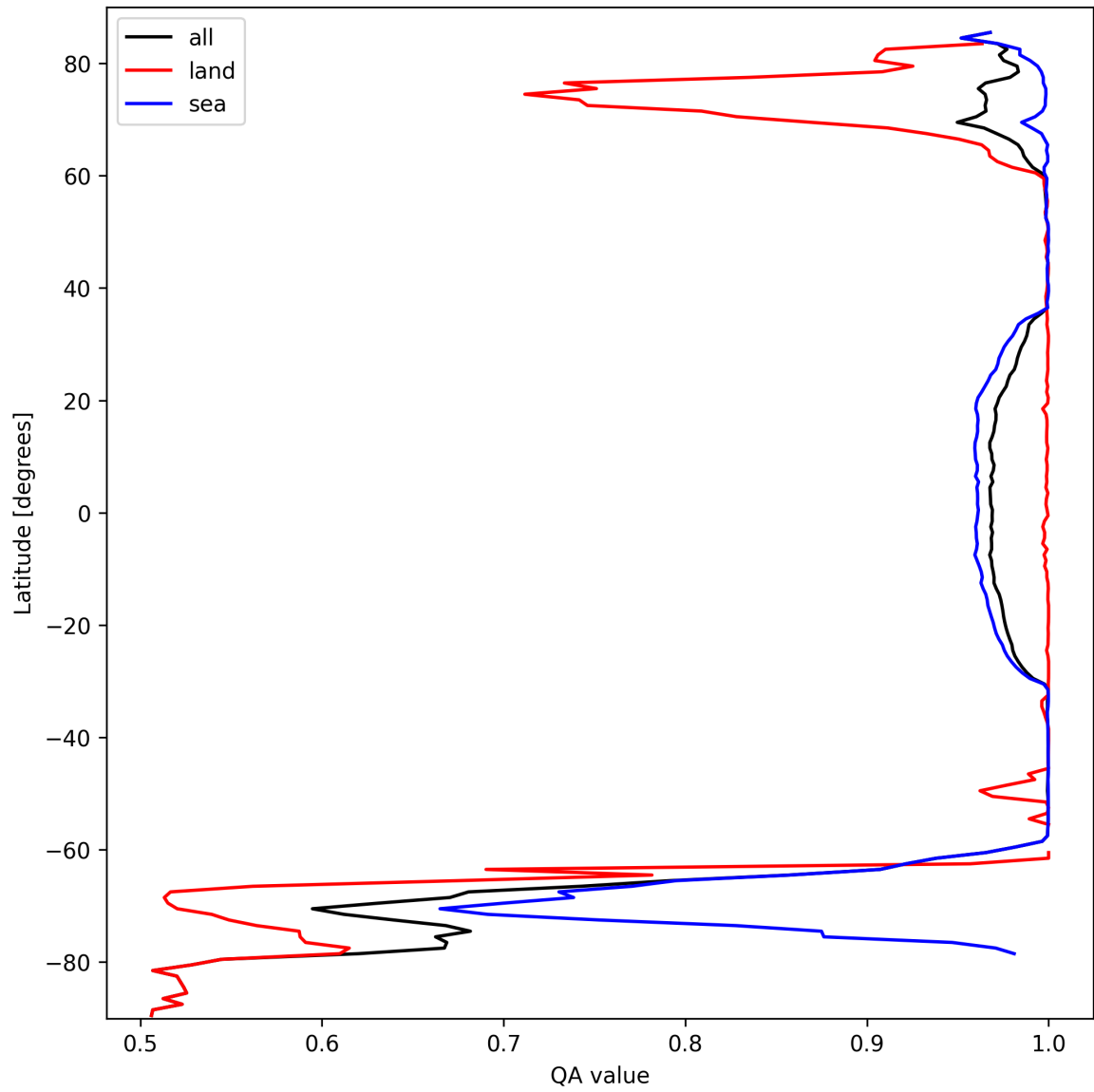
Figure 12: Zonal average of “QA value” for 2024-09-29 to 2024-10-01.
