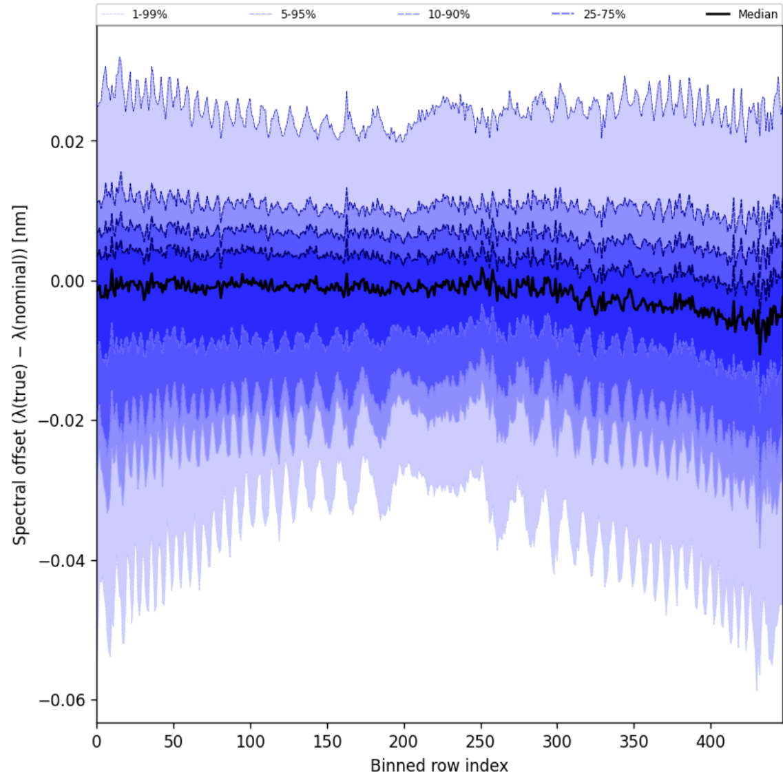
Figure 62: Along track statistics of “Spectral offset ( \lambda_{\text{true}} - \lambda_{\text{nominal}} )” for 2024-09-29 to 2024-10-01
