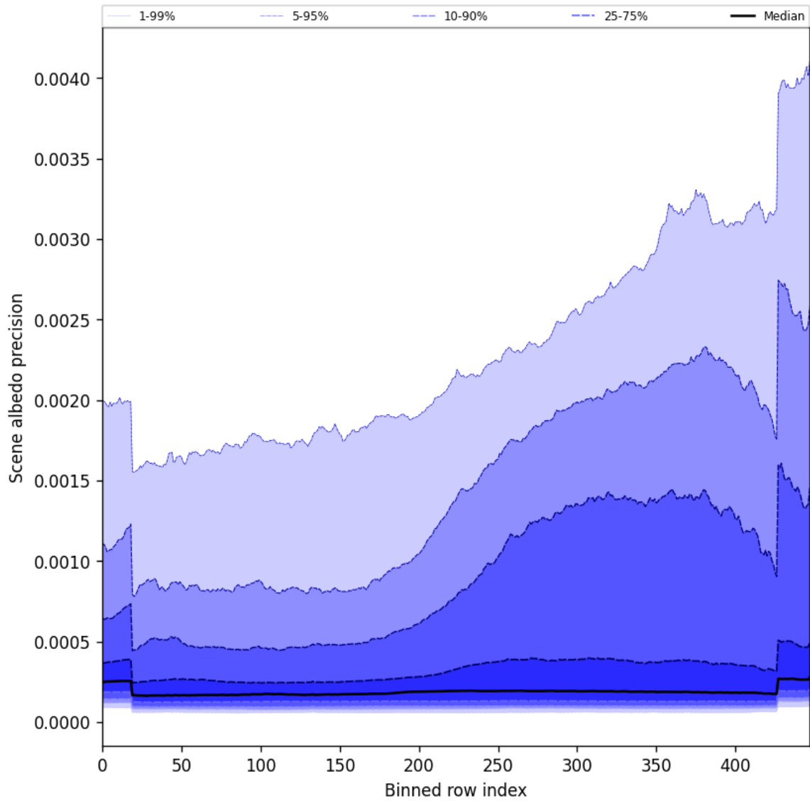
Figure 52: Along track statistics of “Scene albedo precision” for 2024-09-29 to 2024-10-01
