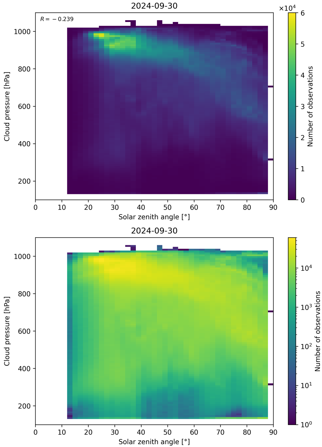
Figure 122: Scatter density plot of “Solar zenith angle” against “Cloud pressure” for 2024-09-29 to 2024-10-01.
