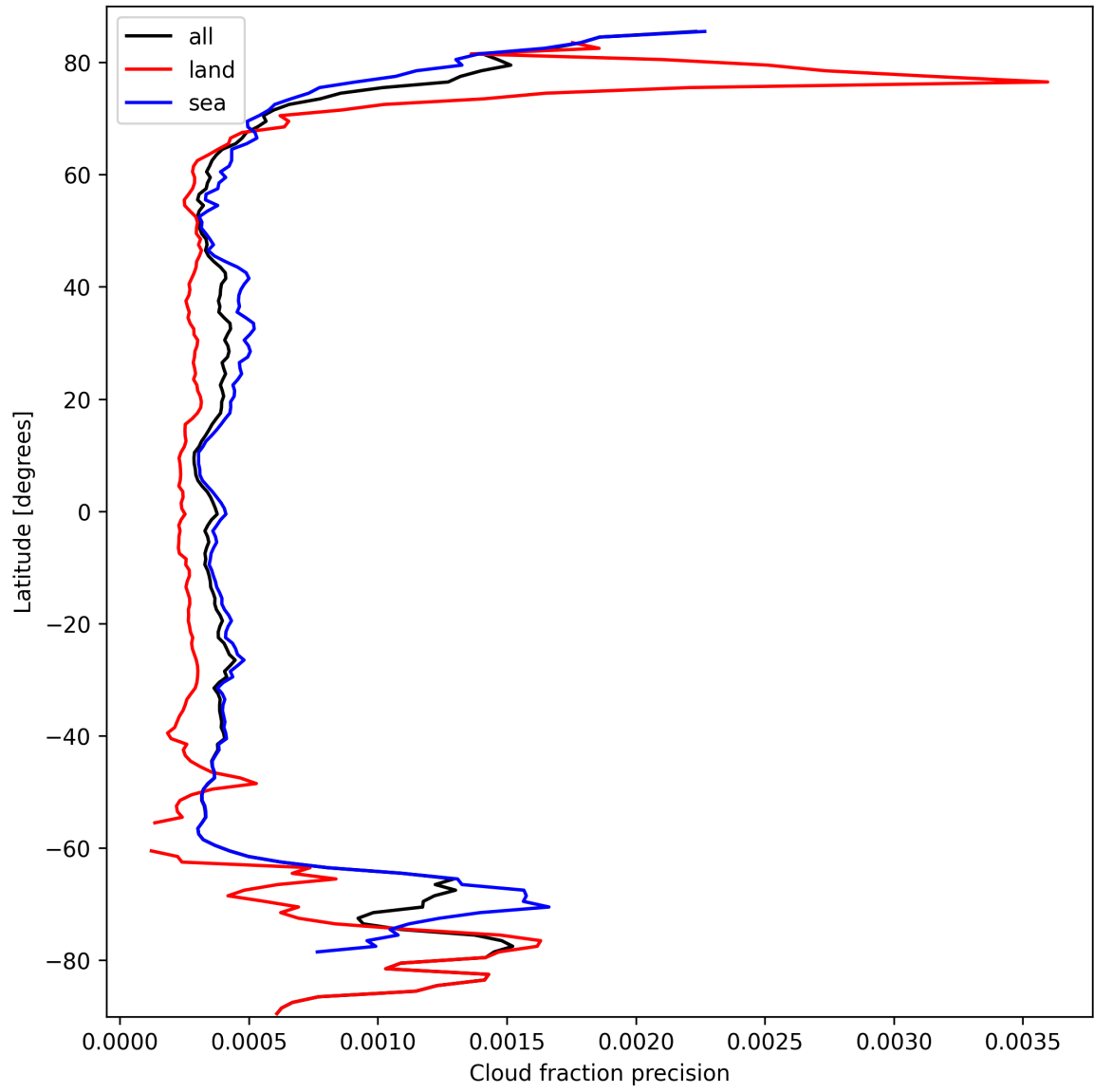
Figure 16: Zonal average of “Cloud fraction precision” for 2024-09-29 to 2024-10-01.
