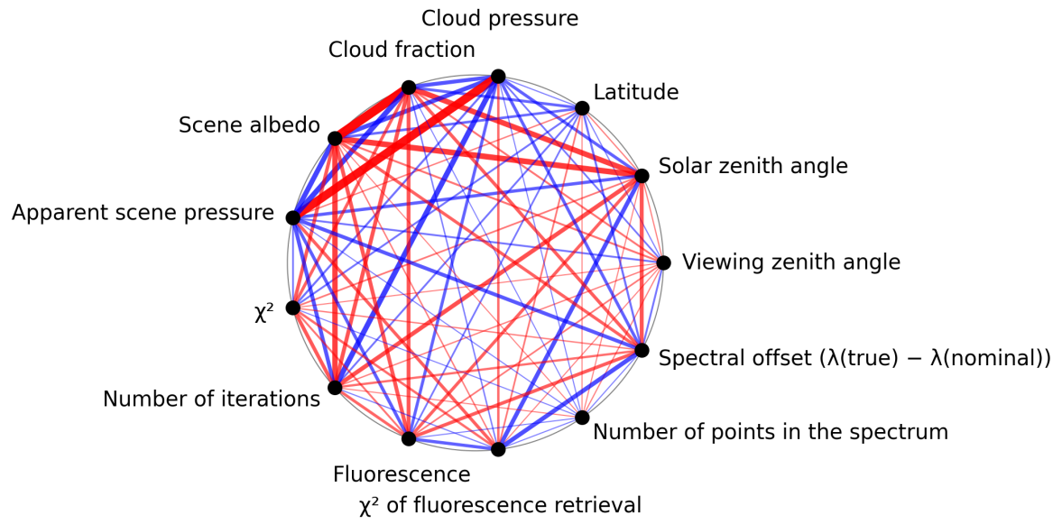
Figure 1: Map of correlation graph for 2024-09-29 to 2024-10-01.
