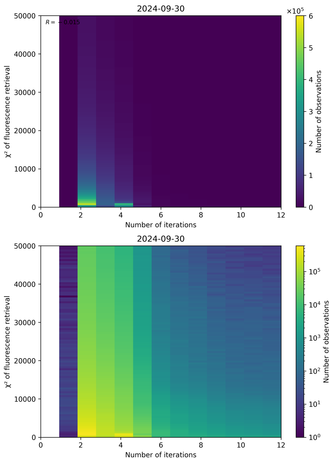
Figure 106: Scatter density plot of “Number of iterations” against “ \chi^2 of fluorescence retrieval” for 2024-09-29 to 2024-10-01.
