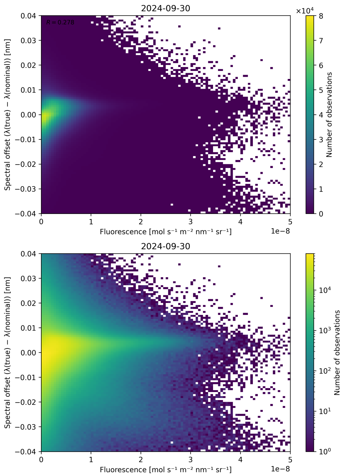
Figure 95: Scatter density plot of “Fluorescence” against “Spectral offset ( \lambda_{\text{true}} - \lambda_{\text{nominal}} )” for 2024-09-29 to 2024-10-01.
