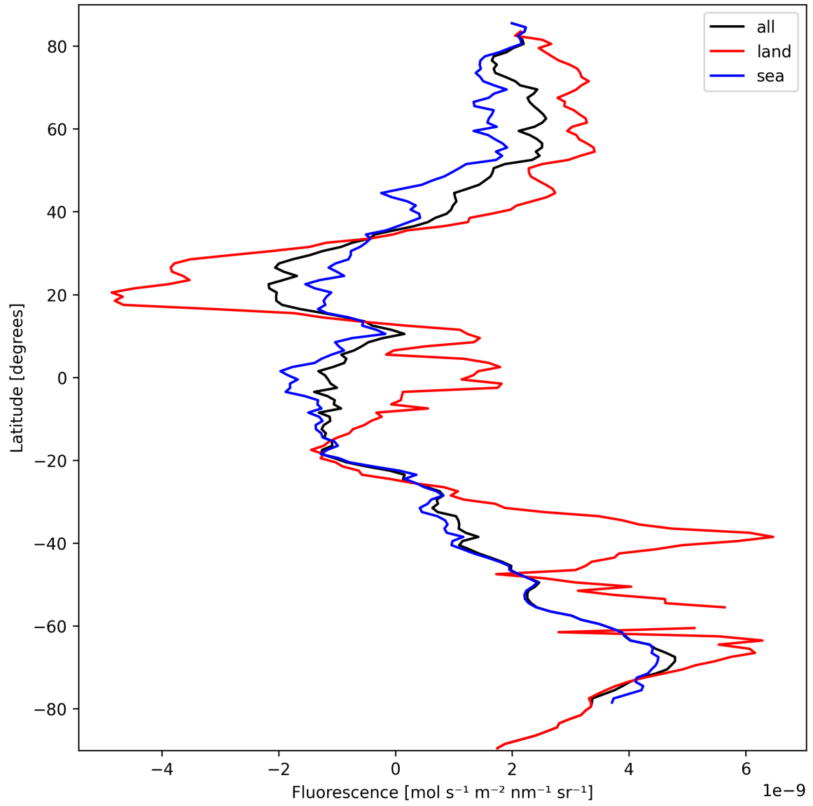
Figure 23: Zonal average of “Fluorescence” for 2024-09-29 to 2024-10-01.
