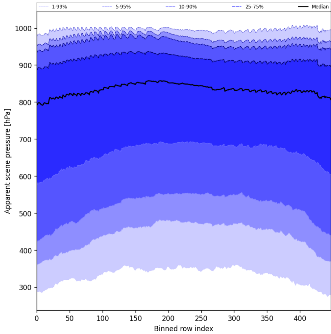
Figure 53: Along track statistics of “Apparent scene pressure” for 2024-09-29 to 2024-10-01
