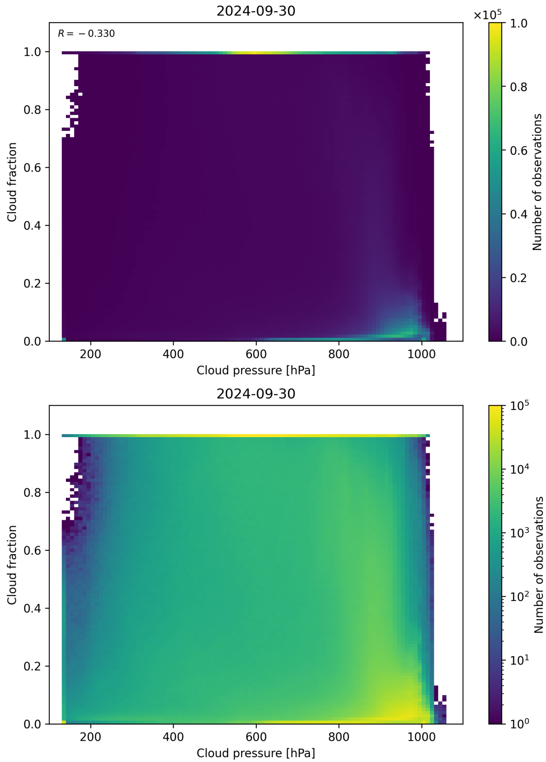
Figure 87: Scatter density plot of “Cloud pressure” against “Cloud fraction” for 2024-09-29 to 2024-10-01.
