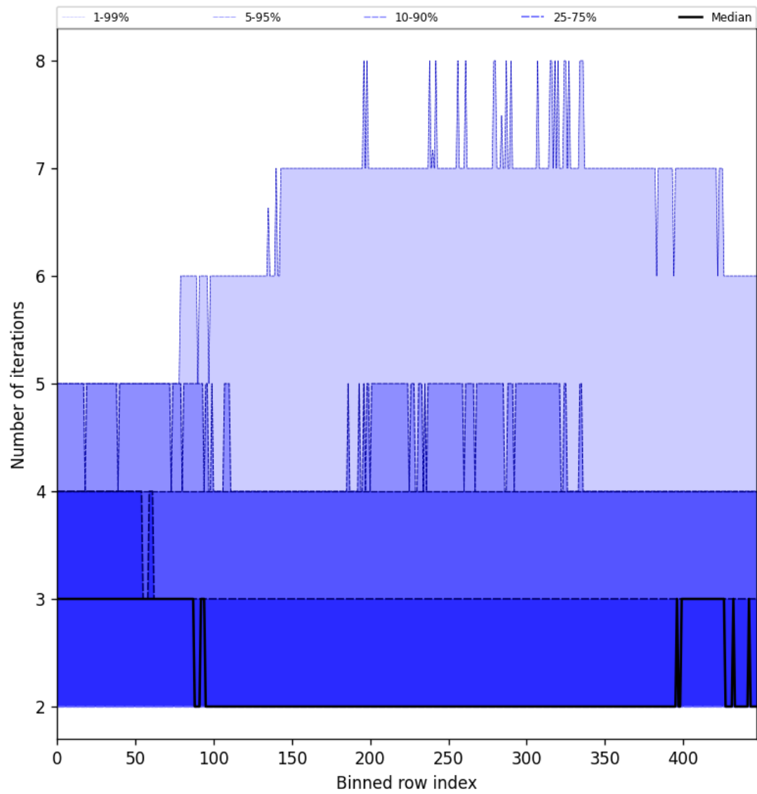
Figure 56: Along track statistics of “Number of iterations” for 2024-09-29 to 2024-10-01
