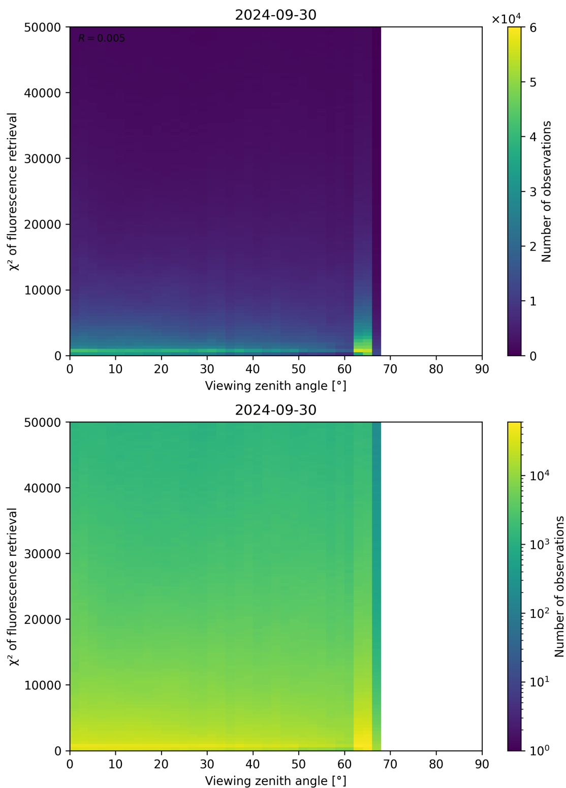
Figure 131: Scatter density plot of “Viewing zenith angle” against “ \chi^2 of fluorescence retrieval” for 2024-09-29 to 2024-10-01.
