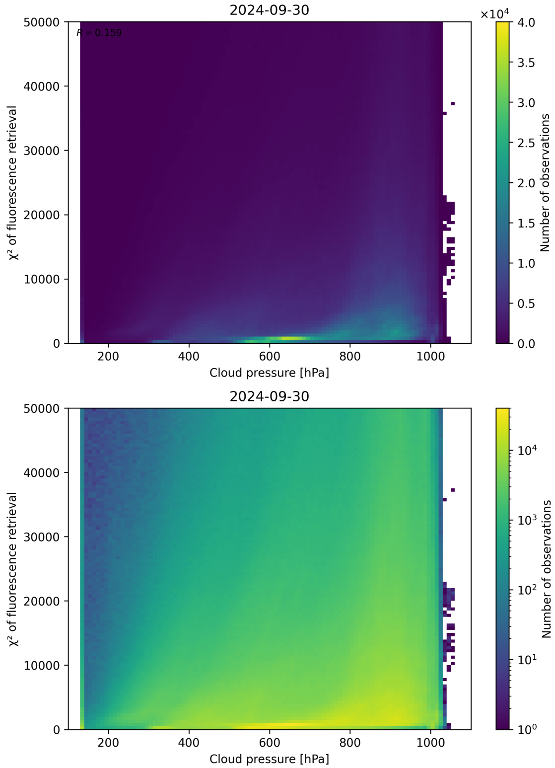
Figure 86: Scatter density plot of “Cloud pressure” against “ \chi^2 of fluorescence retrieval” for 2024-09-29 to 2024-10-01.
