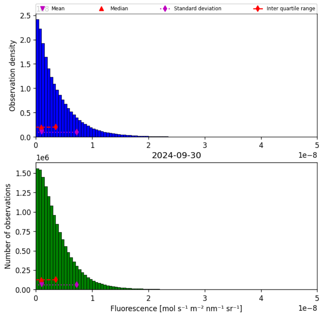
Figure 40: Histogram of “Fluorescence” for 2024-09-29 to 2024-10-01
