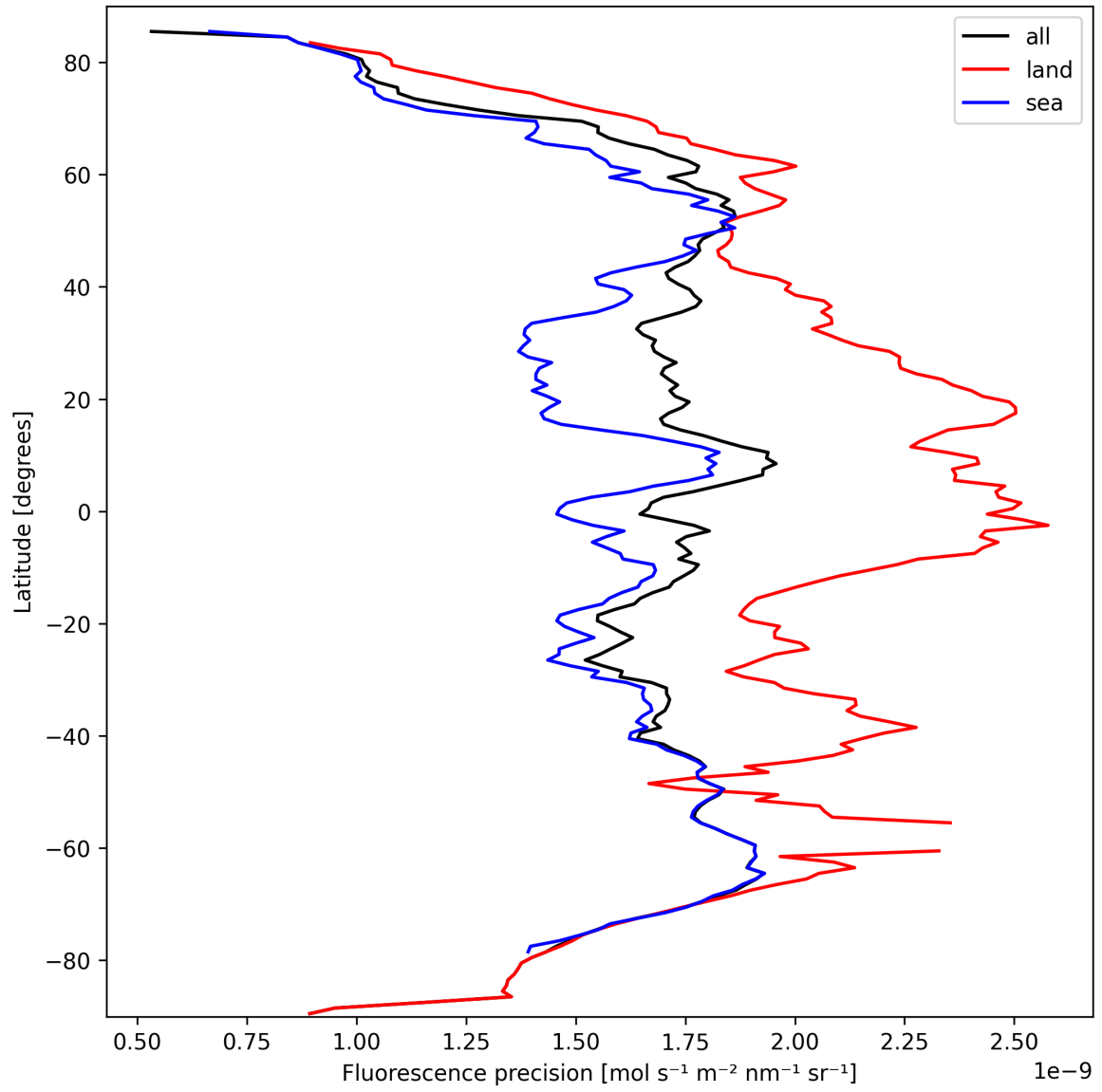
Figure 24: Zonal average of “Fluorescence precision” for 2024-09-29 to 2024-10-01.
