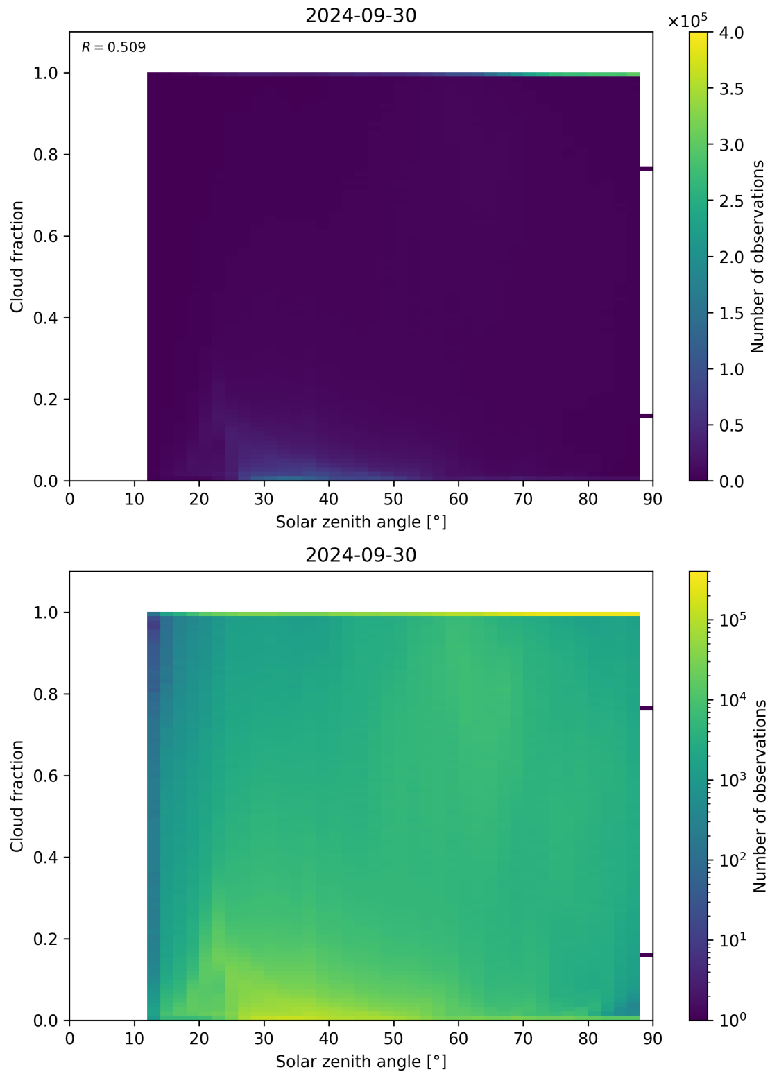
Figure 121: Scatter density plot of “Solar zenith angle” against “Cloud fraction” for 2024-09-29 to 2024-10-01.
