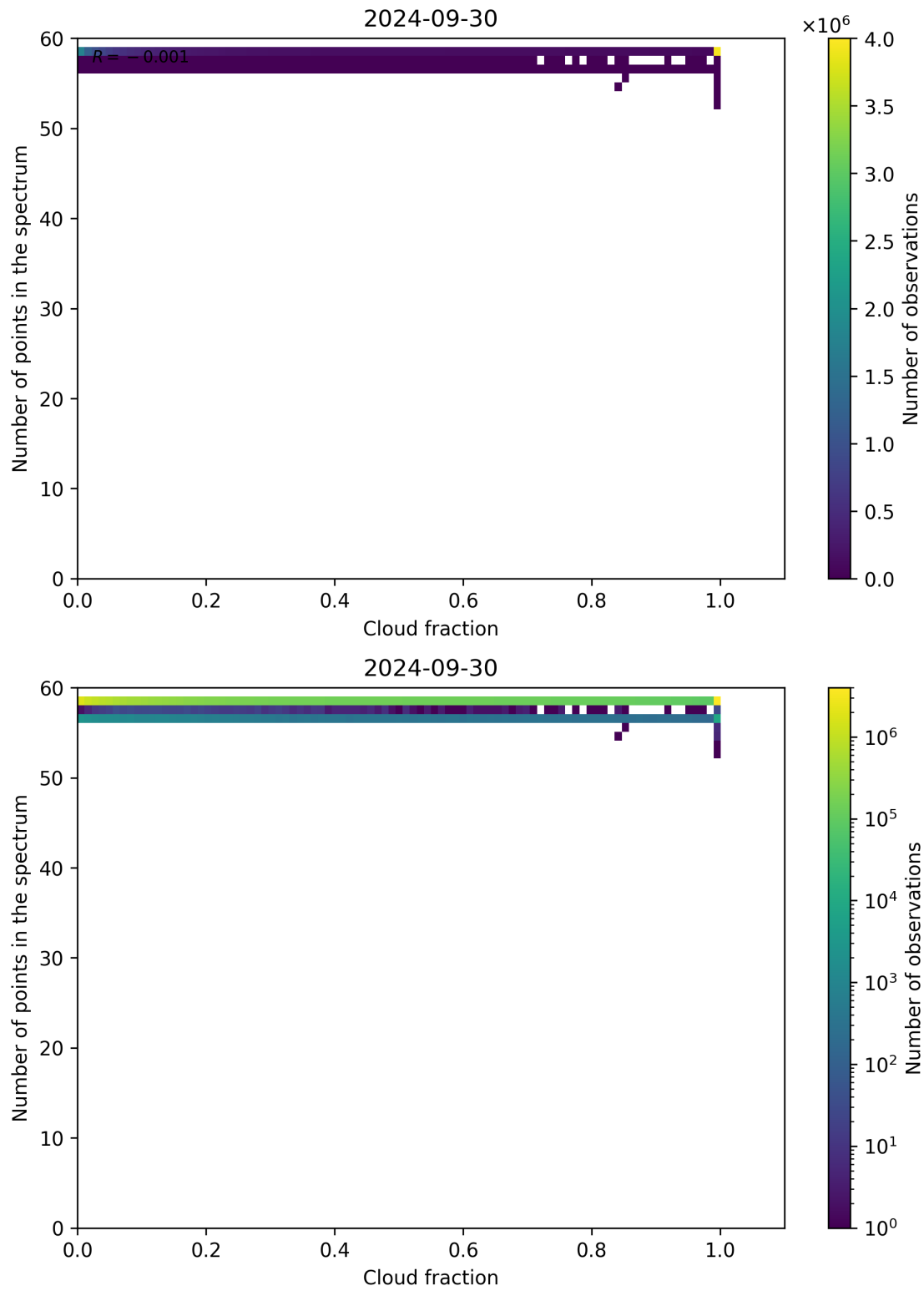
Figure 81: Scatter density plot of “Cloud fraction” against “Number of points in the spectrum” for 2024-09-29 to 2024-10-01.
