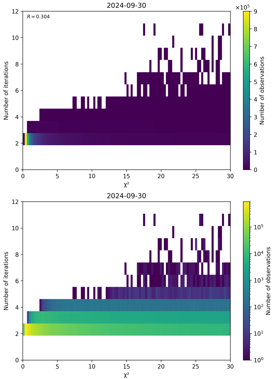
Figure 73: Scatter density plot of “ \chi^2 ” against “Number of iterations” for 2024-09-29 to 2024-10-01.
