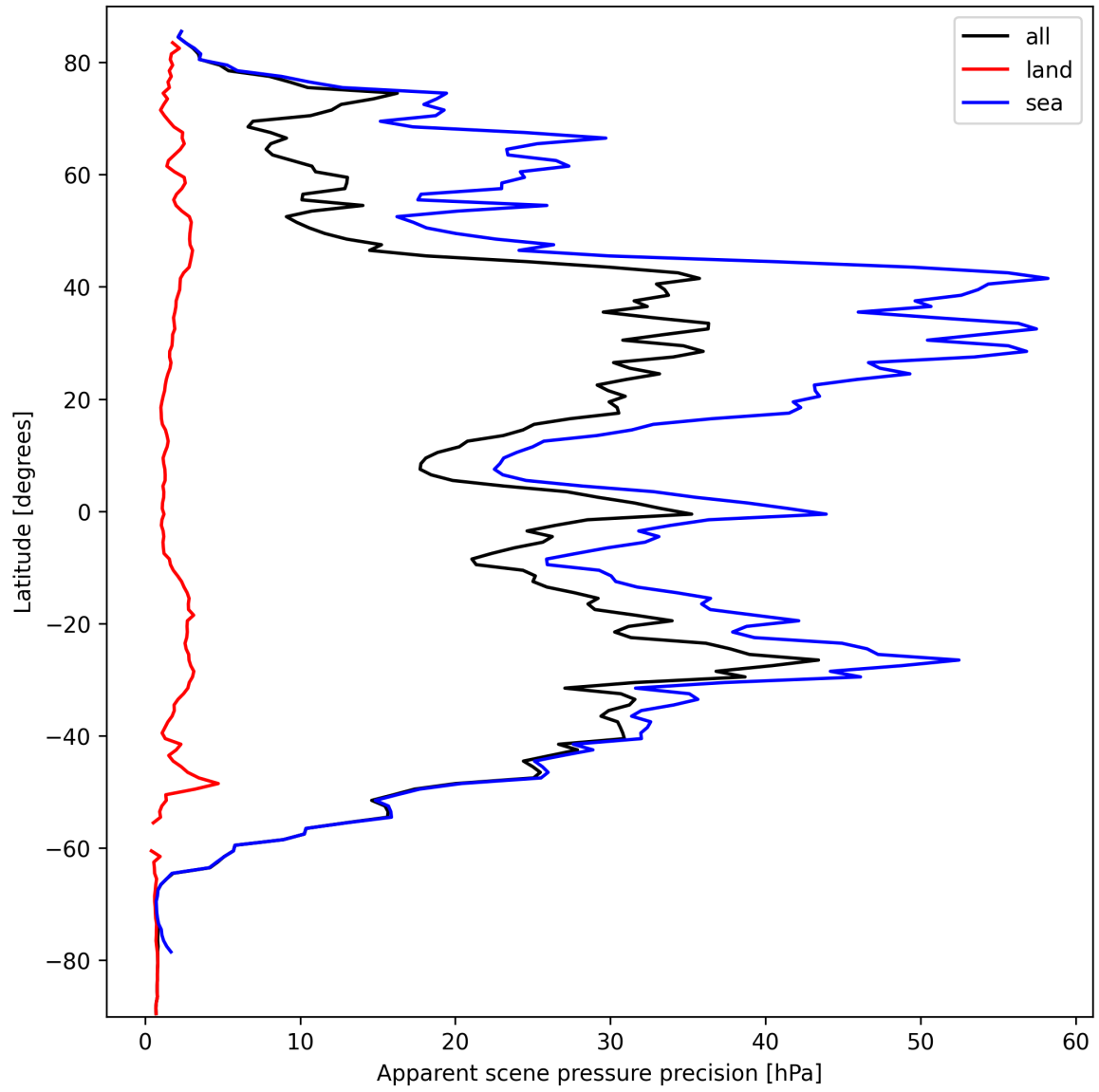
Figure 20: Zonal average of “Apparent scene pressure precision” for 2024-09-29 to 2024-10-01.
