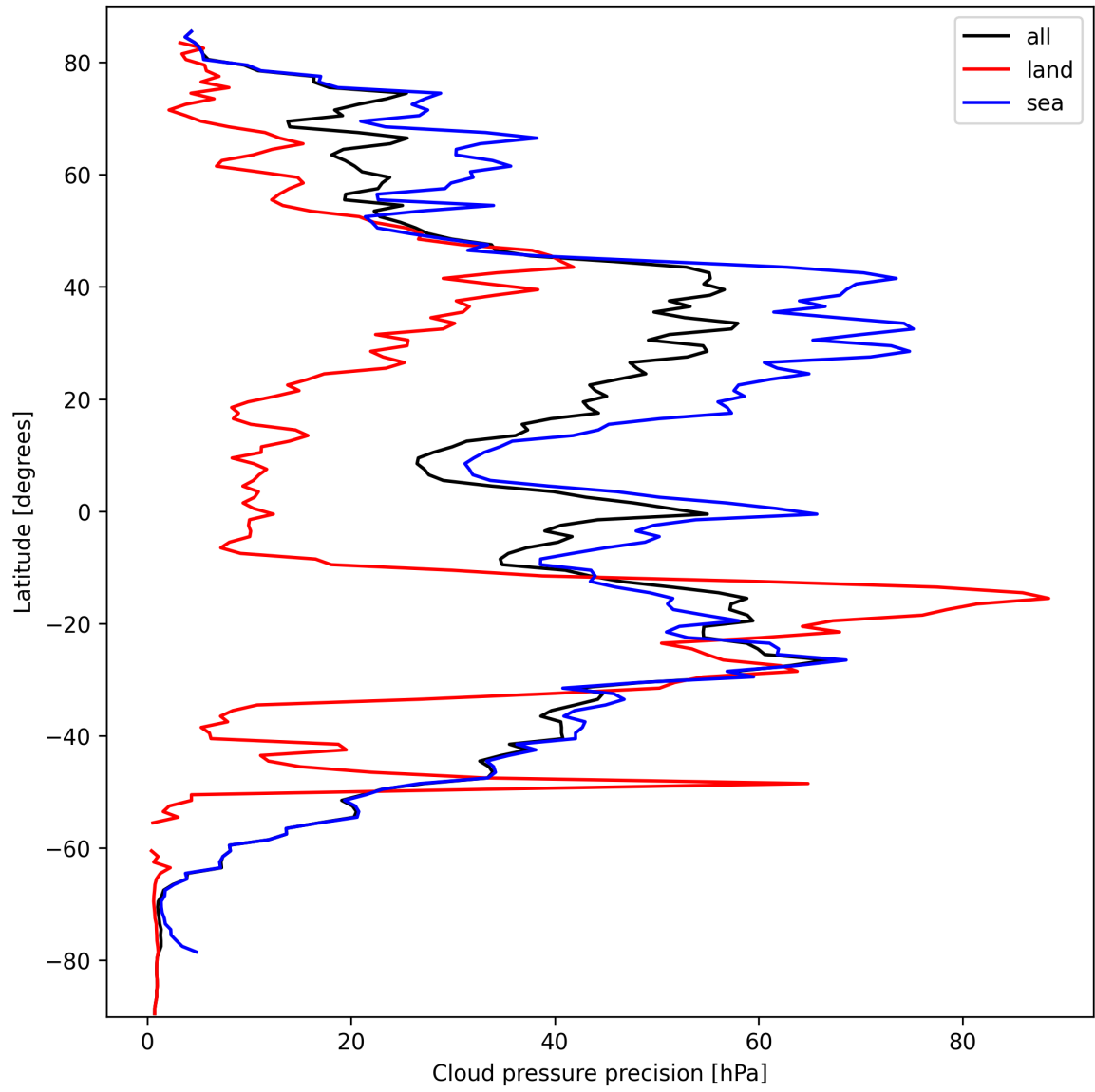
Figure 14: Zonal average of “Cloud pressure precision” for 2024-09-29 to 2024-10-01.
