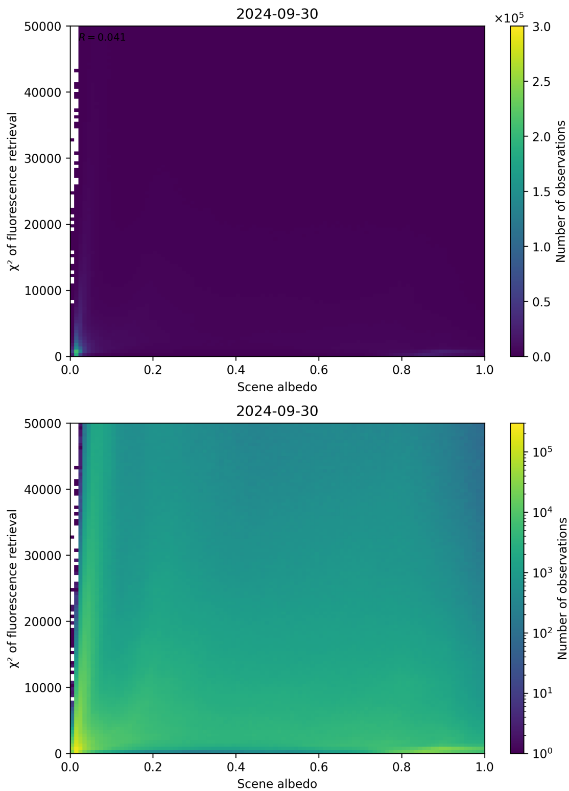
Figure 113: Scatter density plot of “Scene albedo” against “ \chi^2 of fluorescence retrieval” for 2024-09-29 to 2024-10-01.
