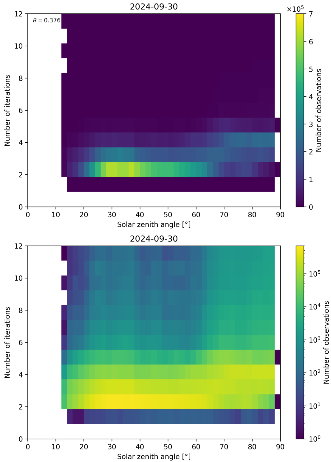
Figure 125: Scatter density plot of “Solar zenith angle” against “Number of iterations” for 2024-09-29 to 2024-10-01.
