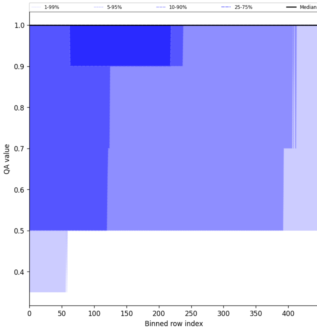
Figure 46: Along track statistics of “QA value” for 2024-09-29 to 2024-10-01
