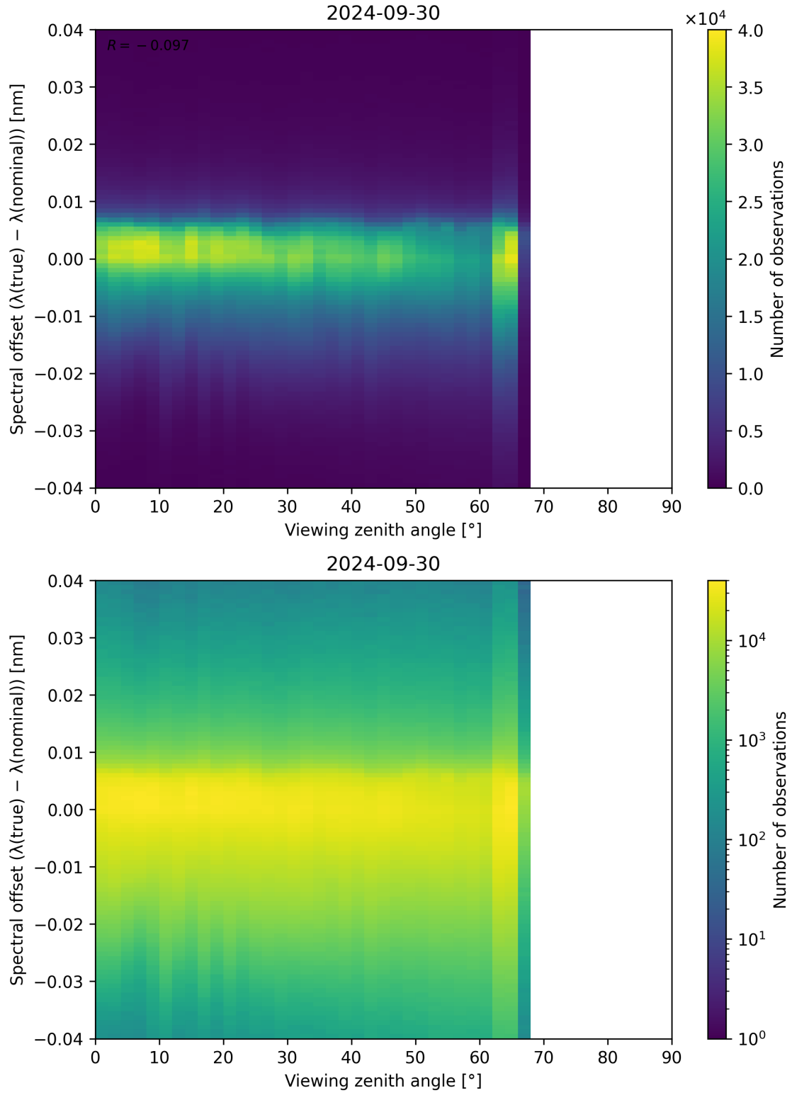
Figure 140: Scatter density plot of “Viewing zenith angle” against “Spectral offset ( \lambda_{\text{true}} - \lambda_{\text{nominal}} )” for 2024-09-29 to 2024-10-01.
