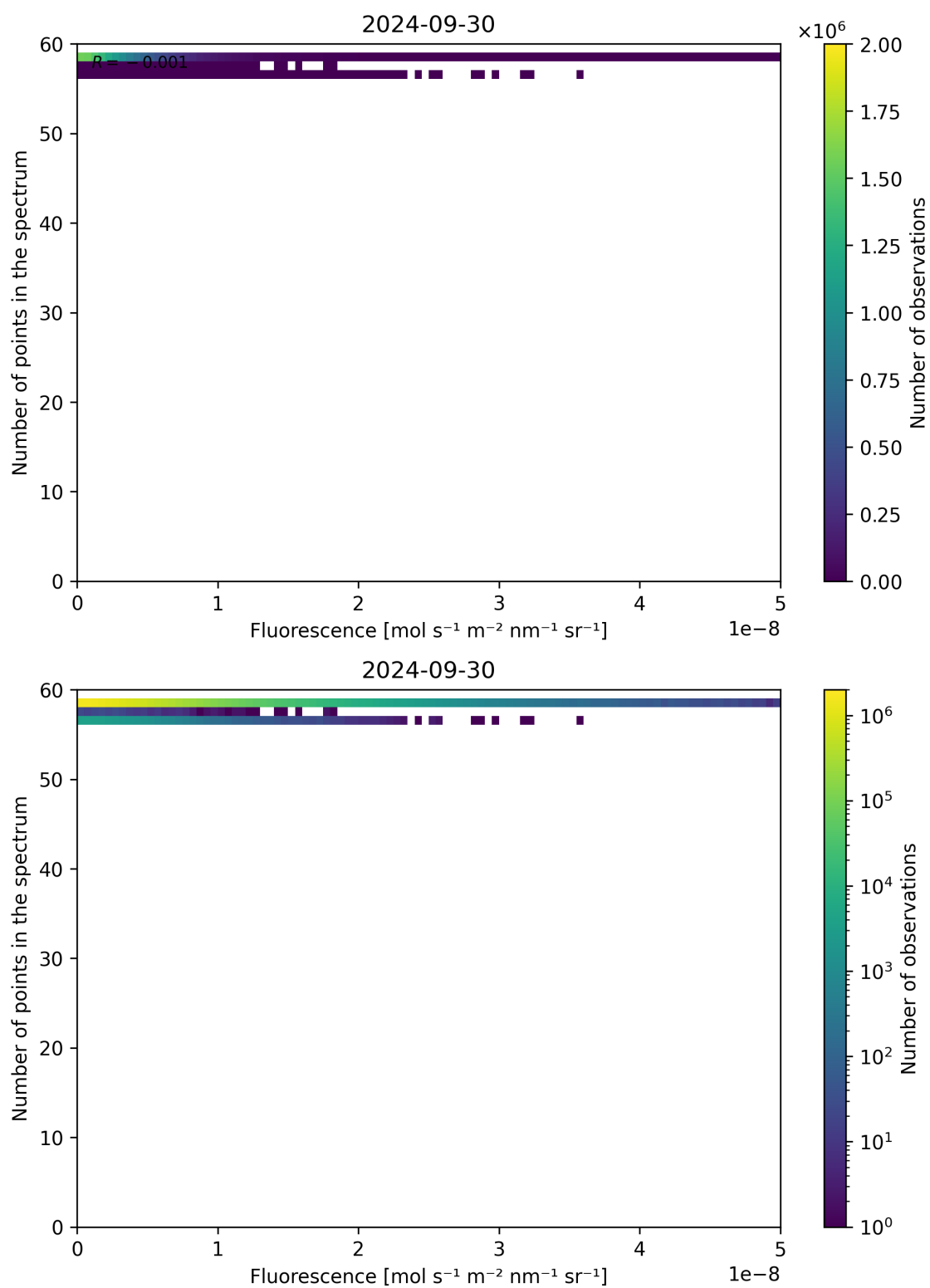
Figure 94: Scatter density plot of “Fluorescence” against “Number of points in the spectrum” for 2024-09-29 to 2024-10-01.
