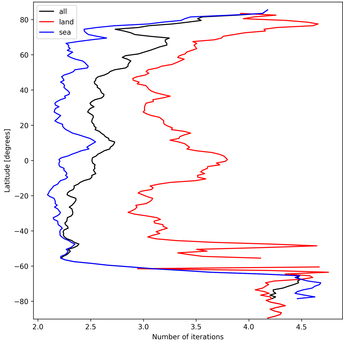
Figure 22: Zonal average of “Number of iterations” for 2024-09-29 to 2024-10-01.
