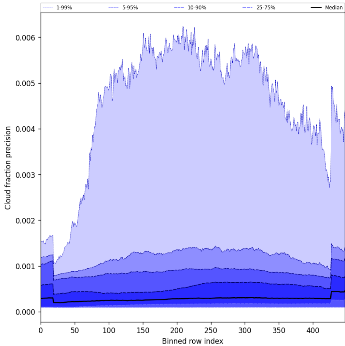
Figure 50: Along track statistics of “Cloud fraction precision” for 2024-09-29 to 2024-10-01
