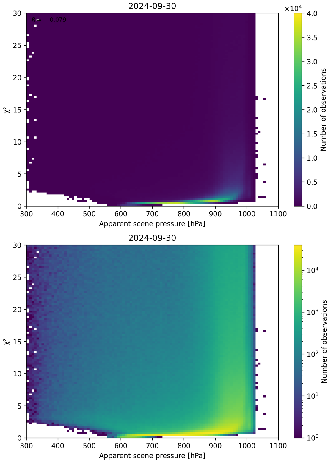
Figure 63: Scatter density plot of “Apparent scene pressure” against “ \chi^2 ” for 2024-09-29 to 2024-10-01.
