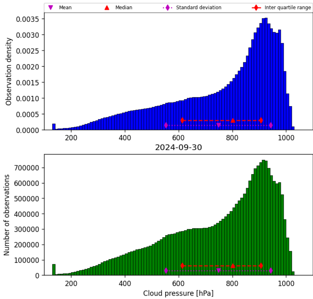
Figure 30: Histogram of “Cloud pressure” for 2024-09-29 to 2024-10-01
