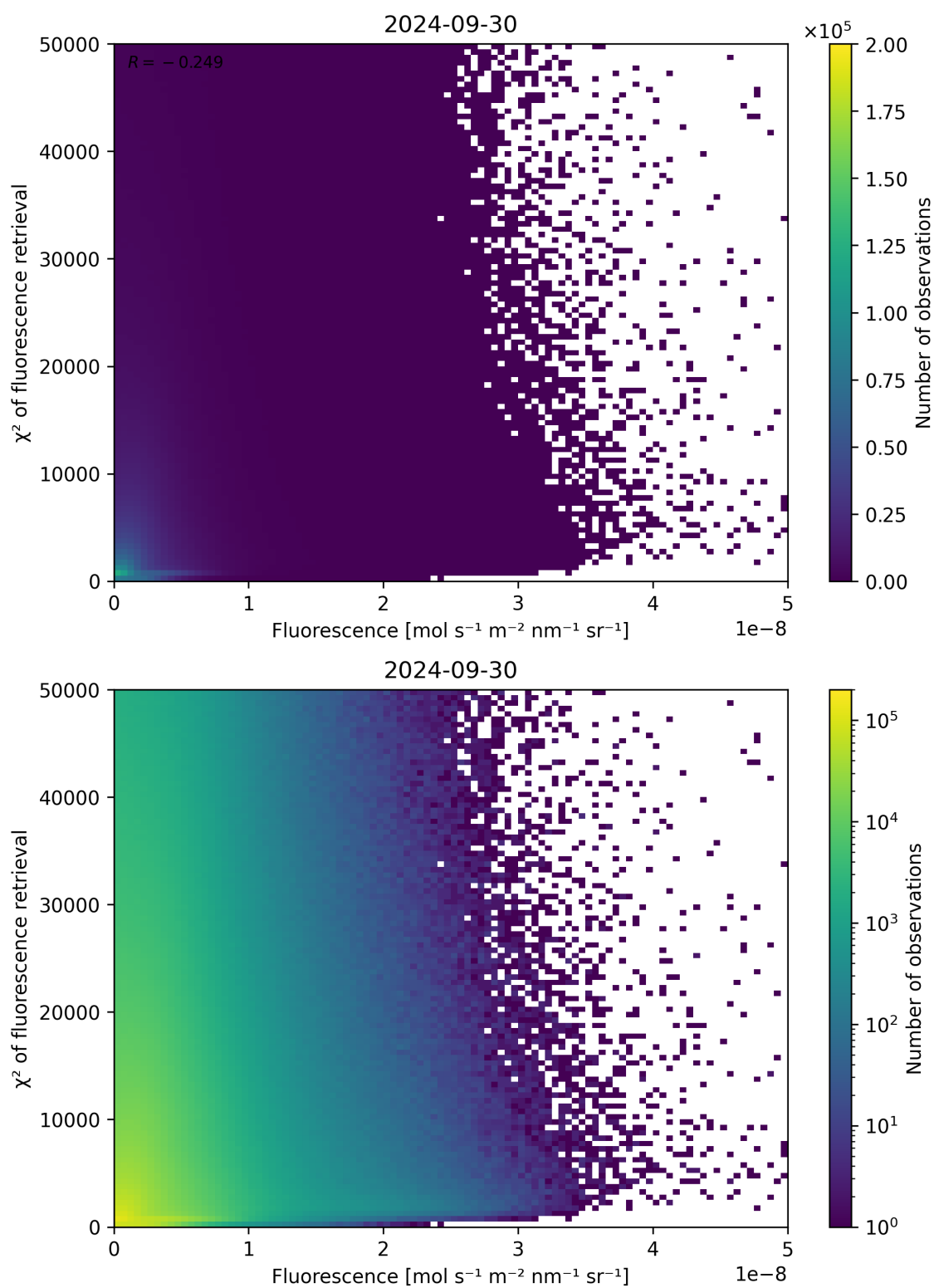
Figure 93: Scatter density plot of “Fluorescence” against “ \chi^2 of fluorescence retrieval” for 2024-09-29 to 2024-10-01.
