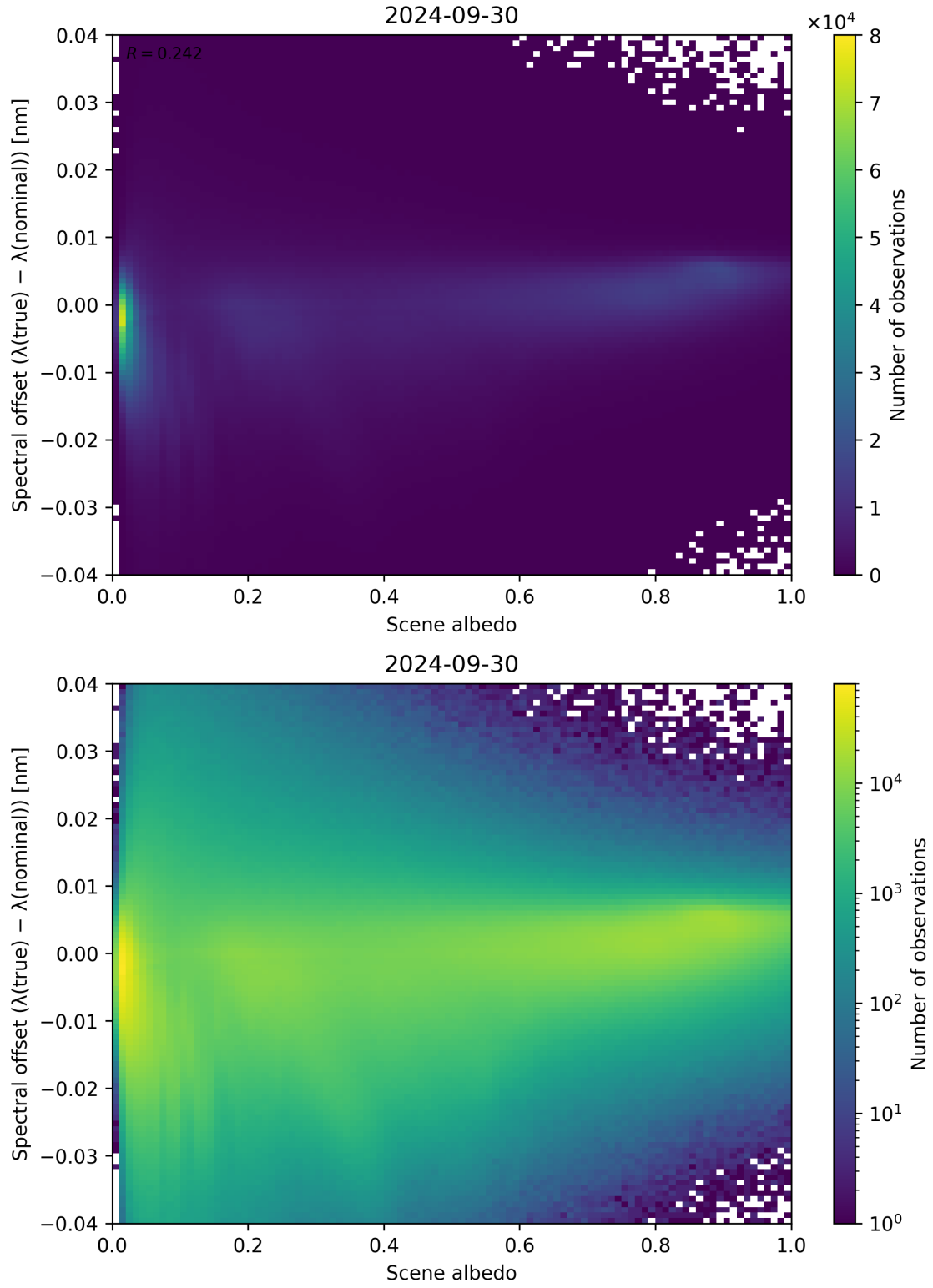
Figure 117: Scatter density plot of “Scene albedo” against “Spectral offset ( \lambda_{\text{true}} - \lambda_{\text{nominal}} )” for 2024-09-29 to 2024-10-01.
