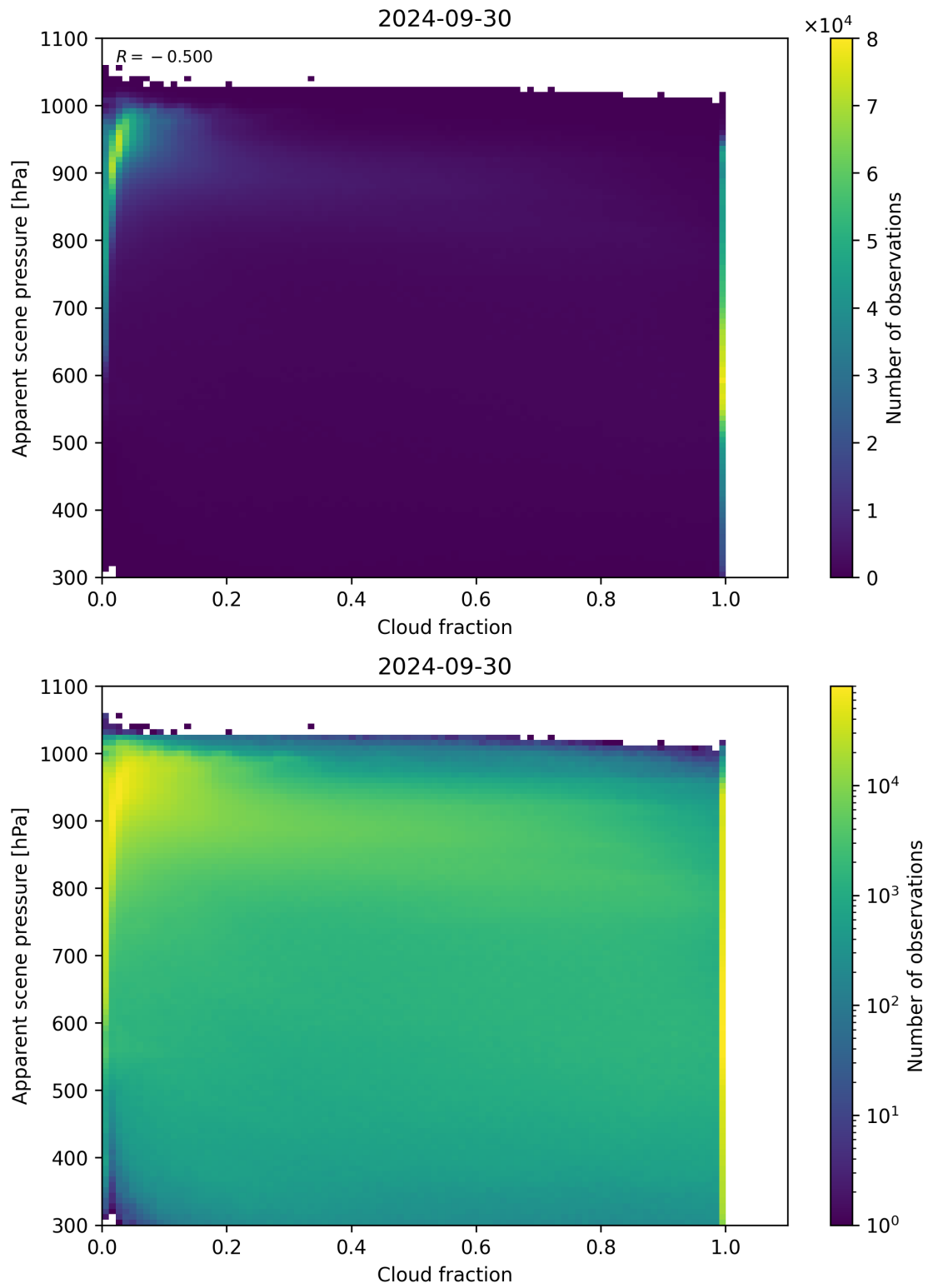
Figure 76: Scatter density plot of “Cloud fraction” against “Apparent scene pressure” for 2024-09-29 to 2024-10-01.
