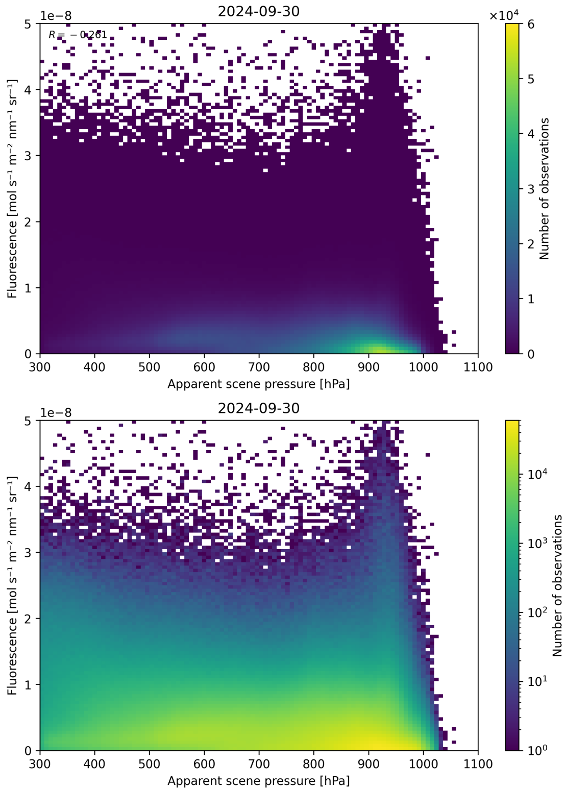
Figure 65: Scatter density plot of “Apparent scene pressure” against “Fluorescence” for 2024-09-29 to 2024-10-01.
