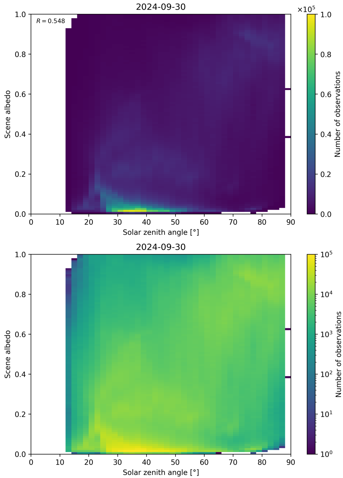
Figure 127: Scatter density plot of “Solar zenith angle” against “Scene albedo” for 2024-09-29 to 2024-10-01.
