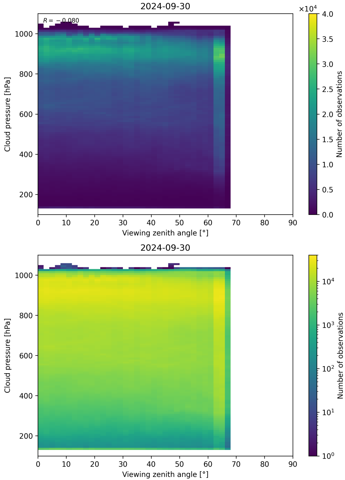
Figure 133: Scatter density plot of “Viewing zenith angle” against “Cloud pressure” for 2024-09-29 to 2024-10-01.
