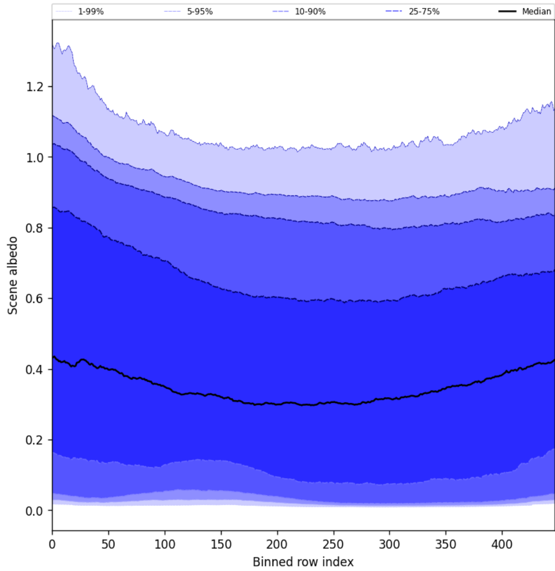
Figure 51: Along track statistics of “Scene albedo” for 2024-09-29 to 2024-10-01
