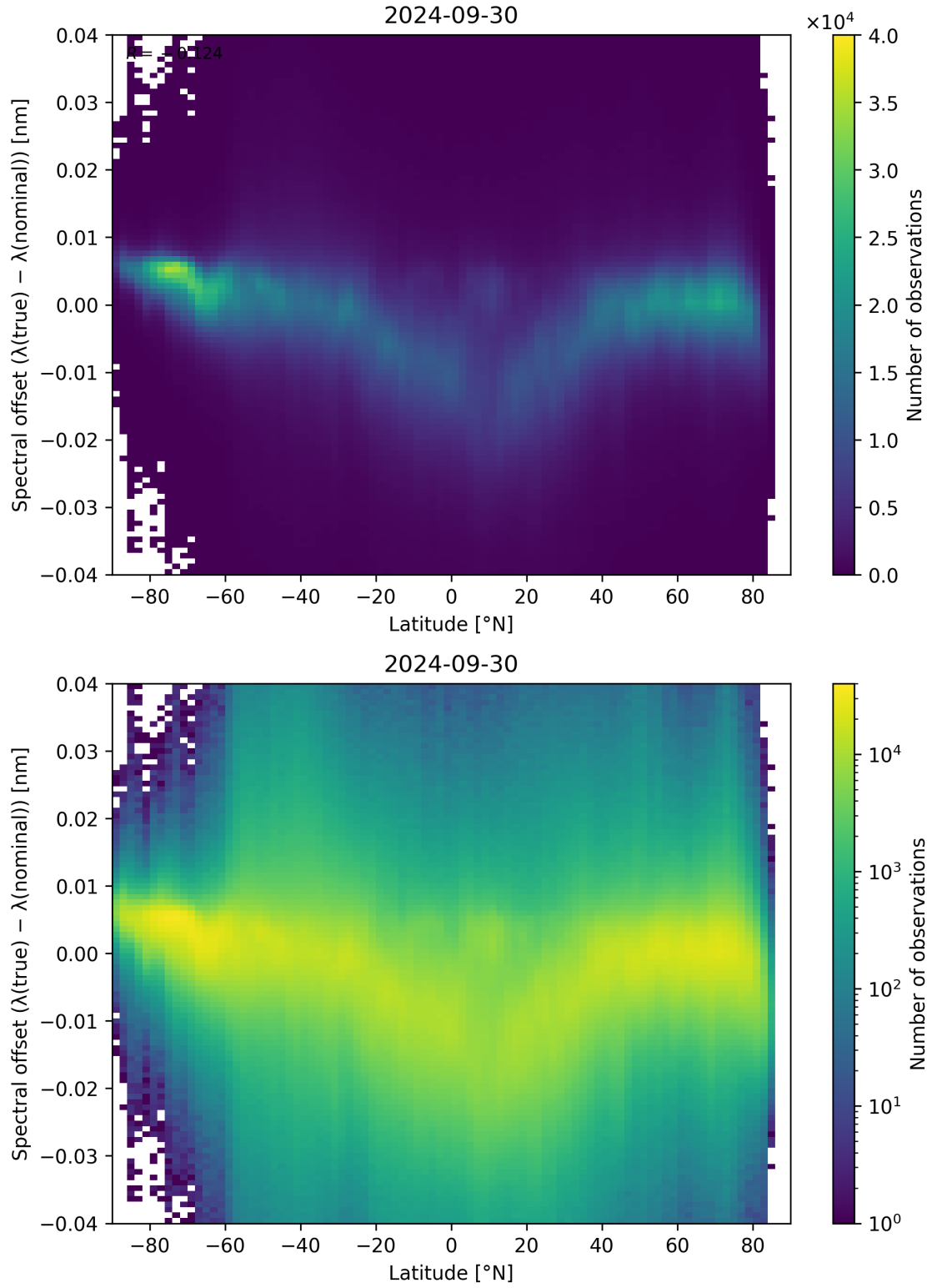
Figure 105: Scatter density plot of “Latitude” against “Spectral offset ( \lambda_{\text{true}} - \lambda_{\text{nominal}} )” for 2024-09-29 to 2024-10-01.
