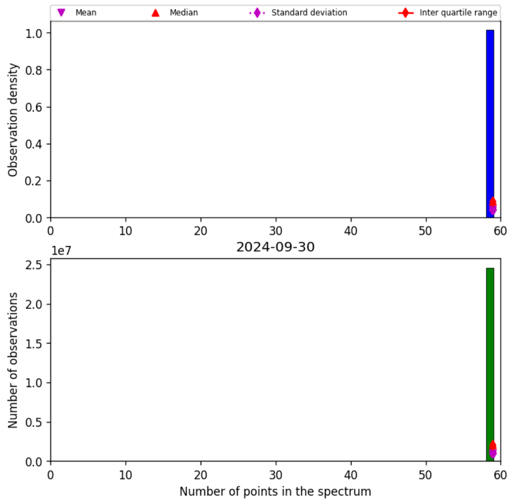
Figure 44: Histogram of “Number of points in the spectrum” for 2024-09-29 to 2024-10-01
