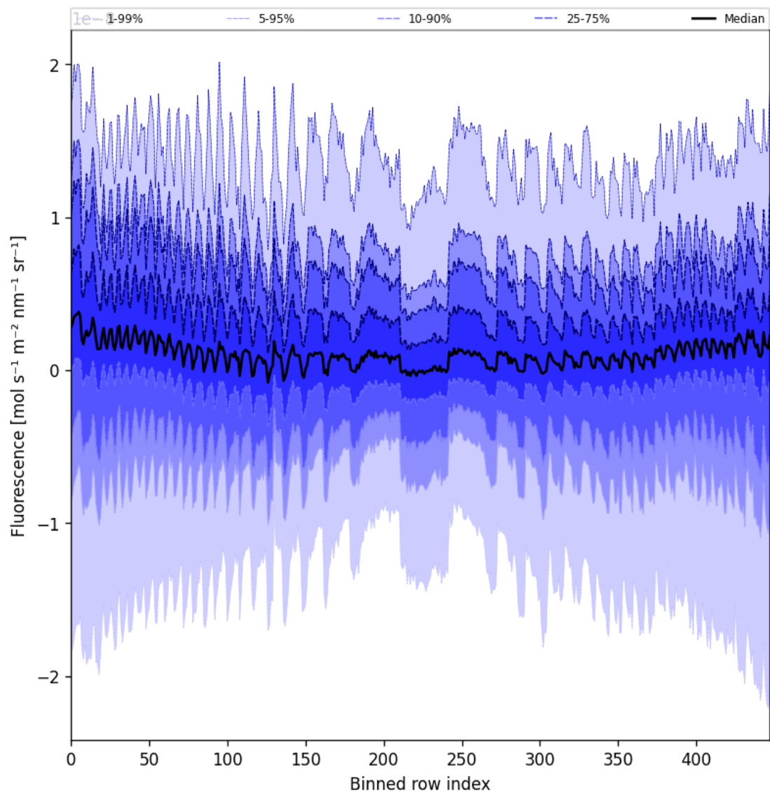
Figure 57: Along track statistics of "Fluorescence" for 2024-09-29 to 2024-10-01
