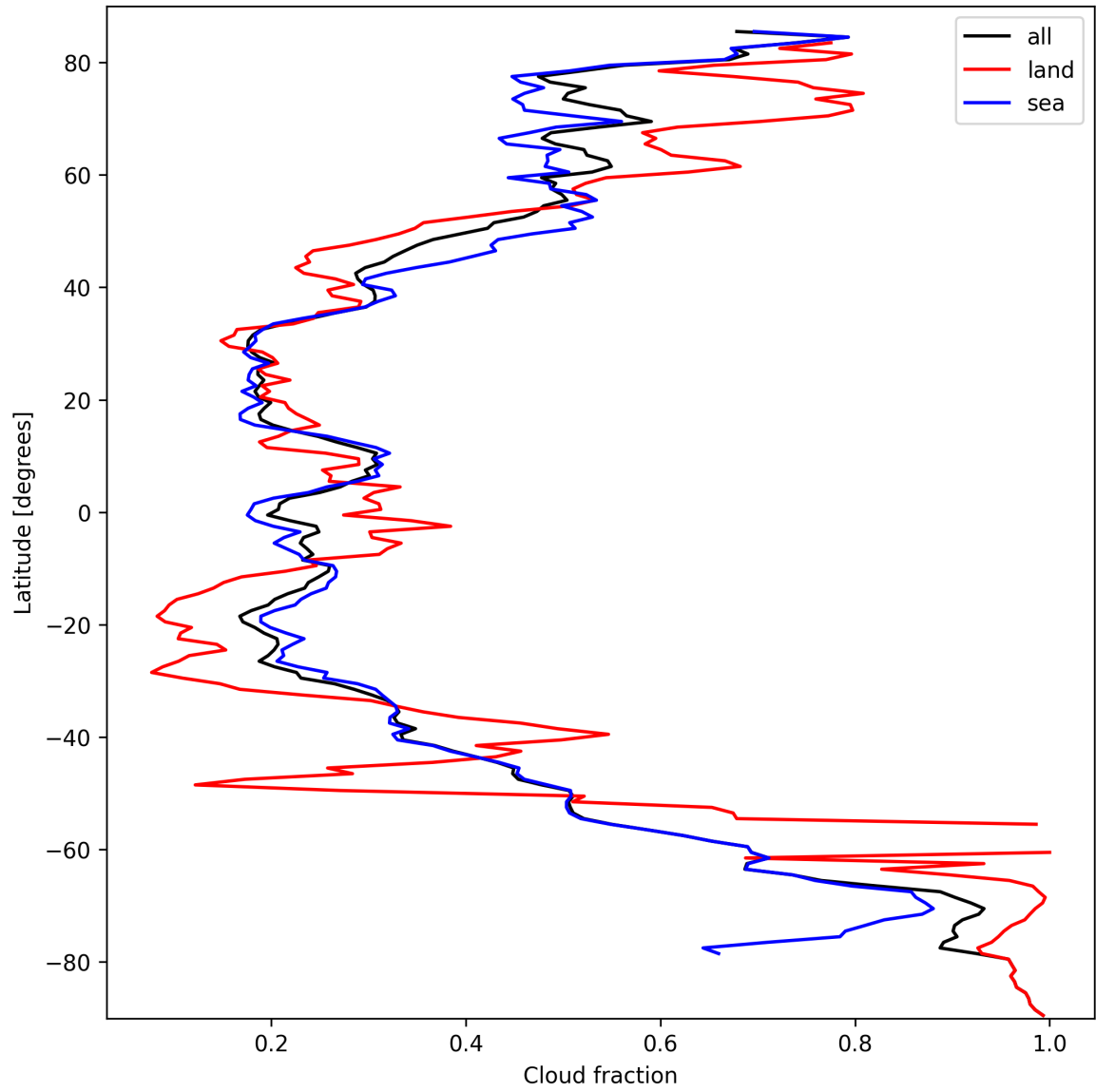
Figure 15: Zonal average of “Cloud fraction” for 2024-09-29 to 2024-10-01.
