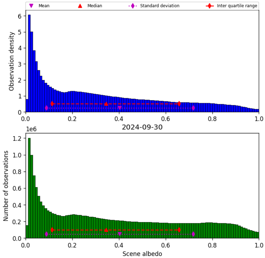
Figure 34: Histogram of “Scene albedo” for 2024-09-29 to 2024-10-01
