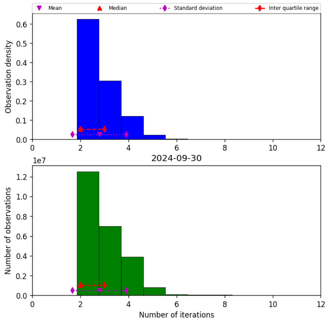
Figure 39: Histogram of “Number of iterations” for 2024-09-29 to 2024-10-01
