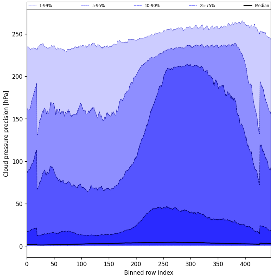
Figure 48: Along track statistics of “Cloud pressure precision” for 2024-09-29 to 2024-10-01
