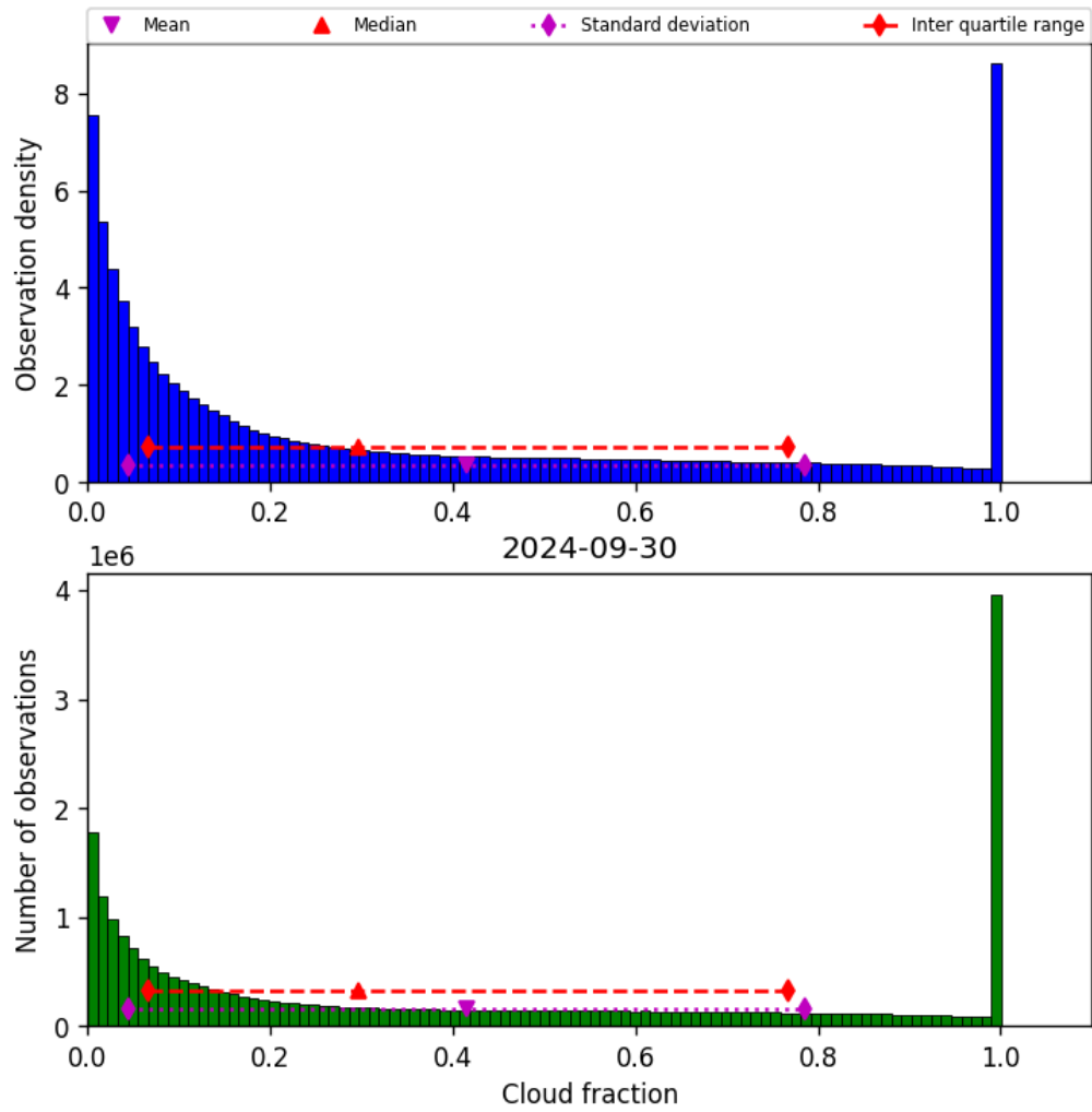
Figure 32: Histogram of “Cloud fraction” for 2024-09-29 to 2024-10-01
