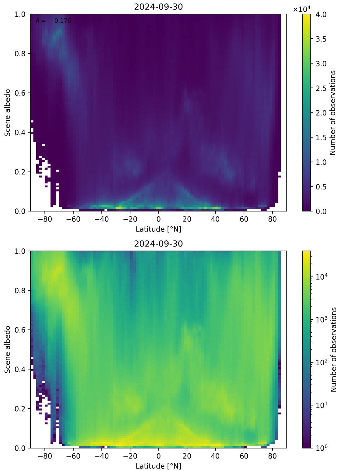
Figure 104: Scatter density plot of “Latitude” against “Scene albedo” for 2024-09-29 to 2024-10-01.
