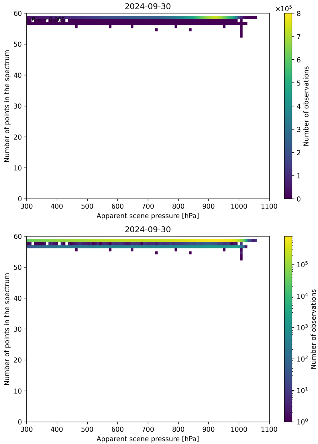
Figure 67: Scatter density plot of “Apparent scene pressure” against “Number of points in the spectrum” for 2024-09-29 to 2024-10-01.
