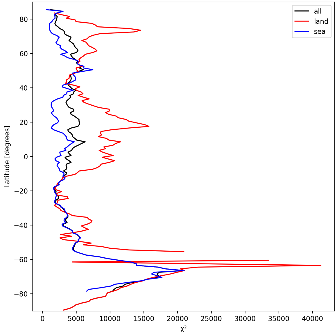
Figure 21: Zonal average of “ \chi^2 ” for 2024-09-29 to 2024-10-01.
