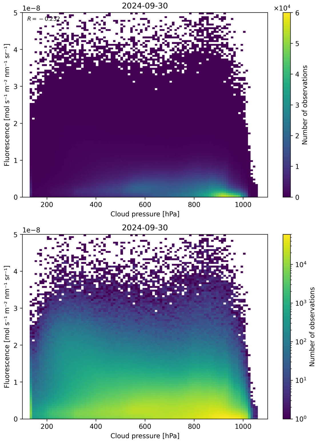
Figure 88: Scatter density plot of “Cloud pressure” against “Fluorescence” for 2024-09-29 to 2024-10-01.
