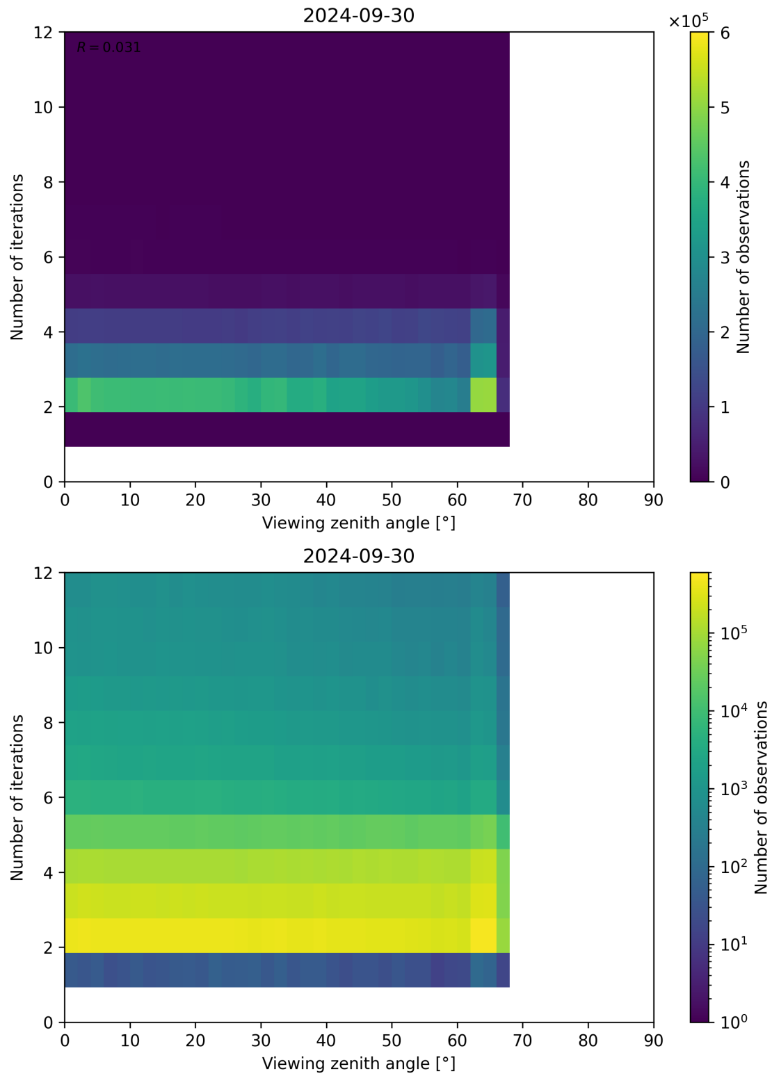
Figure 136: Scatter density plot of “Viewing zenith angle” against “Number of iterations” for 2024-09-29 to 2024-10-01.
