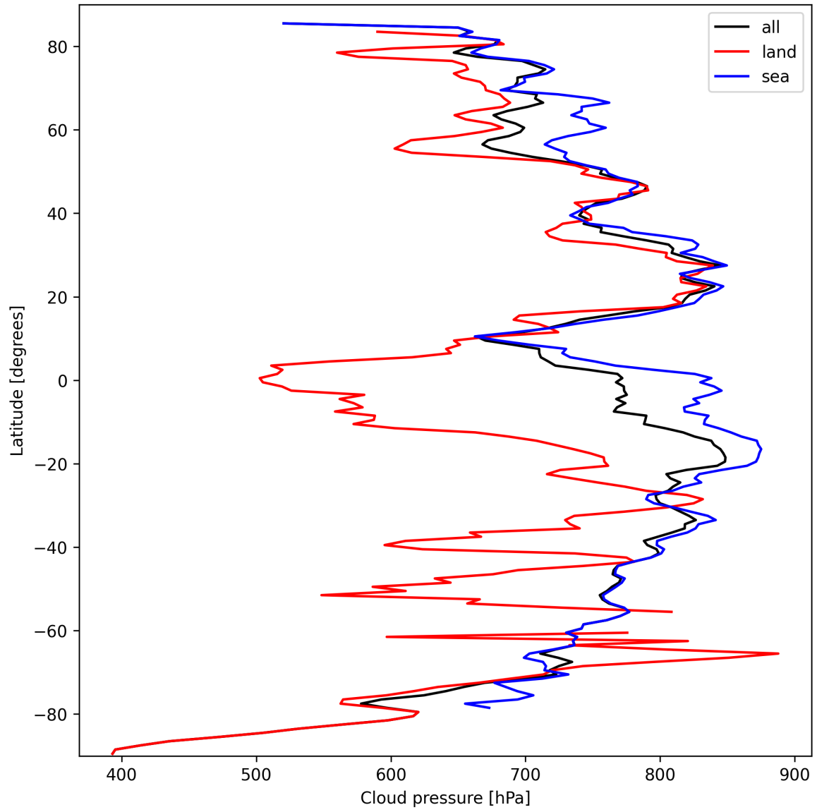
Figure 13: Zonal average of “Cloud pressure” for 2024-09-29 to 2024-10-01.
