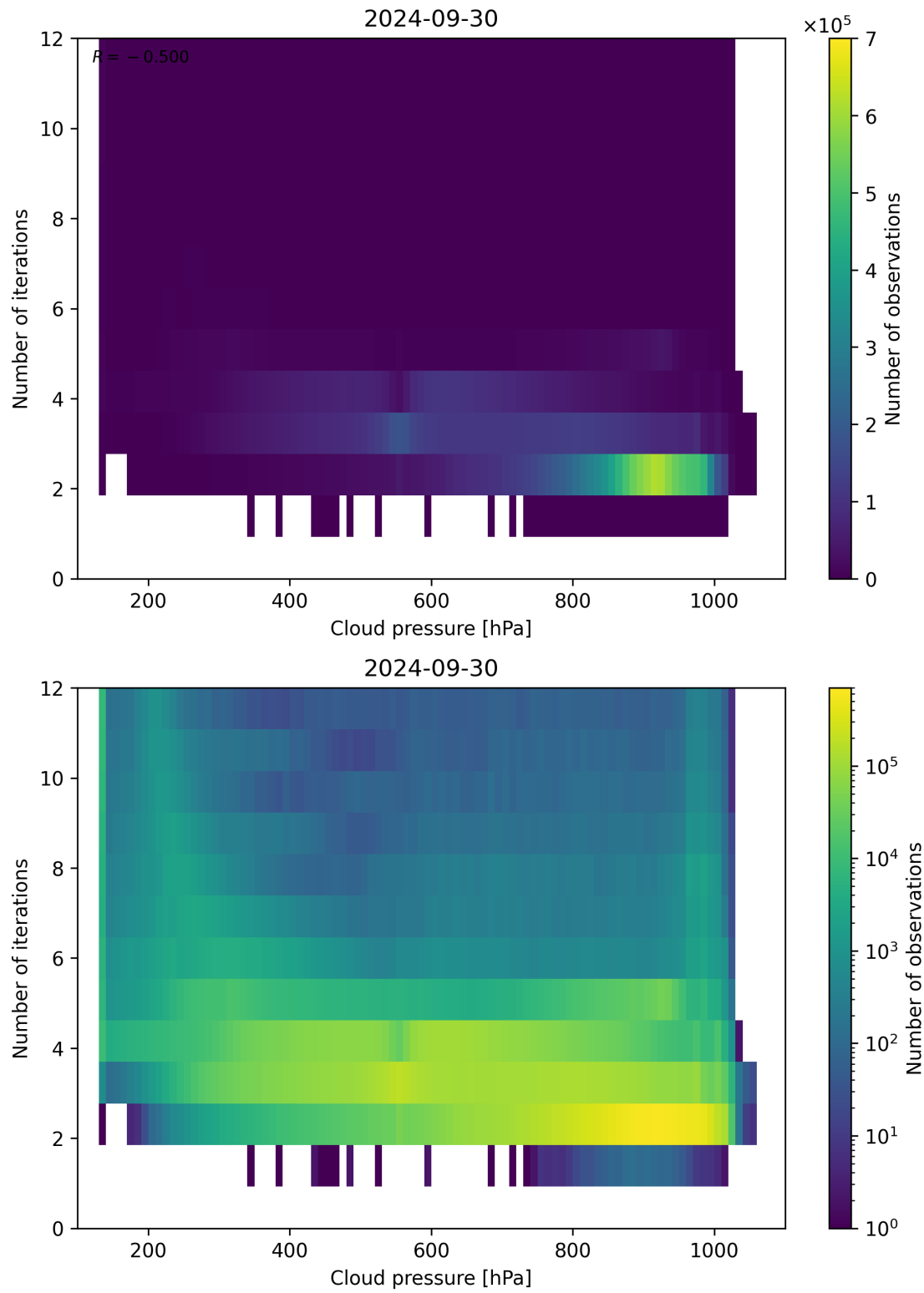
Figure 89: Scatter density plot of “Cloud pressure” against “Number of iterations” for 2024-09-29 to 2024-10-01.
