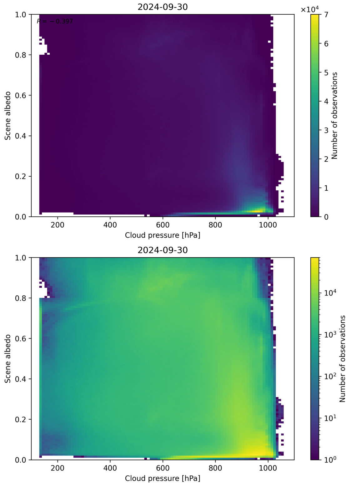
Figure 91: Scatter density plot of “Cloud pressure” against “Scene albedo” for 2024-09-29 to 2024-10-01.
