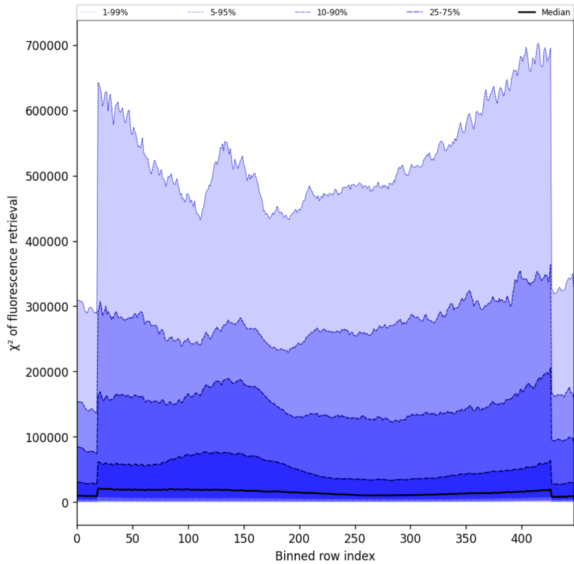
Figure 59: Along track statistics of “ \chi^2 of fluorescence retrieval” for 2024-09-29 to 2024-10-01
