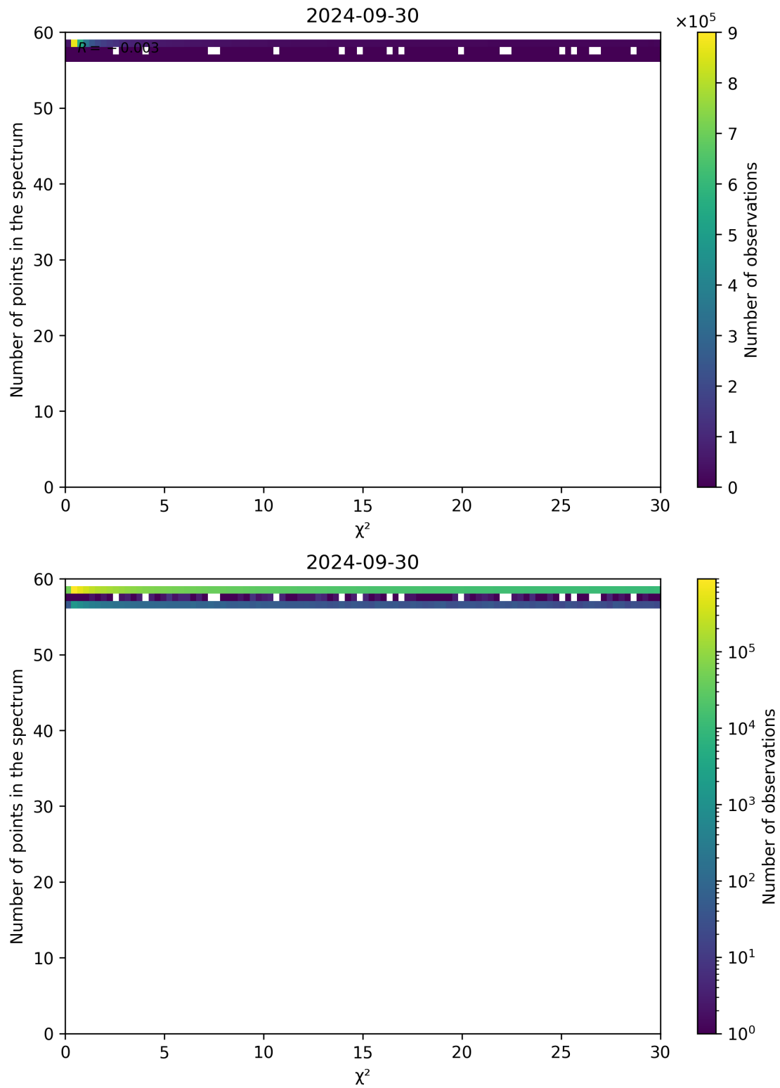
Figure 74: Scatter density plot of " \chi^2 " against "Number of points in the spectrum" for 2024-09-29 to 2024-10-01.
