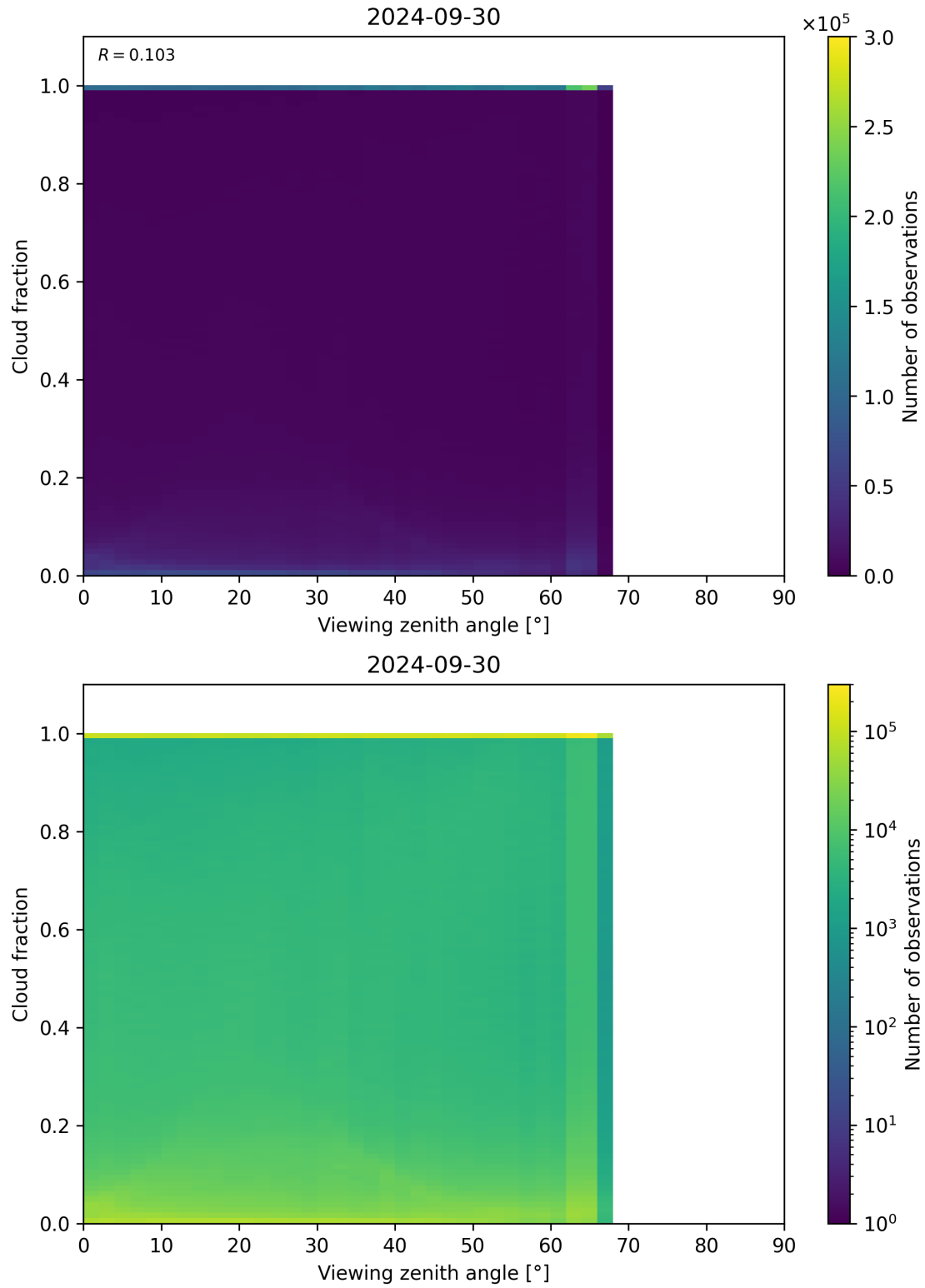
Figure 132: Scatter density plot of “Viewing zenith angle” against “Cloud fraction” for 2024-09-29 to 2024-10-01.
