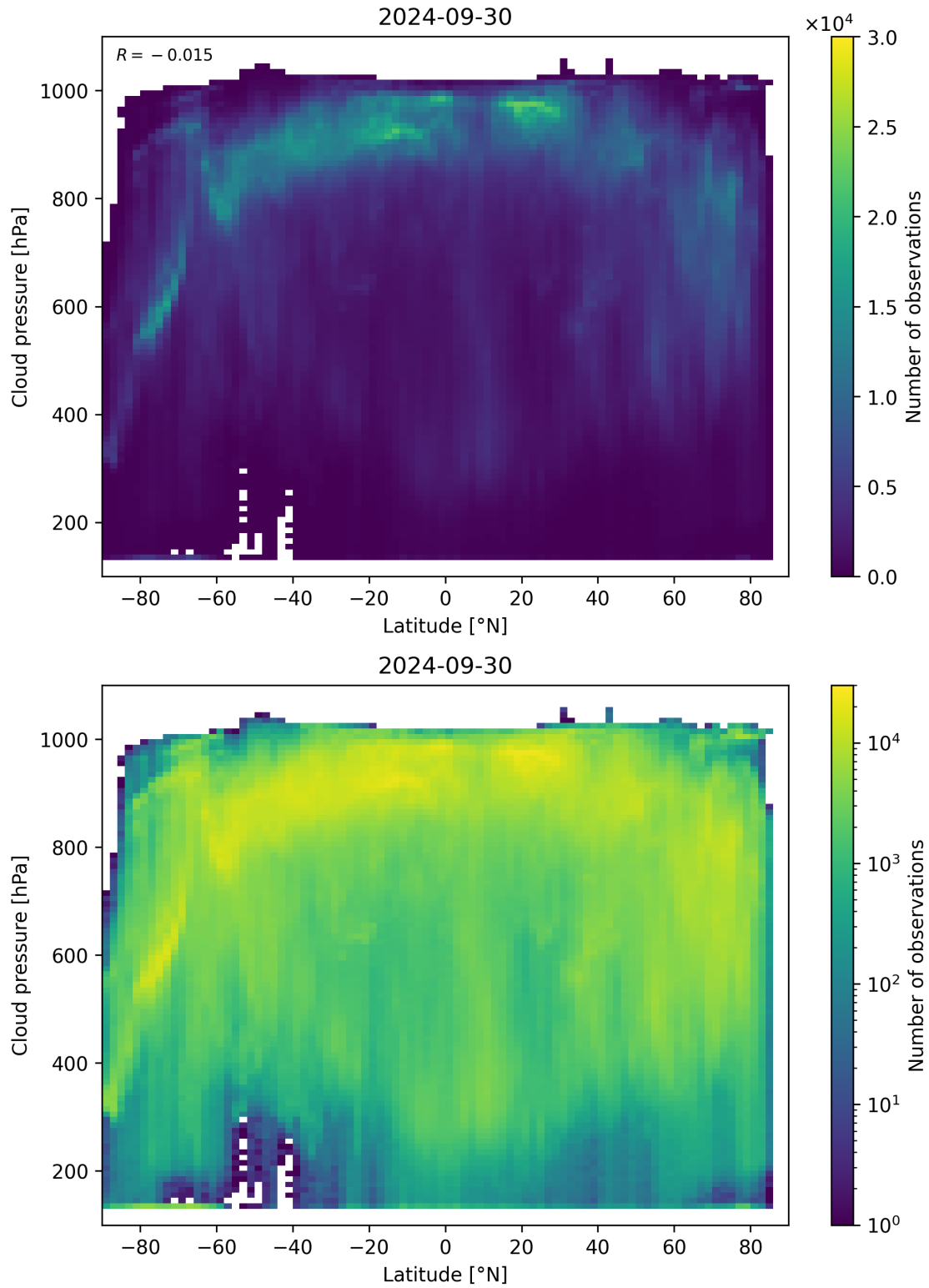
Figure 100: Scatter density plot of “Latitude” against “Cloud pressure” for 2024-09-29 to 2024-10-01.
