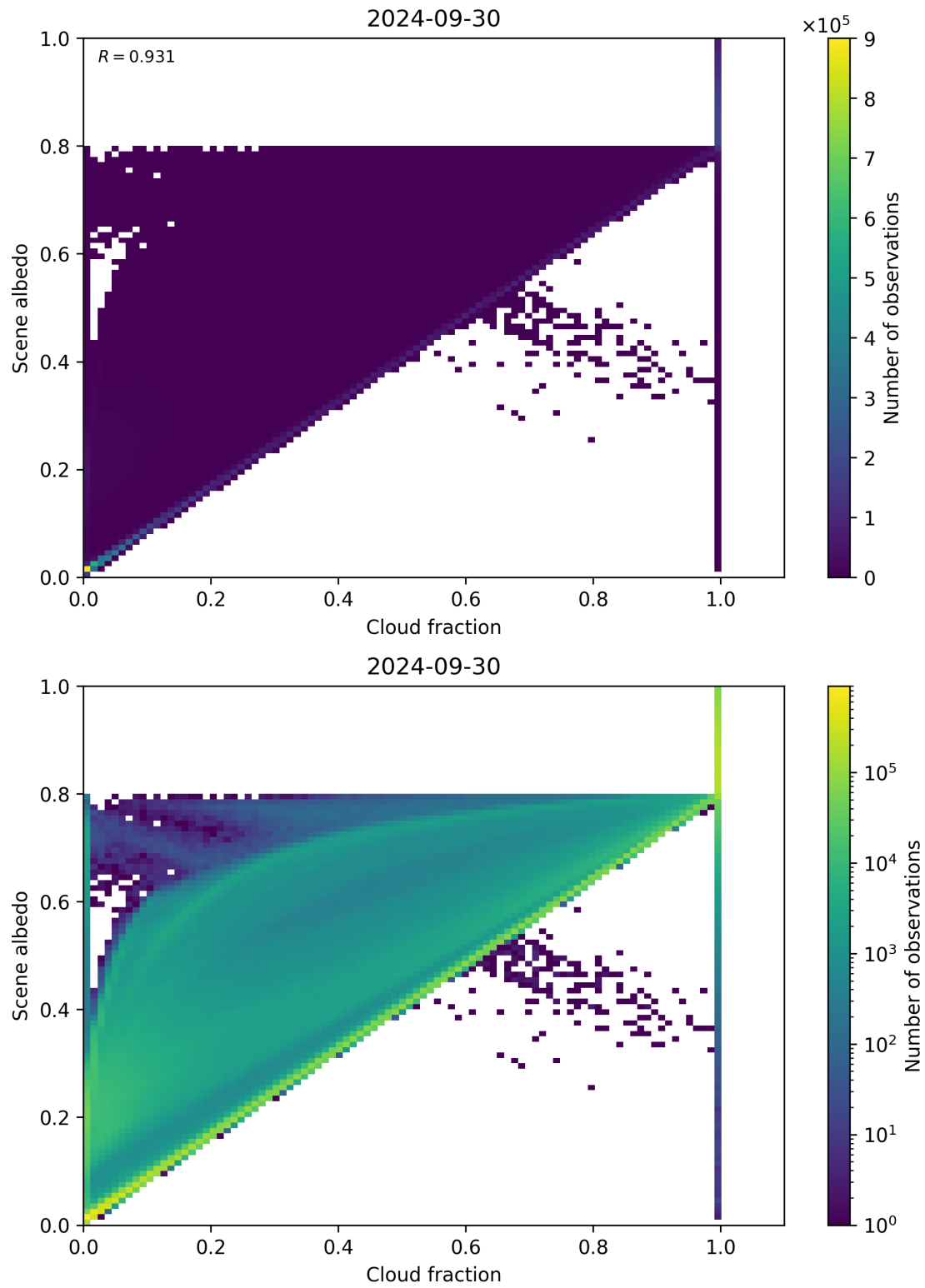
Figure 82: Scatter density plot of “Cloud fraction” against “Scene albedo” for 2024-09-29 to 2024-10-01.
