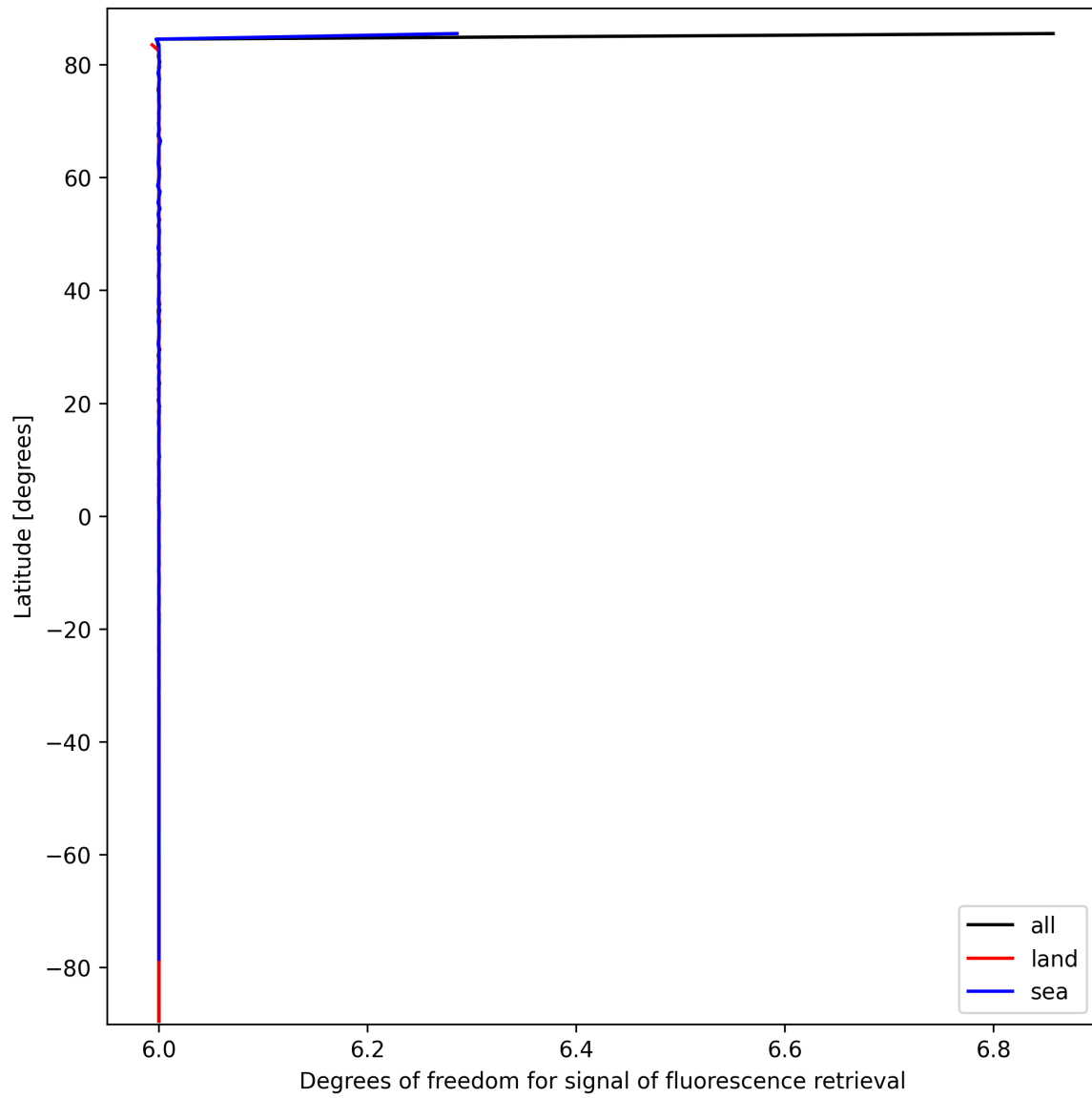
Figure 26: Zonal average of “Degrees of freedom for signal of fluorescence retrieval” for 2024-09-29 to 2024-10-01.
