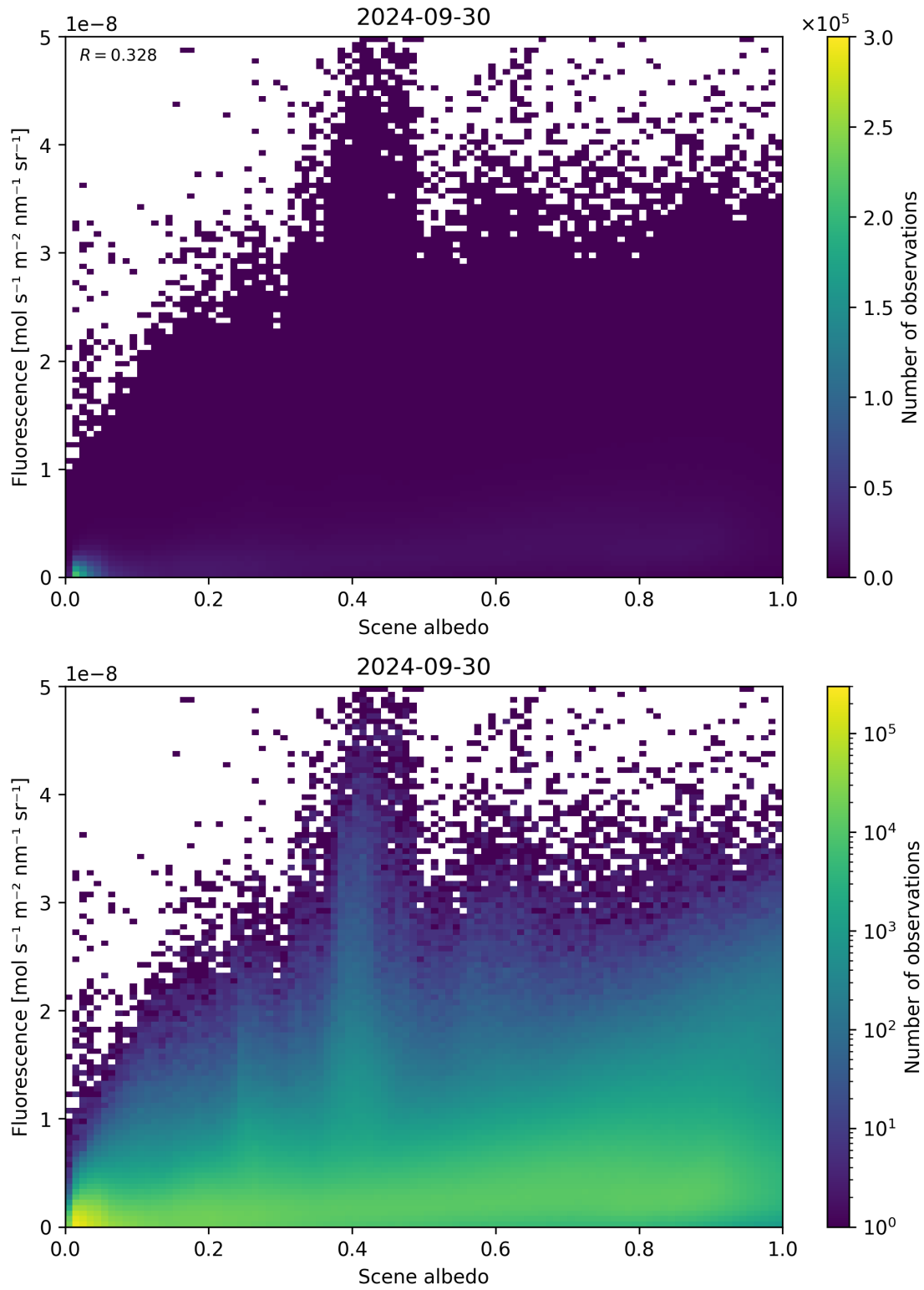
Figure 114: Scatter density plot of “Scene albedo” against “Fluorescence” for 2024-09-29 to 2024-10-01.
