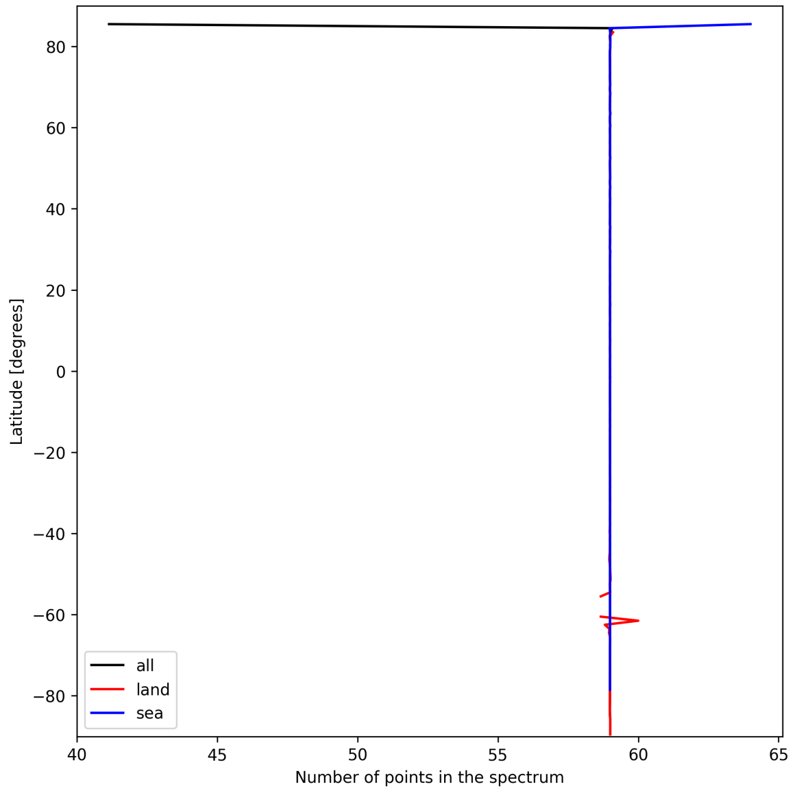
Figure 27: Zonal average of “Number of points in the spectrum” for 2024-09-29 to 2024-10-01.
