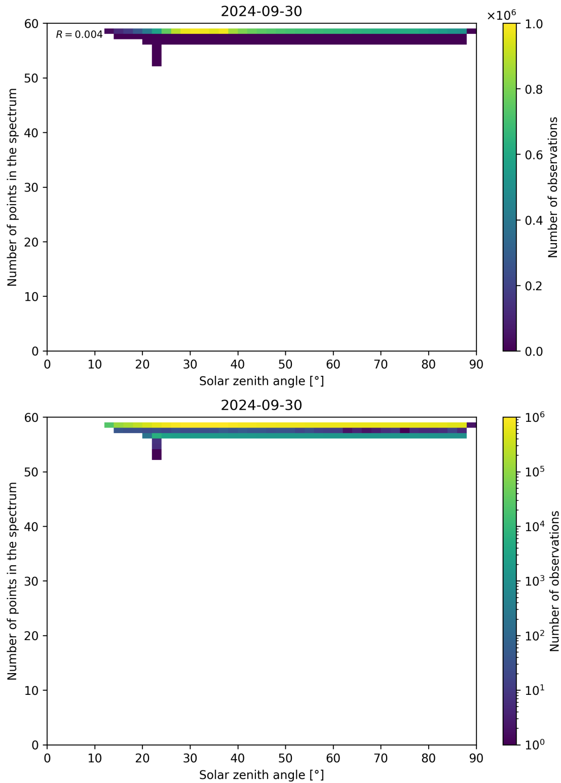
Figure 126: Scatter density plot of “Solar zenith angle” against “Number of points in the spectrum” for 2024-09-29 to 2024-10-01.
