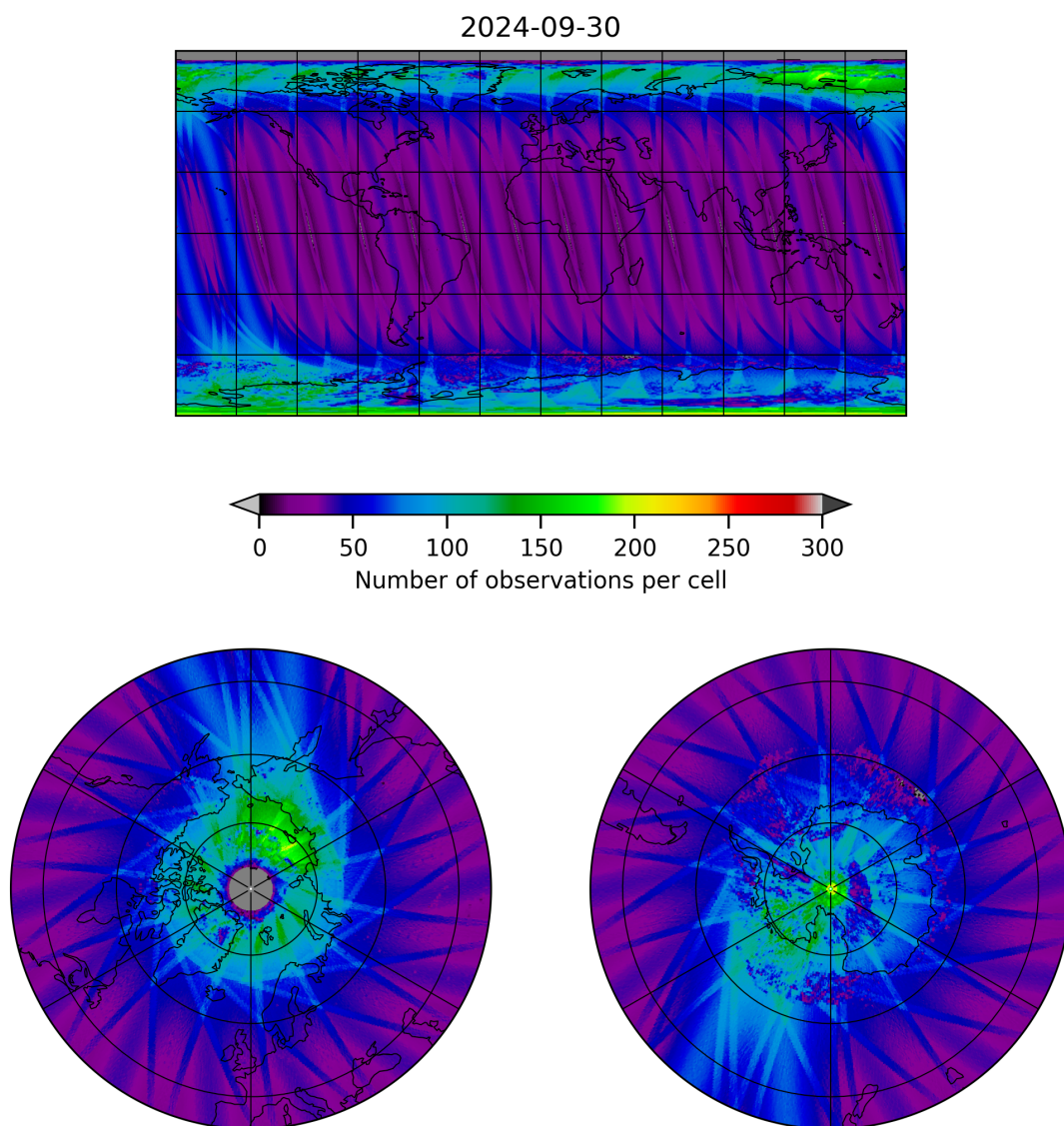
Figure 11: Map of the number of observations for 2024-09-29 to 2024-10-01
