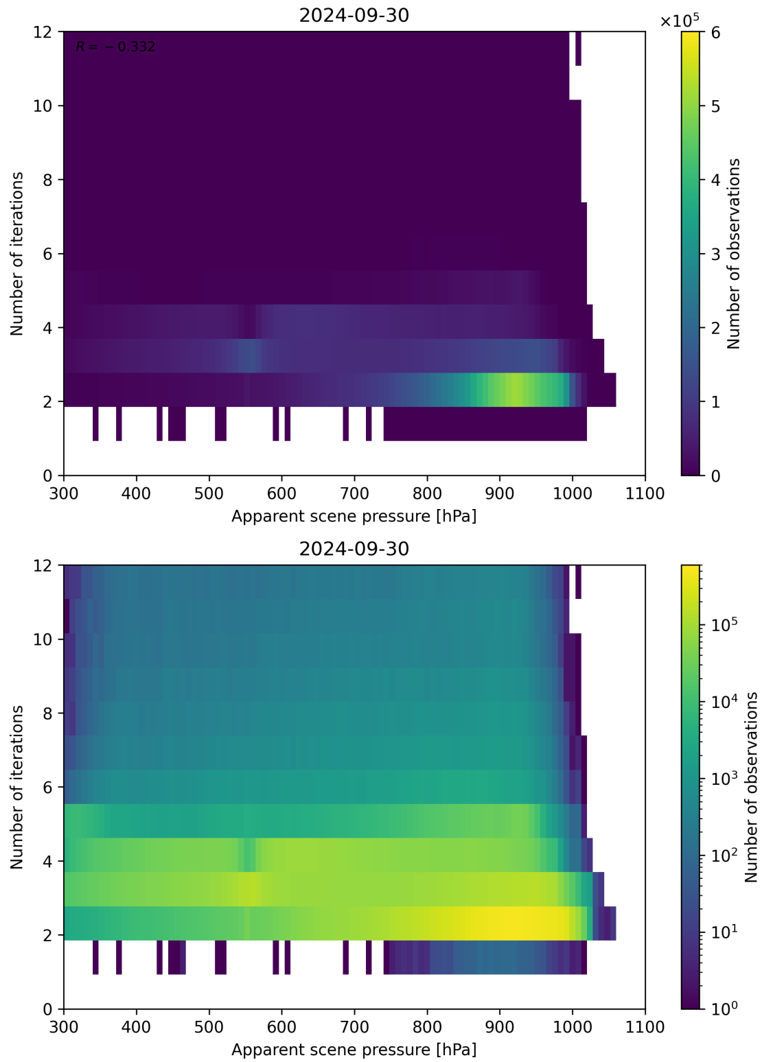
Figure 66: Scatter density plot of “Apparent scene pressure” against “Number of iterations” for 2024-09-29 to 2024-10-01.
