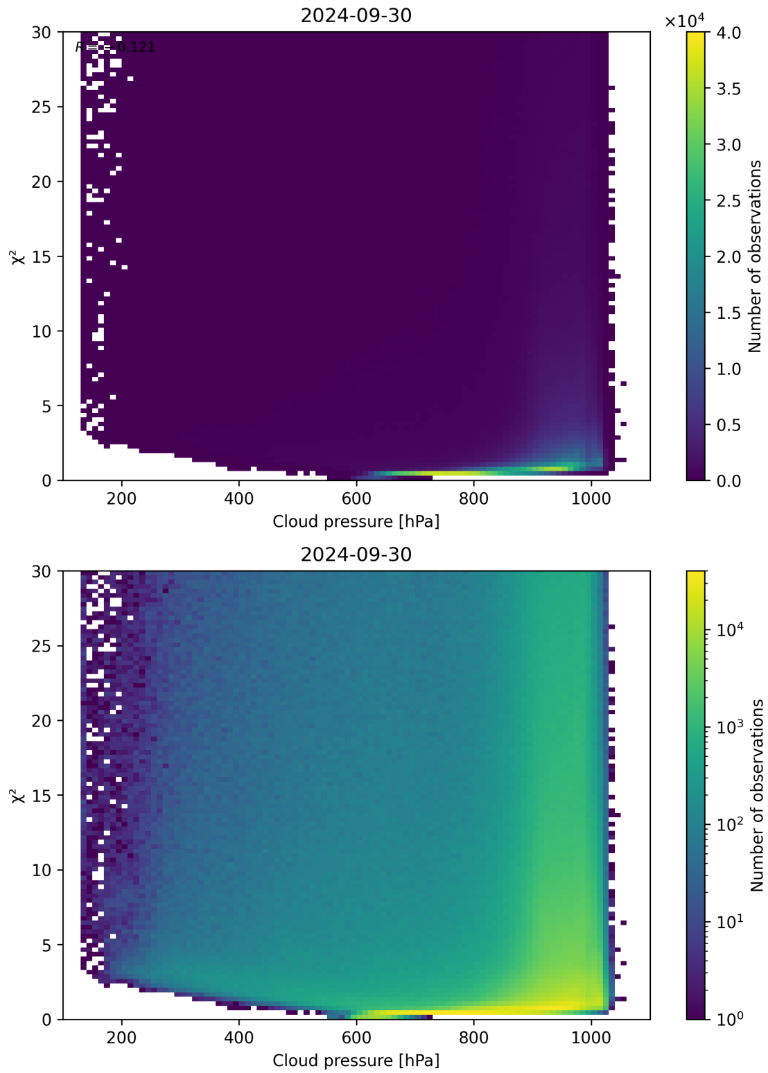
Figure 85: Scatter density plot of “Cloud pressure” against “ \chi^2 ” for 2024-09-29 to 2024-10-01.
