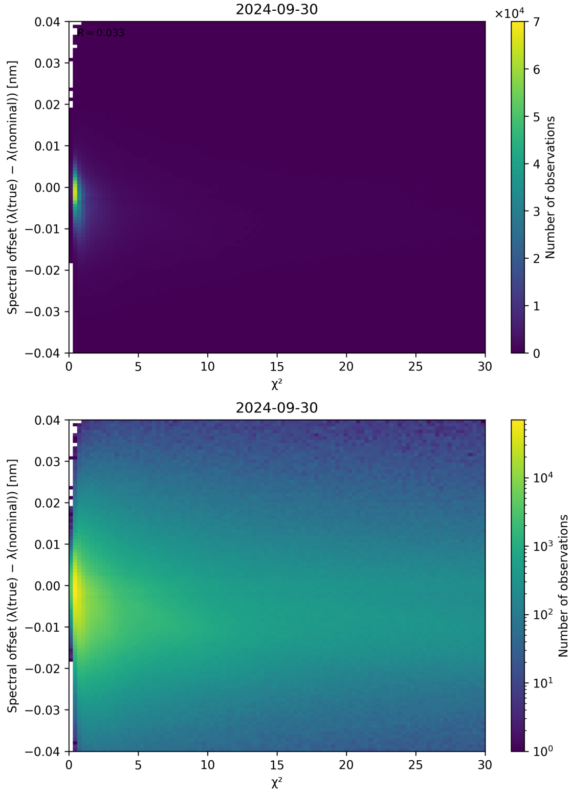
Figure 75: Scatter density plot of “ \chi^2 ” against “Spectral offset ( \lambda_{\text{true}} - \lambda_{\text{nominal}} )” for 2024-09-29 to 2024-10-01.
