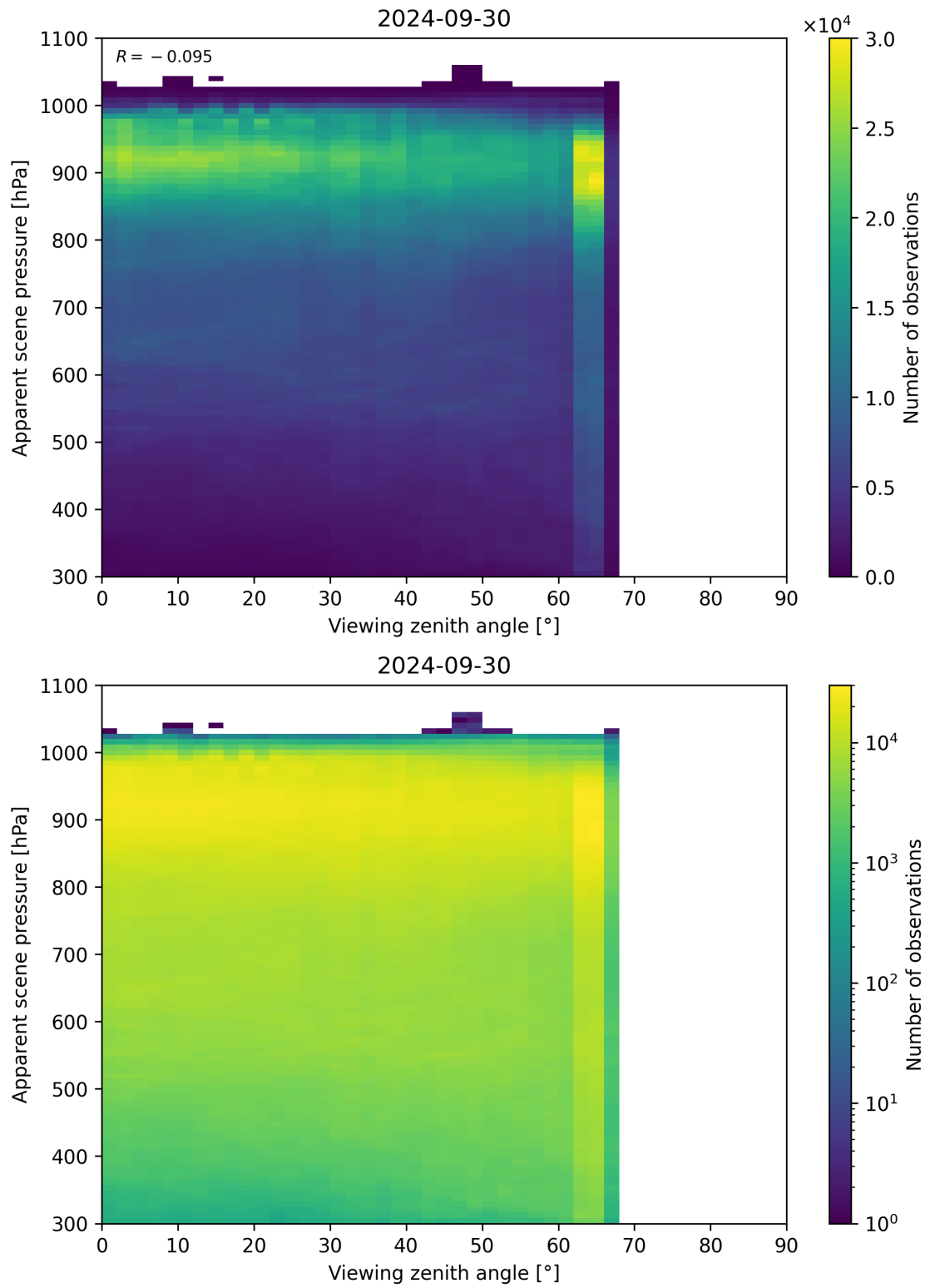
Figure 129: Scatter density plot of “Viewing zenith angle” against “Apparent scene pressure” for 2024-09-29 to 2024-10-01.
