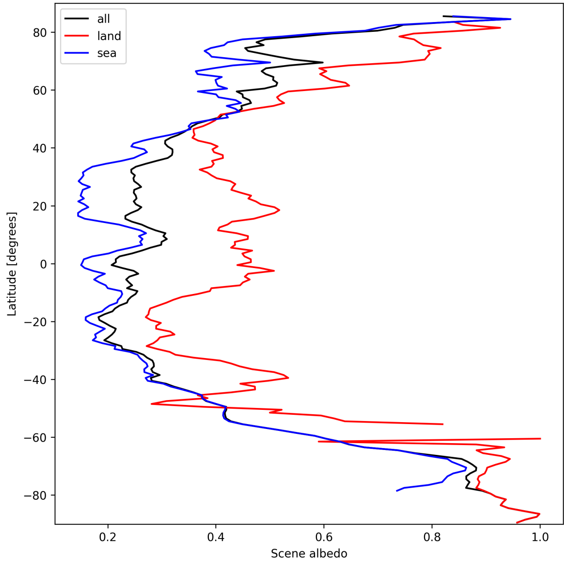
Figure 17: Zonal average of “Scene albedo” for 2024-09-29 to 2024-10-01.
