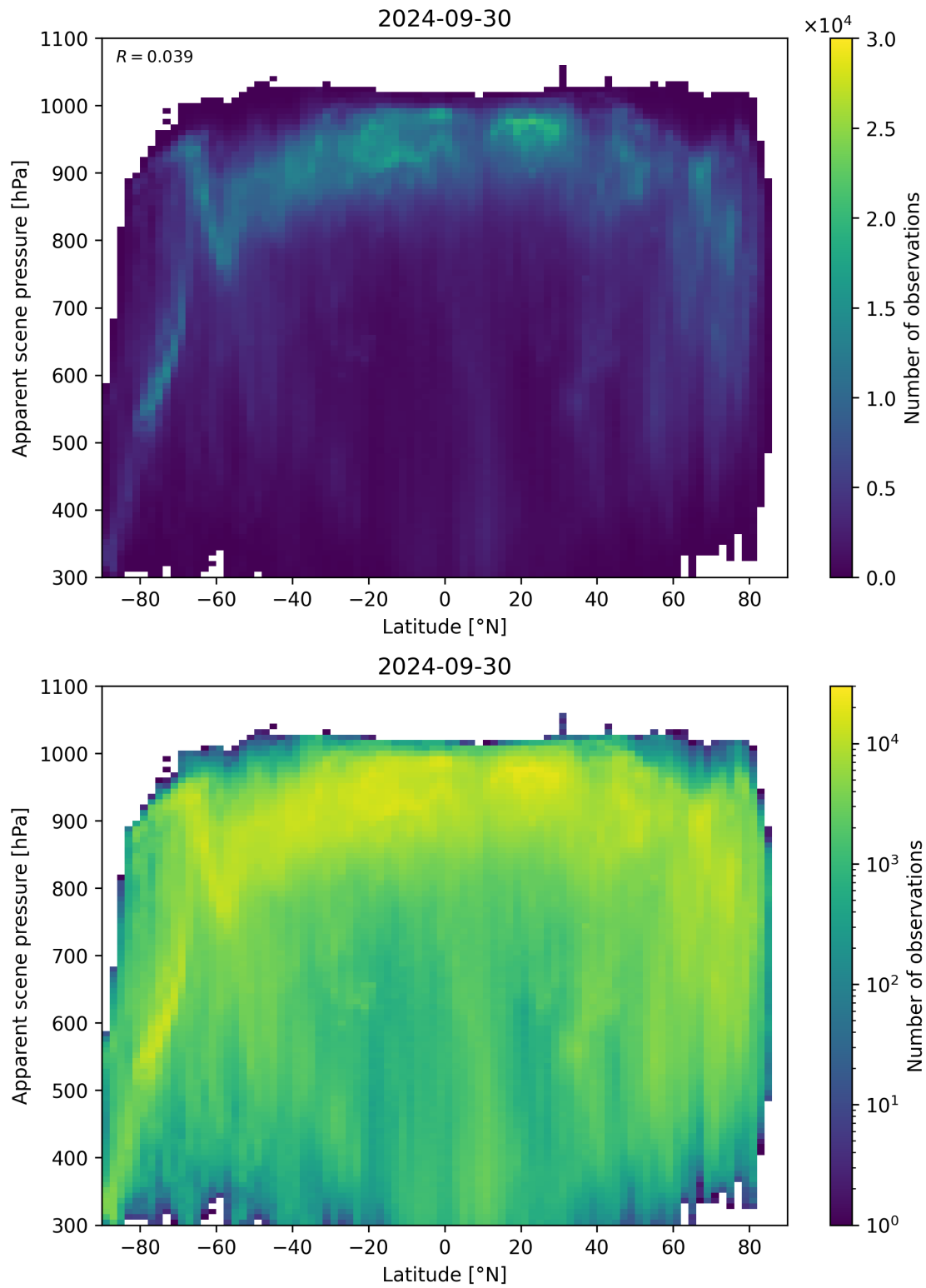
Figure 96: Scatter density plot of “Latitude” against “Apparent scene pressure” for 2024-09-29 to 2024-10-01.
