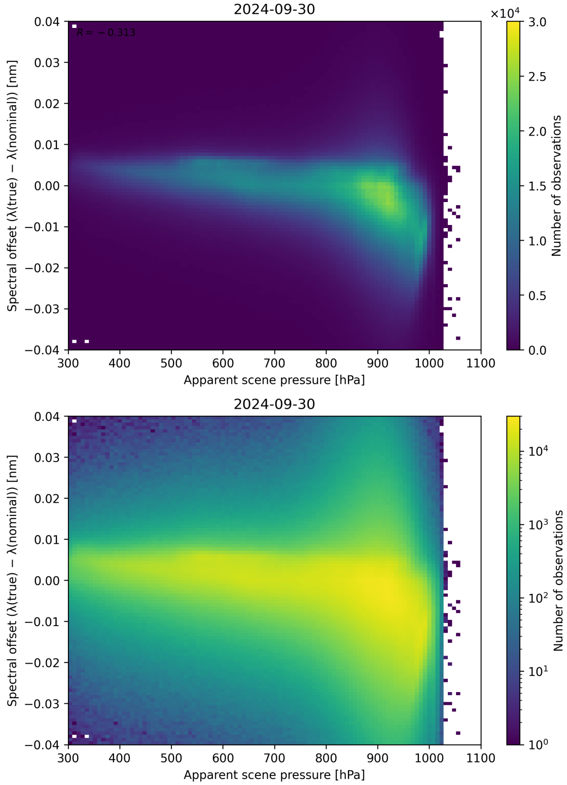
Figure 68: Scatter density plot of “Apparent scene pressure” against “Spectral offset ( \lambda_{\text{true}} - \lambda_{\text{nominal}} )” for 2024-09-29 to 2024-10-01.
