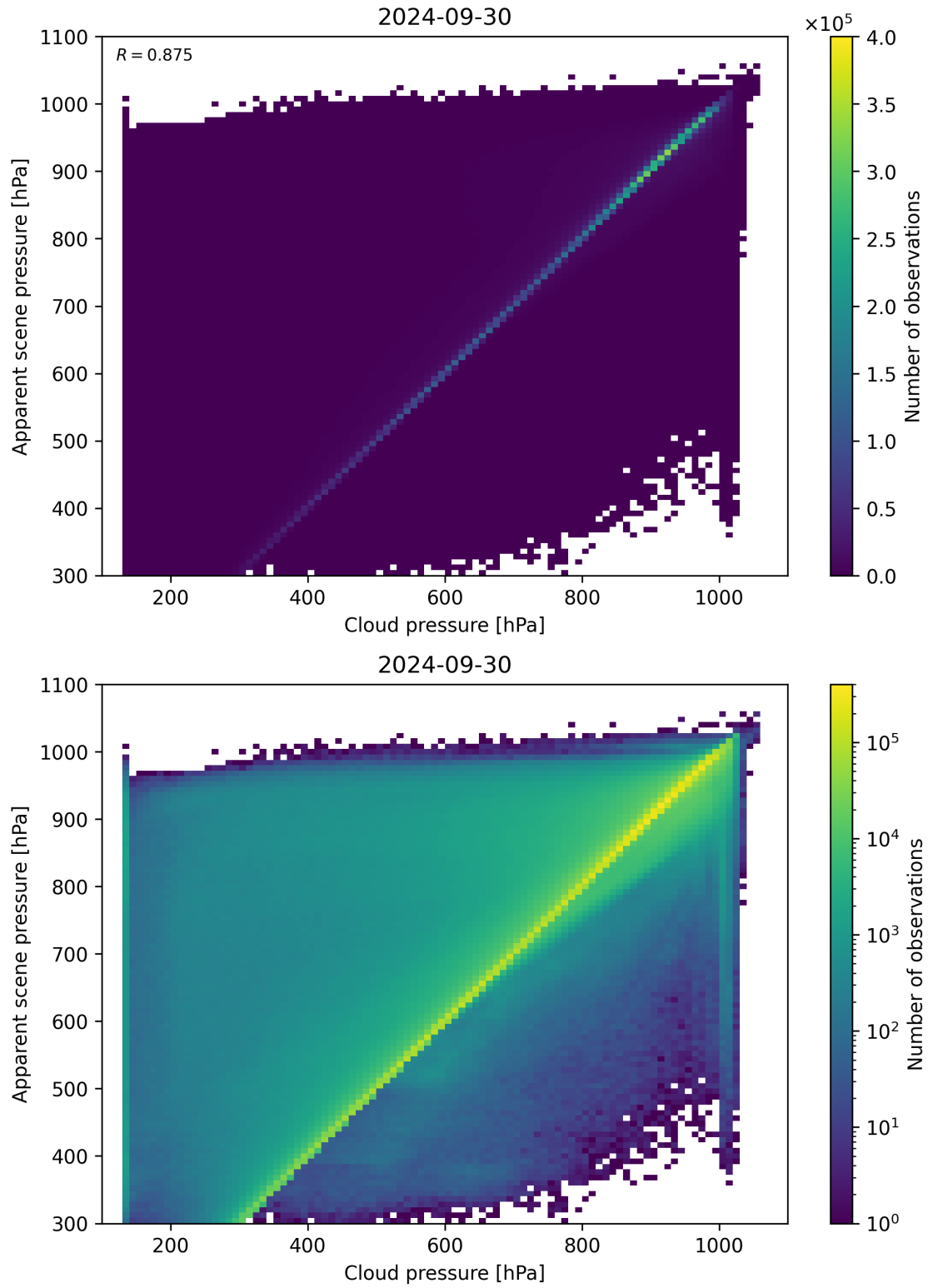
Figure 84: Scatter density plot of “Cloud pressure” against “Apparent scene pressure” for 2024-09-29 to 2024-10-01.
