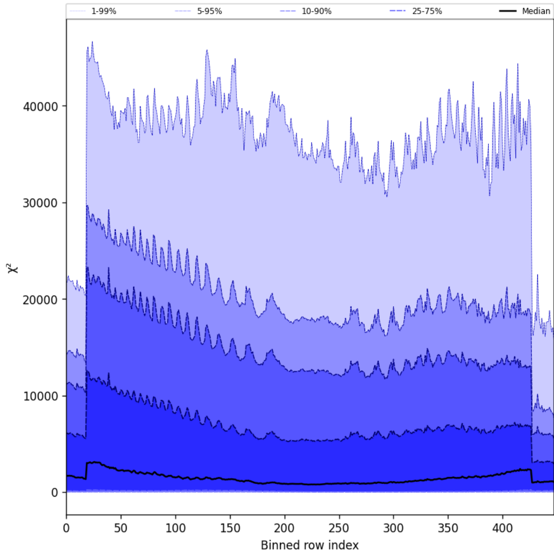
Figure 55: Along track statistics of “ \chi^2 ” for 2024-09-29 to 2024-10-01
