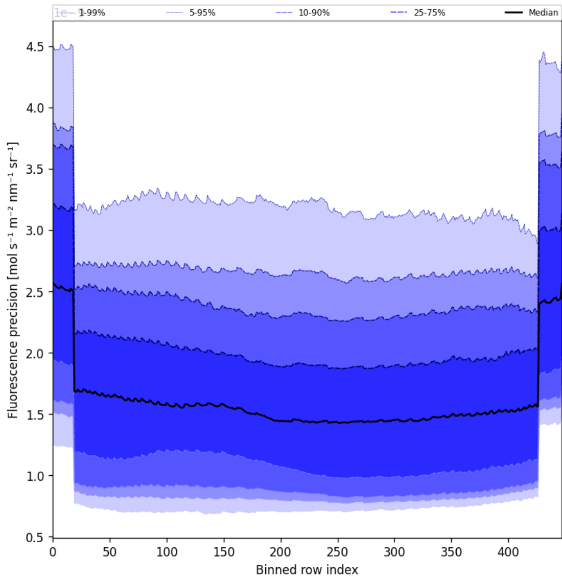
Figure 58: Along track statistics of “Fluorescence precision” for 2024-09-29 to 2024-10-01
