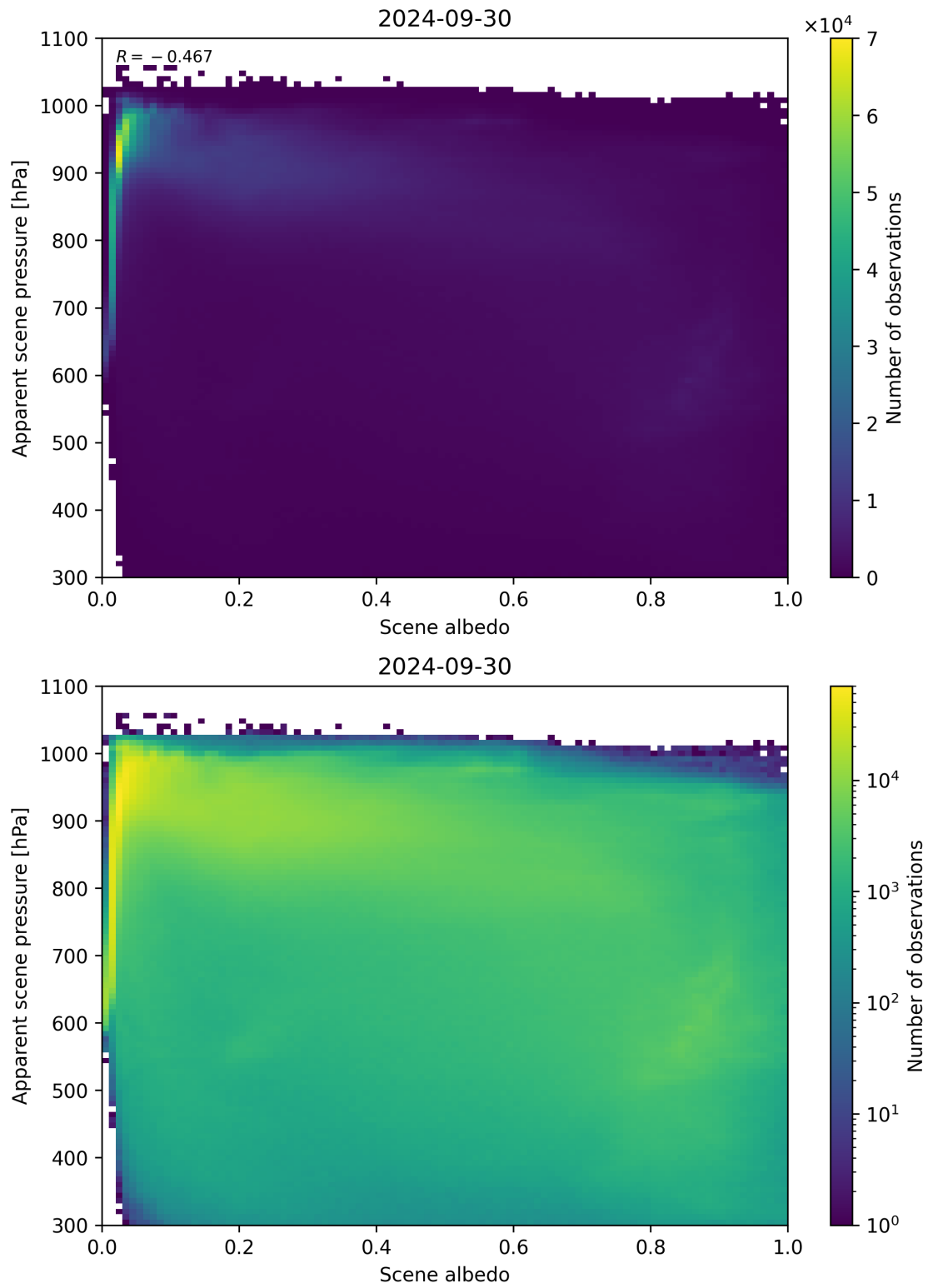
Figure 111: Scatter density plot of “Scene albedo” against “Apparent scene pressure” for 2024-09-29 to 2024-10-01.
