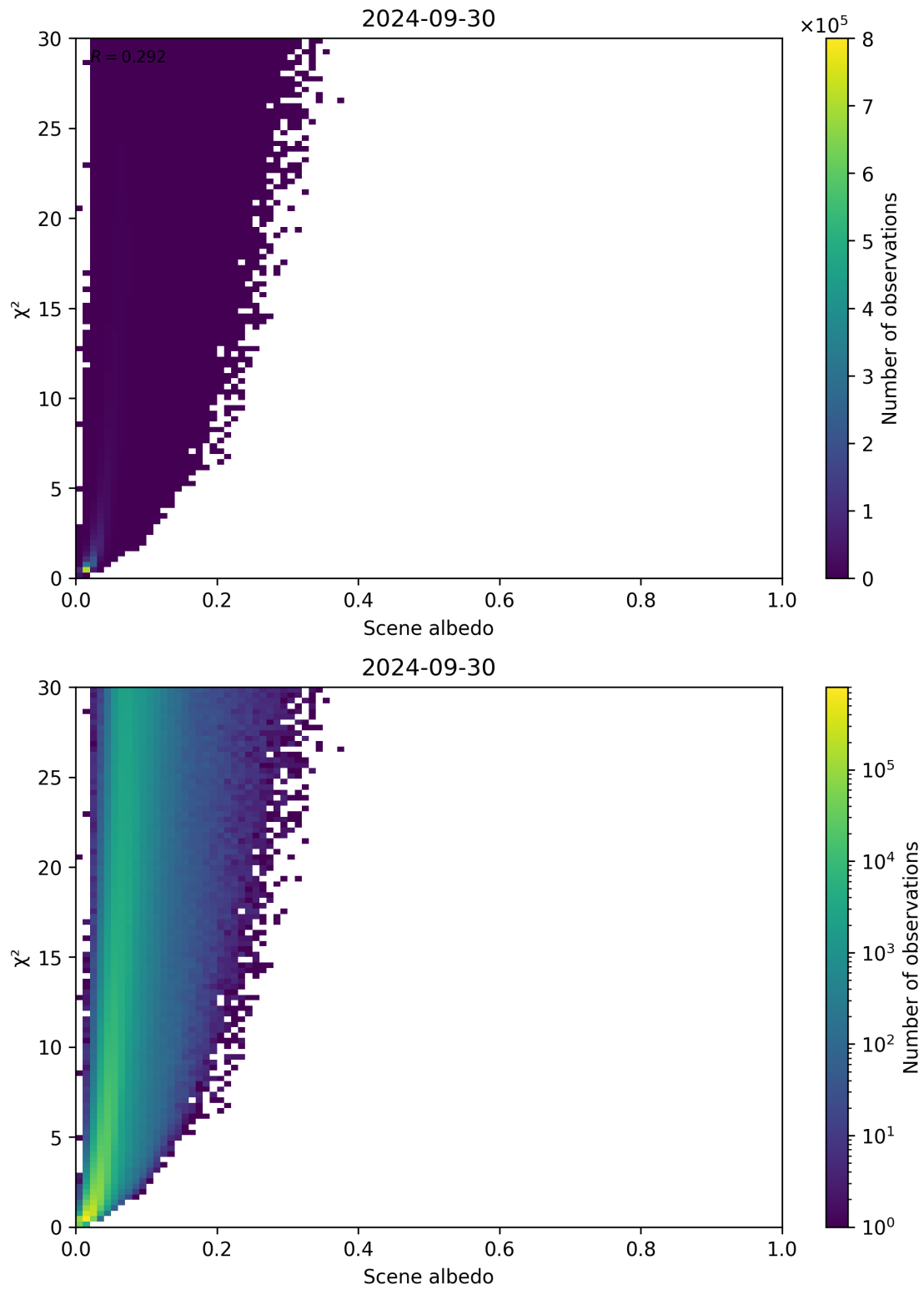
Figure 112: Scatter density plot of “Scene albedo” against “ \chi^2 ” for 2024-09-29 to 2024-10-01.
