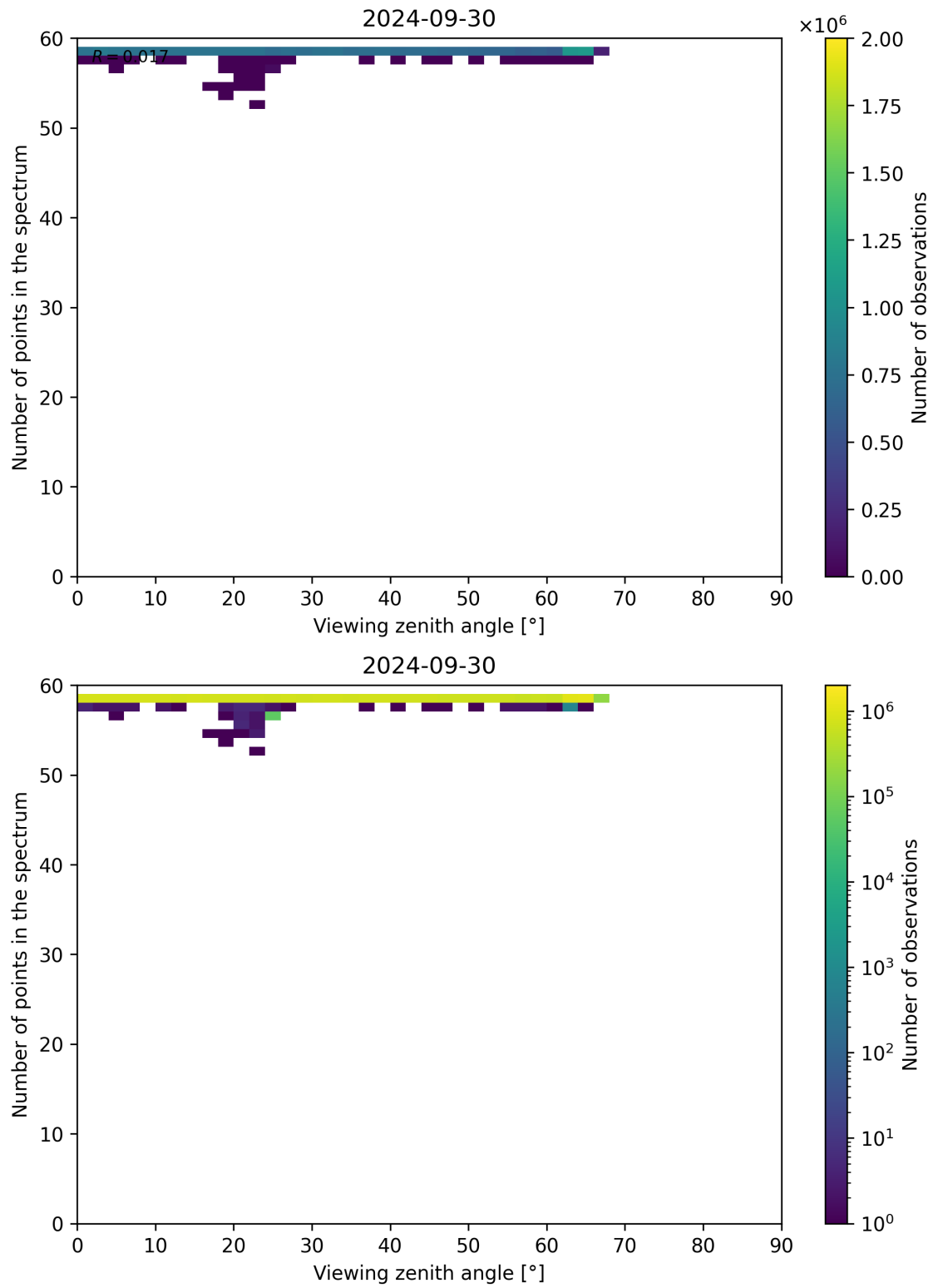
Figure 137: Scatter density plot of “Viewing zenith angle” against “Number of points in the spectrum” for 2024-09-29 to 2024-10-01.
