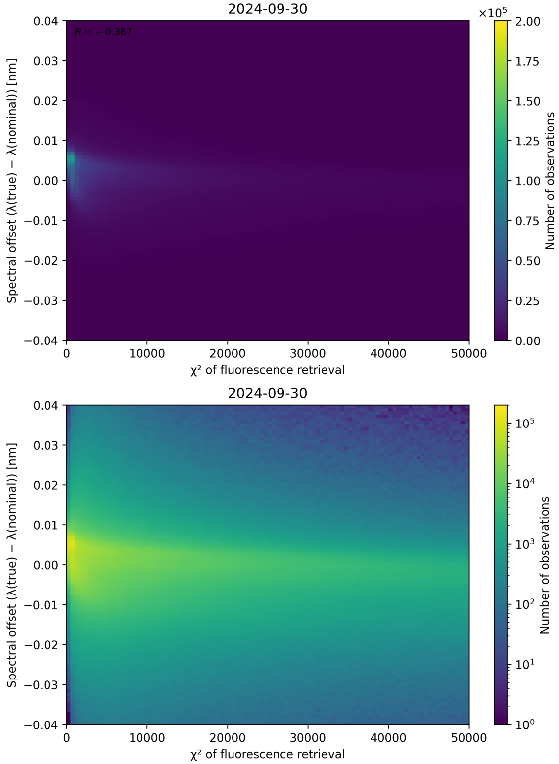
Figure 72: Scatter density plot of “ \chi^2 of fluorescence retrieval” against “Spectral offset ( \lambda_{\text{true}} - \lambda_{\text{nominal}} )” for 2024-09-29 to 2024-10-01.
