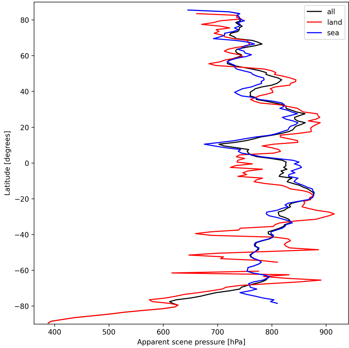
Figure 19: Zonal average of “Apparent scene pressure” for 2024-09-29 to 2024-10-01.
