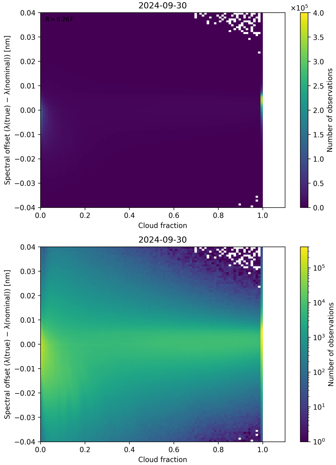
Figure 83: Scatter density plot of “Cloud fraction” against “Spectral offset ( \lambda_{\text{true}} - \lambda_{\text{nominal}} )” for 2024-09-29 to 2024-10-01.
