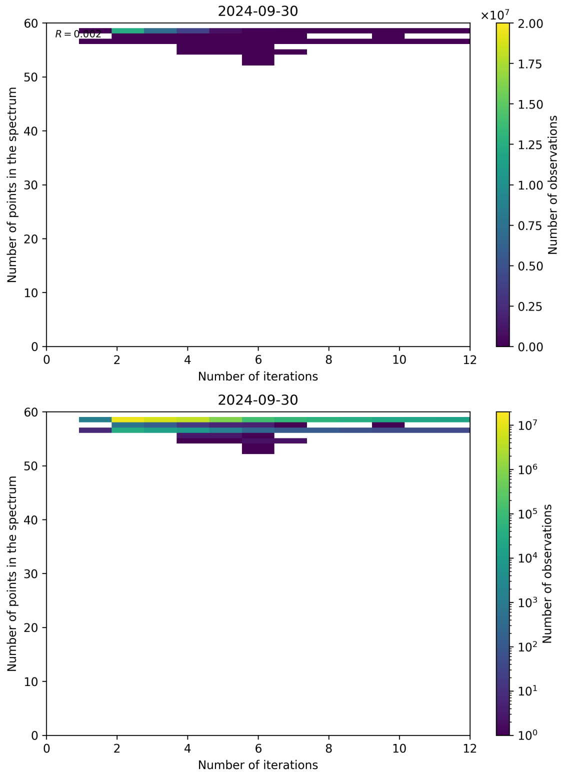
Figure 108: Scatter density plot of “Number of iterations” against “Number of points in the spectrum” for 2024-09-29 to 2024-10-01.
