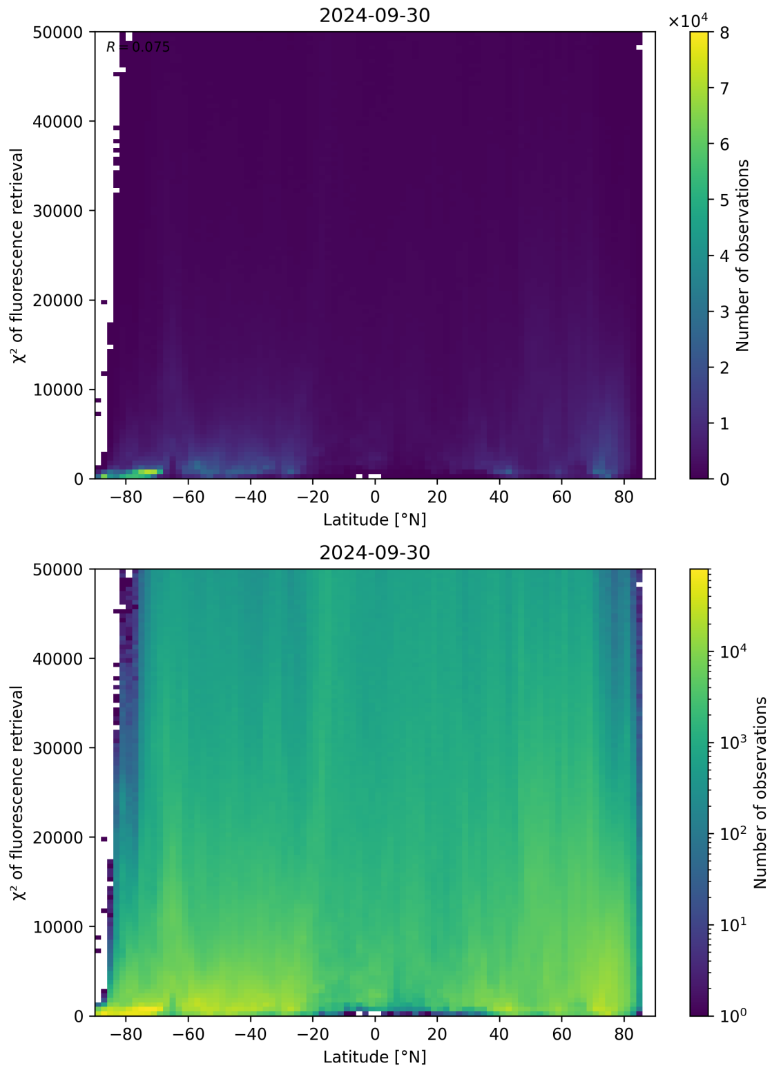
Figure 98: Scatter density plot of “Latitude” against “ \chi^2 of fluorescence retrieval” for 2024-09-29 to 2024-10-01.
