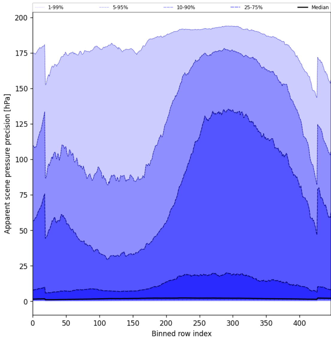
Figure 54: Along track statistics of “Apparent scene pressure precision” for 2024-09-29 to 2024-10-01
