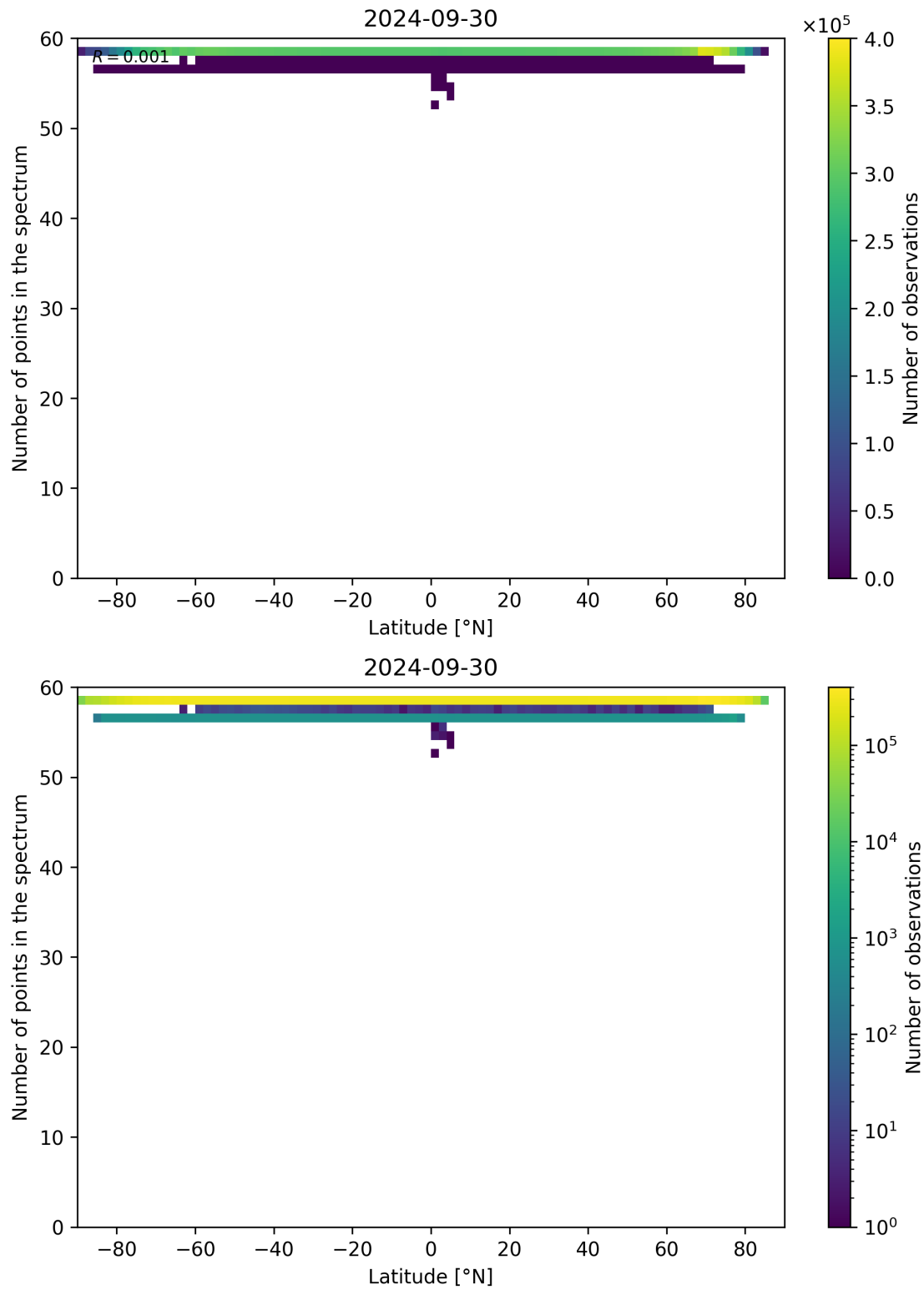
Figure 103: Scatter density plot of “Latitude” against “Number of points in the spectrum” for 2024-09-29 to 2024-10-01.
