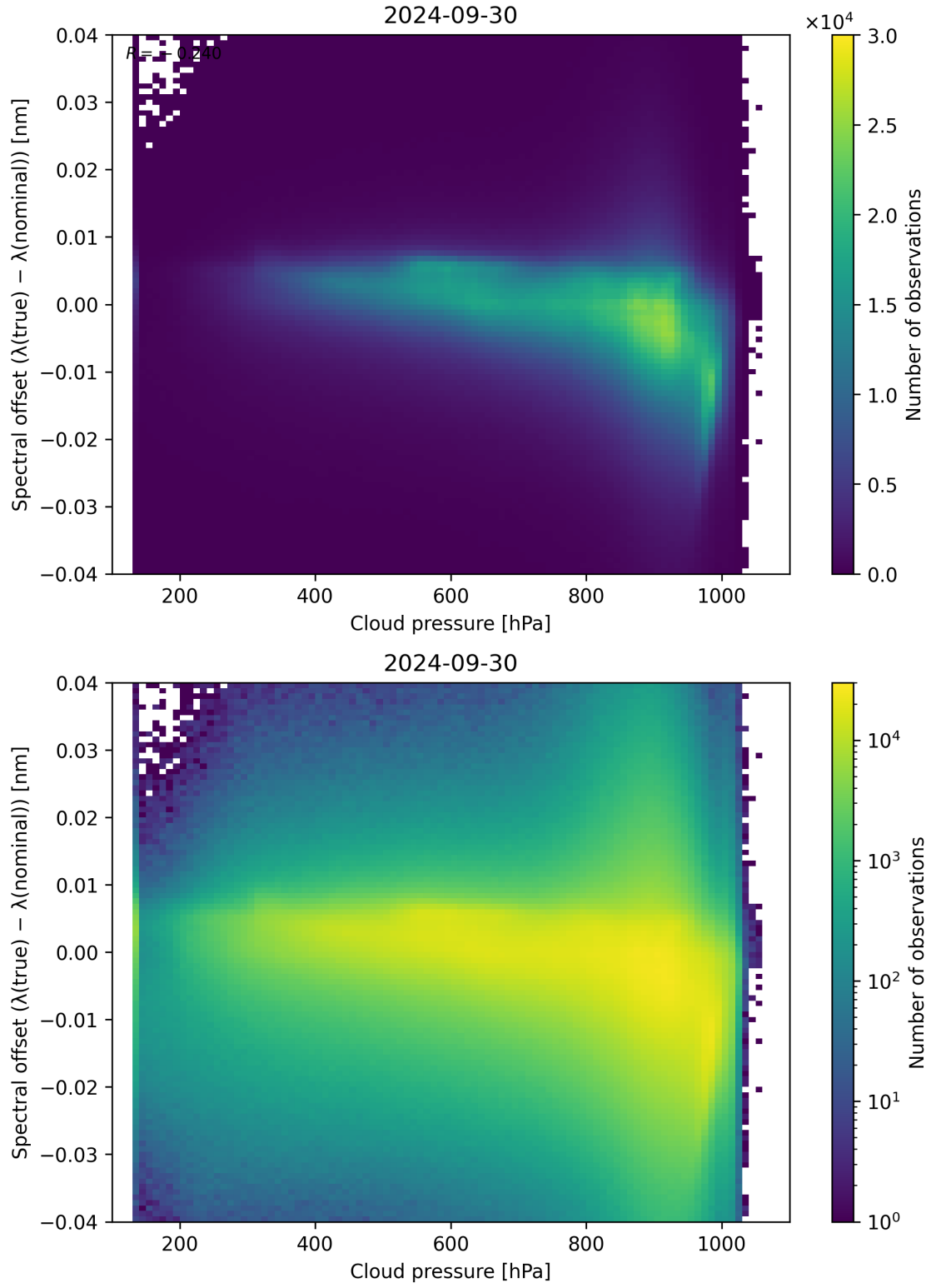
Figure 92: Scatter density plot of “Cloud pressure” against “Spectral offset ( \lambda_{\text{true}} - \lambda_{\text{nominal}} )” for 2024-09-29 to 2024-10-01.
