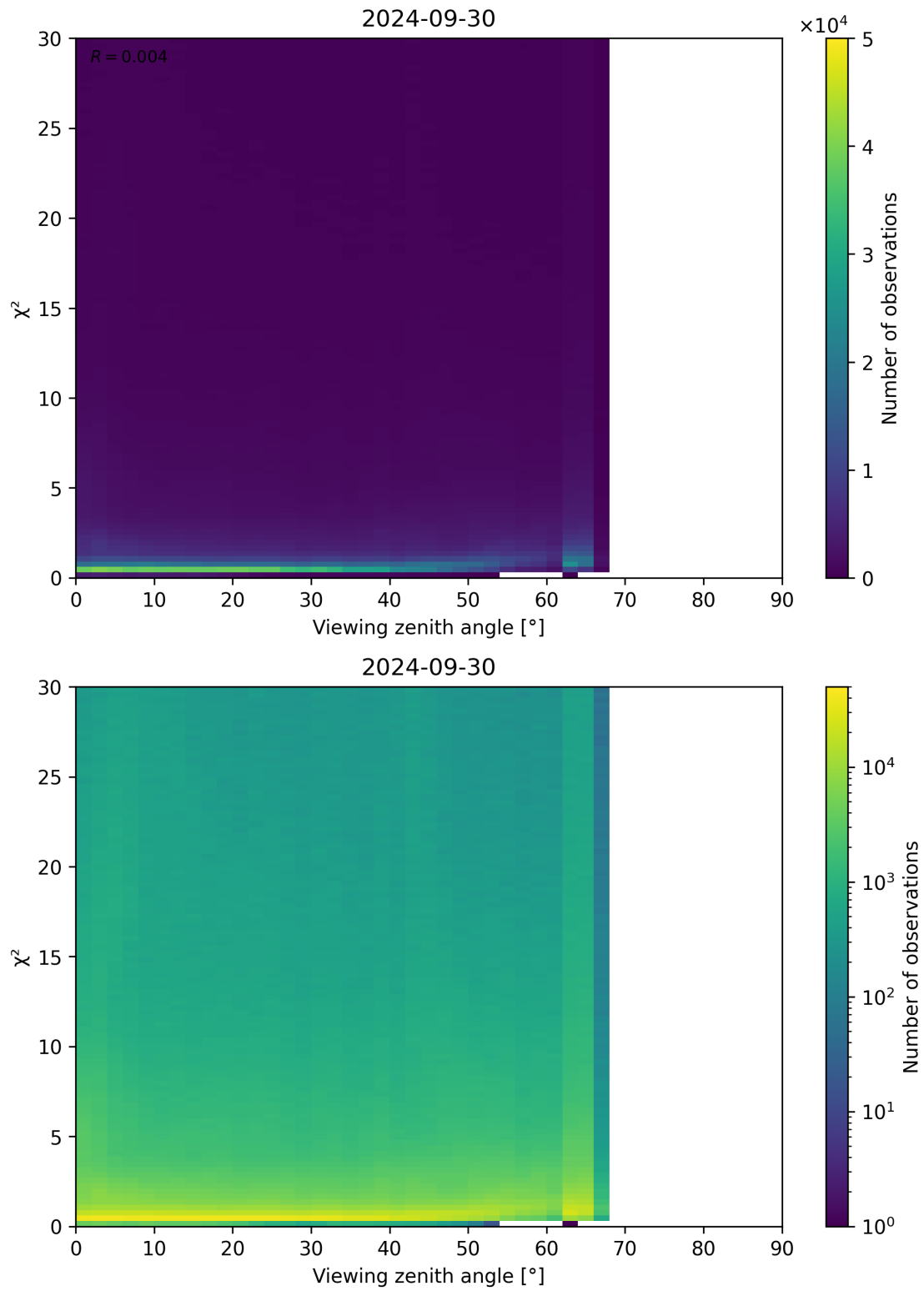
Figure 130: Scatter density plot of “Viewing zenith angle” against “ \chi^2 ” for 2024-09-29 to 2024-10-01.
