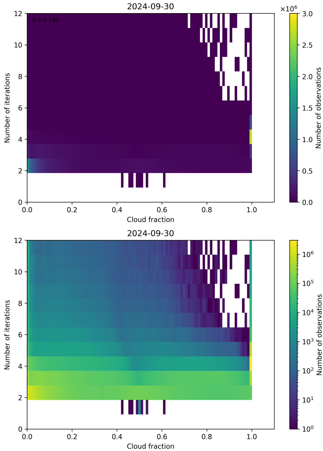
Figure 80: Scatter density plot of “Cloud fraction” against “Number of iterations” for 2024-09-29 to 2024-10-01.
