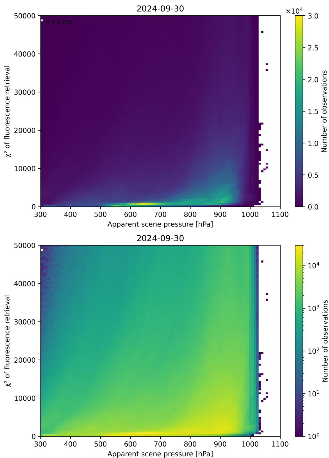
Figure 64: Scatter density plot of “Apparent scene pressure” against “ \chi^2 of fluorescence retrieval” for 2024-09-29 to 2024-10-01.
