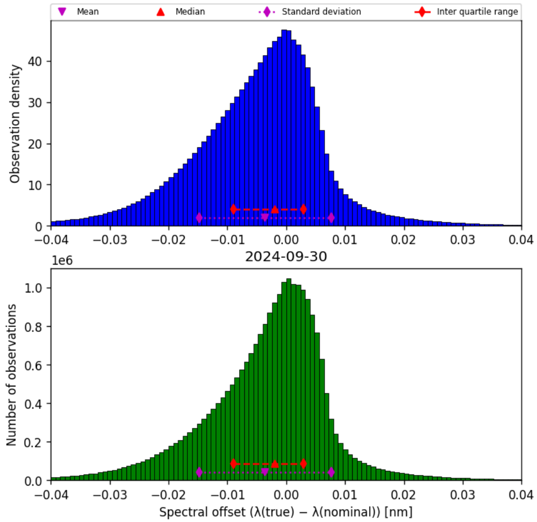
Figure 45: Histogram of “Spectral offset ( \lambda_{\text{true}} - \lambda_{\text{nominal}} )” for 2024-09-29 to 2024-10-01
