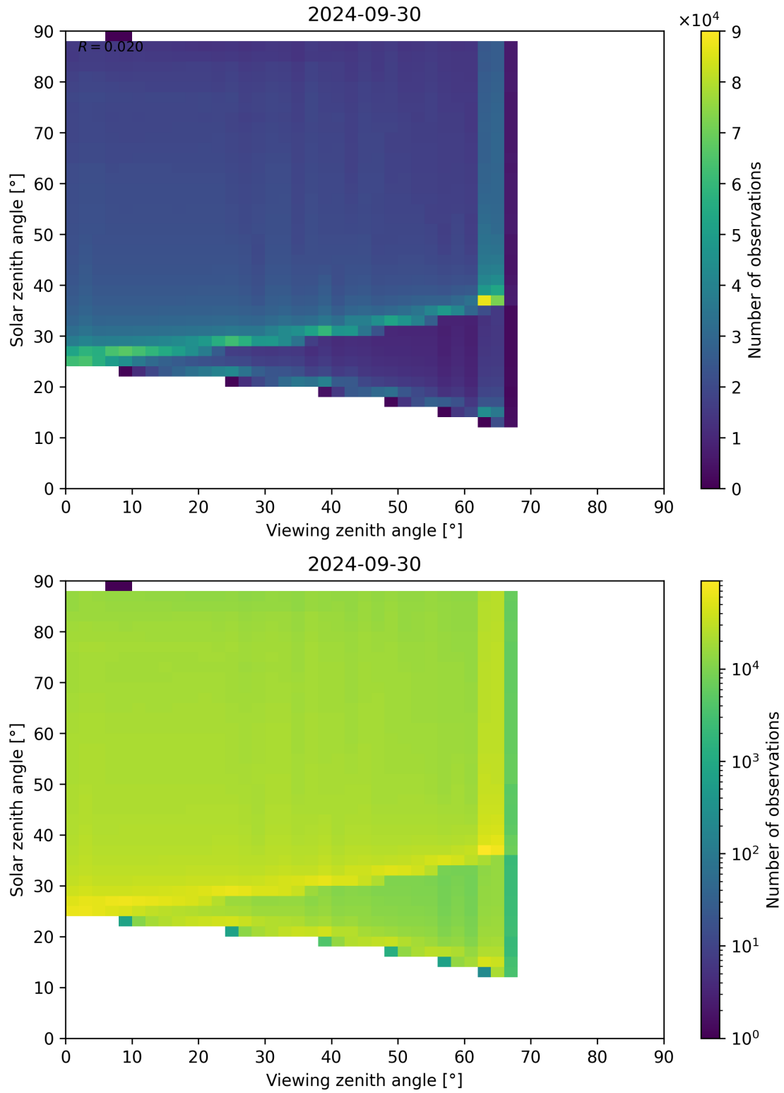
Figure 139: Scatter density plot of “Viewing zenith angle” against “Solar zenith angle” for 2024-09-29 to 2024-10-01.
