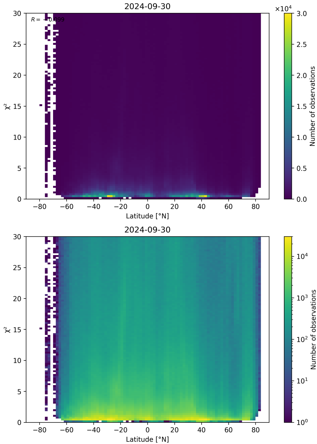
Figure 97: Scatter density plot of “Latitude” against “ \chi^2 ” for 2024-09-29 to 2024-10-01.
