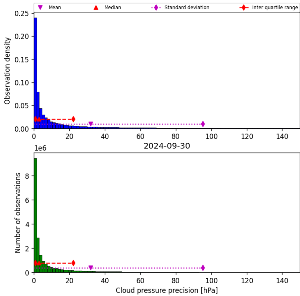
Figure 31: Histogram of “Cloud pressure precision” for 2024-09-29 to 2024-10-01
