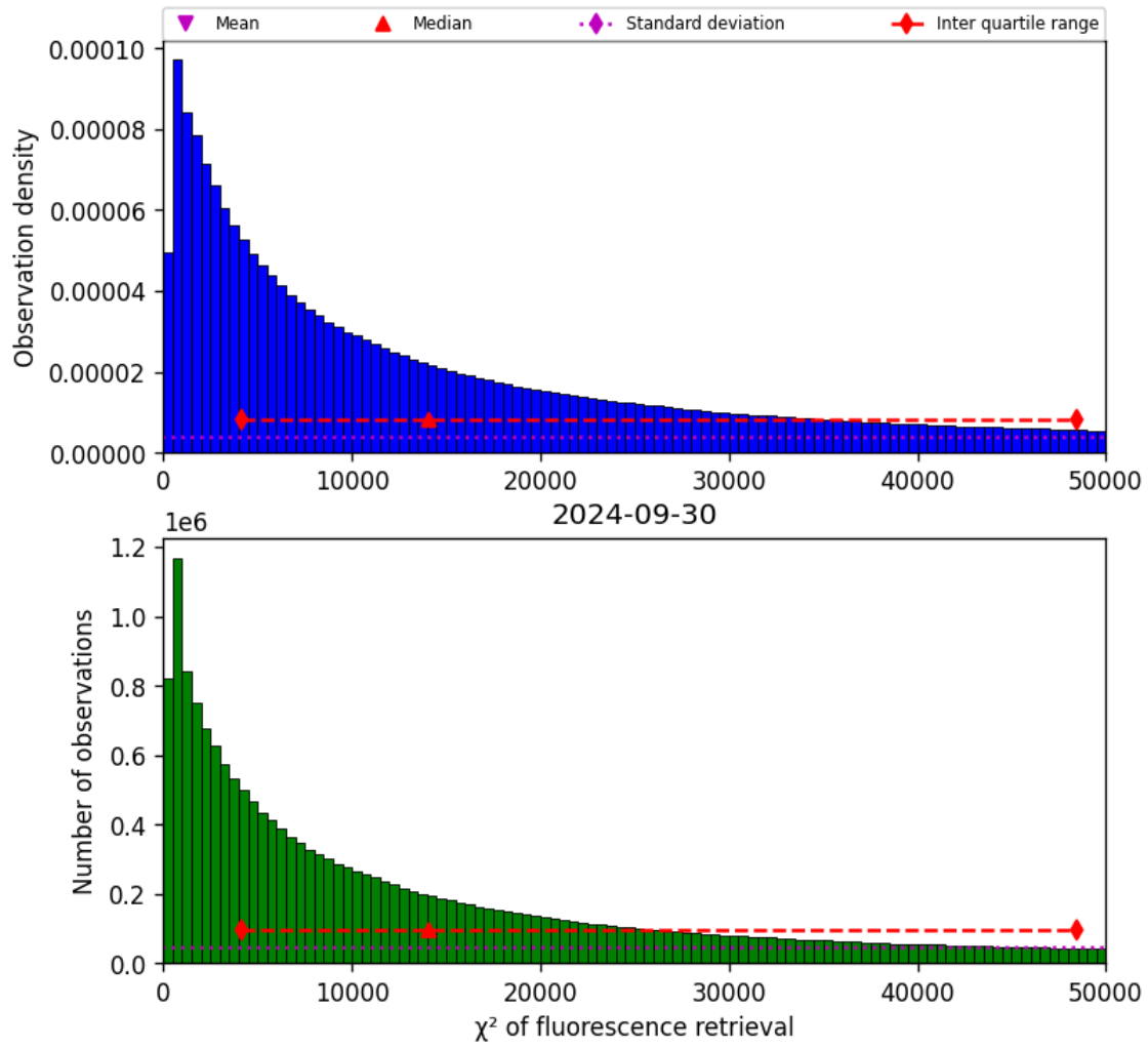
Figure 42: Histogram of “ \chi^2 of fluorescence retrieval” for 2024-09-29 to 2024-10-01
