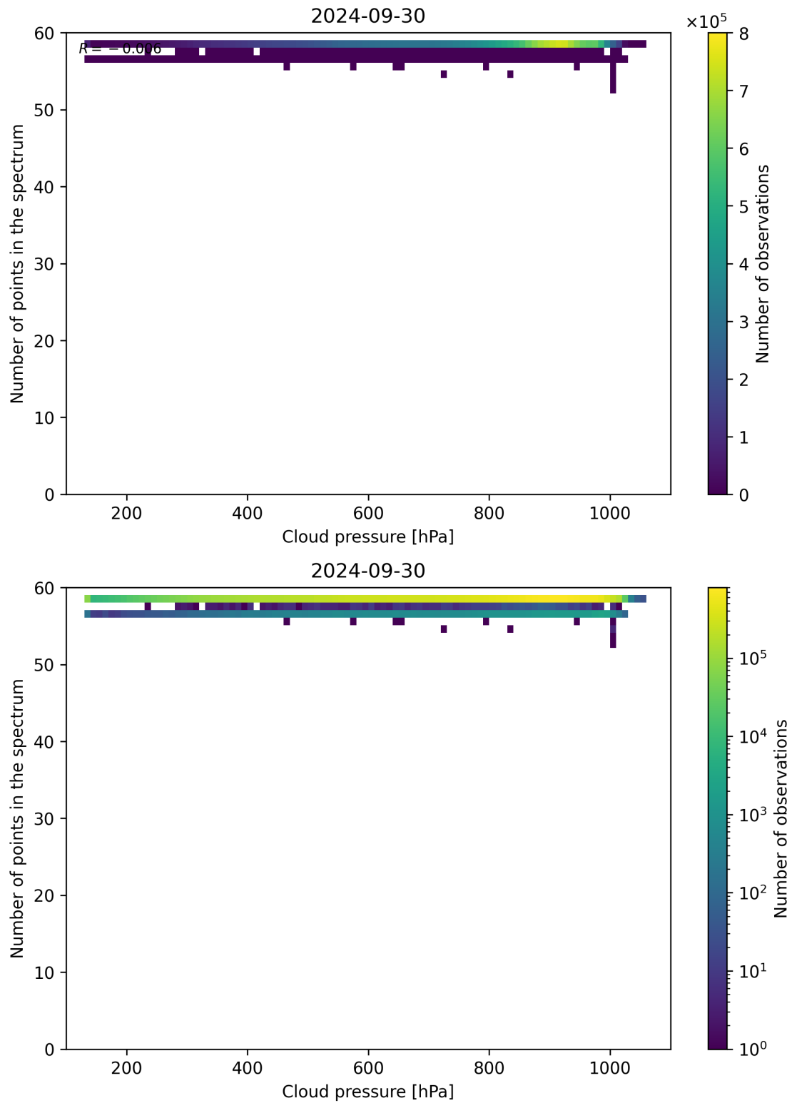
Figure 90: Scatter density plot of “Cloud pressure” against “Number of points in the spectrum” for 2024-09-29 to 2024-10-01.
