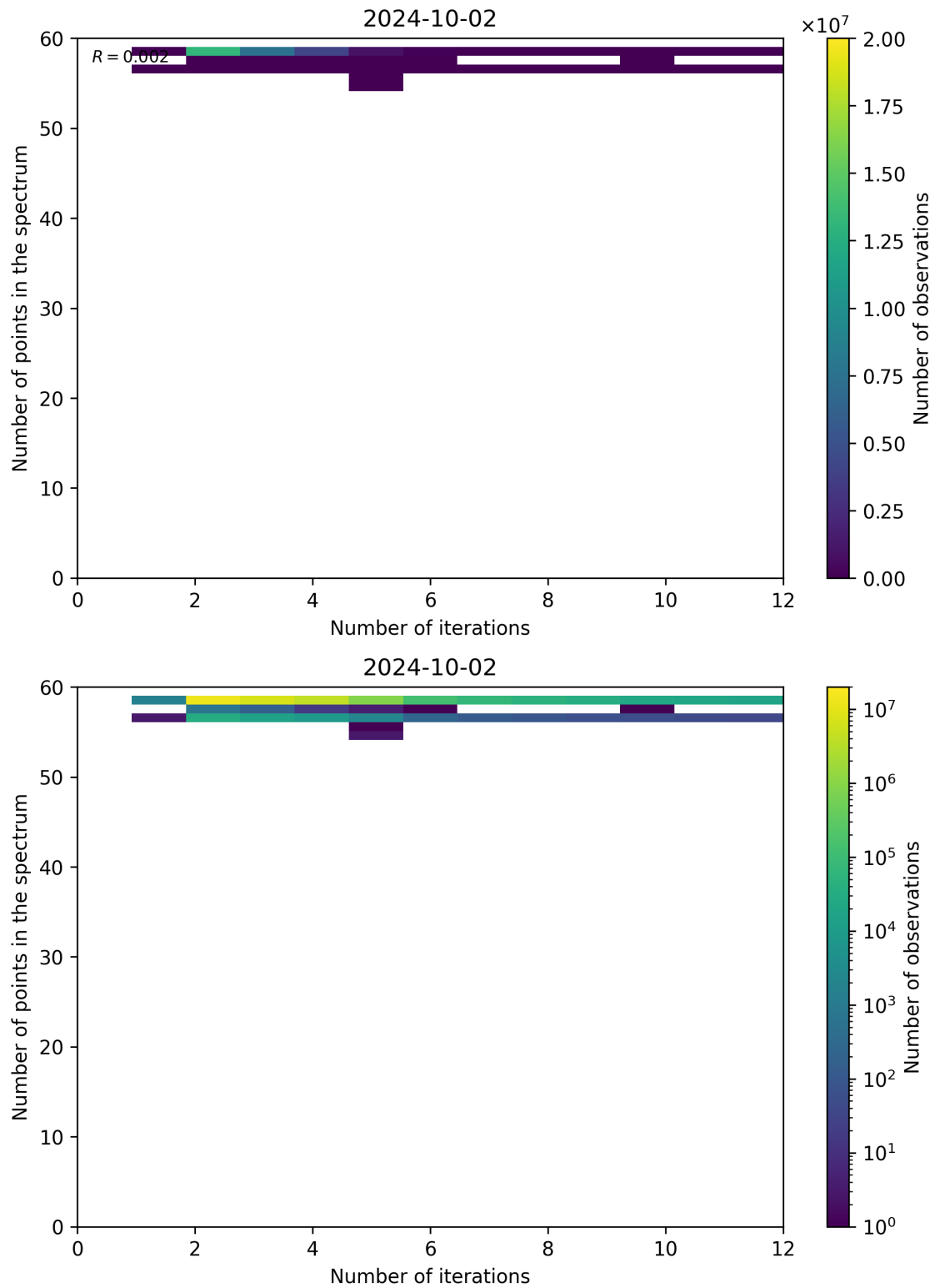
Figure 108: Scatter density plot of “Number of iterations” against “Number of points in the spectrum” for 2024-10-01 to 2024-10-03.
