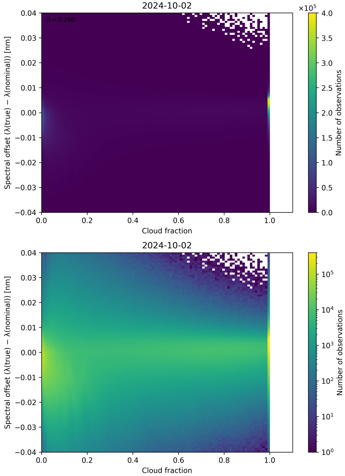
Figure 83: Scatter density plot of “Cloud fraction” against “Spectral offset ( \lambda_{\text{true}} - \lambda_{\text{nominal}} )” for 2024-10-01 to 2024-10-03.
