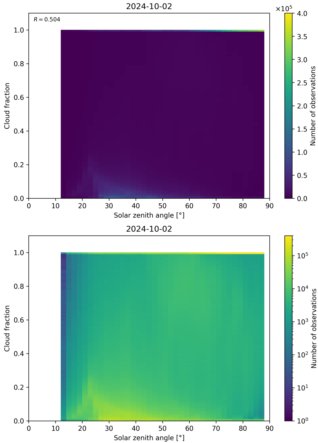
Figure 121: Scatter density plot of “Solar zenith angle” against “Cloud fraction” for 2024-10-01 to 2024-10-03.
