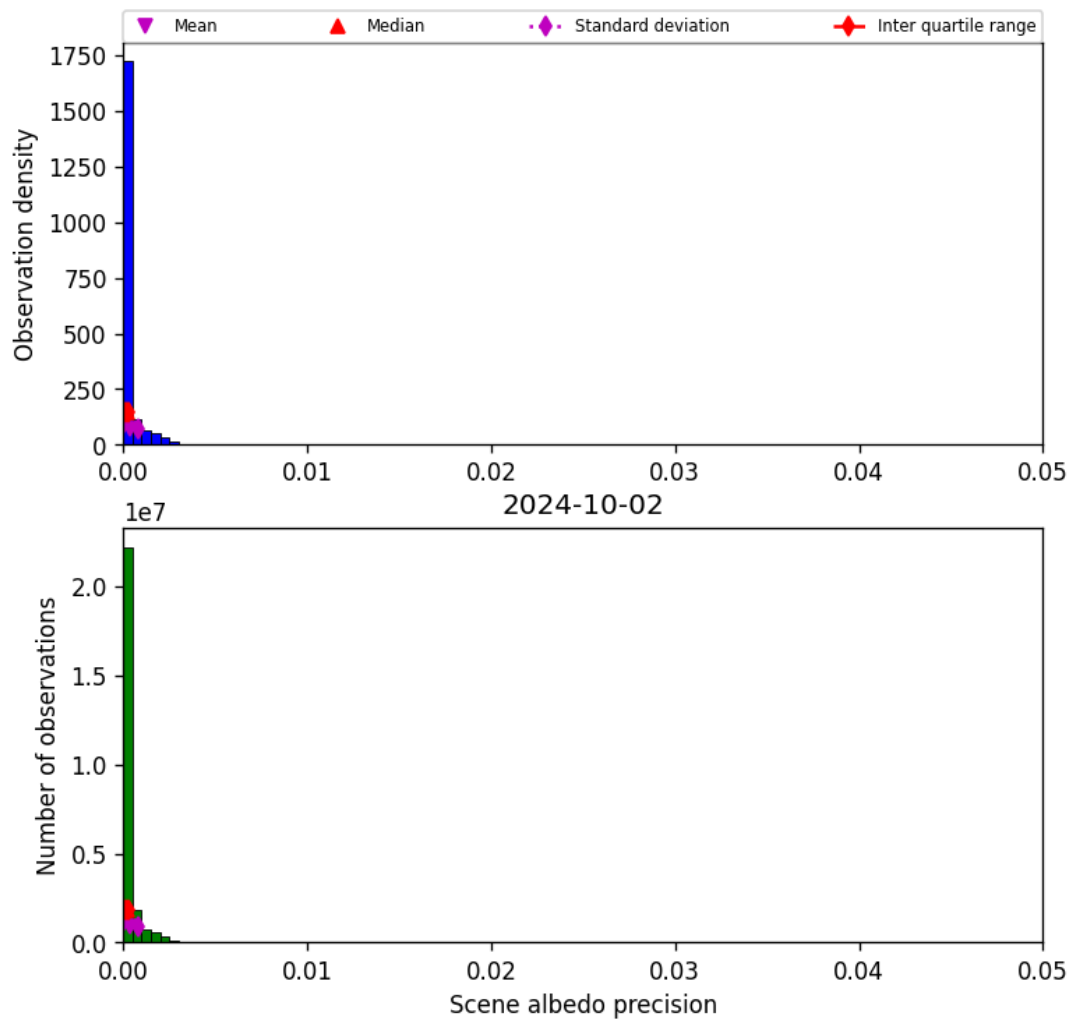
Figure 35: Histogram of “Scene albedo precision” for 2024-10-01 to 2024-10-03
