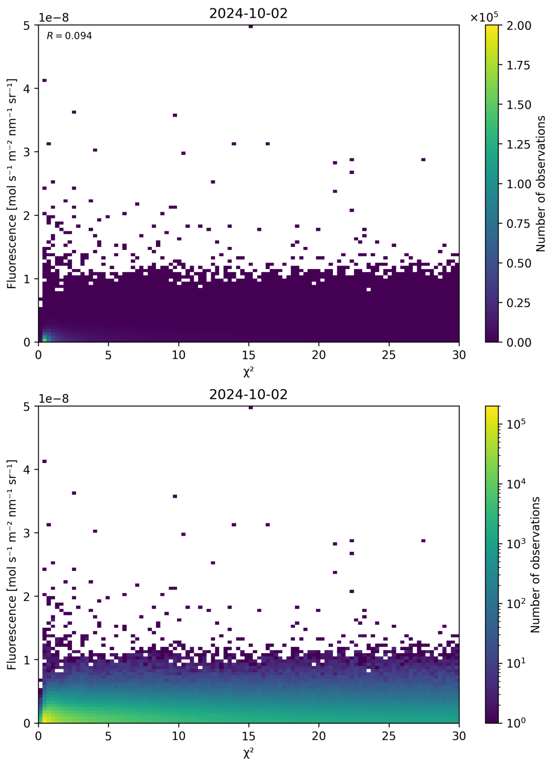
Figure 70: Scatter density plot of “ \chi^2 ” against “Fluorescence” for 2024-10-01 to 2024-10-03.
