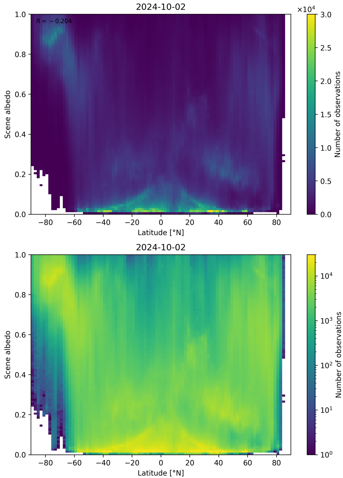
Figure 104: Scatter density plot of “Latitude” against “Scene albedo” for 2024-10-01 to 2024-10-03.
