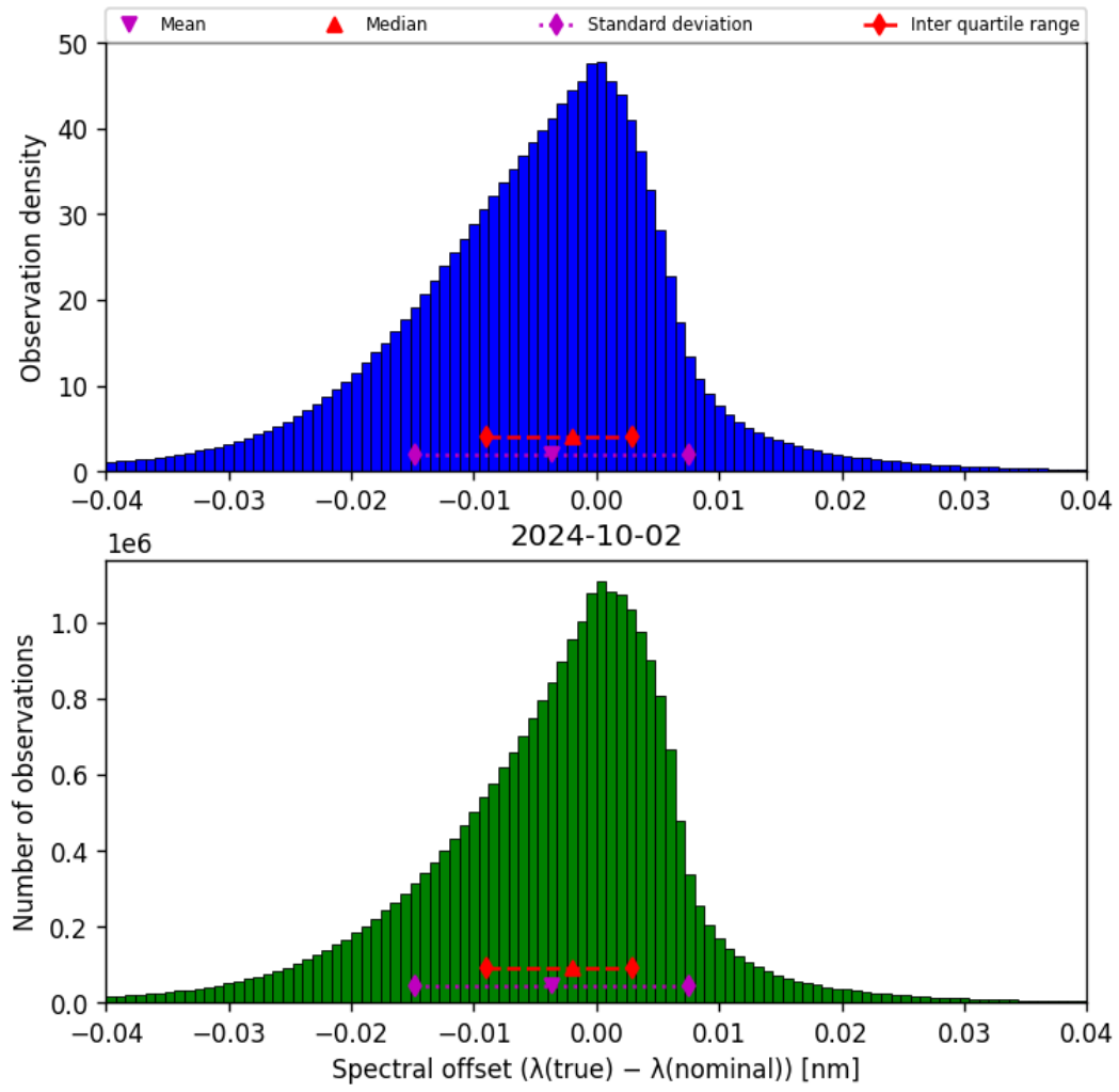
Figure 45: Histogram of “Spectral offset ( \lambda_{\text{true}} - \lambda_{\text{nominal}} )” for 2024-10-01 to 2024-10-03
