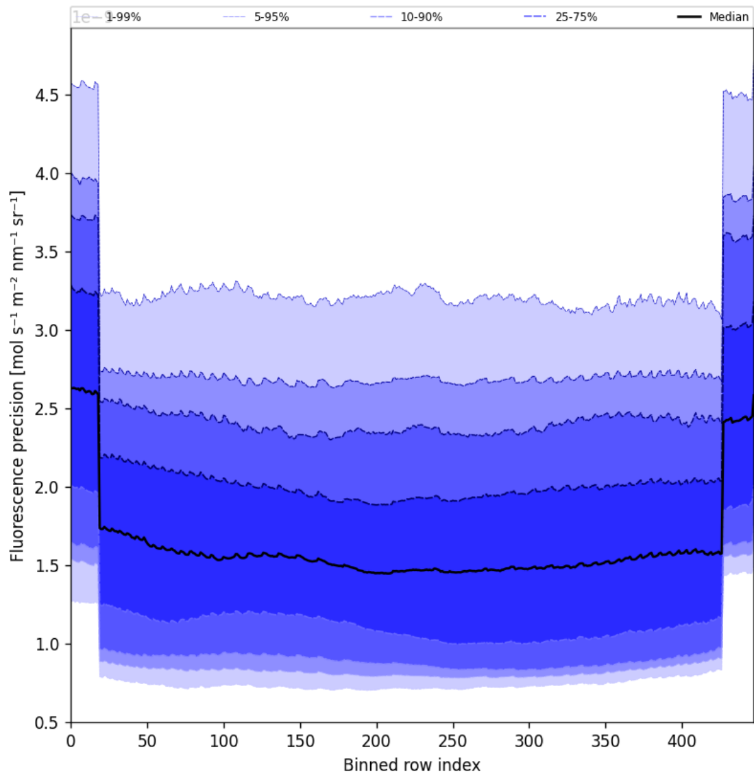
Figure 58: Along track statistics of “Fluorescence precision” for 2024-10-01 to 2024-10-03
