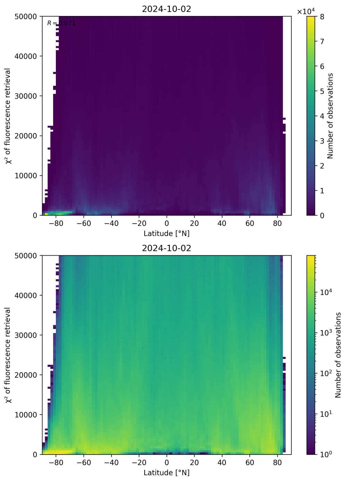
Figure 98: Scatter density plot of “Latitude” against “ \chi^2 of fluorescence retrieval” for 2024-10-01 to 2024-10-03.
