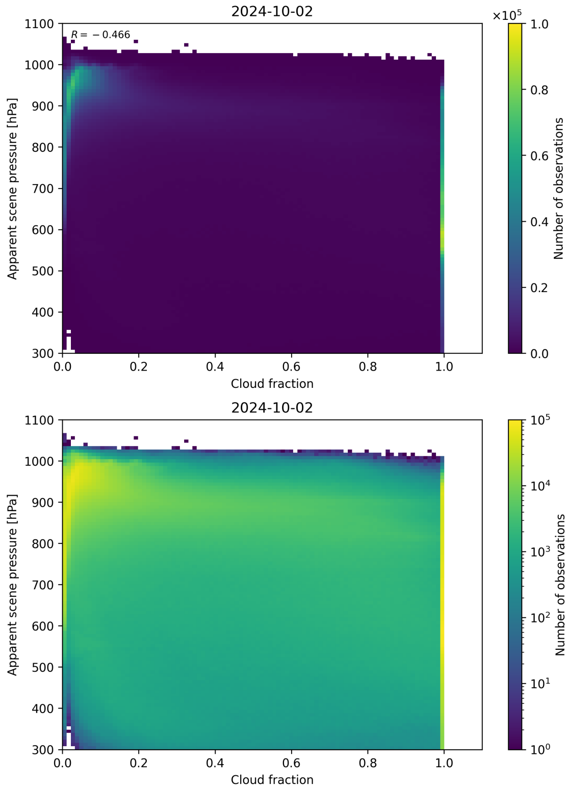
Figure 76: Scatter density plot of “Cloud fraction” against “Apparent scene pressure” for 2024-10-01 to 2024-10-03.
