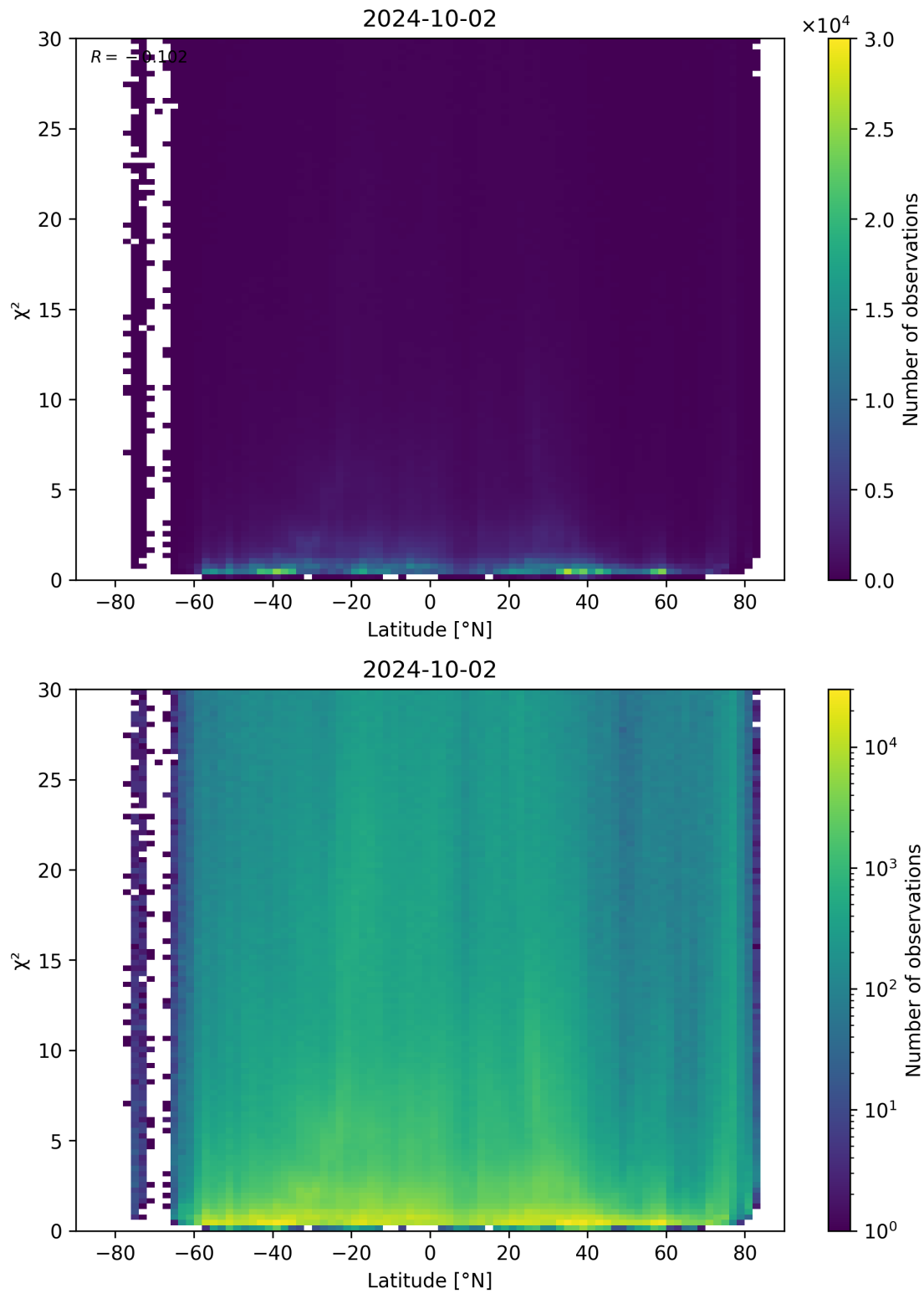
Figure 97: Scatter density plot of “Latitude” against “ \chi^2 ” for 2024-10-01 to 2024-10-03.
