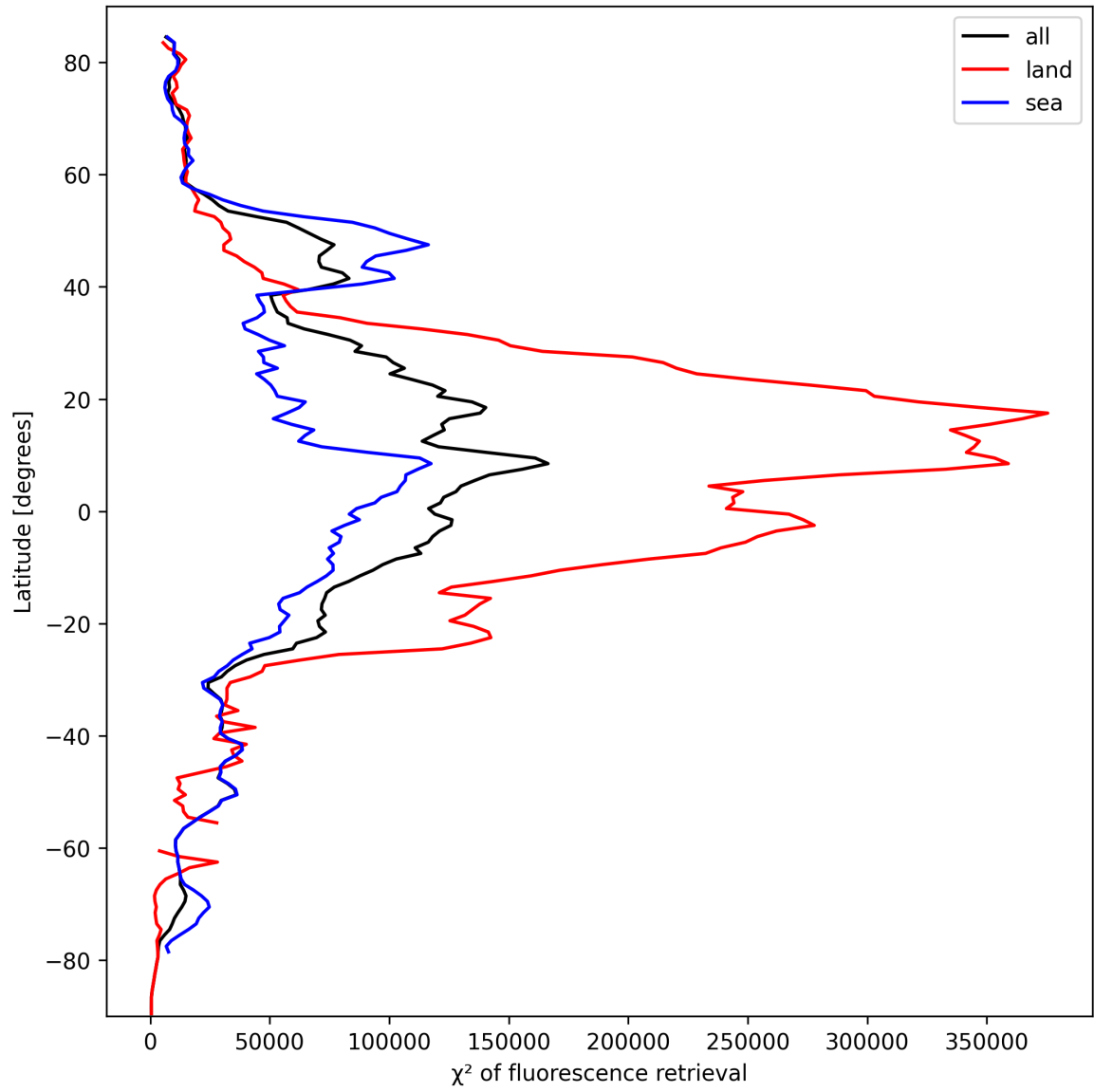
Figure 25: Zonal average of “ \chi^2 of fluorescence retrieval” for 2024-10-01 to 2024-10-03.
