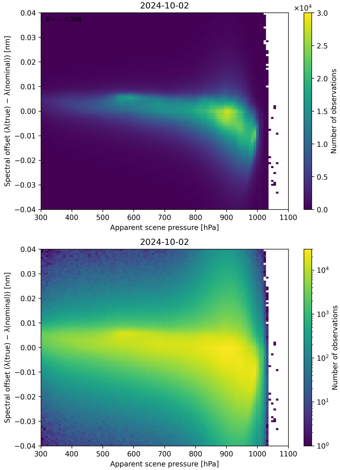
Figure 68: Scatter density plot of “Apparent scene pressure” against “Spectral offset ( \lambda_{\text{true}} - \lambda_{\text{nominal}} )” for 2024-10-01 to 2024-10-03.
