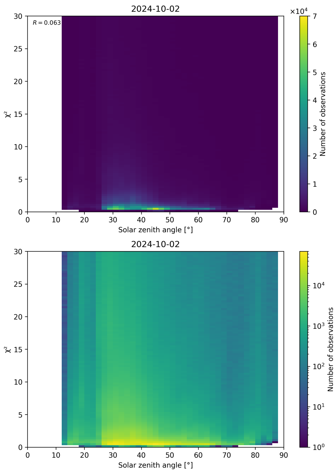
Figure 119: Scatter density plot of “Solar zenith angle” against “ \chi^2 ” for 2024-10-01 to 2024-10-03.
