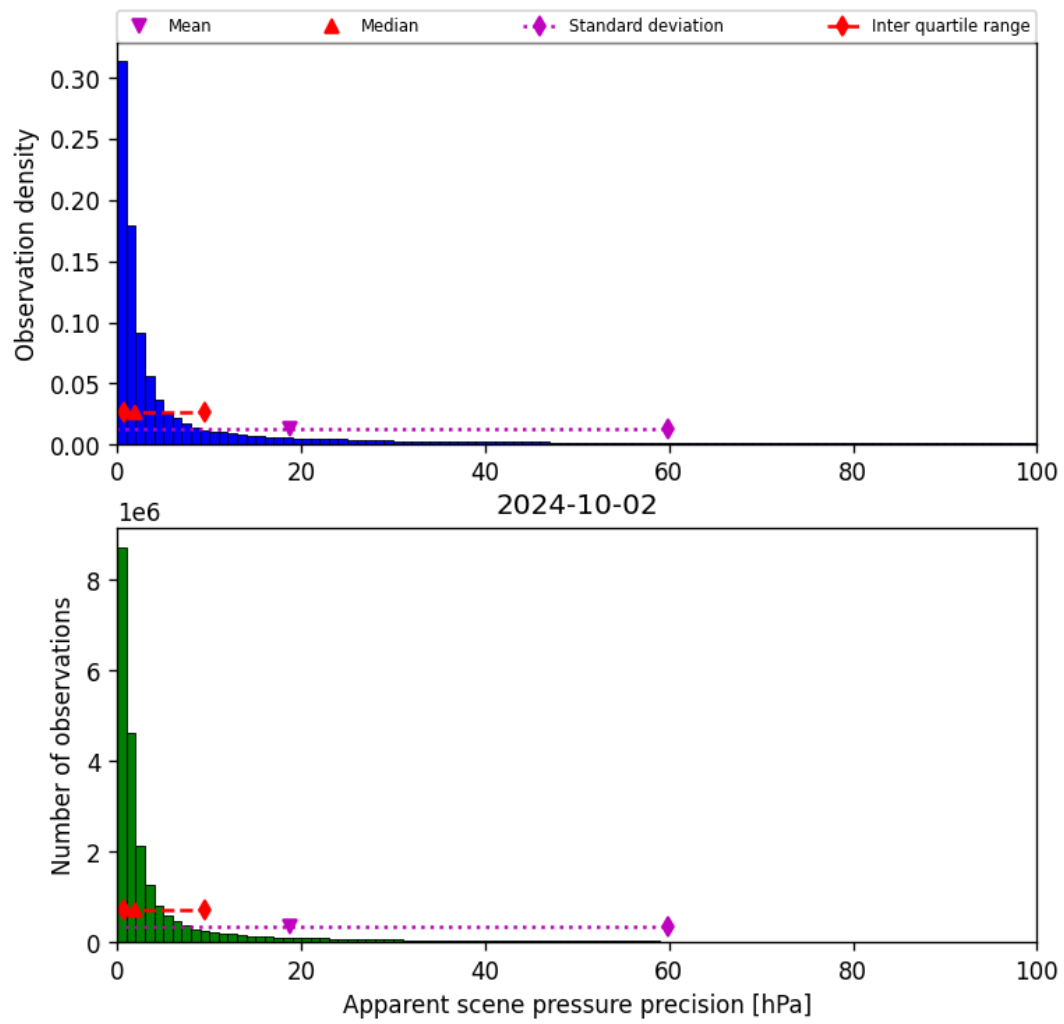
Figure 37: Histogram of “Apparent scene pressure precision” for 2024-10-01 to 2024-10-03
