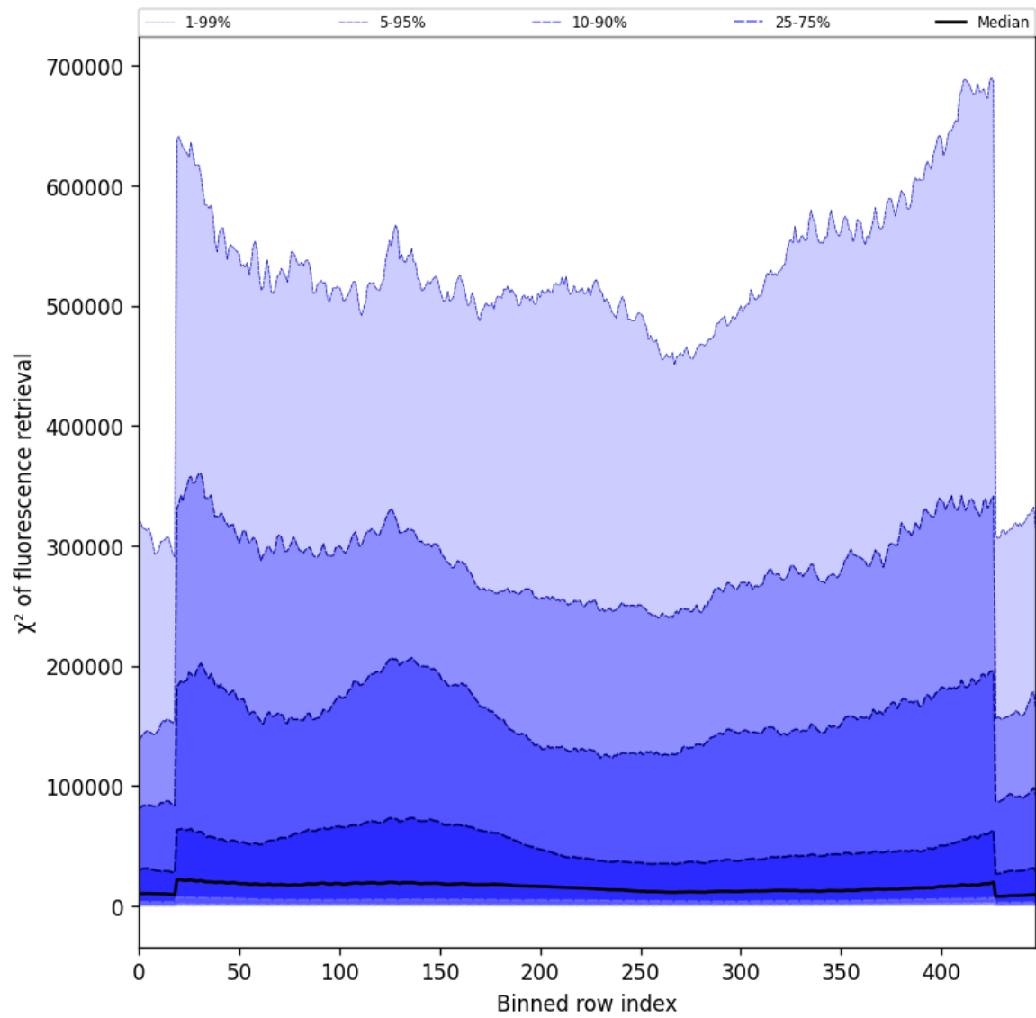
Figure 59: Along track statistics of “ \chi^2 of fluorescence retrieval” for 2024-10-01 to 2024-10-03
