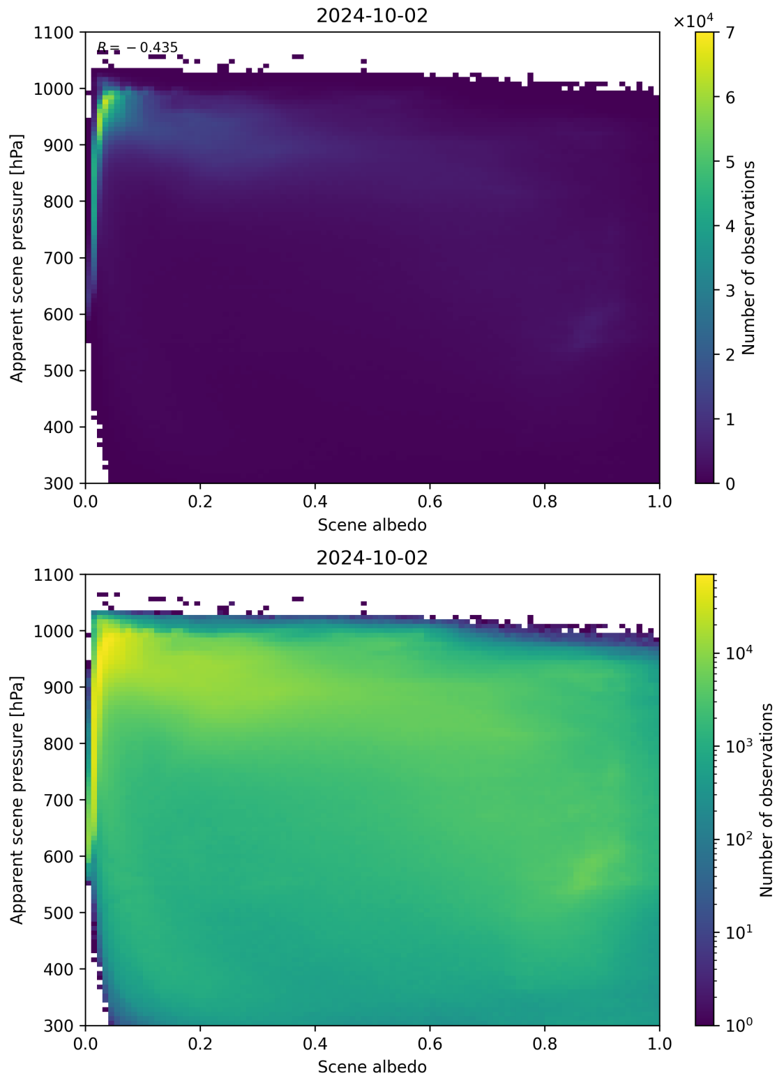
Figure 111: Scatter density plot of “Scene albedo” against “Apparent scene pressure” for 2024-10-01 to 2024-10-03.
