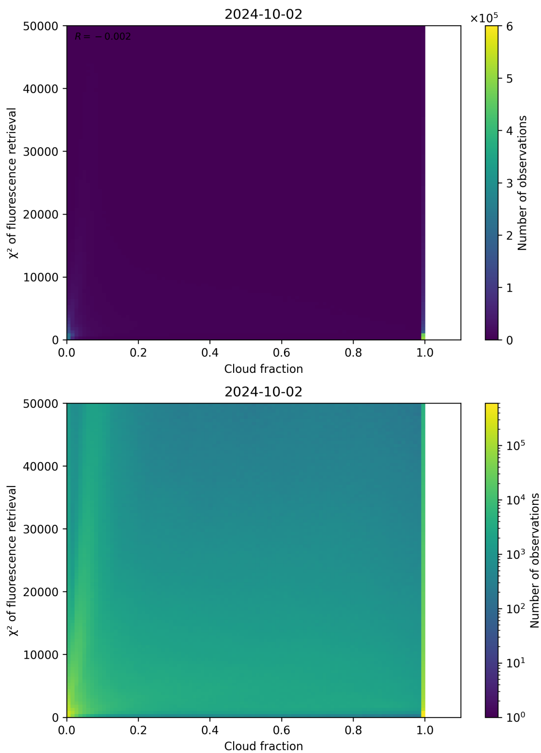
Figure 78: Scatter density plot of “Cloud fraction” against “ \chi^2 of fluorescence retrieval” for 2024-10-01 to 2024-10-03.
