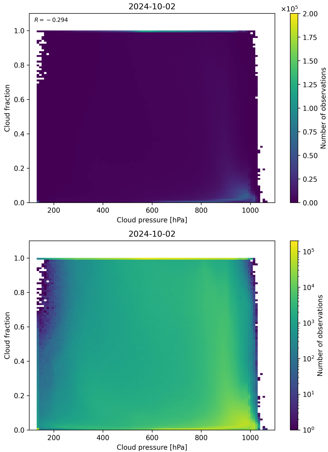
Figure 87: Scatter density plot of “Cloud pressure” against “Cloud fraction” for 2024-10-01 to 2024-10-03.
