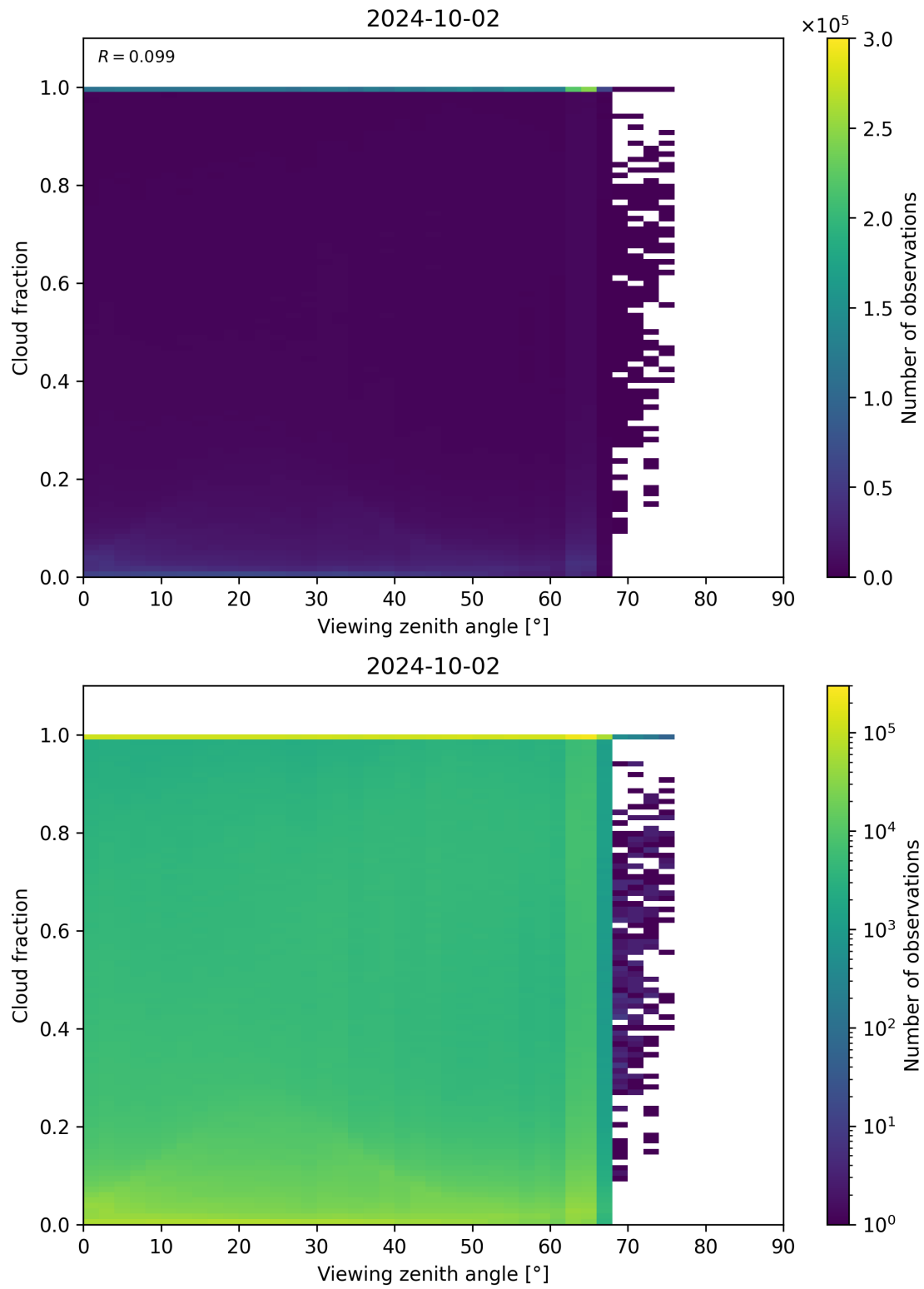
Figure 132: Scatter density plot of “Viewing zenith angle” against “Cloud fraction” for 2024-10-01 to 2024-10-03.
