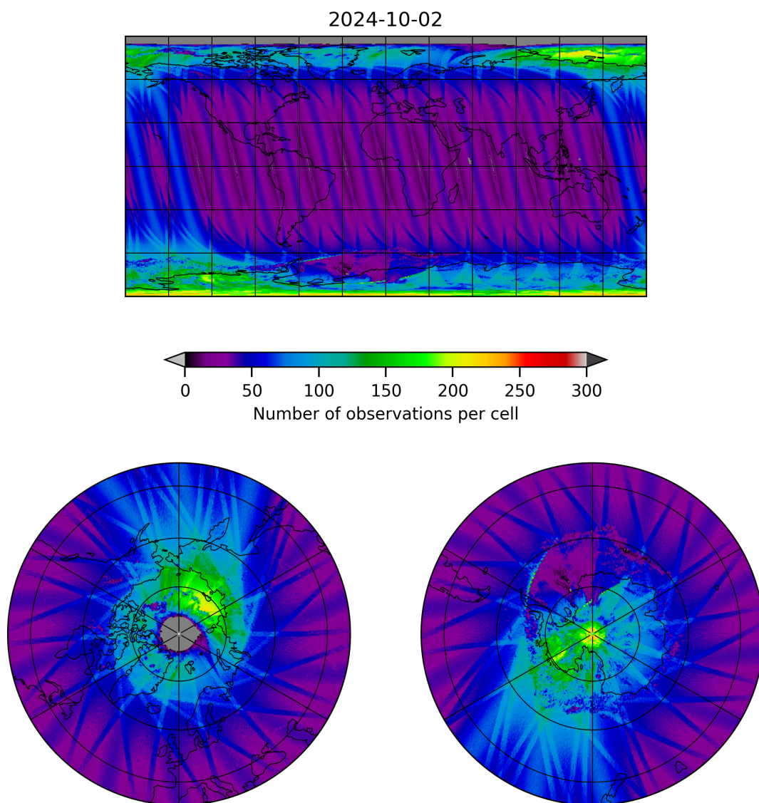
Figure 11: Map of the number of observations for 2024-10-01 to 2024-10-03
