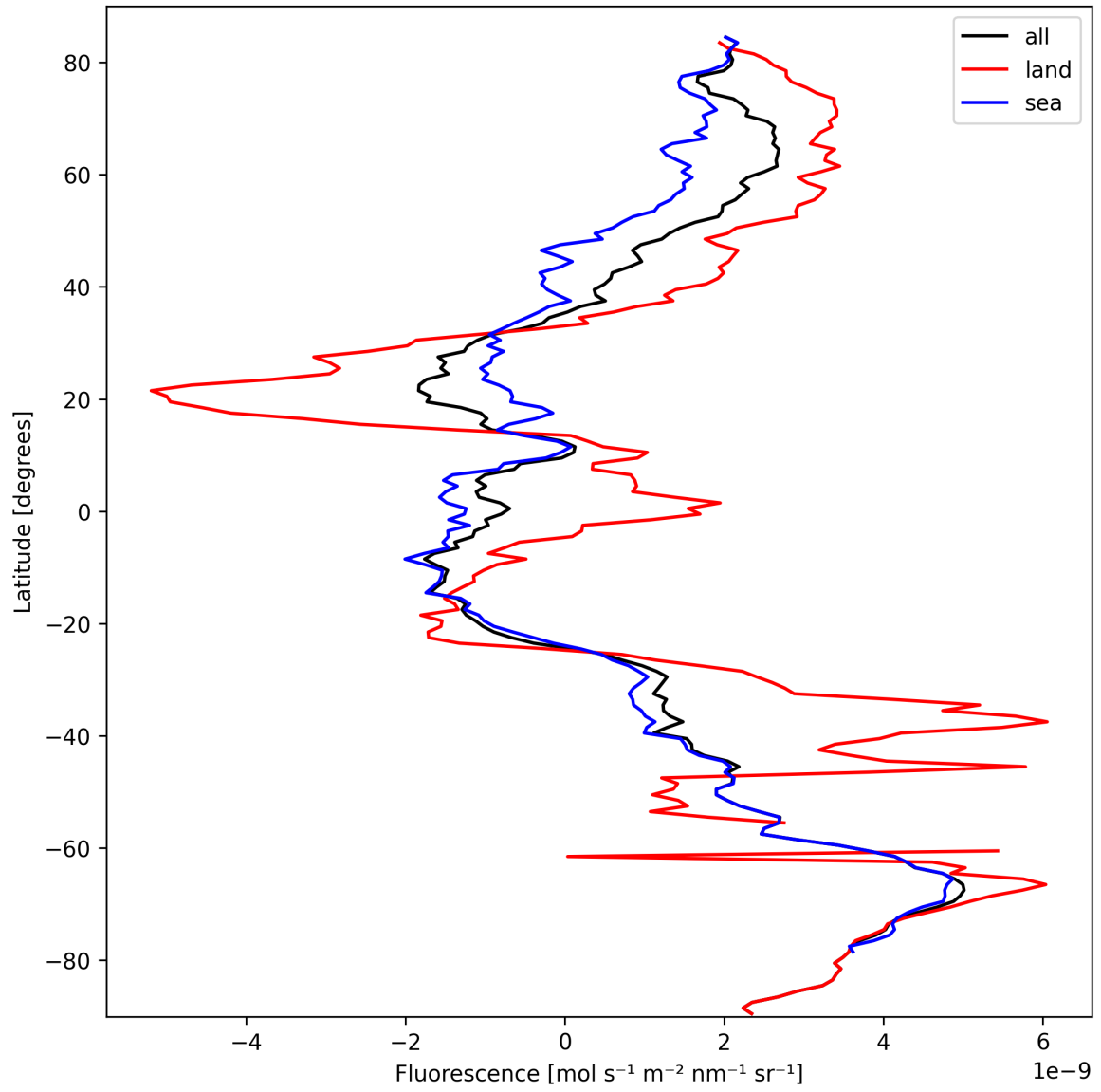
Figure 23: Zonal average of “Fluorescence” for 2024-10-01 to 2024-10-03.
