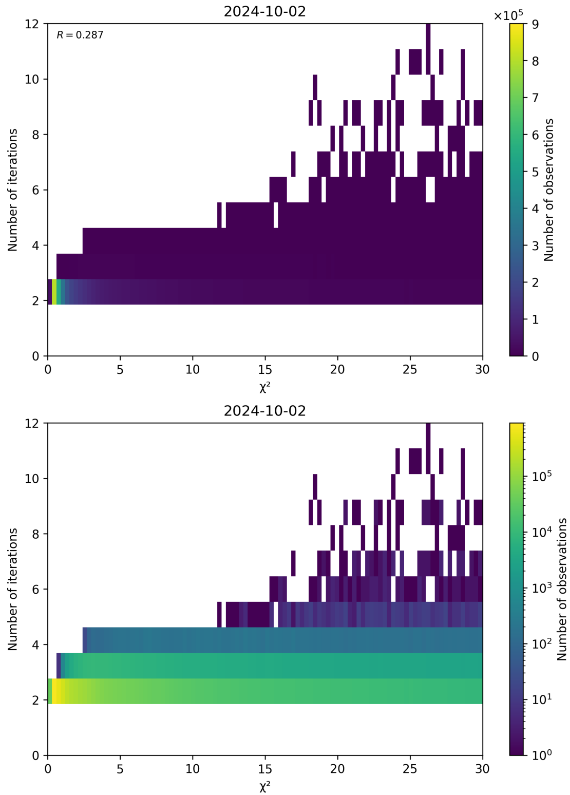
Figure 73: Scatter density plot of “ \chi^2 ” against “Number of iterations” for 2024-10-01 to 2024-10-03.
