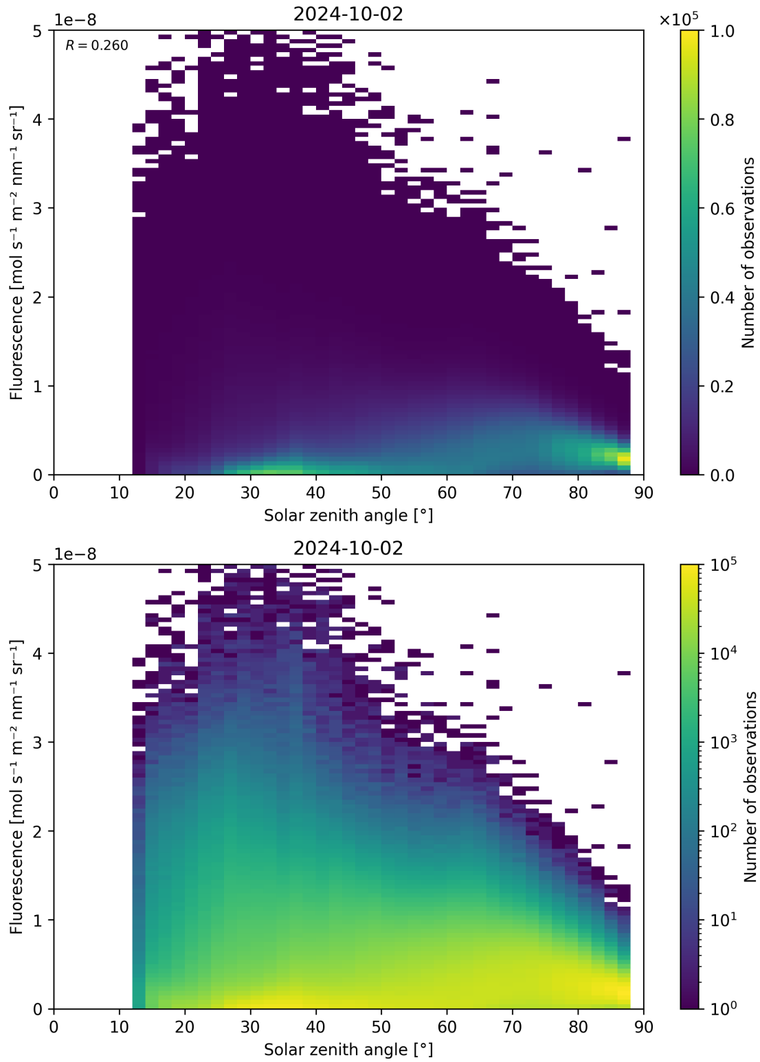
Figure 123: Scatter density plot of “Solar zenith angle” against “Fluorescence” for 2024-10-01 to 2024-10-03.
