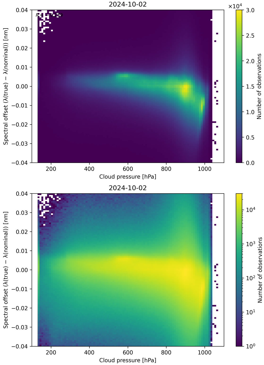
Figure 92: Scatter density plot of “Cloud pressure” against “Spectral offset ( \lambda_{\text{true}} - \lambda_{\text{nominal}} )” for 2024-10-01 to 2024-10-03.
