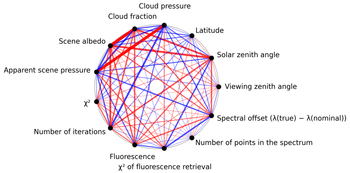
Figure 1: Map of correlation graph for 2024-10-01 to 2024-10-03.
