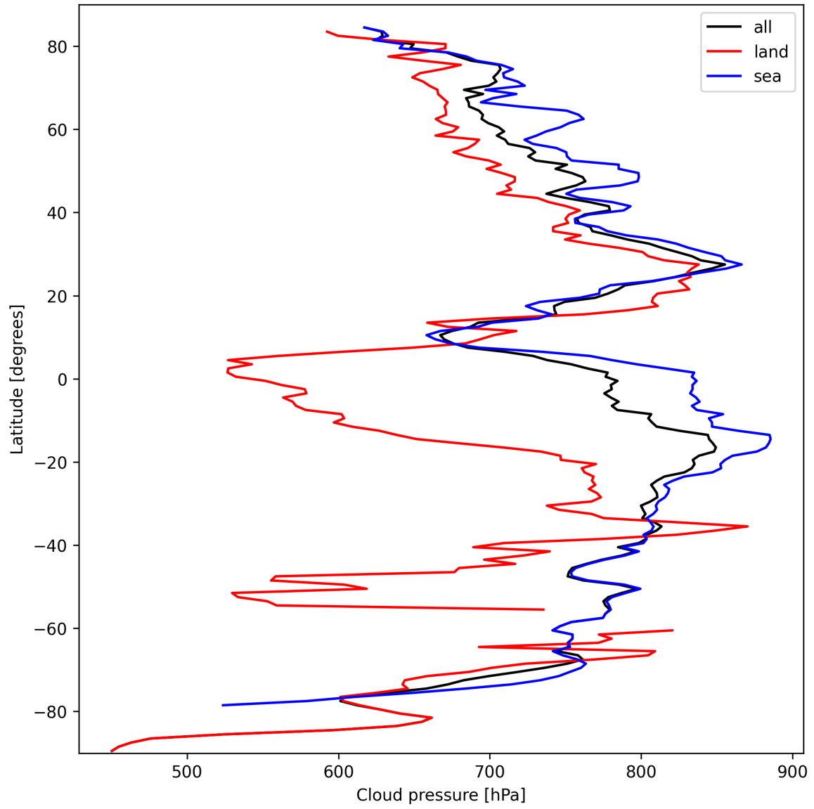
Figure 13: Zonal average of “Cloud pressure” for 2024-10-01 to 2024-10-03.
