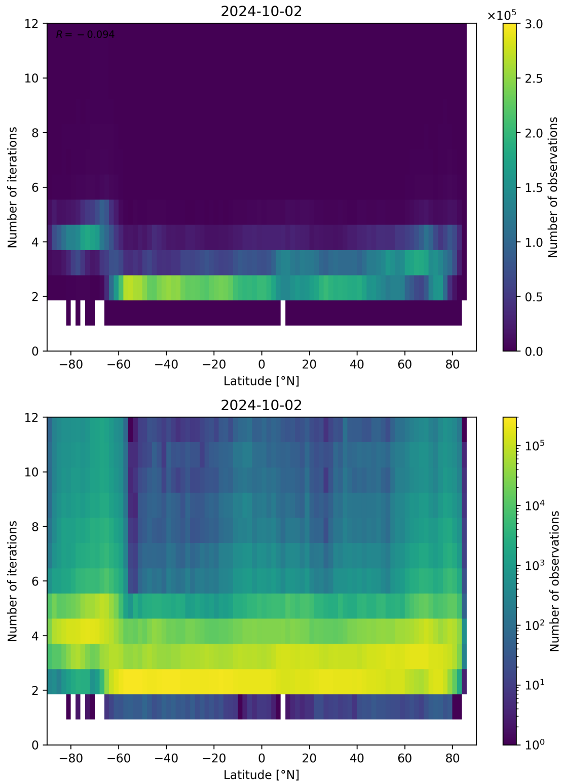
Figure 102: Scatter density plot of “Latitude” against “Number of iterations” for 2024-10-01 to 2024-10-03.
