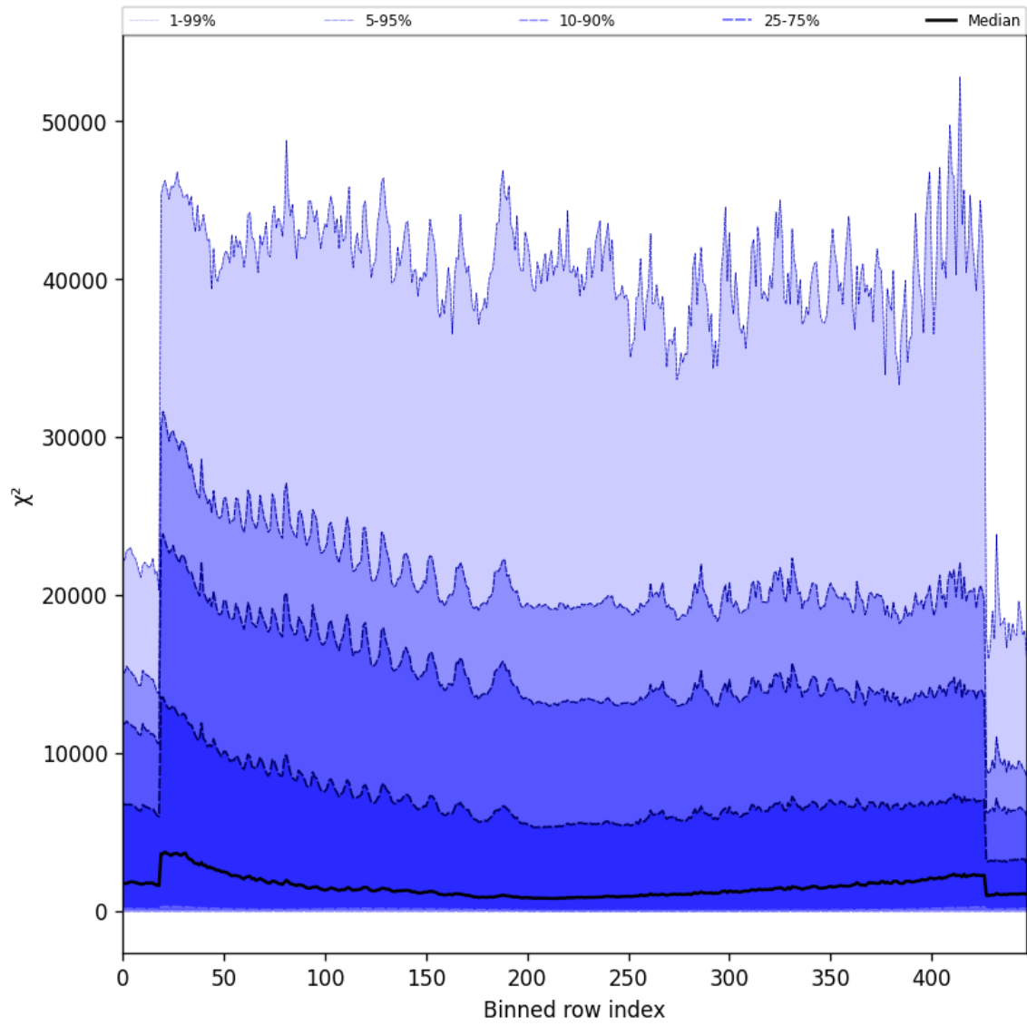
Figure 55: Along track statistics of “ \chi^2 ” for 2024-10-01 to 2024-10-03
