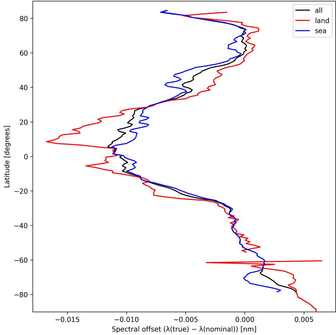
Figure 28: Zonal average of “Spectral offset ( \lambda_{\text{true}} - \lambda_{\text{nominal}} )” for 2024-10-01 to 2024-10-03.
