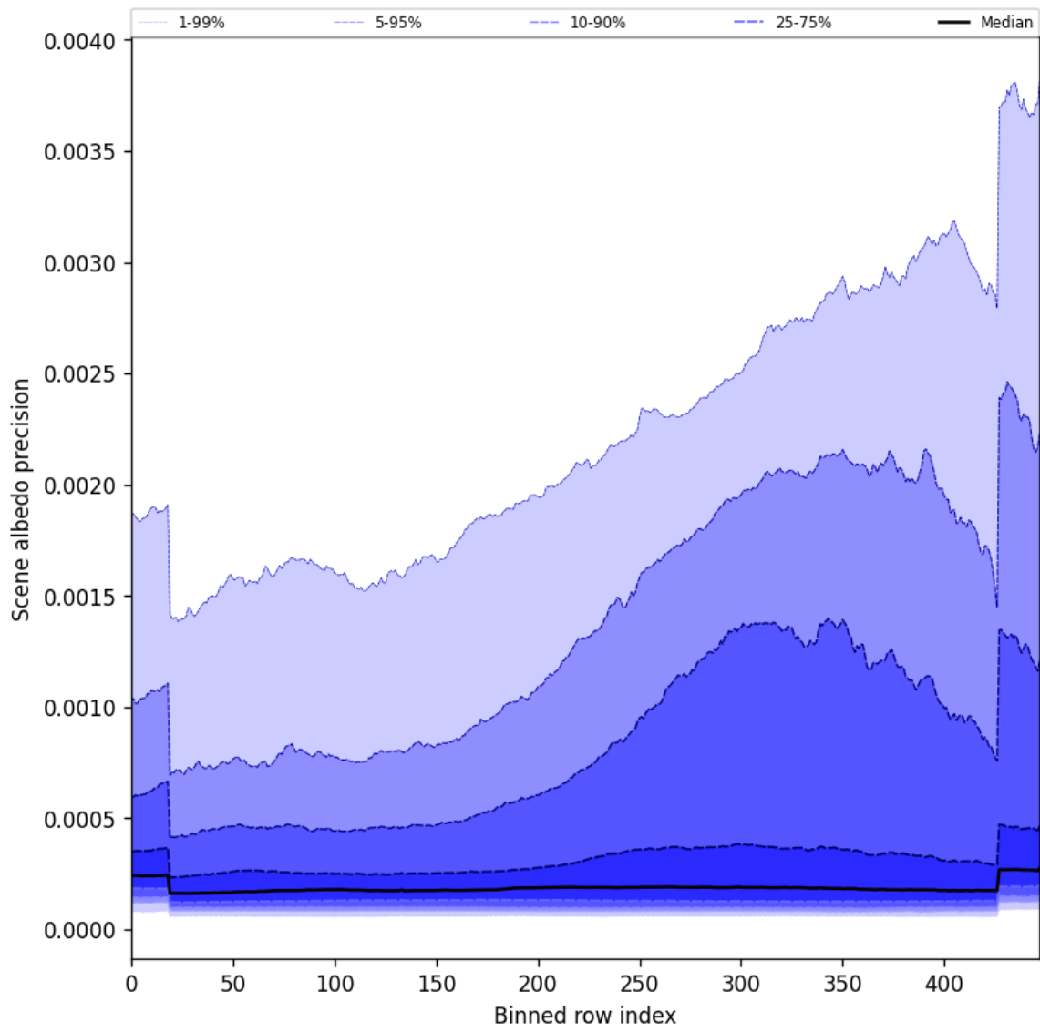
Figure 52: Along track statistics of “Scene albedo precision” for 2024-10-01 to 2024-10-03
