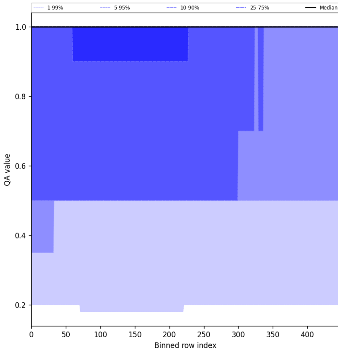
Figure 46: Along track statistics of “QA value” for 2024-10-01 to 2024-10-03
