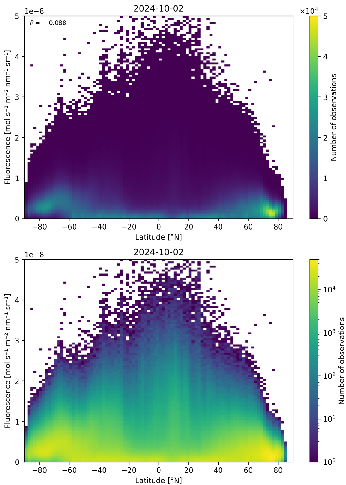
Figure 101: Scatter density plot of “Latitude” against “Fluorescence” for 2024-10-01 to 2024-10-03.
