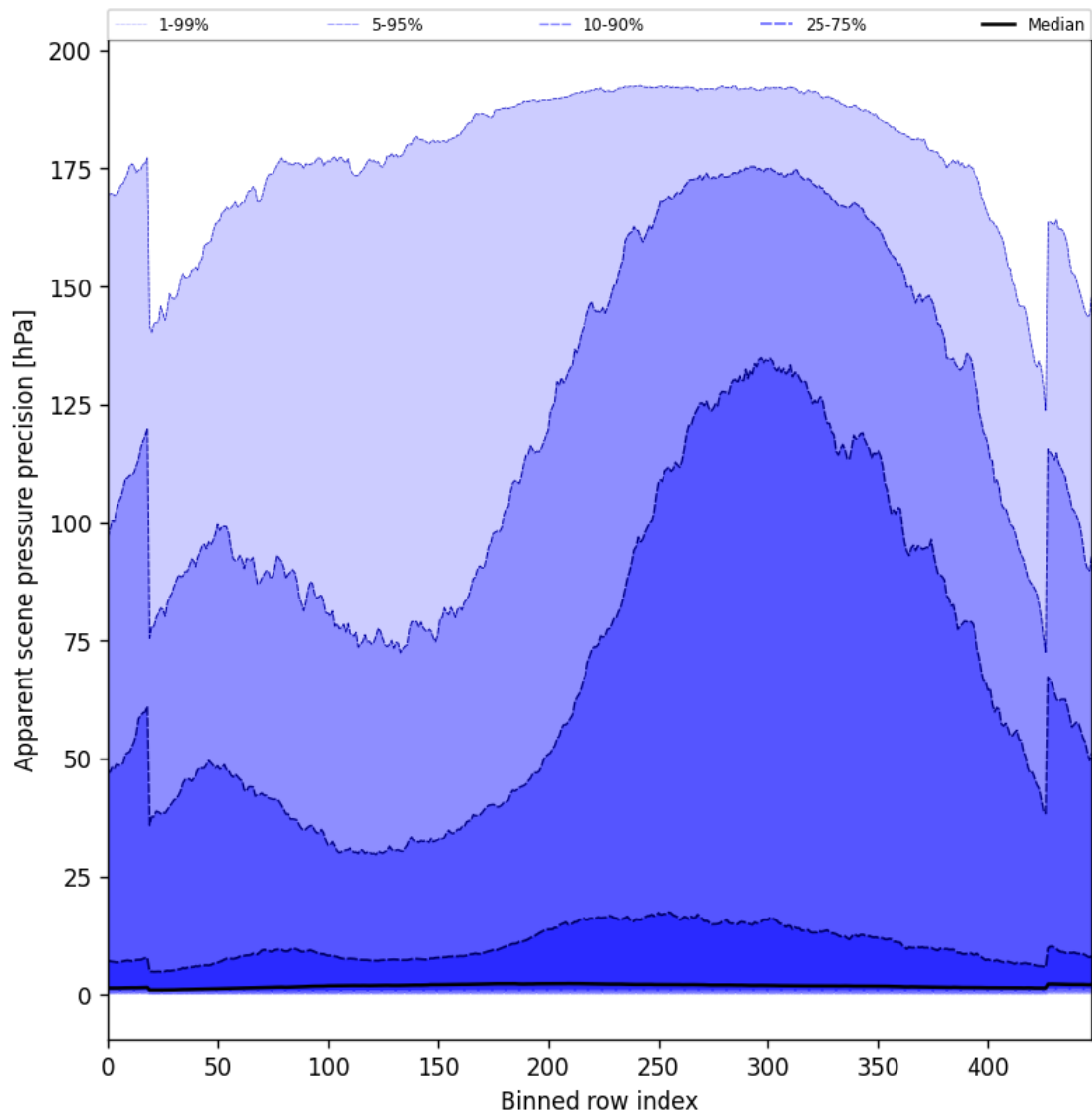
Figure 54: Along track statistics of “Apparent scene pressure precision” for 2024-10-01 to 2024-10-03
