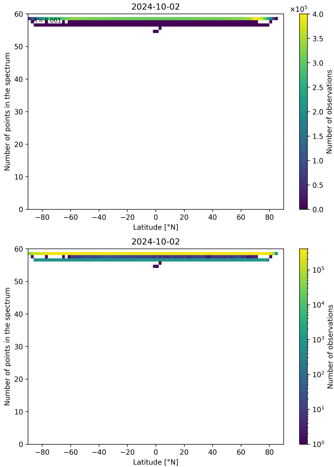
Figure 103: Scatter density plot of “Latitude” against “Number of points in the spectrum” for 2024-10-01 to 2024-10-03.
