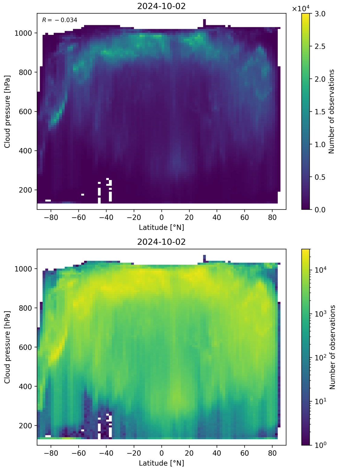
Figure 100: Scatter density plot of “Latitude” against “Cloud pressure” for 2024-10-01 to 2024-10-03.
