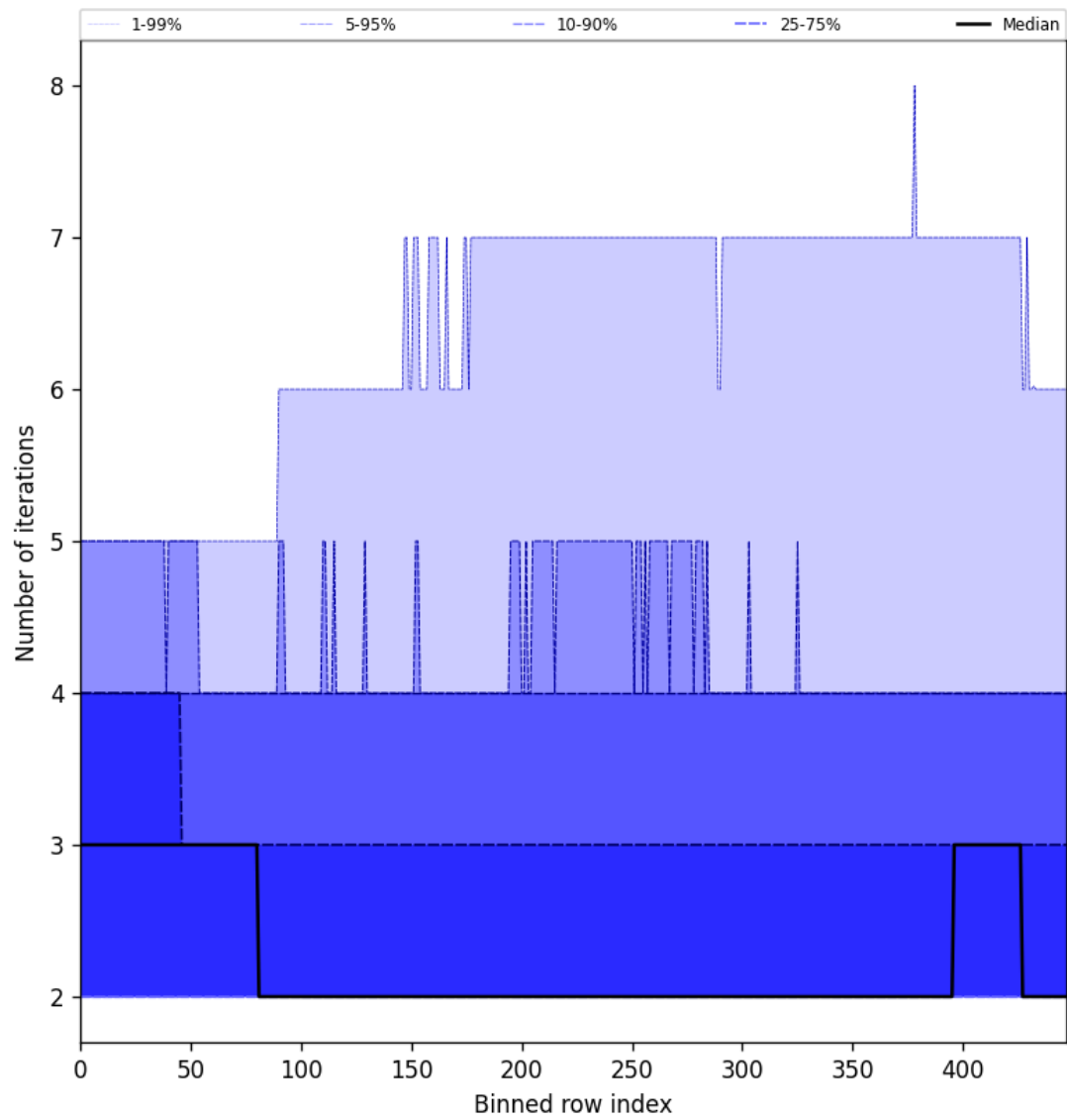
Figure 56: Along track statistics of “Number of iterations” for 2024-10-01 to 2024-10-03
