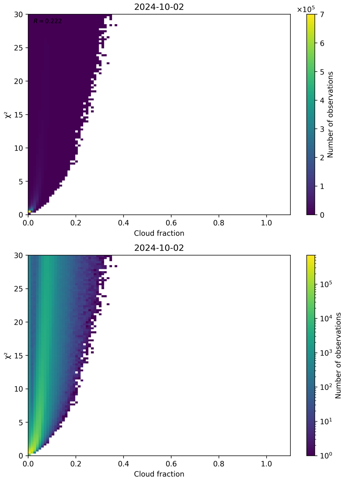
Figure 77: Scatter density plot of “Cloud fraction” against “ \chi^2 ” for 2024-10-01 to 2024-10-03.
