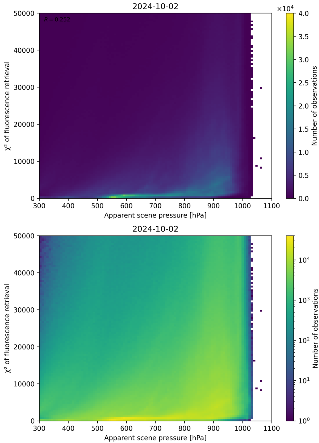
Figure 64: Scatter density plot of “Apparent scene pressure” against “ \chi^2 of fluorescence retrieval” for 2024-10-01 to 2024-10-03.
