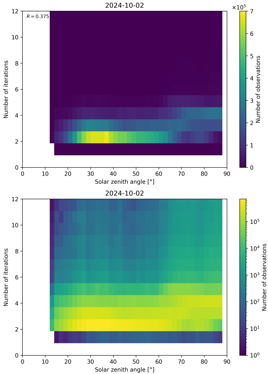
Figure 125: Scatter density plot of “Solar zenith angle” against “Number of iterations” for 2024-10-01 to 2024-10-03.
