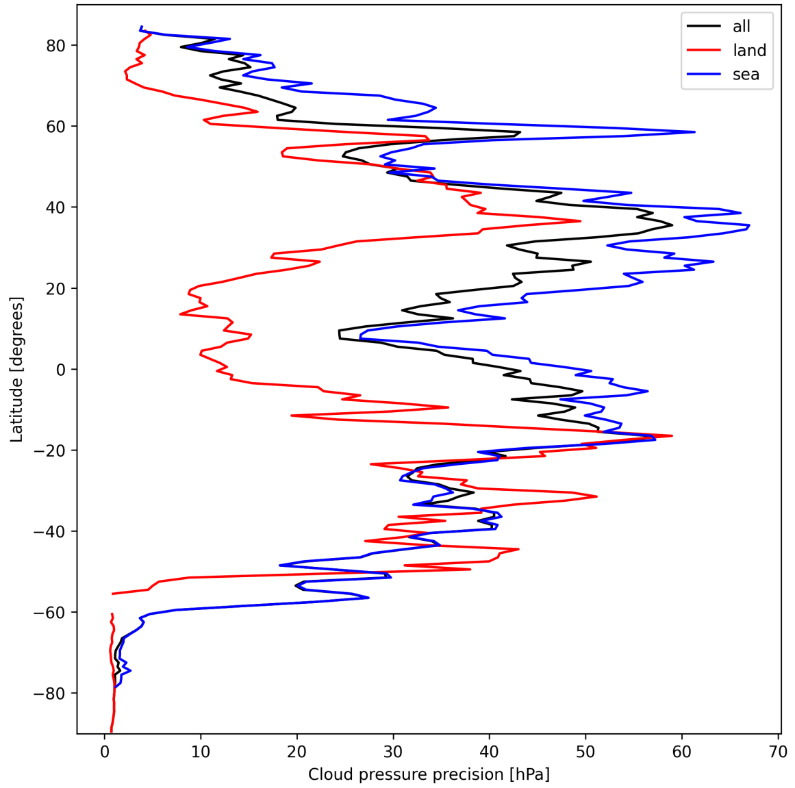
Figure 14: Zonal average of “Cloud pressure precision” for 2024-10-01 to 2024-10-03.
