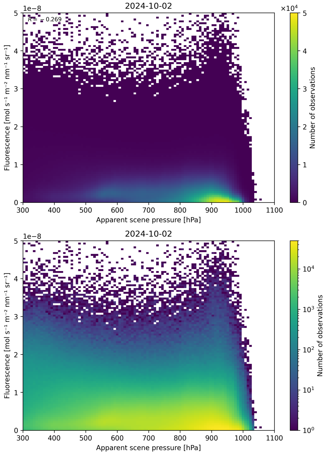
Figure 65: Scatter density plot of “Apparent scene pressure” against “Fluorescence” for 2024-10-01 to 2024-10-03.
