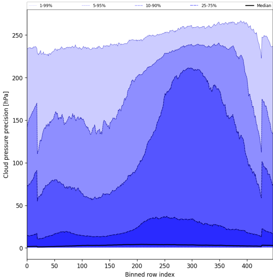
Figure 48: Along track statistics of “Cloud pressure precision” for 2024-10-01 to 2024-10-03
