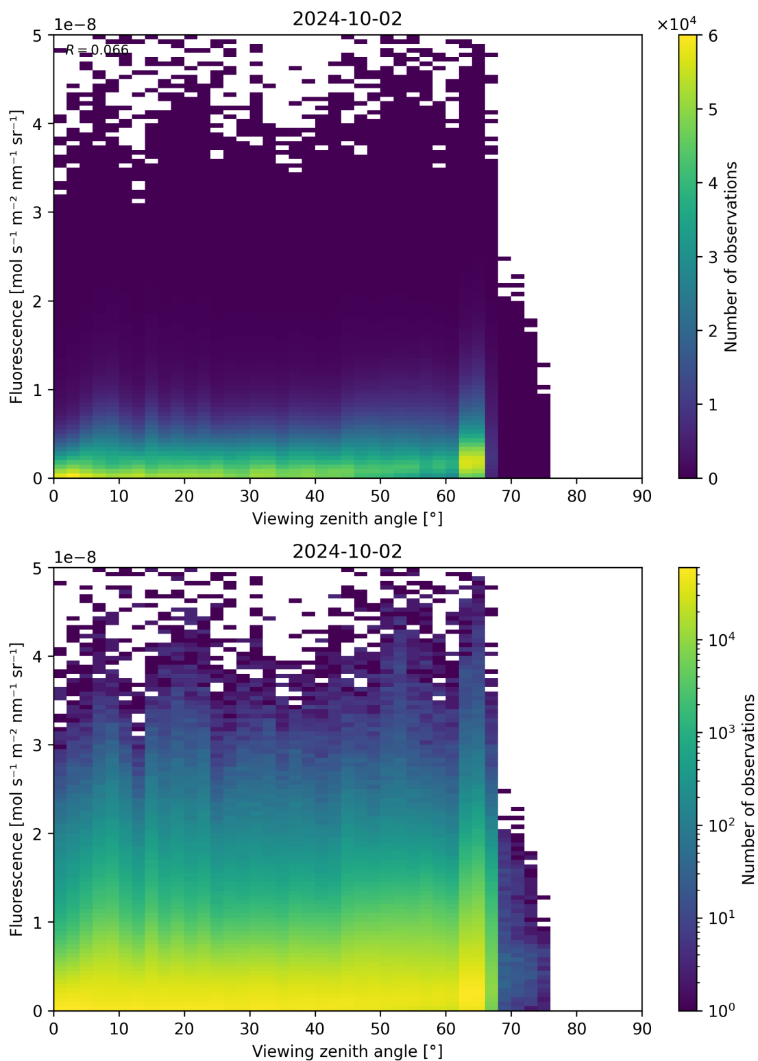
Figure 134: Scatter density plot of “Viewing zenith angle” against “Fluorescence” for 2024-10-01 to 2024-10-03.
