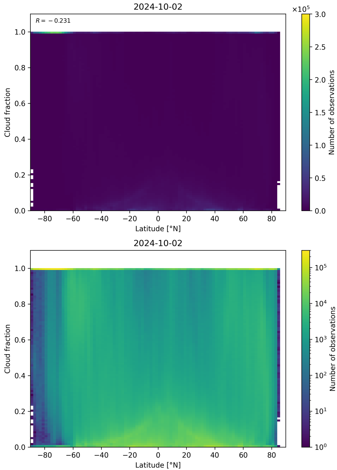
Figure 99: Scatter density plot of “Latitude” against “Cloud fraction” for 2024-10-01 to 2024-10-03.
