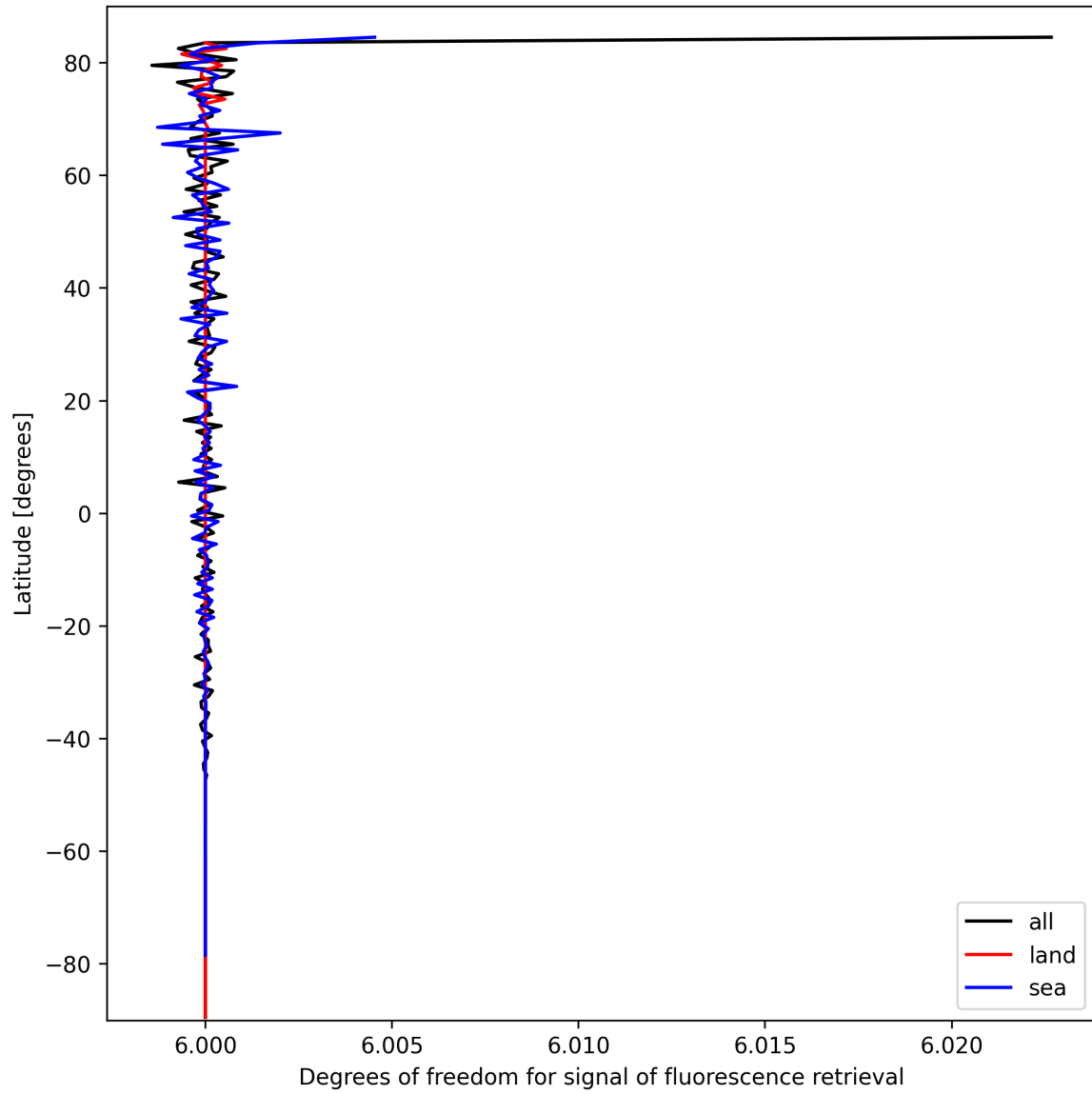
Figure 26: Zonal average of “Degrees of freedom for signal of fluorescence retrieval” for 2024-10-01 to 2024-10-03.
