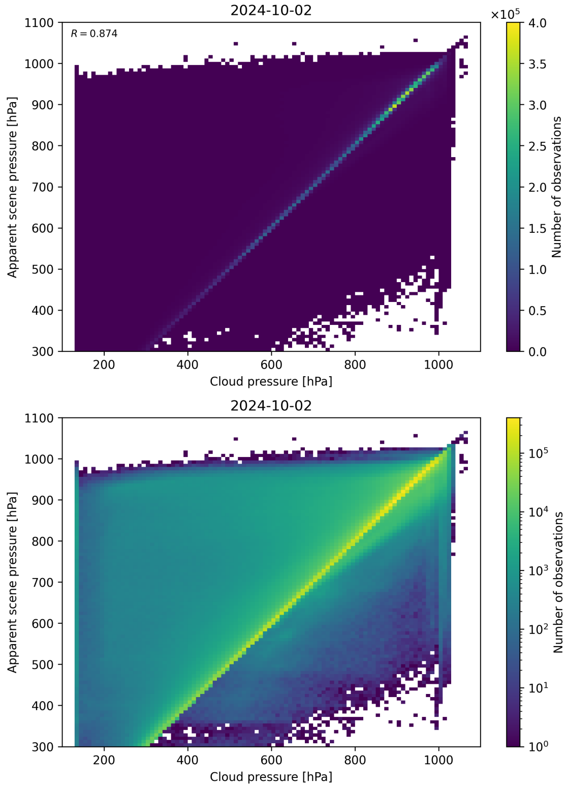
Figure 84: Scatter density plot of “Cloud pressure” against “Apparent scene pressure” for 2024-10-01 to 2024-10-03.
