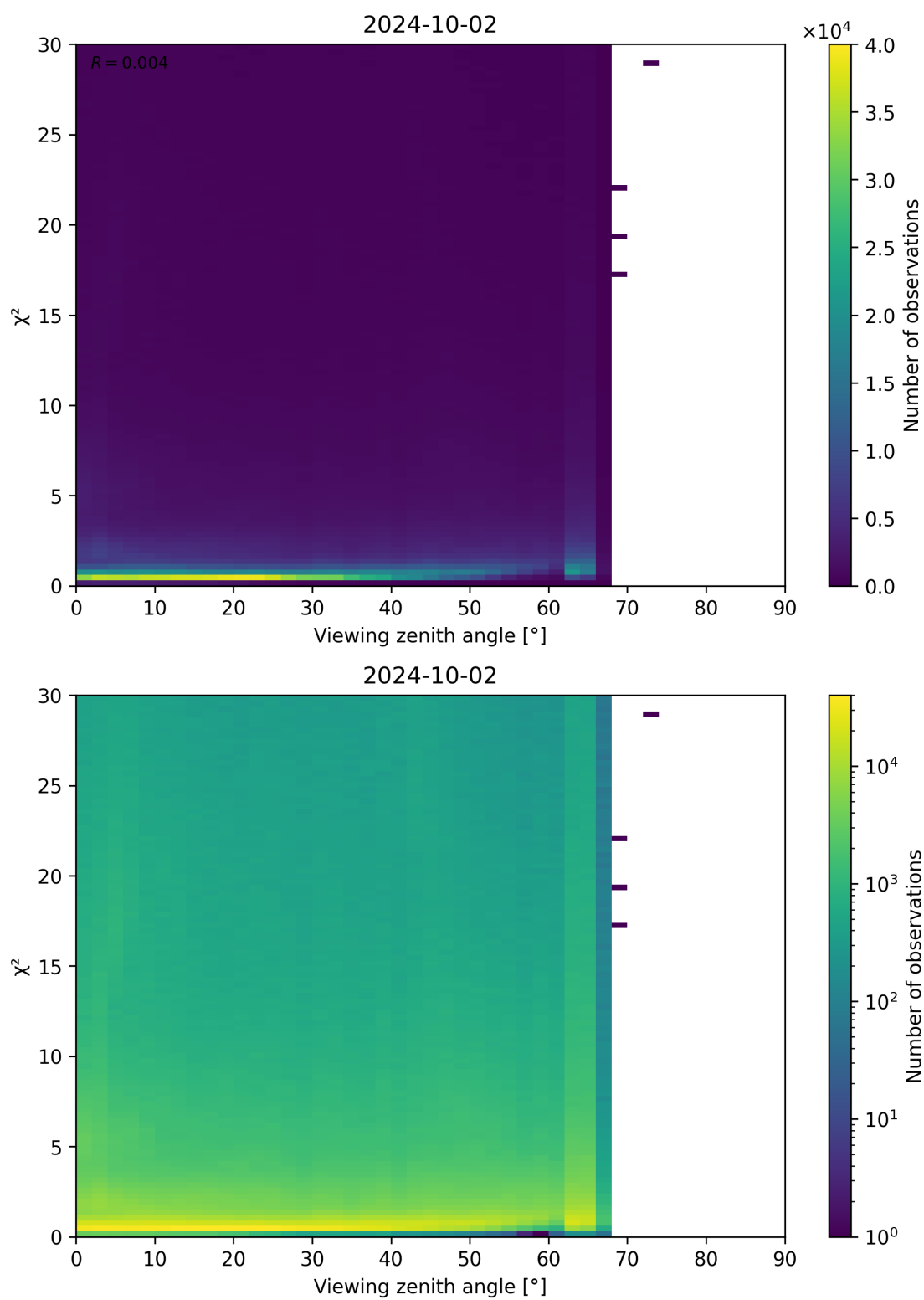
Figure 130: Scatter density plot of “Viewing zenith angle” against “ \chi^2 ” for 2024-10-01 to 2024-10-03.
