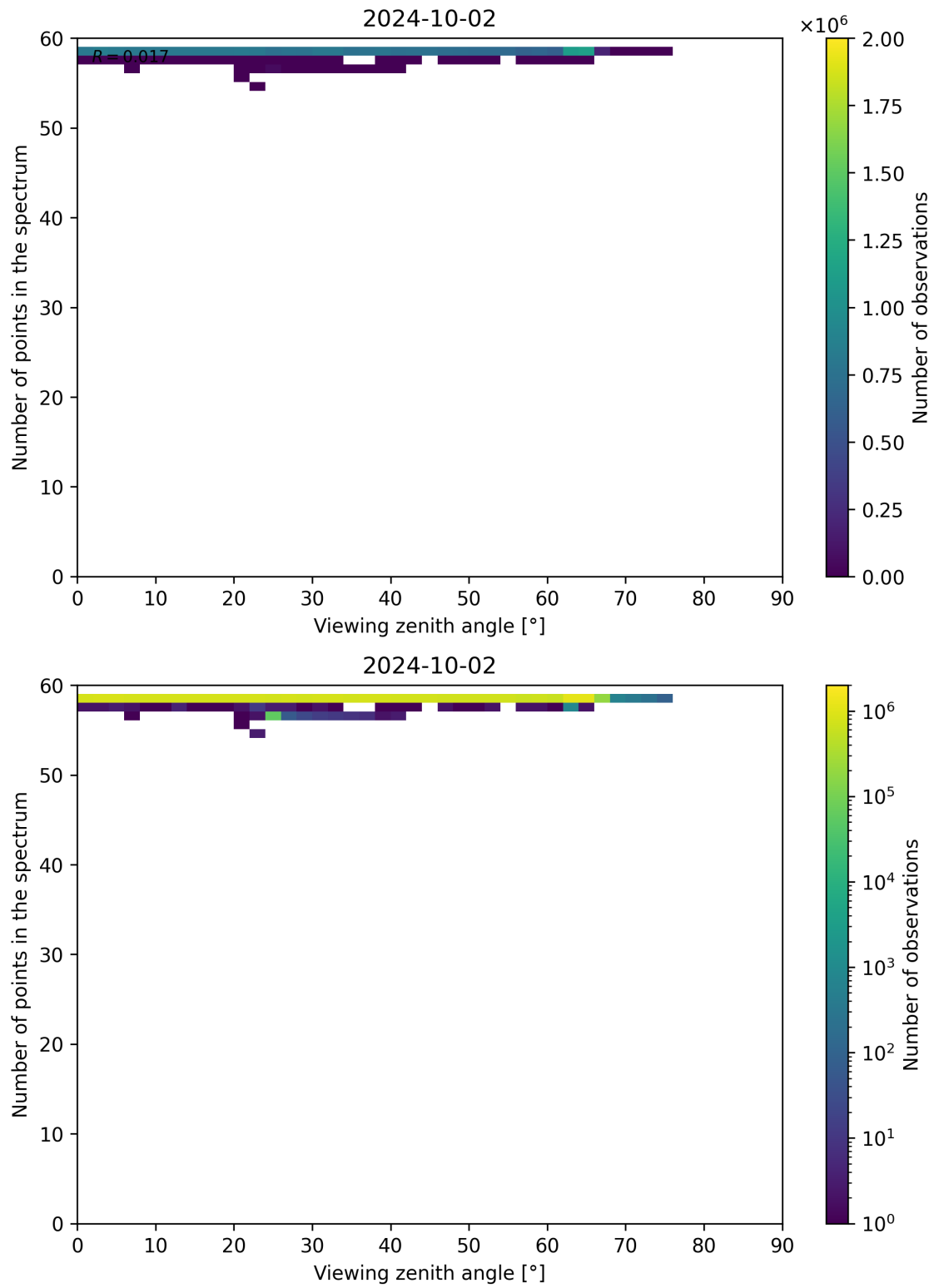
Figure 137: Scatter density plot of “Viewing zenith angle” against “Number of points in the spectrum” for 2024-10-01 to 2024-10-03.
