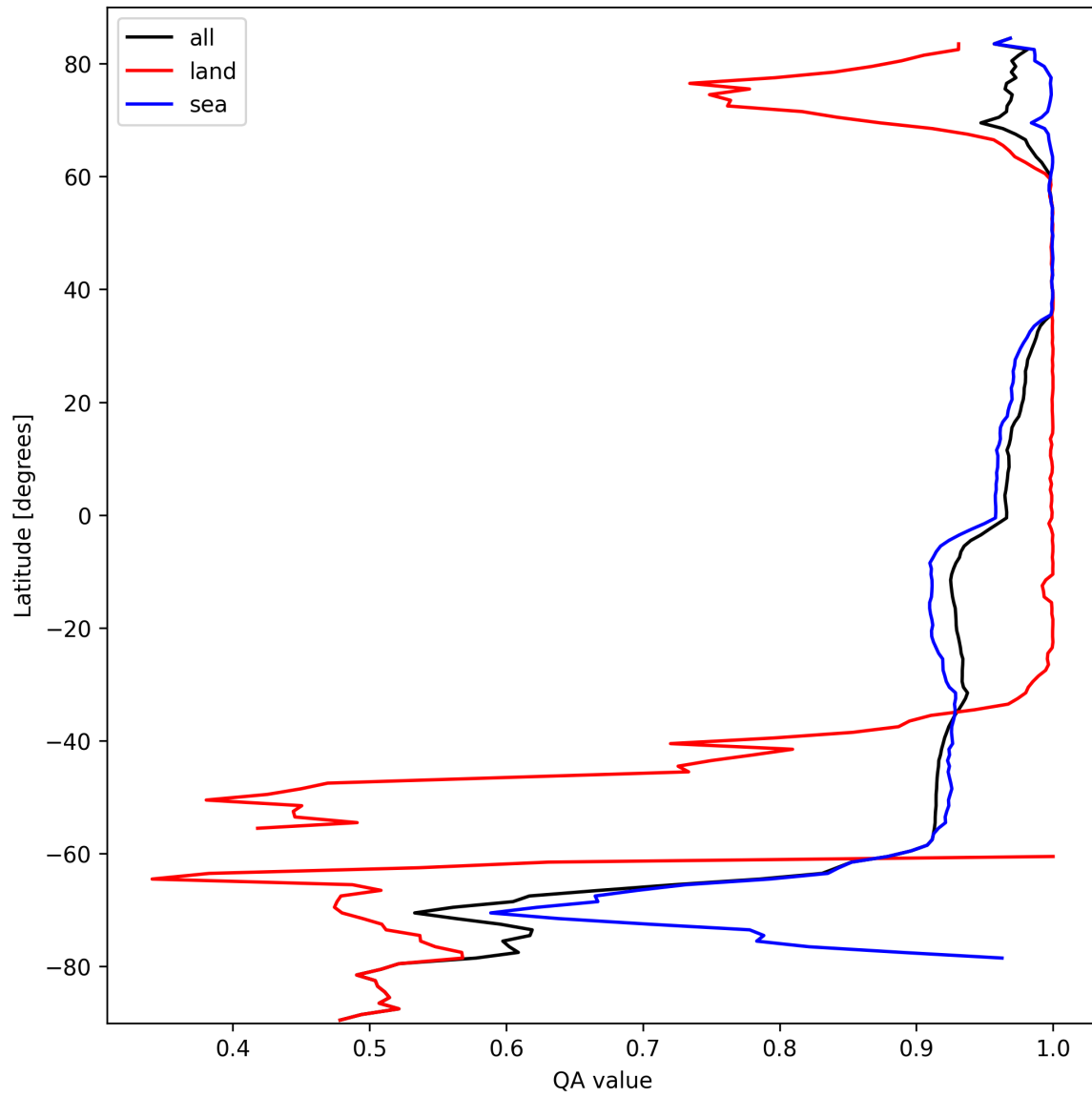
Figure 12: Zonal average of “QA value” for 2024-10-01 to 2024-10-03.
