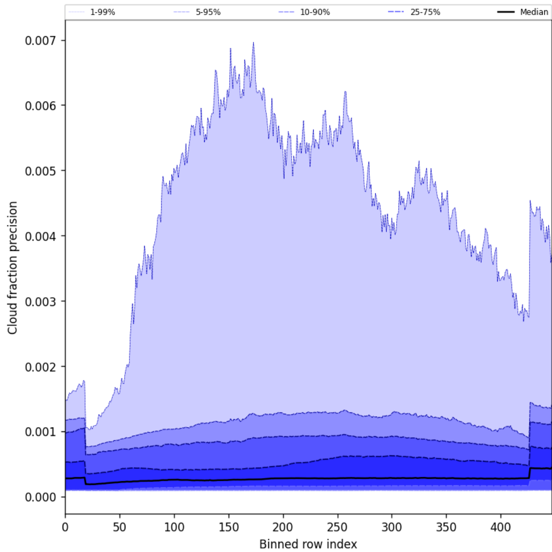
Figure 50: Along track statistics of “Cloud fraction precision” for 2024-10-01 to 2024-10-03
