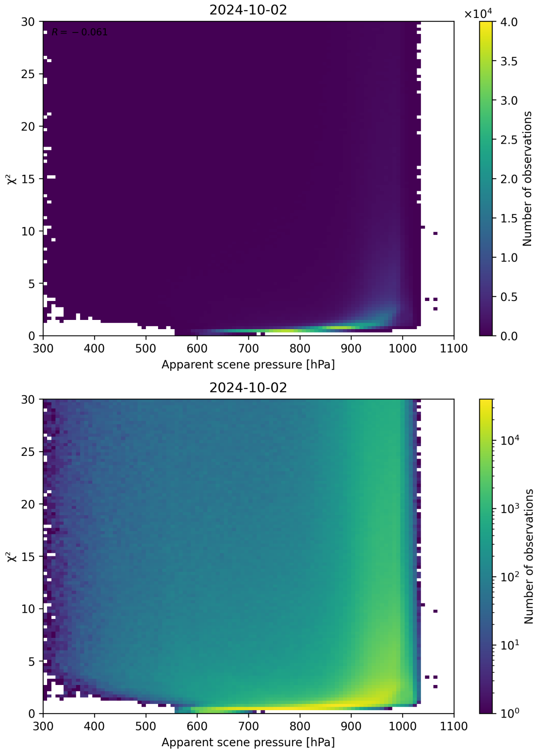
Figure 63: Scatter density plot of “Apparent scene pressure” against “ \chi^2 ” for 2024-10-01 to 2024-10-03.
