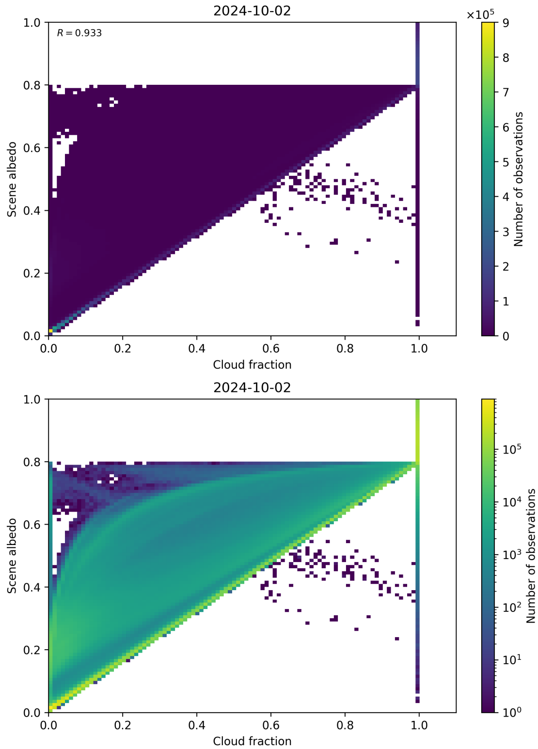
Figure 82: Scatter density plot of “Cloud fraction” against “Scene albedo” for 2024-10-01 to 2024-10-03.
