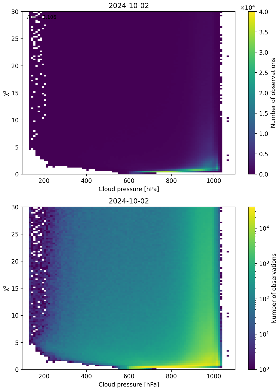
Figure 85: Scatter density plot of “Cloud pressure” against “ \chi^2 ” for 2024-10-01 to 2024-10-03.
