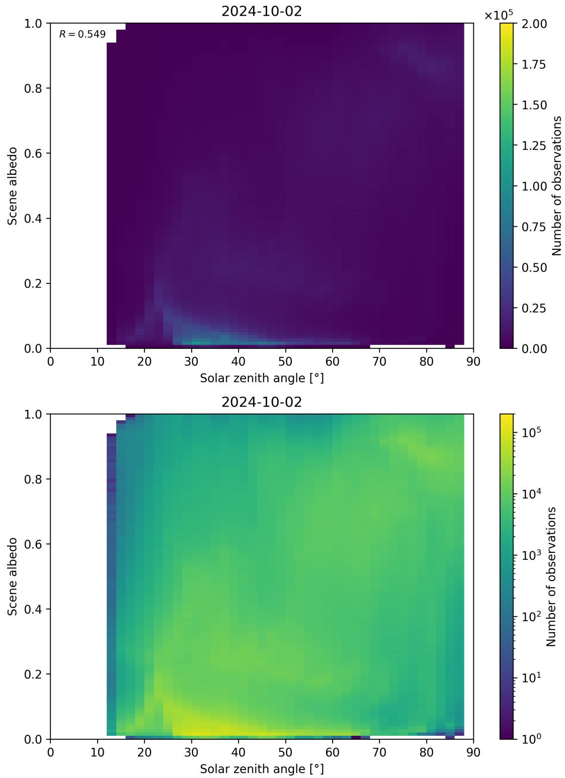
Figure 127: Scatter density plot of “Solar zenith angle” against “Scene albedo” for 2024-10-01 to 2024-10-03.
