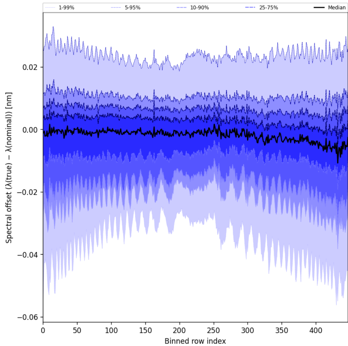
Figure 62: Along track statistics of “Spectral offset ( \lambda_{\text{true}} - \lambda_{\text{nominal}} )” for 2024-10-01 to 2024-10-03
