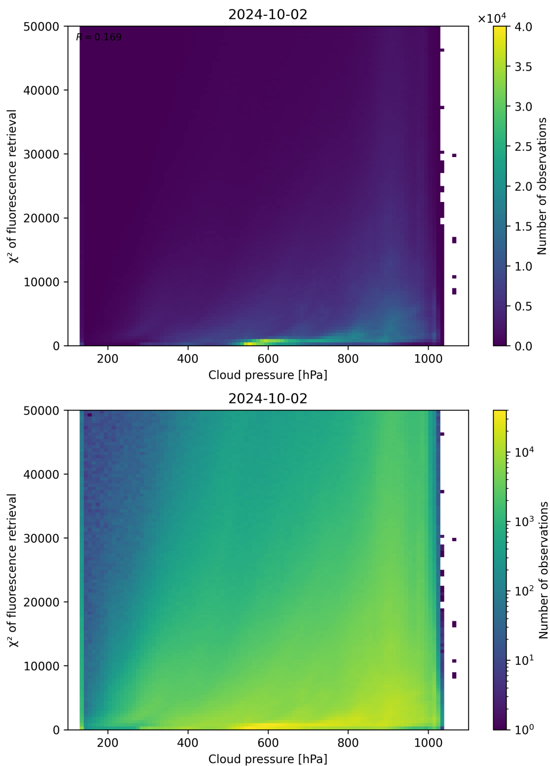
Figure 86: Scatter density plot of “Cloud pressure” against “ \chi^2 of fluorescence retrieval” for 2024-10-01 to 2024-10-03.
