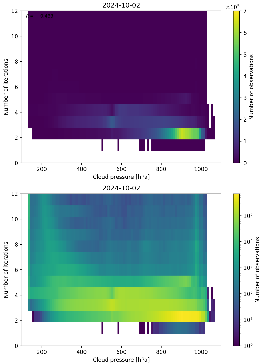
Figure 89: Scatter density plot of “Cloud pressure” against “Number of iterations” for 2024-10-01 to 2024-10-03.
