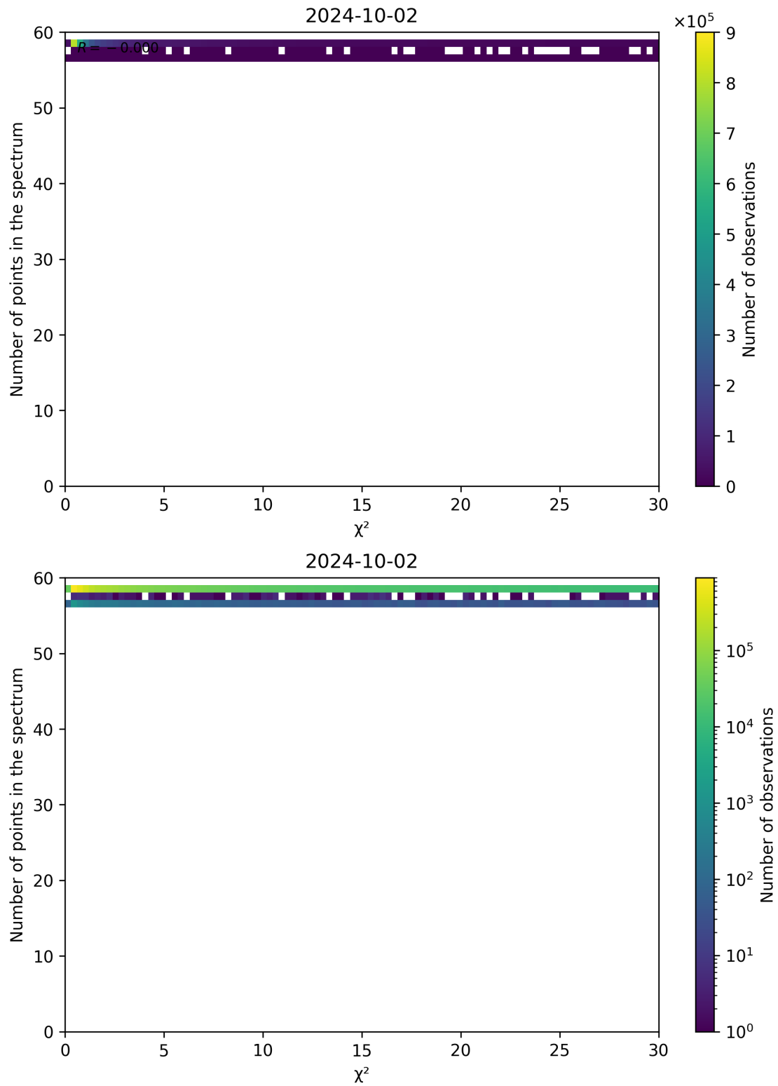
Figure 74: Scatter density plot of “ \chi^2 ” against “Number of points in the spectrum” for 2024-10-01 to 2024-10-03.
