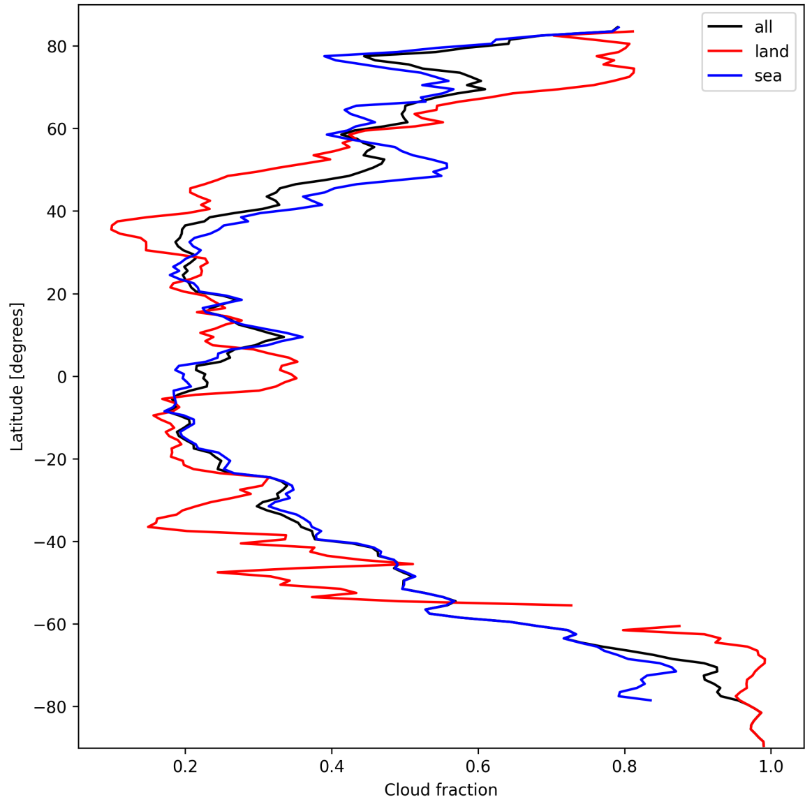
Figure 15: Zonal average of “Cloud fraction” for 2024-10-01 to 2024-10-03.
