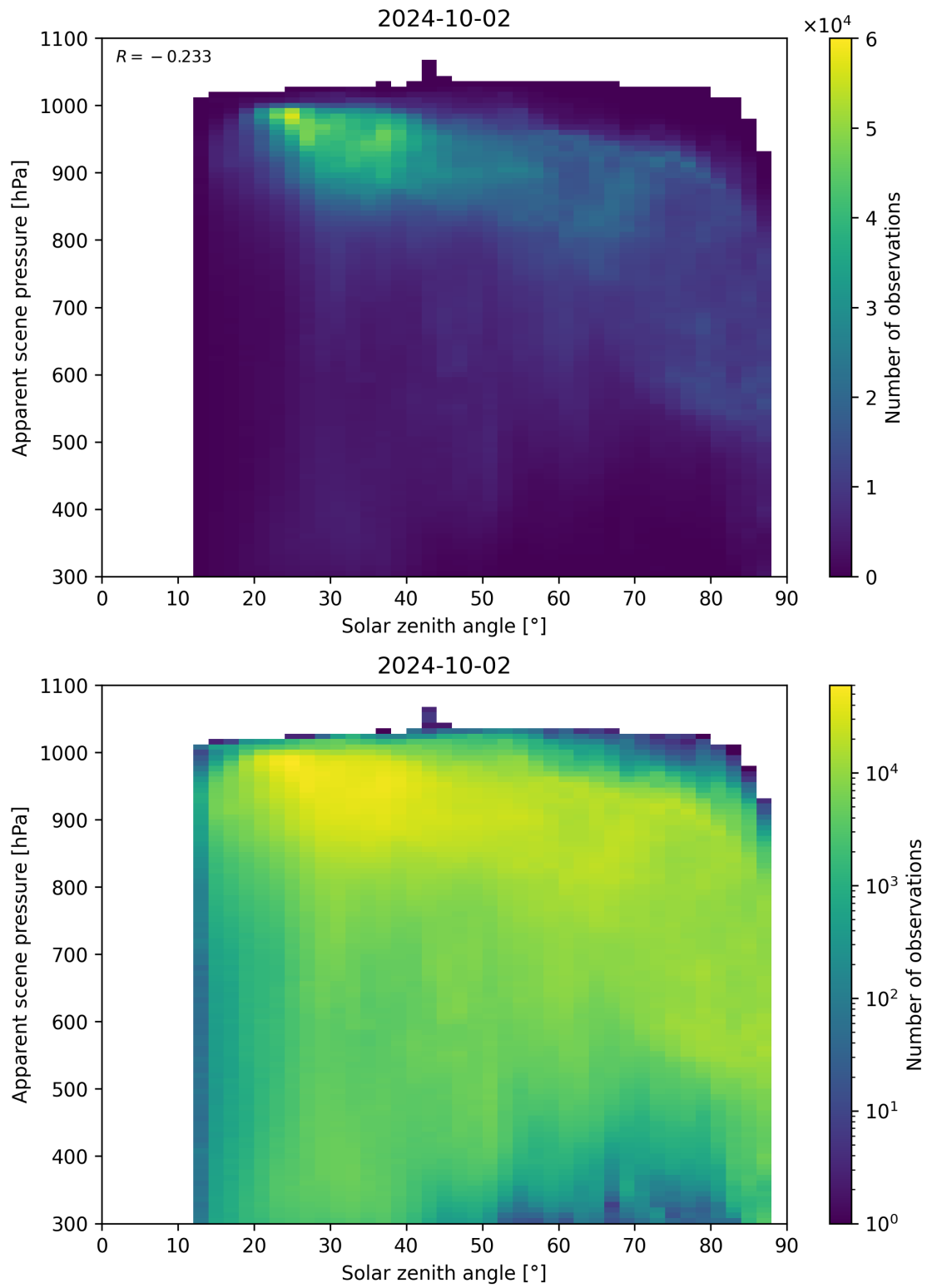
Figure 118: Scatter density plot of “Solar zenith angle” against “Apparent scene pressure” for 2024-10-01 to 2024-10-03.
