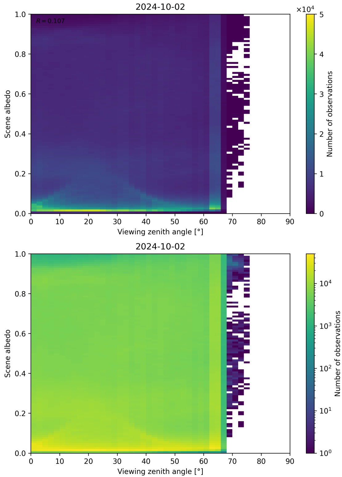
Figure 138: Scatter density plot of “Viewing zenith angle” against “Scene albedo” for 2024-10-01 to 2024-10-03.
