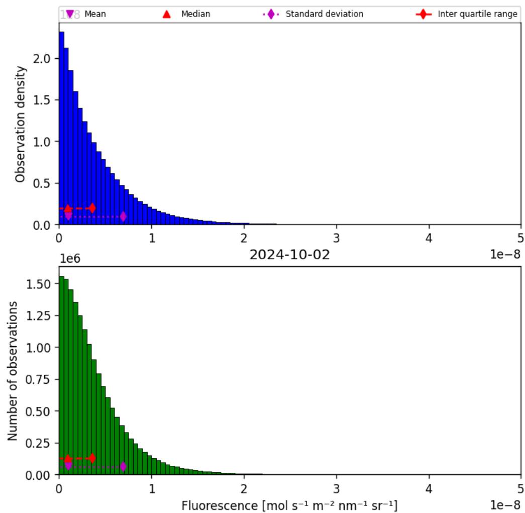
Figure 40: Histogram of “Fluorescence” for 2024-10-01 to 2024-10-03
