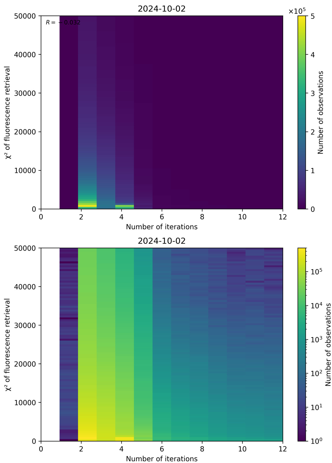
Figure 106: Scatter density plot of “Number of iterations” against “ \chi^2 of fluorescence retrieval” for 2024-10-01 to 2024-10-03.
