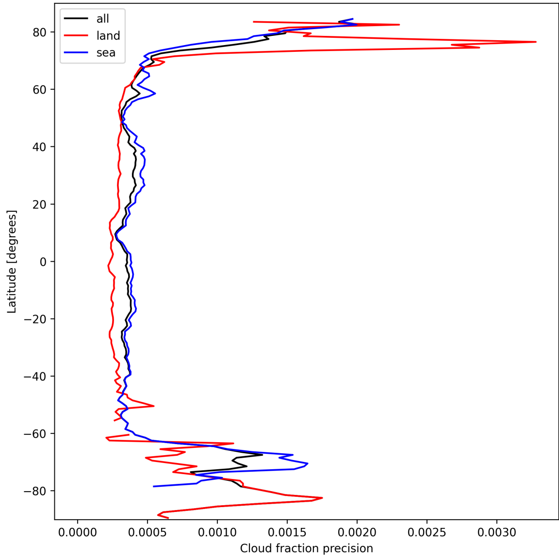
Figure 16: Zonal average of “Cloud fraction precision” for 2024-10-01 to 2024-10-03.
