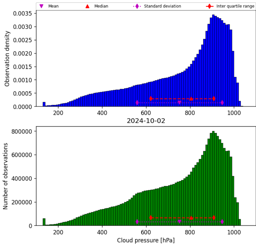
Figure 30: Histogram of “Cloud pressure” for 2024-10-01 to 2024-10-03
