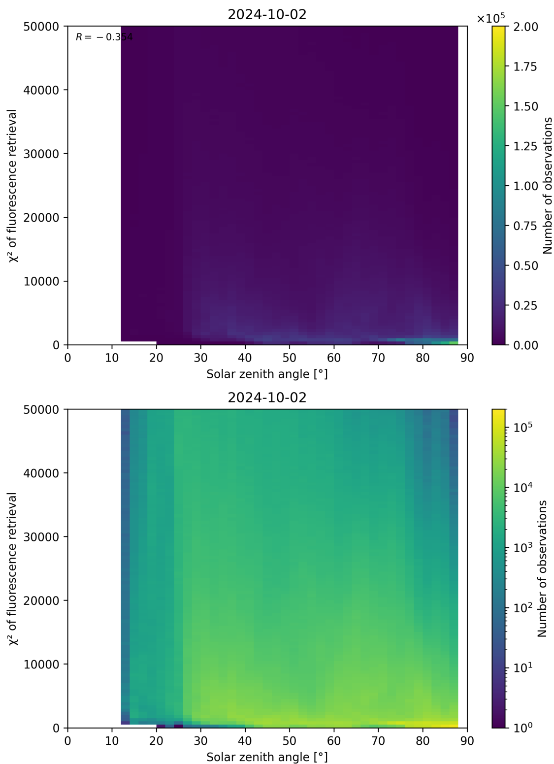
Figure 120: Scatter density plot of “Solar zenith angle” against “ \chi^2 of fluorescence retrieval” for 2024-10-01 to 2024-10-03.
