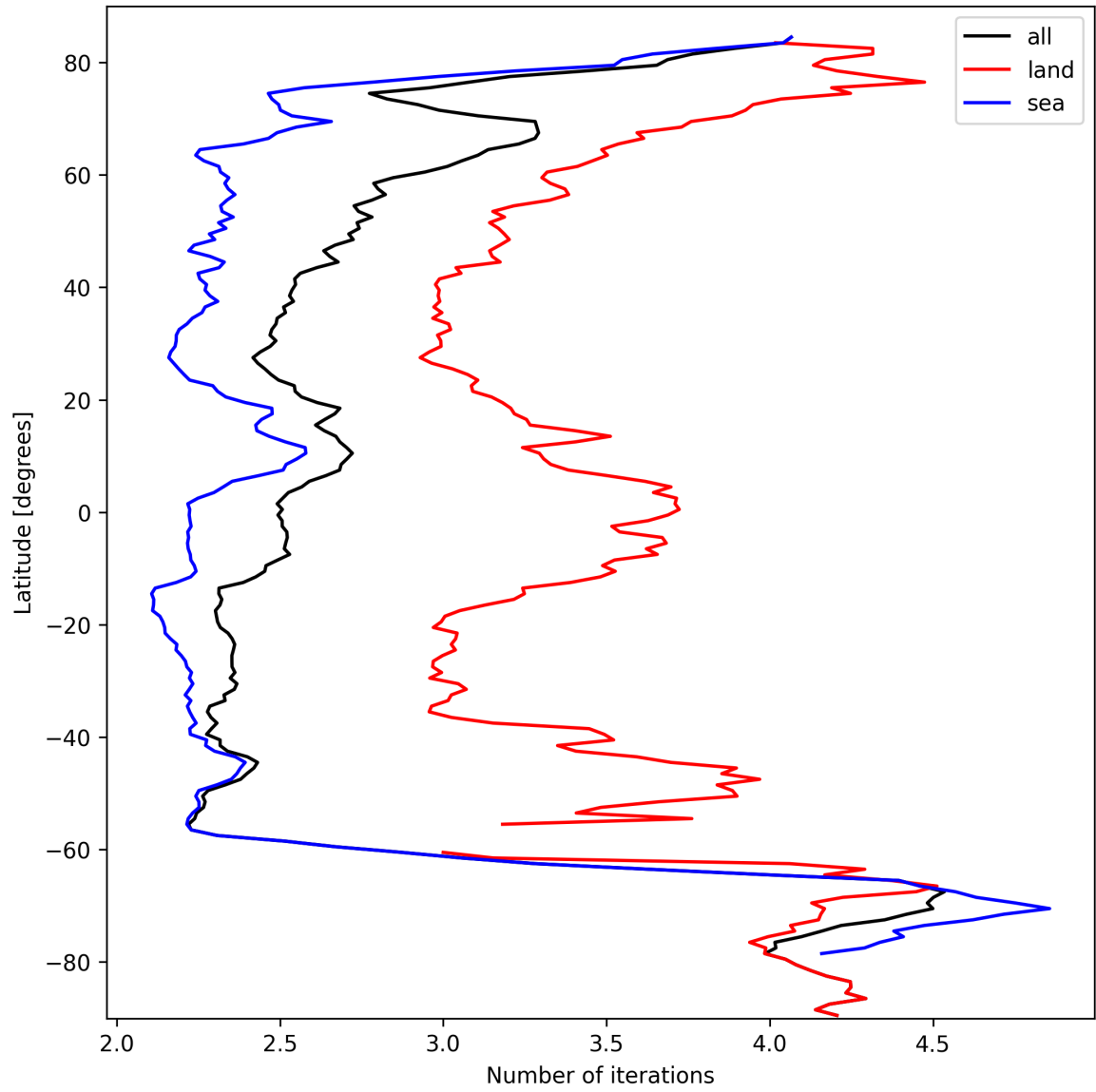
Figure 22: Zonal average of “Number of iterations” for 2024-10-01 to 2024-10-03.
