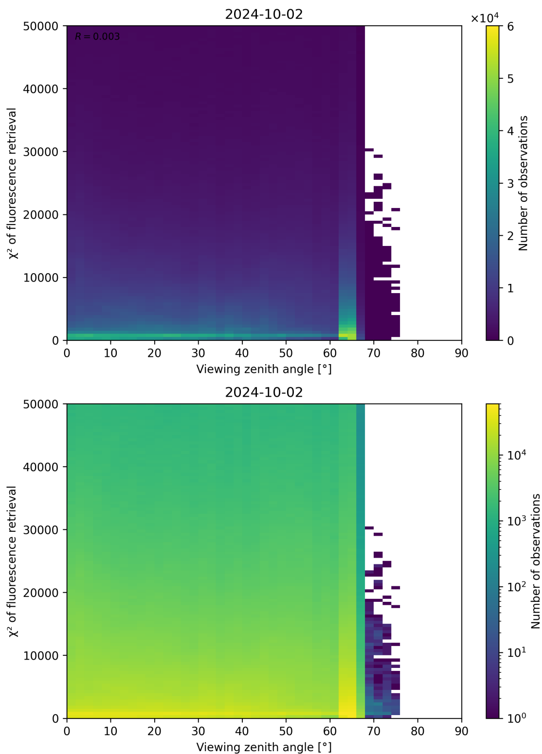
Figure 131: Scatter density plot of “Viewing zenith angle” against “ \chi^2 of fluorescence retrieval” for 2024-10-01 to 2024-10-03.
