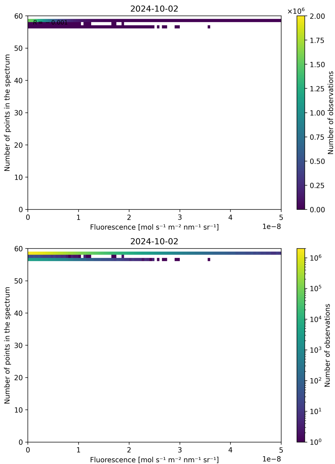
Figure 94: Scatter density plot of “Fluorescence” against “Number of points in the spectrum” for 2024-10-01 to 2024-10-03.
