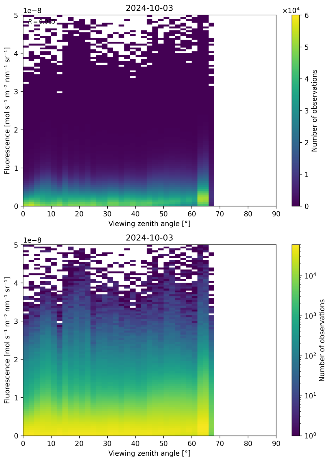
Figure 134: Scatter density plot of “Viewing zenith angle” against “Fluorescence” for 2024-10-03 to 2024-10-04.
