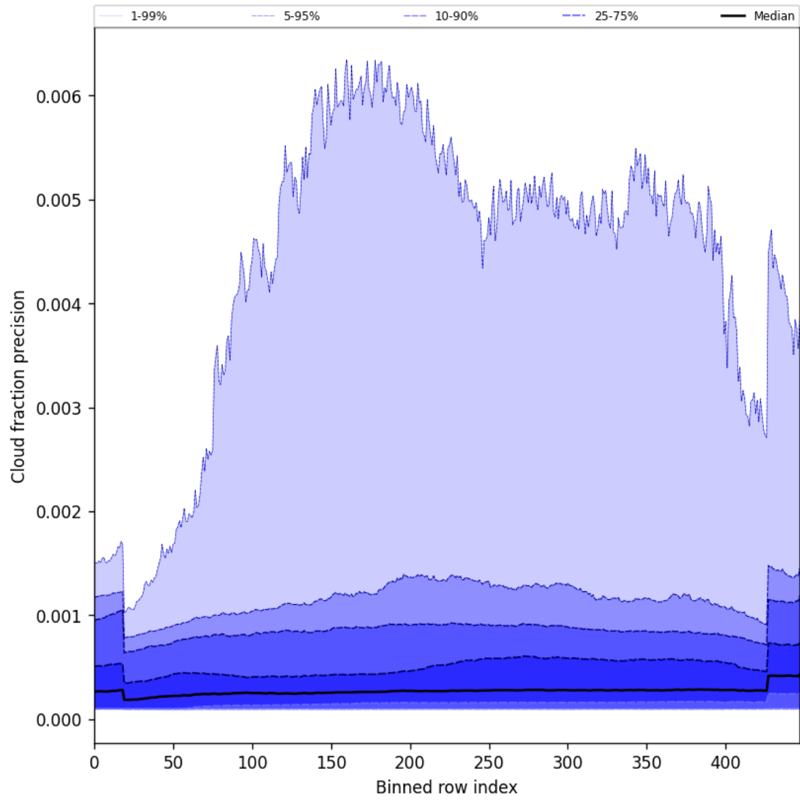
Figure 50: Along track statistics of “Cloud fraction precision” for 2024-10-03 to 2024-10-04
