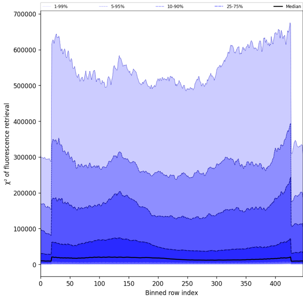
Figure 59: Along track statistics of “ \chi^2 of fluorescence retrieval” for 2024-10-03 to 2024-10-04
