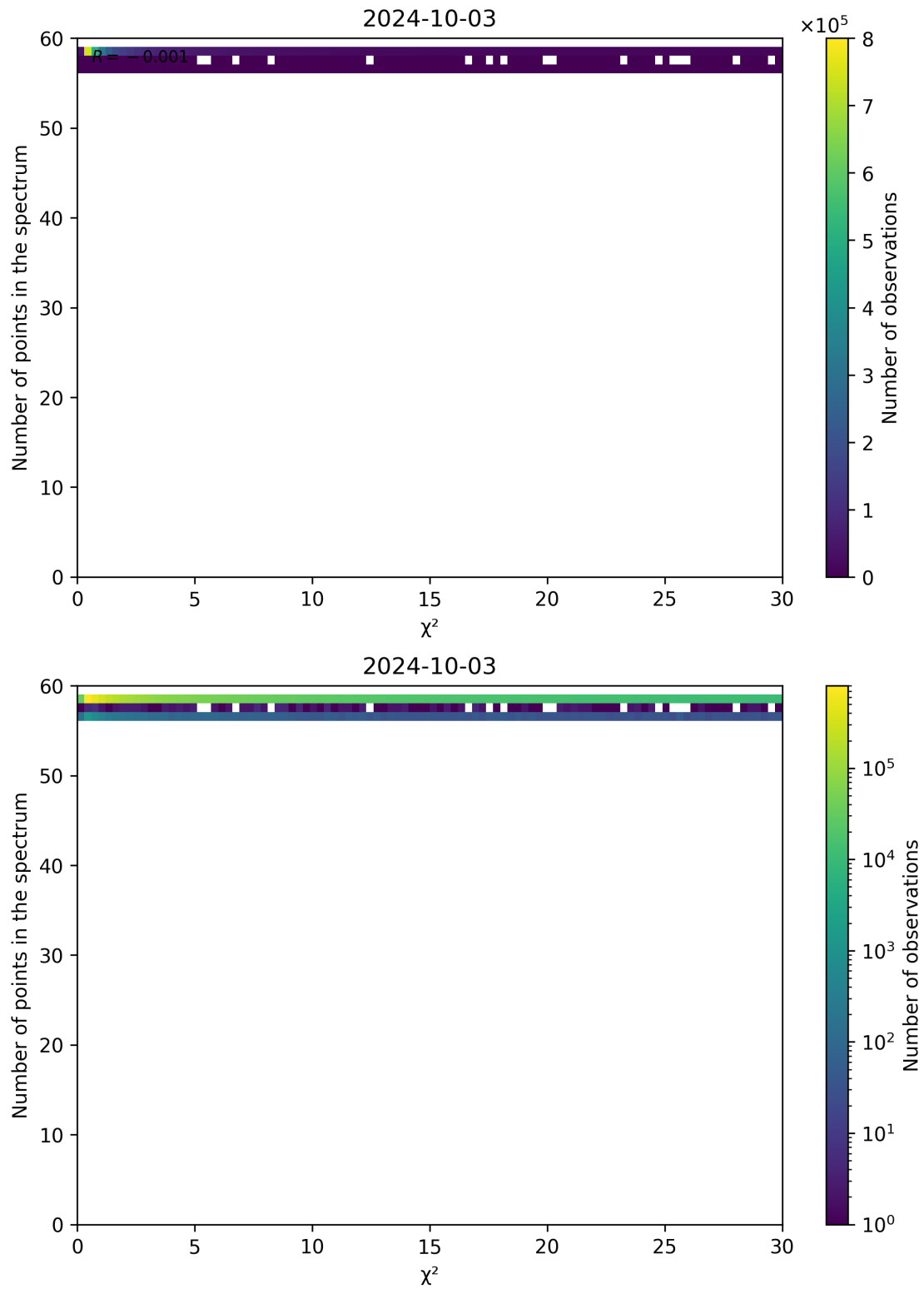
Figure 74: Scatter density plot of “ \chi^2 ” against “Number of points in the spectrum” for 2024-10-03 to 2024-10-04.
