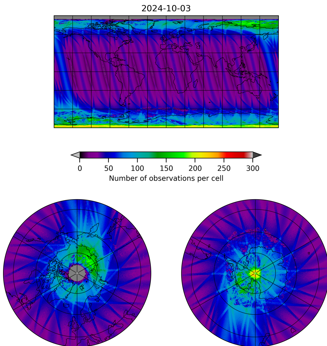
Figure 11: Map of the number of observations for 2024-10-03 to 2024-10-04
