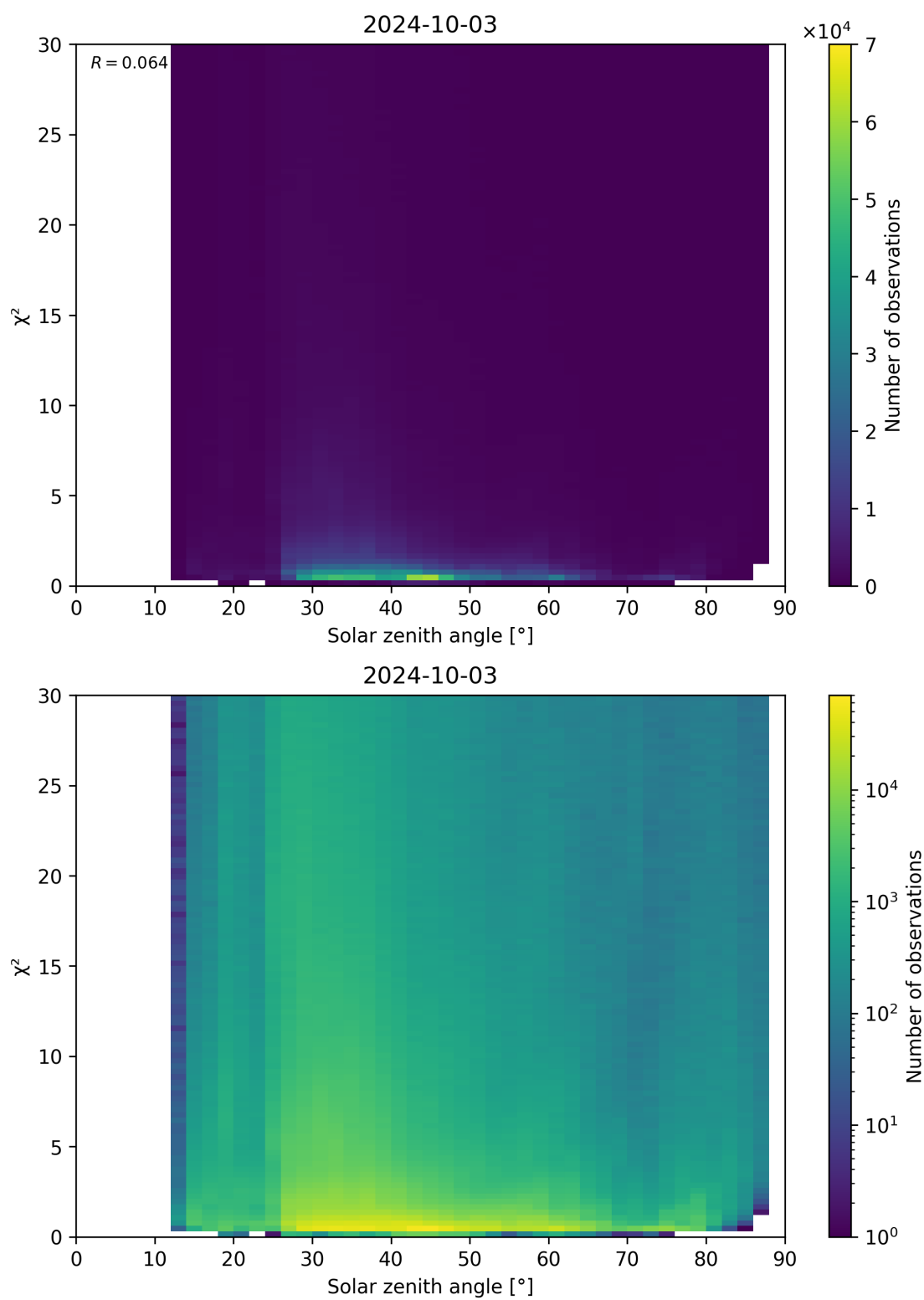
Figure 119: Scatter density plot of “Solar zenith angle” against “ \chi^2 ” for 2024-10-03 to 2024-10-04.
