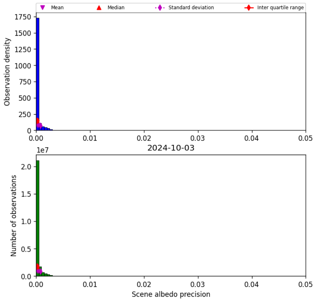
Figure 35: Histogram of “Scene albedo precision” for 2024-10-03 to 2024-10-04
