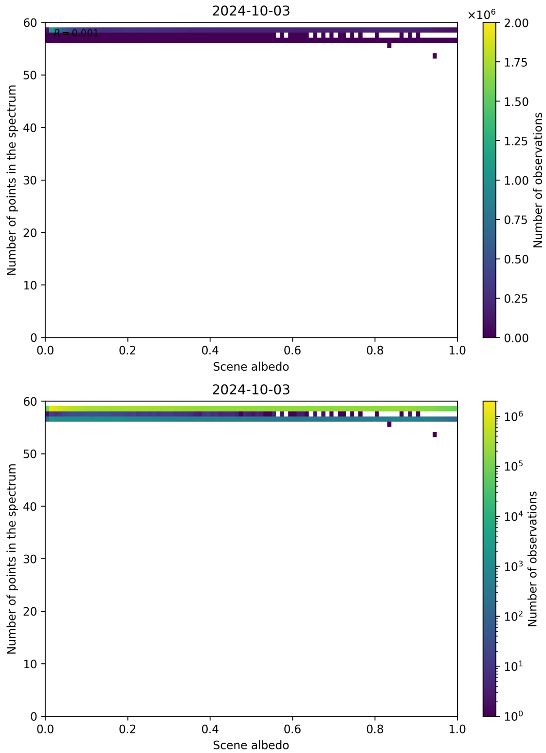
Figure 116: Scatter density plot of “Scene albedo” against “Number of points in the spectrum” for 2024-10-03 to 2024-10-04.
