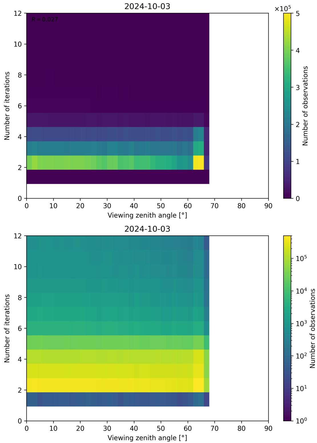
Figure 136: Scatter density plot of “Viewing zenith angle” against “Number of iterations” for 2024-10-03 to 2024-10-04.
