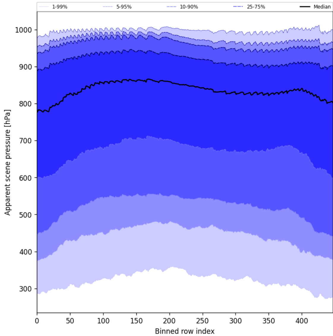
Figure 53: Along track statistics of “Apparent scene pressure” for 2024-10-03 to 2024-10-04
