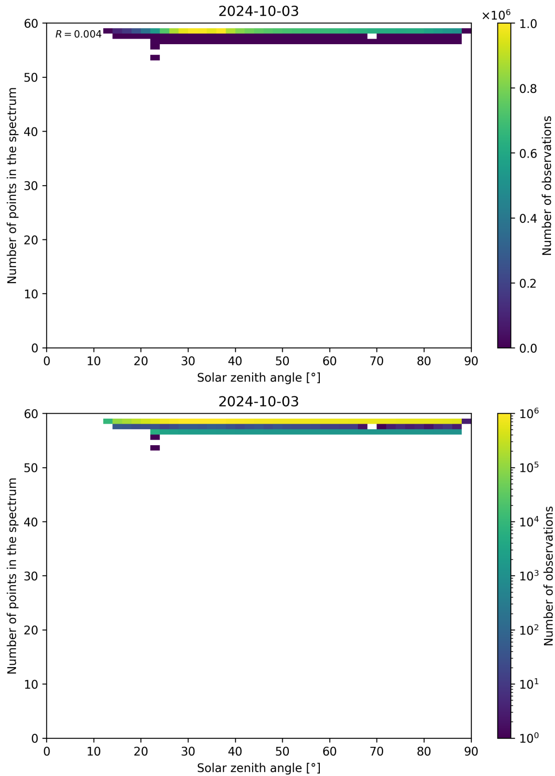
Figure 126: Scatter density plot of “Solar zenith angle” against “Number of points in the spectrum” for 2024-10-03 to 2024-10-04.
