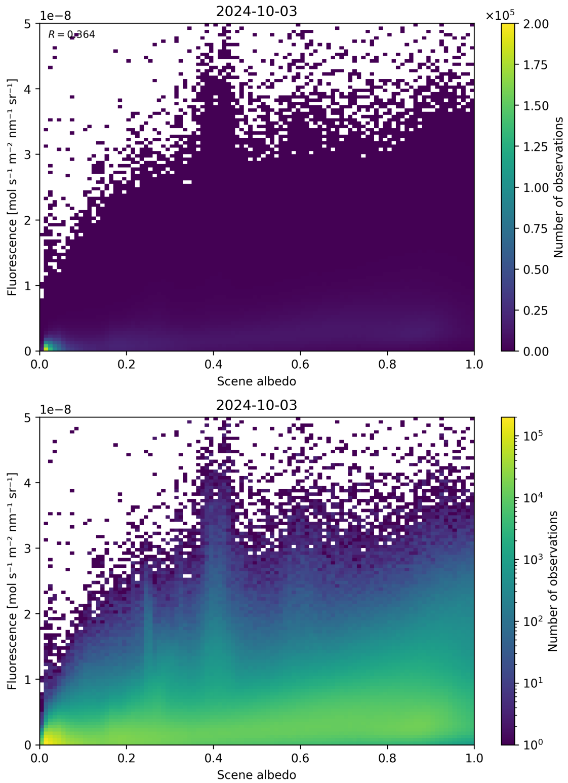
Figure 114: Scatter density plot of “Scene albedo” against “Fluorescence” for 2024-10-03 to 2024-10-04.
