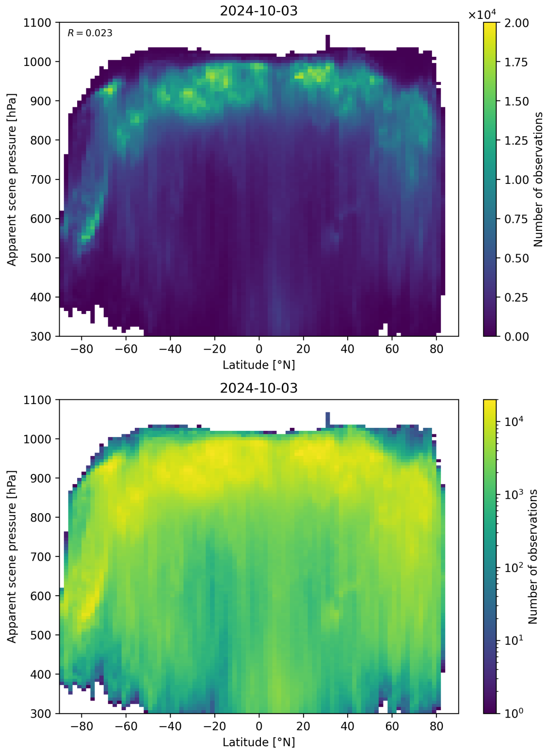
Figure 96: Scatter density plot of “Latitude” against “Apparent scene pressure” for 2024-10-03 to 2024-10-04.
