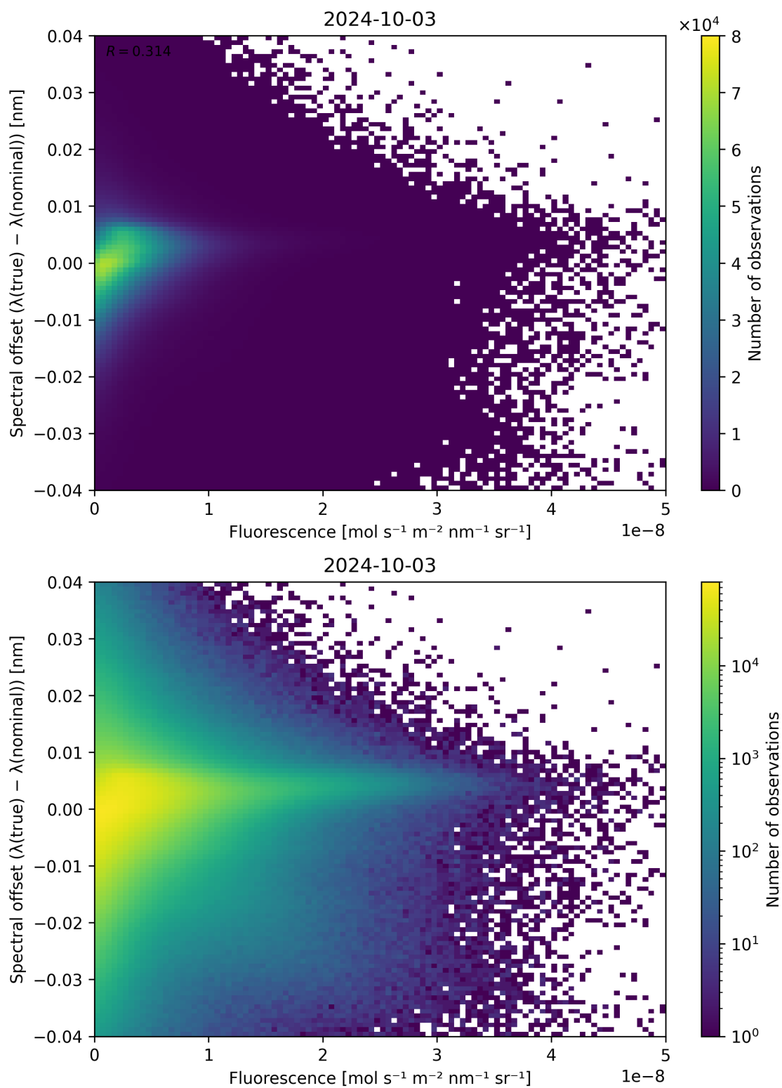
Figure 95: Scatter density plot of “Fluorescence” against “Spectral offset ( \lambda_{\text{true}} - \lambda_{\text{nominal}} )” for 2024-10-03 to 2024-10-04.
