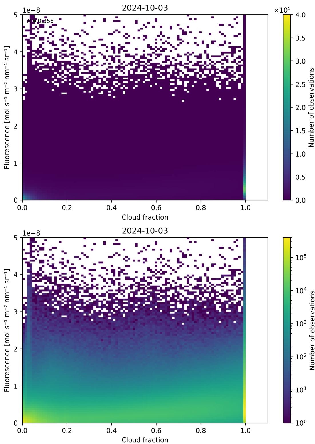
Figure 79: Scatter density plot of “Cloud fraction” against “Fluorescence” for 2024-10-03 to 2024-10-04.
