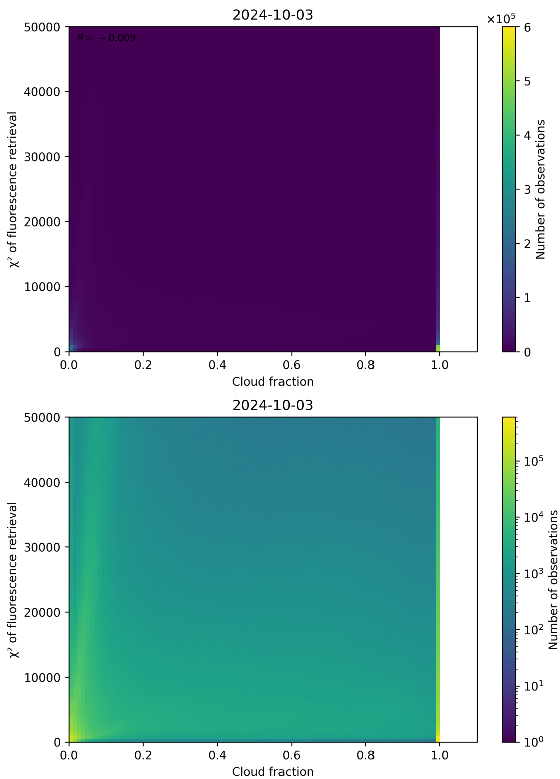
Figure 78: Scatter density plot of “Cloud fraction” against “ \chi^2 of fluorescence retrieval” for 2024-10-03 to 2024-10-04.
