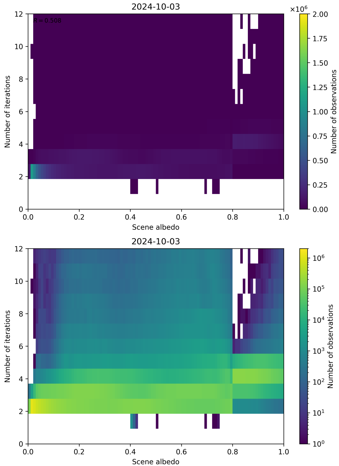
Figure 115: Scatter density plot of “Scene albedo” against “Number of iterations” for 2024-10-03 to 2024-10-04.
