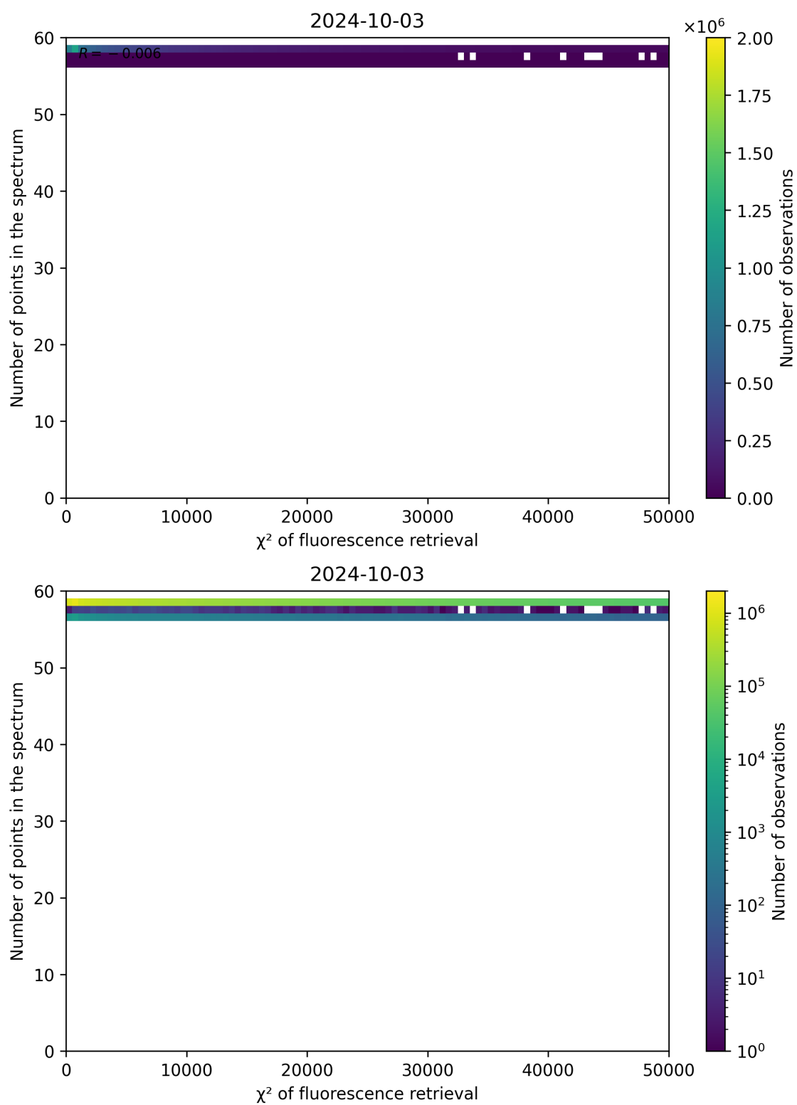
Figure 71: Scatter density plot of “ \chi^2 of fluorescence retrieval” against “Number of points in the spectrum” for 2024-10-03 to 2024-10-04.
