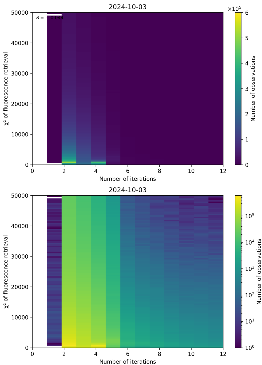
Figure 106: Scatter density plot of “Number of iterations” against “ \chi^2 of fluorescence retrieval” for 2024-10-03 to 2024-10-04.
