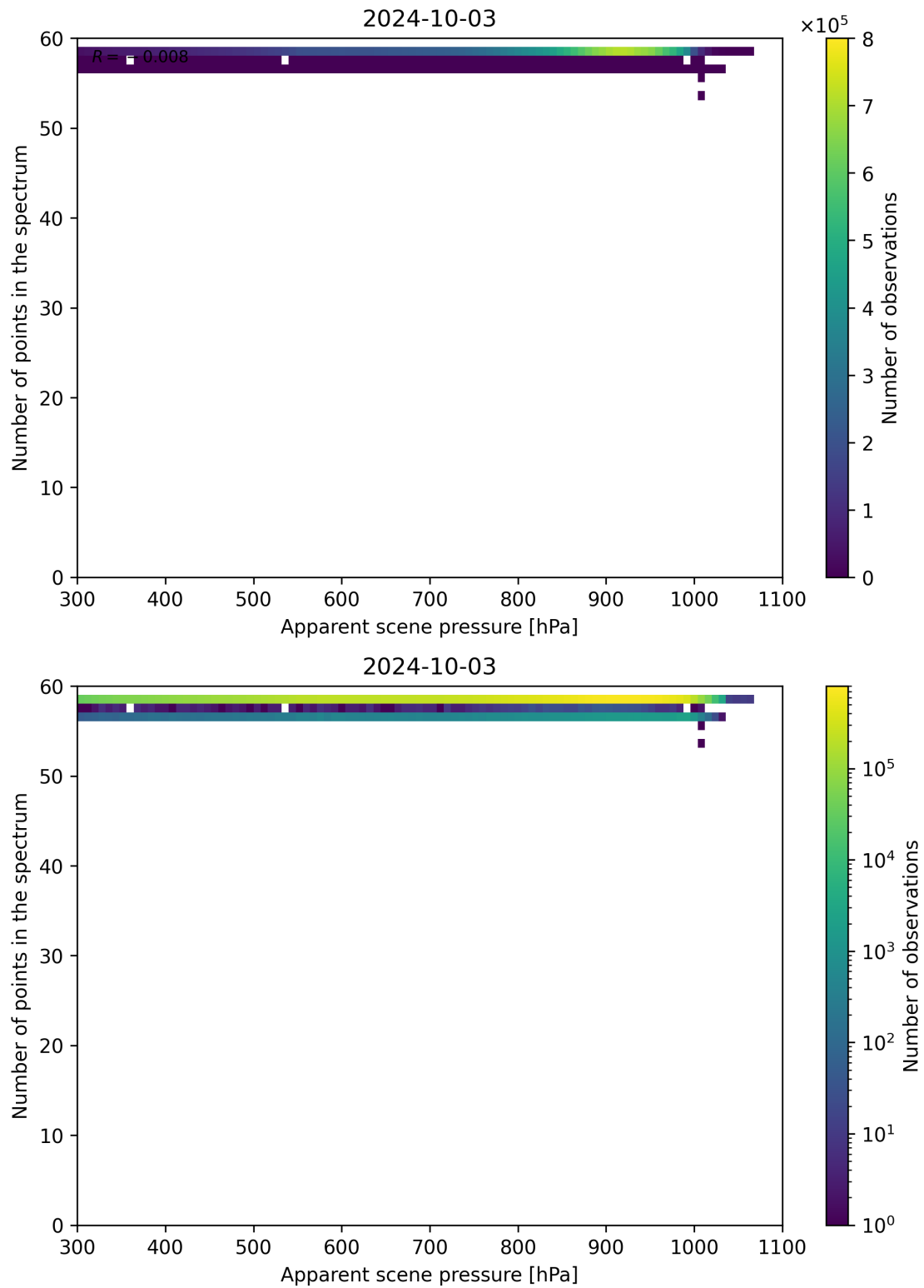
Figure 67: Scatter density plot of “Apparent scene pressure” against “Number of points in the spectrum” for 2024-10-03 to 2024-10-04.
