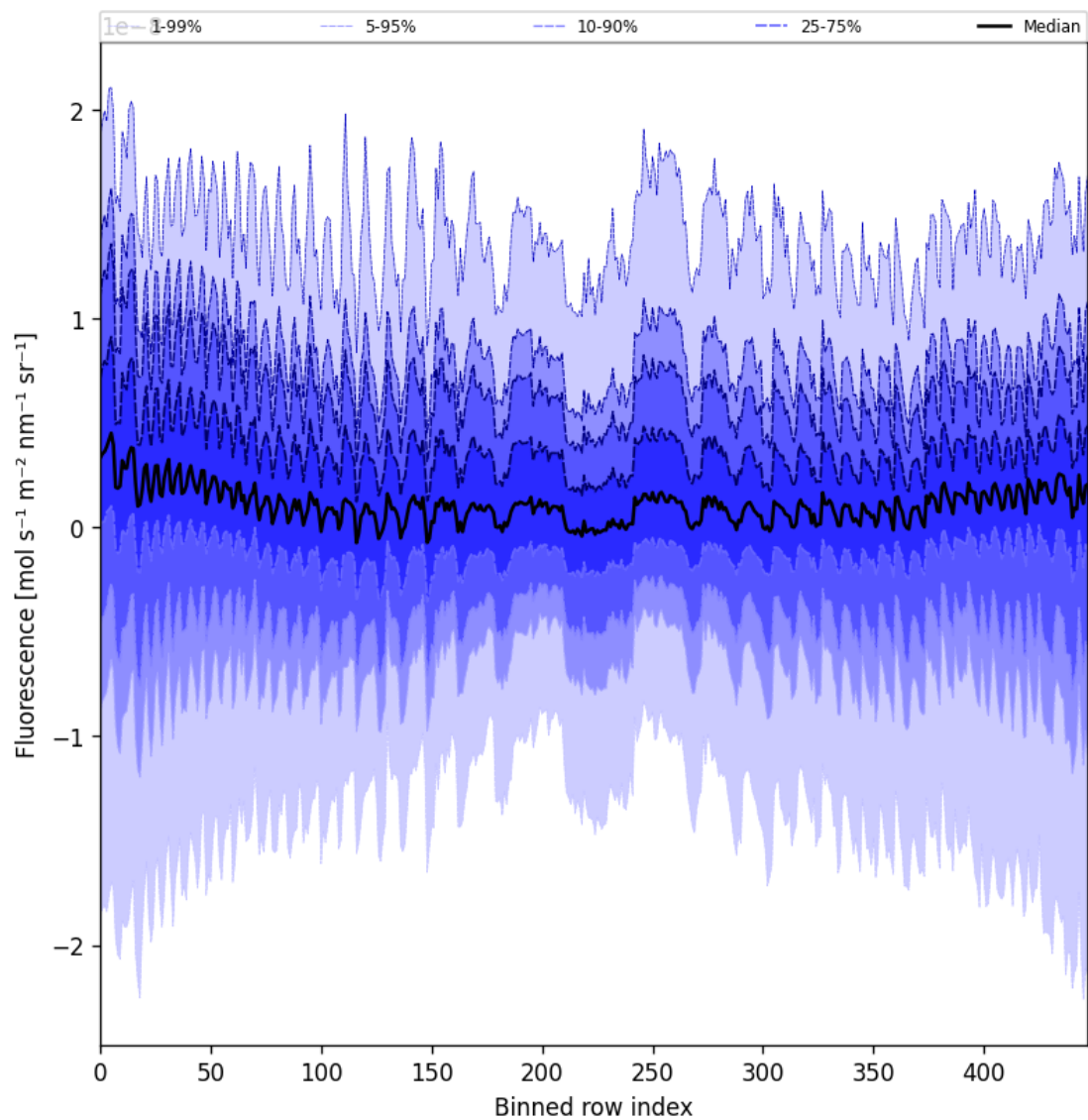
Figure 57: Along track statistics of “Fluorescence” for 2024-10-03 to 2024-10-04
