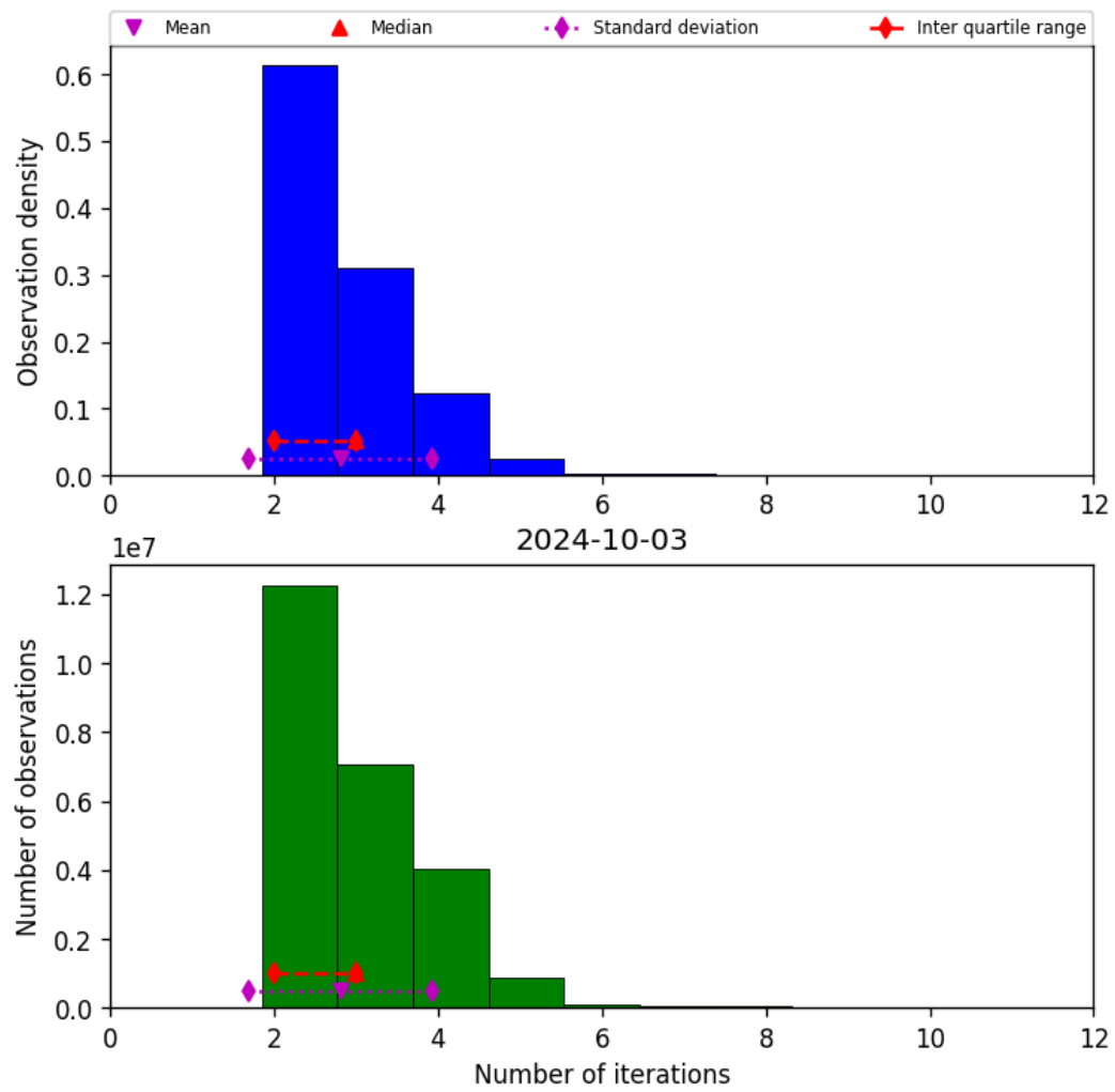
Figure 39: Histogram of “Number of iterations” for 2024-10-03 to 2024-10-04
