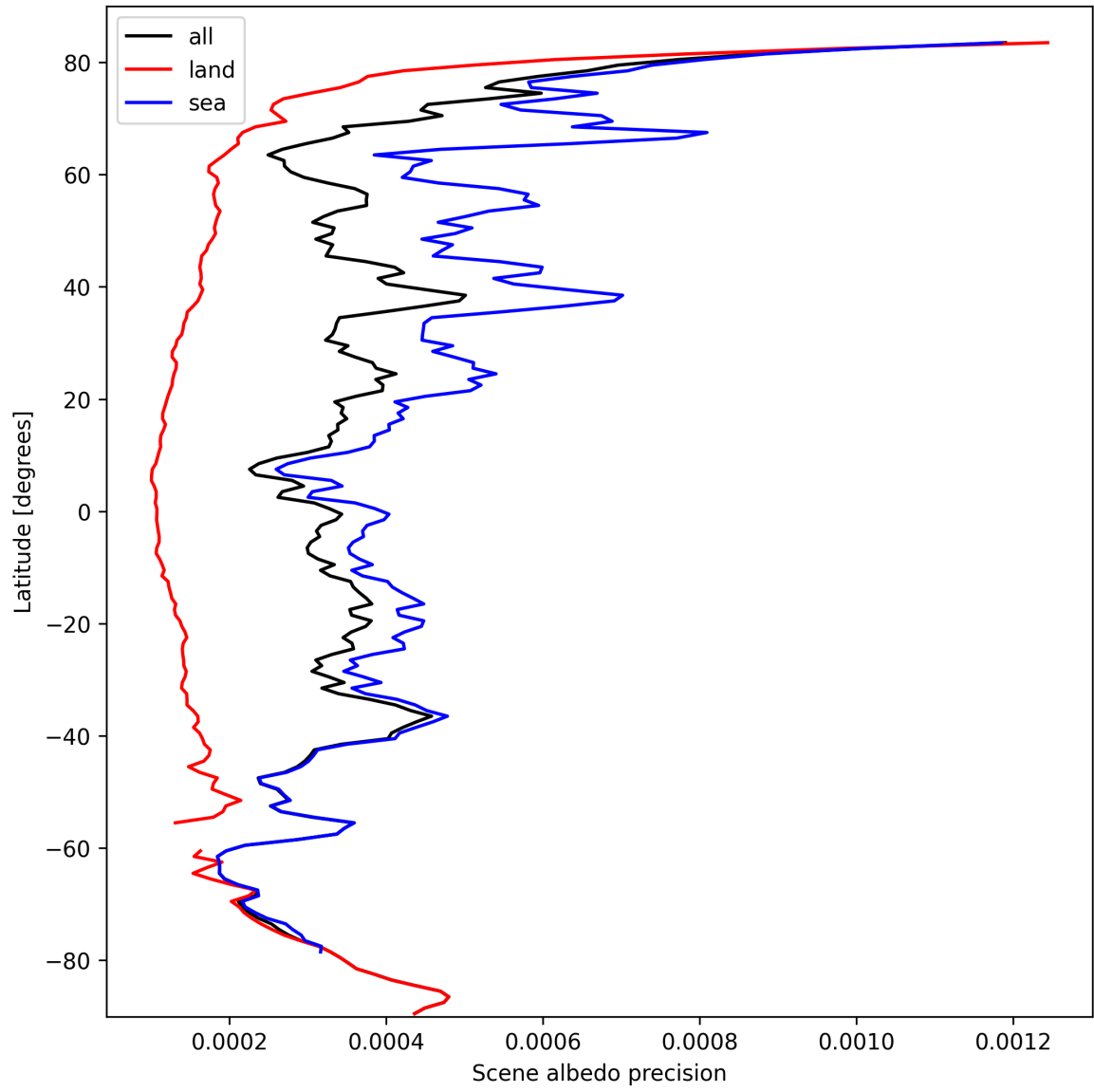
Figure 18: Zonal average of “Scene albedo precision” for 2024-10-03 to 2024-10-04.
