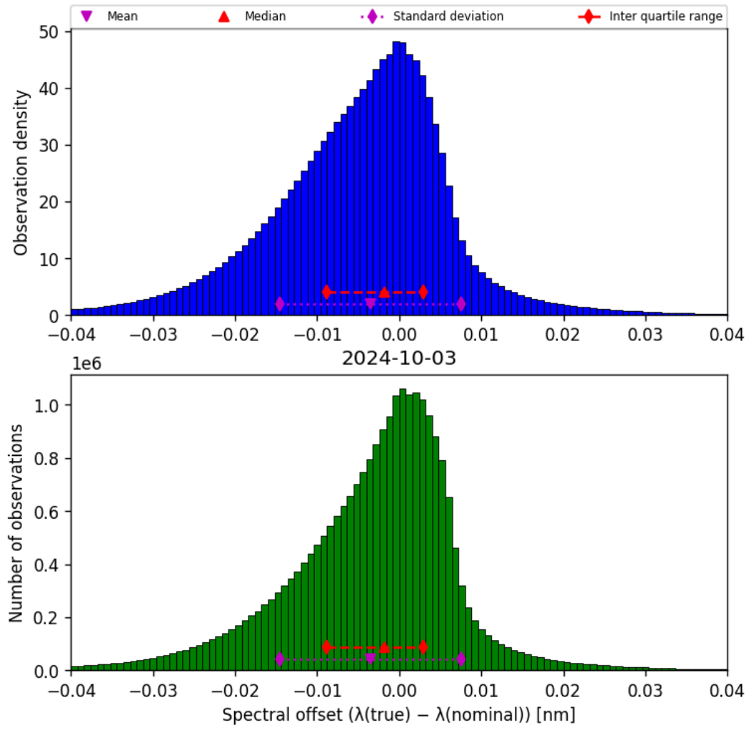
Figure 45: Histogram of “Spectral offset ( \lambda_{\text{true}} - \lambda_{\text{nominal}} )” for 2024-10-03 to 2024-10-04
