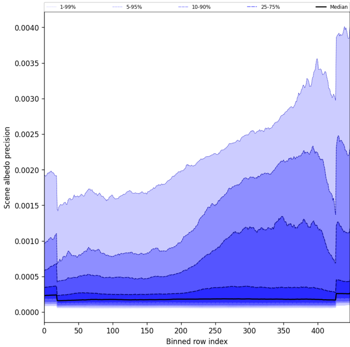
Figure 52: Along track statistics of “Scene albedo precision” for 2024-10-03 to 2024-10-04
