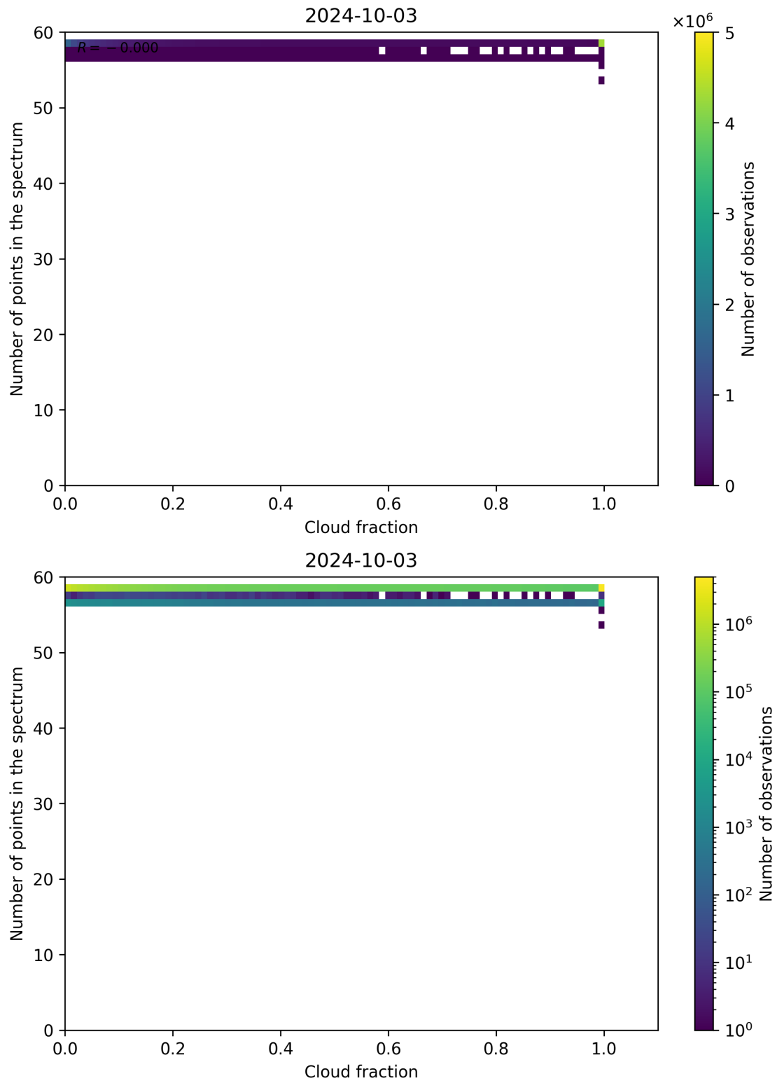
Figure 81: Scatter density plot of “Cloud fraction” against “Number of points in the spectrum” for 2024-10-03 to 2024-10-04.
