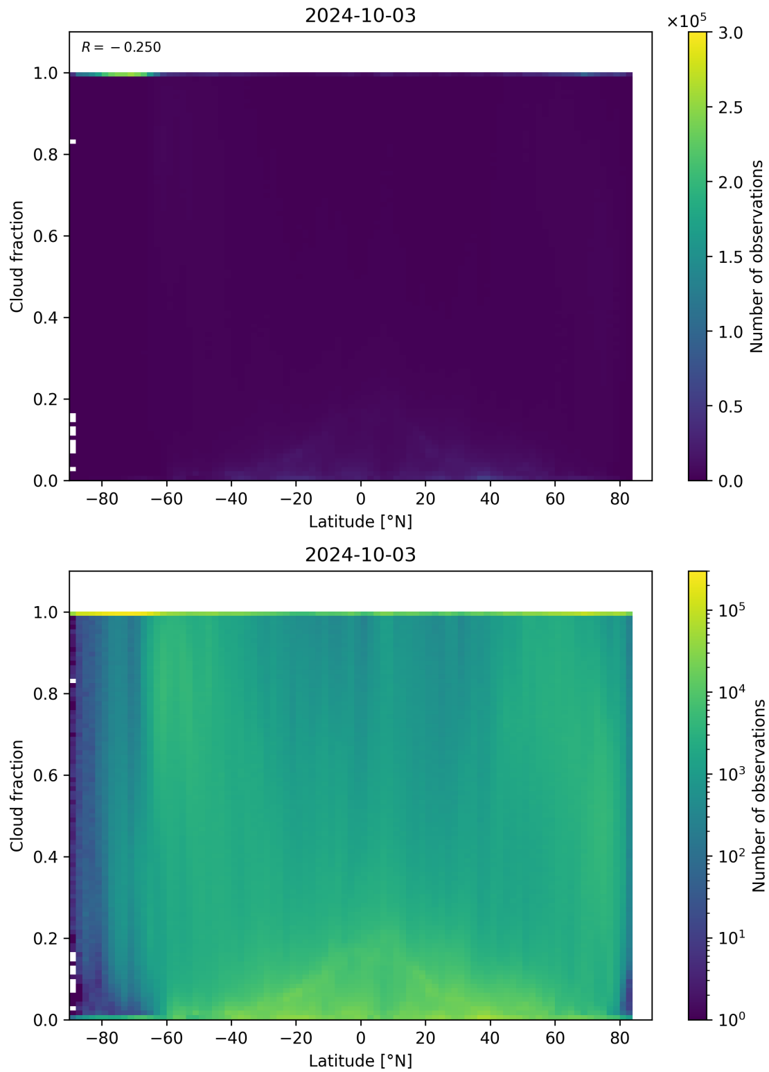
Figure 99: Scatter density plot of “Latitude” against “Cloud fraction” for 2024-10-03 to 2024-10-04.
