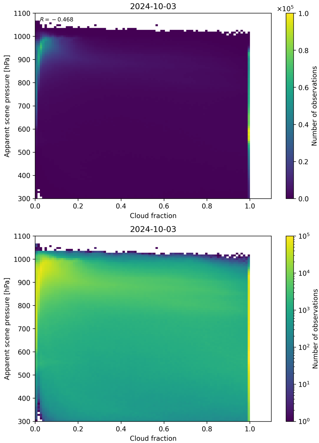
Figure 76: Scatter density plot of “Cloud fraction” against “Apparent scene pressure” for 2024-10-03 to 2024-10-04.
