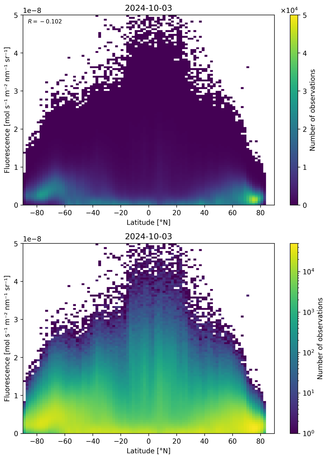
Figure 101: Scatter density plot of “Latitude” against “Fluorescence” for 2024-10-03 to 2024-10-04.
