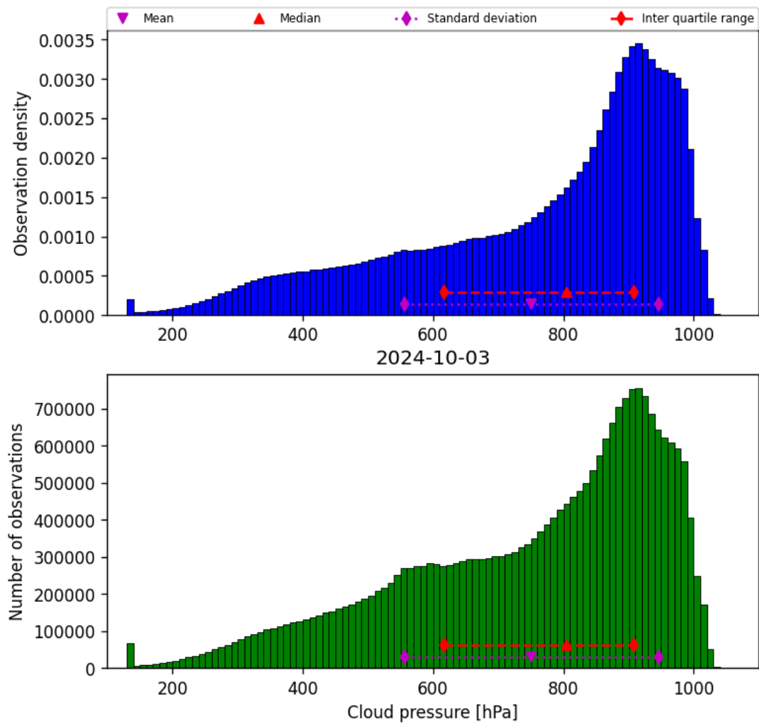
Figure 30: Histogram of “Cloud pressure” for 2024-10-03 to 2024-10-04
