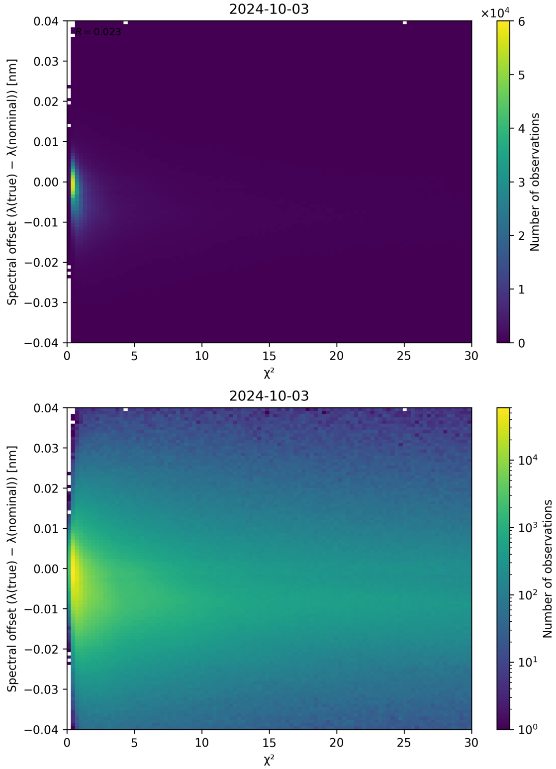
Figure 75: Scatter density plot of “ \chi^2 ” against “Spectral offset ( \lambda_{\text{true}} - \lambda_{\text{nominal}} )” for 2024-10-03 to 2024-10-04.
