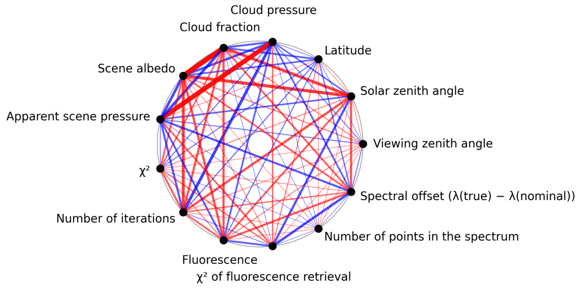
Figure 1: Map of correlation graph for 2024-10-03 to 2024-10-04.
