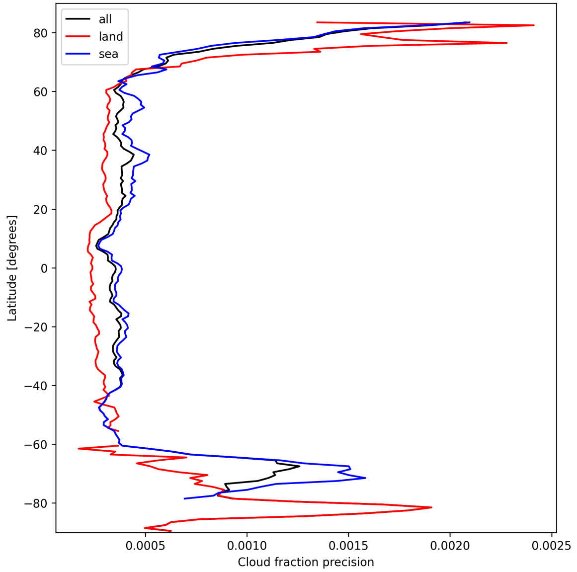
Figure 16: Zonal average of “Cloud fraction precision” for 2024-10-03 to 2024-10-04.
