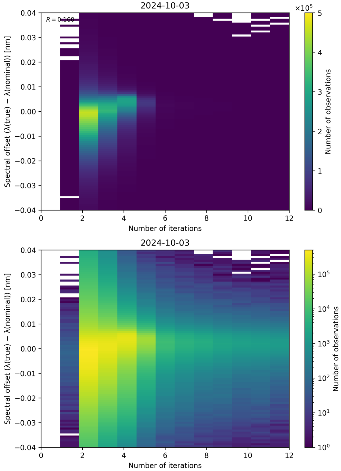
Figure 109: Scatter density plot of “Number of iterations” against “Spectral offset ( \lambda_{\text{true}} - \lambda_{\text{nominal}} )” for 2024-10-03 to 2024-10-04.
