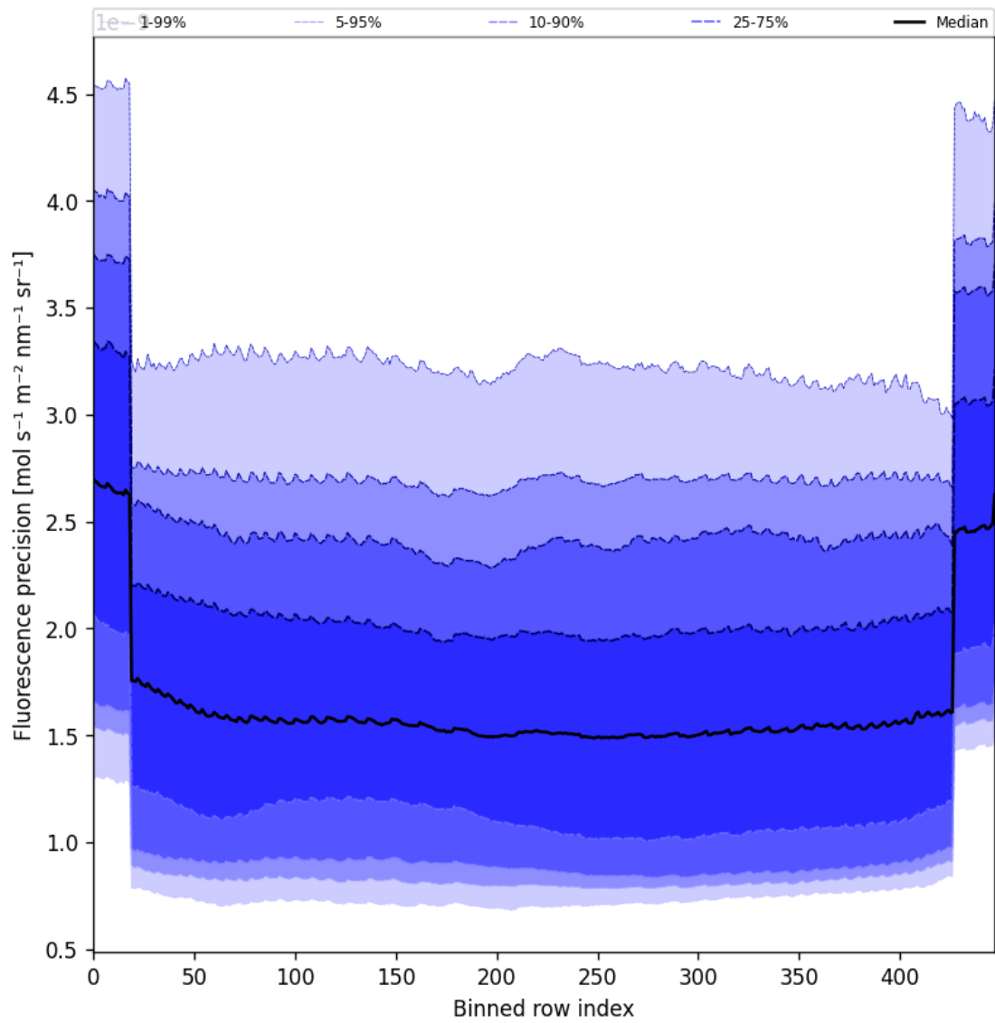
Figure 58: Along track statistics of “Fluorescence precision” for 2024-10-03 to 2024-10-04
