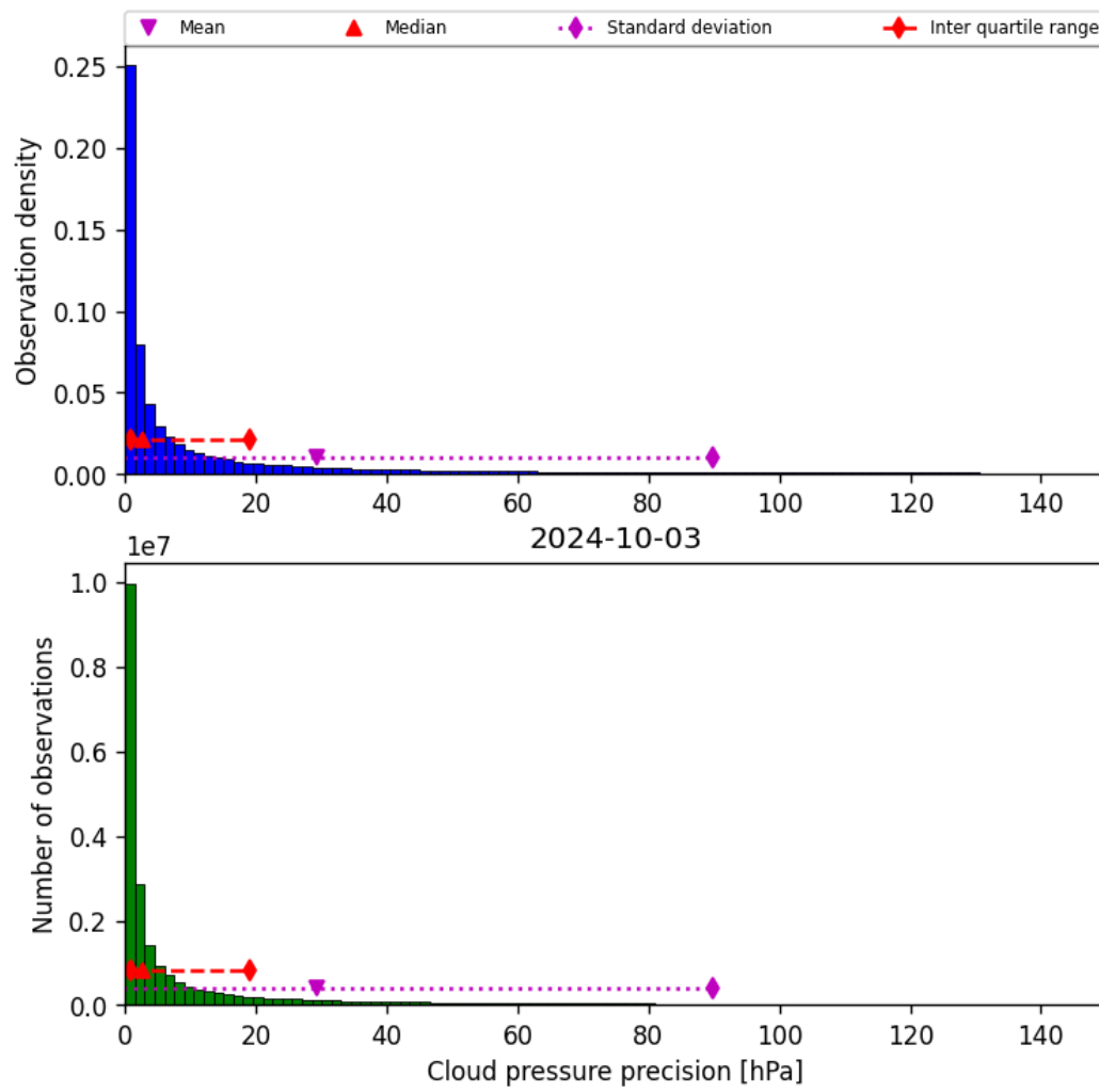
Figure 31: Histogram of “Cloud pressure precision” for 2024-10-03 to 2024-10-04
