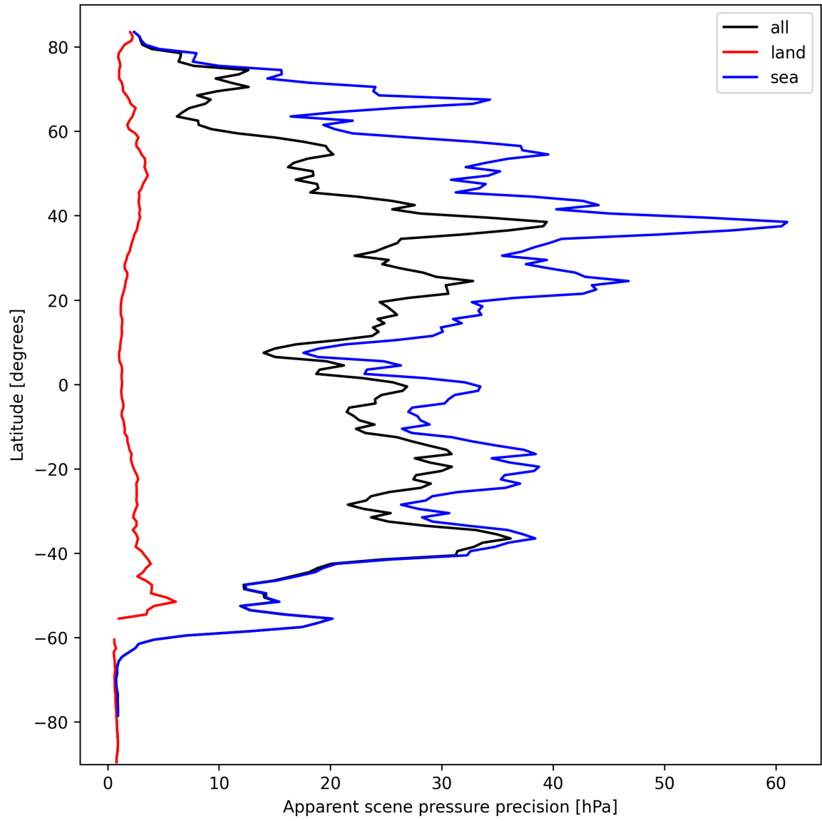
Figure 20: Zonal average of “Apparent scene pressure precision” for 2024-10-03 to 2024-10-04.
