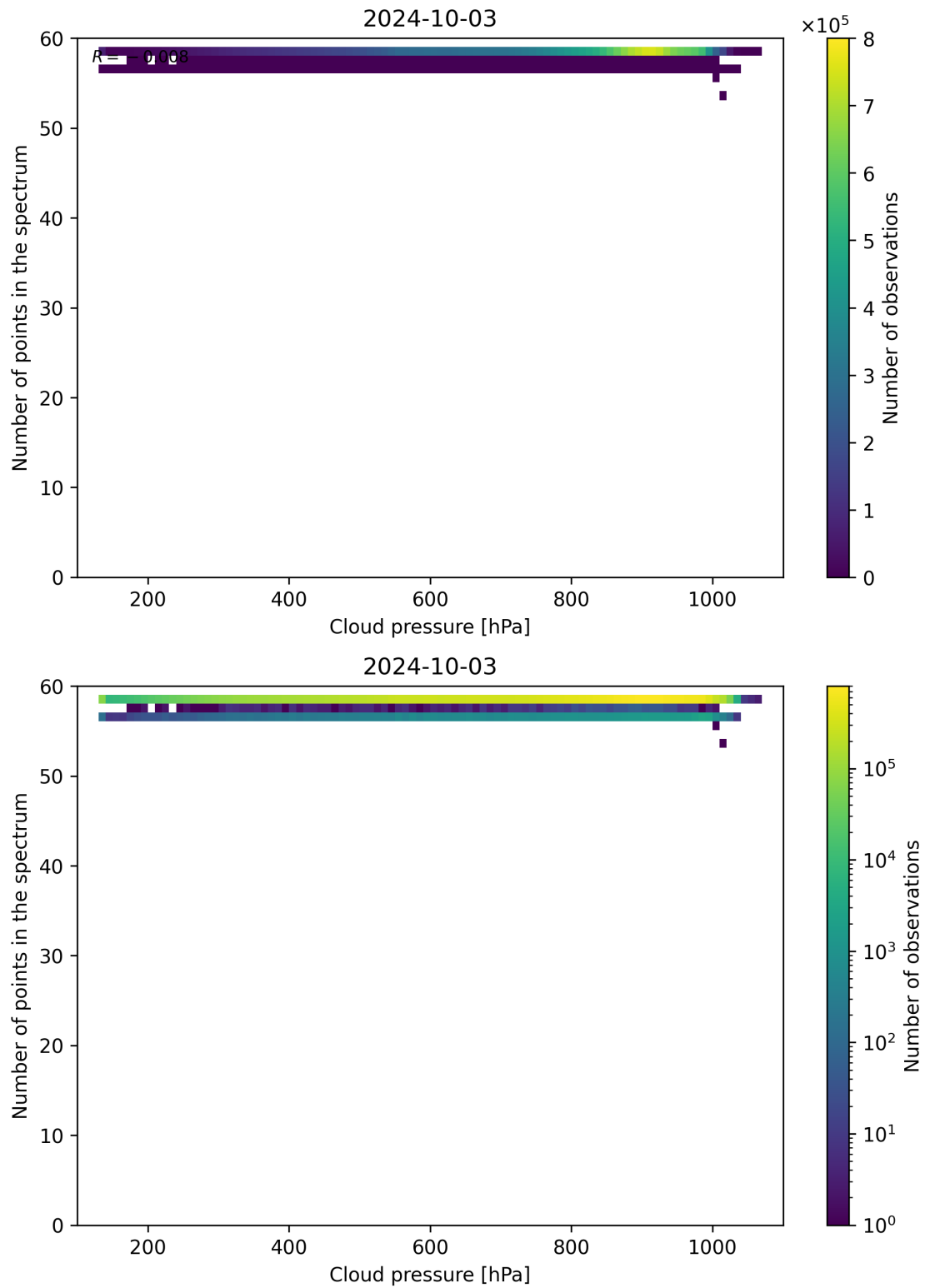
Figure 90: Scatter density plot of “Cloud pressure” against “Number of points in the spectrum” for 2024-10-03 to 2024-10-04.
