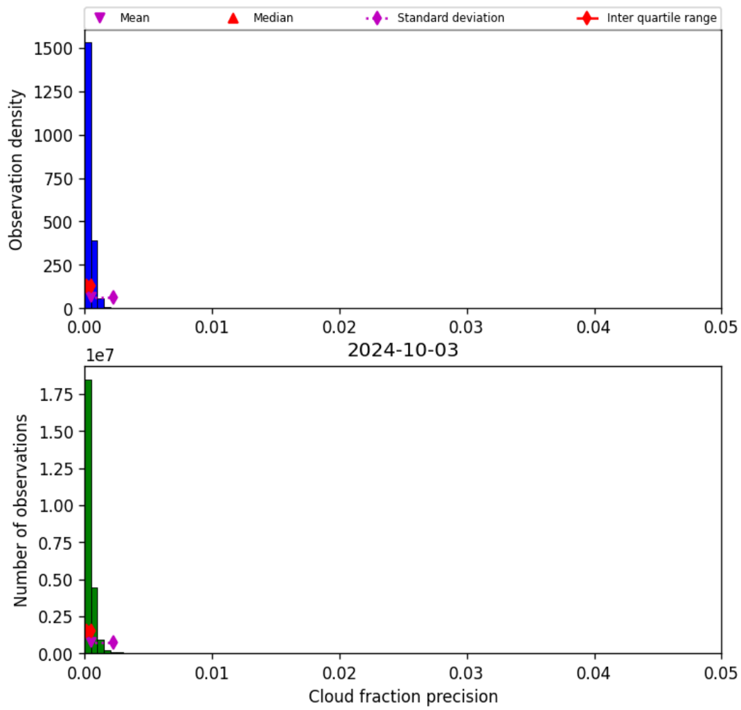
Figure 33: Histogram of “Cloud fraction precision” for 2024-10-03 to 2024-10-04
