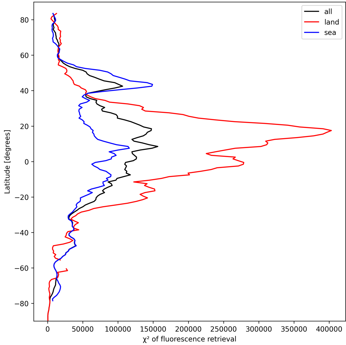
Figure 25: Zonal average of “ \chi^2 of fluorescence retrieval” for 2024-10-03 to 2024-10-04.
