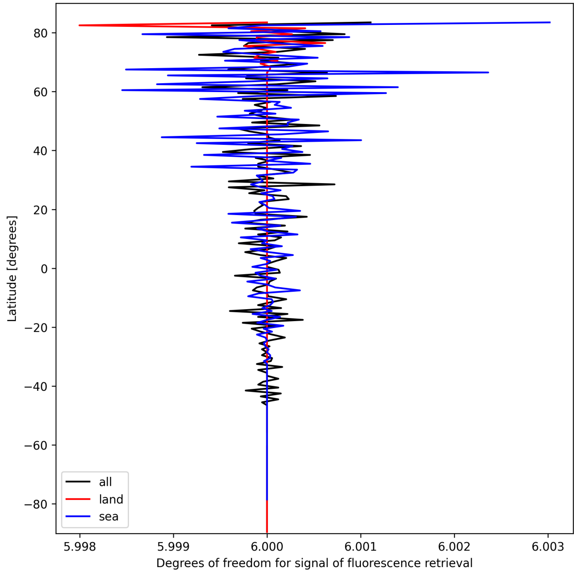
Figure 26: Zonal average of “Degrees of freedom for signal of fluorescence retrieval” for 2024-10-03 to 2024-10-04.
