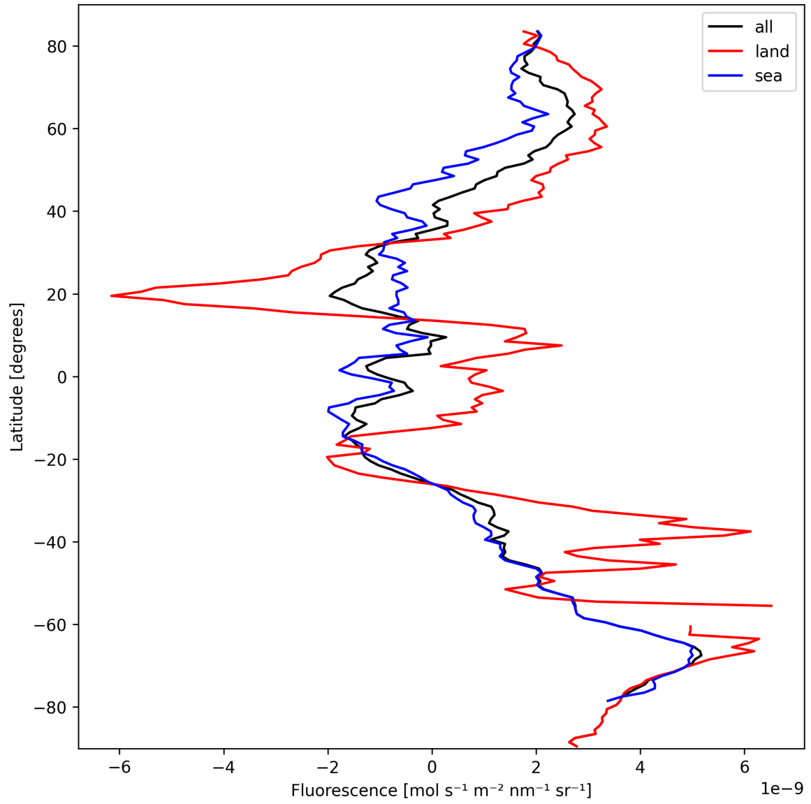
Figure 23: Zonal average of “Fluorescence” for 2024-10-03 to 2024-10-04.
