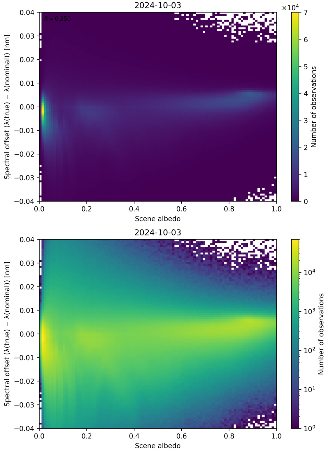
Figure 117: Scatter density plot of “Scene albedo” against “Spectral offset ( \lambda_{\text{true}} - \lambda_{\text{nominal}} )” for 2024-10-03 to 2024-10-04.
