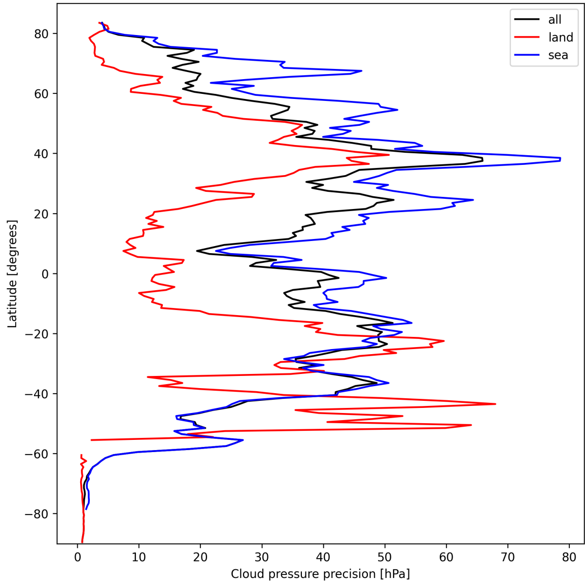
Figure 14: Zonal average of “Cloud pressure precision” for 2024-10-03 to 2024-10-04.
