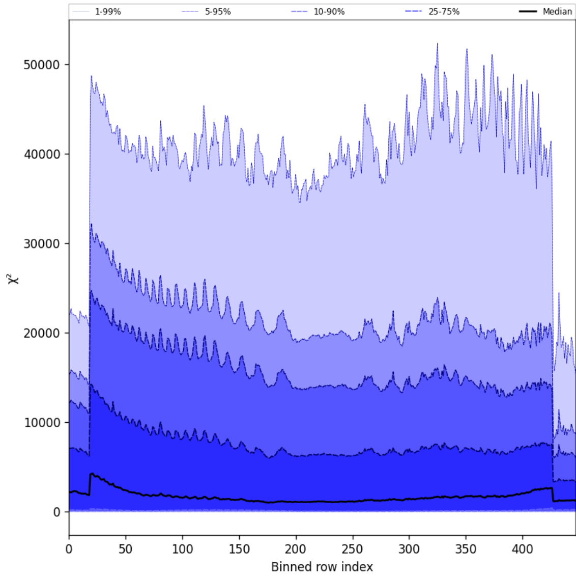
Figure 55: Along track statistics of “ \chi^2 ” for 2024-10-03 to 2024-10-04
