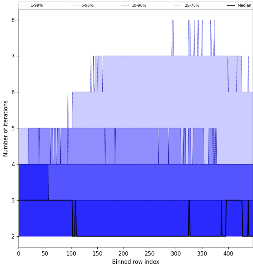
Figure 56: Along track statistics of “Number of iterations” for 2024-10-03 to 2024-10-04
