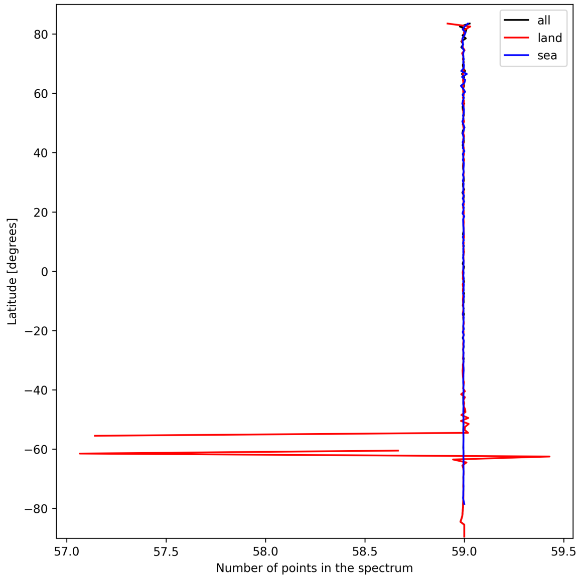
Figure 27: Zonal average of “Number of points in the spectrum” for 2024-10-03 to 2024-10-04.
