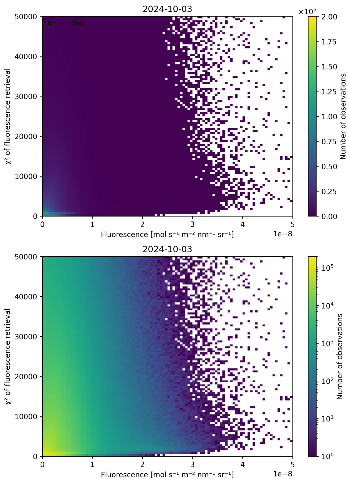
Figure 93: Scatter density plot of “Fluorescence” against “ \chi^2 of fluorescence retrieval” for 2024-10-03 to 2024-10-04.
