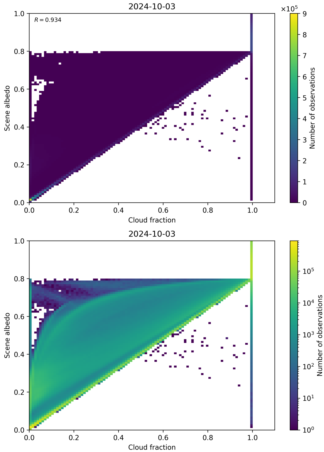
Figure 82: Scatter density plot of “Cloud fraction” against “Scene albedo” for 2024-10-03 to 2024-10-04.
