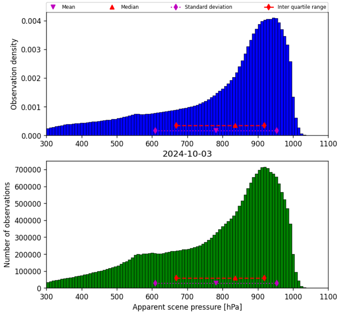
Figure 36: Histogram of “Apparent scene pressure” for 2024-10-03 to 2024-10-04
