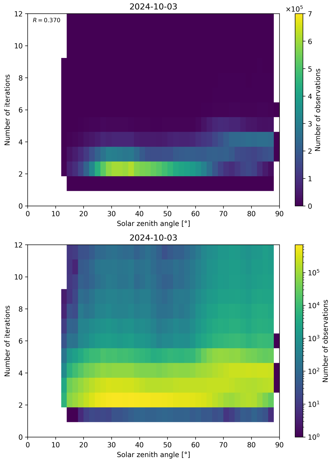
Figure 125: Scatter density plot of “Solar zenith angle” against “Number of iterations” for 2024-10-03 to 2024-10-04.
