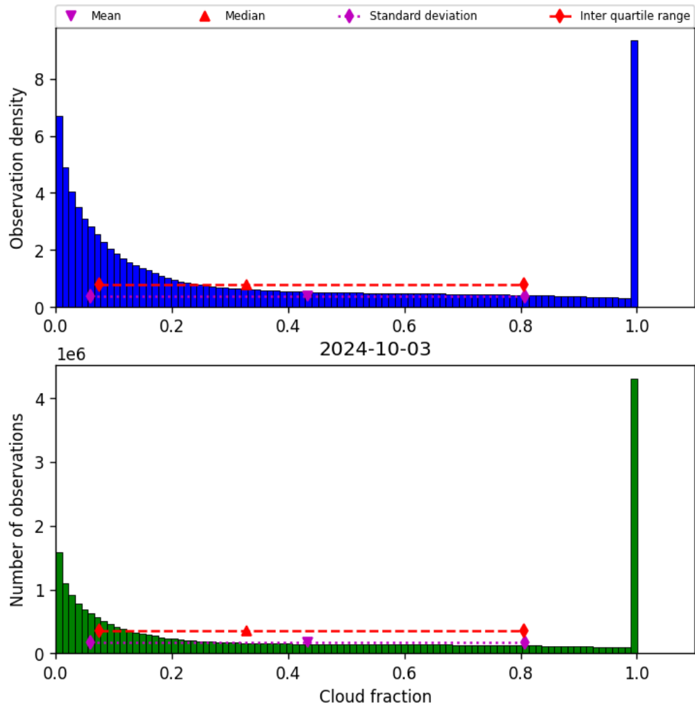
Figure 32: Histogram of “Cloud fraction” for 2024-10-03 to 2024-10-04
