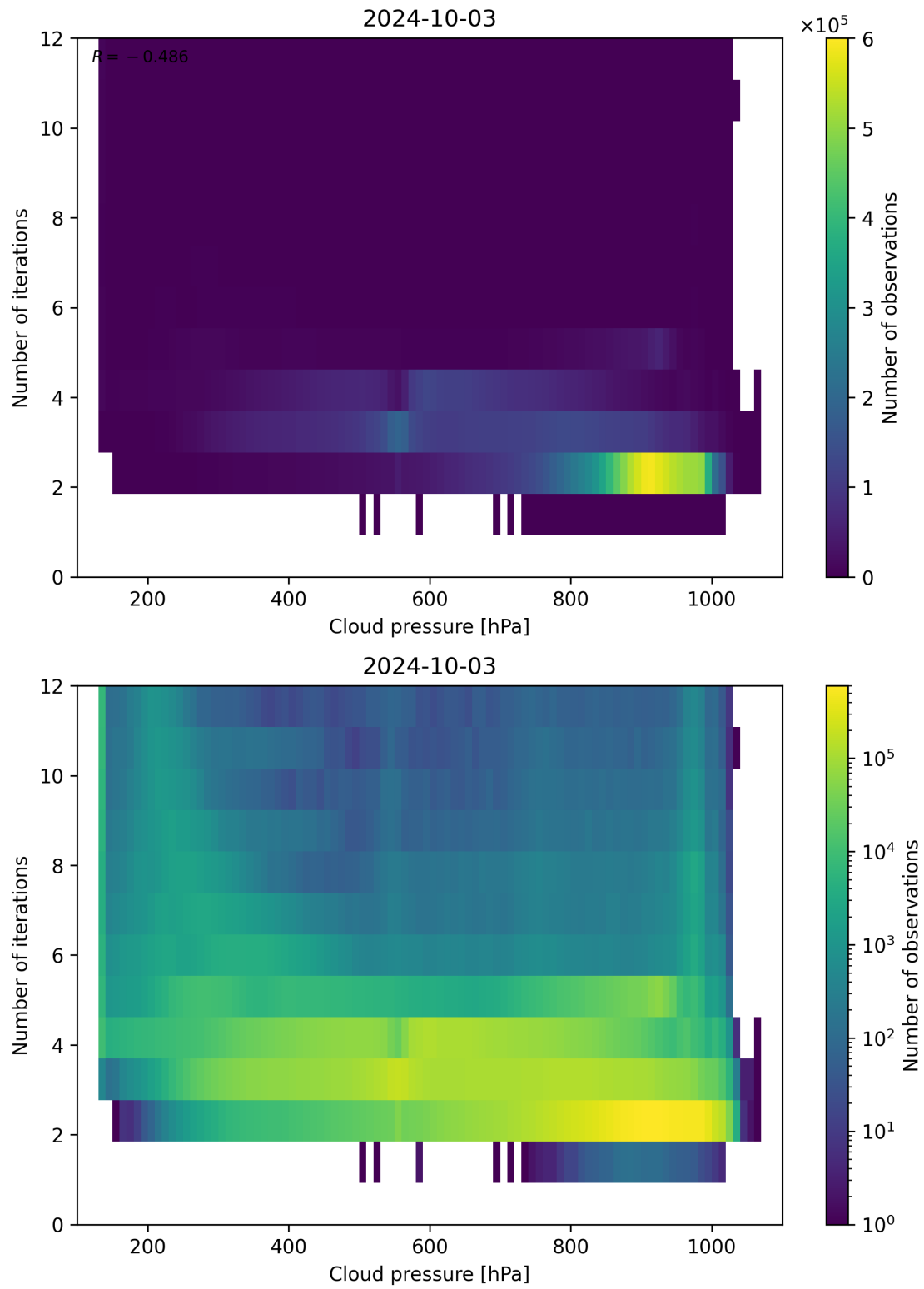
Figure 89: Scatter density plot of “Cloud pressure” against “Number of iterations” for 2024-10-03 to 2024-10-04.
