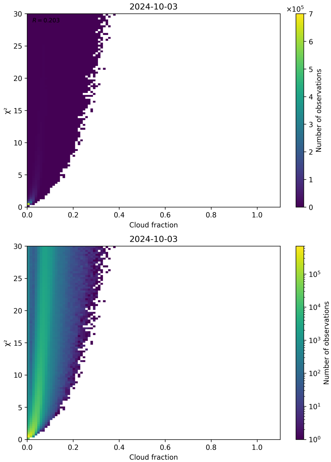
Figure 77: Scatter density plot of “Cloud fraction” against “ \chi^2 ” for 2024-10-03 to 2024-10-04.
