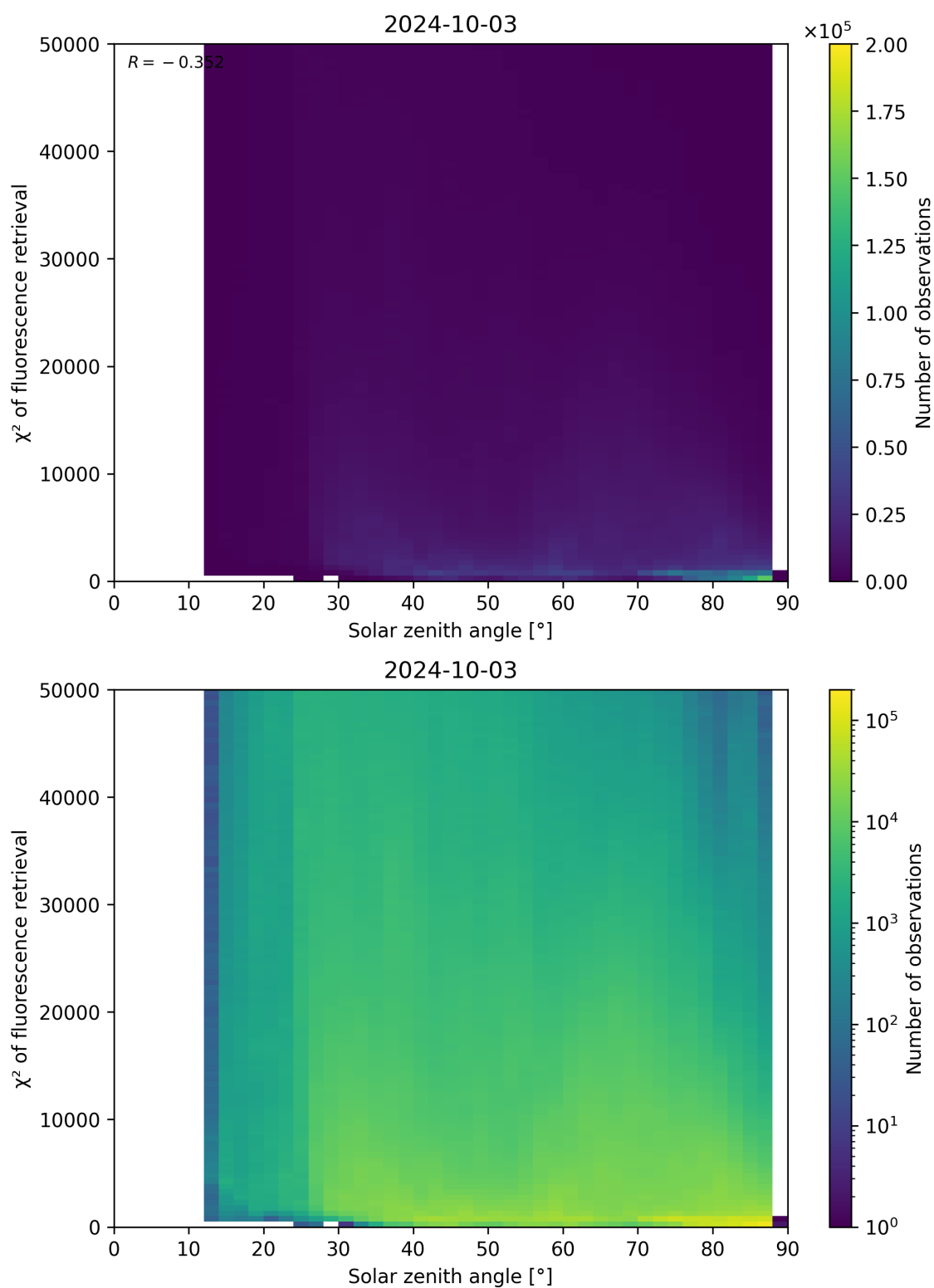
Figure 120: Scatter density plot of “Solar zenith angle” against “ \chi^2 of fluorescence retrieval” for 2024-10-03 to 2024-10-04.
