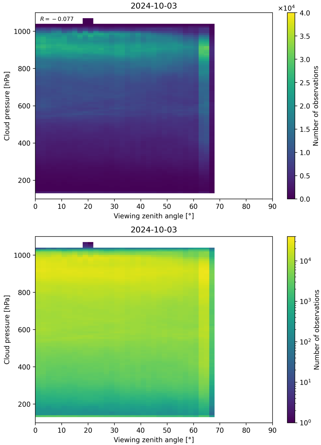
Figure 133: Scatter density plot of “Viewing zenith angle” against “Cloud pressure” for 2024-10-03 to 2024-10-04.
