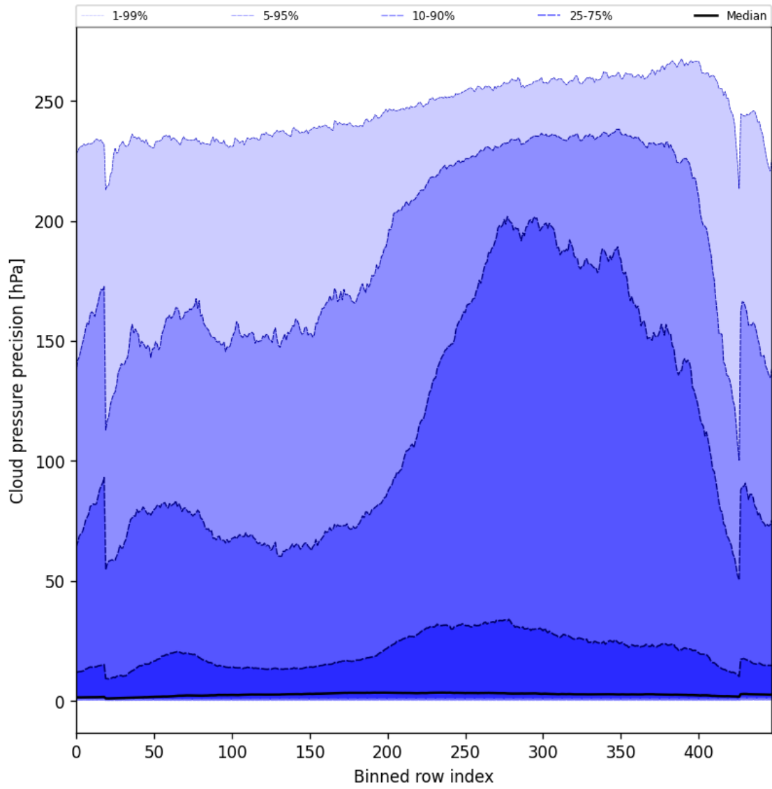
Figure 48: Along track statistics of “Cloud pressure precision” for 2024-10-03 to 2024-10-04
