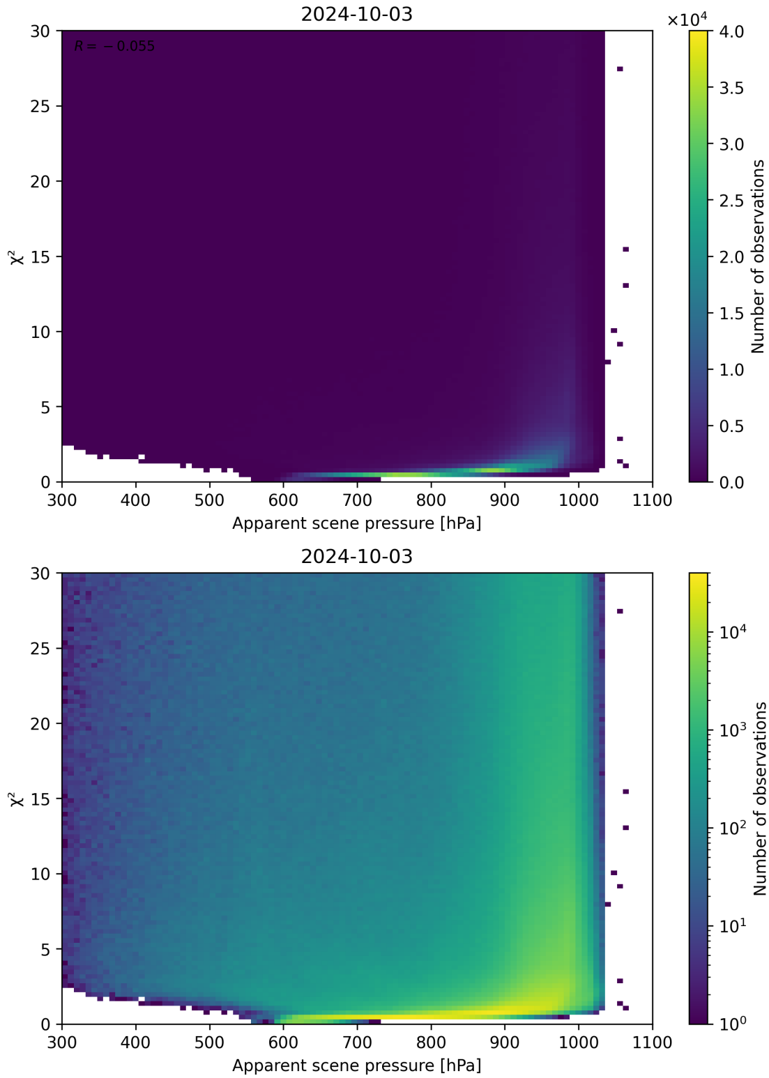
Figure 63: Scatter density plot of “Apparent scene pressure” against “ \chi^2 ” for 2024-10-03 to 2024-10-04.
