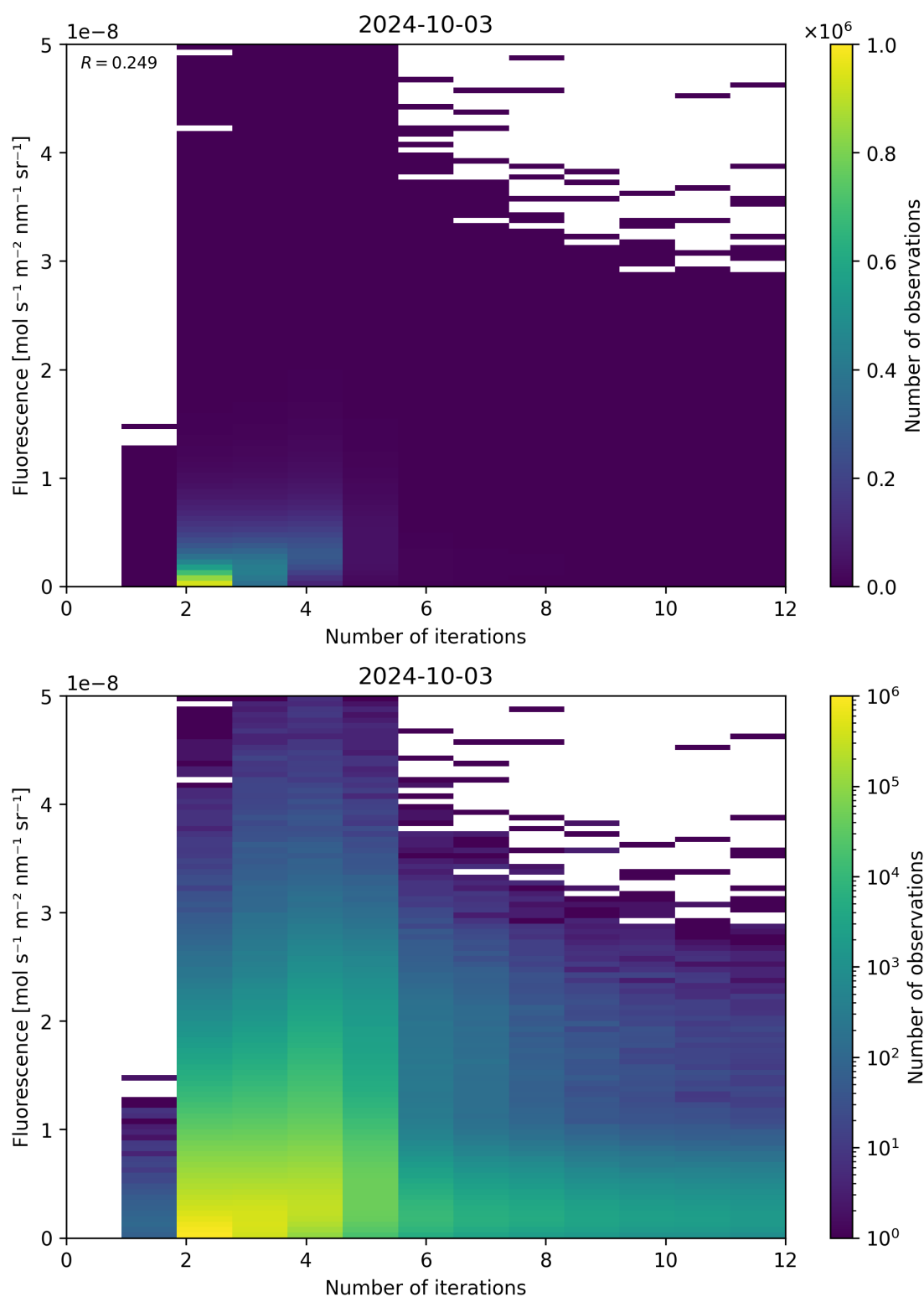
Figure 107: Scatter density plot of “Number of iterations” against “Fluorescence” for 2024-10-03 to 2024-10-04.
