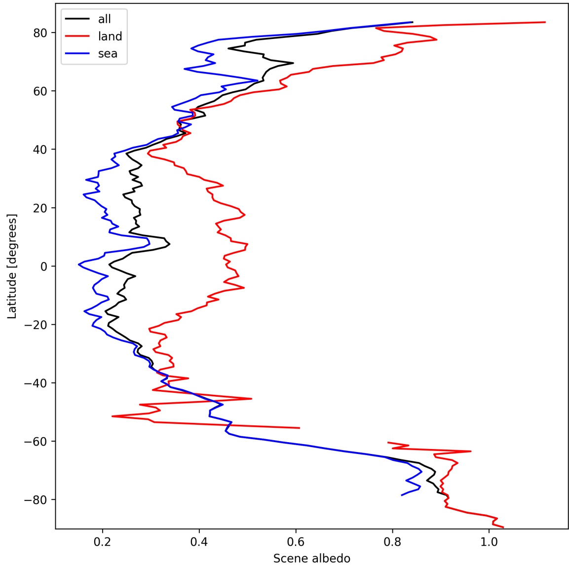
Figure 17: Zonal average of “Scene albedo” for 2024-10-03 to 2024-10-04.
