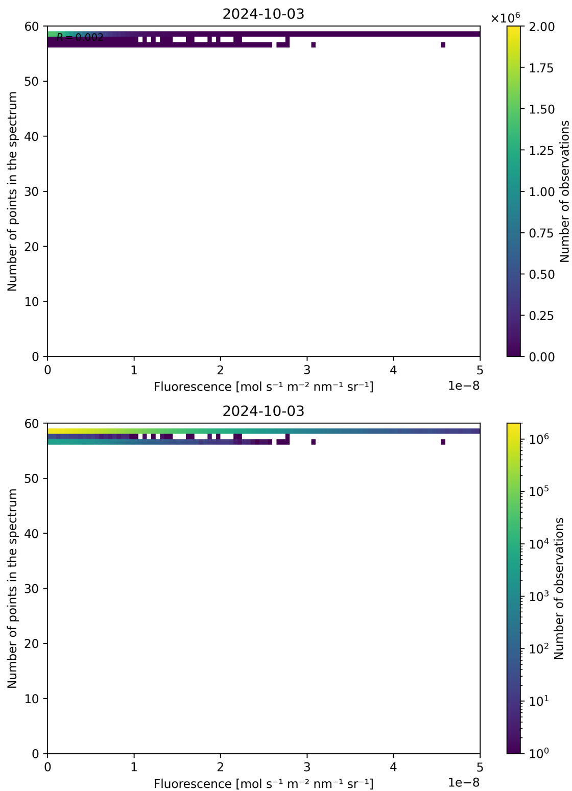
Figure 94: Scatter density plot of “Fluorescence” against “Number of points in the spectrum” for 2024-10-03 to 2024-10-04.
