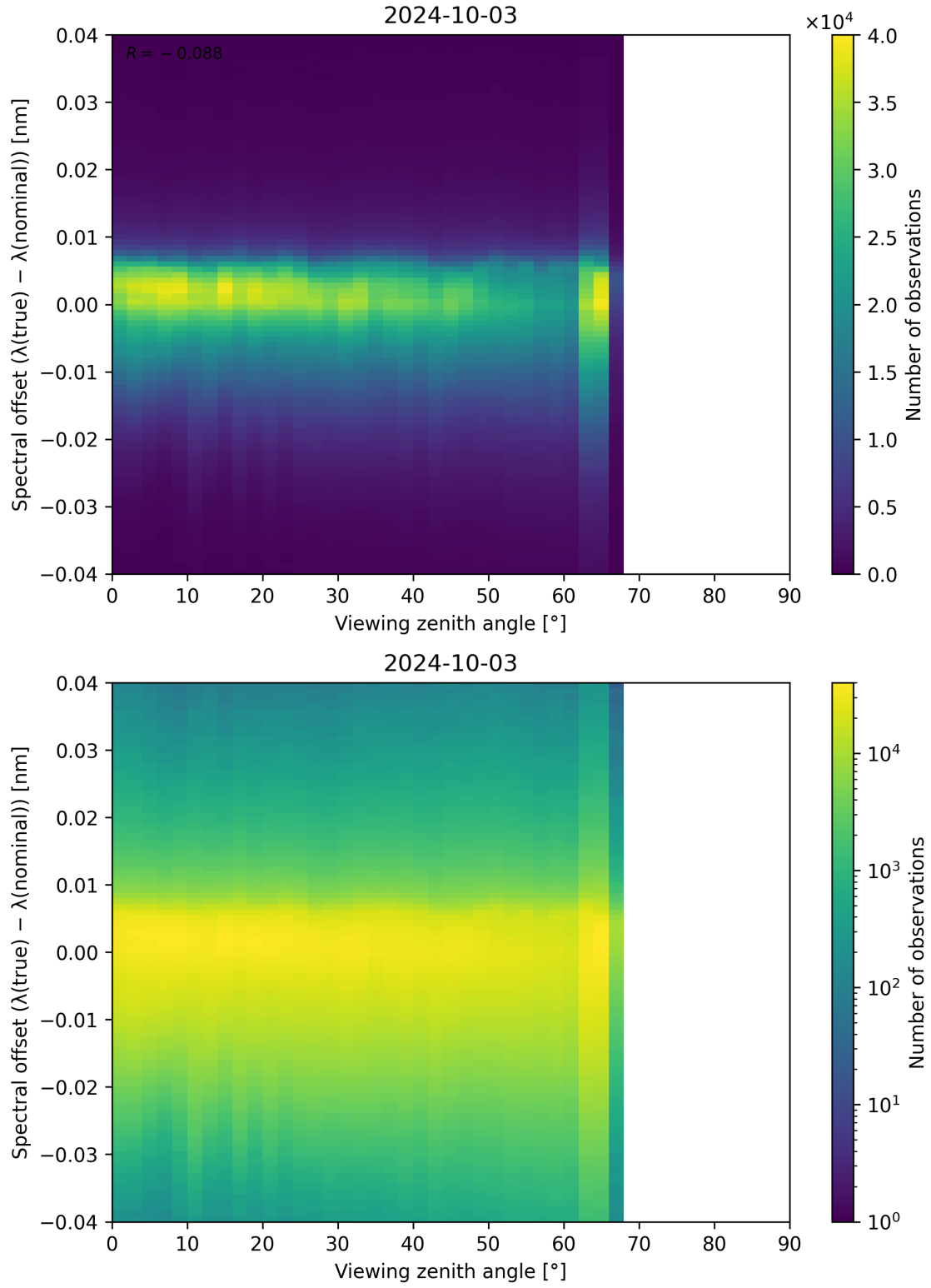
Figure 140: Scatter density plot of “Viewing zenith angle” against “Spectral offset ( \lambda_{\text{true}} - \lambda_{\text{nominal}} )” for 2024-10-03 to 2024-10-04.
