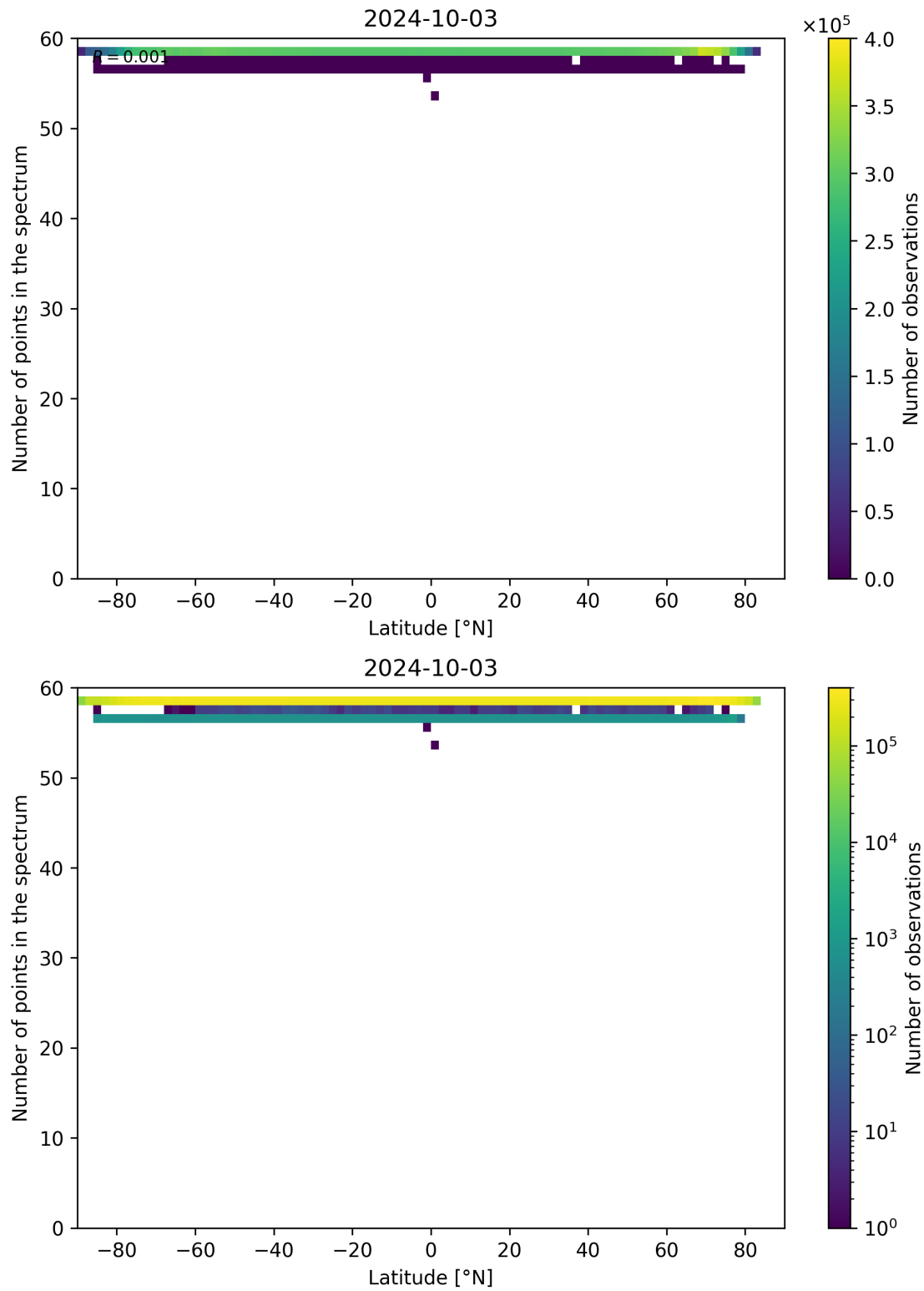
Figure 103: Scatter density plot of “Latitude” against “Number of points in the spectrum” for 2024-10-03 to 2024-10-04.
