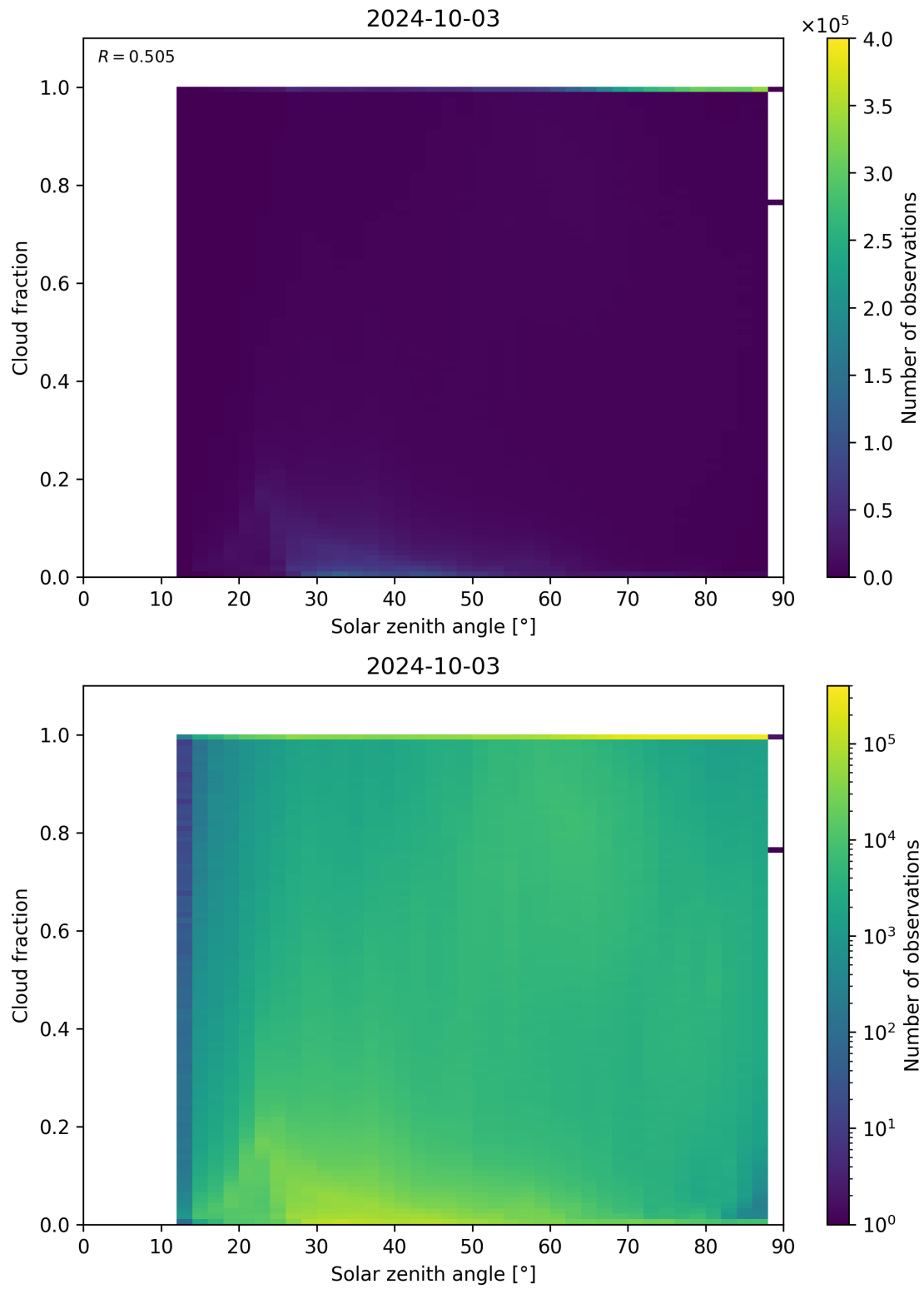
Figure 121: Scatter density plot of “Solar zenith angle” against “Cloud fraction” for 2024-10-03 to 2024-10-04.
