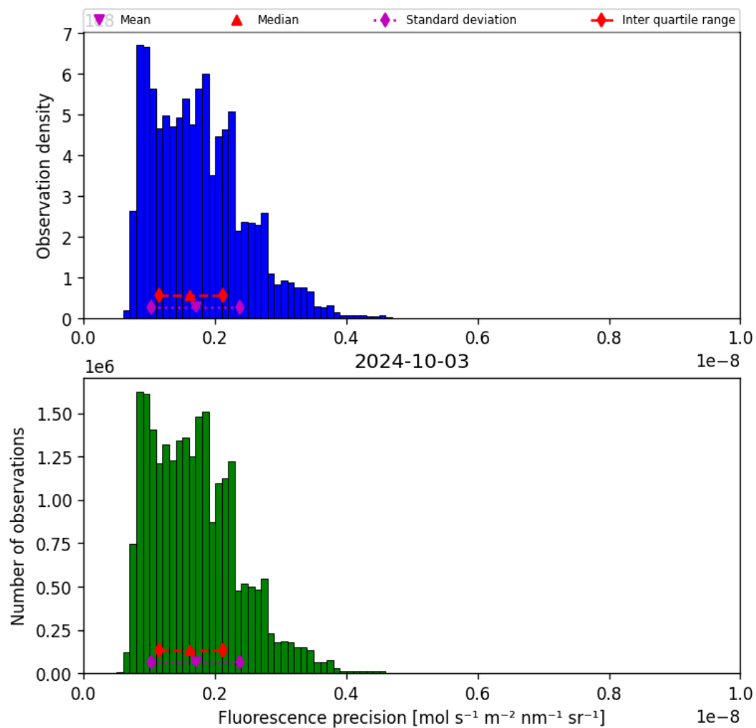
Figure 41: Histogram of “Fluorescence precision” for 2024-10-03 to 2024-10-04
