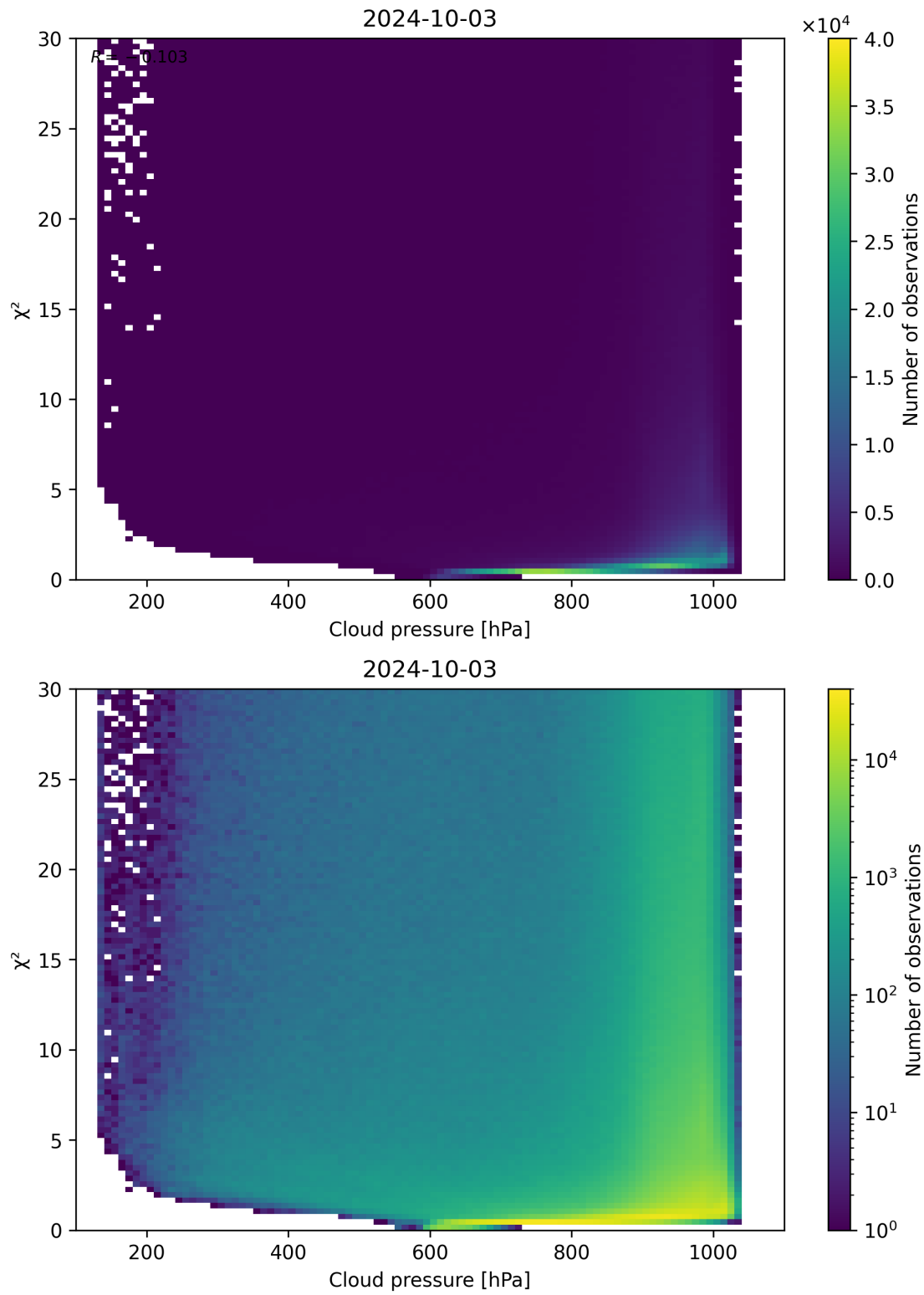
Figure 85: Scatter density plot of “Cloud pressure” against “ \chi^2 ” for 2024-10-03 to 2024-10-04.
