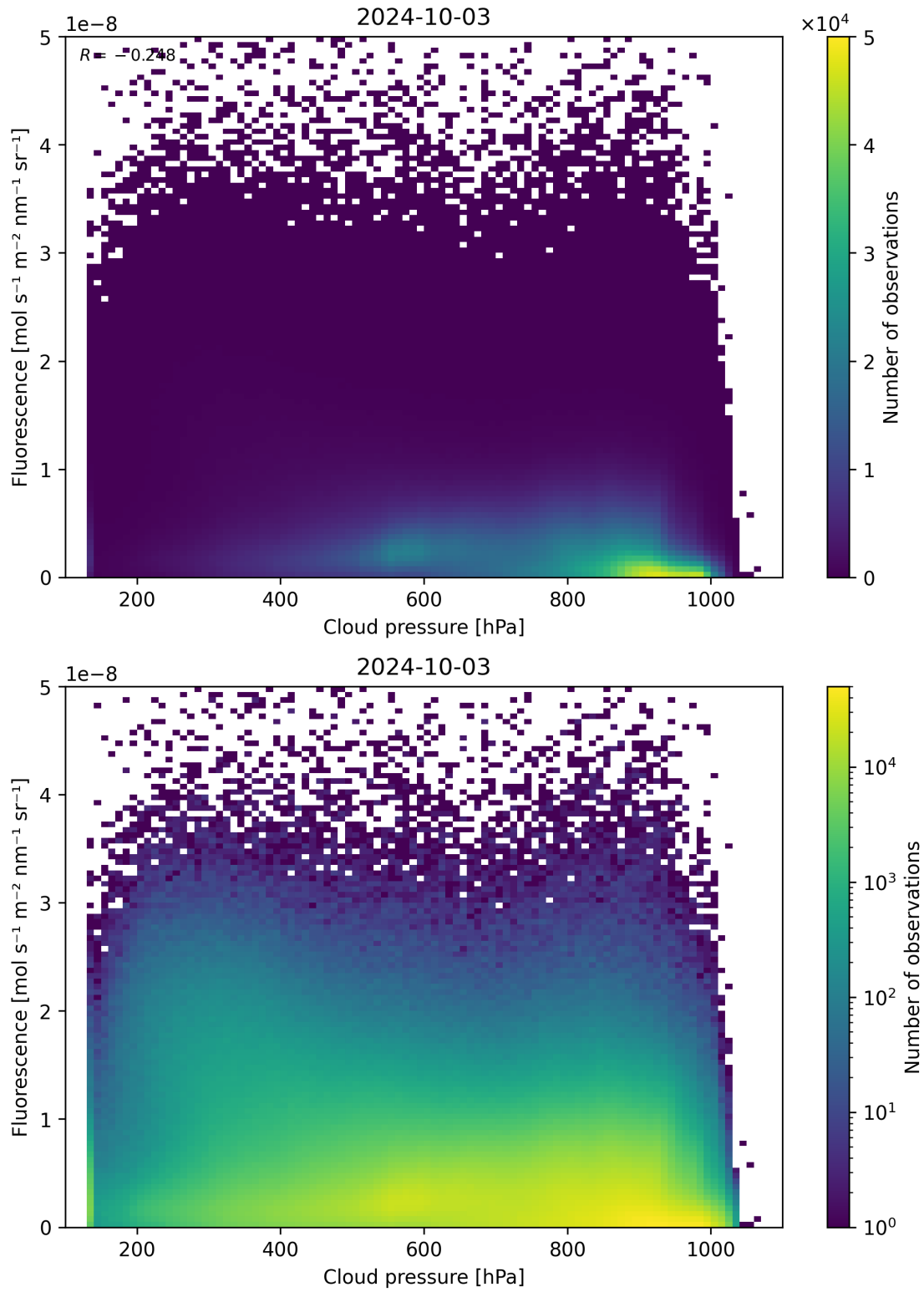
Figure 88: Scatter density plot of “Cloud pressure” against “Fluorescence” for 2024-10-03 to 2024-10-04.
