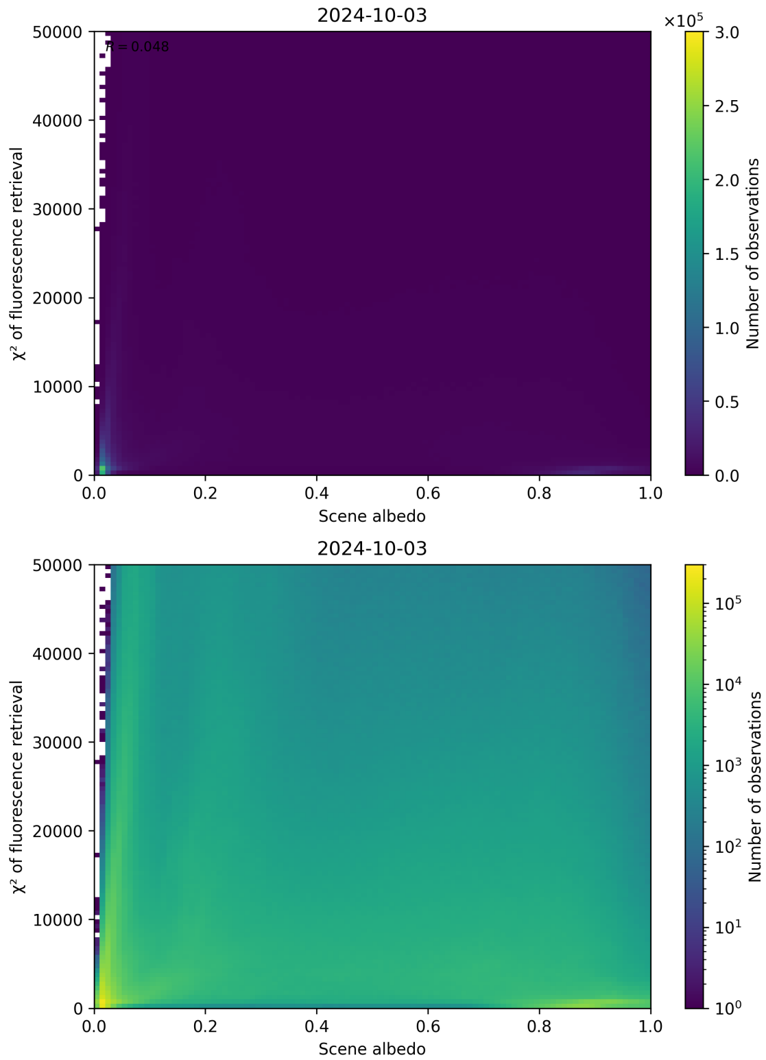
Figure 113: Scatter density plot of “Scene albedo” against “ \chi^2 of fluorescence retrieval” for 2024-10-03 to 2024-10-04.
