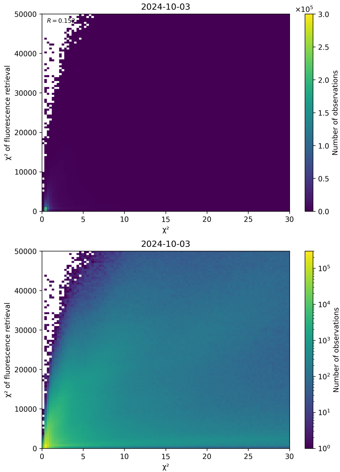
Figure 69: Scatter density plot of “ \chi^2 ” against “ \chi^2 of fluorescence retrieval” for 2024-10-03 to 2024-10-04.
