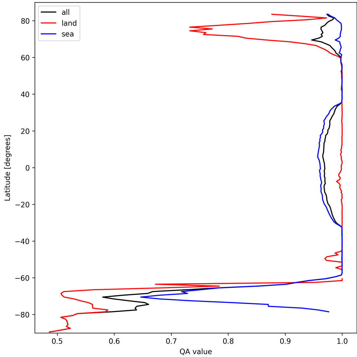
Figure 12: Zonal average of "QA value" for 2024-10-03 to 2024-10-04.
