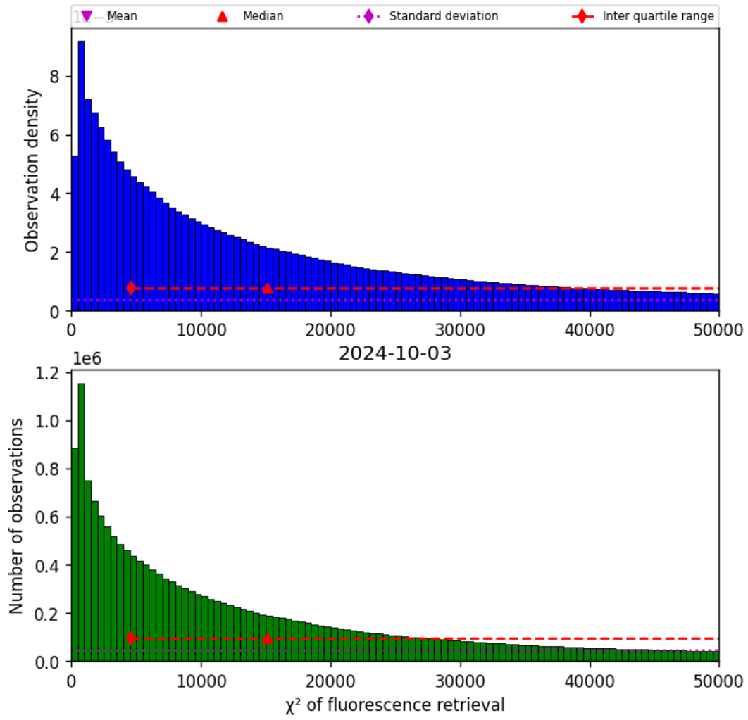
Figure 42: Histogram of “ \chi^2 of fluorescence retrieval” for 2024-10-03 to 2024-10-04
