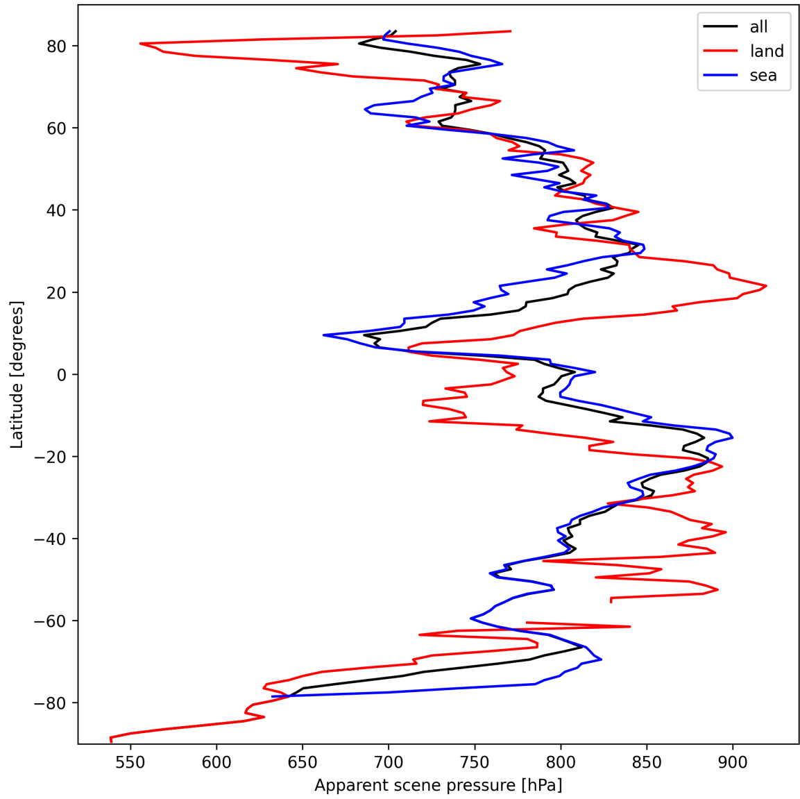
Figure 19: Zonal average of “Apparent scene pressure” for 2024-10-03 to 2024-10-04.
