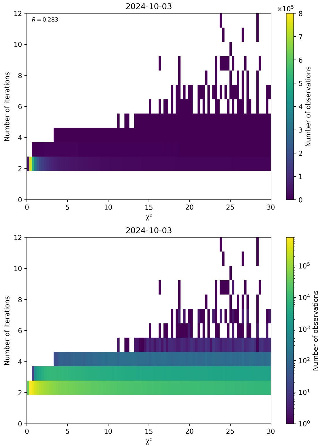
Figure 73: Scatter density plot of “ \chi^2 ” against “Number of iterations” for 2024-10-03 to 2024-10-04.
