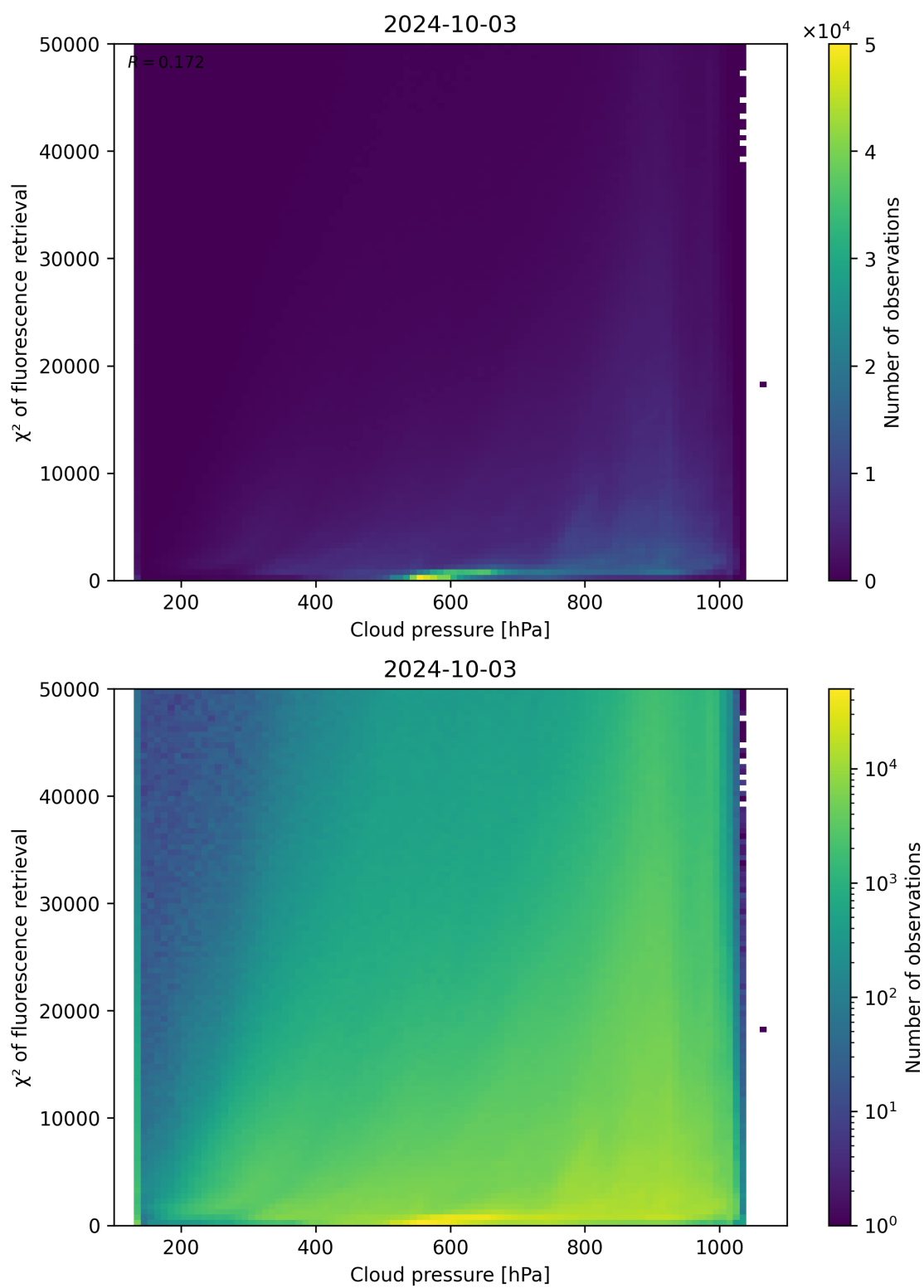
Figure 86: Scatter density plot of “Cloud pressure” against “ \chi^2 of fluorescence retrieval” for 2024-10-03 to 2024-10-04.
