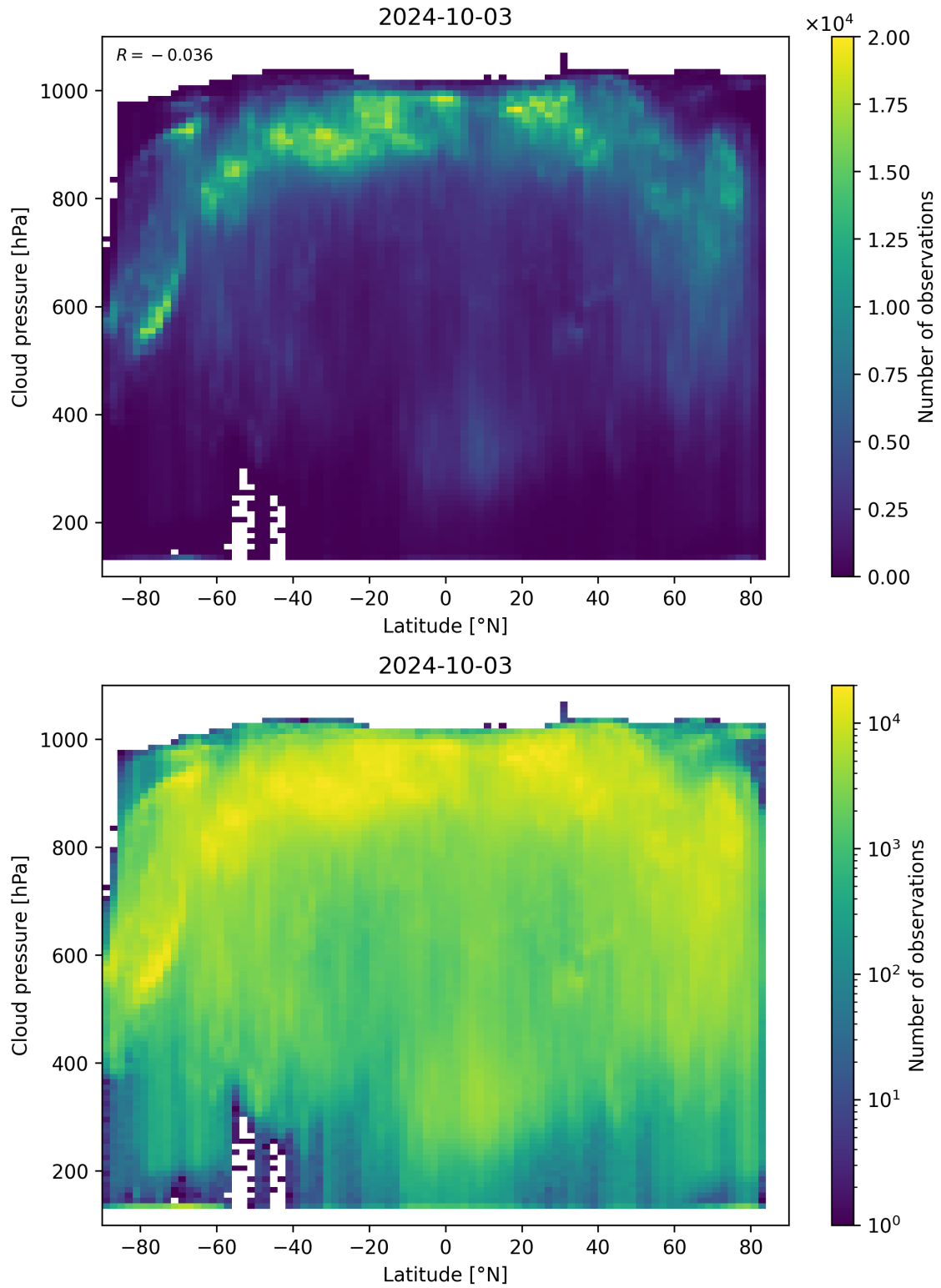
Figure 100: Scatter density plot of “Latitude” against “Cloud pressure” for 2024-10-03 to 2024-10-04.
