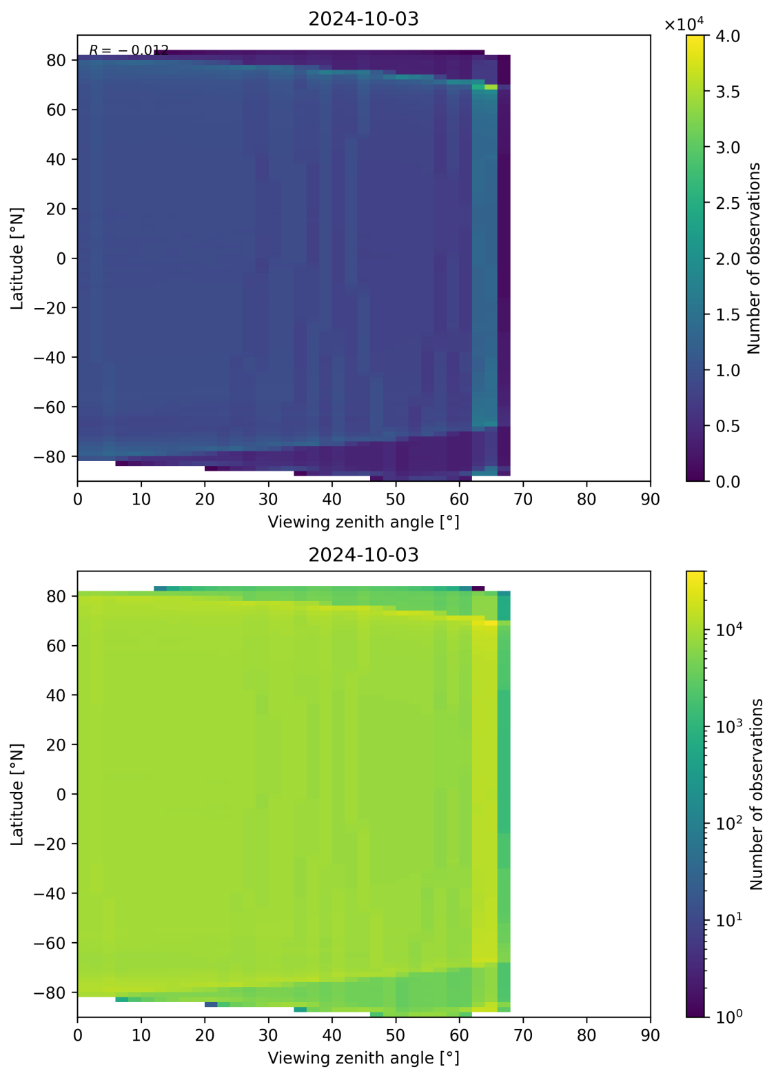
Figure 135: Scatter density plot of “Viewing zenith angle” against “Latitude” for 2024-10-03 to 2024-10-04.
