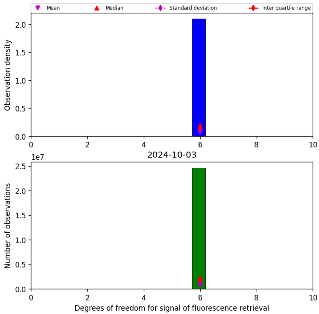
Figure 43: Histogram of “Degrees of freedom for signal of fluorescence retrieval” for 2024-10-03 to 2024-10-04
