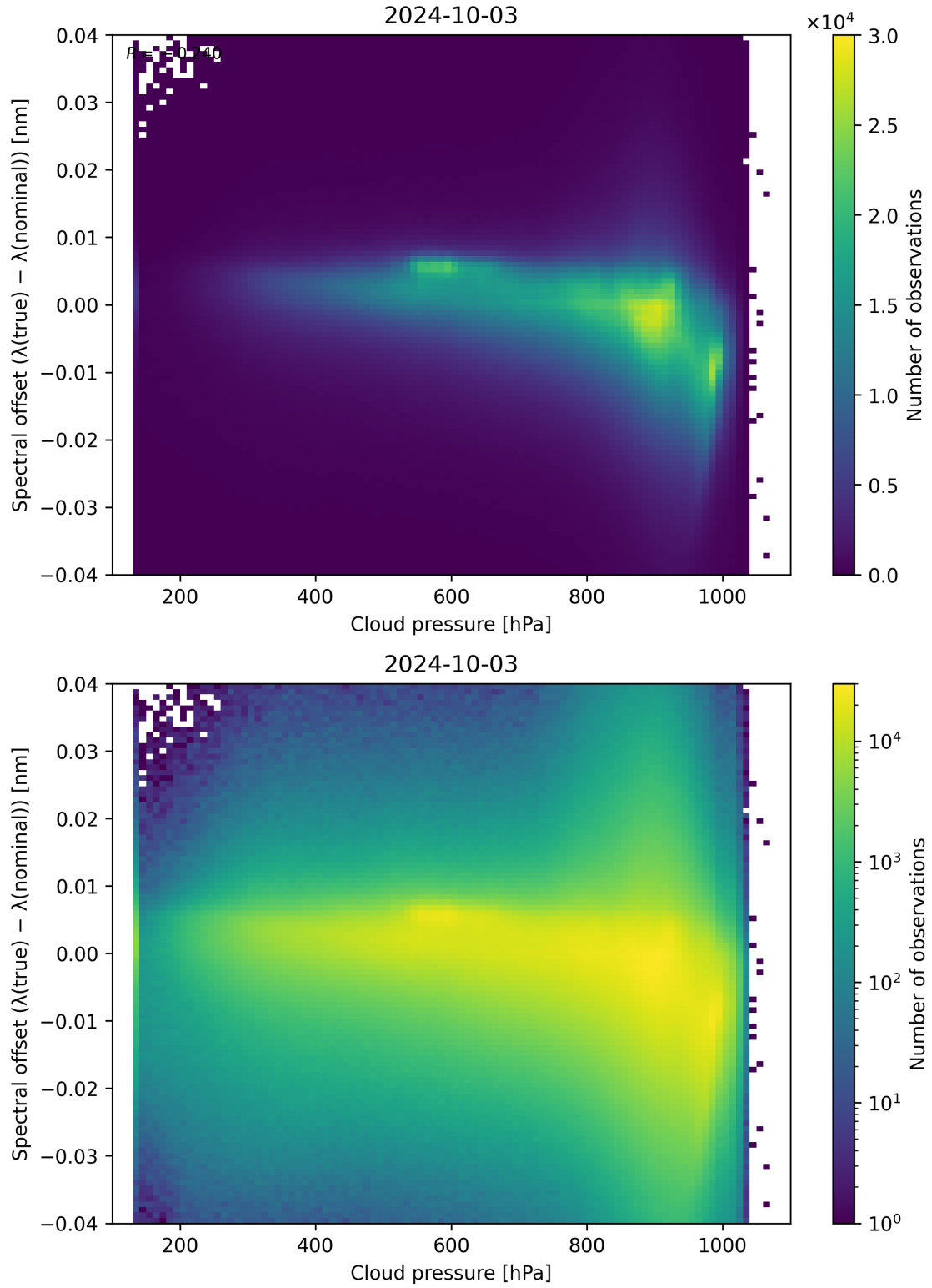
Figure 92: Scatter density plot of “Cloud pressure” against “Spectral offset ( \lambda_{\text{true}} - \lambda_{\text{nominal}} )” for 2024-10-03 to 2024-10-04.
