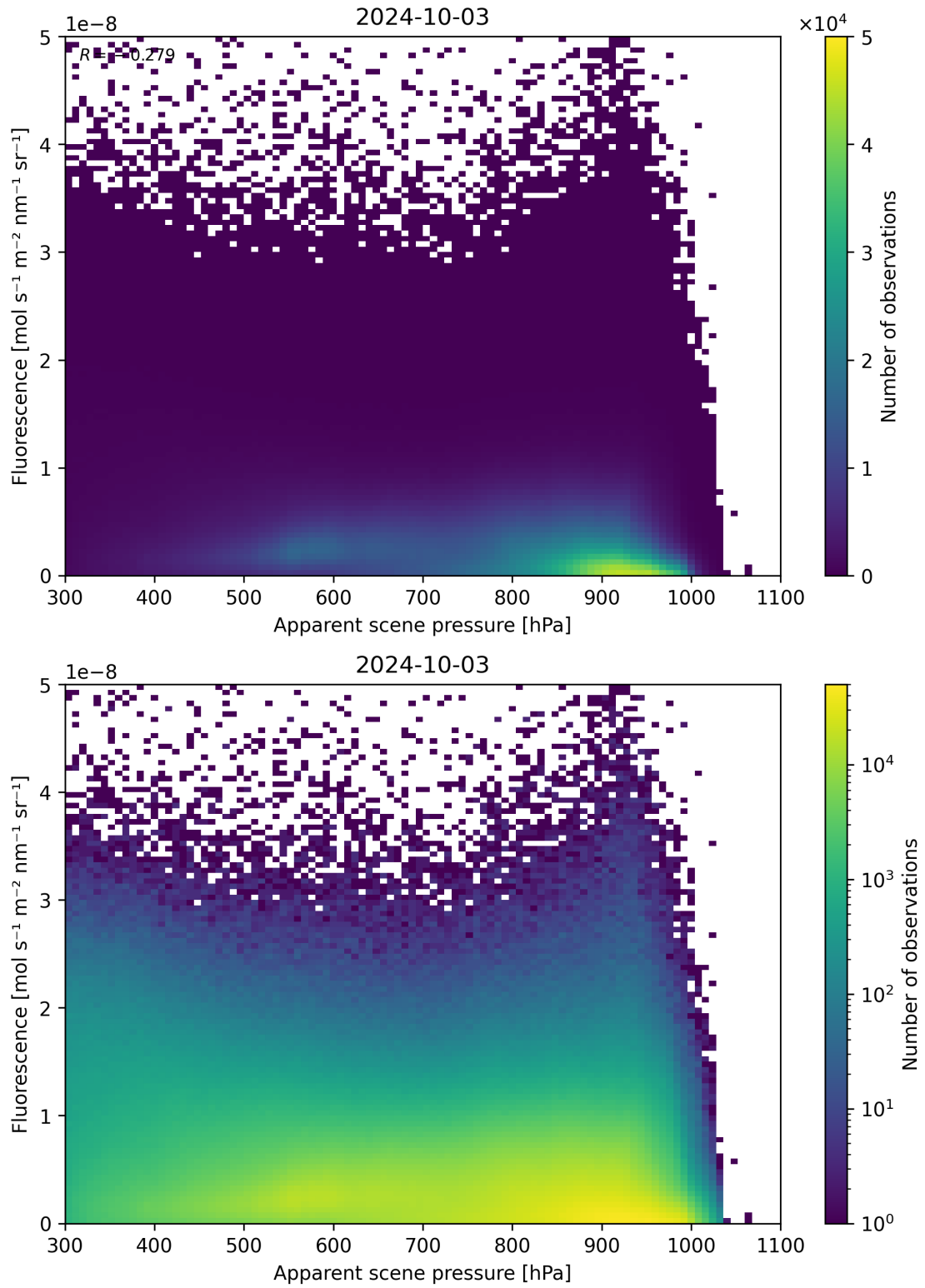
Figure 65: Scatter density plot of “Apparent scene pressure” against “Fluorescence” for 2024-10-03 to 2024-10-04.
