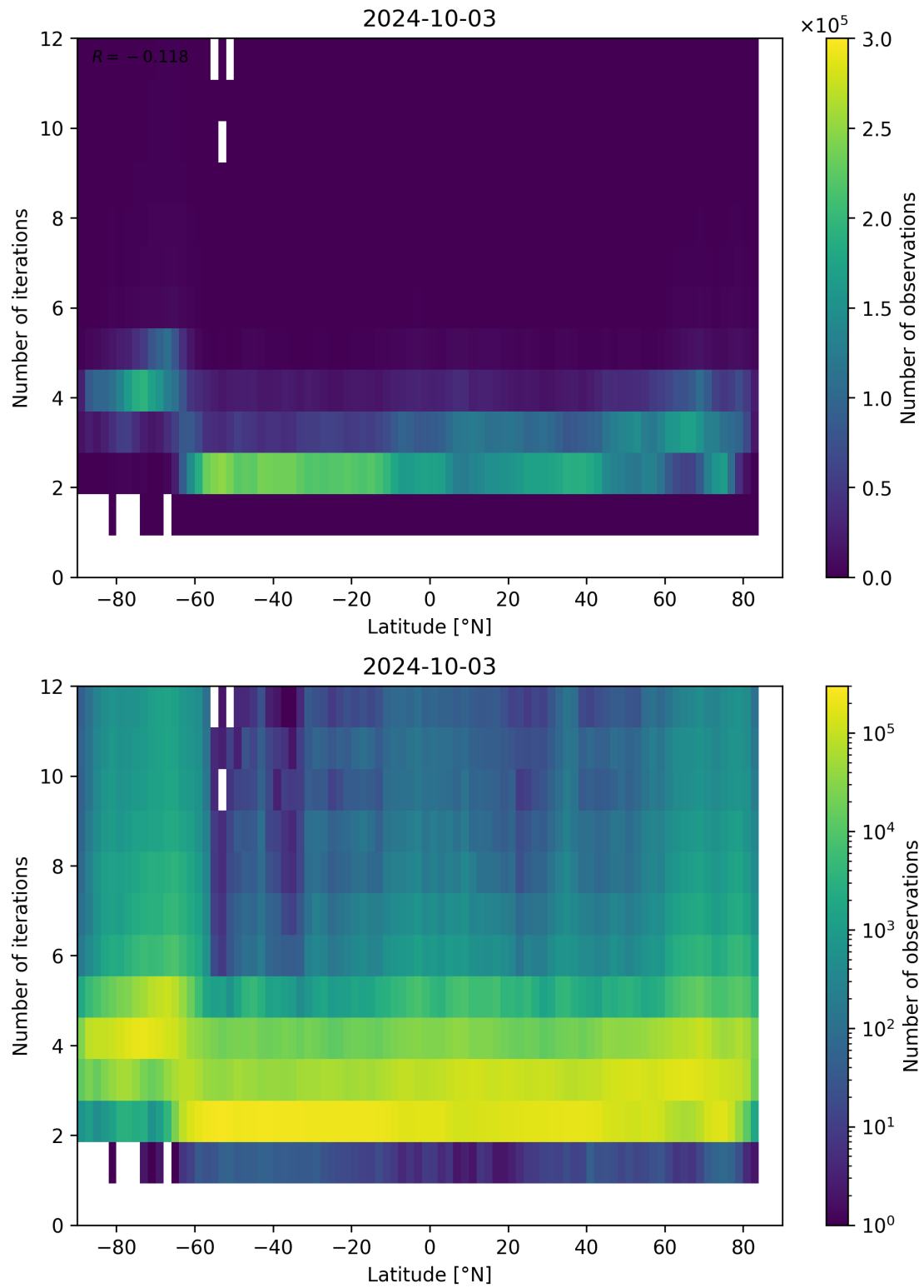
Figure 102: Scatter density plot of “Latitude” against “Number of iterations” for 2024-10-03 to 2024-10-04.
