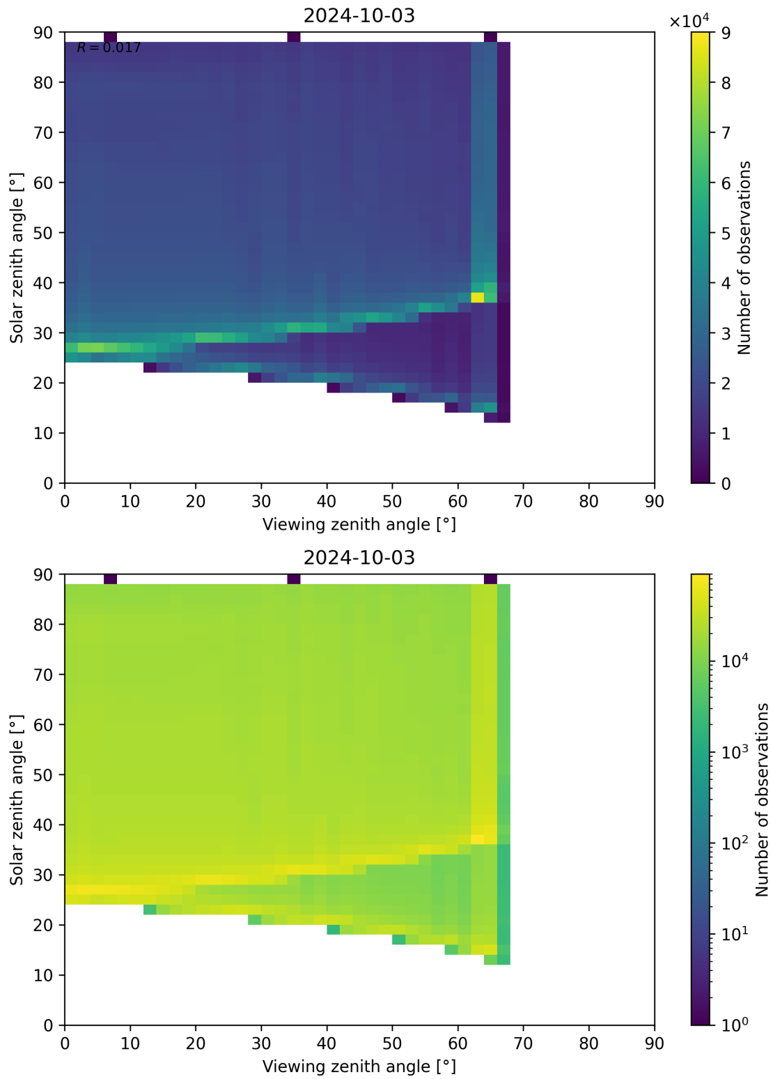
Figure 139: Scatter density plot of “Viewing zenith angle” against “Solar zenith angle” for 2024-10-03 to 2024-10-04.
