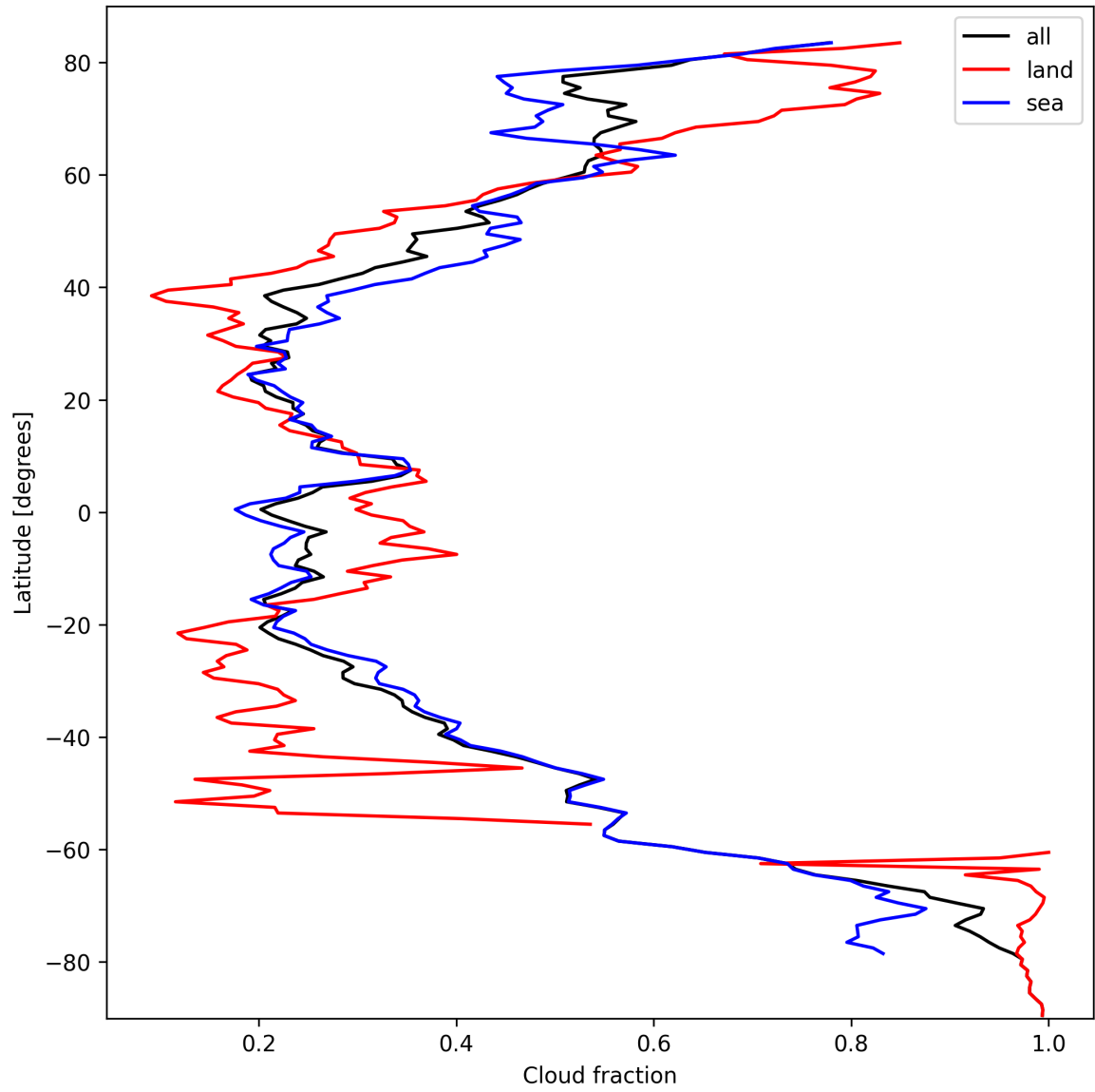
Figure 15: Zonal average of “Cloud fraction” for 2024-10-03 to 2024-10-04.
