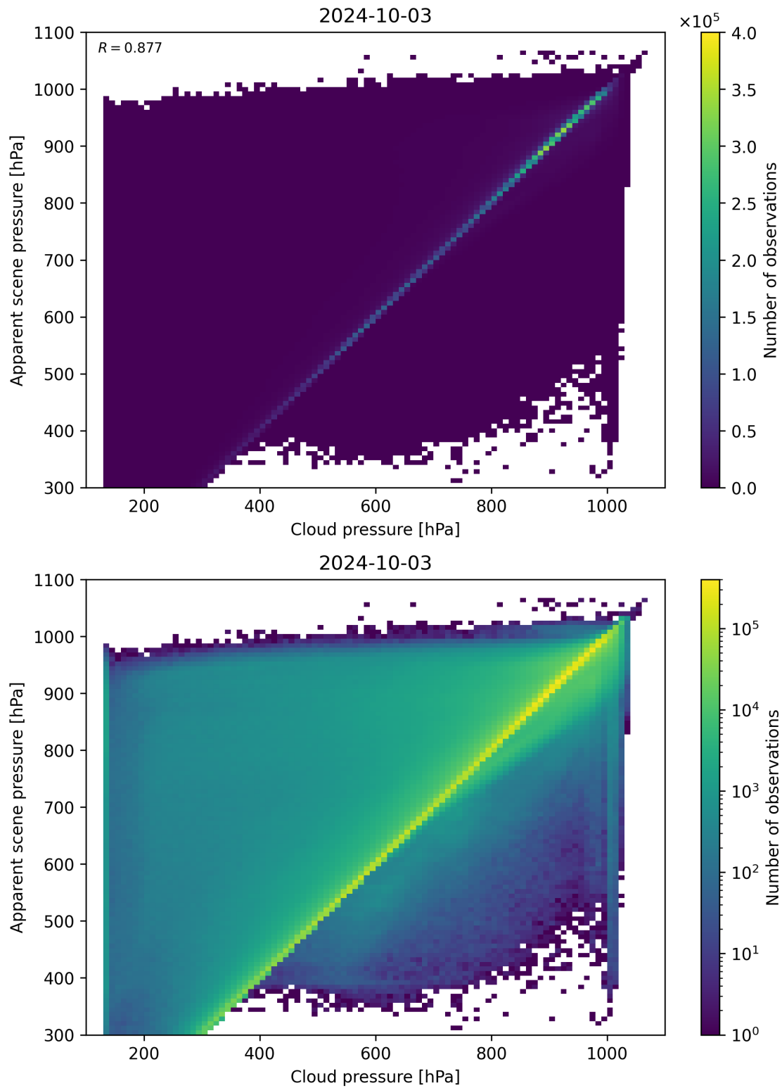
Figure 84: Scatter density plot of “Cloud pressure” against “Apparent scene pressure” for 2024-10-03 to 2024-10-04.
