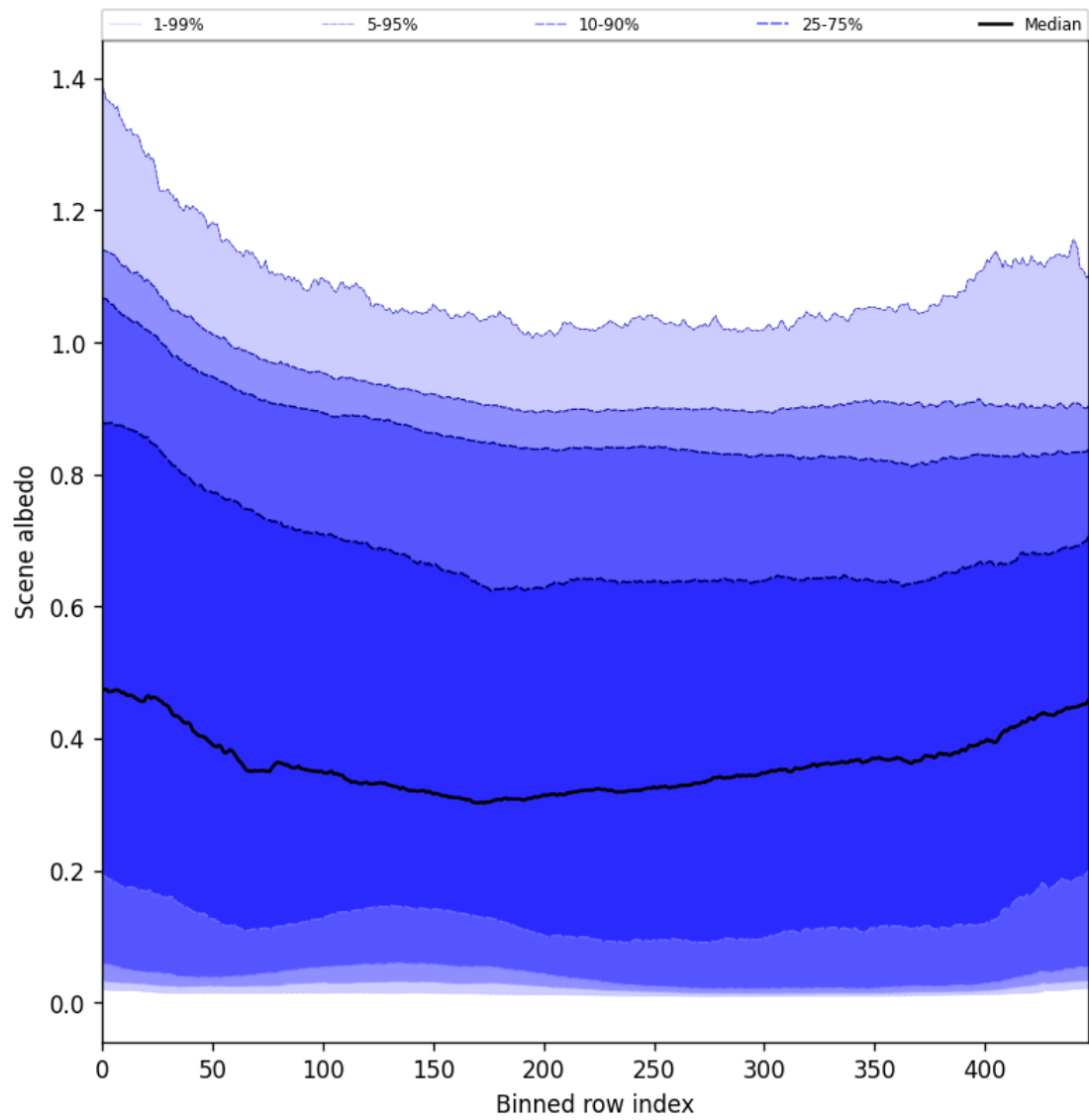
Figure 51: Along track statistics of “Scene albedo” for 2024-10-03 to 2024-10-04
