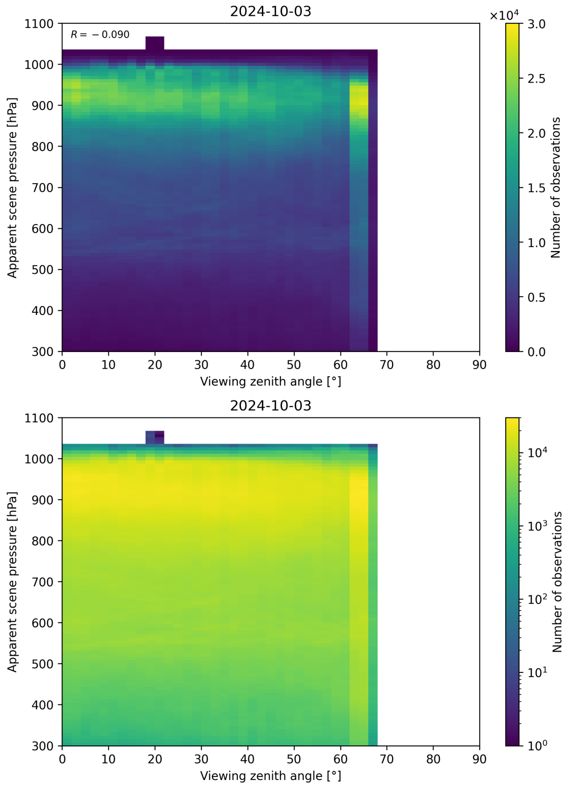
Figure 129: Scatter density plot of “Viewing zenith angle” against “Apparent scene pressure” for 2024-10-03 to 2024-10-04.
