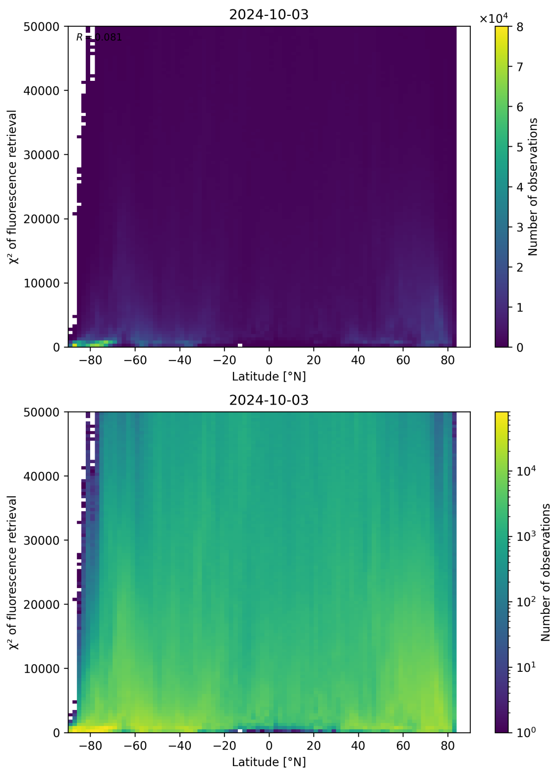
Figure 98: Scatter density plot of “Latitude” against “ \chi^2 of fluorescence retrieval” for 2024-10-03 to 2024-10-04.
