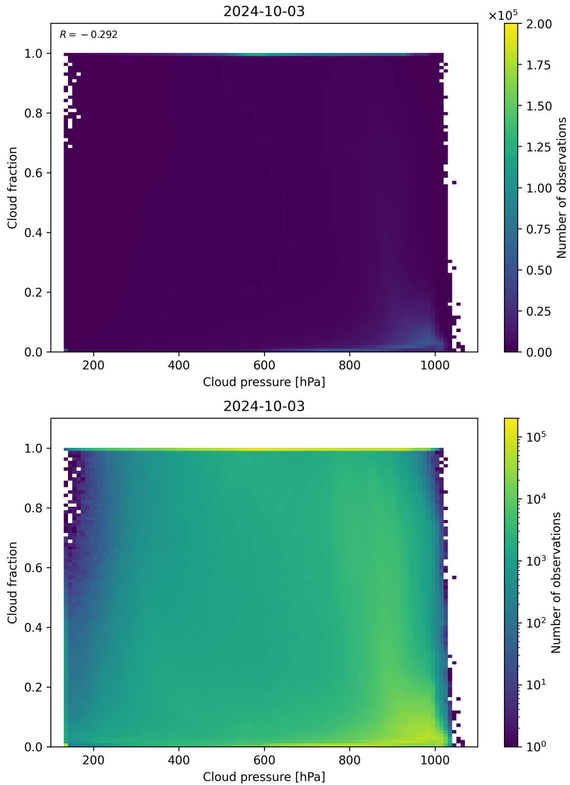
Figure 87: Scatter density plot of “Cloud pressure” against “Cloud fraction” for 2024-10-03 to 2024-10-04.
