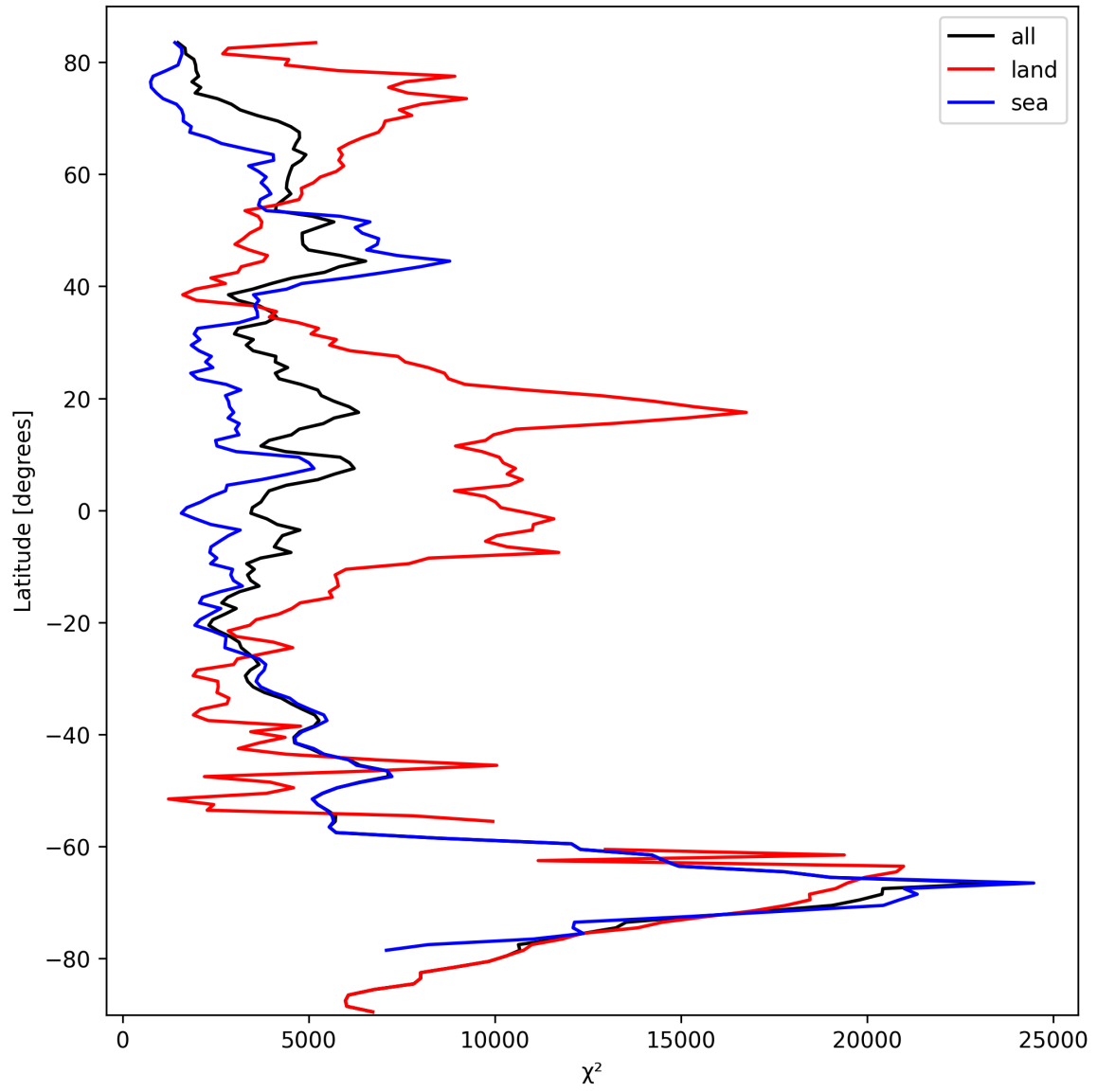
Figure 21: Zonal average of “ \chi^2 ” for 2024-10-03 to 2024-10-04.
