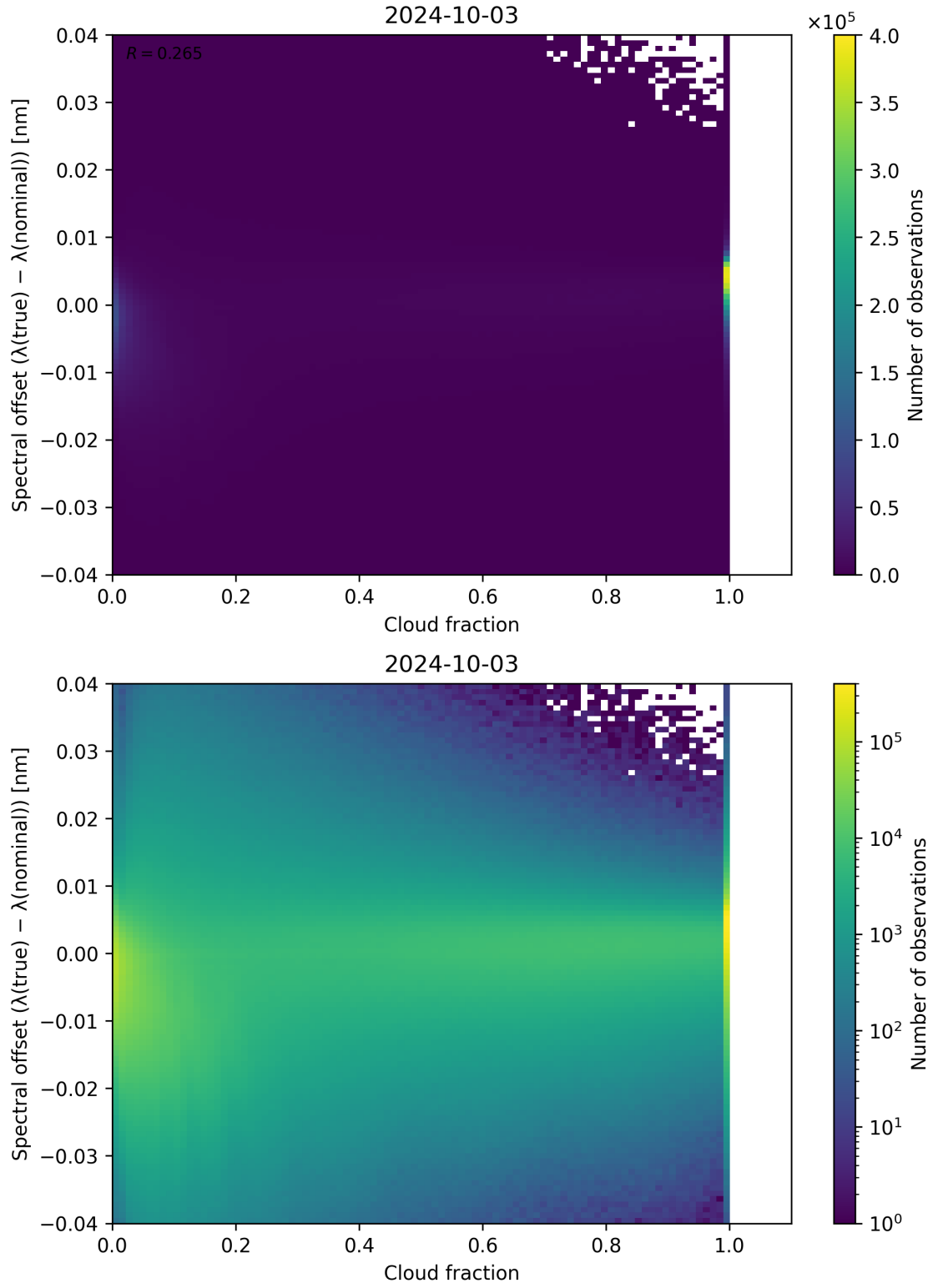
Figure 83: Scatter density plot of “Cloud fraction” against “Spectral offset ( \lambda_{\text{true}} - \lambda_{\text{nominal}} )” for 2024-10-03 to 2024-10-04.
