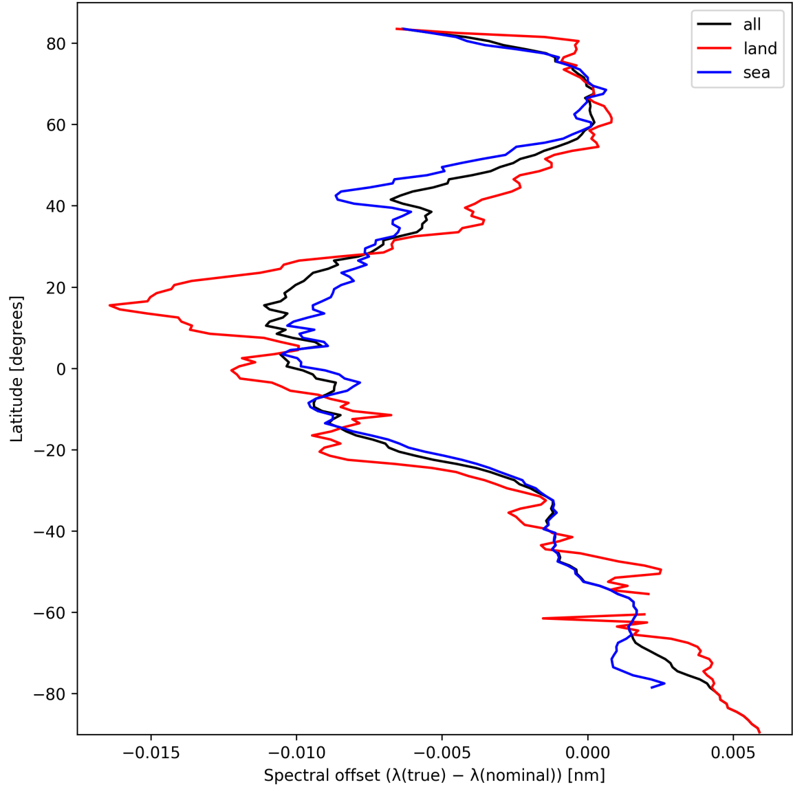
Figure 28: Zonal average of “Spectral offset ( \lambda_{\text{true}} - \lambda_{\text{nominal}} )” for 2024-10-03 to 2024-10-04.
