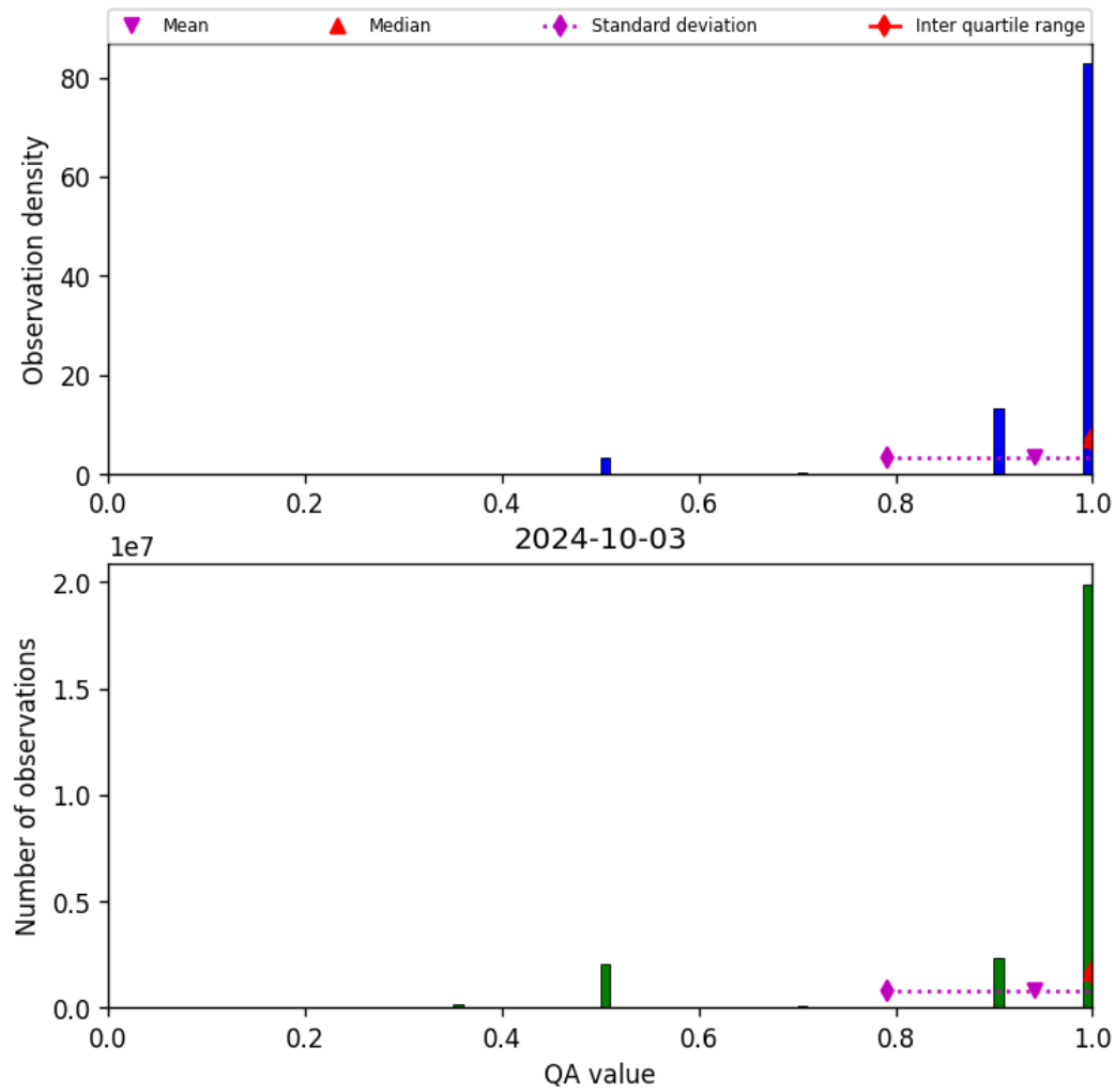
Figure 29: Histogram of “QA value” for 2024-10-03 to 2024-10-04
