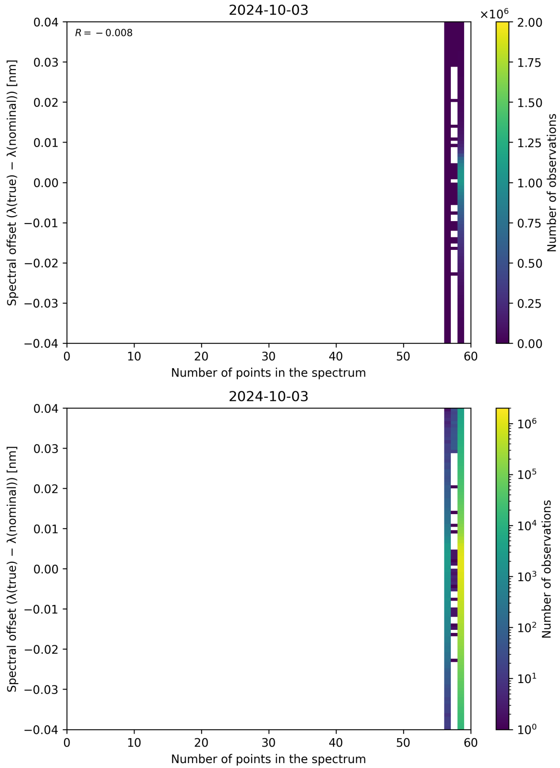
Figure 110: Scatter density plot of “Number of points in the spectrum” against “Spectral offset ( \lambda_{\text{true}} - \lambda_{\text{nominal}} )” for 2024-10-03 to 2024-10-04.
