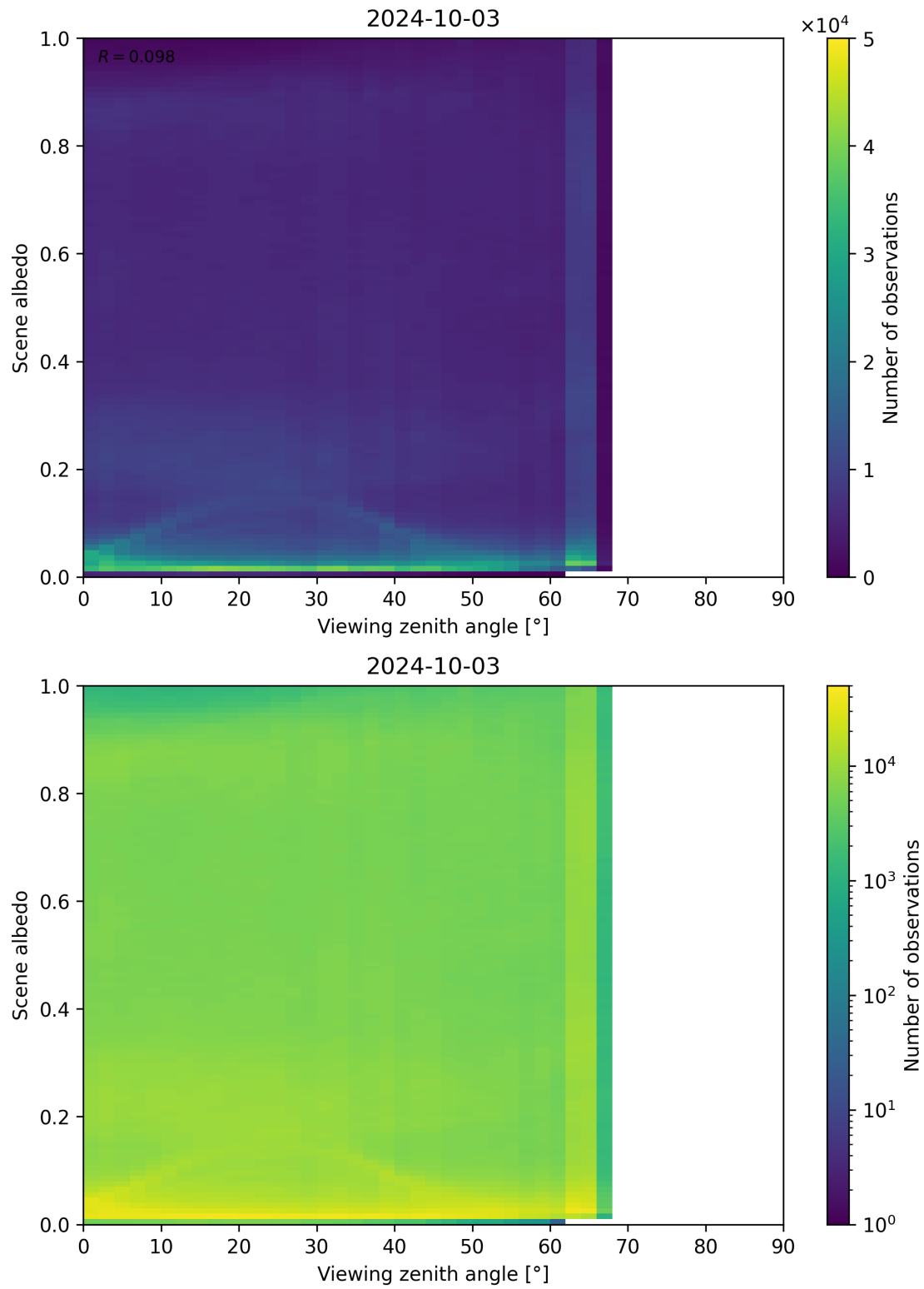
Figure 138: Scatter density plot of “Viewing zenith angle” against “Scene albedo” for 2024-10-03 to 2024-10-04.
