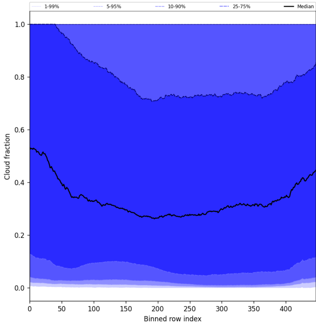
Figure 49: Along track statistics of “Cloud fraction” for 2024-10-03 to 2024-10-04
