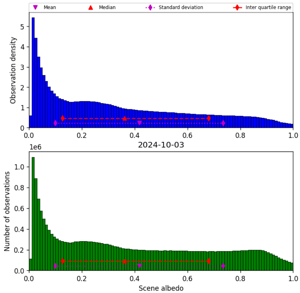
Figure 34: Histogram of “Scene albedo” for 2024-10-03 to 2024-10-04
