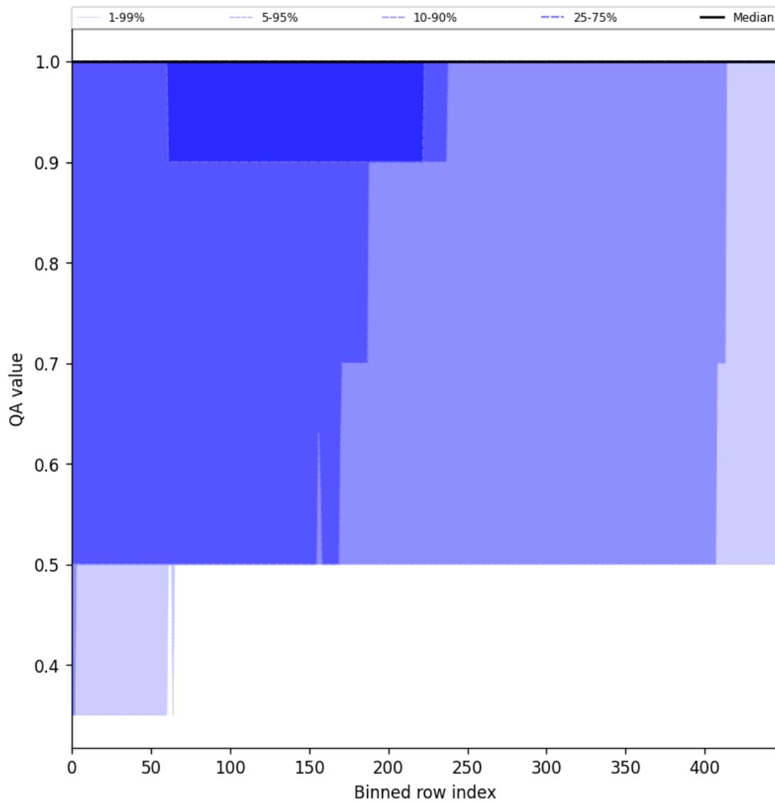
Figure 46: Along track statistics of “QA value” for 2024-10-03 to 2024-10-04
