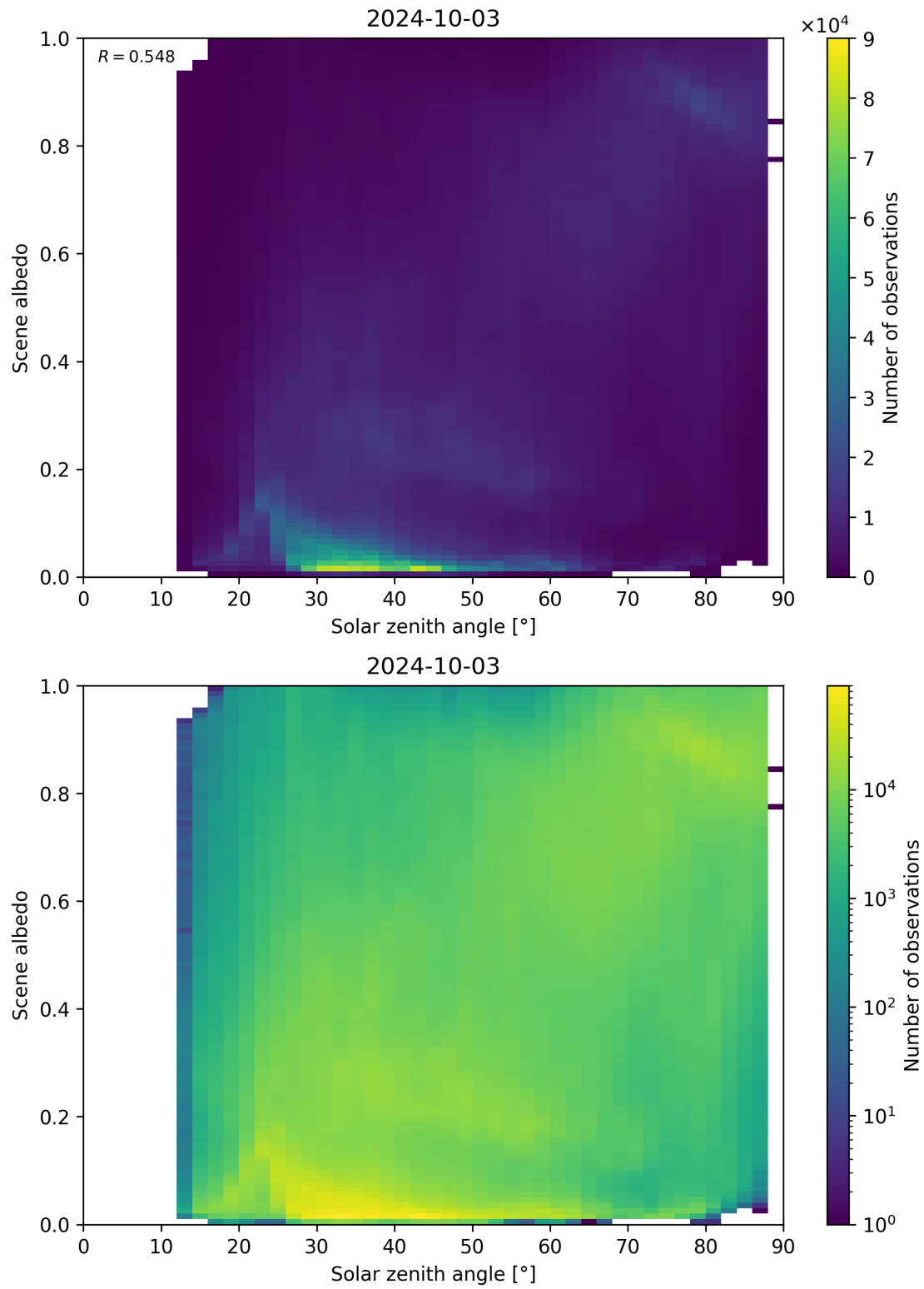
Figure 127: Scatter density plot of “Solar zenith angle” against “Scene albedo” for 2024-10-03 to 2024-10-04.
