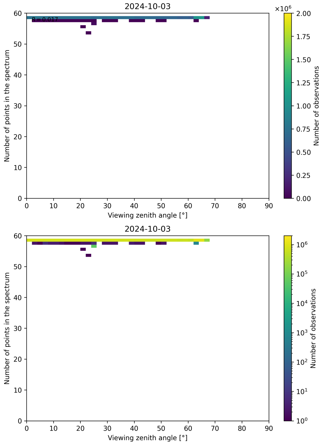
Figure 137: Scatter density plot of “Viewing zenith angle” against “Number of points in the spectrum” for 2024-10-03 to 2024-10-04.
