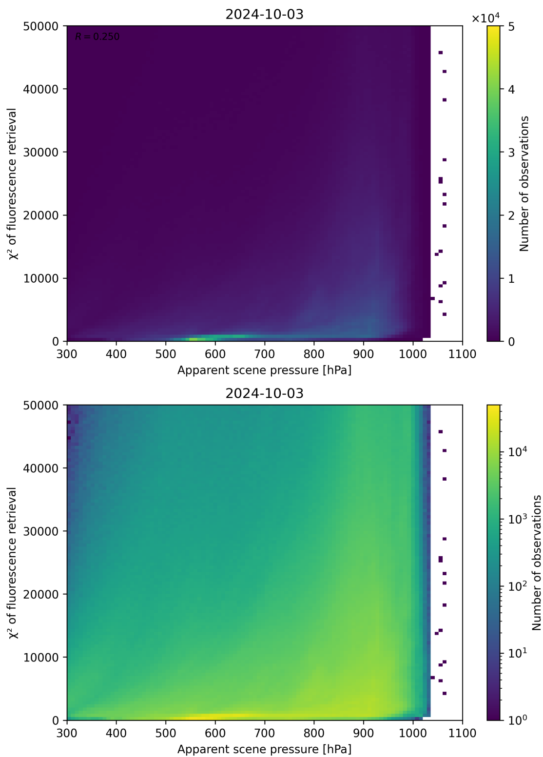
Figure 64: Scatter density plot of “Apparent scene pressure” against “ \chi^2 of fluorescence retrieval” for 2024-10-03 to 2024-10-04.
