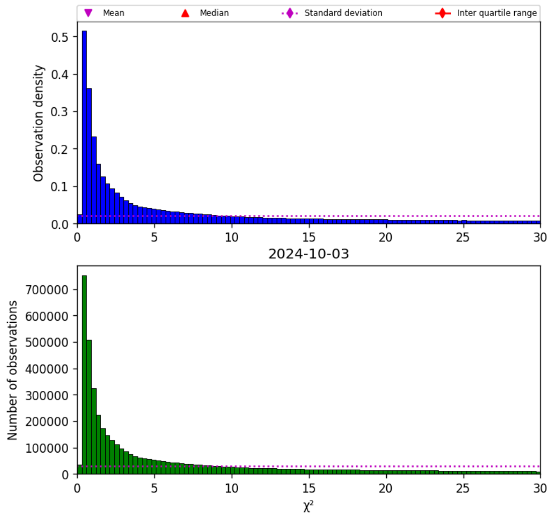
Figure 38: Histogram of “ \chi^2 ” for 2024-10-03 to 2024-10-04
