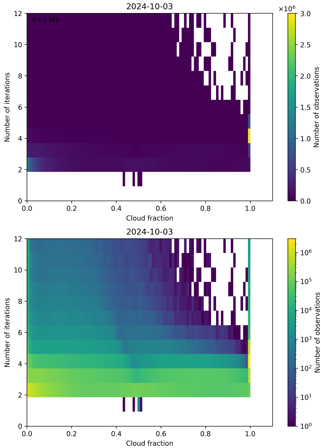
Figure 80: Scatter density plot of “Cloud fraction” against “Number of iterations” for 2024-10-03 to 2024-10-04.
