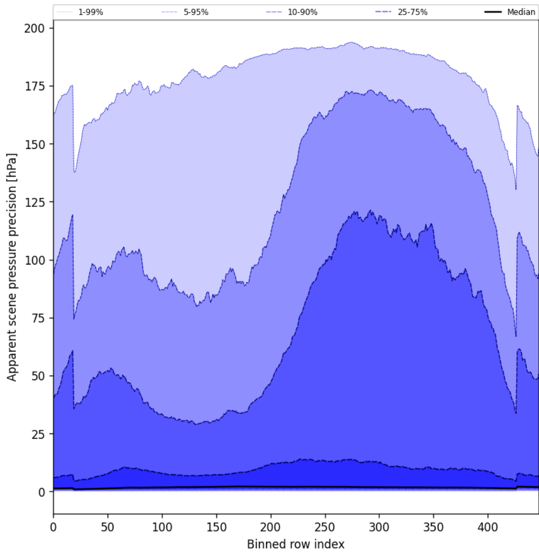
Figure 54: Along track statistics of “Apparent scene pressure precision” for 2024-10-03 to 2024-10-04
