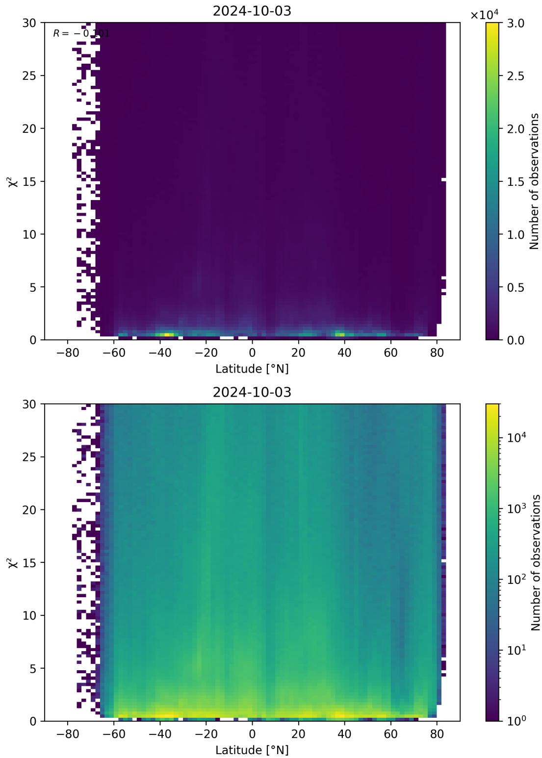
Figure 97: Scatter density plot of “Latitude” against “ \chi^2 ” for 2024-10-03 to 2024-10-04.
