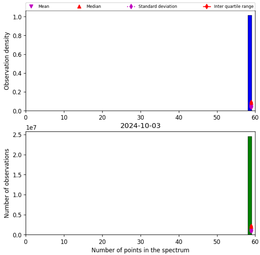
Figure 44: Histogram of “Number of points in the spectrum” for 2024-10-03 to 2024-10-04
