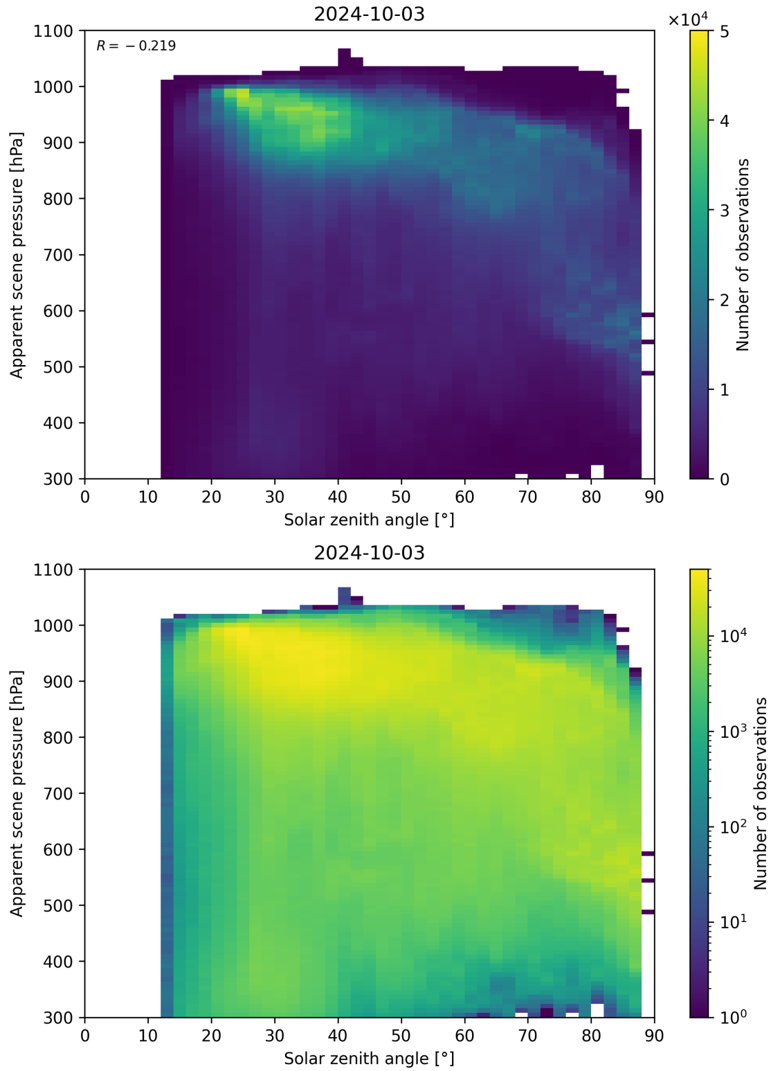
Figure 118: Scatter density plot of “Solar zenith angle” against “Apparent scene pressure” for 2024-10-03 to 2024-10-04.
