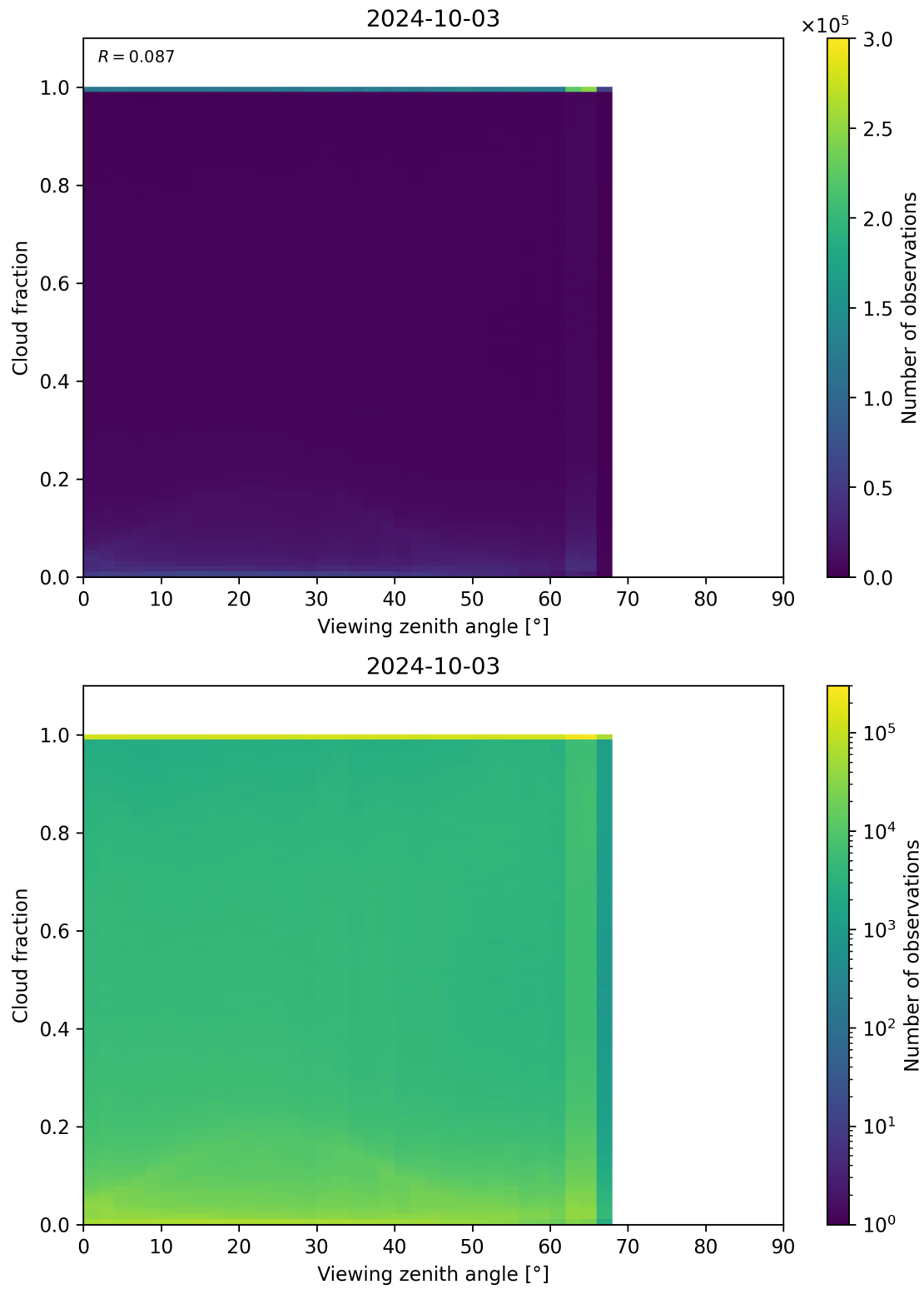
Figure 132: Scatter density plot of “Viewing zenith angle” against “Cloud fraction” for 2024-10-03 to 2024-10-04.
