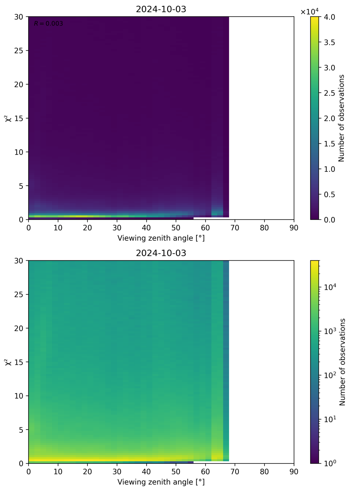
Figure 130: Scatter density plot of “Viewing zenith angle” against “ \chi^2 ” for 2024-10-03 to 2024-10-04.
