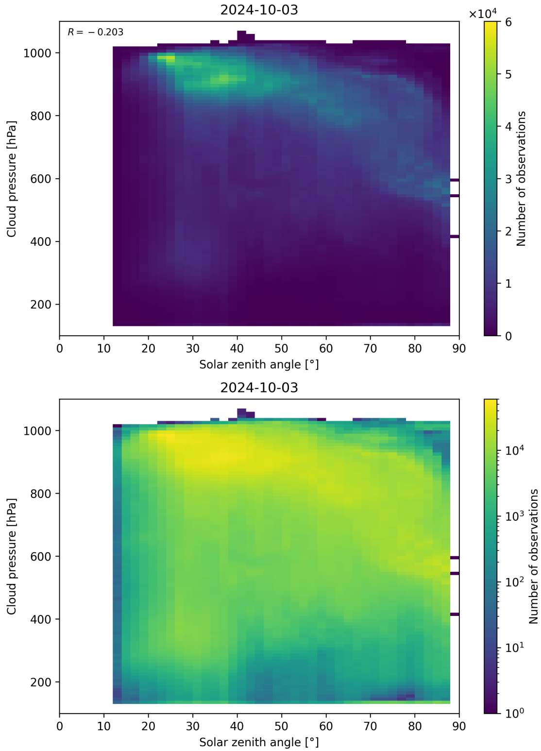
Figure 122: Scatter density plot of “Solar zenith angle” against “Cloud pressure” for 2024-10-03 to 2024-10-04.
