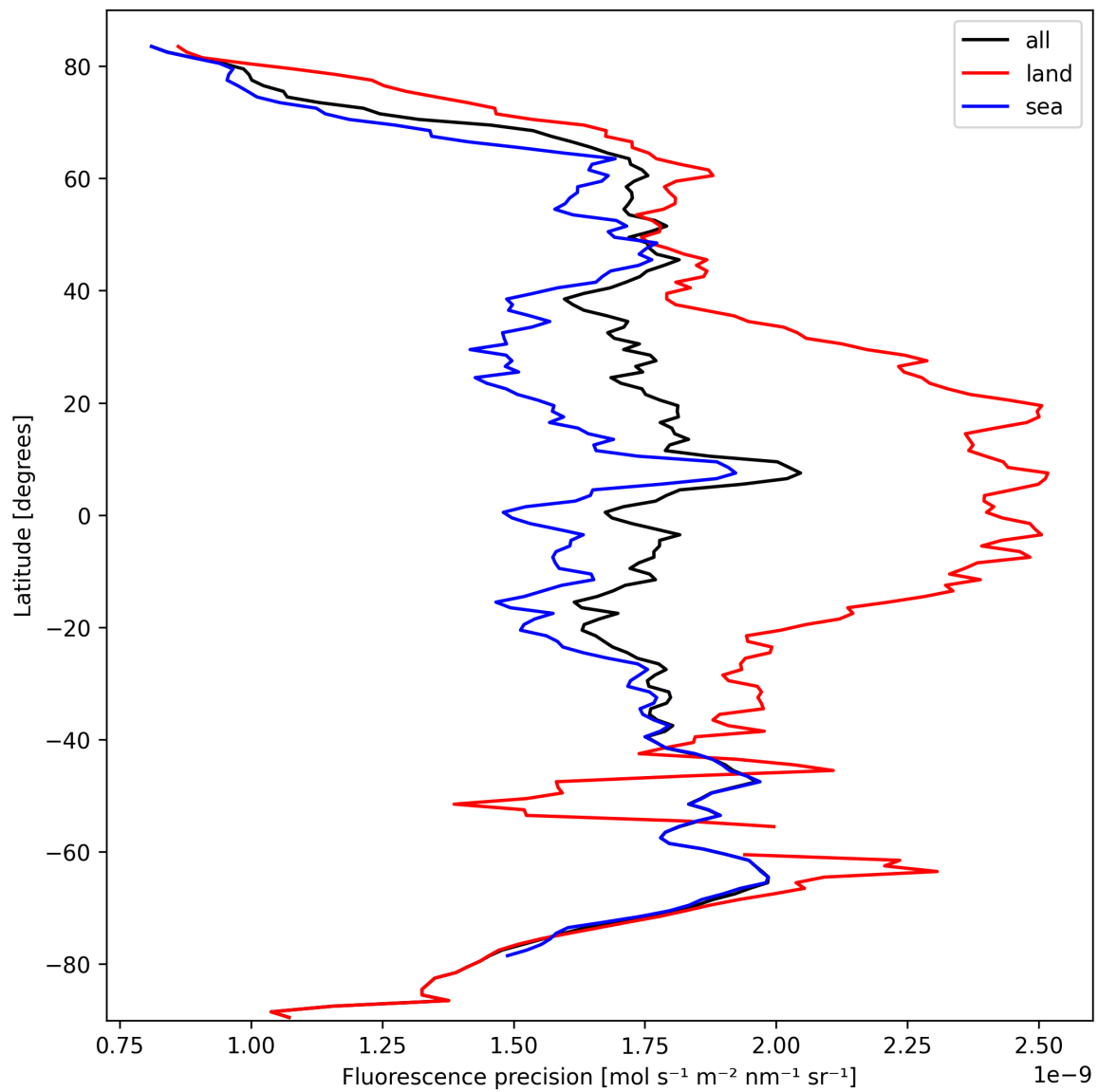
Figure 24: Zonal average of “Fluorescence precision” for 2024-10-03 to 2024-10-04.
