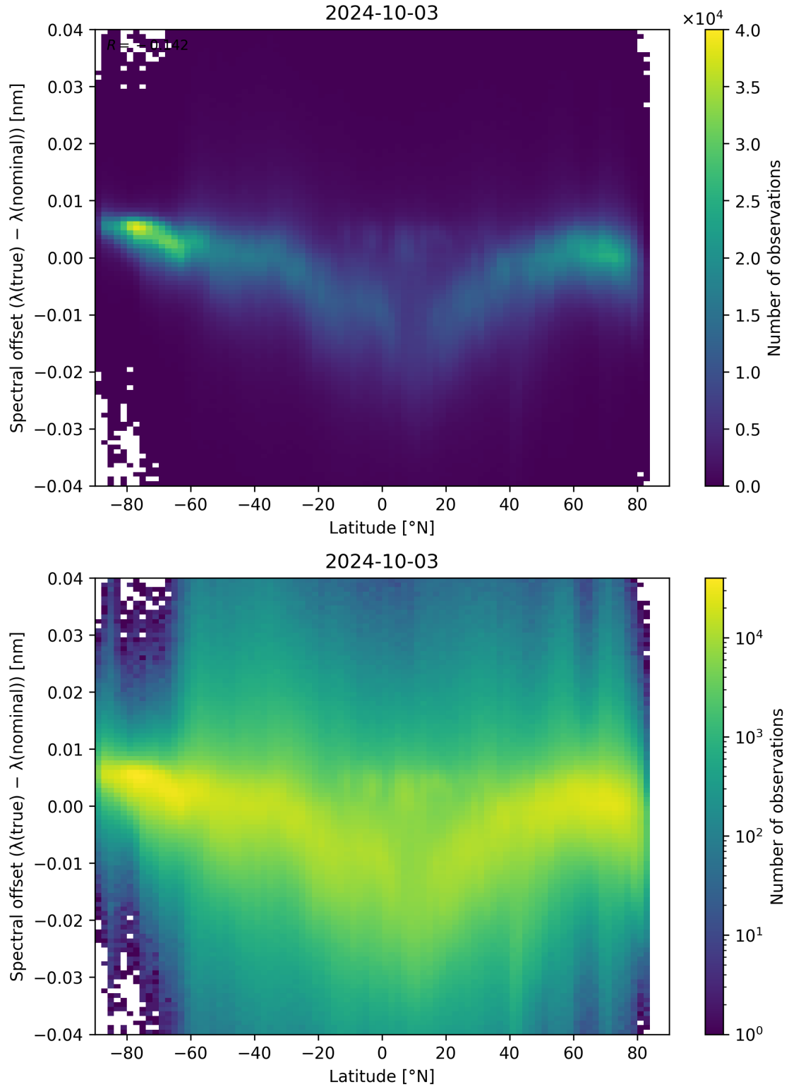
Figure 105: Scatter density plot of “Latitude” against “Spectral offset ( \lambda_{\text{true}} - \lambda_{\text{nominal}} )” for 2024-10-03 to 2024-10-04.
