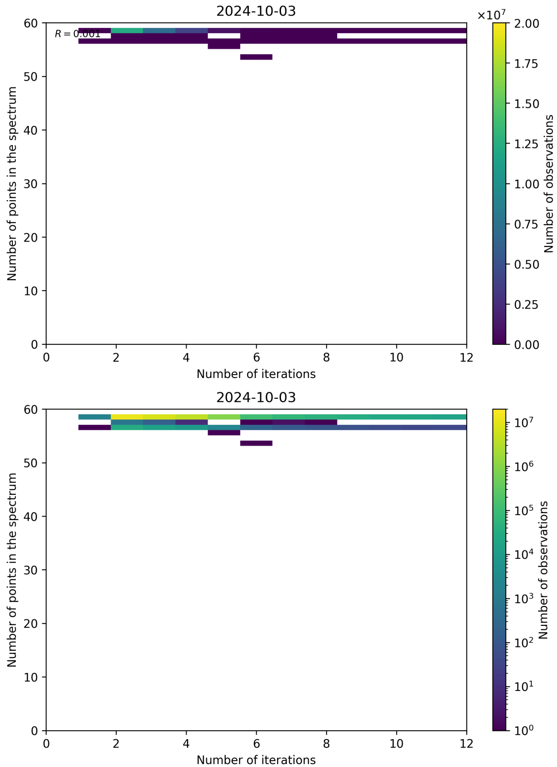
Figure 108: Scatter density plot of “Number of iterations” against “Number of points in the spectrum” for 2024-10-03 to 2024-10-04.
