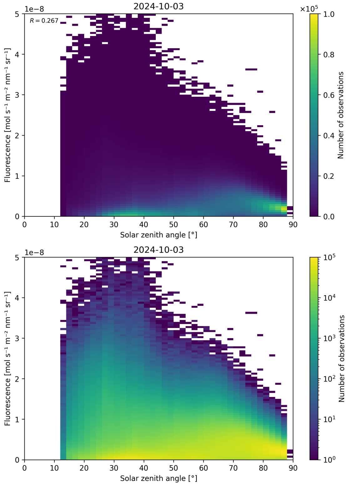
Figure 123: Scatter density plot of “Solar zenith angle” against “Fluorescence” for 2024-10-03 to 2024-10-04.
