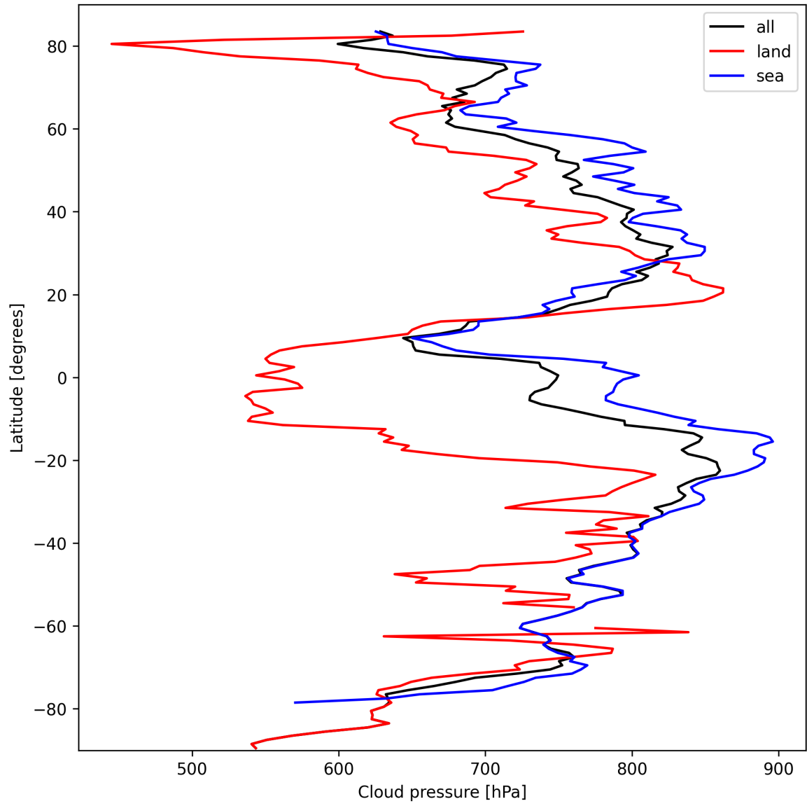
Figure 13: Zonal average of “Cloud pressure” for 2024-10-03 to 2024-10-04.
