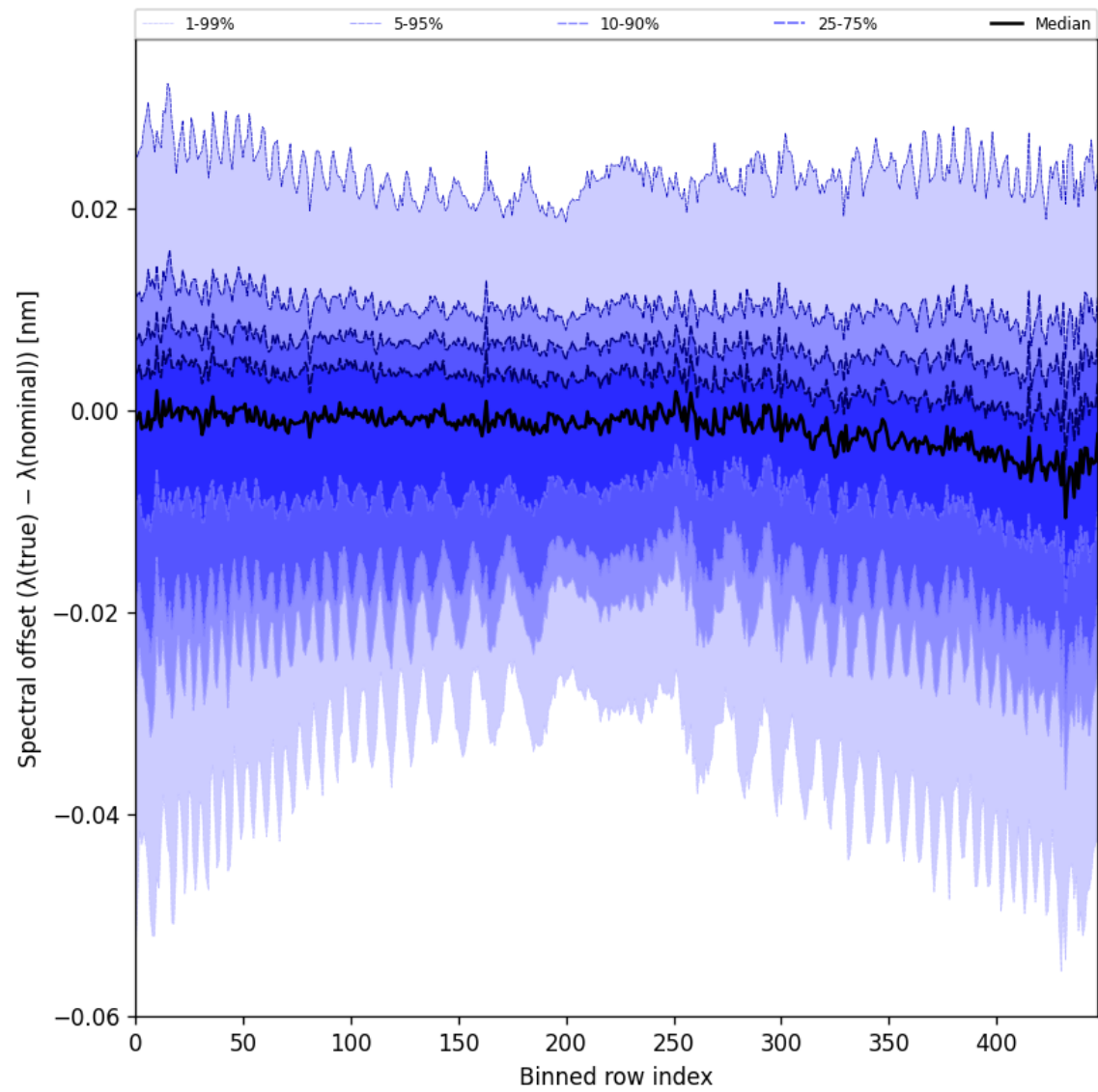
Figure 62: Along track statistics of “Spectral offset ( \lambda_{\text{true}} - \lambda_{\text{nominal}} )” for 2024-10-03 to 2024-10-04
