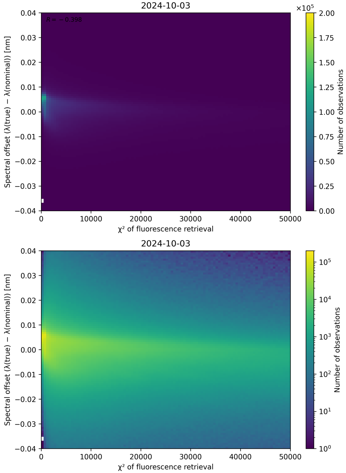
Figure 72: Scatter density plot of “ \chi^2 of fluorescence retrieval” against “Spectral offset ( \lambda_{\text{true}} - \lambda_{\text{nominal}} )” for 2024-10-03 to 2024-10-04.
