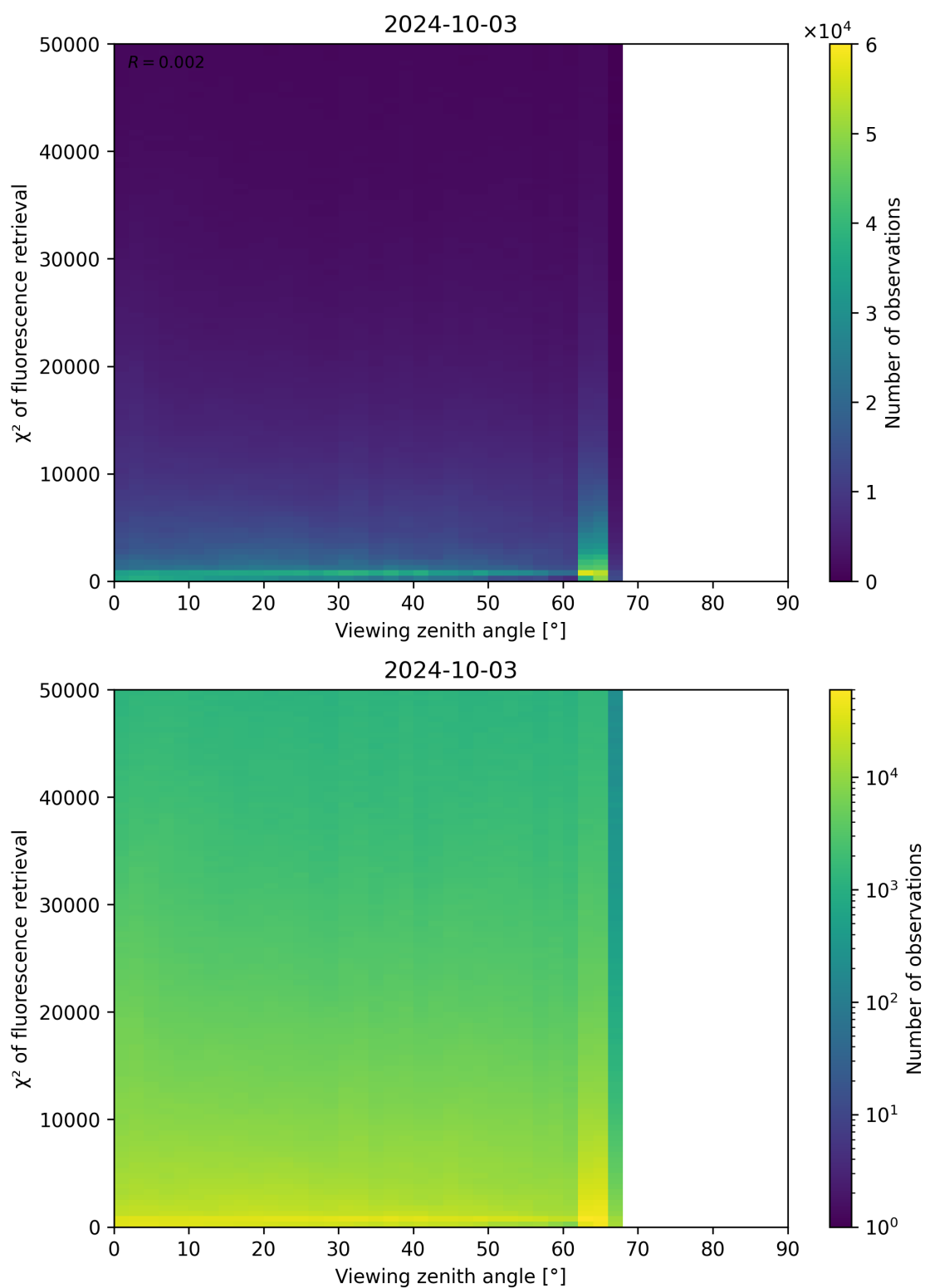
Figure 131: Scatter density plot of “Viewing zenith angle” against “ \chi^2 of fluorescence retrieval” for 2024-10-03 to 2024-10-04.
