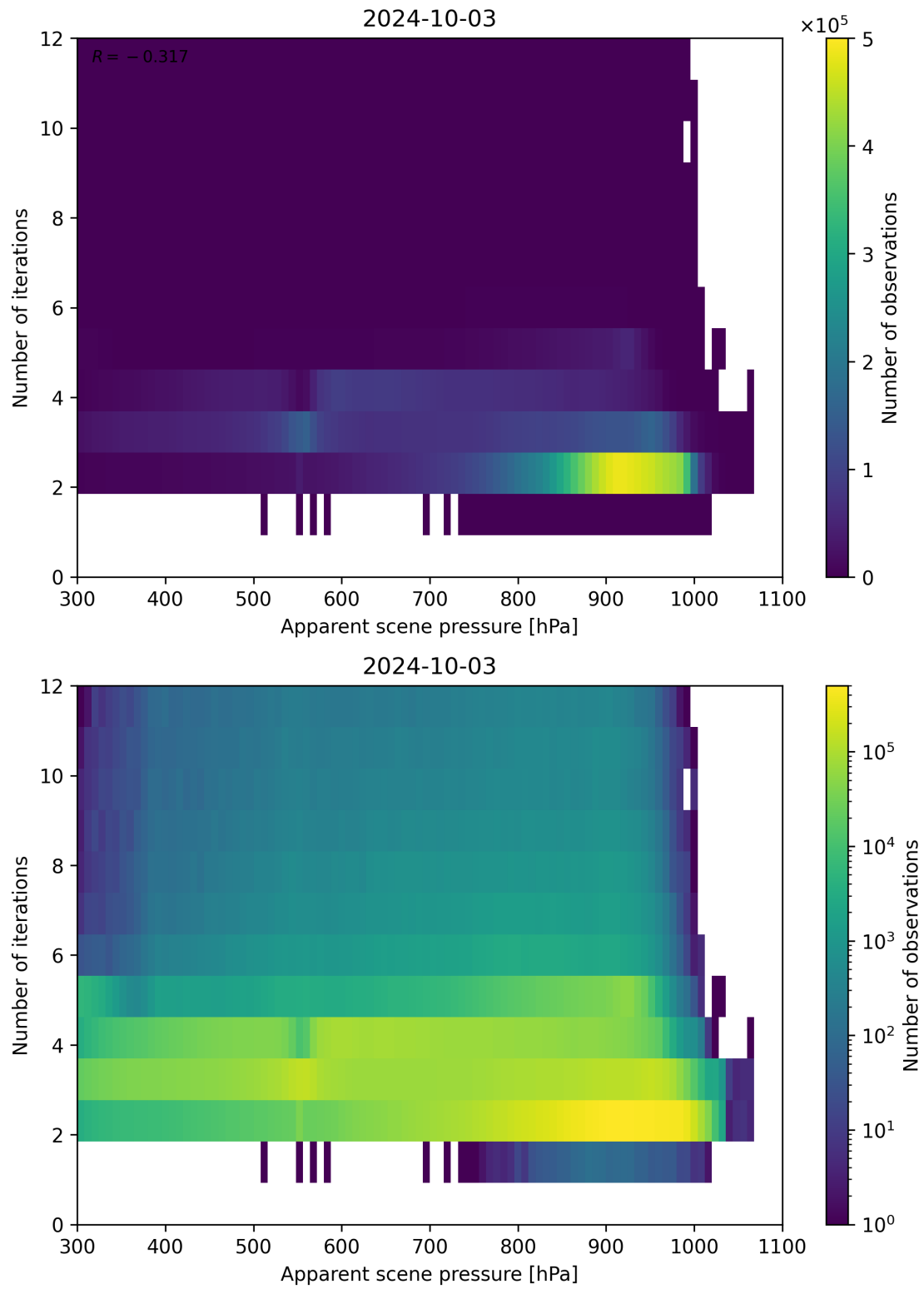
Figure 66: Scatter density plot of “Apparent scene pressure” against “Number of iterations” for 2024-10-03 to 2024-10-04.
