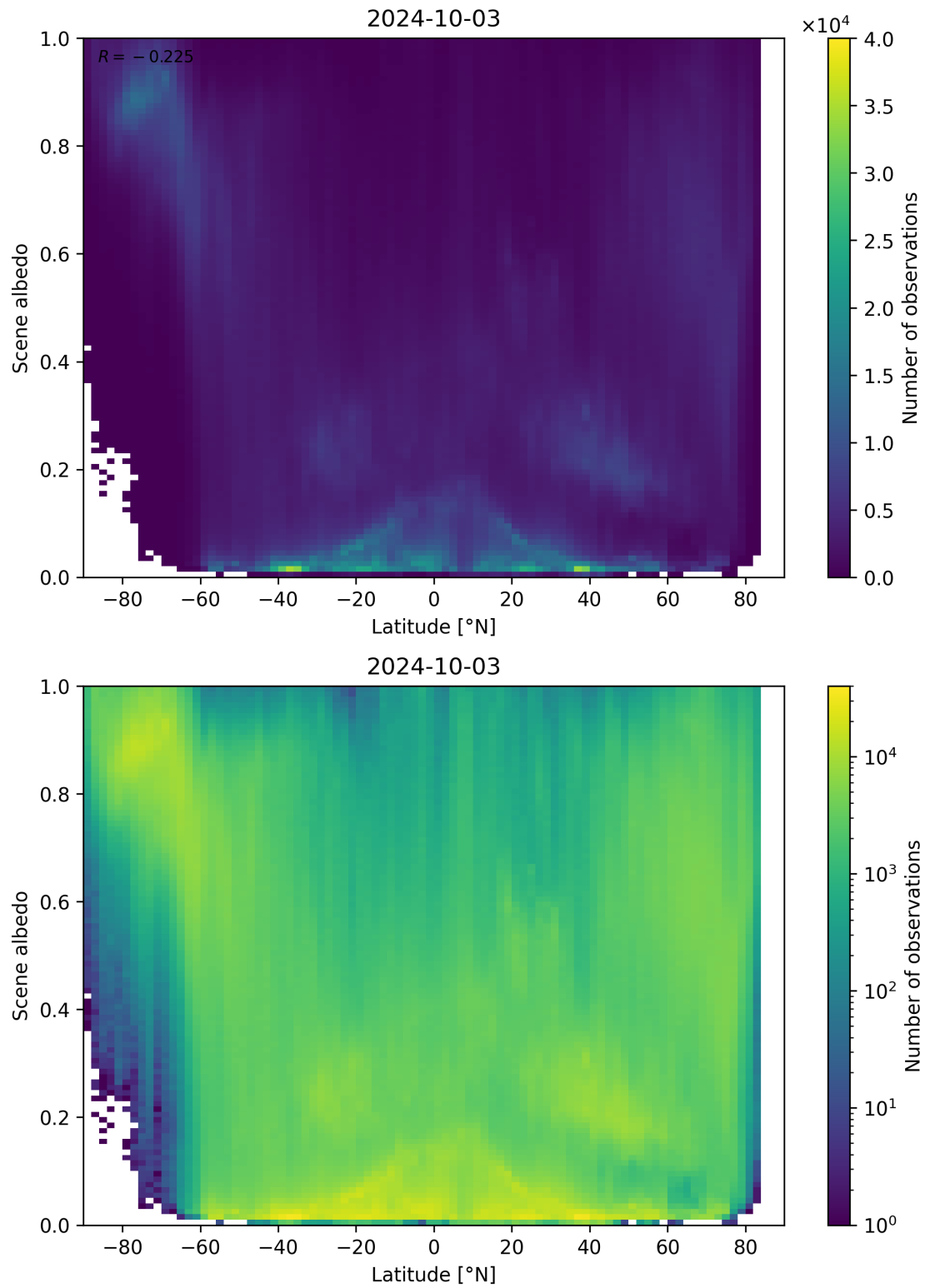
Figure 104: Scatter density plot of “Latitude” against “Scene albedo” for 2024-10-03 to 2024-10-04.
