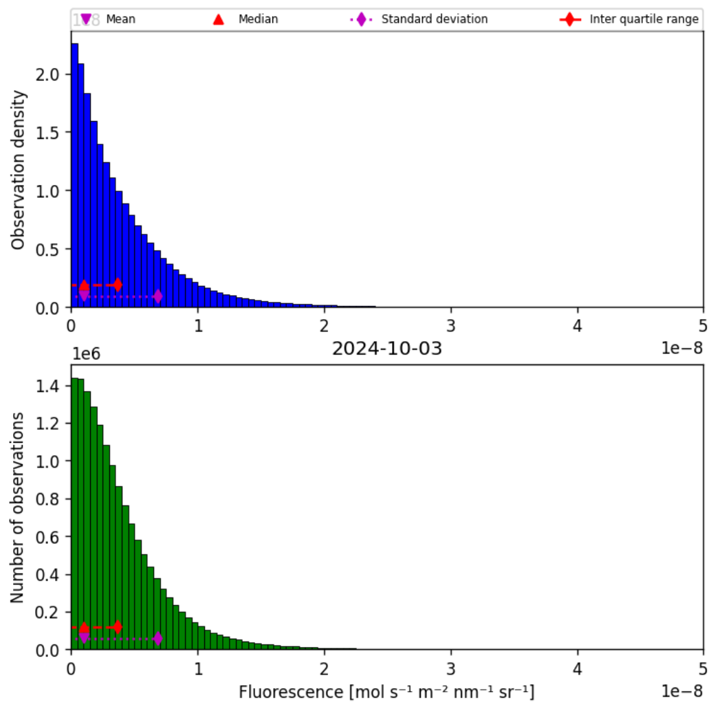
Figure 40: Histogram of “Fluorescence” for 2024-10-03 to 2024-10-04
