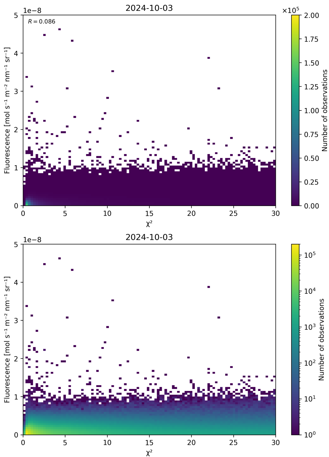
Figure 70: Scatter density plot of “ \chi^2 ” against “Fluorescence” for 2024-10-03 to 2024-10-04.
