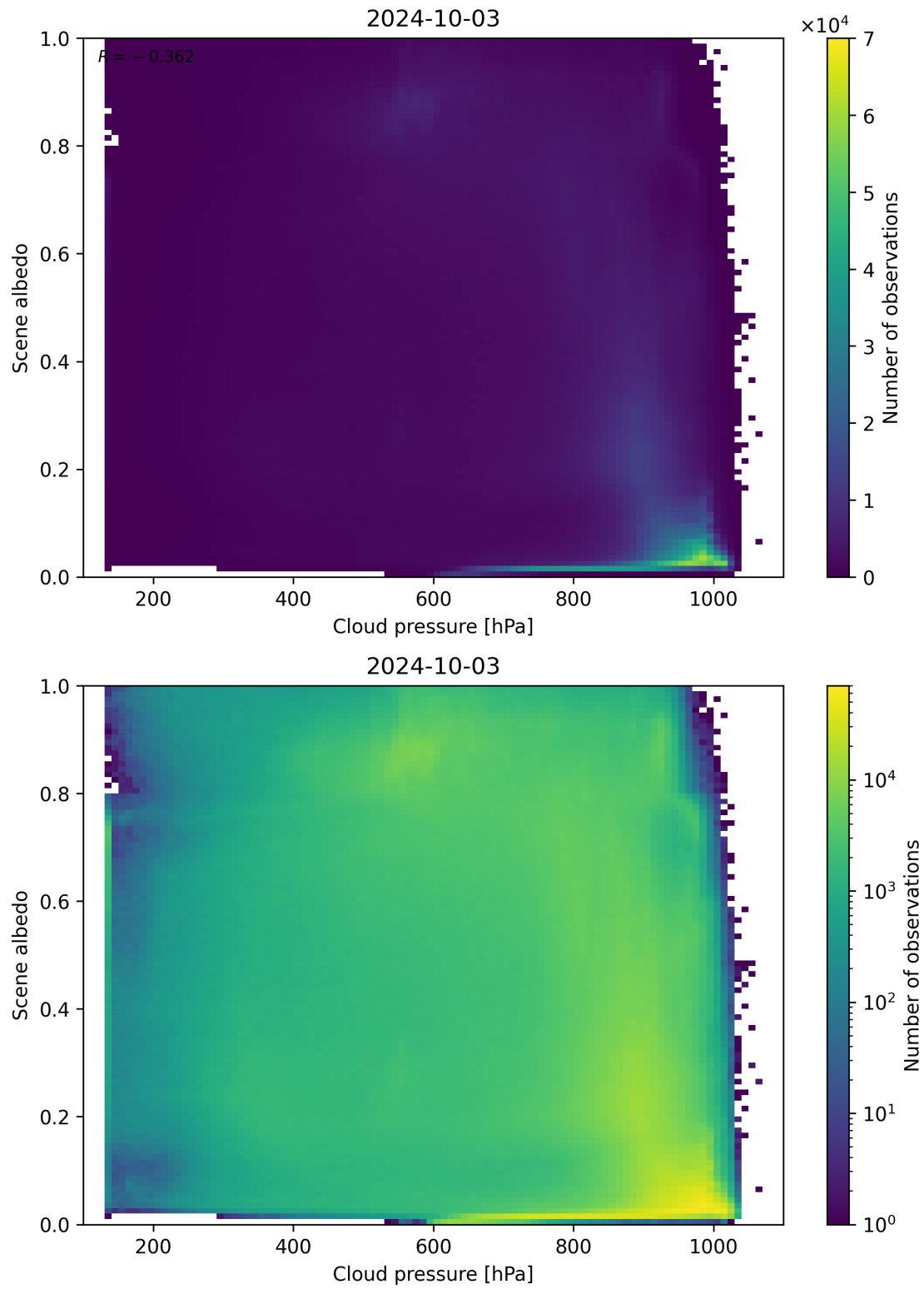
Figure 91: Scatter density plot of “Cloud pressure” against “Scene albedo” for 2024-10-03 to 2024-10-04.
