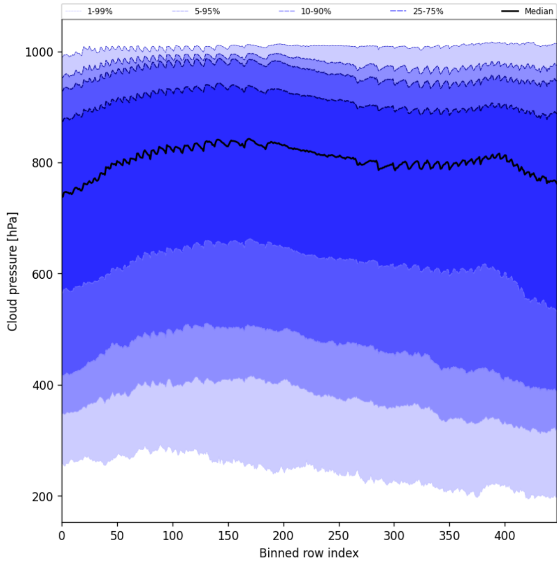
Figure 47: Along track statistics of “Cloud pressure” for 2024-10-03 to 2024-10-04
