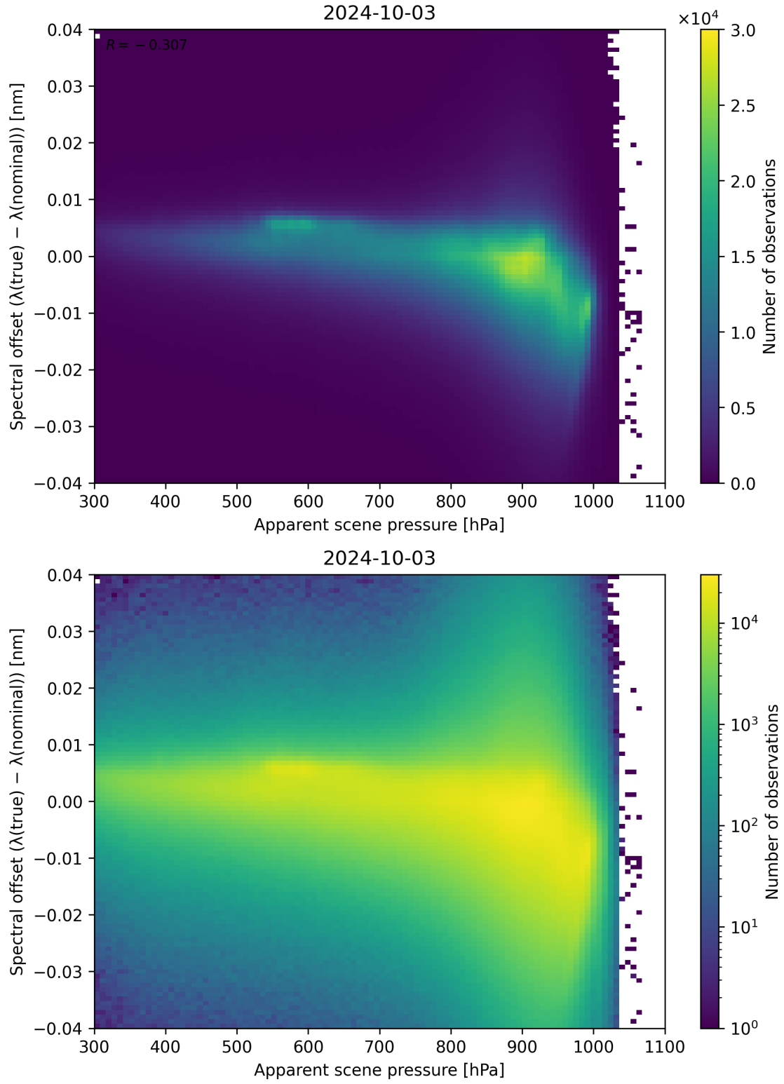
Figure 68: Scatter density plot of “Apparent scene pressure” against “Spectral offset ( \lambda_{\text{true}} - \lambda_{\text{nominal}} )” for 2024-10-03 to 2024-10-04.
