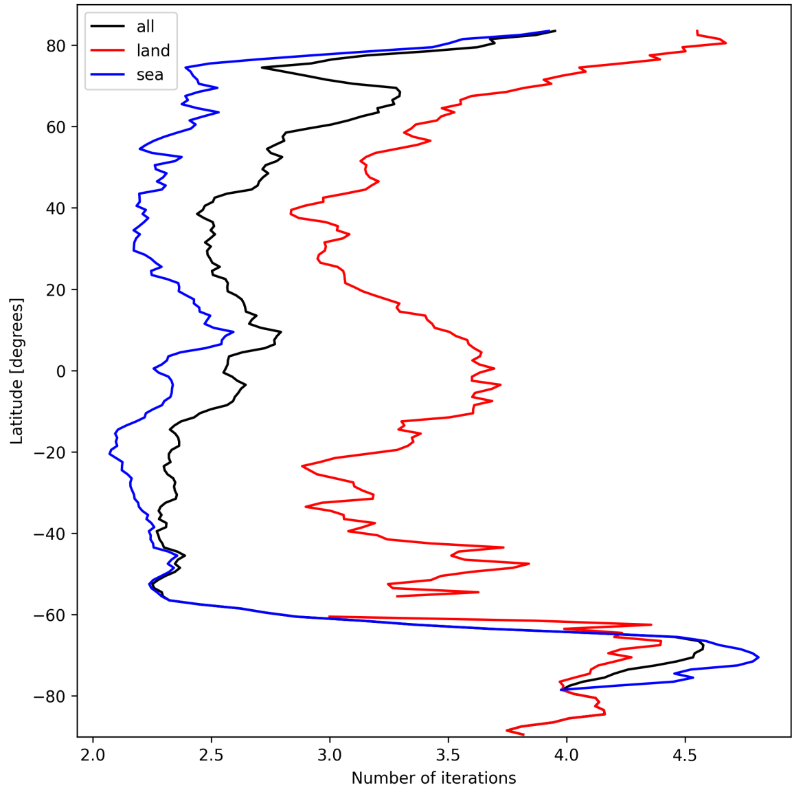
Figure 22: Zonal average of “Number of iterations” for 2024-10-03 to 2024-10-04.
