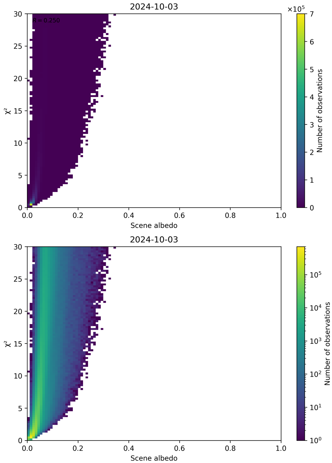
Figure 112: Scatter density plot of “Scene albedo” against “ \chi^2 ” for 2024-10-03 to 2024-10-04.
