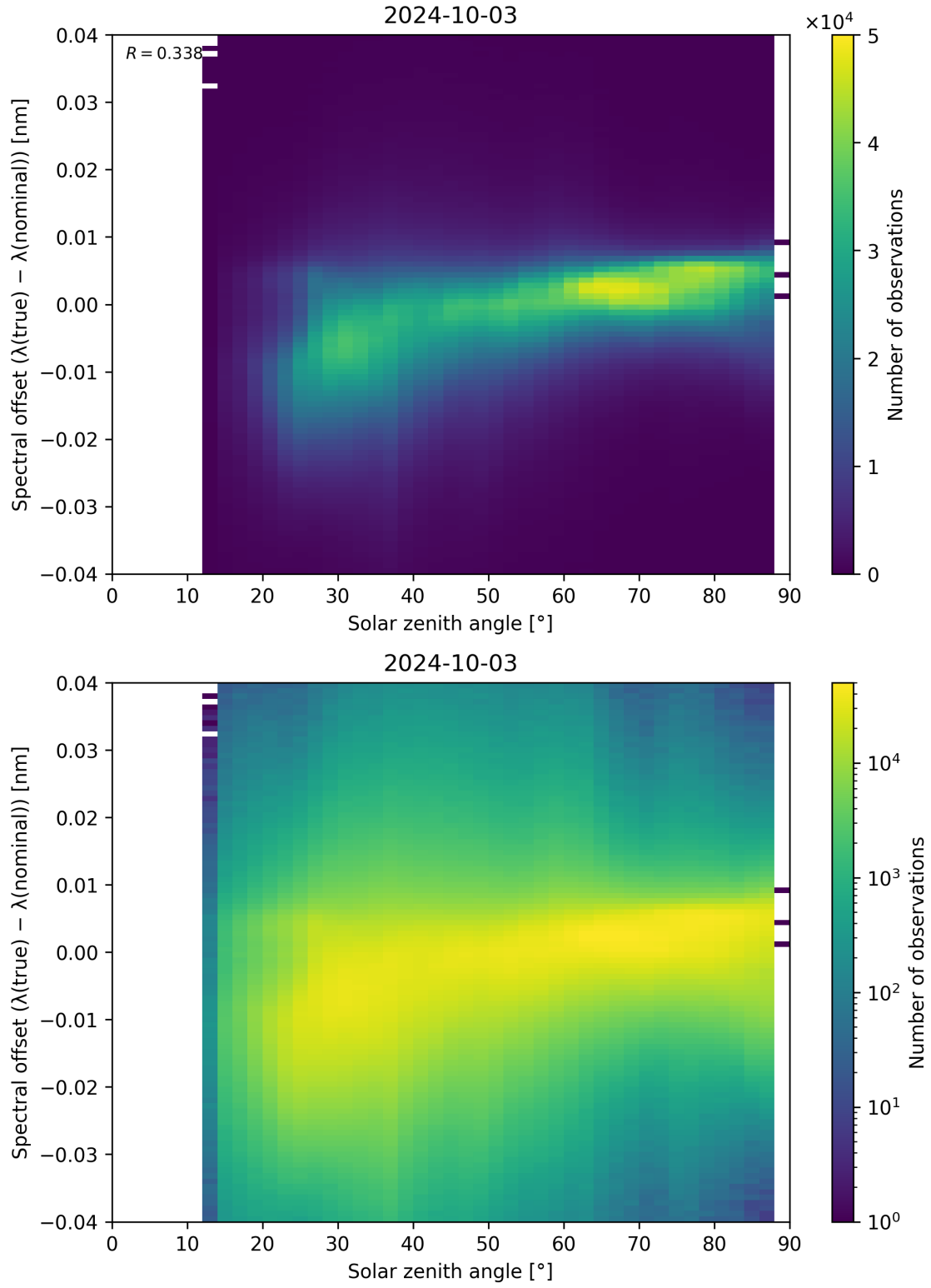
Figure 128: Scatter density plot of “Solar zenith angle” against “Spectral offset ( \lambda_{\text{true}} - \lambda_{\text{nominal}} )” for 2024-10-03 to 2024-10-04.
