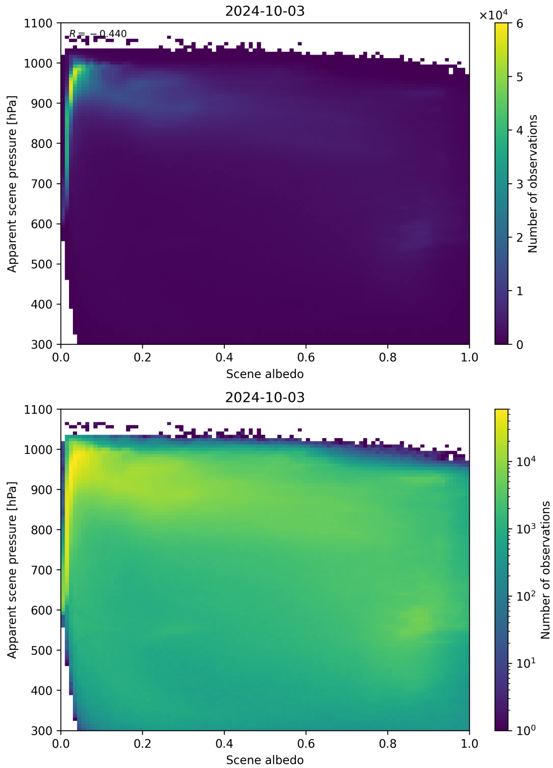
Figure 111: Scatter density plot of “Scene albedo” against “Apparent scene pressure” for 2024-10-03 to 2024-10-04.
