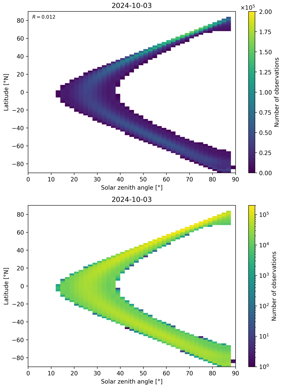
Figure 124: Scatter density plot of “Solar zenith angle” against “Latitude” for 2024-10-03 to 2024-10-04.
