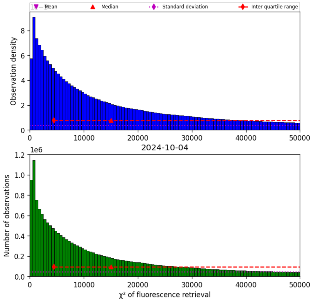
Figure 42: Histogram of “ \chi^2 of fluorescence retrieval” for 2024-10-03 to 2024-10-05
