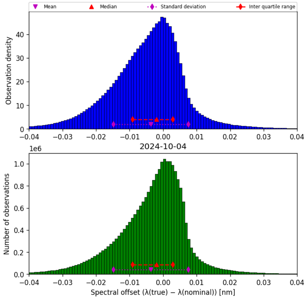
Figure 45: Histogram of “Spectral offset ( \lambda_{\text{true}} - \lambda_{\text{nominal}} )” for 2024-10-03 to 2024-10-05
