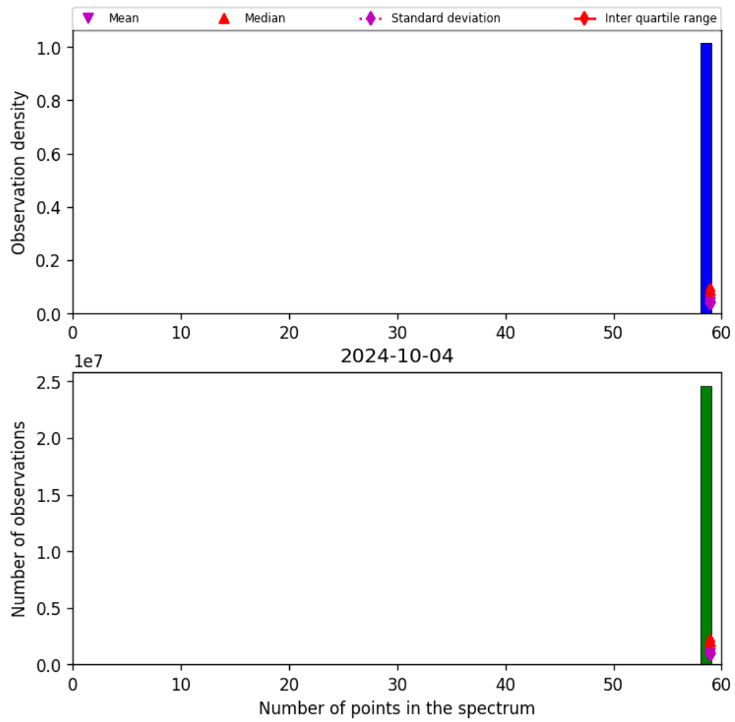
Figure 44: Histogram of “Number of points in the spectrum” for 2024-10-03 to 2024-10-05
