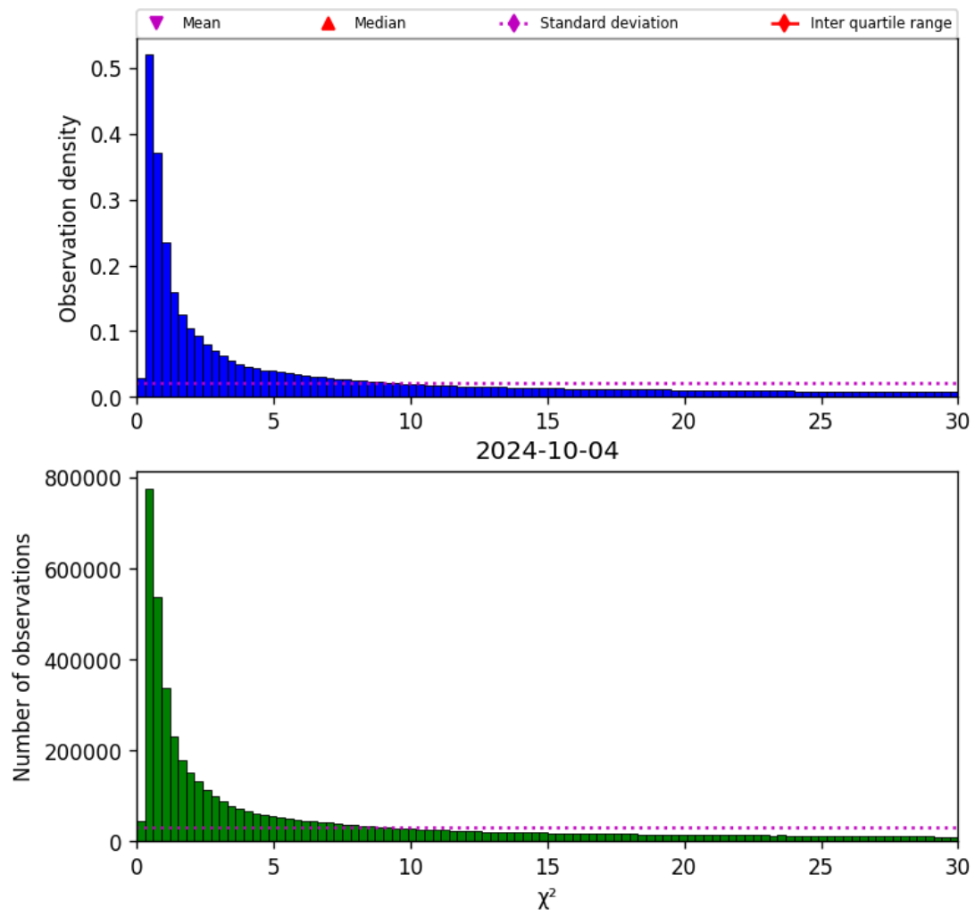
Figure 38: Histogram of " \chi^2 " for 2024-10-03 to 2024-10-05
