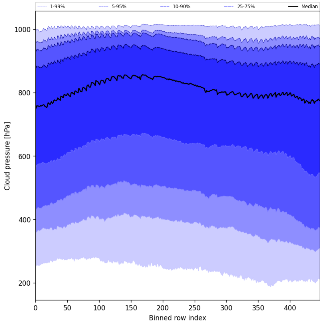
Figure 47: Along track statistics of “Cloud pressure” for 2024-10-03 to 2024-10-05
