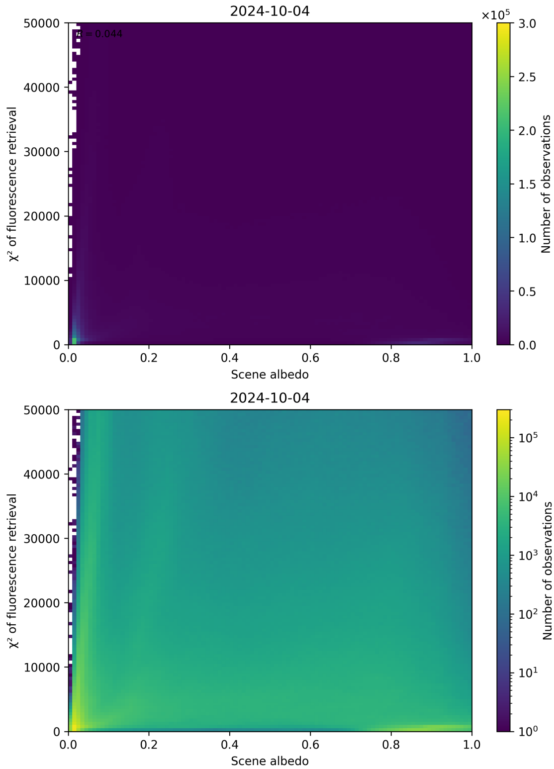
Figure 113: Scatter density plot of “Scene albedo” against “ \chi^2 of fluorescence retrieval” for 2024-10-03 to 2024-10-05.
