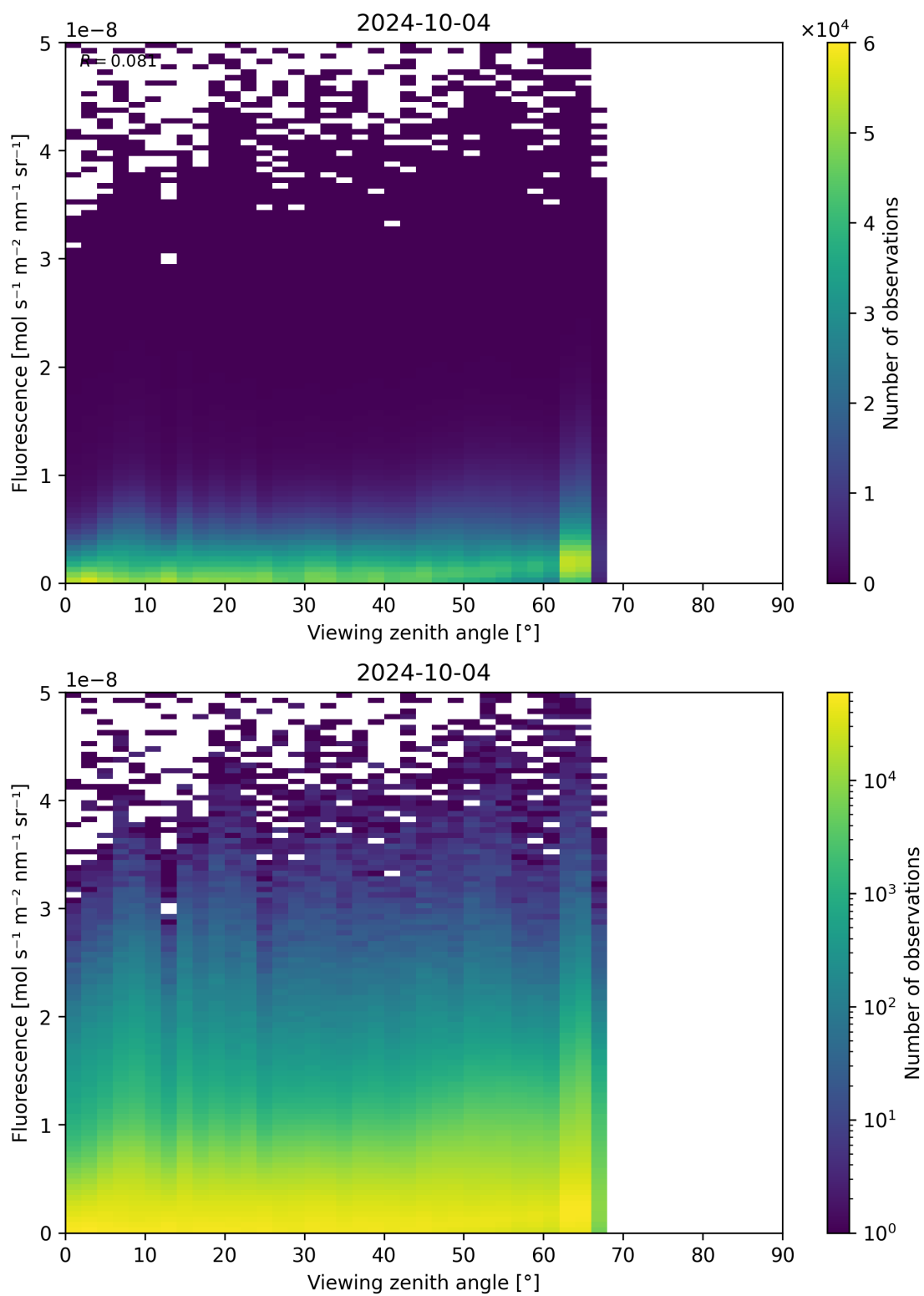
Figure 134: Scatter density plot of “Viewing zenith angle” against “Fluorescence” for 2024-10-03 to 2024-10-05.
