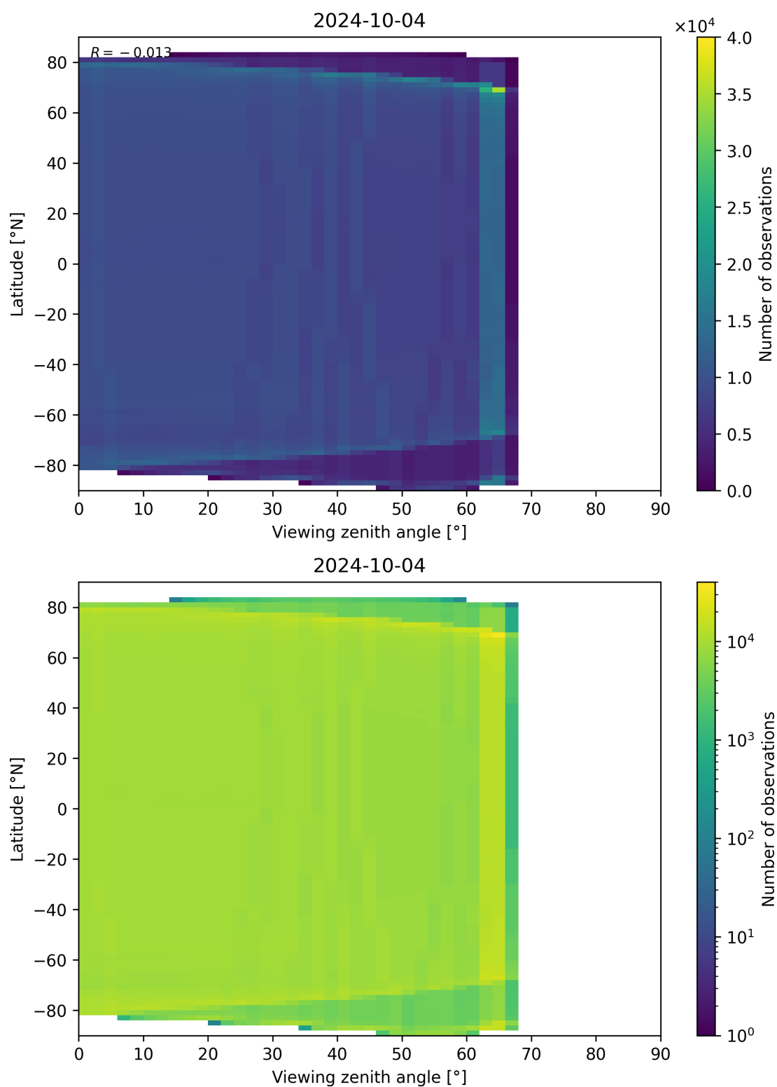
Figure 135: Scatter density plot of “Viewing zenith angle” against “Latitude” for 2024-10-03 to 2024-10-05.
