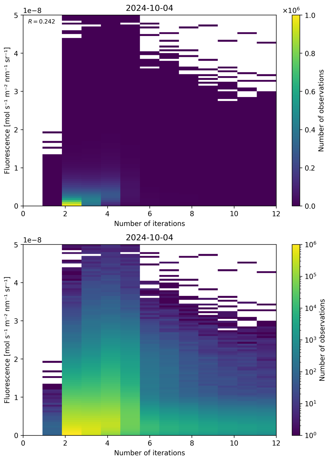
Figure 107: Scatter density plot of “Number of iterations” against “Fluorescence” for 2024-10-03 to 2024-10-05.
