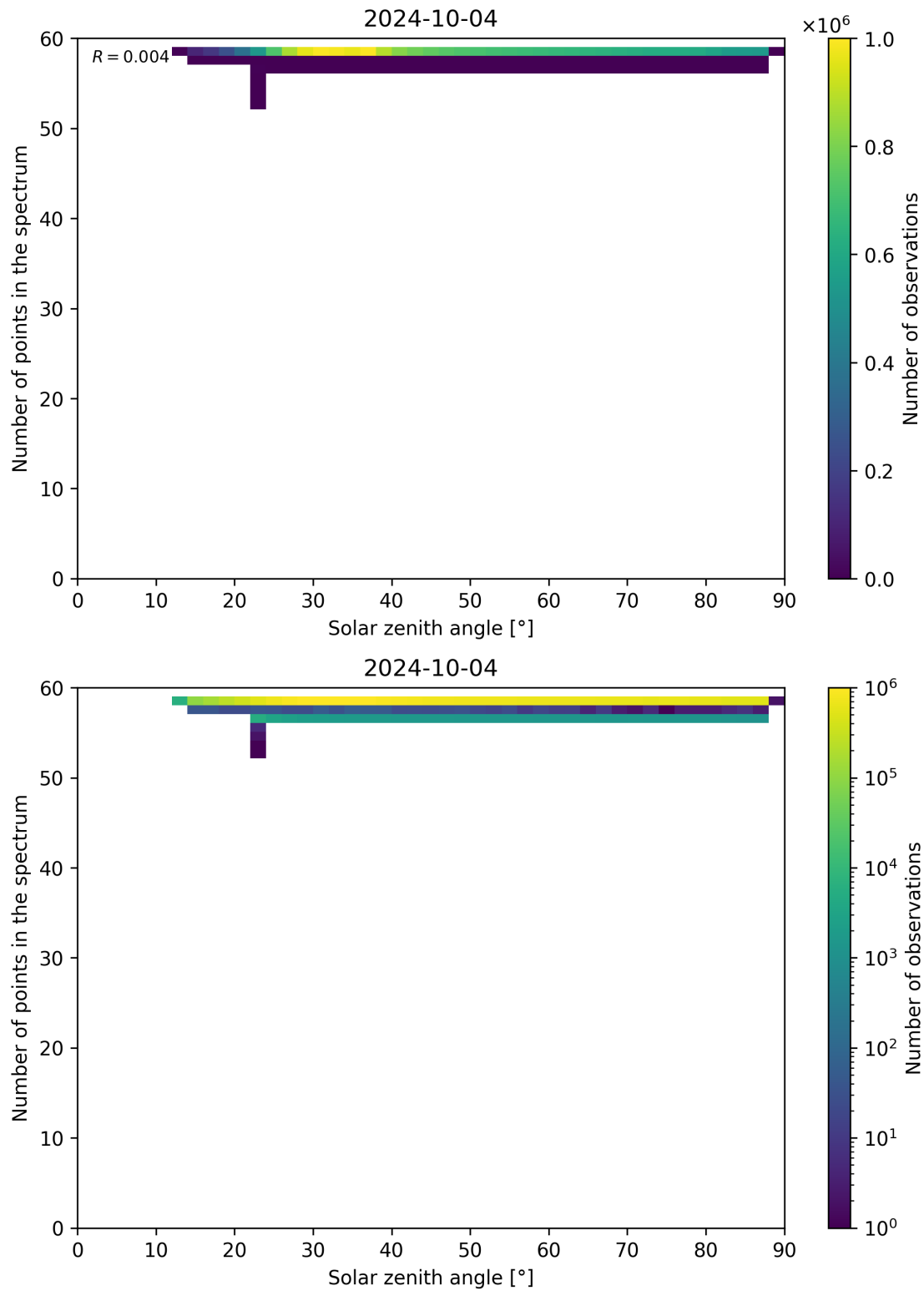
Figure 126: Scatter density plot of “Solar zenith angle” against “Number of points in the spectrum” for 2024-10-03 to 2024-10-05.
