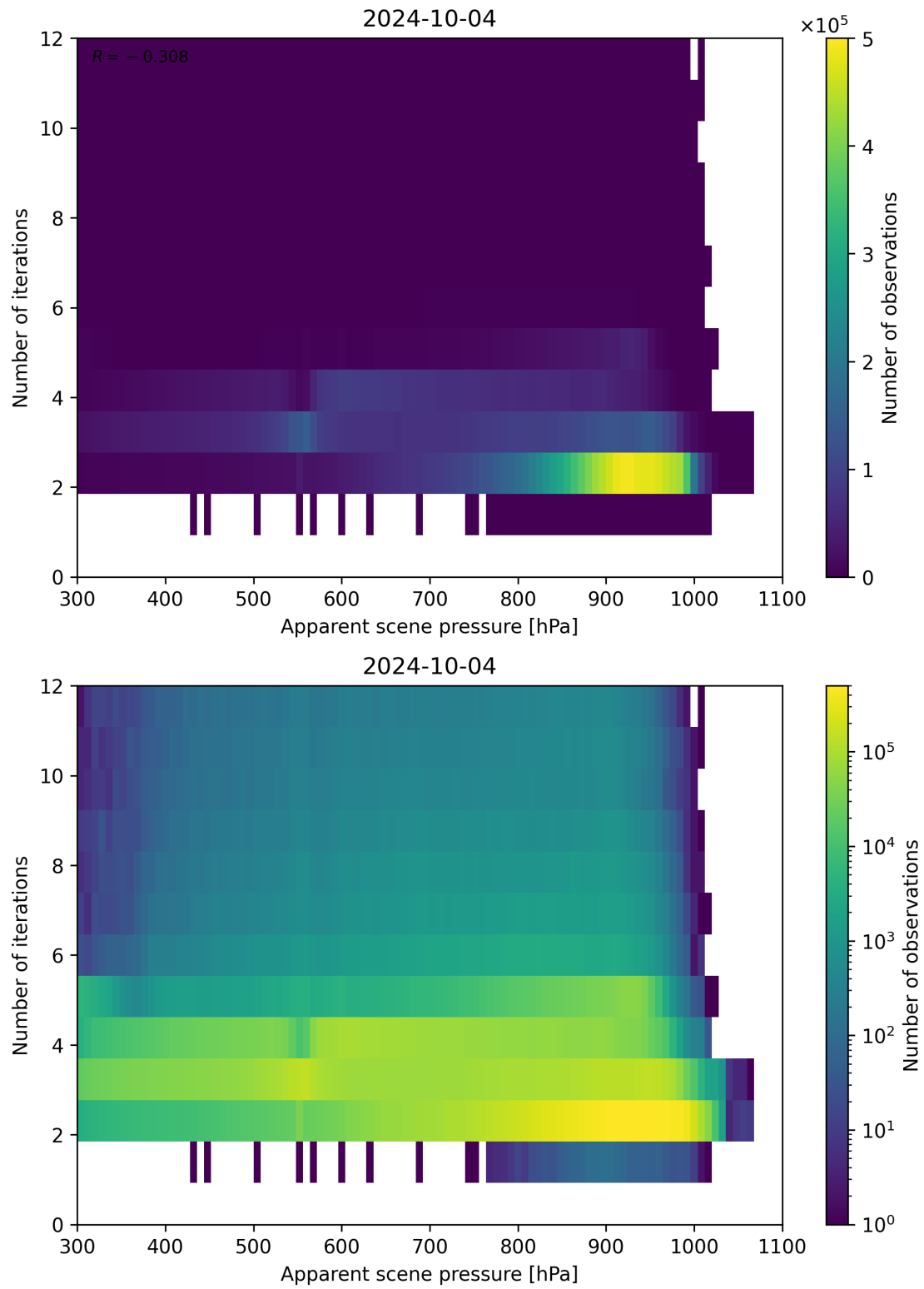
Figure 66: Scatter density plot of “Apparent scene pressure” against “Number of iterations” for 2024-10-03 to 2024-10-05.
