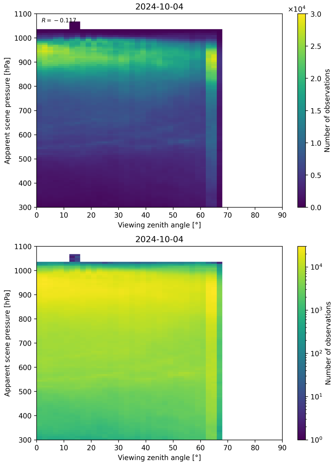
Figure 129: Scatter density plot of “Viewing zenith angle” against “Apparent scene pressure” for 2024-10-03 to 2024-10-05.
