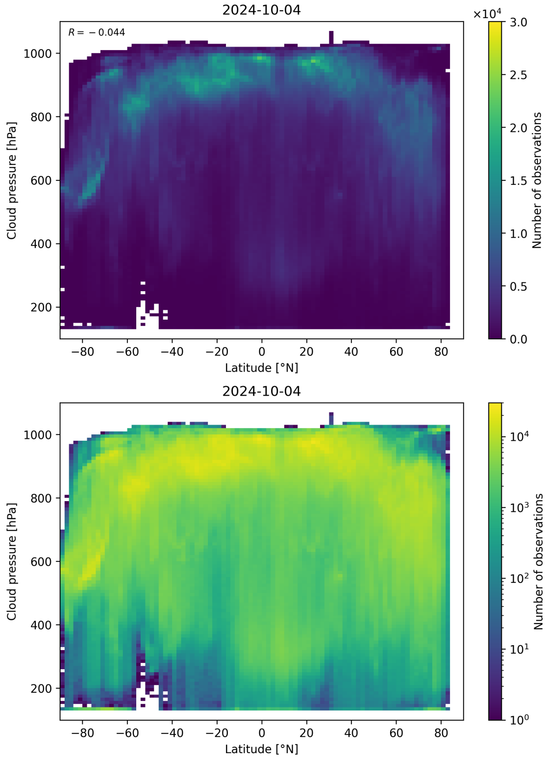
Figure 100: Scatter density plot of “Latitude” against “Cloud pressure” for 2024-10-03 to 2024-10-05.
