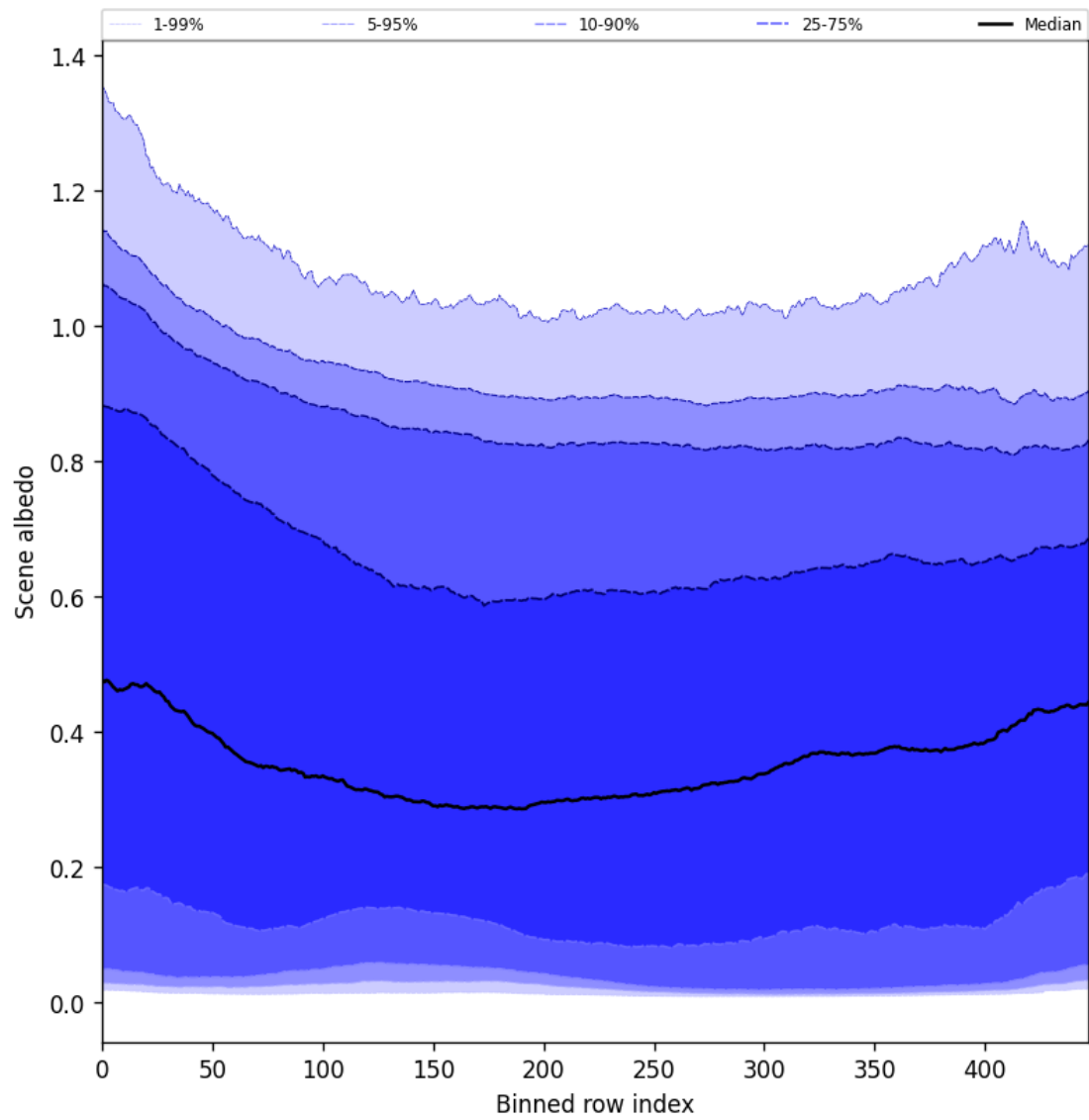
Figure 51: Along track statistics of “Scene albedo” for 2024-10-03 to 2024-10-05
