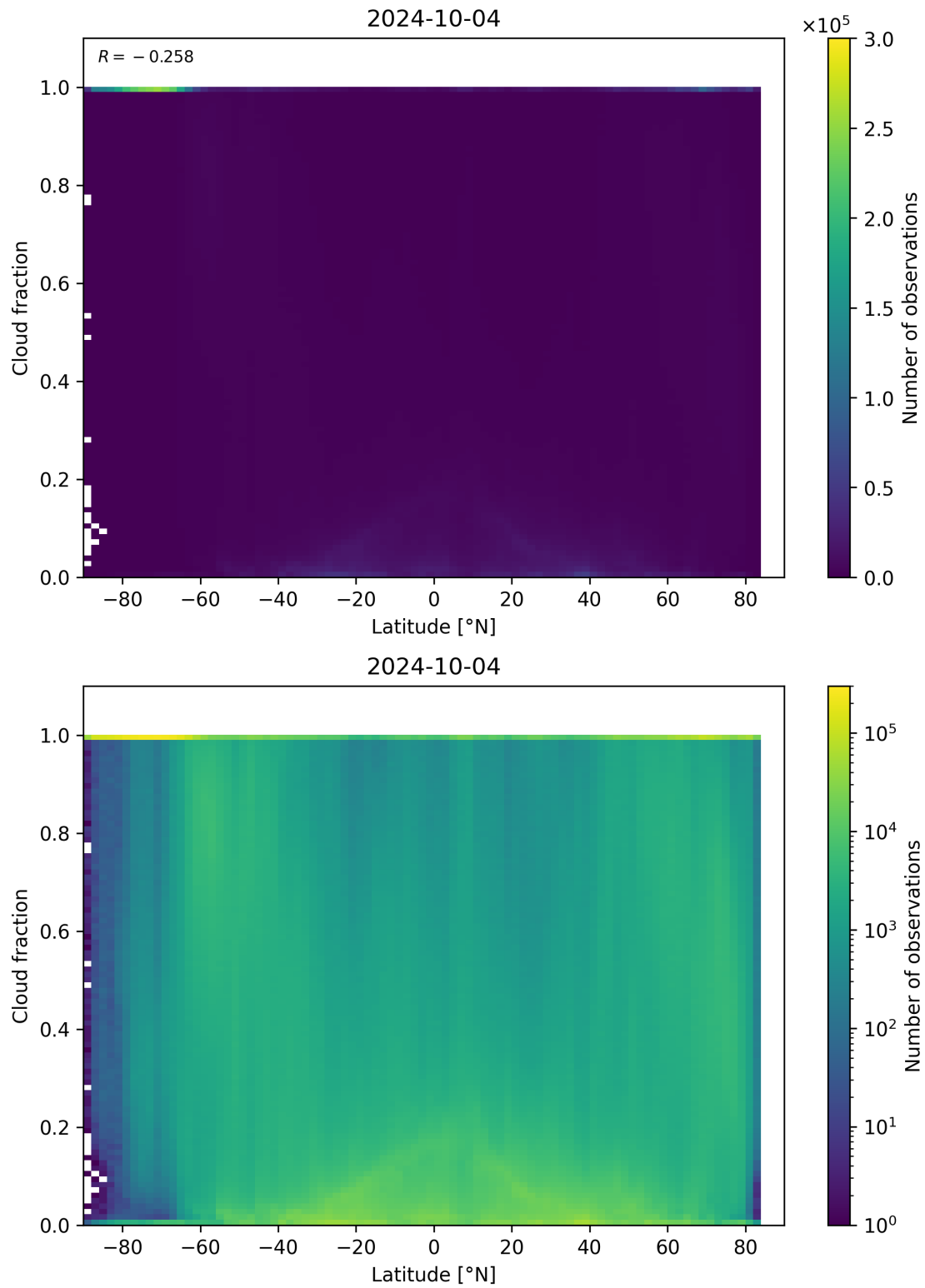
Figure 99: Scatter density plot of “Latitude” against “Cloud fraction” for 2024-10-03 to 2024-10-05.
