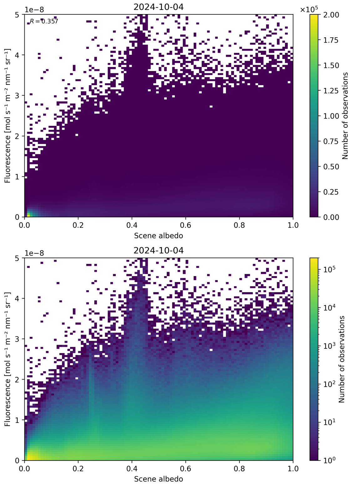
Figure 114: Scatter density plot of “Scene albedo” against “Fluorescence” for 2024-10-03 to 2024-10-05.
