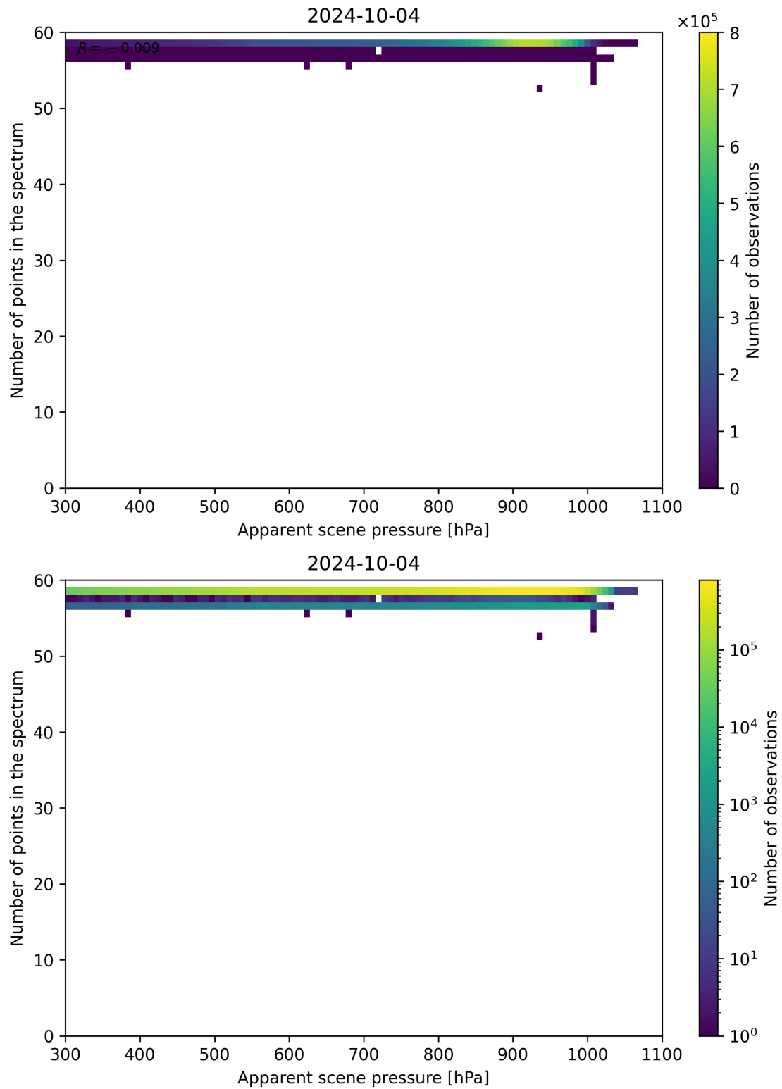
Figure 67: Scatter density plot of “Apparent scene pressure” against “Number of points in the spectrum” for 2024-10-03 to 2024-10-05.
