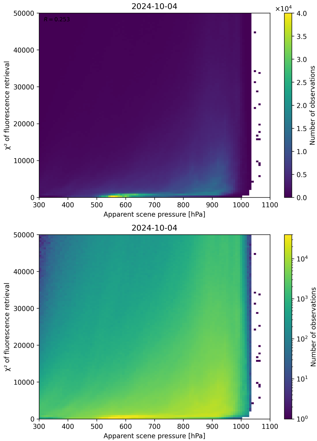
Figure 64: Scatter density plot of “Apparent scene pressure” against “ \chi^2 of fluorescence retrieval” for 2024-10-03 to 2024-10-05.
