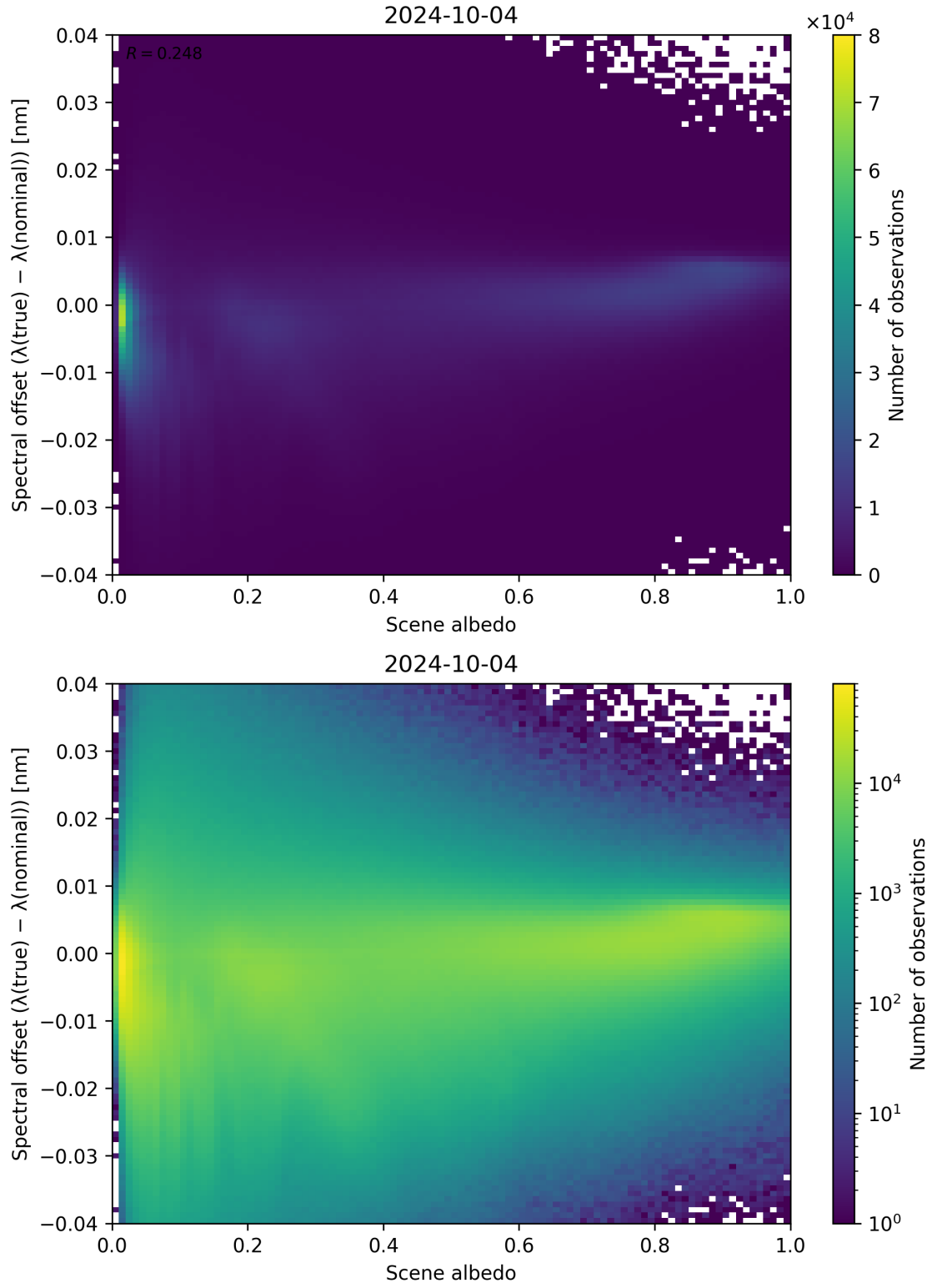
Figure 117: Scatter density plot of “Scene albedo” against “Spectral offset ( \lambda_{\text{true}} - \lambda_{\text{nominal}} )” for 2024-10-03 to 2024-10-05.
