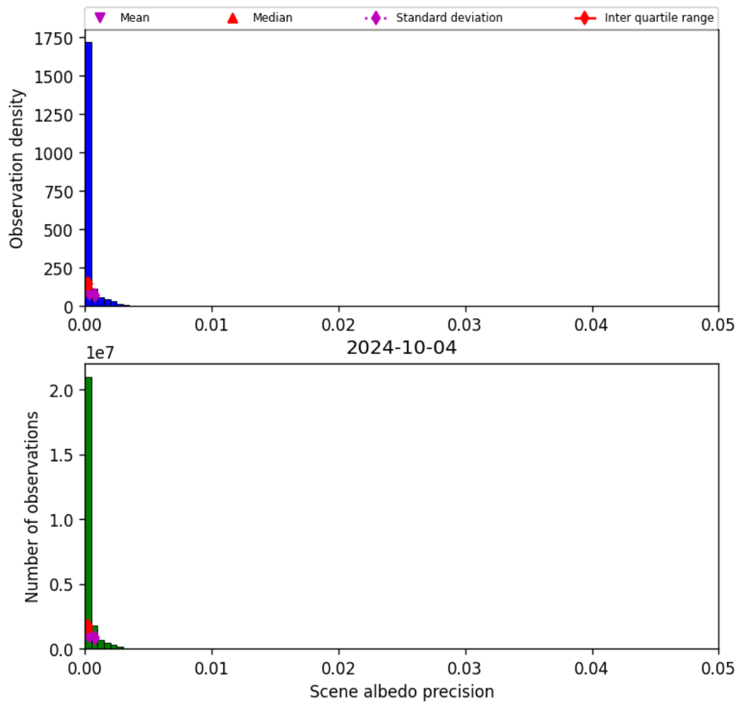
Figure 35: Histogram of “Scene albedo precision” for 2024-10-03 to 2024-10-05
