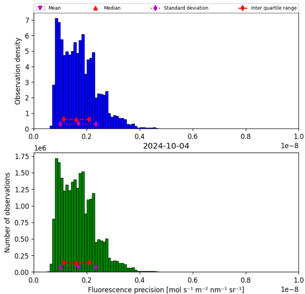
Figure 41: Histogram of “Fluorescence precision” for 2024-10-03 to 2024-10-05
