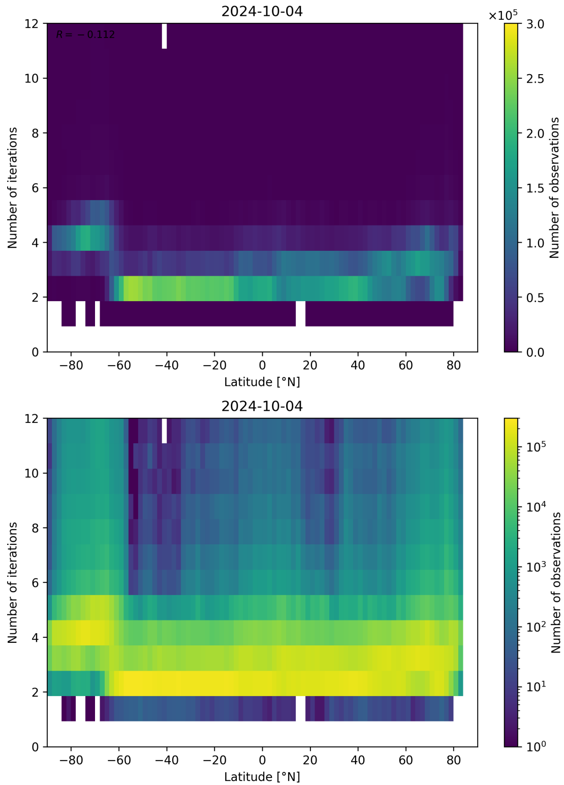
Figure 102: Scatter density plot of “Latitude” against “Number of iterations” for 2024-10-03 to 2024-10-05.
