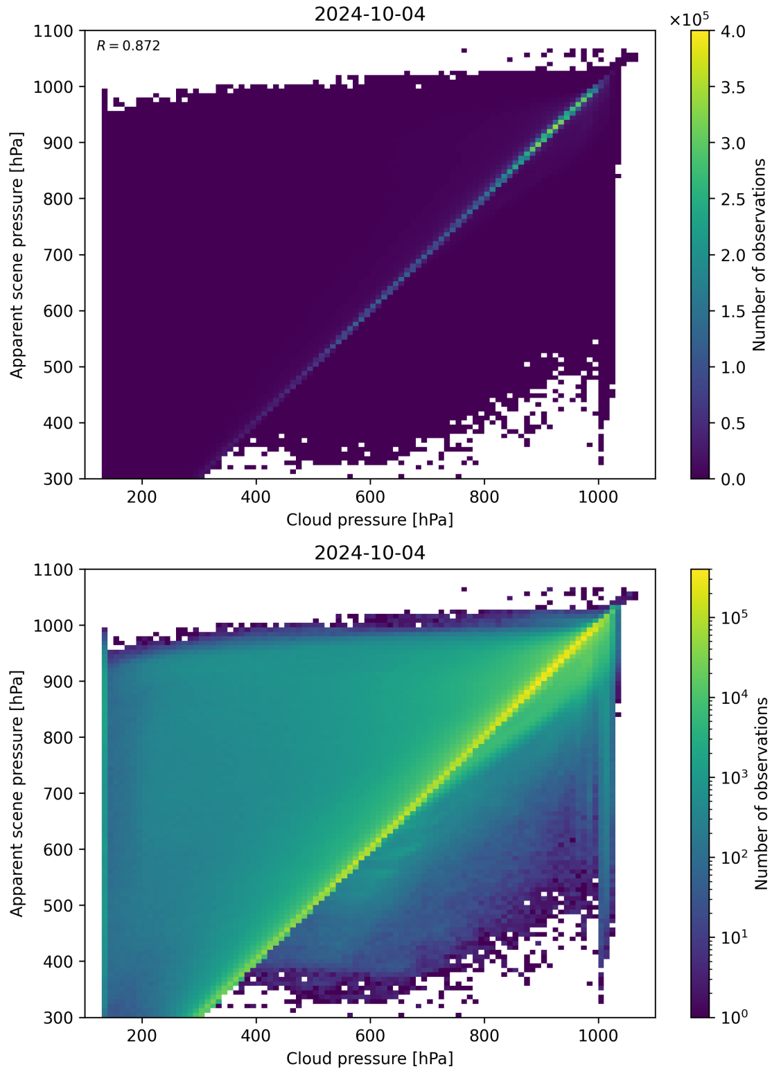
Figure 84: Scatter density plot of “Cloud pressure” against “Apparent scene pressure” for 2024-10-03 to 2024-10-05.
