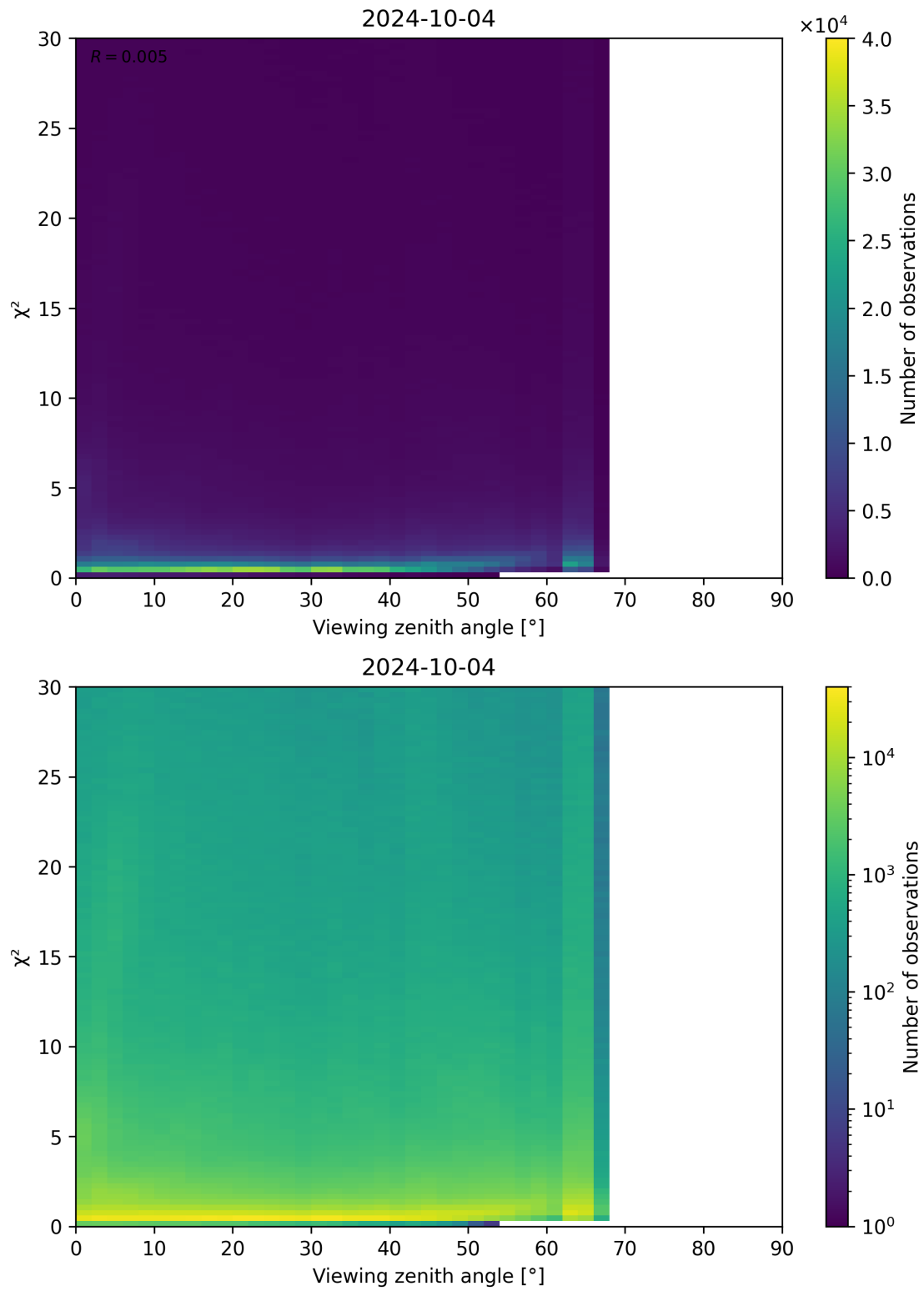
Figure 130: Scatter density plot of “Viewing zenith angle” against “ \chi^2 ” for 2024-10-03 to 2024-10-05.
