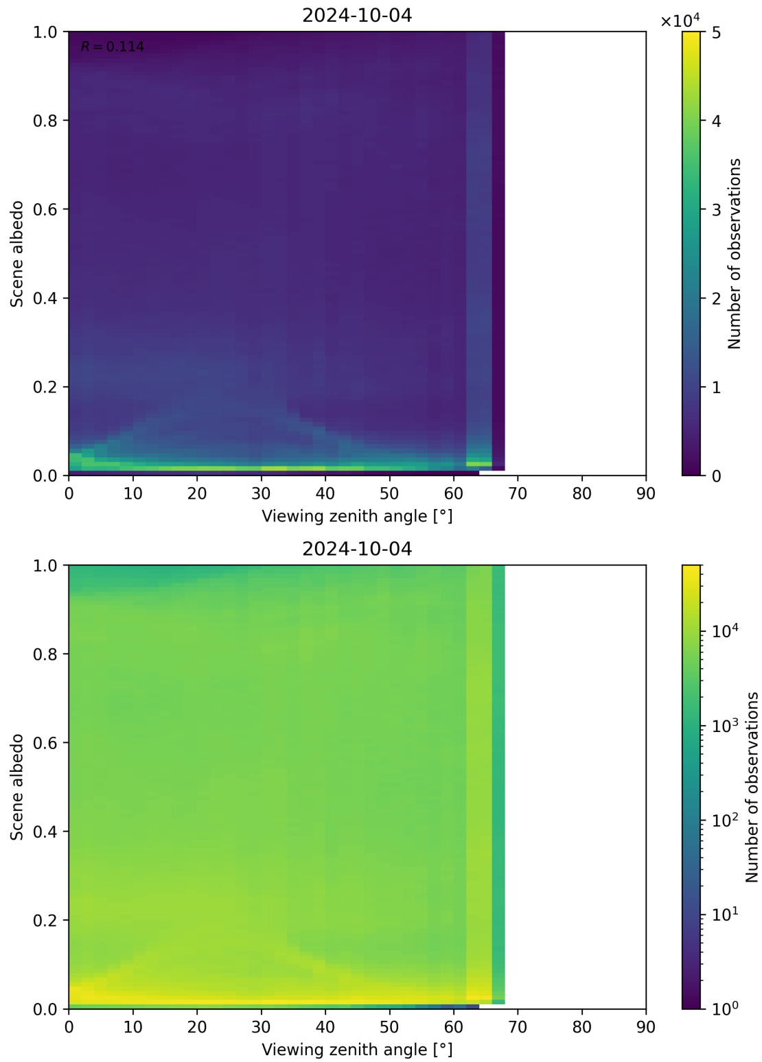
Figure 138: Scatter density plot of “Viewing zenith angle” against “Scene albedo” for 2024-10-03 to 2024-10-05.
