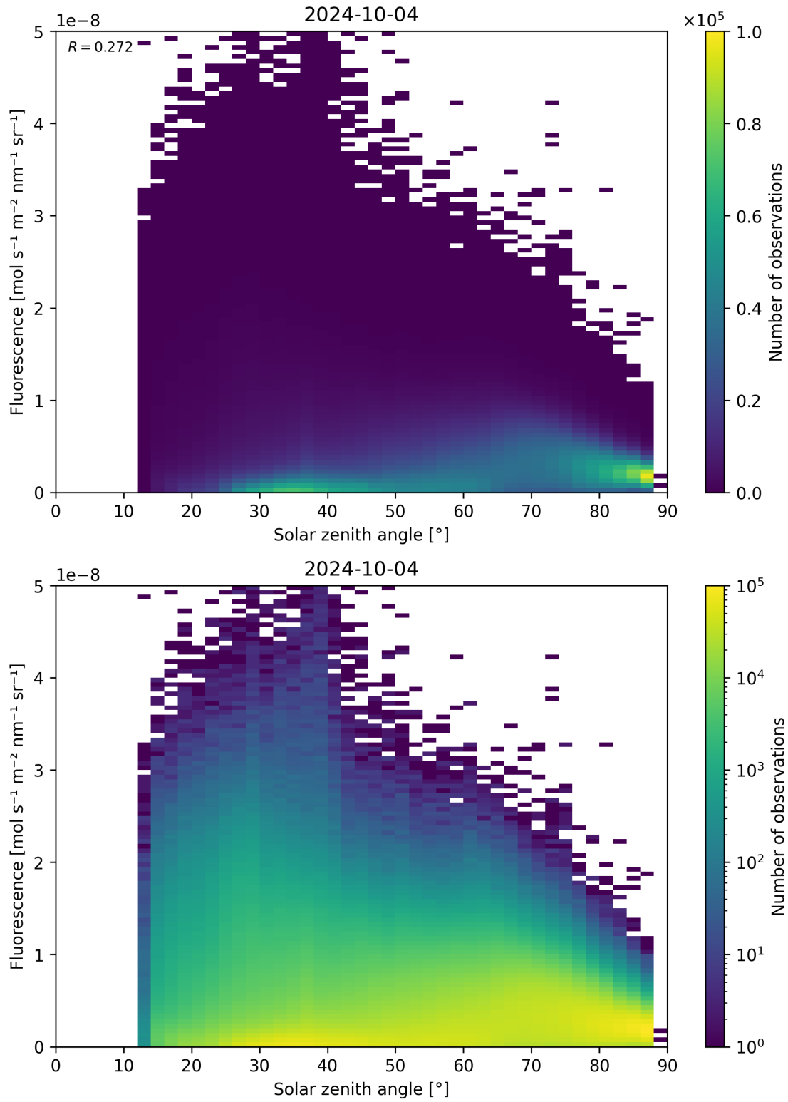
Figure 123: Scatter density plot of “Solar zenith angle” against “Fluorescence” for 2024-10-03 to 2024-10-05.
