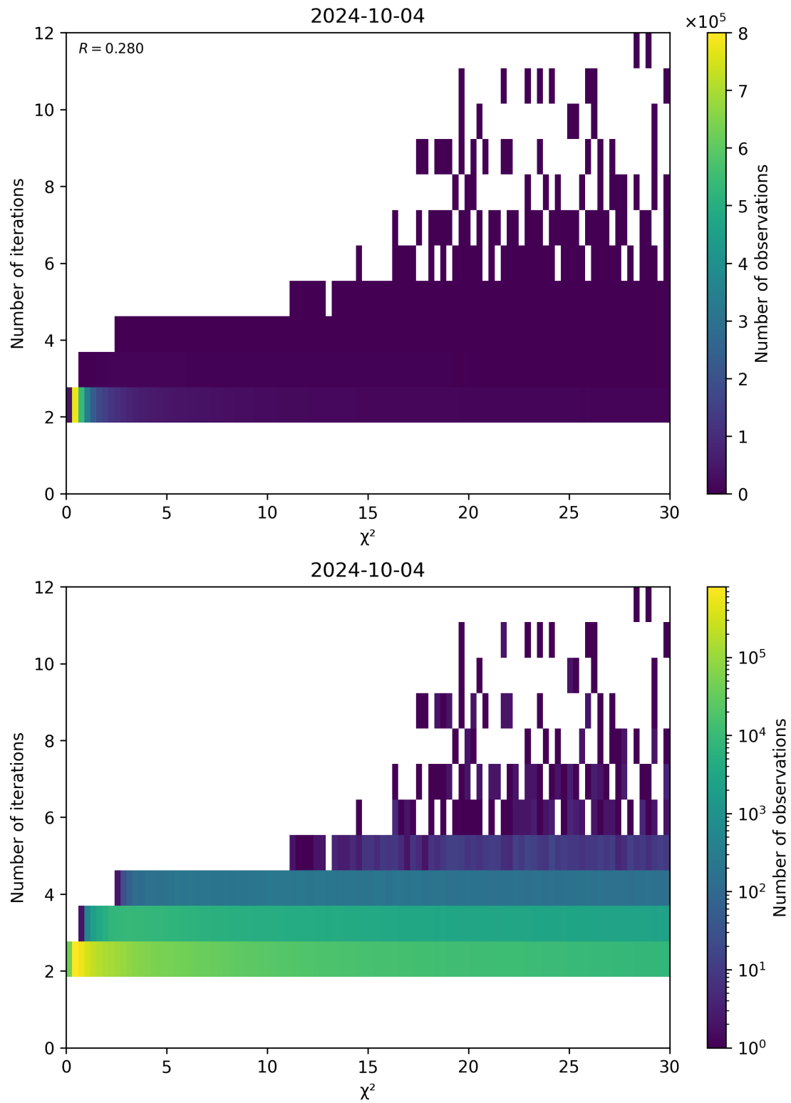
Figure 73: Scatter density plot of “ \chi^2 ” against “Number of iterations” for 2024-10-03 to 2024-10-05.
