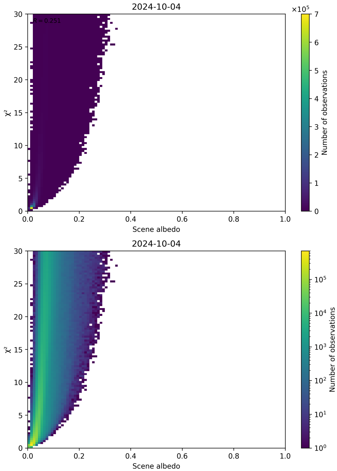
Figure 112: Scatter density plot of “Scene albedo” against “ \chi^2 ” for 2024-10-03 to 2024-10-05.
