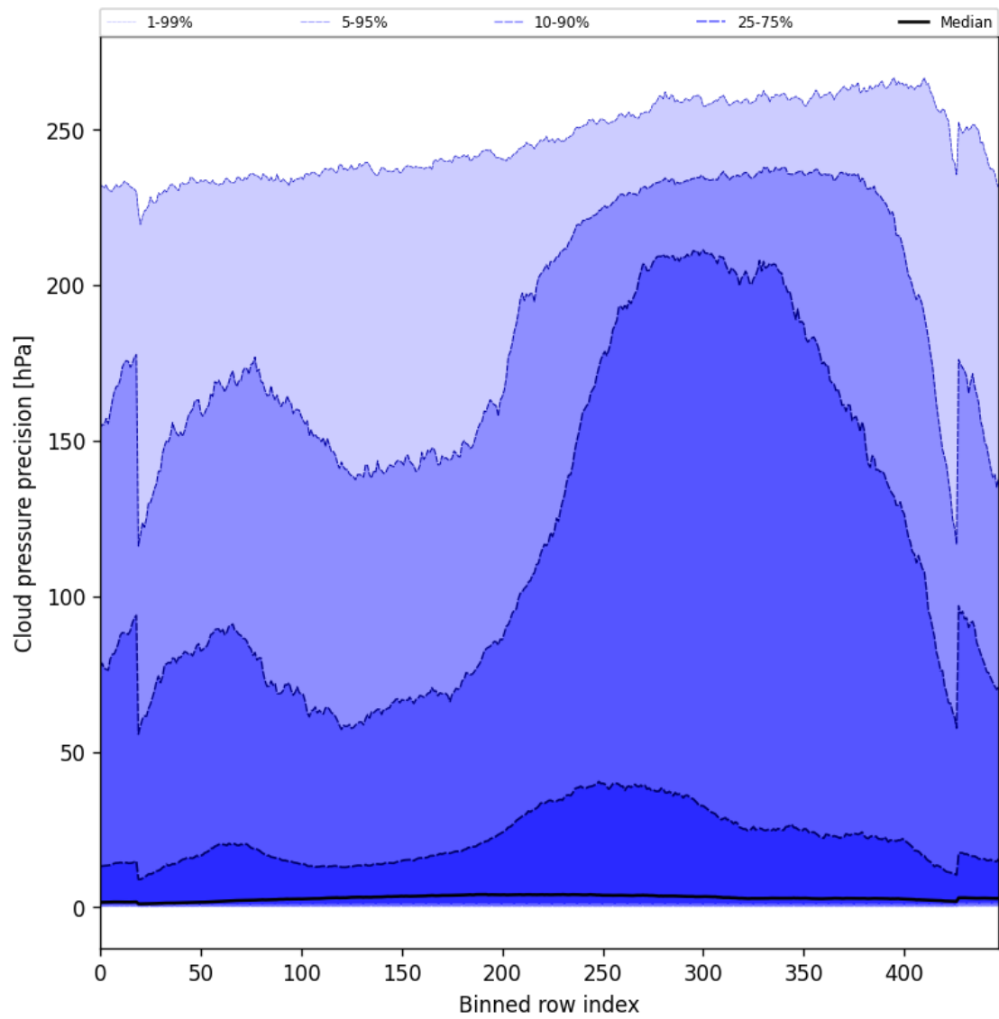
Figure 48: Along track statistics of “Cloud pressure precision” for 2024-10-03 to 2024-10-05
