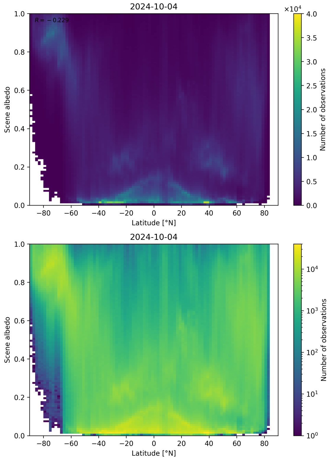
Figure 104: Scatter density plot of “Latitude” against “Scene albedo” for 2024-10-03 to 2024-10-05.
