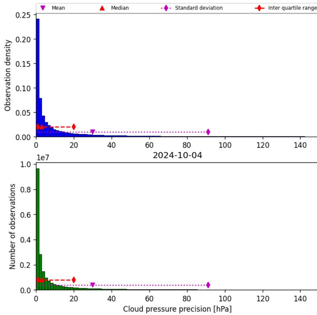
Figure 31: Histogram of “Cloud pressure precision” for 2024-10-03 to 2024-10-05
