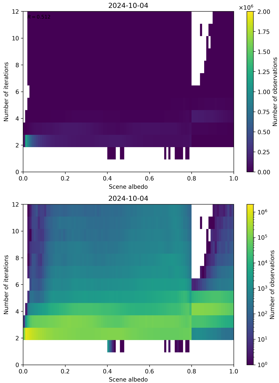
Figure 115: Scatter density plot of “Scene albedo” against “Number of iterations” for 2024-10-03 to 2024-10-05.
