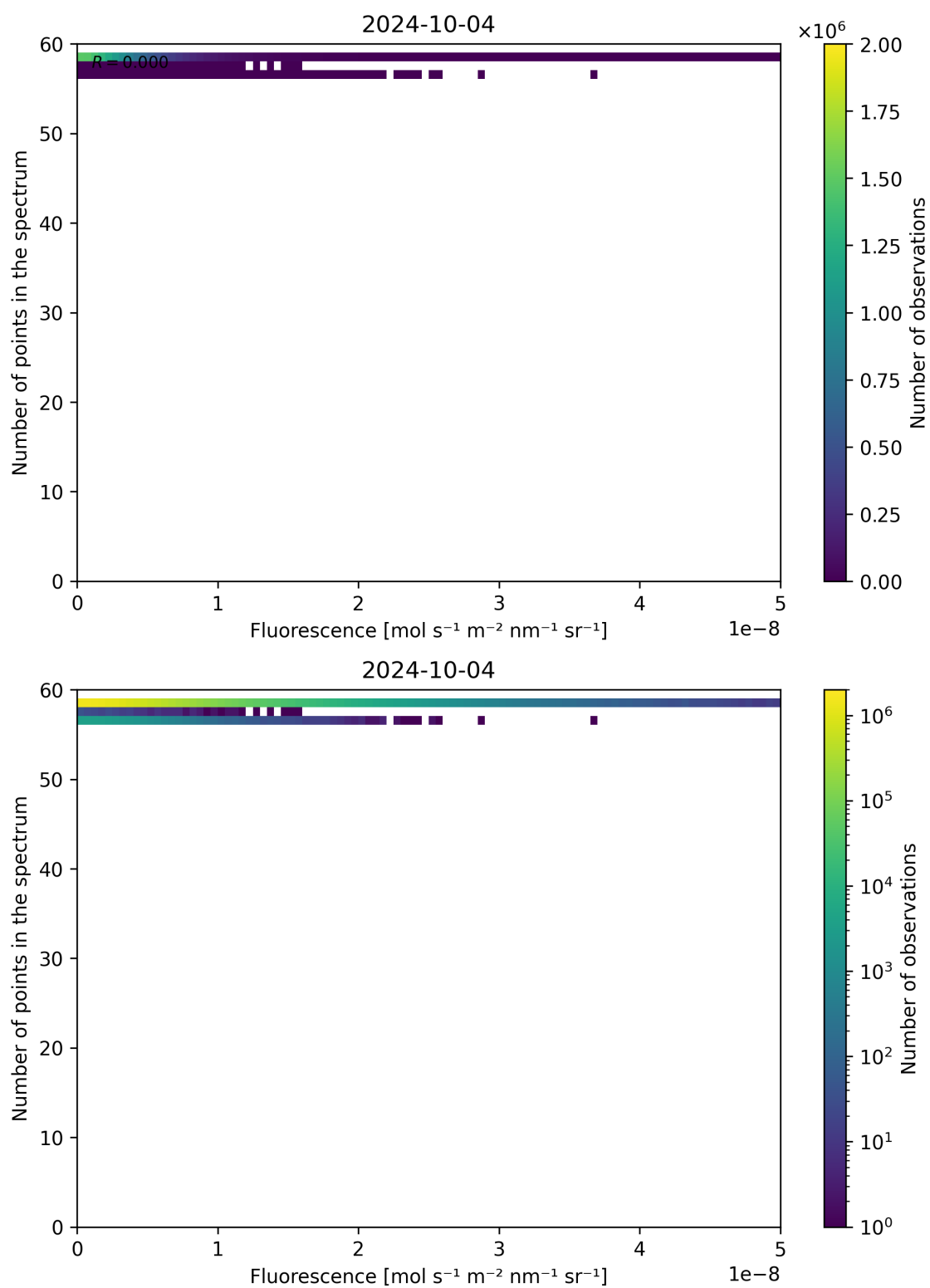
Figure 94: Scatter density plot of “Fluorescence” against “Number of points in the spectrum” for 2024-10-03 to 2024-10-05.
