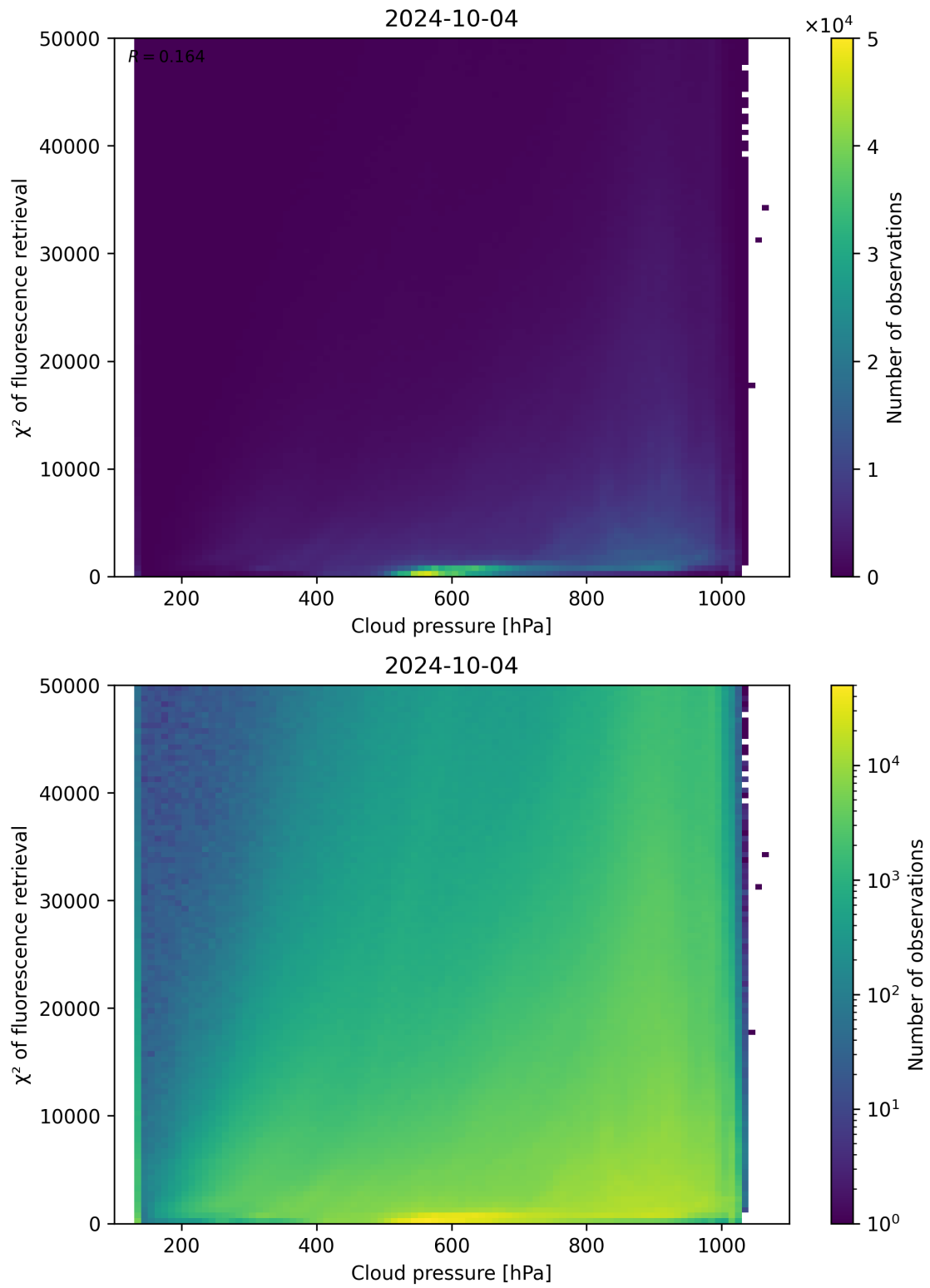
Figure 86: Scatter density plot of “Cloud pressure” against “ \chi^2 of fluorescence retrieval” for 2024-10-03 to 2024-10-05.
