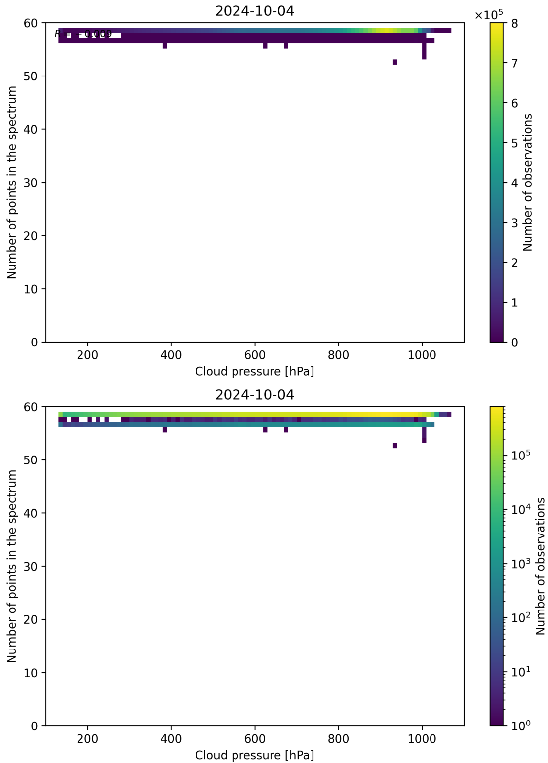
Figure 90: Scatter density plot of “Cloud pressure” against “Number of points in the spectrum” for 2024-10-03 to 2024-10-05.
