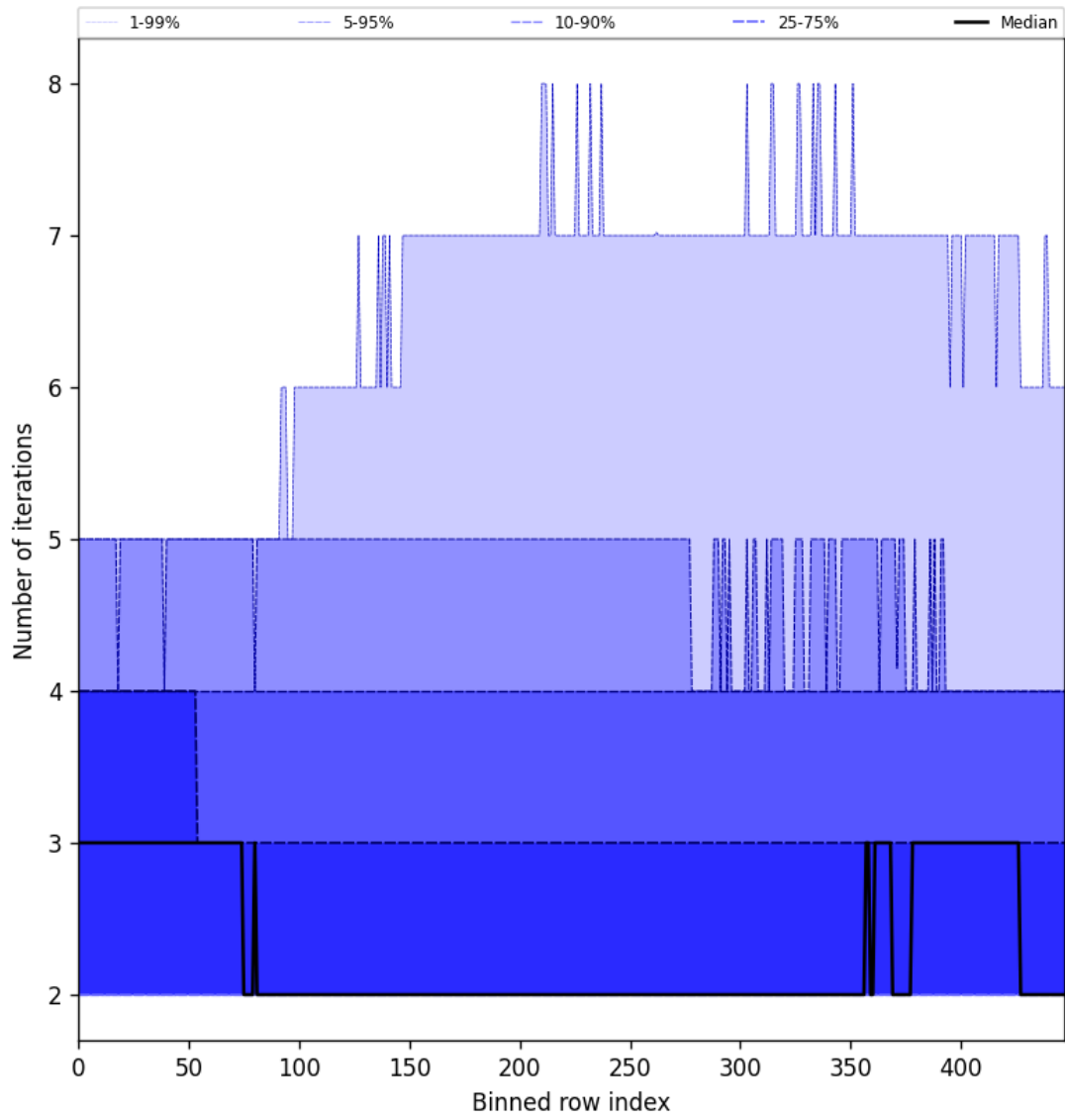
Figure 56: Along track statistics of “Number of iterations” for 2024-10-03 to 2024-10-05
