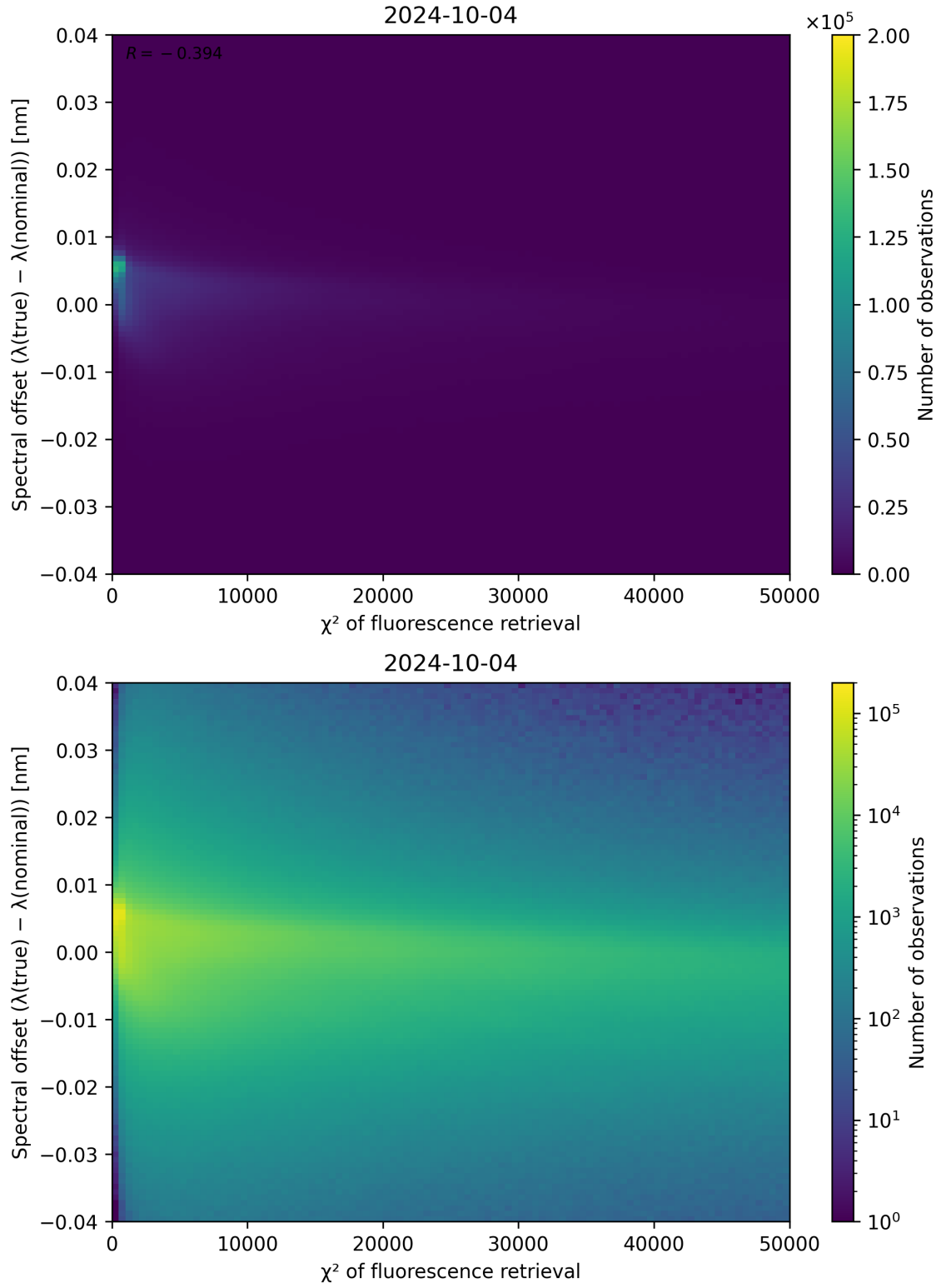
Figure 72: Scatter density plot of “ \chi^2 of fluorescence retrieval” against “Spectral offset ( \lambda_{\text{true}} - \lambda_{\text{nominal}} )” for 2024-10-03 to 2024-10-05.
