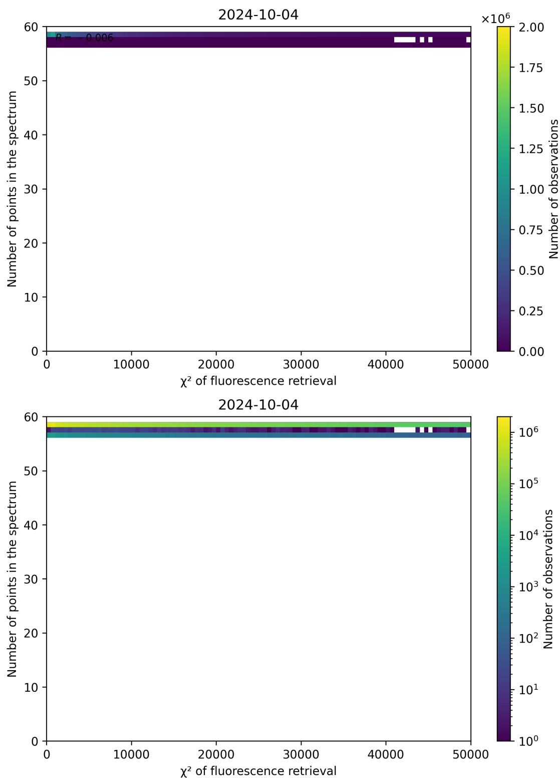
Figure 71: Scatter density plot of “ \chi^2 of fluorescence retrieval” against “Number of points in the spectrum” for 2024-10-03 to 2024-10-05.
