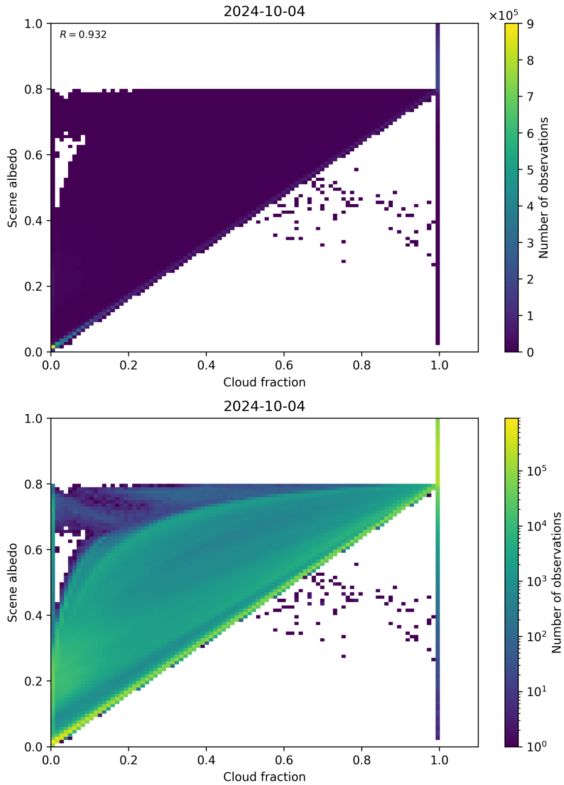
Figure 82: Scatter density plot of “Cloud fraction” against “Scene albedo” for 2024-10-03 to 2024-10-05.
