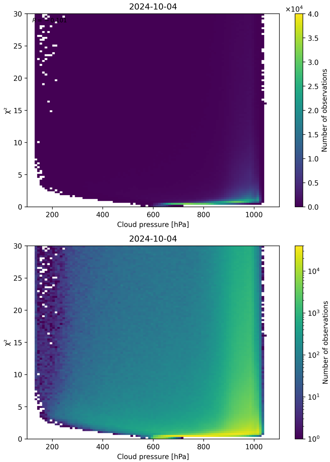
Figure 85: Scatter density plot of “Cloud pressure” against “ \chi^2 ” for 2024-10-03 to 2024-10-05.
