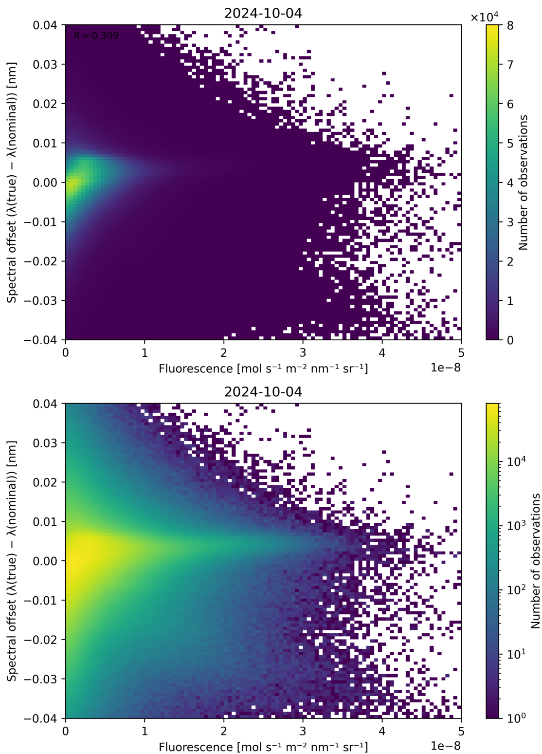
Figure 95: Scatter density plot of “Fluorescence” against “Spectral offset ( \lambda_{\text{true}} - \lambda_{\text{nominal}} )” for 2024-10-03 to 2024-10-05.
