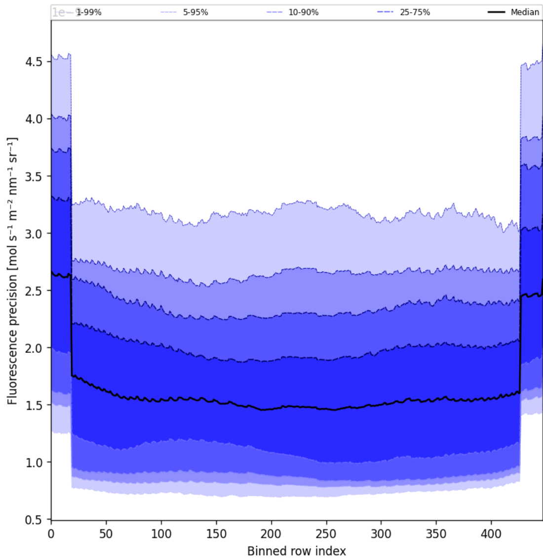
Figure 58: Along track statistics of “Fluorescence precision” for 2024-10-03 to 2024-10-05
