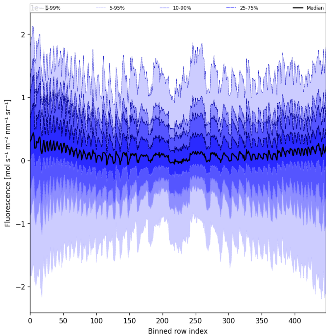
Figure 57: Along track statistics of “Fluorescence” for 2024-10-03 to 2024-10-05
