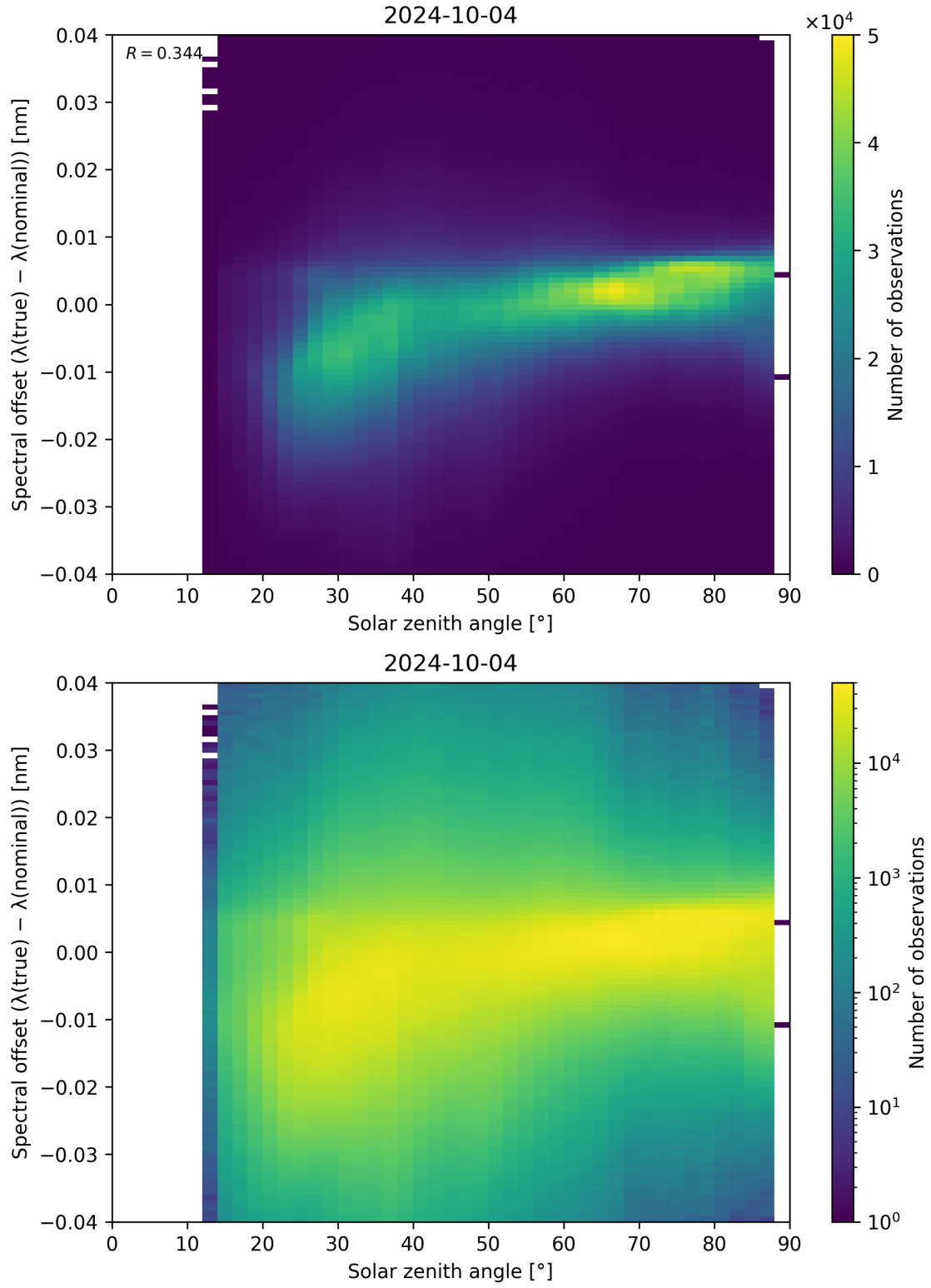
Figure 128: Scatter density plot of “Solar zenith angle” against “Spectral offset ( \lambda_{\text{true}} - \lambda_{\text{nominal}} )” for 2024-10-03 to 2024-10-05.
