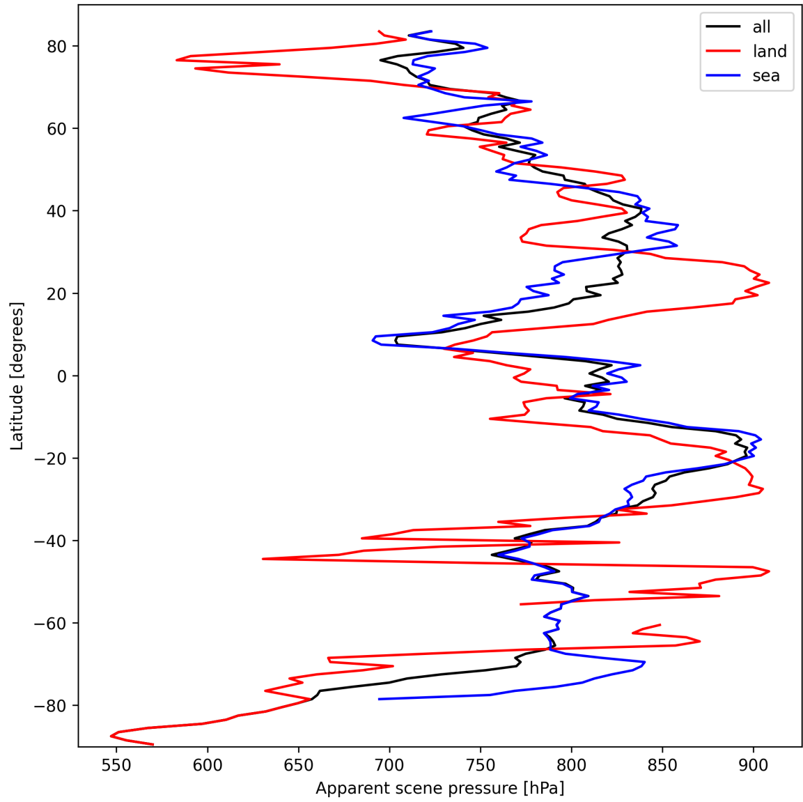
Figure 19: Zonal average of “Apparent scene pressure” for 2024-10-03 to 2024-10-05.
