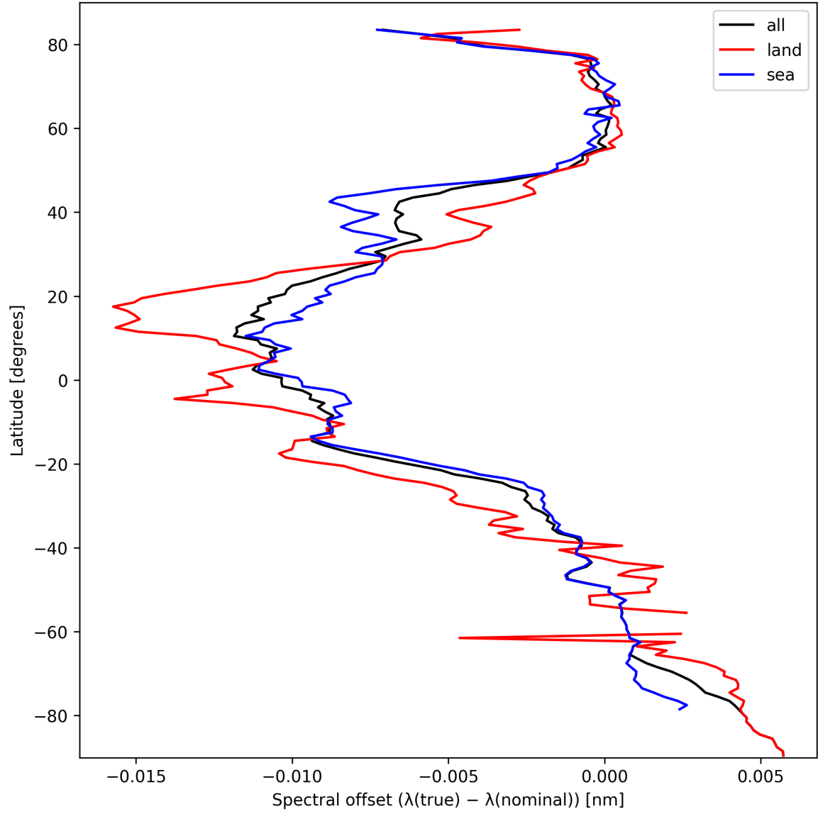
Figure 28: Zonal average of “Spectral offset ( \lambda_{\text{true}} - \lambda_{\text{nominal}} )” for 2024-10-03 to 2024-10-05.
