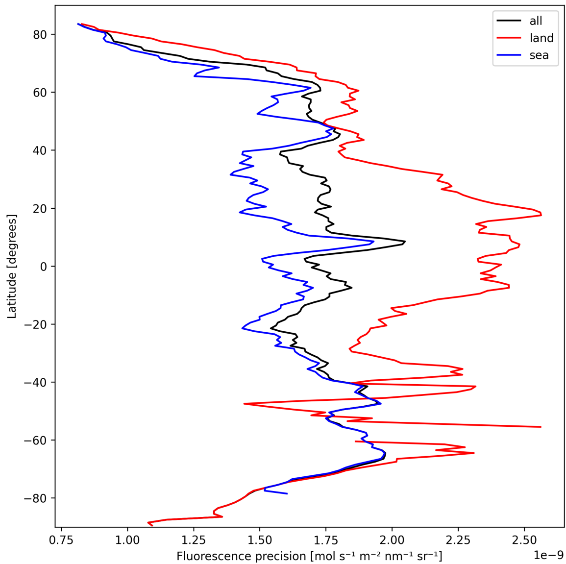
Figure 24: Zonal average of “Fluorescence precision” for 2024-10-03 to 2024-10-05.
