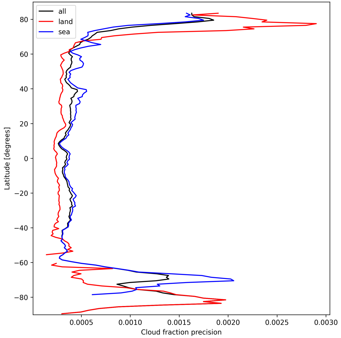
Figure 16: Zonal average of “Cloud fraction precision” for 2024-10-03 to 2024-10-05.
