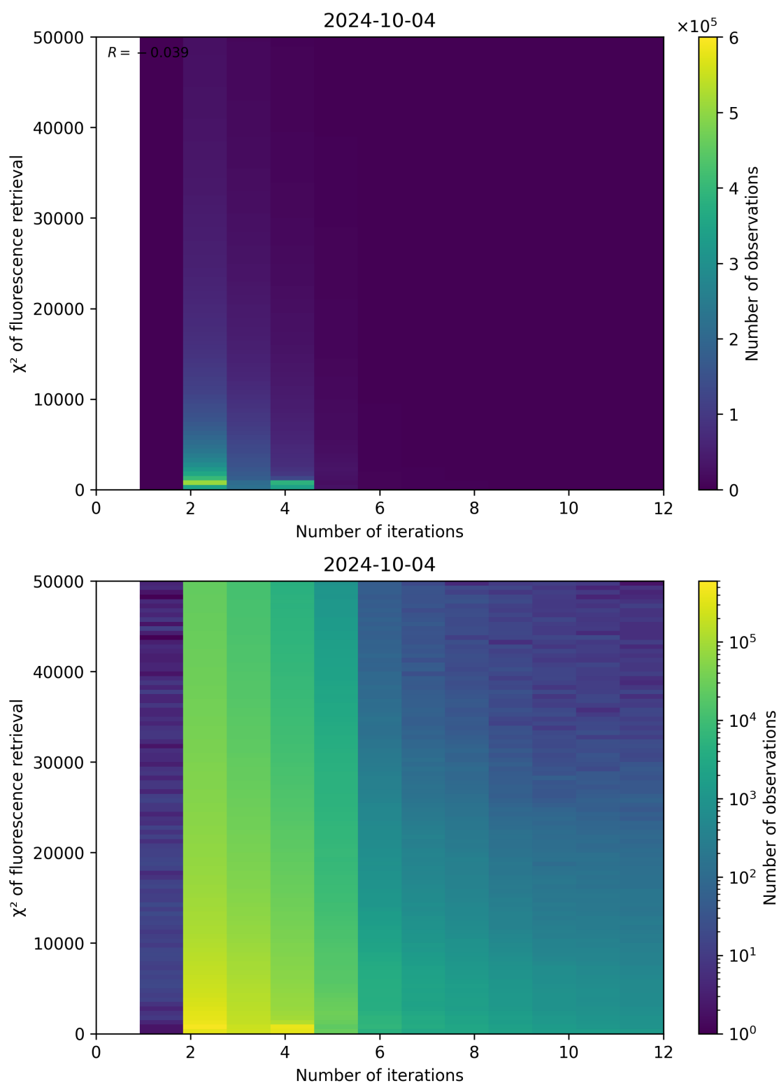
Figure 106: Scatter density plot of “Number of iterations” against “ \chi^2 of fluorescence retrieval” for 2024-10-03 to 2024-10-05.
