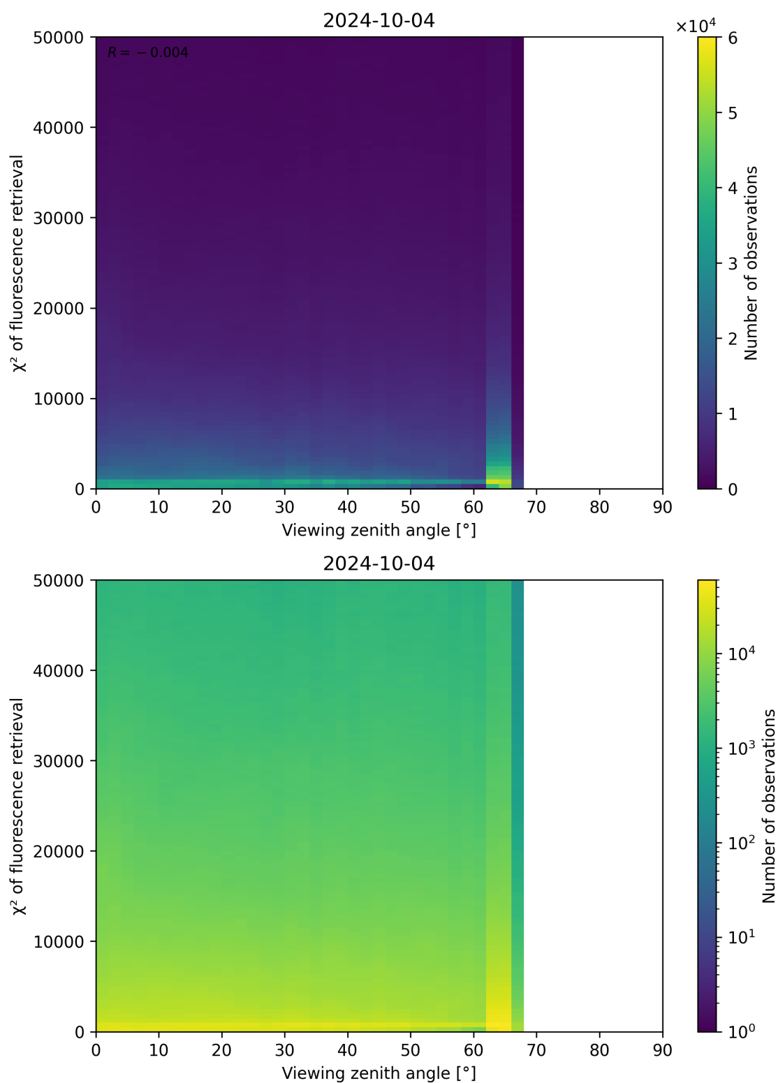
Figure 131: Scatter density plot of “Viewing zenith angle” against “ \chi^2 of fluorescence retrieval” for 2024-10-03 to 2024-10-05.
