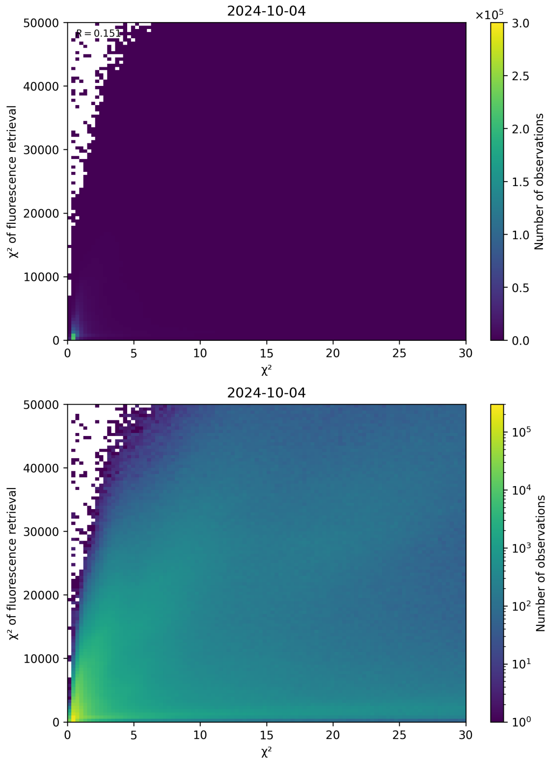
Figure 69: Scatter density plot of “ \chi^2 ” against “ \chi^2 of fluorescence retrieval” for 2024-10-03 to 2024-10-05.
