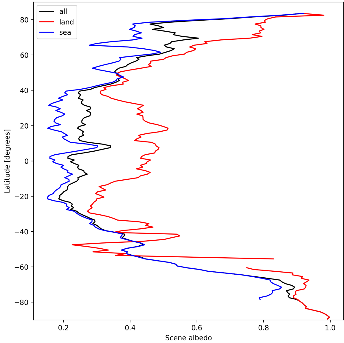
Figure 17: Zonal average of “Scene albedo” for 2024-10-03 to 2024-10-05.
