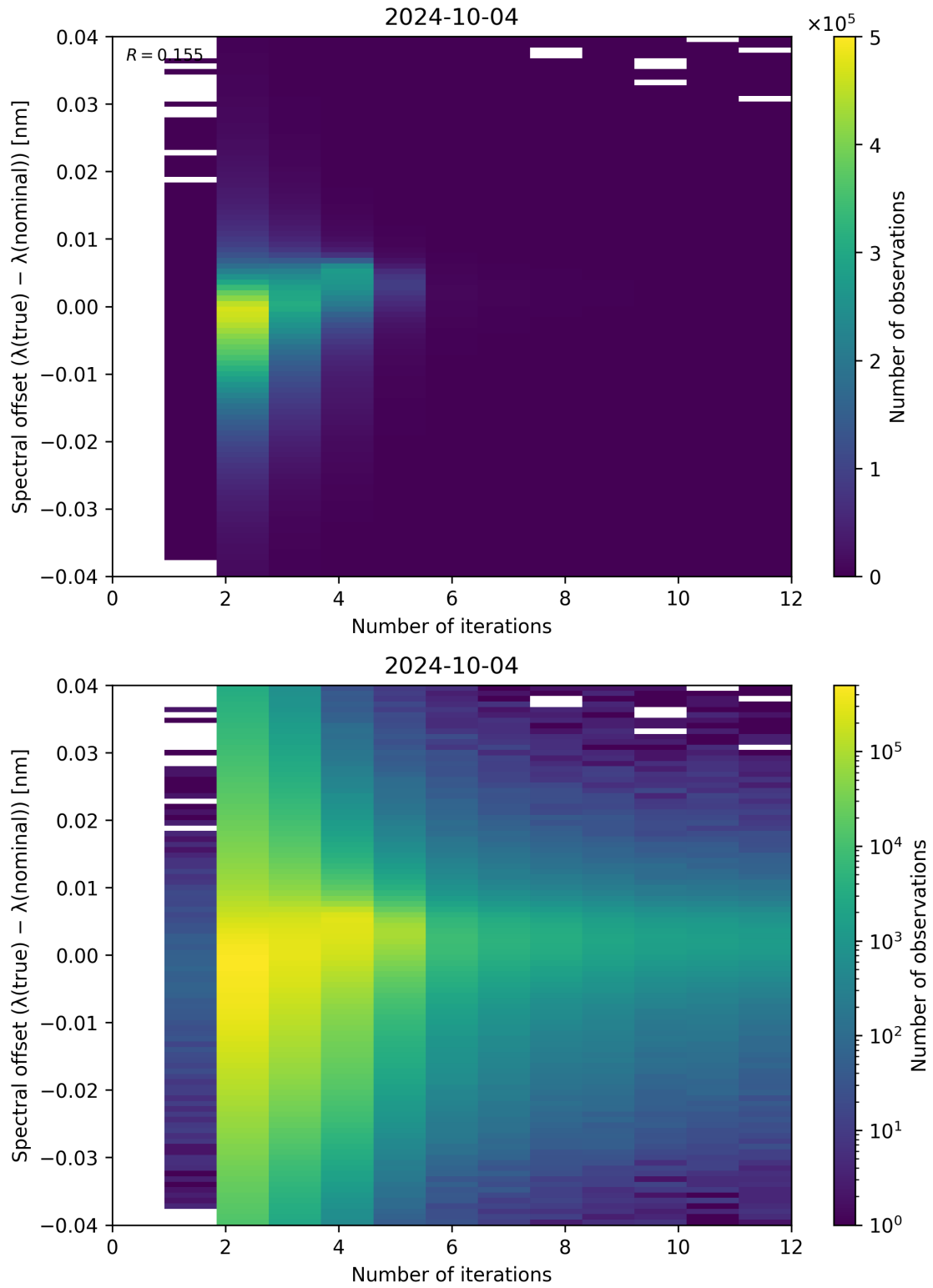
Figure 109: Scatter density plot of “Number of iterations” against “Spectral offset ( \lambda_{\text{true}} - \lambda_{\text{nominal}} )” for 2024-10-03 to 2024-10-05.
