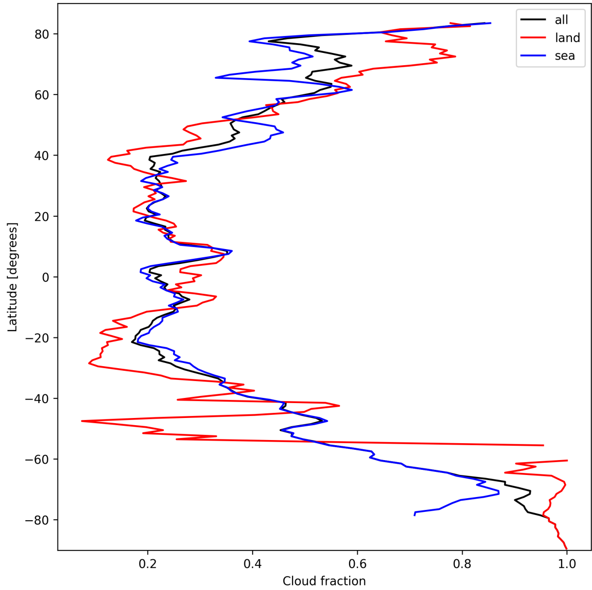
Figure 15: Zonal average of “Cloud fraction” for 2024-10-03 to 2024-10-05.
