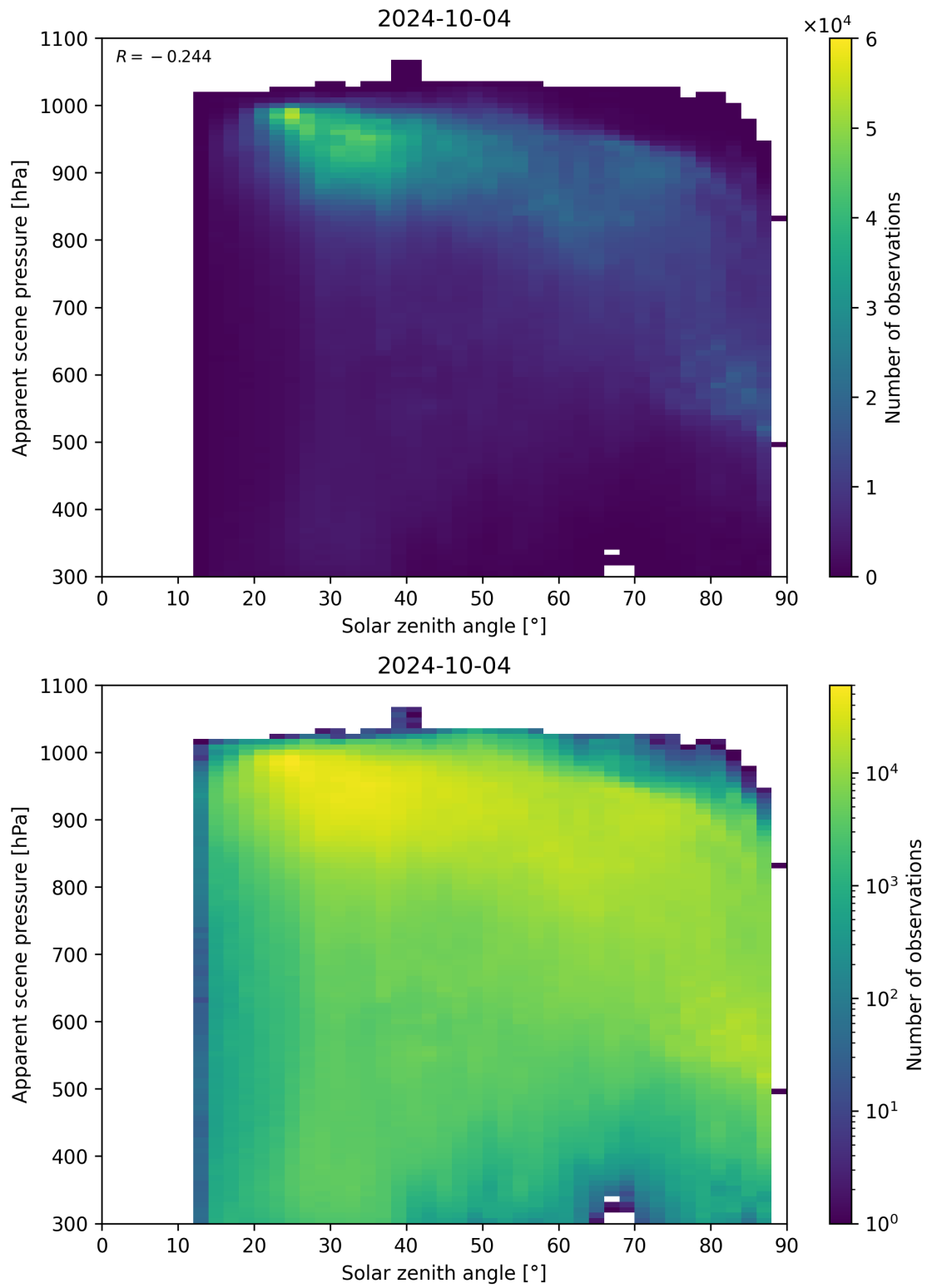
Figure 118: Scatter density plot of “Solar zenith angle” against “Apparent scene pressure” for 2024-10-03 to 2024-10-05.
