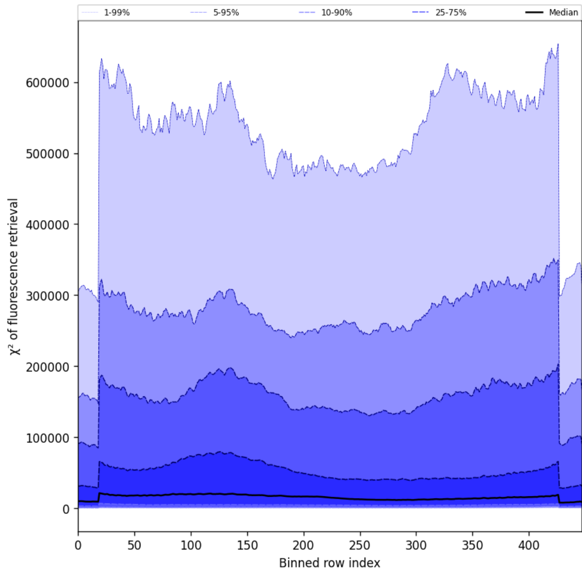
Figure 59: Along track statistics of “ \chi^2 of fluorescence retrieval” for 2024-10-03 to 2024-10-05
