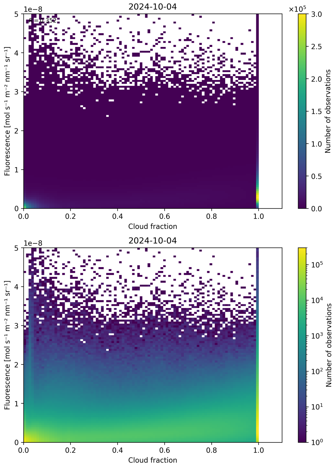
Figure 79: Scatter density plot of “Cloud fraction” against “Fluorescence” for 2024-10-03 to 2024-10-05.
