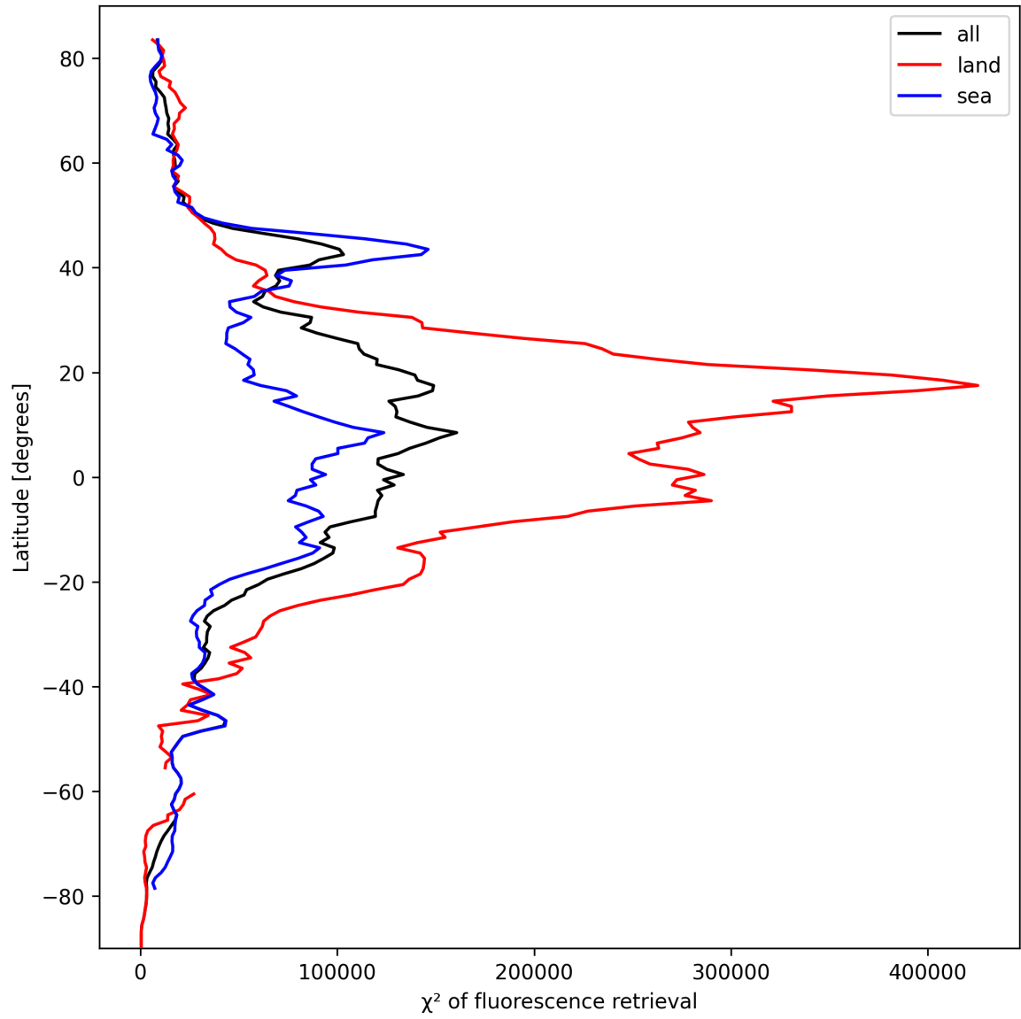
Figure 25: Zonal average of “ \chi^2 of fluorescence retrieval” for 2024-10-03 to 2024-10-05.
