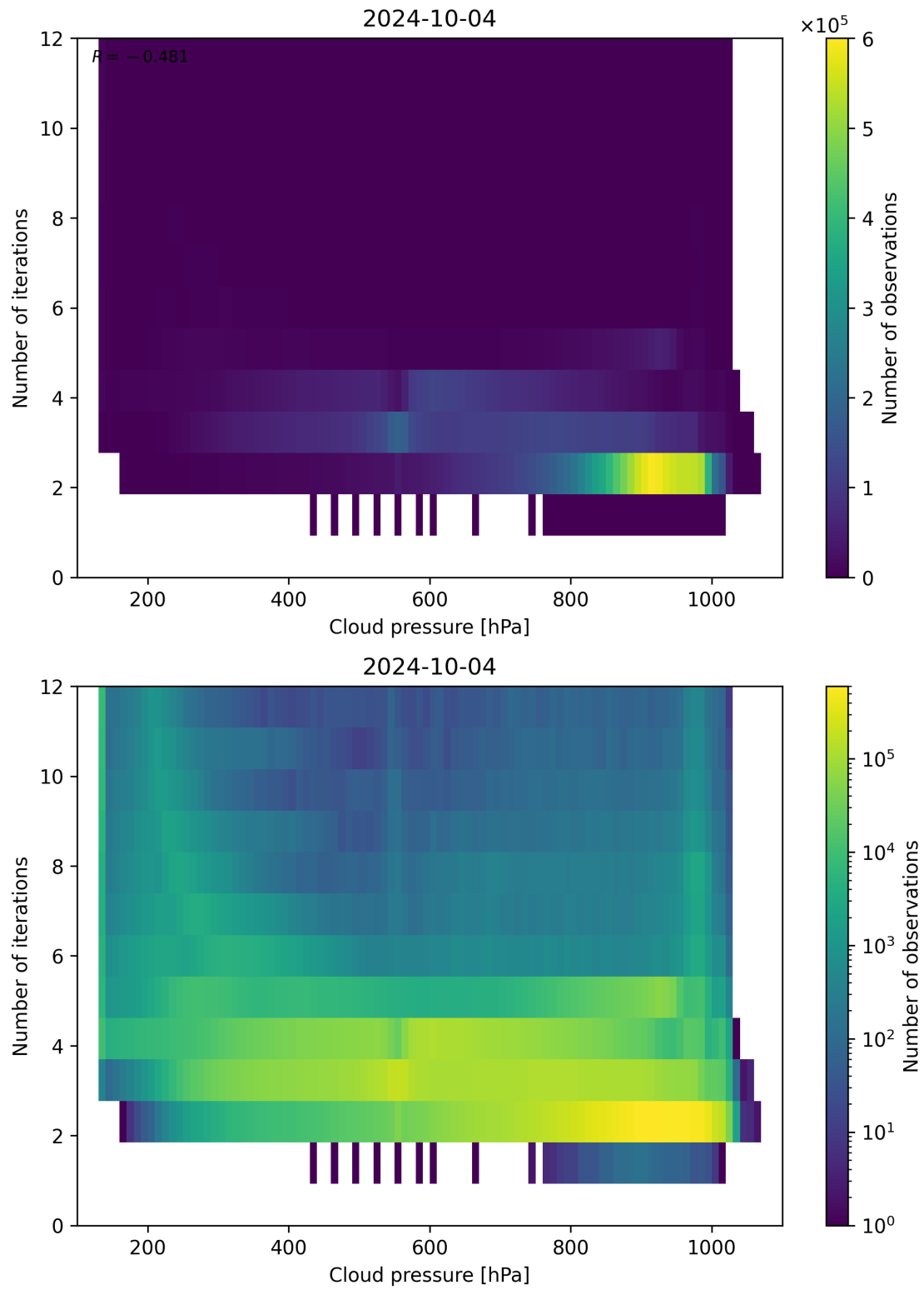
Figure 89: Scatter density plot of “Cloud pressure” against “Number of iterations” for 2024-10-03 to 2024-10-05.
