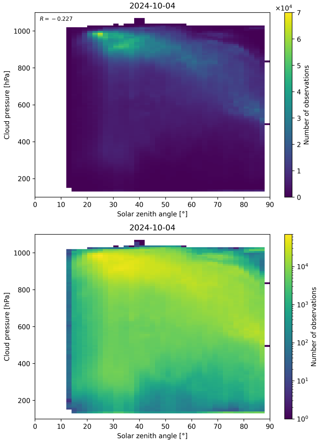
Figure 122: Scatter density plot of “Solar zenith angle” against “Cloud pressure” for 2024-10-03 to 2024-10-05.
