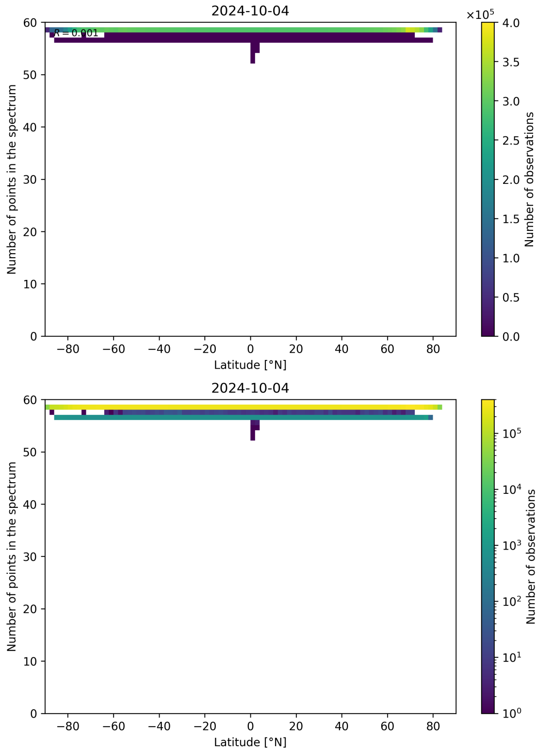
Figure 103: Scatter density plot of “Latitude” against “Number of points in the spectrum” for 2024-10-03 to 2024-10-05.
