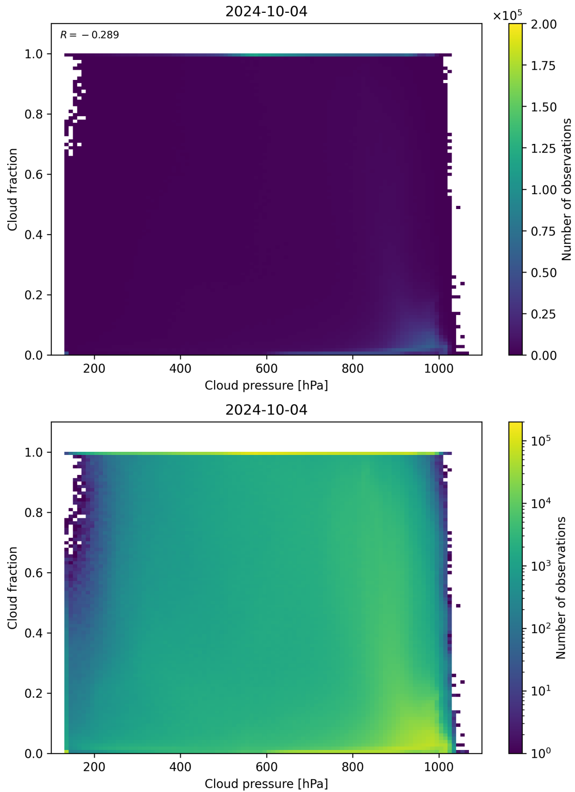
Figure 87: Scatter density plot of “Cloud pressure” against “Cloud fraction” for 2024-10-03 to 2024-10-05.
