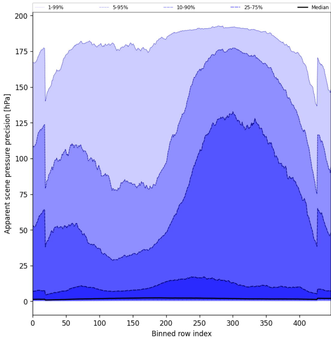
Figure 54: Along track statistics of “Apparent scene pressure precision” for 2024-10-03 to 2024-10-05
