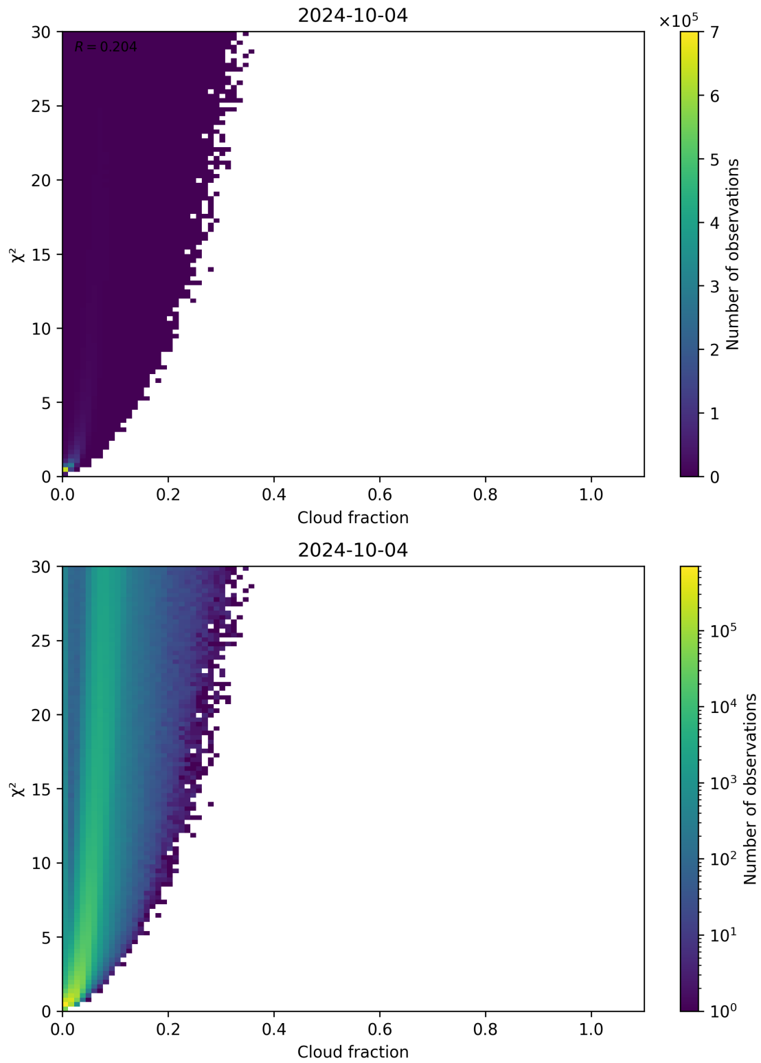
Figure 77: Scatter density plot of “Cloud fraction” against “ \chi^2 ” for 2024-10-03 to 2024-10-05.
