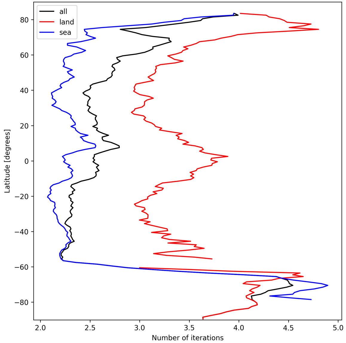
Figure 22: Zonal average of “Number of iterations” for 2024-10-03 to 2024-10-05.
