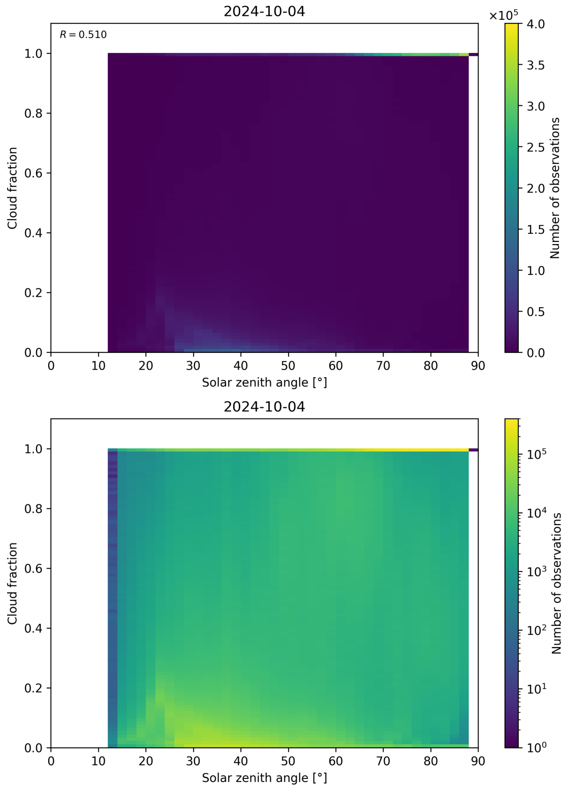
Figure 121: Scatter density plot of “Solar zenith angle” against “Cloud fraction” for 2024-10-03 to 2024-10-05.
