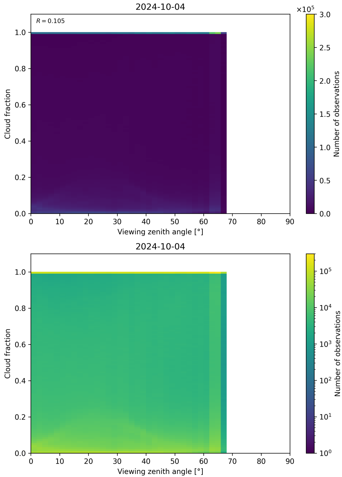
Figure 132: Scatter density plot of “Viewing zenith angle” against “Cloud fraction” for 2024-10-03 to 2024-10-05.
