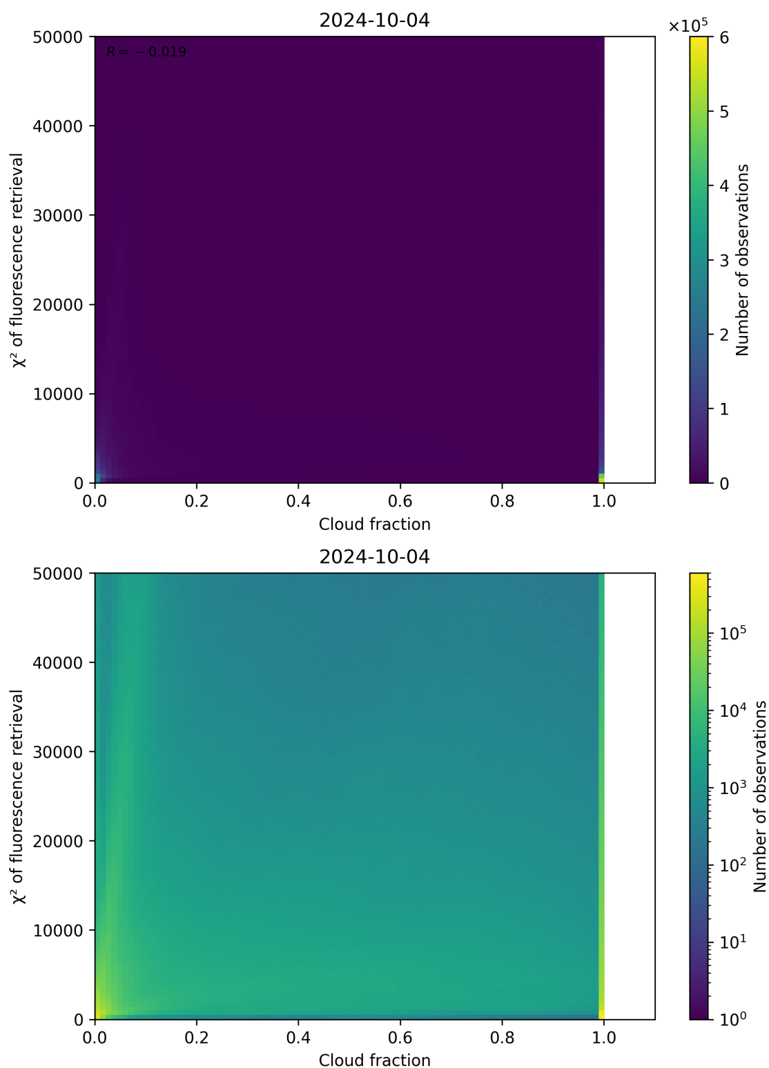
Figure 78: Scatter density plot of “Cloud fraction” against “ \chi^2 of fluorescence retrieval” for 2024-10-03 to 2024-10-05.
