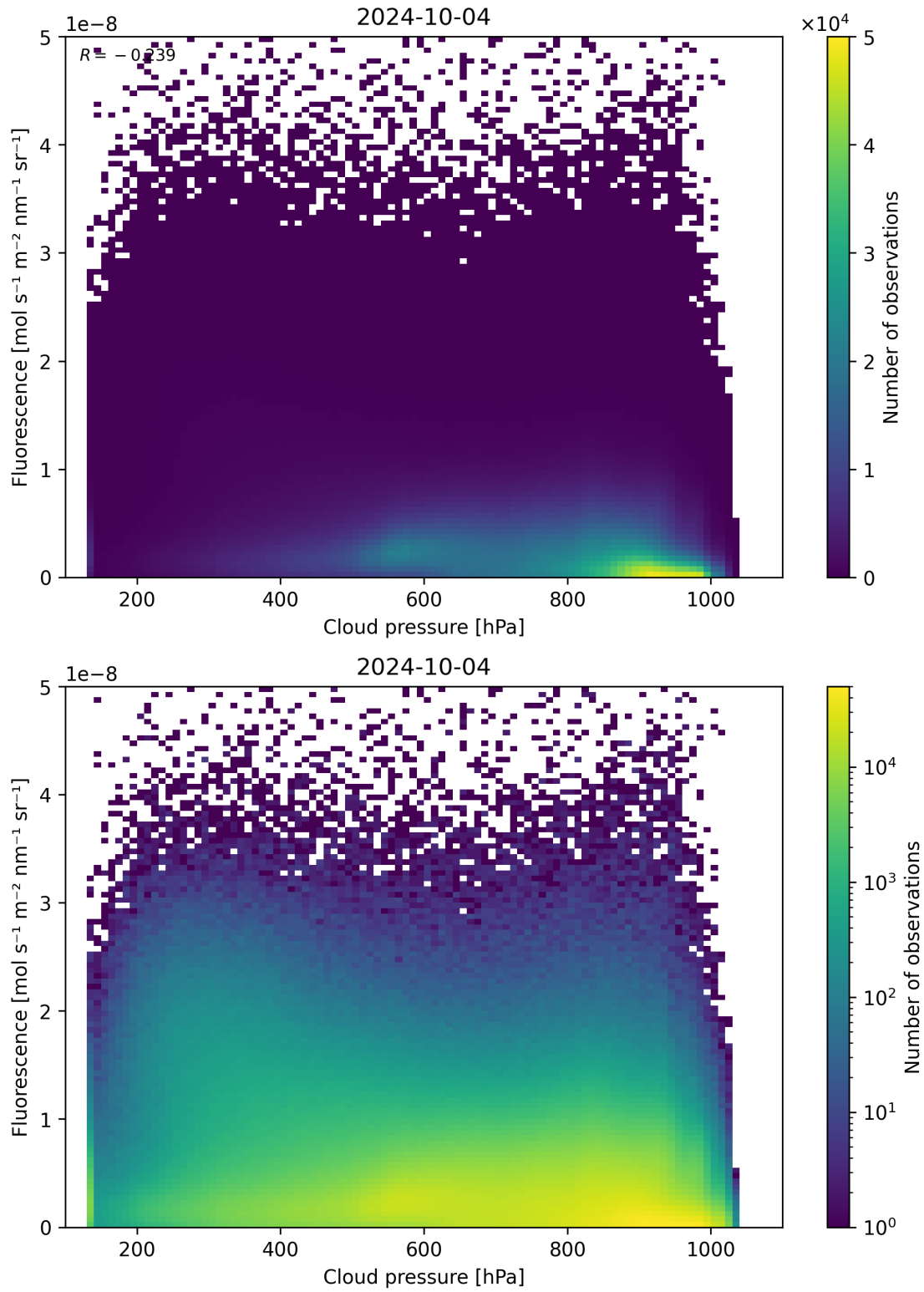
Figure 88: Scatter density plot of “Cloud pressure” against “Fluorescence” for 2024-10-03 to 2024-10-05.
