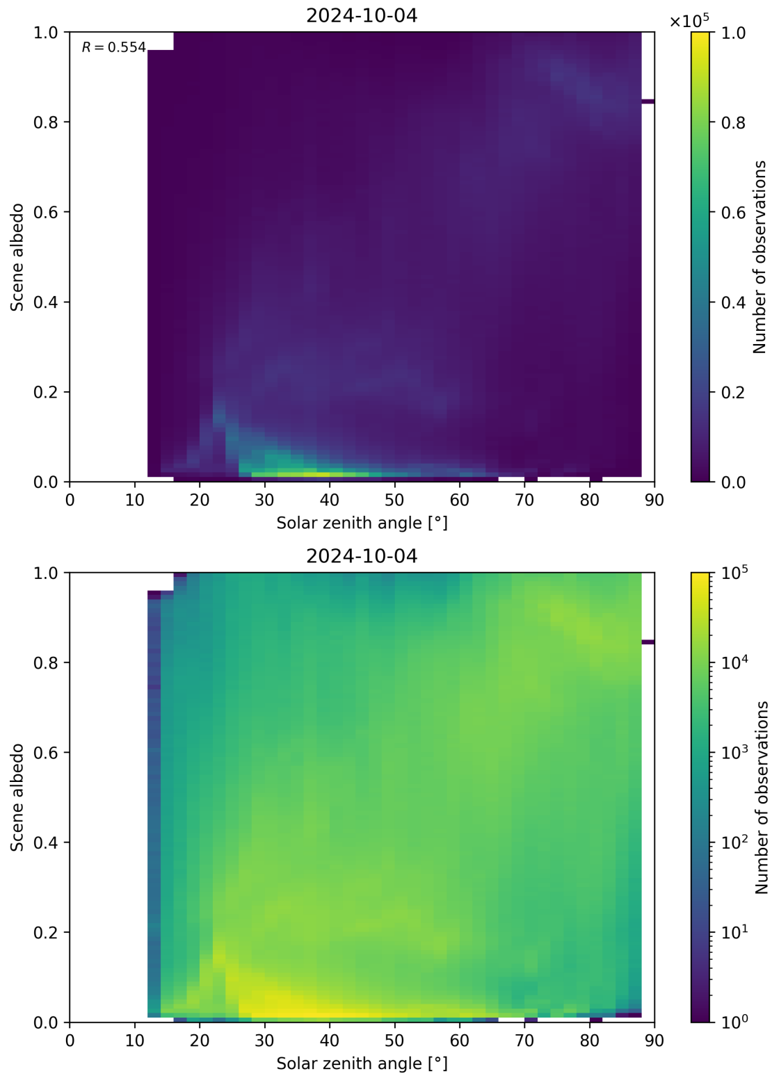
Figure 127: Scatter density plot of “Solar zenith angle” against “Scene albedo” for 2024-10-03 to 2024-10-05.
