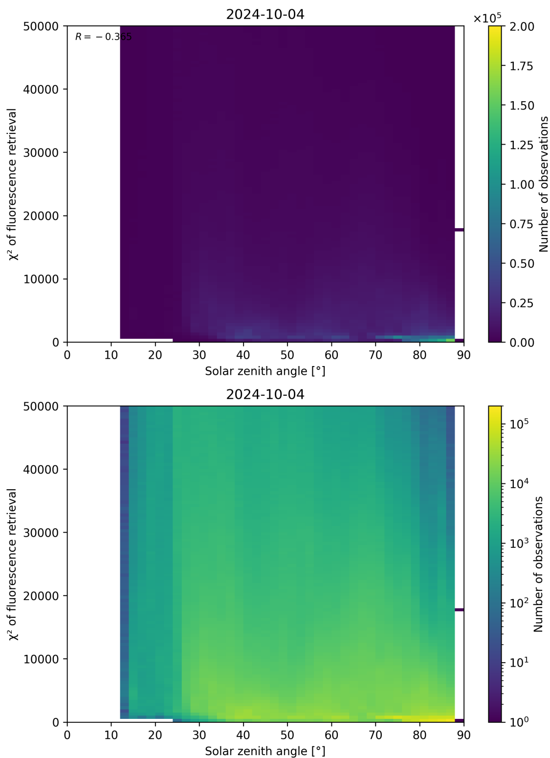
Figure 120: Scatter density plot of “Solar zenith angle” against “ \chi^2 of fluorescence retrieval” for 2024-10-03 to 2024-10-05.
