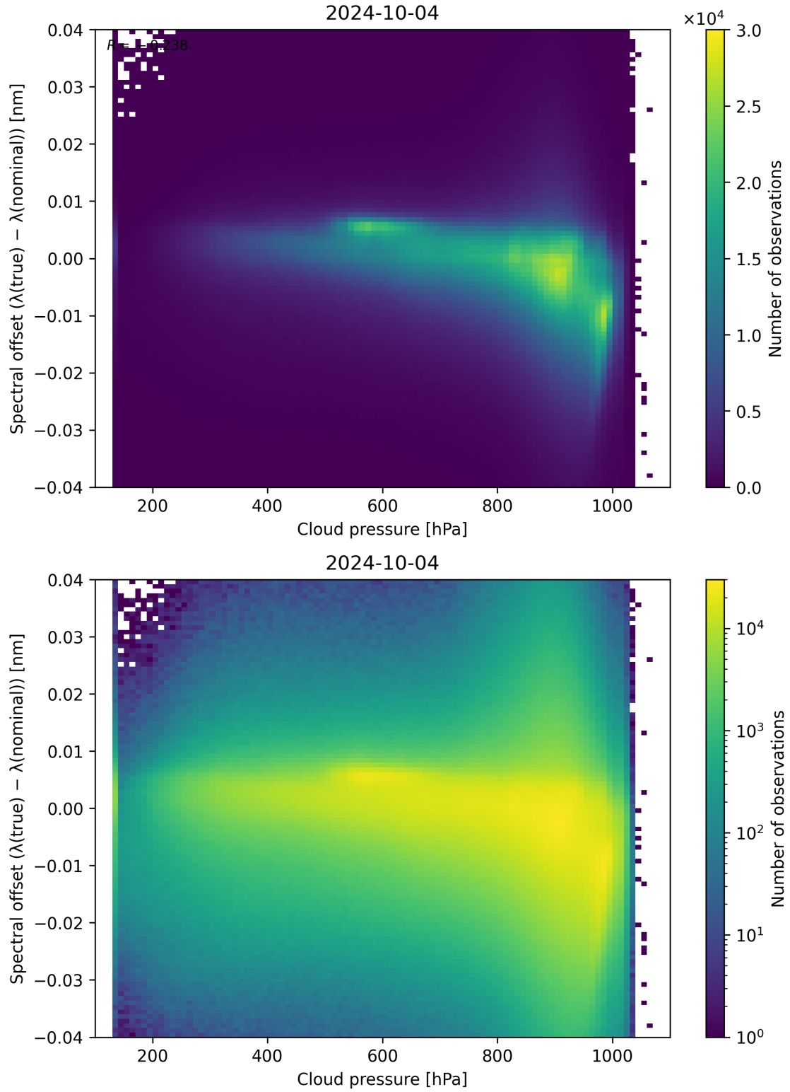
Figure 92: Scatter density plot of “Cloud pressure” against “Spectral offset ( \lambda_{\text{true}} - \lambda_{\text{nominal}} )” for 2024-10-03 to 2024-10-05.
