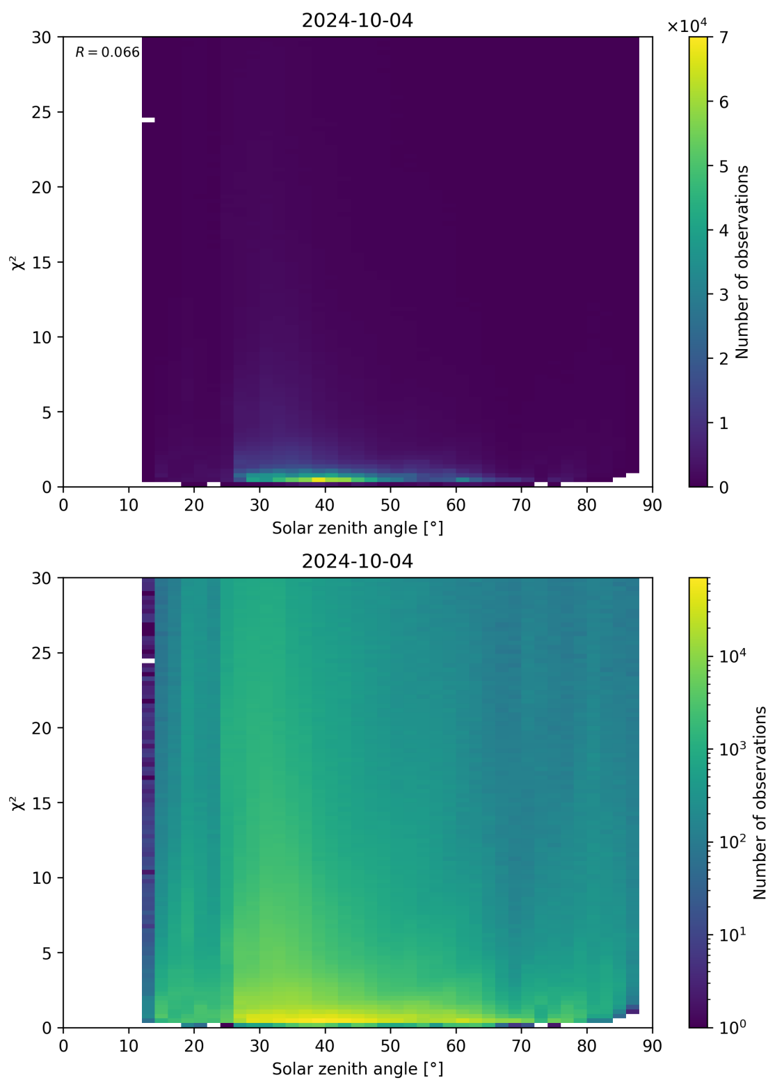
Figure 119: Scatter density plot of “Solar zenith angle” against “ \chi^2 ” for 2024-10-03 to 2024-10-05.
