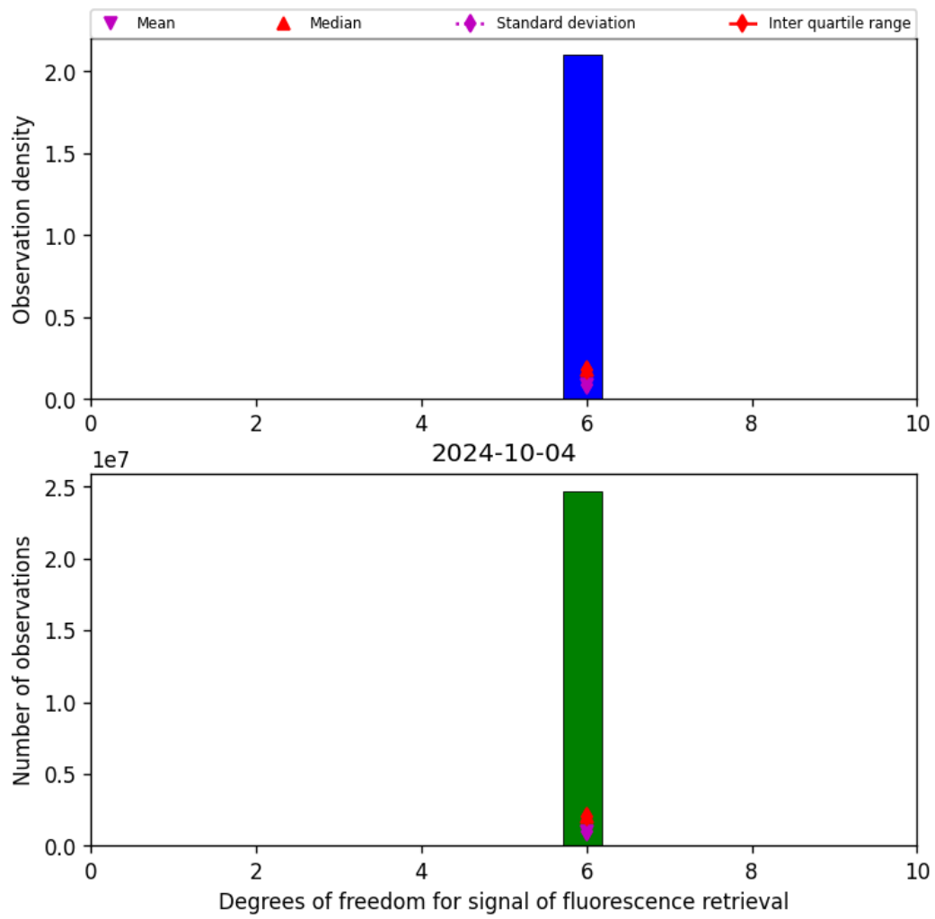
Figure 43: Histogram of “Degrees of freedom for signal of fluorescence retrieval” for 2024-10-03 to 2024-10-05
