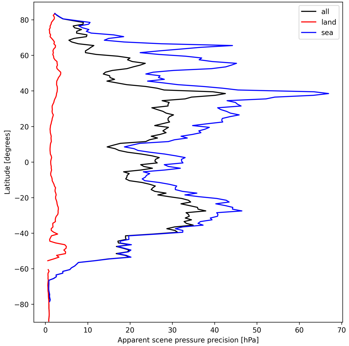
Figure 20: Zonal average of “Apparent scene pressure precision” for 2024-10-03 to 2024-10-05.
