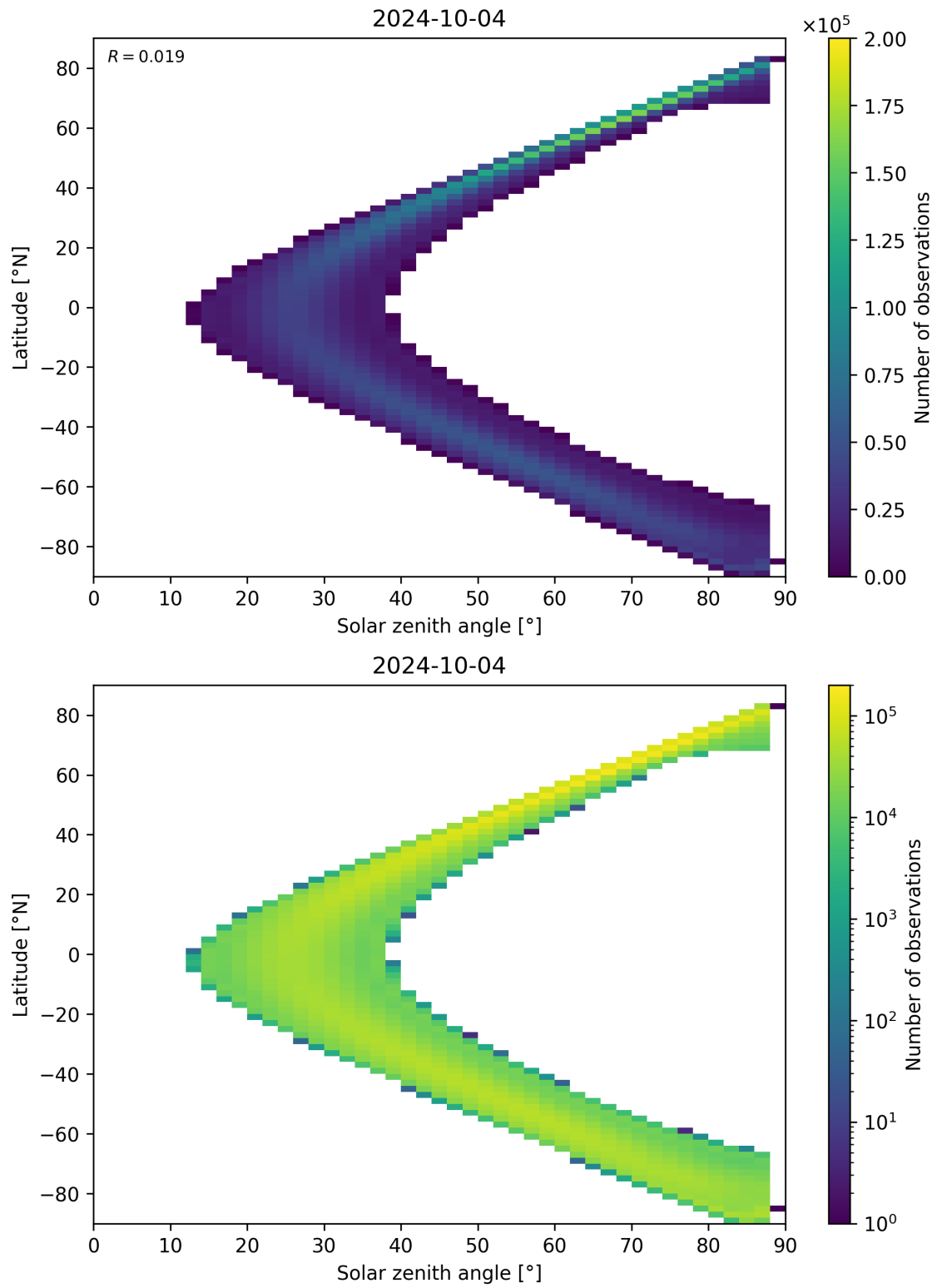
Figure 124: Scatter density plot of “Solar zenith angle” against “Latitude” for 2024-10-03 to 2024-10-05.
