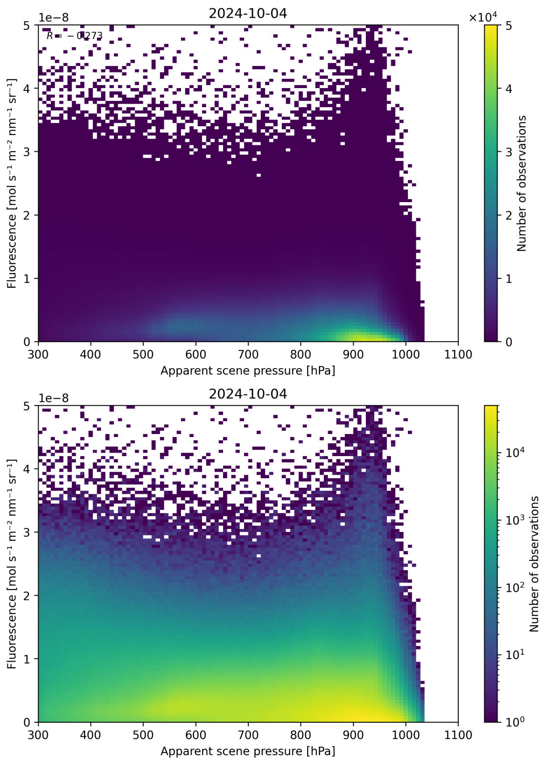
Figure 65: Scatter density plot of “Apparent scene pressure” against “Fluorescence” for 2024-10-03 to 2024-10-05.
