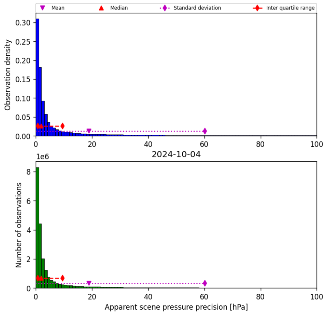
Figure 37: Histogram of “Apparent scene pressure precision” for 2024-10-03 to 2024-10-05
