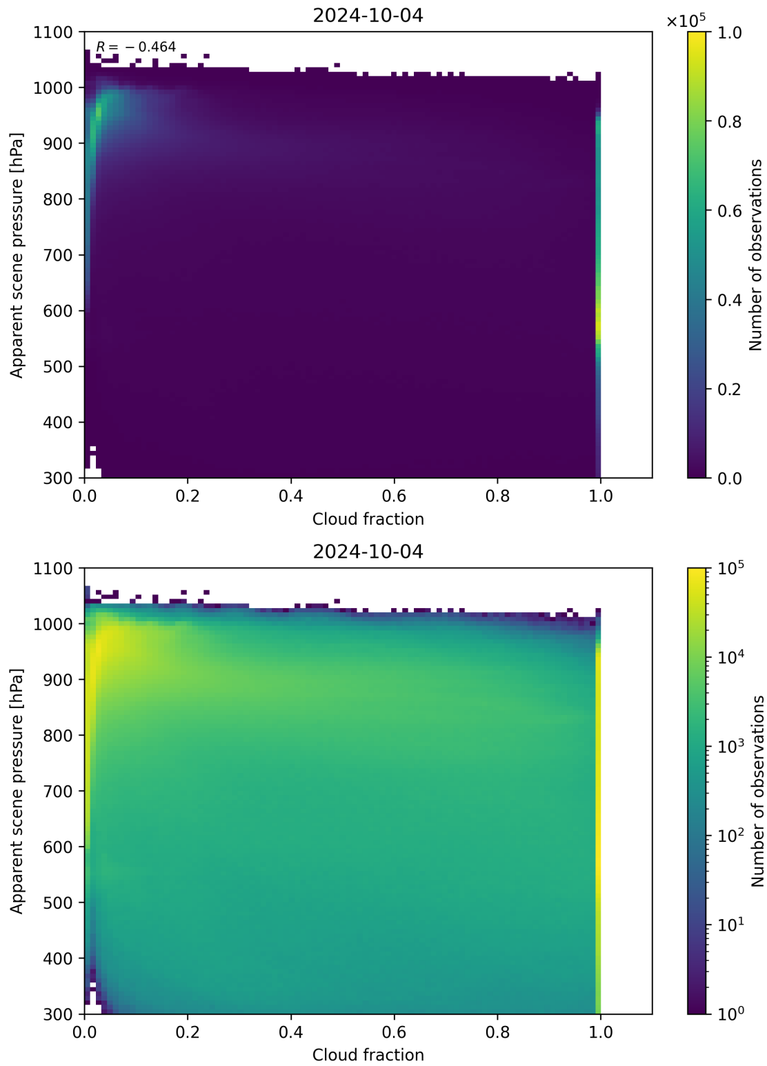
Figure 76: Scatter density plot of “Cloud fraction” against “Apparent scene pressure” for 2024-10-03 to 2024-10-05.
