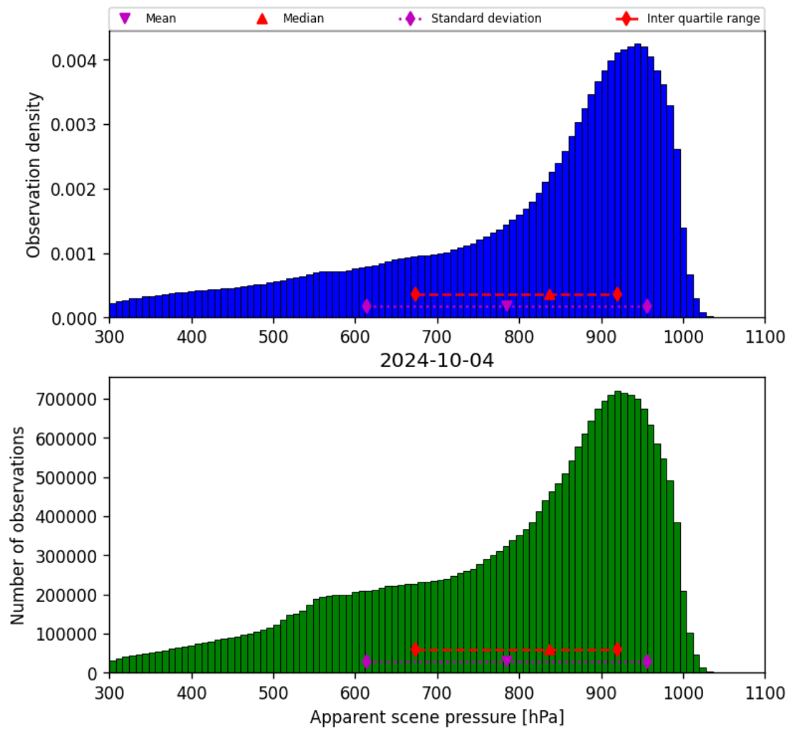
Figure 36: Histogram of “Apparent scene pressure” for 2024-10-03 to 2024-10-05
