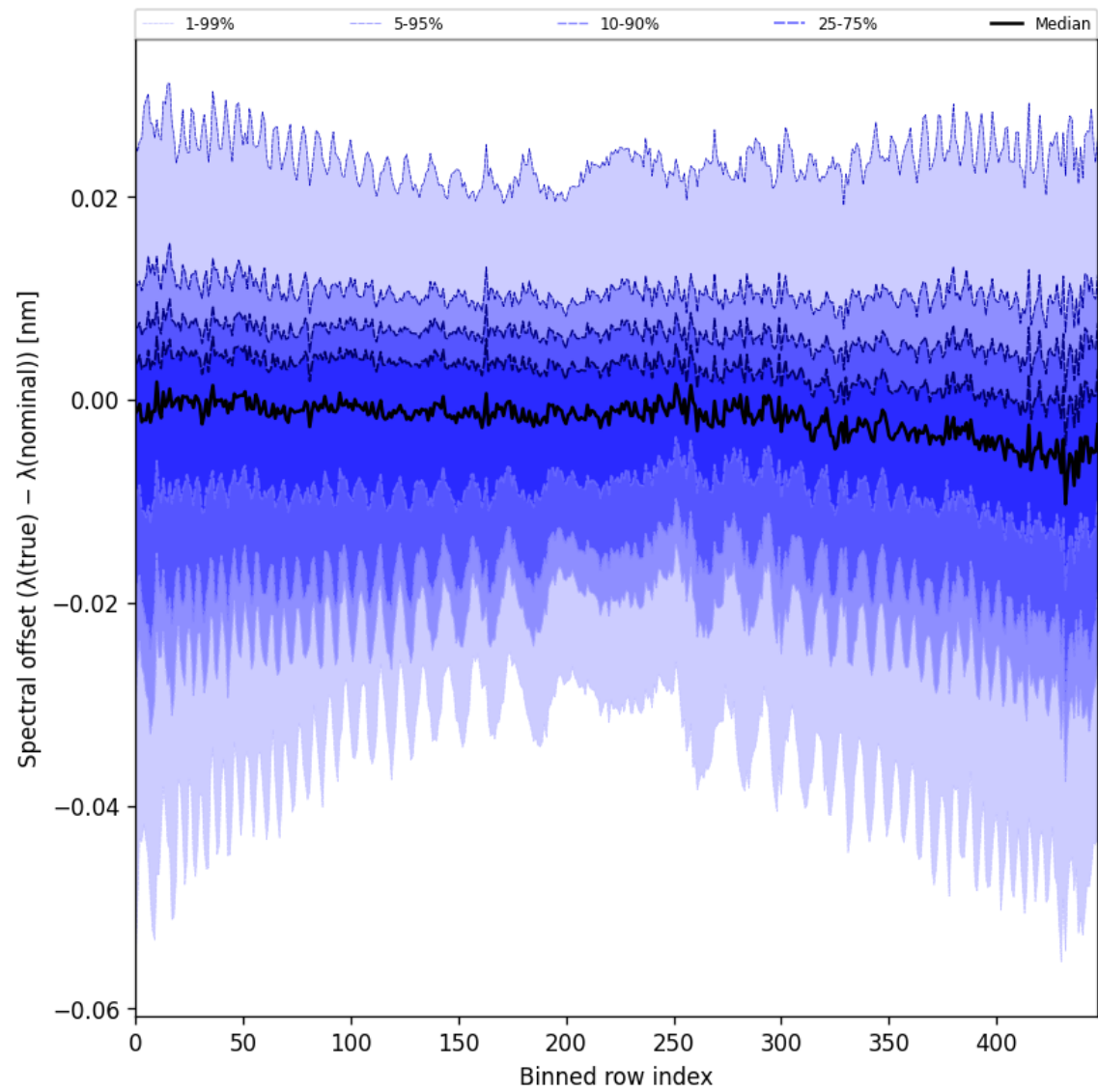
Figure 62: Along track statistics of “Spectral offset ( \lambda_{\text{true}} - \lambda_{\text{nominal}} )” for 2024-10-03 to 2024-10-05
