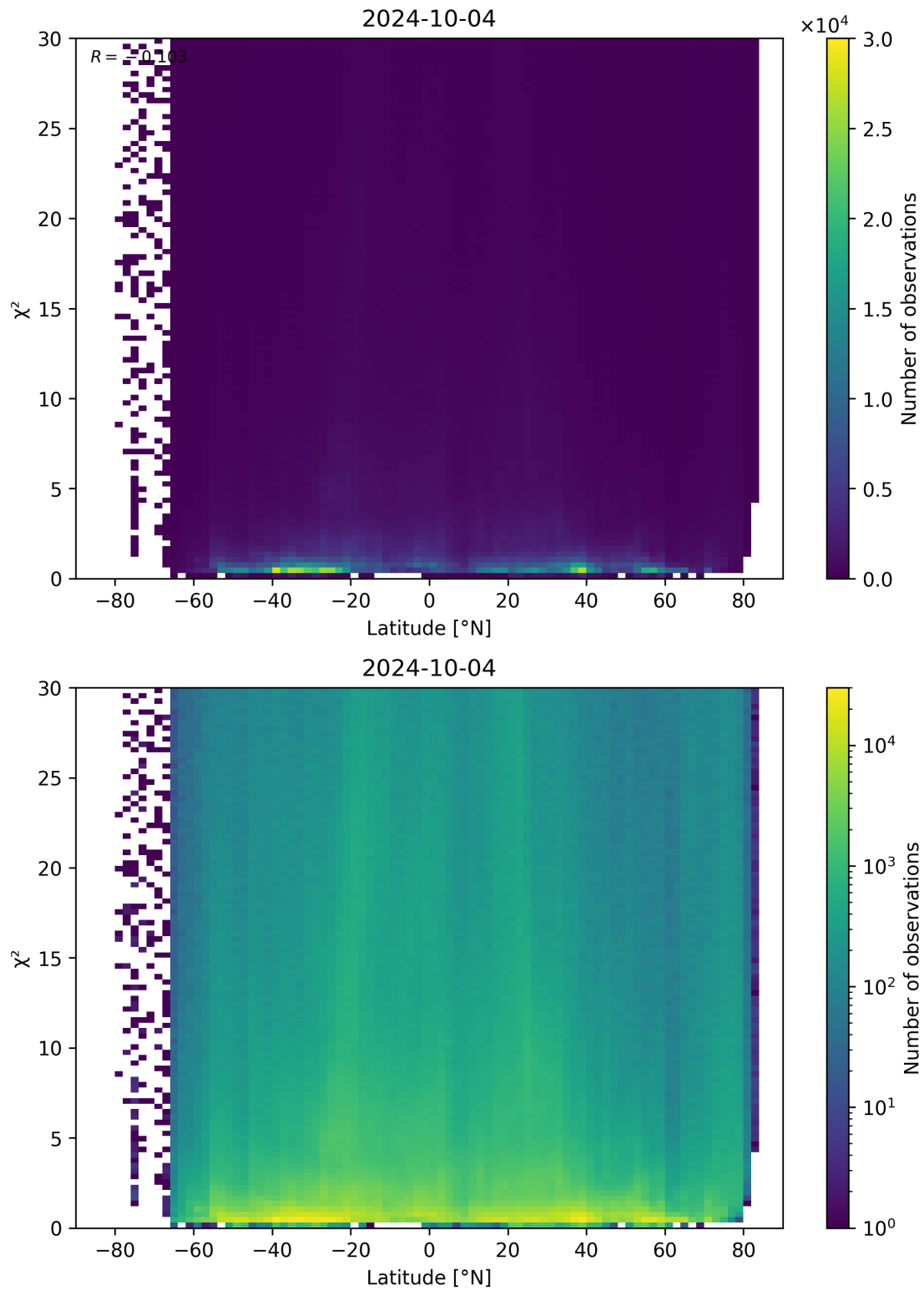
Figure 97: Scatter density plot of “Latitude” against “ \chi^2 ” for 2024-10-03 to 2024-10-05.
