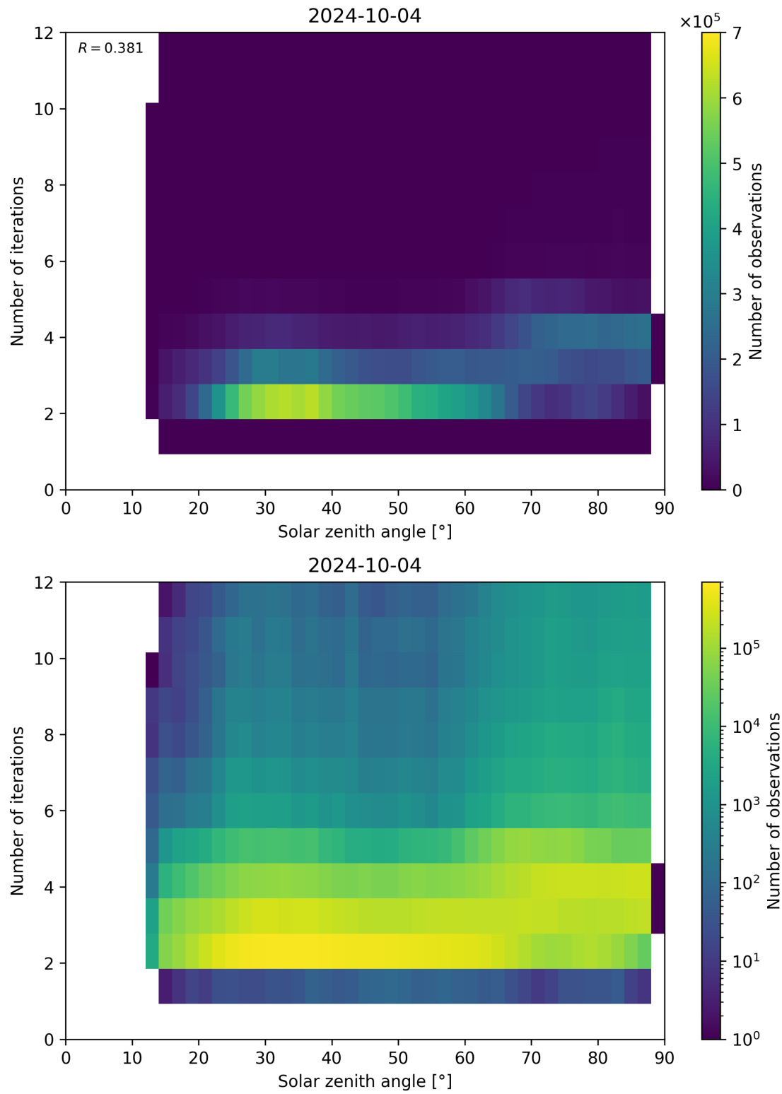
Figure 125: Scatter density plot of “Solar zenith angle” against “Number of iterations” for 2024-10-03 to 2024-10-05.
