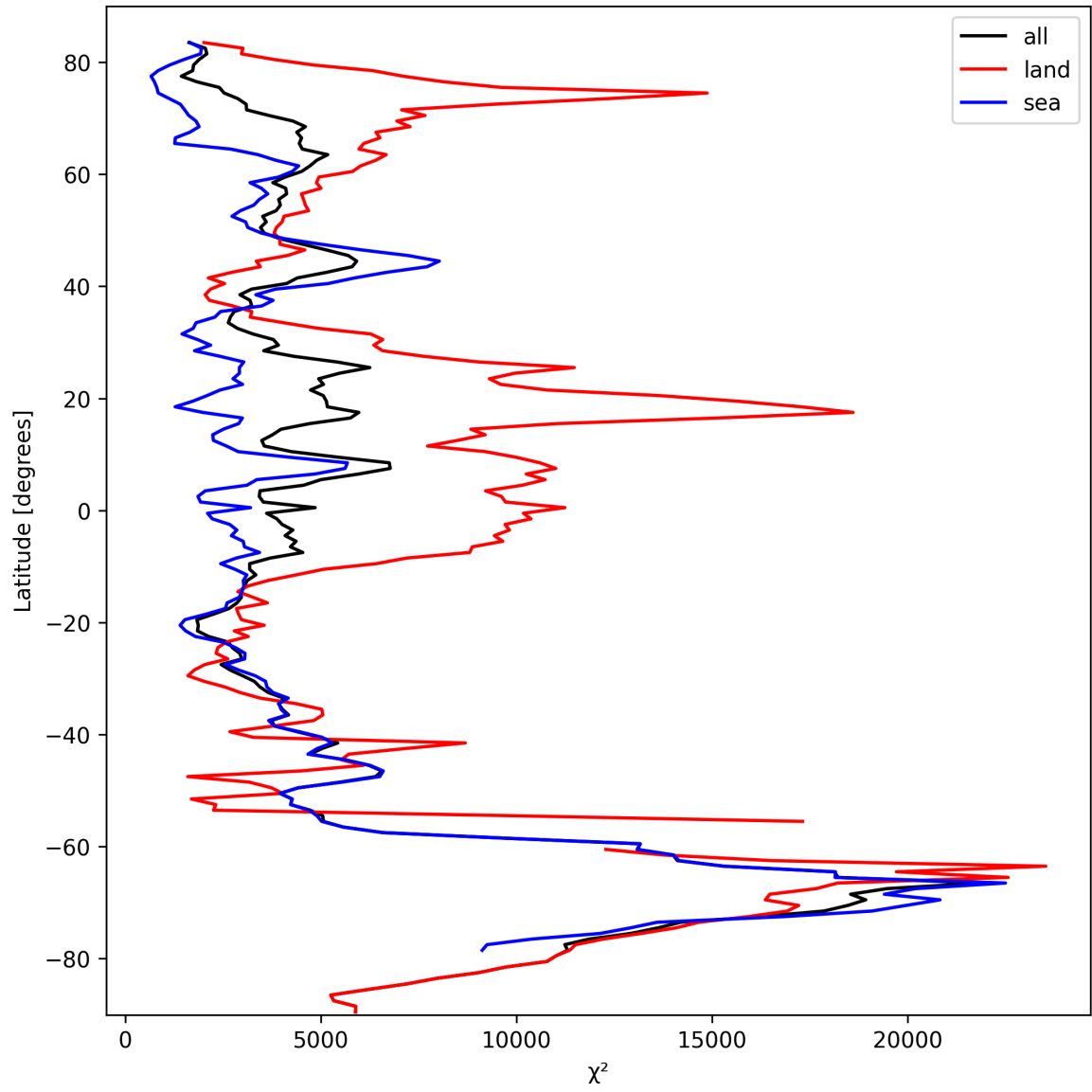
Figure 21: Zonal average of “ \chi^2 ” for 2024-10-03 to 2024-10-05.
