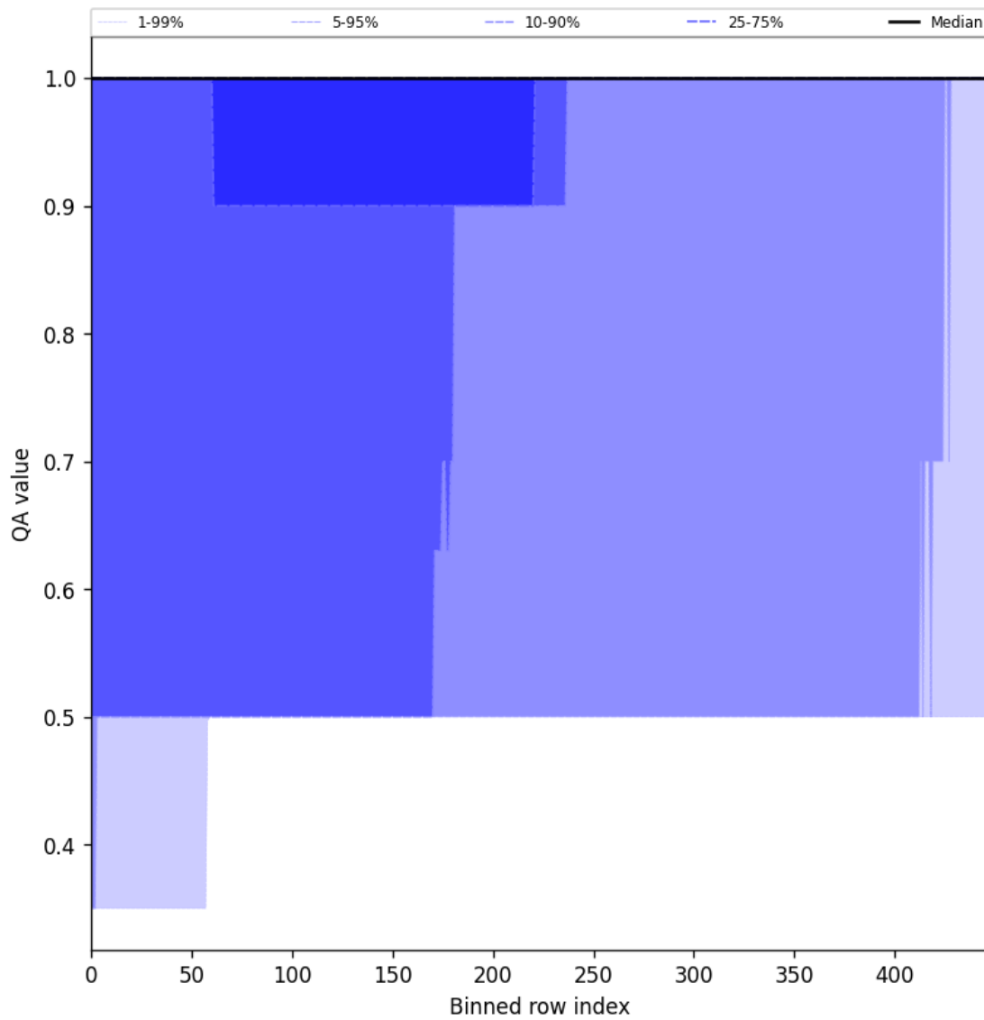
Figure 46: Along track statistics of “QA value” for 2024-10-03 to 2024-10-05
