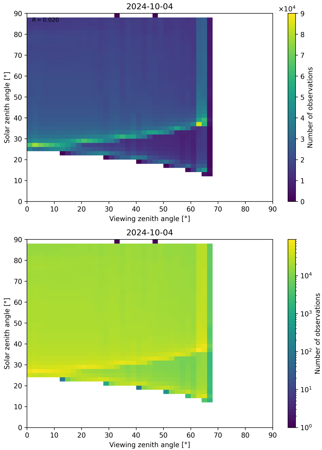
Figure 139: Scatter density plot of “Viewing zenith angle” against “Solar zenith angle” for 2024-10-03 to 2024-10-05.
