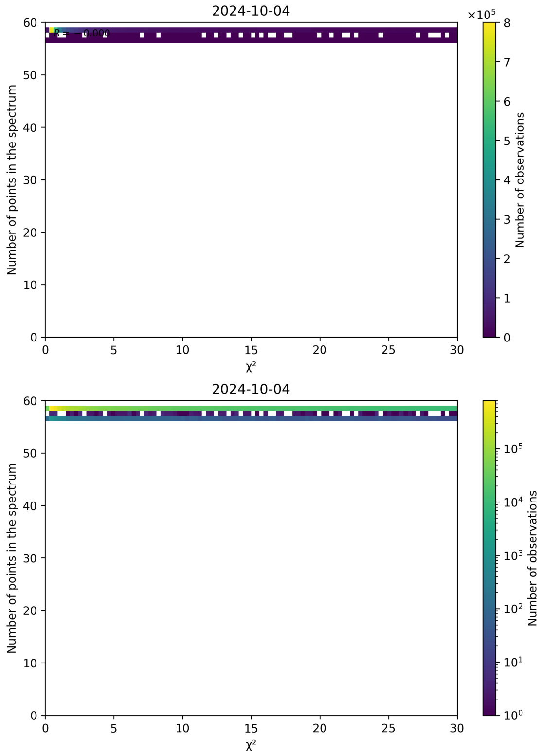
Figure 74: Scatter density plot of " \chi^2 " against "Number of points in the spectrum" for 2024-10-03 to 2024-10-05.
