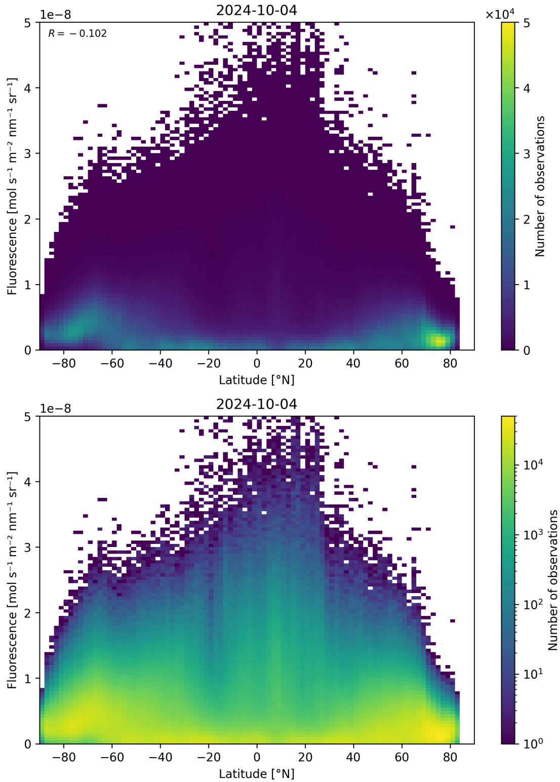
Figure 101: Scatter density plot of “Latitude” against “Fluorescence” for 2024-10-03 to 2024-10-05.
