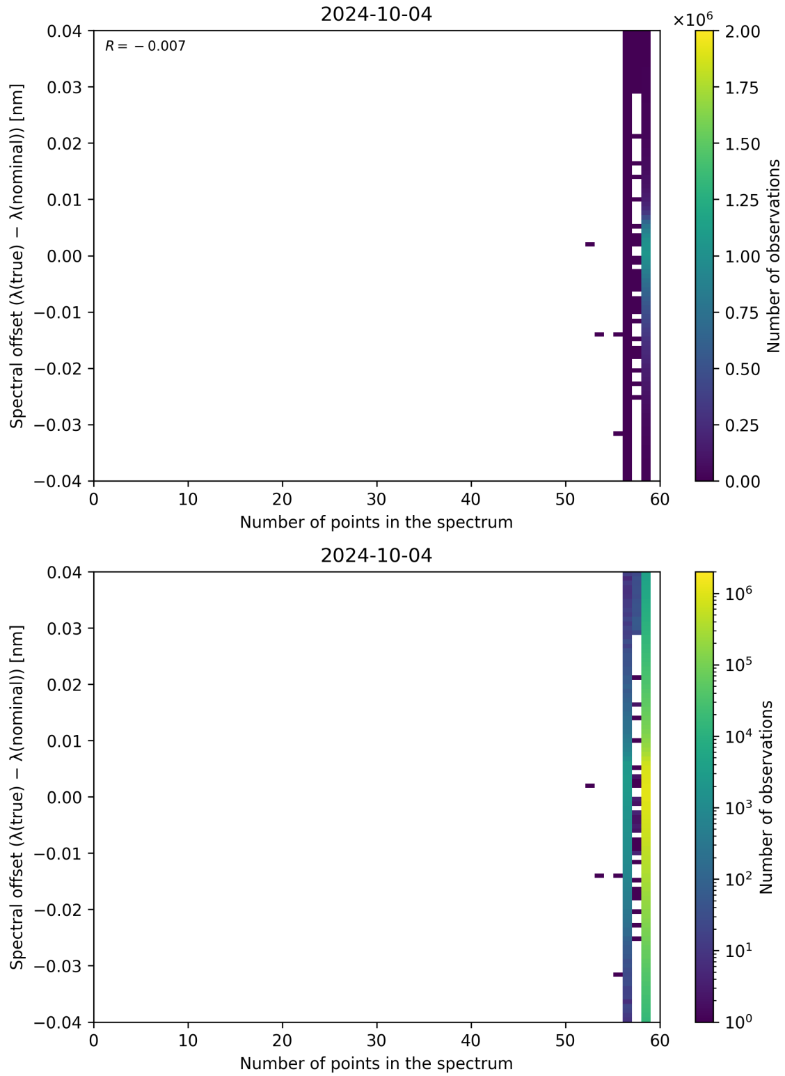
Figure 110: Scatter density plot of “Number of points in the spectrum” against “Spectral offset ( \lambda_{\text{true}} - \lambda_{\text{nominal}} )” for 2024-10-03 to 2024-10-05.
