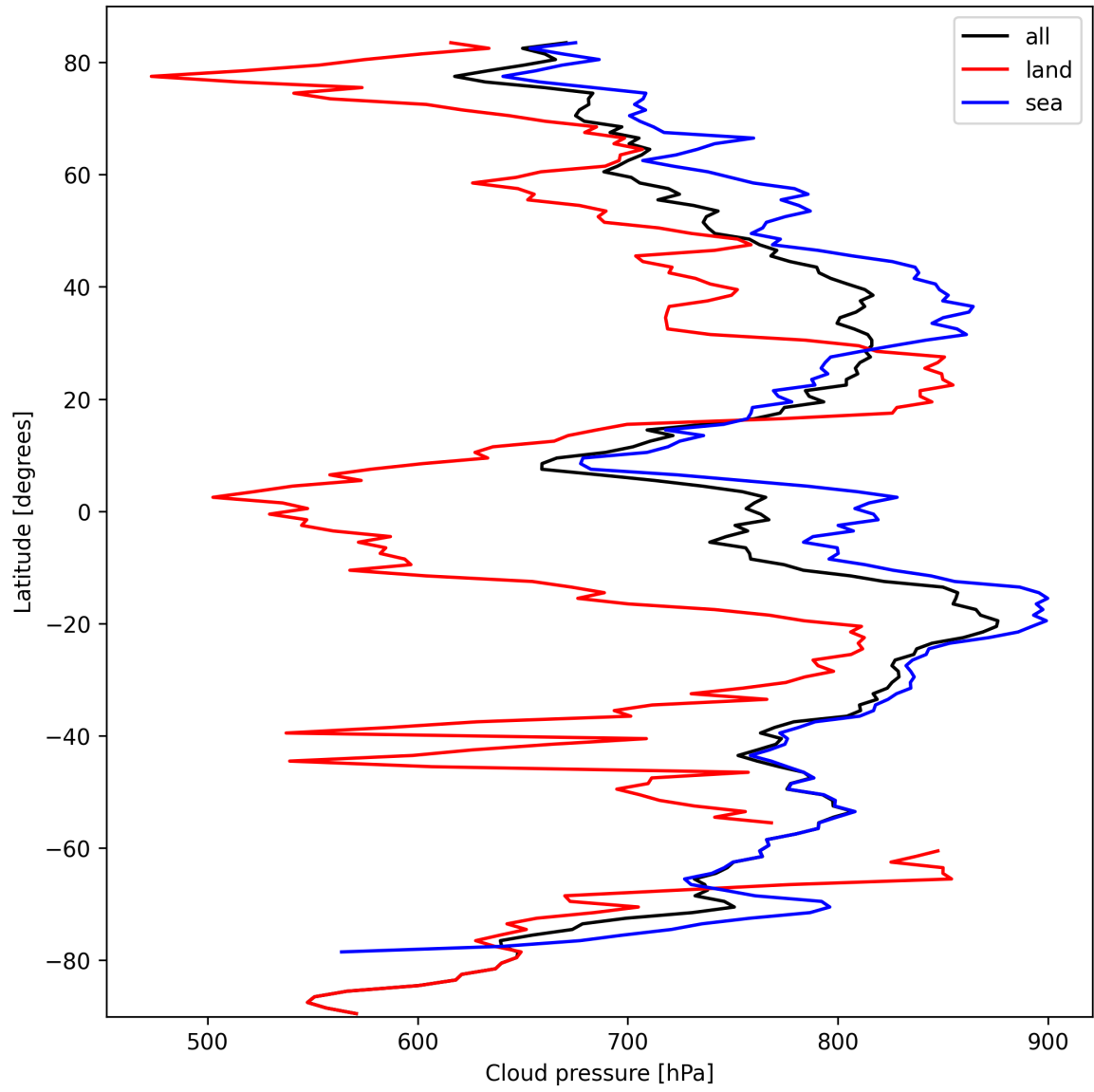
Figure 13: Zonal average of “Cloud pressure” for 2024-10-03 to 2024-10-05.
