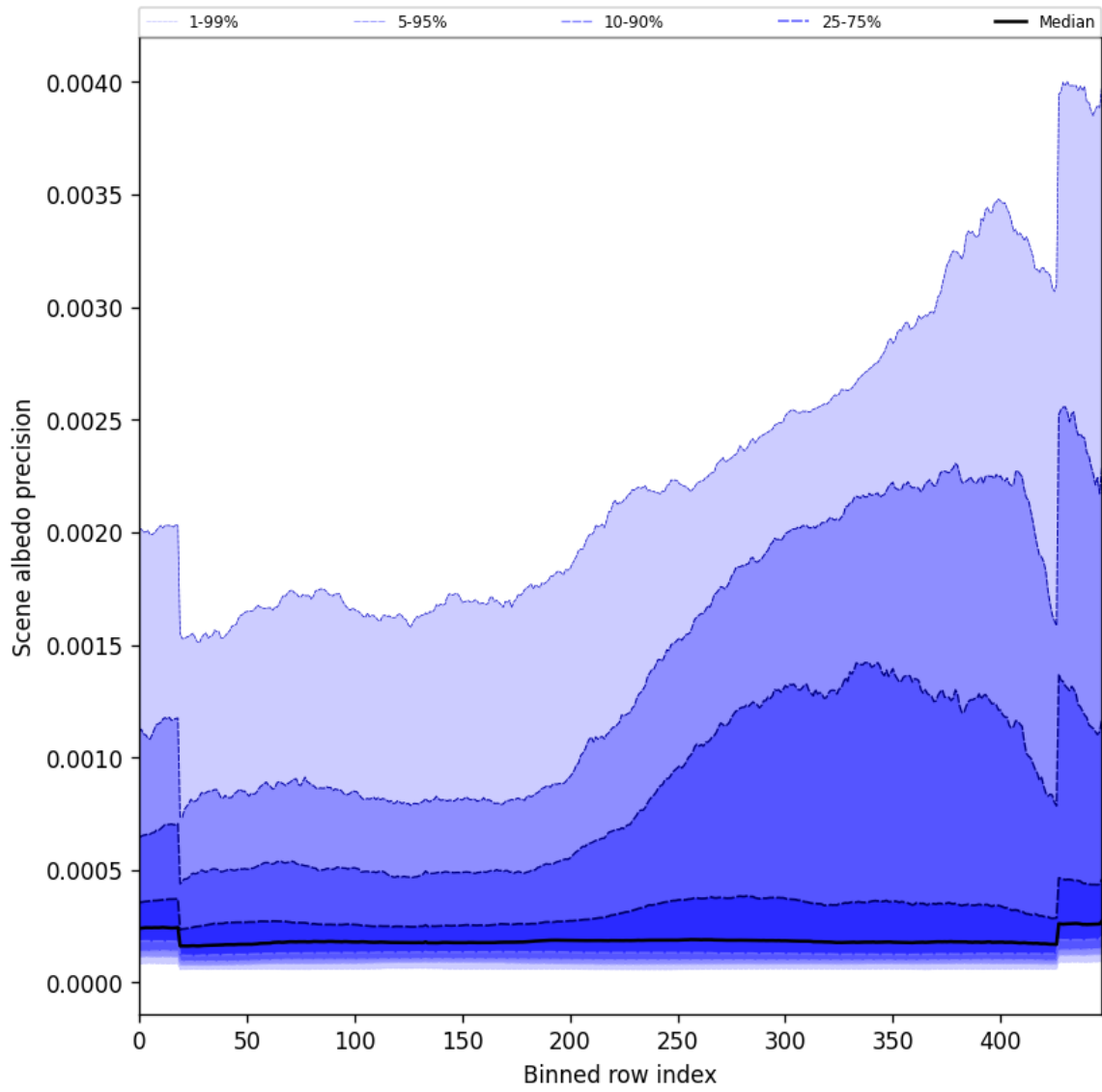
Figure 52: Along track statistics of “Scene albedo precision” for 2024-10-03 to 2024-10-05
