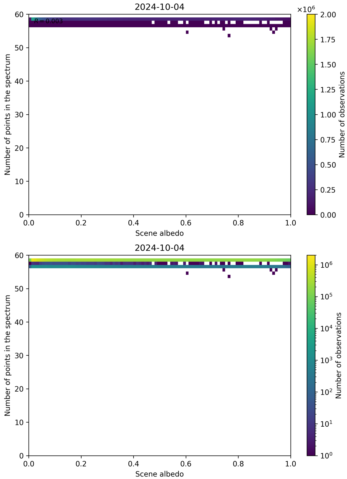
Figure 116: Scatter density plot of “Scene albedo” against “Number of points in the spectrum” for 2024-10-03 to 2024-10-05.
