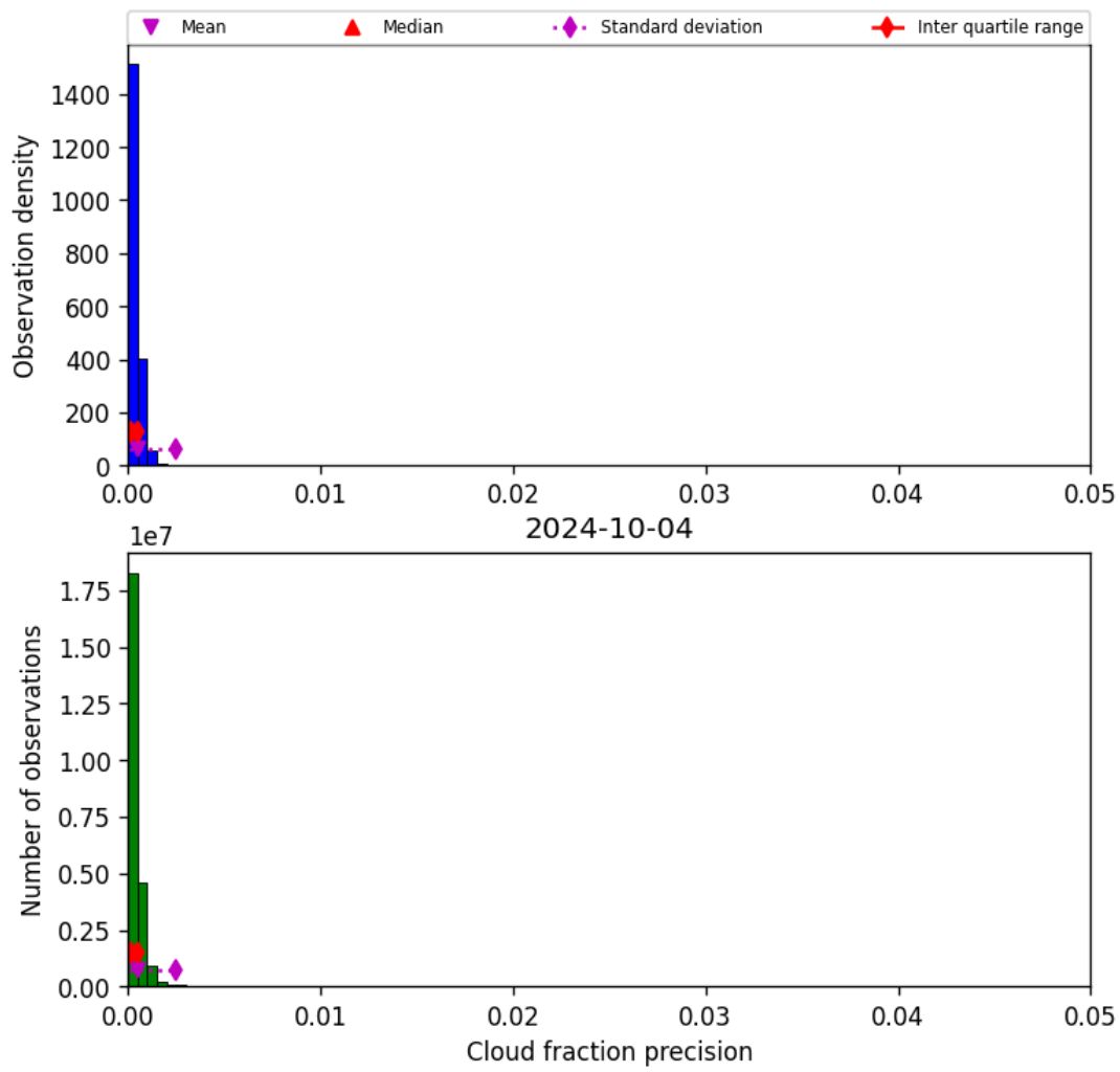
Figure 33: Histogram of “Cloud fraction precision” for 2024-10-03 to 2024-10-05
