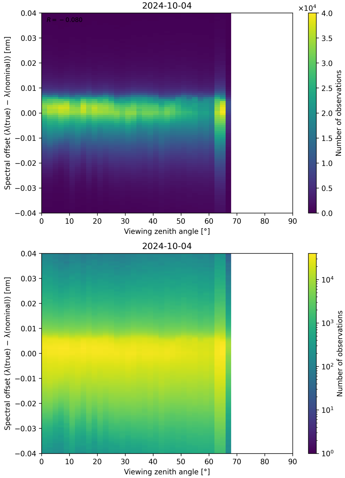
Figure 140: Scatter density plot of “Viewing zenith angle” against “Spectral offset ( \lambda_{\text{true}} - \lambda_{\text{nominal}} )” for 2024-10-03 to 2024-10-05.
