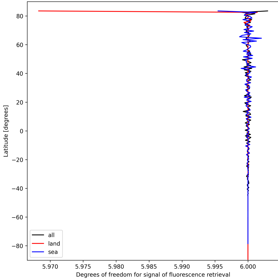
Figure 26: Zonal average of “Degrees of freedom for signal of fluorescence retrieval” for 2024-10-03 to 2024-10-05.
