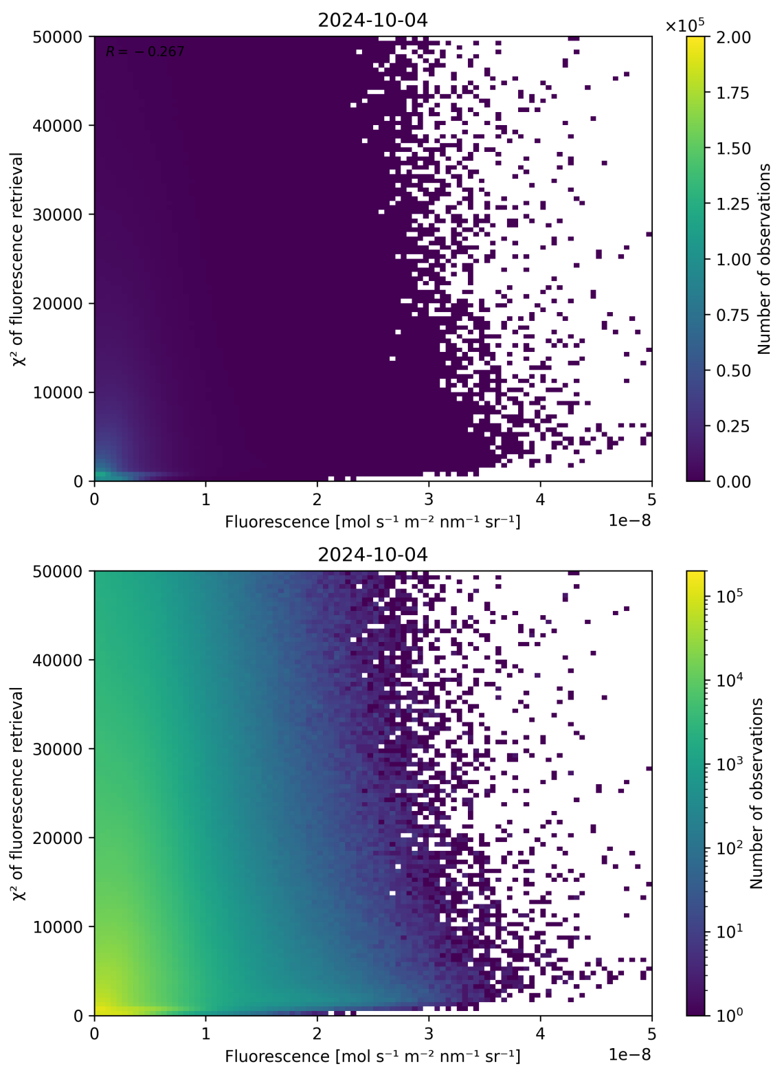
Figure 93: Scatter density plot of “Fluorescence” against “ \chi^2 of fluorescence retrieval” for 2024-10-03 to 2024-10-05.
