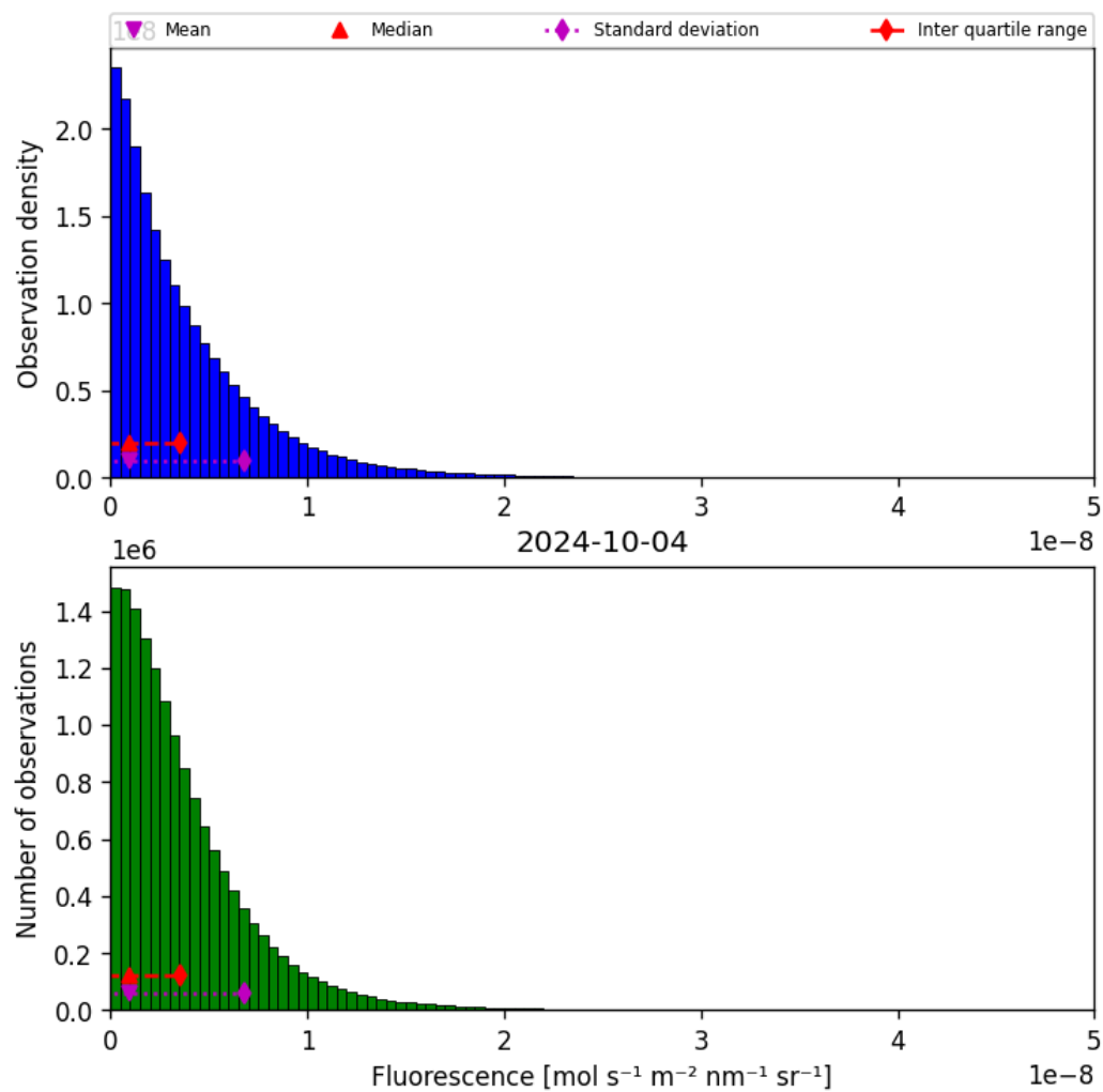
Figure 40: Histogram of “Fluorescence” for 2024-10-03 to 2024-10-05
