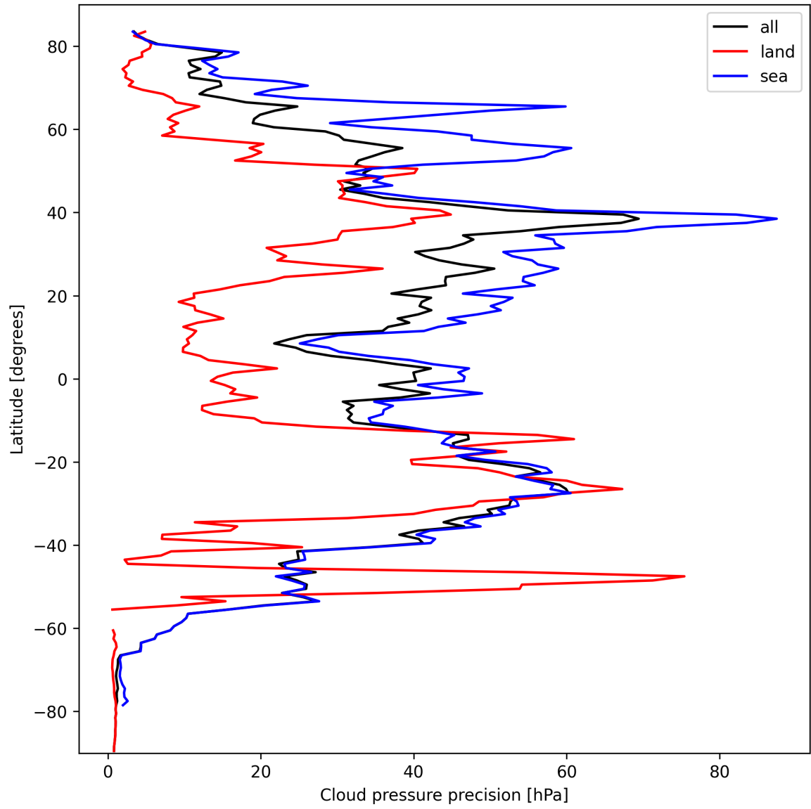
Figure 14: Zonal average of “Cloud pressure precision” for 2024-10-03 to 2024-10-05.
