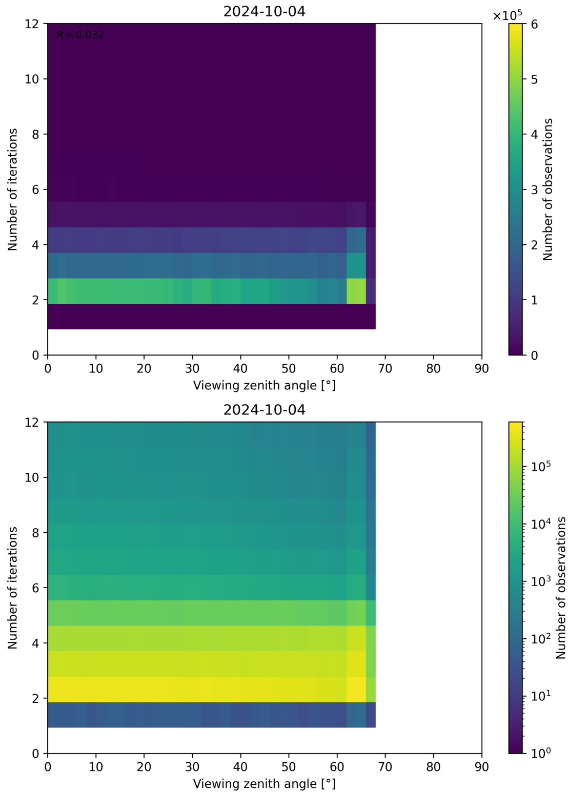
Figure 136: Scatter density plot of “Viewing zenith angle” against “Number of iterations” for 2024-10-03 to 2024-10-05.
