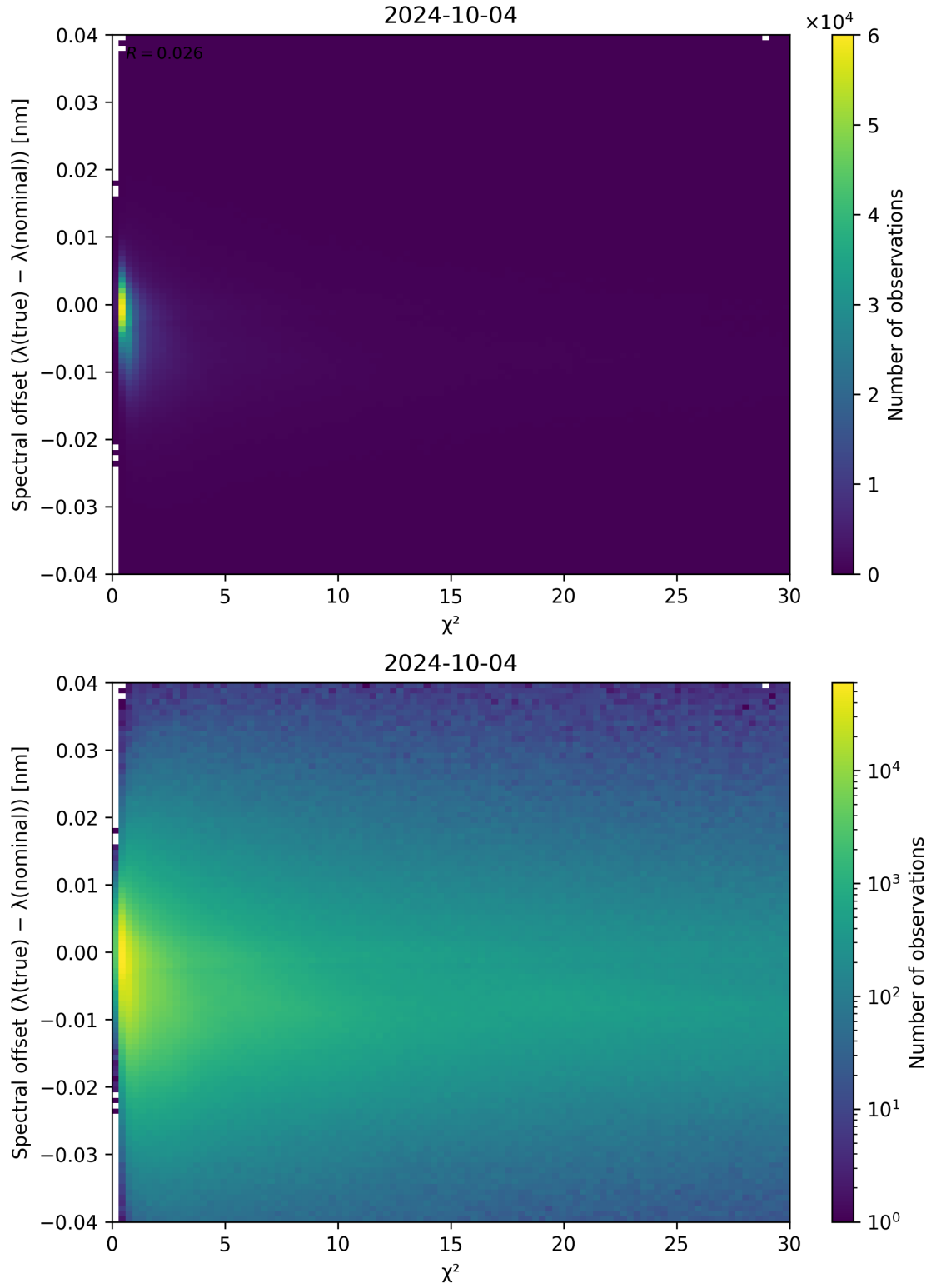
Figure 75: Scatter density plot of “ \chi^2 ” against “Spectral offset ( \lambda_{\text{true}} - \lambda_{\text{nominal}} )” for 2024-10-03 to 2024-10-05.
