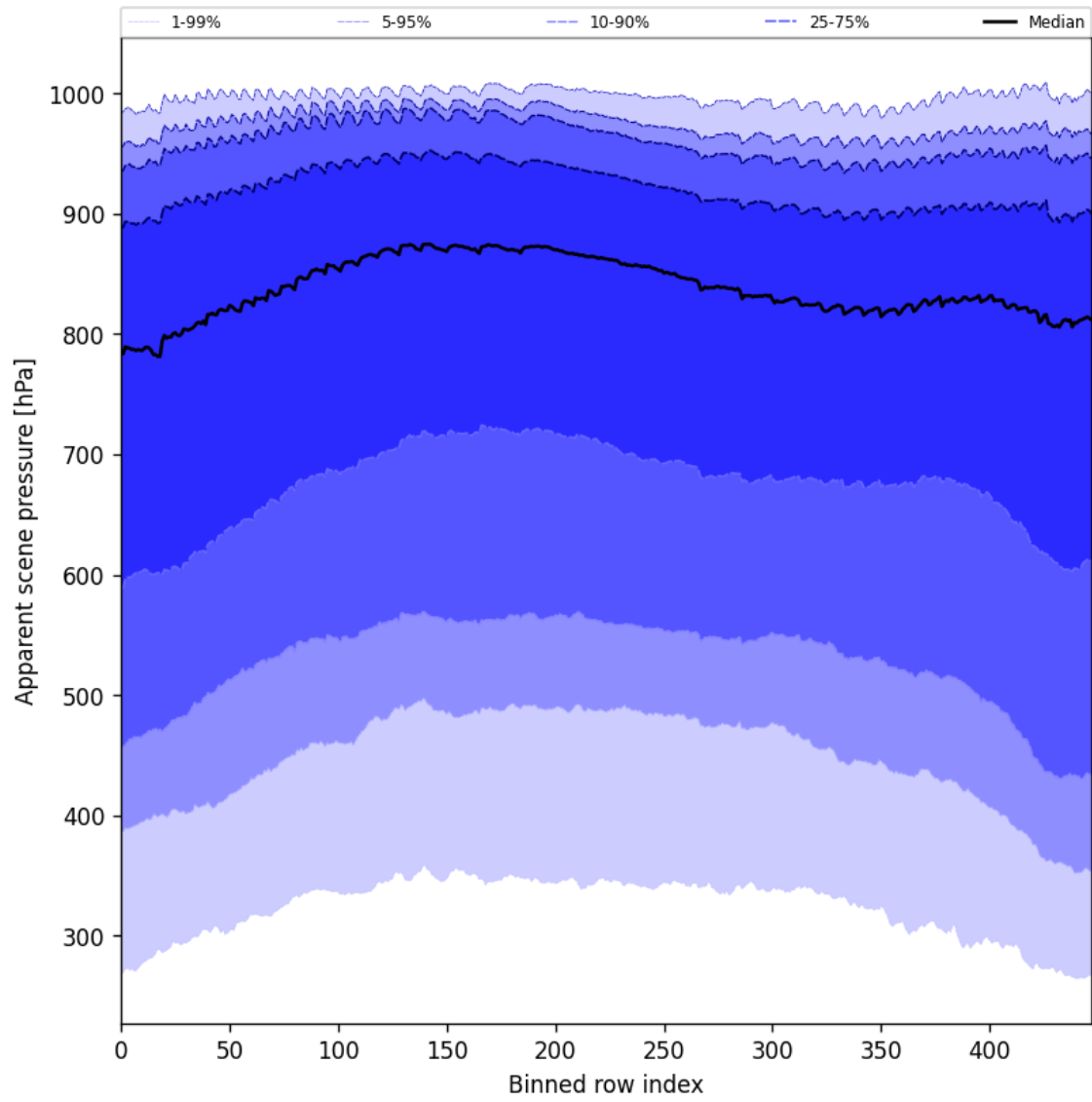
Figure 53: Along track statistics of “Apparent scene pressure” for 2024-10-03 to 2024-10-05
