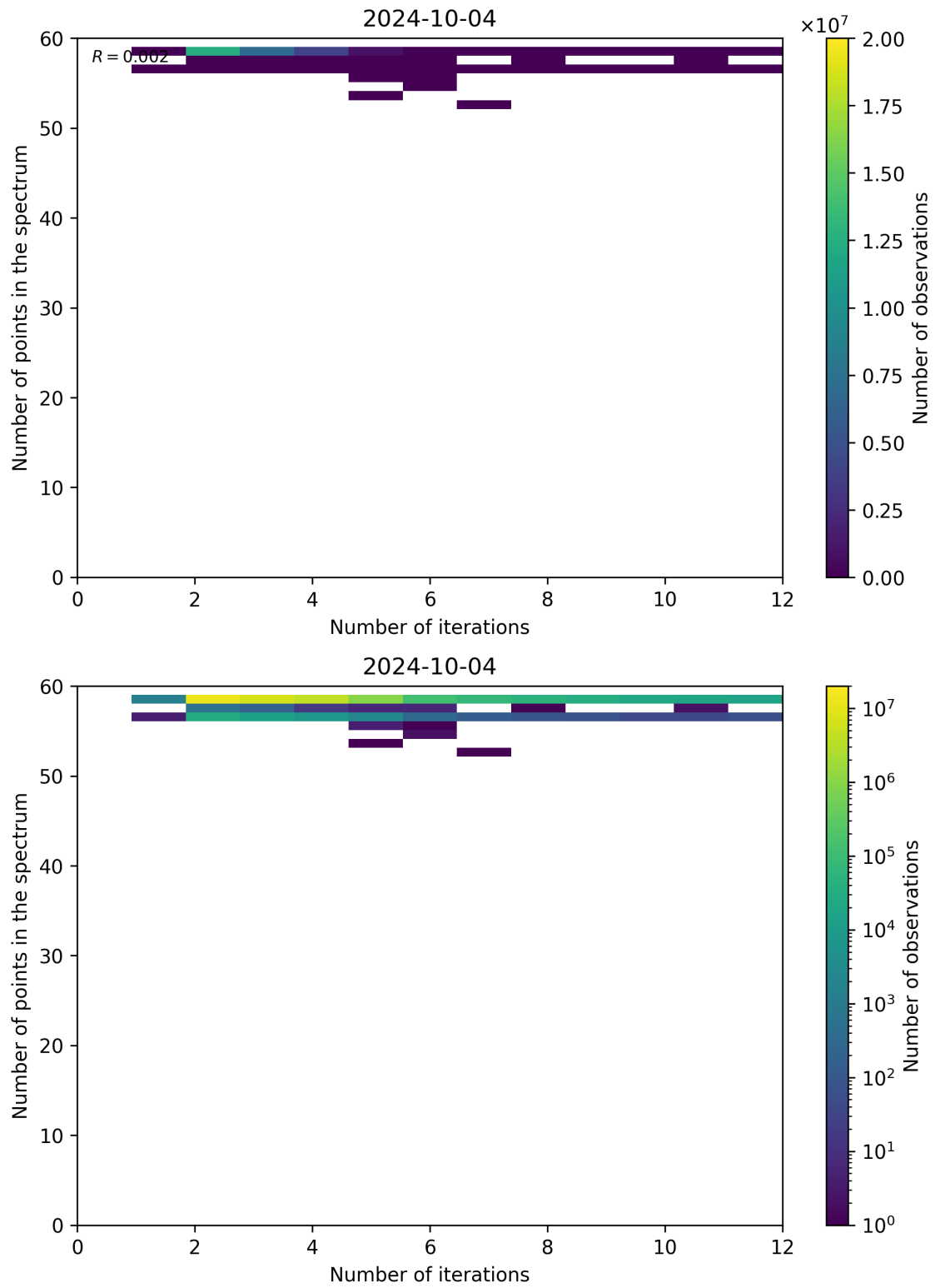
Figure 108: Scatter density plot of “Number of iterations” against “Number of points in the spectrum” for 2024-10-03 to 2024-10-05.
