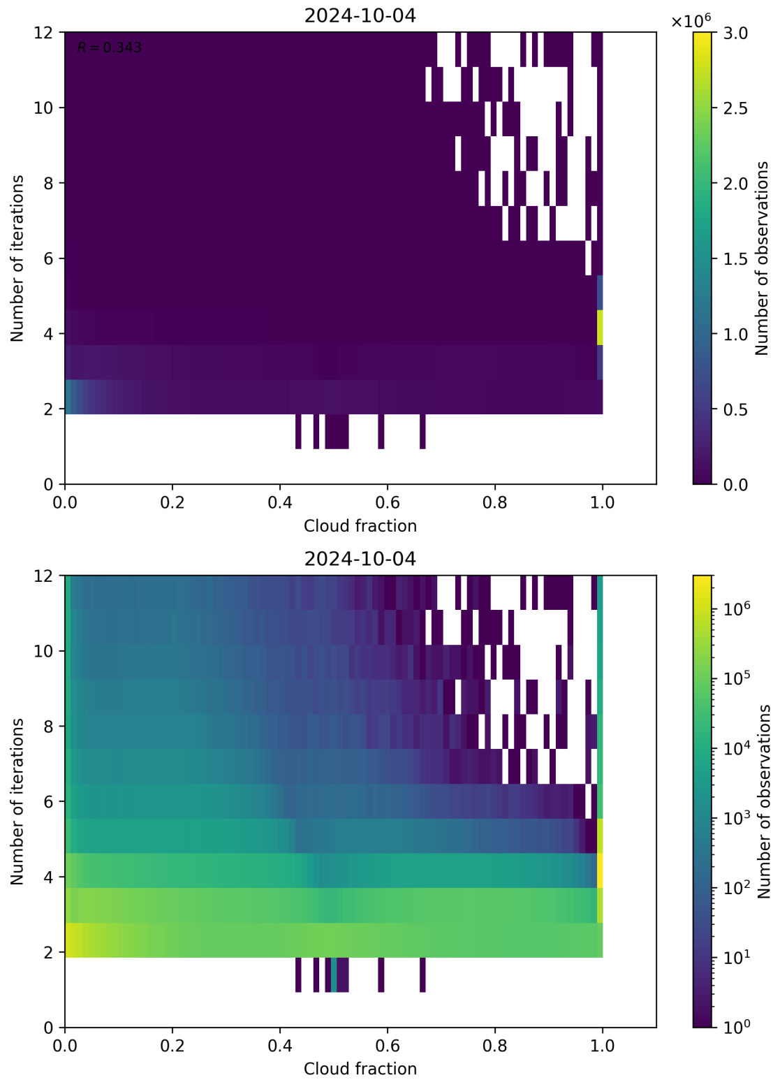
Figure 80: Scatter density plot of “Cloud fraction” against “Number of iterations” for 2024-10-03 to 2024-10-05.
