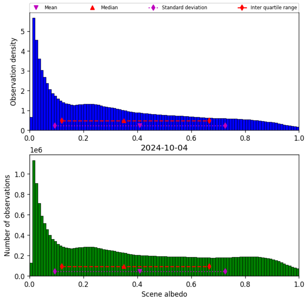
Figure 34: Histogram of “Scene albedo” for 2024-10-03 to 2024-10-05
