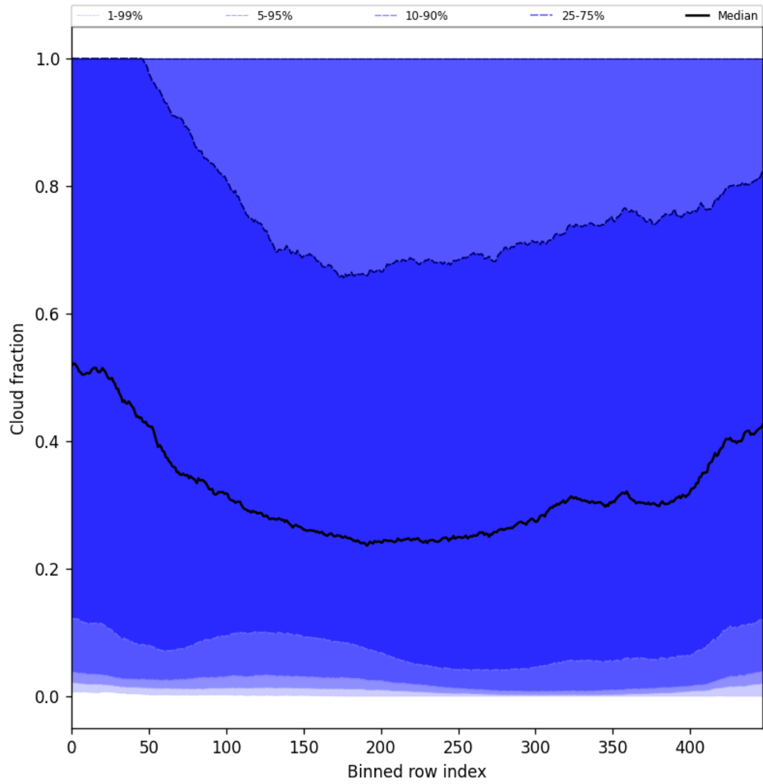
Figure 49: Along track statistics of “Cloud fraction” for 2024-10-03 to 2024-10-05
