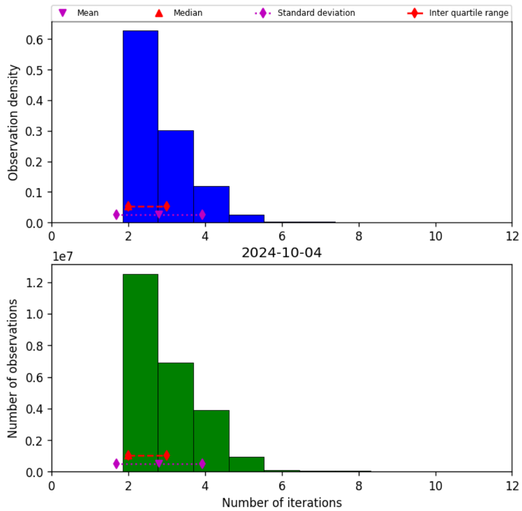
Figure 39: Histogram of “Number of iterations” for 2024-10-03 to 2024-10-05
