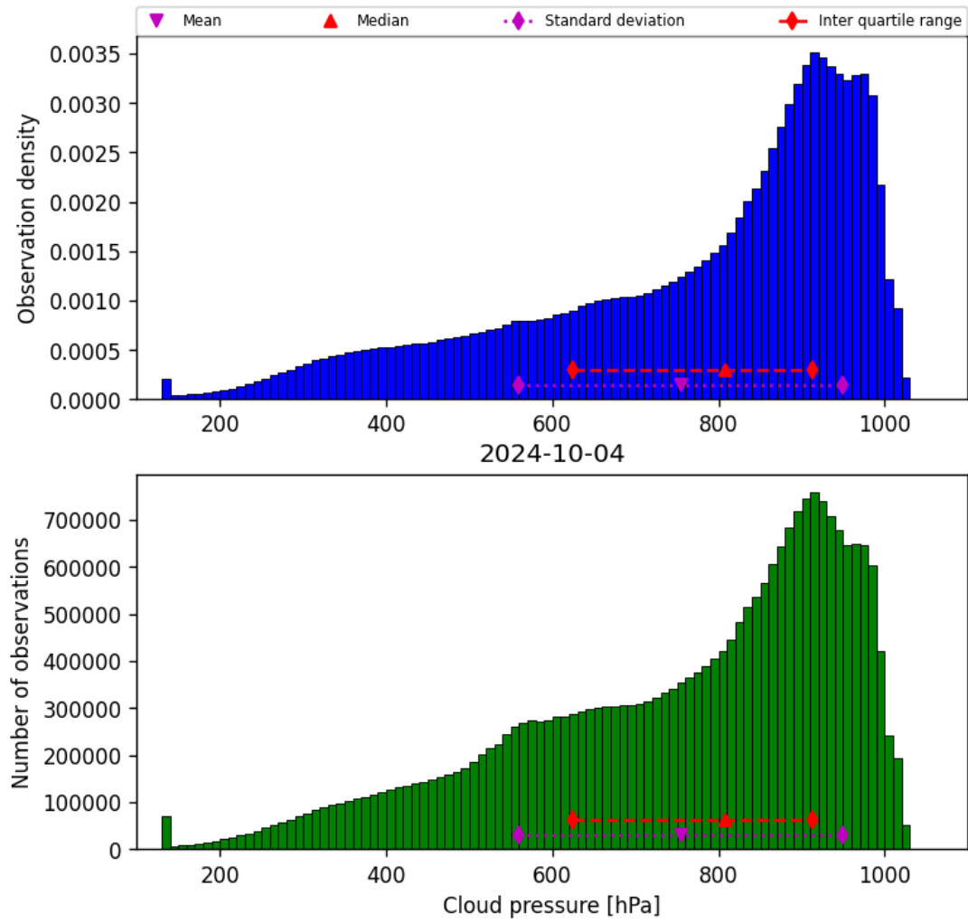
Figure 30: Histogram of “Cloud pressure” for 2024-10-03 to 2024-10-05
