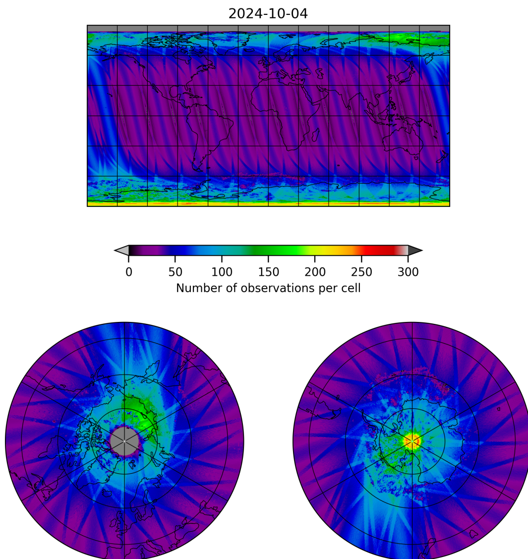
Figure 11: Map of the number of observations for 2024-10-03 to 2024-10-05
