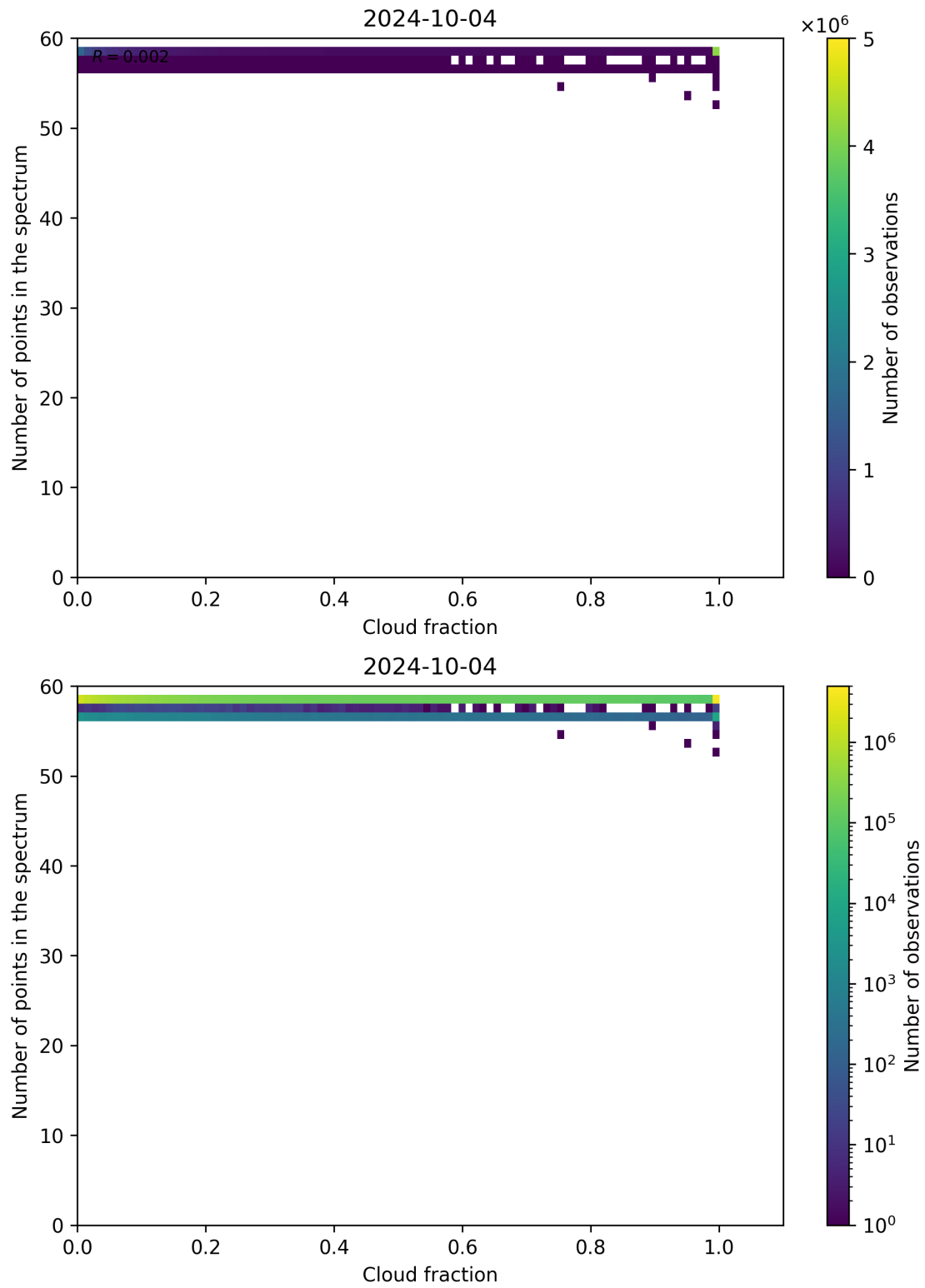
Figure 81: Scatter density plot of “Cloud fraction” against “Number of points in the spectrum” for 2024-10-03 to 2024-10-05.
