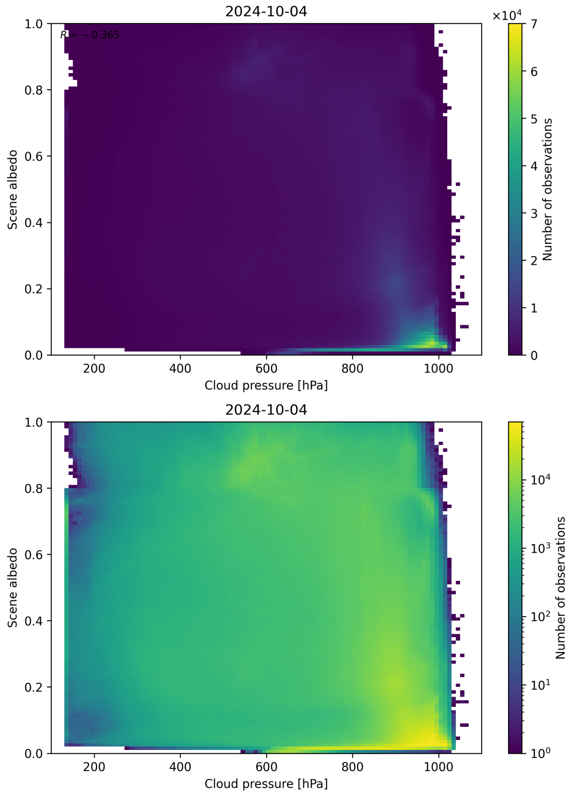
Figure 91: Scatter density plot of “Cloud pressure” against “Scene albedo” for 2024-10-03 to 2024-10-05.
