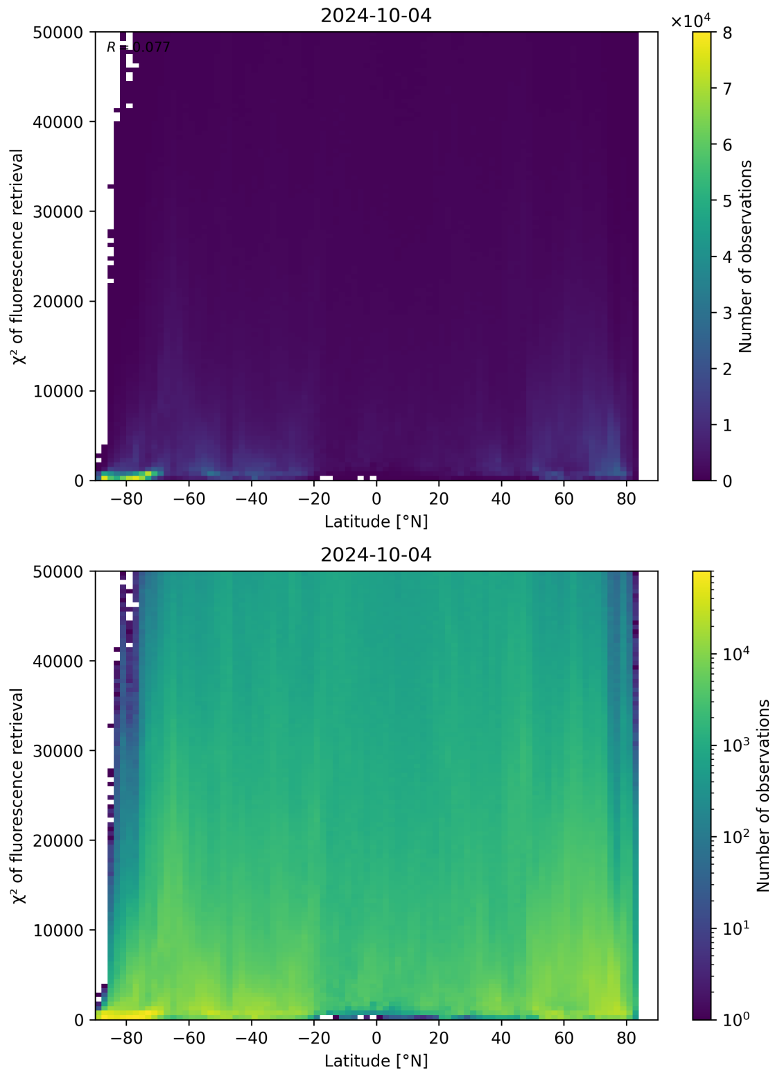
Figure 98: Scatter density plot of “Latitude” against “ \chi^2 of fluorescence retrieval” for 2024-10-03 to 2024-10-05.
