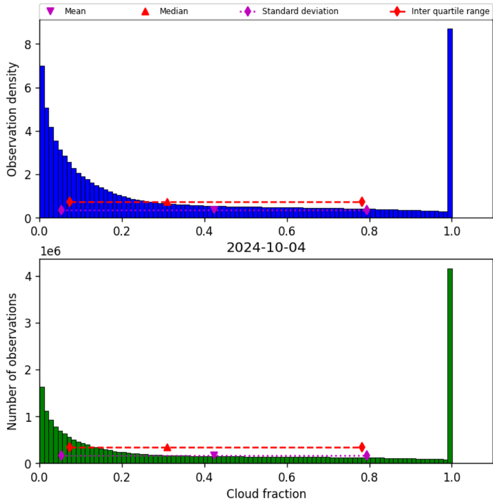
Figure 32: Histogram of “Cloud fraction” for 2024-10-03 to 2024-10-05
