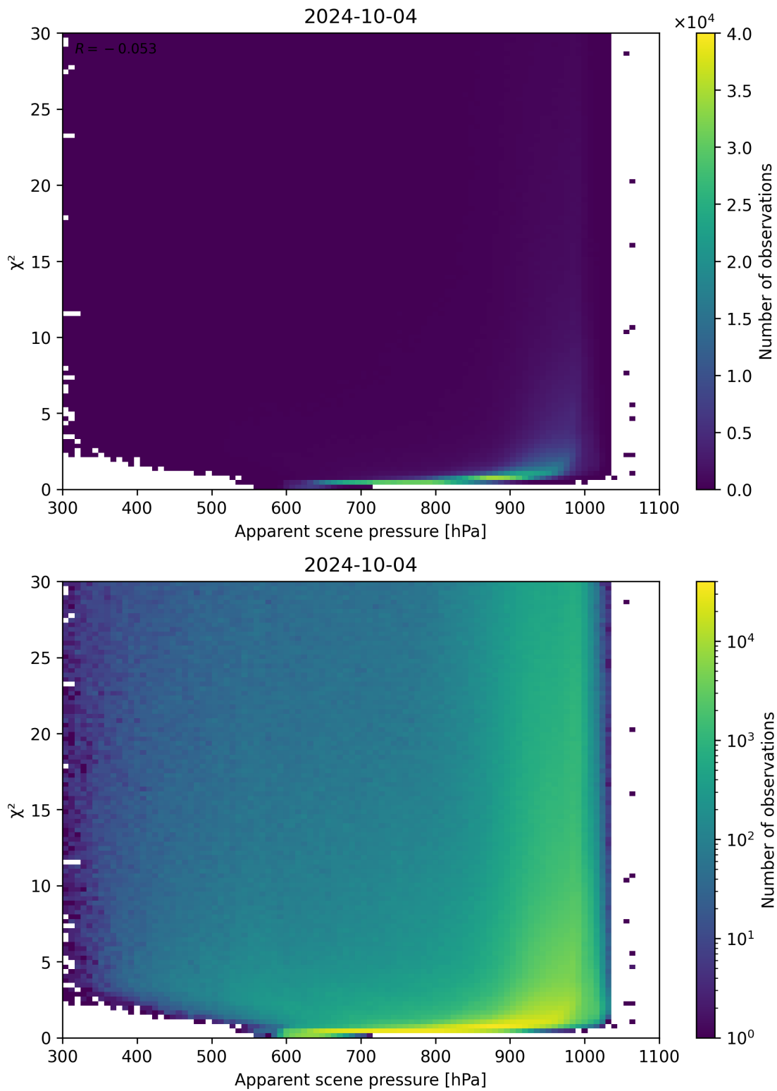
Figure 63: Scatter density plot of “Apparent scene pressure” against “ \chi^2 ” for 2024-10-03 to 2024-10-05.
