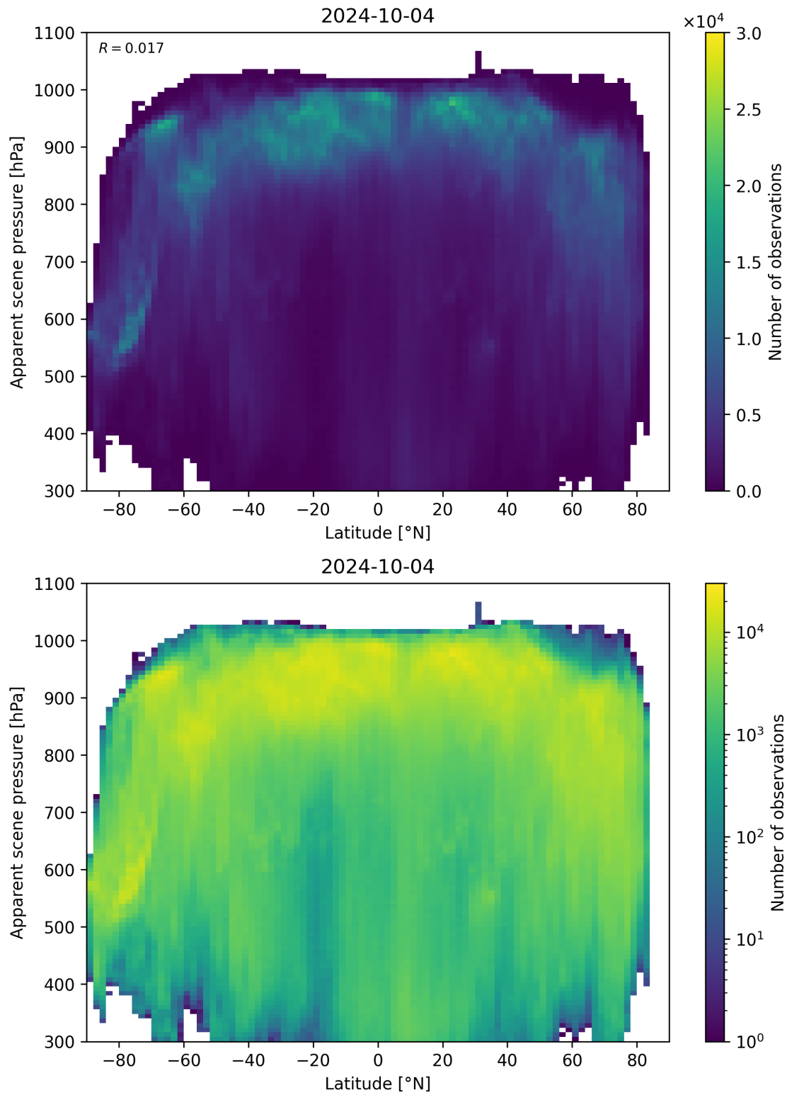
Figure 96: Scatter density plot of “Latitude” against “Apparent scene pressure” for 2024-10-03 to 2024-10-05.
