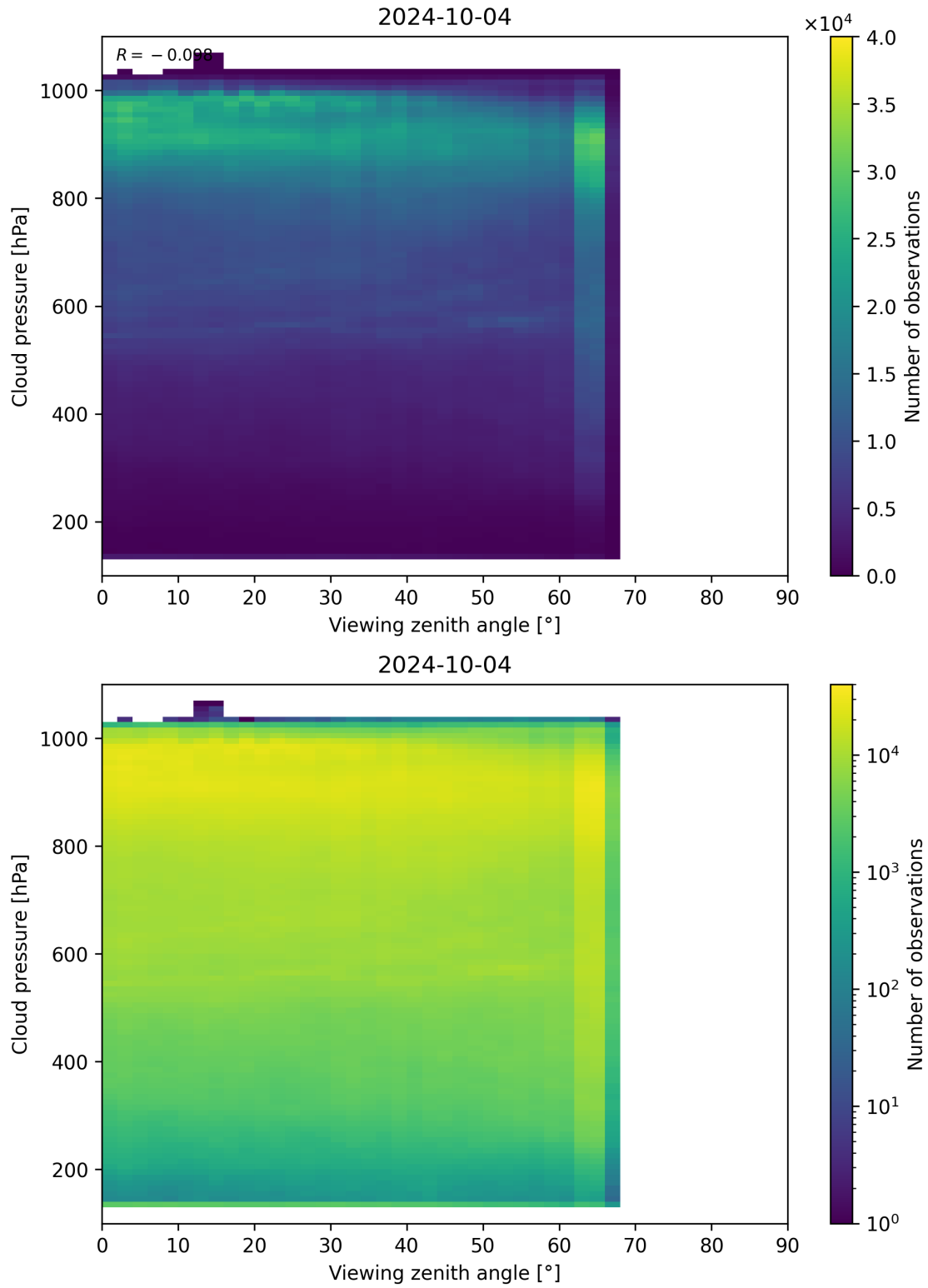
Figure 133: Scatter density plot of “Viewing zenith angle” against “Cloud pressure” for 2024-10-03 to 2024-10-05.
