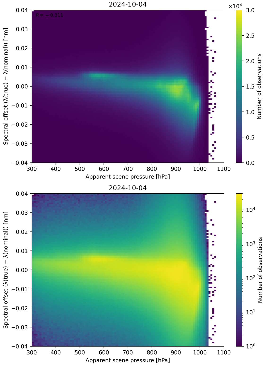
Figure 68: Scatter density plot of “Apparent scene pressure” against “Spectral offset ( \lambda_{\text{true}} - \lambda_{\text{nominal}} )” for 2024-10-03 to 2024-10-05.
