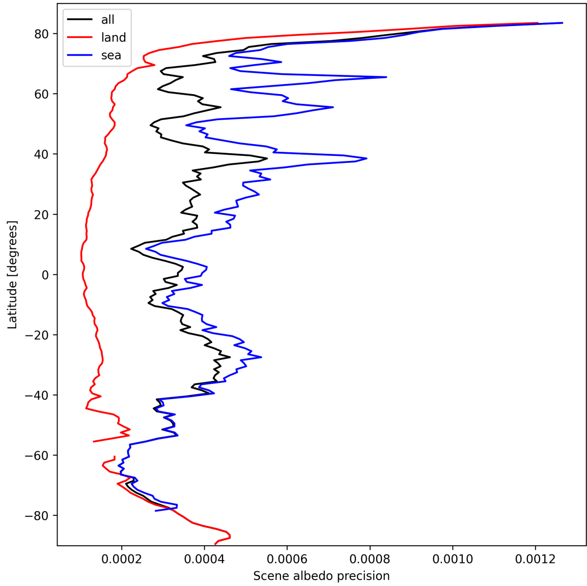
Figure 18: Zonal average of “Scene albedo precision” for 2024-10-03 to 2024-10-05.
