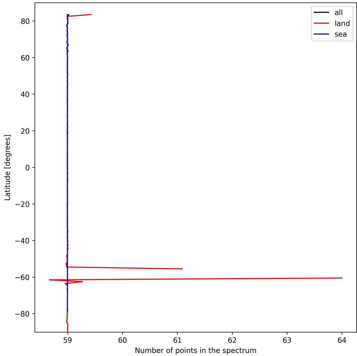
Figure 27: Zonal average of “Number of points in the spectrum” for 2024-10-03 to 2024-10-05.
