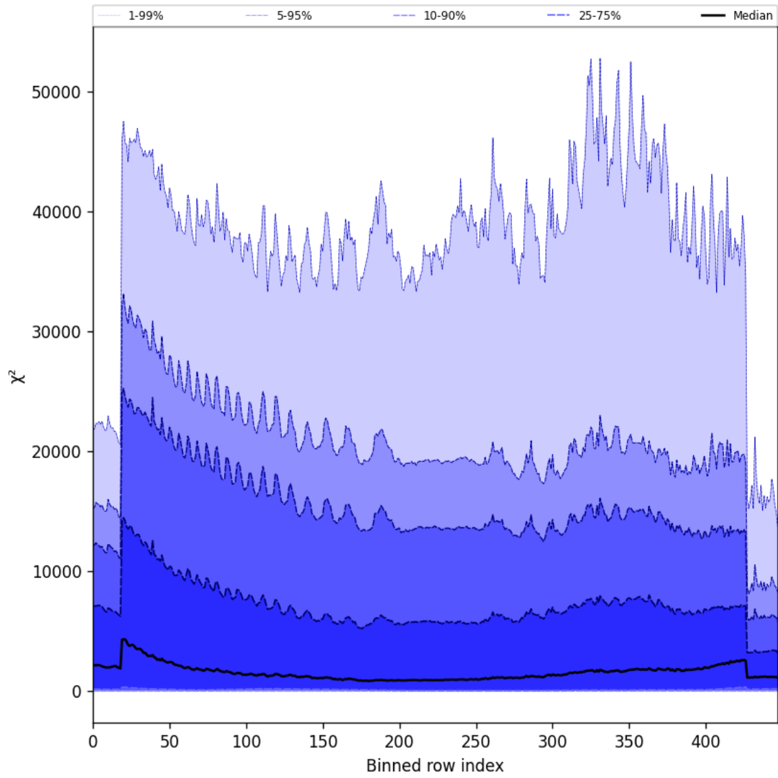
Figure 55: Along track statistics of “ \chi^2 ” for 2024-10-03 to 2024-10-05
