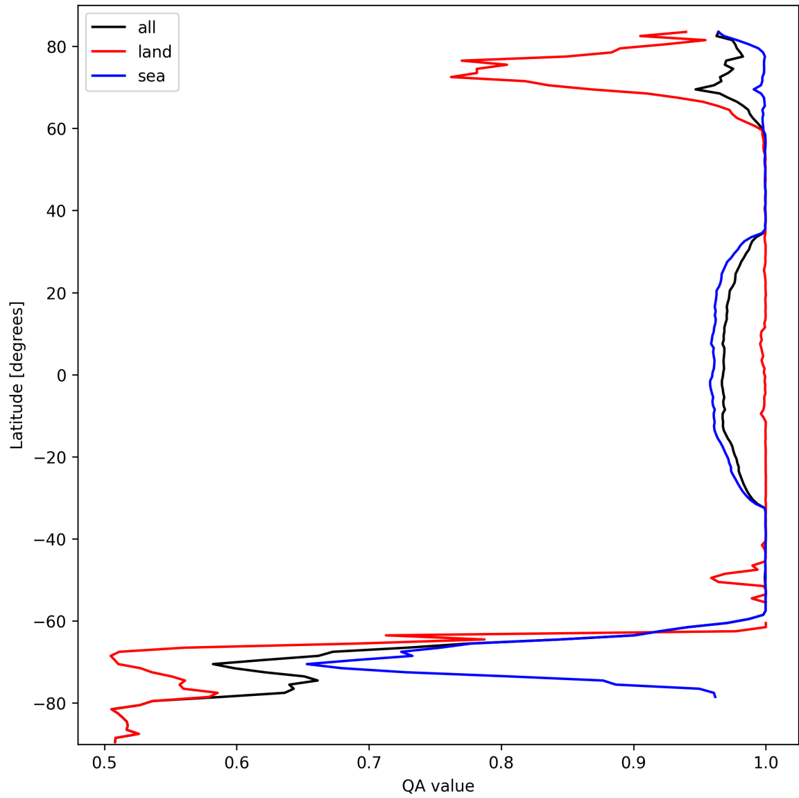
Figure 12: Zonal average of “QA value” for 2024-10-03 to 2024-10-05.
