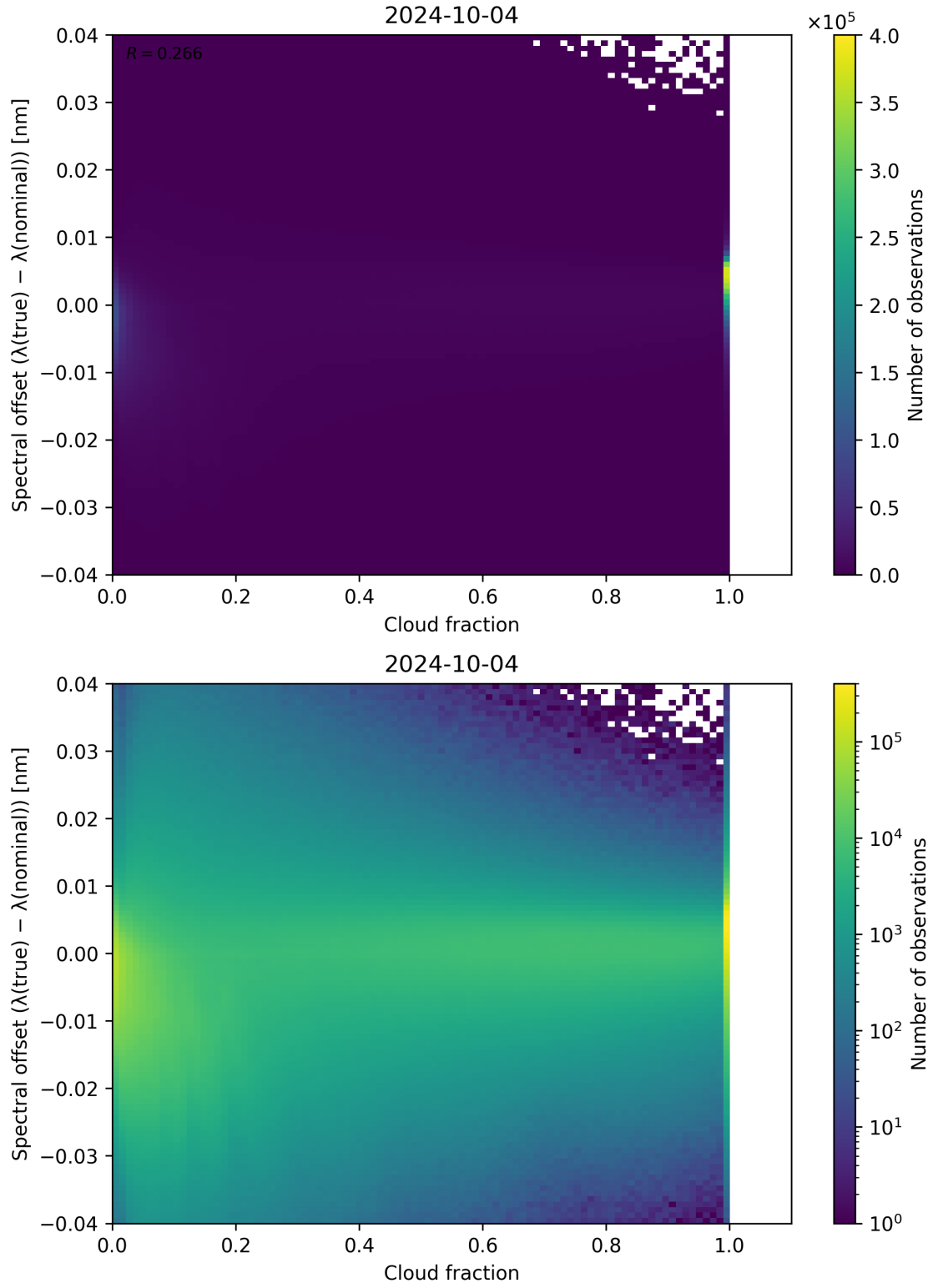
Figure 83: Scatter density plot of “Cloud fraction” against “Spectral offset ( \lambda_{\text{true}} - \lambda_{\text{nominal}} )” for 2024-10-03 to 2024-10-05.
