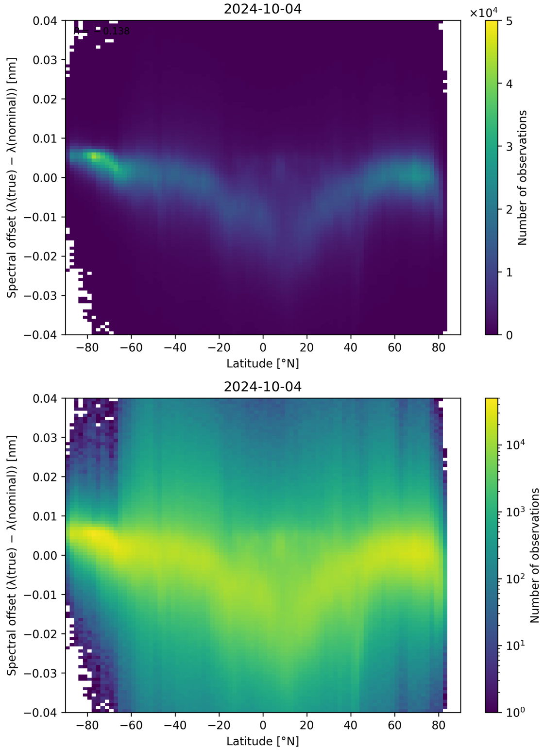
Figure 105: Scatter density plot of “Latitude” against “Spectral offset ( \lambda_{\text{true}} - \lambda_{\text{nominal}} )” for 2024-10-03 to 2024-10-05.
