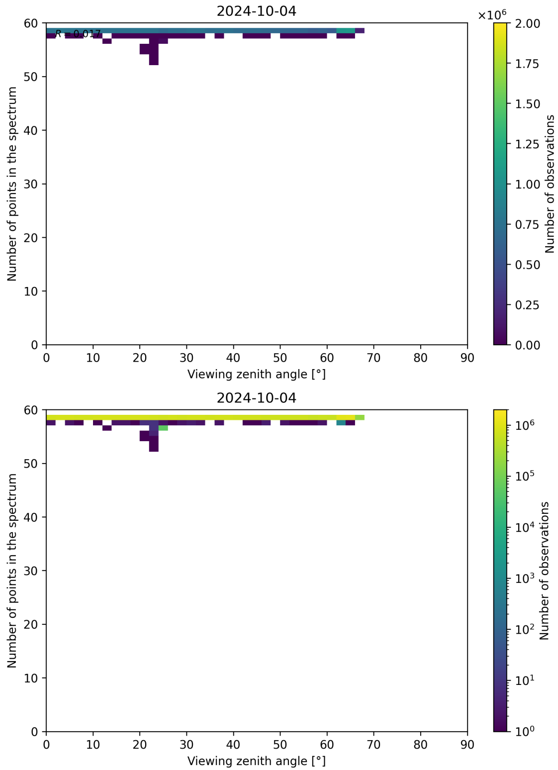
Figure 137: Scatter density plot of “Viewing zenith angle” against “Number of points in the spectrum” for 2024-10-03 to 2024-10-05.
