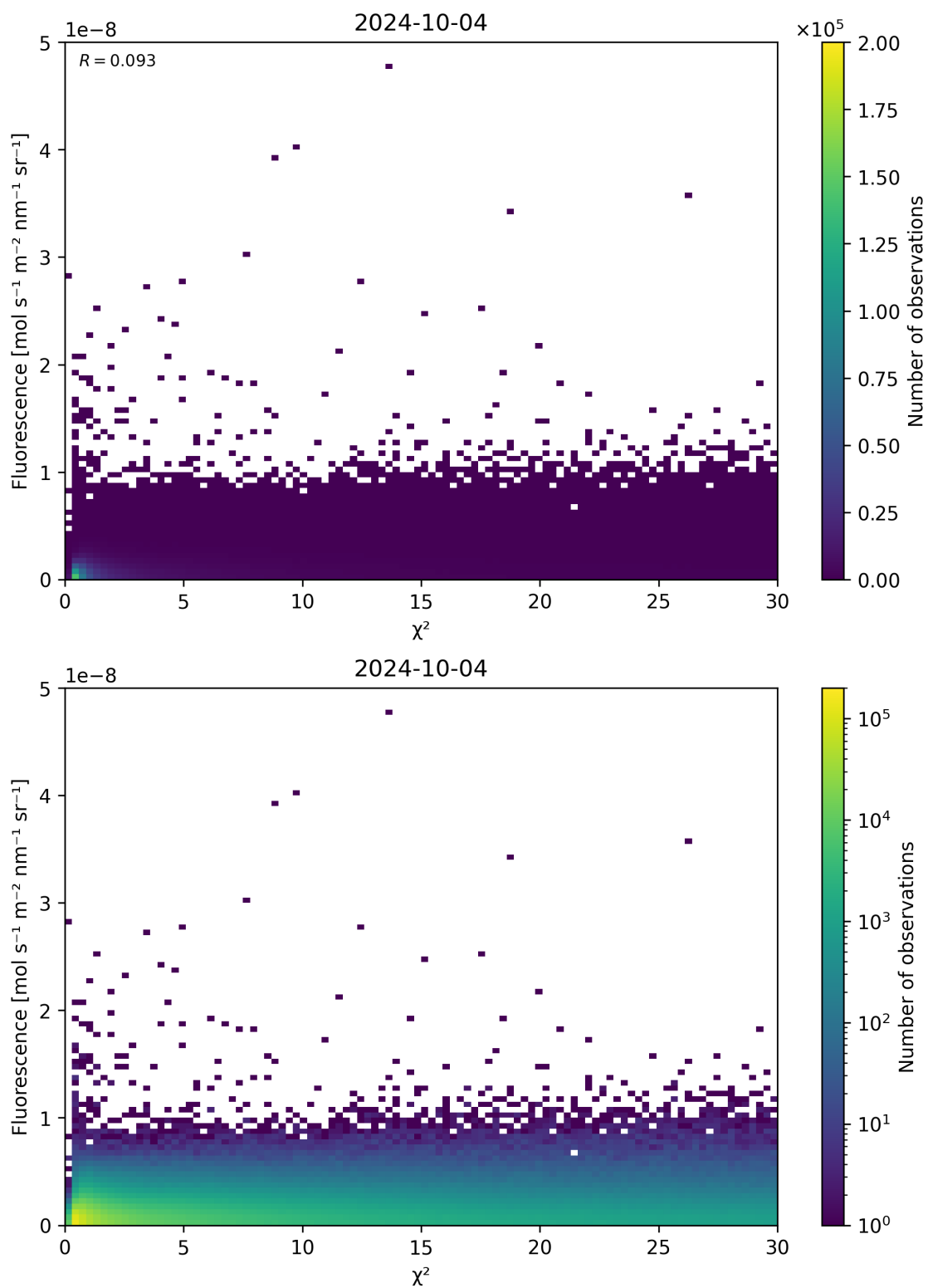
Figure 70: Scatter density plot of “ \chi^2 ” against “Fluorescence” for 2024-10-03 to 2024-10-05.
