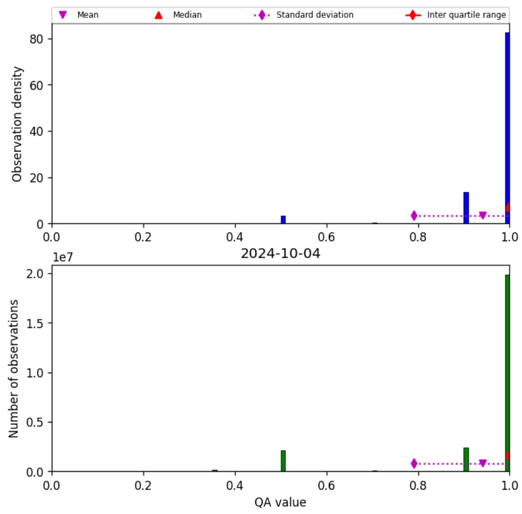
Figure 29: Histogram of “QA value” for 2024-10-03 to 2024-10-05
