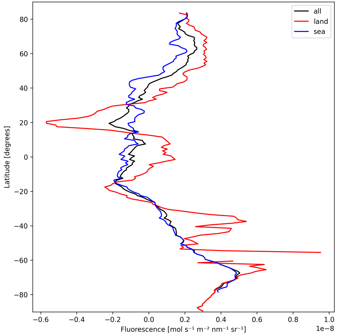
Figure 23: Zonal average of “Fluorescence” for 2024-10-03 to 2024-10-05.
