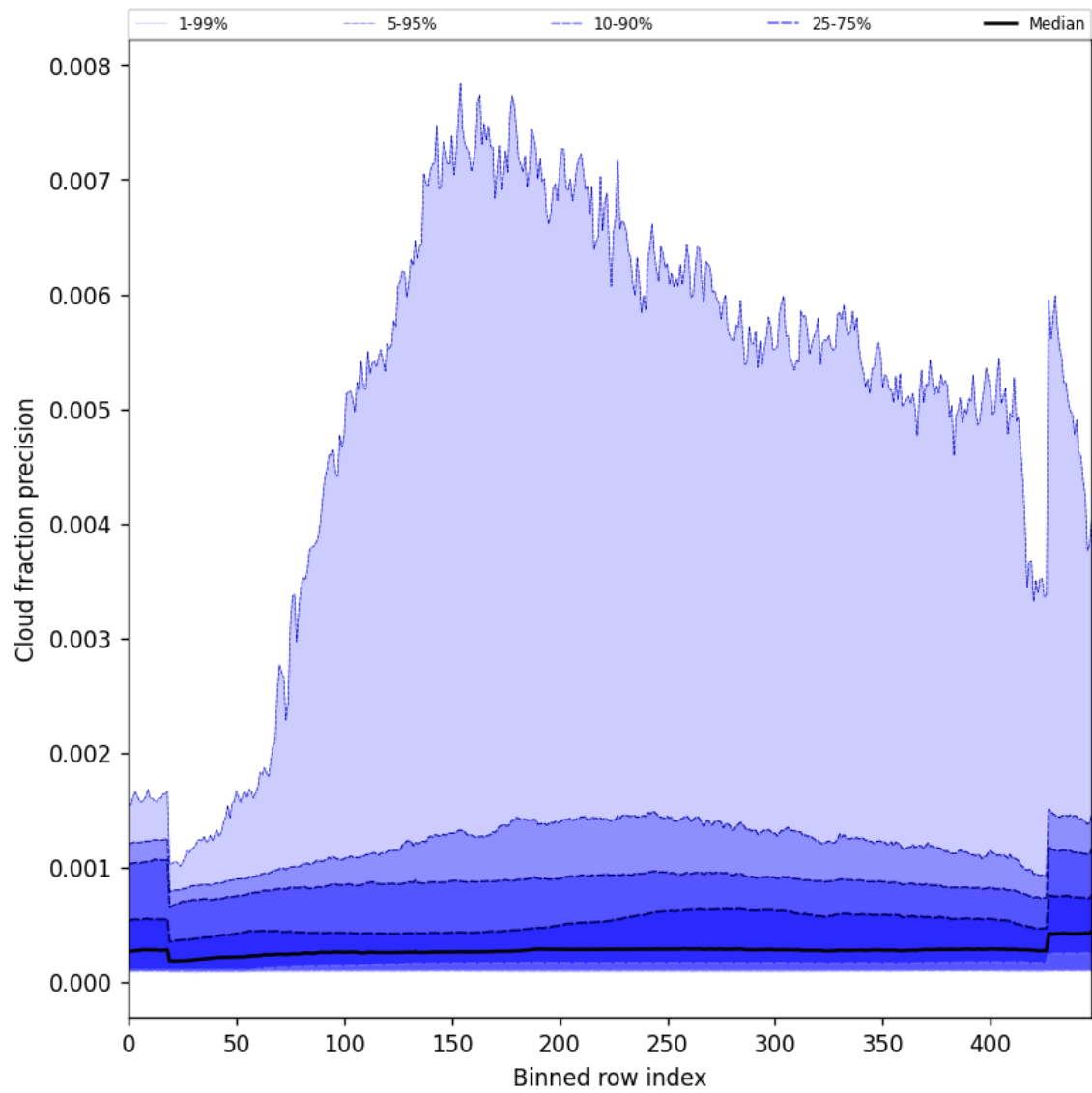
Figure 50: Along track statistics of “Cloud fraction precision” for 2024-10-03 to 2024-10-05
