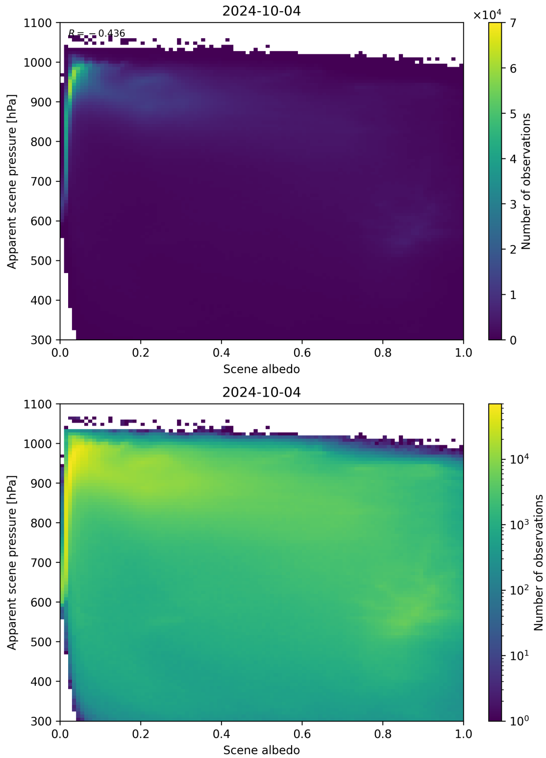
Figure 111: Scatter density plot of “Scene albedo” against “Apparent scene pressure” for 2024-10-03 to 2024-10-05.
