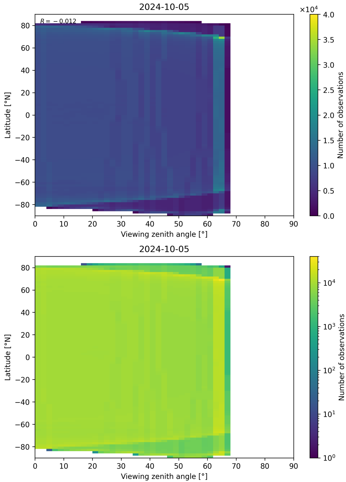
Figure 135: Scatter density plot of “Viewing zenith angle” against “Latitude” for 2024-10-04 to 2024-10-06.
