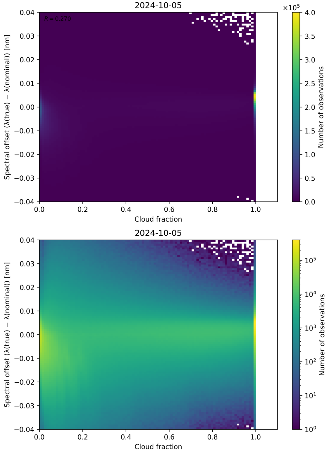
Figure 83: Scatter density plot of “Cloud fraction” against “Spectral offset ( \lambda_{\text{true}} - \lambda_{\text{nominal}} )” for 2024-10-04 to 2024-10-06.
