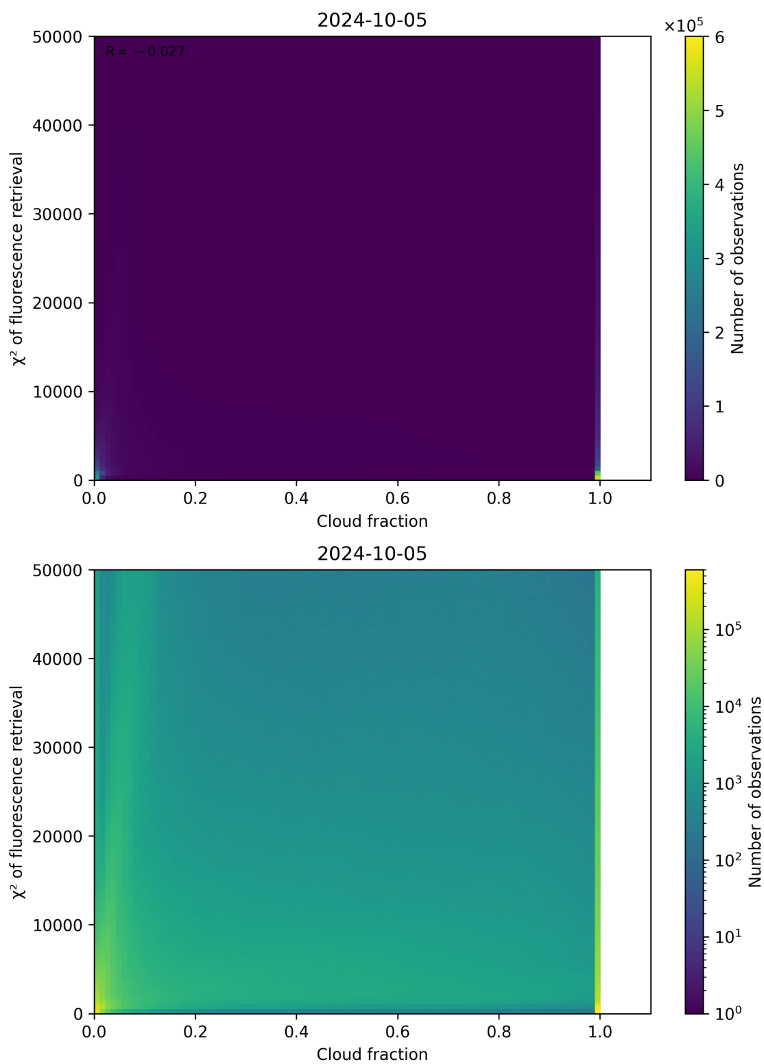
Figure 78: Scatter density plot of “Cloud fraction” against “ \chi^2 of fluorescence retrieval” for 2024-10-04 to 2024-10-06.
