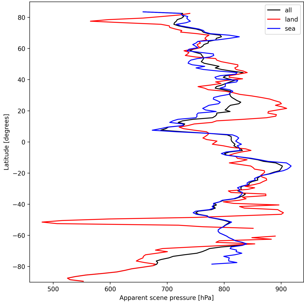
Figure 19: Zonal average of “Apparent scene pressure” for 2024-10-04 to 2024-10-06.
