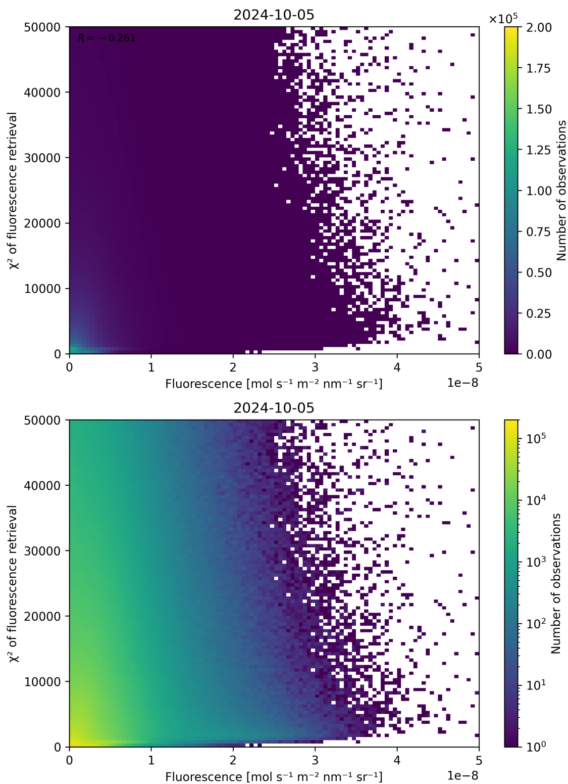
Figure 93: Scatter density plot of “Fluorescence” against “ \chi^2 of fluorescence retrieval” for 2024-10-04 to 2024-10-06.
