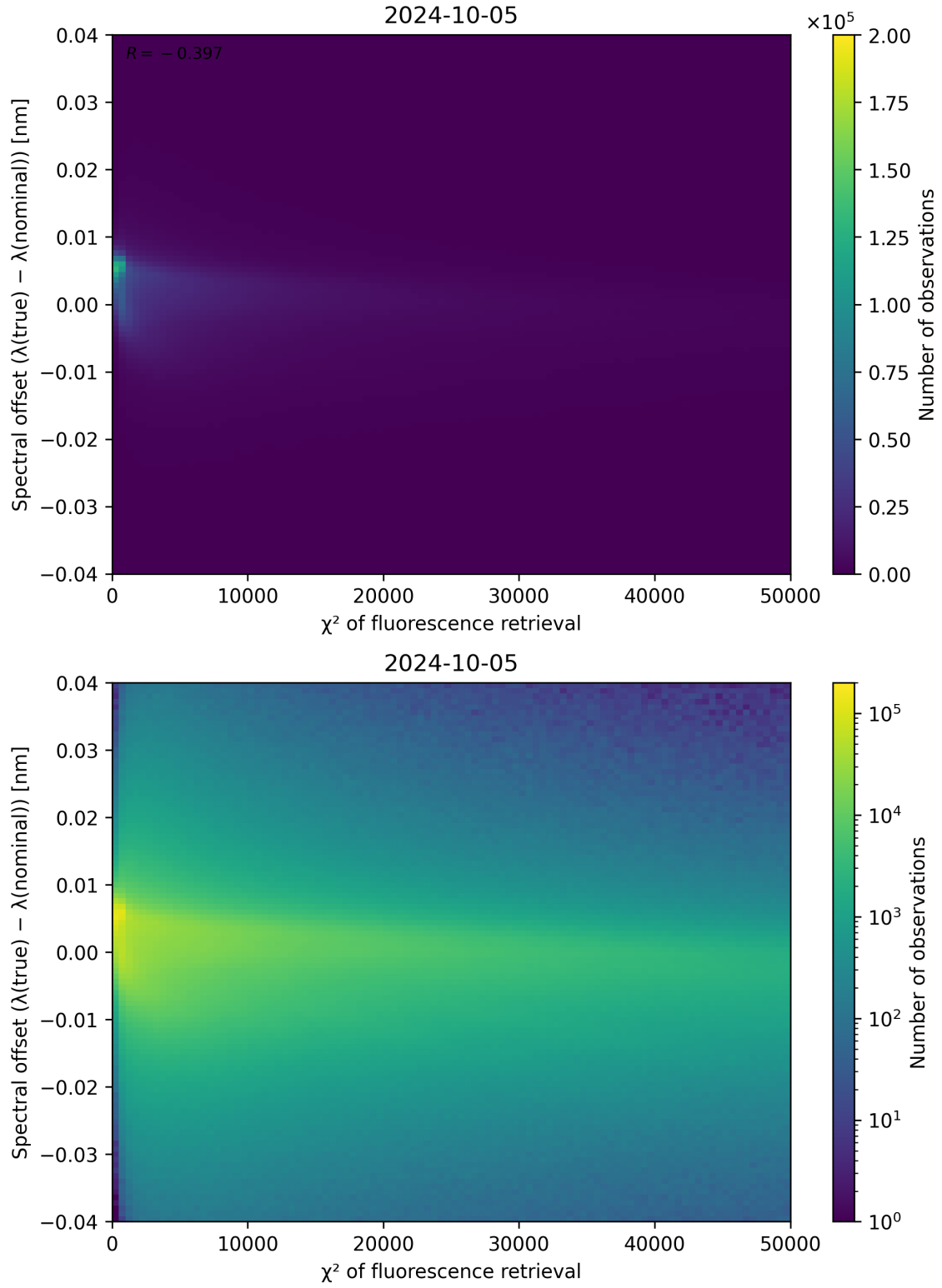
Figure 72: Scatter density plot of “ \chi^2 of fluorescence retrieval” against “Spectral offset ( \lambda_{\text{true}} - \lambda_{\text{nominal}} )” for 2024-10-04 to 2024-10-06.
