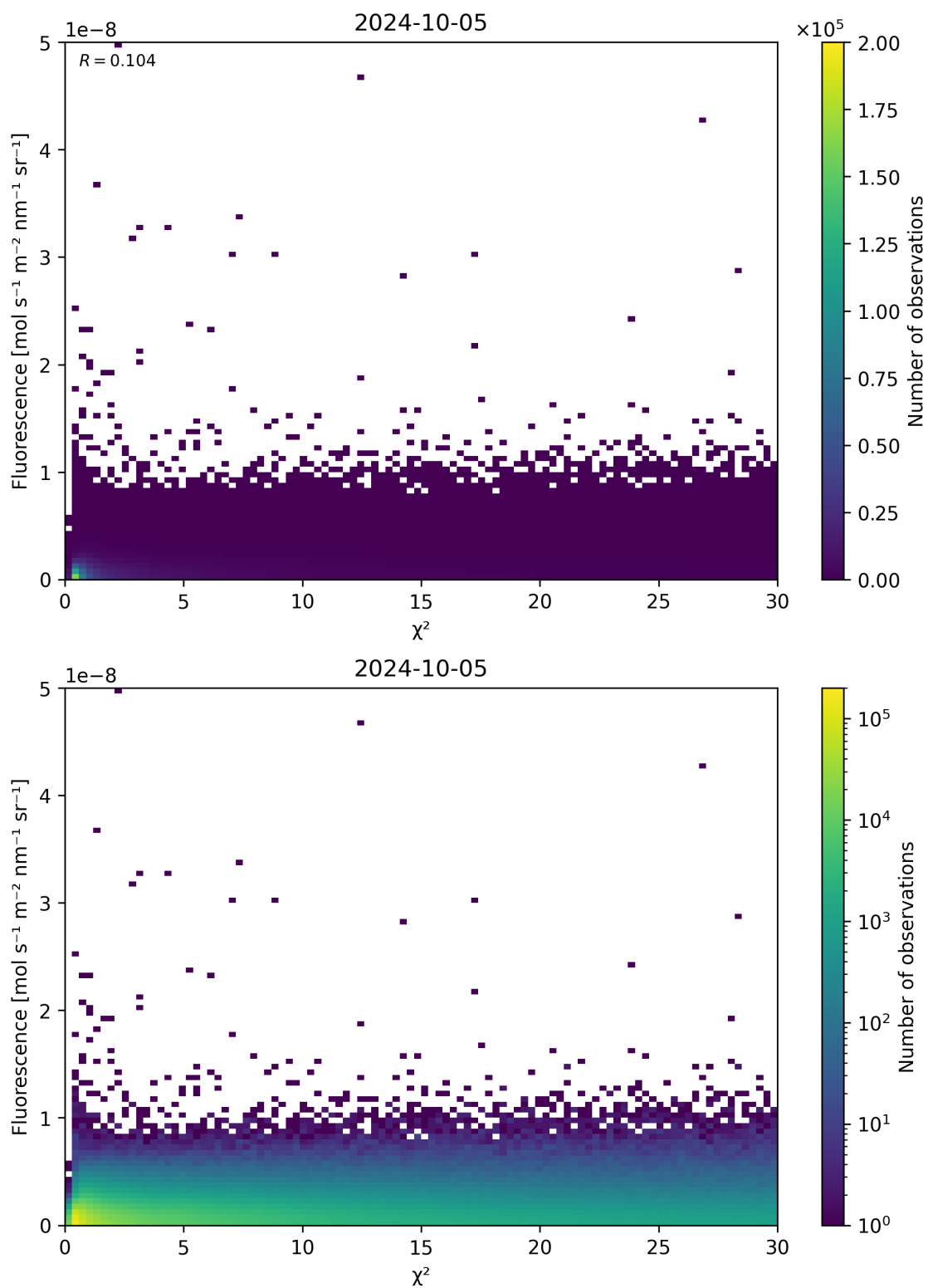
Figure 70: Scatter density plot of “ \chi^2 ” against “Fluorescence” for 2024-10-04 to 2024-10-06.
