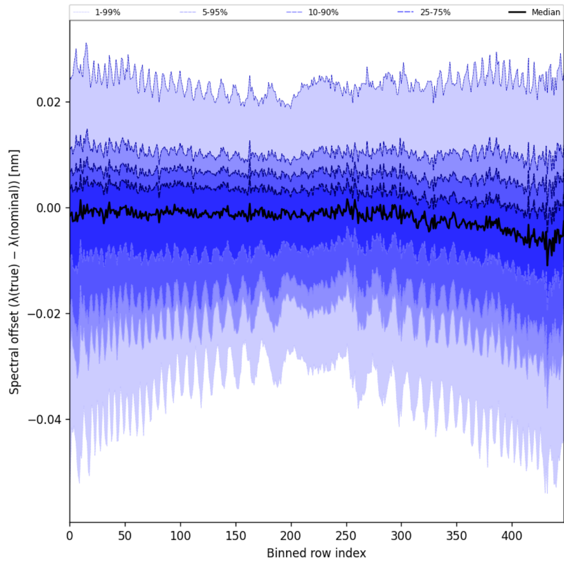
Figure 62: Along track statistics of “Spectral offset ( \lambda_{\text{true}} - \lambda_{\text{nominal}} )” for 2024-10-04 to 2024-10-06
