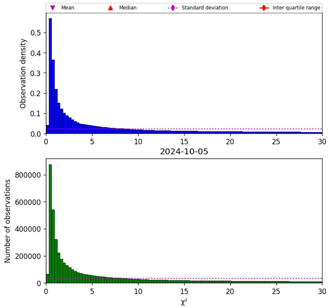
Figure 38: Histogram of “ \chi^2 ” for 2024-10-04 to 2024-10-06
