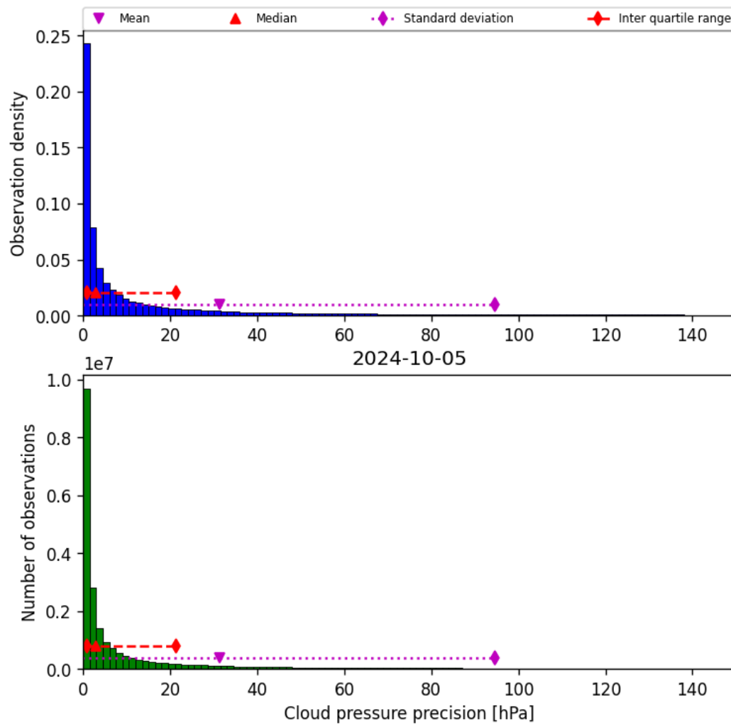
Figure 31: Histogram of “Cloud pressure precision” for 2024-10-04 to 2024-10-06
