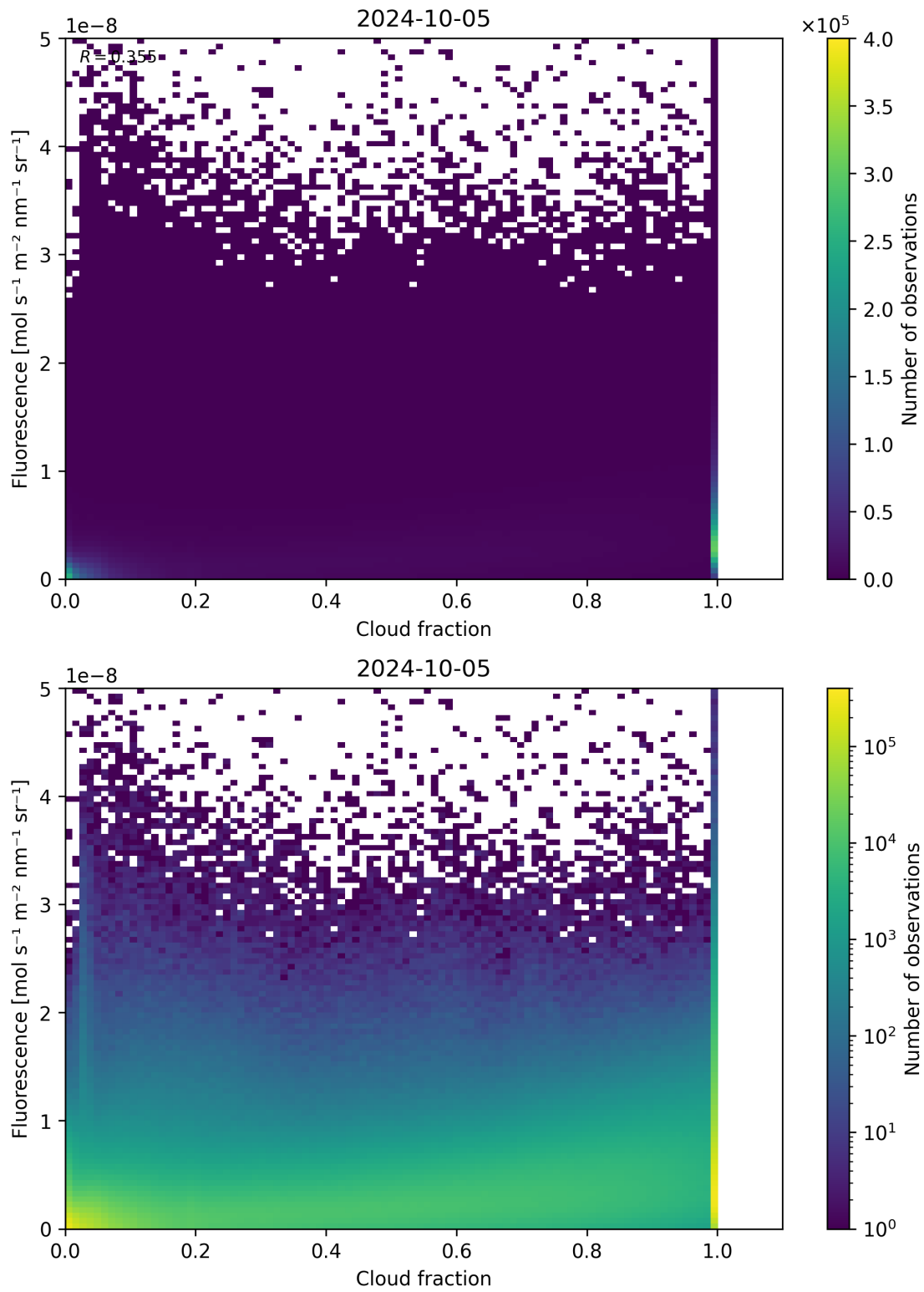
Figure 79: Scatter density plot of “Cloud fraction” against “Fluorescence” for 2024-10-04 to 2024-10-06.
