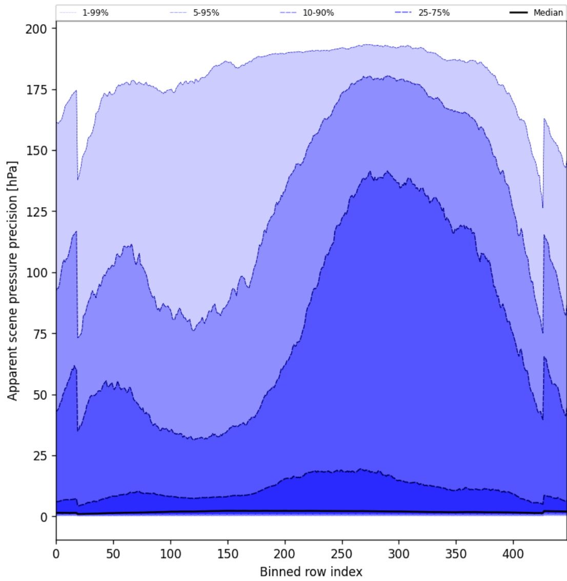
Figure 54: Along track statistics of “Apparent scene pressure precision” for 2024-10-04 to 2024-10-06
