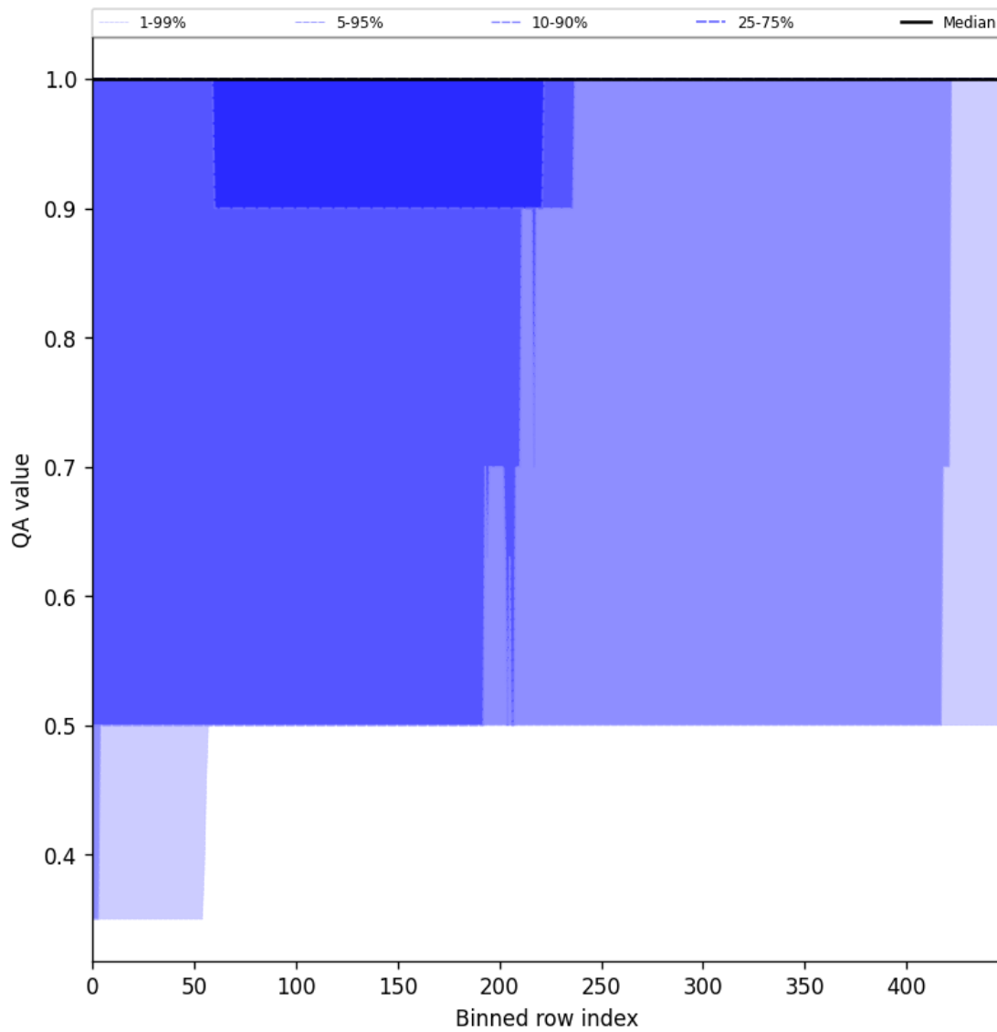
Figure 46: Along track statistics of “QA value” for 2024-10-04 to 2024-10-06
