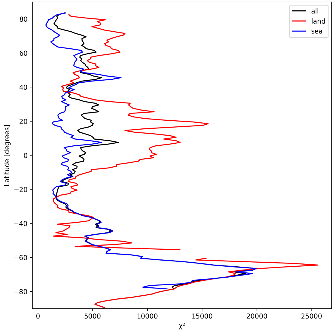
Figure 21: Zonal average of “ \chi^2 ” for 2024-10-04 to 2024-10-06.
