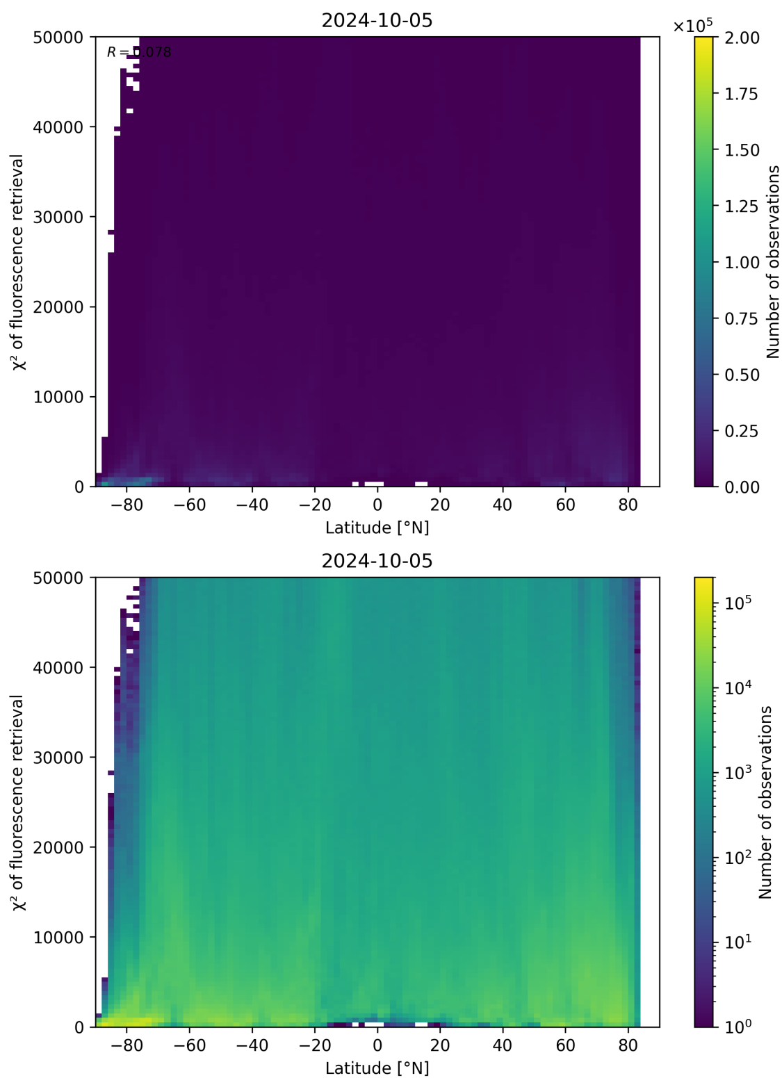
Figure 98: Scatter density plot of “Latitude” against “ \chi^2 of fluorescence retrieval” for 2024-10-04 to 2024-10-06.
