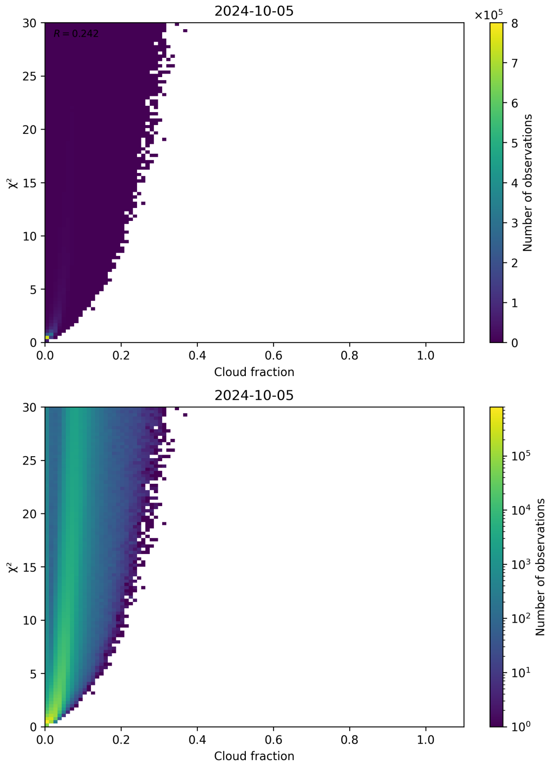
Figure 77: Scatter density plot of “Cloud fraction” against “ \chi^2 ” for 2024-10-04 to 2024-10-06.
