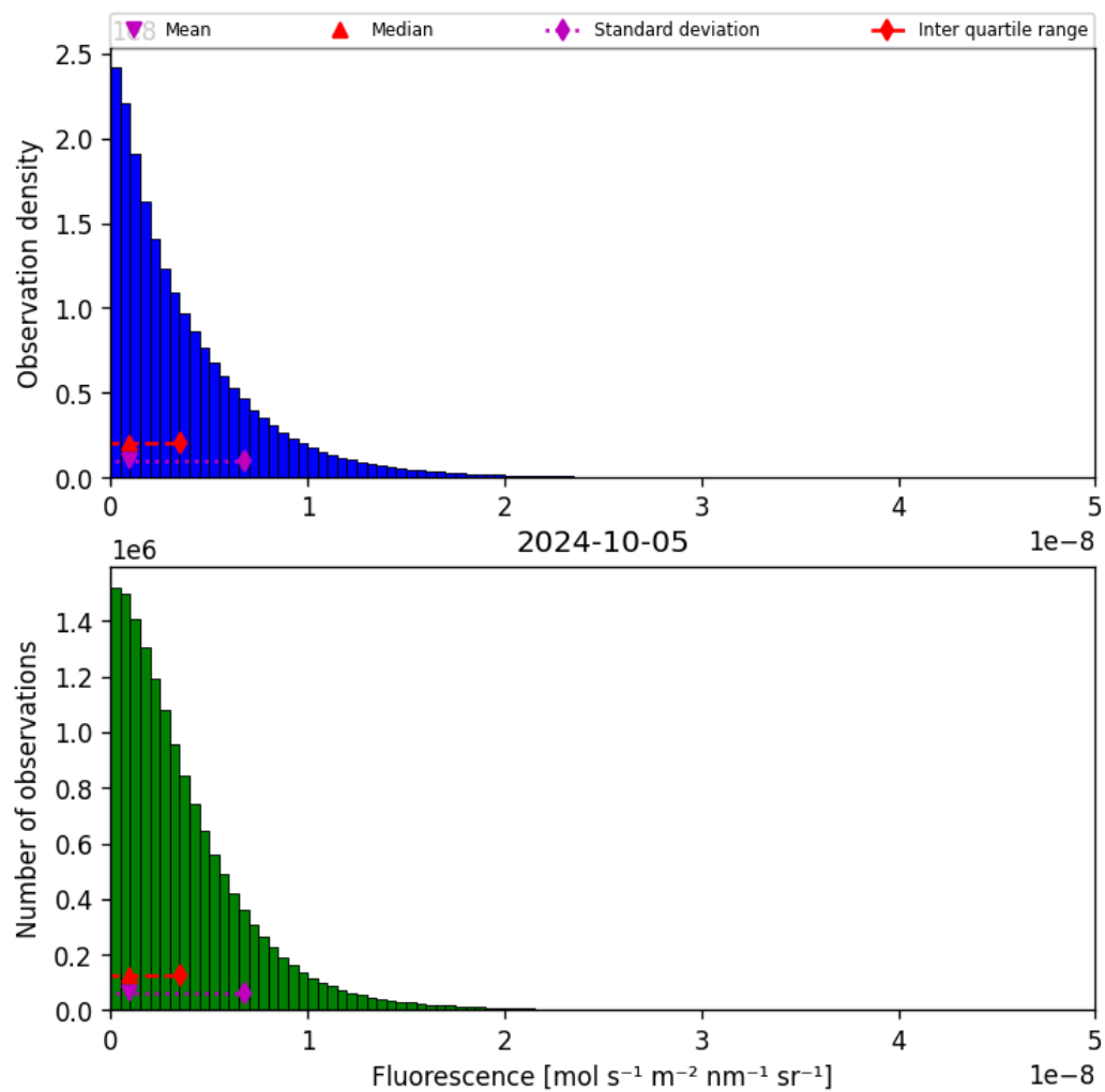
Figure 40: Histogram of “Fluorescence” for 2024-10-04 to 2024-10-06
