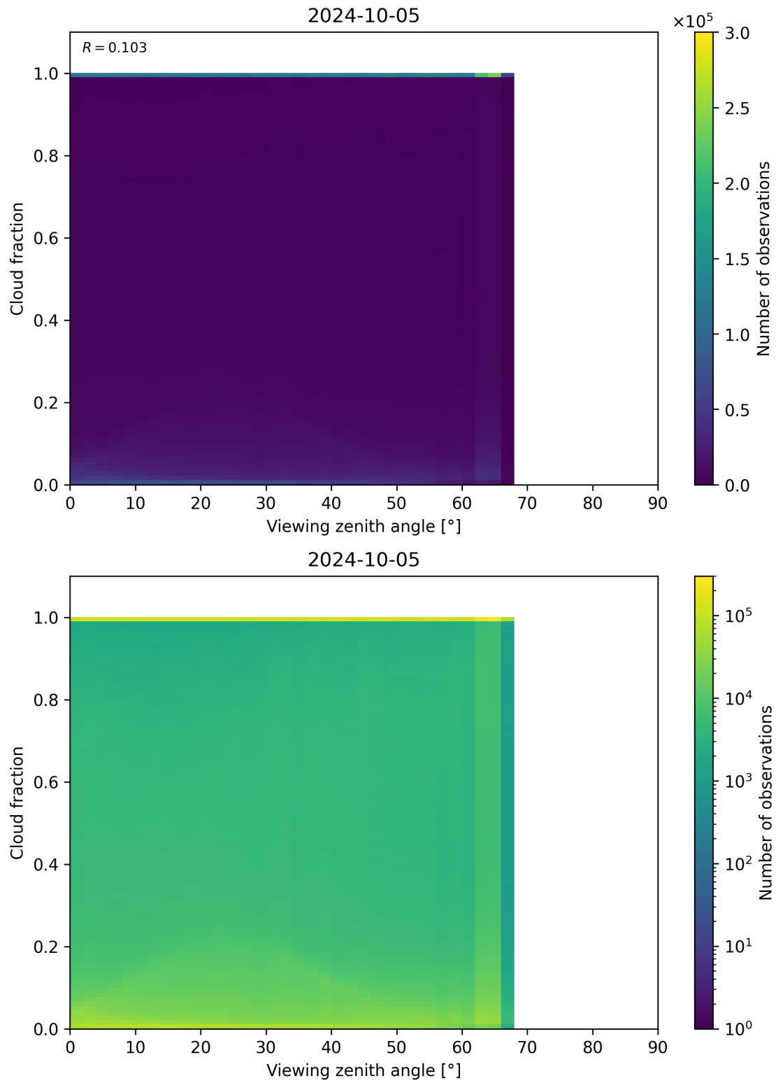
Figure 132: Scatter density plot of “Viewing zenith angle” against “Cloud fraction” for 2024-10-04 to 2024-10-06.
