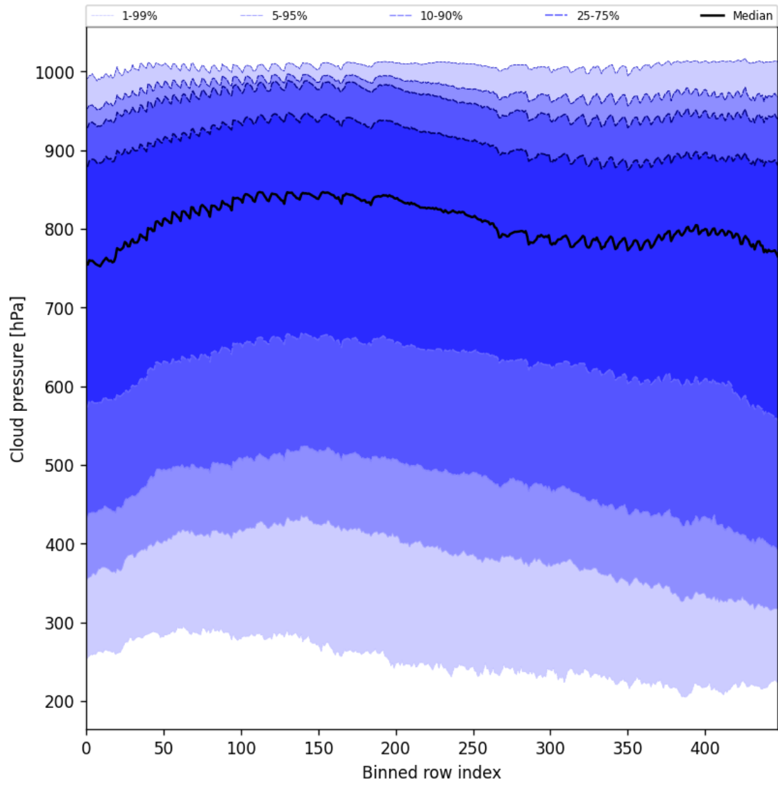
Figure 47: Along track statistics of “Cloud pressure” for 2024-10-04 to 2024-10-06
