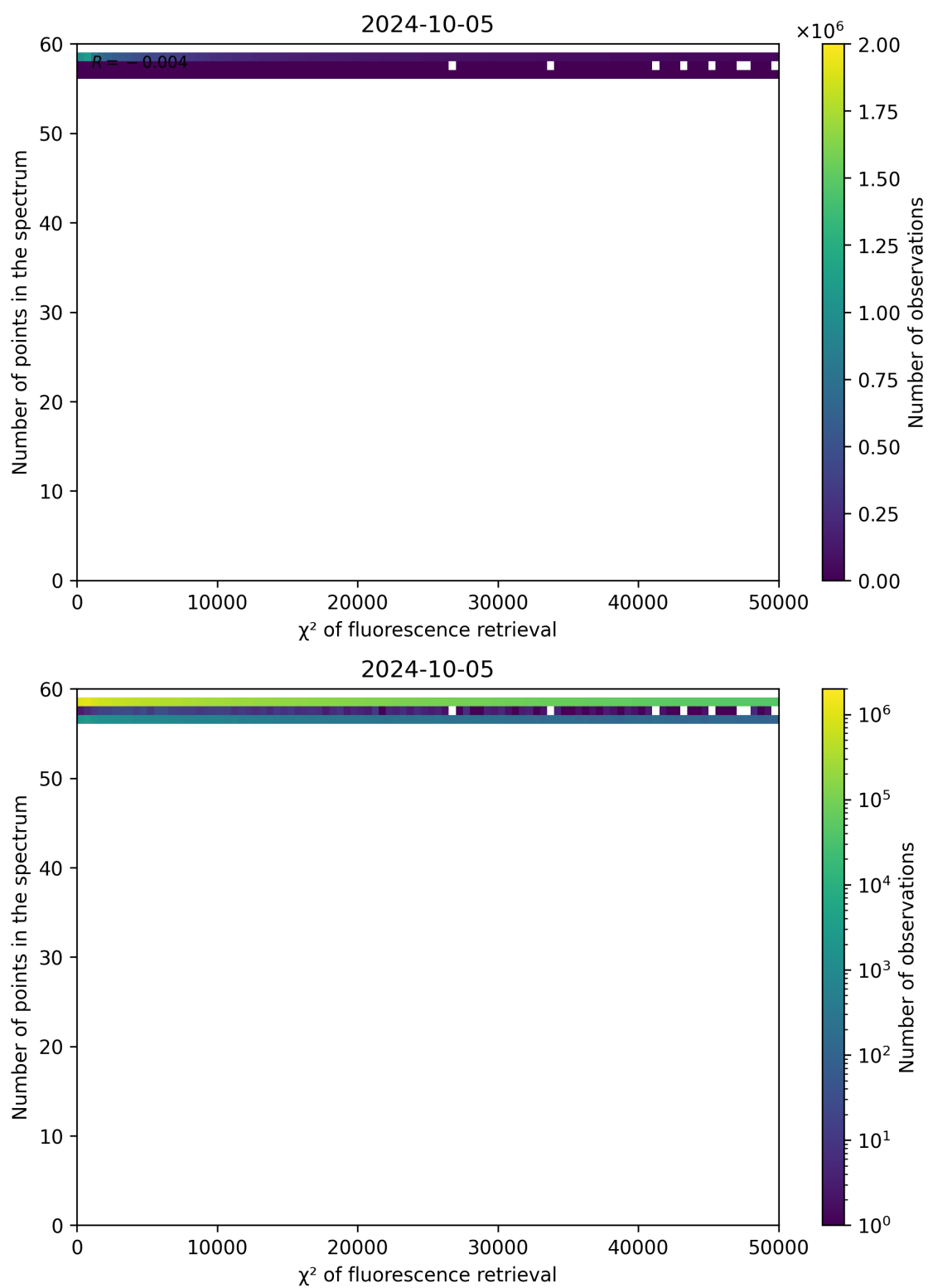
Figure 71: Scatter density plot of " \chi^2 of fluorescence retrieval" against "Number of points in the spectrum" for 2024-10-04 to 2024-10-06.
