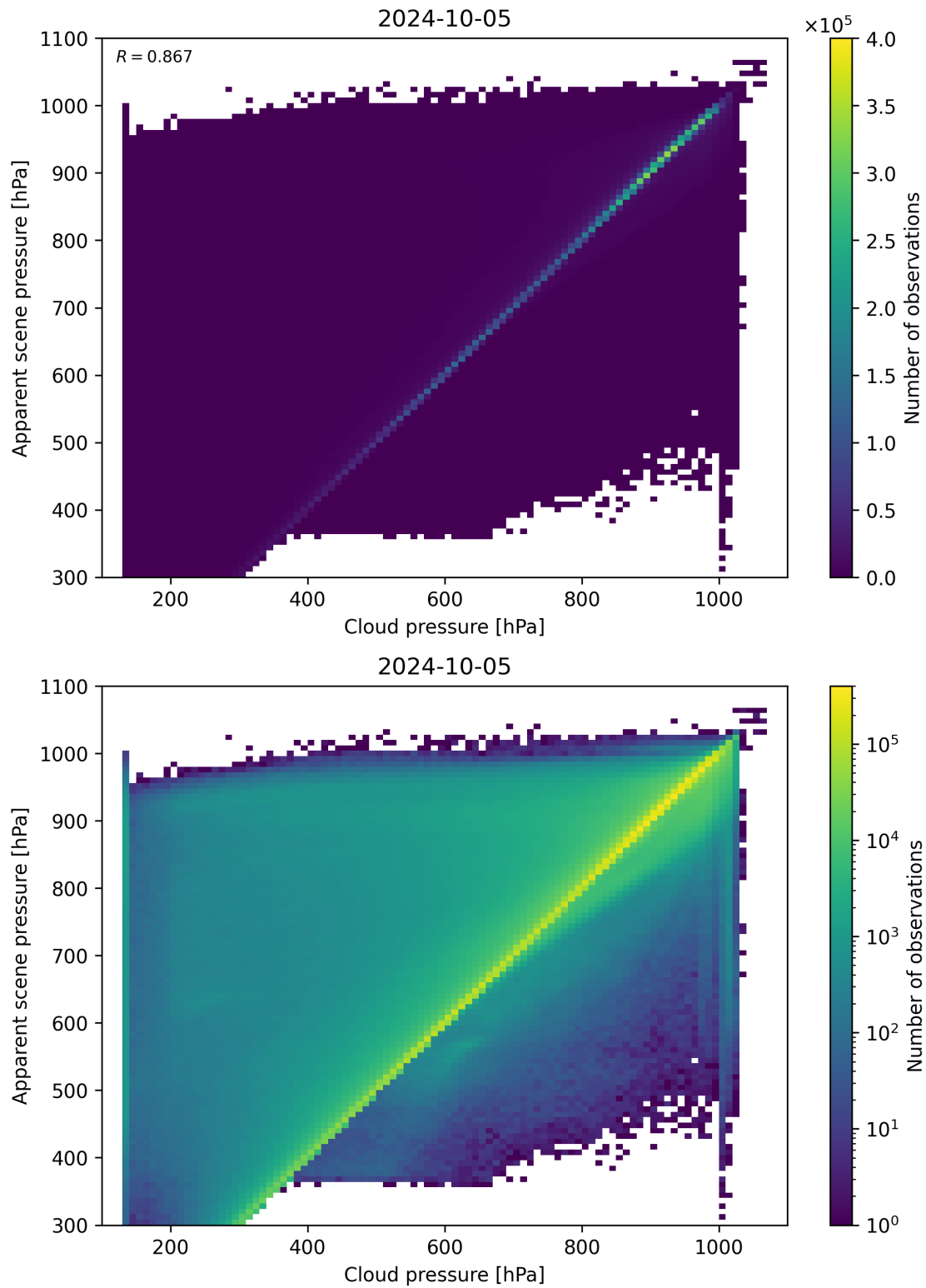
Figure 84: Scatter density plot of “Cloud pressure” against “Apparent scene pressure” for 2024-10-04 to 2024-10-06.
