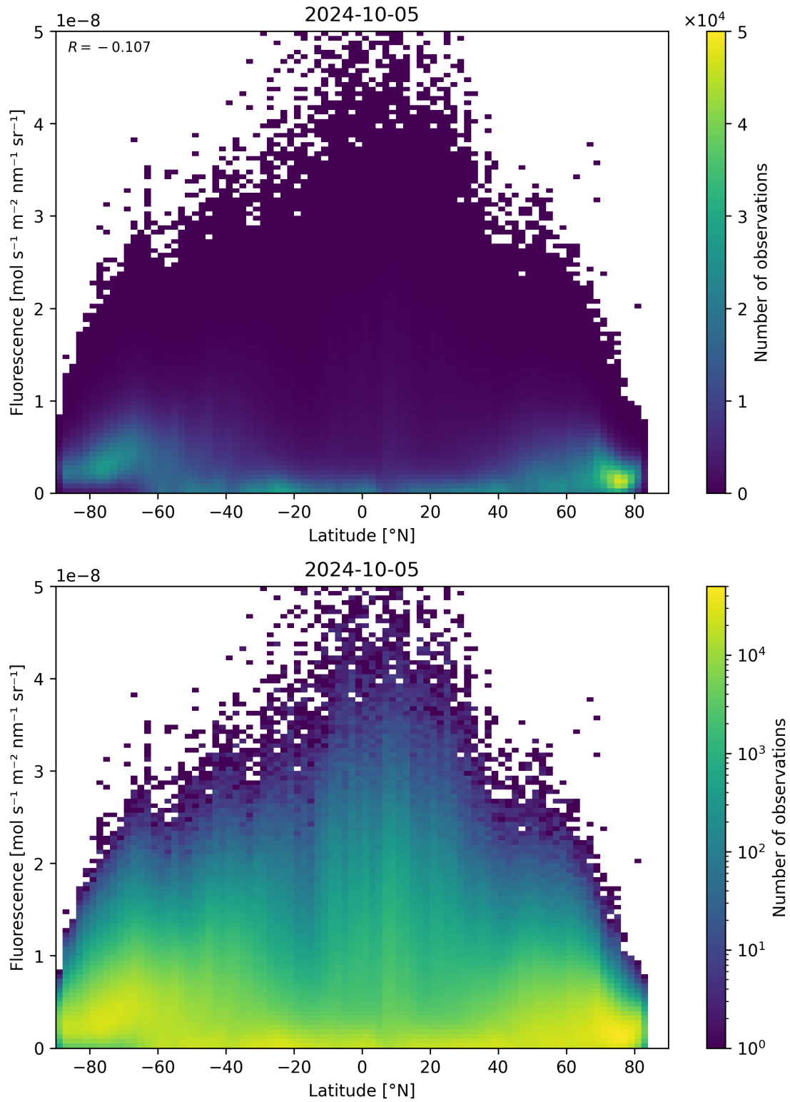
Figure 101: Scatter density plot of “Latitude” against “Fluorescence” for 2024-10-04 to 2024-10-06.
