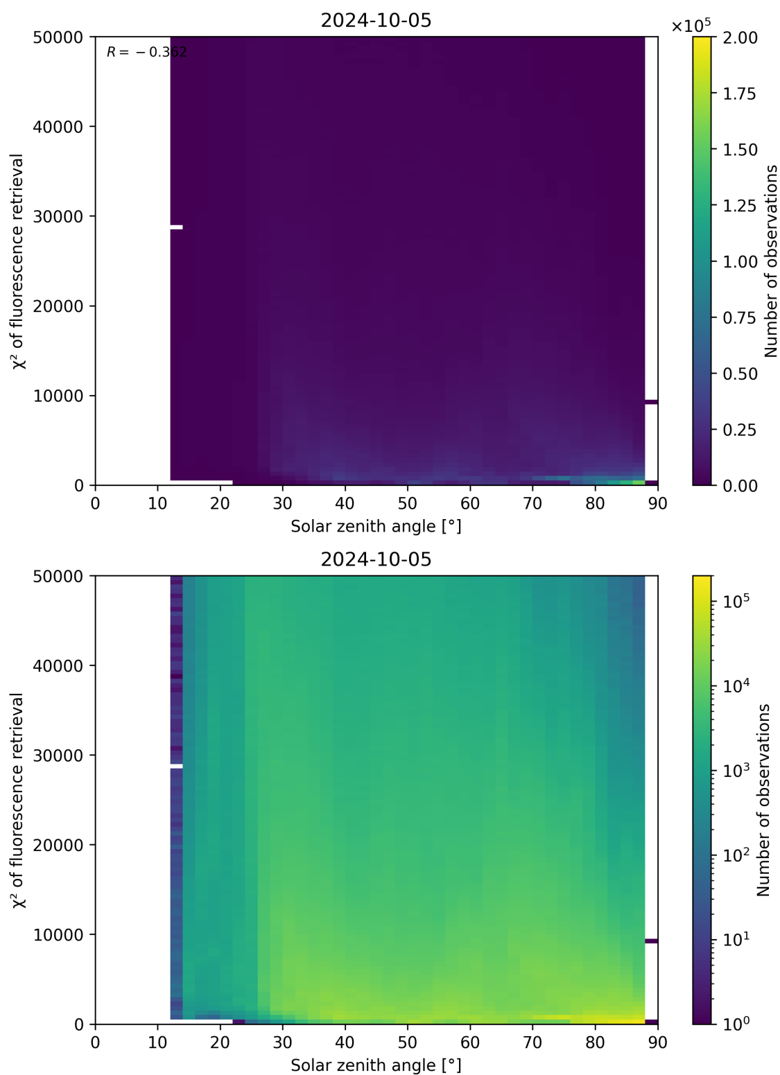
Figure 120: Scatter density plot of “Solar zenith angle” against “ \chi^2 of fluorescence retrieval” for 2024-10-04 to 2024-10-06.
