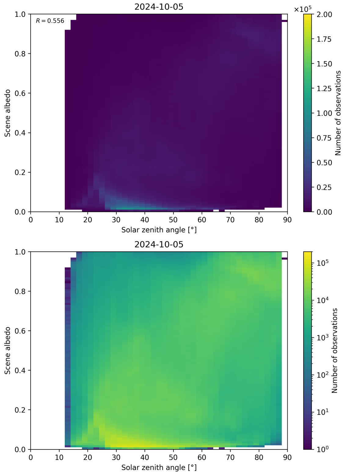
Figure 127: Scatter density plot of “Solar zenith angle” against “Scene albedo” for 2024-10-04 to 2024-10-06.
