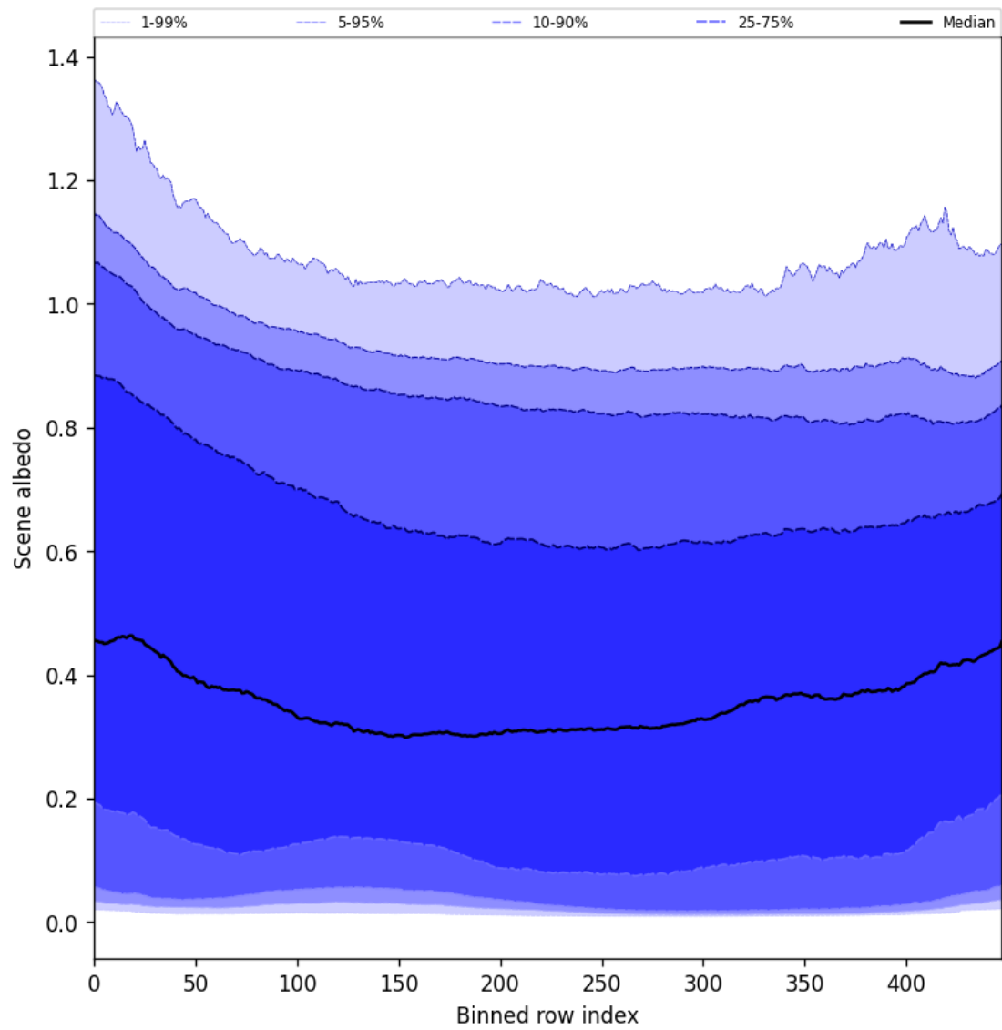
Figure 51: Along track statistics of “Scene albedo” for 2024-10-04 to 2024-10-06
