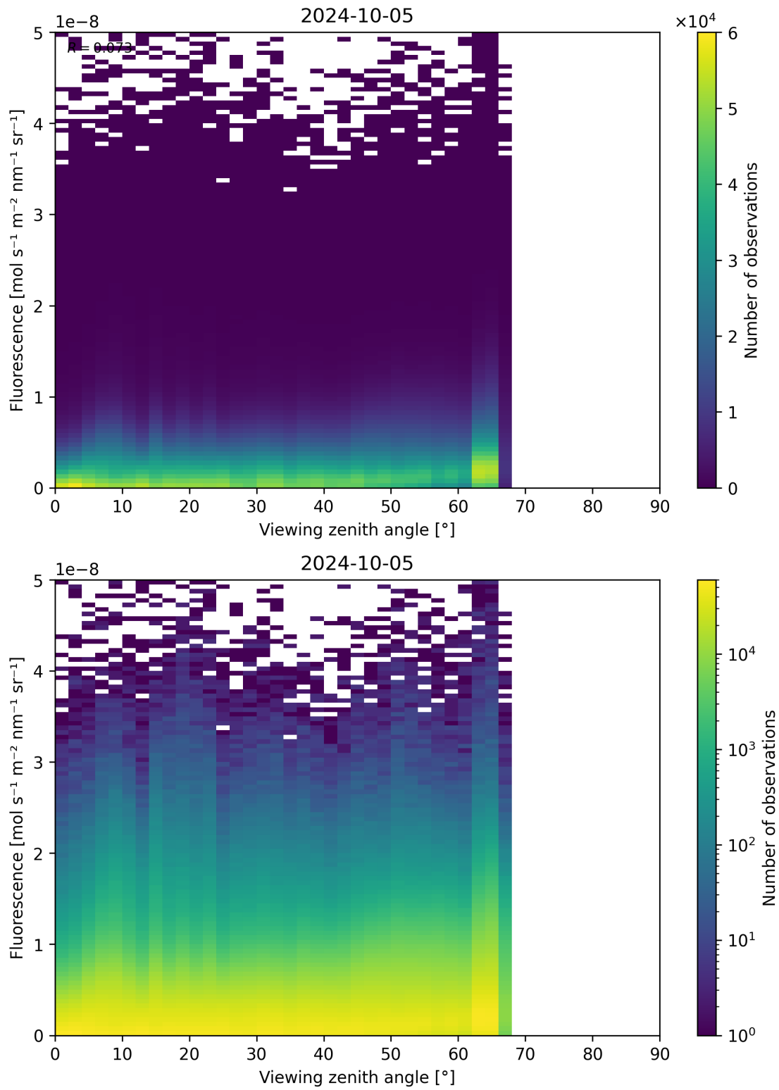
Figure 134: Scatter density plot of “Viewing zenith angle” against “Fluorescence” for 2024-10-04 to 2024-10-06.
