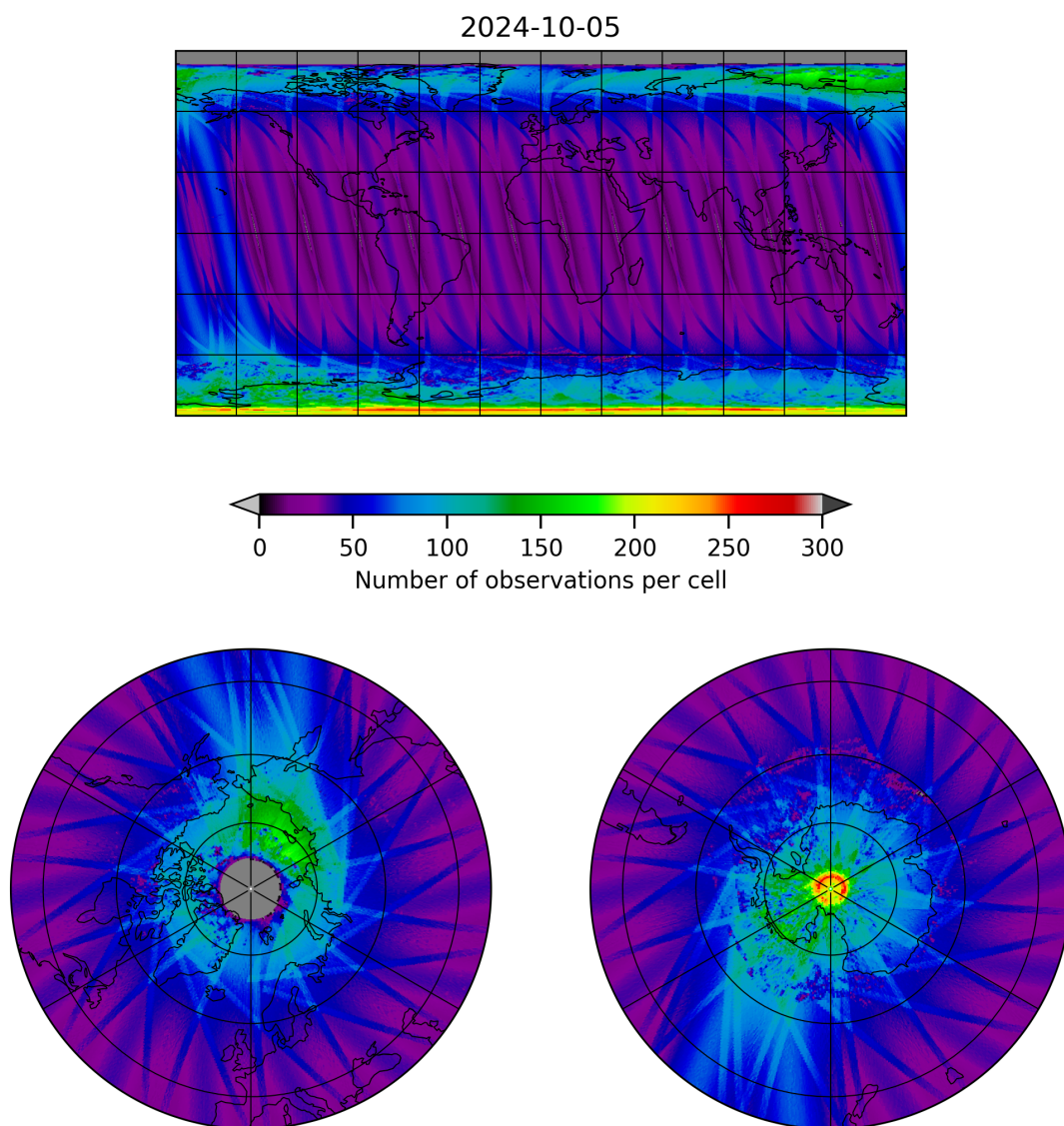
Figure 11: Map of the number of observations for 2024-10-04 to 2024-10-06
