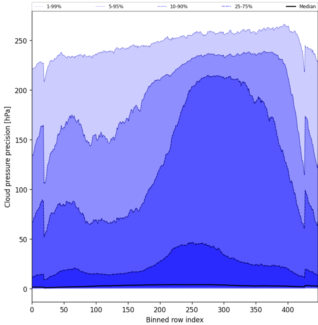
Figure 48: Along track statistics of “Cloud pressure precision” for 2024-10-04 to 2024-10-06
