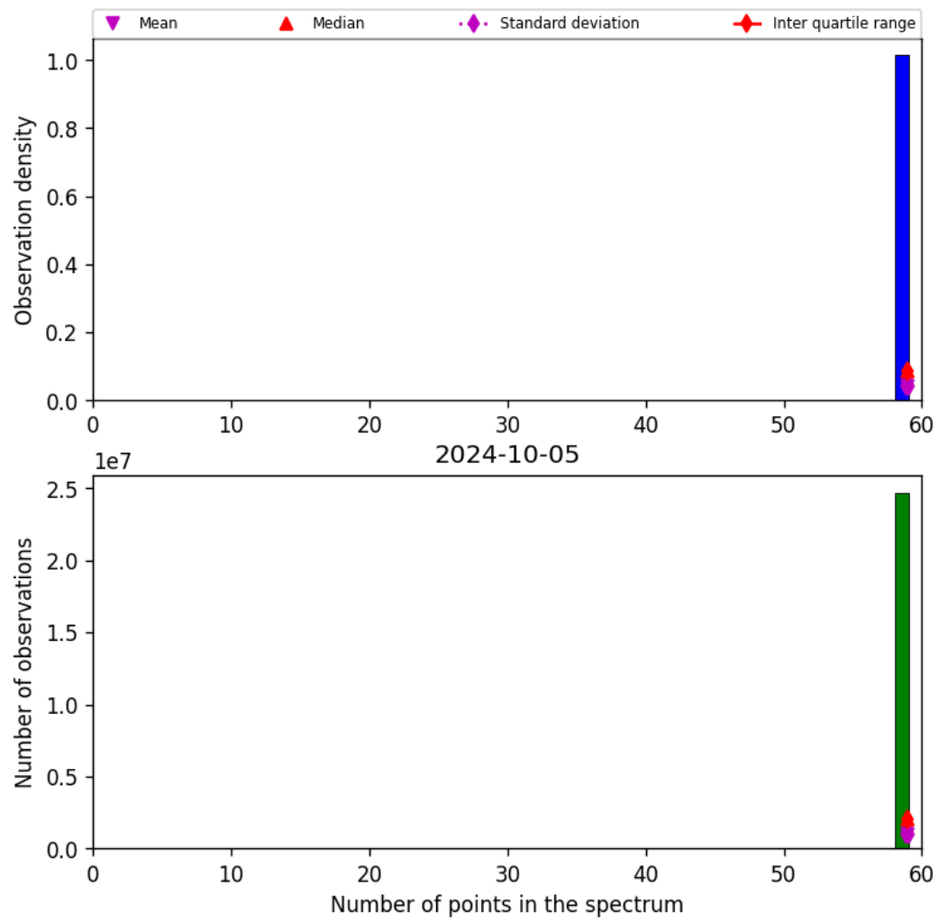
Figure 44: Histogram of “Number of points in the spectrum” for 2024-10-04 to 2024-10-06
