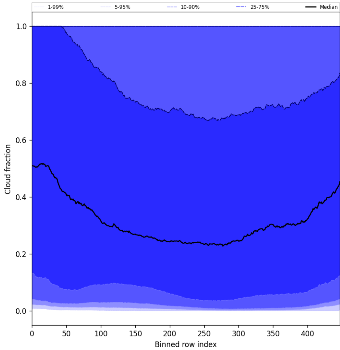
Figure 49: Along track statistics of “Cloud fraction” for 2024-10-04 to 2024-10-06
