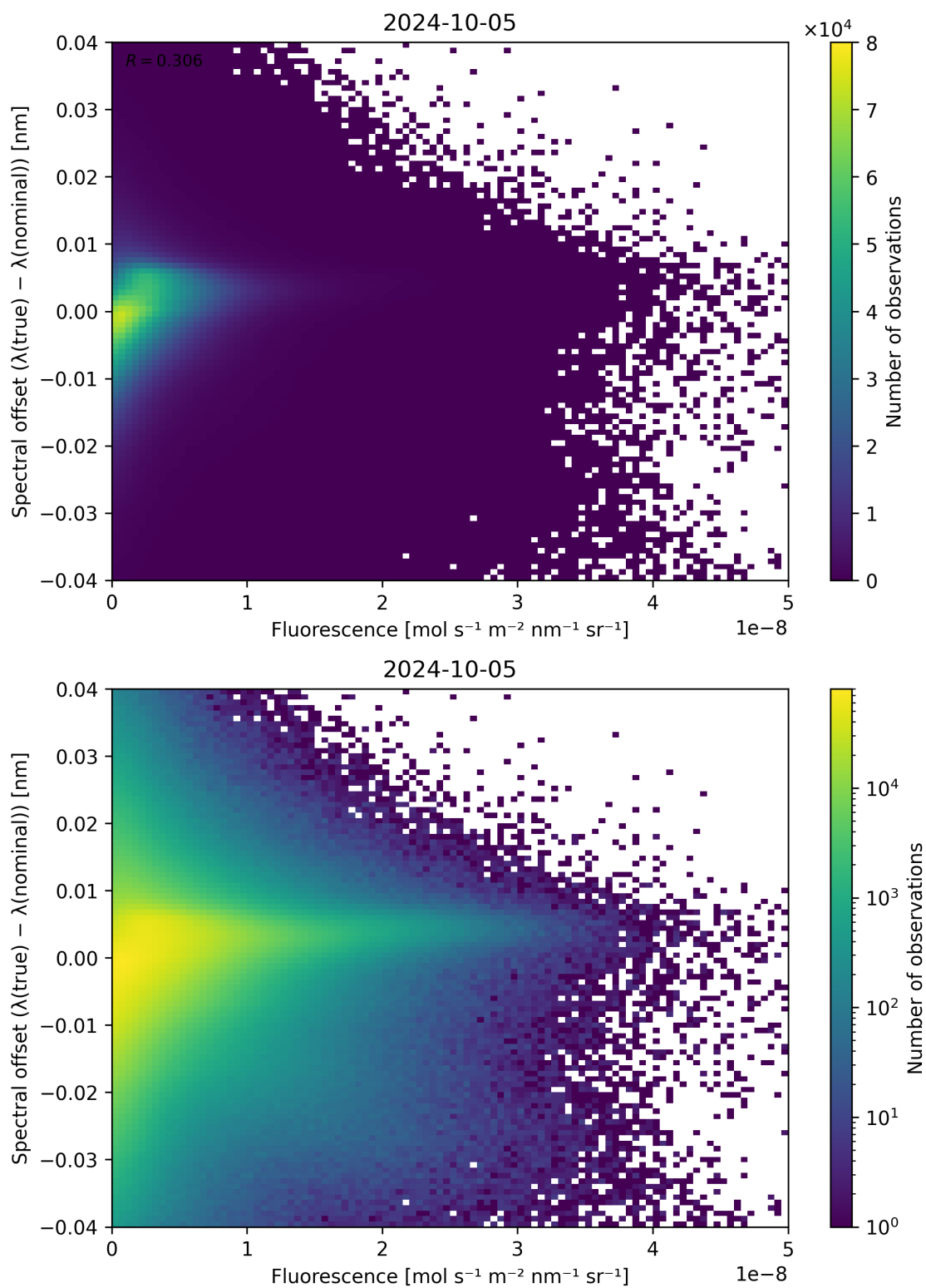
Figure 95: Scatter density plot of “Fluorescence” against “Spectral offset ( \lambda_{\text{true}} - \lambda_{\text{nominal}} )” for 2024-10-04 to 2024-10-06.
