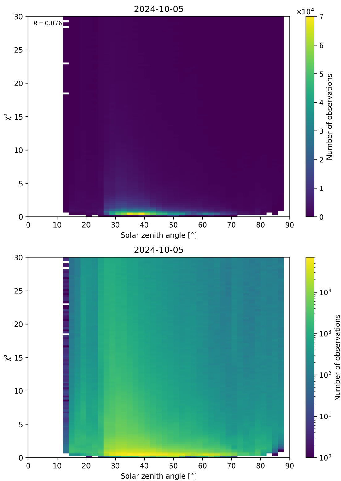
Figure 119: Scatter density plot of “Solar zenith angle” against “ \chi^2 ” for 2024-10-04 to 2024-10-06.
