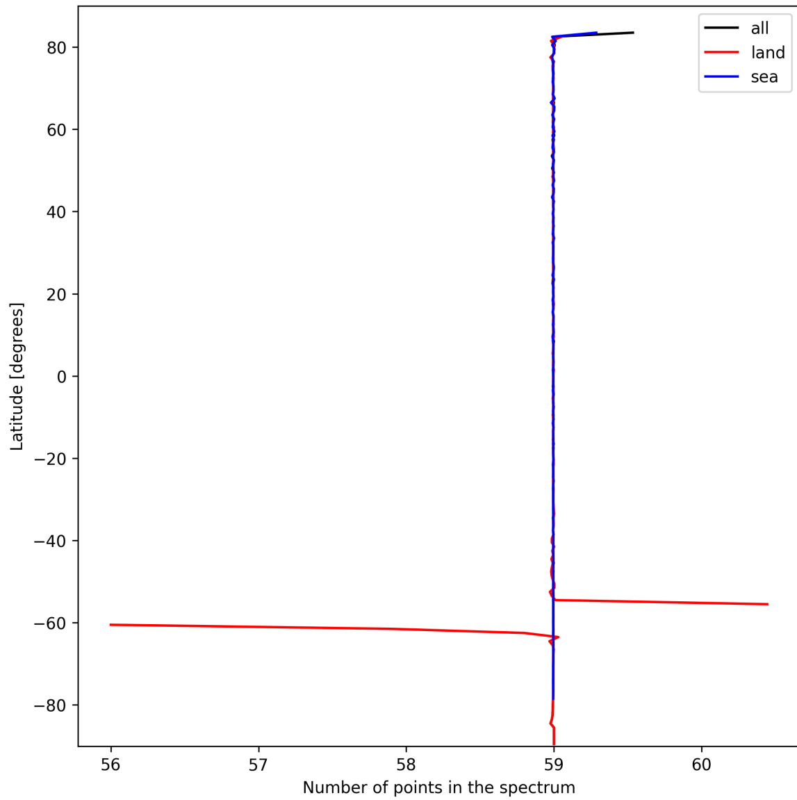
Figure 27: Zonal average of “Number of points in the spectrum” for 2024-10-04 to 2024-10-06.
