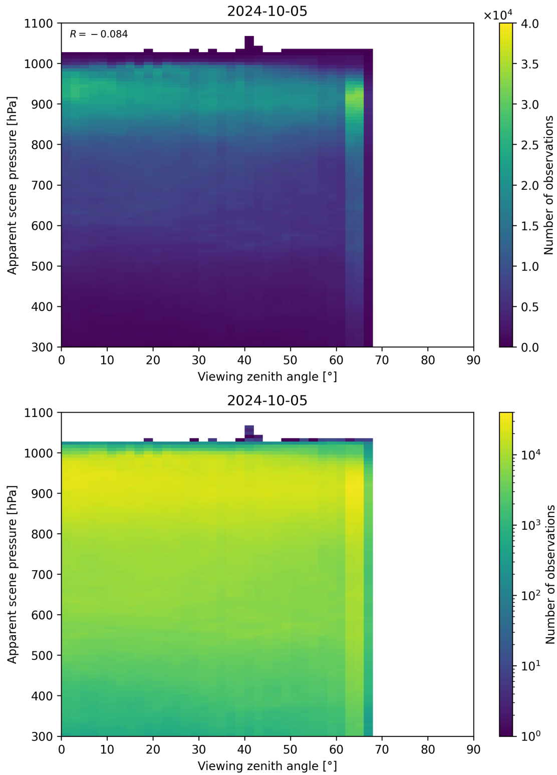
Figure 129: Scatter density plot of “Viewing zenith angle” against “Apparent scene pressure” for 2024-10-04 to 2024-10-06.
