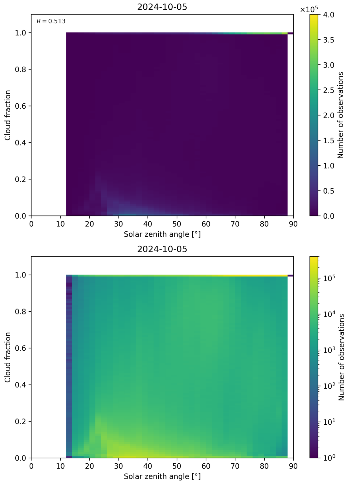
Figure 121: Scatter density plot of “Solar zenith angle” against “Cloud fraction” for 2024-10-04 to 2024-10-06.
