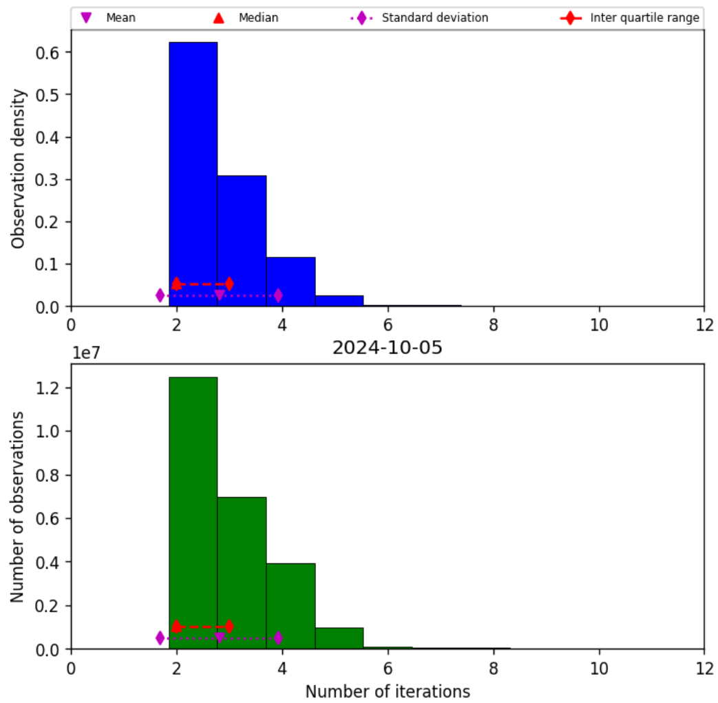
Figure 39: Histogram of “Number of iterations” for 2024-10-04 to 2024-10-06
