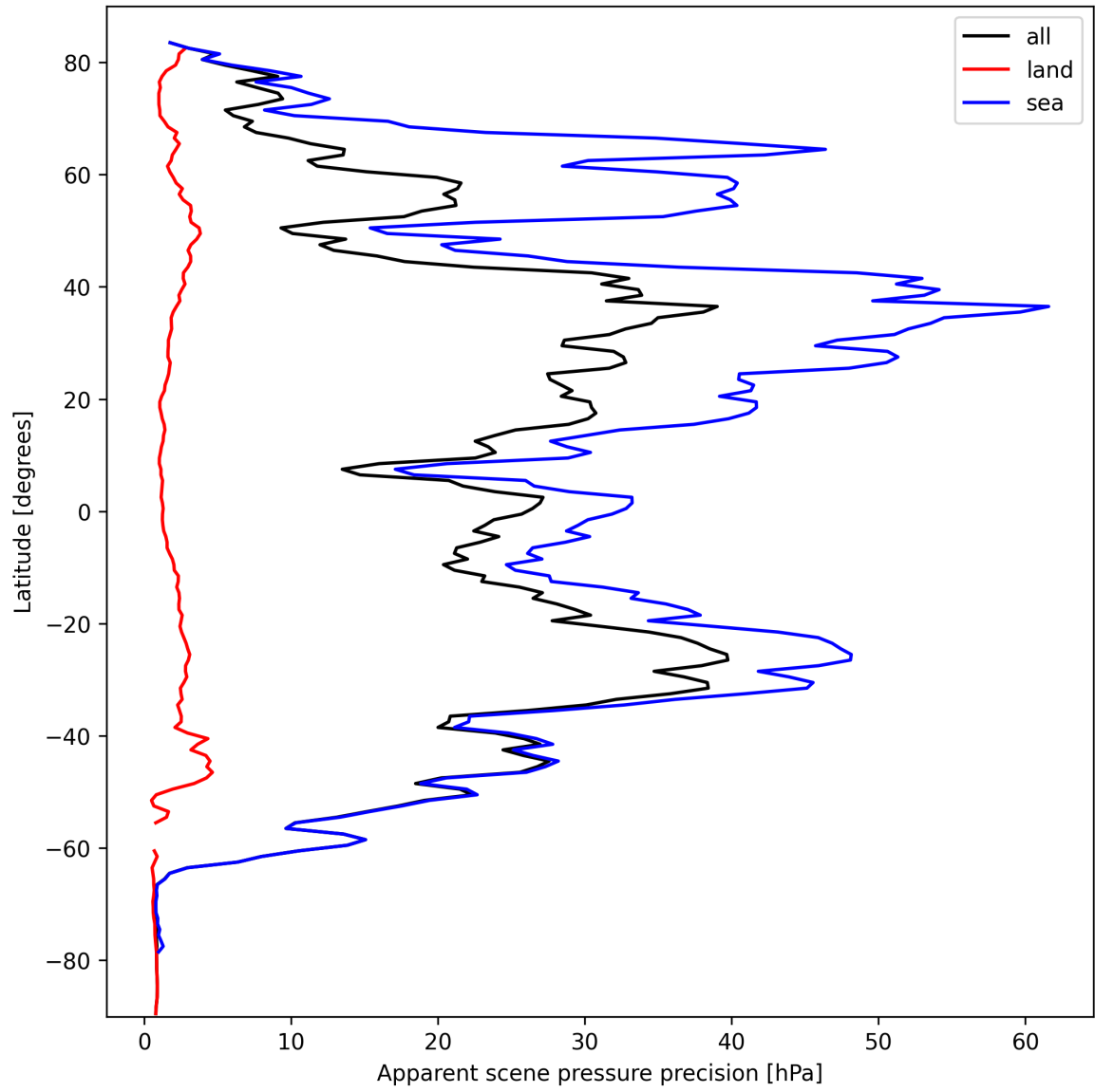
Figure 20: Zonal average of “Apparent scene pressure precision” for 2024-10-04 to 2024-10-06.
