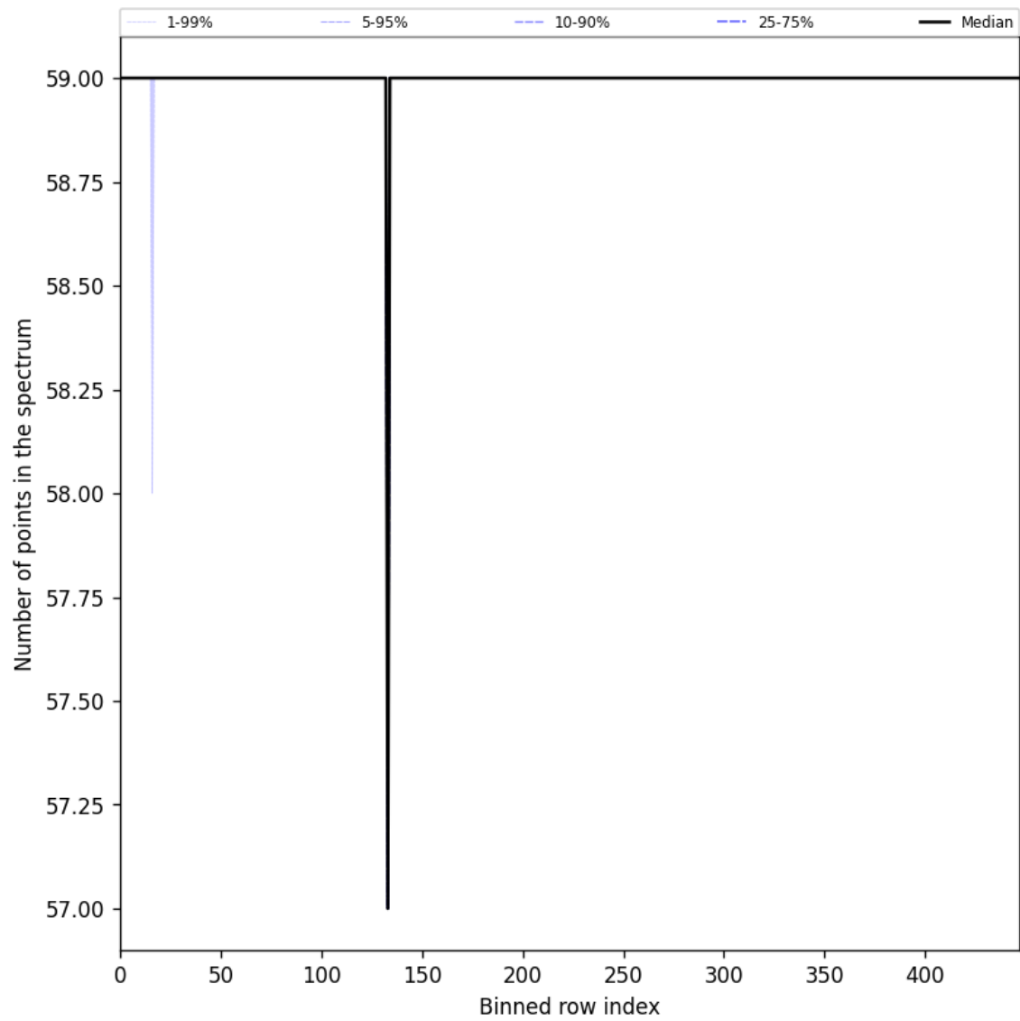
Figure 61: Along track statistics of “Number of points in the spectrum” for 2024-10-04 to 2024-10-06
