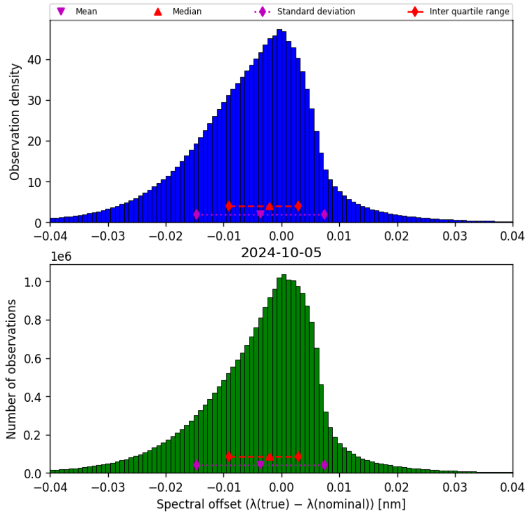
Figure 45: Histogram of “Spectral offset ( \lambda_{\text{true}} - \lambda_{\text{nominal}} )” for 2024-10-04 to 2024-10-06
