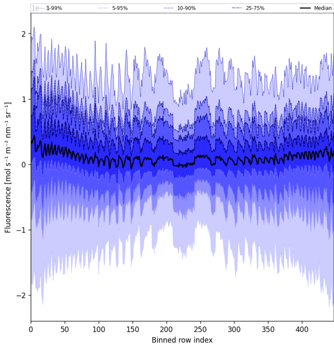
Figure 57: Along track statistics of “Fluorescence” for 2024-10-04 to 2024-10-06
