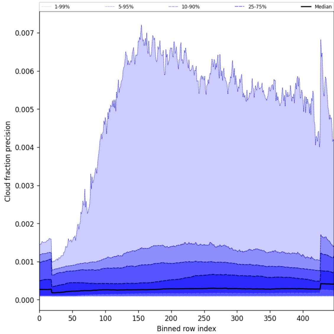
Figure 50: Along track statistics of “Cloud fraction precision” for 2024-10-04 to 2024-10-06
