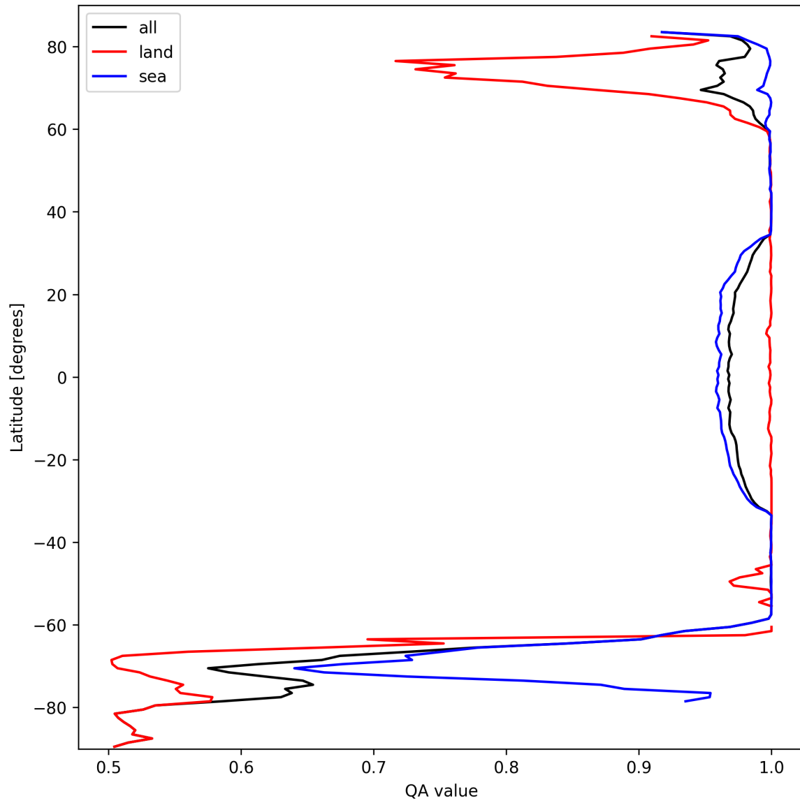
Figure 12: Zonal average of “QA value” for 2024-10-04 to 2024-10-06.
