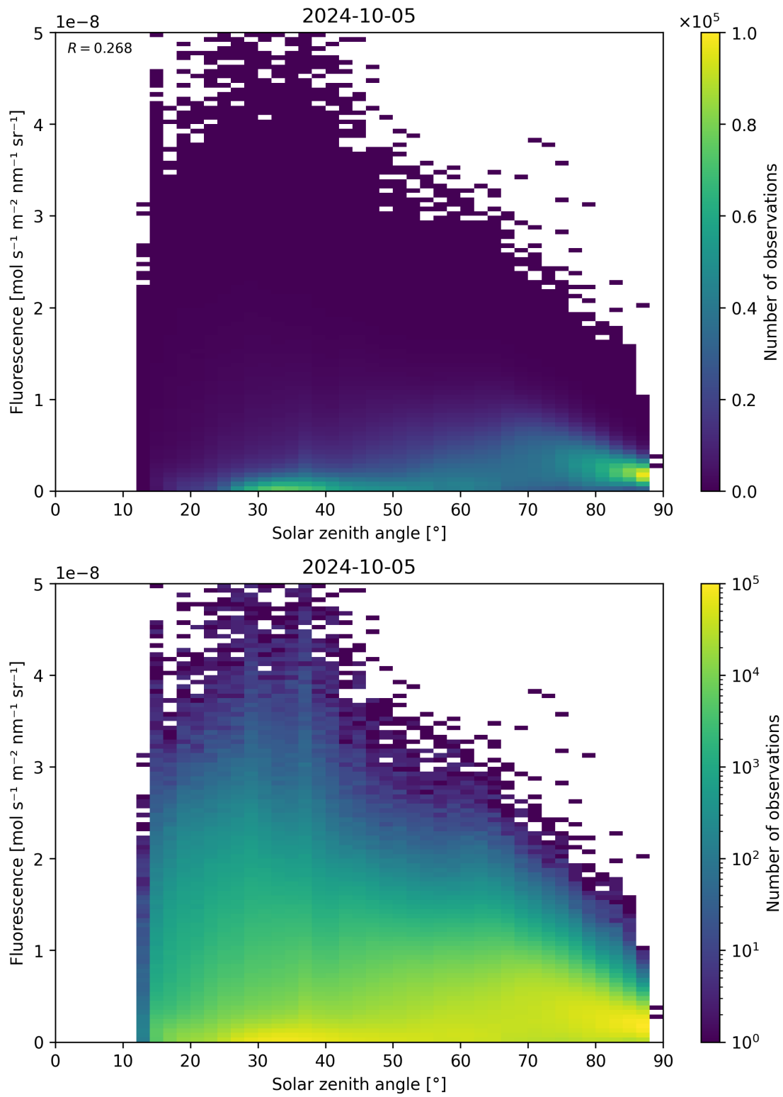
Figure 123: Scatter density plot of “Solar zenith angle” against “Fluorescence” for 2024-10-04 to 2024-10-06.
