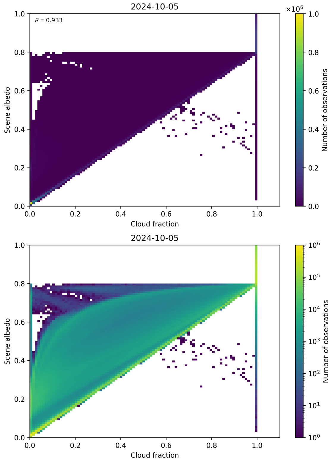
Figure 82: Scatter density plot of “Cloud fraction” against “Scene albedo” for 2024-10-04 to 2024-10-06.
