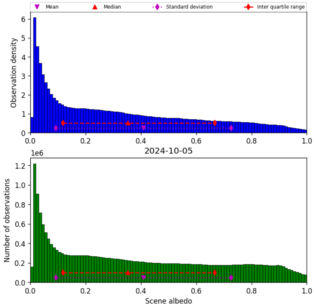
Figure 34: Histogram of “Scene albedo” for 2024-10-04 to 2024-10-06
