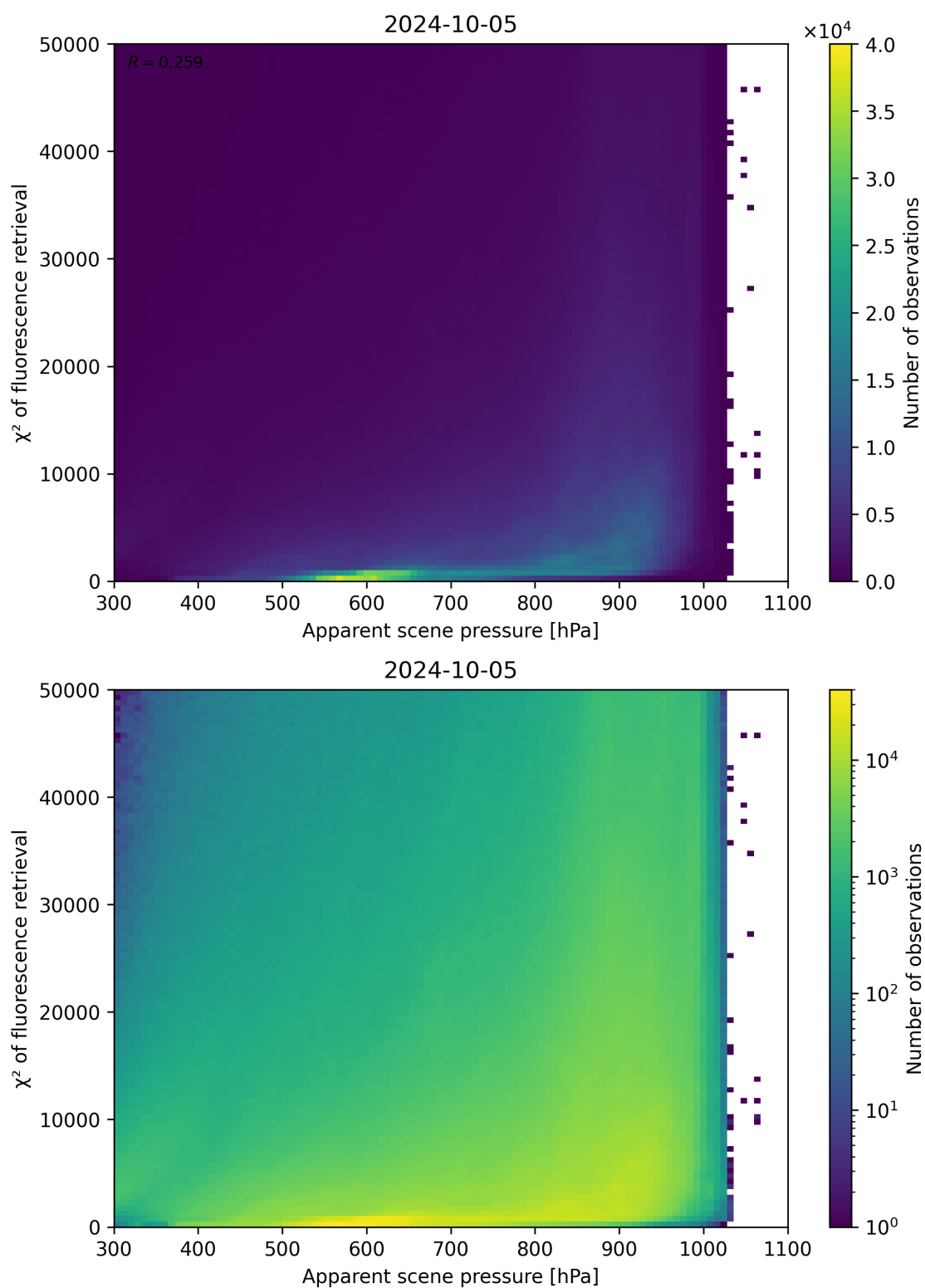
Figure 64: Scatter density plot of “Apparent scene pressure” against “ \chi^2 of fluorescence retrieval” for 2024-10-04 to 2024-10-06.
