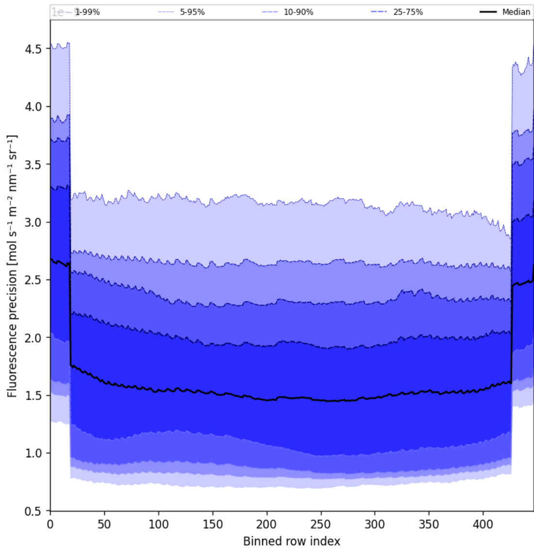
Figure 58: Along track statistics of “Fluorescence precision” for 2024-10-04 to 2024-10-06
