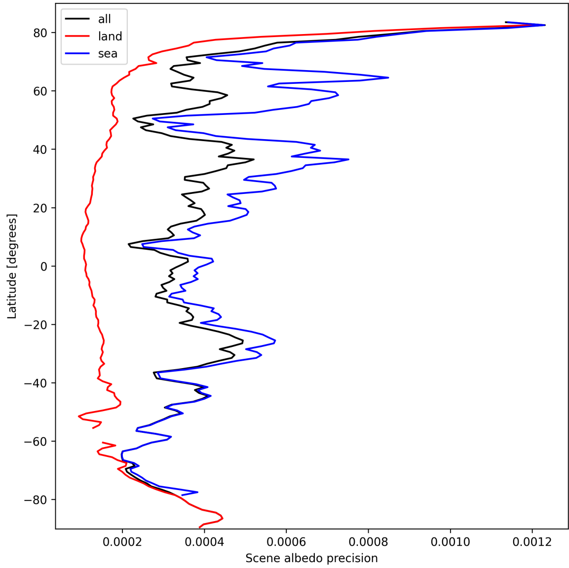
Figure 18: Zonal average of “Scene albedo precision” for 2024-10-04 to 2024-10-06.
