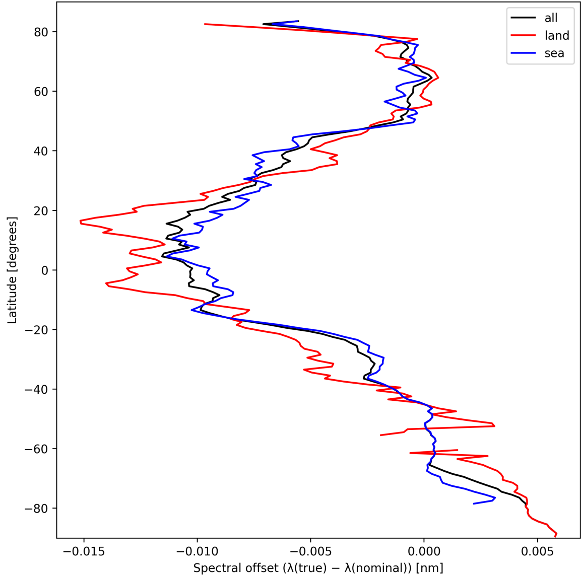
Figure 28: Zonal average of “Spectral offset ( \lambda_{\text{true}} - \lambda_{\text{nominal}} )” for 2024-10-04 to 2024-10-06.
