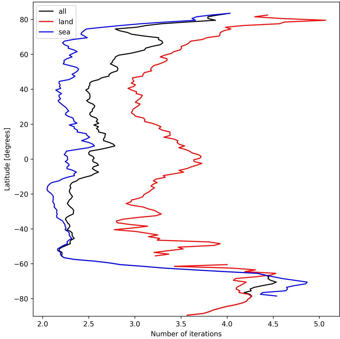
Figure 22: Zonal average of “Number of iterations” for 2024-10-04 to 2024-10-06.
