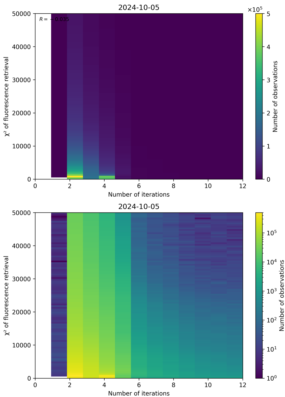
Figure 106: Scatter density plot of “Number of iterations” against “ \chi^2 of fluorescence retrieval” for 2024-10-04 to 2024-10-06.
