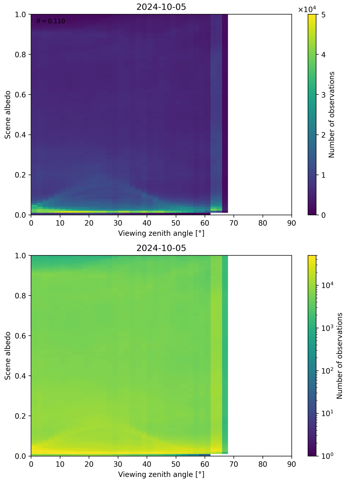
Figure 138: Scatter density plot of “Viewing zenith angle” against “Scene albedo” for 2024-10-04 to 2024-10-06.
