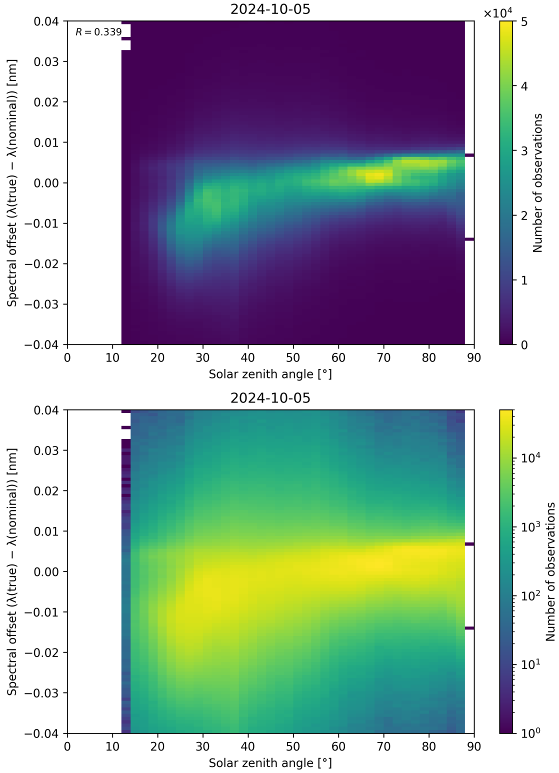
Figure 128: Scatter density plot of “Solar zenith angle” against “Spectral offset ( \lambda_{\text{true}} - \lambda_{\text{nominal}} )” for 2024-10-04 to 2024-10-06.
