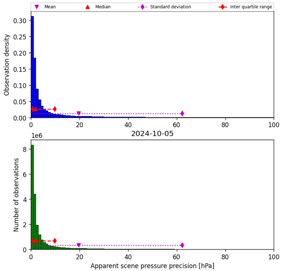
Figure 37: Histogram of “Apparent scene pressure precision” for 2024-10-04 to 2024-10-06
