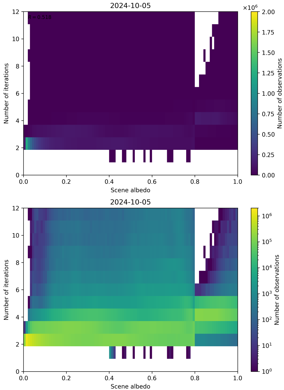
Figure 115: Scatter density plot of “Scene albedo” against “Number of iterations” for 2024-10-04 to 2024-10-06.
