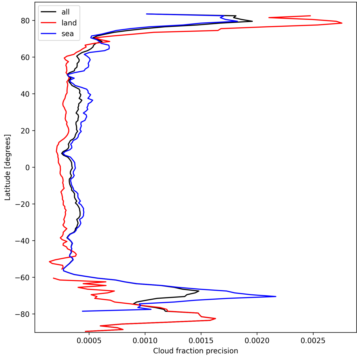
Figure 16: Zonal average of “Cloud fraction precision” for 2024-10-04 to 2024-10-06.
