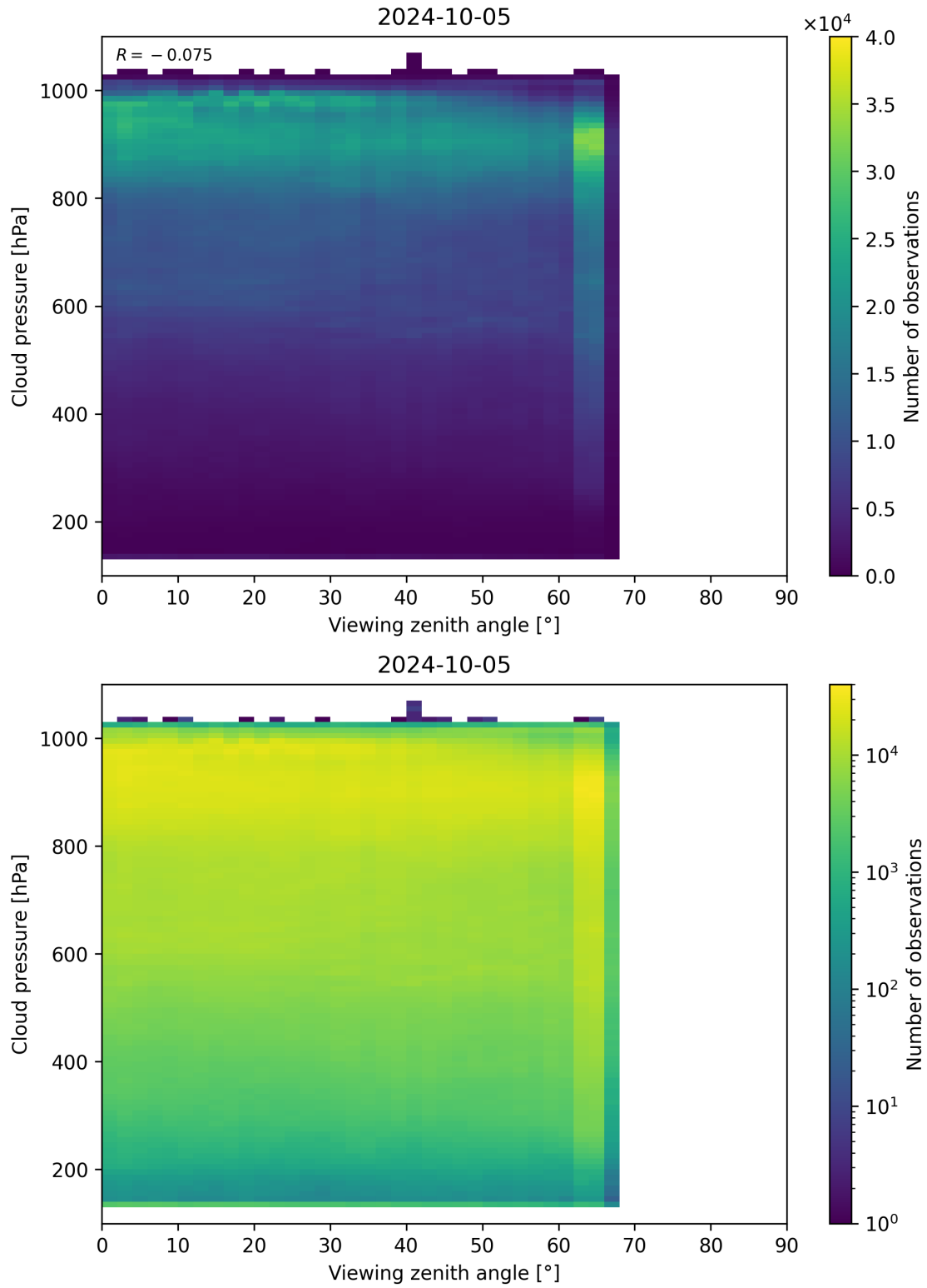
Figure 133: Scatter density plot of “Viewing zenith angle” against “Cloud pressure” for 2024-10-04 to 2024-10-06.
