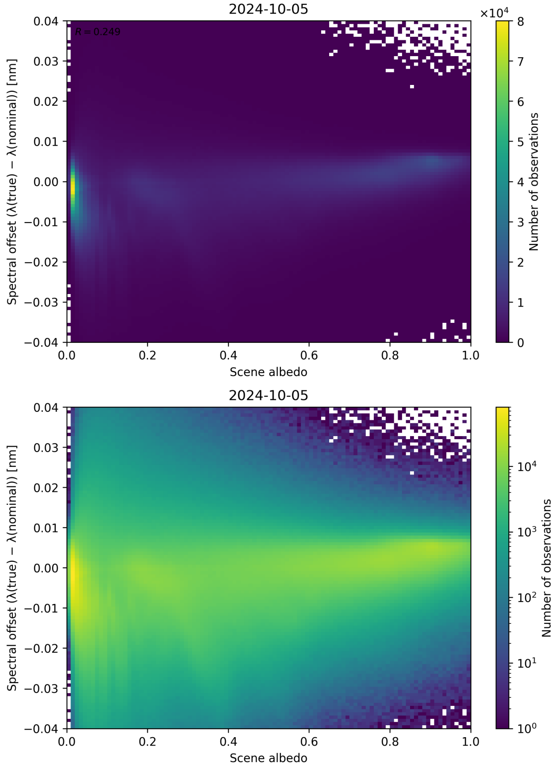
Figure 117: Scatter density plot of “Scene albedo” against “Spectral offset ( \lambda_{\text{true}} - \lambda_{\text{nominal}} )” for 2024-10-04 to 2024-10-06.
