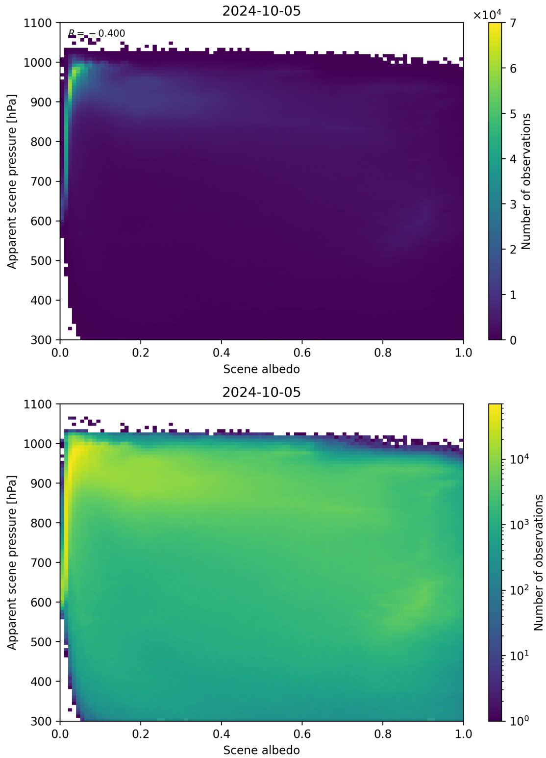
Figure 111: Scatter density plot of “Scene albedo” against “Apparent scene pressure” for 2024-10-04 to 2024-10-06.
