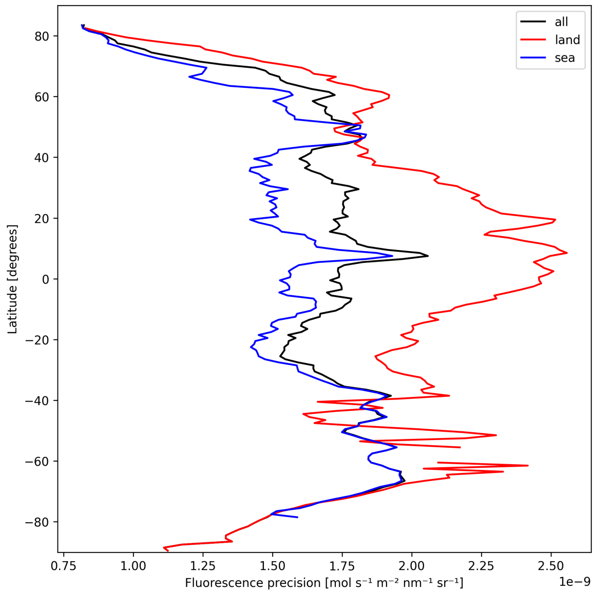
Figure 24: Zonal average of “Fluorescence precision” for 2024-10-04 to 2024-10-06.
