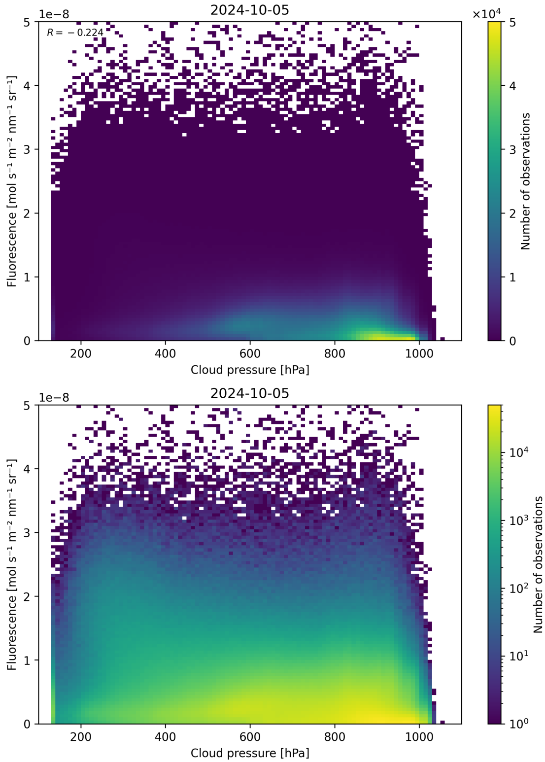
Figure 88: Scatter density plot of “Cloud pressure” against “Fluorescence” for 2024-10-04 to 2024-10-06.
