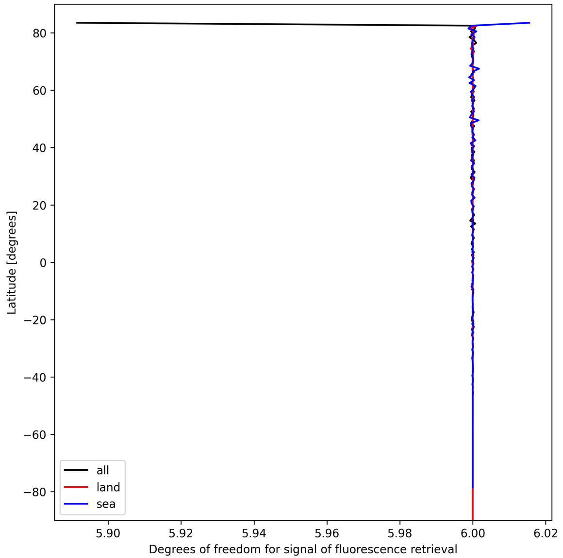
Figure 26: Zonal average of “Degrees of freedom for signal of fluorescence retrieval” for 2024-10-04 to 2024-10-06.
