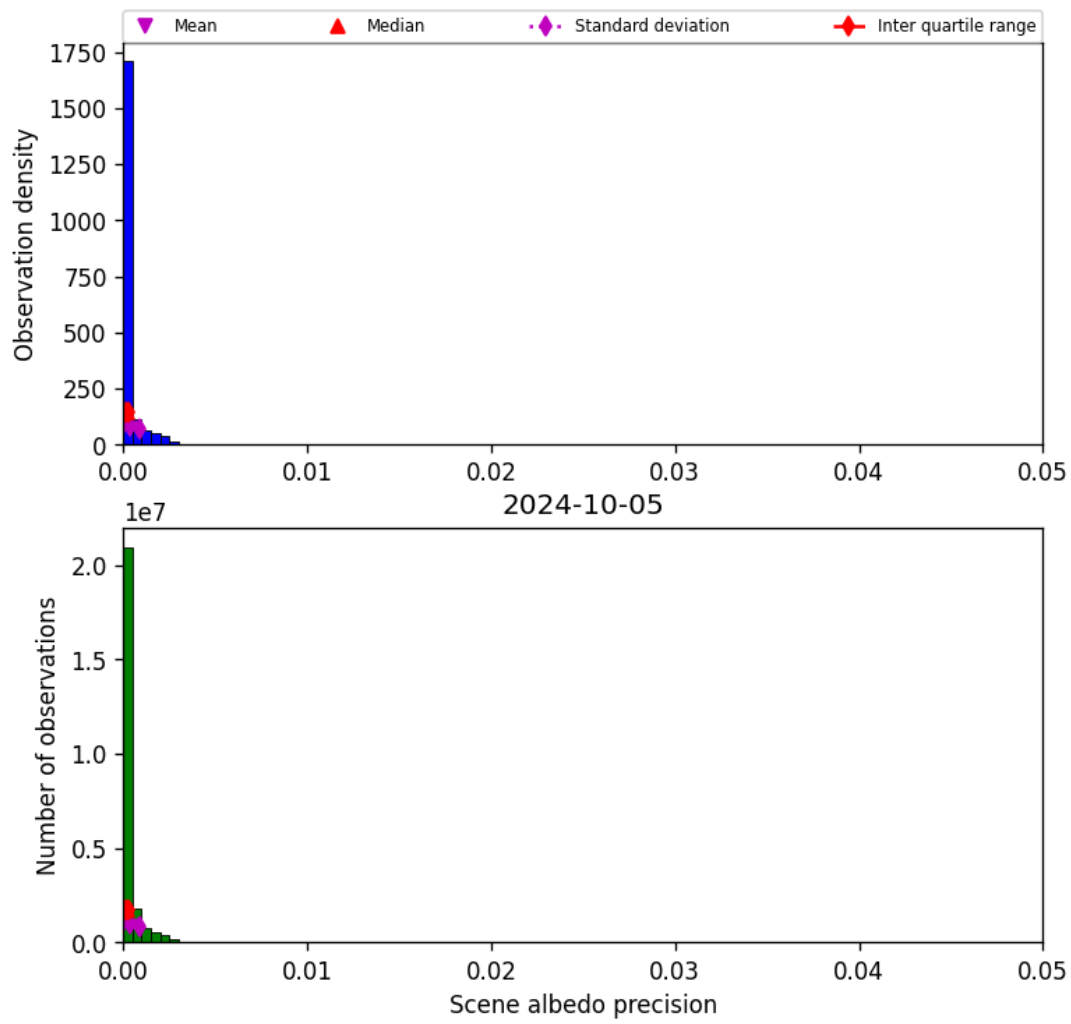
Figure 35: Histogram of “Scene albedo precision” for 2024-10-04 to 2024-10-06
