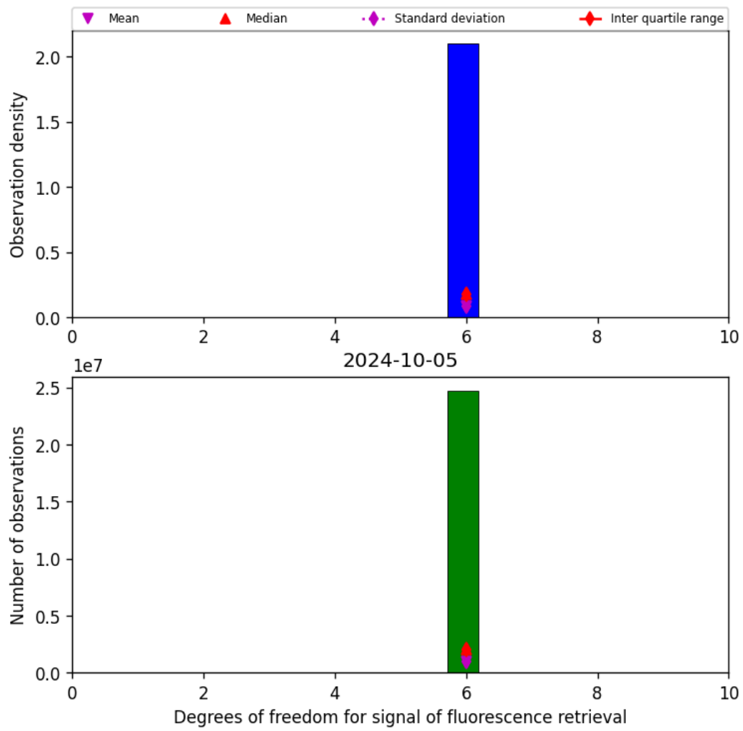
Figure 43: Histogram of "Degrees of freedom for signal of fluorescence retrieval" for 2024-10-04 to 2024-10-06
