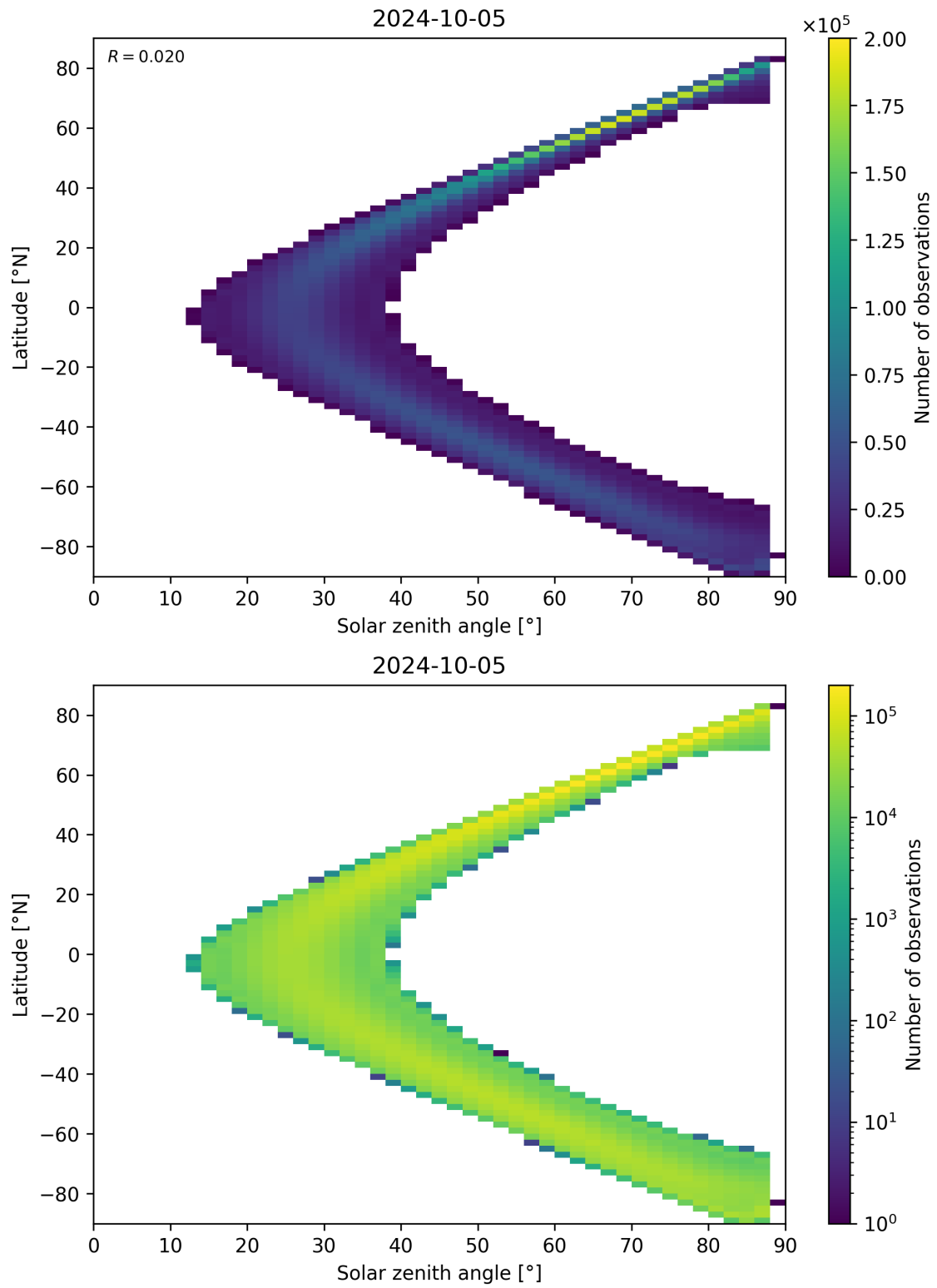
Figure 124: Scatter density plot of “Solar zenith angle” against “Latitude” for 2024-10-04 to 2024-10-06.
