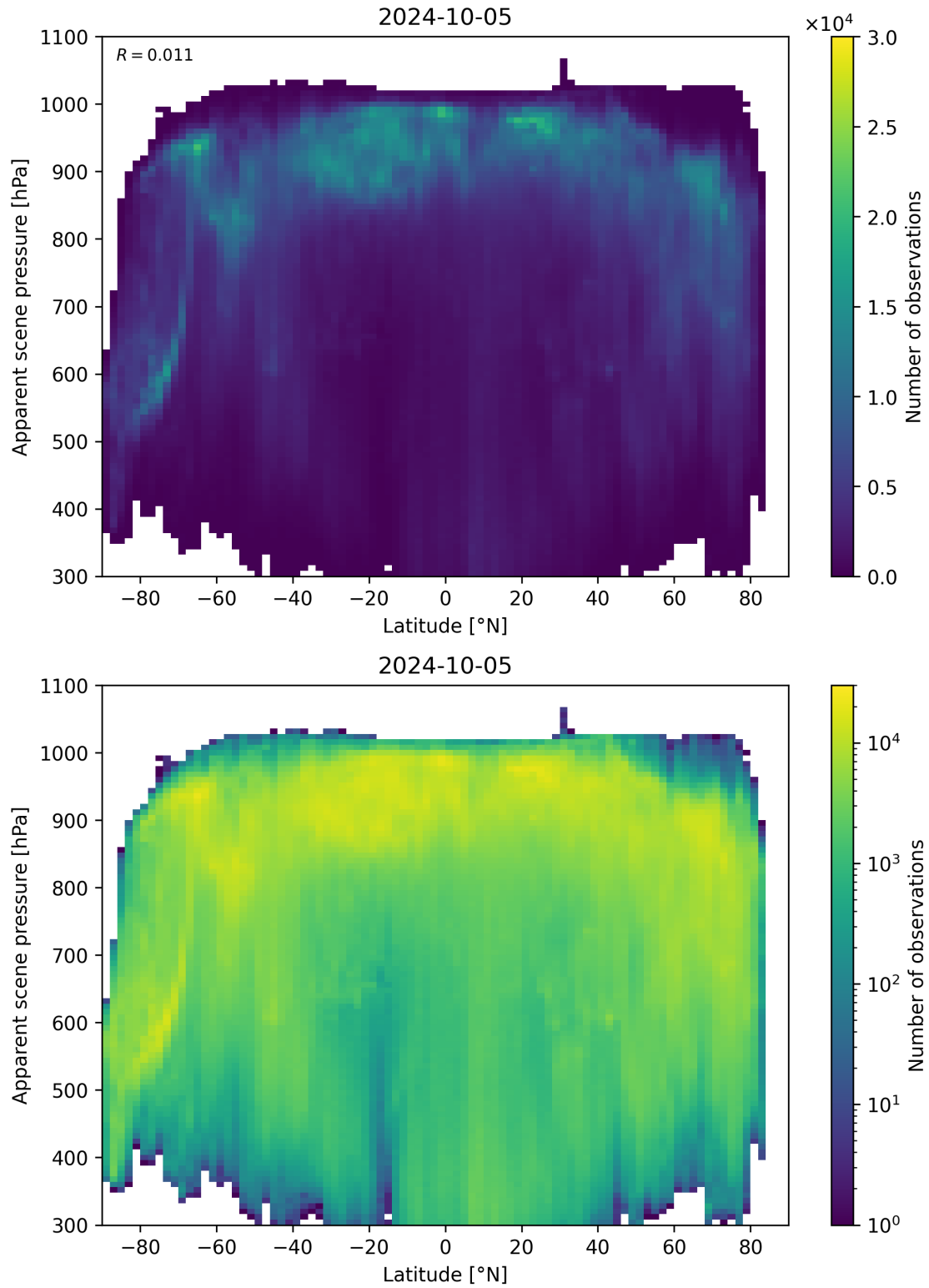
Figure 96: Scatter density plot of “Latitude” against “Apparent scene pressure” for 2024-10-04 to 2024-10-06.
