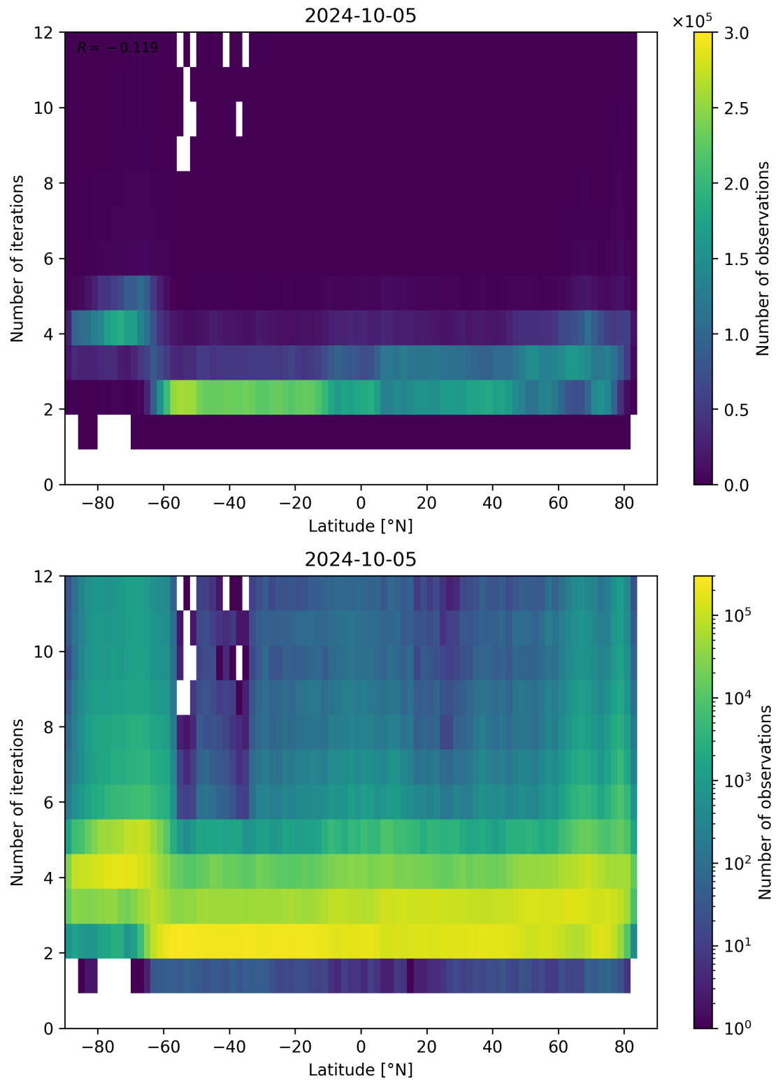
Figure 102: Scatter density plot of “Latitude” against “Number of iterations” for 2024-10-04 to 2024-10-06.
