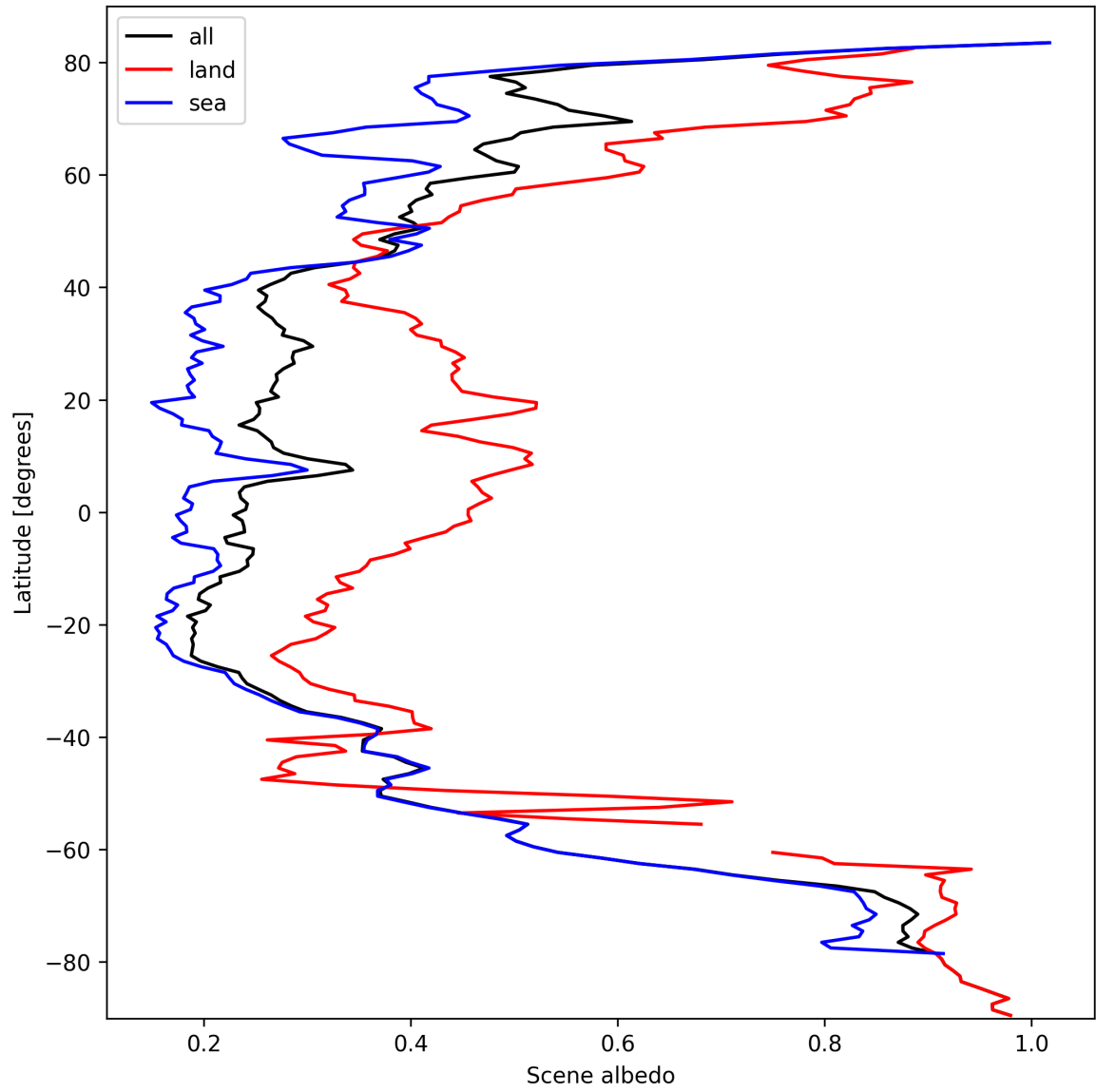
Figure 17: Zonal average of “Scene albedo” for 2024-10-04 to 2024-10-06.
