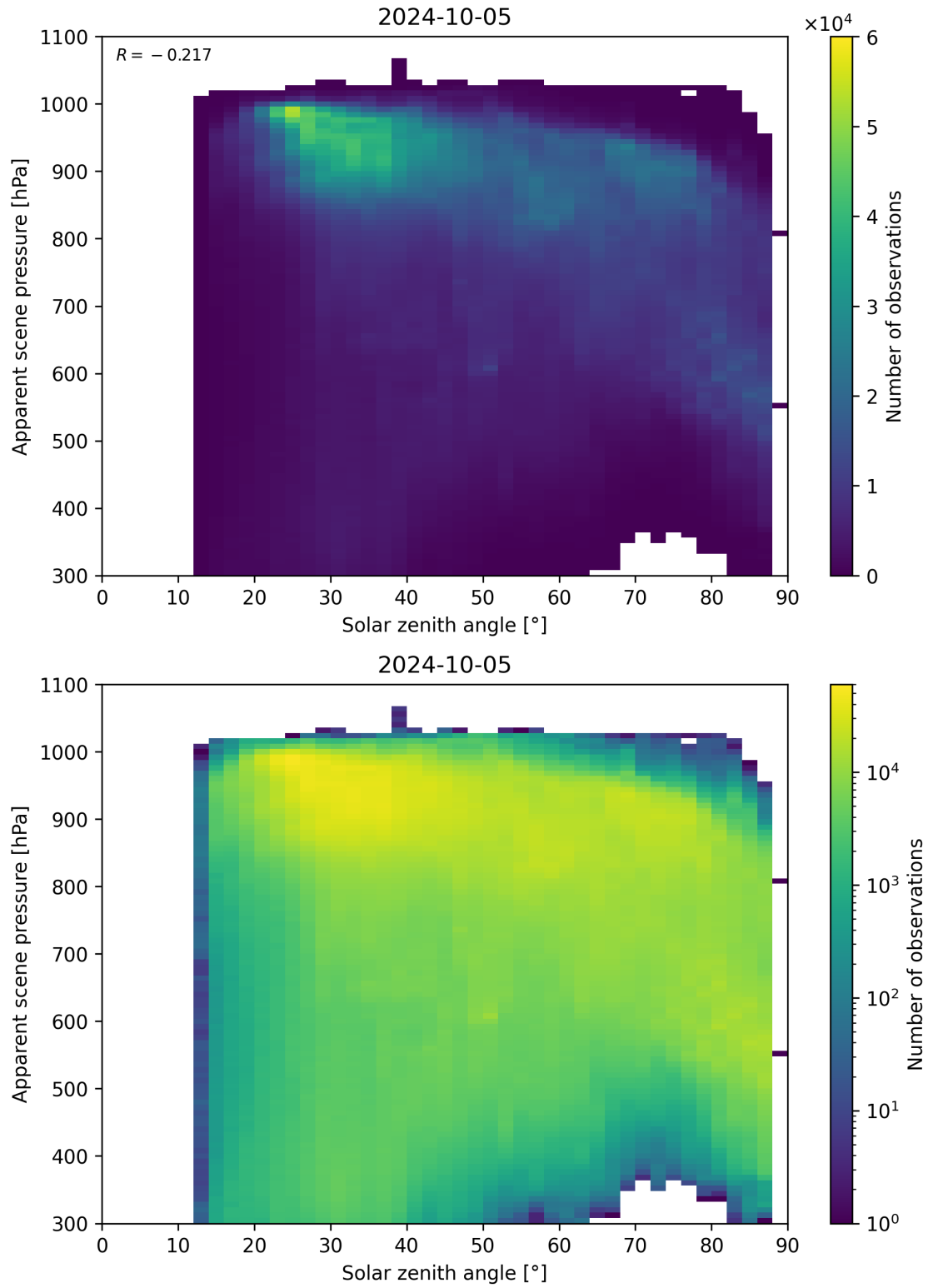
Figure 118: Scatter density plot of “Solar zenith angle” against “Apparent scene pressure” for 2024-10-04 to 2024-10-06.
