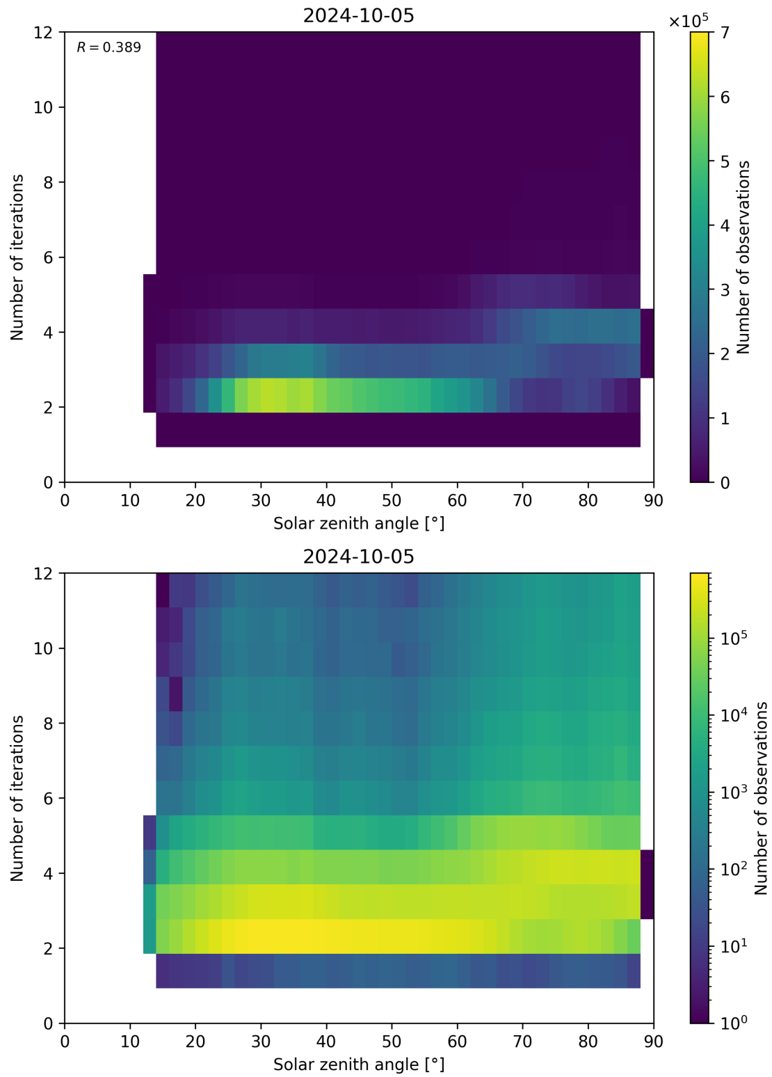
Figure 125: Scatter density plot of “Solar zenith angle” against “Number of iterations” for 2024-10-04 to 2024-10-06.
