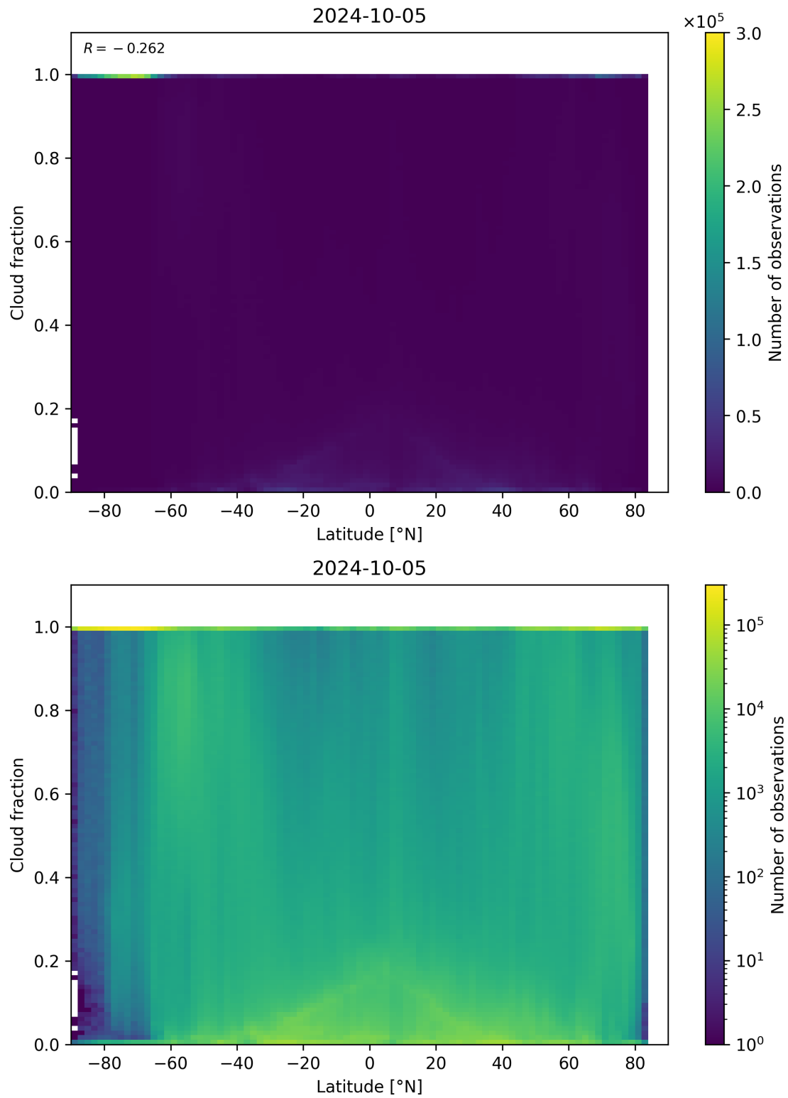
Figure 99: Scatter density plot of “Latitude” against “Cloud fraction” for 2024-10-04 to 2024-10-06.
