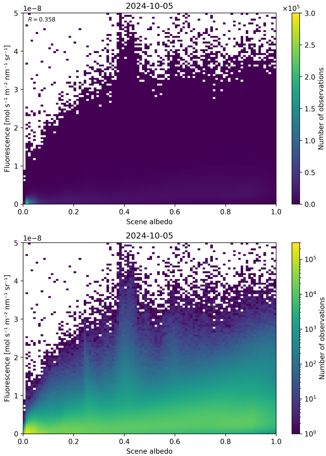
Figure 114: Scatter density plot of “Scene albedo” against “Fluorescence” for 2024-10-04 to 2024-10-06.
