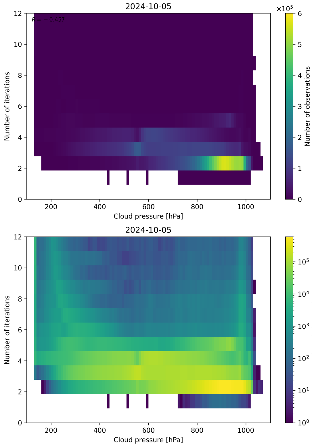
Figure 89: Scatter density plot of “Cloud pressure” against “Number of iterations” for 2024-10-04 to 2024-10-06.
