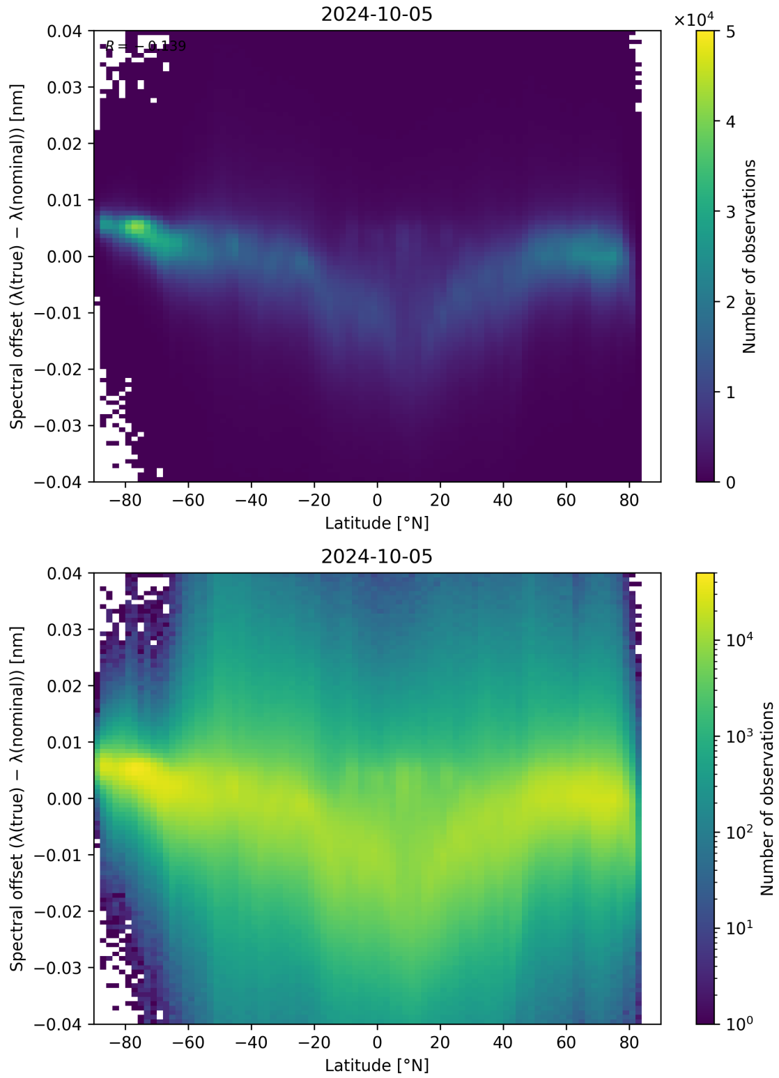
Figure 105: Scatter density plot of “Latitude” against “Spectral offset ( \lambda_{\text{true}} - \lambda_{\text{nominal}} )” for 2024-10-04 to 2024-10-06.
