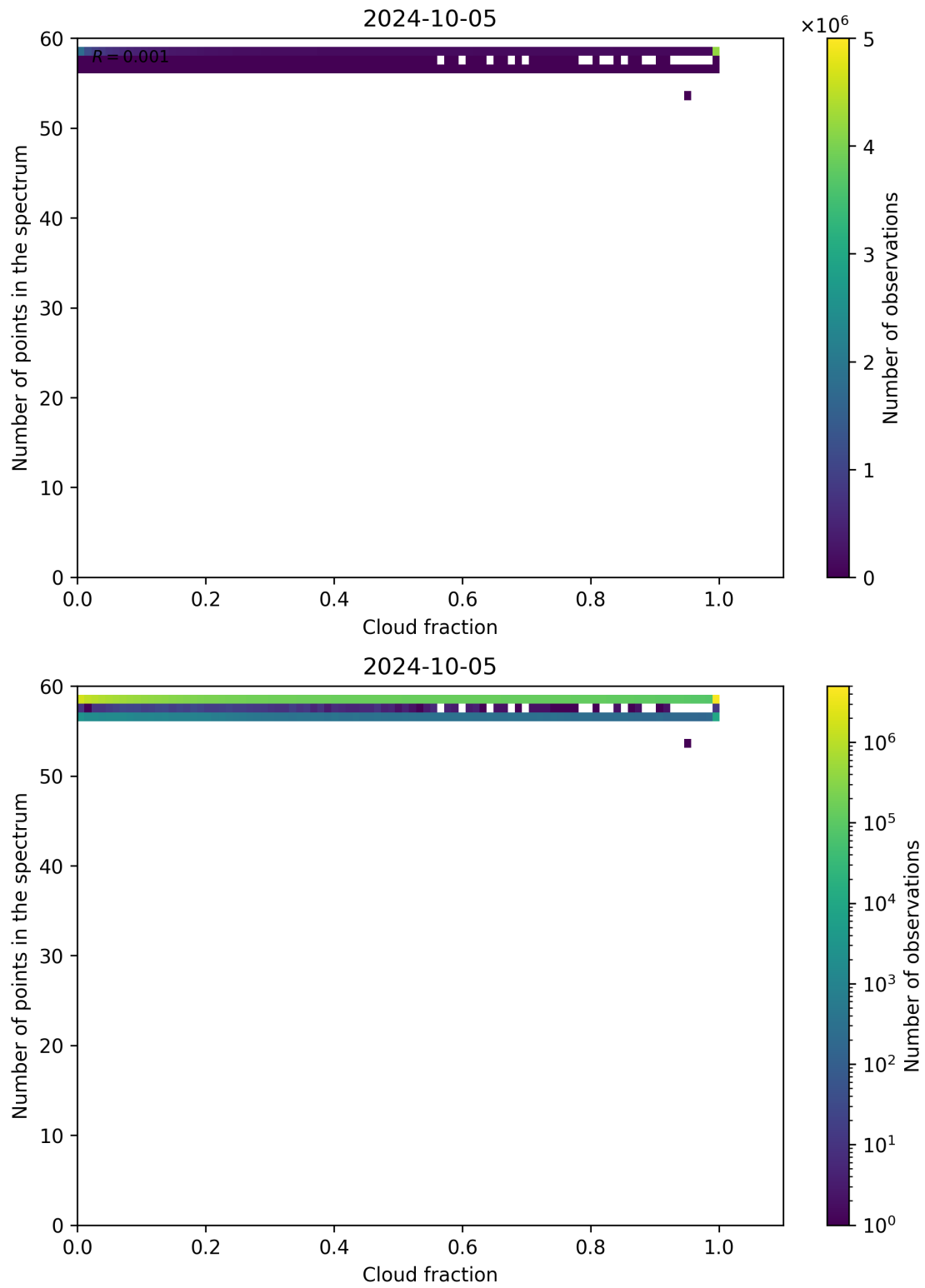
Figure 81: Scatter density plot of “Cloud fraction” against “Number of points in the spectrum” for 2024-10-04 to 2024-10-06.
