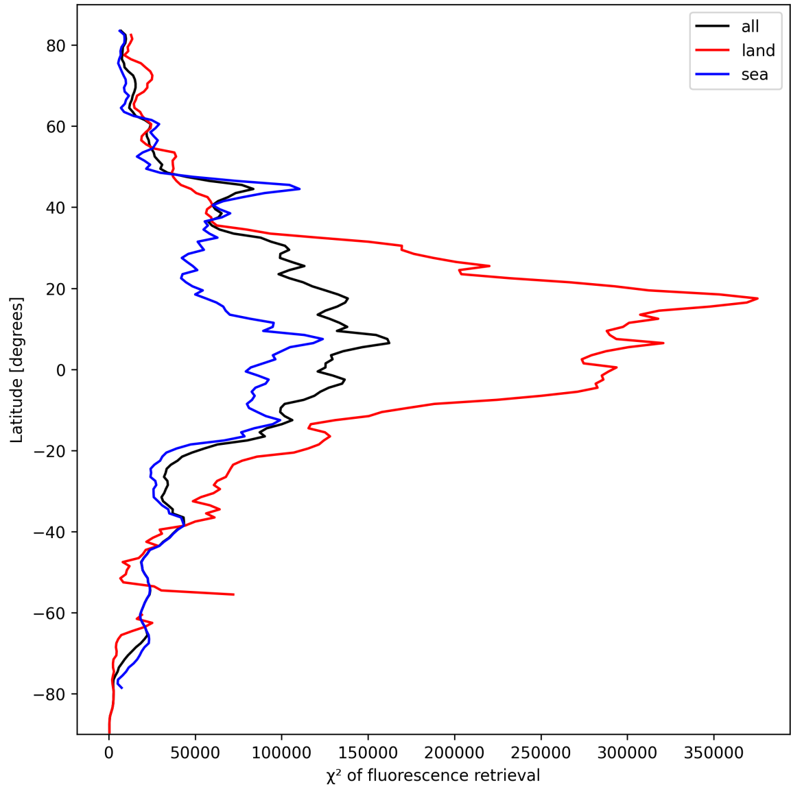
Figure 25: Zonal average of “ \chi^2 of fluorescence retrieval” for 2024-10-04 to 2024-10-06.
