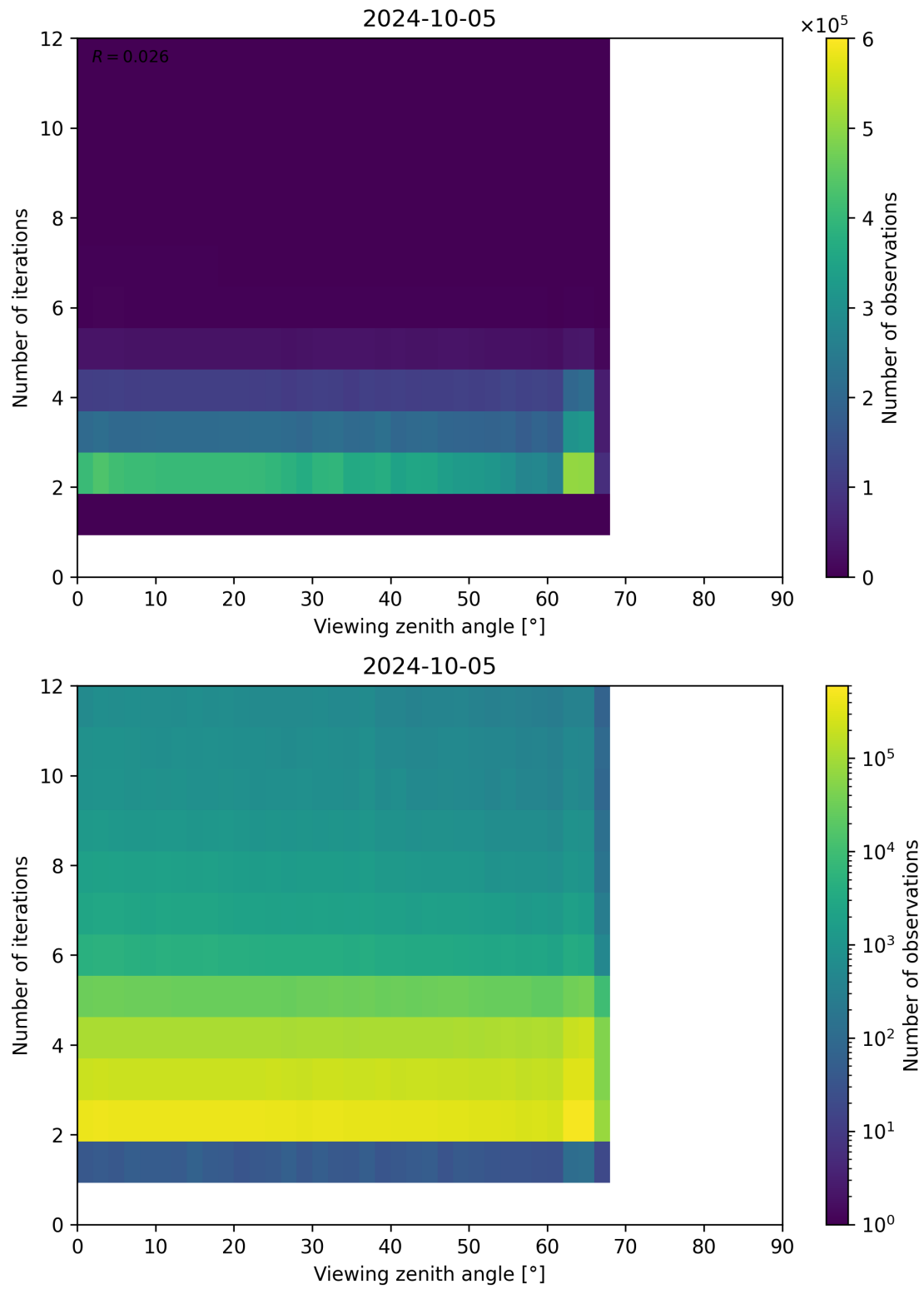
Figure 136: Scatter density plot of “Viewing zenith angle” against “Number of iterations” for 2024-10-04 to 2024-10-06.
