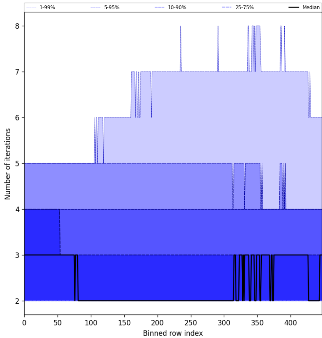
Figure 56: Along track statistics of “Number of iterations” for 2024-10-04 to 2024-10-06
