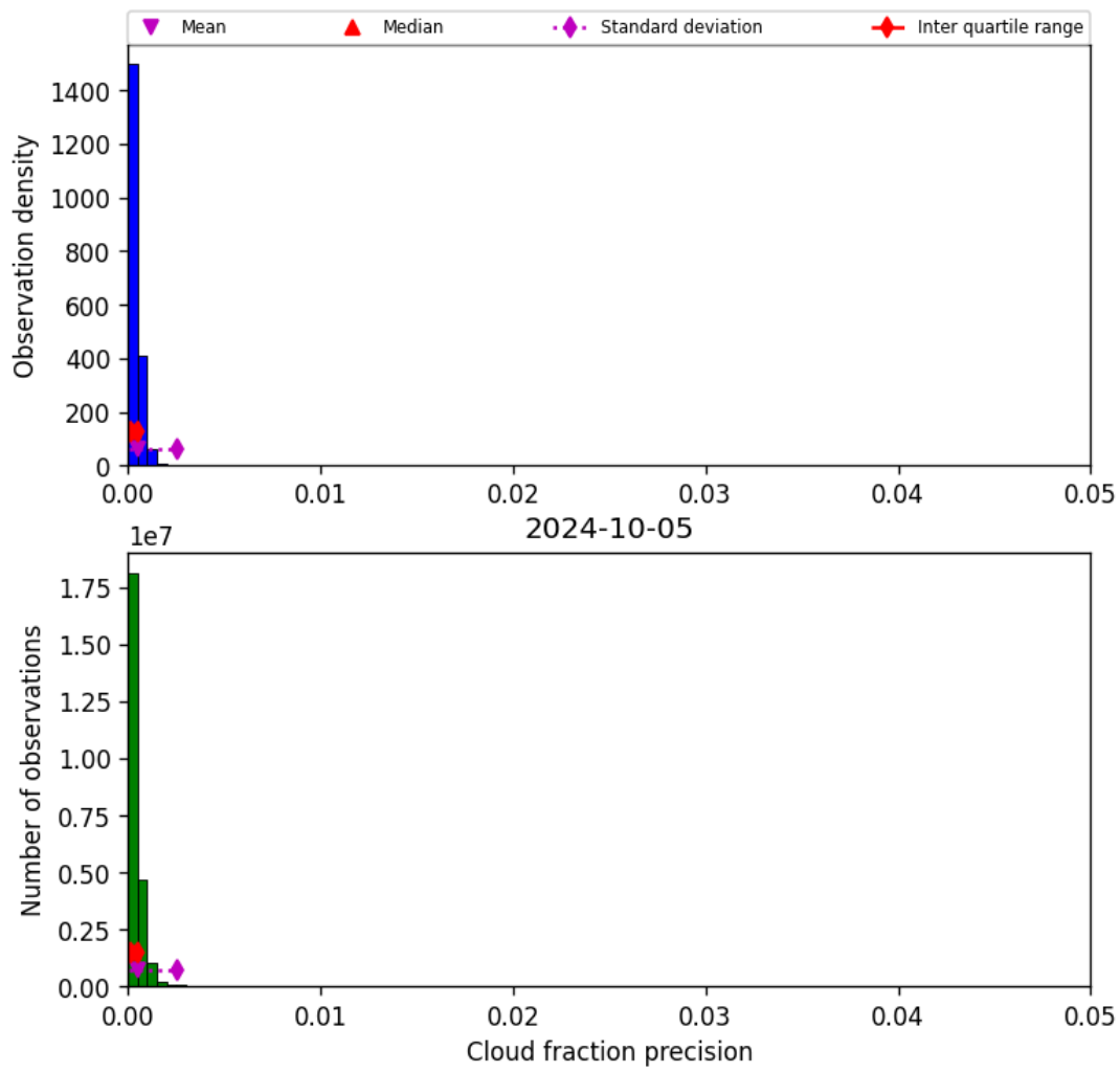
Figure 33: Histogram of “Cloud fraction precision” for 2024-10-04 to 2024-10-06
