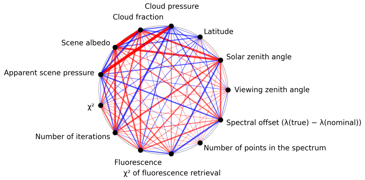
Figure 1: Map of correlation graph for 2024-10-04 to 2024-10-06.
