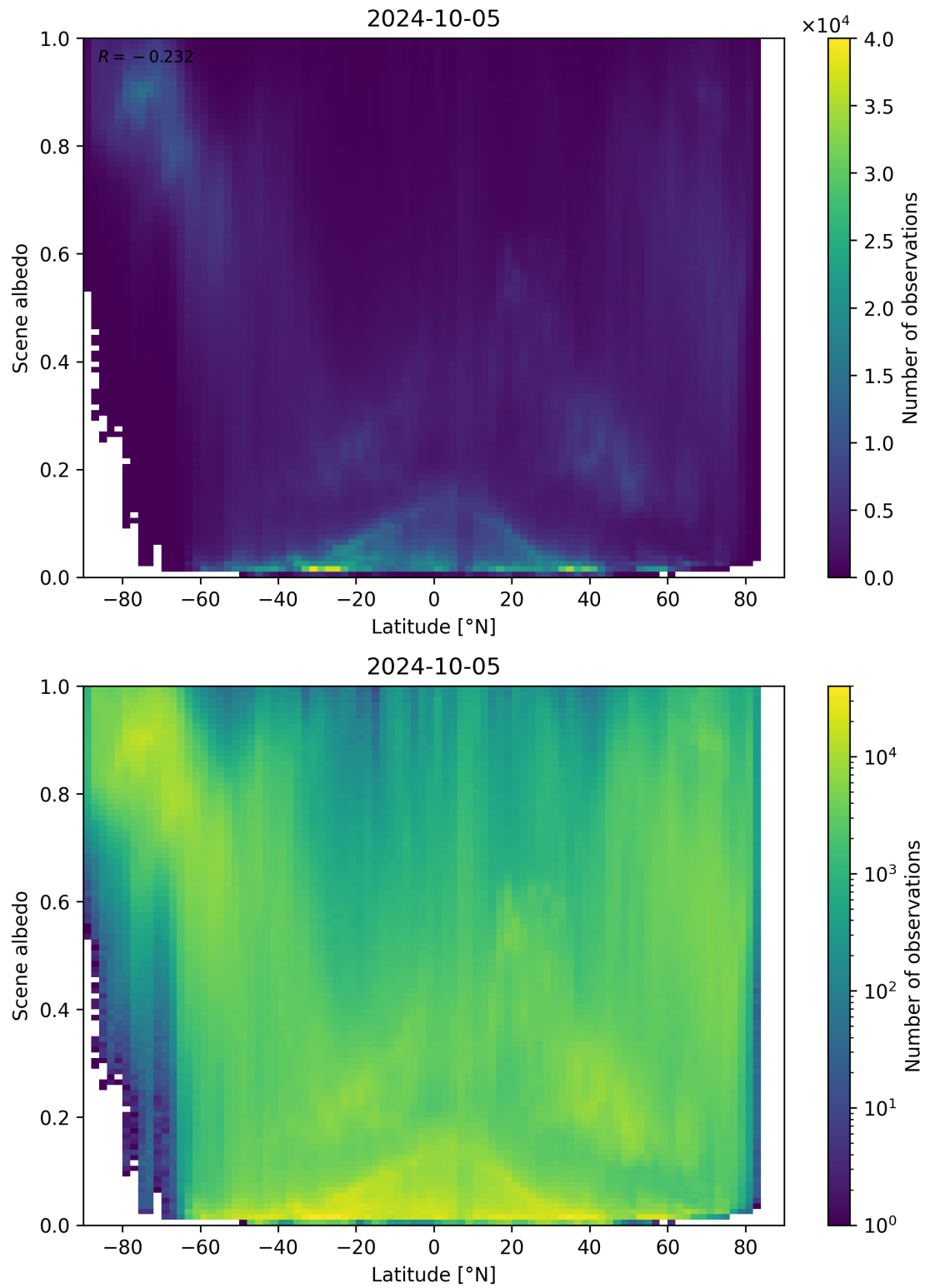
Figure 104: Scatter density plot of “Latitude” against “Scene albedo” for 2024-10-04 to 2024-10-06.
