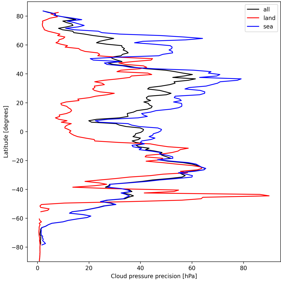
Figure 14: Zonal average of “Cloud pressure precision” for 2024-10-04 to 2024-10-06.
