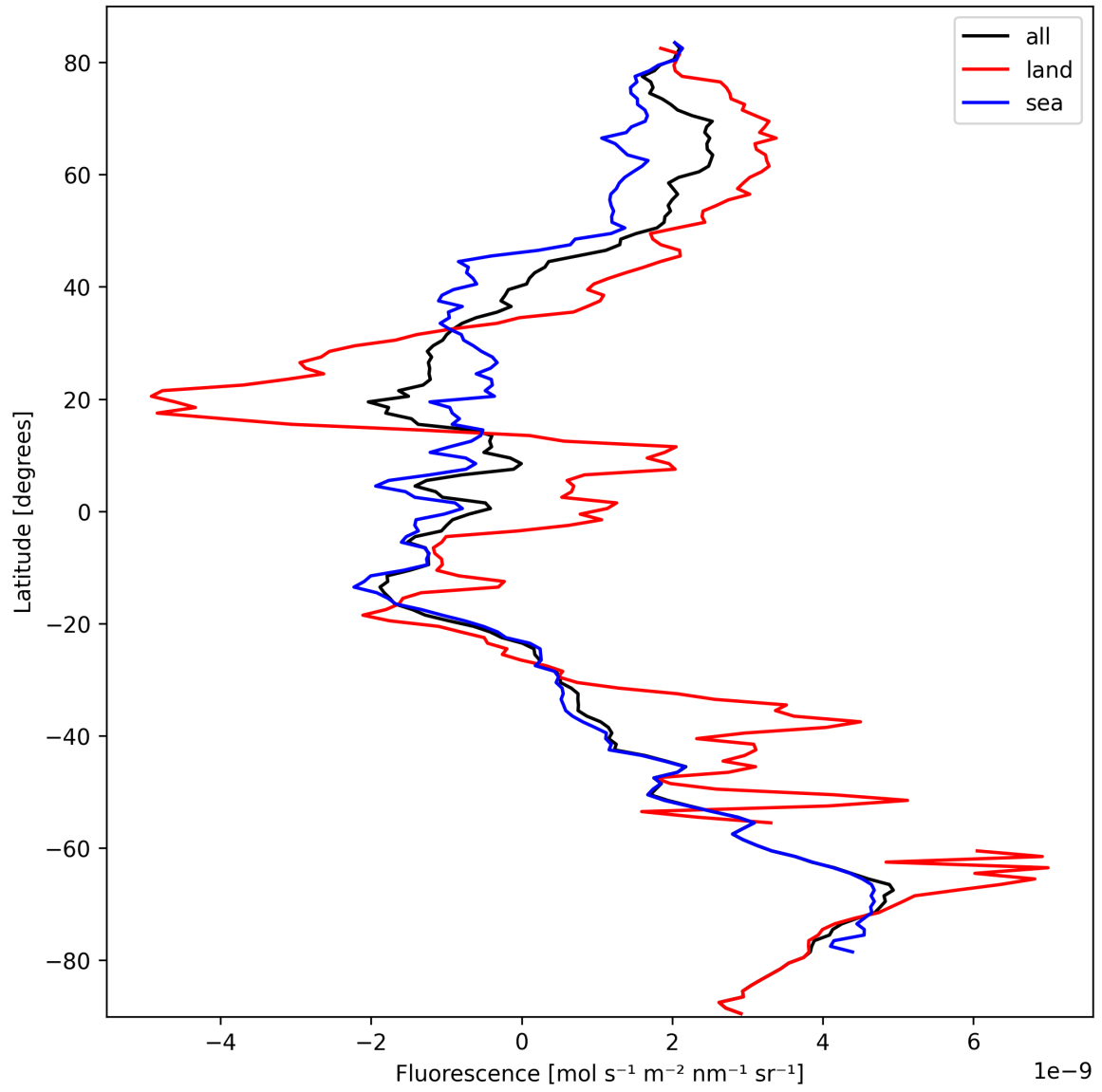
Figure 23: Zonal average of “Fluorescence” for 2024-10-04 to 2024-10-06.
