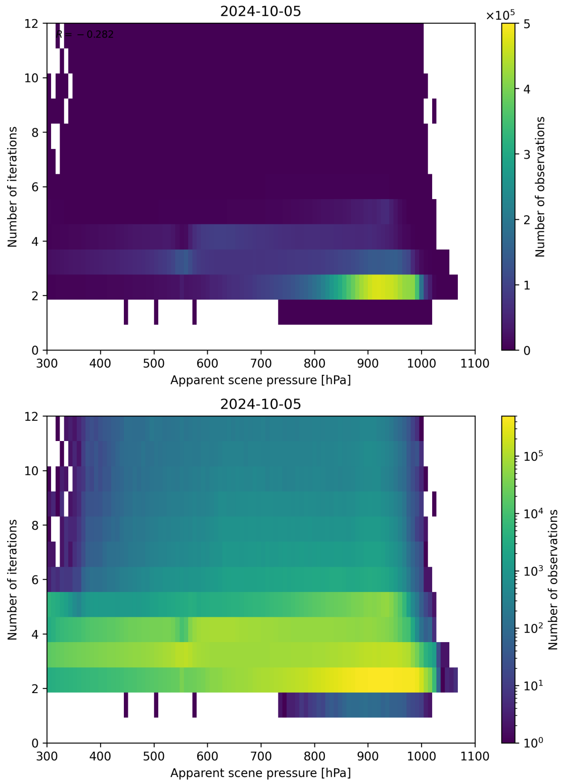
Figure 66: Scatter density plot of “Apparent scene pressure” against “Number of iterations” for 2024-10-04 to 2024-10-06.
