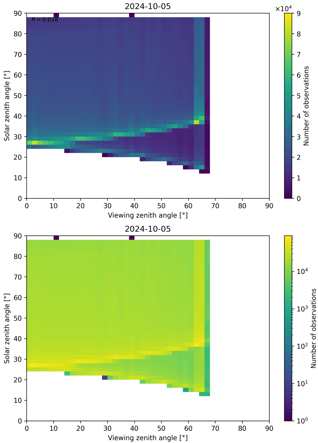
Figure 139: Scatter density plot of “Viewing zenith angle” against “Solar zenith angle” for 2024-10-04 to 2024-10-06.
