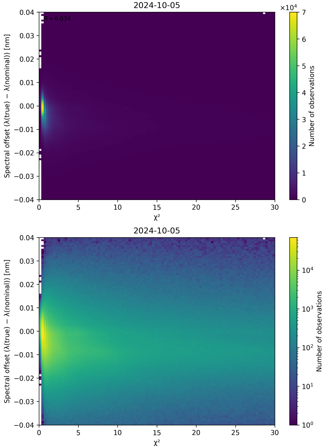
Figure 75: Scatter density plot of “ \chi^2 ” against “Spectral offset ( \lambda_{\text{true}} - \lambda_{\text{nominal}} )” for 2024-10-04 to 2024-10-06.
