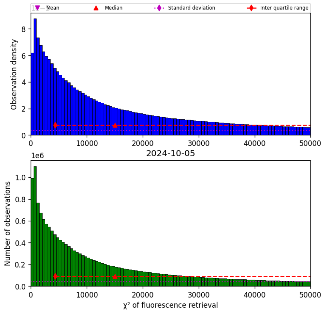
Figure 42: Histogram of “ \chi^2 of fluorescence retrieval” for 2024-10-04 to 2024-10-06
