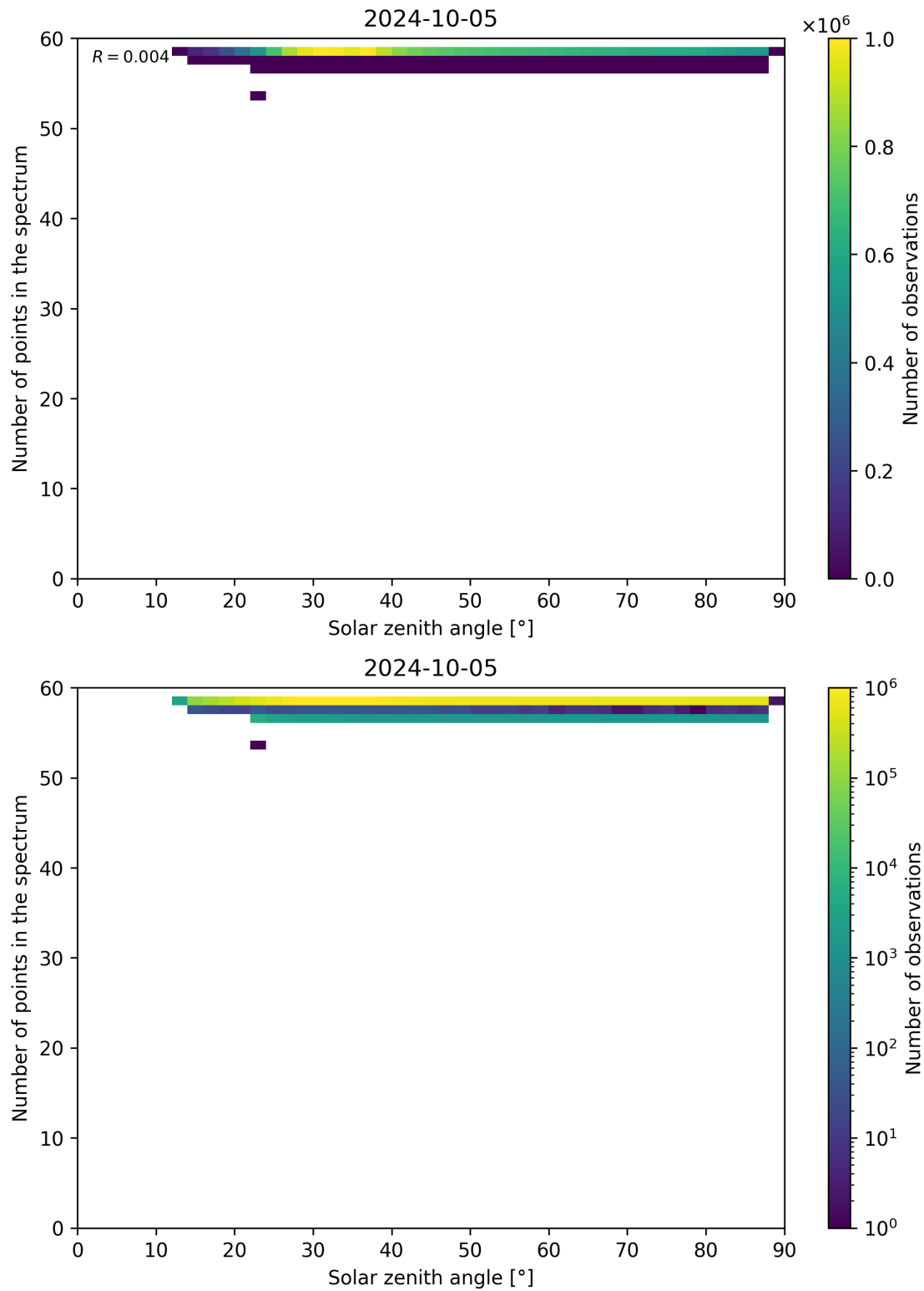
Figure 126: Scatter density plot of “Solar zenith angle” against “Number of points in the spectrum” for 2024-10-04 to 2024-10-06.
