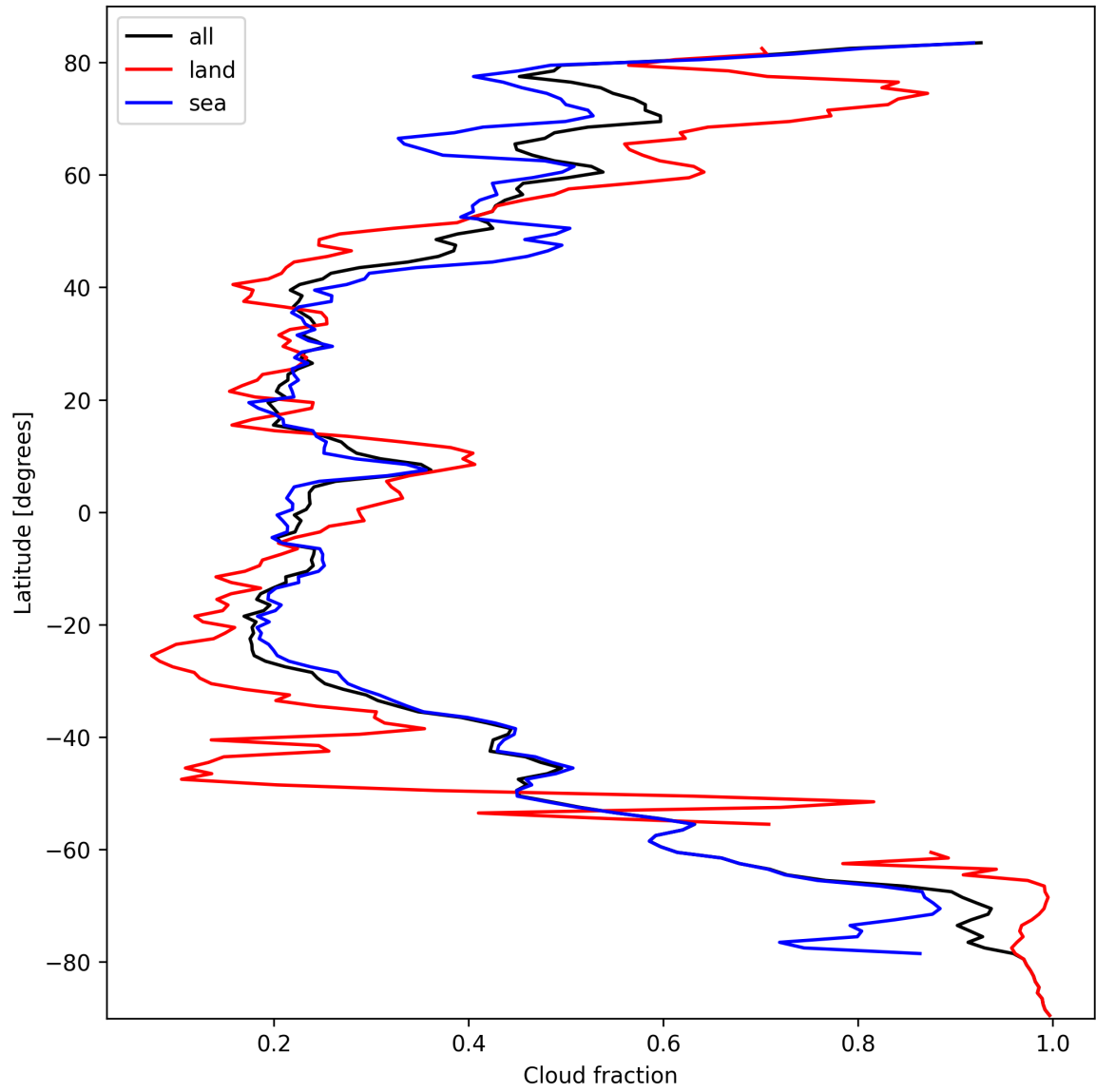
Figure 15: Zonal average of “Cloud fraction” for 2024-10-04 to 2024-10-06.
