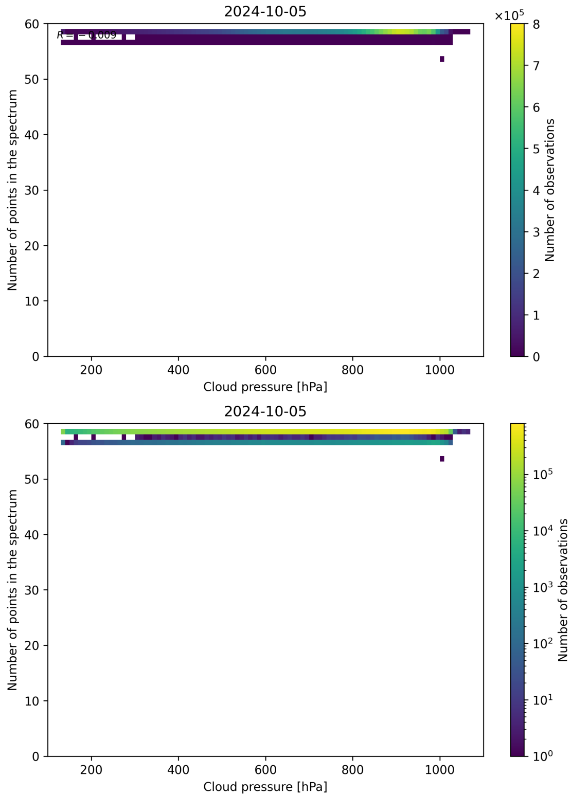
Figure 90: Scatter density plot of “Cloud pressure” against “Number of points in the spectrum” for 2024-10-04 to 2024-10-06.
