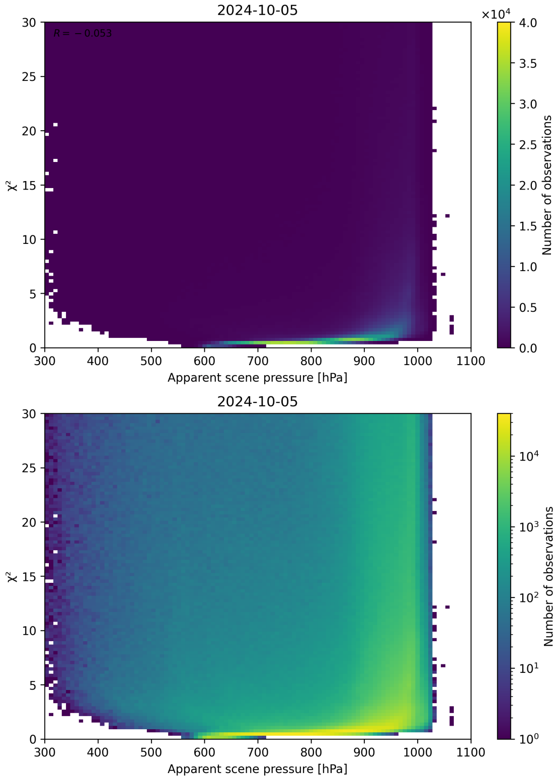
Figure 63: Scatter density plot of “Apparent scene pressure” against “ \chi^2 ” for 2024-10-04 to 2024-10-06.
