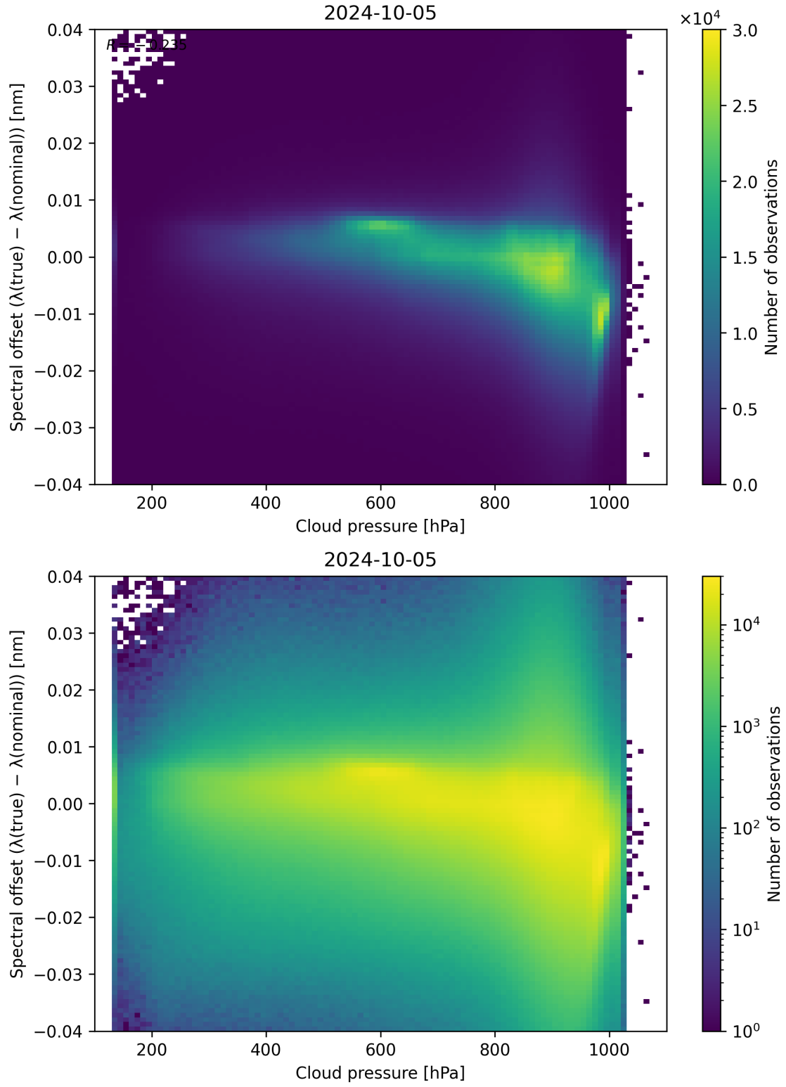
Figure 92: Scatter density plot of “Cloud pressure” against “Spectral offset ( \lambda_{\text{true}} - \lambda_{\text{nominal}} )” for 2024-10-04 to 2024-10-06.
