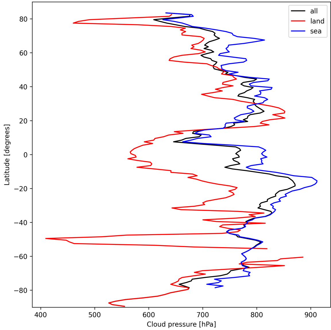
Figure 13: Zonal average of “Cloud pressure” for 2024-10-04 to 2024-10-06.
