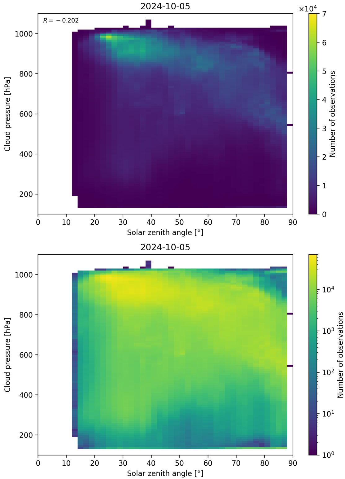
Figure 122: Scatter density plot of “Solar zenith angle” against “Cloud pressure” for 2024-10-04 to 2024-10-06.
