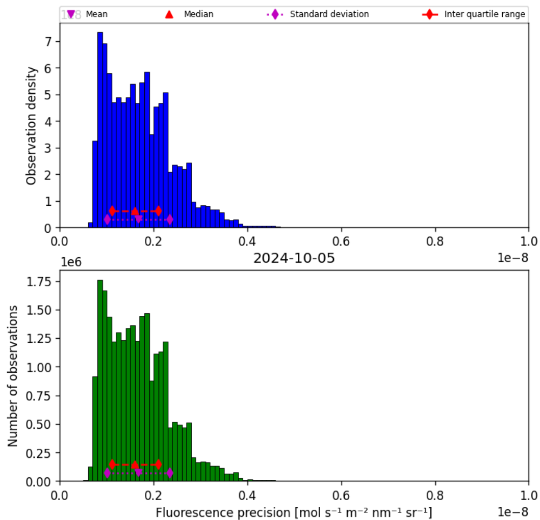
Figure 41: Histogram of “Fluorescence precision” for 2024-10-04 to 2024-10-06
