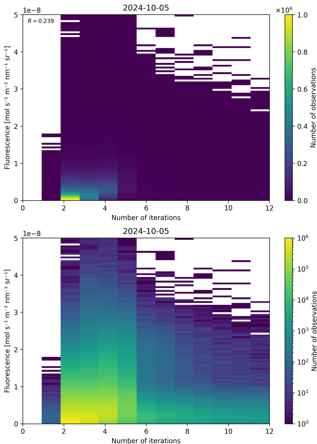
Figure 107: Scatter density plot of “Number of iterations” against “Fluorescence” for 2024-10-04 to 2024-10-06.
