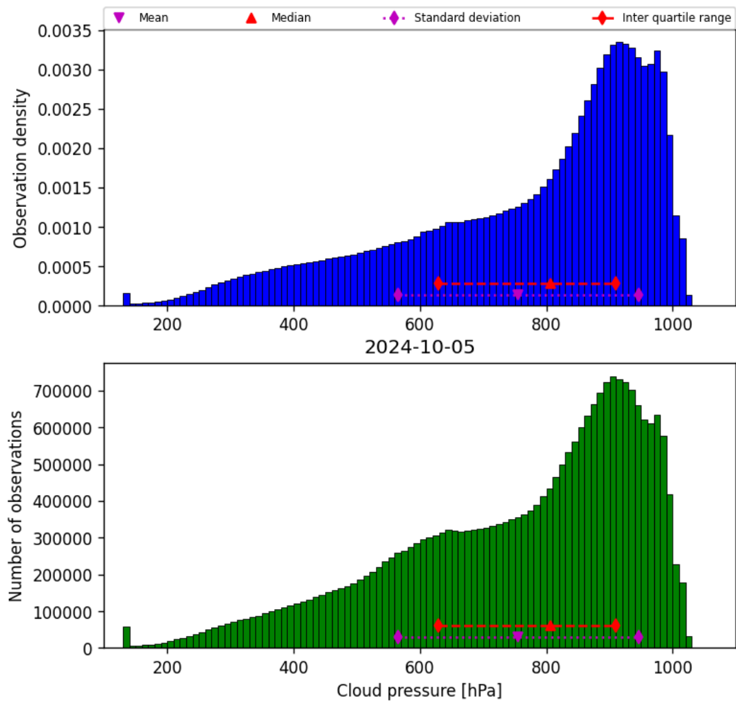
Figure 30: Histogram of “Cloud pressure” for 2024-10-04 to 2024-10-06
