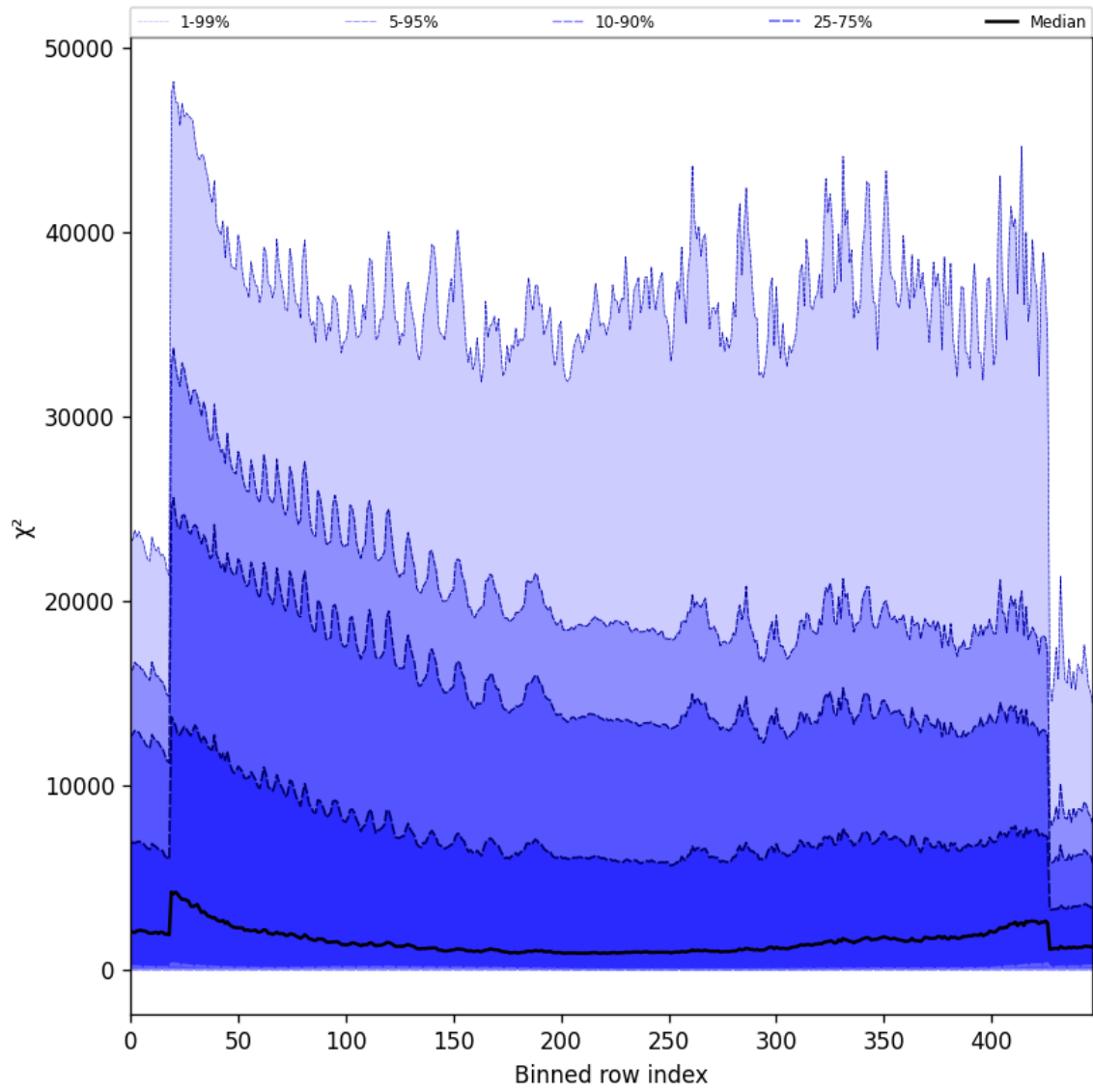
Figure 55: Along track statistics of “ \chi^2 ” for 2024-10-04 to 2024-10-06
