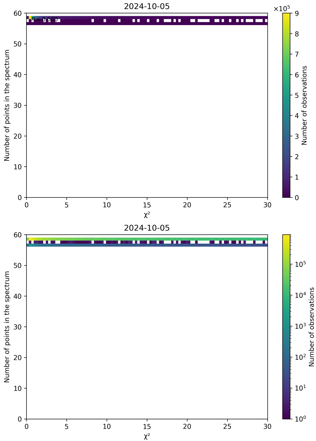
Figure 74: Scatter density plot of “ \chi^2 ” against “Number of points in the spectrum” for 2024-10-04 to 2024-10-06.
