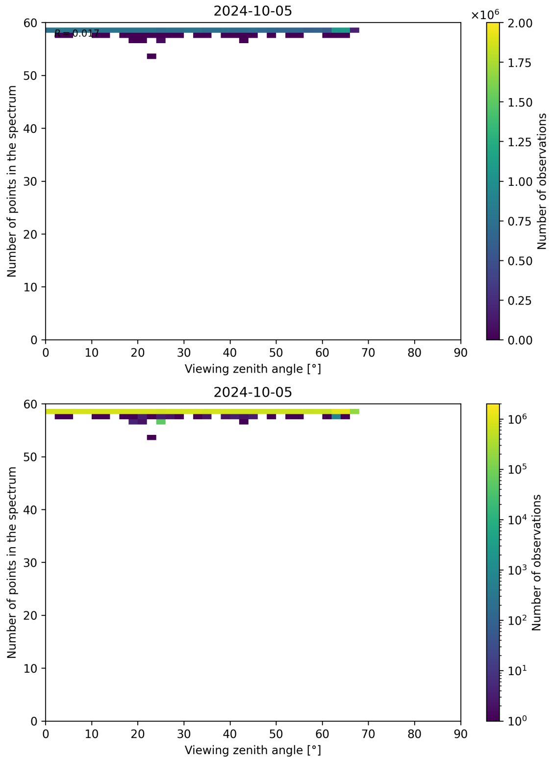
Figure 137: Scatter density plot of “Viewing zenith angle” against “Number of points in the spectrum” for 2024-10-04 to 2024-10-06.
