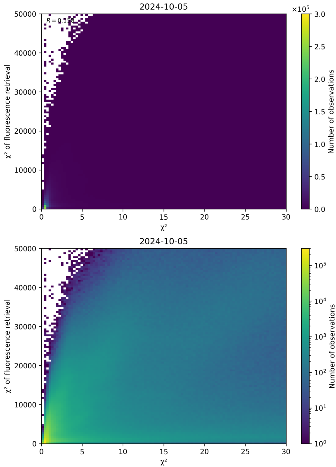
Figure 69: Scatter density plot of “ \chi^2 ” against “ \chi^2 of fluorescence retrieval” for 2024-10-04 to 2024-10-06.
