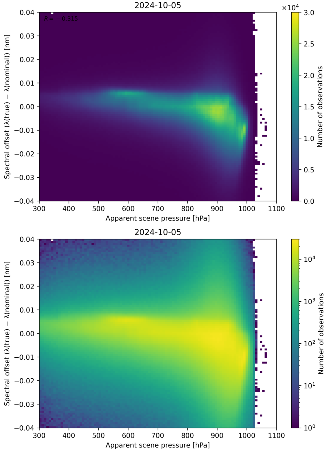
Figure 68: Scatter density plot of “Apparent scene pressure” against “Spectral offset ( \lambda_{\text{true}} - \lambda_{\text{nominal}} )” for 2024-10-04 to 2024-10-06.
