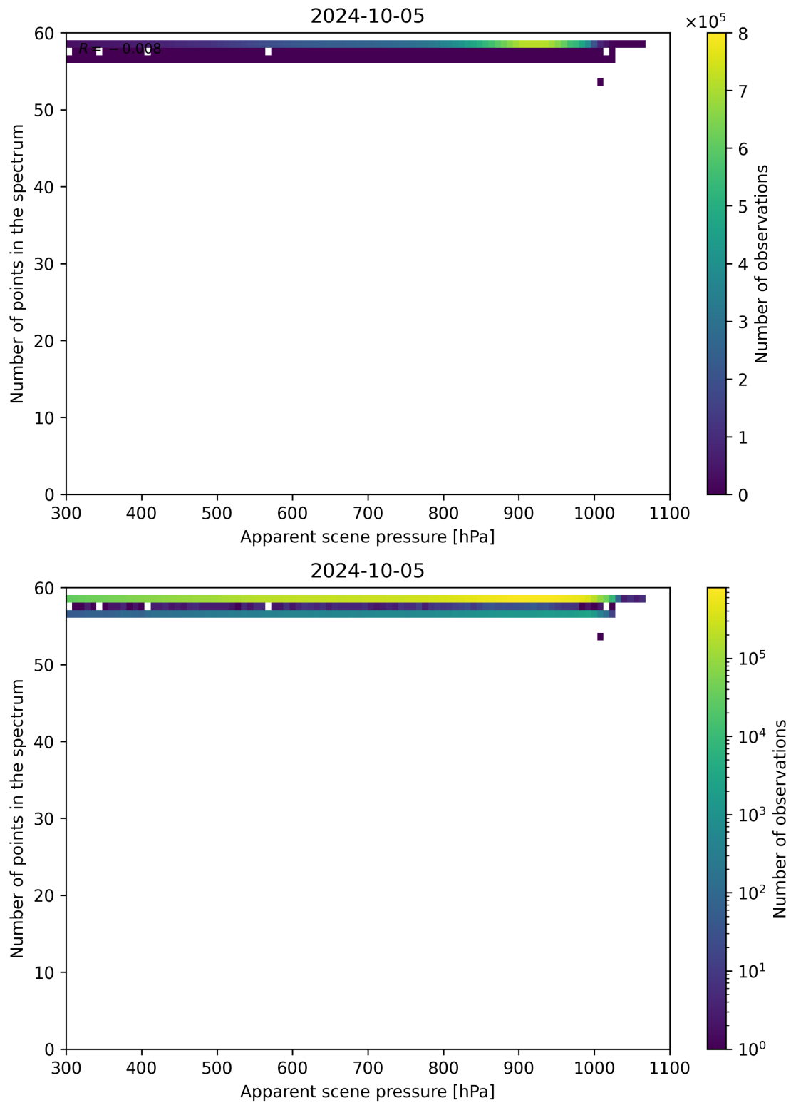
Figure 67: Scatter density plot of “Apparent scene pressure” against “Number of points in the spectrum” for 2024-10-04 to 2024-10-06.
