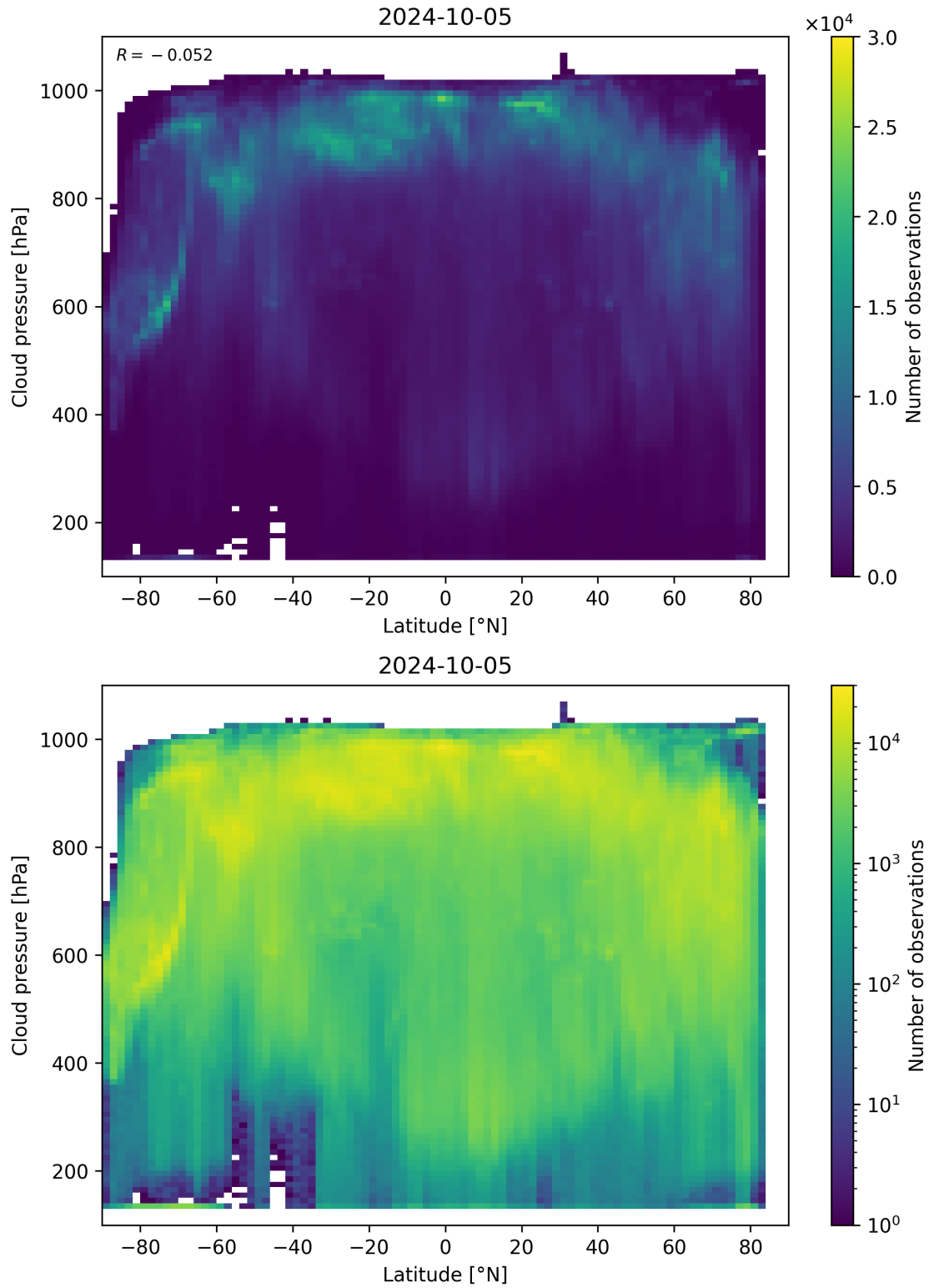
Figure 100: Scatter density plot of “Latitude” against “Cloud pressure” for 2024-10-04 to 2024-10-06.
