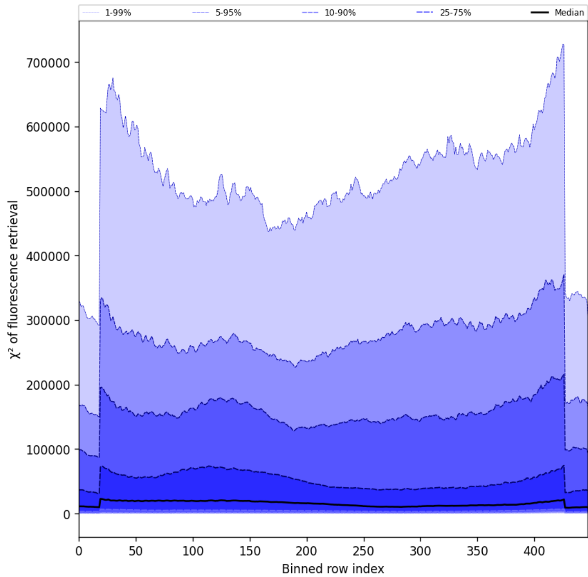
Figure 59: Along track statistics of “ \chi^2 of fluorescence retrieval” for 2024-10-04 to 2024-10-06
