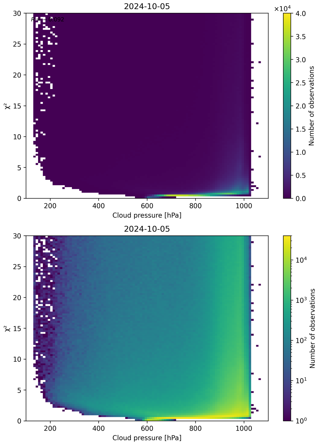
Figure 85: Scatter density plot of “Cloud pressure” against “ \chi^2 ” for 2024-10-04 to 2024-10-06.
