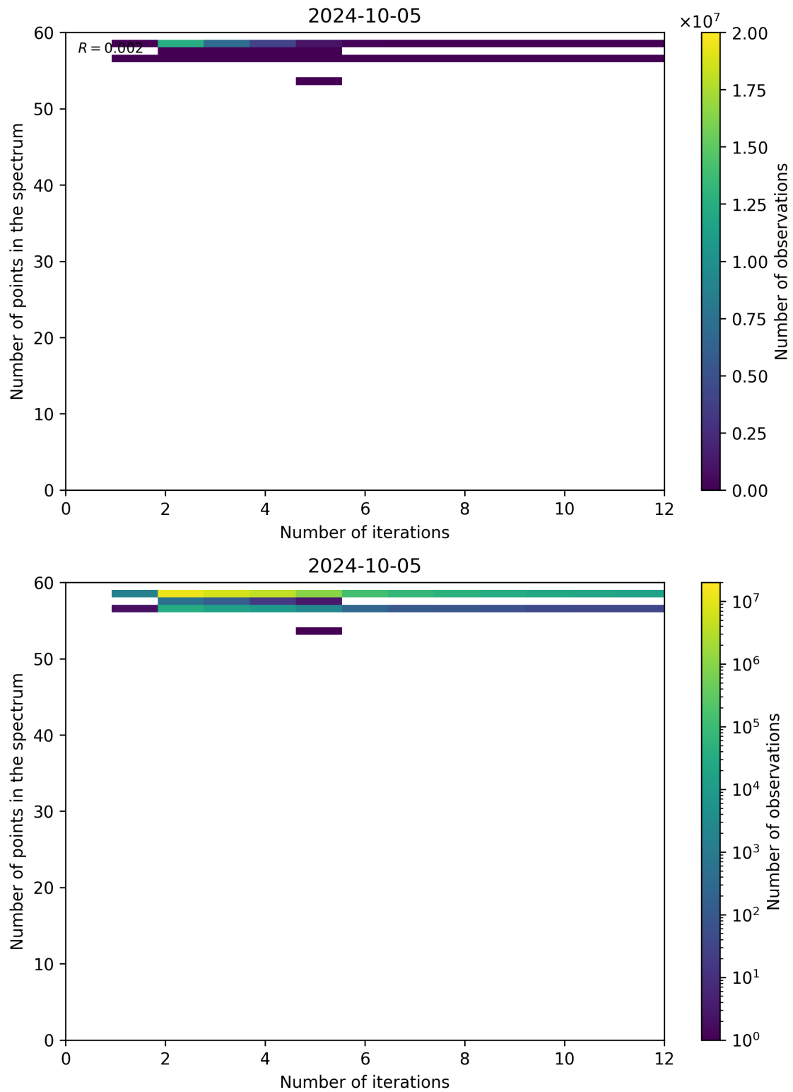
Figure 108: Scatter density plot of “Number of iterations” against “Number of points in the spectrum” for 2024-10-04 to 2024-10-06.
