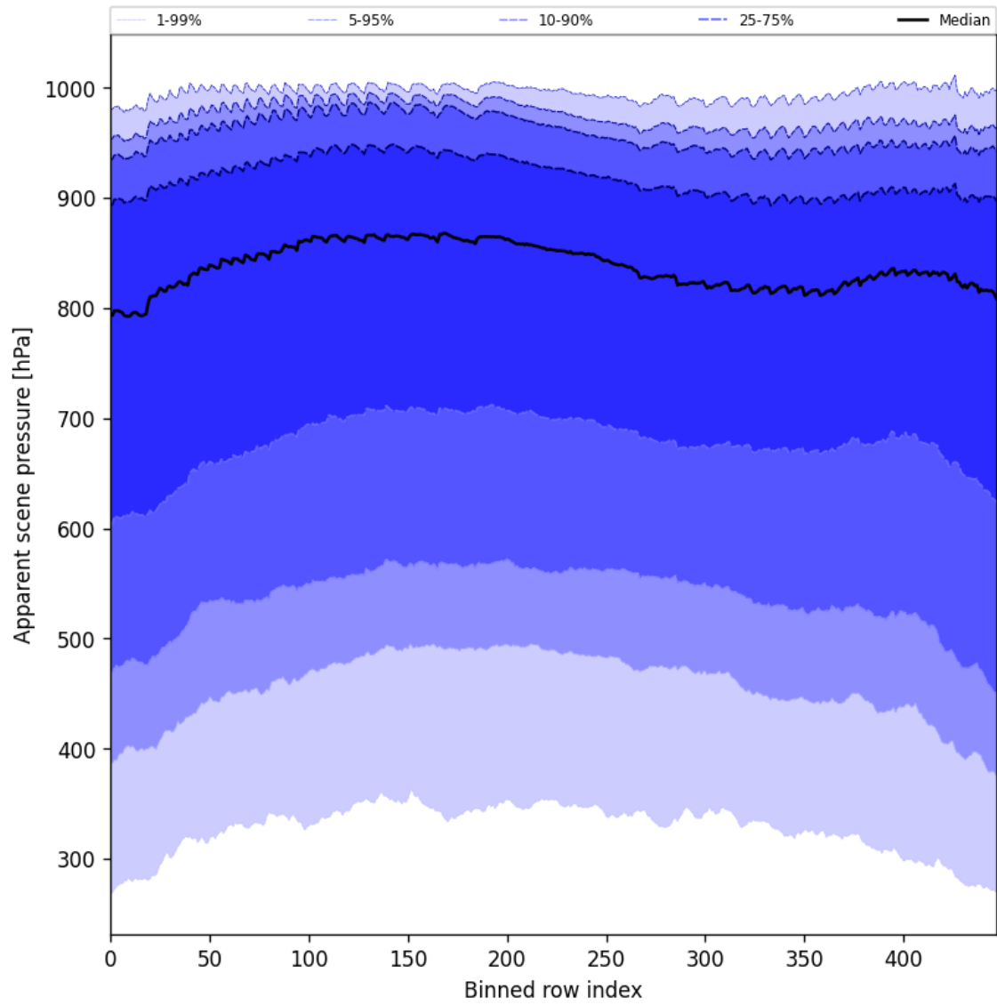
Figure 53: Along track statistics of “Apparent scene pressure” for 2024-10-04 to 2024-10-06
