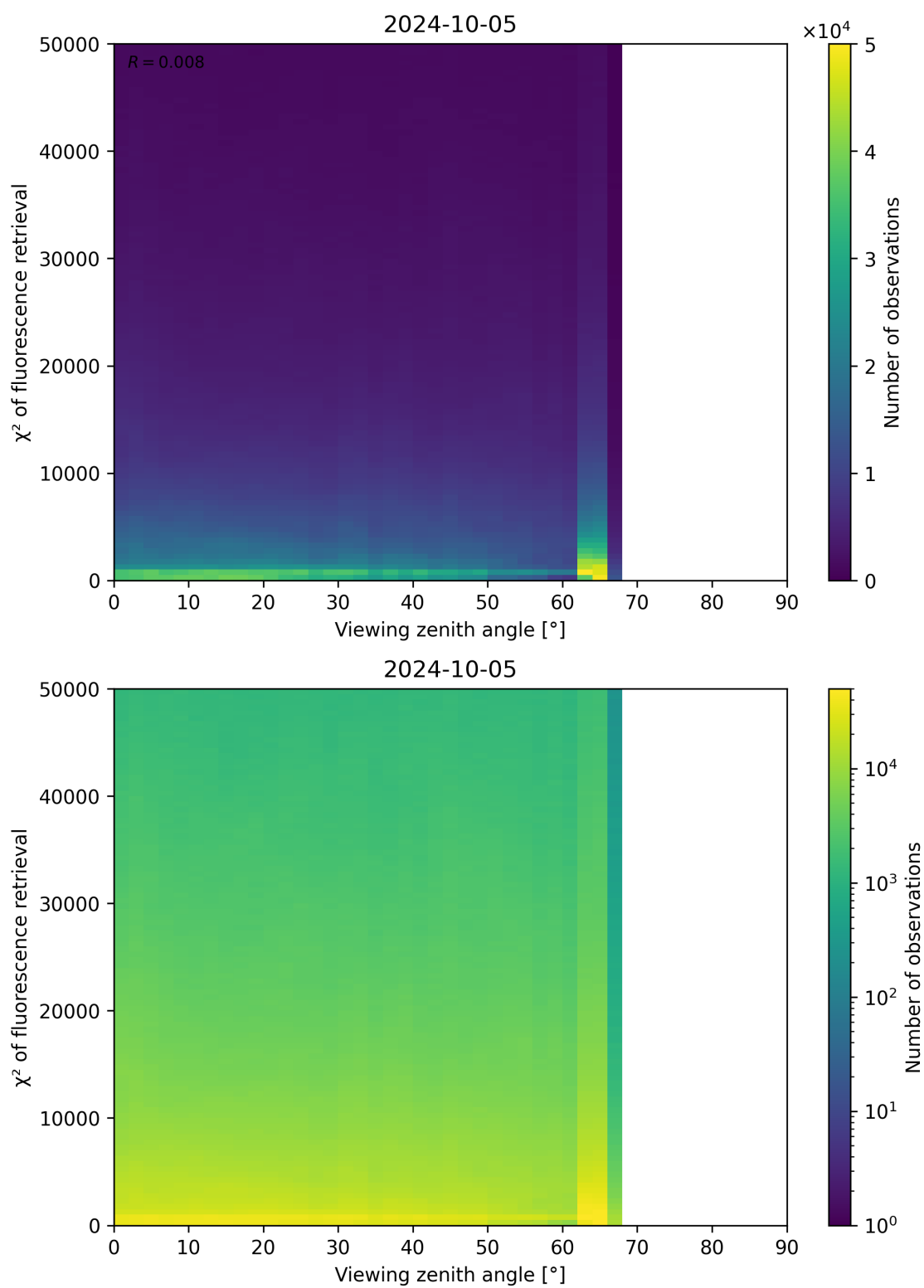
Figure 131: Scatter density plot of “Viewing zenith angle” against “ \chi^2 of fluorescence retrieval” for 2024-10-04 to 2024-10-06.
