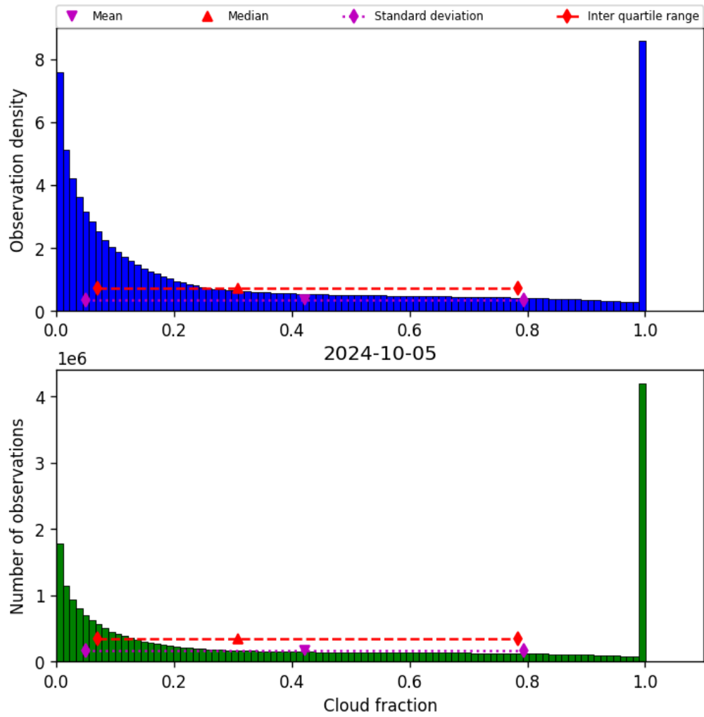
Figure 32: Histogram of "Cloud fraction" for 2024-10-04 to 2024-10-06
