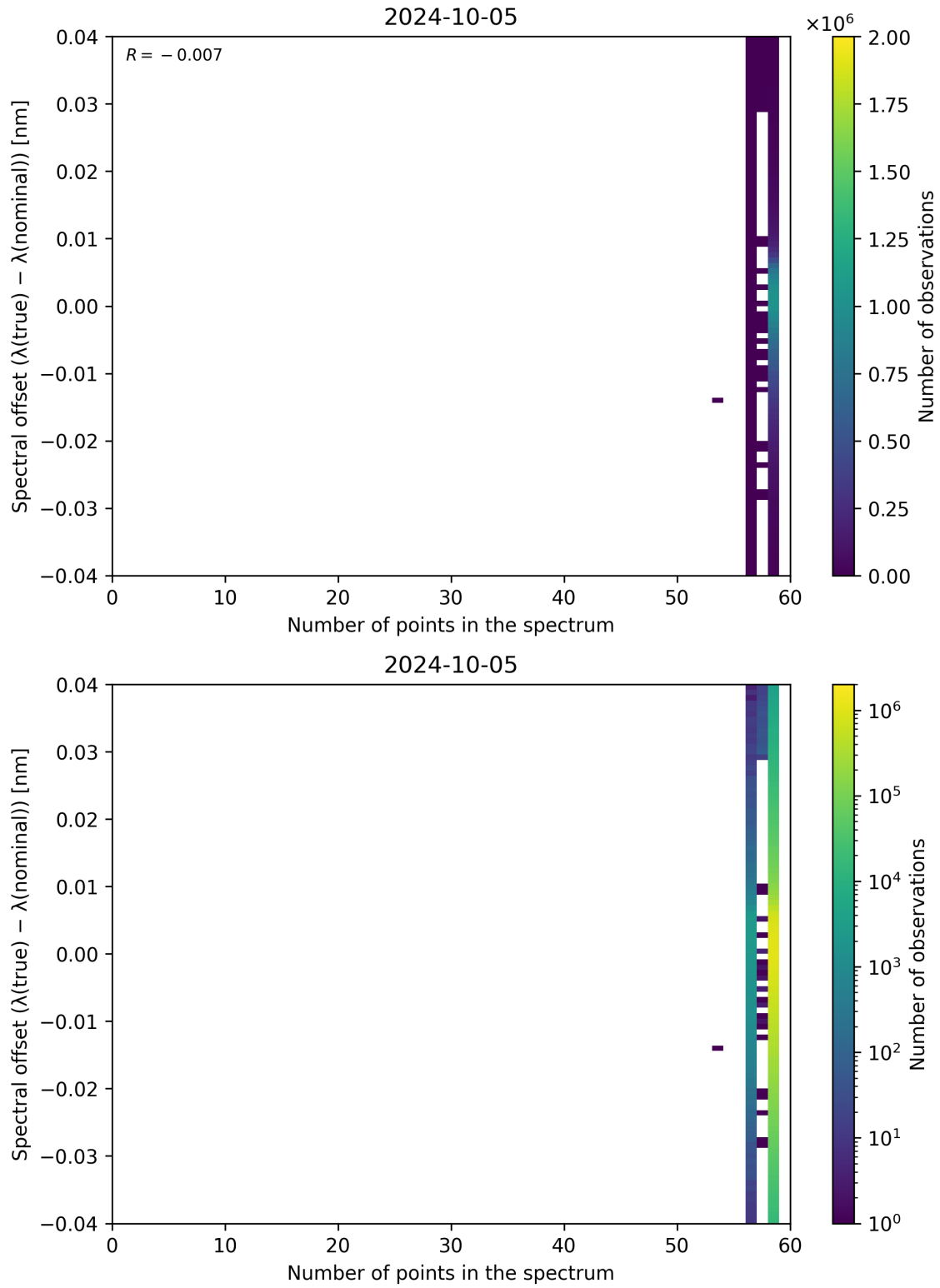
Figure 110: Scatter density plot of “Number of points in the spectrum” against “Spectral offset ( \lambda_{\text{true}} - \lambda_{\text{nominal}} )” for 2024-10-04 to 2024-10-06.
