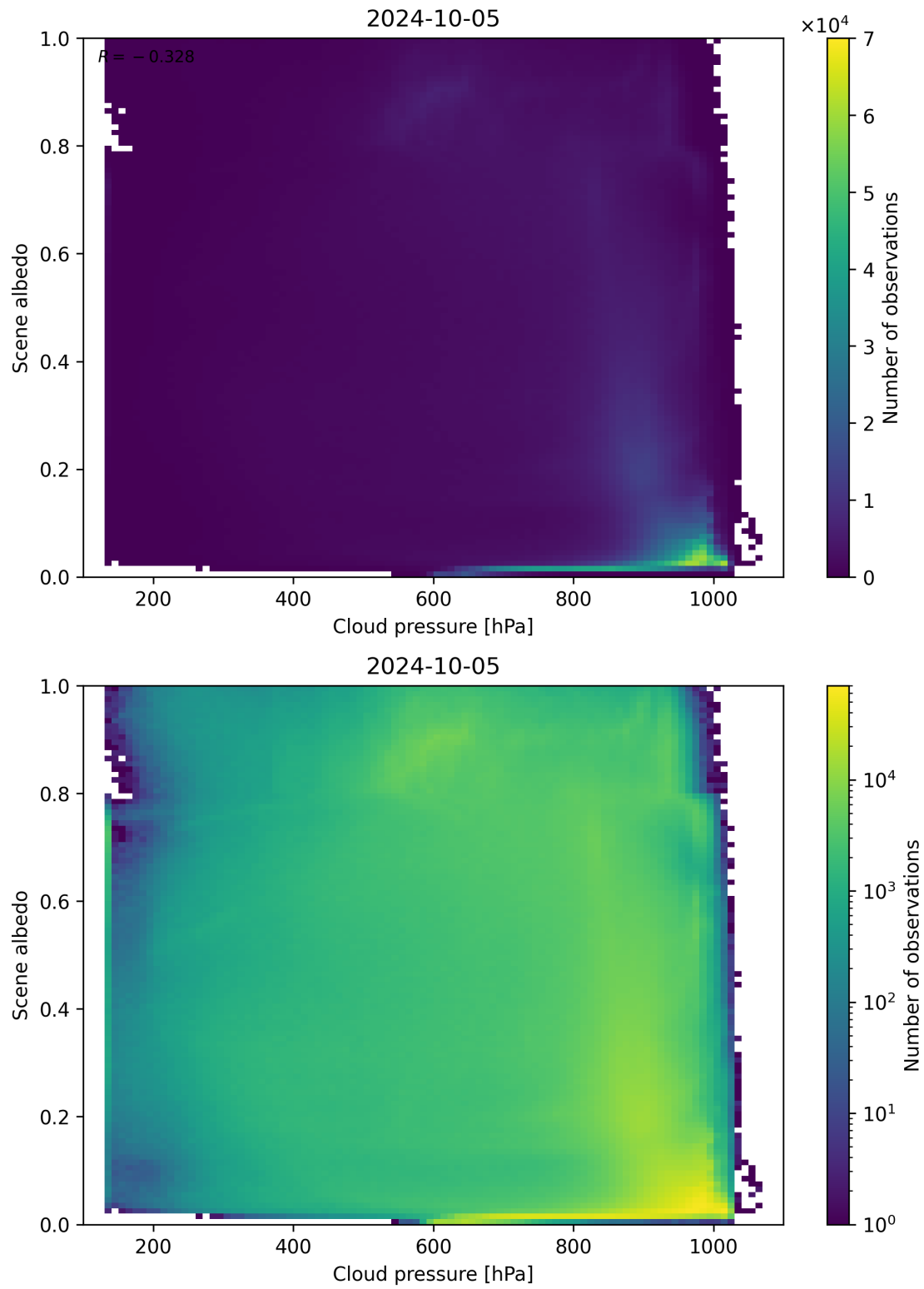
Figure 91: Scatter density plot of “Cloud pressure” against “Scene albedo” for 2024-10-04 to 2024-10-06.
