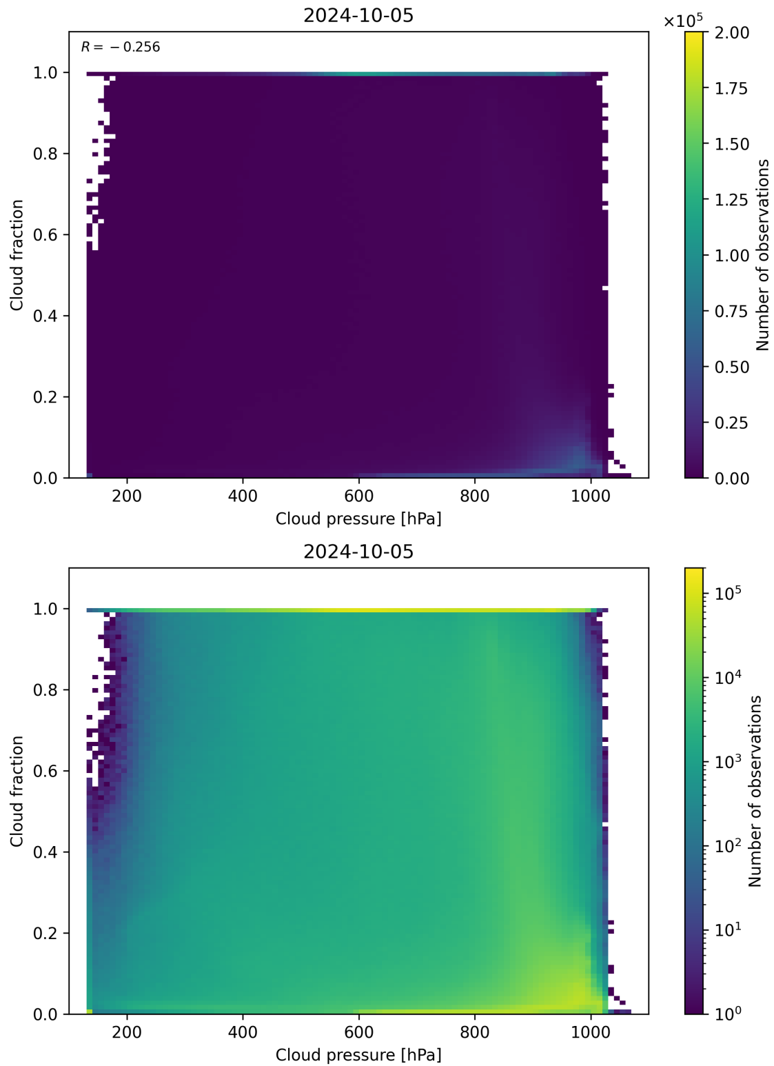
Figure 87: Scatter density plot of “Cloud pressure” against “Cloud fraction” for 2024-10-04 to 2024-10-06.
