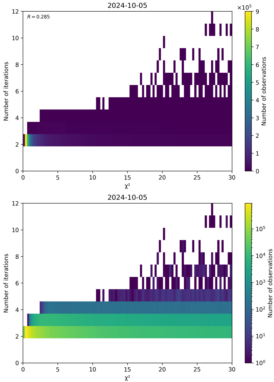
Figure 73: Scatter density plot of “ \chi^2 ” against “Number of iterations” for 2024-10-04 to 2024-10-06.
