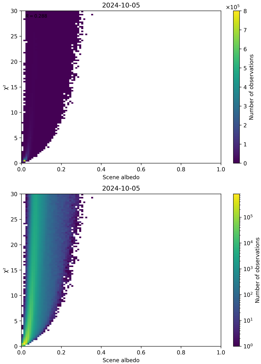
Figure 112: Scatter density plot of “Scene albedo” against “ \chi^2 ” for 2024-10-04 to 2024-10-06.
