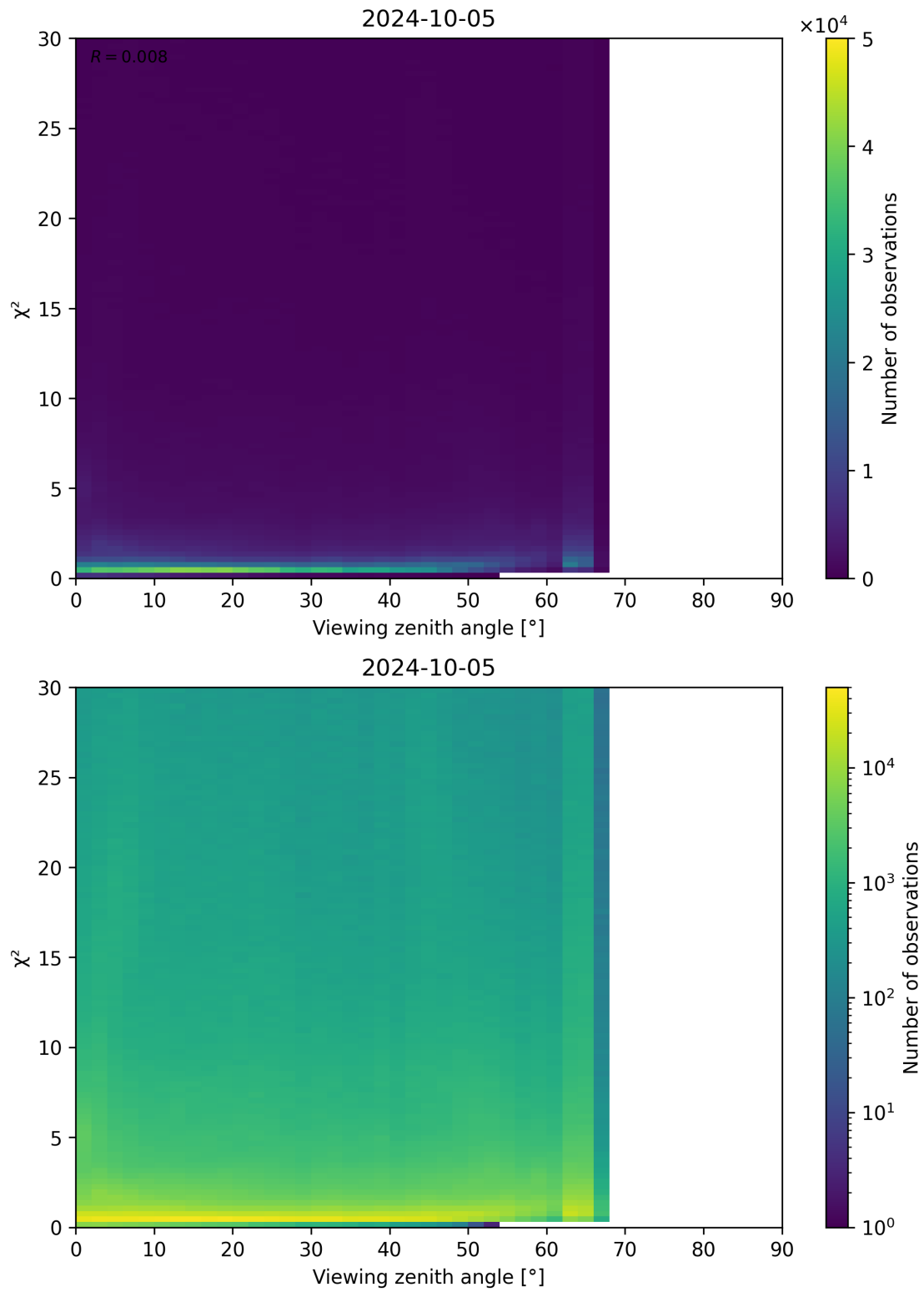
Figure 130: Scatter density plot of “Viewing zenith angle” against “ \chi^2 ” for 2024-10-04 to 2024-10-06.
