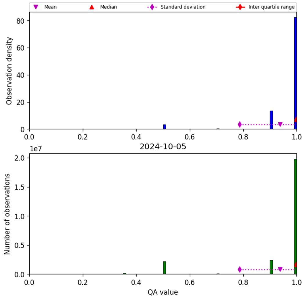
Figure 29: Histogram of “QA value” for 2024-10-04 to 2024-10-06
