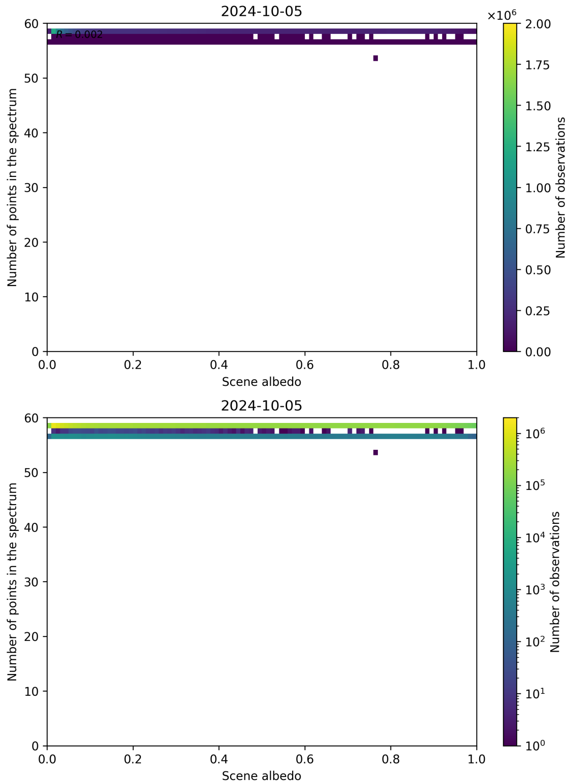
Figure 116: Scatter density plot of “Scene albedo” against “Number of points in the spectrum” for 2024-10-04 to 2024-10-06.
