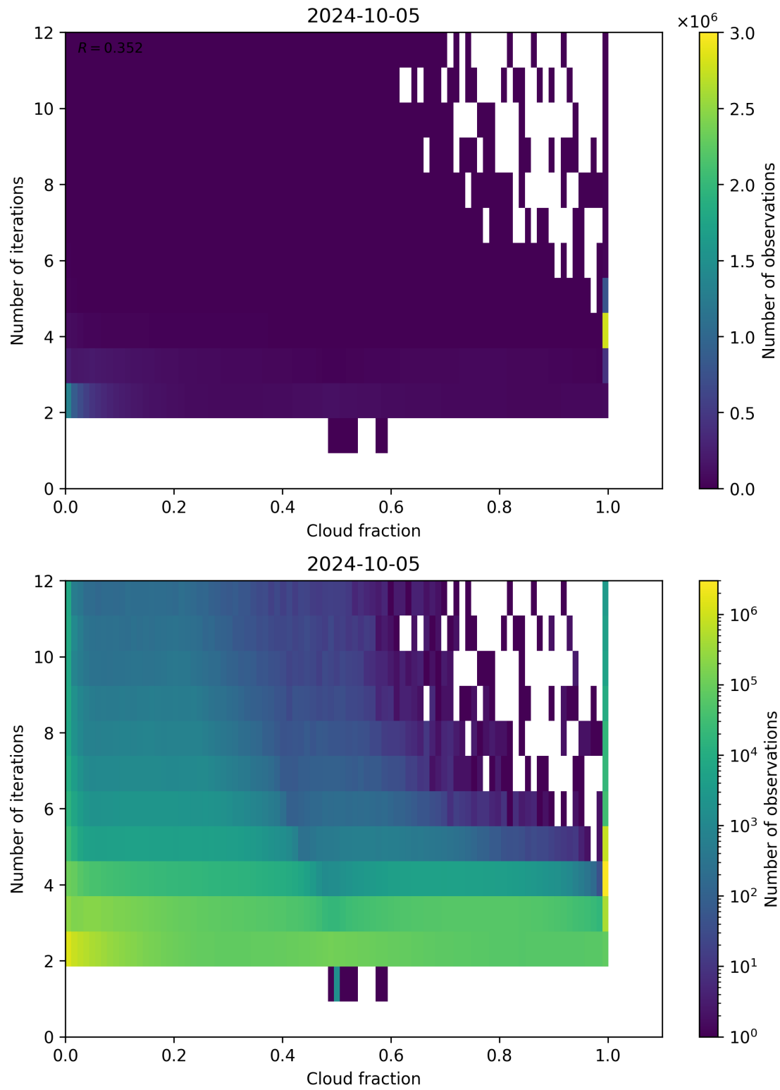
Figure 80: Scatter density plot of “Cloud fraction” against “Number of iterations” for 2024-10-04 to 2024-10-06.
