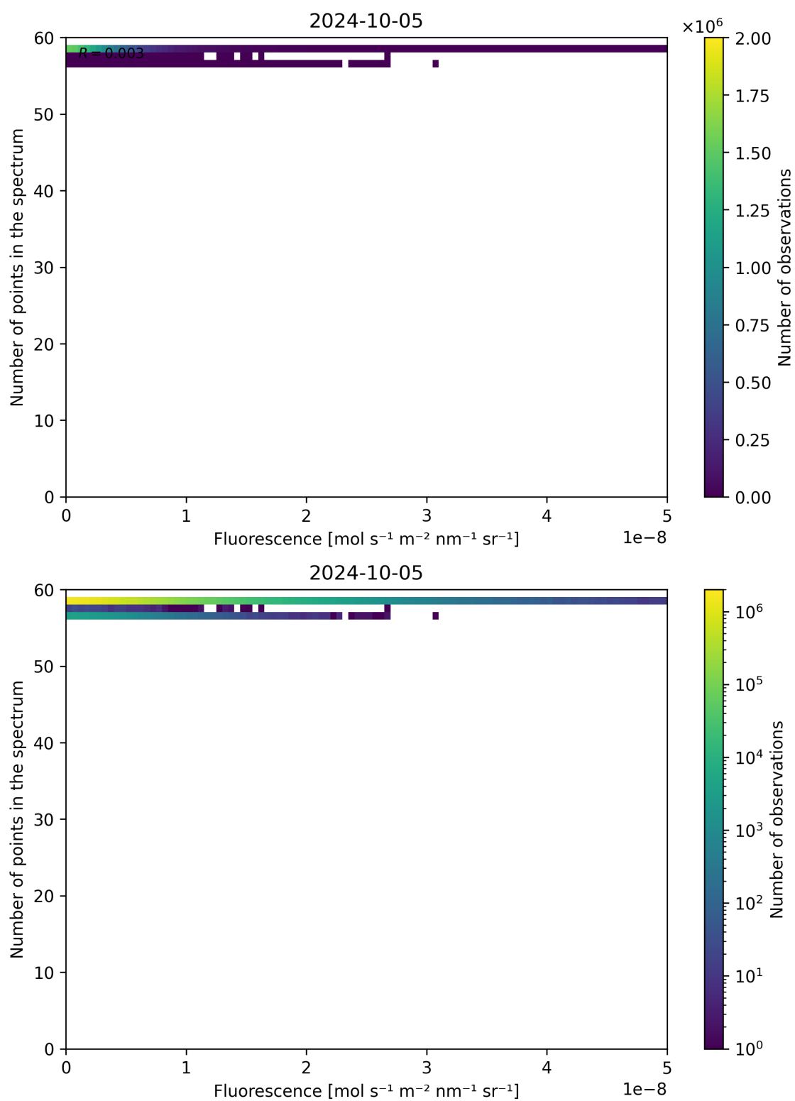
Figure 94: Scatter density plot of “Fluorescence” against “Number of points in the spectrum” for 2024-10-04 to 2024-10-06.
