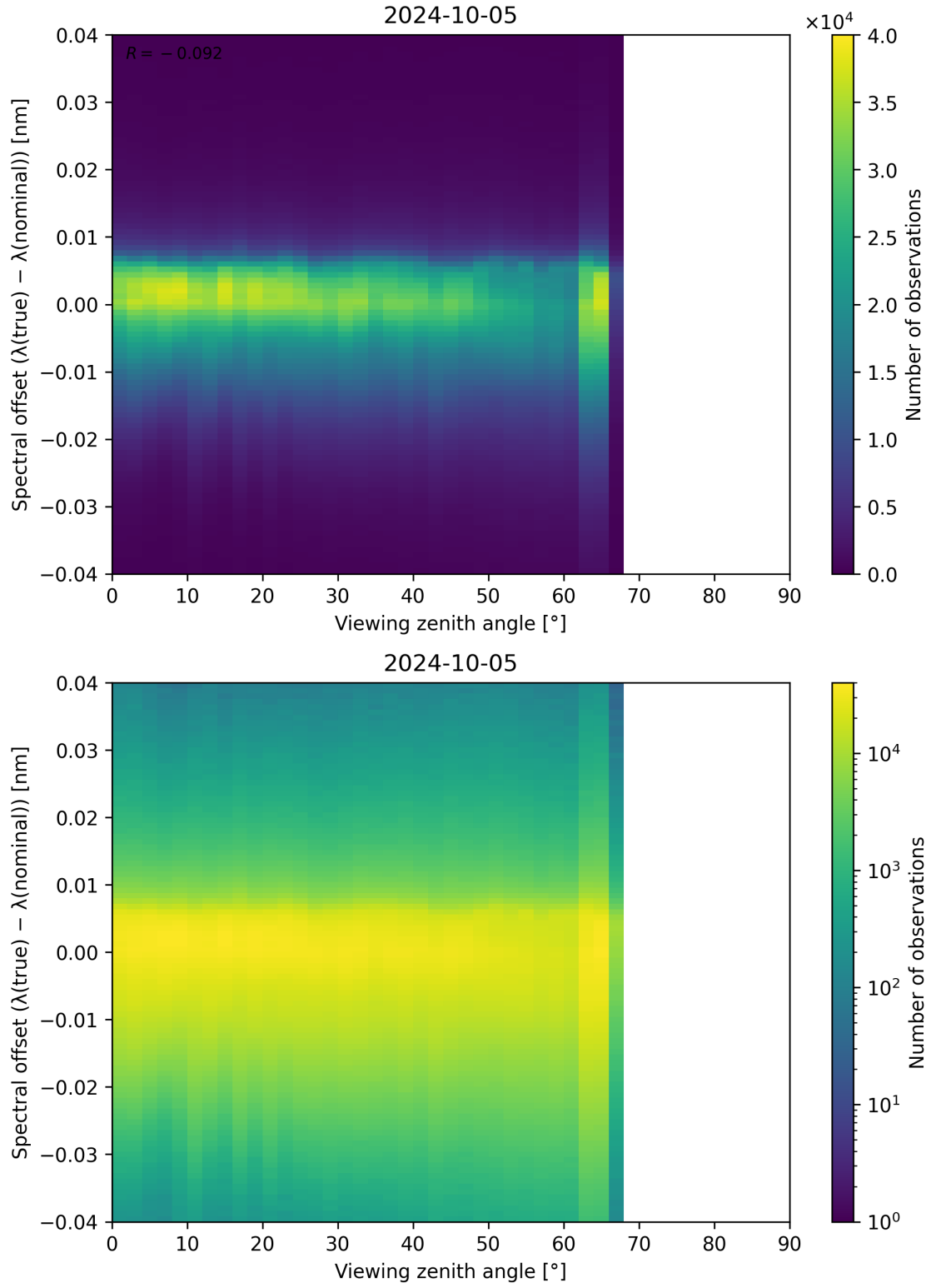
Figure 140: Scatter density plot of “Viewing zenith angle” against “Spectral offset ( \lambda_{\text{true}} - \lambda_{\text{nominal}} )” for 2024-10-04 to 2024-10-06.
