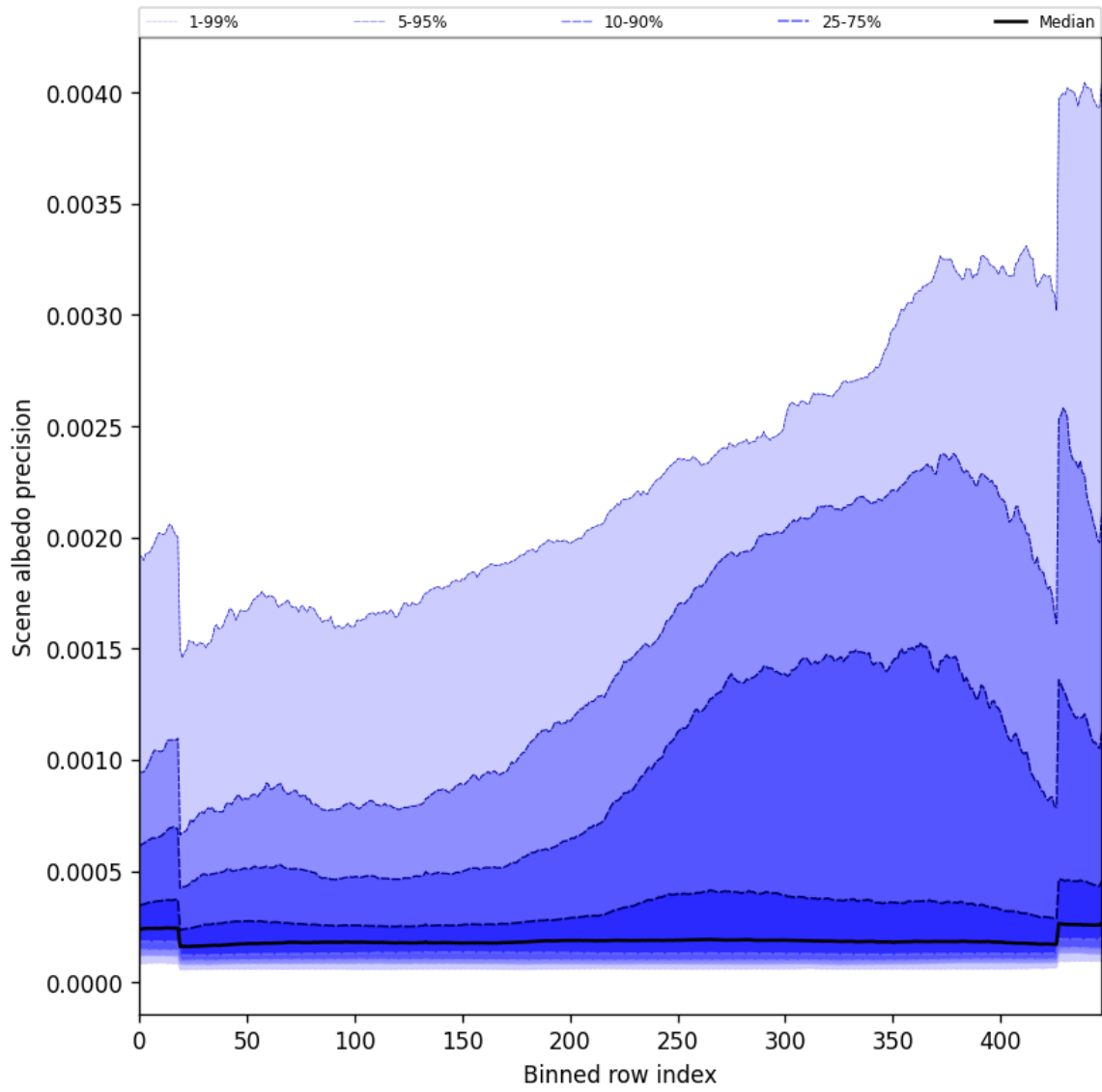
Figure 52: Along track statistics of “Scene albedo precision” for 2024-10-04 to 2024-10-06
