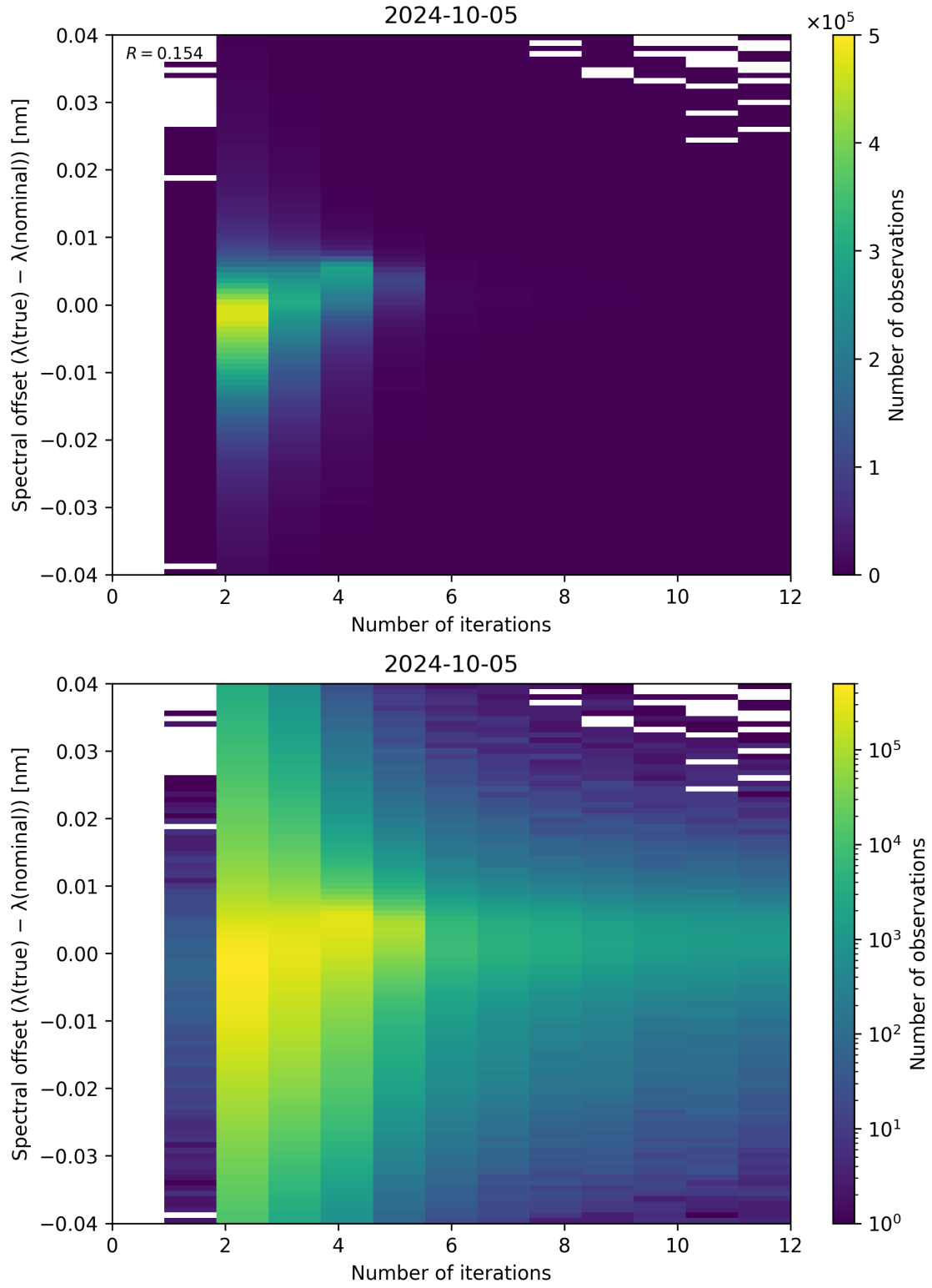
Figure 109: Scatter density plot of “Number of iterations” against “Spectral offset ( \lambda_{\text{true}} - \lambda_{\text{nominal}} )” for 2024-10-04 to 2024-10-06.
