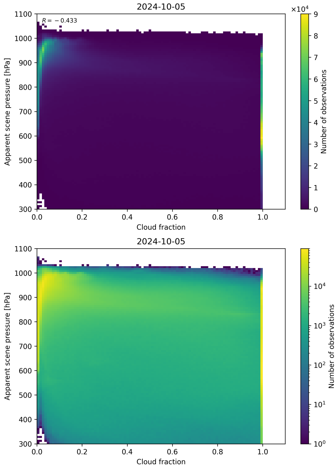
Figure 76: Scatter density plot of “Cloud fraction” against “Apparent scene pressure” for 2024-10-04 to 2024-10-06.
