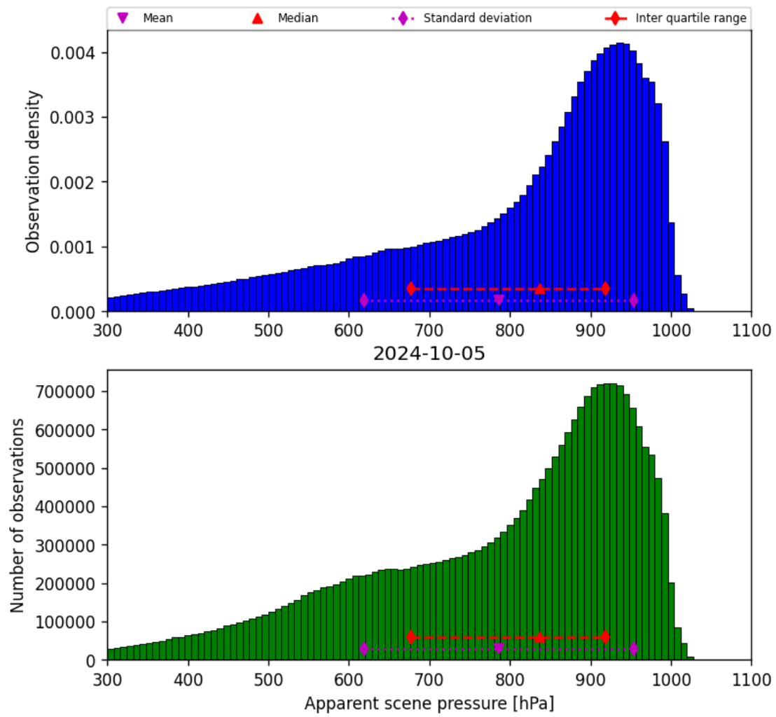
Figure 36: Histogram of “Apparent scene pressure” for 2024-10-04 to 2024-10-06
