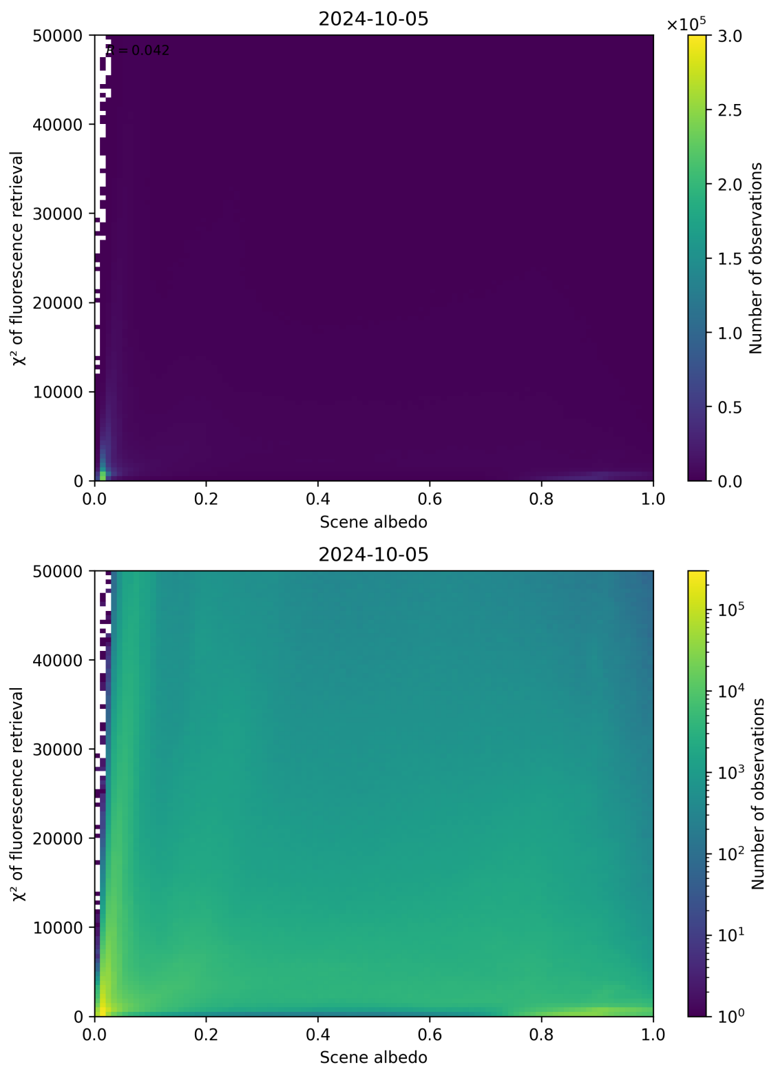
Figure 113: Scatter density plot of “Scene albedo” against “ \chi^2 of fluorescence retrieval” for 2024-10-04 to 2024-10-06.
