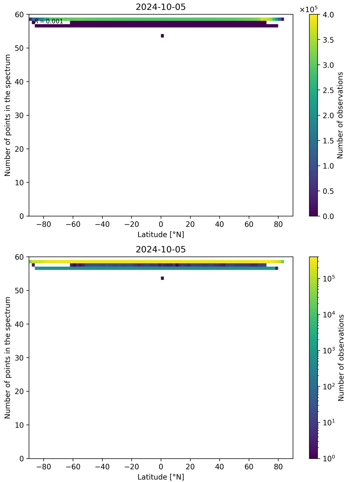
Figure 103: Scatter density plot of “Latitude” against “Number of points in the spectrum” for 2024-10-04 to 2024-10-06.
