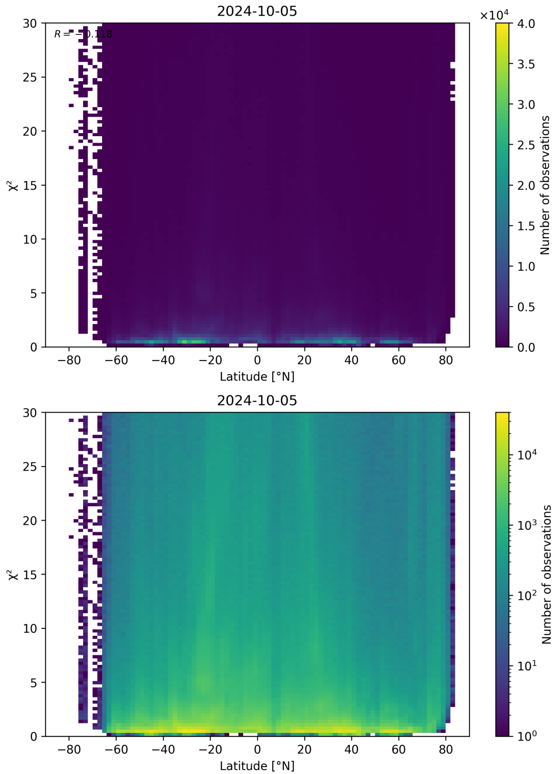
Figure 97: Scatter density plot of “Latitude” against “ \chi^2 ” for 2024-10-04 to 2024-10-06.
