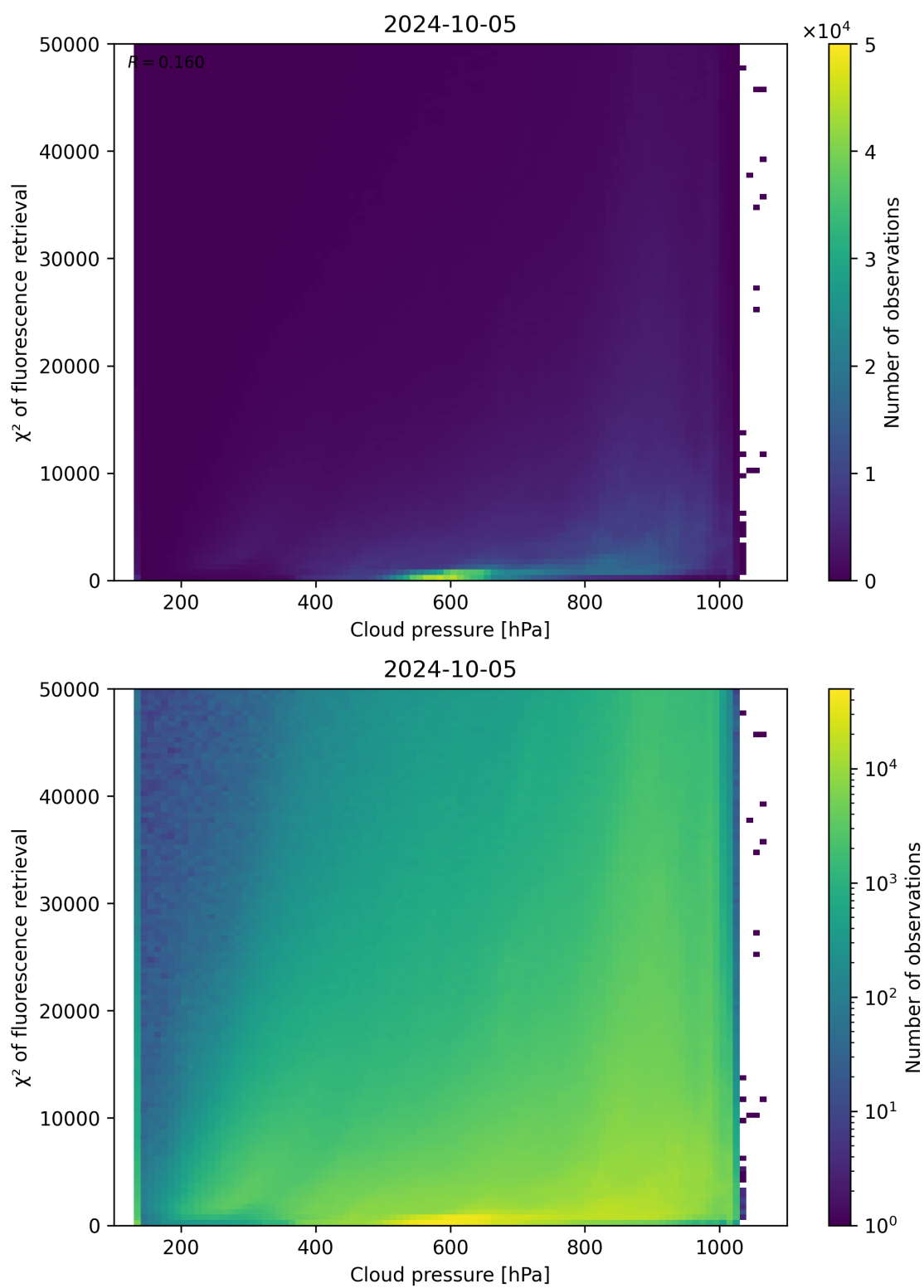
Figure 86: Scatter density plot of “Cloud pressure” against “ \chi^2 of fluorescence retrieval” for 2024-10-04 to 2024-10-06.
