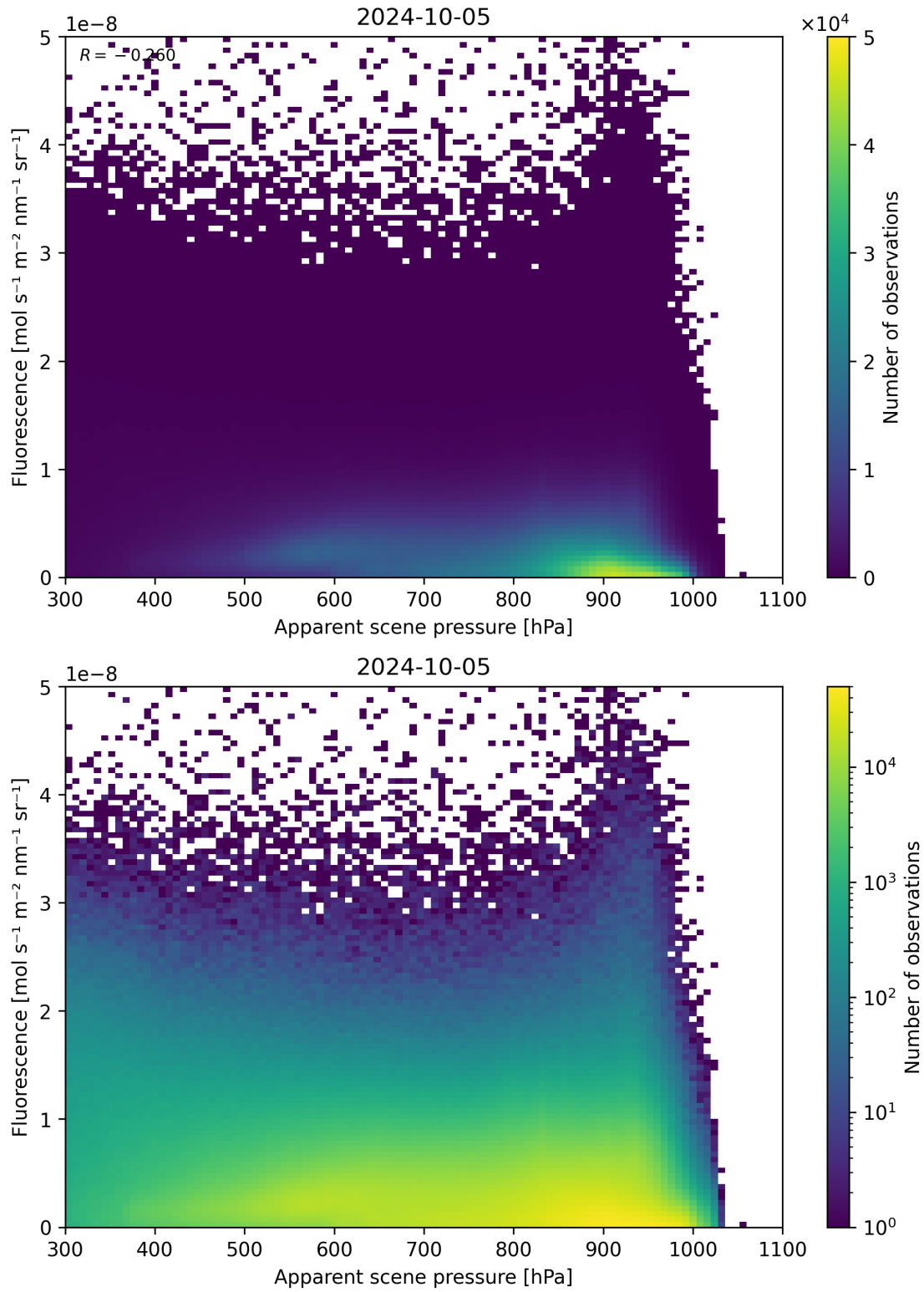
Figure 65: Scatter density plot of “Apparent scene pressure” against “Fluorescence” for 2024-10-04 to 2024-10-06.
