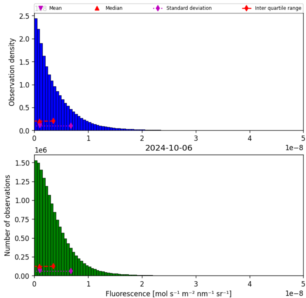
Figure 40: Histogram of “Fluorescence” for 2024-10-05 to 2024-10-07
