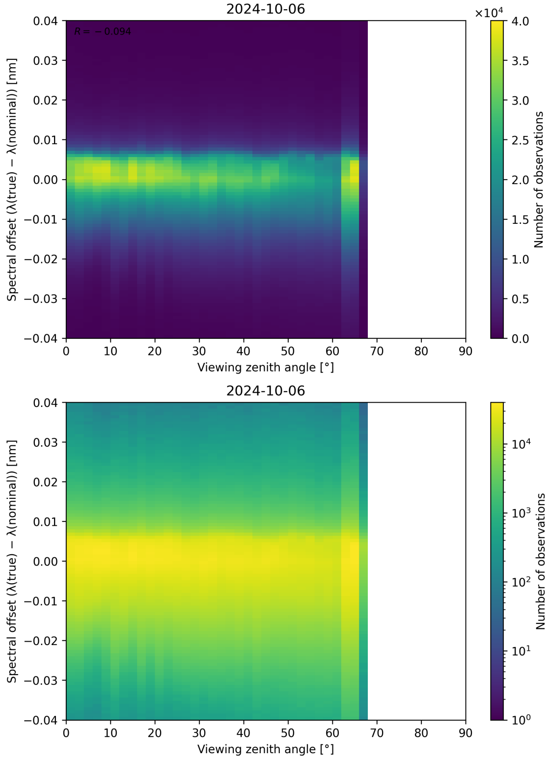
Figure 140: Scatter density plot of “Viewing zenith angle” against “Spectral offset ( \lambda_{\text{true}} - \lambda_{\text{nominal}} )” for 2024-10-05 to 2024-10-07.
