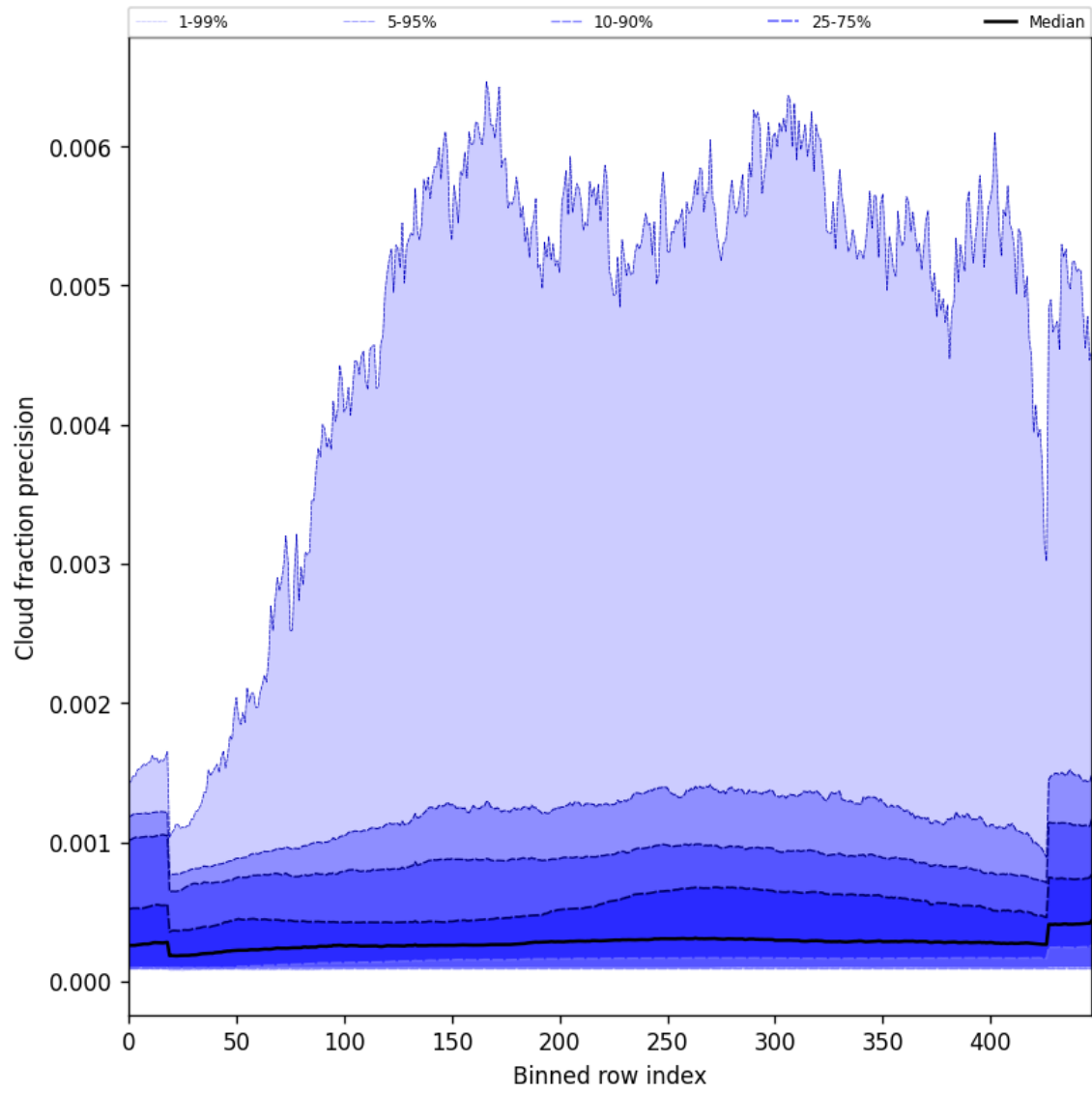
Figure 50: Along track statistics of “Cloud fraction precision” for 2024-10-05 to 2024-10-07
