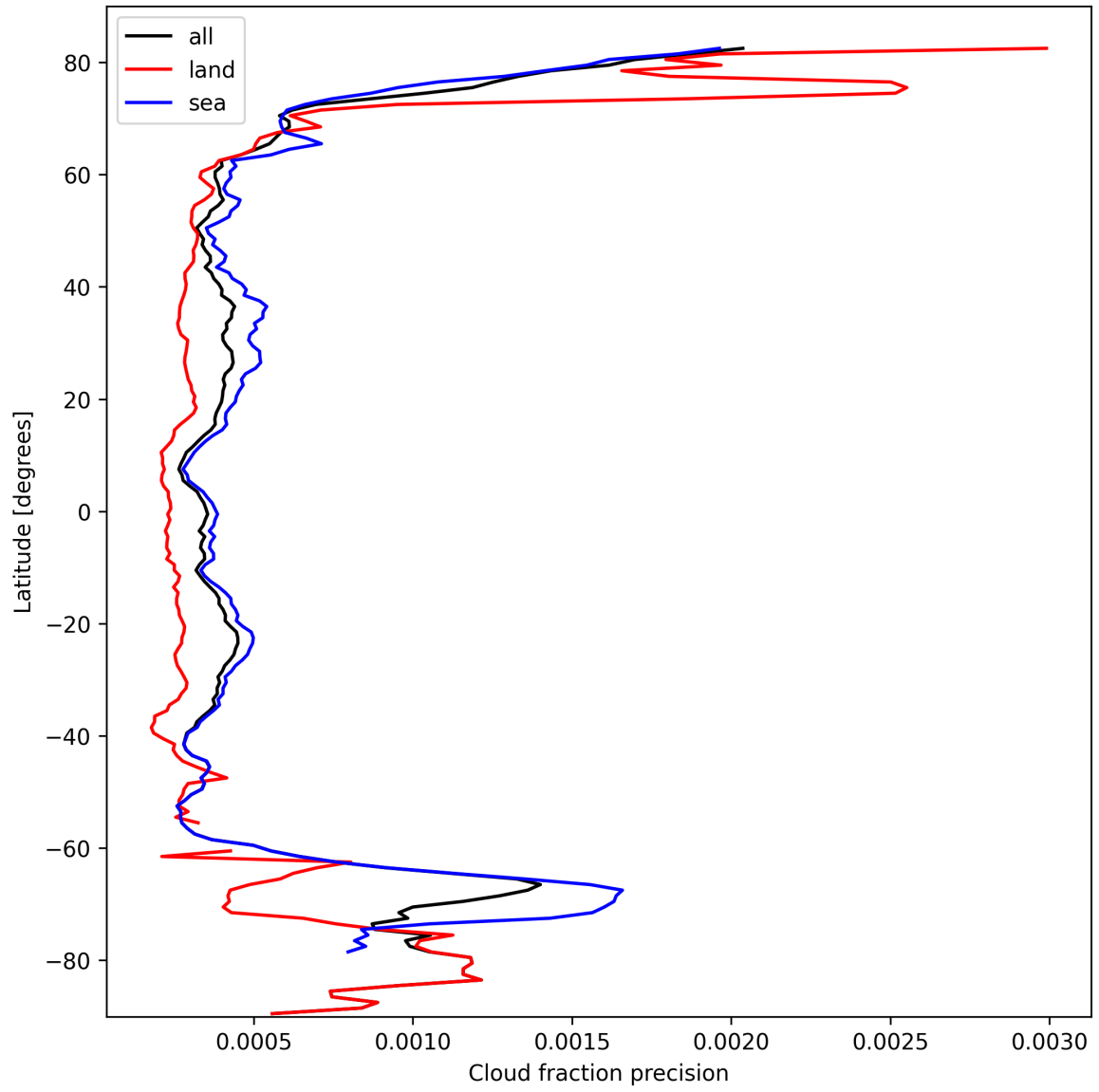
Figure 16: Zonal average of “Cloud fraction precision” for 2024-10-05 to 2024-10-07.
