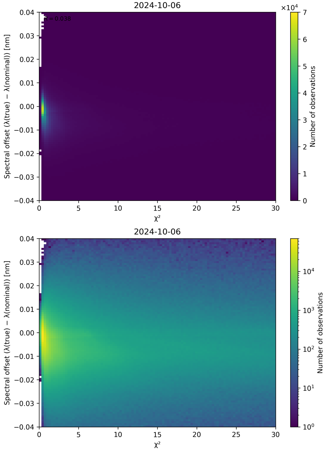
Figure 75: Scatter density plot of “ \chi^2 ” against “Spectral offset ( \lambda_{\text{true}} - \lambda_{\text{nominal}} )” for 2024-10-05 to 2024-10-07.
