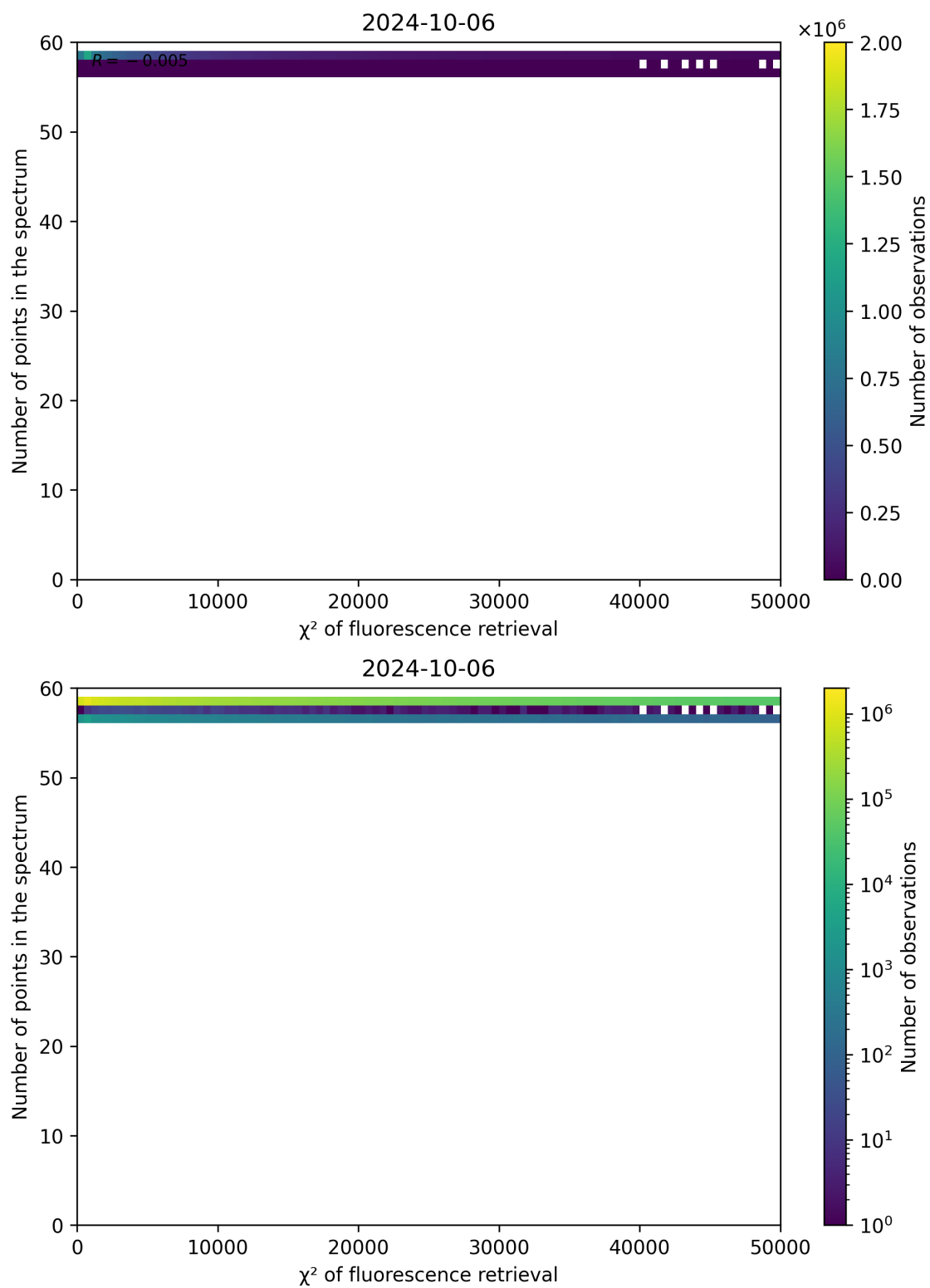
Figure 71: Scatter density plot of " \chi^2 of fluorescence retrieval" against "Number of points in the spectrum" for 2024-10-05 to 2024-10-07.
