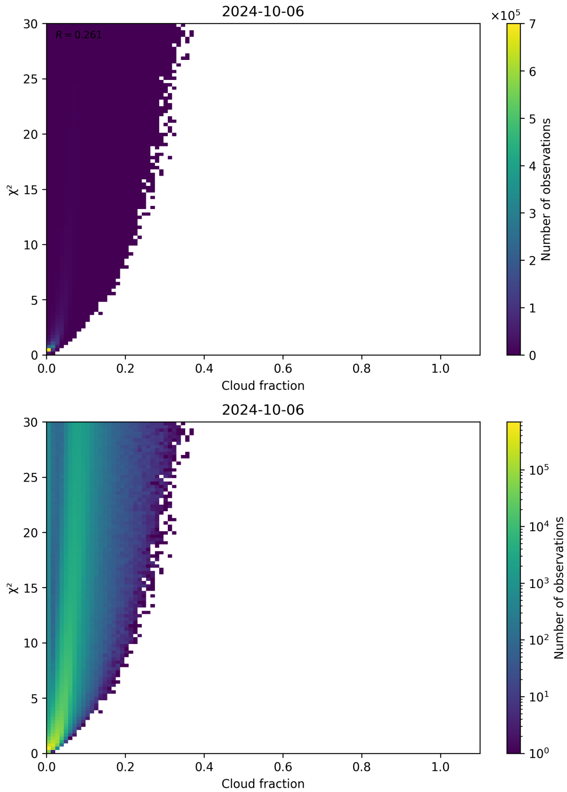
Figure 77: Scatter density plot of “Cloud fraction” against “ \chi^2 ” for 2024-10-05 to 2024-10-07.
