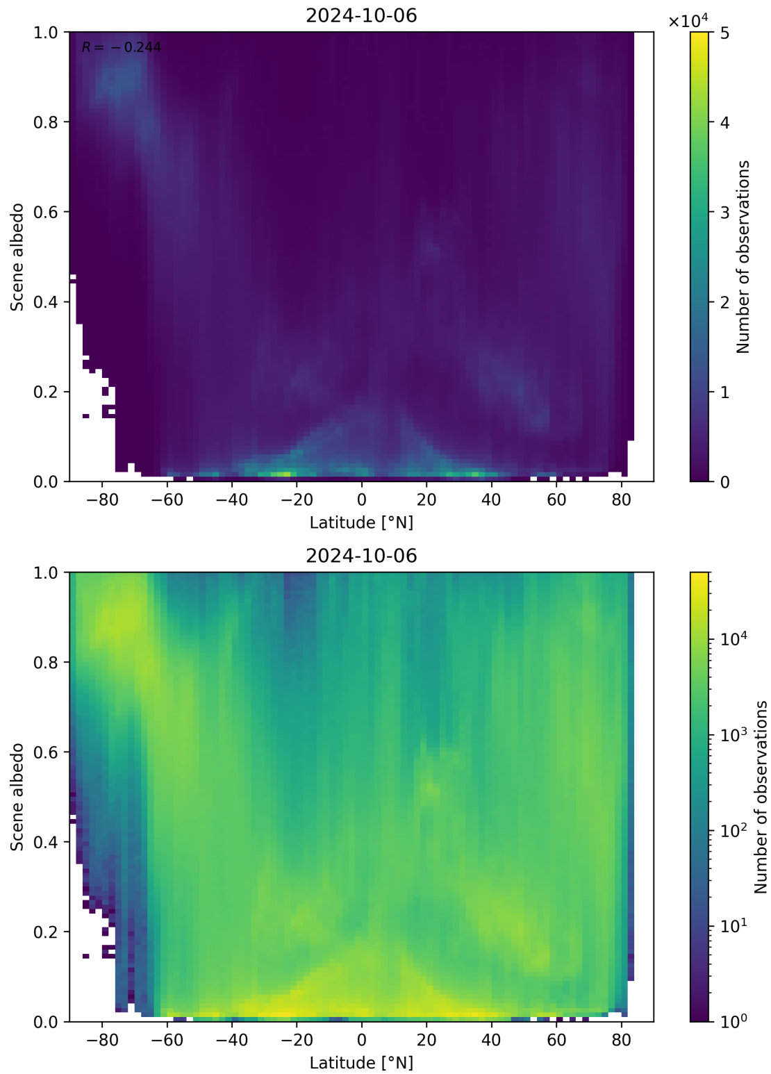
Figure 104: Scatter density plot of “Latitude” against “Scene albedo” for 2024-10-05 to 2024-10-07.
