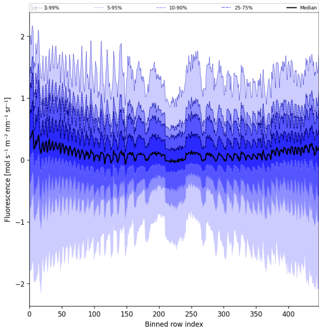
Figure 57: Along track statistics of “Fluorescence” for 2024-10-05 to 2024-10-07
