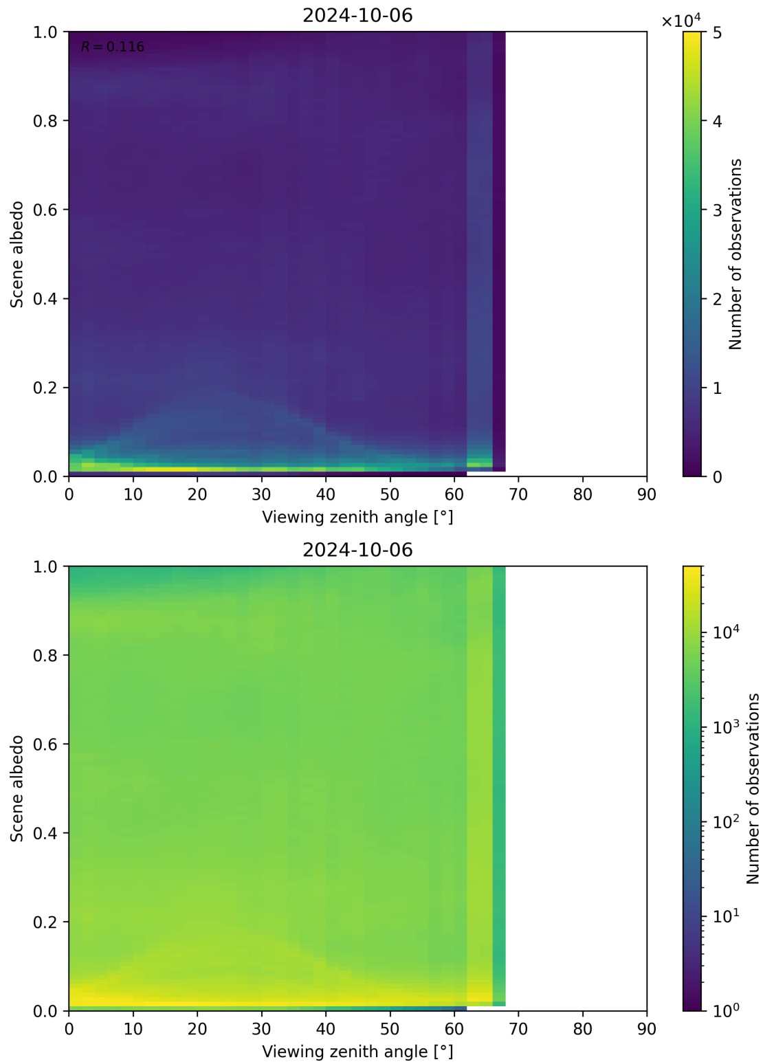
Figure 138: Scatter density plot of “Viewing zenith angle” against “Scene albedo” for 2024-10-05 to 2024-10-07.
