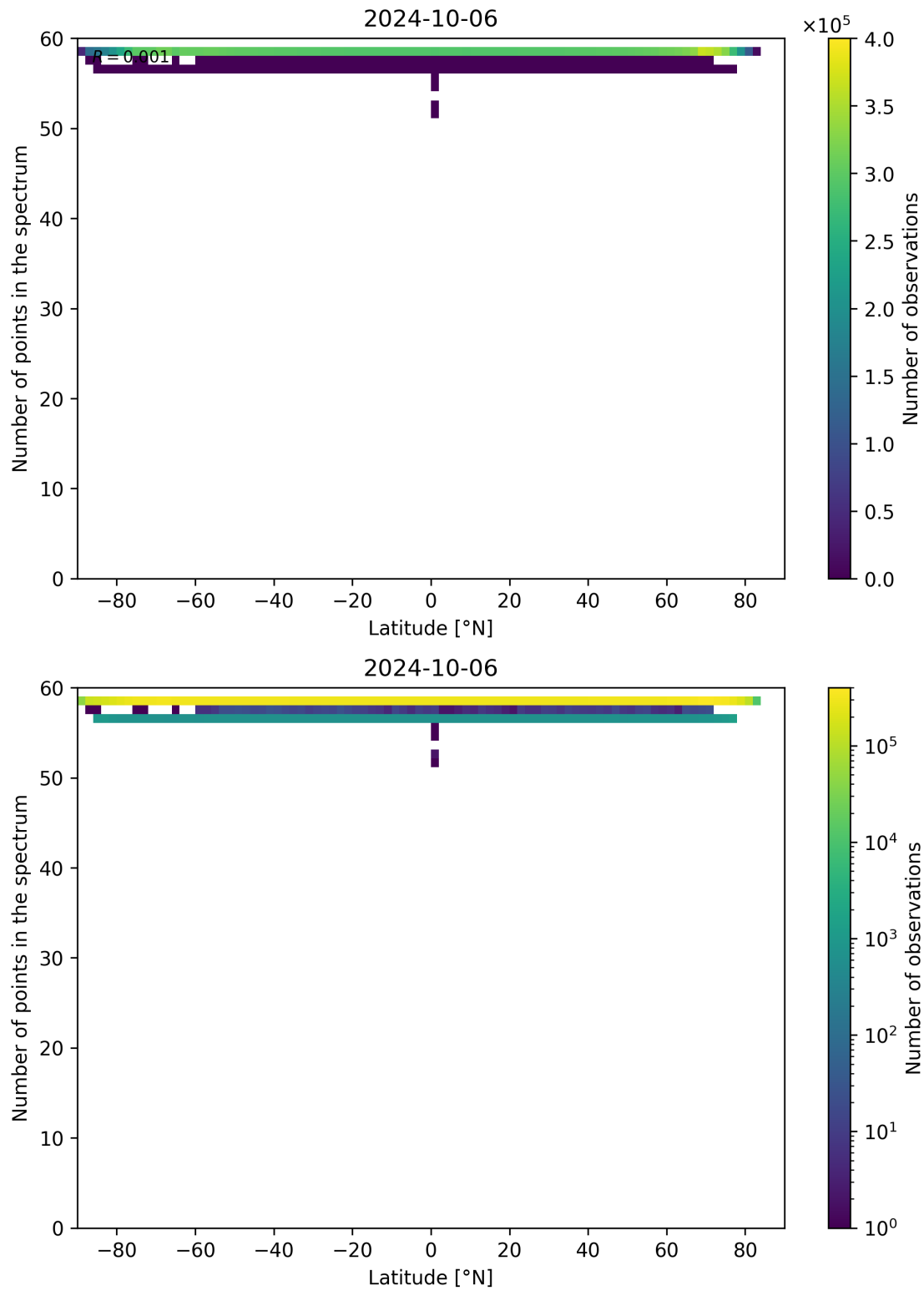
Figure 103: Scatter density plot of “Latitude” against “Number of points in the spectrum” for 2024-10-05 to 2024-10-07.
