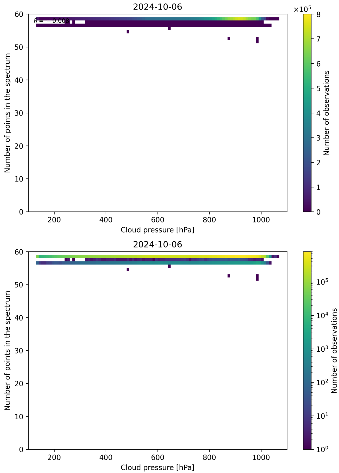
Figure 90: Scatter density plot of “Cloud pressure” against “Number of points in the spectrum” for 2024-10-05 to 2024-10-07.
