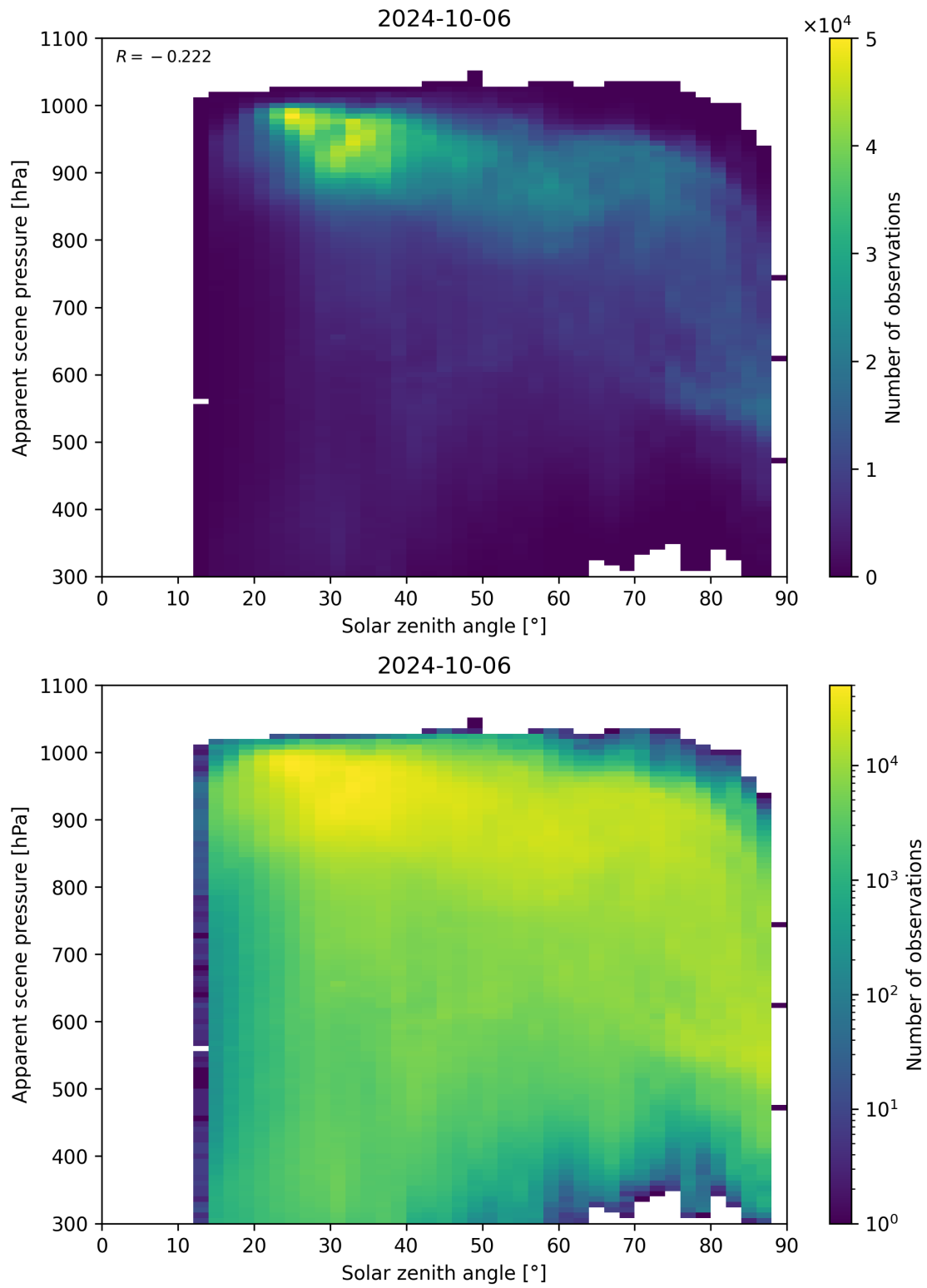
Figure 118: Scatter density plot of “Solar zenith angle” against “Apparent scene pressure” for 2024-10-05 to 2024-10-07.
