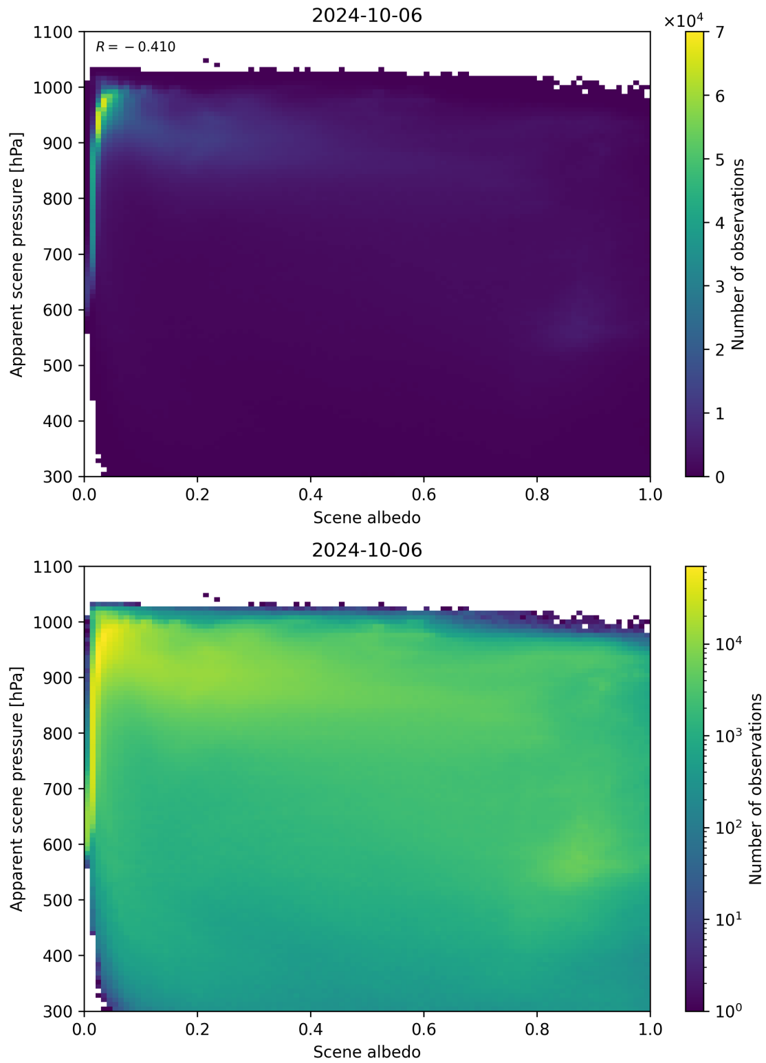
Figure 111: Scatter density plot of “Scene albedo” against “Apparent scene pressure” for 2024-10-05 to 2024-10-07.
