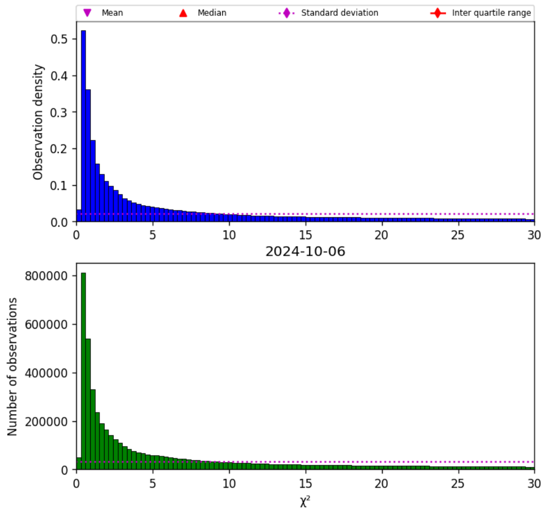
Figure 38: Histogram of " \chi^2 " for 2024-10-05 to 2024-10-07
