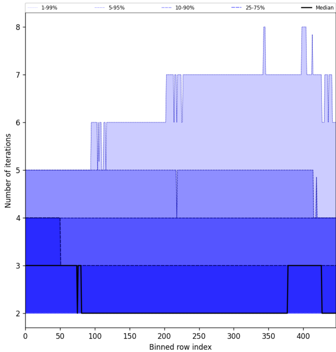
Figure 56: Along track statistics of “Number of iterations” for 2024-10-05 to 2024-10-07
