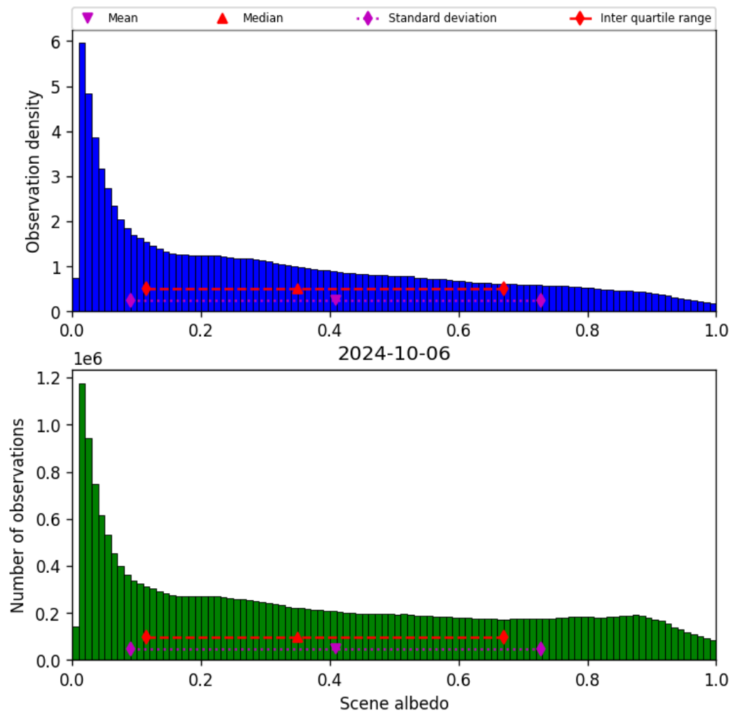
Figure 34: Histogram of “Scene albedo” for 2024-10-05 to 2024-10-07
