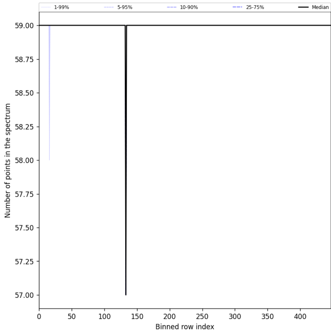
Figure 61: Along track statistics of “Number of points in the spectrum” for 2024-10-05 to 2024-10-07
