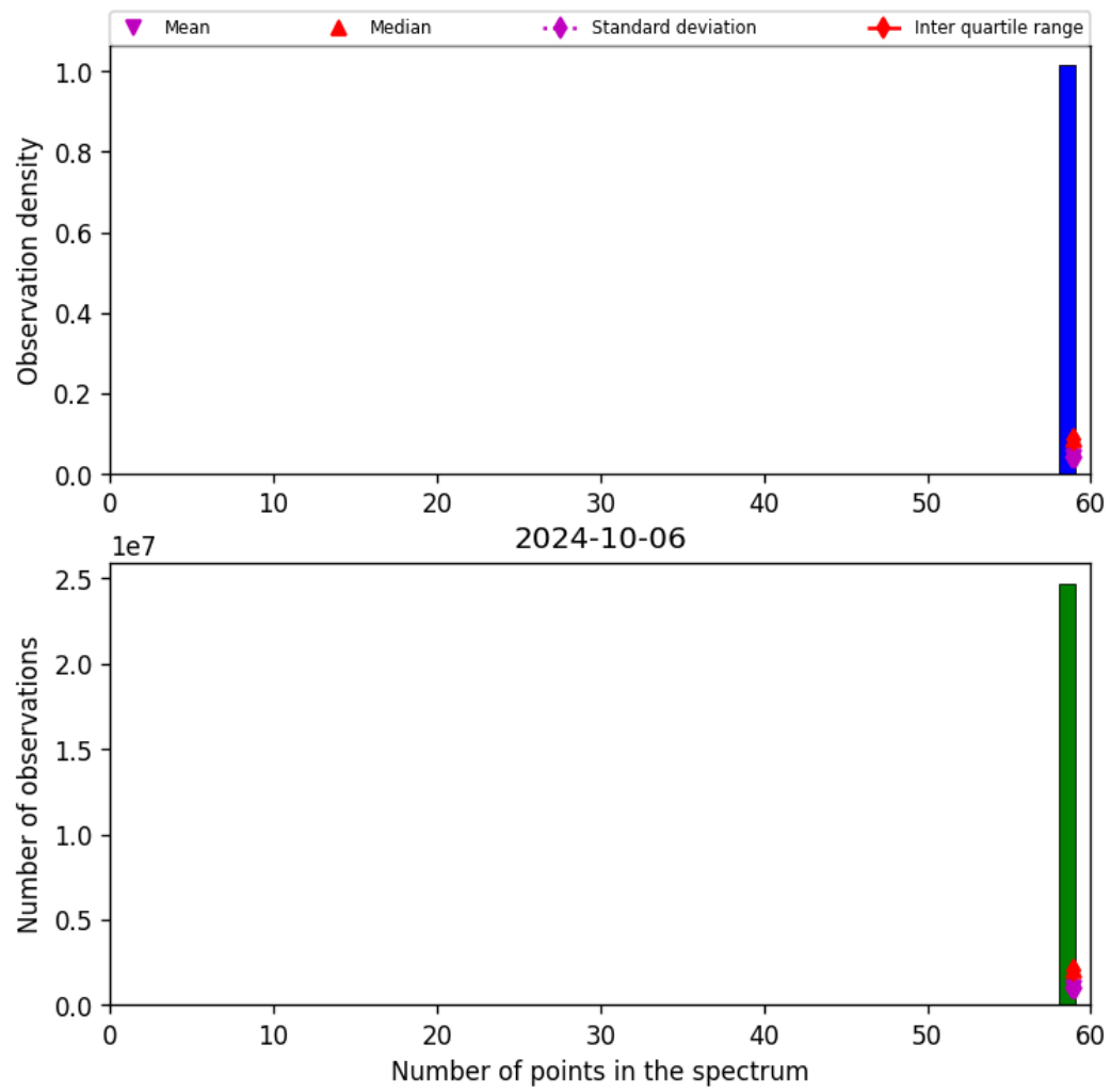
Figure 44: Histogram of “Number of points in the spectrum” for 2024-10-05 to 2024-10-07
