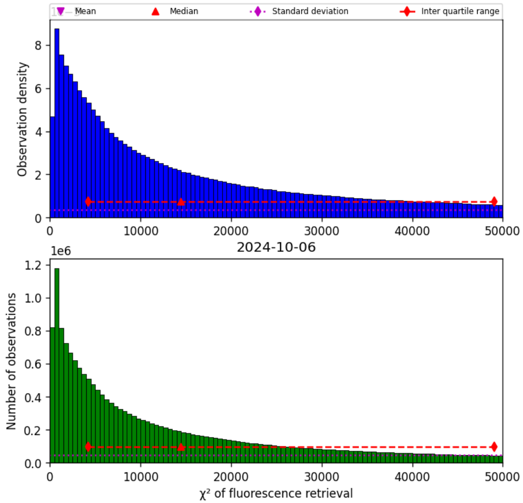
Figure 42: Histogram of “ \chi^2 of fluorescence retrieval” for 2024-10-05 to 2024-10-07
