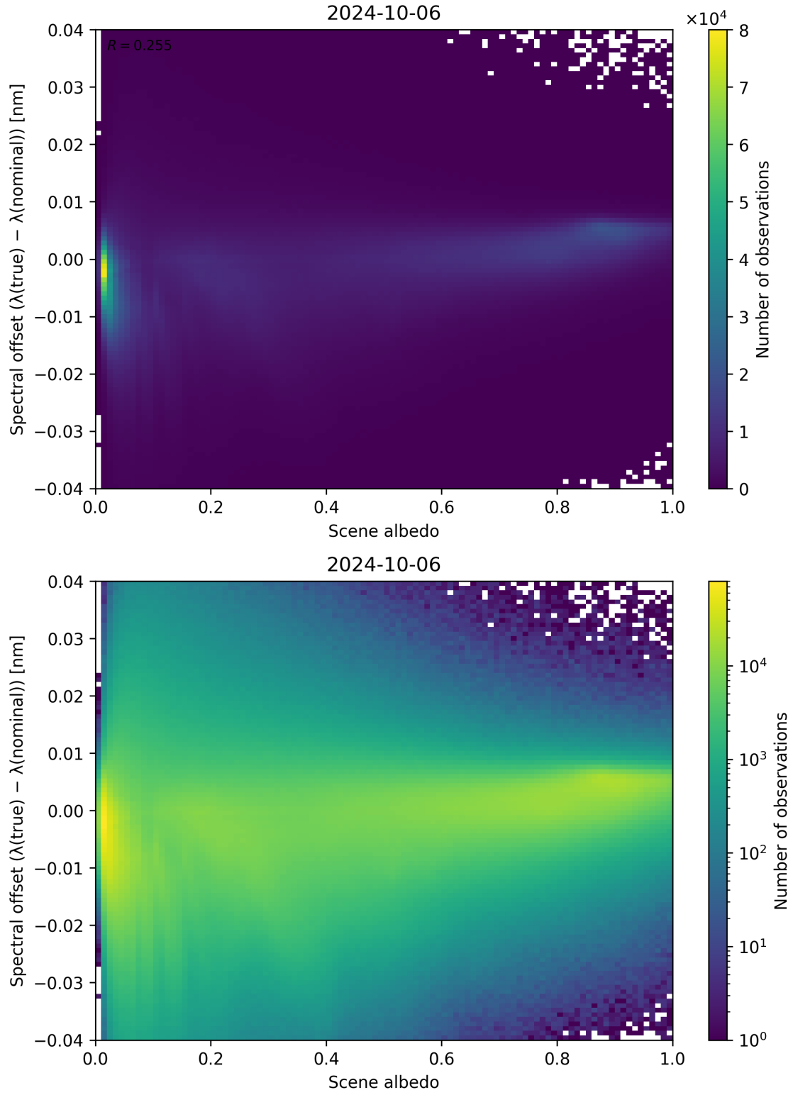
Figure 117: Scatter density plot of “Scene albedo” against “Spectral offset ( \lambda_{\text{true}} - \lambda_{\text{nominal}} )” for 2024-10-05 to 2024-10-07.
