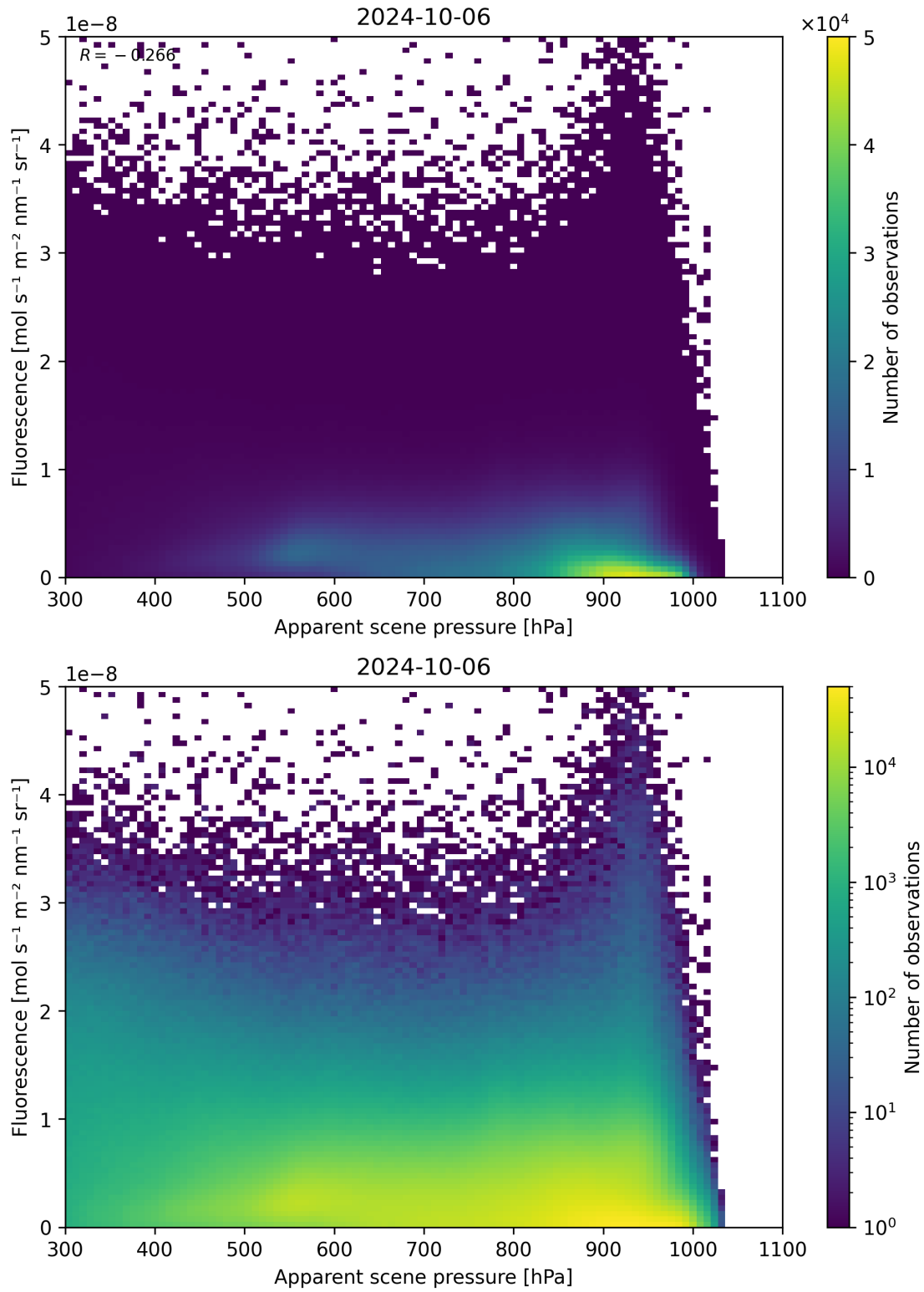
Figure 65: Scatter density plot of “Apparent scene pressure” against “Fluorescence” for 2024-10-05 to 2024-10-07.
