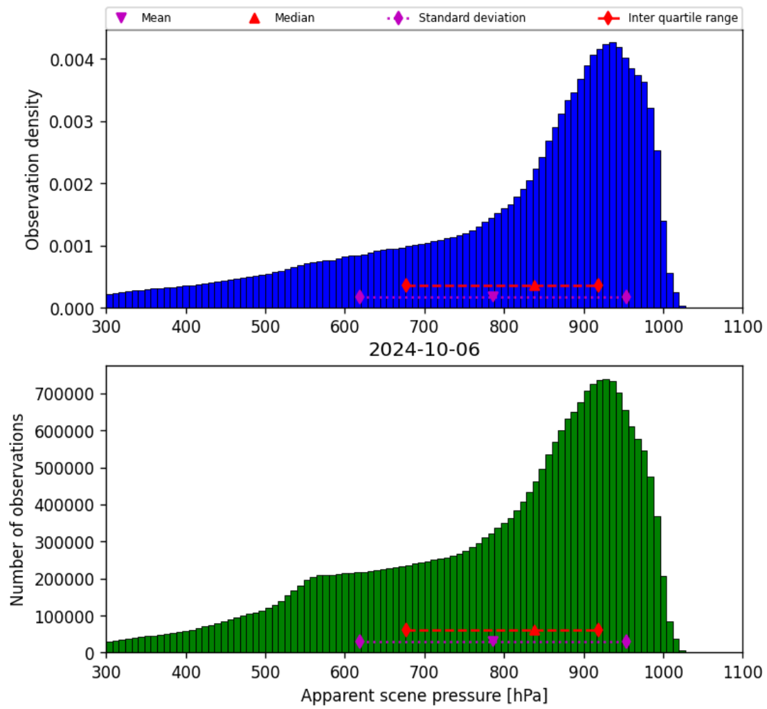
Figure 36: Histogram of “Apparent scene pressure” for 2024-10-05 to 2024-10-07
