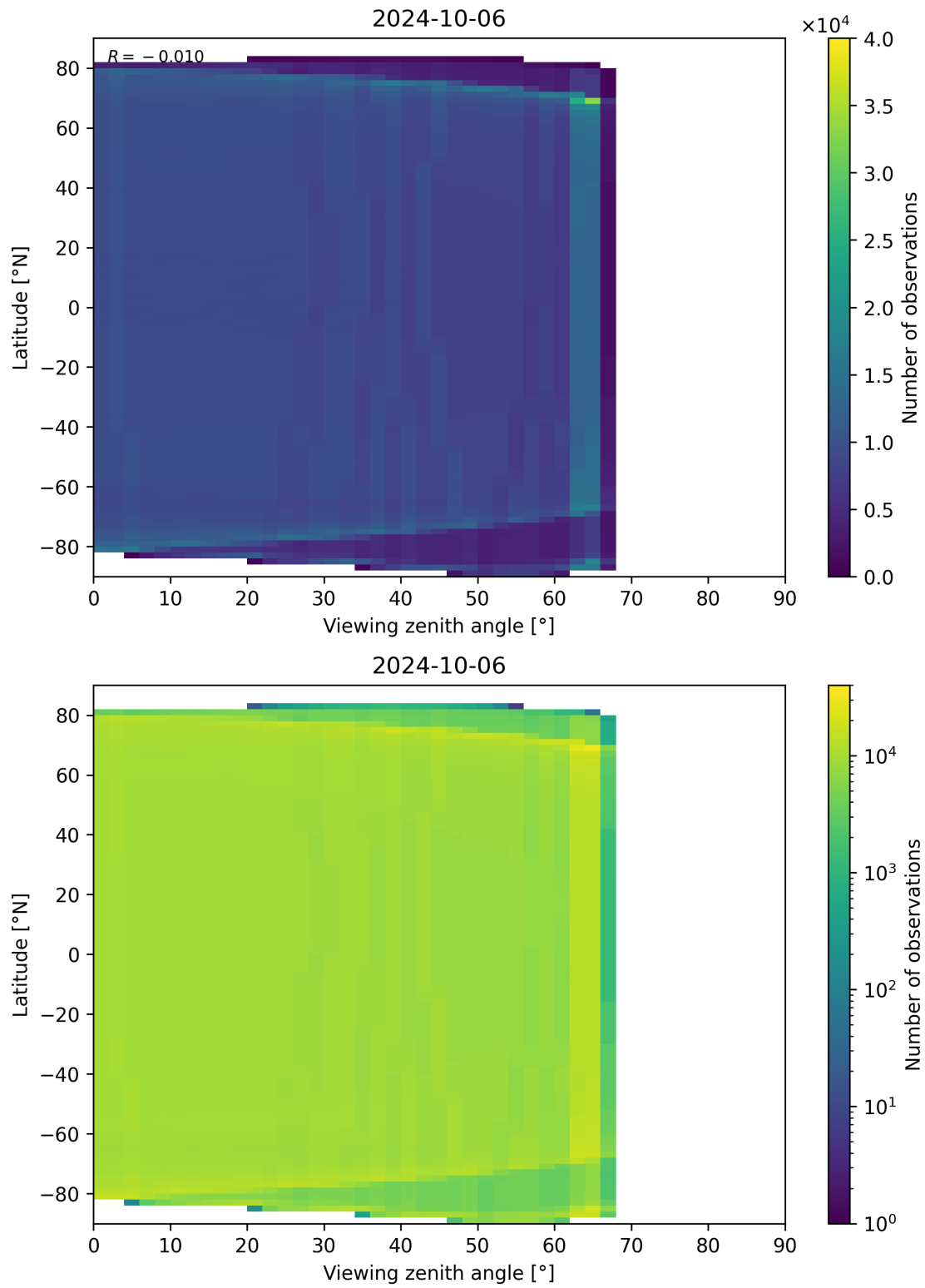
Figure 135: Scatter density plot of “Viewing zenith angle” against “Latitude” for 2024-10-05 to 2024-10-07.
