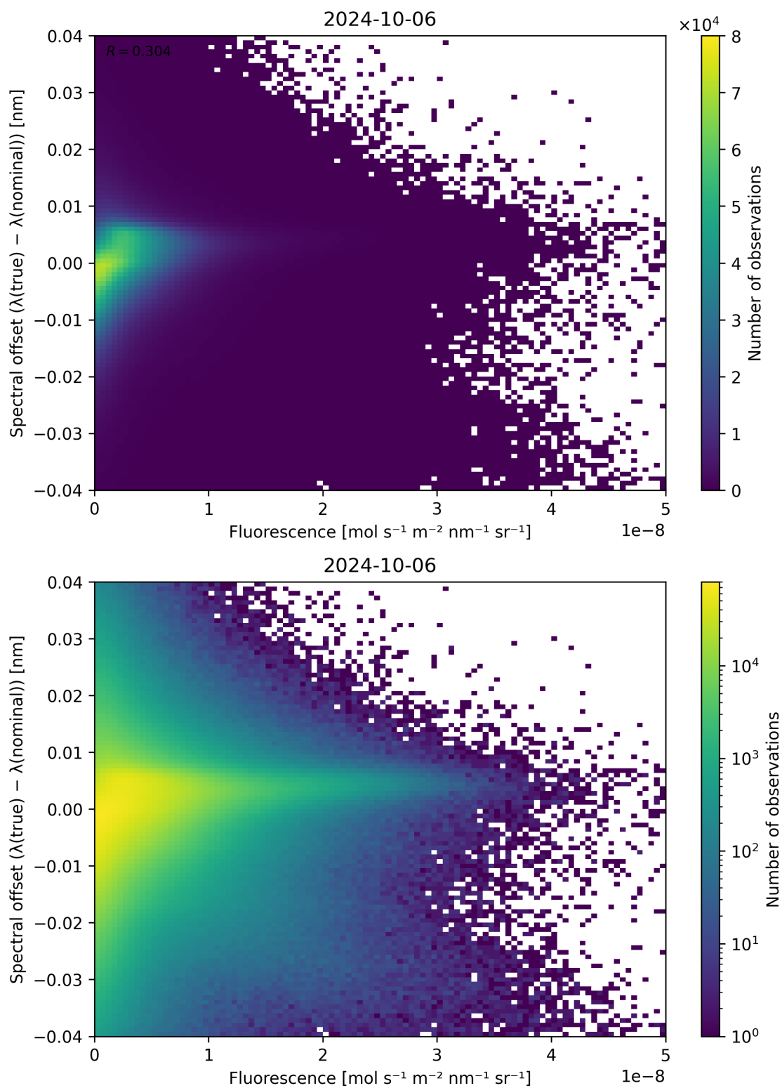
Figure 95: Scatter density plot of “Fluorescence” against “Spectral offset ( \lambda_{\text{true}} - \lambda_{\text{nominal}} )” for 2024-10-05 to 2024-10-07.
