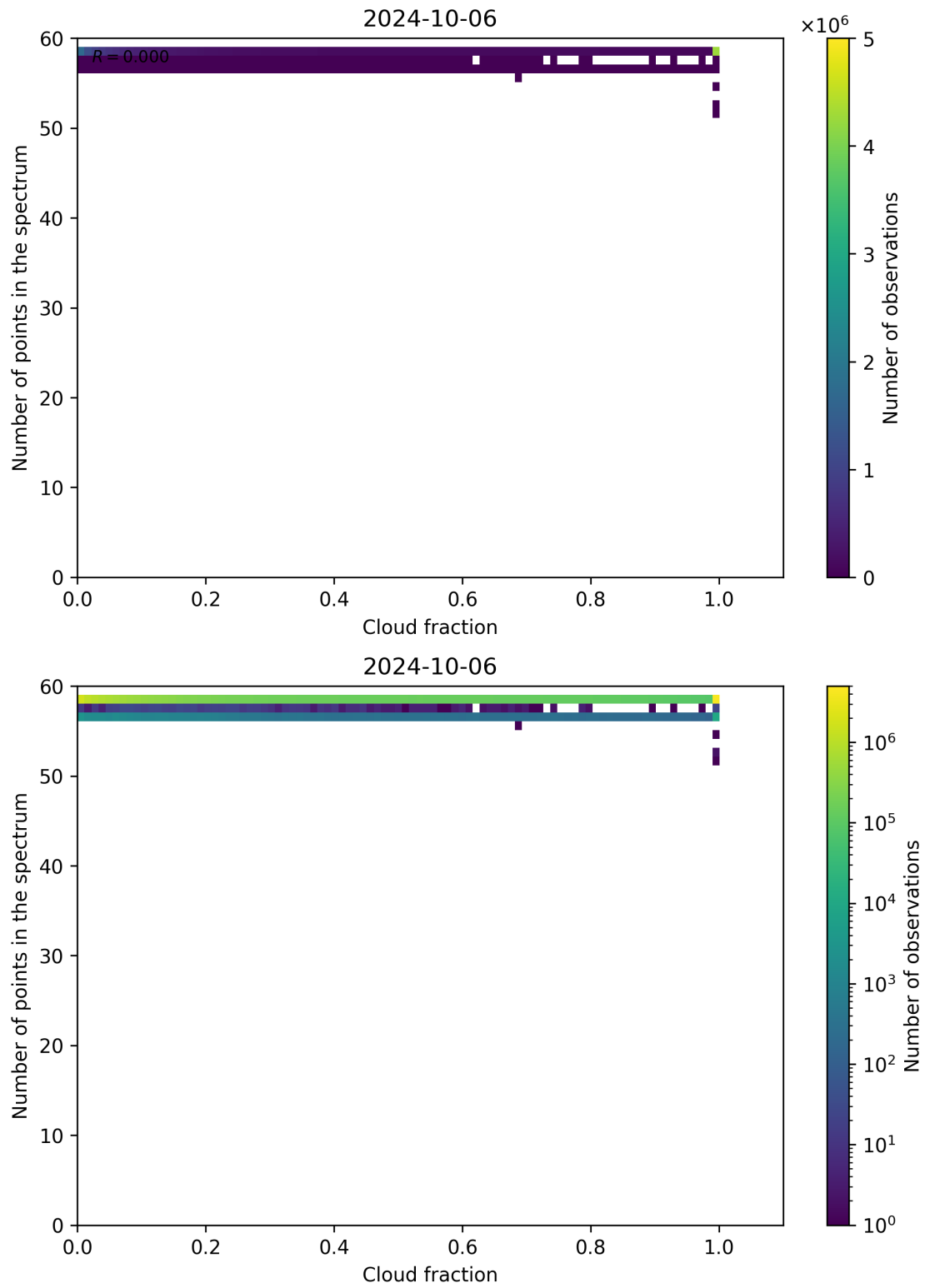
Figure 81: Scatter density plot of “Cloud fraction” against “Number of points in the spectrum” for 2024-10-05 to 2024-10-07.
