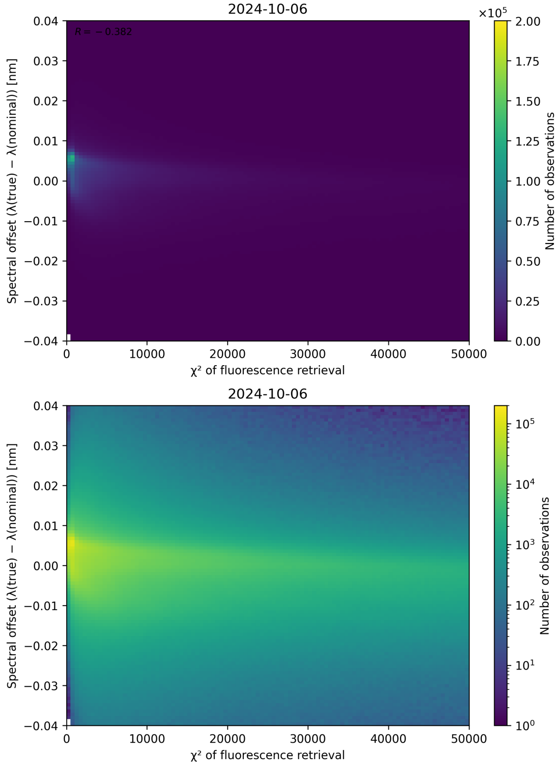
Figure 72: Scatter density plot of “ \chi^2 of fluorescence retrieval” against “Spectral offset ( \lambda_{\text{true}} - \lambda_{\text{nominal}} )” for 2024-10-05 to 2024-10-07.
