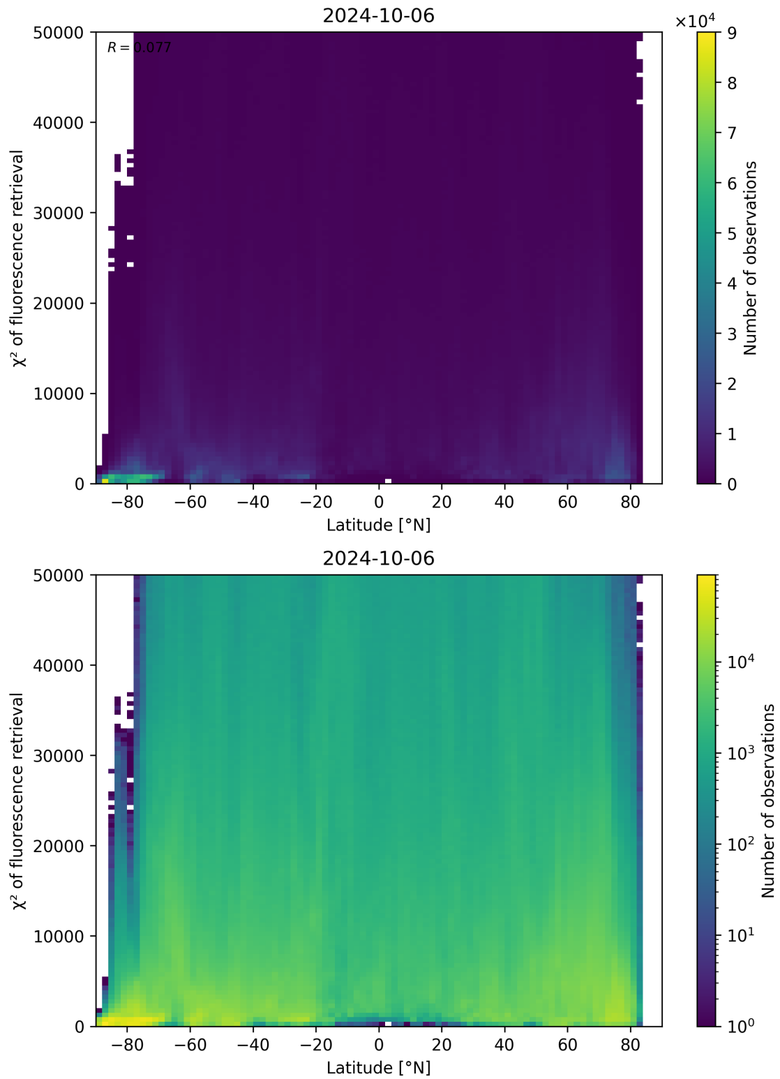
Figure 98: Scatter density plot of “Latitude” against “ \chi^2 of fluorescence retrieval” for 2024-10-05 to 2024-10-07.
