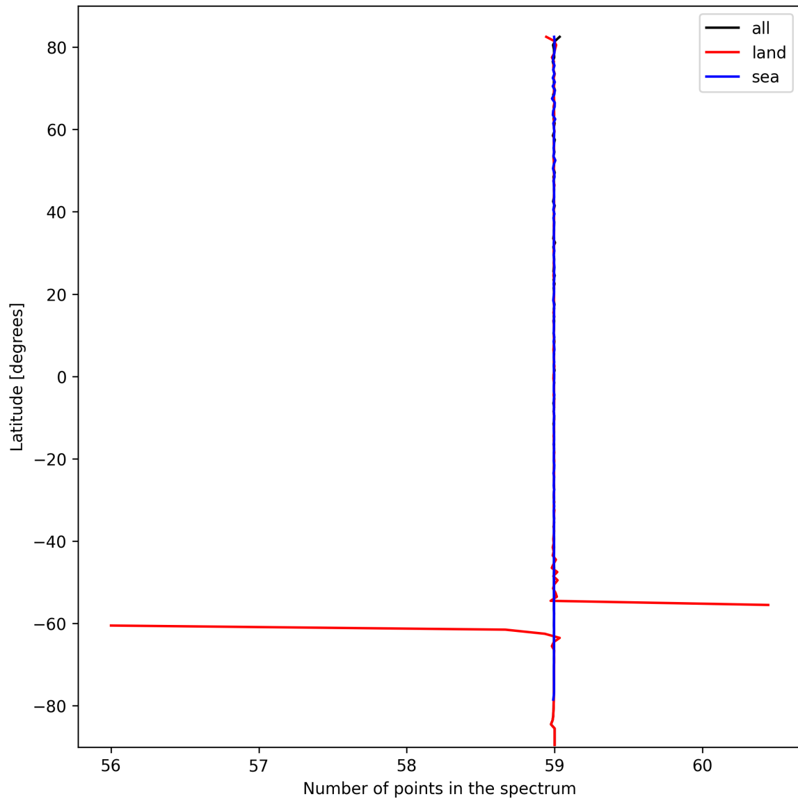
Figure 27: Zonal average of “Number of points in the spectrum” for 2024-10-05 to 2024-10-07.
