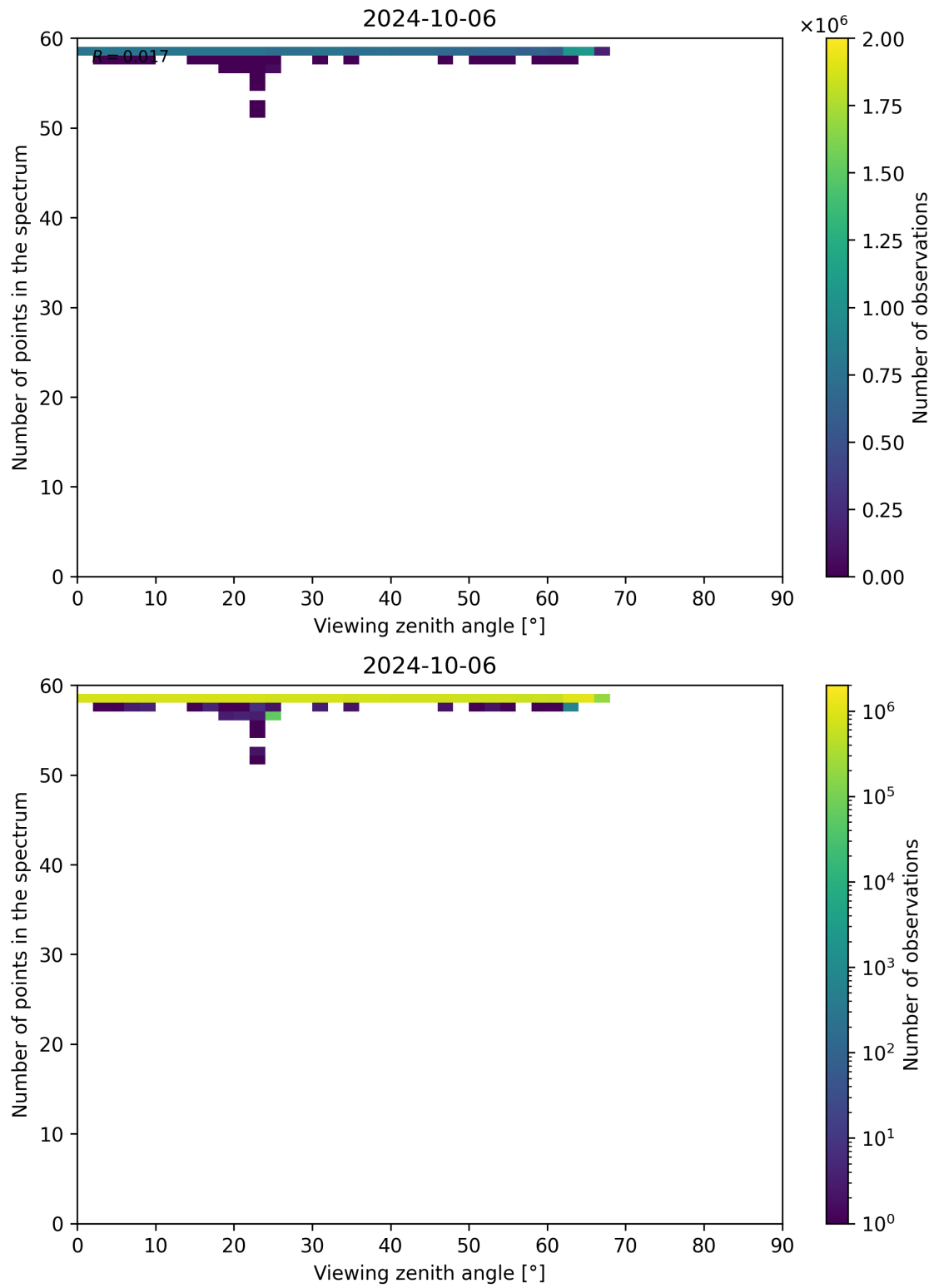
Figure 137: Scatter density plot of “Viewing zenith angle” against “Number of points in the spectrum” for 2024-10-05 to 2024-10-07.
