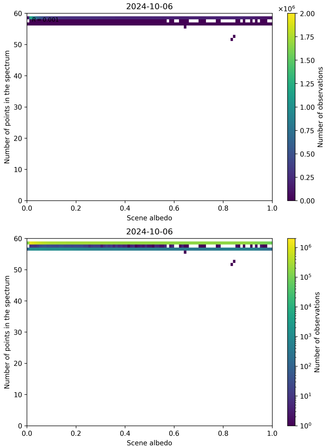
Figure 116: Scatter density plot of “Scene albedo” against “Number of points in the spectrum” for 2024-10-05 to 2024-10-07.
