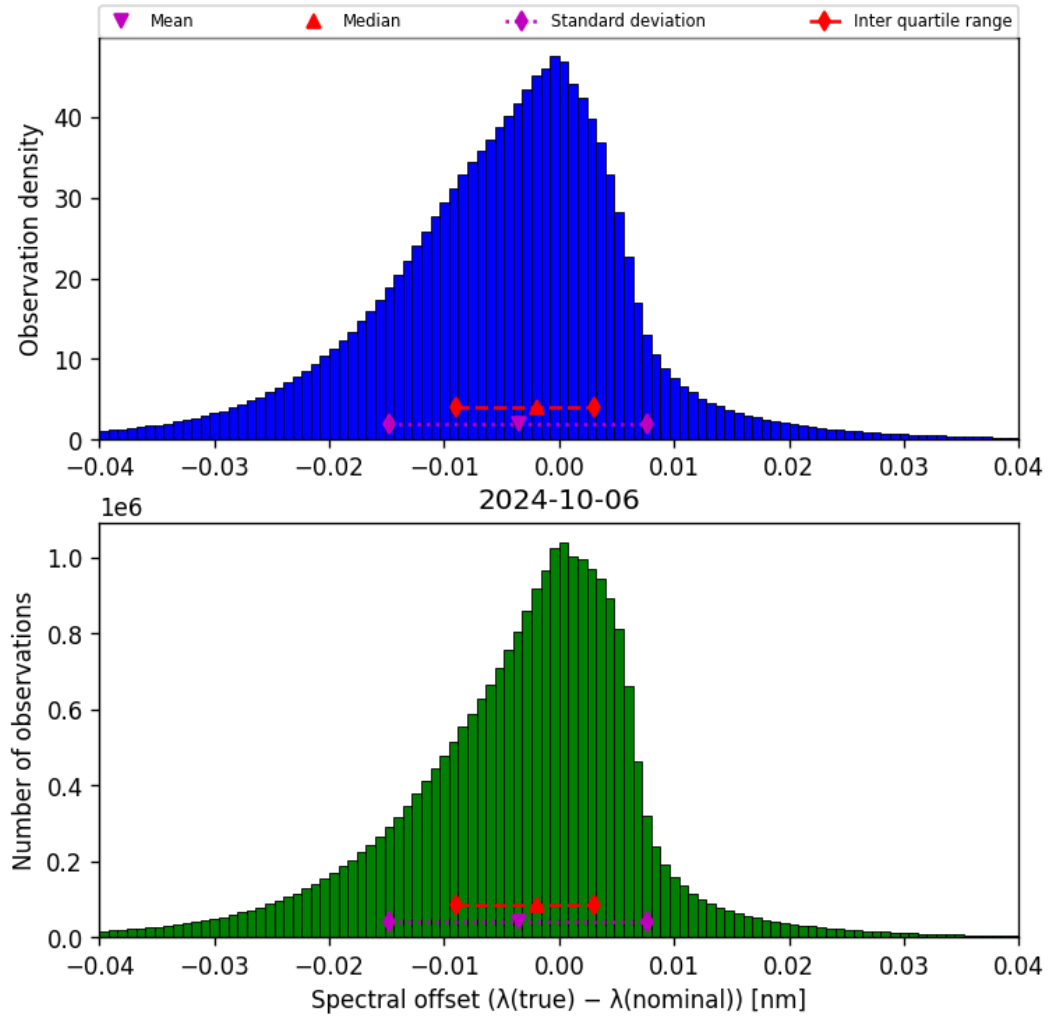
Figure 45: Histogram of “Spectral offset ( \lambda_{\text{true}} - \lambda_{\text{nominal}} )” for 2024-10-05 to 2024-10-07
