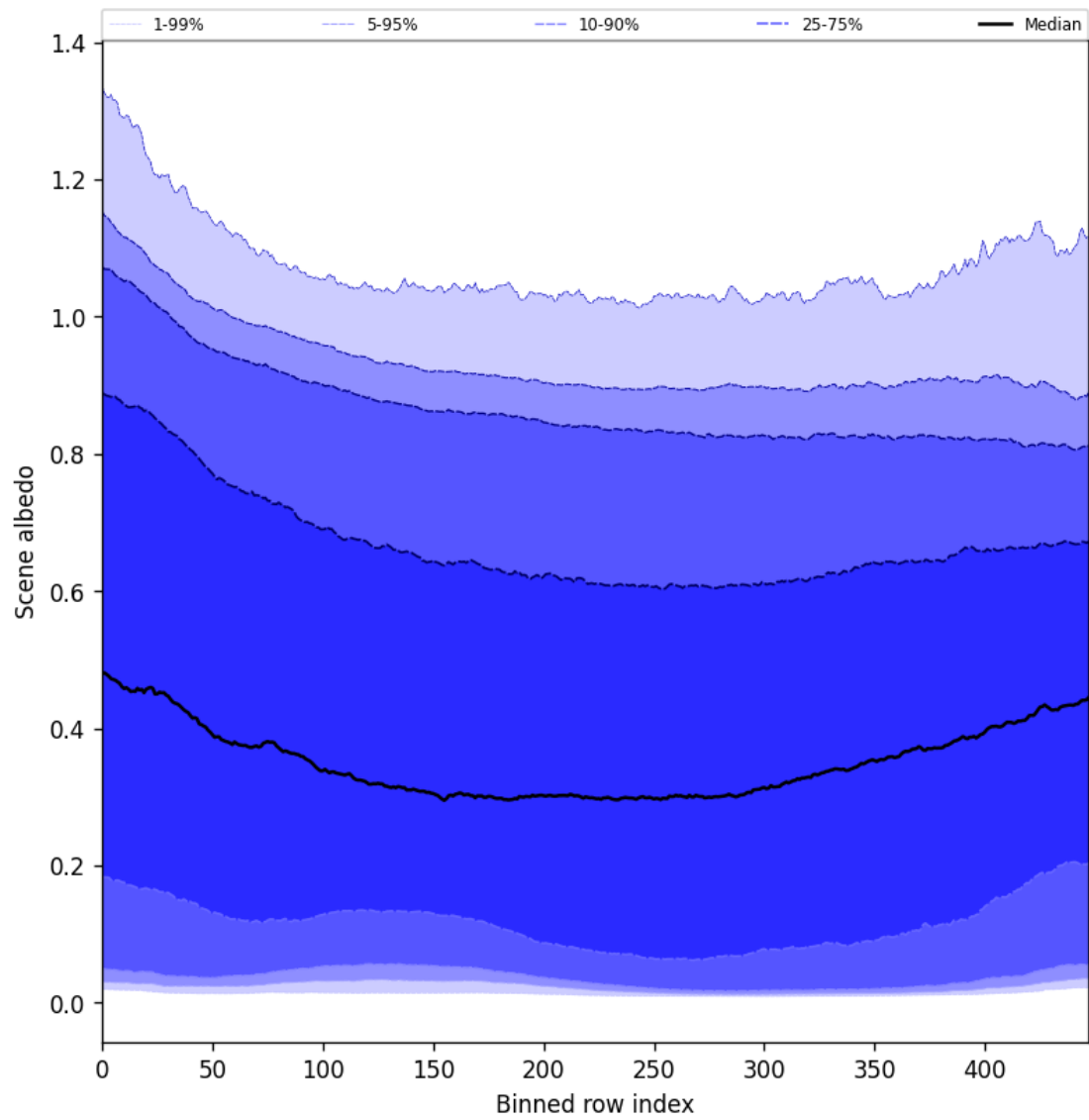
Figure 51: Along track statistics of “Scene albedo” for 2024-10-05 to 2024-10-07
