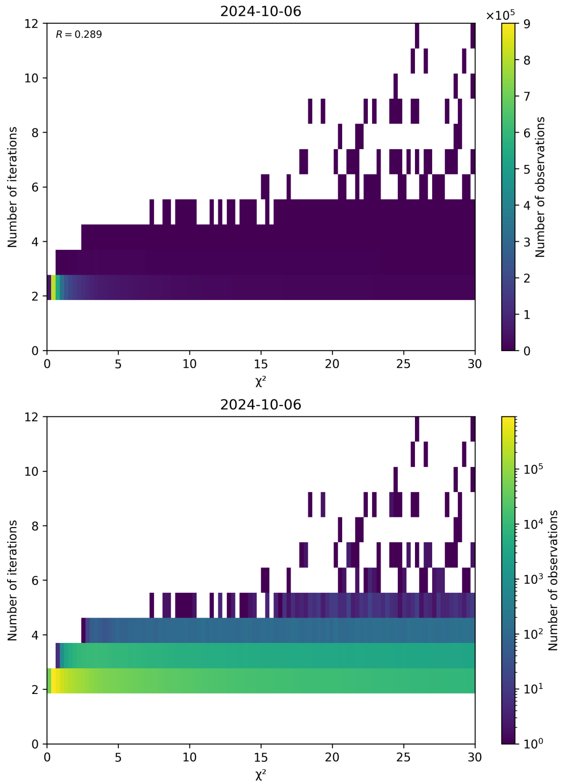
Figure 73: Scatter density plot of “ \chi^2 ” against “Number of iterations” for 2024-10-05 to 2024-10-07.
