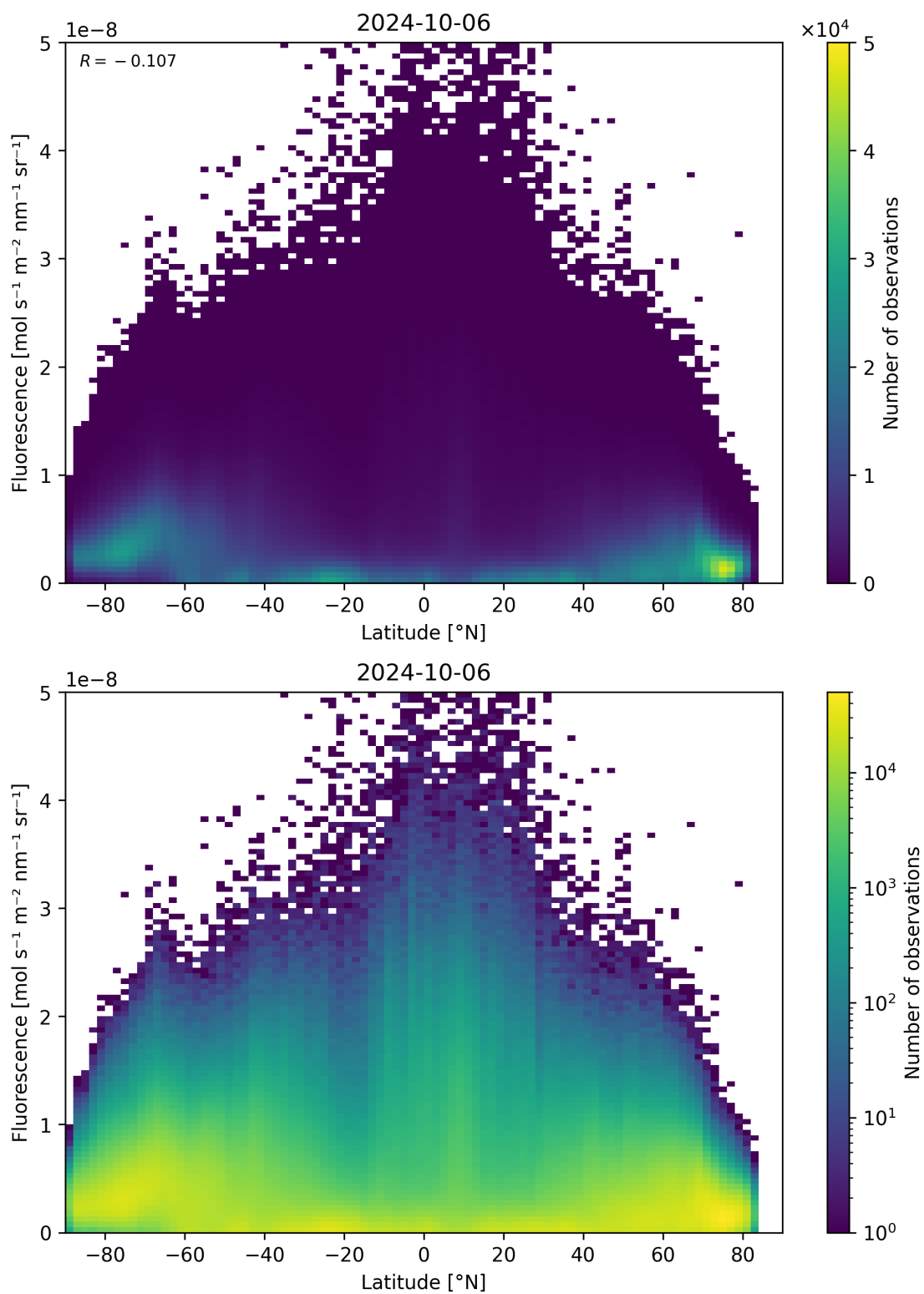
Figure 101: Scatter density plot of “Latitude” against “Fluorescence” for 2024-10-05 to 2024-10-07.
