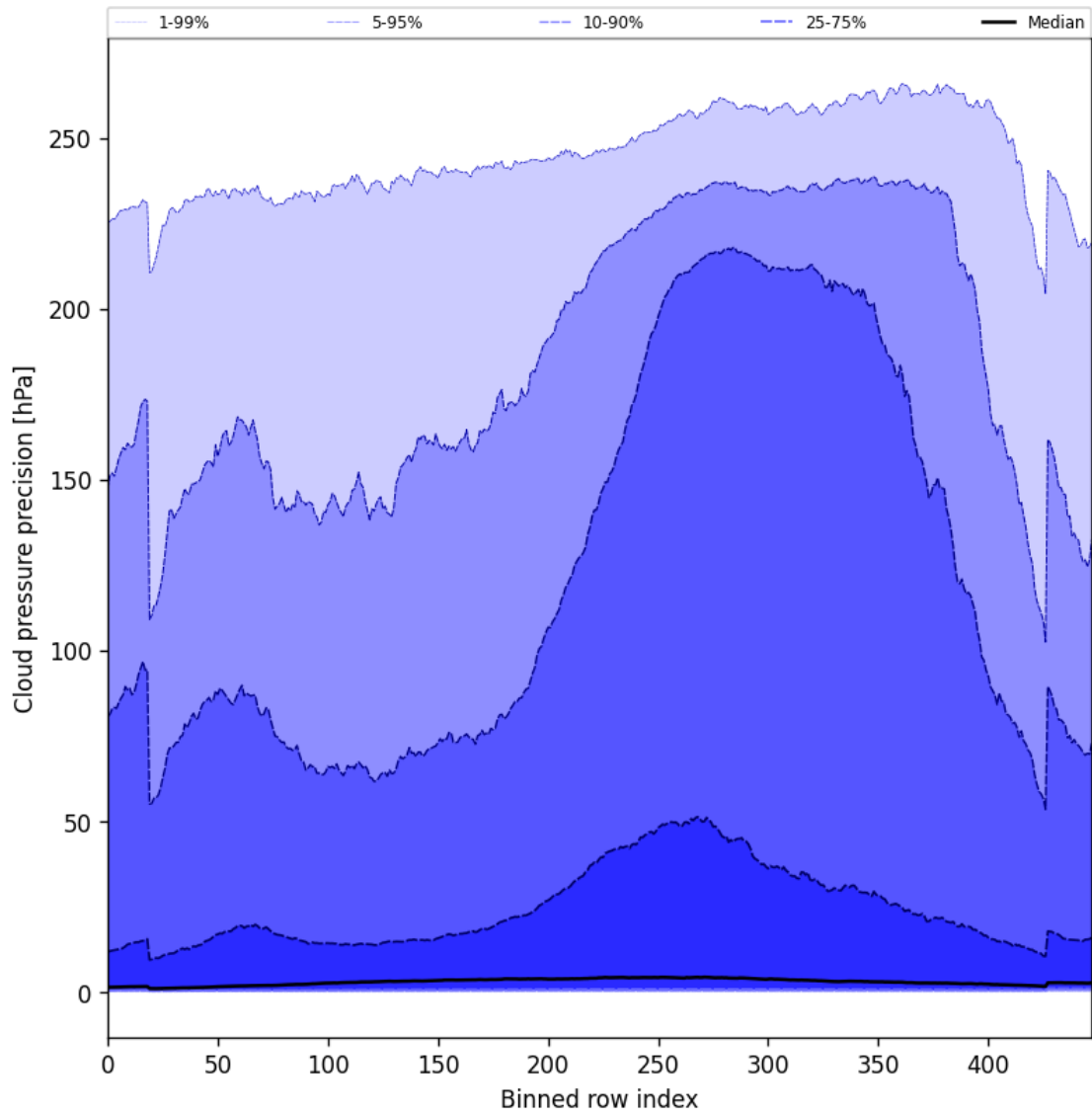
Figure 48: Along track statistics of “Cloud pressure precision” for 2024-10-05 to 2024-10-07
