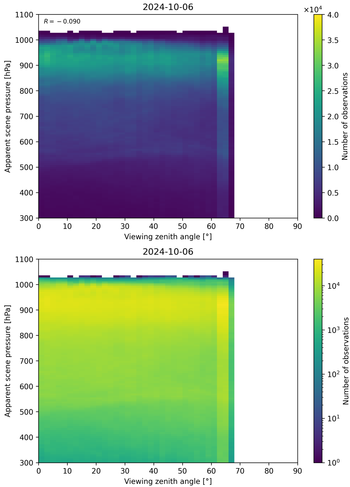
Figure 129: Scatter density plot of “Viewing zenith angle” against “Apparent scene pressure” for 2024-10-05 to 2024-10-07.
