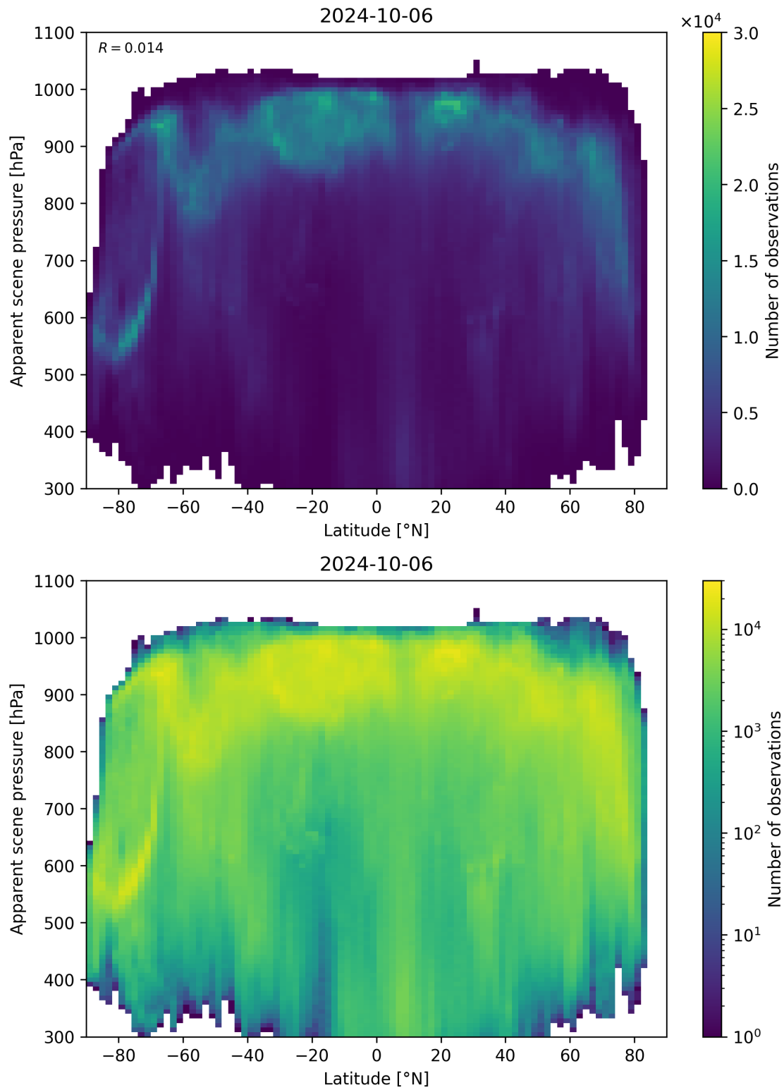
Figure 96: Scatter density plot of “Latitude” against “Apparent scene pressure” for 2024-10-05 to 2024-10-07.
