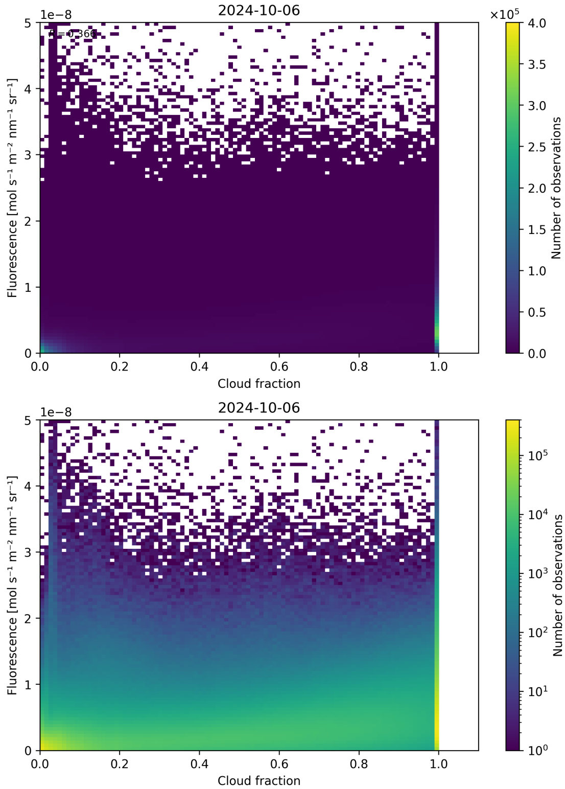
Figure 79: Scatter density plot of “Cloud fraction” against “Fluorescence” for 2024-10-05 to 2024-10-07.
