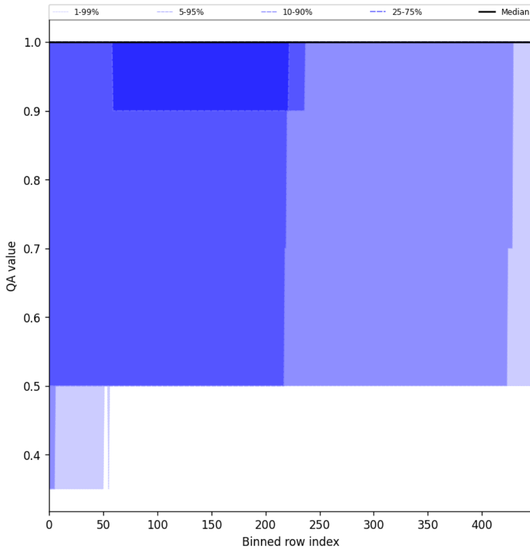
Figure 46: Along track statistics of “QA value” for 2024-10-05 to 2024-10-07
