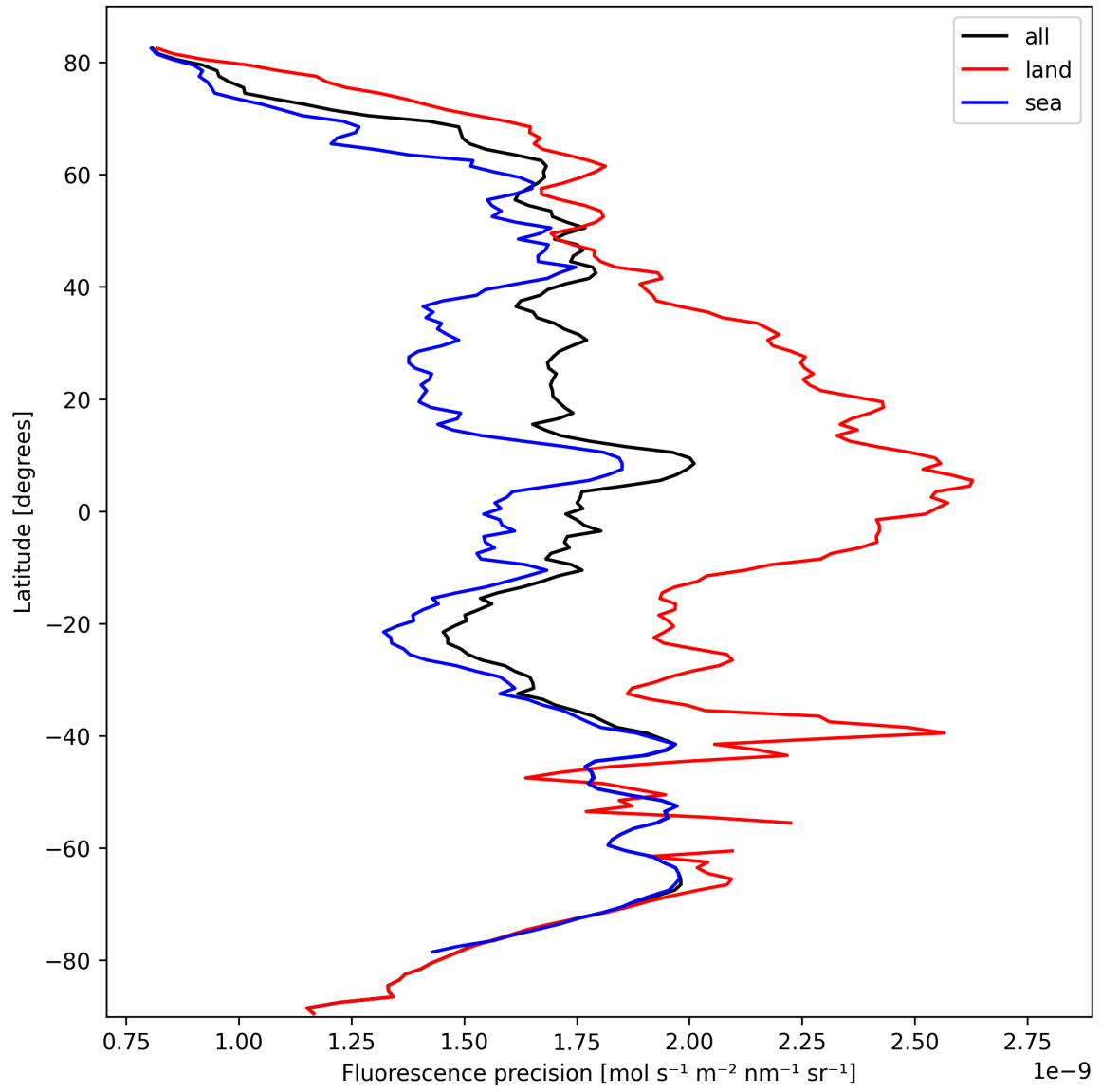
Figure 24: Zonal average of “Fluorescence precision” for 2024-10-05 to 2024-10-07.
