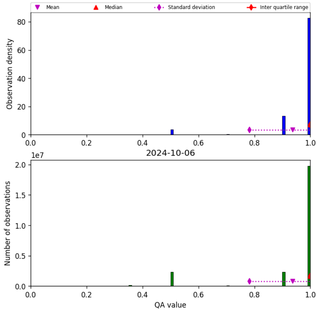
Figure 29: Histogram of “QA value” for 2024-10-05 to 2024-10-07
