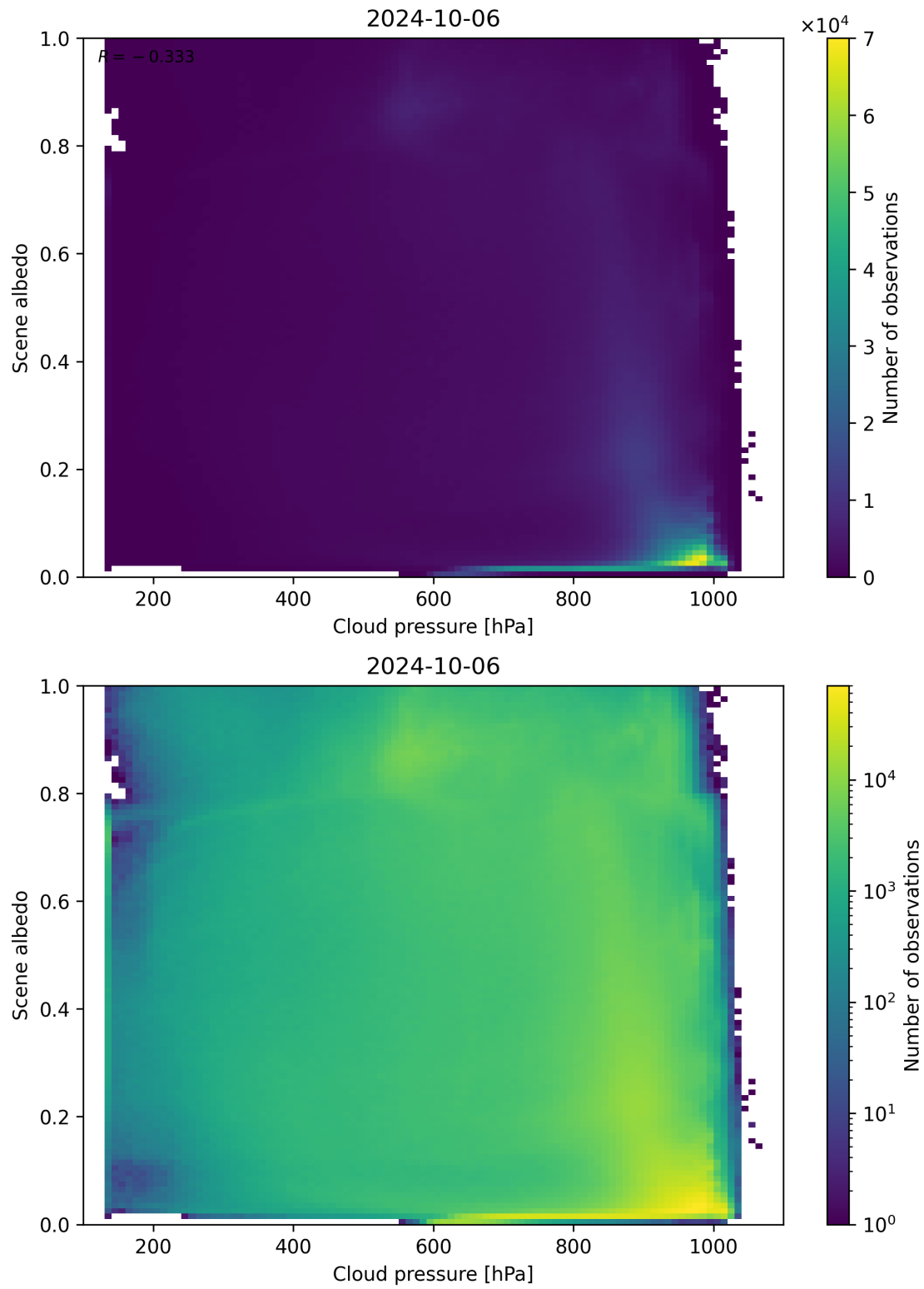
Figure 91: Scatter density plot of “Cloud pressure” against “Scene albedo” for 2024-10-05 to 2024-10-07.
