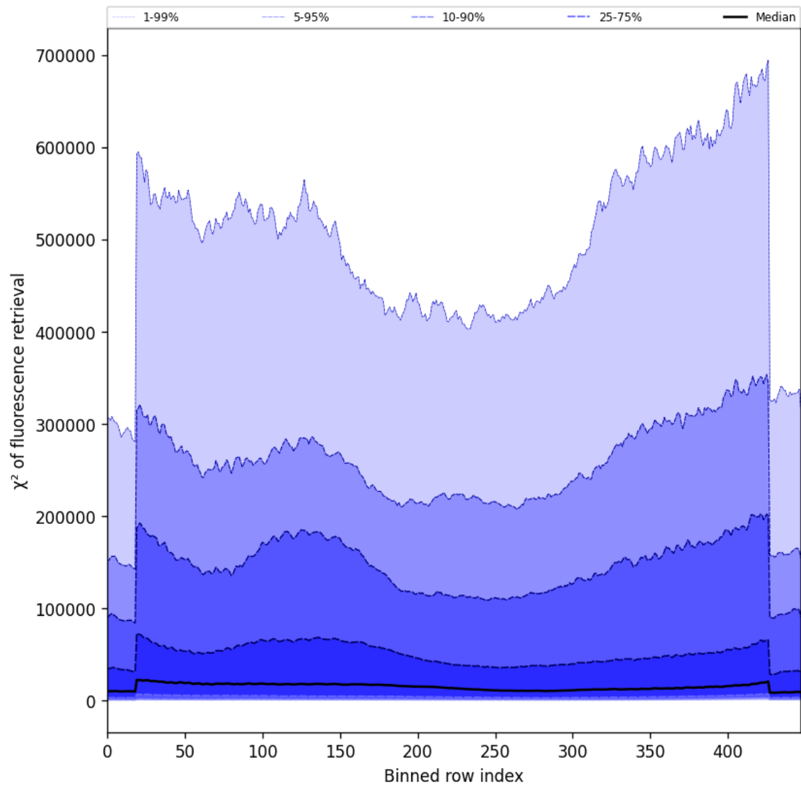
Figure 59: Along track statistics of “ \chi^2 of fluorescence retrieval” for 2024-10-05 to 2024-10-07
