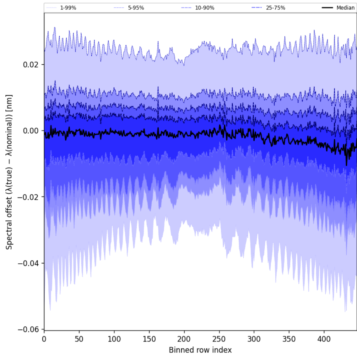
Figure 62: Along track statistics of “Spectral offset ( \lambda_{\text{true}} - \lambda_{\text{nominal}} )” for 2024-10-05 to 2024-10-07
