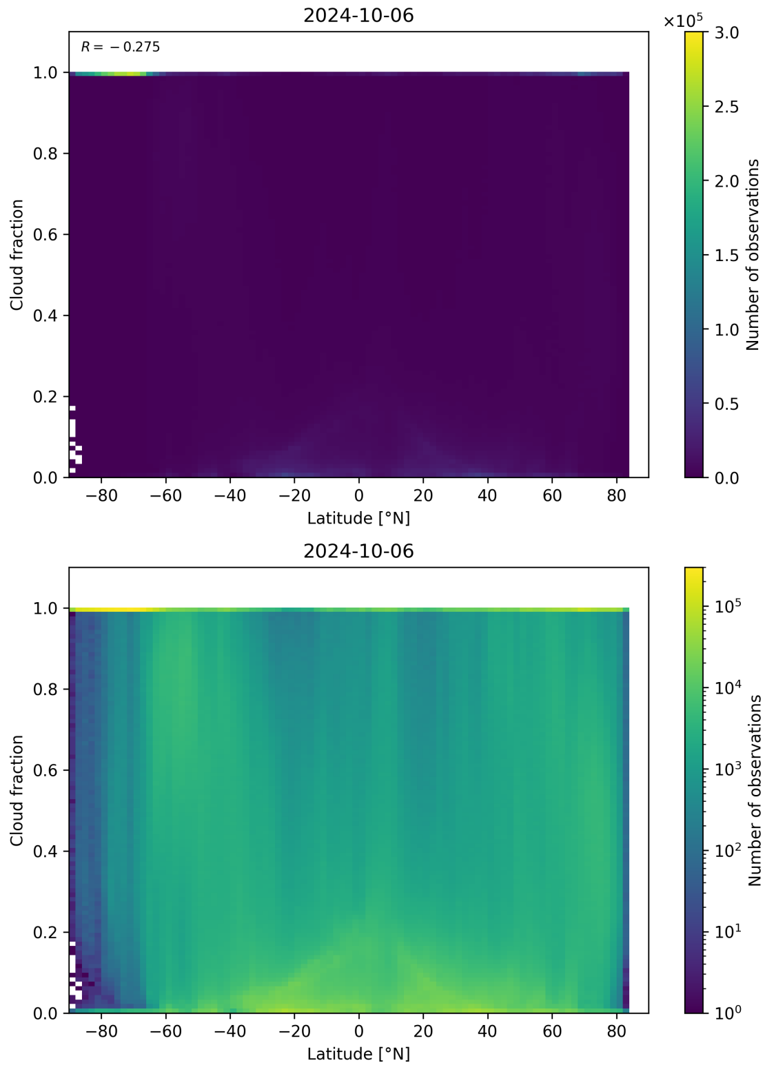
Figure 99: Scatter density plot of “Latitude” against “Cloud fraction” for 2024-10-05 to 2024-10-07.
