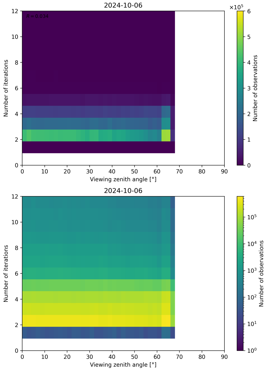
Figure 136: Scatter density plot of “Viewing zenith angle” against “Number of iterations” for 2024-10-05 to 2024-10-07.
