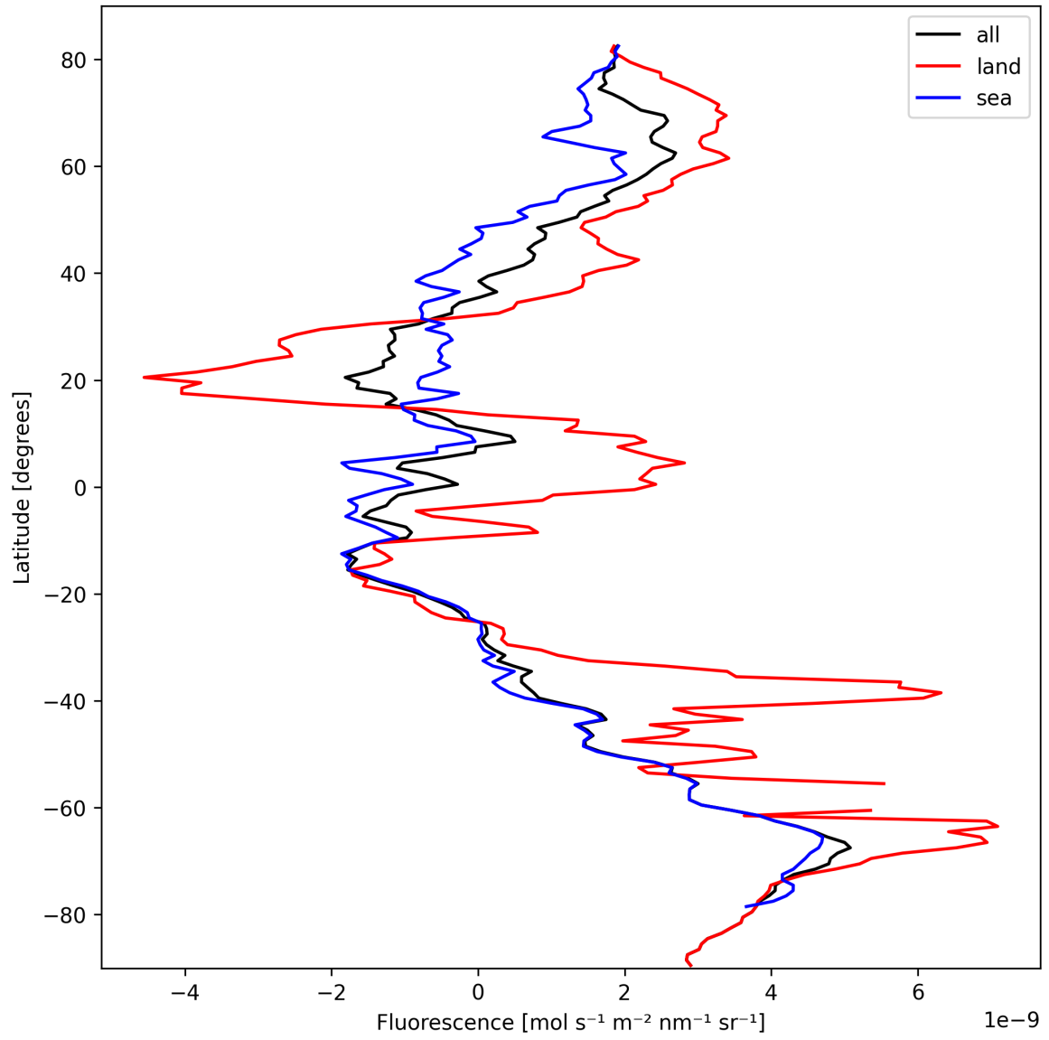
Figure 23: Zonal average of “Fluorescence” for 2024-10-05 to 2024-10-07.
