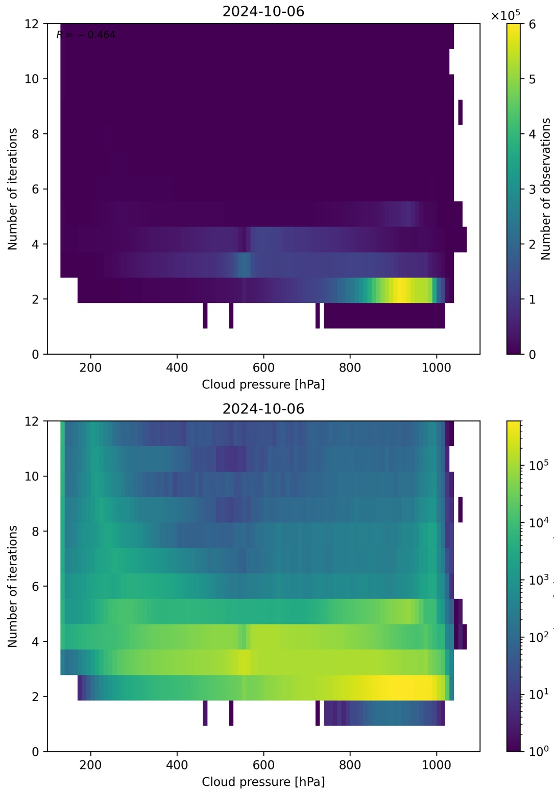
Figure 89: Scatter density plot of “Cloud pressure” against “Number of iterations” for 2024-10-05 to 2024-10-07.
