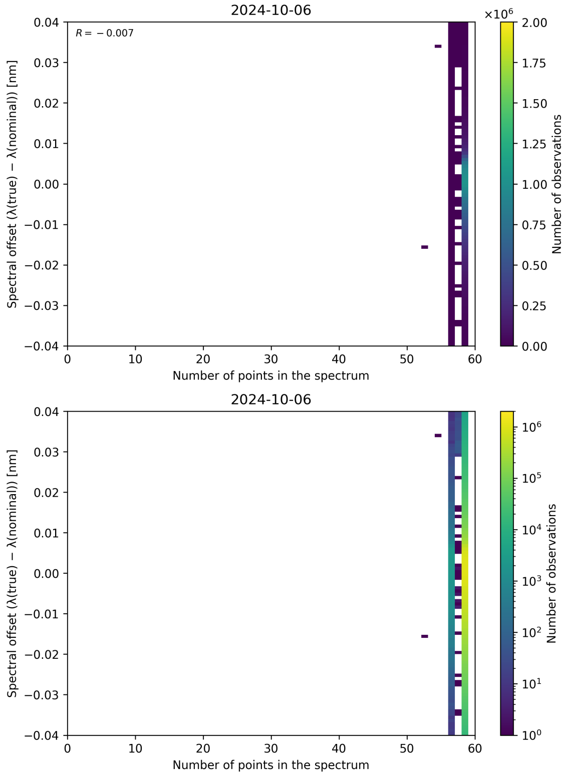
Figure 110: Scatter density plot of “Number of points in the spectrum” against “Spectral offset ( \lambda_{\text{true}} - \lambda_{\text{nominal}} )” for 2024-10-05 to 2024-10-07.
