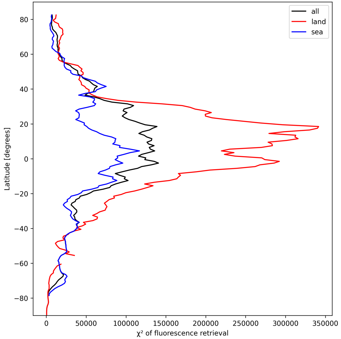
Figure 25: Zonal average of “ \chi^2 of fluorescence retrieval” for 2024-10-05 to 2024-10-07.
