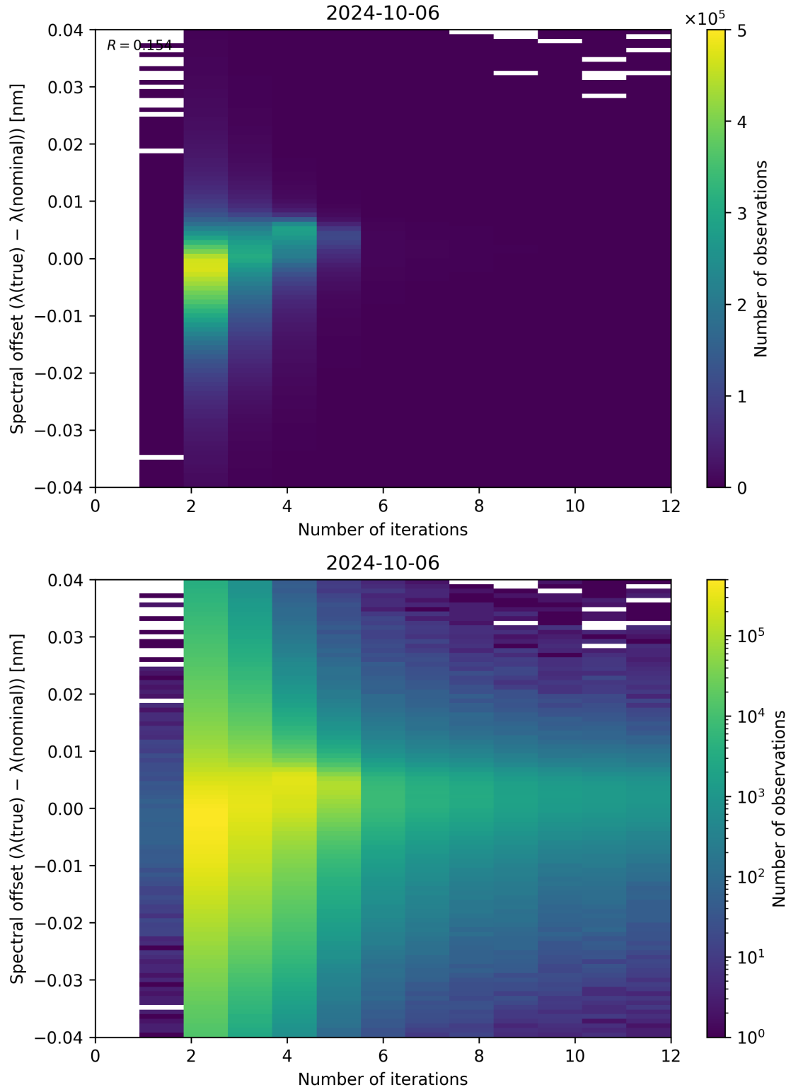
Figure 109: Scatter density plot of “Number of iterations” against “Spectral offset ( \lambda_{\text{true}} - \lambda_{\text{nominal}} )” for 2024-10-05 to 2024-10-07.
