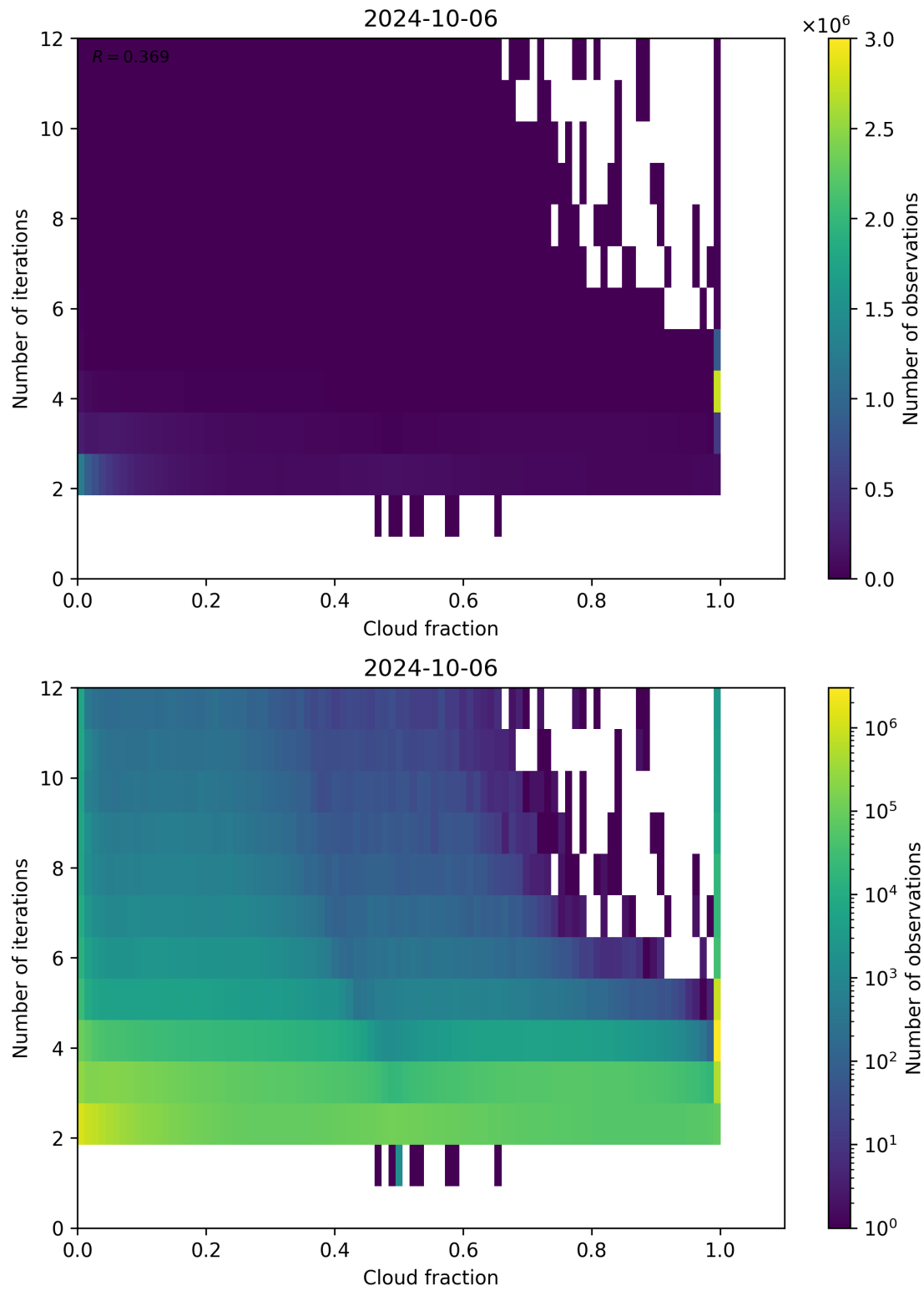
Figure 80: Scatter density plot of “Cloud fraction” against “Number of iterations” for 2024-10-05 to 2024-10-07.
