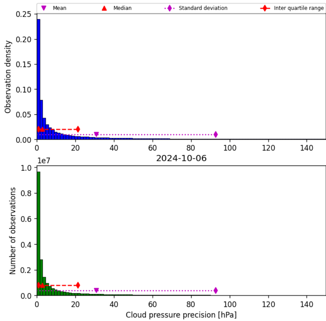
Figure 31: Histogram of “Cloud pressure precision” for 2024-10-05 to 2024-10-07
