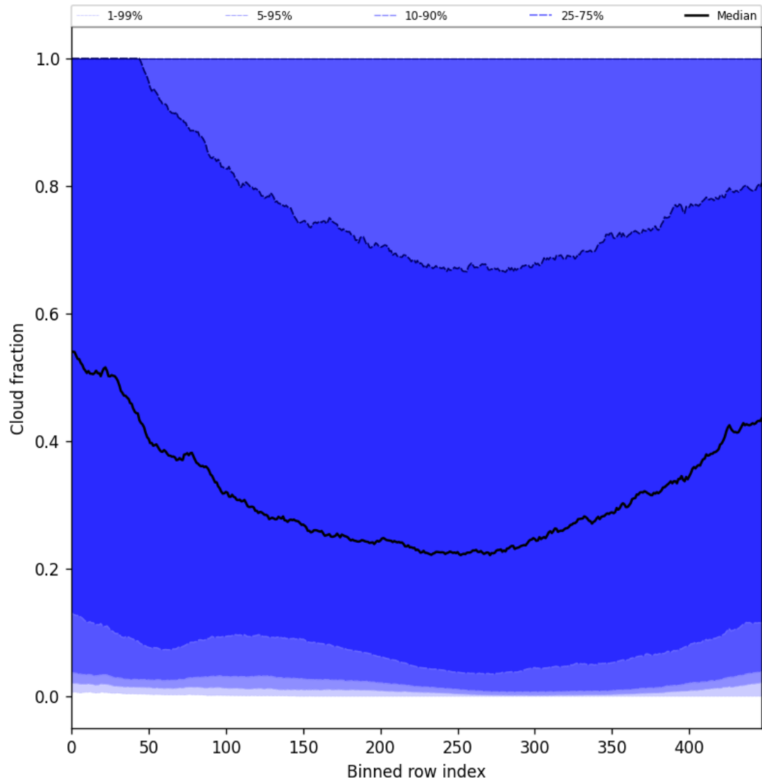
Figure 49: Along track statistics of “Cloud fraction” for 2024-10-05 to 2024-10-07
