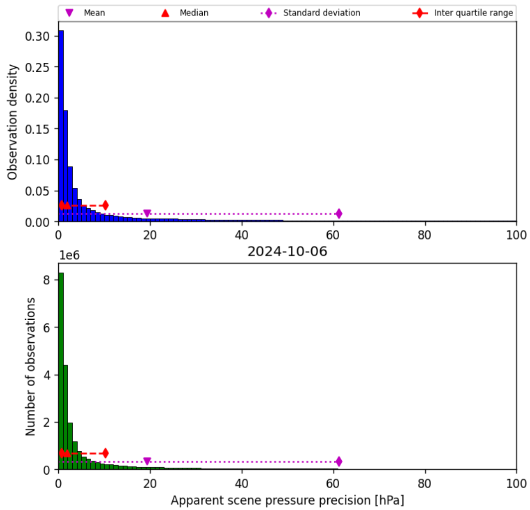
Figure 37: Histogram of “Apparent scene pressure precision” for 2024-10-05 to 2024-10-07
