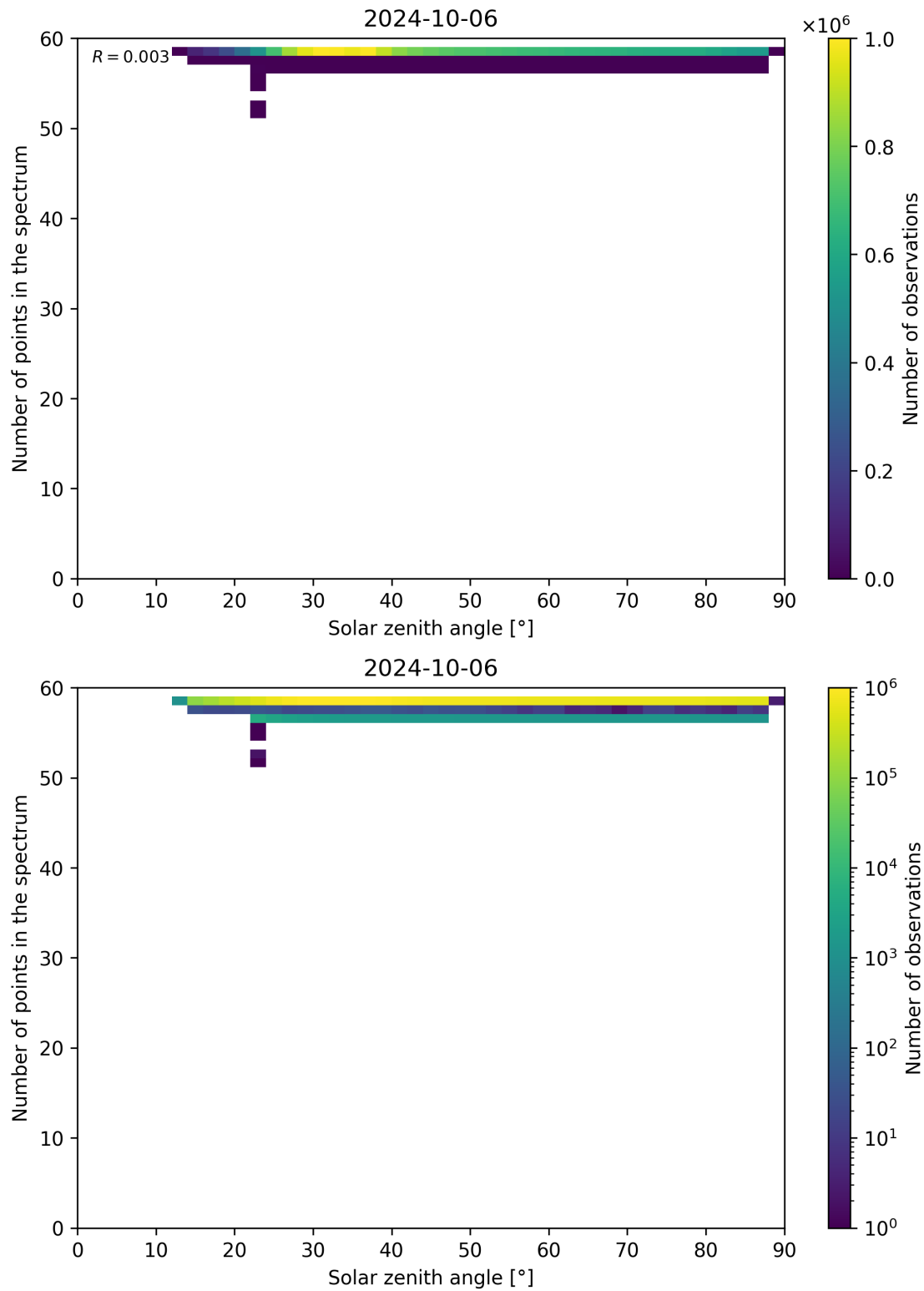
Figure 126: Scatter density plot of “Solar zenith angle” against “Number of points in the spectrum” for 2024-10-05 to 2024-10-07.
