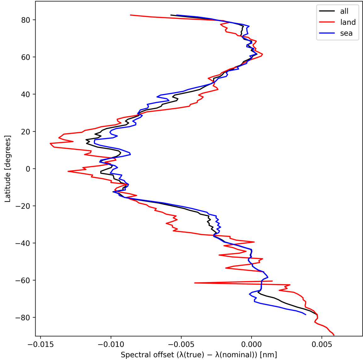
Figure 28: Zonal average of “Spectral offset ( \lambda_{\text{true}} - \lambda_{\text{nominal}} )” for 2024-10-05 to 2024-10-07.
