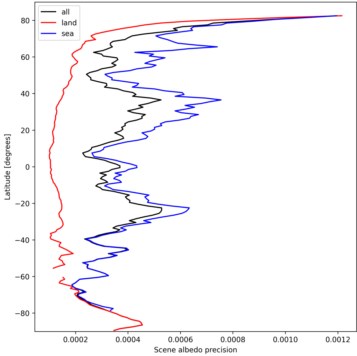
Figure 18: Zonal average of “Scene albedo precision” for 2024-10-05 to 2024-10-07.
