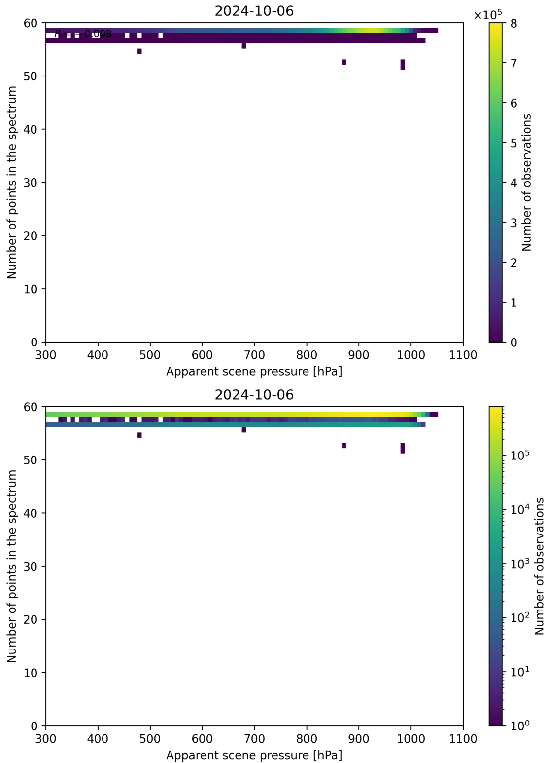
Figure 67: Scatter density plot of “Apparent scene pressure” against “Number of points in the spectrum” for 2024-10-05 to 2024-10-07.
