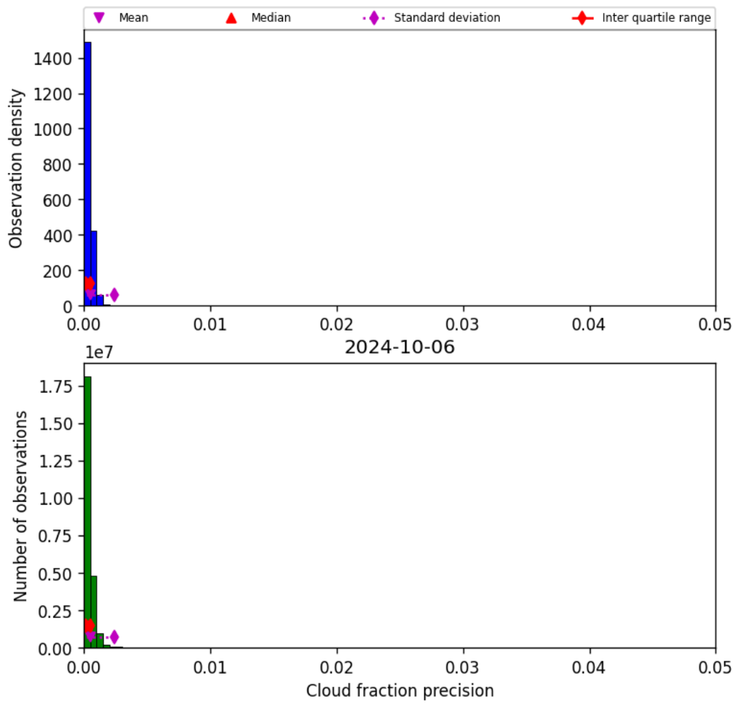
Figure 33: Histogram of “Cloud fraction precision” for 2024-10-05 to 2024-10-07
