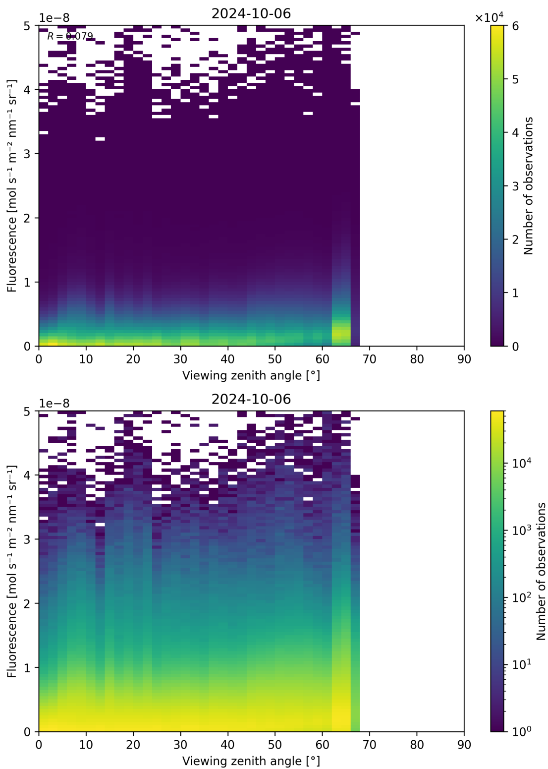
Figure 134: Scatter density plot of “Viewing zenith angle” against “Fluorescence” for 2024-10-05 to 2024-10-07.
