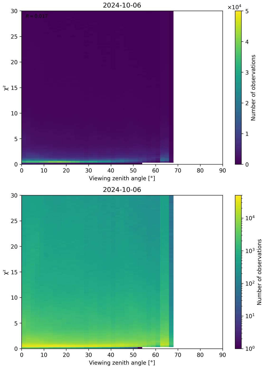
Figure 130: Scatter density plot of “Viewing zenith angle” against “ \chi^2 ” for 2024-10-05 to 2024-10-07.
