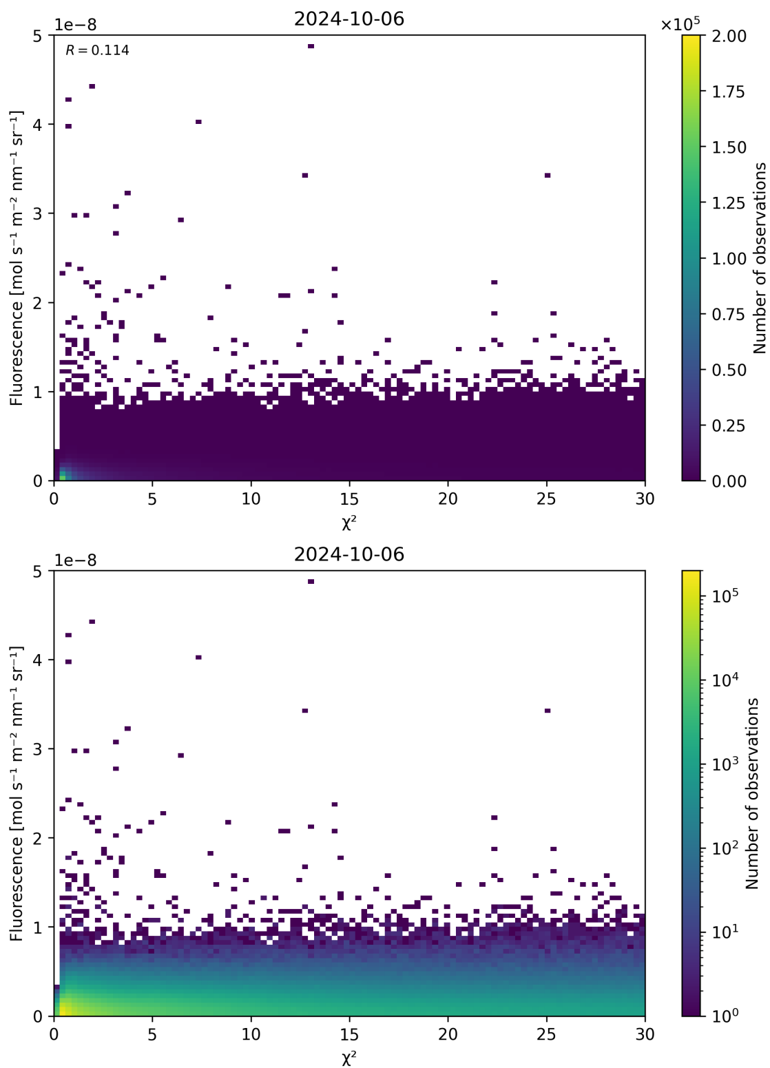
Figure 70: Scatter density plot of “ \chi^2 ” against “Fluorescence” for 2024-10-05 to 2024-10-07.
