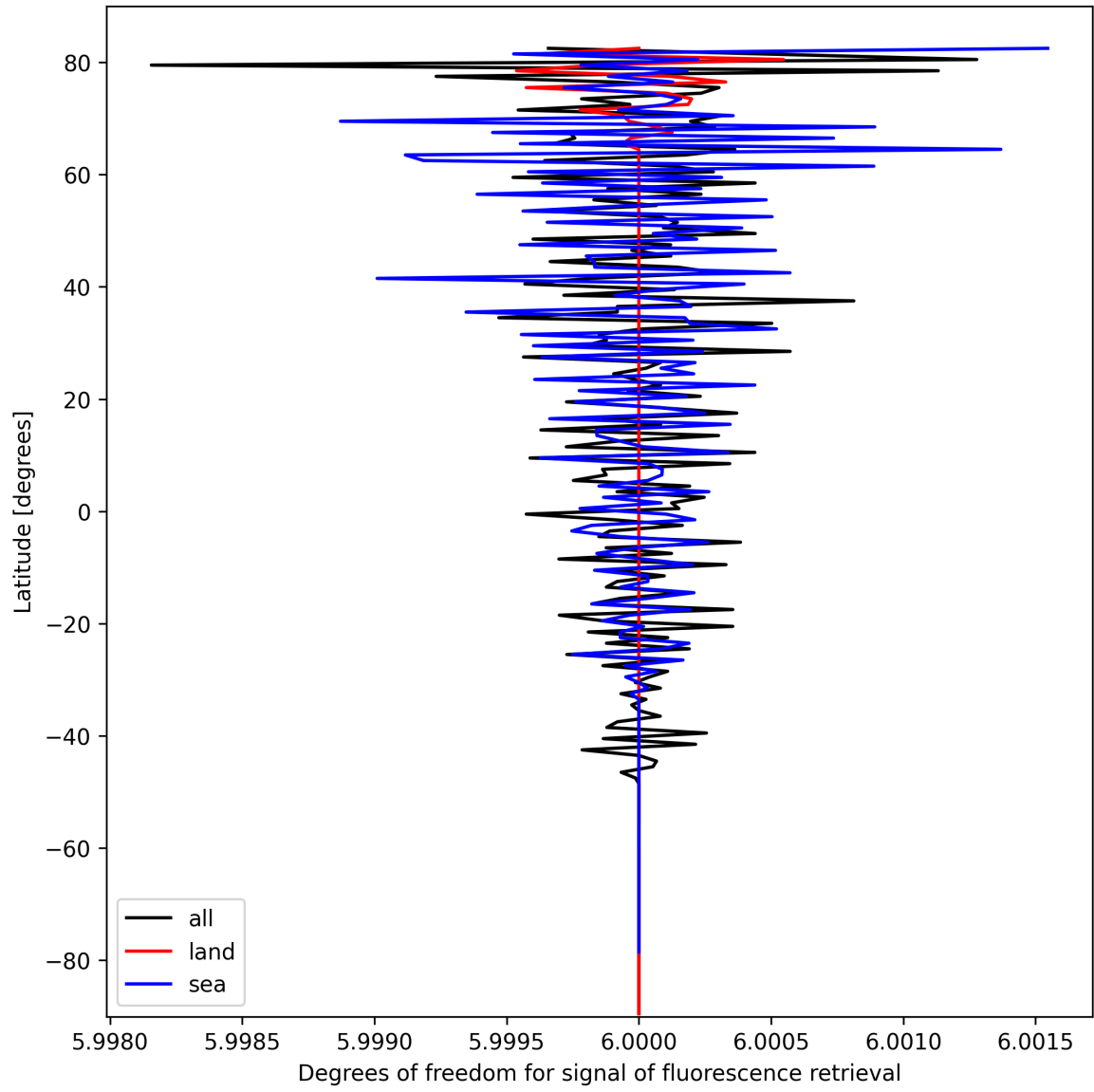
Figure 26: Zonal average of “Degrees of freedom for signal of fluorescence retrieval” for 2024-10-05 to 2024-10-07.
