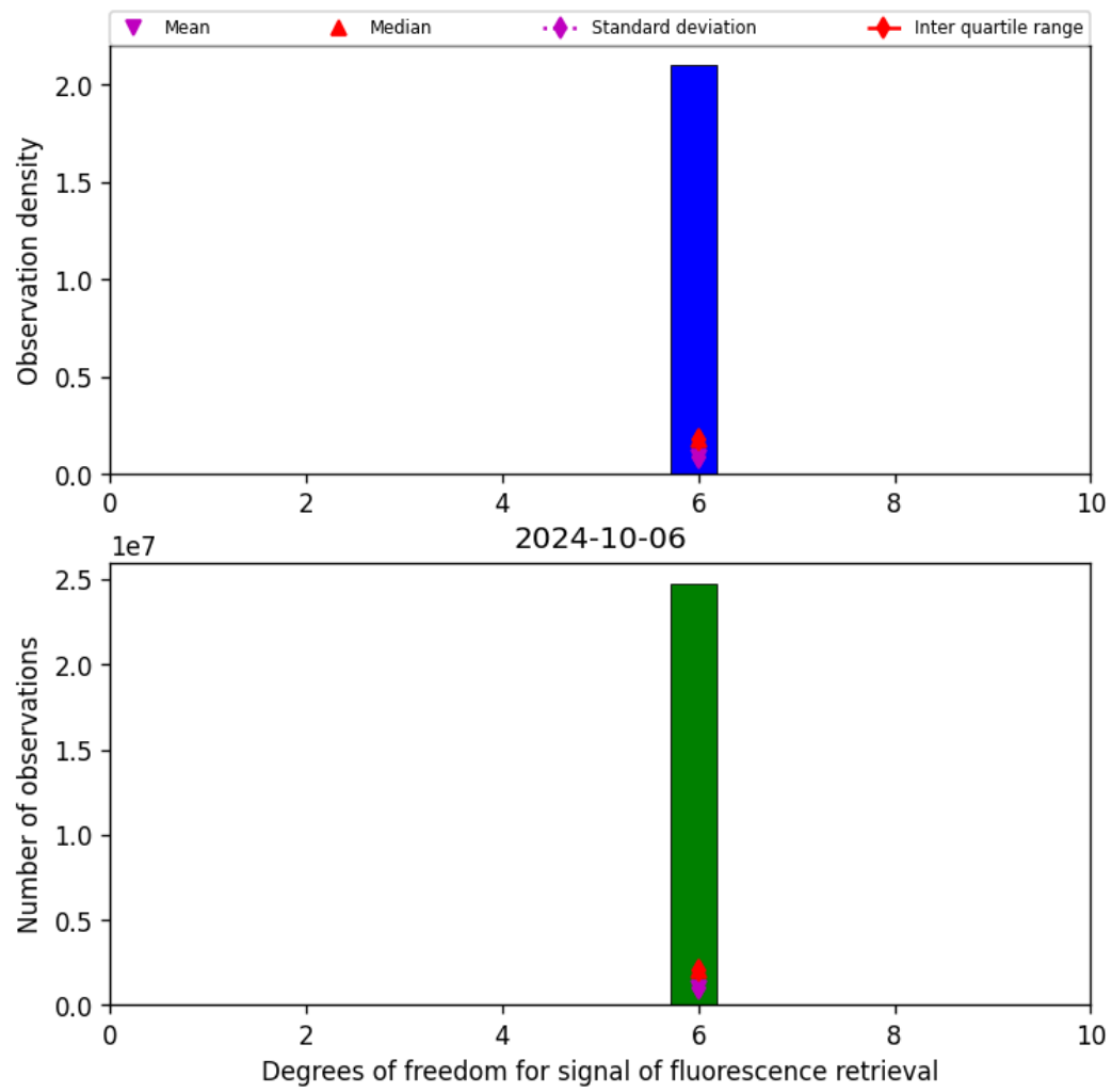
Figure 43: Histogram of “Degrees of freedom for signal of fluorescence retrieval” for 2024-10-05 to 2024-10-07
