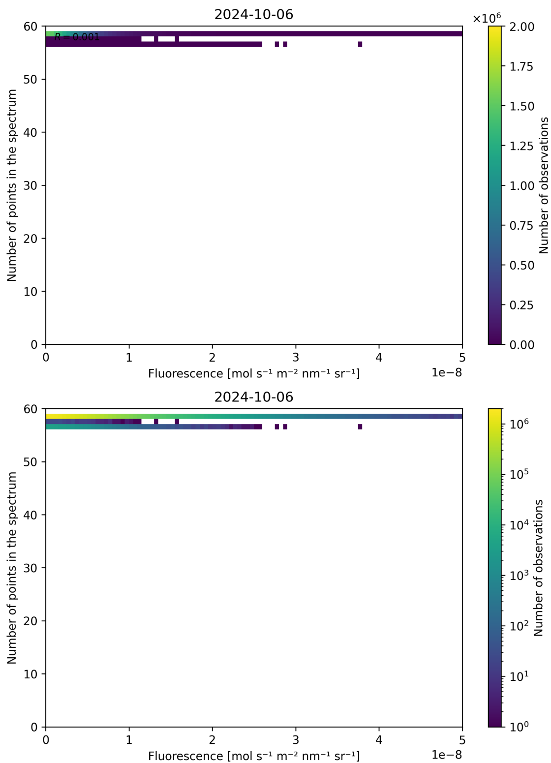
Figure 94: Scatter density plot of “Fluorescence” against “Number of points in the spectrum” for 2024-10-05 to 2024-10-07.
