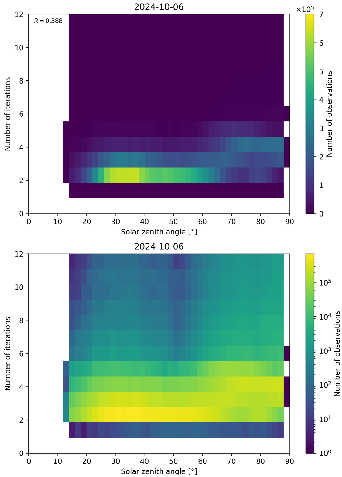
Figure 125: Scatter density plot of “Solar zenith angle” against “Number of iterations” for 2024-10-05 to 2024-10-07.
