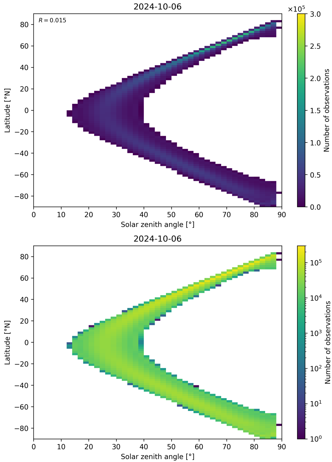
Figure 124: Scatter density plot of “Solar zenith angle” against “Latitude” for 2024-10-05 to 2024-10-07.
