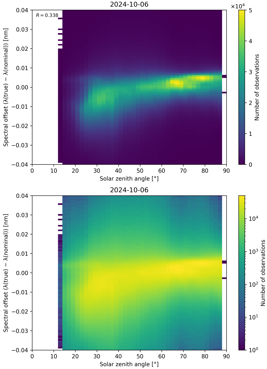
Figure 128: Scatter density plot of “Solar zenith angle” against “Spectral offset ( \lambda_{\text{true}} - \lambda_{\text{nominal}} )” for 2024-10-05 to 2024-10-07.
