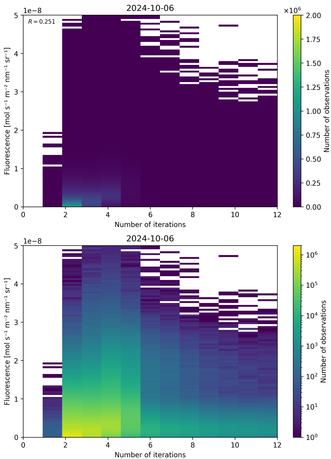
Figure 107: Scatter density plot of “Number of iterations” against “Fluorescence” for 2024-10-05 to 2024-10-07.
