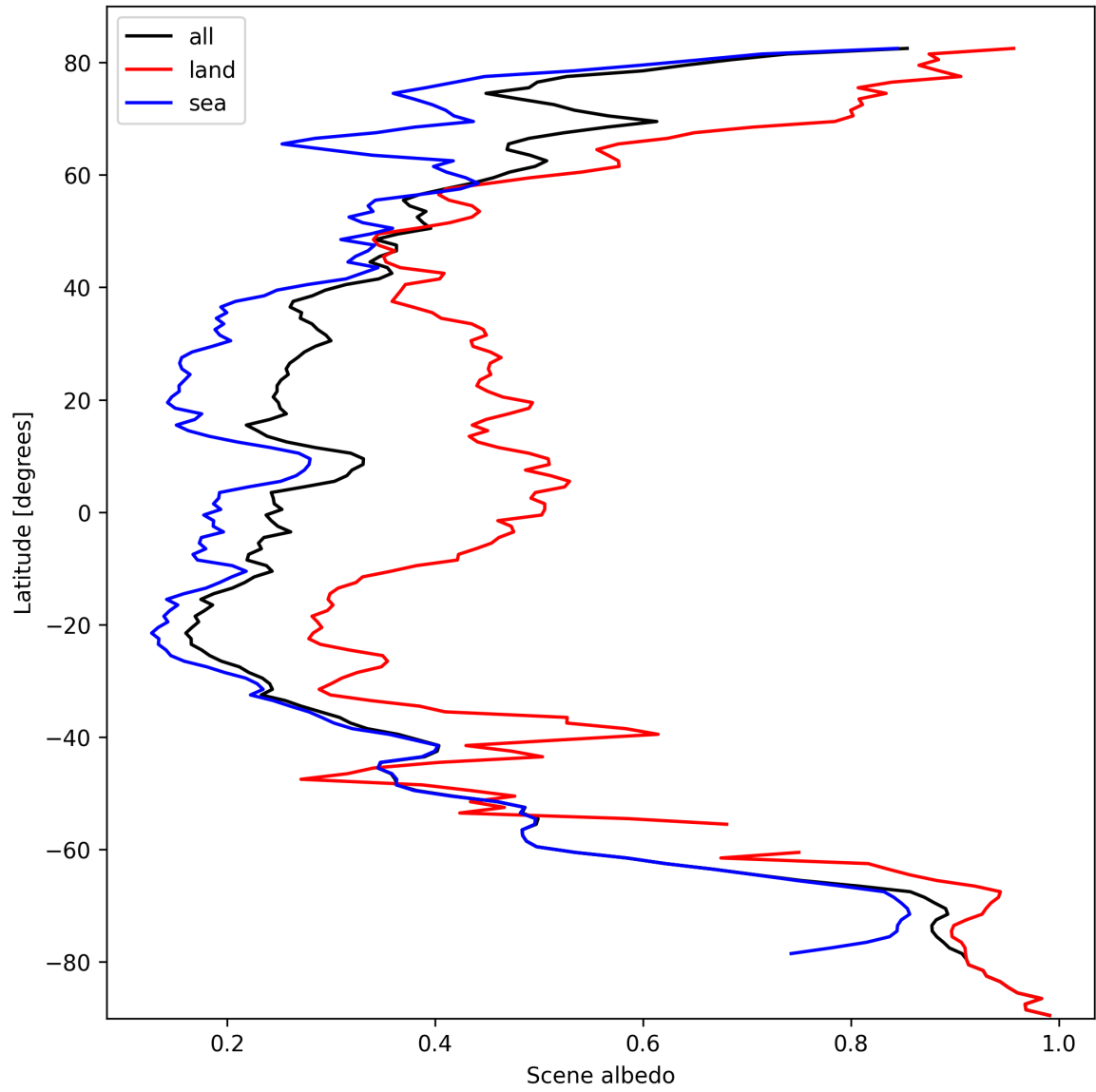
Figure 17: Zonal average of “Scene albedo” for 2024-10-05 to 2024-10-07.
