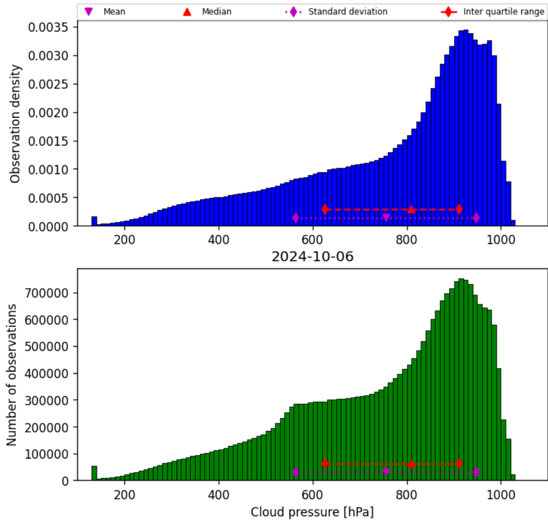
Figure 30: Histogram of “Cloud pressure” for 2024-10-05 to 2024-10-07
