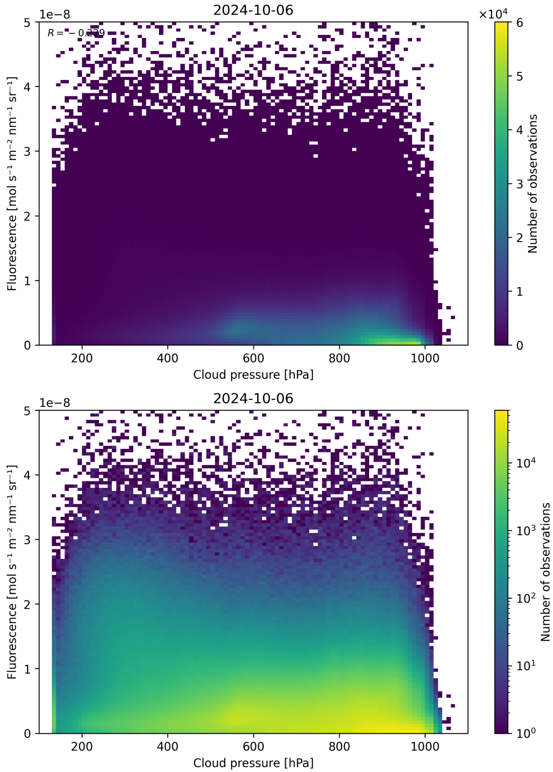
Figure 88: Scatter density plot of “Cloud pressure” against “Fluorescence” for 2024-10-05 to 2024-10-07.
