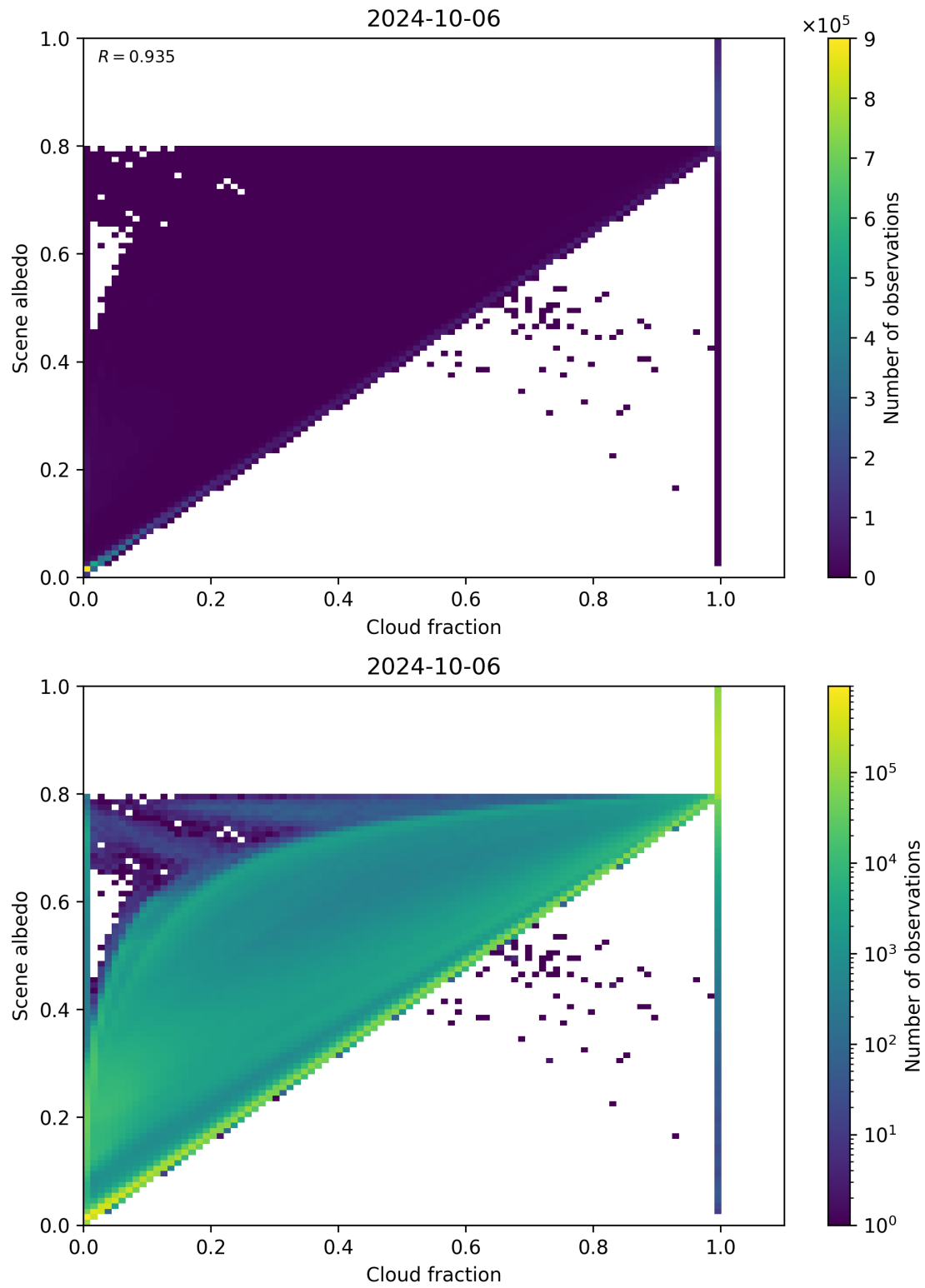
Figure 82: Scatter density plot of “Cloud fraction” against “Scene albedo” for 2024-10-05 to 2024-10-07.
