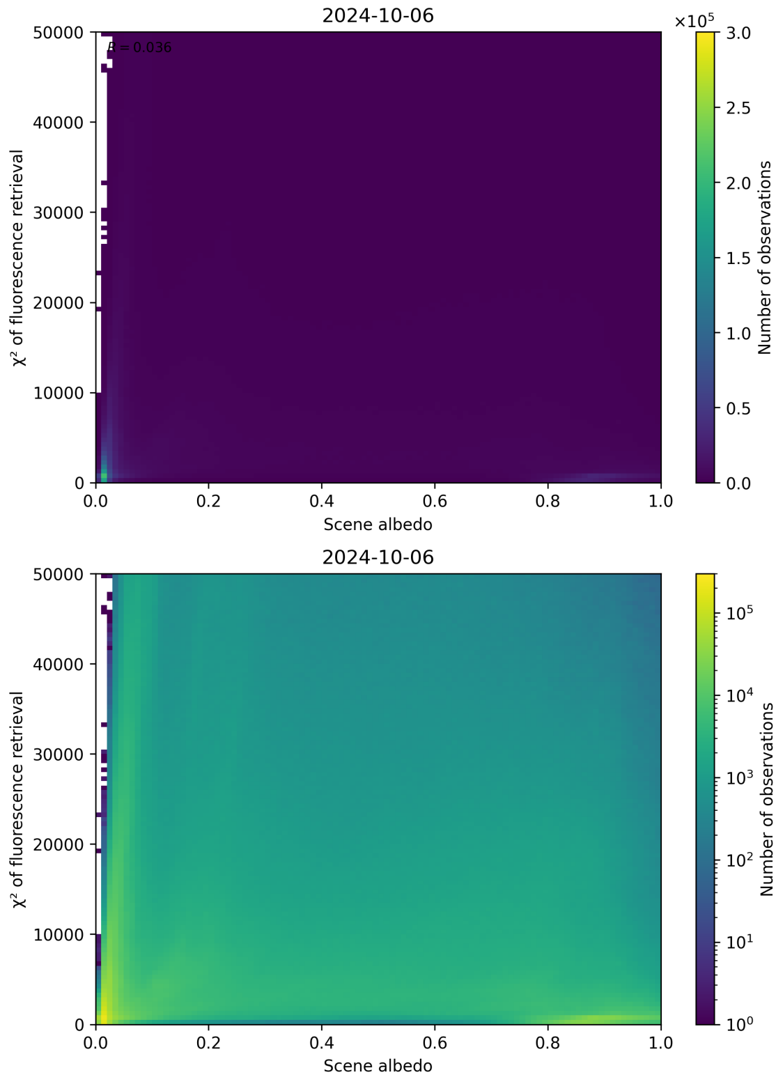
Figure 113: Scatter density plot of “Scene albedo” against “ \chi^2 of fluorescence retrieval” for 2024-10-05 to 2024-10-07.
