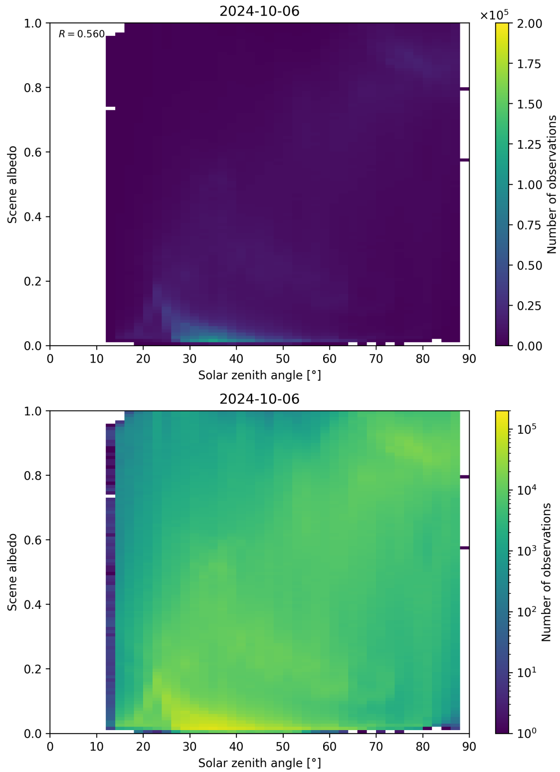
Figure 127: Scatter density plot of “Solar zenith angle” against “Scene albedo” for 2024-10-05 to 2024-10-07.
