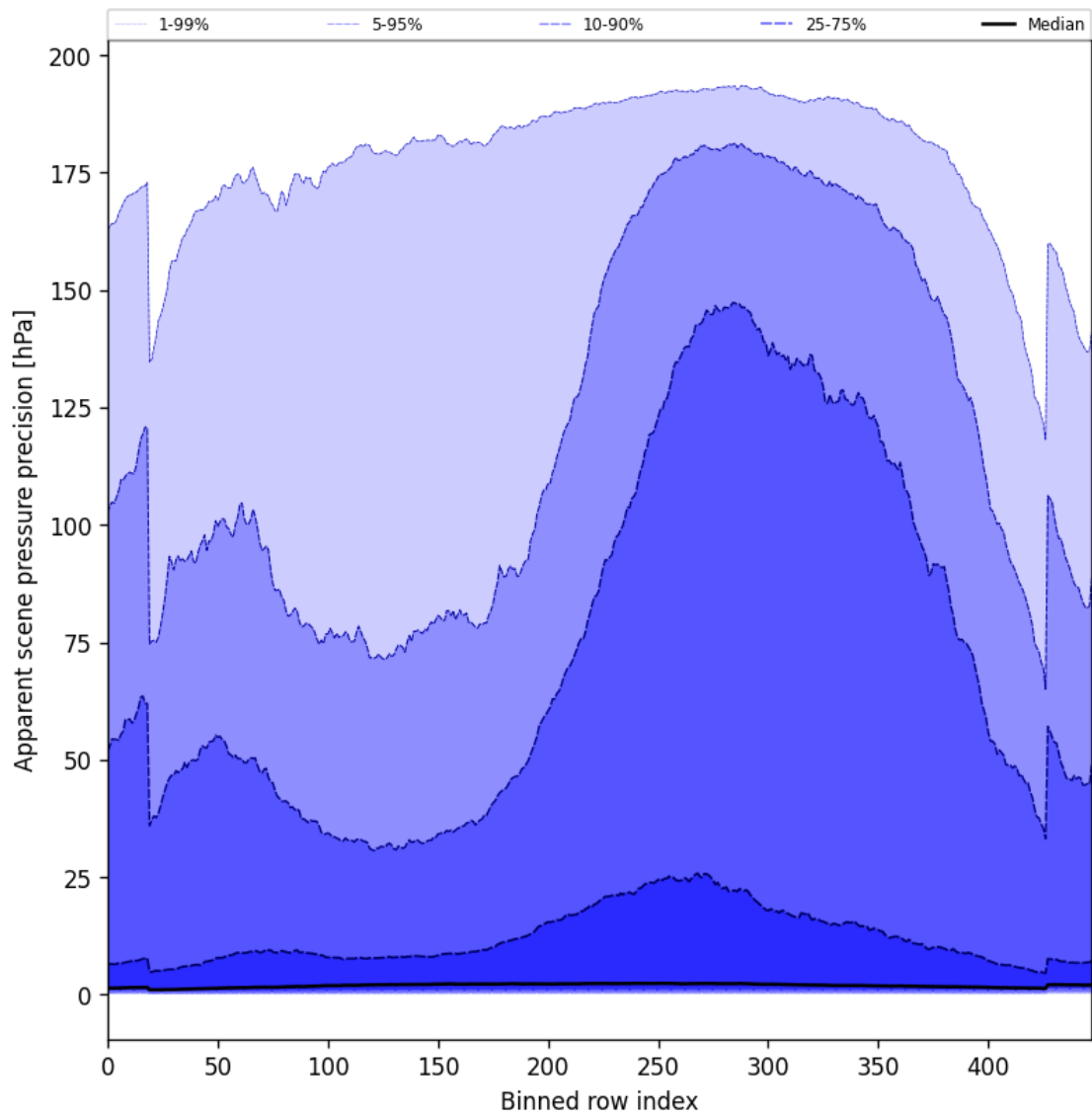
Figure 54: Along track statistics of “Apparent scene pressure precision” for 2024-10-05 to 2024-10-07
