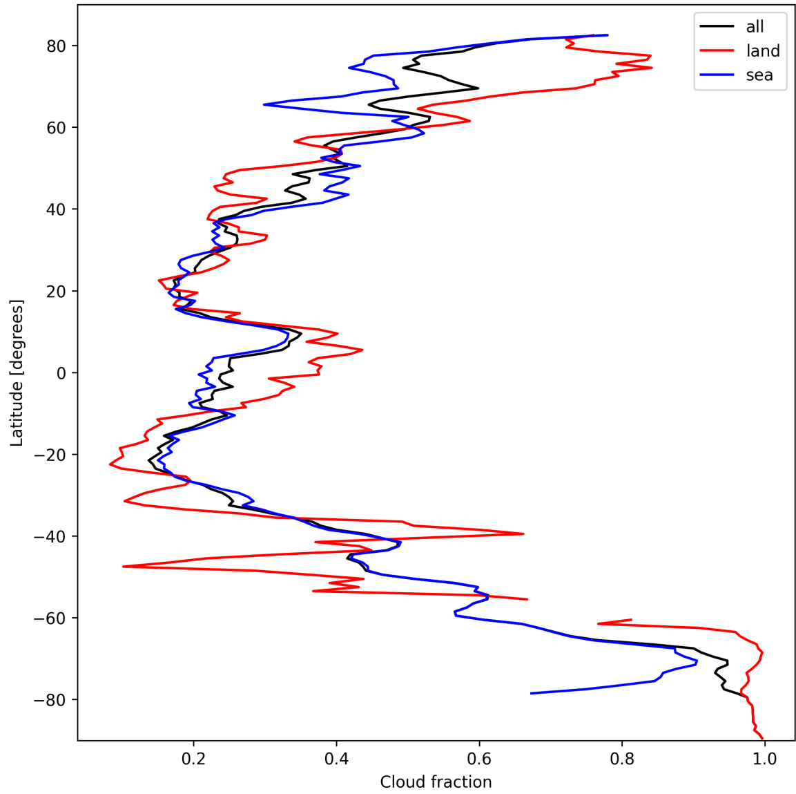
Figure 15: Zonal average of “Cloud fraction” for 2024-10-05 to 2024-10-07.
