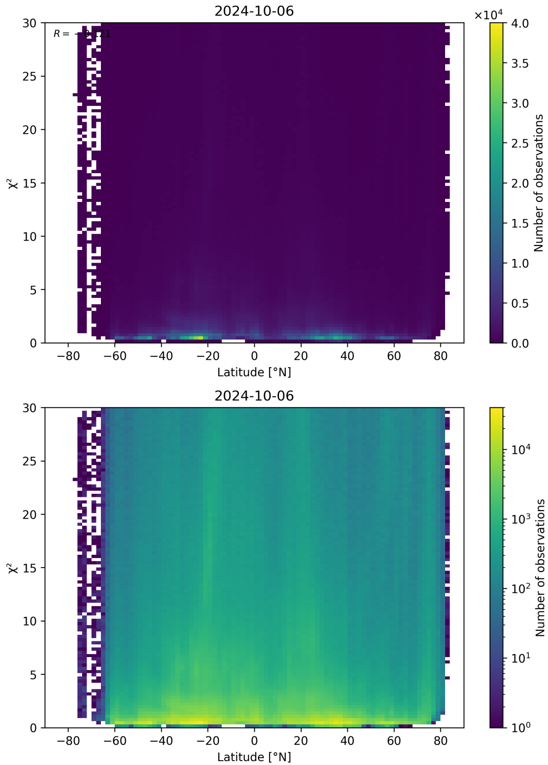
Figure 97: Scatter density plot of “Latitude” against “ \chi^2 ” for 2024-10-05 to 2024-10-07.
