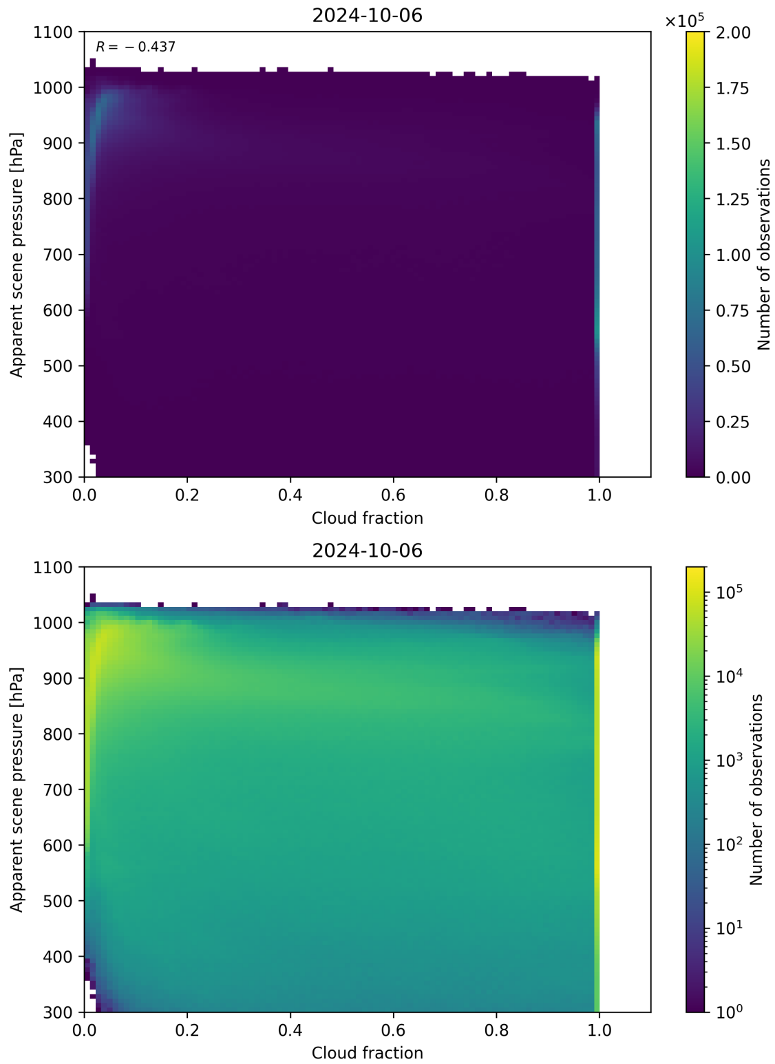
Figure 76: Scatter density plot of “Cloud fraction” against “Apparent scene pressure” for 2024-10-05 to 2024-10-07.
