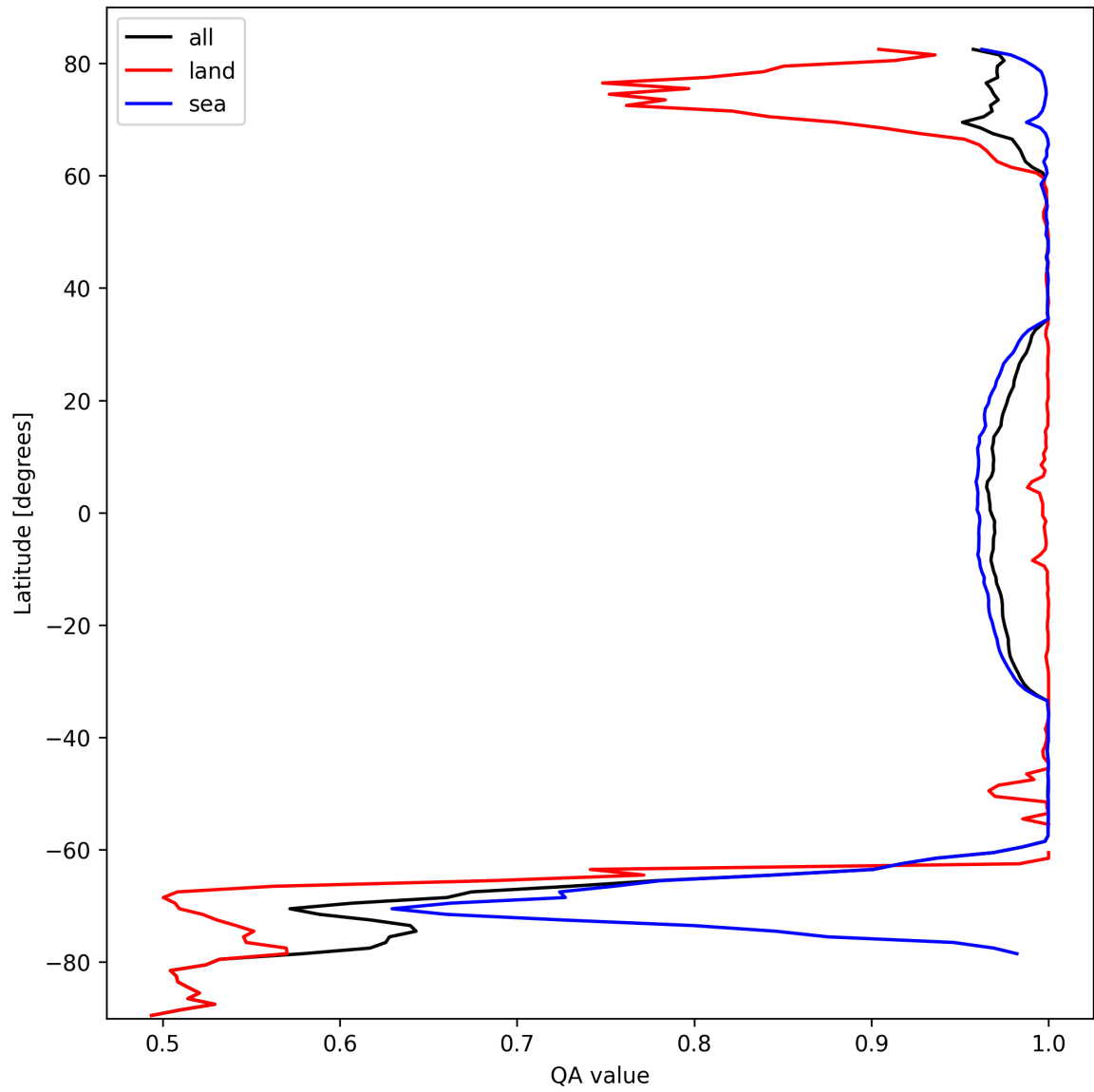
Figure 12: Zonal average of “QA value” for 2024-10-05 to 2024-10-07.
