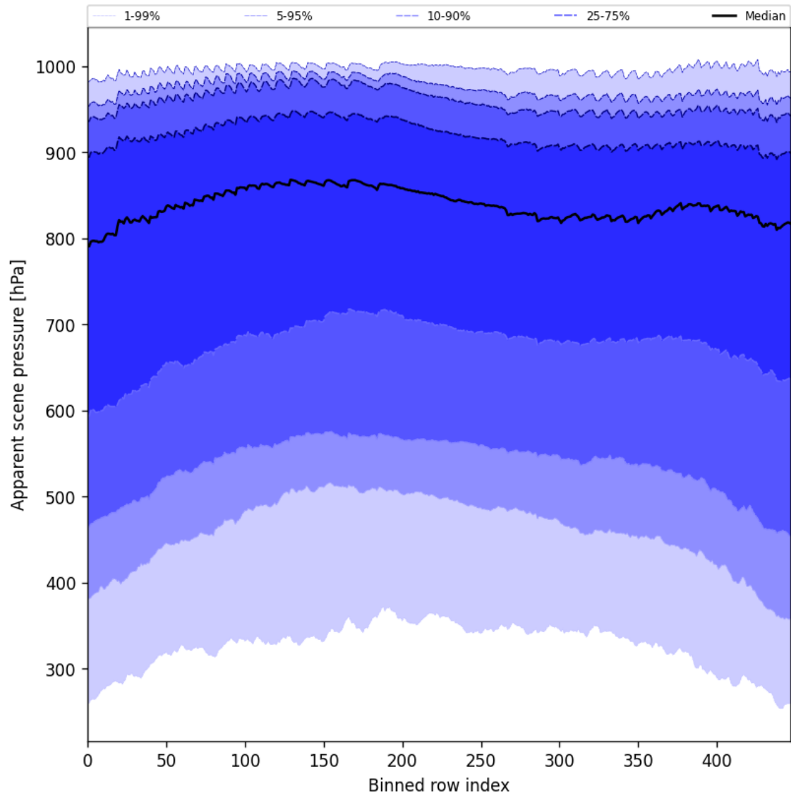
Figure 53: Along track statistics of “Apparent scene pressure” for 2024-10-05 to 2024-10-07
