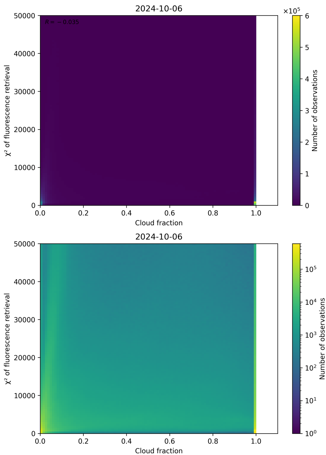
Figure 78: Scatter density plot of “Cloud fraction” against “ \chi^2 of fluorescence retrieval” for 2024-10-05 to 2024-10-07.
