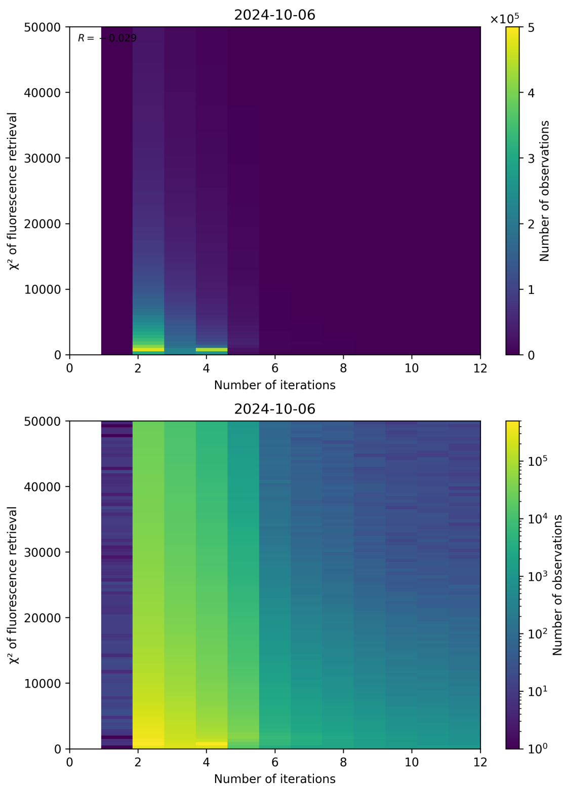
Figure 106: Scatter density plot of “Number of iterations” against “ \chi^2 of fluorescence retrieval” for 2024-10-05 to 2024-10-07.
