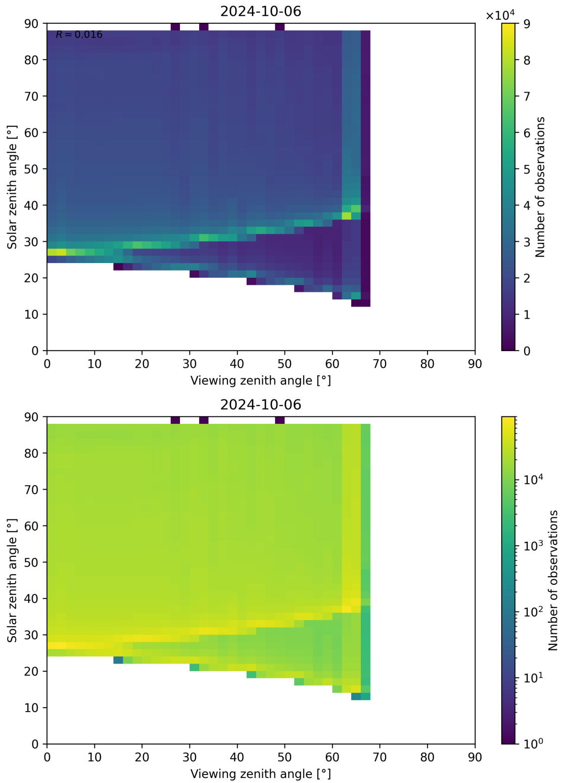
Figure 139: Scatter density plot of “Viewing zenith angle” against “Solar zenith angle” for 2024-10-05 to 2024-10-07.
