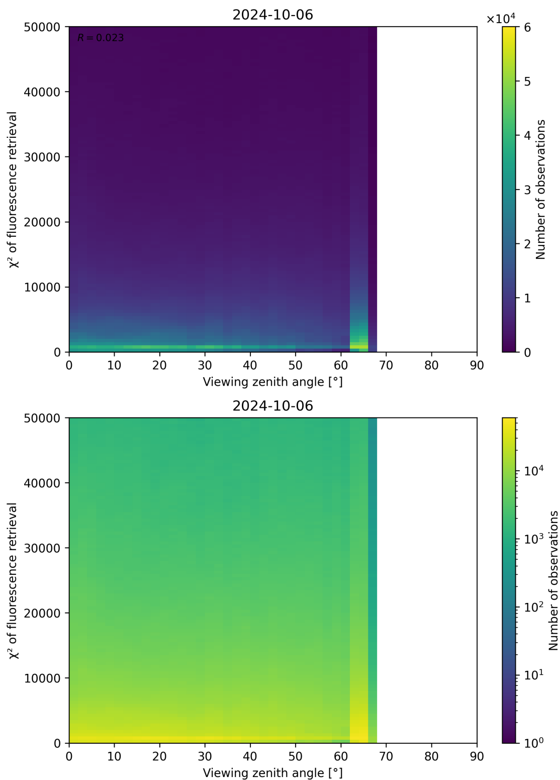
Figure 131: Scatter density plot of “Viewing zenith angle” against “ \chi^2 of fluorescence retrieval” for 2024-10-05 to 2024-10-07.
