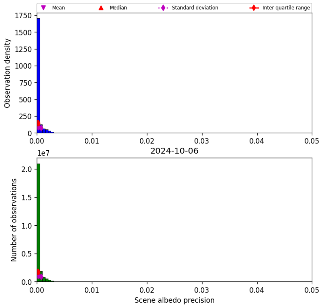
Figure 35: Histogram of “Scene albedo precision” for 2024-10-05 to 2024-10-07
