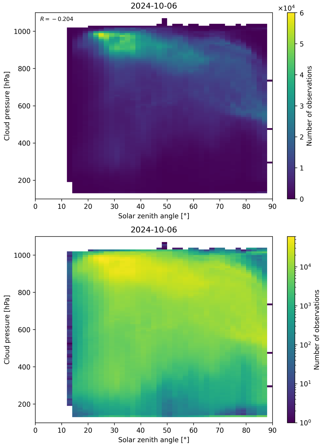
Figure 122: Scatter density plot of “Solar zenith angle” against “Cloud pressure” for 2024-10-05 to 2024-10-07.
