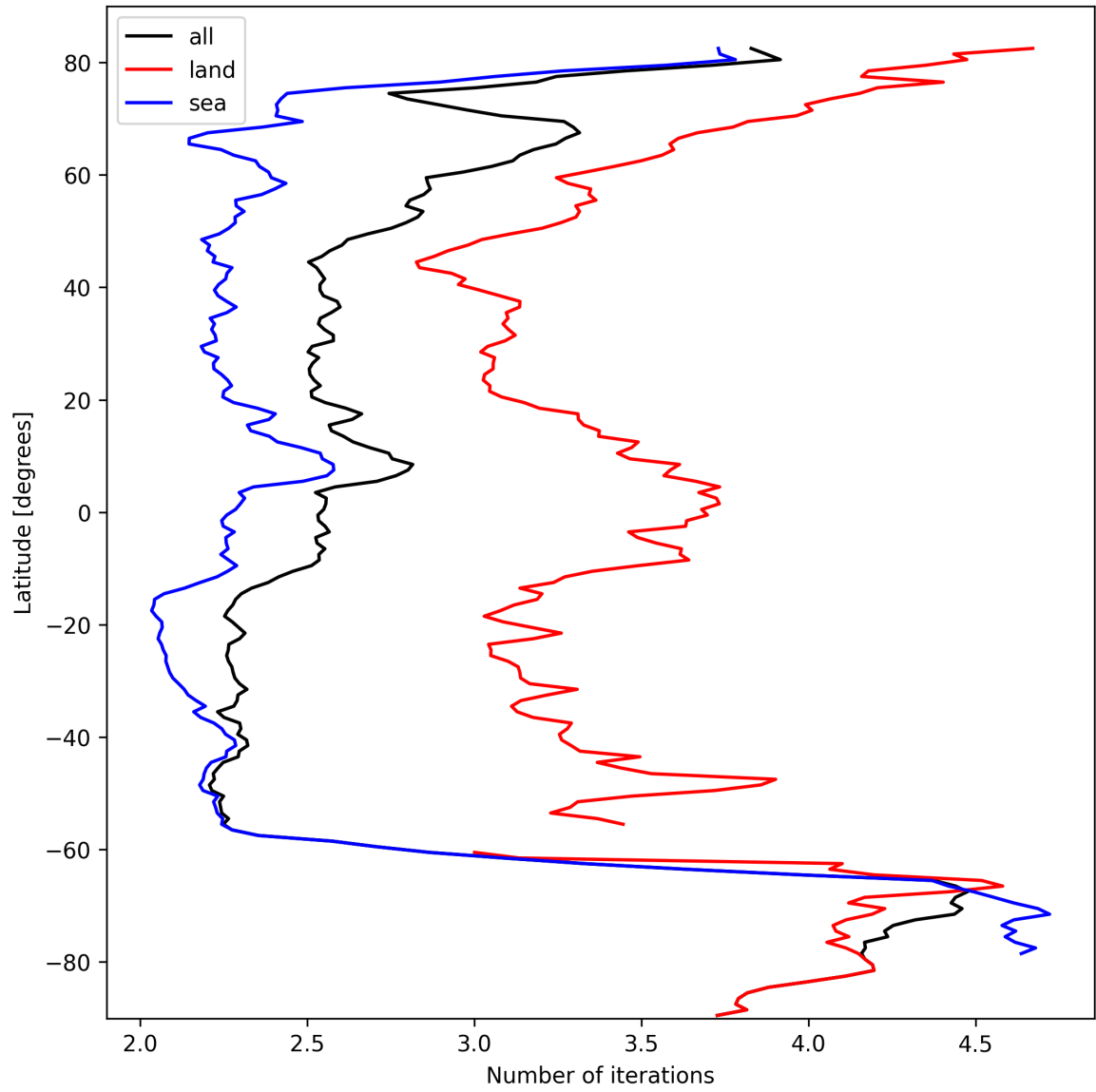
Figure 22: Zonal average of “Number of iterations” for 2024-10-05 to 2024-10-07.
