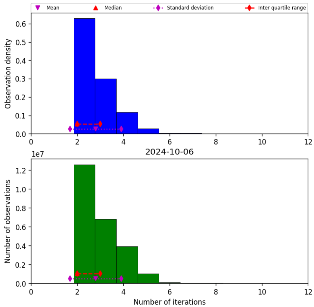
Figure 39: Histogram of “Number of iterations” for 2024-10-05 to 2024-10-07
