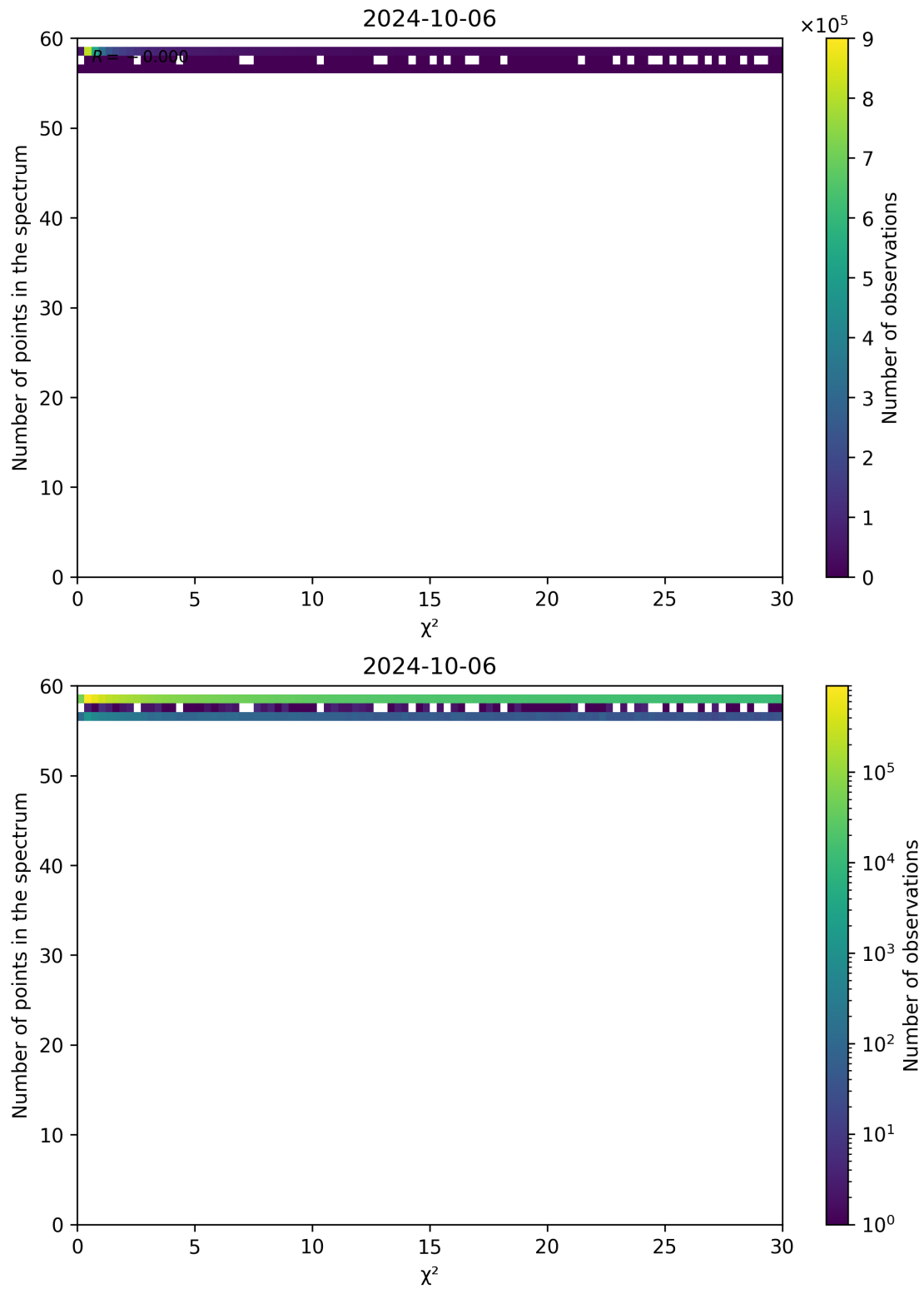
Figure 74: Scatter density plot of " \chi^2 " against "Number of points in the spectrum" for 2024-10-05 to 2024-10-07.
