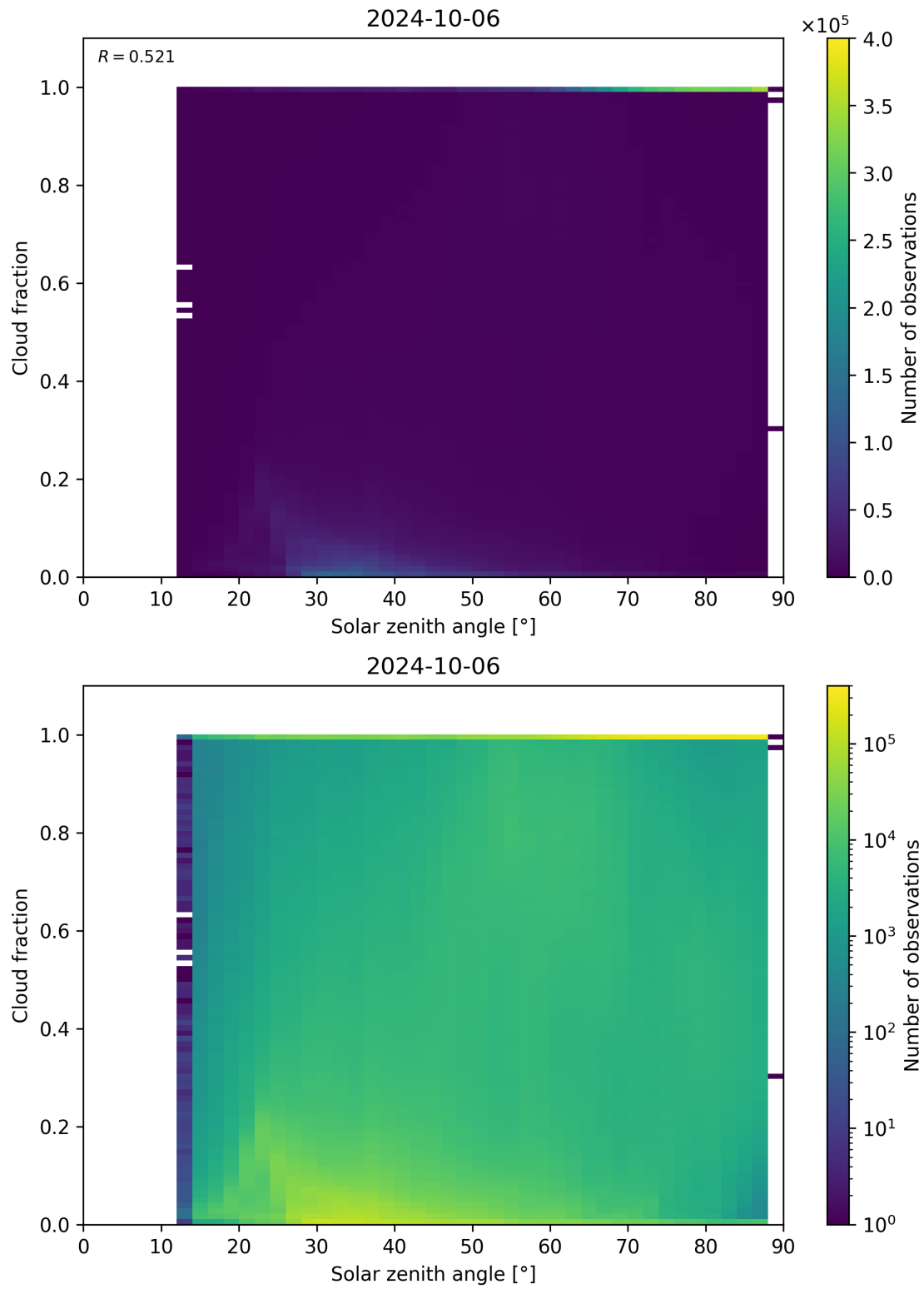
Figure 121: Scatter density plot of “Solar zenith angle” against “Cloud fraction” for 2024-10-05 to 2024-10-07.
