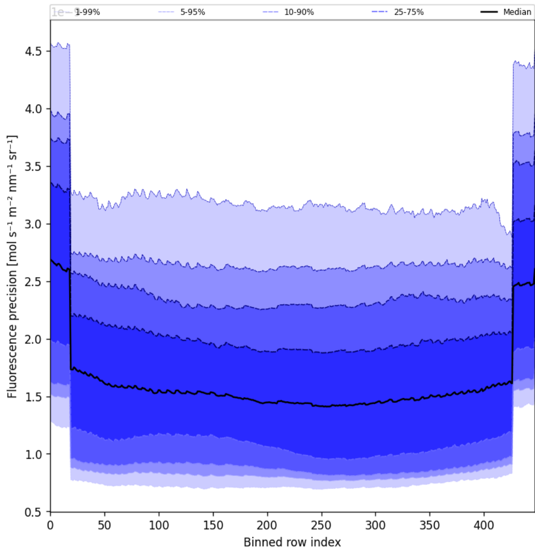
Figure 58: Along track statistics of “Fluorescence precision” for 2024-10-05 to 2024-10-07
