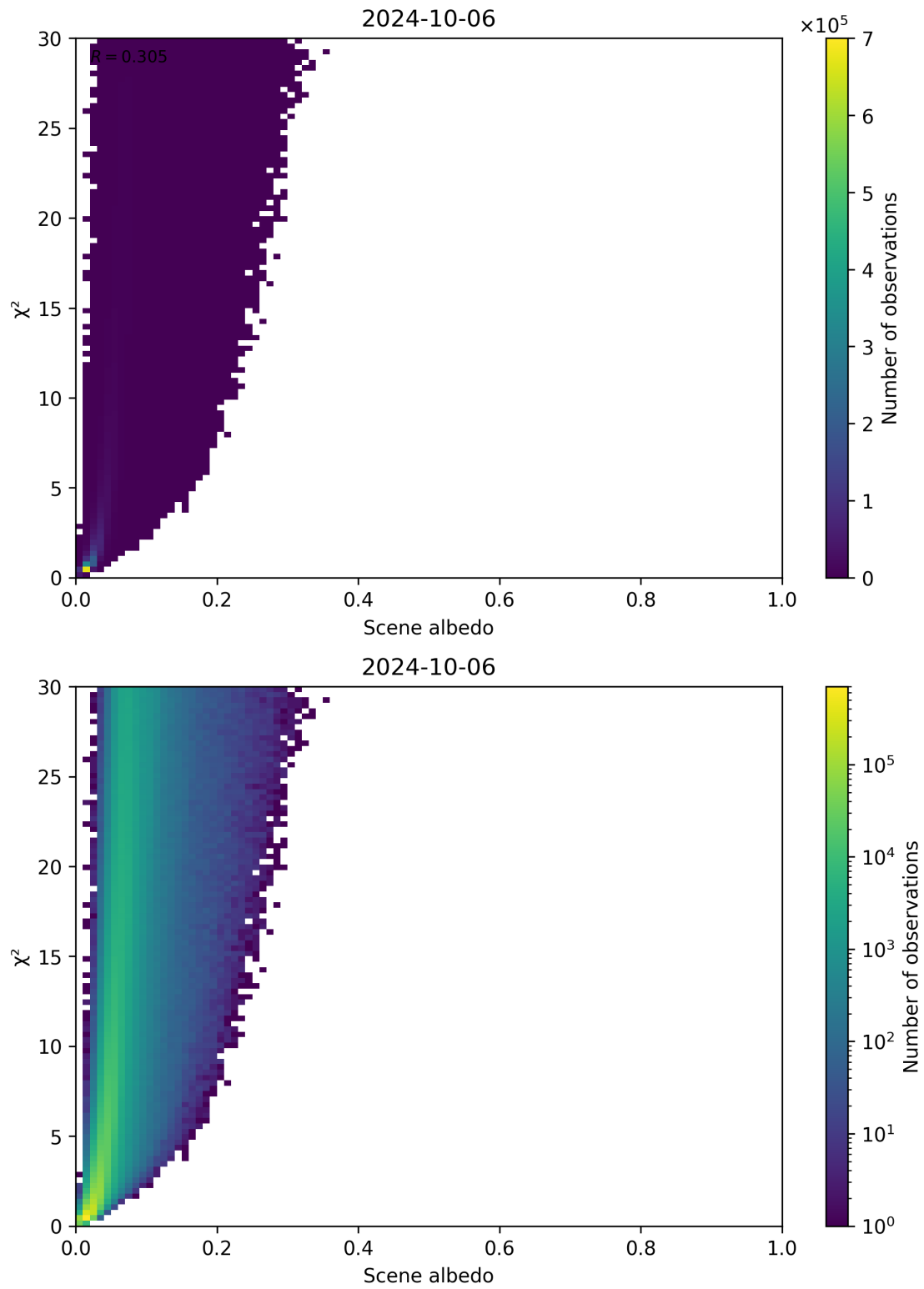
Figure 112: Scatter density plot of “Scene albedo” against “ \chi^2 ” for 2024-10-05 to 2024-10-07.
