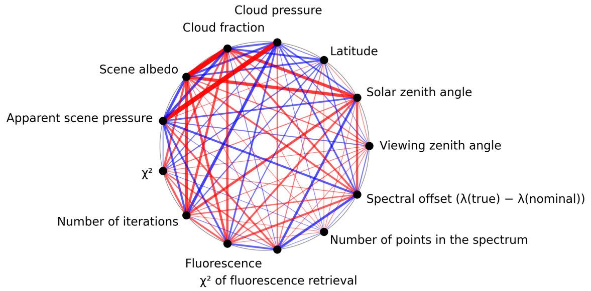
Figure 1: Map of correlation graph for 2024-10-05 to 2024-10-07.
