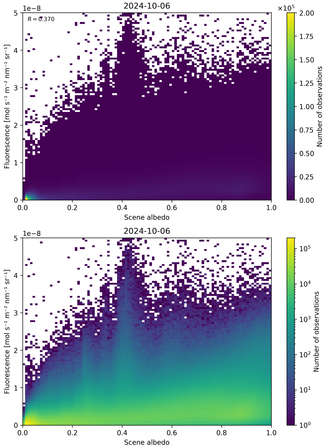
Figure 114: Scatter density plot of “Scene albedo” against “Fluorescence” for 2024-10-05 to 2024-10-07.
