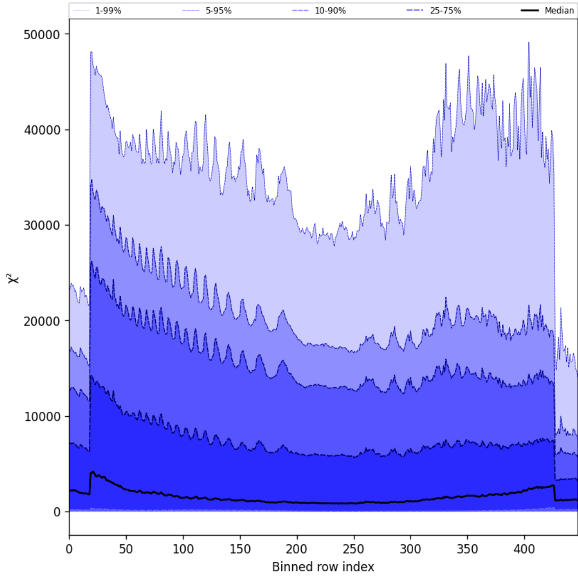
Figure 55: Along track statistics of “ \chi^2 ” for 2024-10-05 to 2024-10-07
