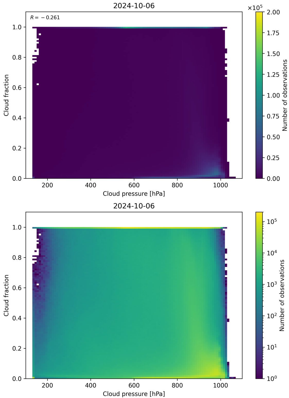
Figure 87: Scatter density plot of “Cloud pressure” against “Cloud fraction” for 2024-10-05 to 2024-10-07.
