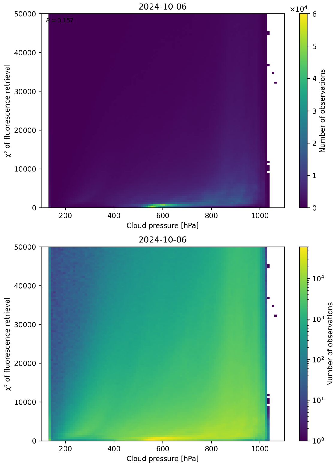
Figure 86: Scatter density plot of “Cloud pressure” against “ \chi^2 of fluorescence retrieval” for 2024-10-05 to 2024-10-07.
