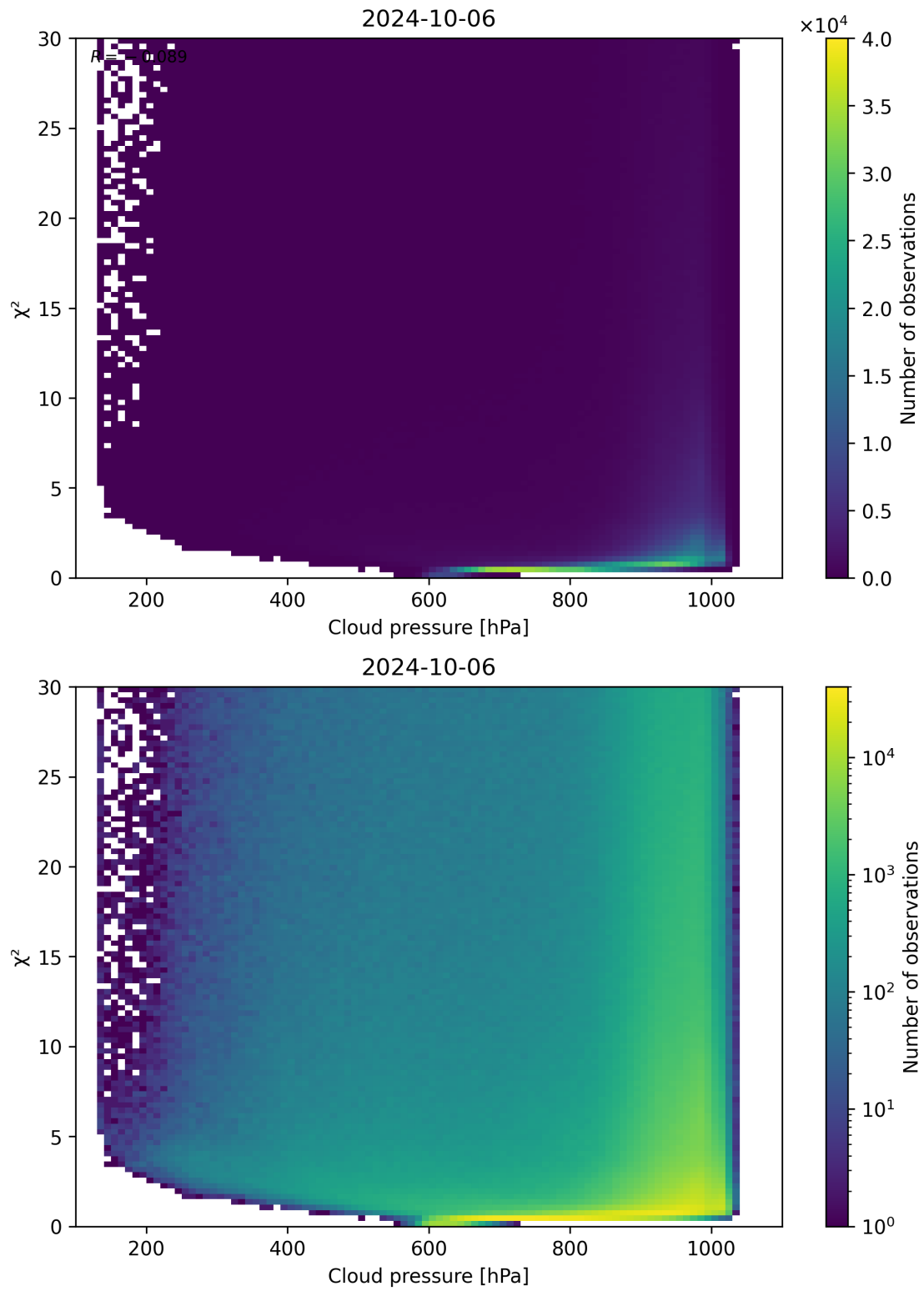
Figure 85: Scatter density plot of “Cloud pressure” against “ \chi^2 ” for 2024-10-05 to 2024-10-07.
