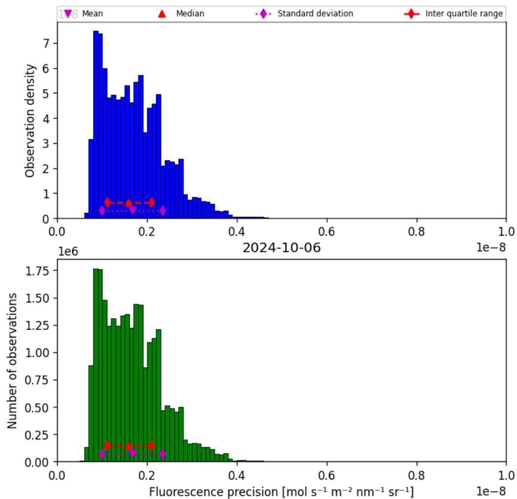
Figure 41: Histogram of “Fluorescence precision” for 2024-10-05 to 2024-10-07
