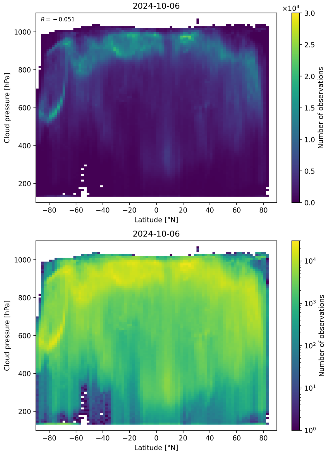
Figure 100: Scatter density plot of “Latitude” against “Cloud pressure” for 2024-10-05 to 2024-10-07.
