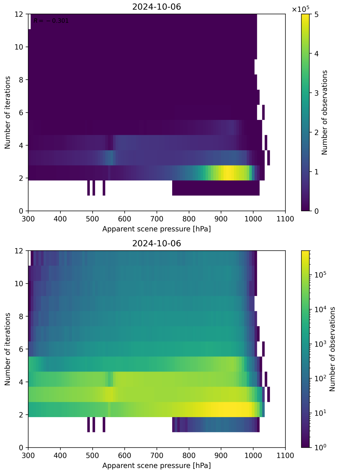
Figure 66: Scatter density plot of “Apparent scene pressure” against “Number of iterations” for 2024-10-05 to 2024-10-07.
