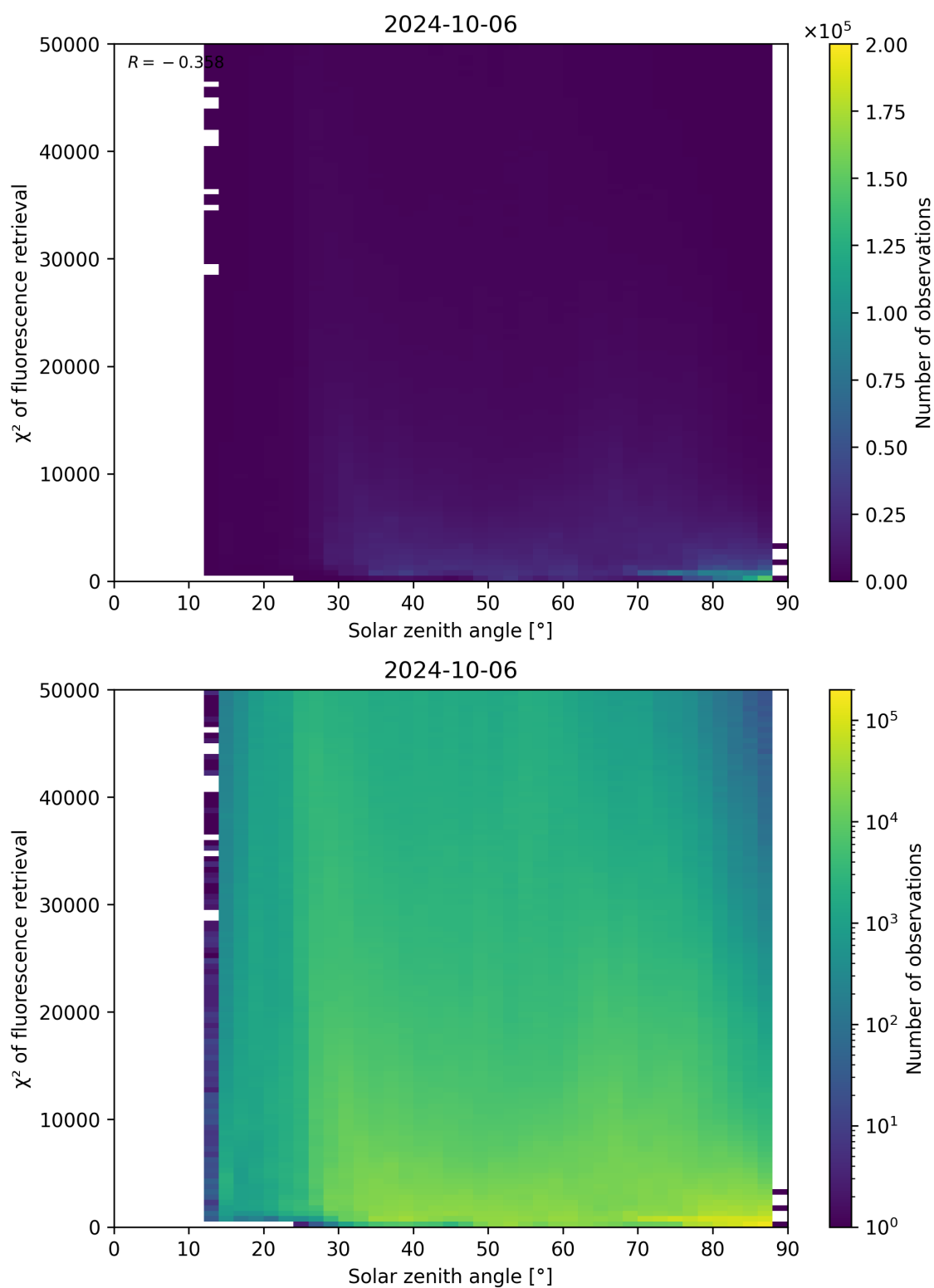
Figure 120: Scatter density plot of “Solar zenith angle” against “ \chi^2 of fluorescence retrieval” for 2024-10-05 to 2024-10-07.
