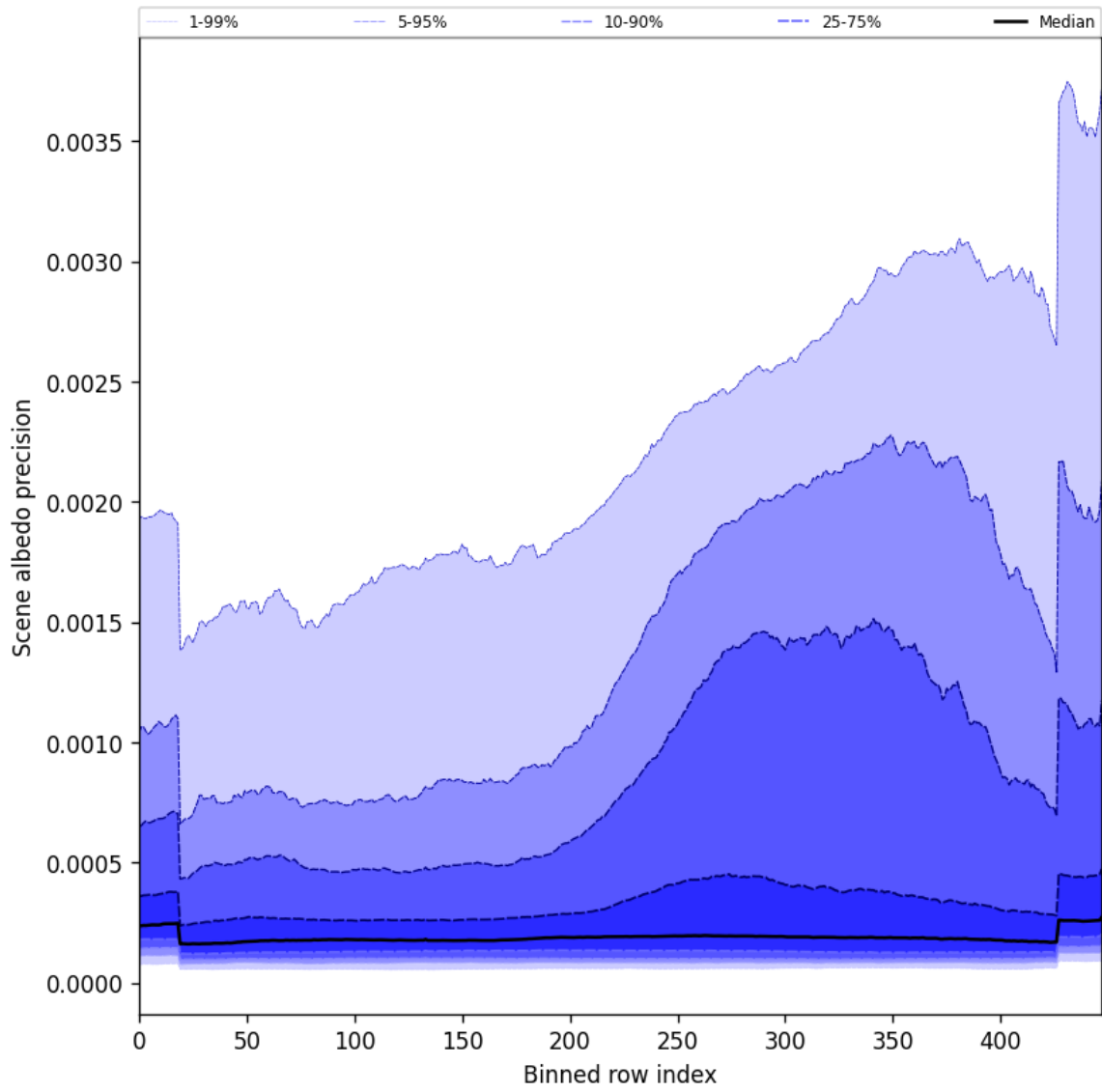
Figure 52: Along track statistics of “Scene albedo precision” for 2024-10-05 to 2024-10-07
