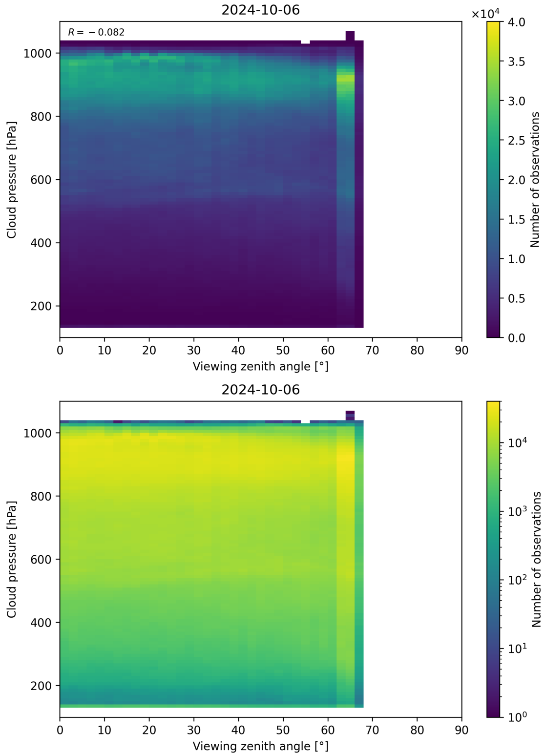
Figure 133: Scatter density plot of “Viewing zenith angle” against “Cloud pressure” for 2024-10-05 to 2024-10-07.
