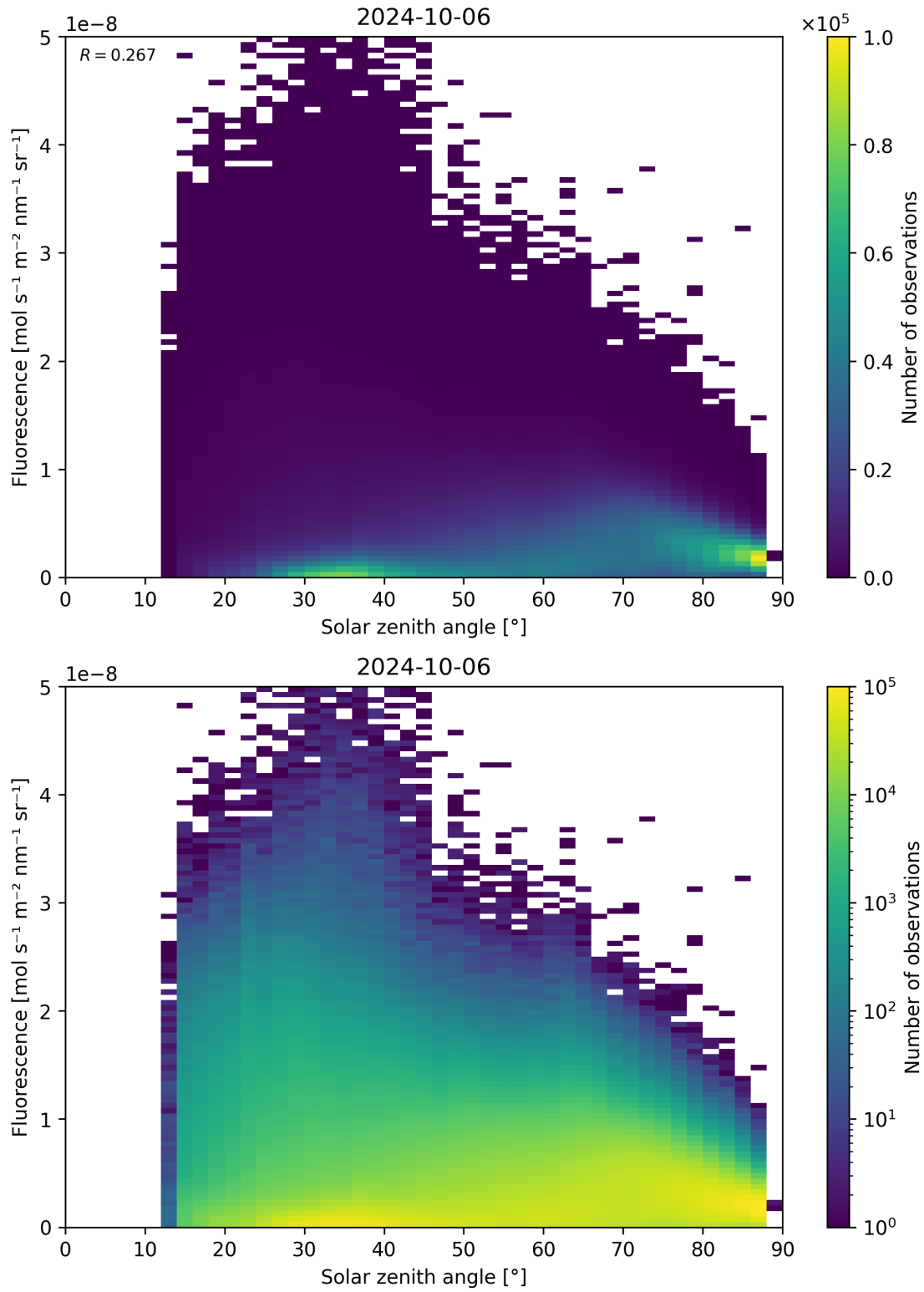
Figure 123: Scatter density plot of “Solar zenith angle” against “Fluorescence” for 2024-10-05 to 2024-10-07.
