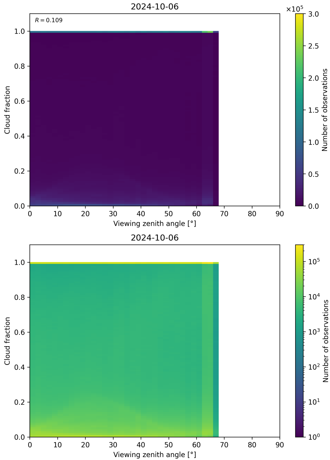
Figure 132: Scatter density plot of “Viewing zenith angle” against “Cloud fraction” for 2024-10-05 to 2024-10-07.
