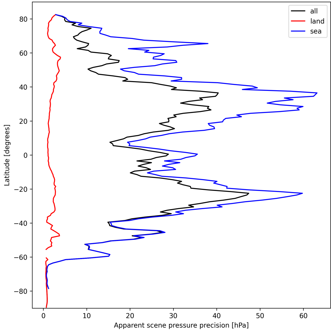
Figure 20: Zonal average of “Apparent scene pressure precision” for 2024-10-05 to 2024-10-07.
