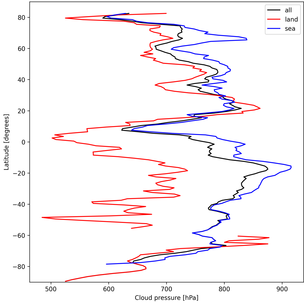
Figure 13: Zonal average of “Cloud pressure” for 2024-10-05 to 2024-10-07.
