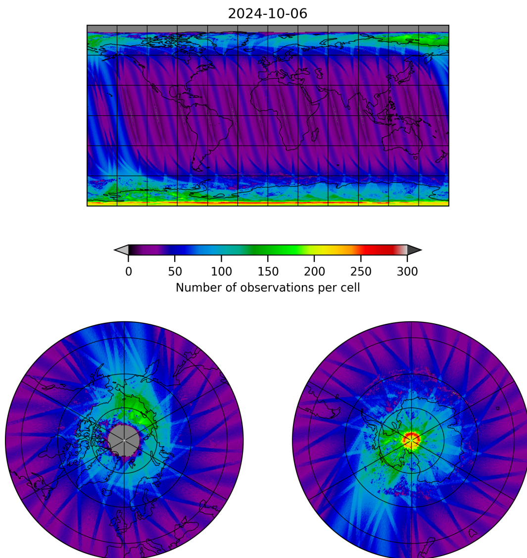
Figure 11: Map of the number of observations for 2024-10-05 to 2024-10-07
