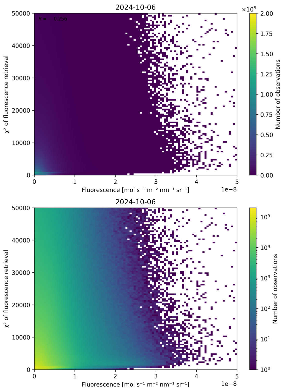
Figure 93: Scatter density plot of “Fluorescence” against “ \chi^2 of fluorescence retrieval” for 2024-10-05 to 2024-10-07.
