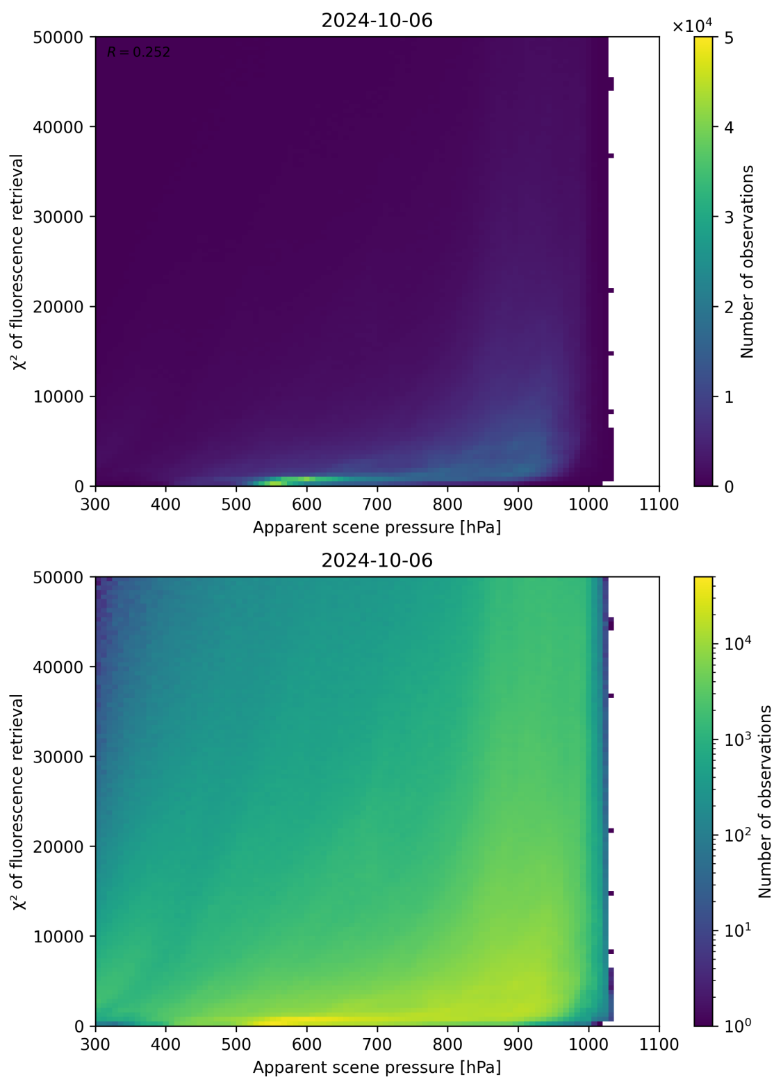
Figure 64: Scatter density plot of “Apparent scene pressure” against “ \chi^2 of fluorescence retrieval” for 2024-10-05 to 2024-10-07.
