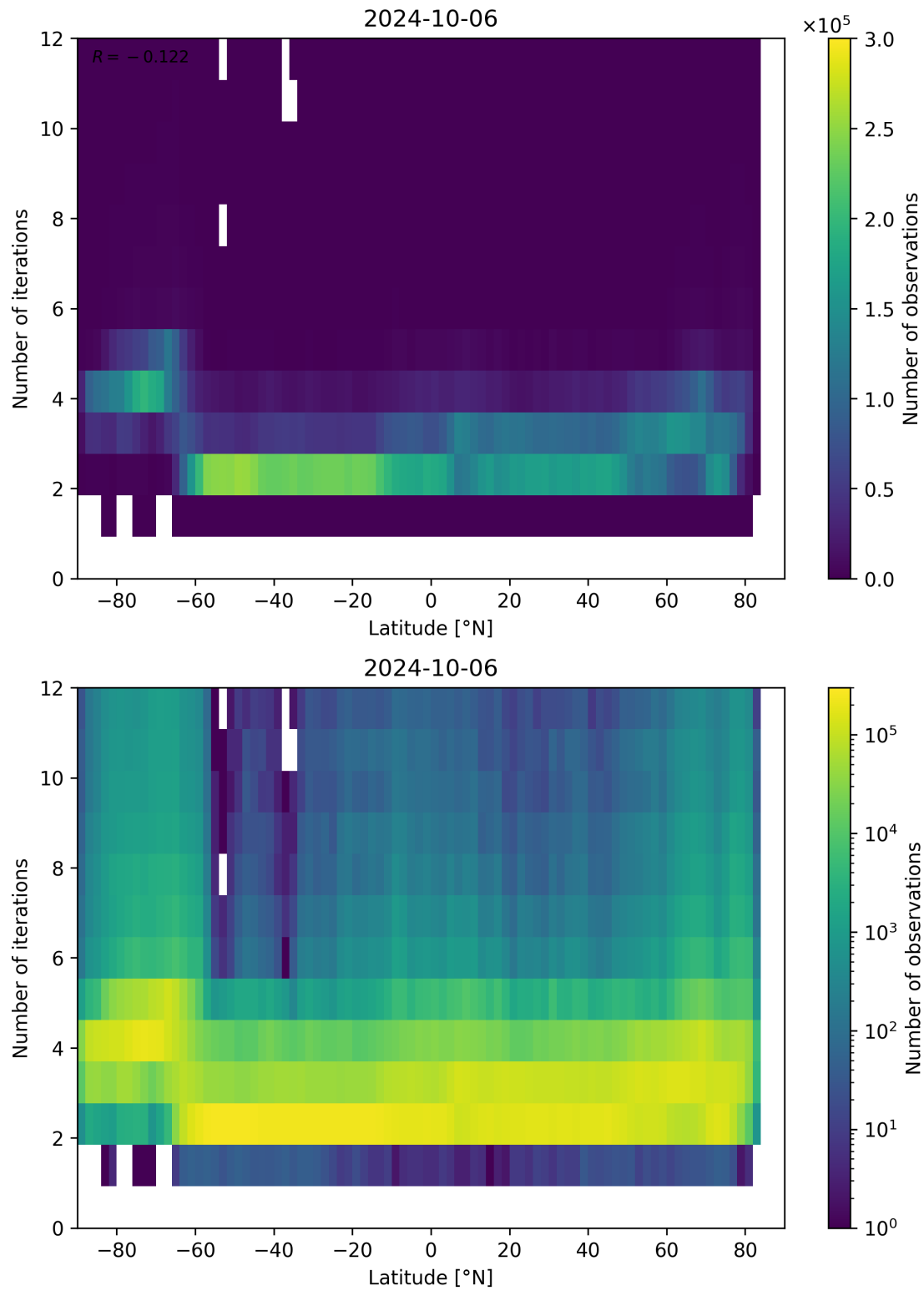
Figure 102: Scatter density plot of “Latitude” against “Number of iterations” for 2024-10-05 to 2024-10-07.
