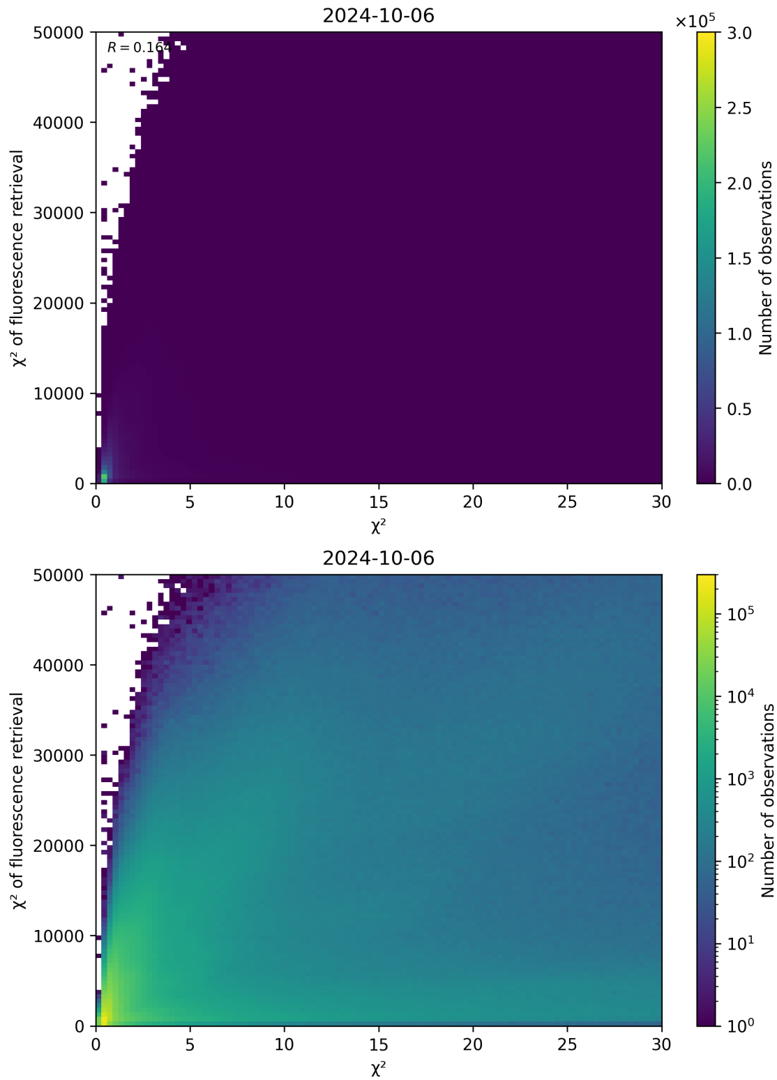
Figure 69: Scatter density plot of “ \chi^2 ” against “ \chi^2 of fluorescence retrieval” for 2024-10-05 to 2024-10-07.
