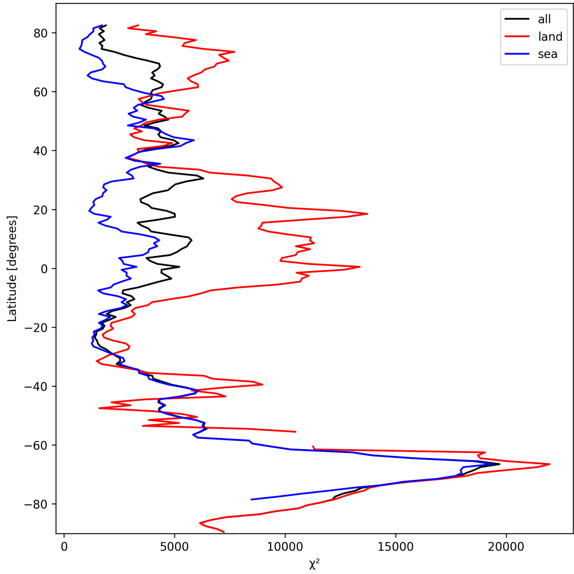
Figure 21: Zonal average of “ \chi^2 ” for 2024-10-05 to 2024-10-07.
