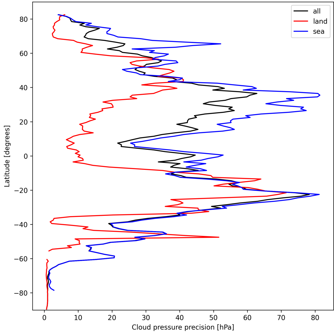
Figure 14: Zonal average of “Cloud pressure precision” for 2024-10-05 to 2024-10-07.
