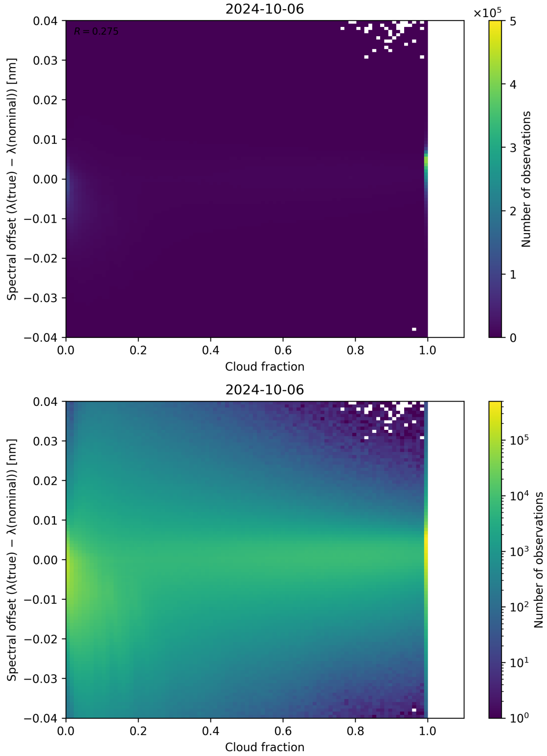
Figure 83: Scatter density plot of “Cloud fraction” against “Spectral offset ( \lambda_{\text{true}} - \lambda_{\text{nominal}} )” for 2024-10-05 to 2024-10-07.
