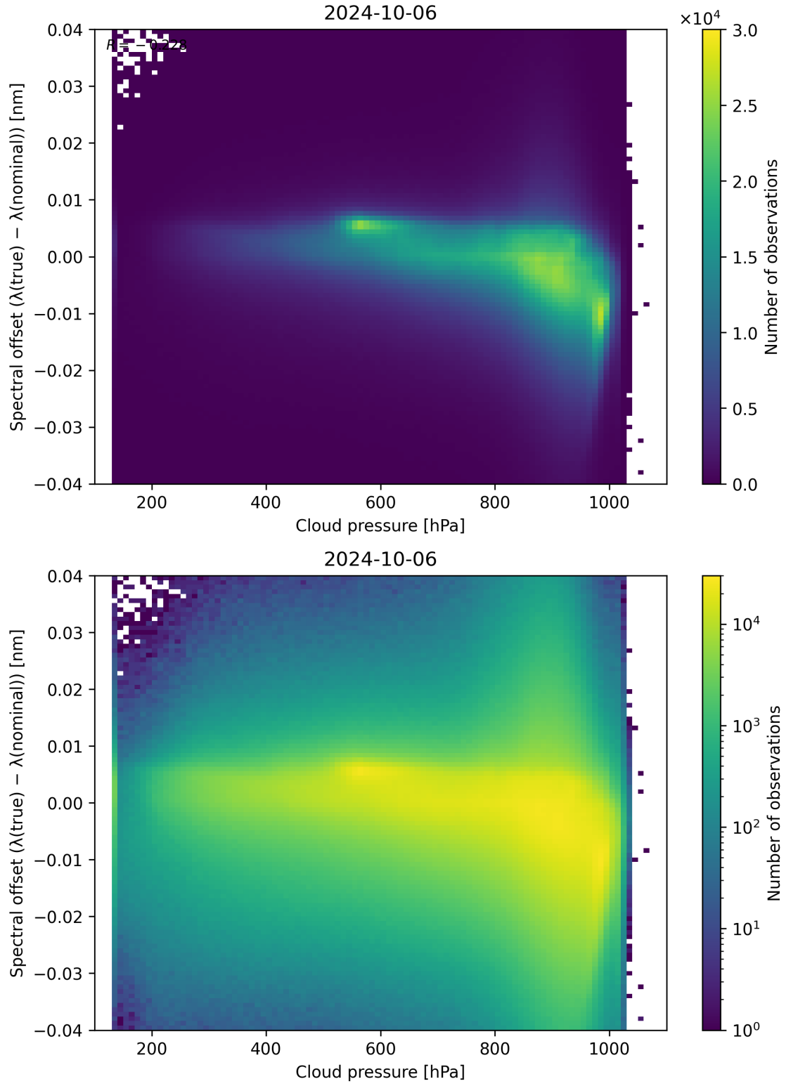
Figure 92: Scatter density plot of “Cloud pressure” against “Spectral offset ( \lambda_{\text{true}} - \lambda_{\text{nominal}} )” for 2024-10-05 to 2024-10-07.
