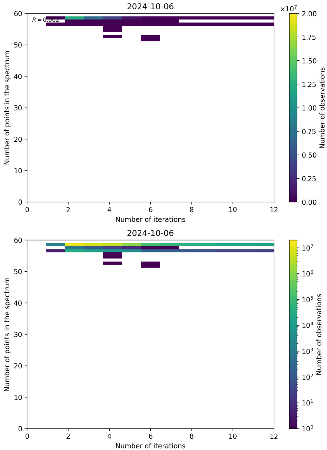
Figure 108: Scatter density plot of “Number of iterations” against “Number of points in the spectrum” for 2024-10-05 to 2024-10-07.
