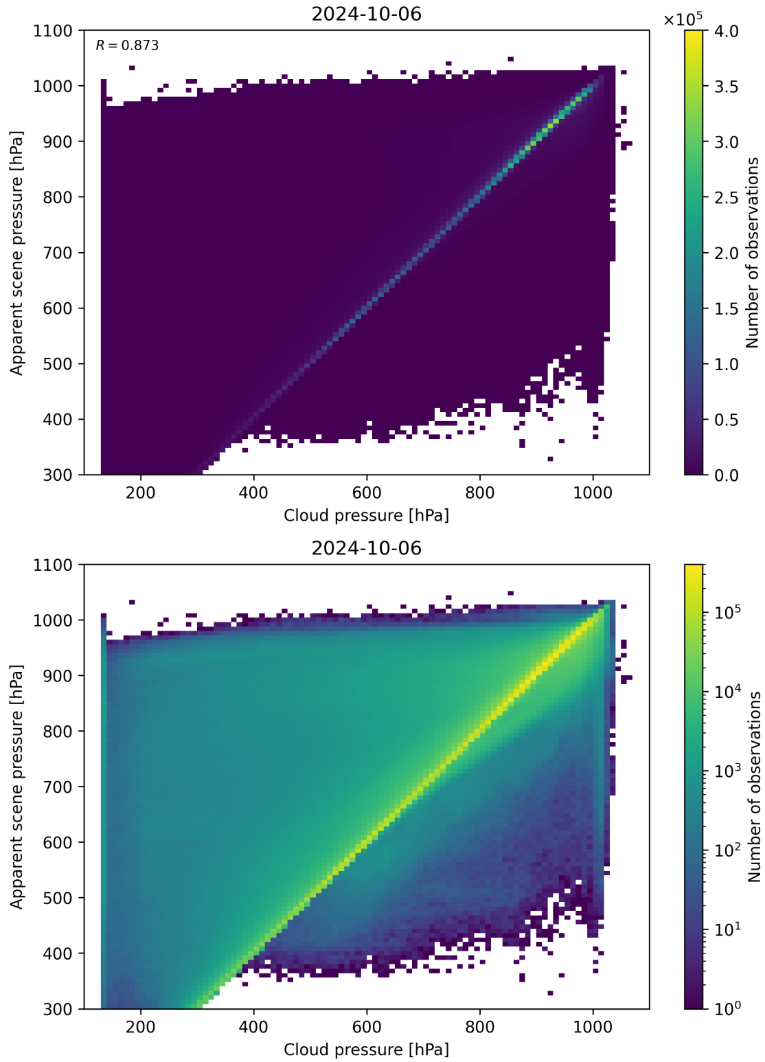
Figure 84: Scatter density plot of “Cloud pressure” against “Apparent scene pressure” for 2024-10-05 to 2024-10-07.
