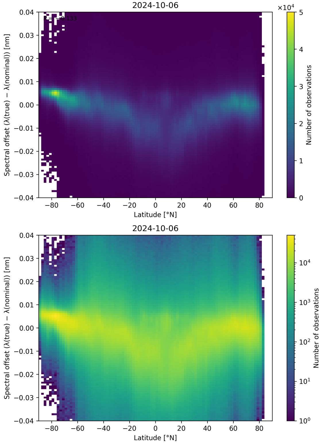
Figure 105: Scatter density plot of “Latitude” against “Spectral offset ( \lambda_{\text{true}} - \lambda_{\text{nominal}} )” for 2024-10-05 to 2024-10-07.
