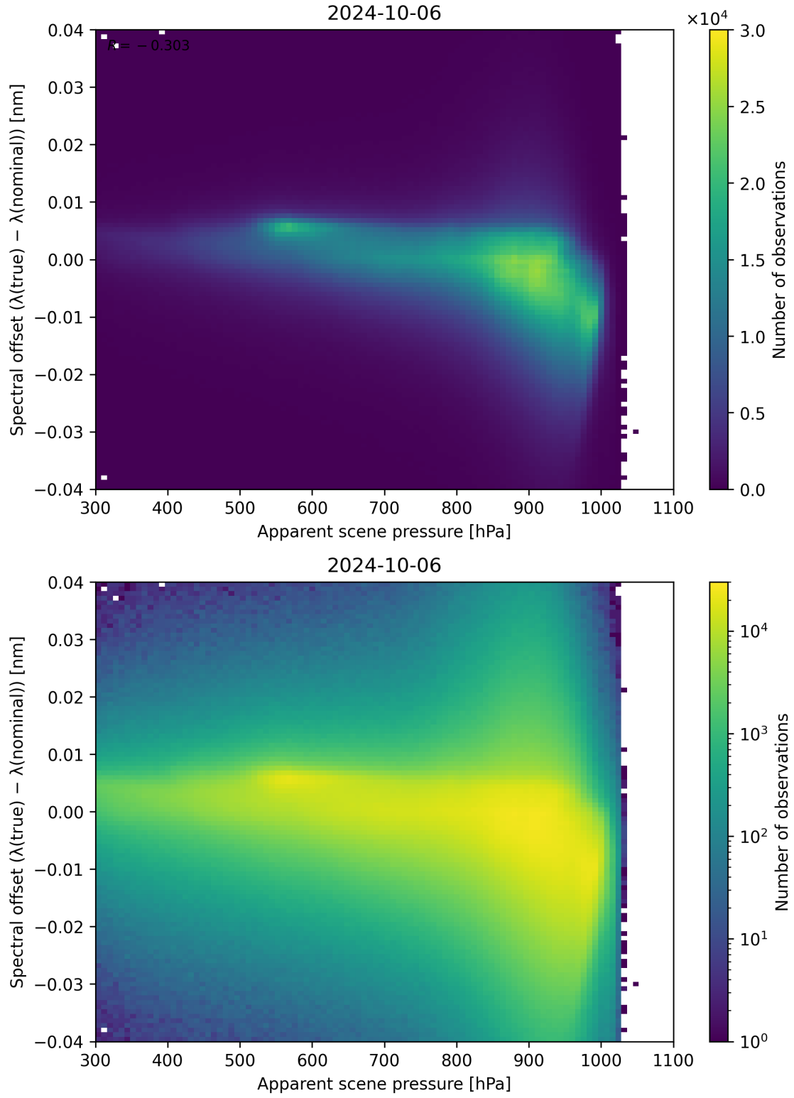
Figure 68: Scatter density plot of “Apparent scene pressure” against “Spectral offset ( \lambda_{\text{true}} - \lambda_{\text{nominal}} )” for 2024-10-05 to 2024-10-07.
