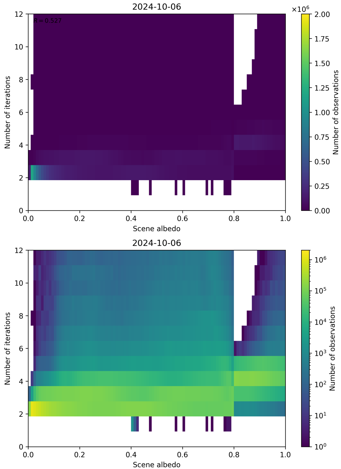
Figure 115: Scatter density plot of “Scene albedo” against “Number of iterations” for 2024-10-05 to 2024-10-07.
