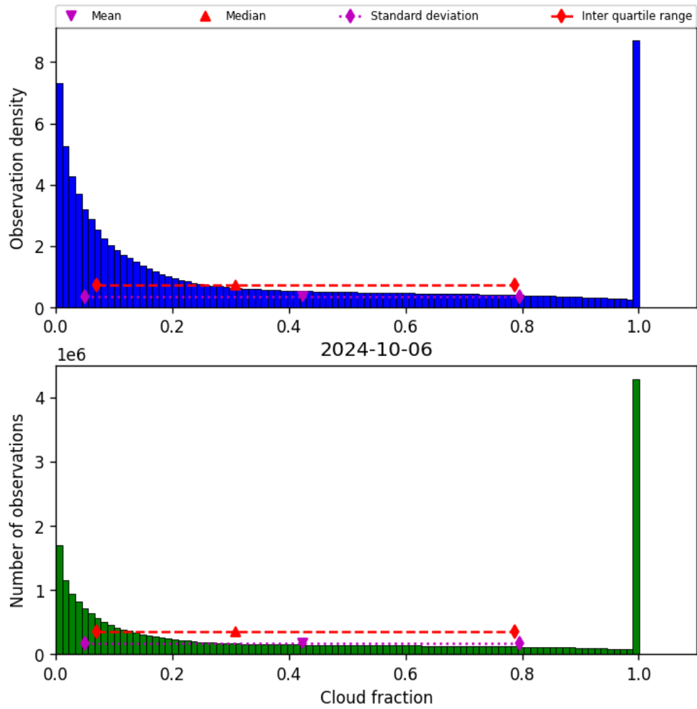
Figure 32: Histogram of “Cloud fraction” for 2024-10-05 to 2024-10-07
