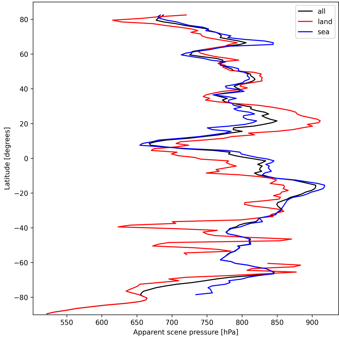
Figure 19: Zonal average of “Apparent scene pressure” for 2024-10-05 to 2024-10-07.
