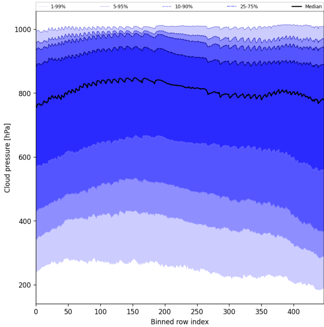
Figure 47: Along track statistics of “Cloud pressure” for 2024-10-05 to 2024-10-07
