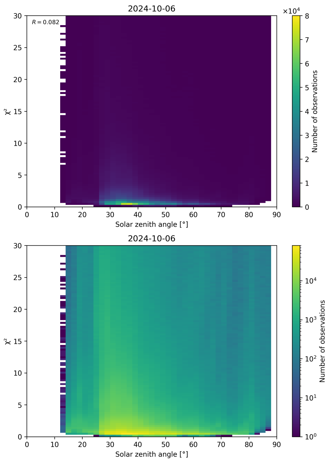
Figure 119: Scatter density plot of “Solar zenith angle” against “ \chi^2 ” for 2024-10-05 to 2024-10-07.
