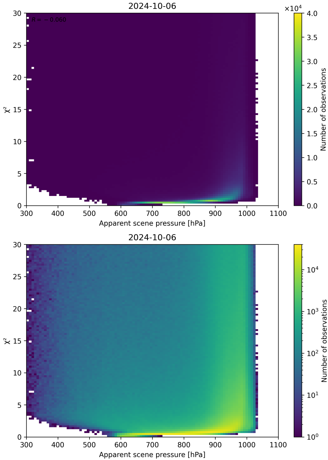
Figure 63: Scatter density plot of “Apparent scene pressure” against “ \chi^2 ” for 2024-10-05 to 2024-10-07.
