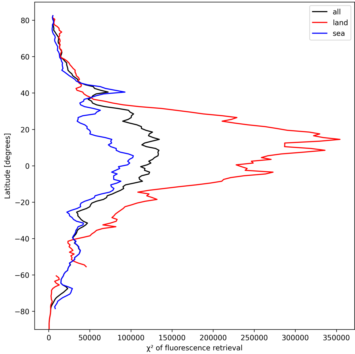
Figure 25: Zonal average of “ \chi^2 of fluorescence retrieval” for 2024-10-06 to 2024-10-08.
