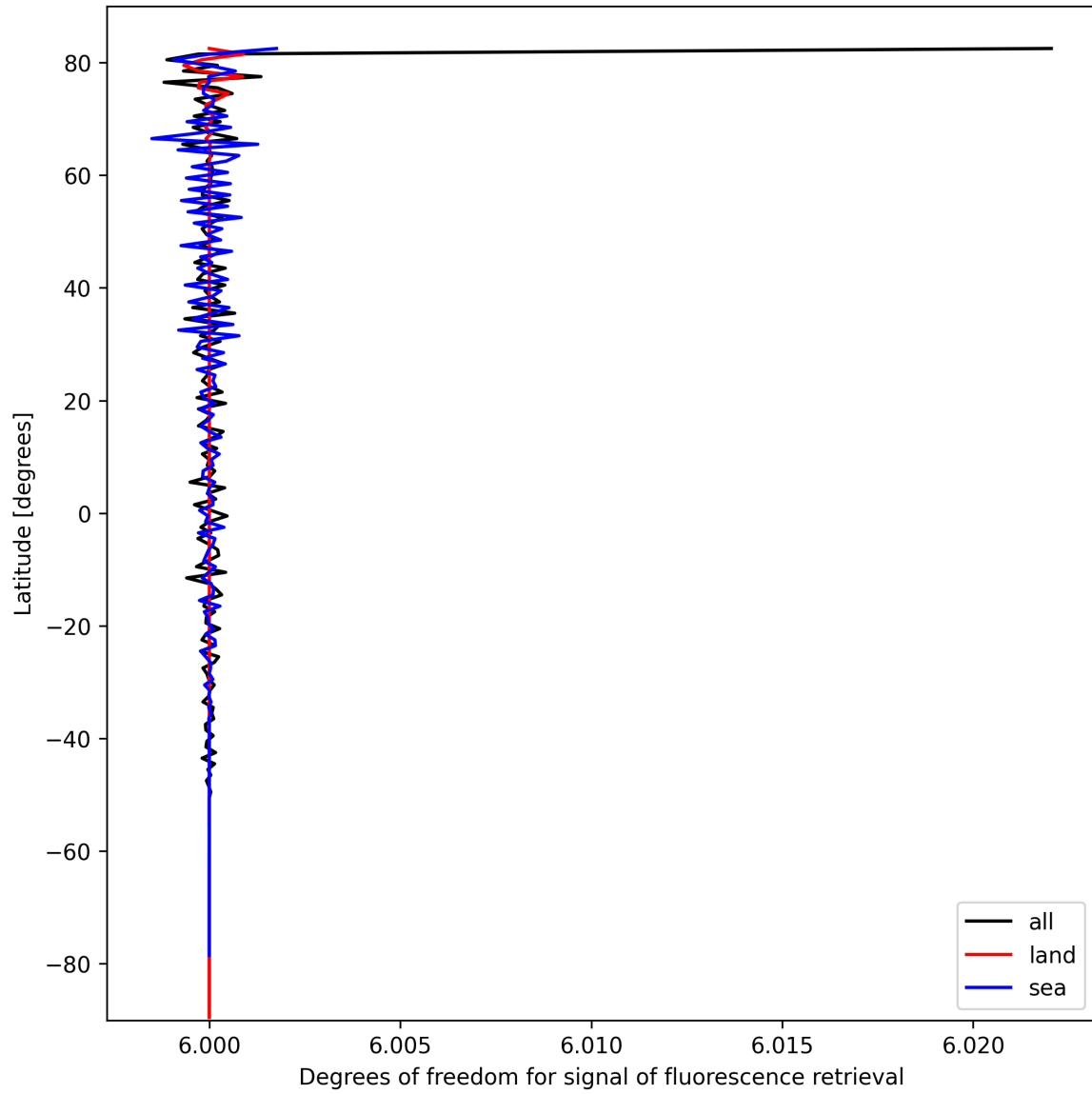
Figure 26: Zonal average of “Degrees of freedom for signal of fluorescence retrieval” for 2024-10-06 to 2024-10-08.
