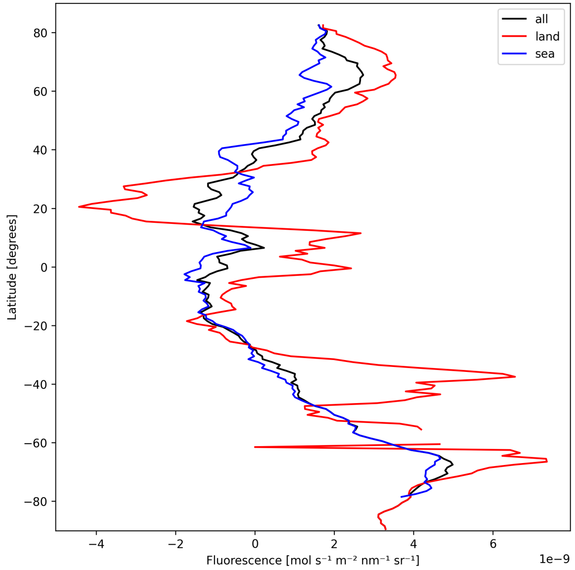
Figure 23: Zonal average of “Fluorescence” for 2024-10-06 to 2024-10-08.
