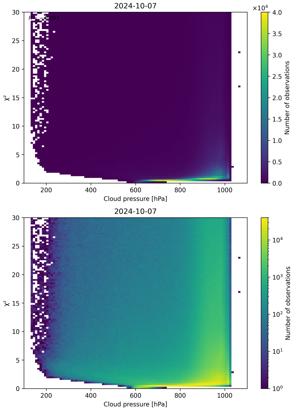
Figure 85: Scatter density plot of “Cloud pressure” against “ \chi^2 ” for 2024-10-06 to 2024-10-08.
