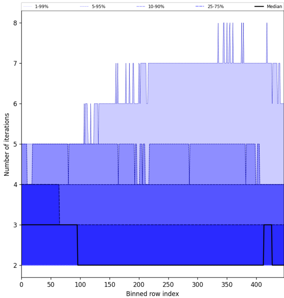
Figure 56: Along track statistics of “Number of iterations” for 2024-10-06 to 2024-10-08
