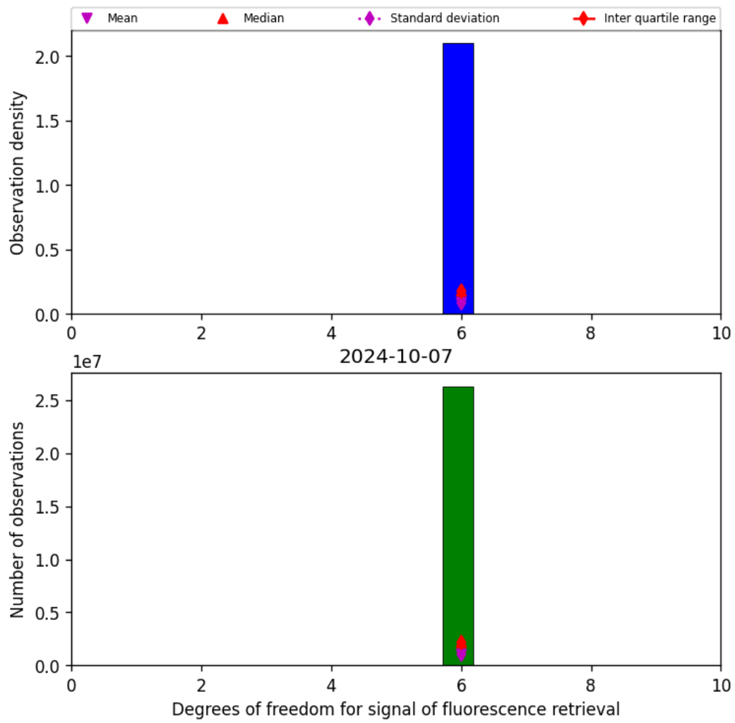
Figure 43: Histogram of “Degrees of freedom for signal of fluorescence retrieval” for 2024-10-06 to 2024-10-08
