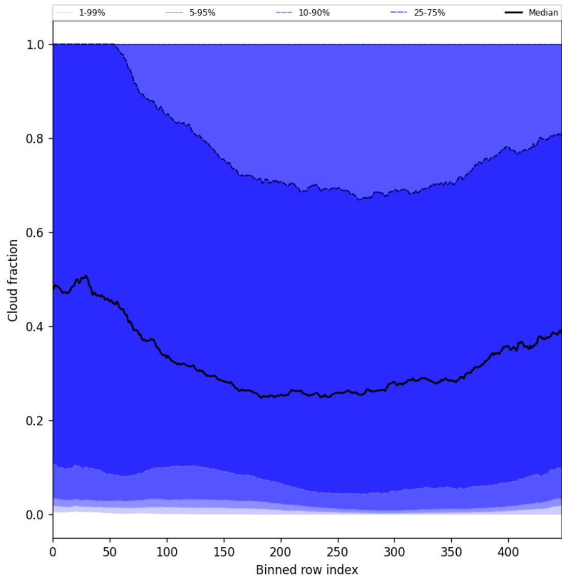
Figure 49: Along track statistics of “Cloud fraction” for 2024-10-06 to 2024-10-08
