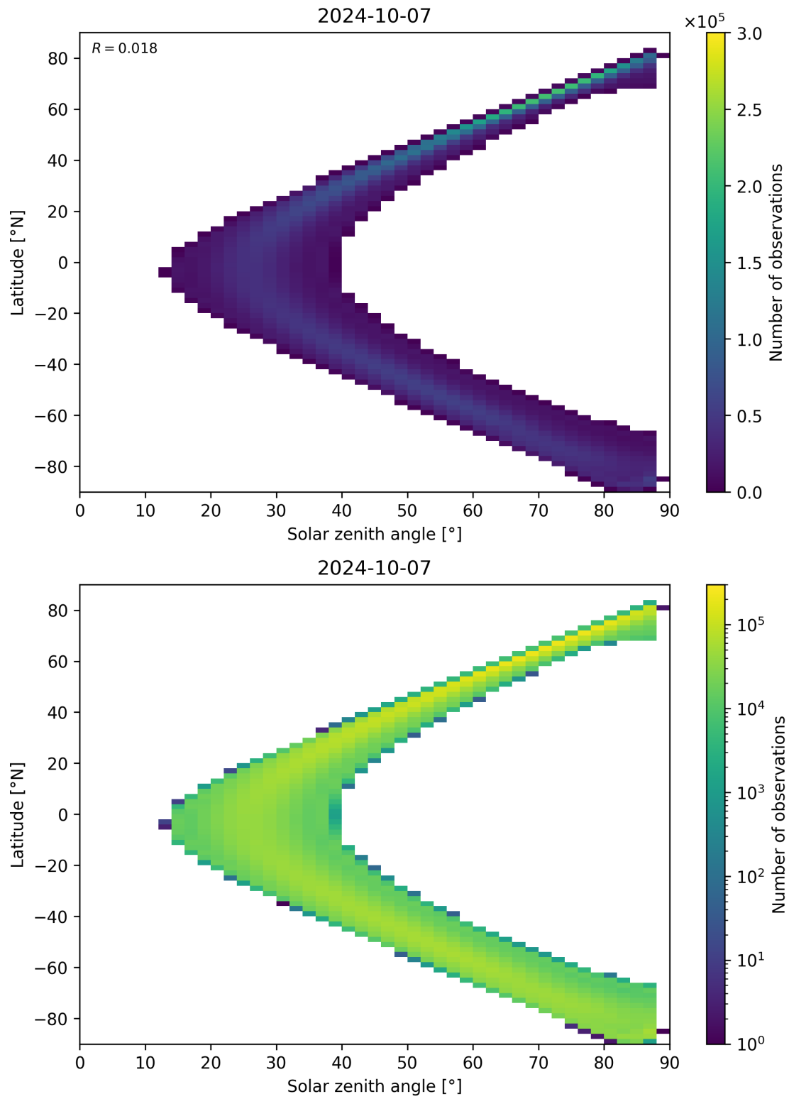
Figure 124: Scatter density plot of “Solar zenith angle” against “Latitude” for 2024-10-06 to 2024-10-08.
