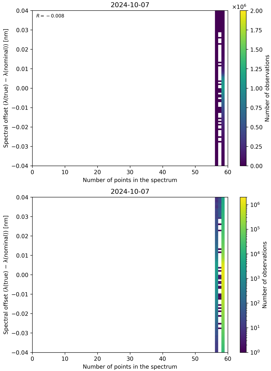
Figure 110: Scatter density plot of “Number of points in the spectrum” against “Spectral offset ( \lambda_{\text{true}} - \lambda_{\text{nominal}} )” for 2024-10-06 to 2024-10-08.
