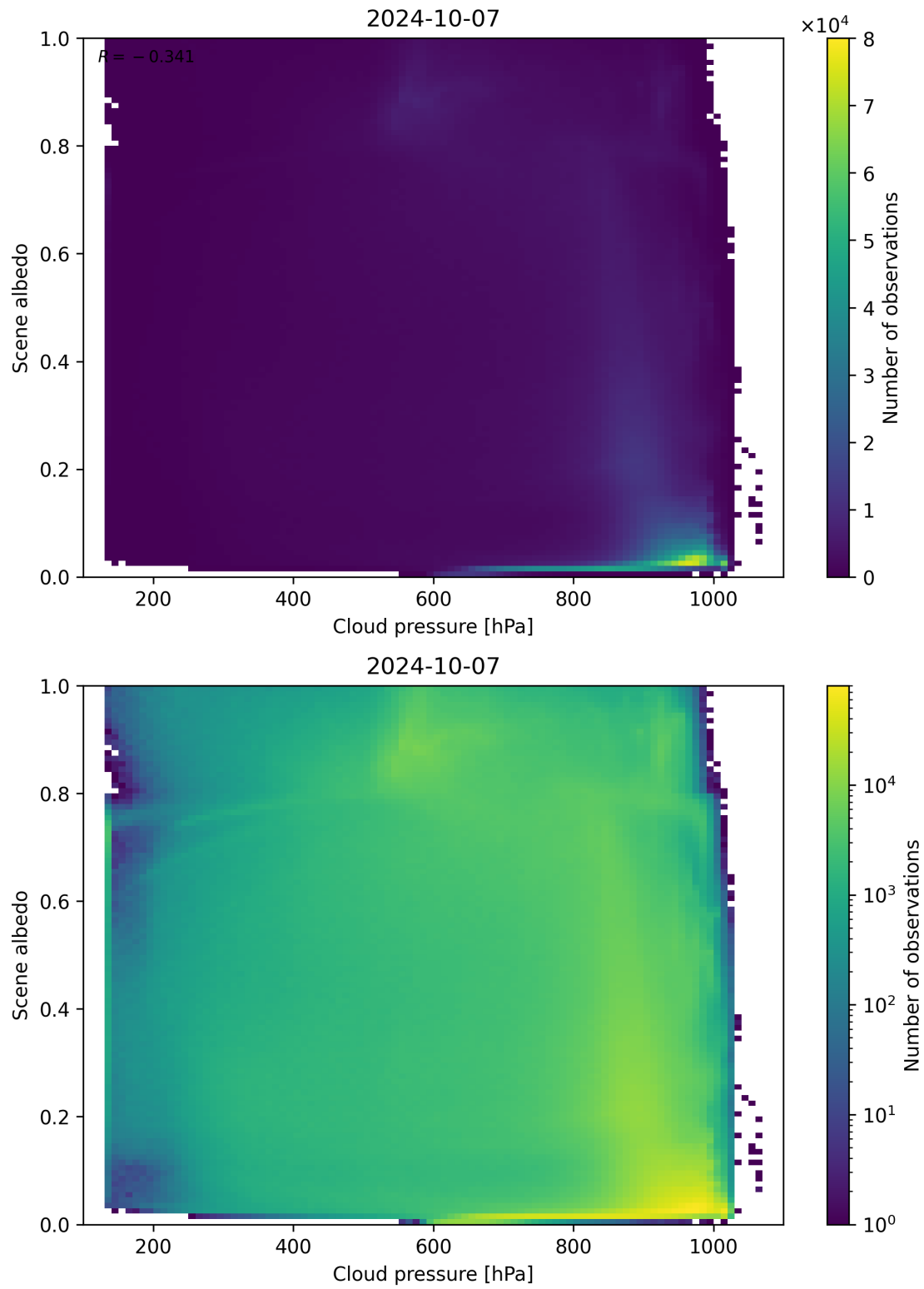
Figure 91: Scatter density plot of “Cloud pressure” against “Scene albedo” for 2024-10-06 to 2024-10-08.
