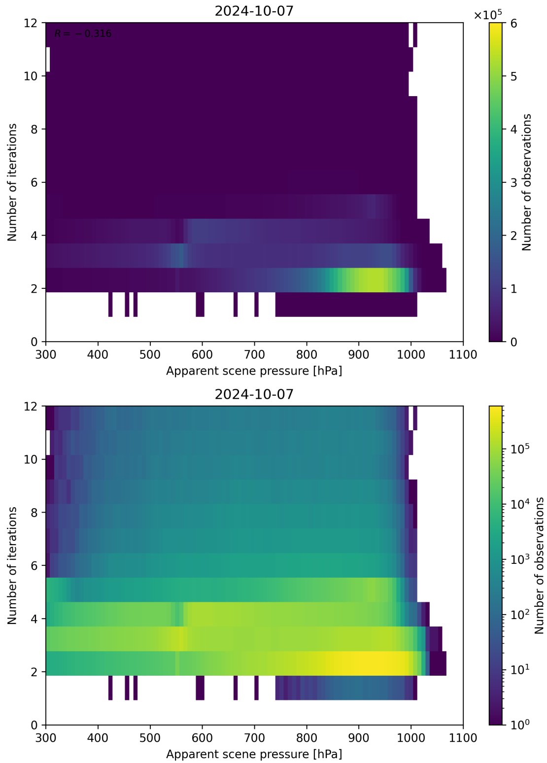
Figure 66: Scatter density plot of “Apparent scene pressure” against “Number of iterations” for 2024-10-06 to 2024-10-08.
