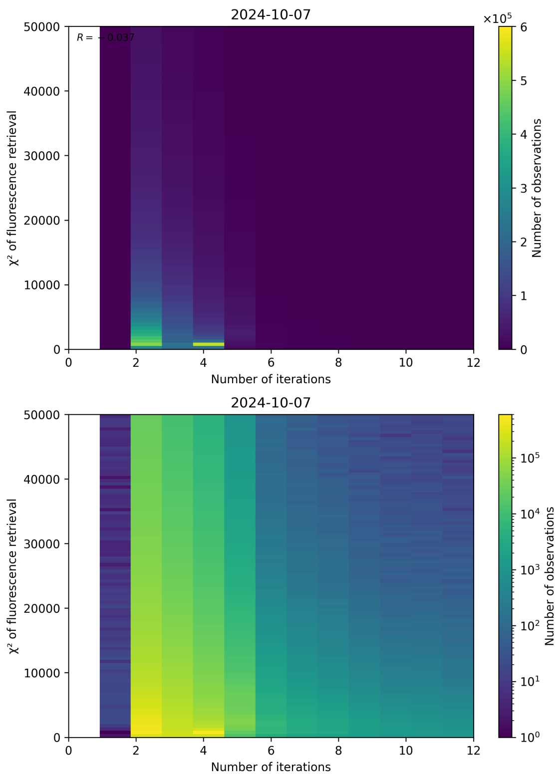
Figure 106: Scatter density plot of “Number of iterations” against “ \chi^2 of fluorescence retrieval” for 2024-10-06 to 2024-10-08.
