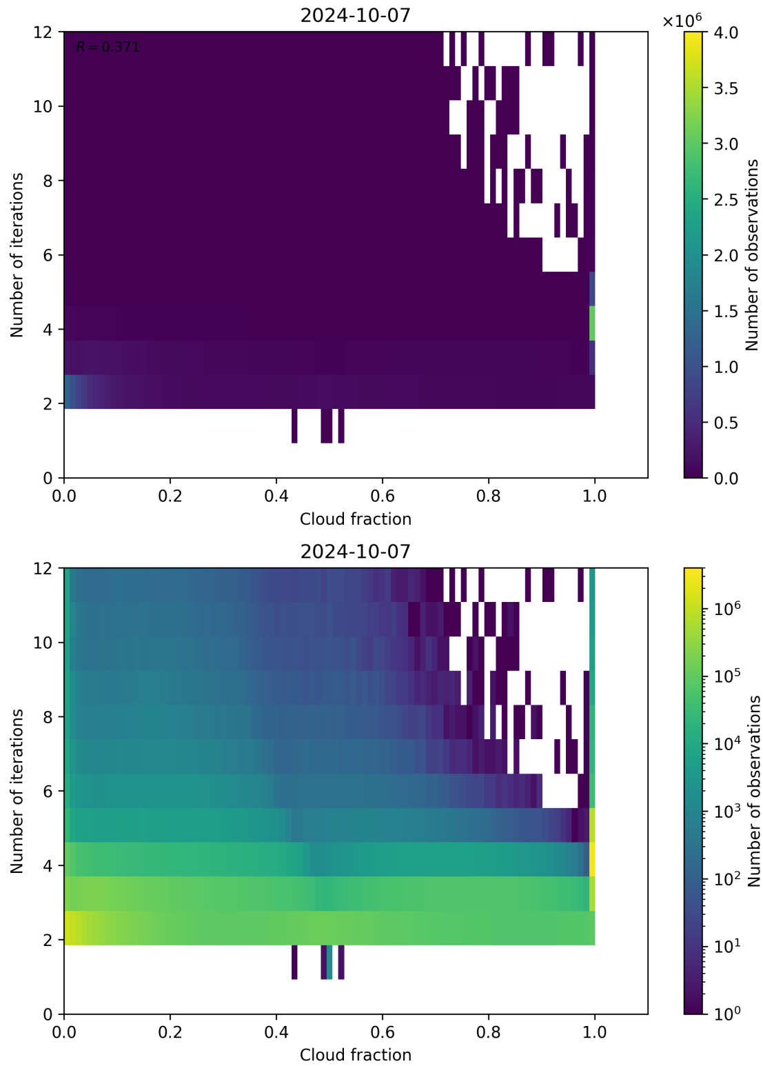
Figure 80: Scatter density plot of “Cloud fraction” against “Number of iterations” for 2024-10-06 to 2024-10-08.
