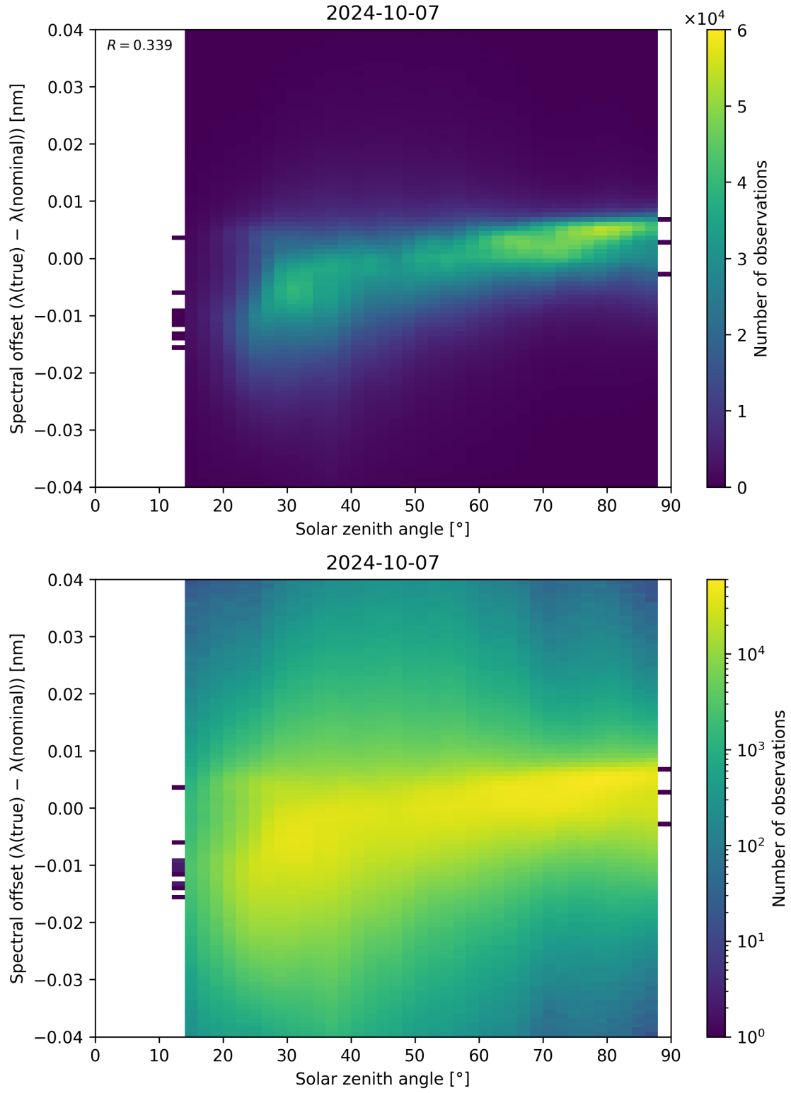
Figure 128: Scatter density plot of “Solar zenith angle” against “Spectral offset ( \lambda_{\text{true}} - \lambda_{\text{nominal}} )” for 2024-10-06 to 2024-10-08.
