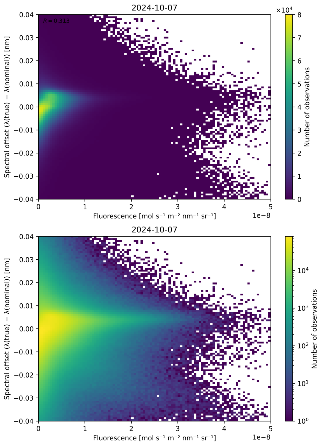
Figure 95: Scatter density plot of “Fluorescence” against “Spectral offset ( \lambda_{\text{true}} - \lambda_{\text{nominal}} )” for 2024-10-06 to 2024-10-08.
