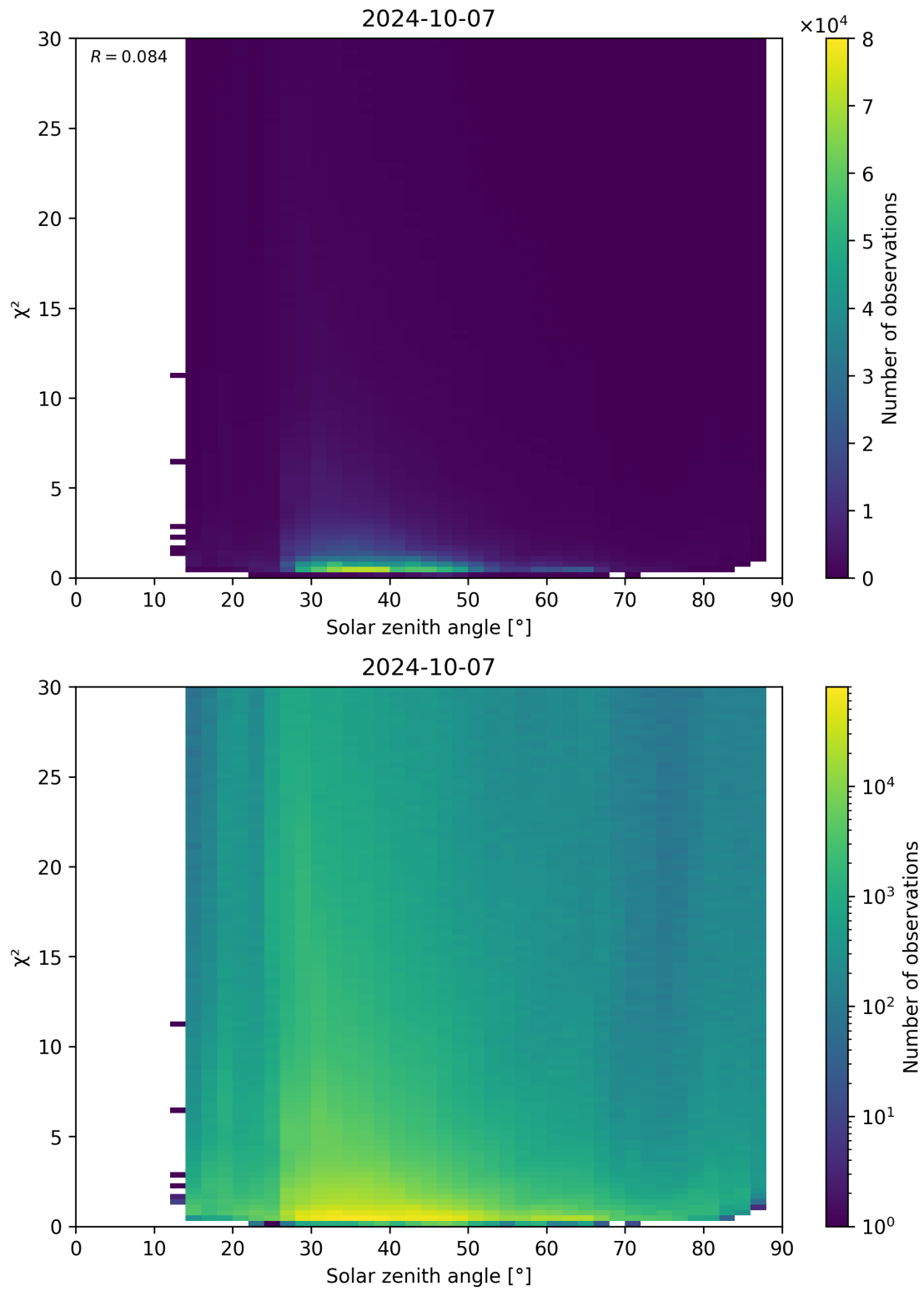
Figure 119: Scatter density plot of “Solar zenith angle” against “ \chi^2 ” for 2024-10-06 to 2024-10-08.
