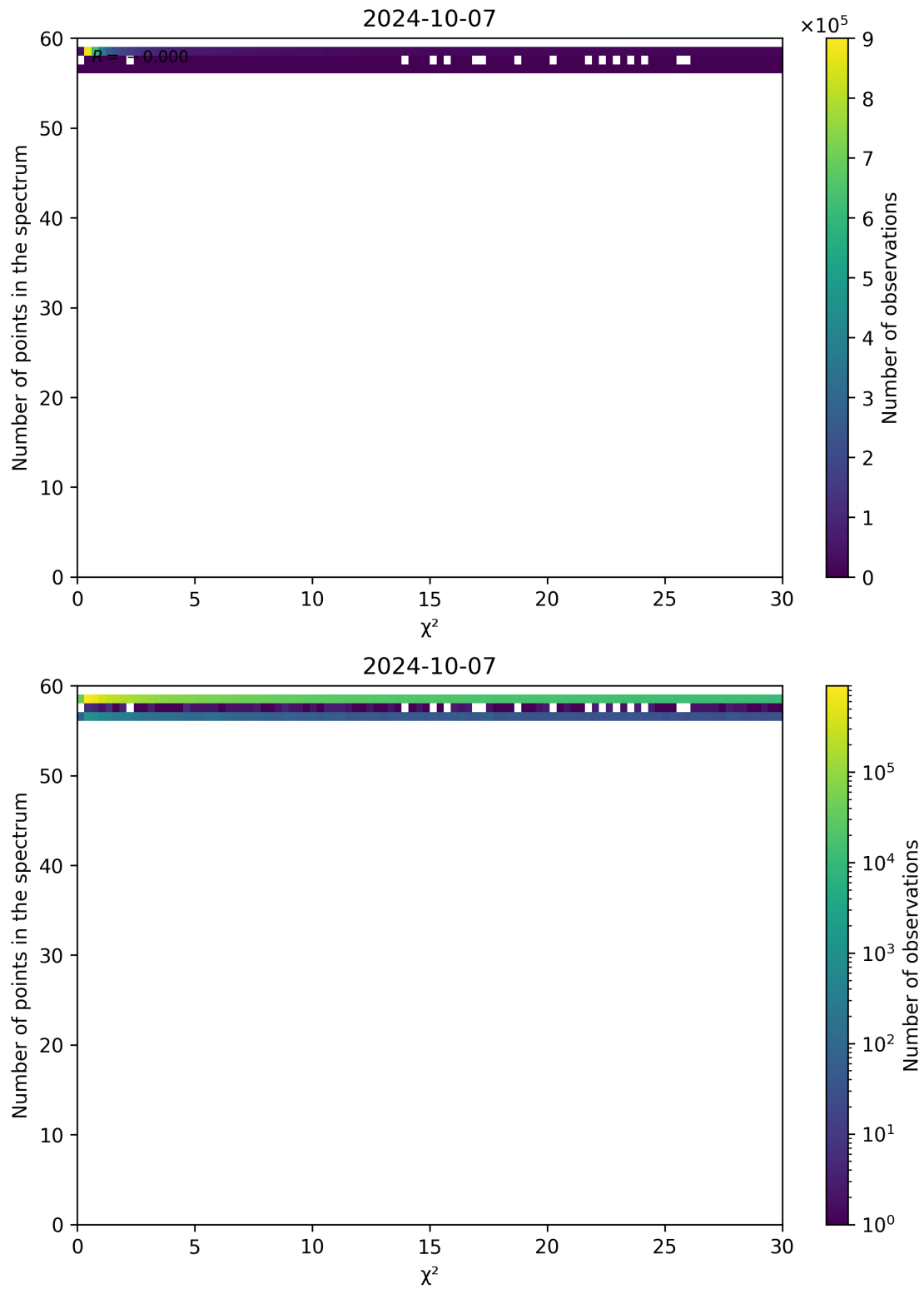
Figure 74: Scatter density plot of “ \chi^2 ” against “Number of points in the spectrum” for 2024-10-06 to 2024-10-08.
