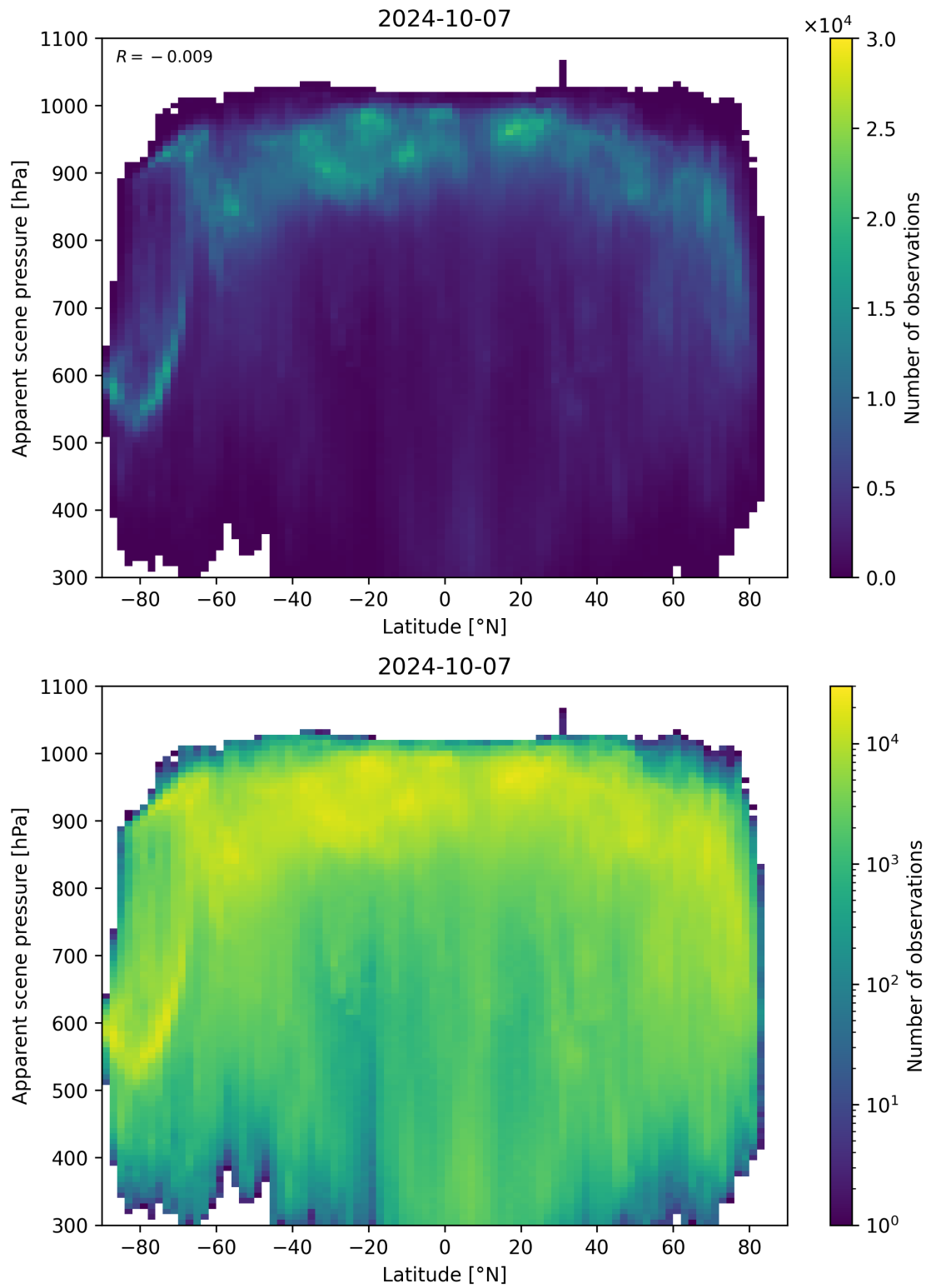
Figure 96: Scatter density plot of “Latitude” against “Apparent scene pressure” for 2024-10-06 to 2024-10-08.
