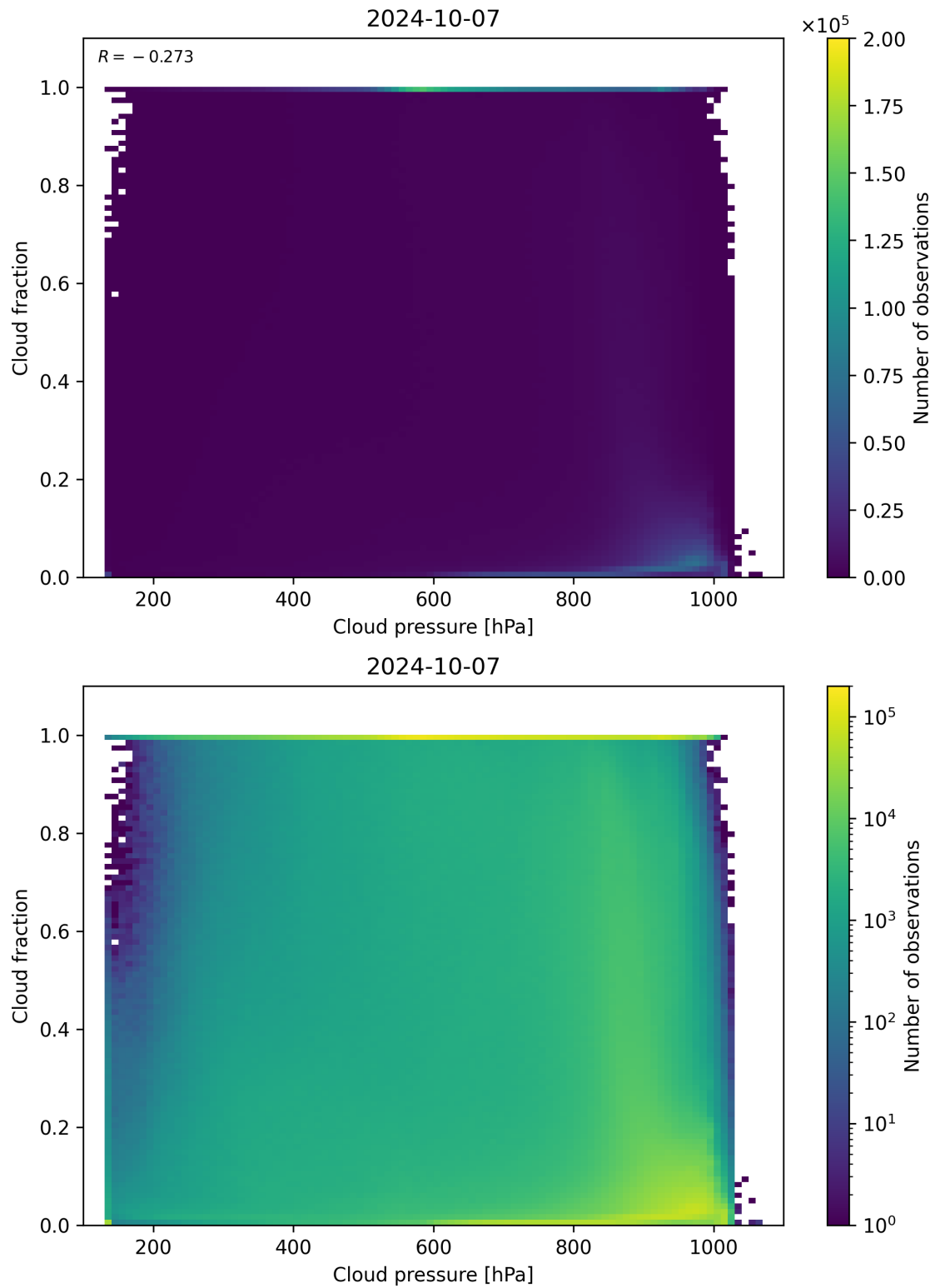
Figure 87: Scatter density plot of “Cloud pressure” against “Cloud fraction” for 2024-10-06 to 2024-10-08.
