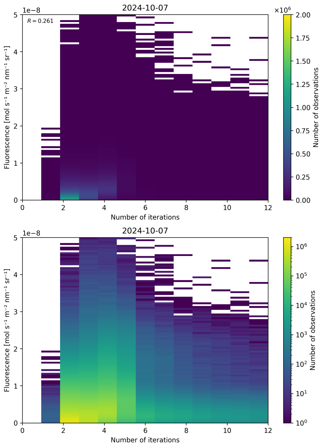
Figure 107: Scatter density plot of “Number of iterations” against “Fluorescence” for 2024-10-06 to 2024-10-08.
