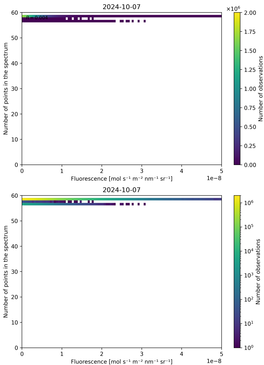
Figure 94: Scatter density plot of “Fluorescence” against “Number of points in the spectrum” for 2024-10-06 to 2024-10-08.
