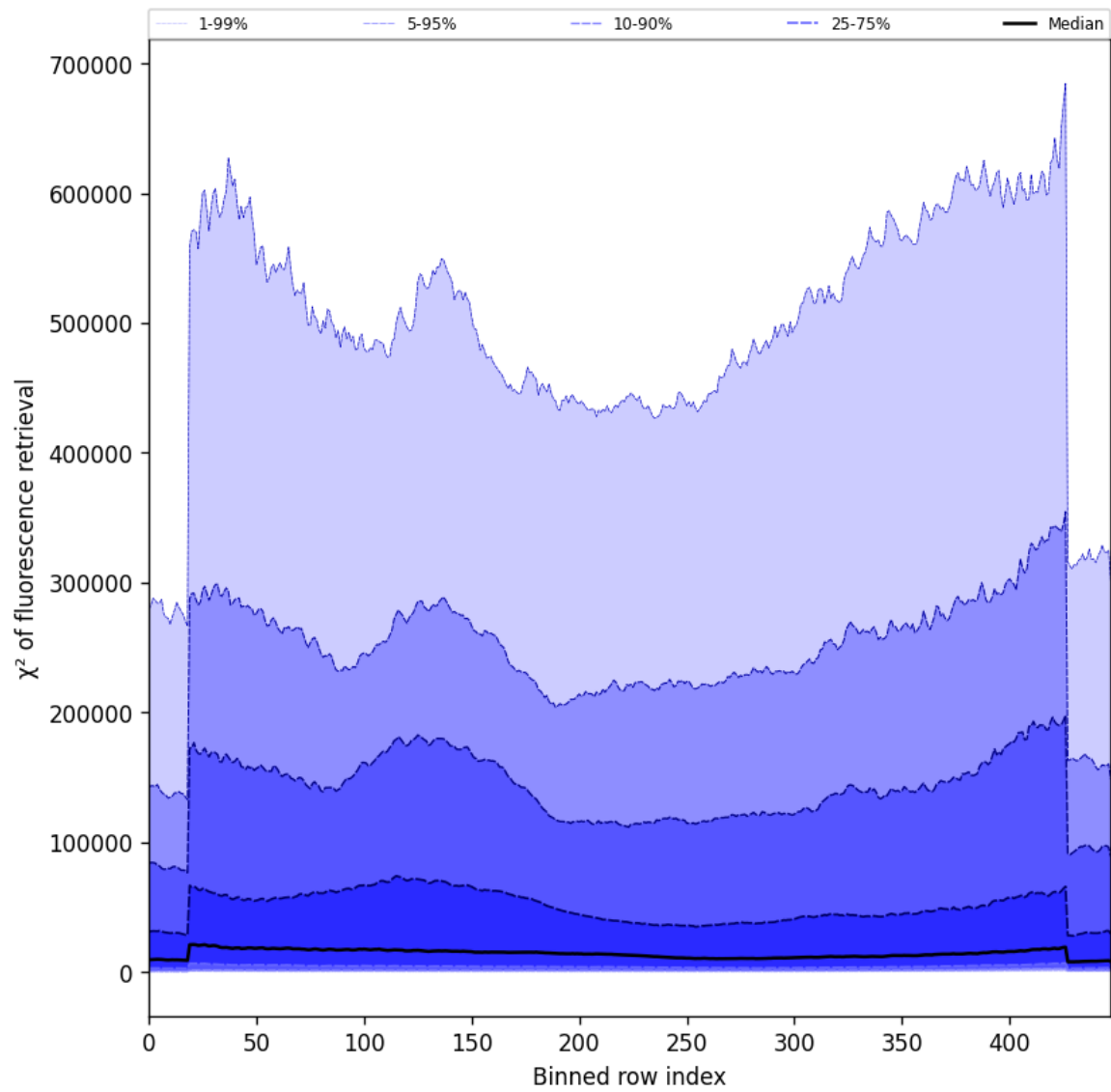
Figure 59: Along track statistics of “ \chi^2 of fluorescence retrieval” for 2024-10-06 to 2024-10-08
