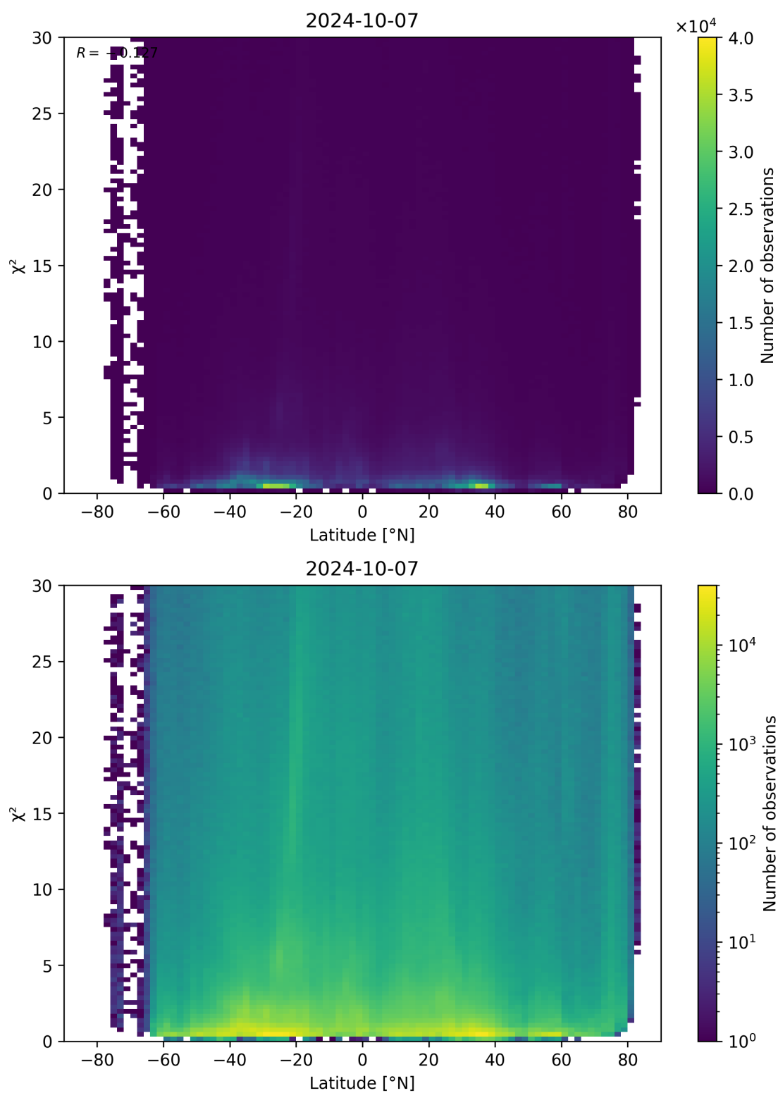
Figure 97: Scatter density plot of “Latitude” against “ \chi^2 ” for 2024-10-06 to 2024-10-08.
