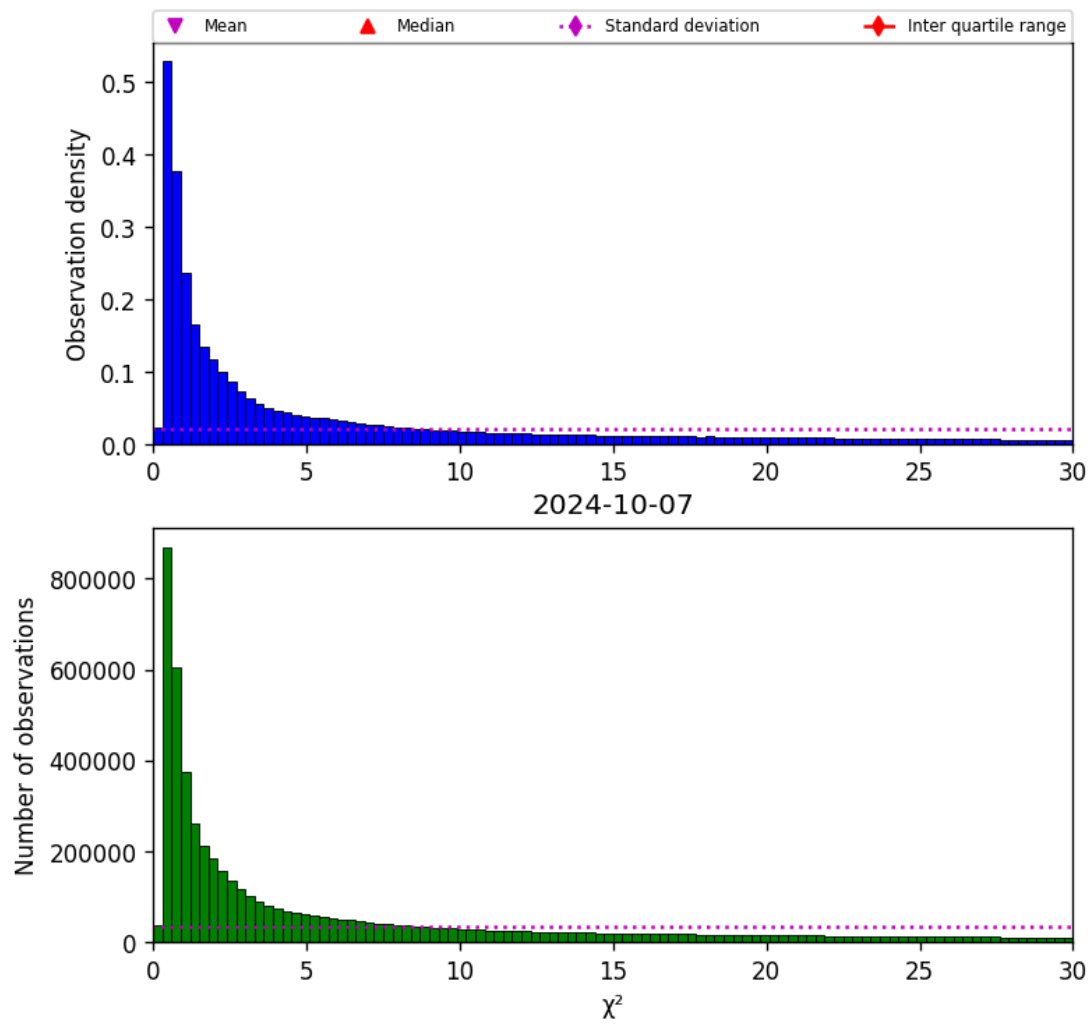
Figure 38: Histogram of “ \chi^2 ” for 2024-10-06 to 2024-10-08
