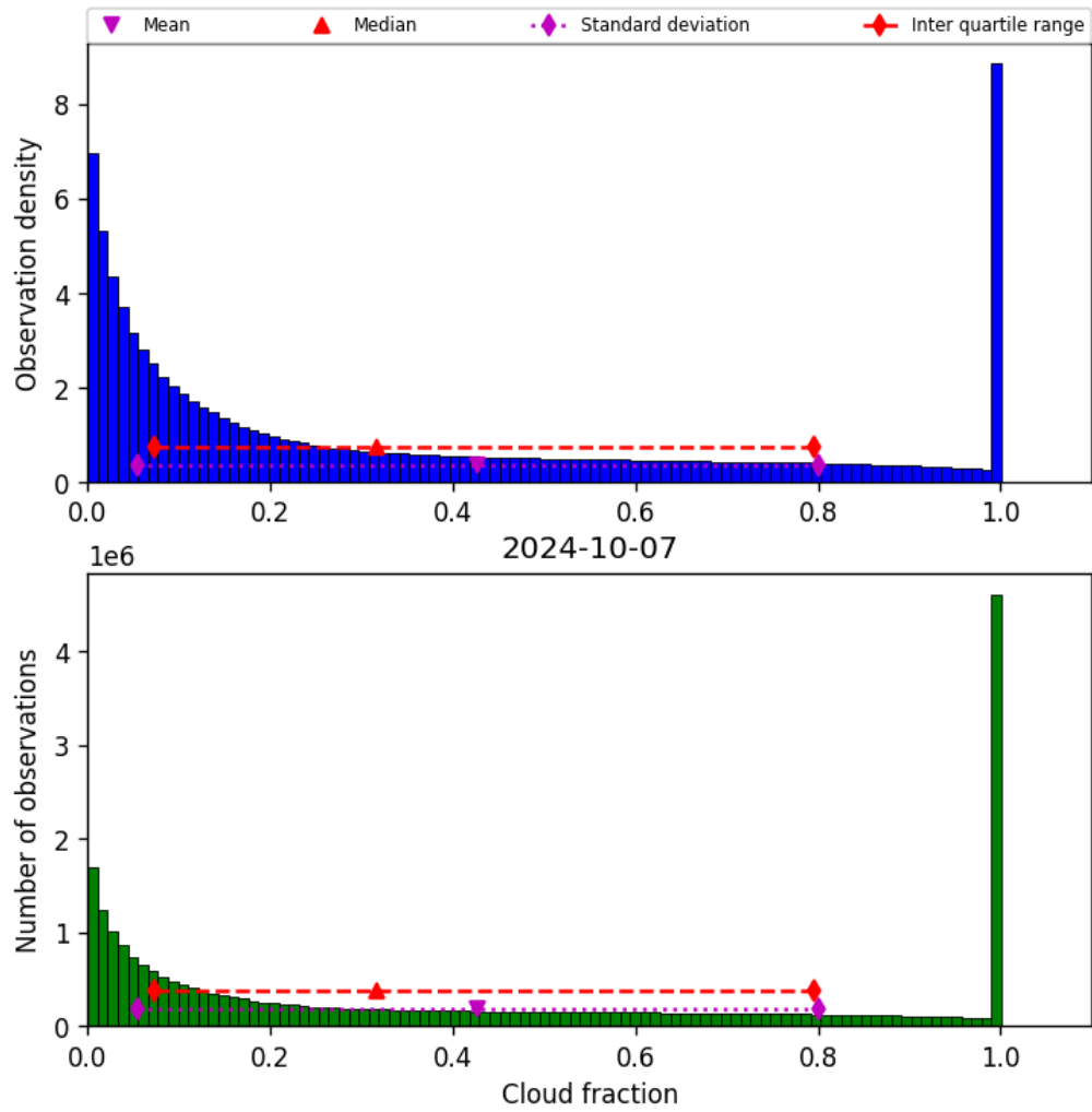
Figure 32: Histogram of “Cloud fraction” for 2024-10-06 to 2024-10-08
