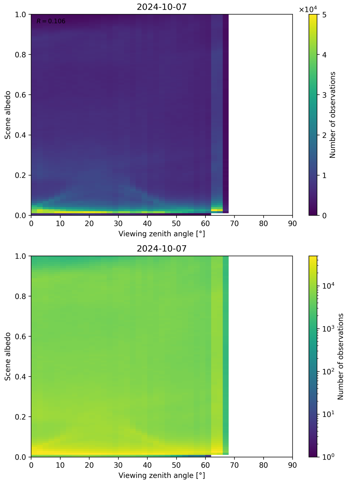
Figure 138: Scatter density plot of “Viewing zenith angle” against “Scene albedo” for 2024-10-06 to 2024-10-08.
