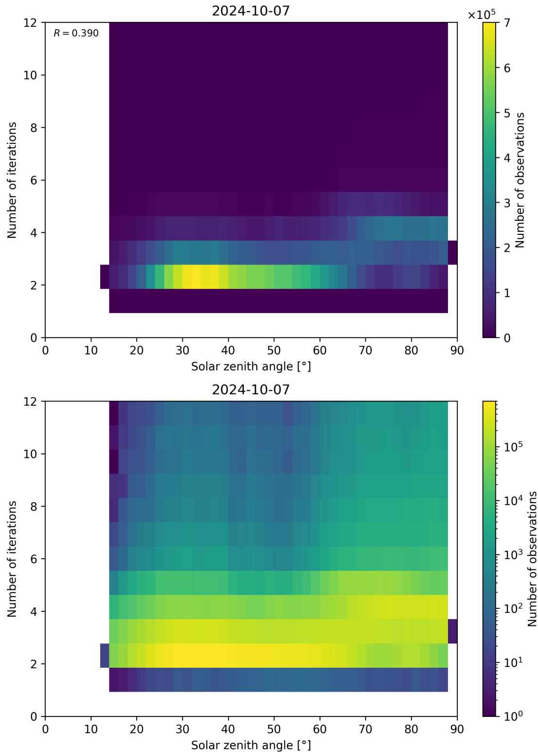
Figure 125: Scatter density plot of “Solar zenith angle” against “Number of iterations” for 2024-10-06 to 2024-10-08.
