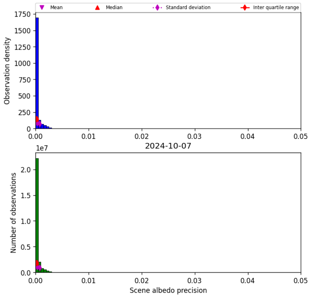
Figure 35: Histogram of “Scene albedo precision” for 2024-10-06 to 2024-10-08
