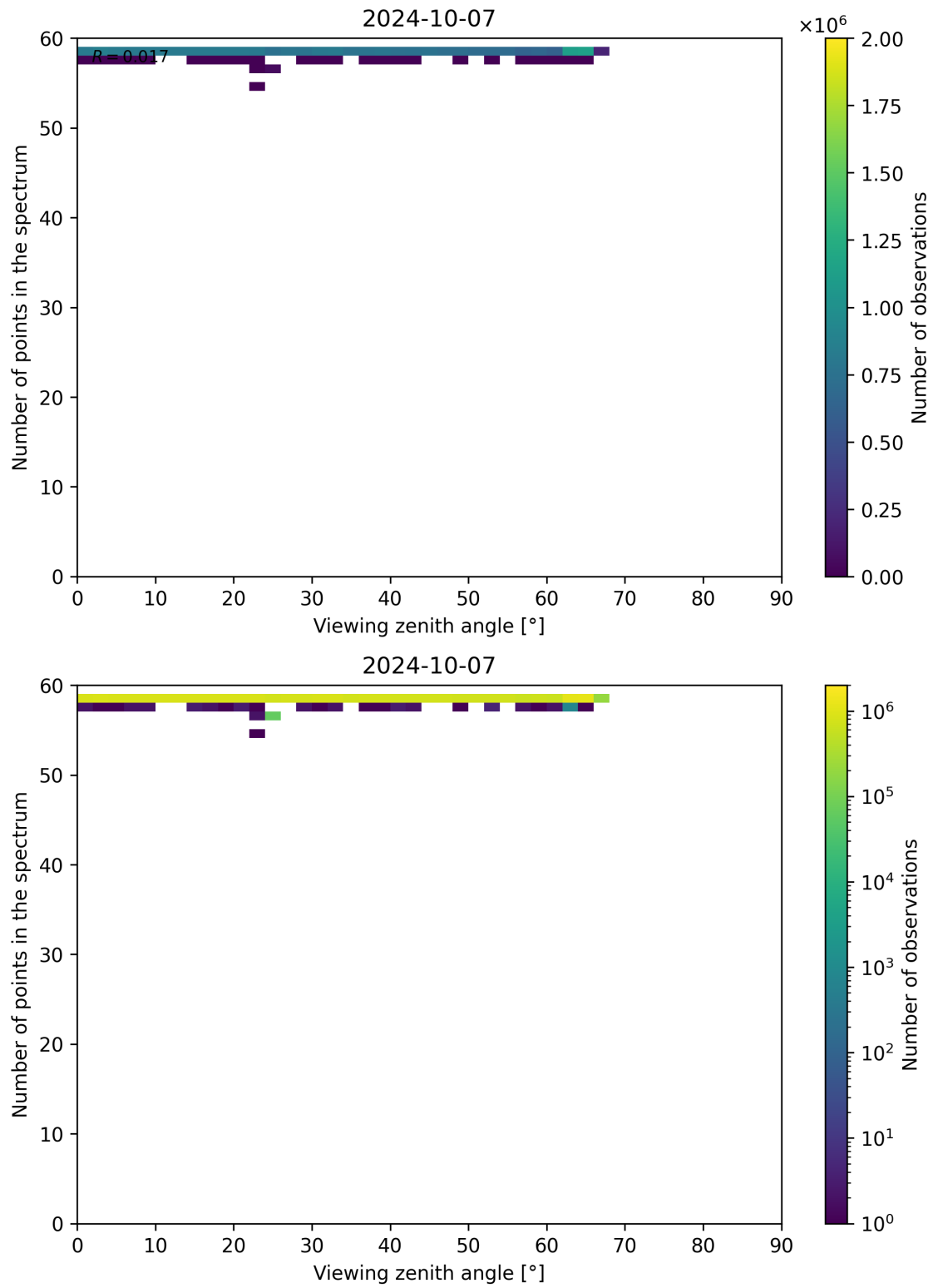
Figure 137: Scatter density plot of “Viewing zenith angle” against “Number of points in the spectrum” for 2024-10-06 to 2024-10-08.
