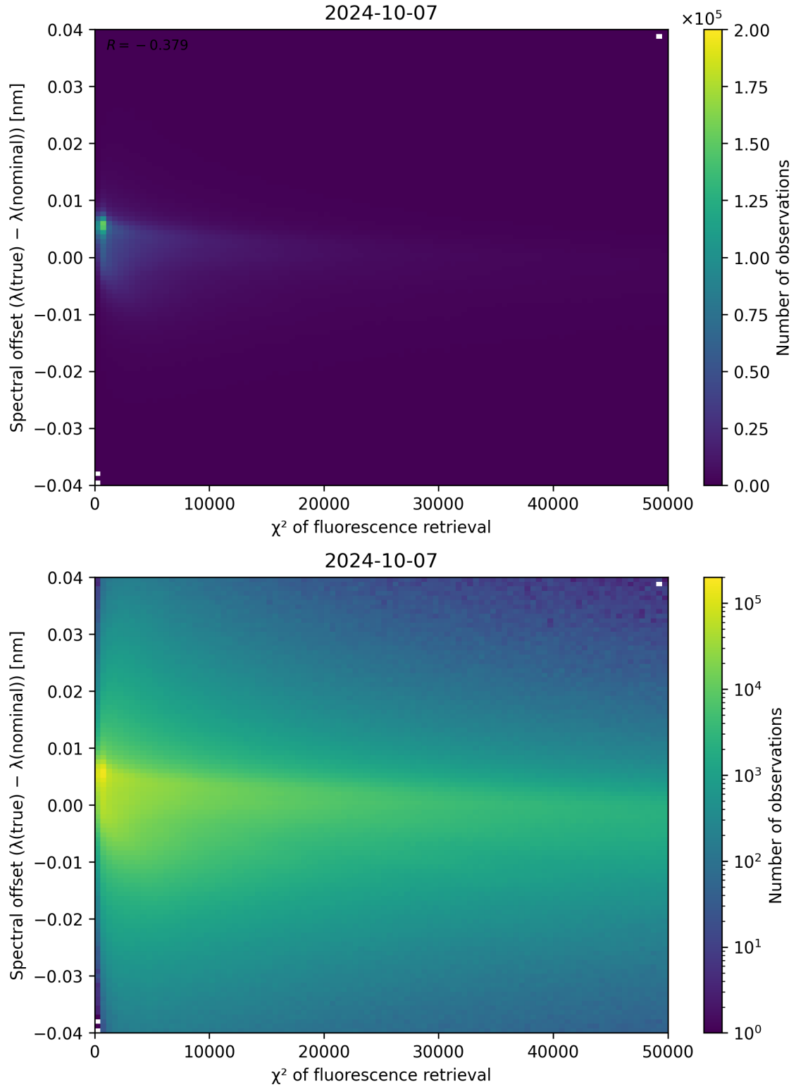
Figure 72: Scatter density plot of “ \chi^2 of fluorescence retrieval” against “Spectral offset ( \lambda_{\text{true}} - \lambda_{\text{nominal}} )” for 2024-10-06 to 2024-10-08.
