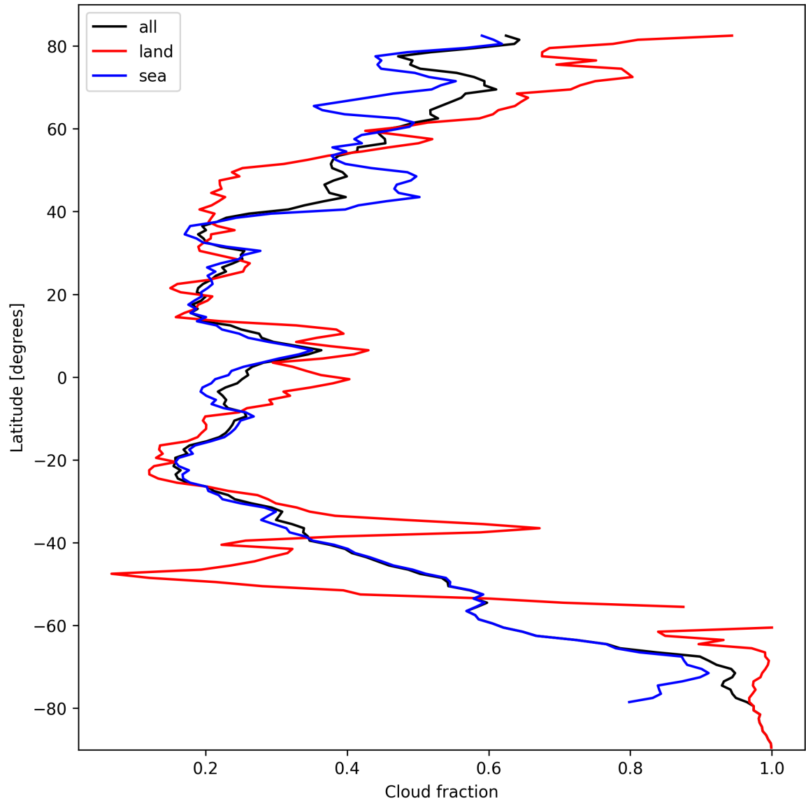
Figure 15: Zonal average of “Cloud fraction” for 2024-10-06 to 2024-10-08.
