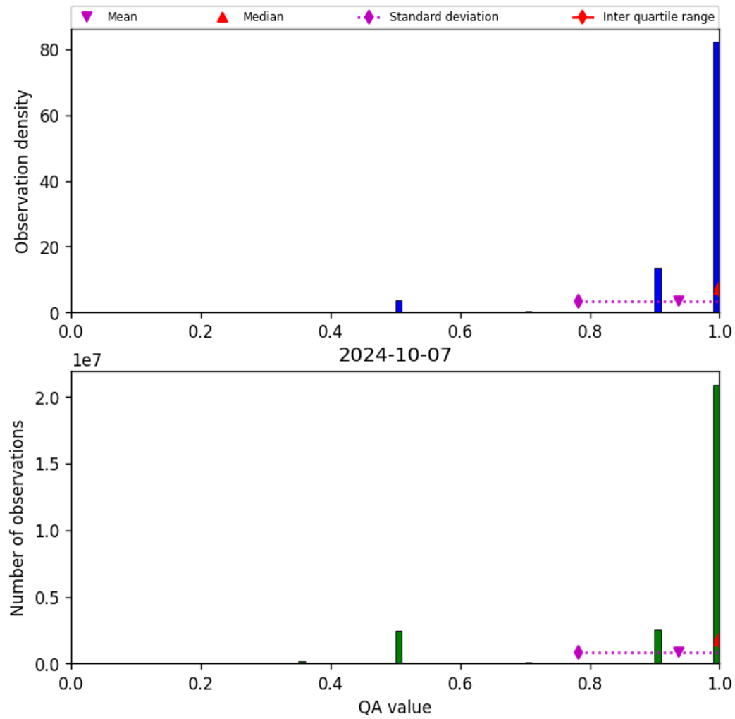
Figure 29: Histogram of “QA value” for 2024-10-06 to 2024-10-08
