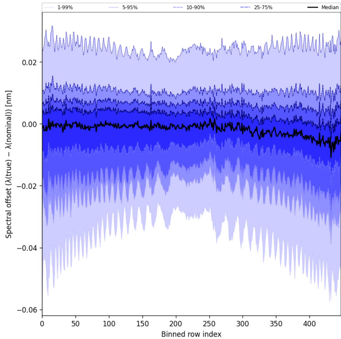
Figure 62: Along track statistics of “Spectral offset ( \lambda_{\text{true}} - \lambda_{\text{nominal}} )” for 2024-10-06 to 2024-10-08
