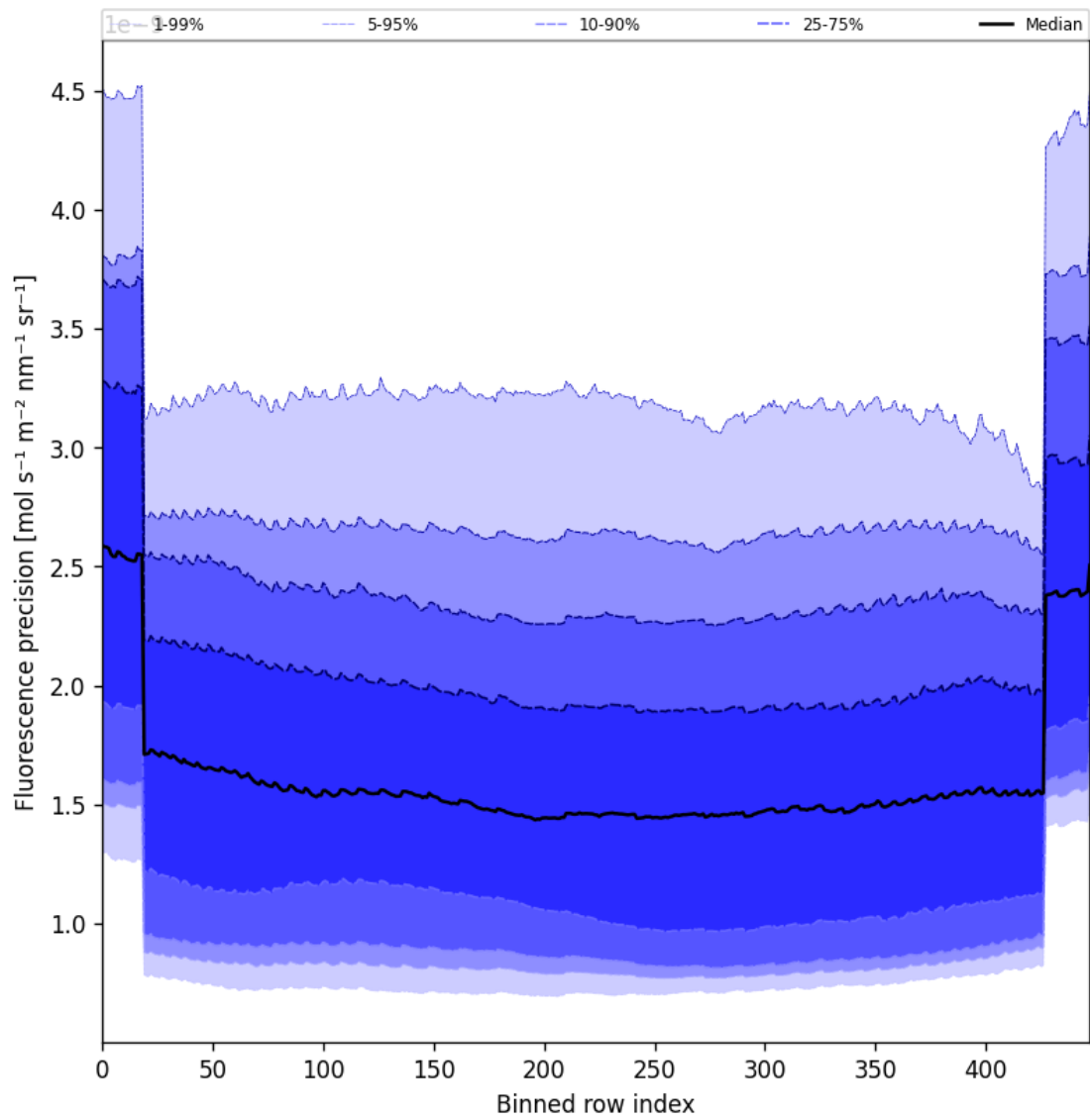
Figure 58: Along track statistics of “Fluorescence precision” for 2024-10-06 to 2024-10-08
