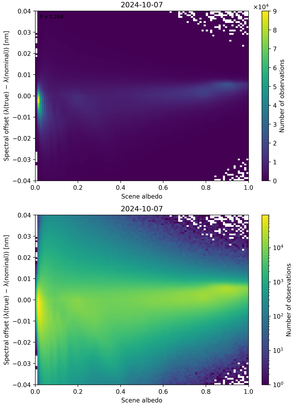
Figure 117: Scatter density plot of “Scene albedo” against “Spectral offset ( \lambda_{\text{true}} - \lambda_{\text{nominal}} )” for 2024-10-06 to 2024-10-08.
