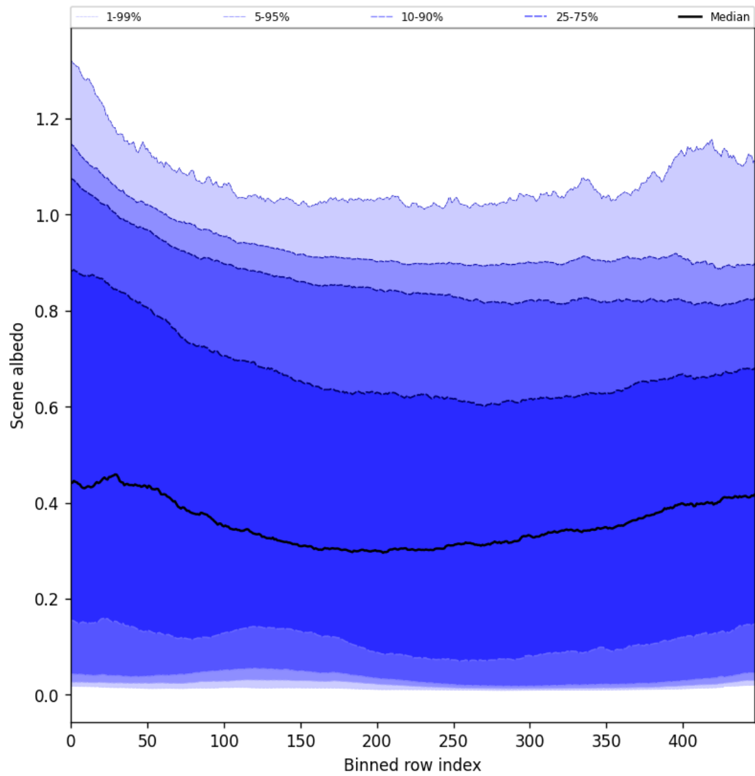
Figure 51: Along track statistics of “Scene albedo” for 2024-10-06 to 2024-10-08
