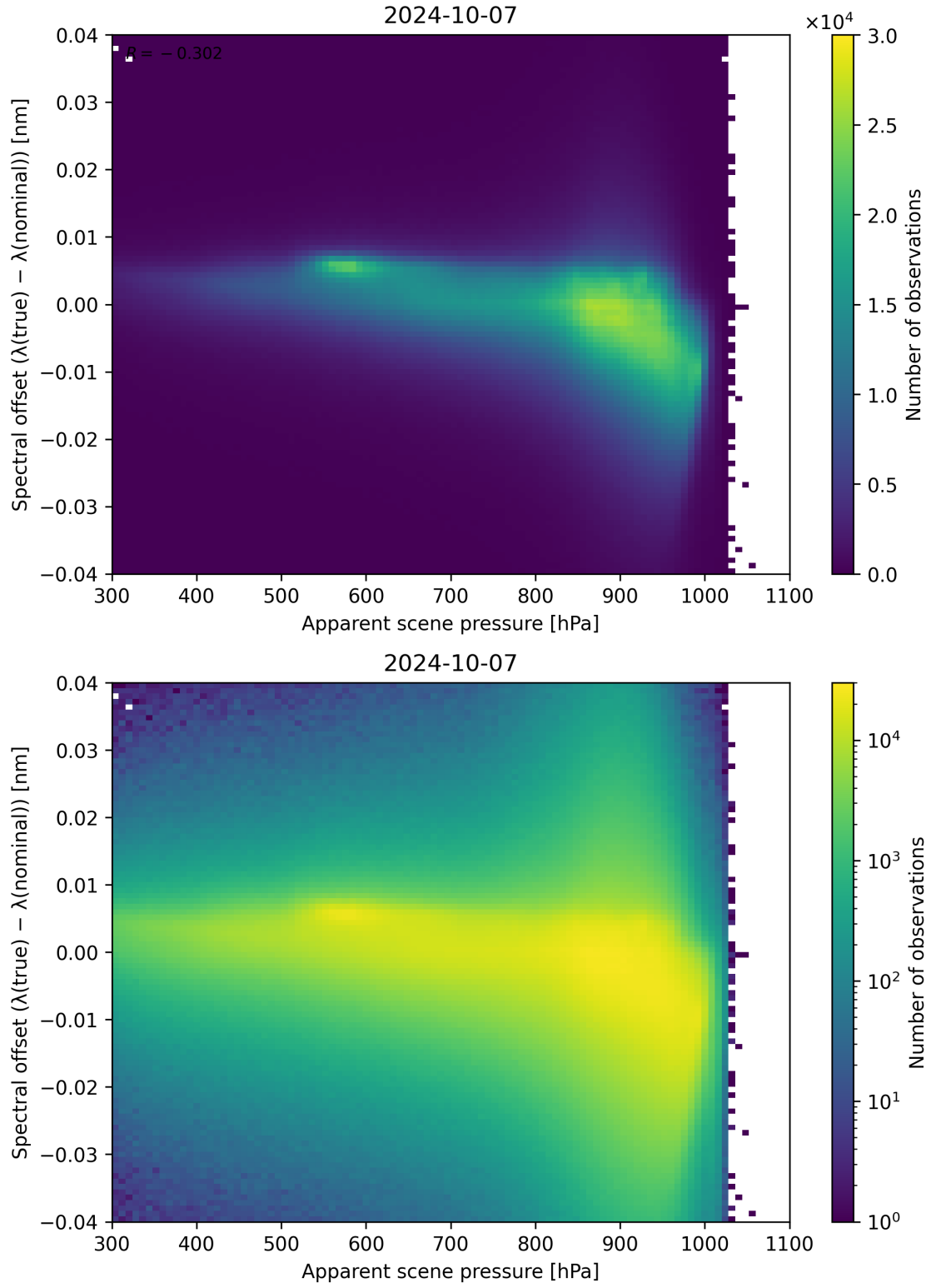
Figure 68: Scatter density plot of “Apparent scene pressure” against “Spectral offset ( \lambda_{\text{true}} - \lambda_{\text{nominal}} )” for 2024-10-06 to 2024-10-08.
