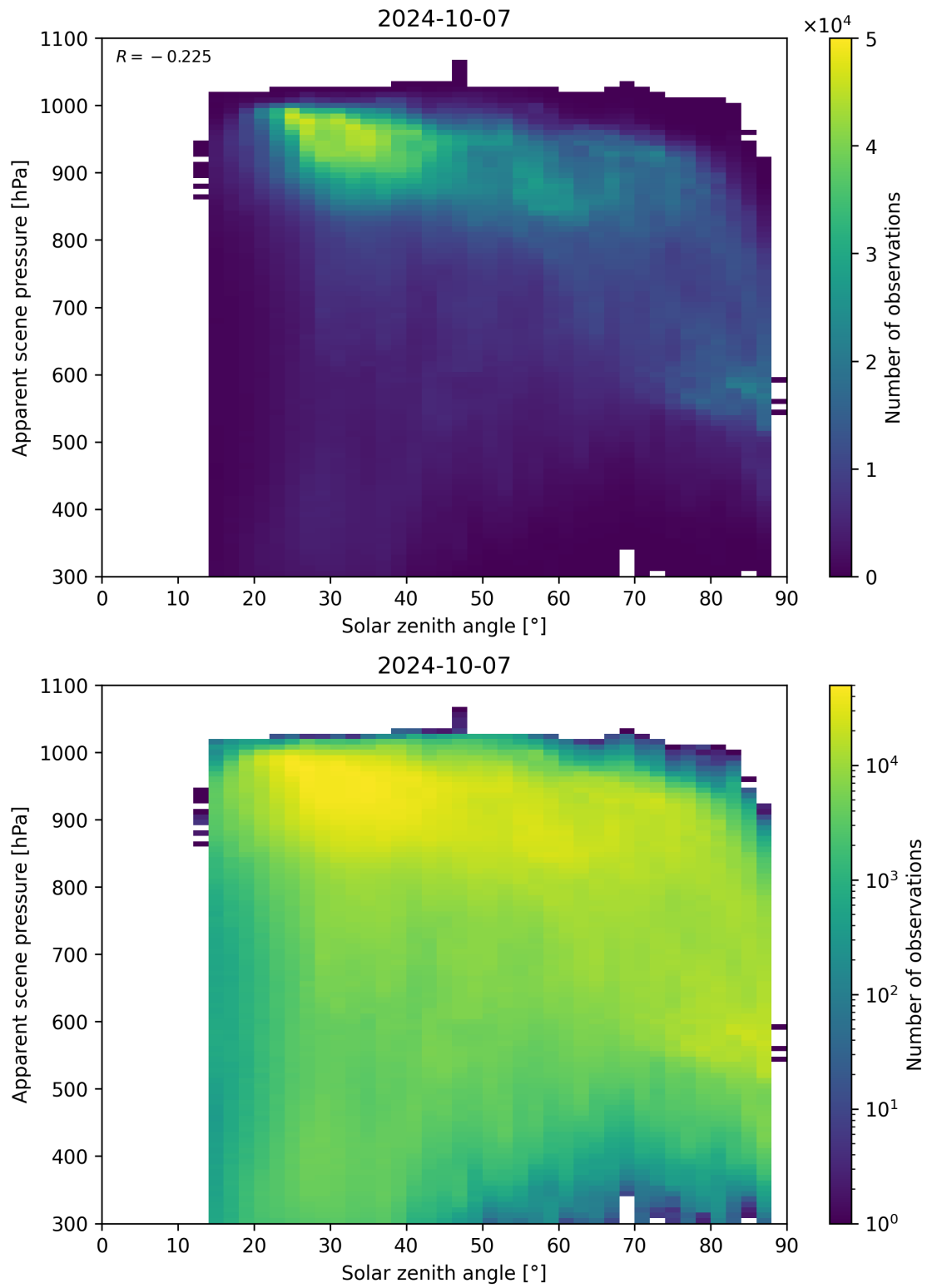
Figure 118: Scatter density plot of “Solar zenith angle” against “Apparent scene pressure” for 2024-10-06 to 2024-10-08.
