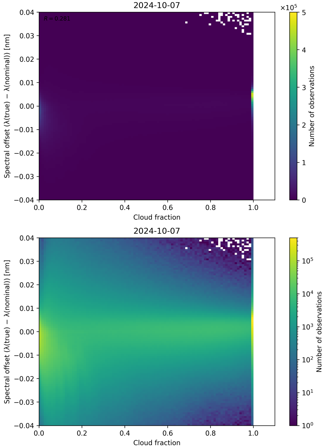
Figure 83: Scatter density plot of “Cloud fraction” against “Spectral offset ( \lambda_{\text{true}} - \lambda_{\text{nominal}} )” for 2024-10-06 to 2024-10-08.
