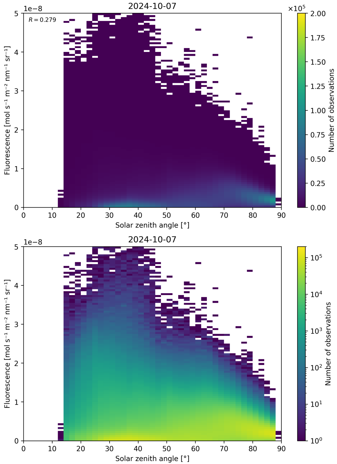
Figure 123: Scatter density plot of “Solar zenith angle” against “Fluorescence” for 2024-10-06 to 2024-10-08.
