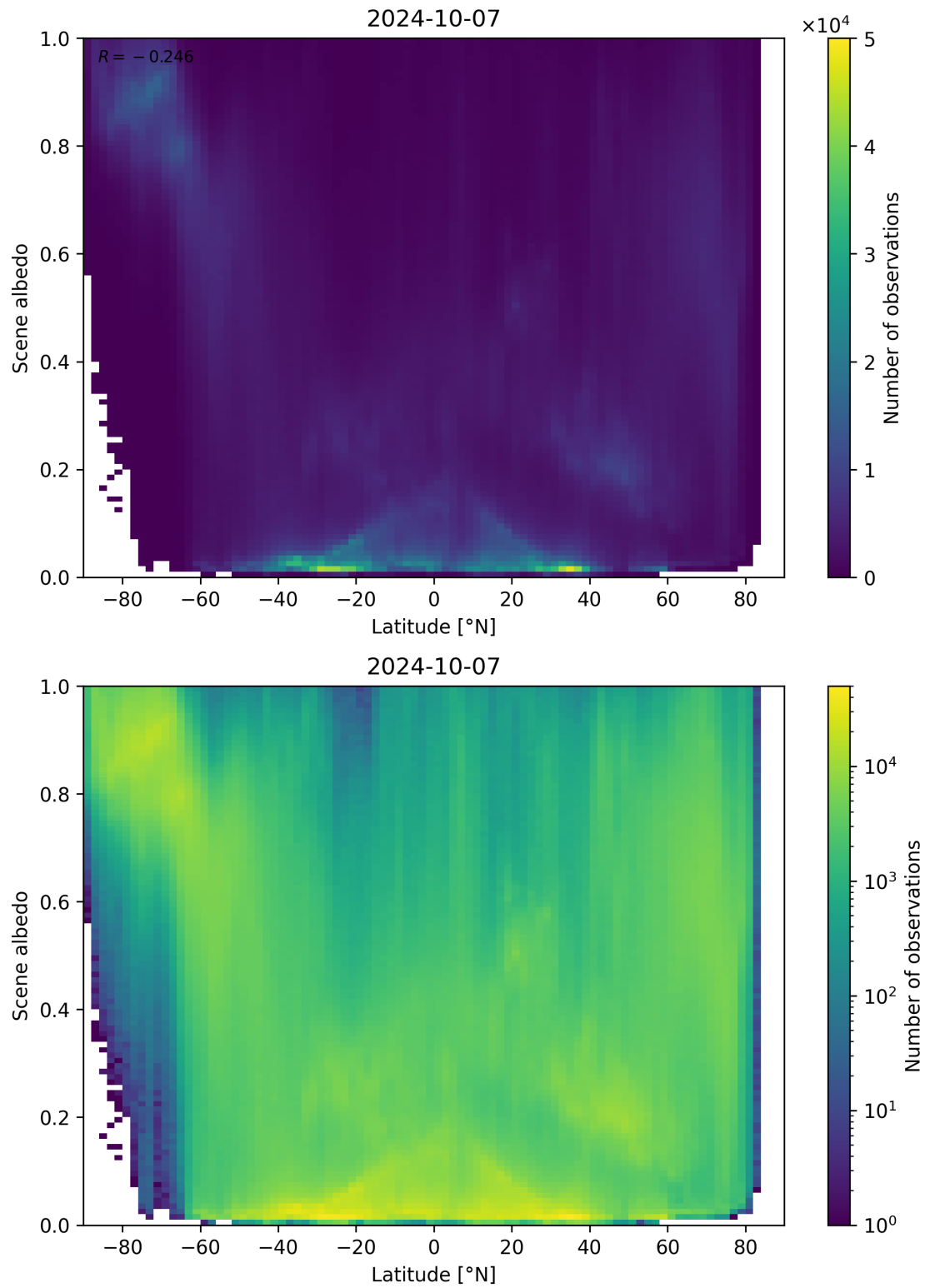
Figure 104: Scatter density plot of “Latitude” against “Scene albedo” for 2024-10-06 to 2024-10-08.
