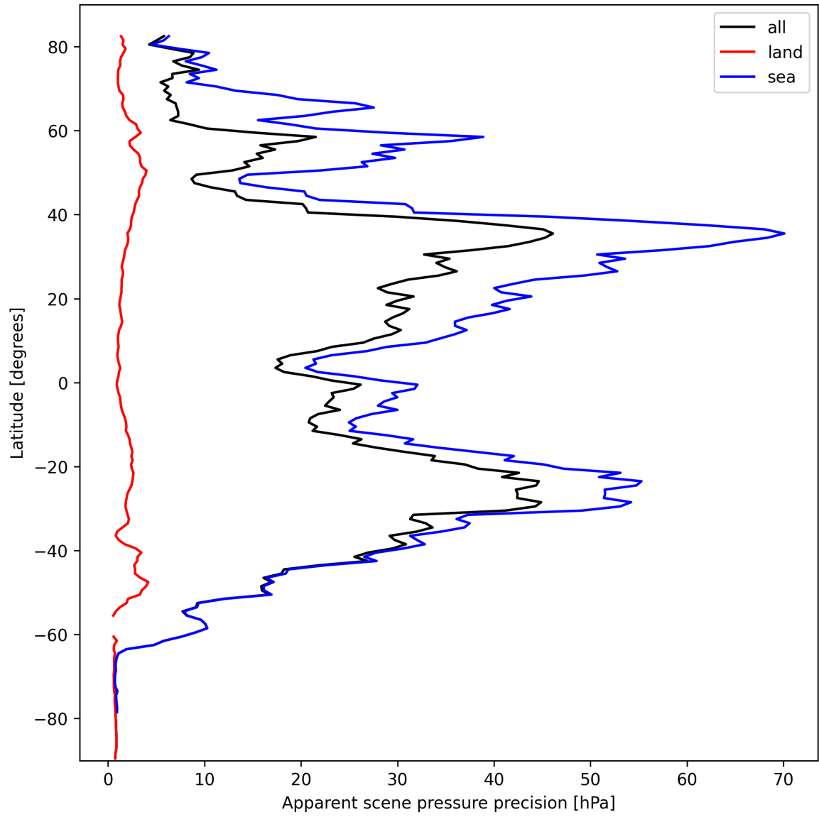
Figure 20: Zonal average of “Apparent scene pressure precision” for 2024-10-06 to 2024-10-08.
