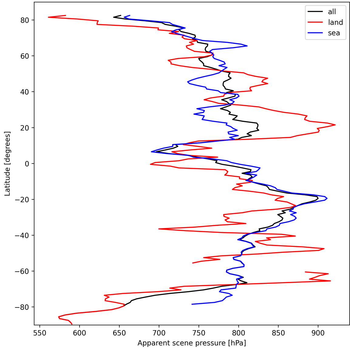
Figure 19: Zonal average of “Apparent scene pressure” for 2024-10-06 to 2024-10-08.
