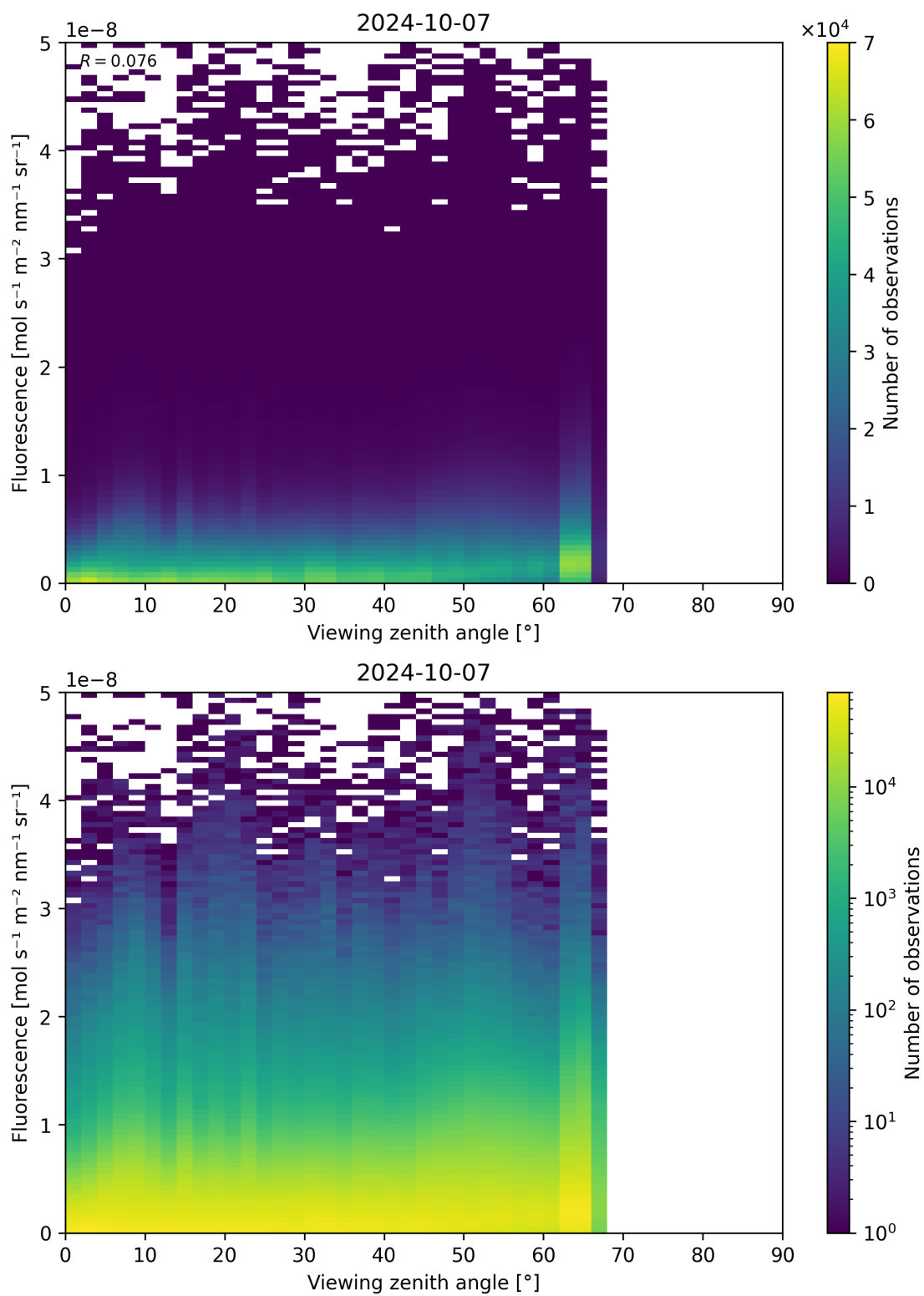
Figure 134: Scatter density plot of “Viewing zenith angle” against “Fluorescence” for 2024-10-06 to 2024-10-08.
