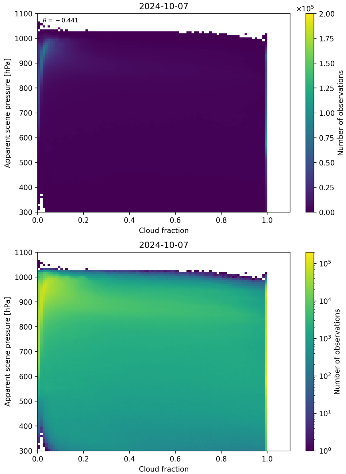
Figure 76: Scatter density plot of “Cloud fraction” against “Apparent scene pressure” for 2024-10-06 to 2024-10-08.
