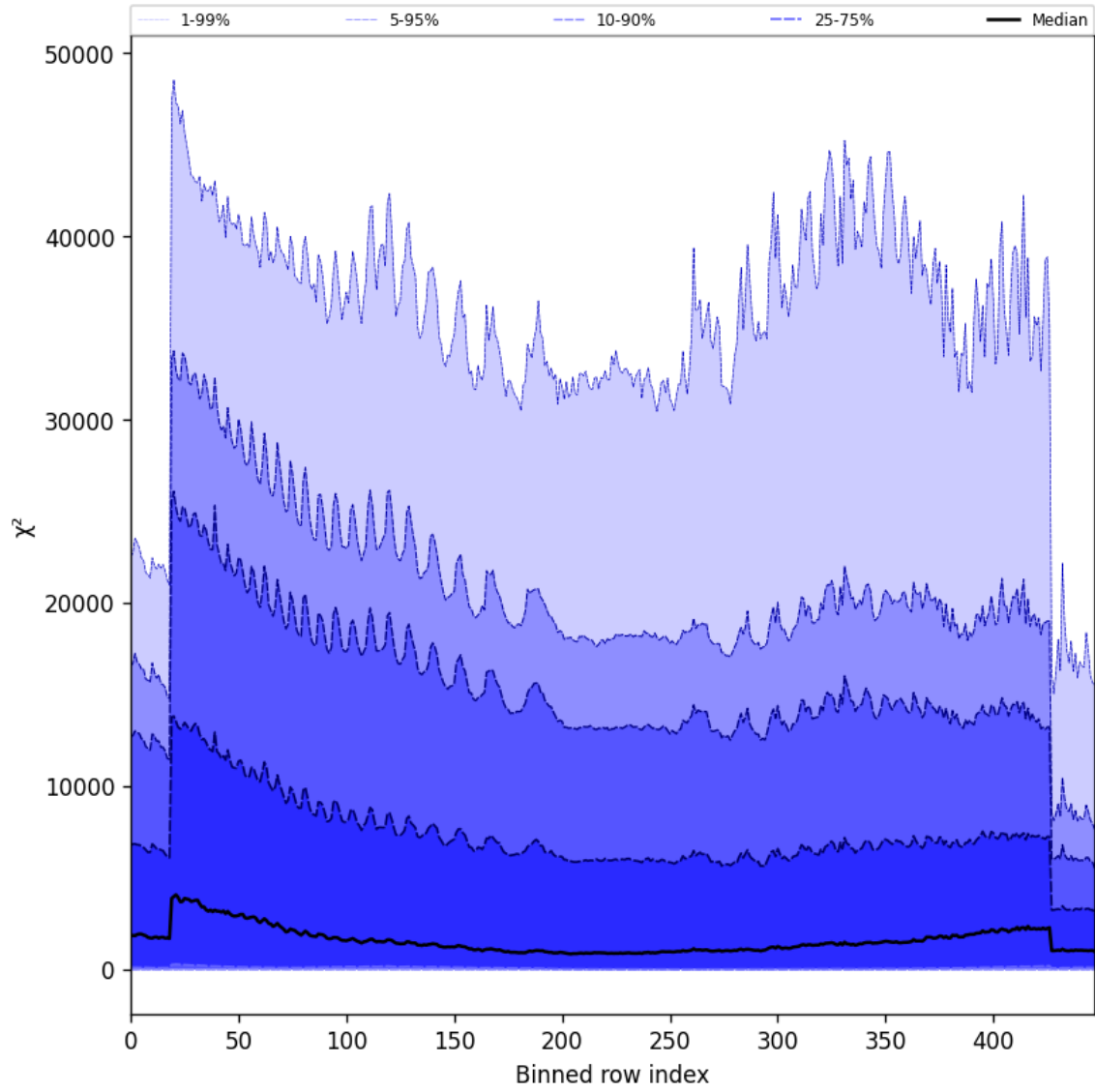
Figure 55: Along track statistics of “ \chi^2 ” for 2024-10-06 to 2024-10-08
