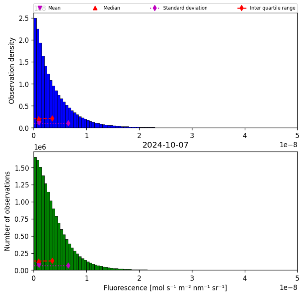
Figure 40: Histogram of “Fluorescence” for 2024-10-06 to 2024-10-08
