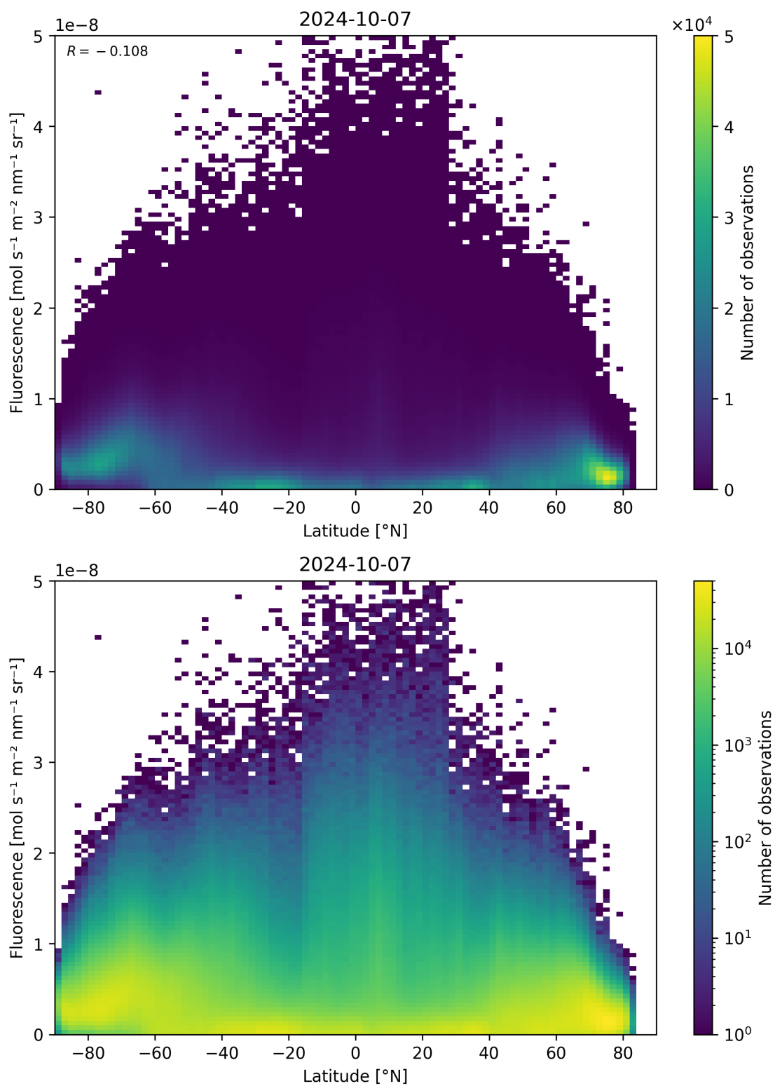
Figure 101: Scatter density plot of “Latitude” against “Fluorescence” for 2024-10-06 to 2024-10-08.
