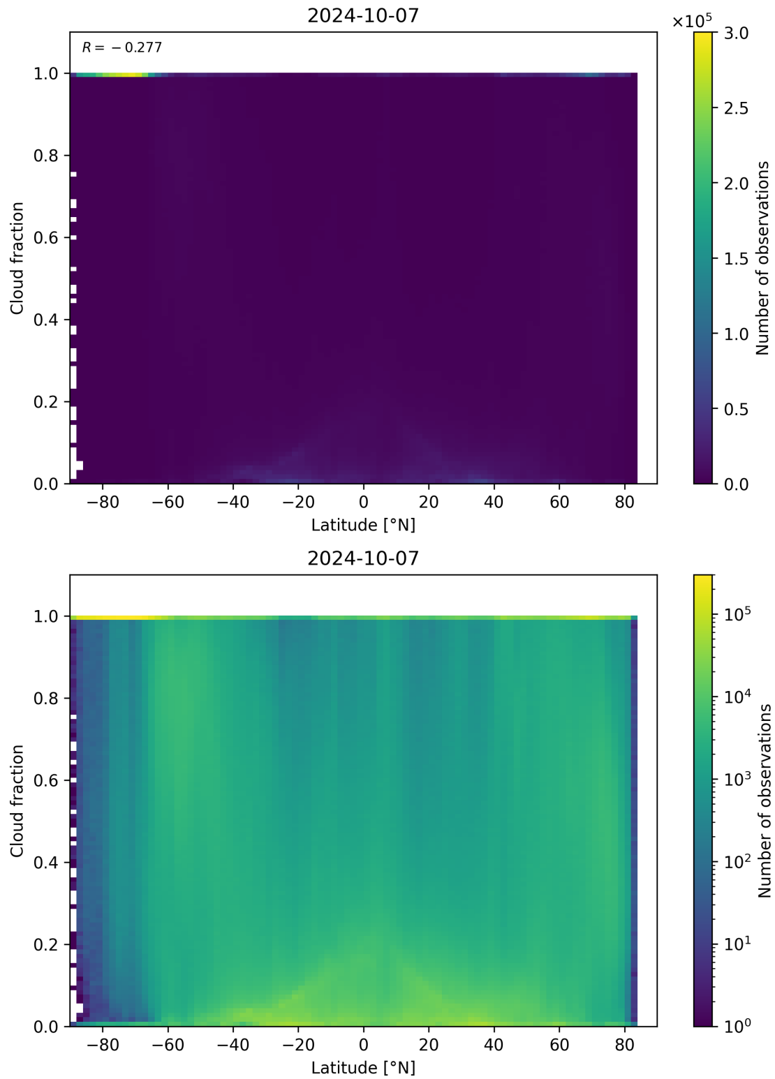
Figure 99: Scatter density plot of “Latitude” against “Cloud fraction” for 2024-10-06 to 2024-10-08.
