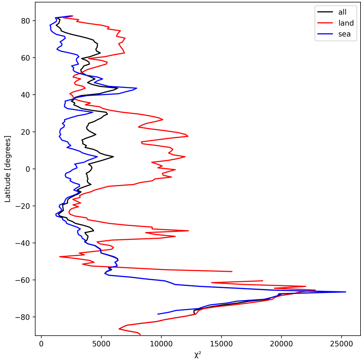
Figure 21: Zonal average of “ \chi^2 ” for 2024-10-06 to 2024-10-08.
