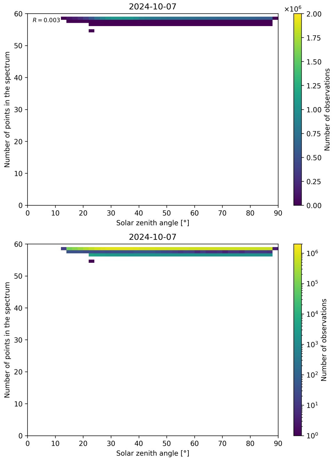
Figure 126: Scatter density plot of “Solar zenith angle” against “Number of points in the spectrum” for 2024-10-06 to 2024-10-08.
