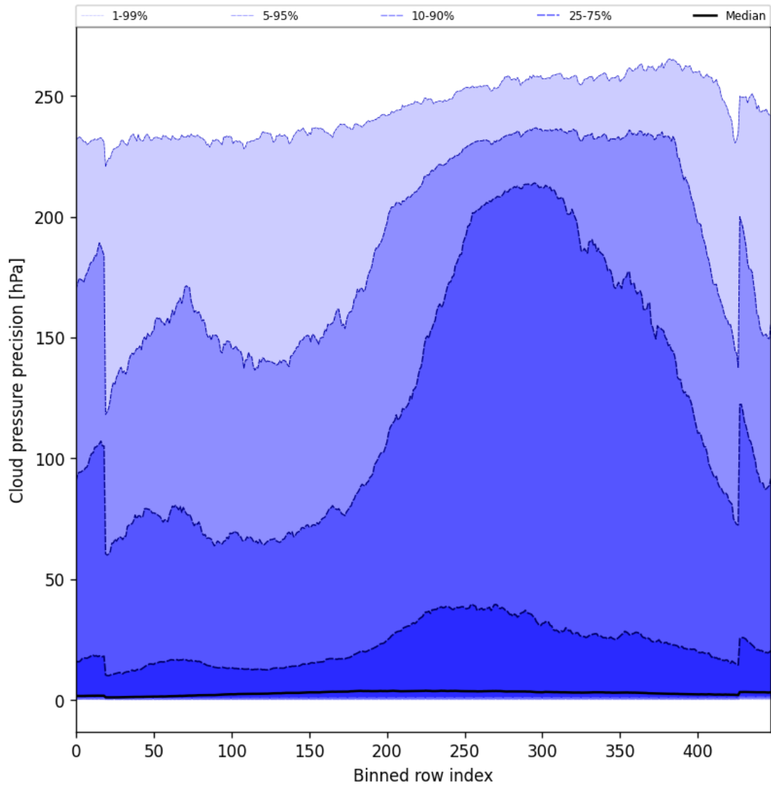
Figure 48: Along track statistics of “Cloud pressure precision” for 2024-10-06 to 2024-10-08
