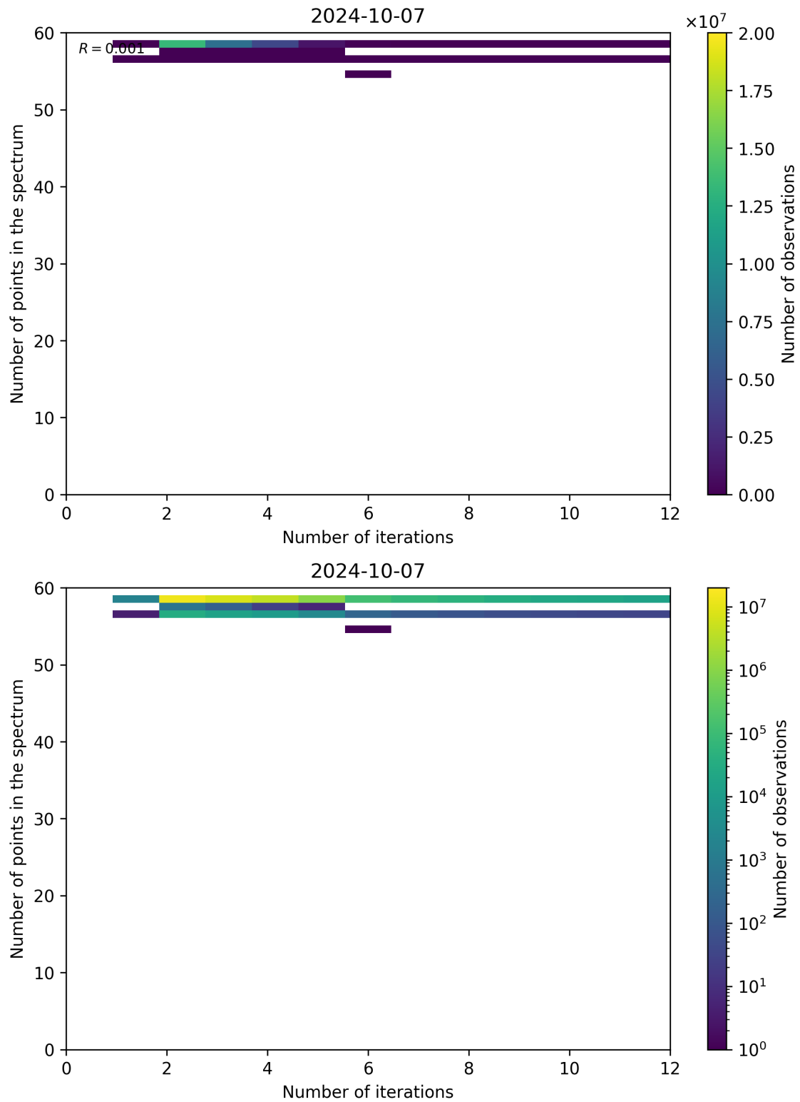
Figure 108: Scatter density plot of “Number of iterations” against “Number of points in the spectrum” for 2024-10-06 to 2024-10-08.
