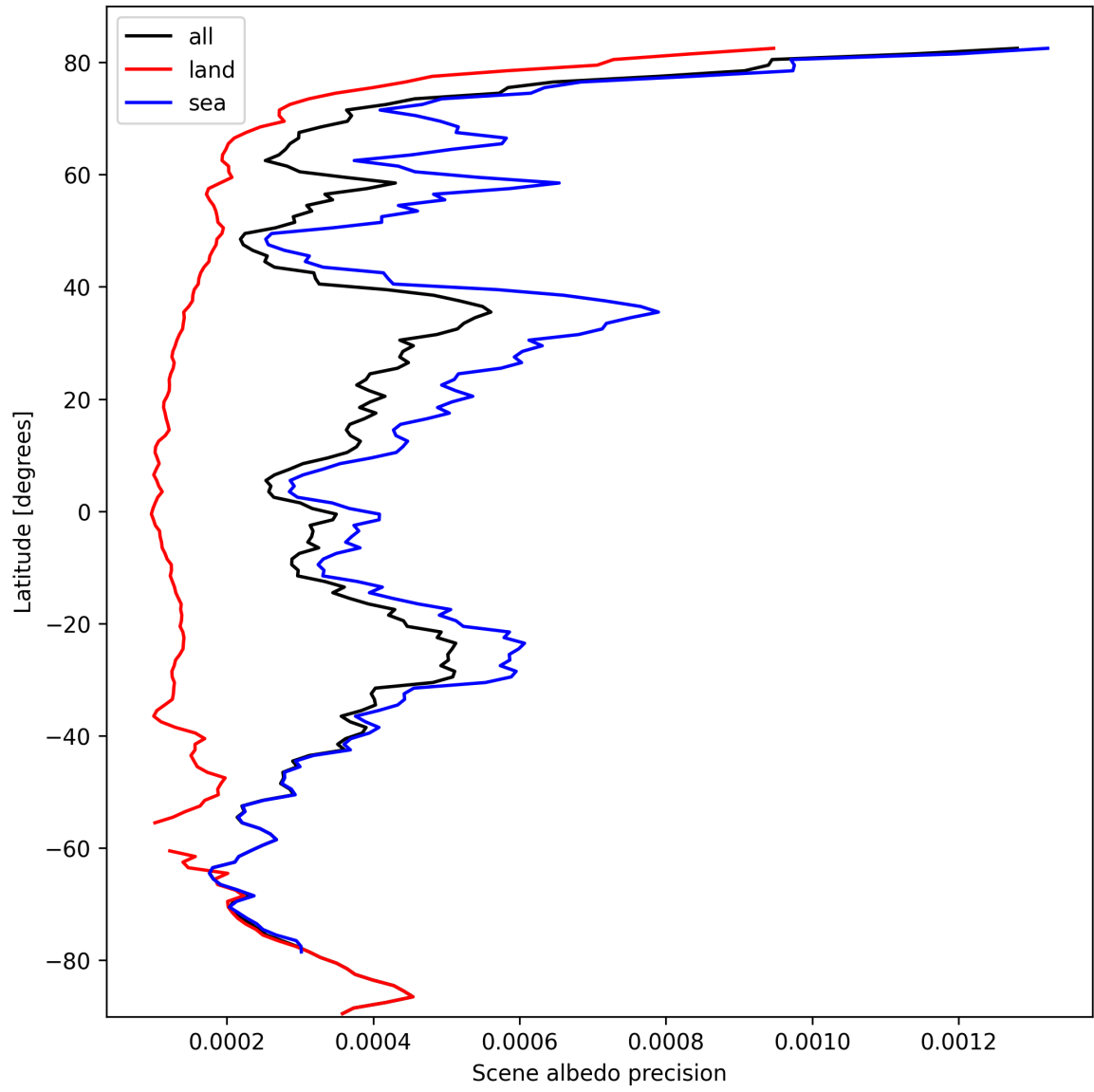
Figure 18: Zonal average of "Scene albedo precision" for 2024-10-06 to 2024-10-08.
