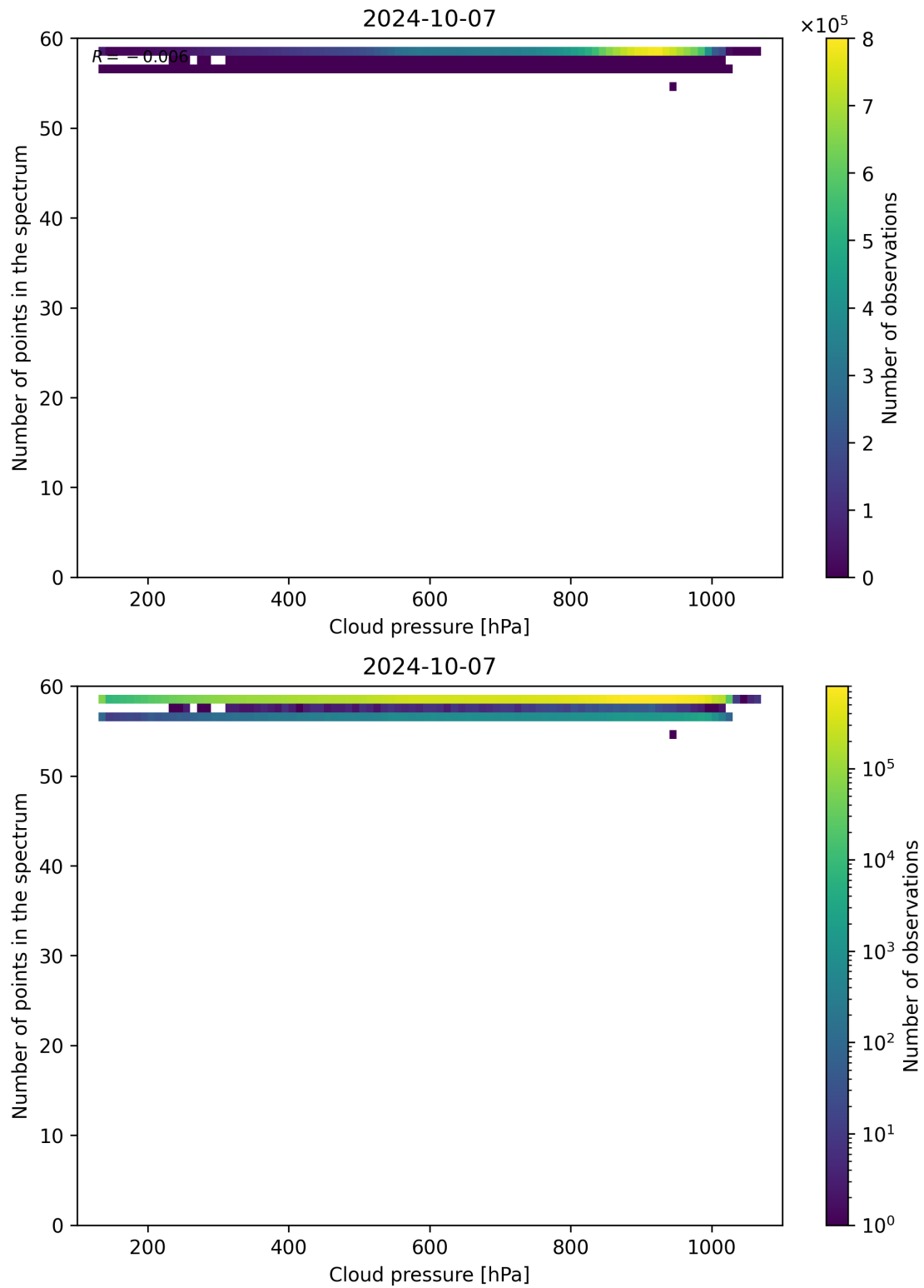
Figure 90: Scatter density plot of “Cloud pressure” against “Number of points in the spectrum” for 2024-10-06 to 2024-10-08.
