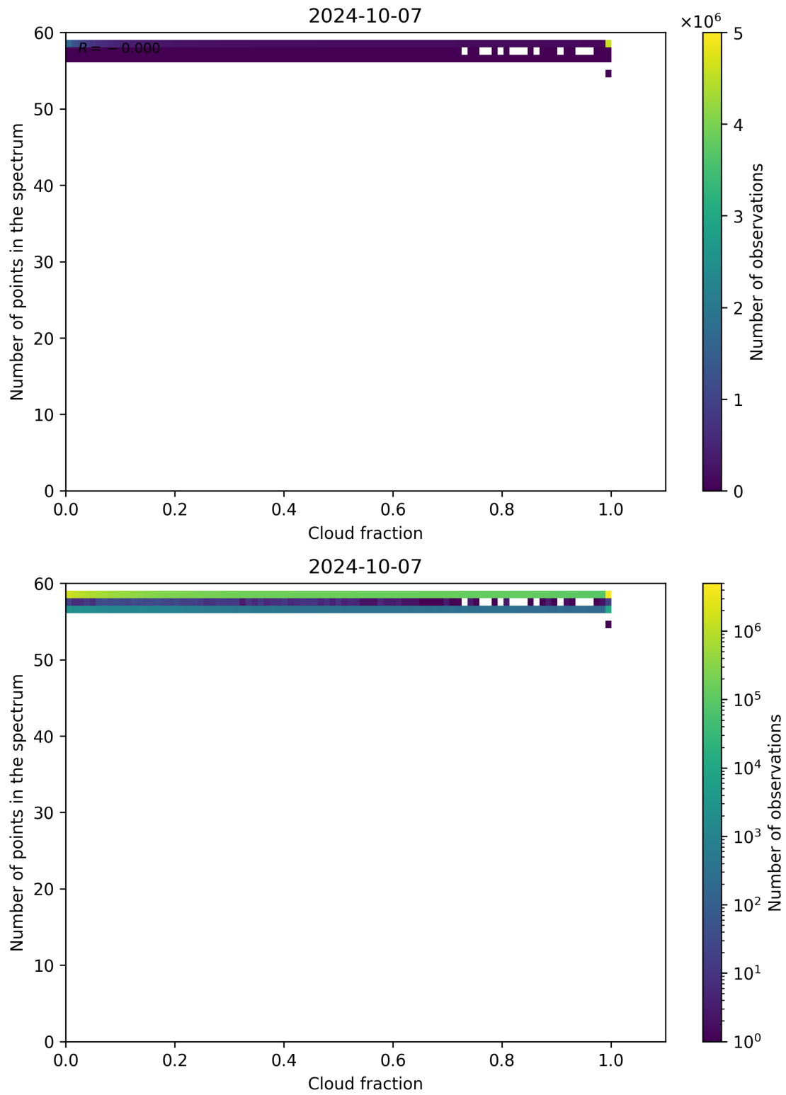
Figure 81: Scatter density plot of “Cloud fraction” against “Number of points in the spectrum” for 2024-10-06 to 2024-10-08.
