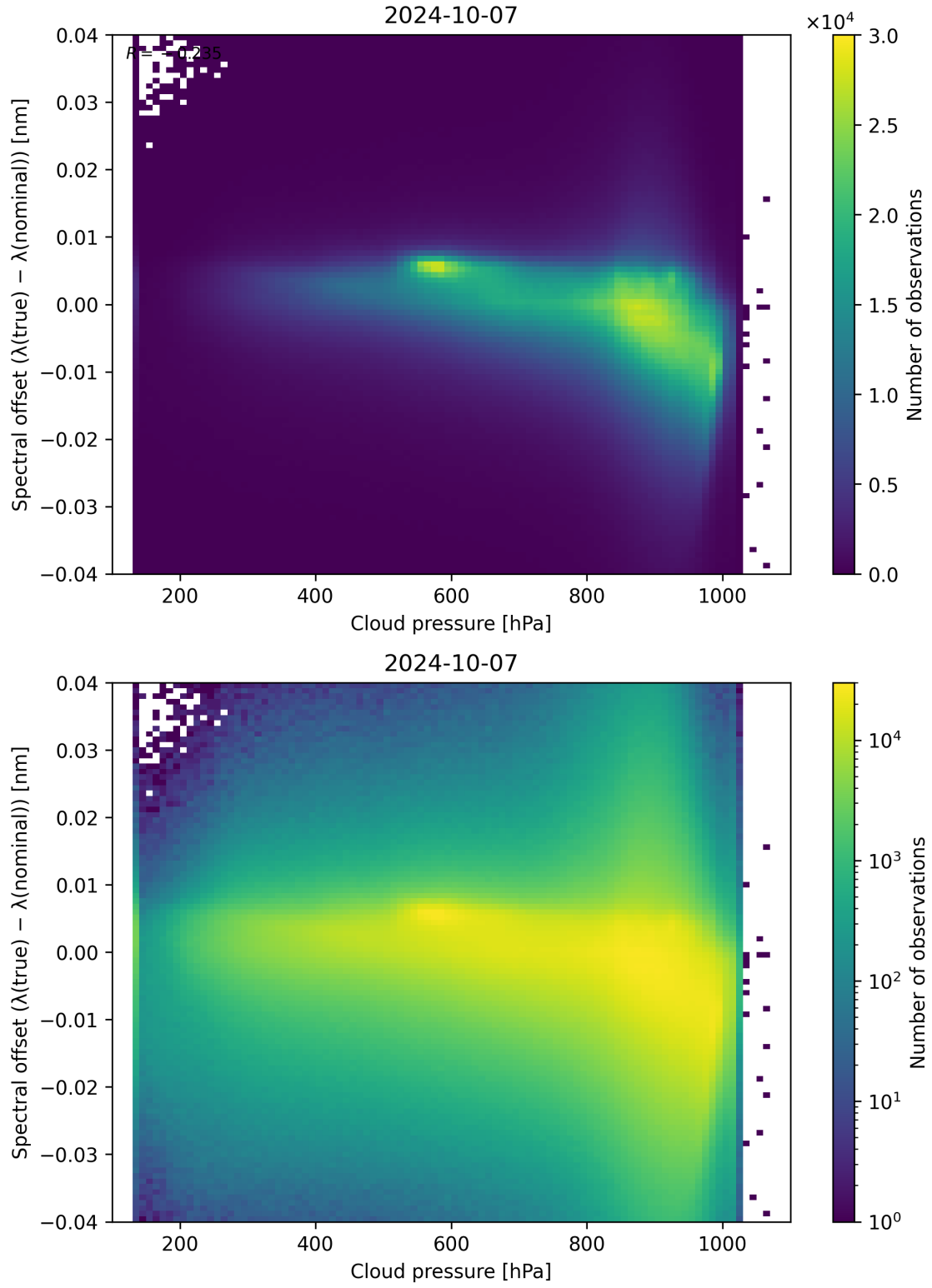
Figure 92: Scatter density plot of “Cloud pressure” against “Spectral offset ( \lambda_{\text{true}} - \lambda_{\text{nominal}} )” for 2024-10-06 to 2024-10-08.
