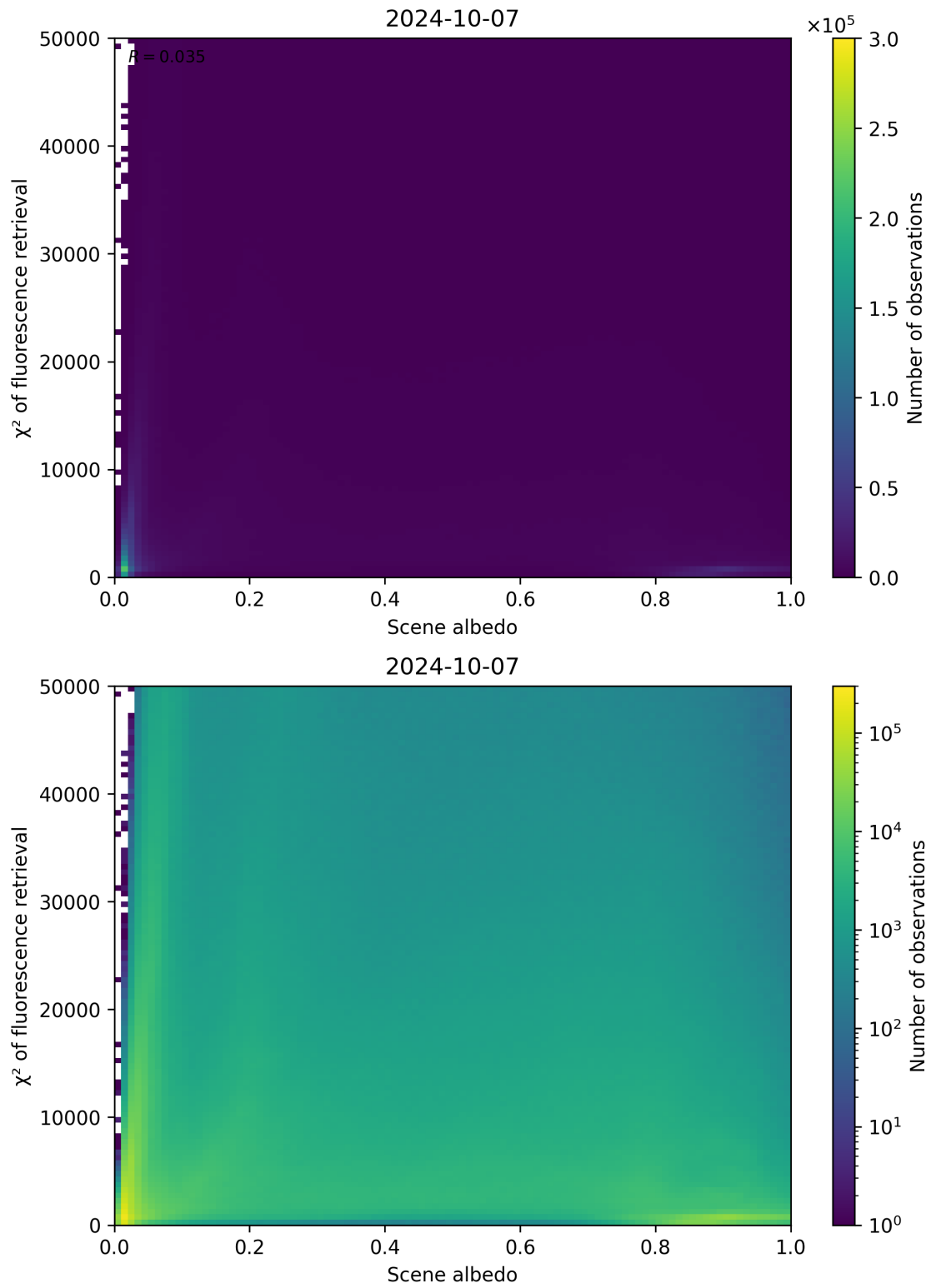
Figure 113: Scatter density plot of “Scene albedo” against “ \chi^2 of fluorescence retrieval” for 2024-10-06 to 2024-10-08.
