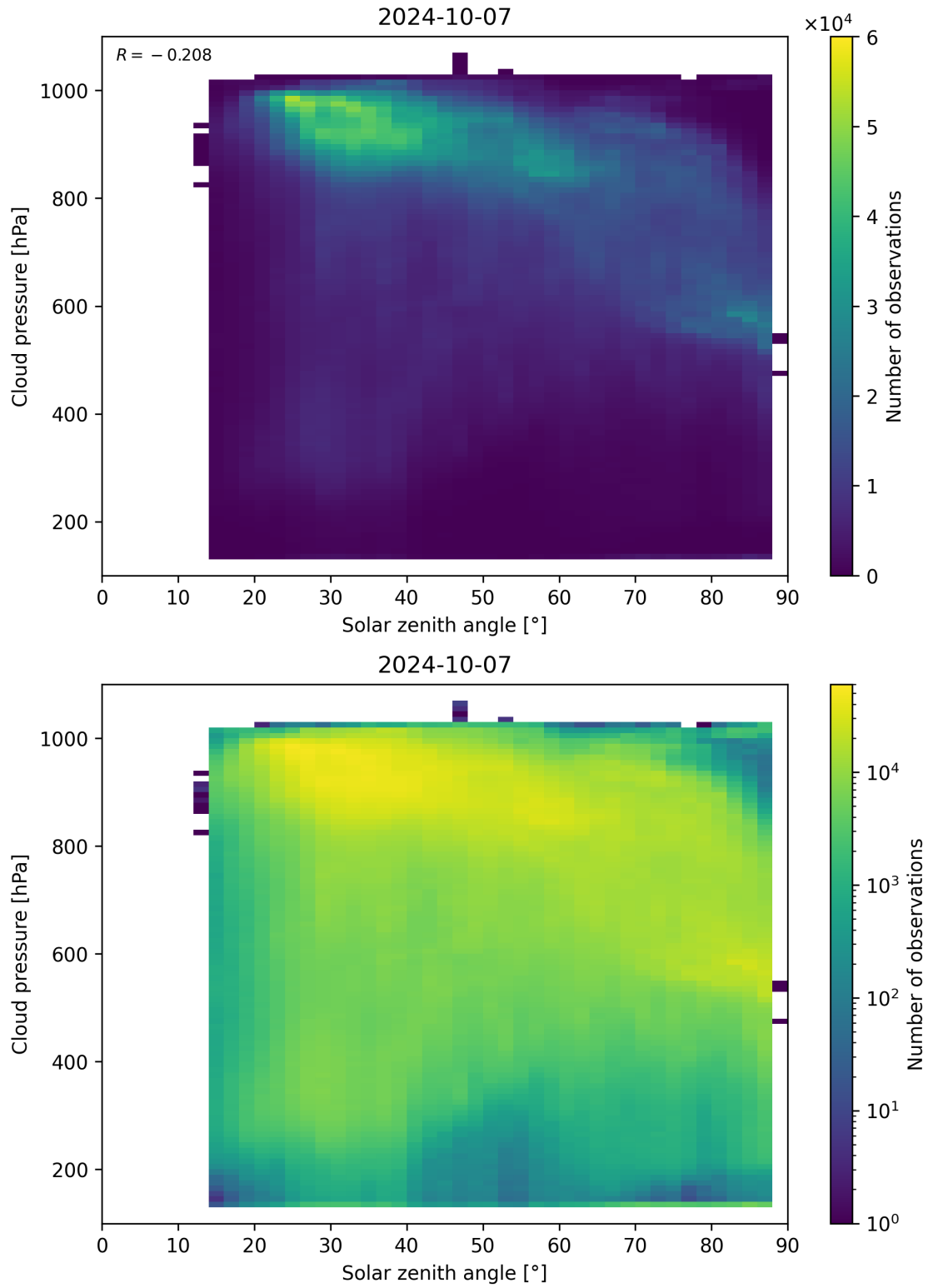
Figure 122: Scatter density plot of “Solar zenith angle” against “Cloud pressure” for 2024-10-06 to 2024-10-08.
