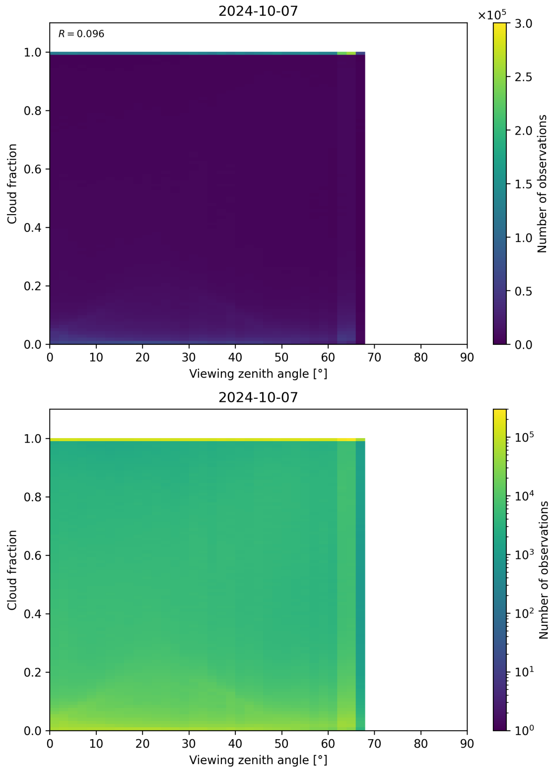
Figure 132: Scatter density plot of “Viewing zenith angle” against “Cloud fraction” for 2024-10-06 to 2024-10-08.
