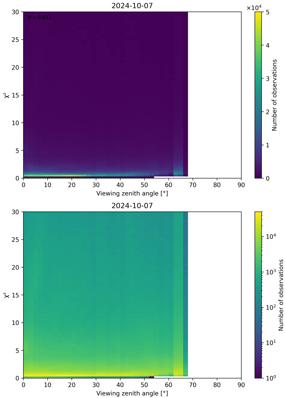
Figure 130: Scatter density plot of “Viewing zenith angle” against “ \chi^2 ” for 2024-10-06 to 2024-10-08.
