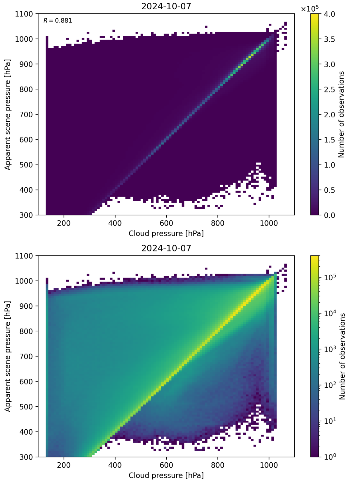
Figure 84: Scatter density plot of “Cloud pressure” against “Apparent scene pressure” for 2024-10-06 to 2024-10-08.
