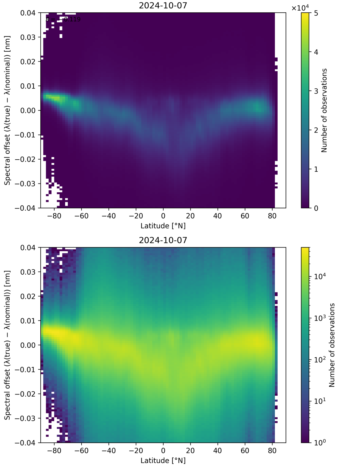
Figure 105: Scatter density plot of “Latitude” against “Spectral offset ( \lambda_{\text{true}} - \lambda_{\text{nominal}} )” for 2024-10-06 to 2024-10-08.
