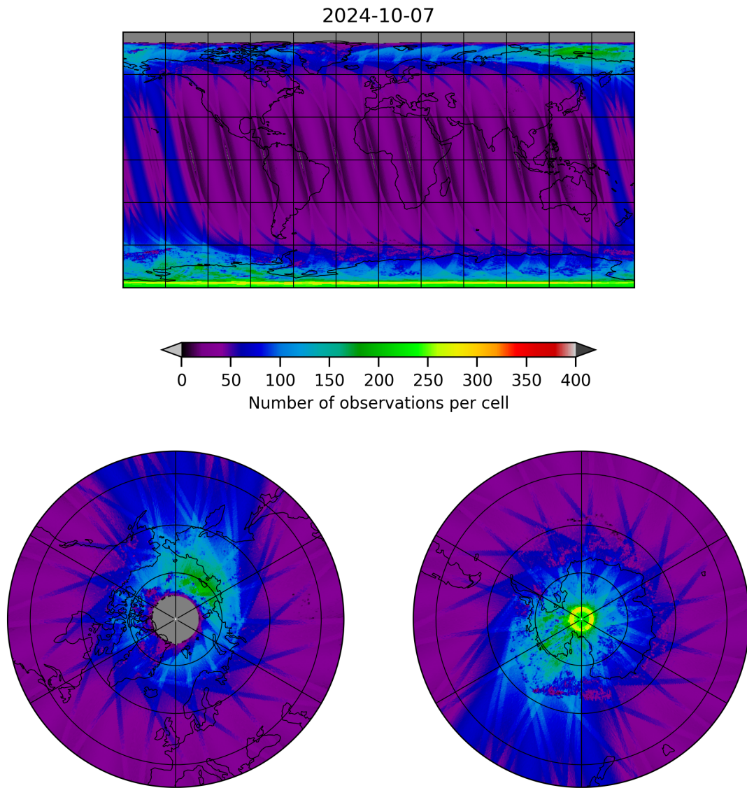
Figure 11: Map of the number of observations for 2024-10-06 to 2024-10-08
