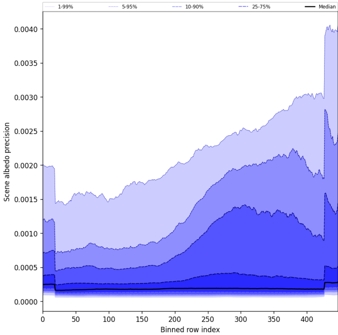
Figure 52: Along track statistics of “Scene albedo precision” for 2024-10-06 to 2024-10-08
