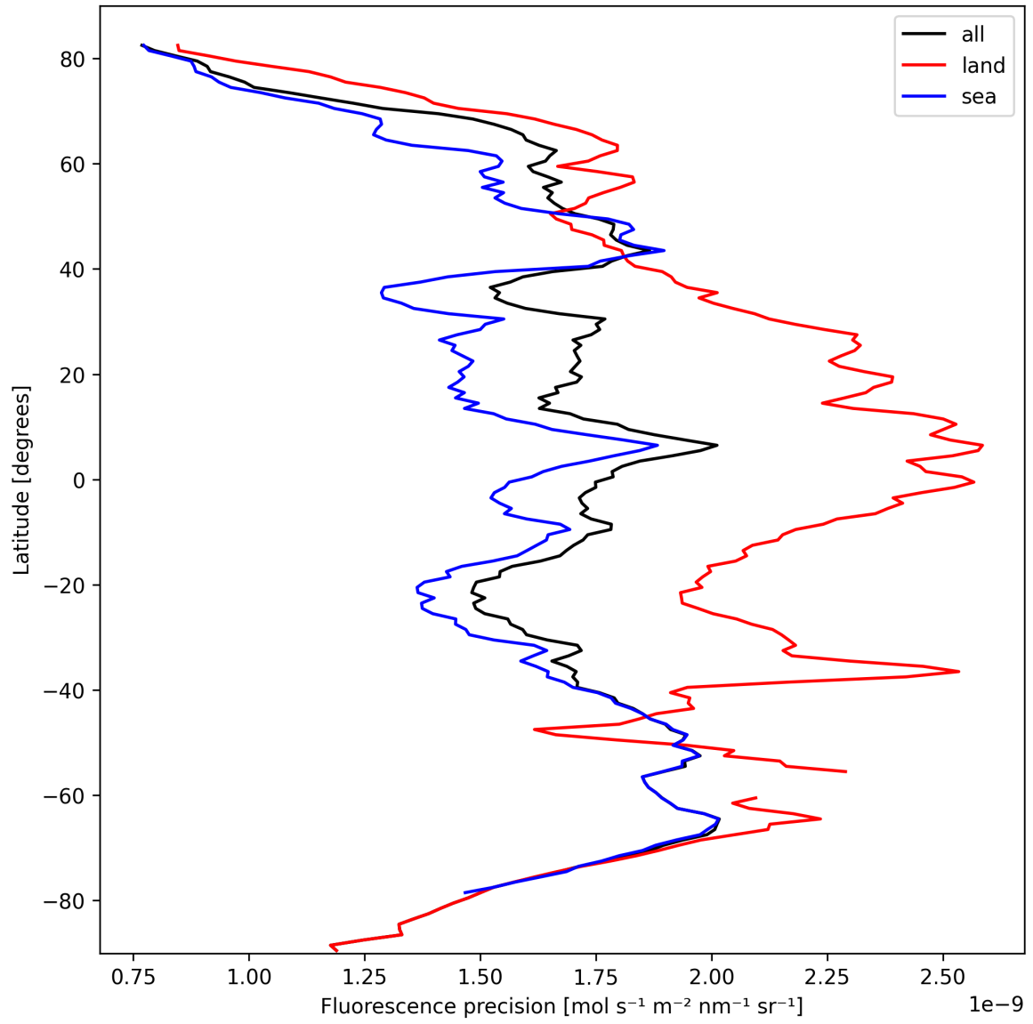
Figure 24: Zonal average of “Fluorescence precision” for 2024-10-06 to 2024-10-08.
