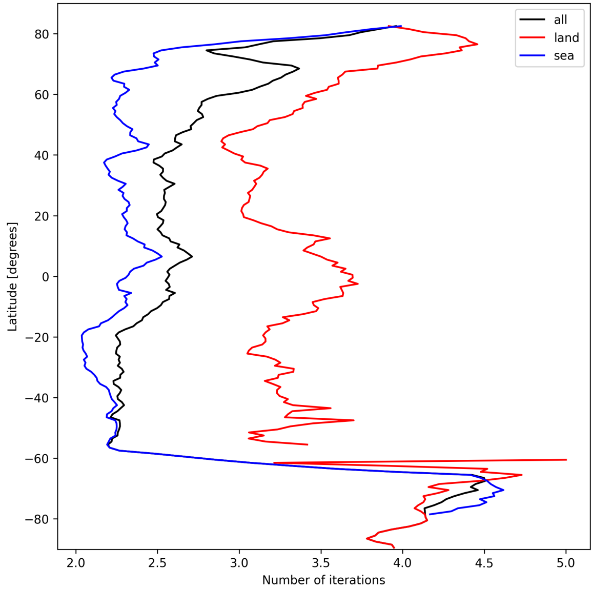
Figure 22: Zonal average of “Number of iterations” for 2024-10-06 to 2024-10-08.
