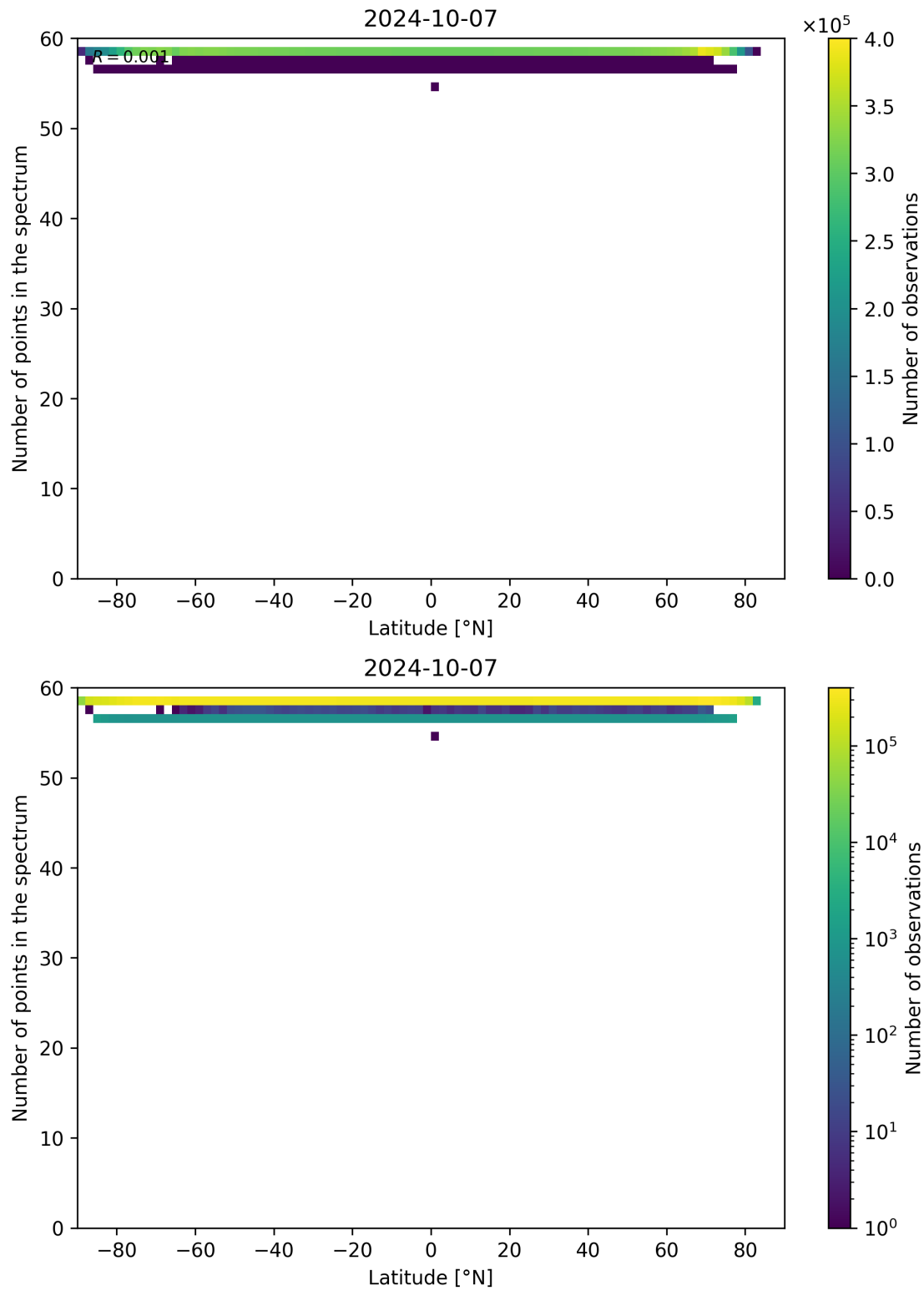
Figure 103: Scatter density plot of “Latitude” against “Number of points in the spectrum” for 2024-10-06 to 2024-10-08.
