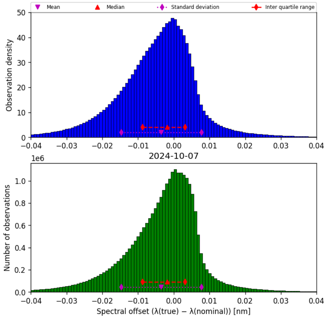
Figure 45: Histogram of “Spectral offset ( \lambda_{\text{true}} - \lambda_{\text{nominal}} )” for 2024-10-06 to 2024-10-08
