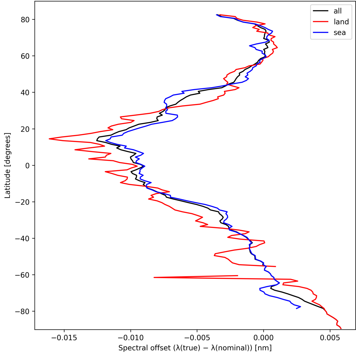
Figure 28: Zonal average of “Spectral offset ( \lambda_{\text{true}} - \lambda_{\text{nominal}} )” for 2024-10-06 to 2024-10-08.
