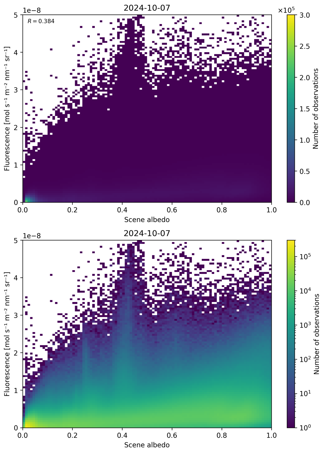
Figure 114: Scatter density plot of “Scene albedo” against “Fluorescence” for 2024-10-06 to 2024-10-08.
