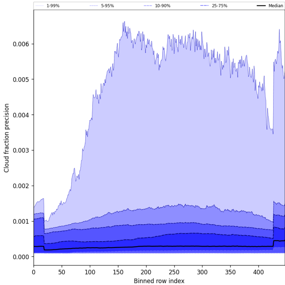
Figure 50: Along track statistics of “Cloud fraction precision” for 2024-10-06 to 2024-10-08
