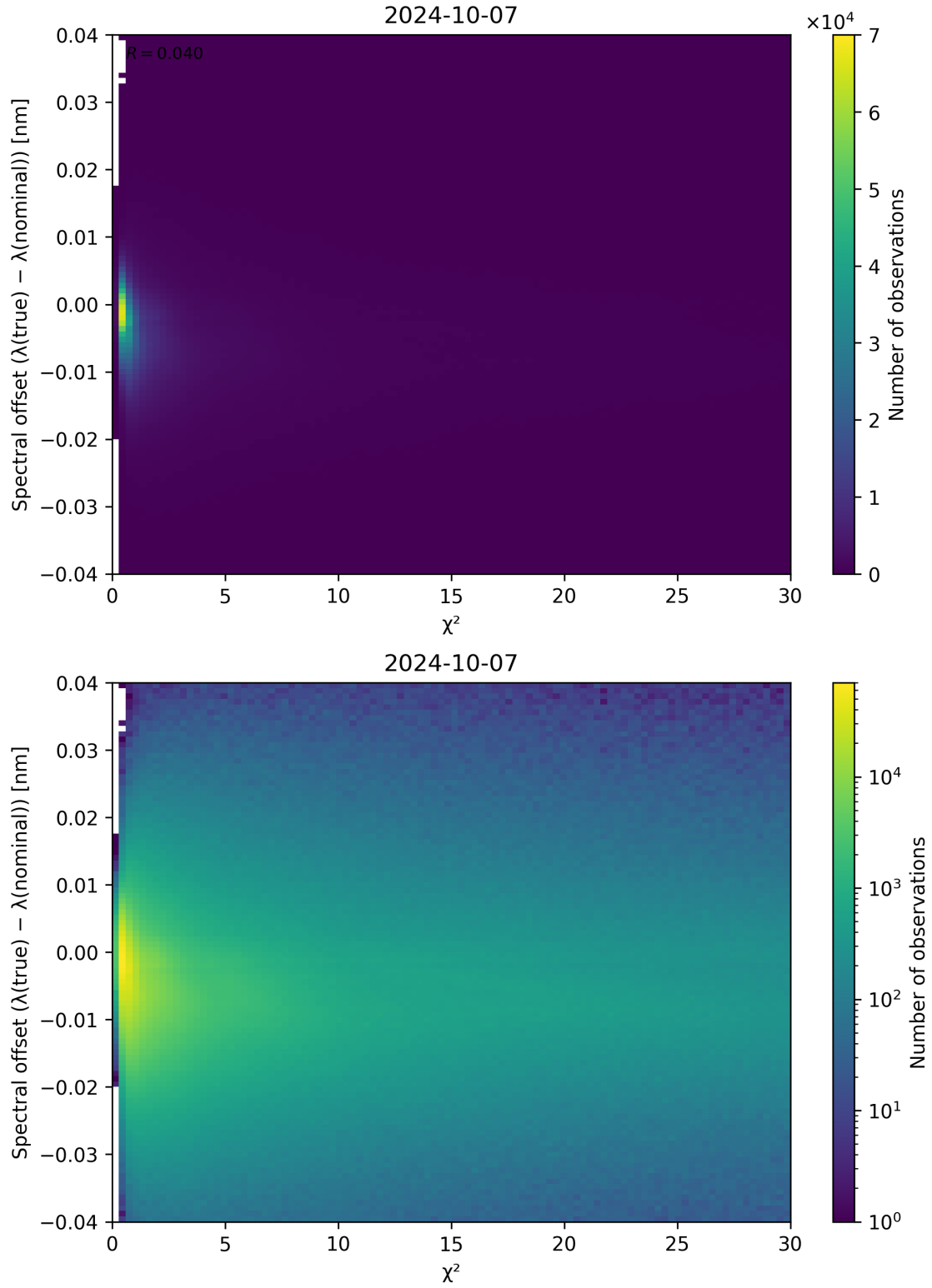
Figure 75: Scatter density plot of “ \chi^2 ” against “Spectral offset ( \lambda_{\text{true}} - \lambda_{\text{nominal}} )” for 2024-10-06 to 2024-10-08.
