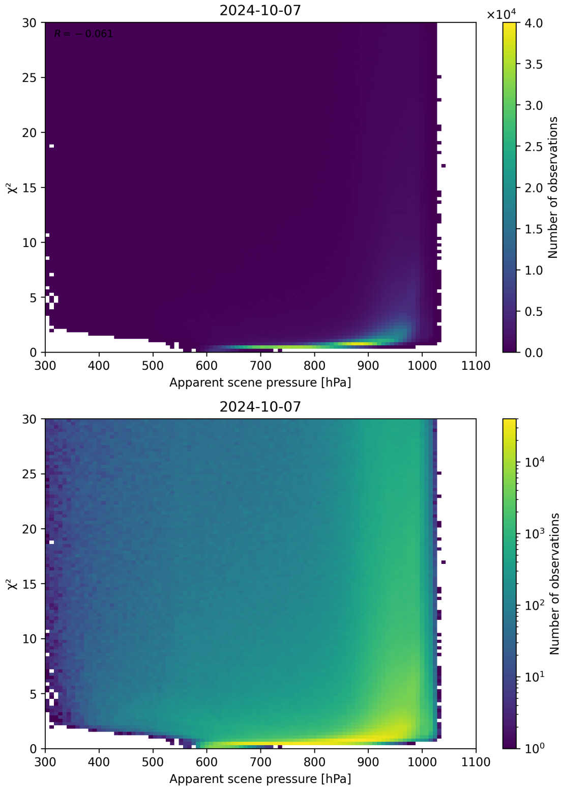
Figure 63: Scatter density plot of “Apparent scene pressure” against “ \chi^2 ” for 2024-10-06 to 2024-10-08.
