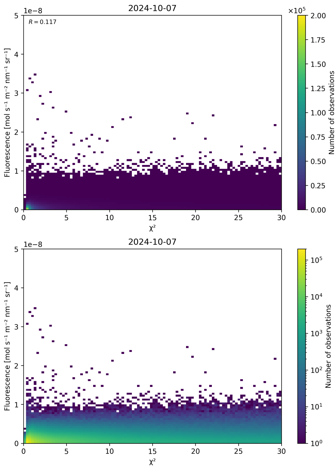
Figure 70: Scatter density plot of “ \chi^2 ” against “Fluorescence” for 2024-10-06 to 2024-10-08.
