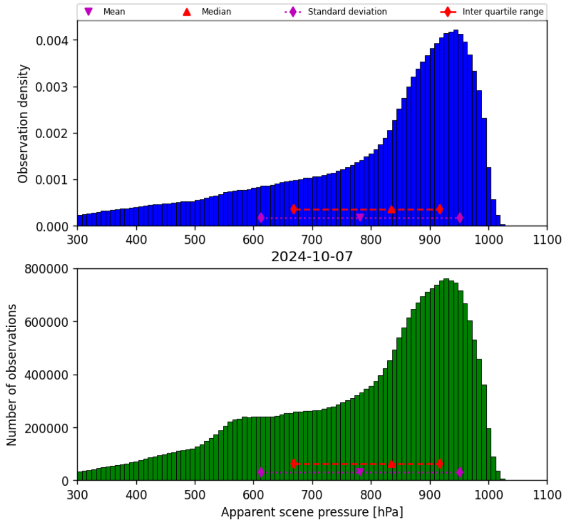
Figure 36: Histogram of “Apparent scene pressure” for 2024-10-06 to 2024-10-08
