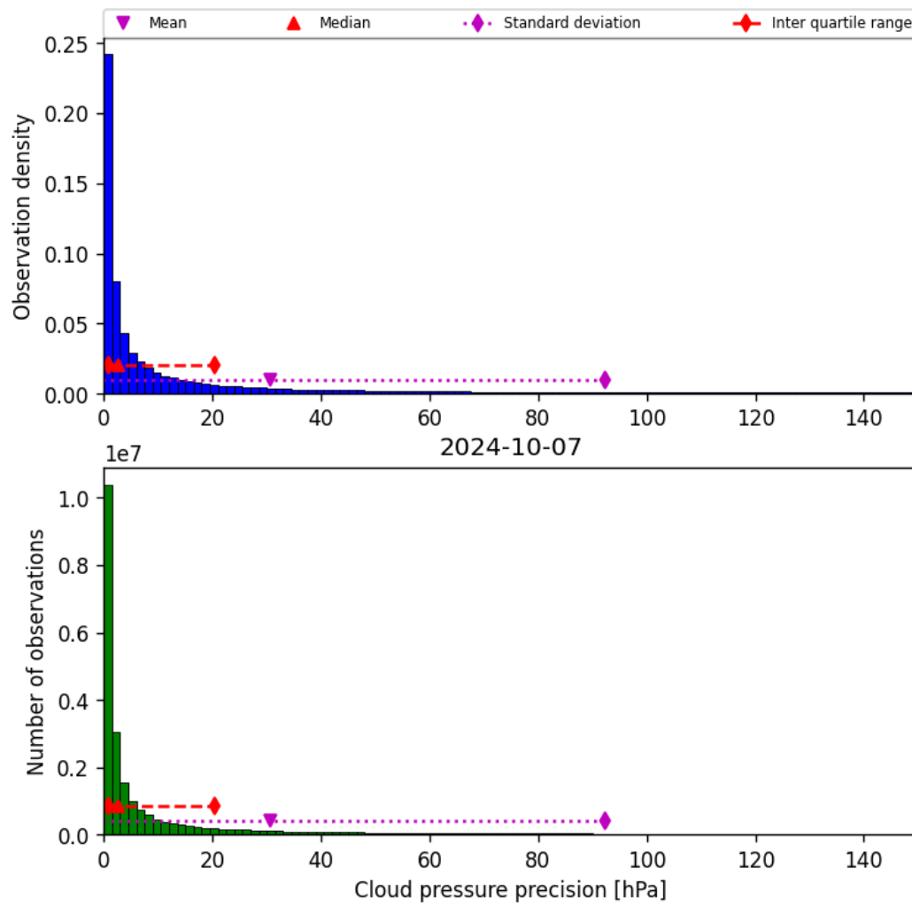
Figure 31: Histogram of “Cloud pressure precision” for 2024-10-06 to 2024-10-08
