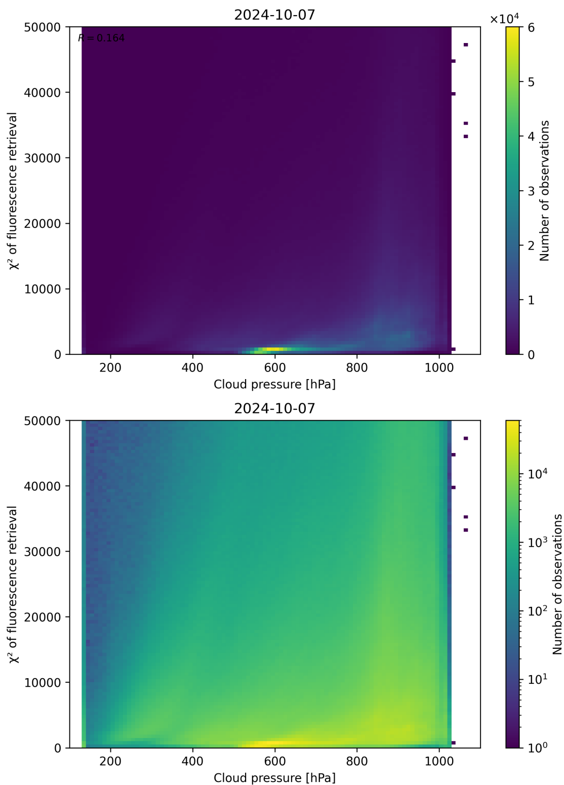
Figure 86: Scatter density plot of “Cloud pressure” against “ \chi^2 of fluorescence retrieval” for 2024-10-06 to 2024-10-08.
