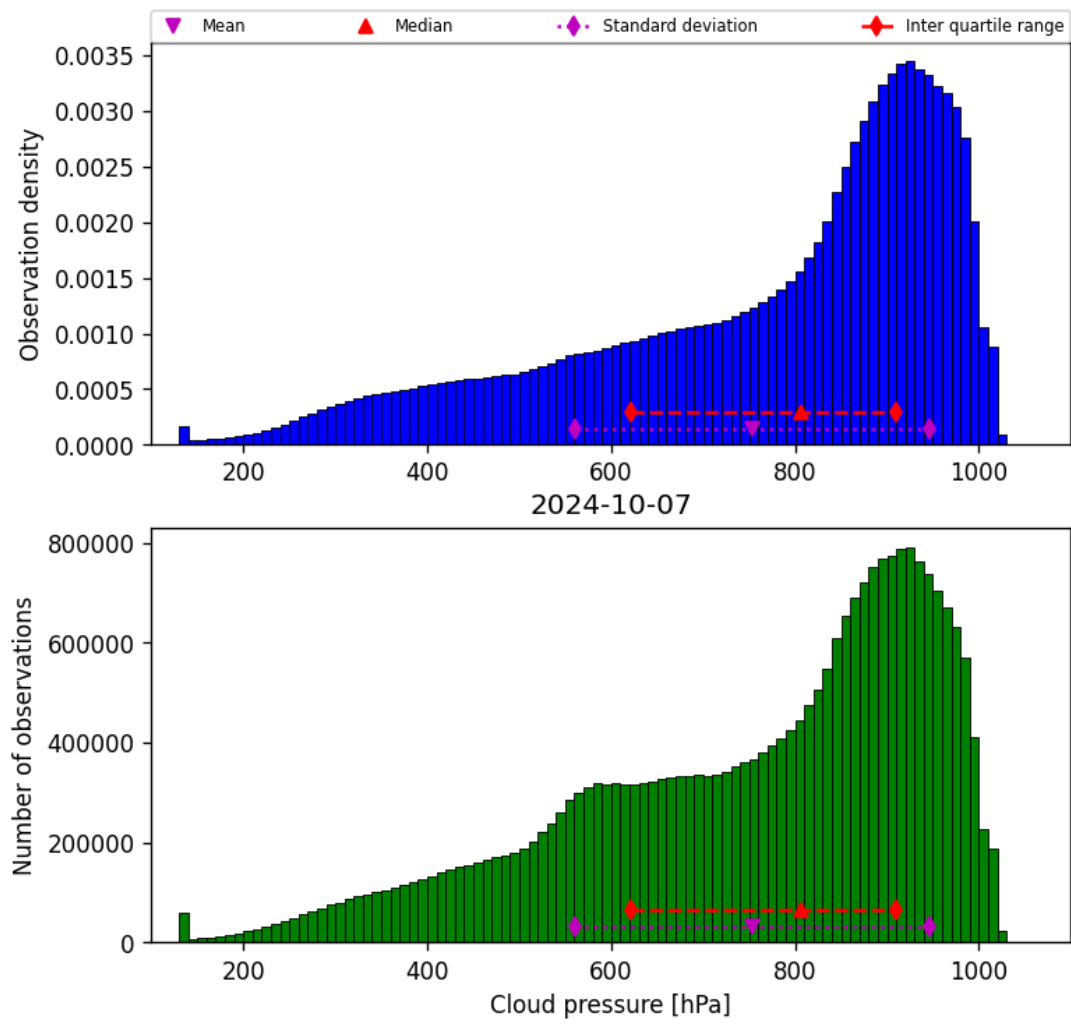
Figure 30: Histogram of “Cloud pressure” for 2024-10-06 to 2024-10-08
