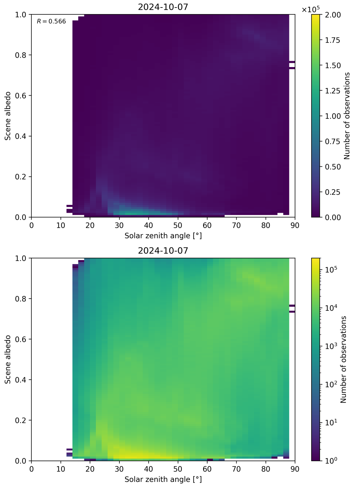
Figure 127: Scatter density plot of “Solar zenith angle” against “Scene albedo” for 2024-10-06 to 2024-10-08.
