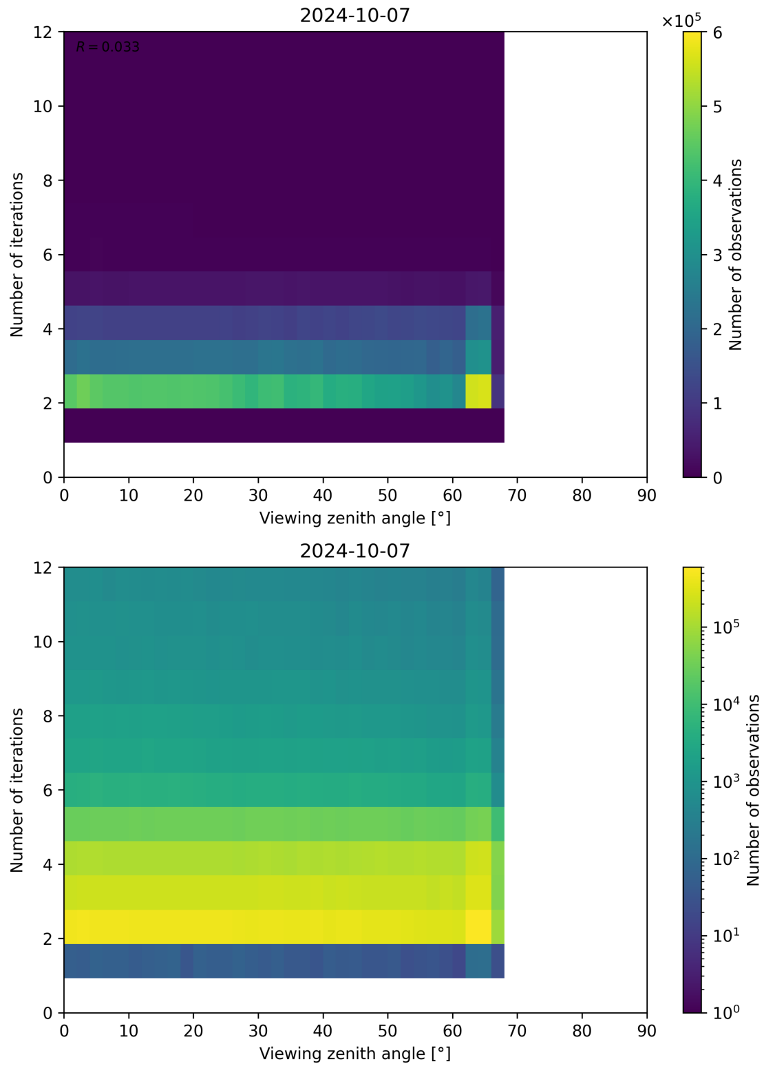
Figure 136: Scatter density plot of “Viewing zenith angle” against “Number of iterations” for 2024-10-06 to 2024-10-08.
