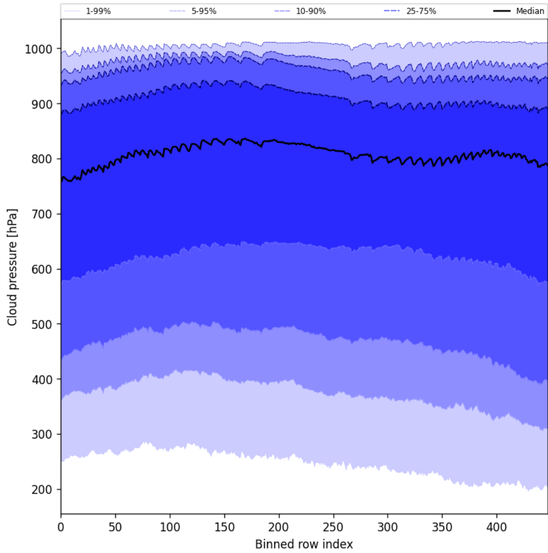
Figure 47: Along track statistics of “Cloud pressure” for 2024-10-06 to 2024-10-08
