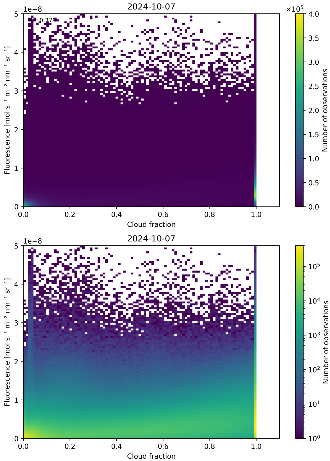
Figure 79: Scatter density plot of “Cloud fraction” against “Fluorescence” for 2024-10-06 to 2024-10-08.
