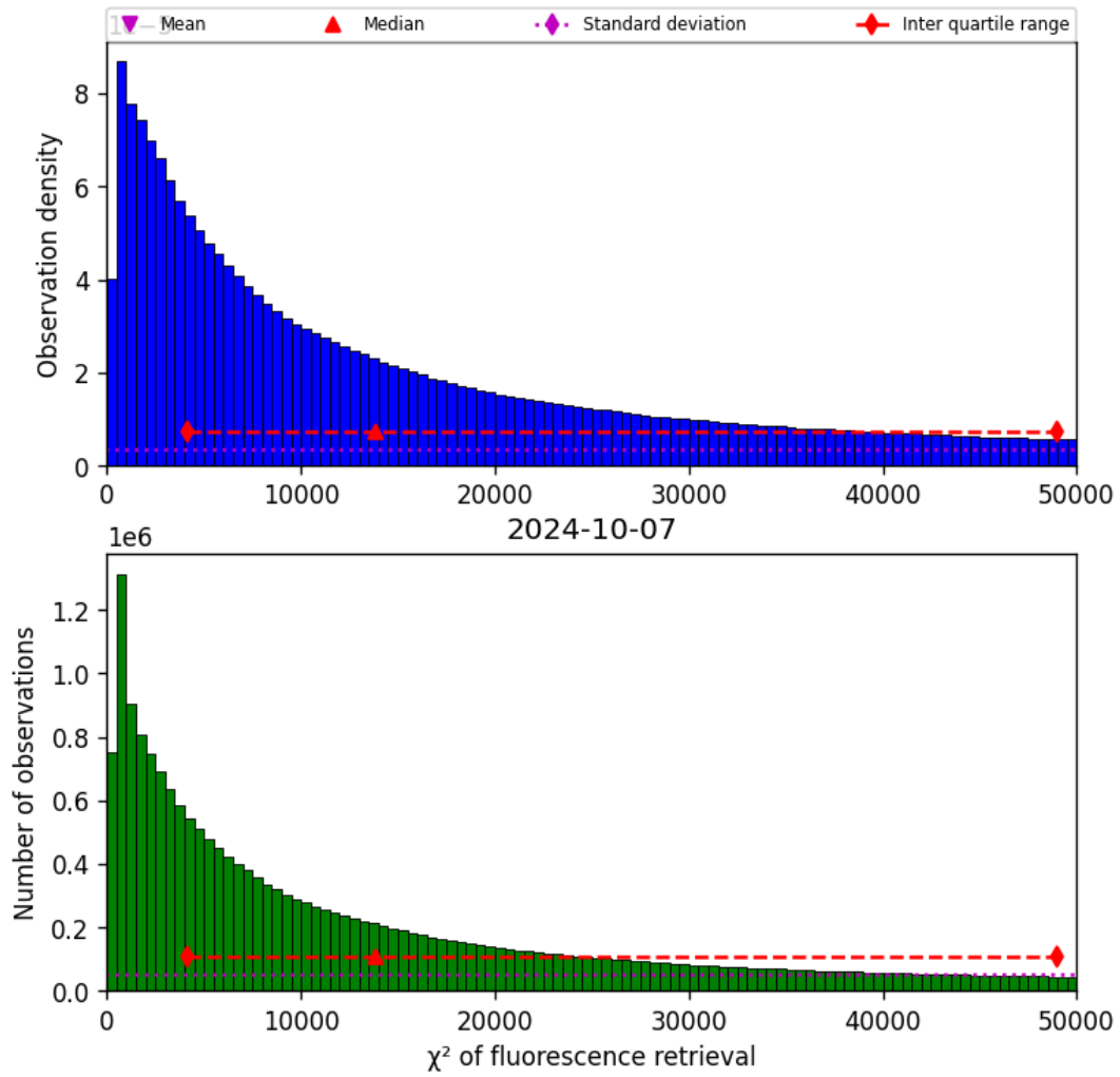
Figure 42: Histogram of “ \chi^2 of fluorescence retrieval” for 2024-10-06 to 2024-10-08
