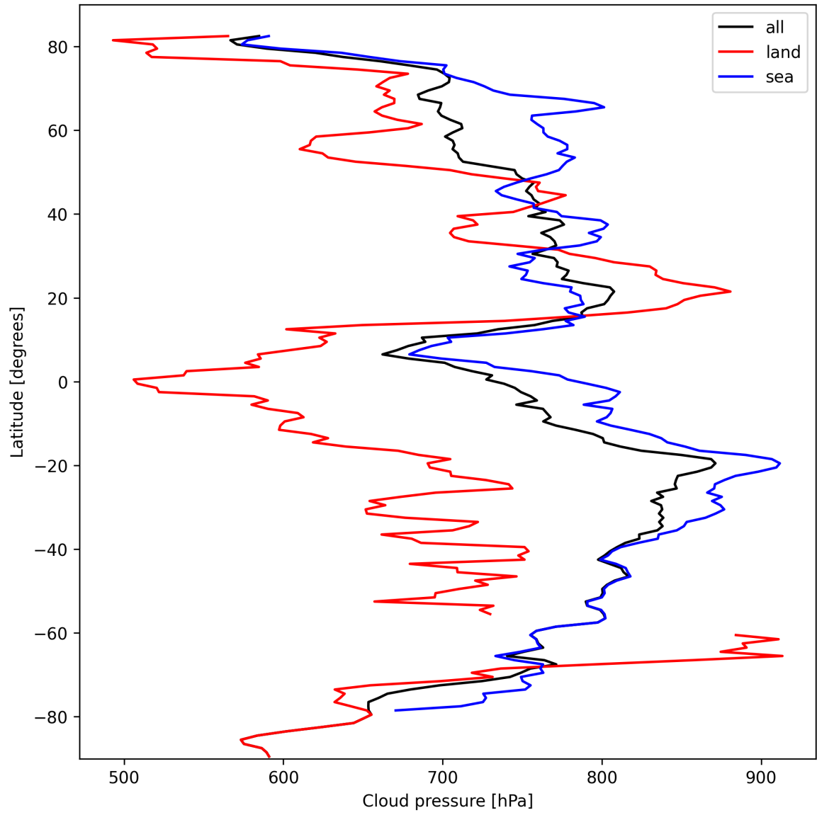
Figure 13: Zonal average of “Cloud pressure” for 2024-10-06 to 2024-10-08.
