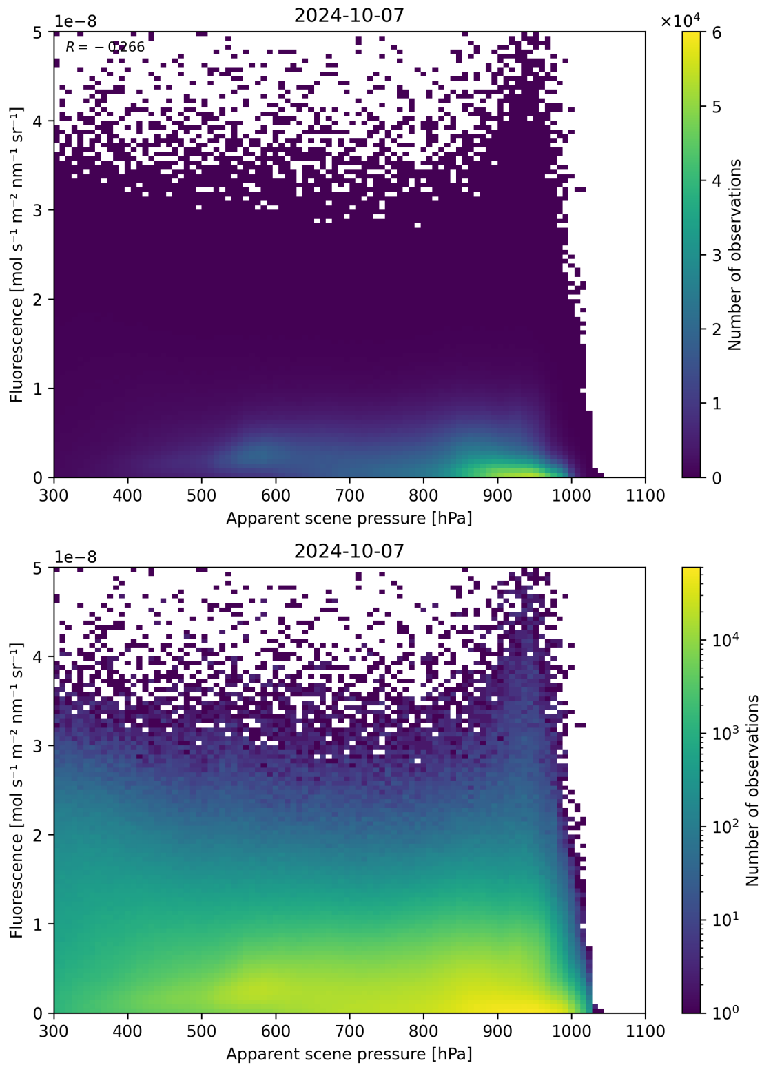
Figure 65: Scatter density plot of “Apparent scene pressure” against “Fluorescence” for 2024-10-06 to 2024-10-08.
