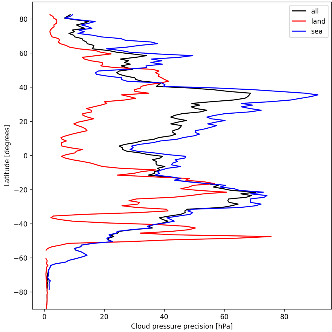
Figure 14: Zonal average of “Cloud pressure precision” for 2024-10-06 to 2024-10-08.
