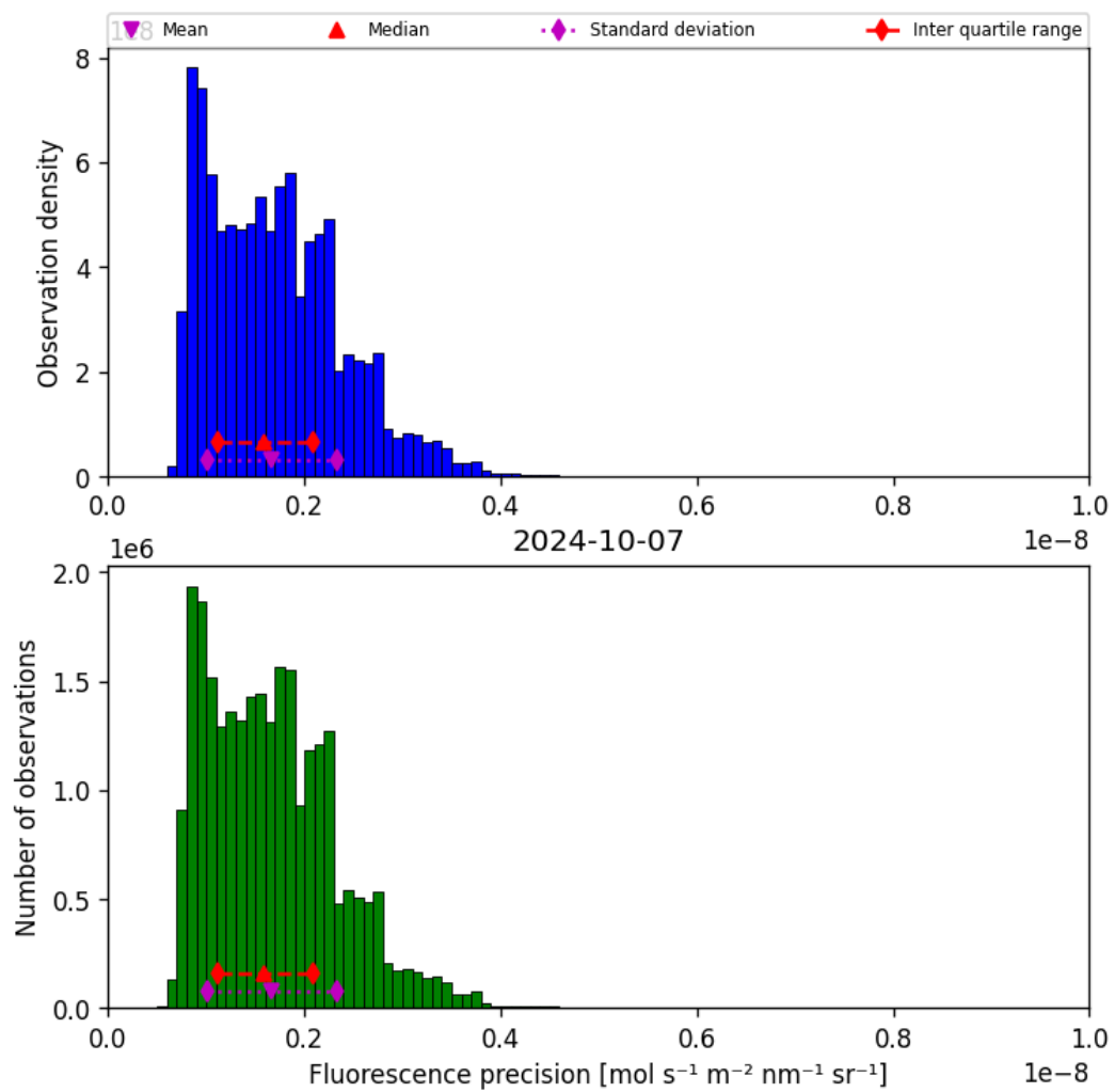
Figure 41: Histogram of “Fluorescence precision” for 2024-10-06 to 2024-10-08
