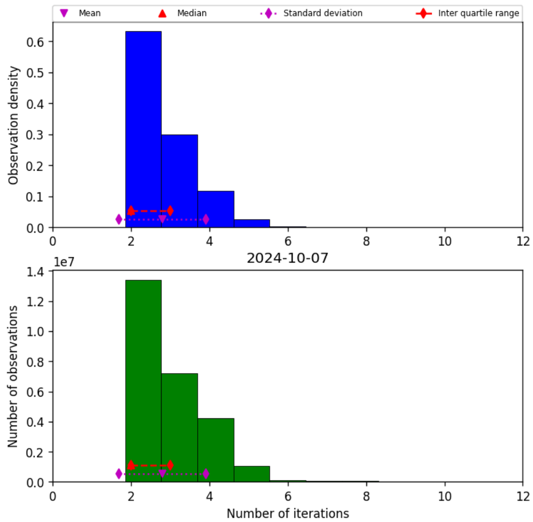
Figure 39: Histogram of “Number of iterations” for 2024-10-06 to 2024-10-08
