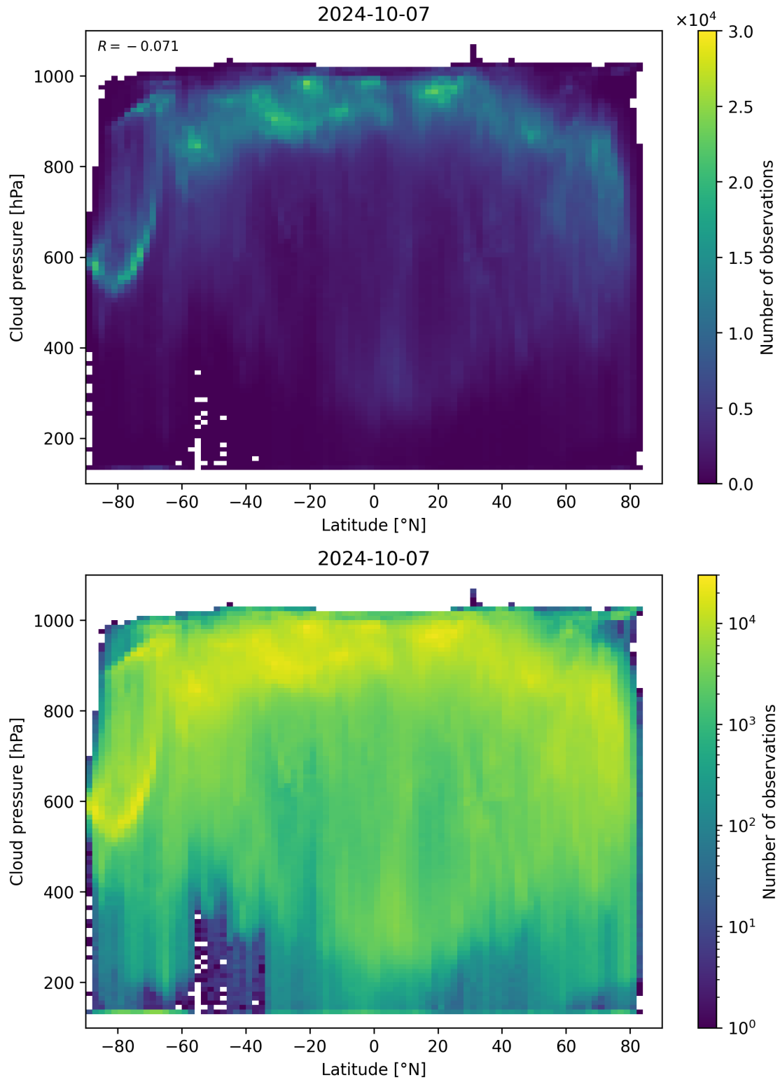
Figure 100: Scatter density plot of “Latitude” against “Cloud pressure” for 2024-10-06 to 2024-10-08.
