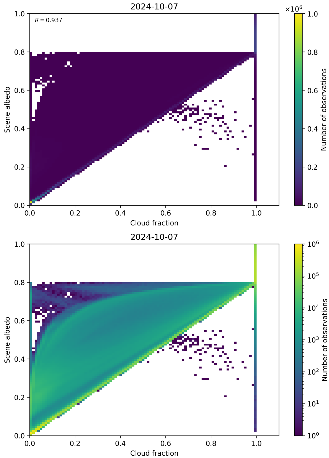
Figure 82: Scatter density plot of “Cloud fraction” against “Scene albedo” for 2024-10-06 to 2024-10-08.
