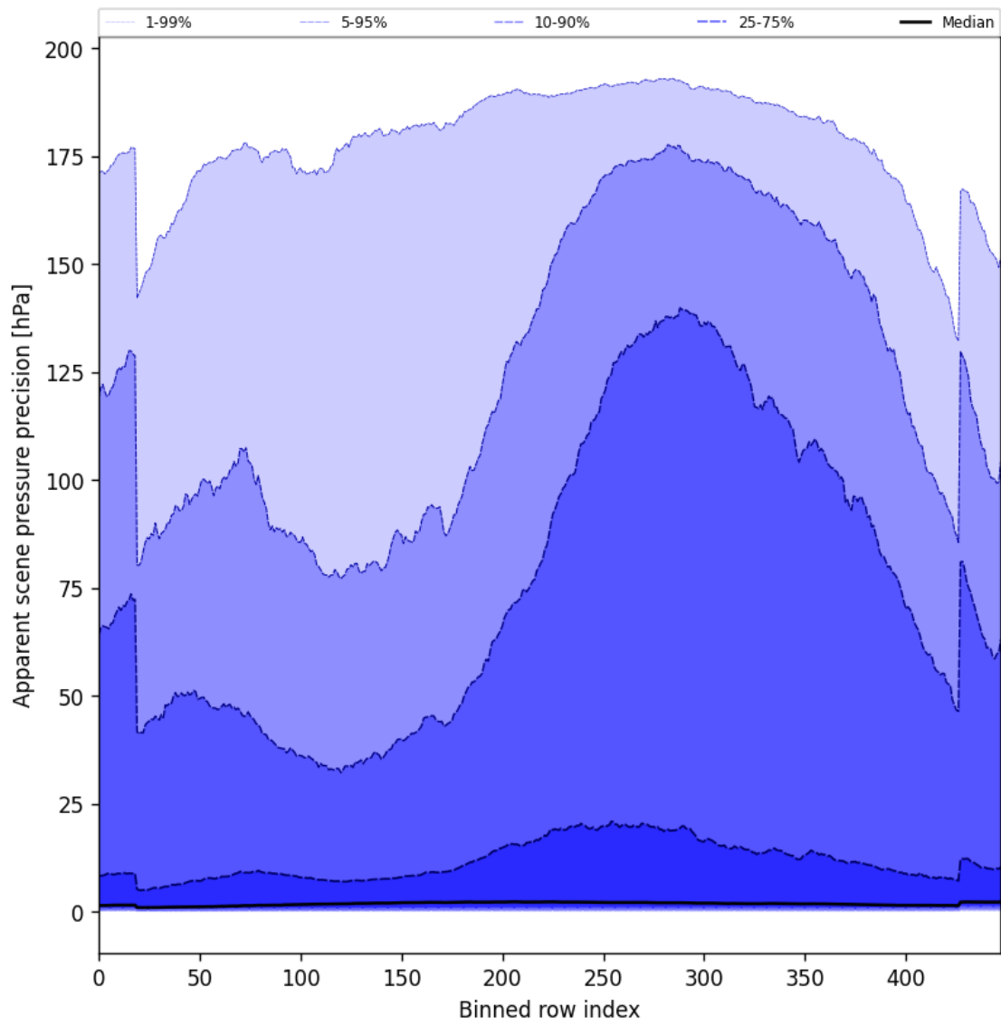
Figure 54: Along track statistics of “Apparent scene pressure precision” for 2024-10-06 to 2024-10-08
