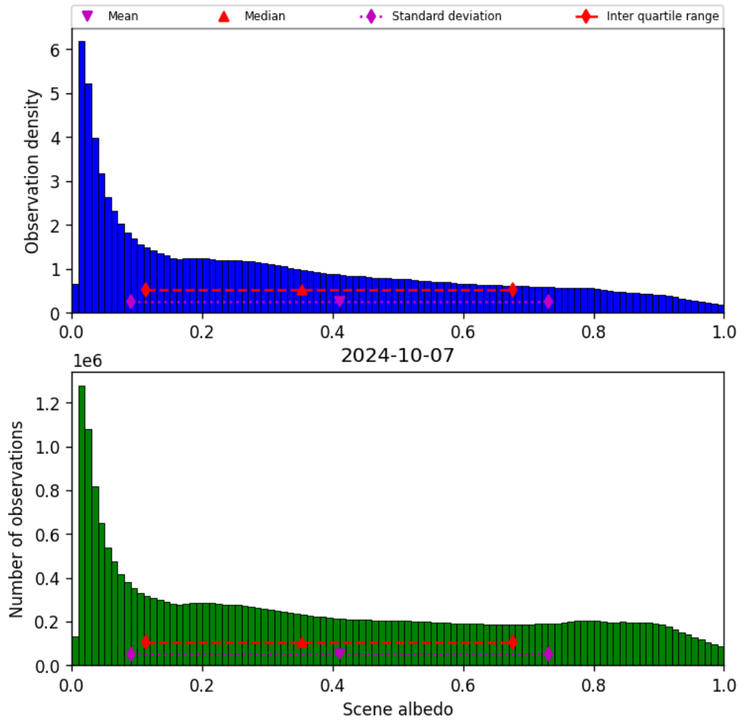
Figure 34: Histogram of “Scene albedo” for 2024-10-06 to 2024-10-08
