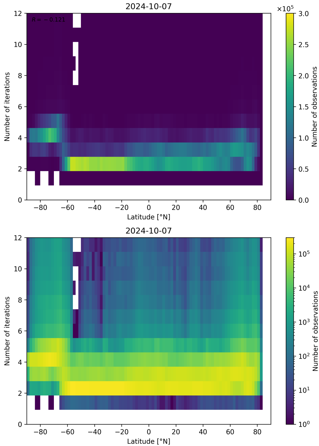
Figure 102: Scatter density plot of “Latitude” against “Number of iterations” for 2024-10-06 to 2024-10-08.
