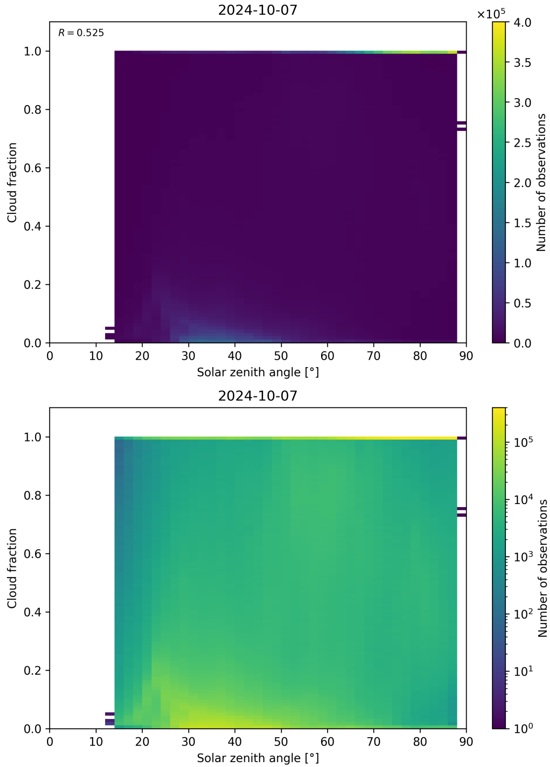
Figure 121: Scatter density plot of “Solar zenith angle” against “Cloud fraction” for 2024-10-06 to 2024-10-08.
