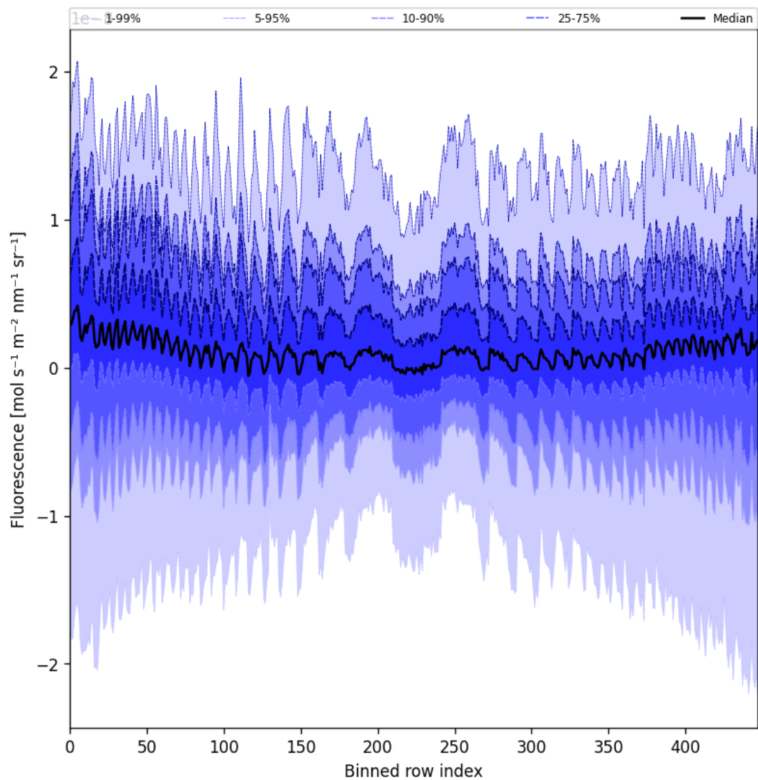
Figure 57: Along track statistics of “Fluorescence” for 2024-10-06 to 2024-10-08
