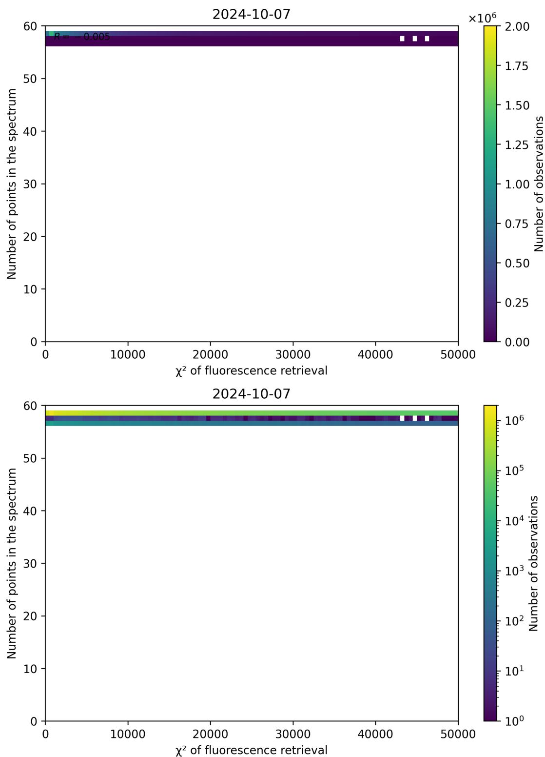
Figure 71: Scatter density plot of “ \chi^2 of fluorescence retrieval” against “Number of points in the spectrum” for 2024-10-06 to 2024-10-08.
