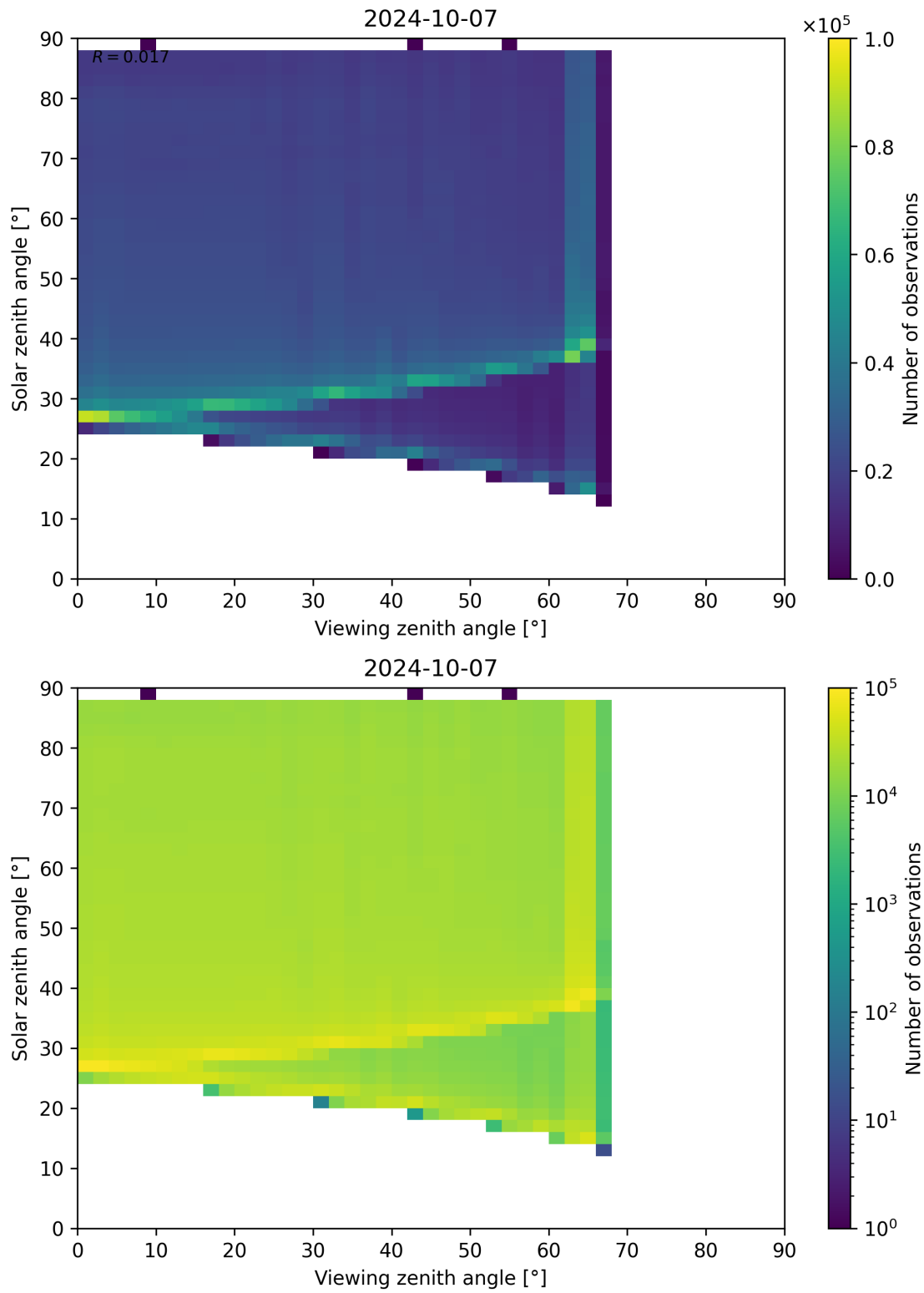
Figure 139: Scatter density plot of “Viewing zenith angle” against “Solar zenith angle” for 2024-10-06 to 2024-10-08.
