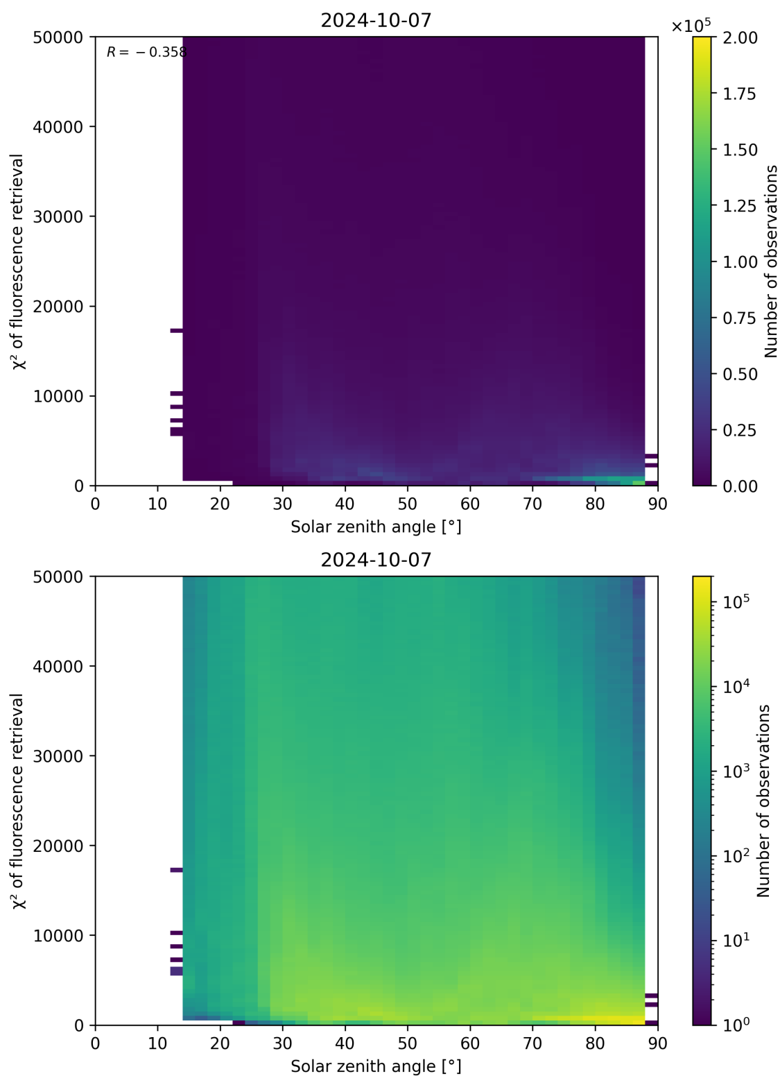
Figure 120: Scatter density plot of “Solar zenith angle” against “ \chi^2 of fluorescence retrieval” for 2024-10-06 to 2024-10-08.
