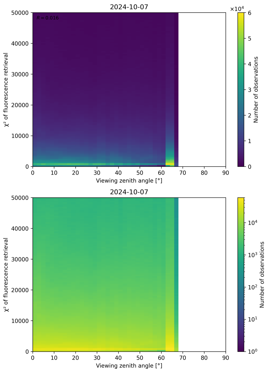
Figure 131: Scatter density plot of “Viewing zenith angle” against “ \chi^2 of fluorescence retrieval” for 2024-10-06 to 2024-10-08.
