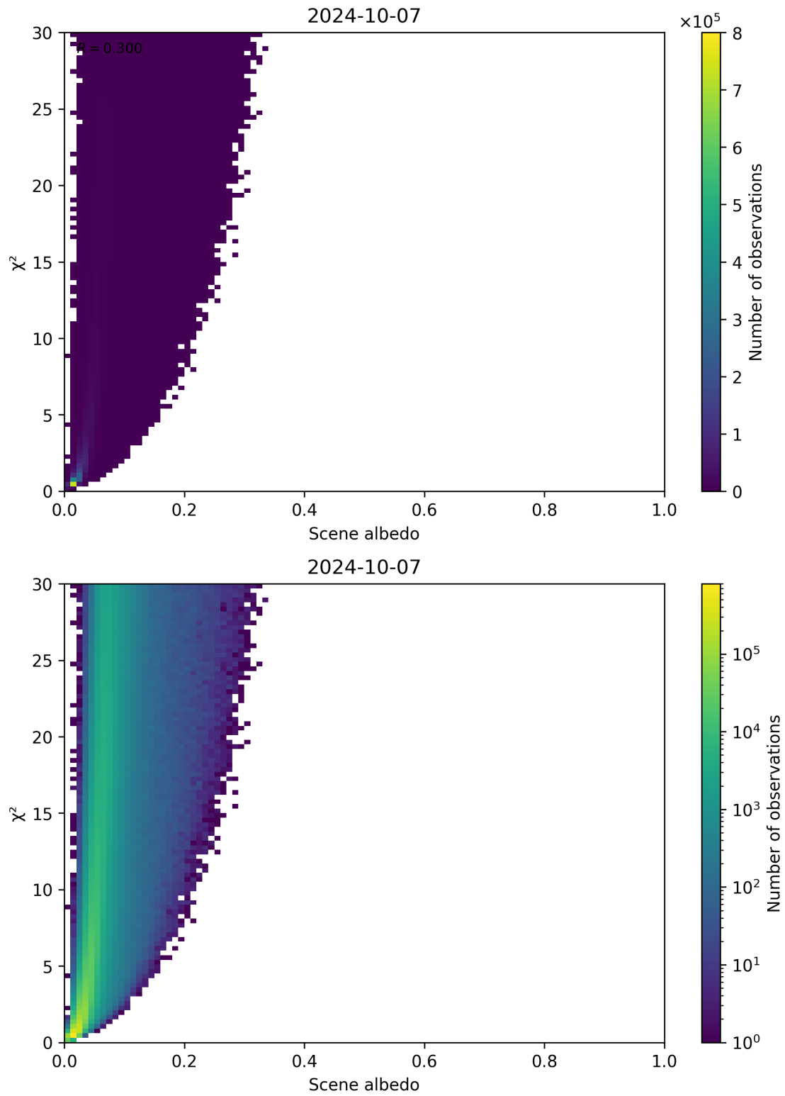
Figure 112: Scatter density plot of “Scene albedo” against “ \chi^2 ” for 2024-10-06 to 2024-10-08.
