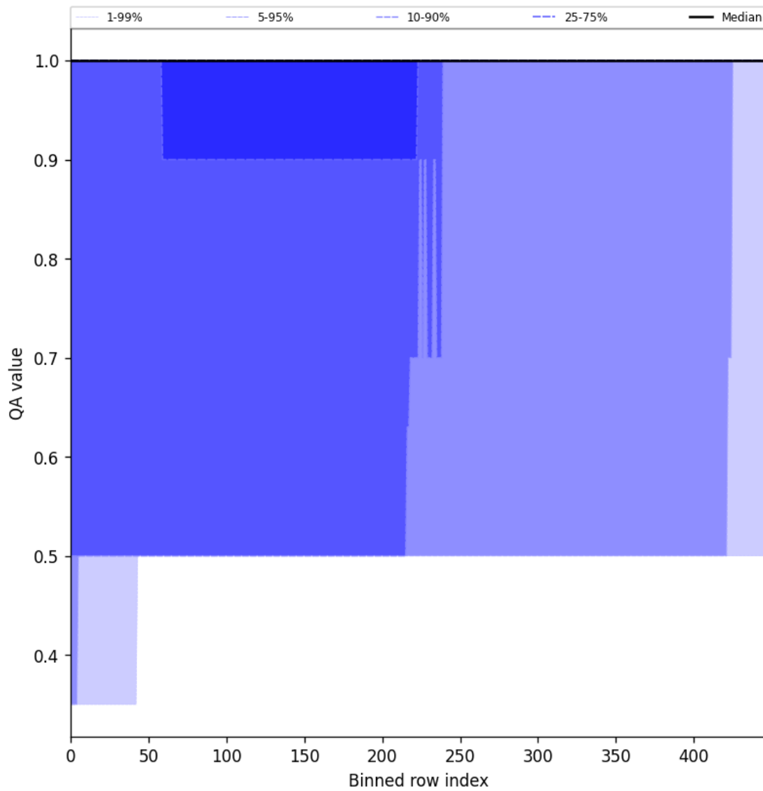
Figure 46: Along track statistics of “QA value” for 2024-10-06 to 2024-10-08
