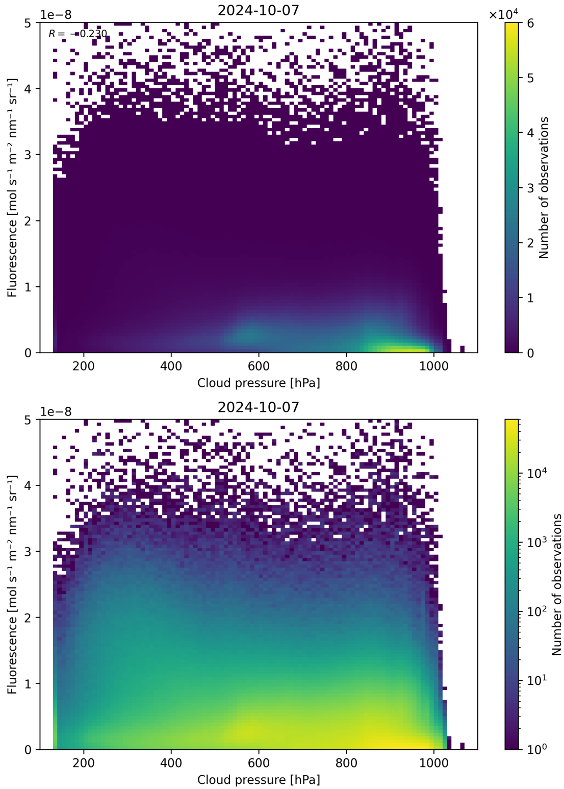
Figure 88: Scatter density plot of “Cloud pressure” against “Fluorescence” for 2024-10-06 to 2024-10-08.
