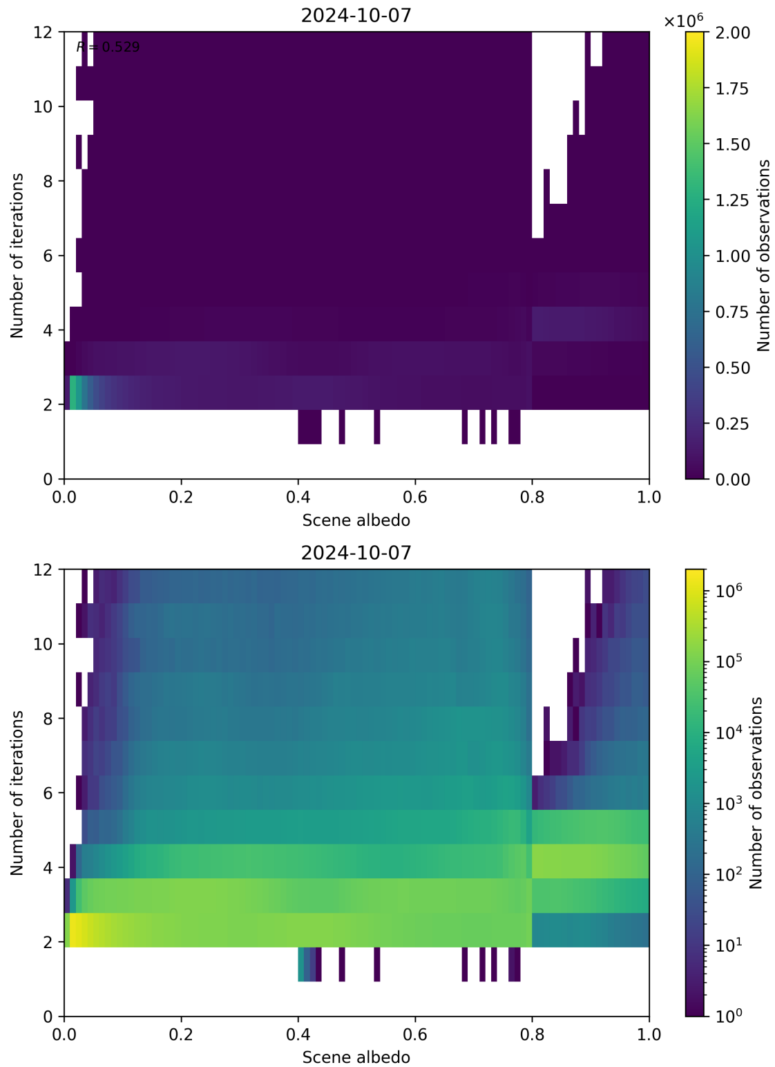
Figure 115: Scatter density plot of “Scene albedo” against “Number of iterations” for 2024-10-06 to 2024-10-08.
