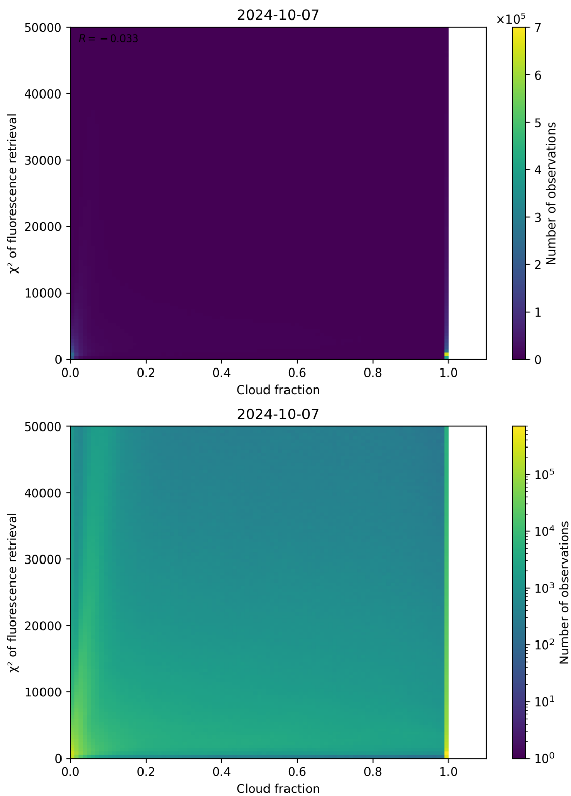
Figure 78: Scatter density plot of “Cloud fraction” against “ \chi^2 of fluorescence retrieval” for 2024-10-06 to 2024-10-08.
