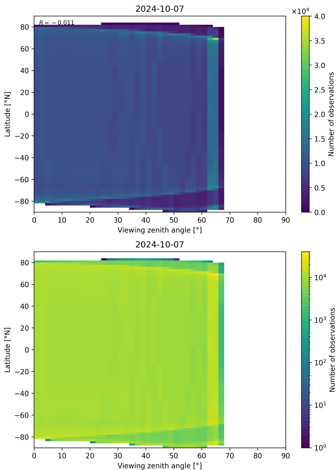
Figure 135: Scatter density plot of “Viewing zenith angle” against “Latitude” for 2024-10-06 to 2024-10-08.
