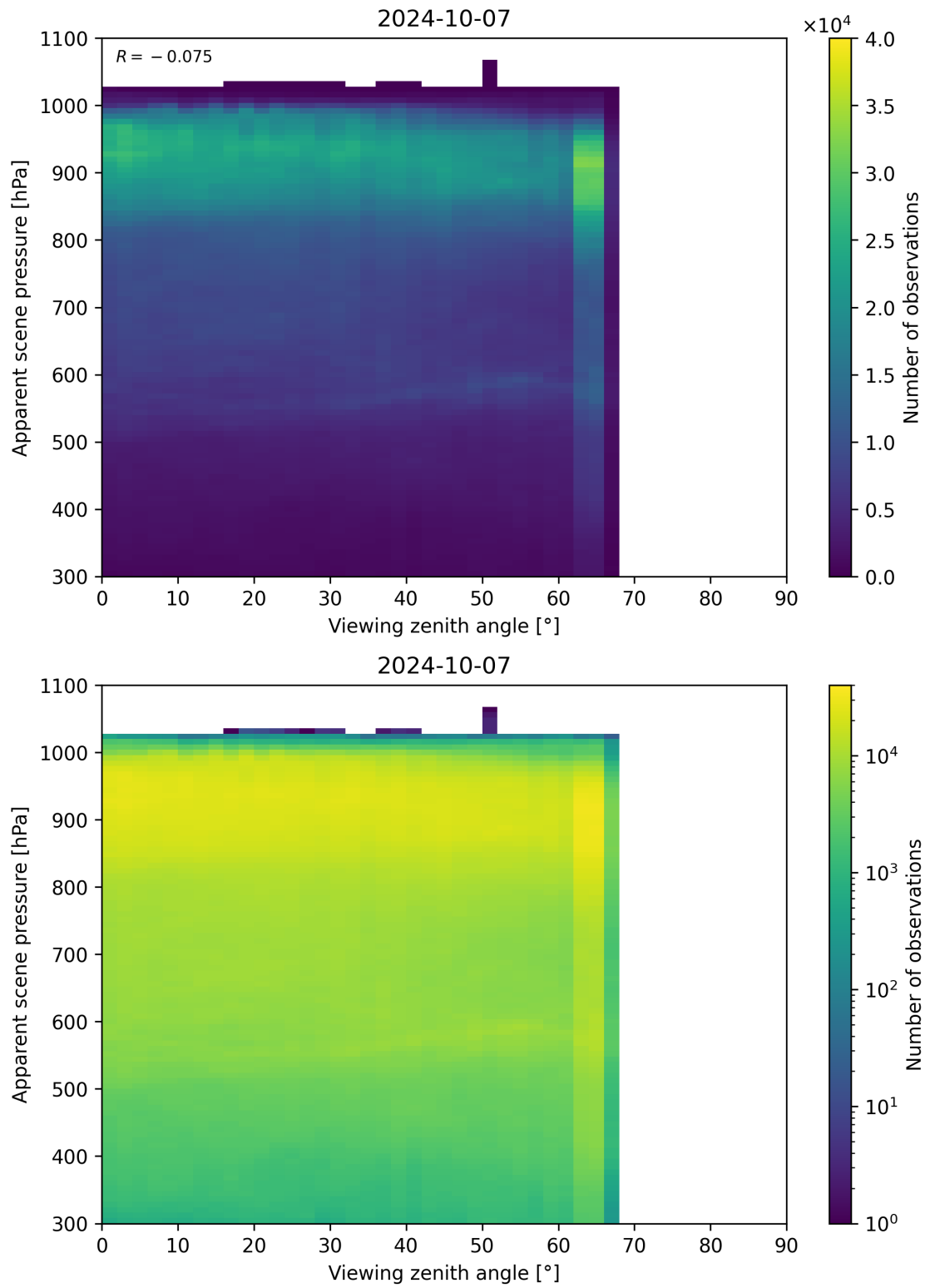
Figure 129: Scatter density plot of “Viewing zenith angle” against “Apparent scene pressure” for 2024-10-06 to 2024-10-08.
