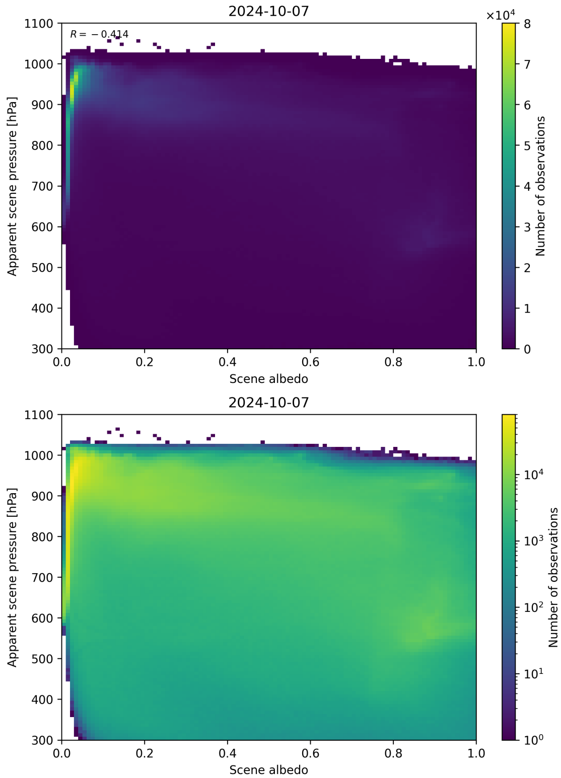
Figure 111: Scatter density plot of “Scene albedo” against “Apparent scene pressure” for 2024-10-06 to 2024-10-08.
