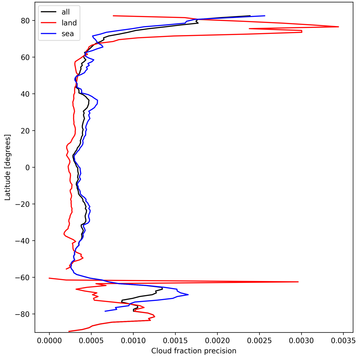
Figure 16: Zonal average of “Cloud fraction precision” for 2024-10-06 to 2024-10-08.
