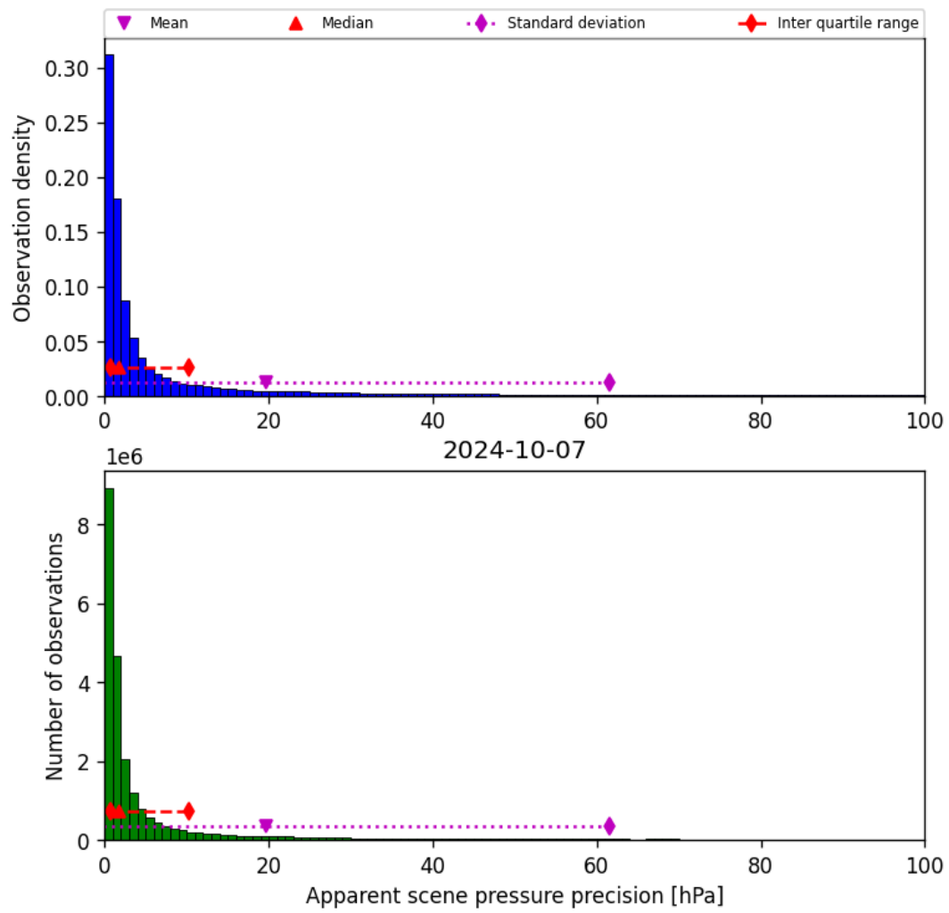
Figure 37: Histogram of “Apparent scene pressure precision” for 2024-10-06 to 2024-10-08
