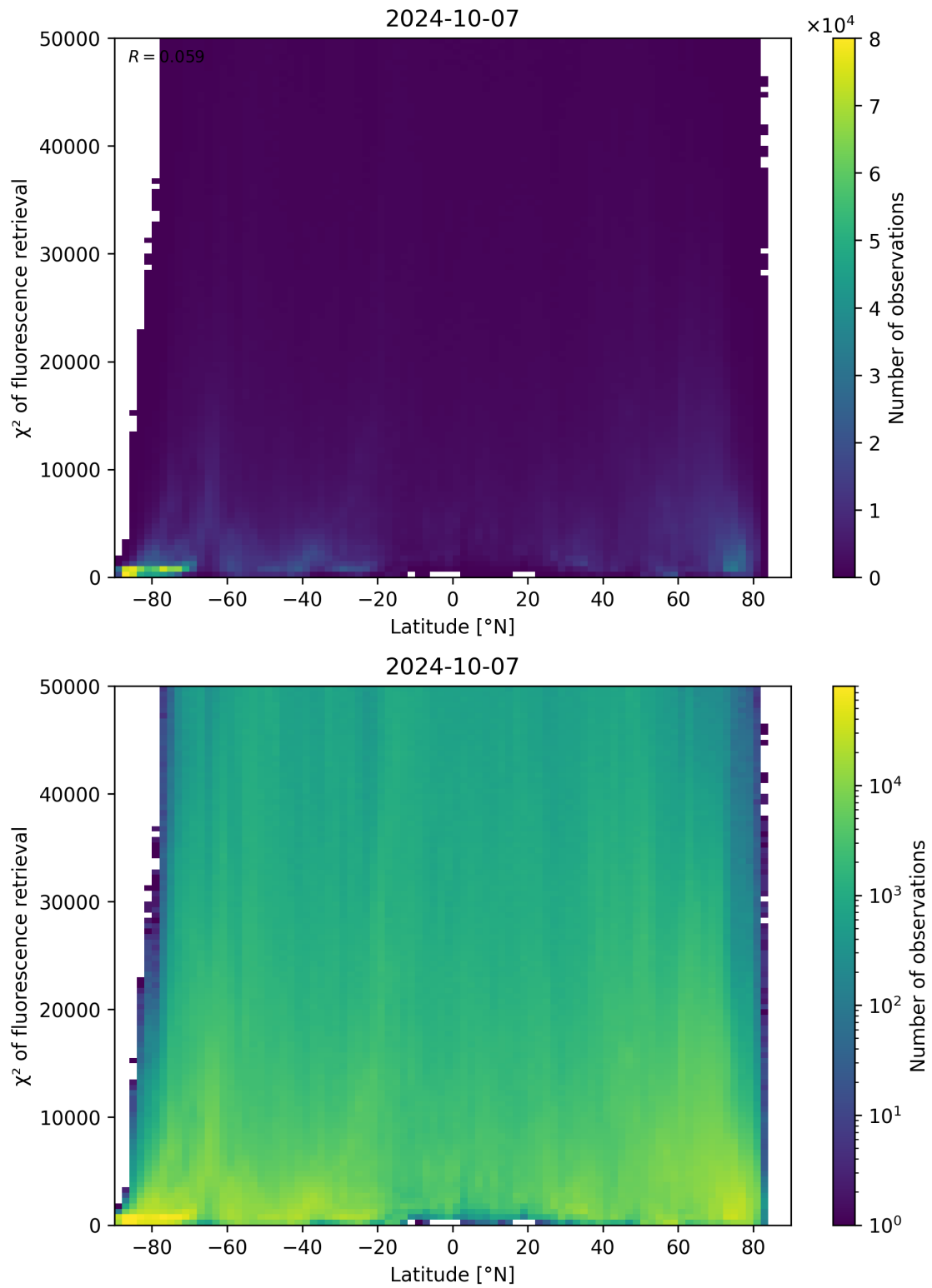
Figure 98: Scatter density plot of “Latitude” against “ \chi^2 of fluorescence retrieval” for 2024-10-06 to 2024-10-08.
