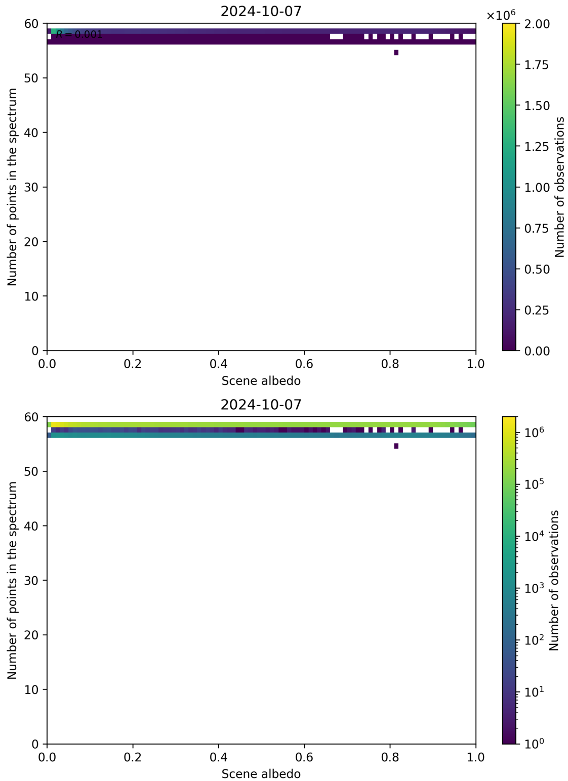
Figure 116: Scatter density plot of “Scene albedo” against “Number of points in the spectrum” for 2024-10-06 to 2024-10-08.
