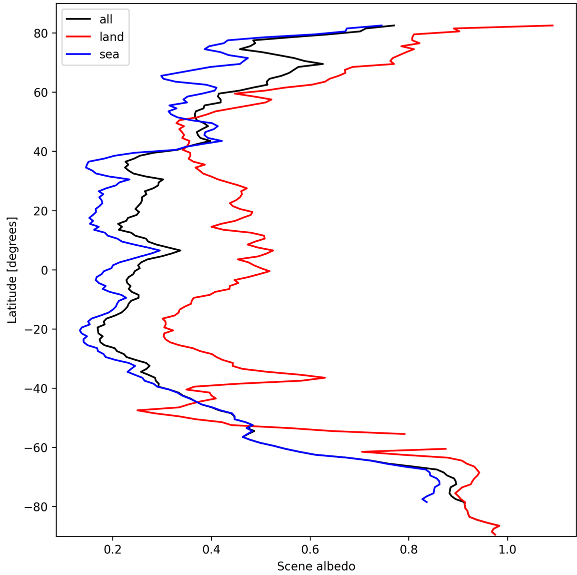
Figure 17: Zonal average of “Scene albedo” for 2024-10-06 to 2024-10-08.
