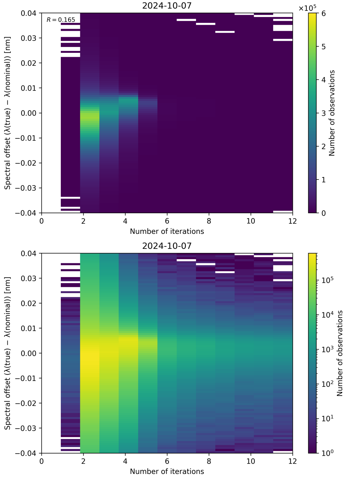
Figure 109: Scatter density plot of “Number of iterations” against “Spectral offset ( \lambda_{\text{true}} - \lambda_{\text{nominal}} )” for 2024-10-06 to 2024-10-08.
