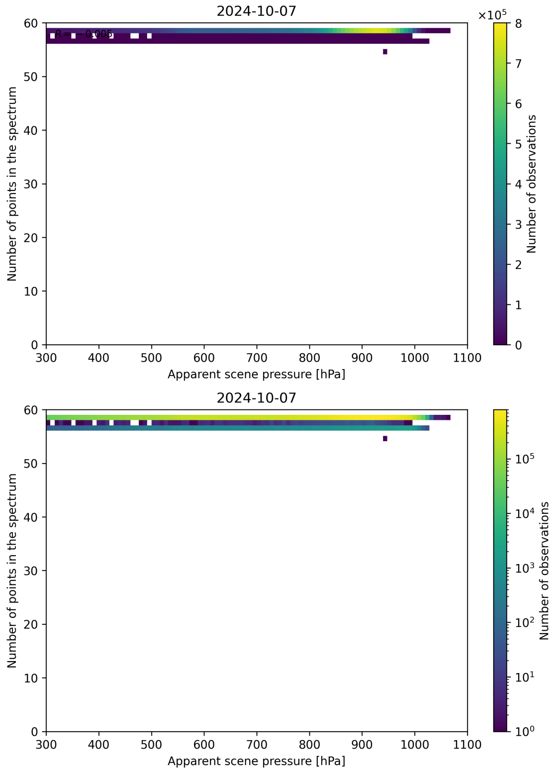
Figure 67: Scatter density plot of “Apparent scene pressure” against “Number of points in the spectrum” for 2024-10-06 to 2024-10-08.
