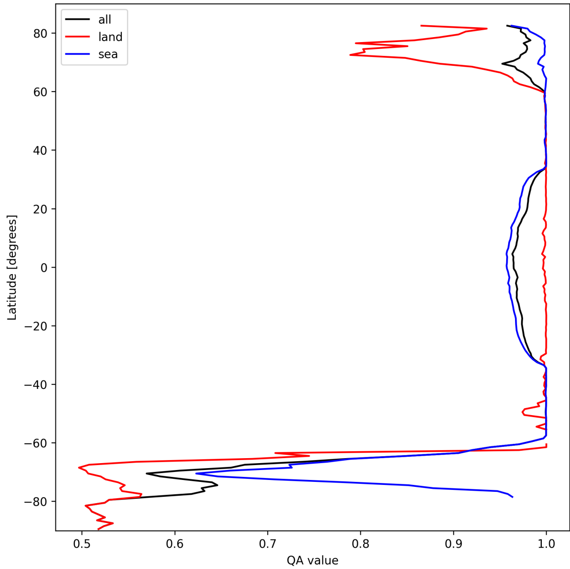
Figure 12: Zonal average of “QA value” for 2024-10-06 to 2024-10-08.
