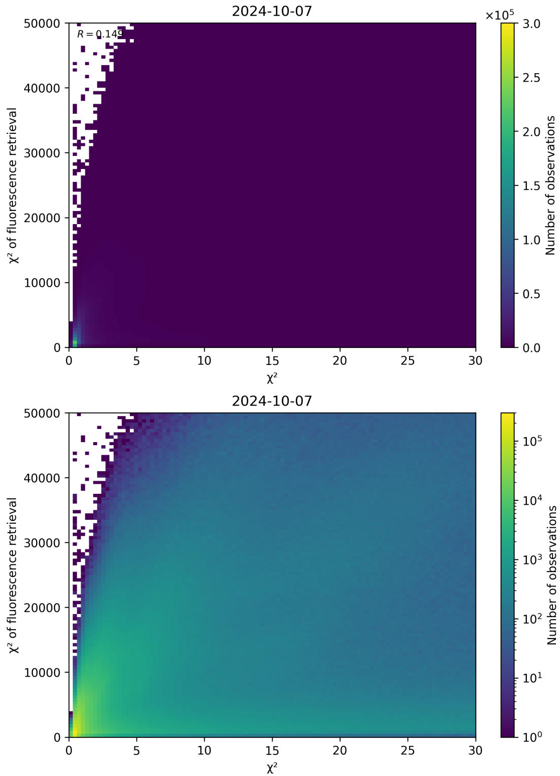
Figure 69: Scatter density plot of “ \chi^2 ” against “ \chi^2 of fluorescence retrieval” for 2024-10-06 to 2024-10-08.
