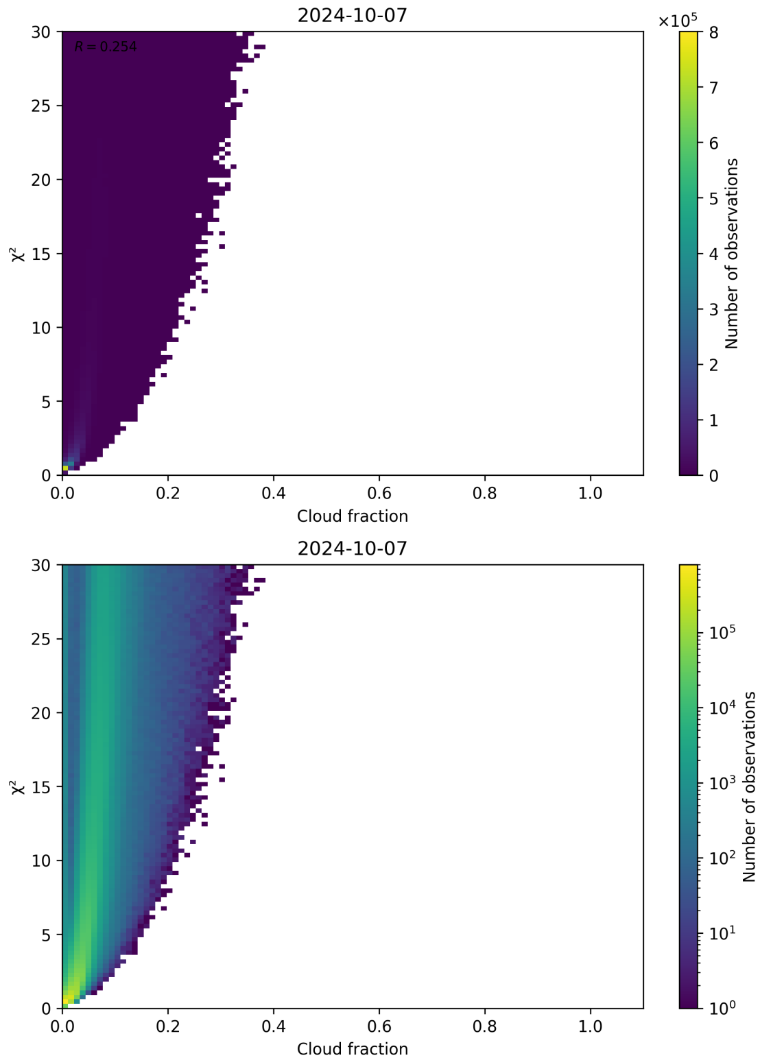
Figure 77: Scatter density plot of “Cloud fraction” against “ \chi^2 ” for 2024-10-06 to 2024-10-08.
