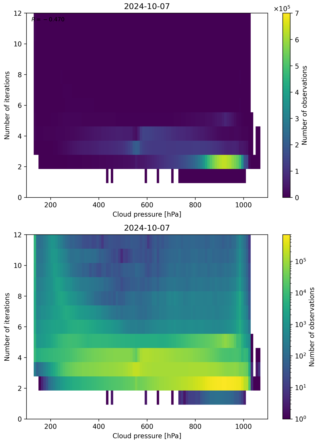
Figure 89: Scatter density plot of “Cloud pressure” against “Number of iterations” for 2024-10-06 to 2024-10-08.
