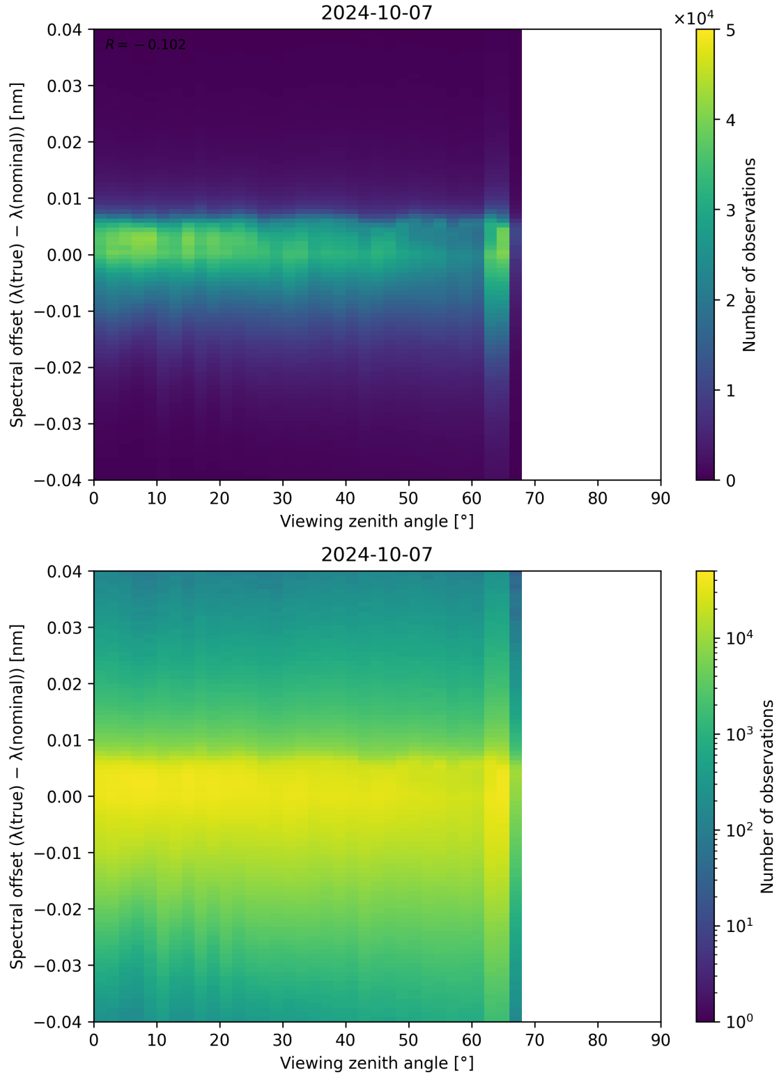
Figure 140: Scatter density plot of “Viewing zenith angle” against “Spectral offset ( \lambda_{\text{true}} - \lambda_{\text{nominal}} )” for 2024-10-06 to 2024-10-08.
