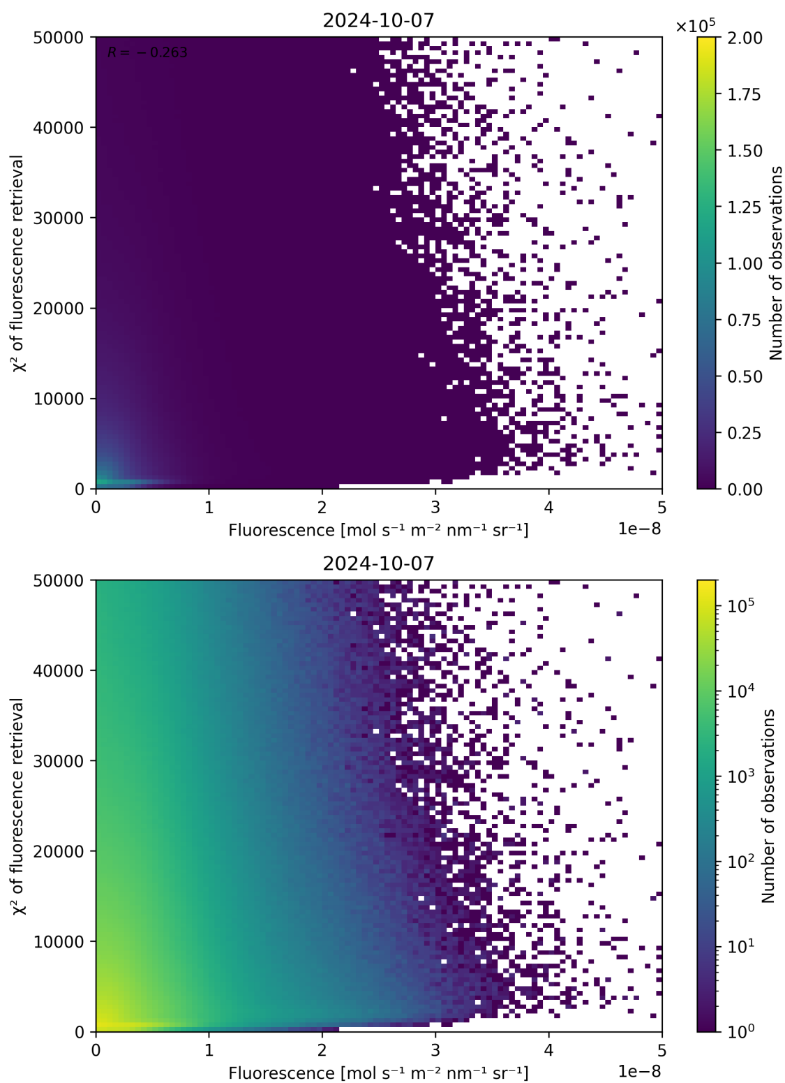
Figure 93: Scatter density plot of “Fluorescence” against “ \chi^2 of fluorescence retrieval” for 2024-10-06 to 2024-10-08.
