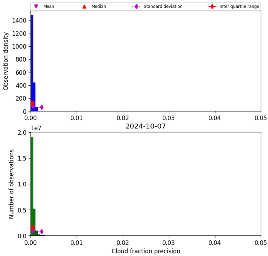
Figure 33: Histogram of “Cloud fraction precision” for 2024-10-06 to 2024-10-08
