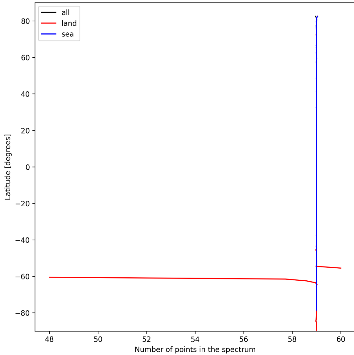
Figure 27: Zonal average of “Number of points in the spectrum” for 2024-10-06 to 2024-10-08.
