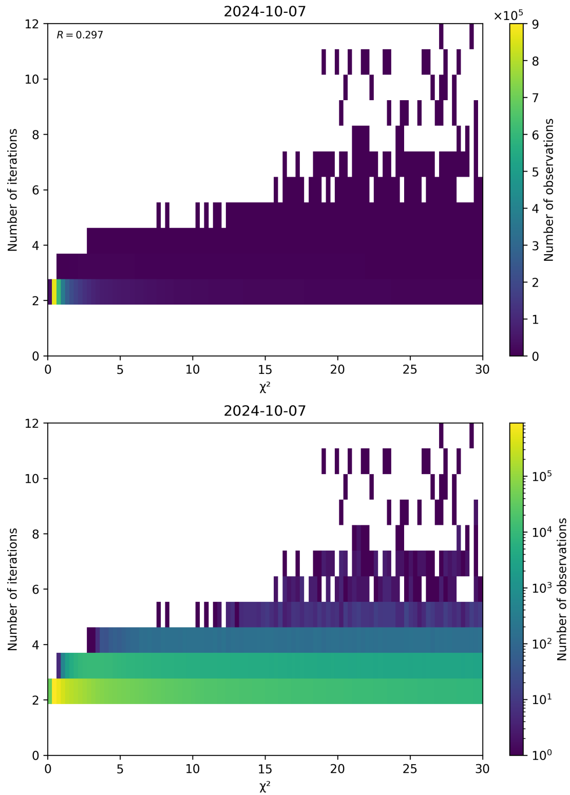
Figure 73: Scatter density plot of “ \chi^2 ” against “Number of iterations” for 2024-10-06 to 2024-10-08.
