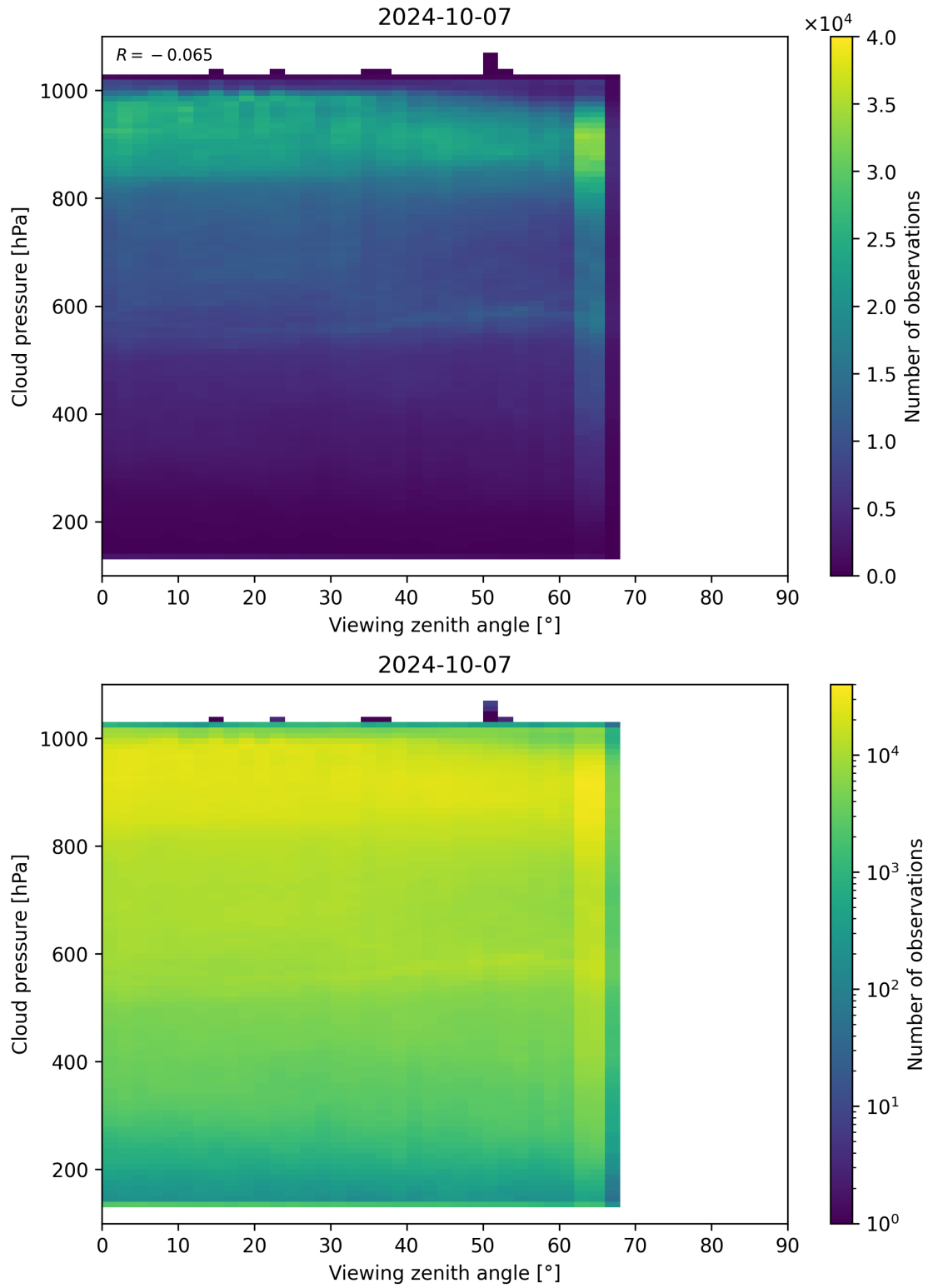
Figure 133: Scatter density plot of “Viewing zenith angle” against “Cloud pressure” for 2024-10-06 to 2024-10-08.
