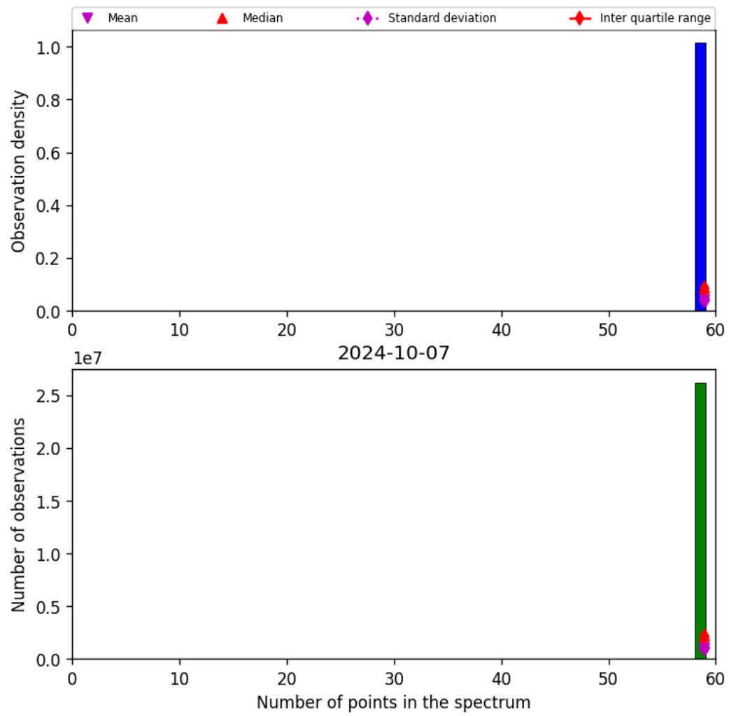
Figure 44: Histogram of “Number of points in the spectrum” for 2024-10-06 to 2024-10-08
