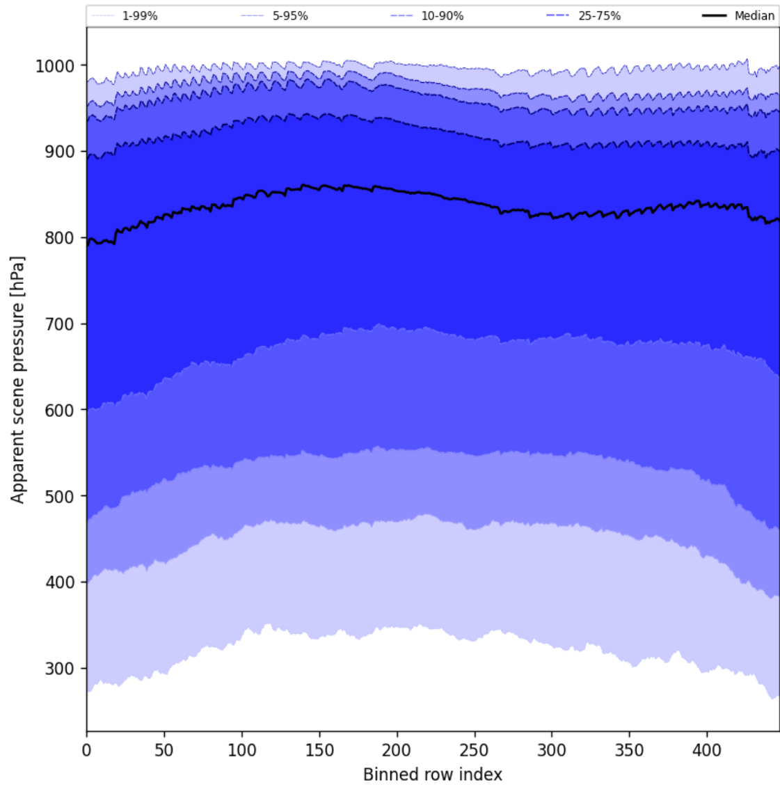
Figure 53: Along track statistics of “Apparent scene pressure” for 2024-10-06 to 2024-10-08
