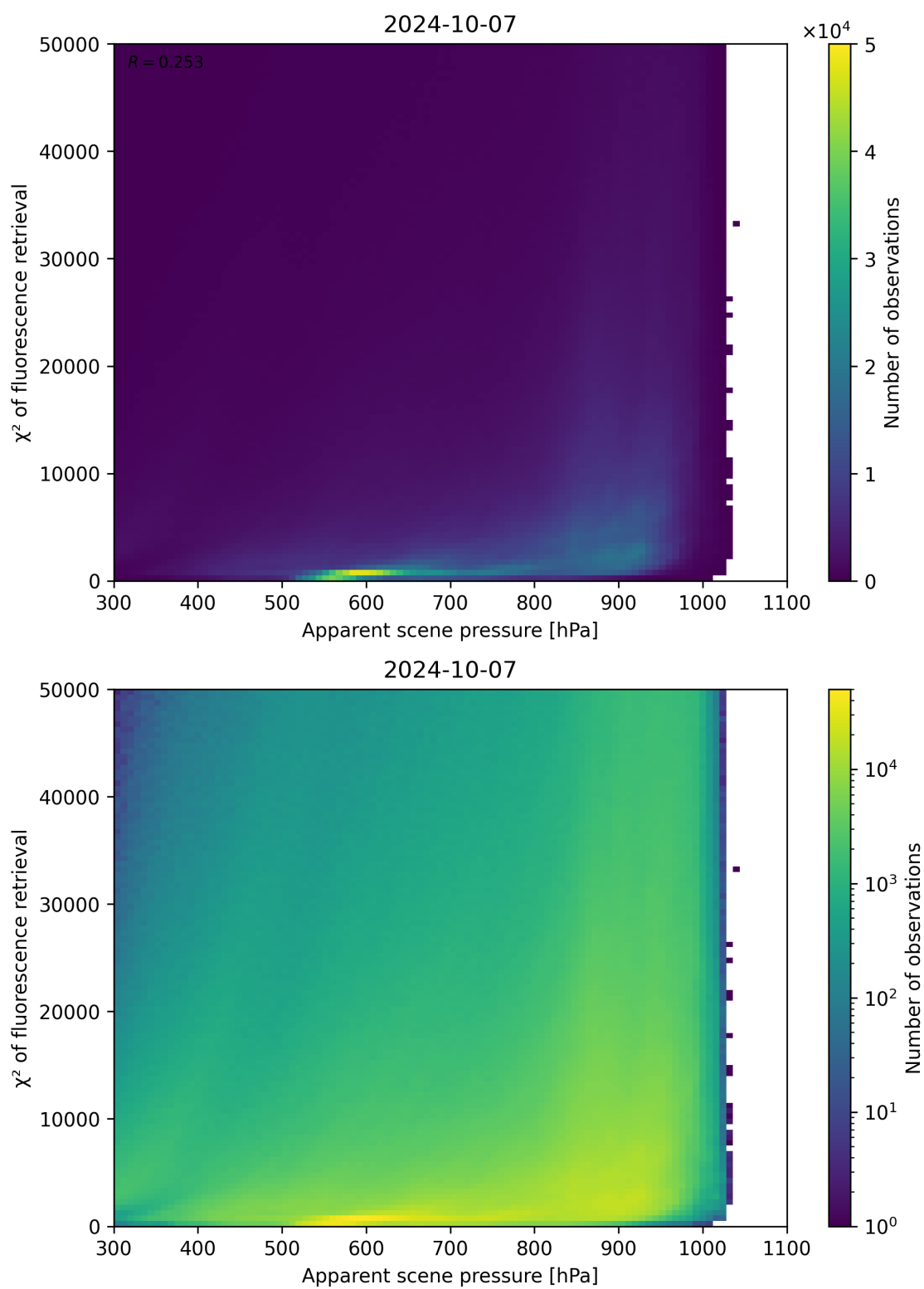
Figure 64: Scatter density plot of “Apparent scene pressure” against “ \chi^2 of fluorescence retrieval” for 2024-10-06 to 2024-10-08.
