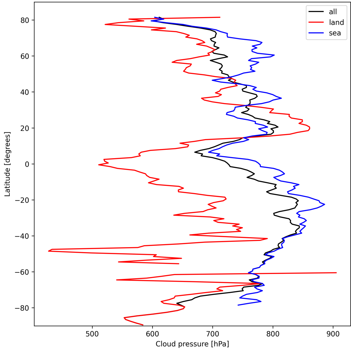
Figure 13: Zonal average of “Cloud pressure” for 2024-10-08 to 2024-10-09.
