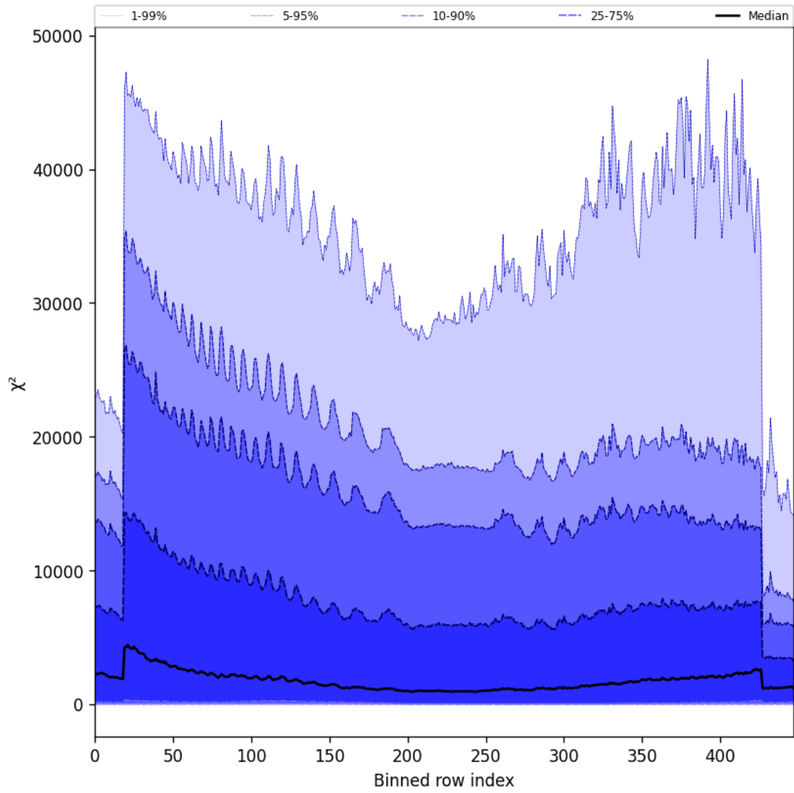
Figure 55: Along track statistics of “ \chi^2 ” for 2024-10-08 to 2024-10-09
