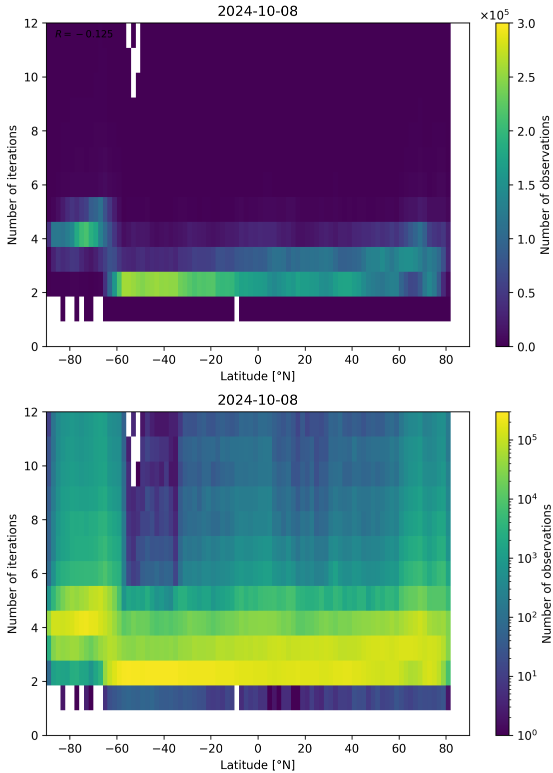
Figure 102: Scatter density plot of “Latitude” against “Number of iterations” for 2024-10-08 to 2024-10-09.
