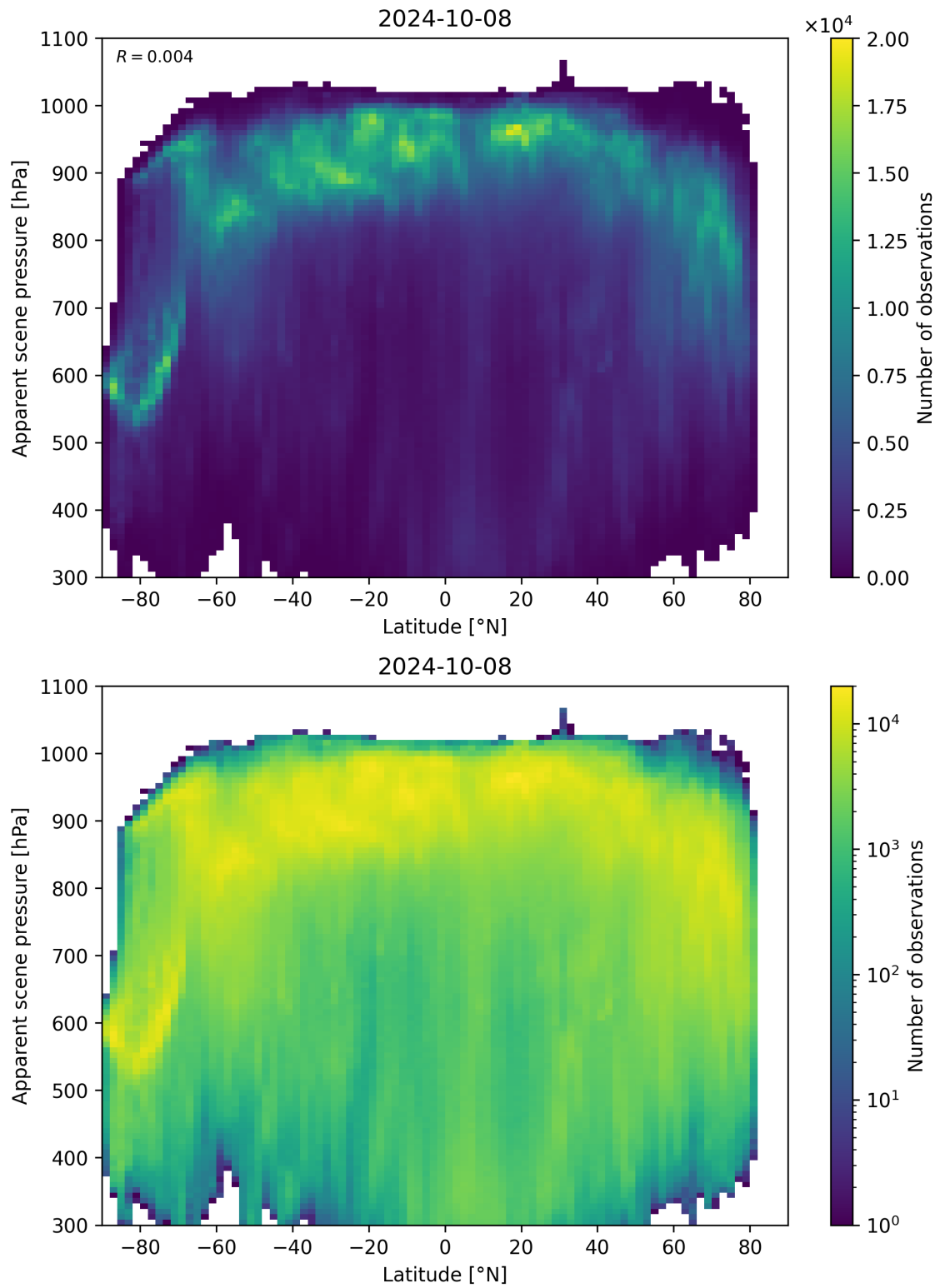
Figure 96: Scatter density plot of “Latitude” against “Apparent scene pressure” for 2024-10-08 to 2024-10-09.
