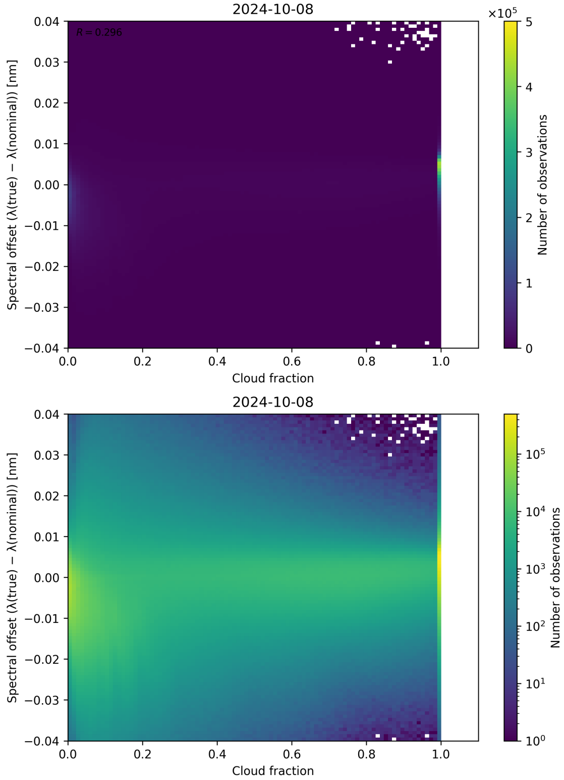
Figure 83: Scatter density plot of “Cloud fraction” against “Spectral offset ( \lambda_{\text{true}} - \lambda_{\text{nominal}} )” for 2024-10-08 to 2024-10-09.
