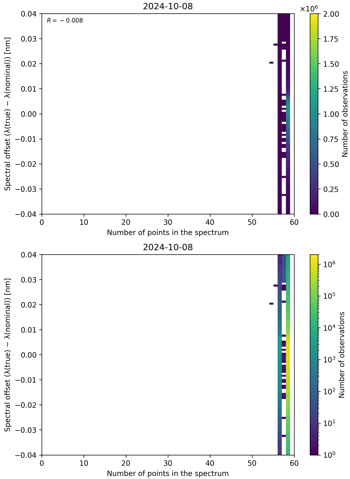
Figure 110: Scatter density plot of “Number of points in the spectrum” against “Spectral offset ( \lambda_{\text{true}} - \lambda_{\text{nominal}} )” for 2024-10-08 to 2024-10-09.
