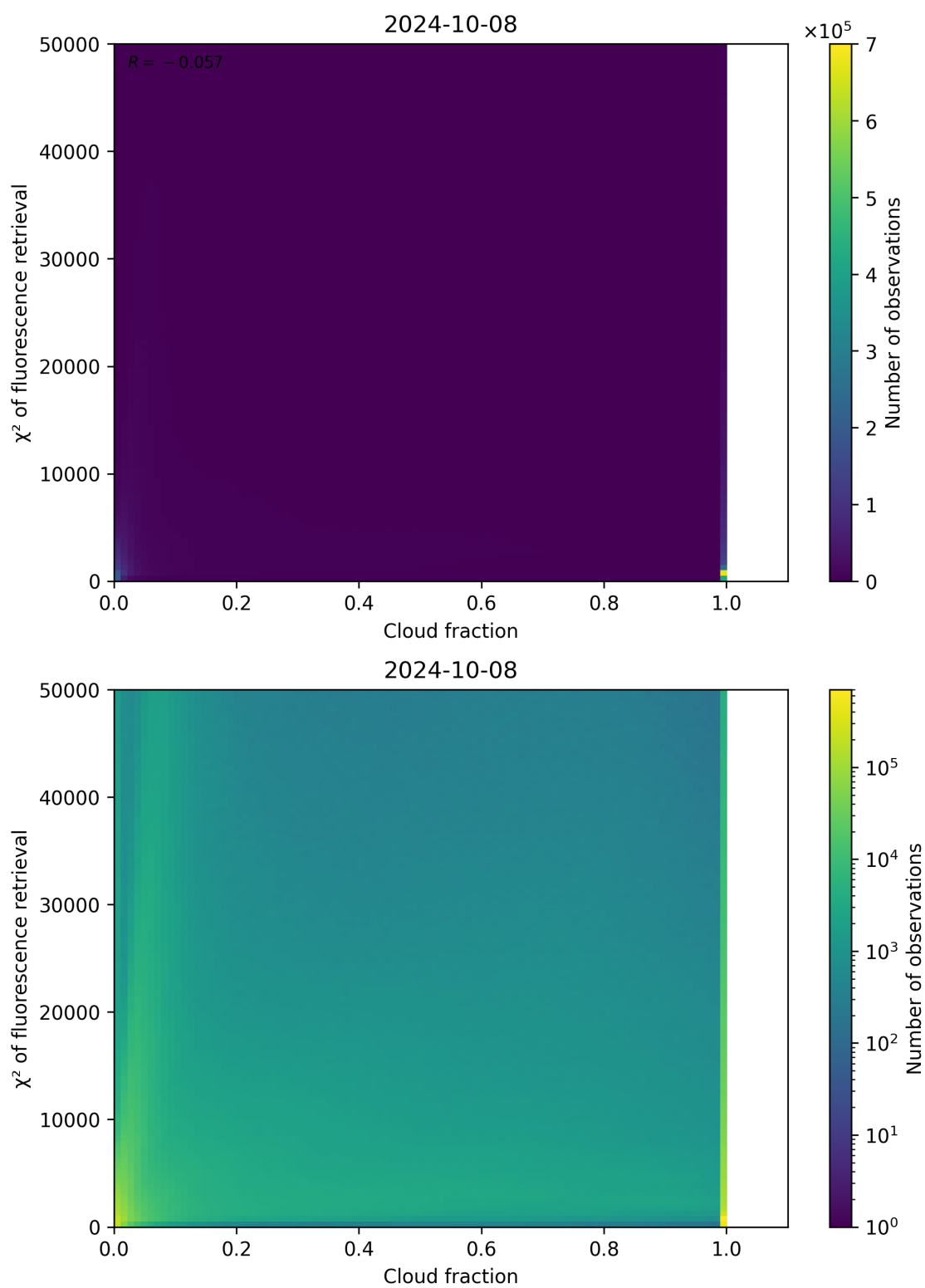
Figure 78: Scatter density plot of “Cloud fraction” against “ \chi^2 of fluorescence retrieval” for 2024-10-08 to 2024-10-09.
