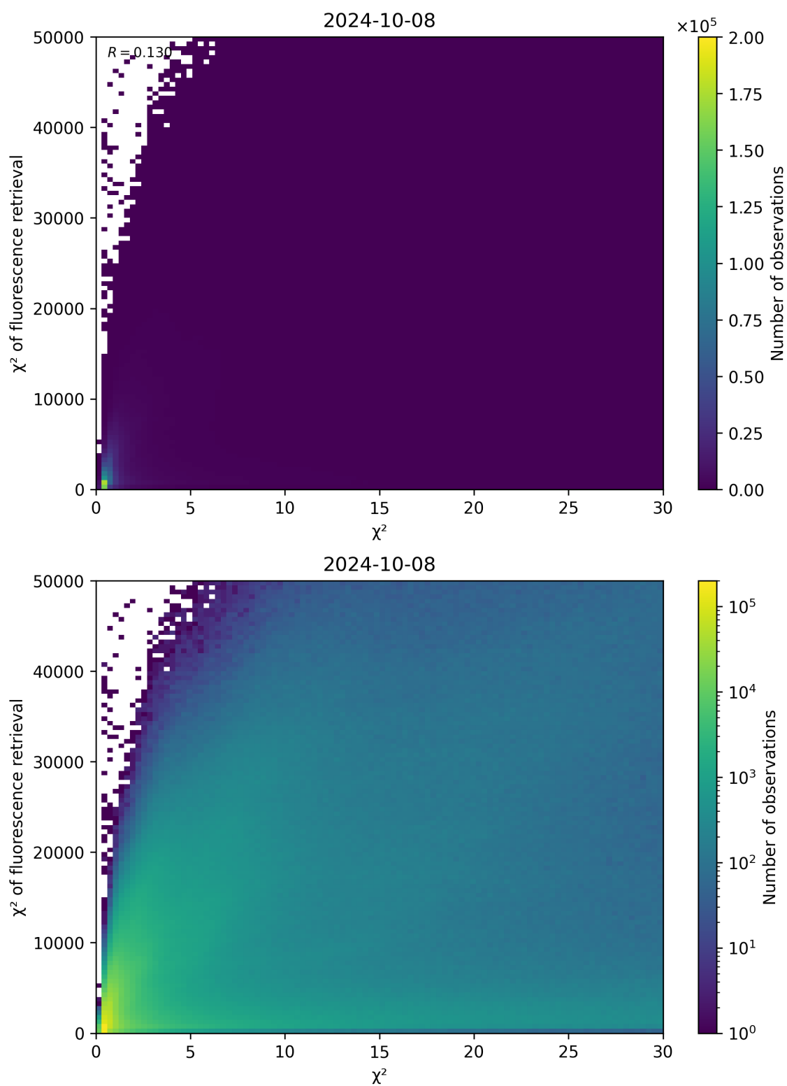
Figure 69: Scatter density plot of “ \chi^2 ” against “ \chi^2 of fluorescence retrieval” for 2024-10-08 to 2024-10-09.
