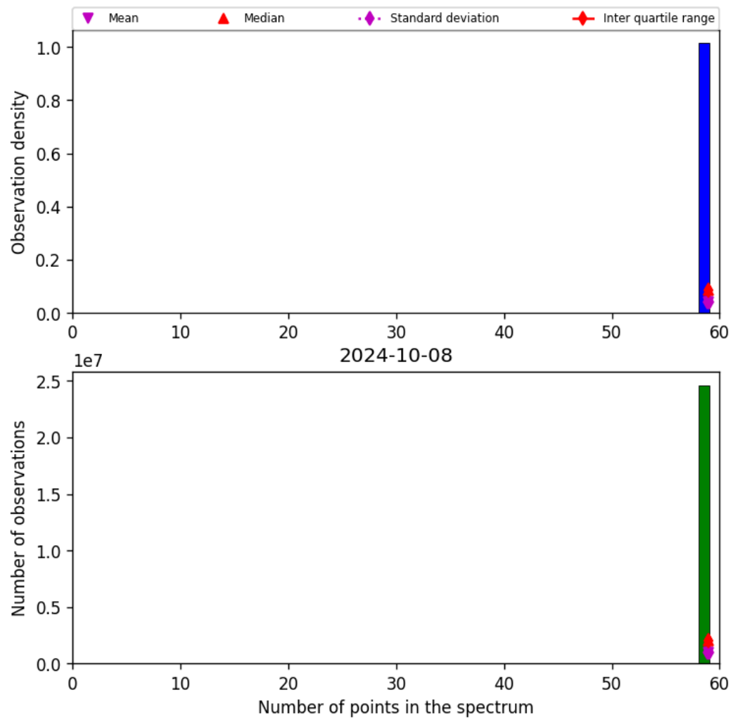
Figure 44: Histogram of “Number of points in the spectrum” for 2024-10-08 to 2024-10-09
