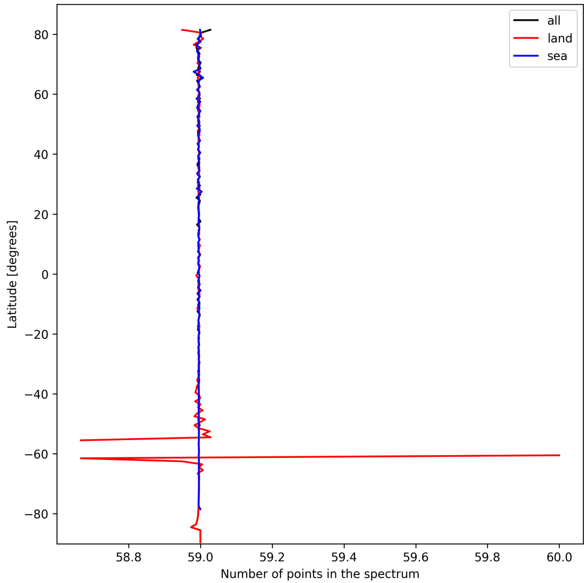
Figure 27: Zonal average of “Number of points in the spectrum” for 2024-10-08 to 2024-10-09.
