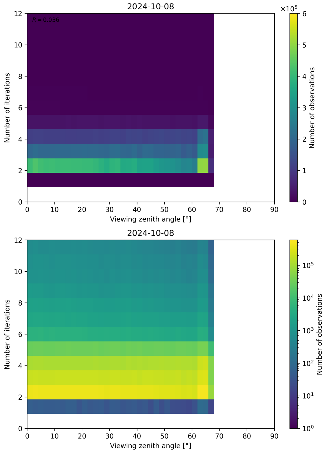
Figure 136: Scatter density plot of “Viewing zenith angle” against “Number of iterations” for 2024-10-08 to 2024-10-09.
