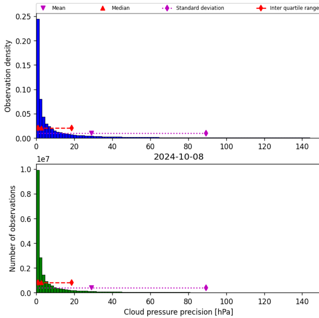
Figure 31: Histogram of “Cloud pressure precision” for 2024-10-08 to 2024-10-09
