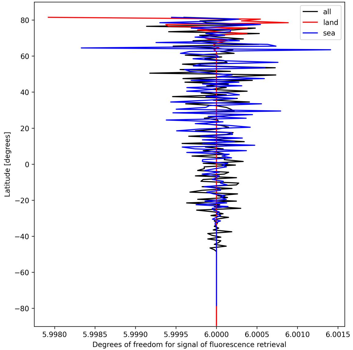
Figure 26: Zonal average of “Degrees of freedom for signal of fluorescence retrieval” for 2024-10-08 to 2024-10-09.
