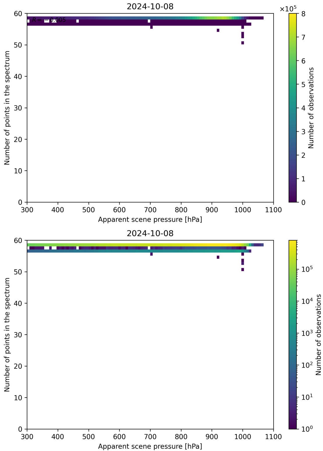
Figure 67: Scatter density plot of “Apparent scene pressure” against “Number of points in the spectrum” for 2024-10-08 to 2024-10-09.
