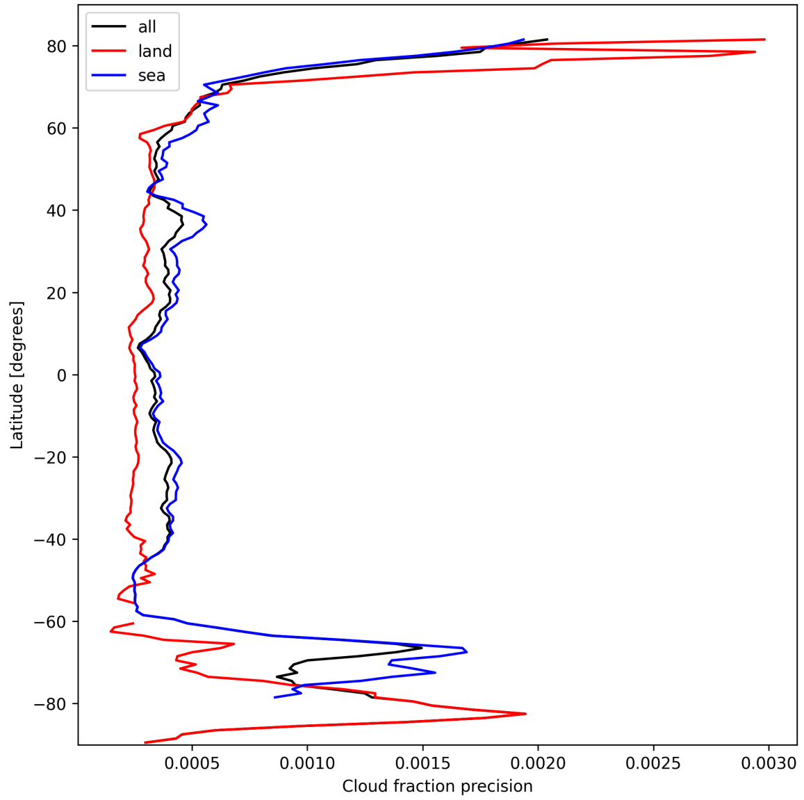
Figure 16: Zonal average of “Cloud fraction precision” for 2024-10-08 to 2024-10-09.
