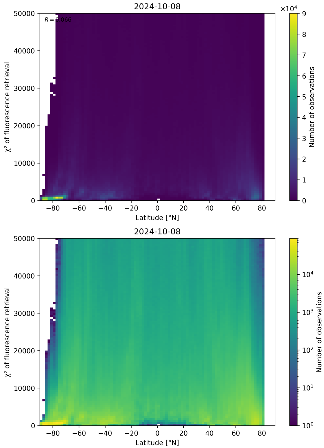
Figure 98: Scatter density plot of “Latitude” against “ \chi^2 of fluorescence retrieval” for 2024-10-08 to 2024-10-09.
