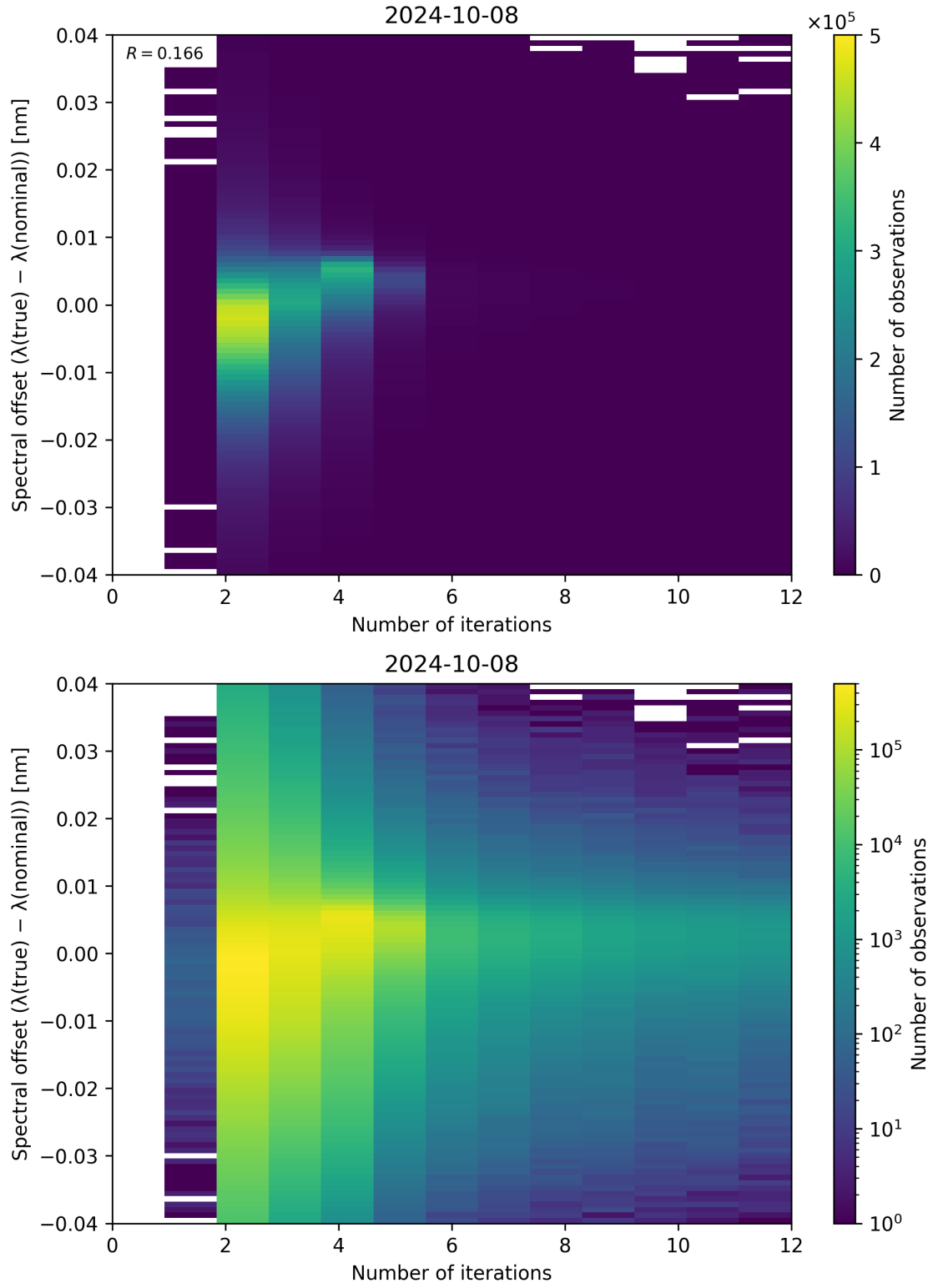
Figure 109: Scatter density plot of “Number of iterations” against “Spectral offset ( \lambda_{\text{true}} - \lambda_{\text{nominal}} )” for 2024-10-08 to 2024-10-09.
