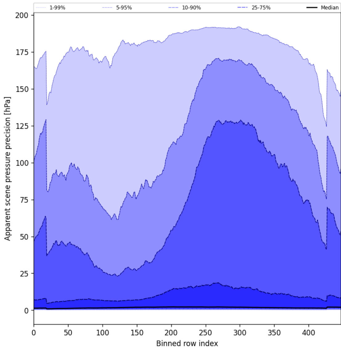
Figure 54: Along track statistics of “Apparent scene pressure precision” for 2024-10-08 to 2024-10-09
