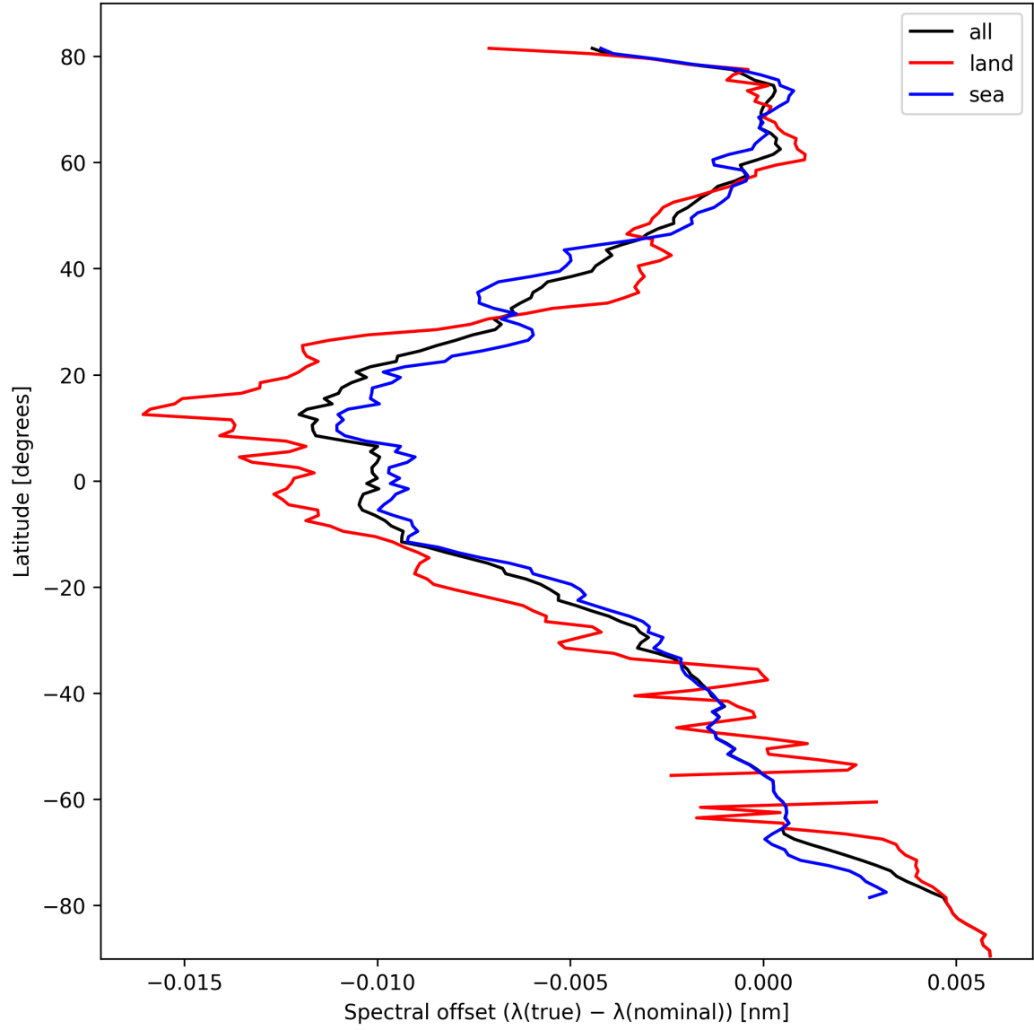
Figure 28: Zonal average of “Spectral offset ( \lambda_{\text{true}} - \lambda_{\text{nominal}} )” for 2024-10-08 to 2024-10-09.
