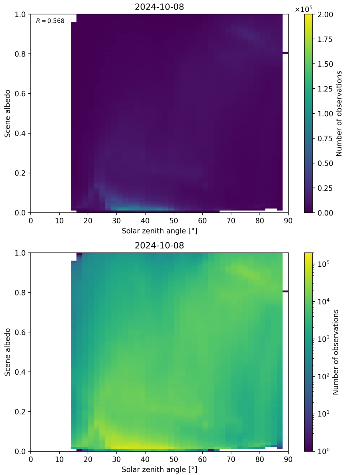
Figure 127: Scatter density plot of “Solar zenith angle” against “Scene albedo” for 2024-10-08 to 2024-10-09.
