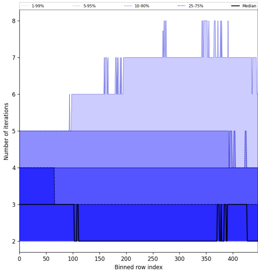
Figure 56: Along track statistics of “Number of iterations” for 2024-10-08 to 2024-10-09
