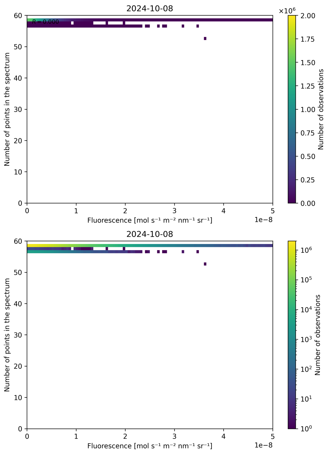
Figure 94: Scatter density plot of “Fluorescence” against “Number of points in the spectrum” for 2024-10-08 to 2024-10-09.
