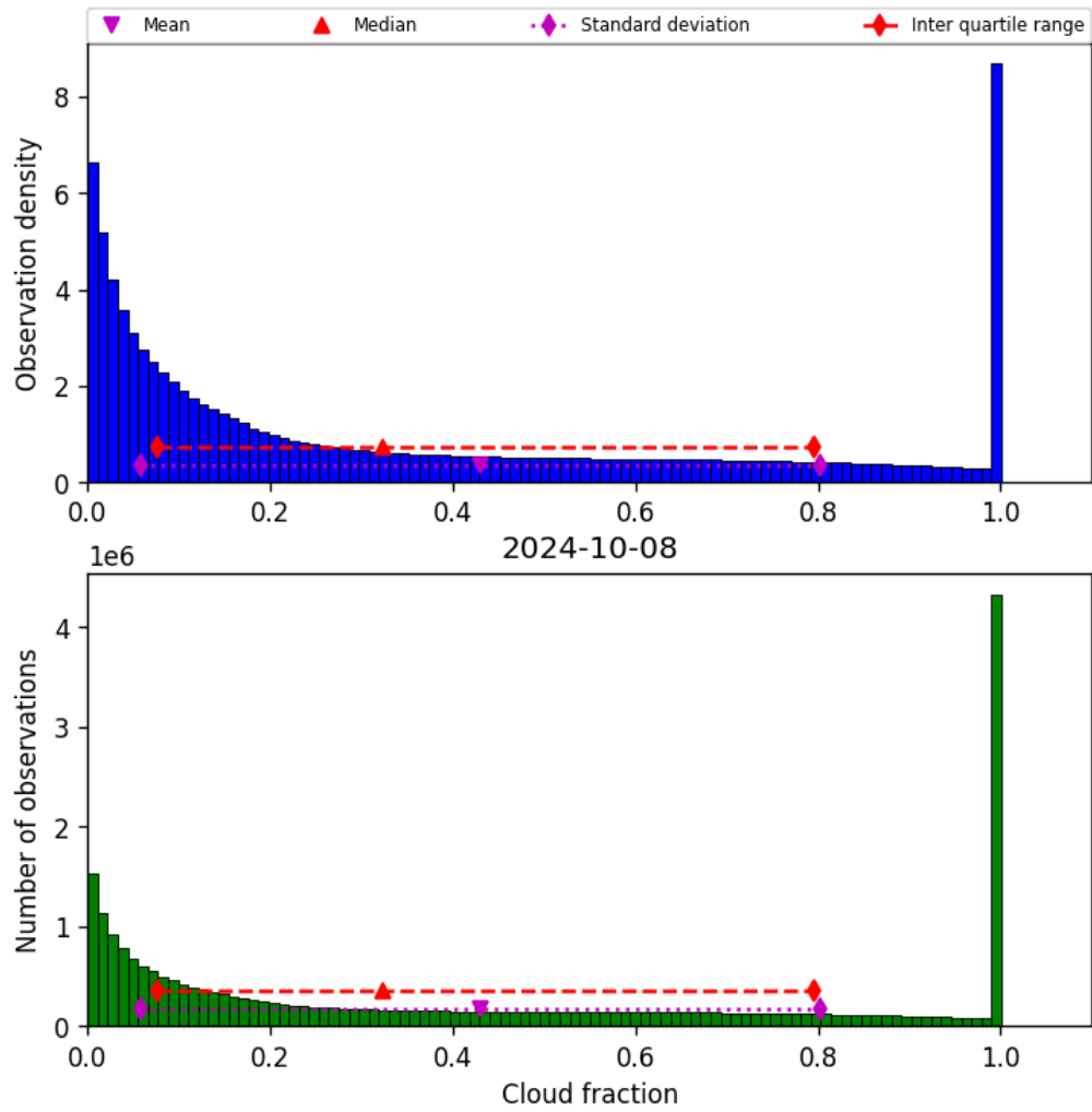
Figure 32: Histogram of “Cloud fraction” for 2024-10-08 to 2024-10-09
