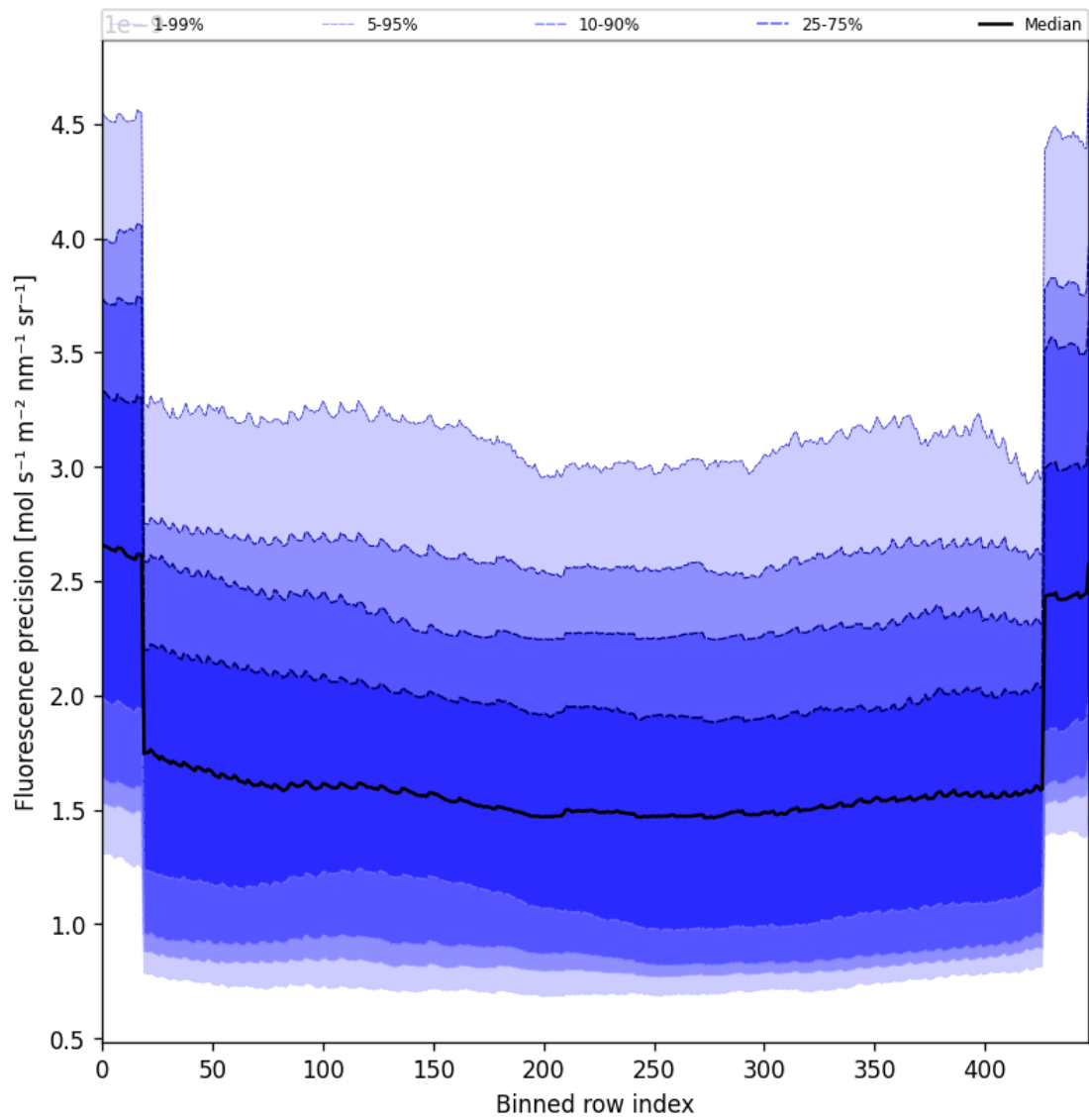
Figure 58: Along track statistics of “Fluorescence precision” for 2024-10-08 to 2024-10-09
