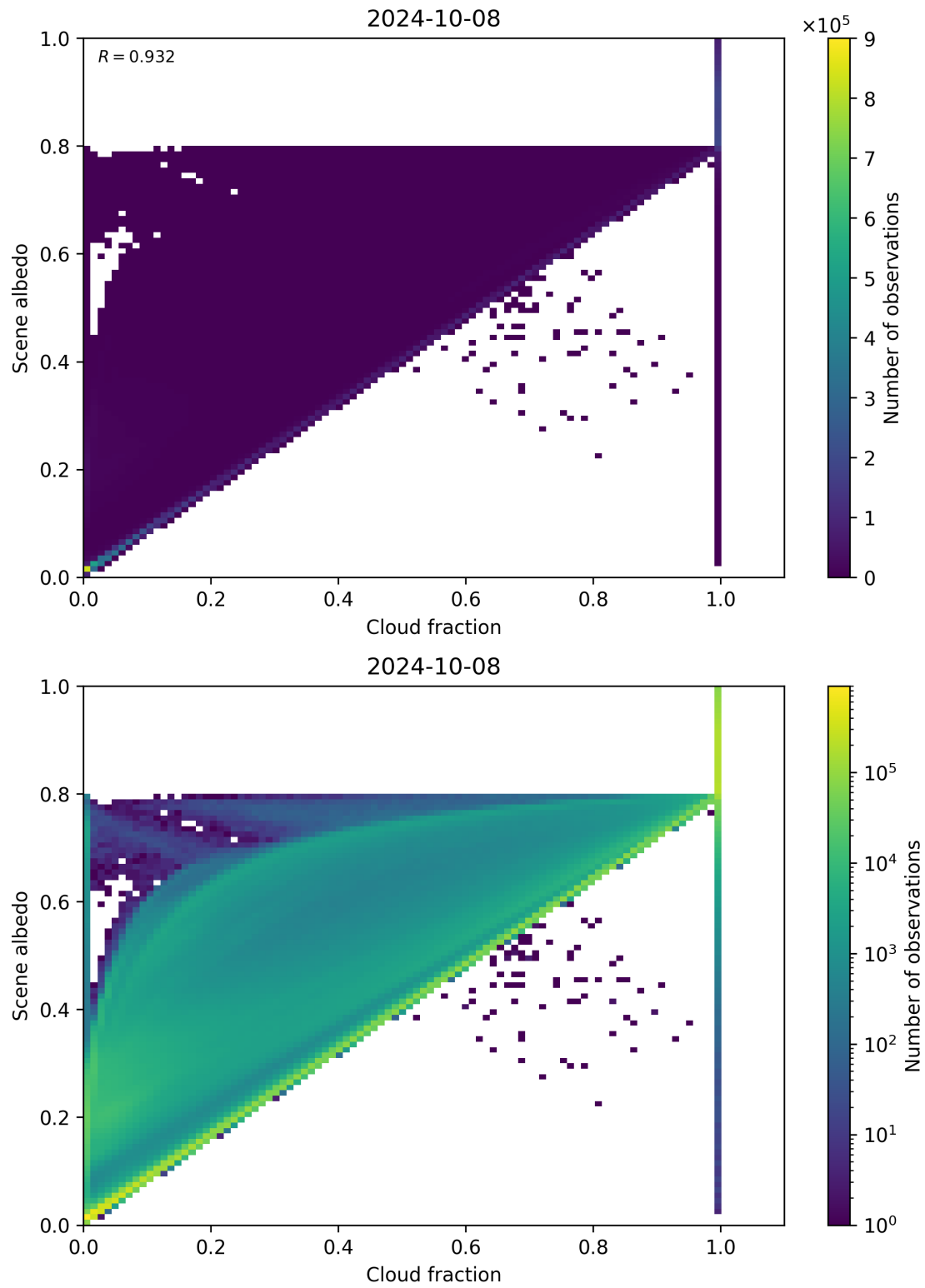
Figure 82: Scatter density plot of “Cloud fraction” against “Scene albedo” for 2024-10-08 to 2024-10-09.
