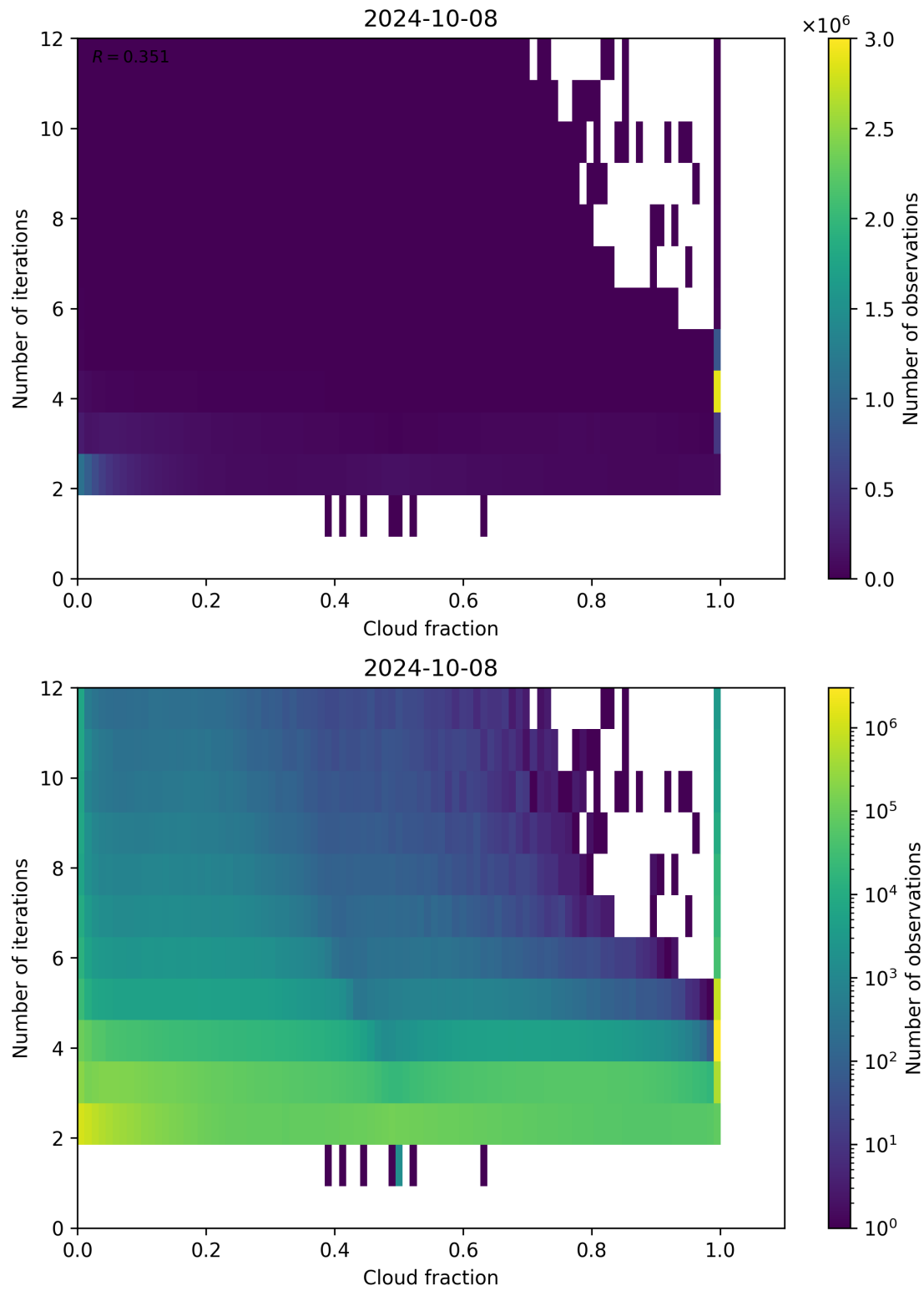
Figure 80: Scatter density plot of “Cloud fraction” against “Number of iterations” for 2024-10-08 to 2024-10-09.
