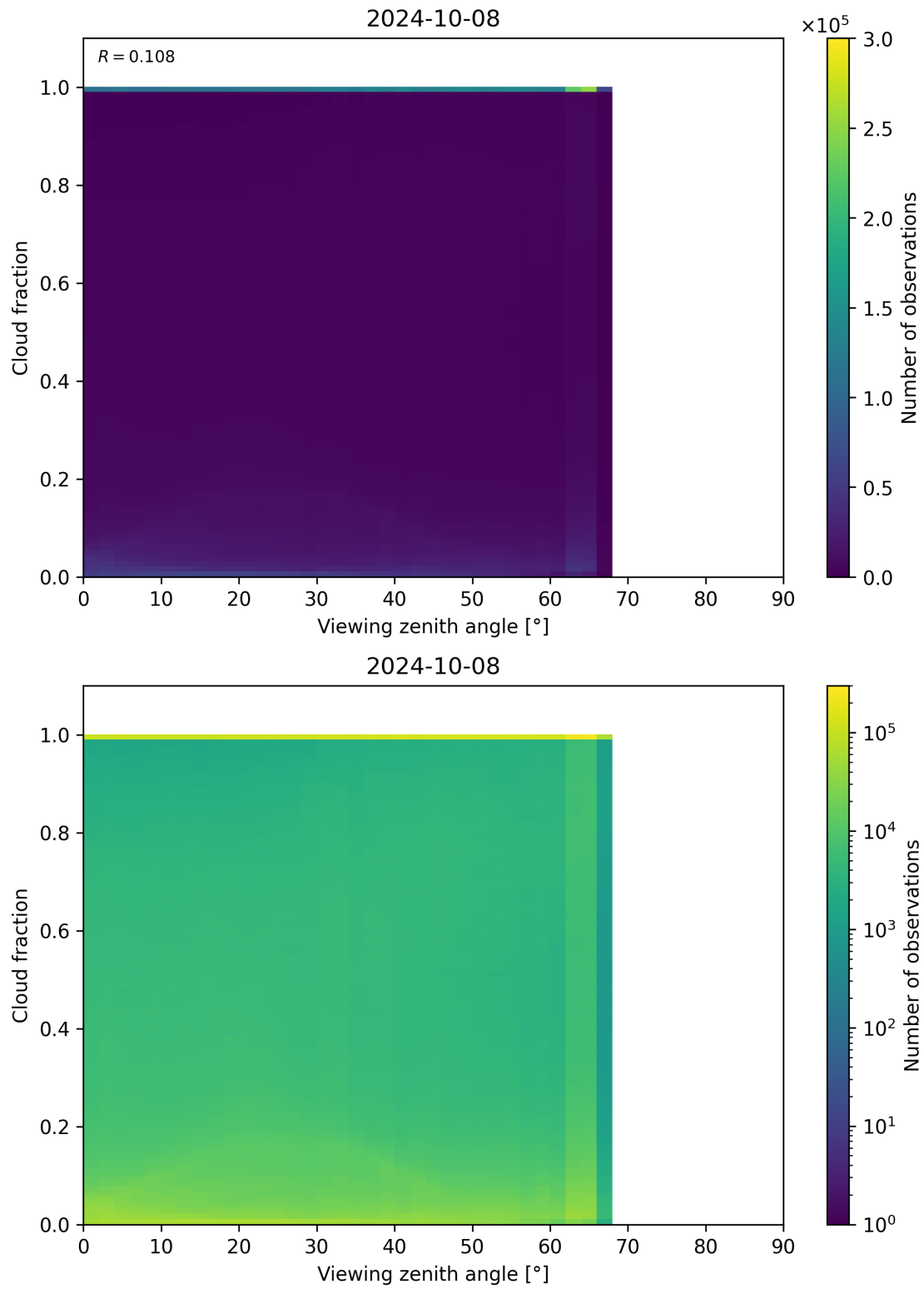
Figure 132: Scatter density plot of “Viewing zenith angle” against “Cloud fraction” for 2024-10-08 to 2024-10-09.
