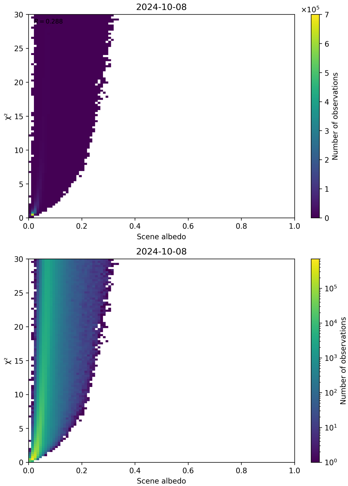
Figure 112: Scatter density plot of “Scene albedo” against “ \chi^2 ” for 2024-10-08 to 2024-10-09.
