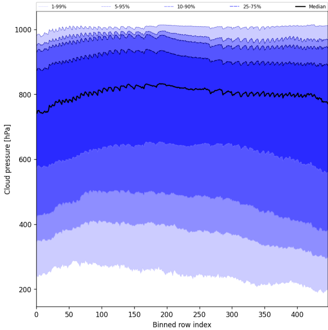
Figure 47: Along track statistics of “Cloud pressure” for 2024-10-08 to 2024-10-09
