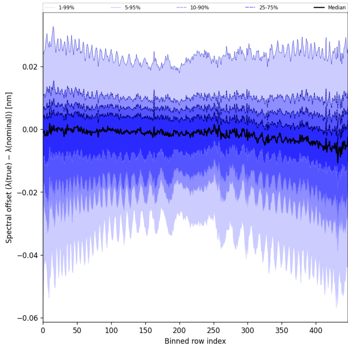
Figure 62: Along track statistics of “Spectral offset ( \lambda_{\text{true}} - \lambda_{\text{nominal}} )” for 2024-10-08 to 2024-10-09
