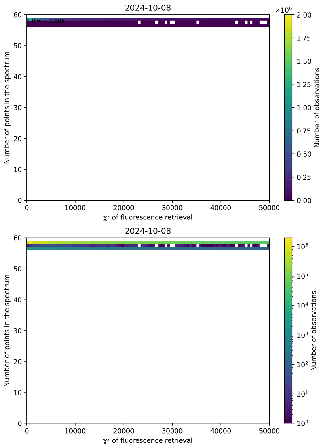
Figure 71: Scatter density plot of “ \chi^2 of fluorescence retrieval” against “Number of points in the spectrum” for 2024-10-08 to 2024-10-09.
