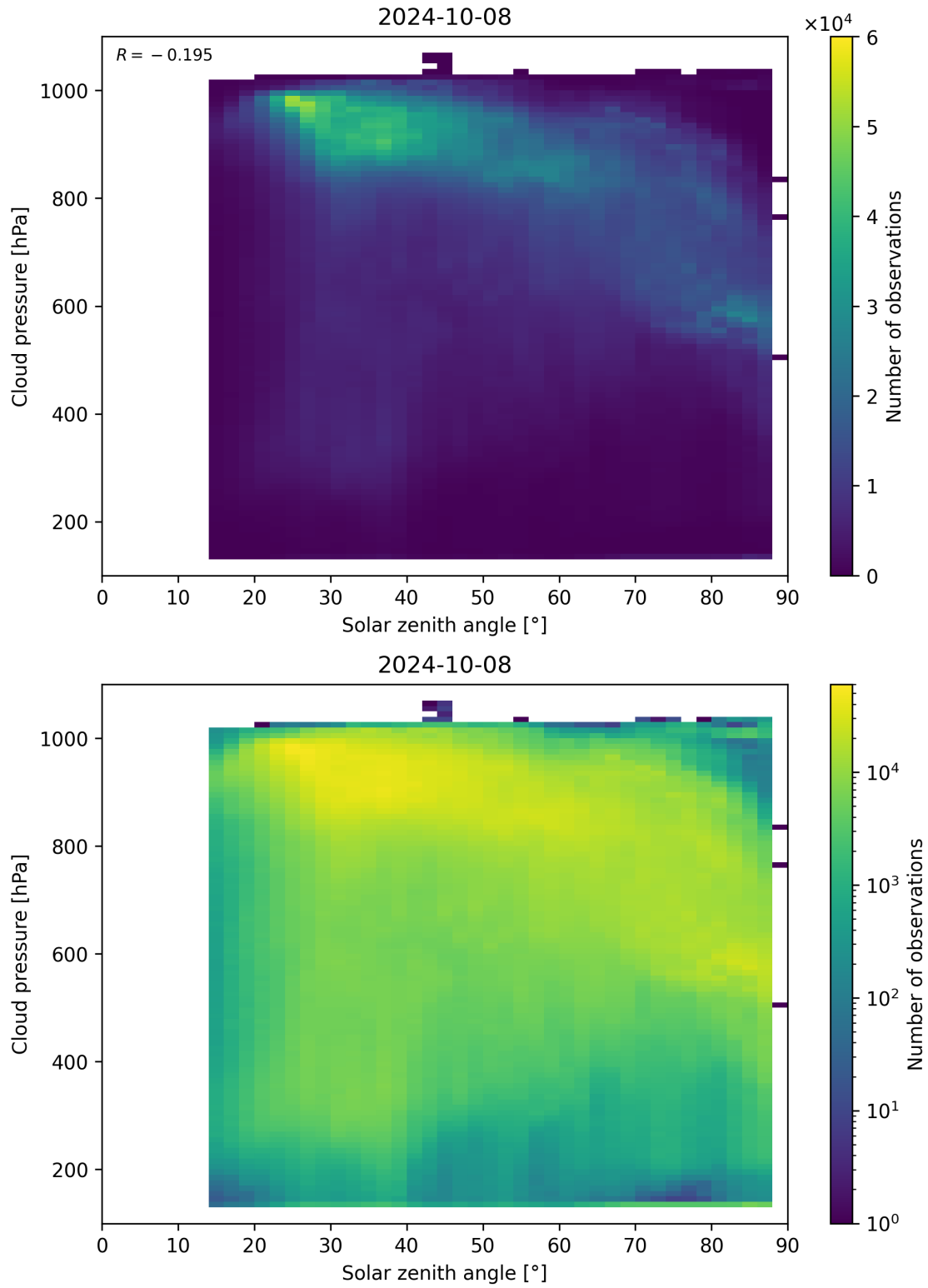
Figure 122: Scatter density plot of “Solar zenith angle” against “Cloud pressure” for 2024-10-08 to 2024-10-09.
