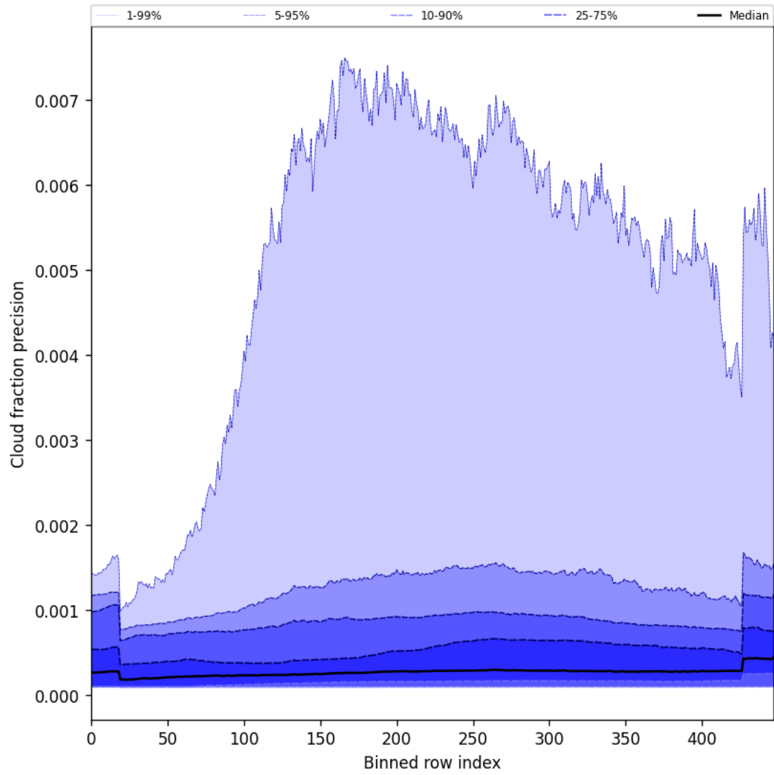
Figure 50: Along track statistics of “Cloud fraction precision” for 2024-10-08 to 2024-10-09
