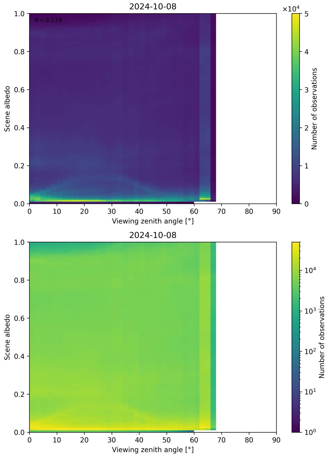
Figure 138: Scatter density plot of “Viewing zenith angle” against “Scene albedo” for 2024-10-08 to 2024-10-09.
