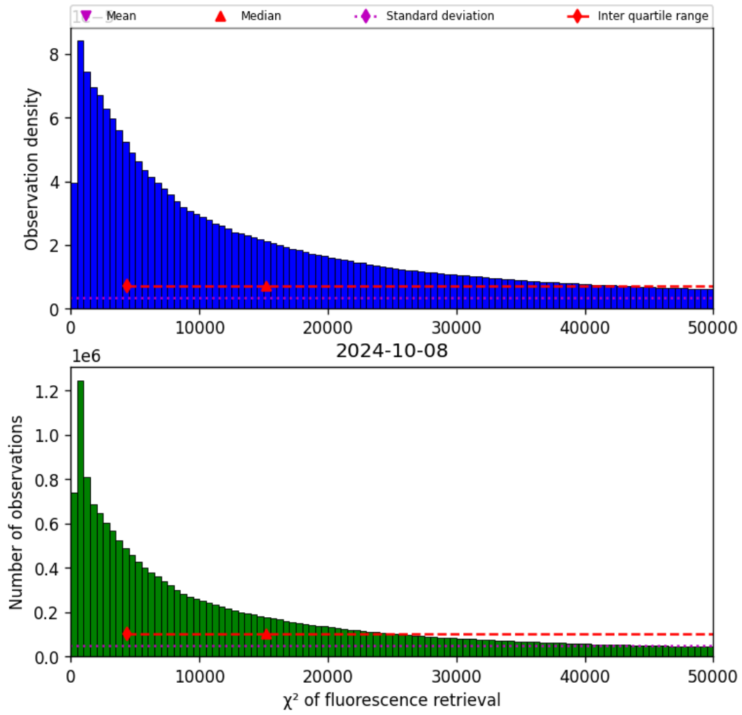
Figure 42: Histogram of “ \chi^2 of fluorescence retrieval” for 2024-10-08 to 2024-10-09
