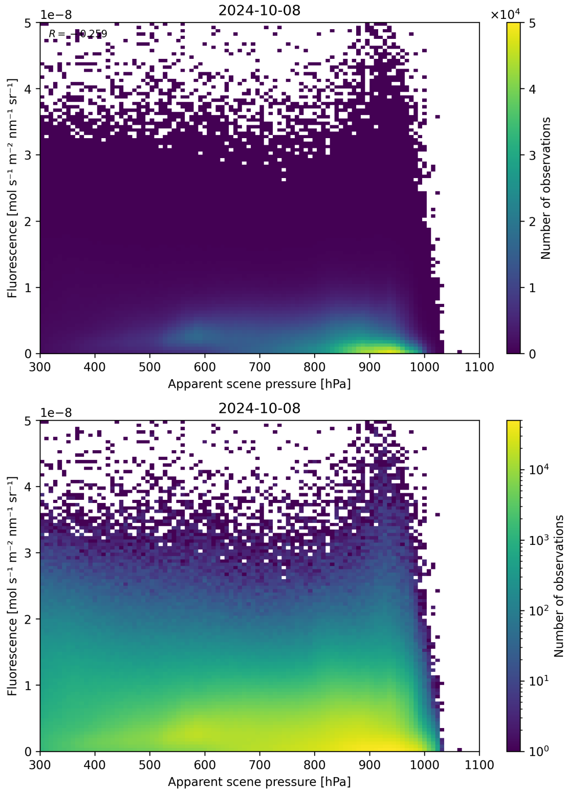
Figure 65: Scatter density plot of “Apparent scene pressure” against “Fluorescence” for 2024-10-08 to 2024-10-09.
