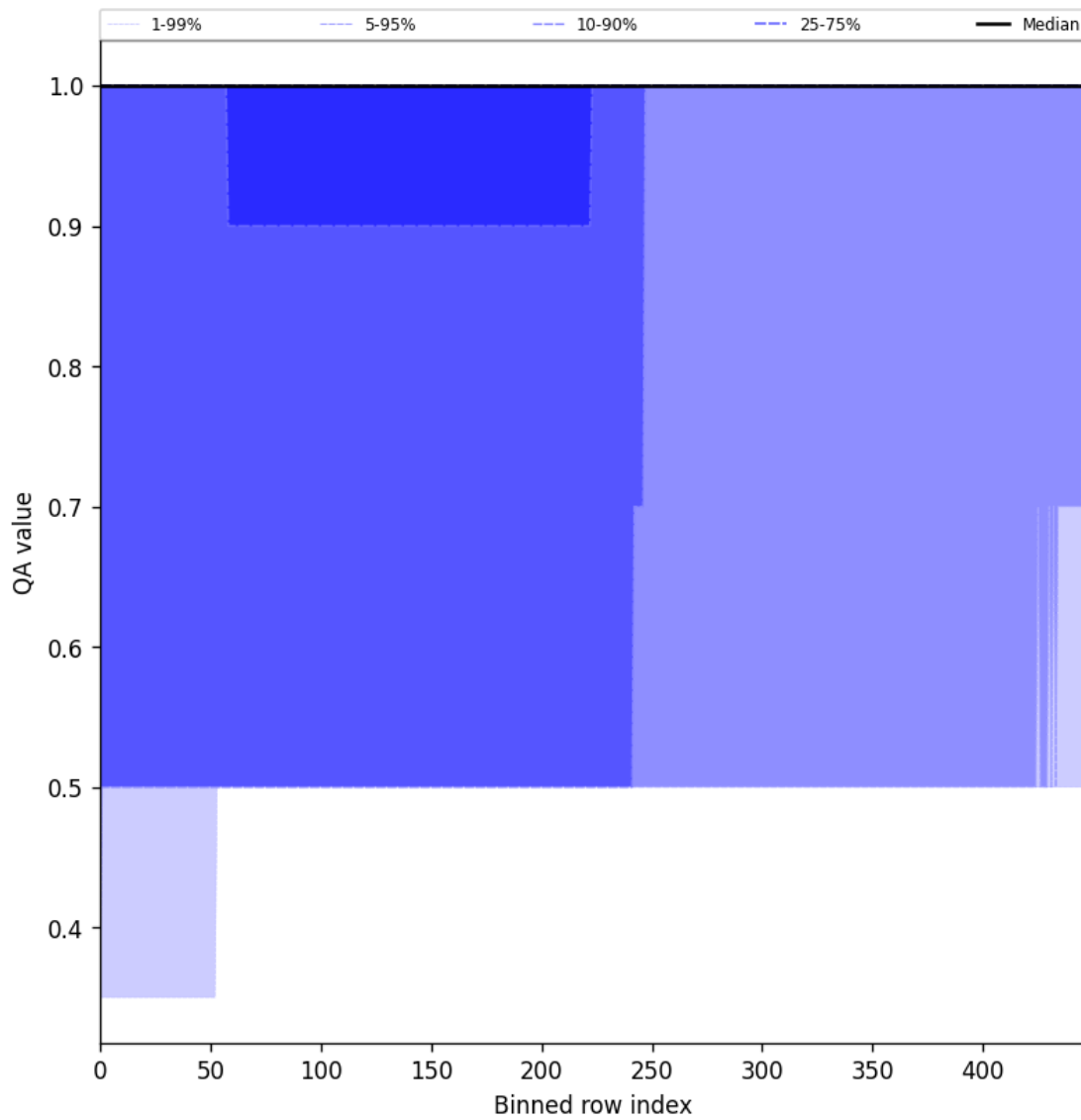
Figure 46: Along track statistics of “QA value” for 2024-10-08 to 2024-10-09
