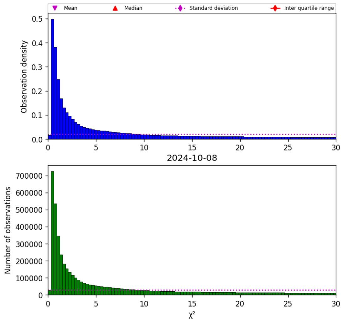
Figure 38: Histogram of " \chi^2 " for 2024-10-08 to 2024-10-09
