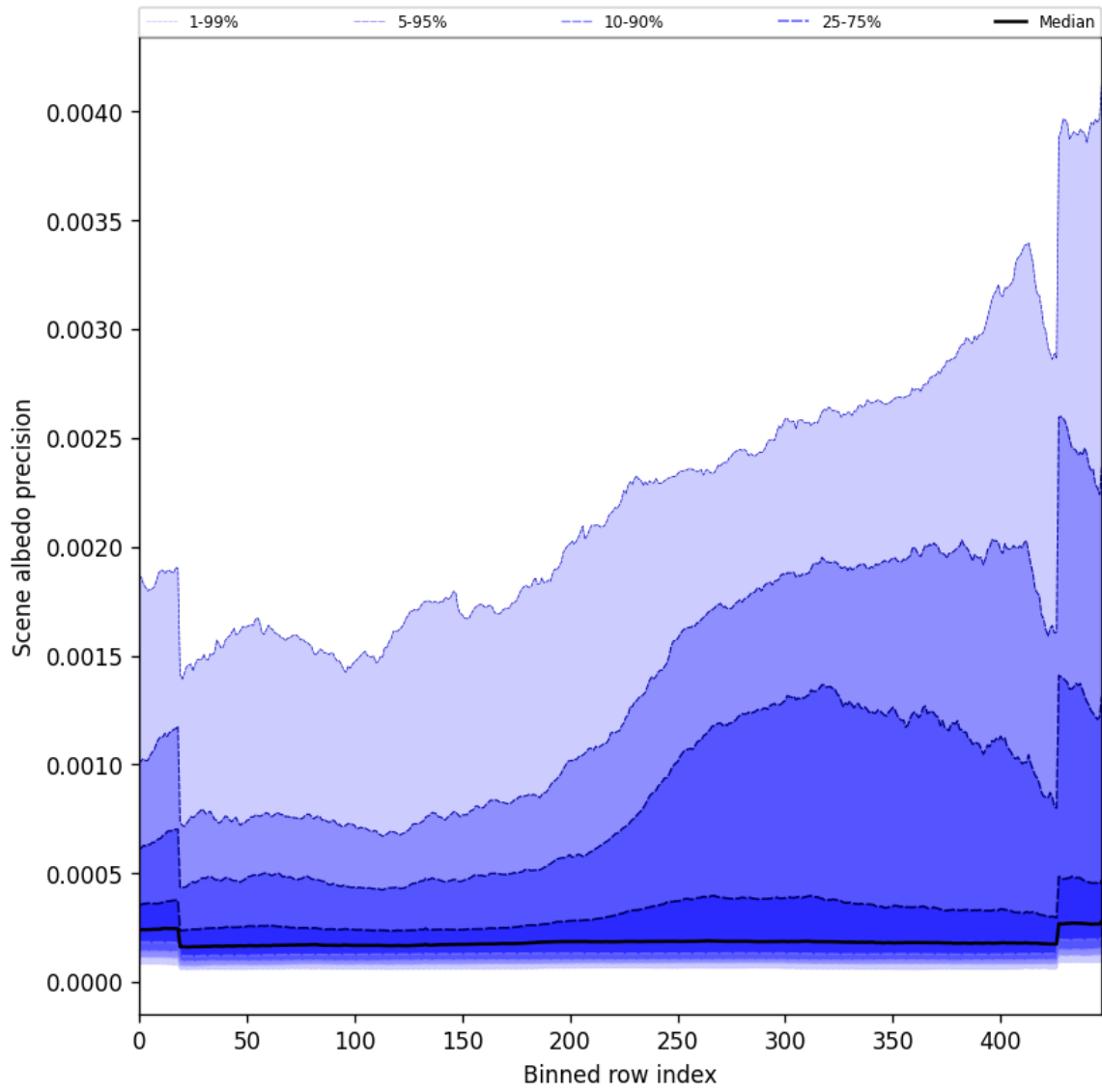
Figure 52: Along track statistics of “Scene albedo precision” for 2024-10-08 to 2024-10-09
