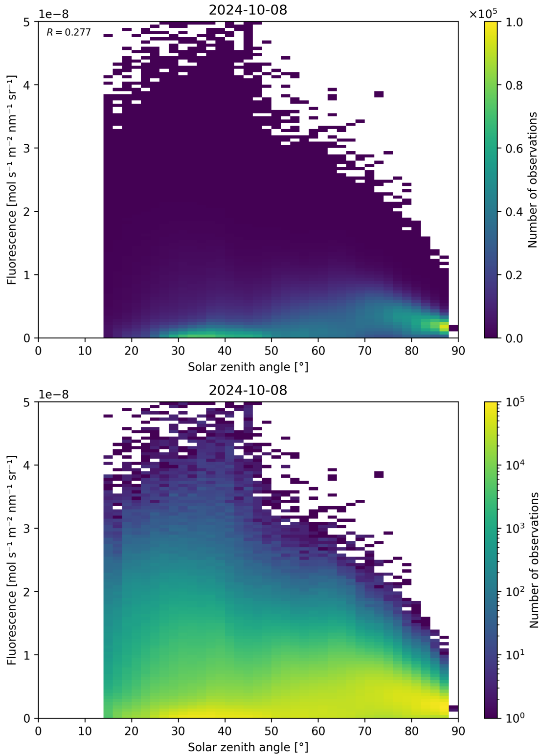
Figure 123: Scatter density plot of “Solar zenith angle” against “Fluorescence” for 2024-10-08 to 2024-10-09.
