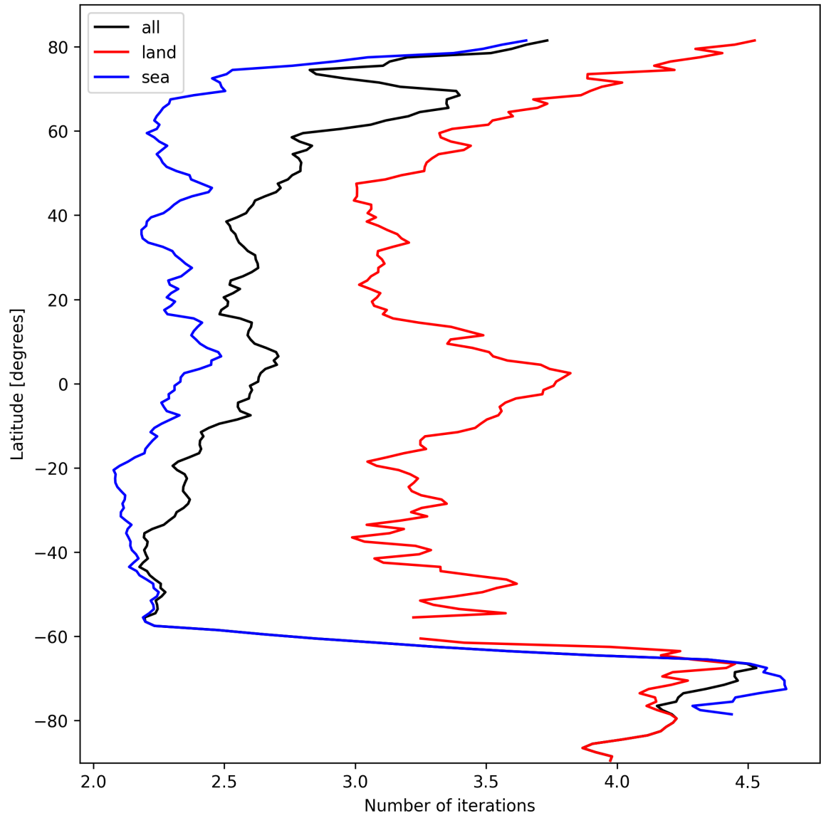
Figure 22: Zonal average of “Number of iterations” for 2024-10-08 to 2024-10-09.
