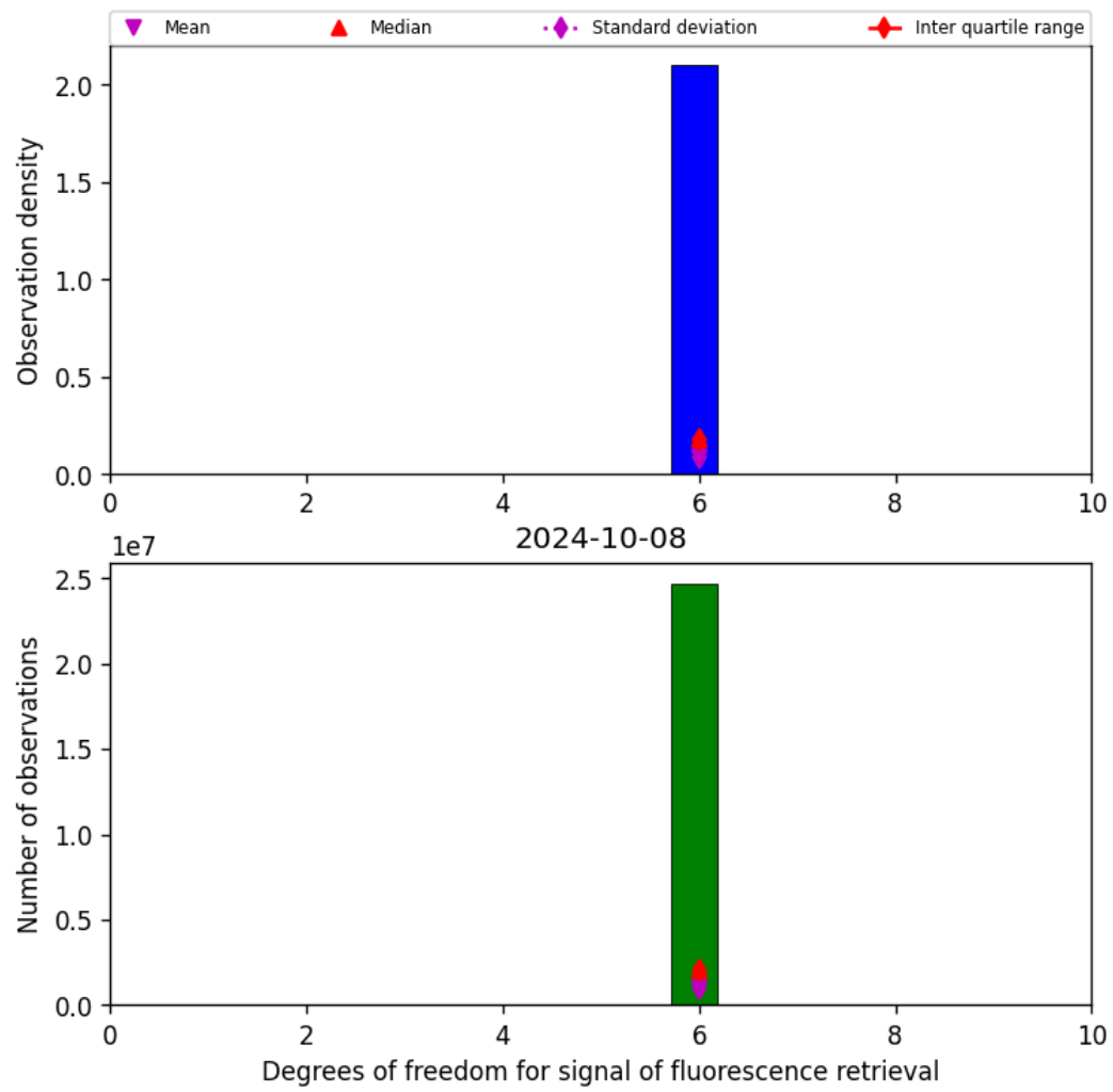
Figure 43: Histogram of “Degrees of freedom for signal of fluorescence retrieval” for 2024-10-08 to 2024-10-09
