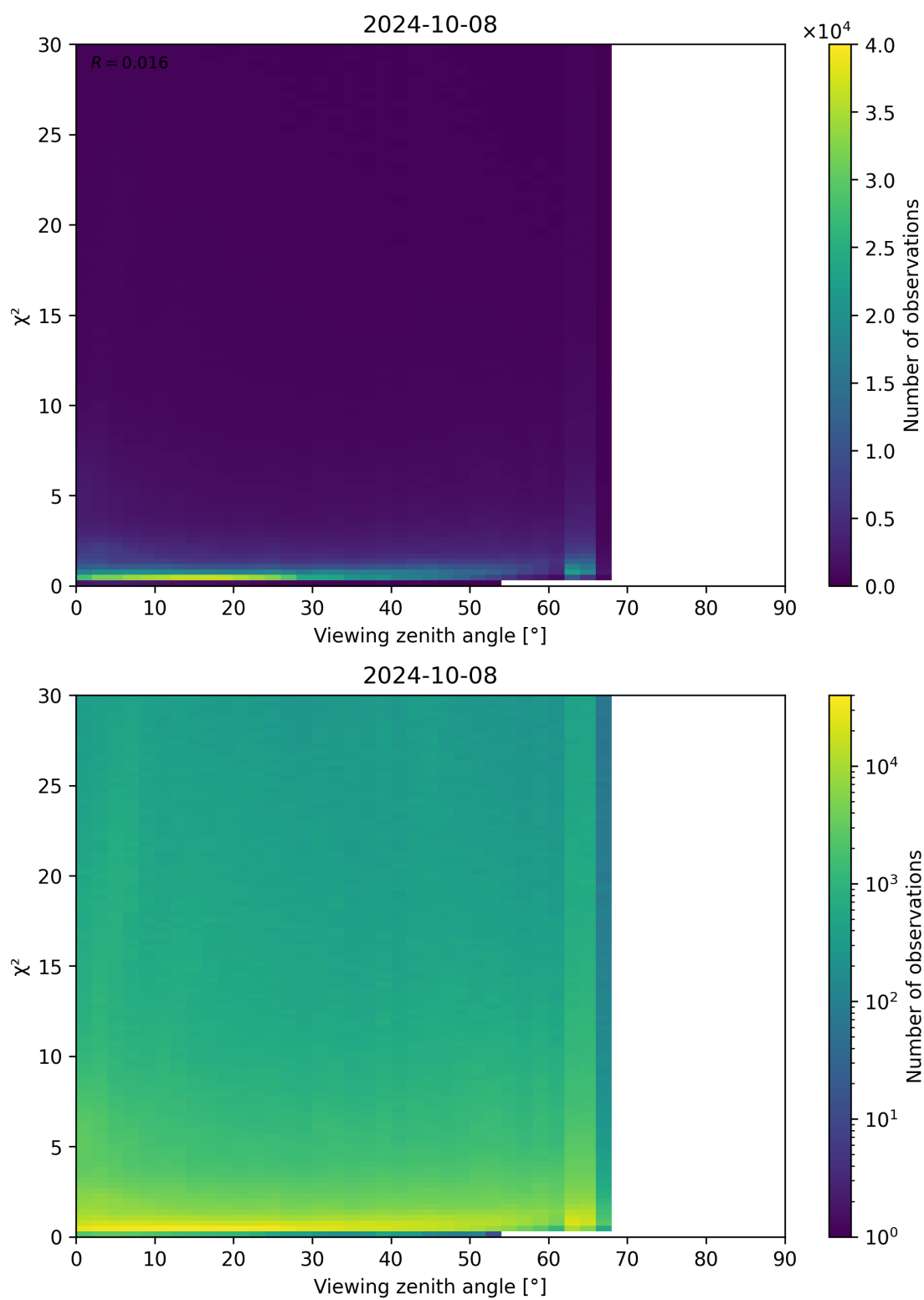
Figure 130: Scatter density plot of “Viewing zenith angle” against “ \chi^2 ” for 2024-10-08 to 2024-10-09.
