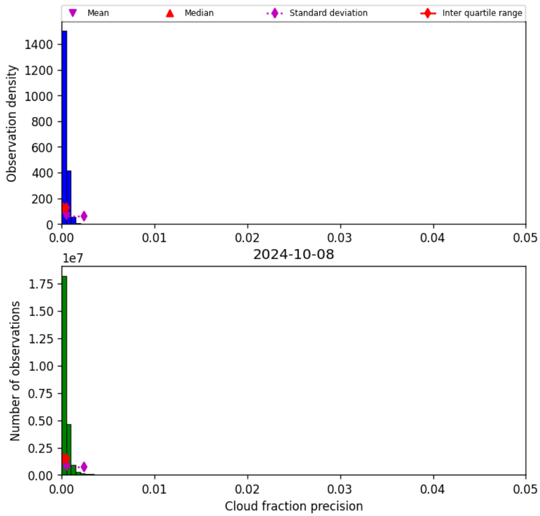
Figure 33: Histogram of “Cloud fraction precision” for 2024-10-08 to 2024-10-09
