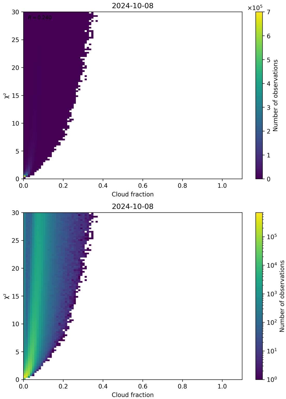
Figure 77: Scatter density plot of “Cloud fraction” against “ \chi^2 ” for 2024-10-08 to 2024-10-09.
