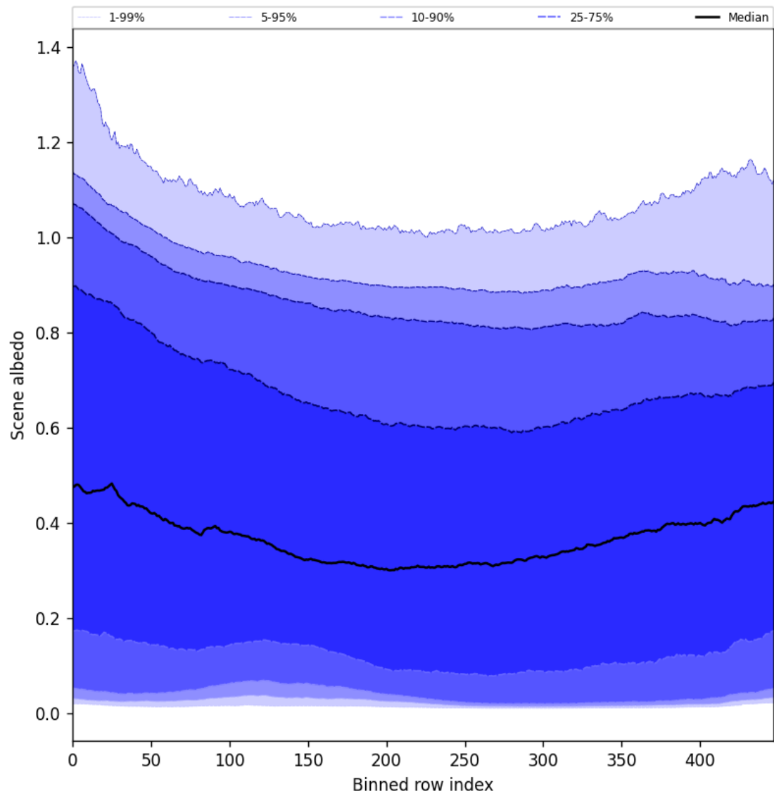
Figure 51: Along track statistics of “Scene albedo” for 2024-10-08 to 2024-10-09
