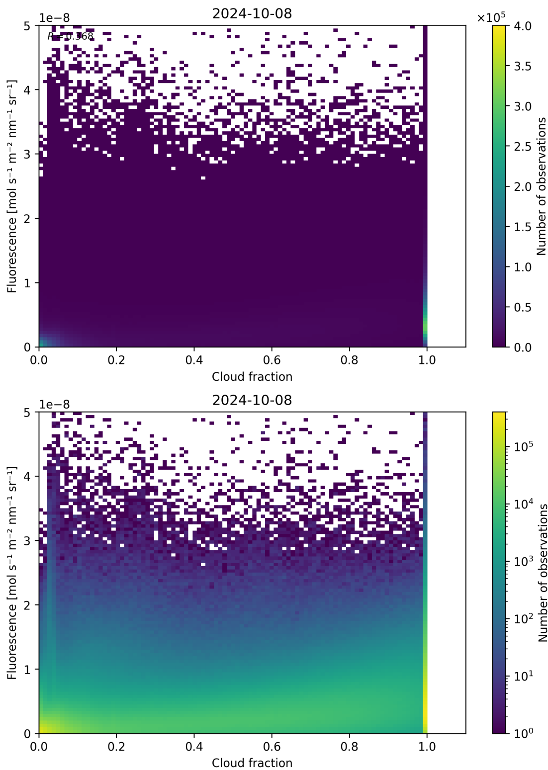
Figure 79: Scatter density plot of “Cloud fraction” against “Fluorescence” for 2024-10-08 to 2024-10-09.
