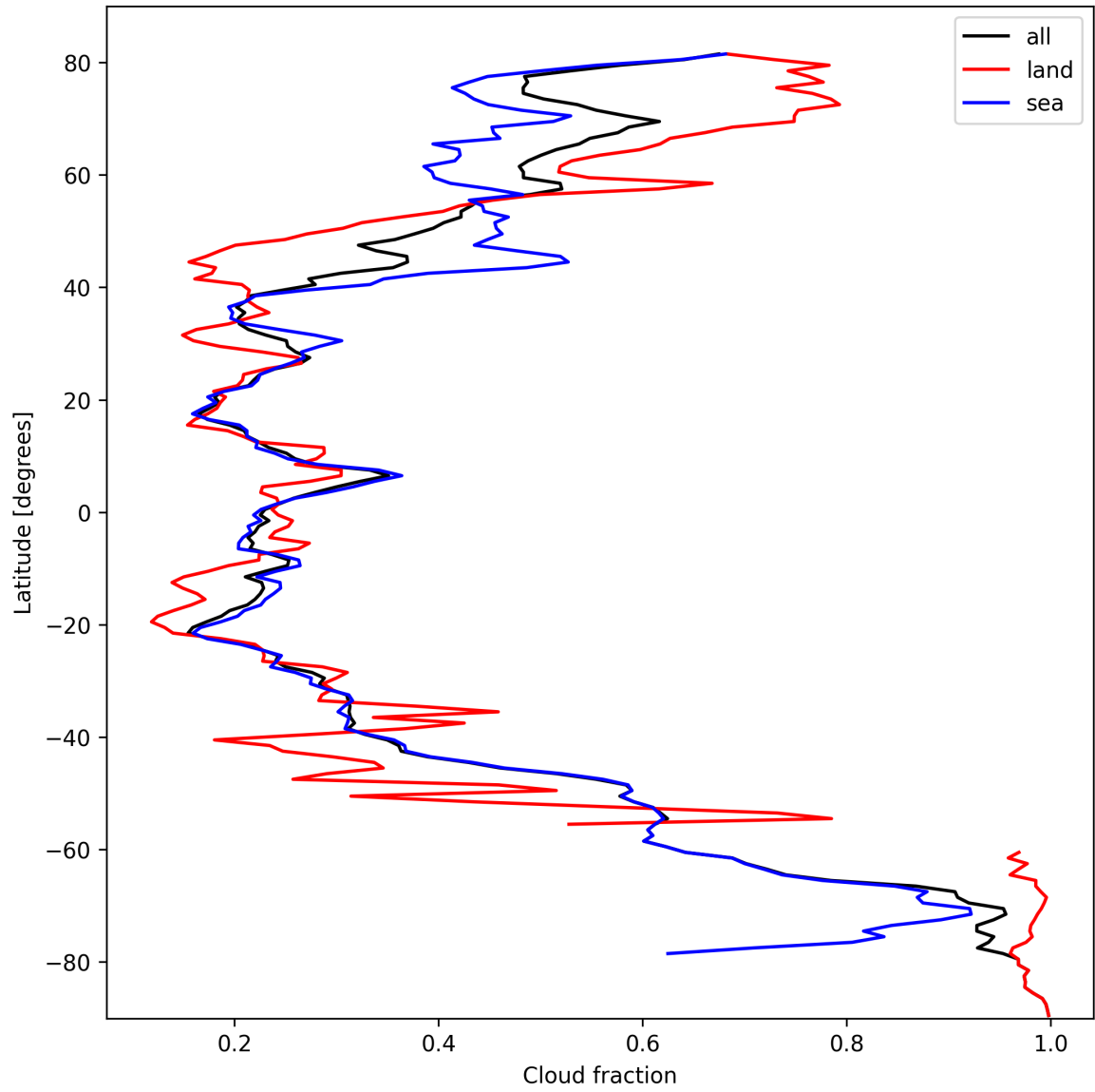
Figure 15: Zonal average of “Cloud fraction” for 2024-10-08 to 2024-10-09.
