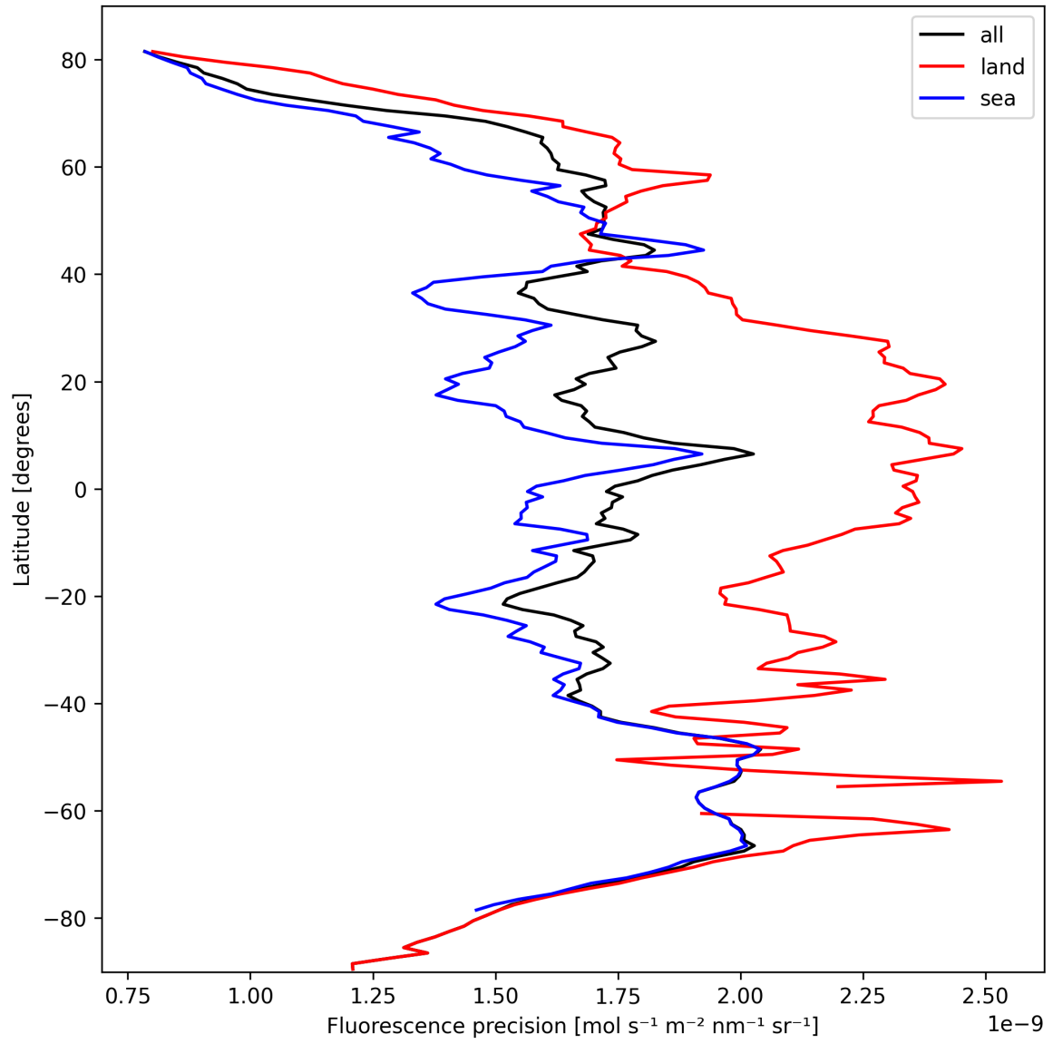
Figure 24: Zonal average of “Fluorescence precision” for 2024-10-08 to 2024-10-09.
