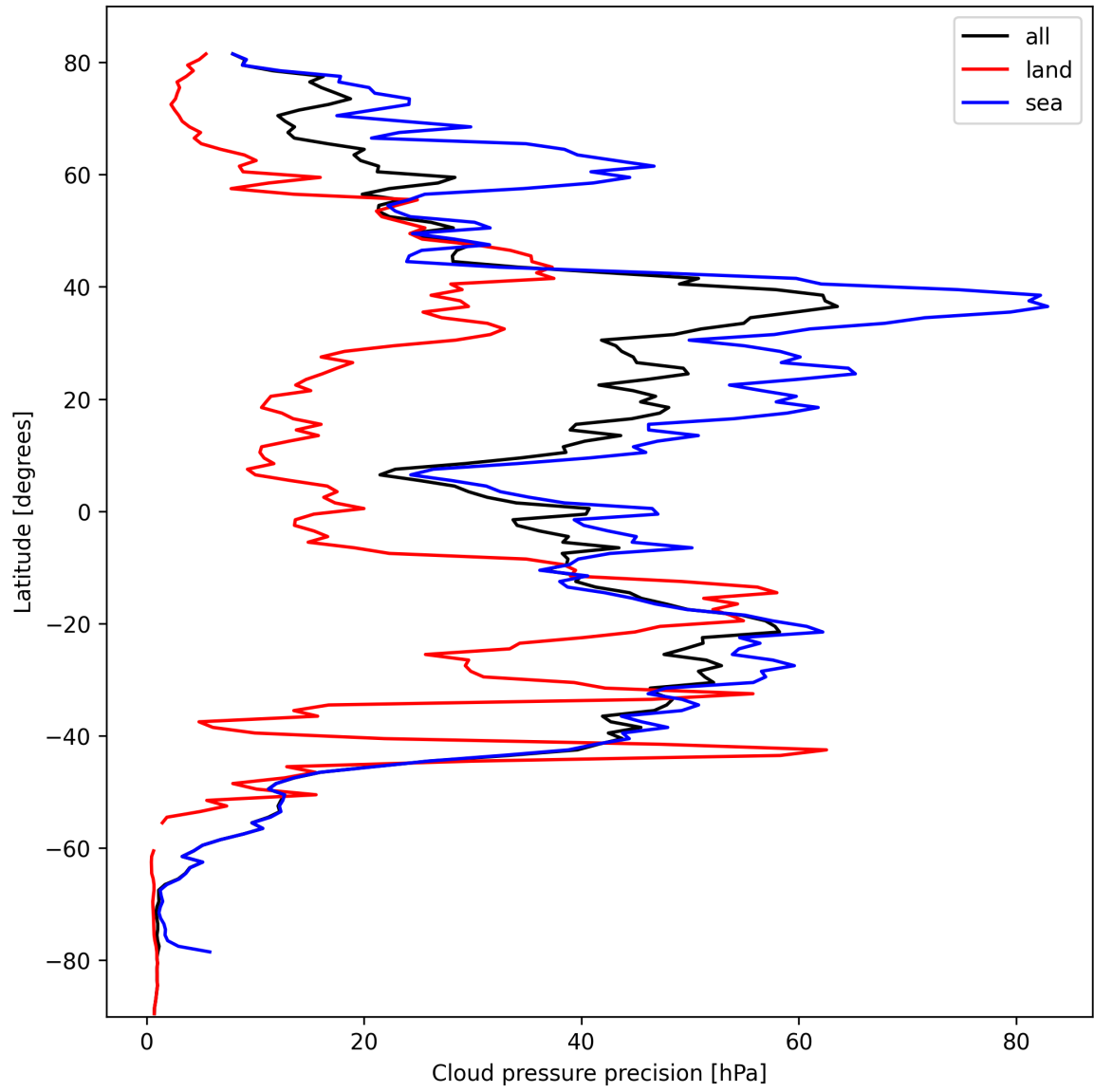
Figure 14: Zonal average of “Cloud pressure precision” for 2024-10-08 to 2024-10-09.
