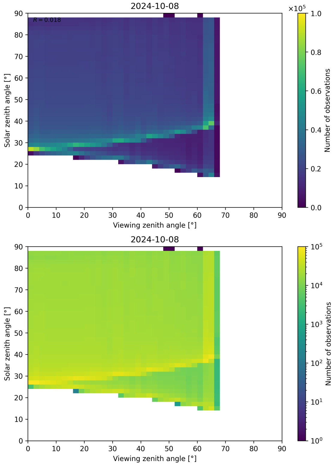
Figure 139: Scatter density plot of “Viewing zenith angle” against “Solar zenith angle” for 2024-10-08 to 2024-10-09.
