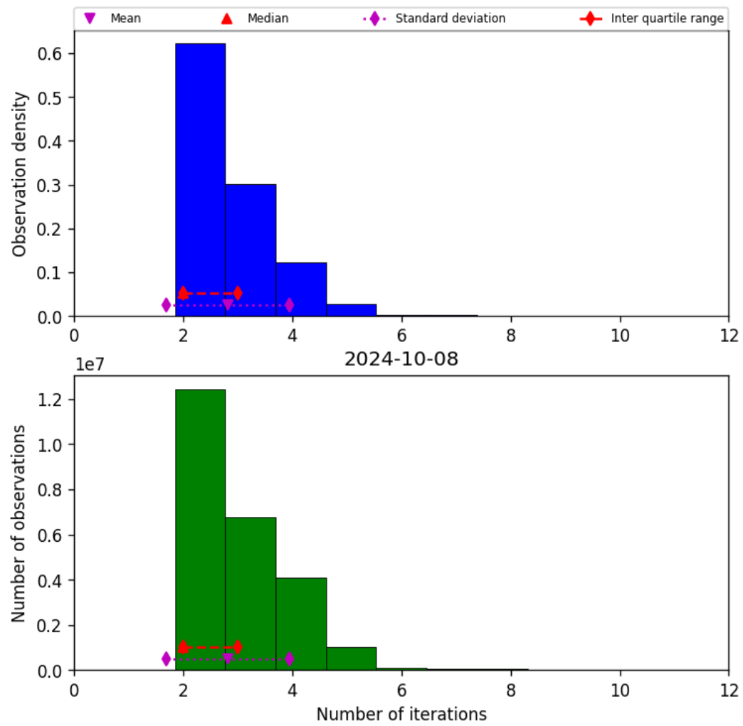
Figure 39: Histogram of “Number of iterations” for 2024-10-08 to 2024-10-09
