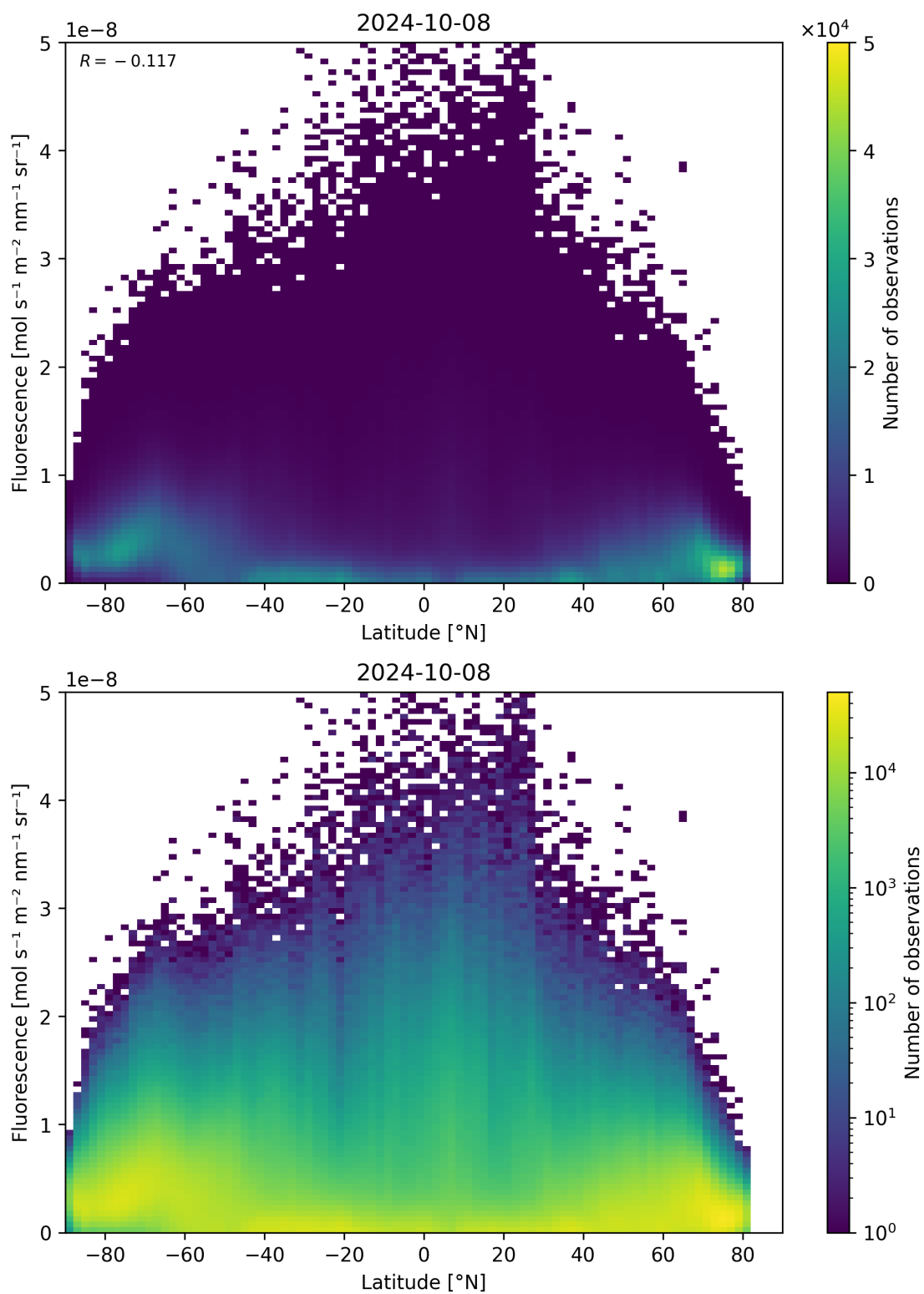
Figure 101: Scatter density plot of “Latitude” against “Fluorescence” for 2024-10-08 to 2024-10-09.
