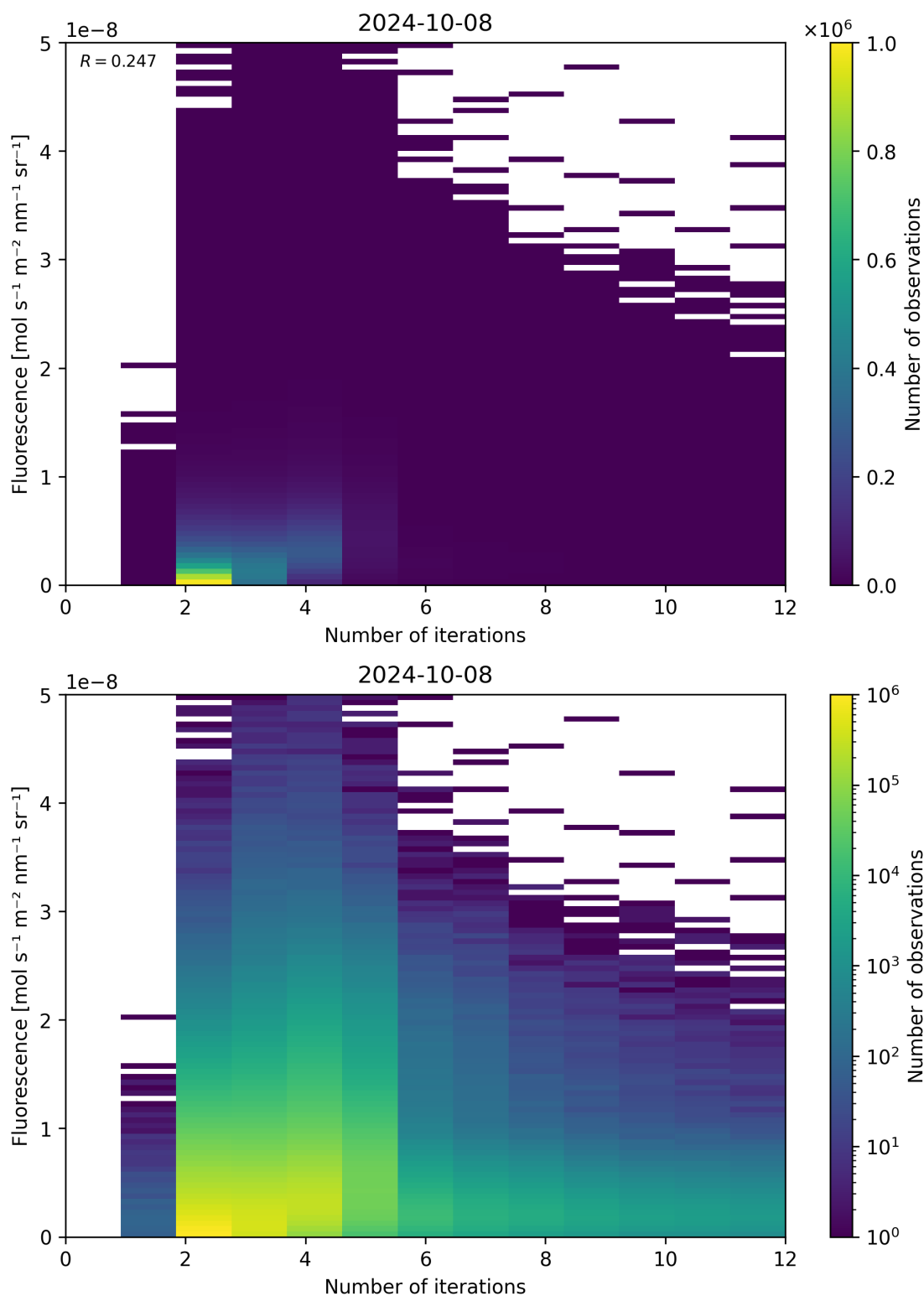
Figure 107: Scatter density plot of “Number of iterations” against “Fluorescence” for 2024-10-08 to 2024-10-09.
