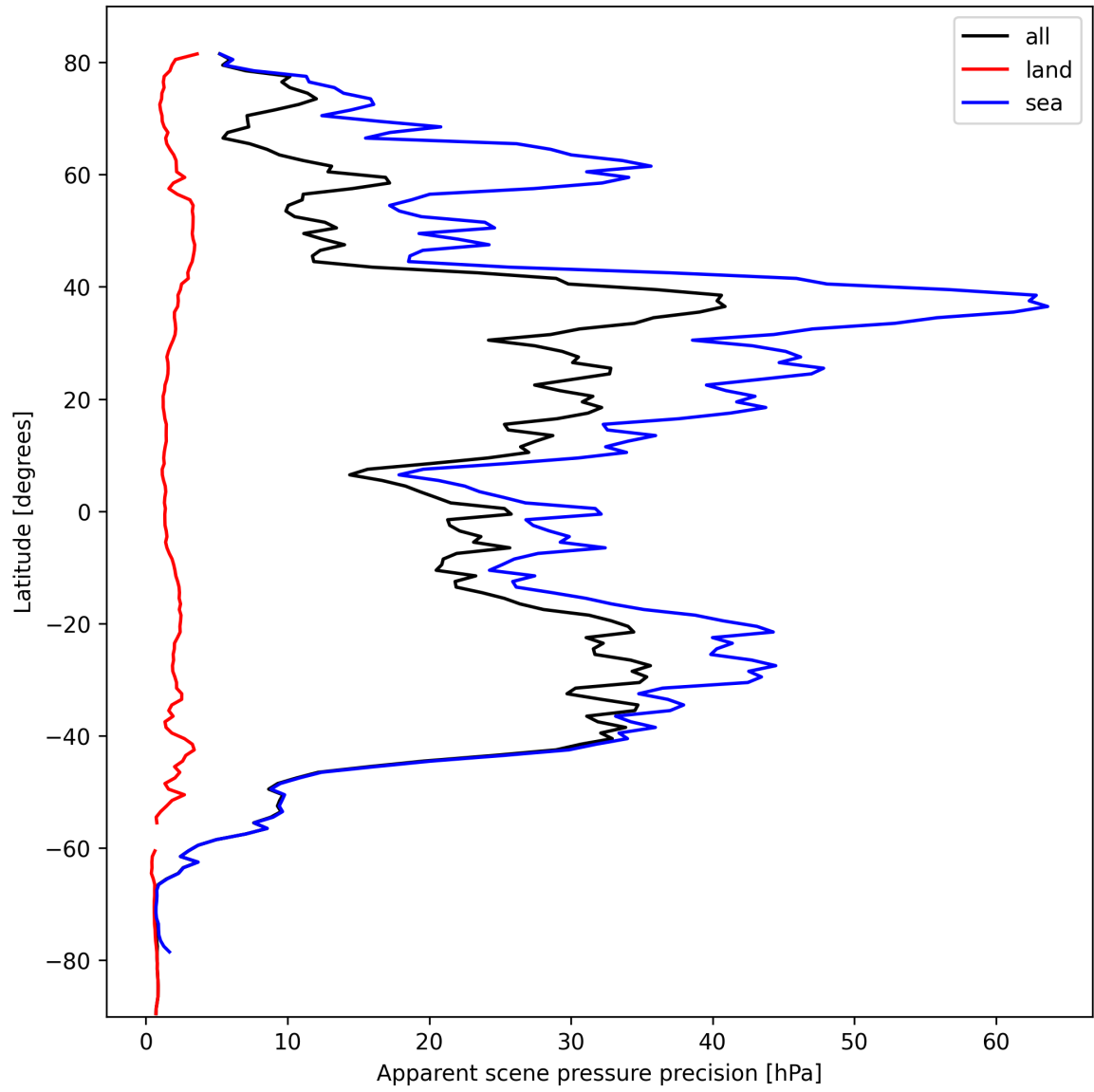
Figure 20: Zonal average of “Apparent scene pressure precision” for 2024-10-08 to 2024-10-09.
