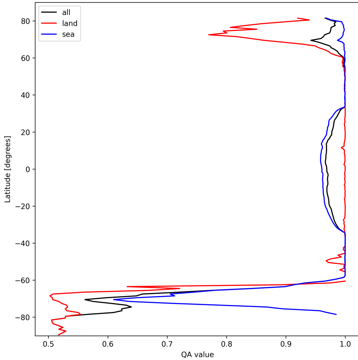
Figure 12: Zonal average of “QA value” for 2024-10-08 to 2024-10-09.
