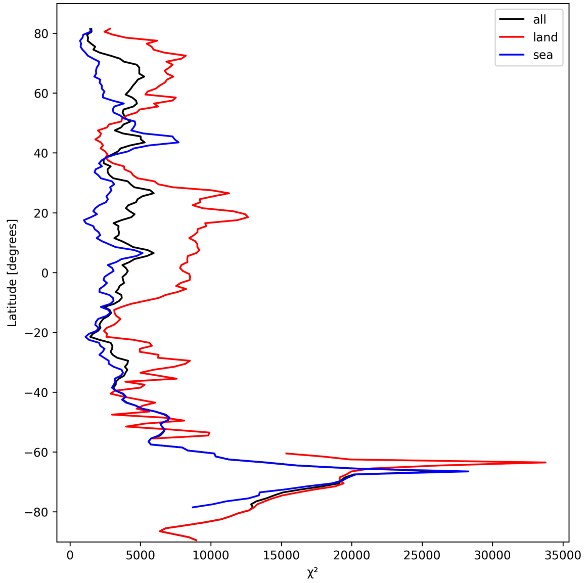
Figure 21: Zonal average of “ \chi^2 ” for 2024-10-08 to 2024-10-09.
