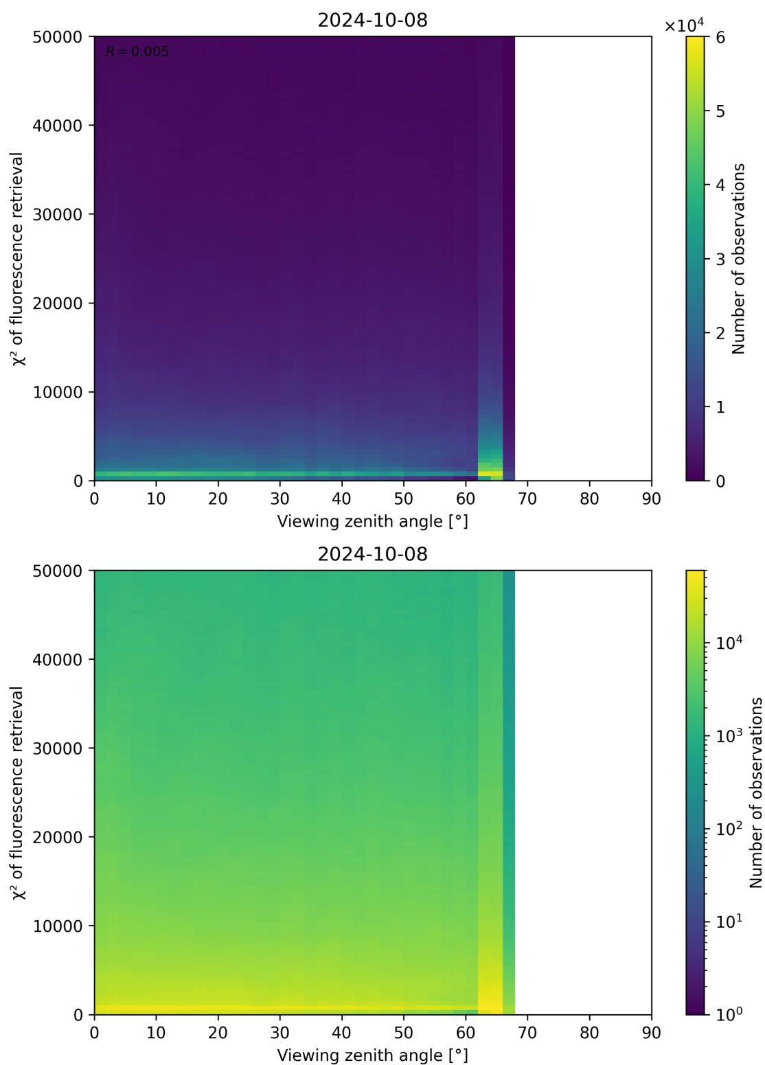
Figure 131: Scatter density plot of “Viewing zenith angle” against “ \chi^2 of fluorescence retrieval” for 2024-10-08 to 2024-10-09.
