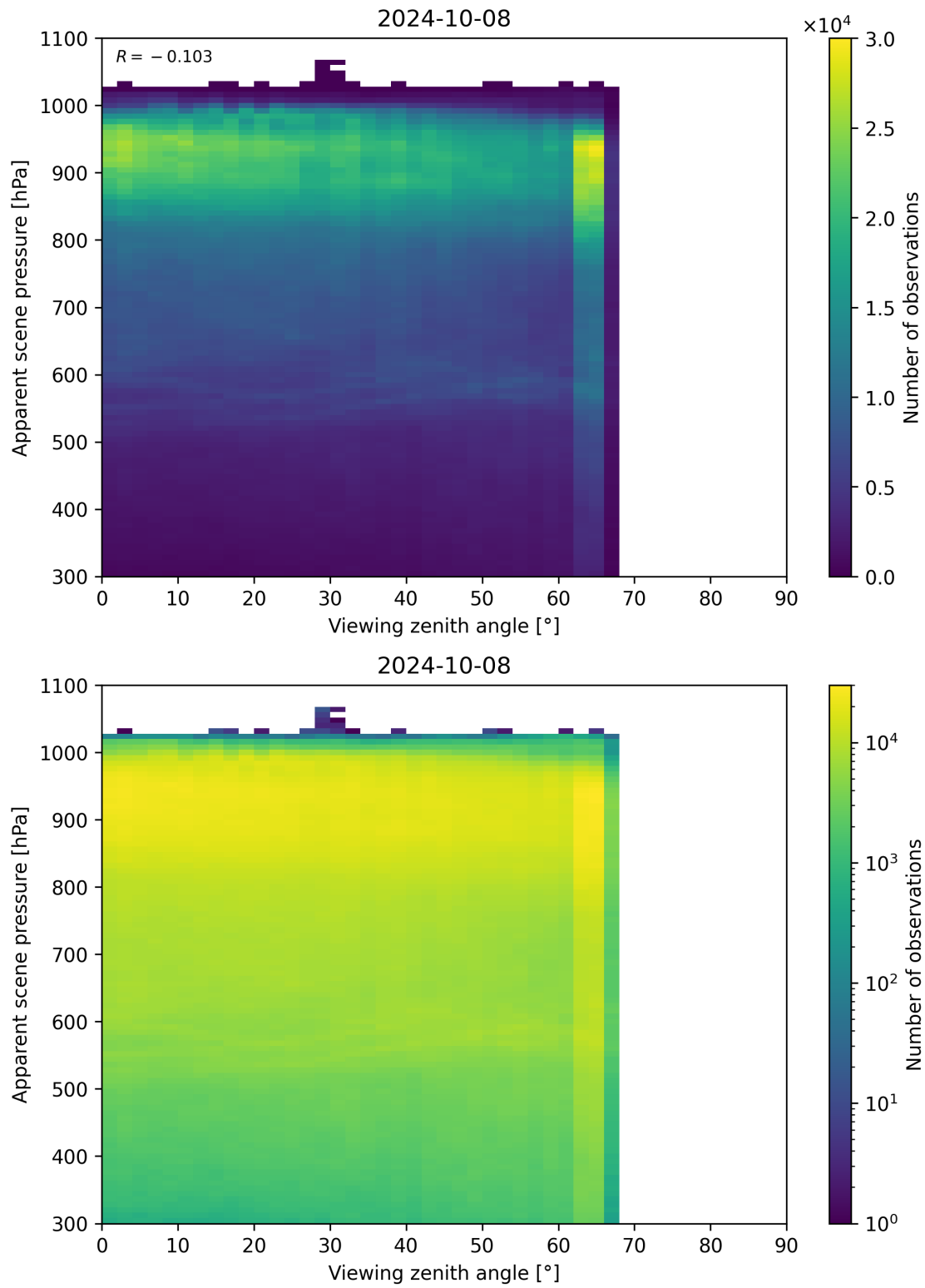
Figure 129: Scatter density plot of “Viewing zenith angle” against “Apparent scene pressure” for 2024-10-08 to 2024-10-09.
