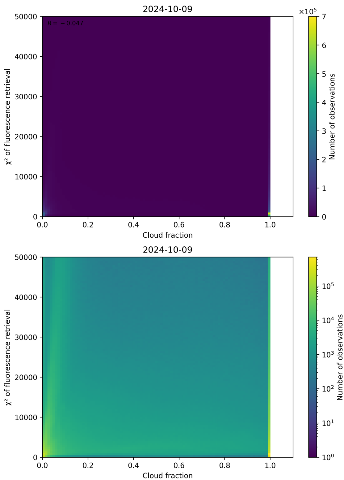
Figure 78: Scatter density plot of “Cloud fraction” against “ \chi^2 of fluorescence retrieval” for 2024-10-08 to 2024-10-10.
