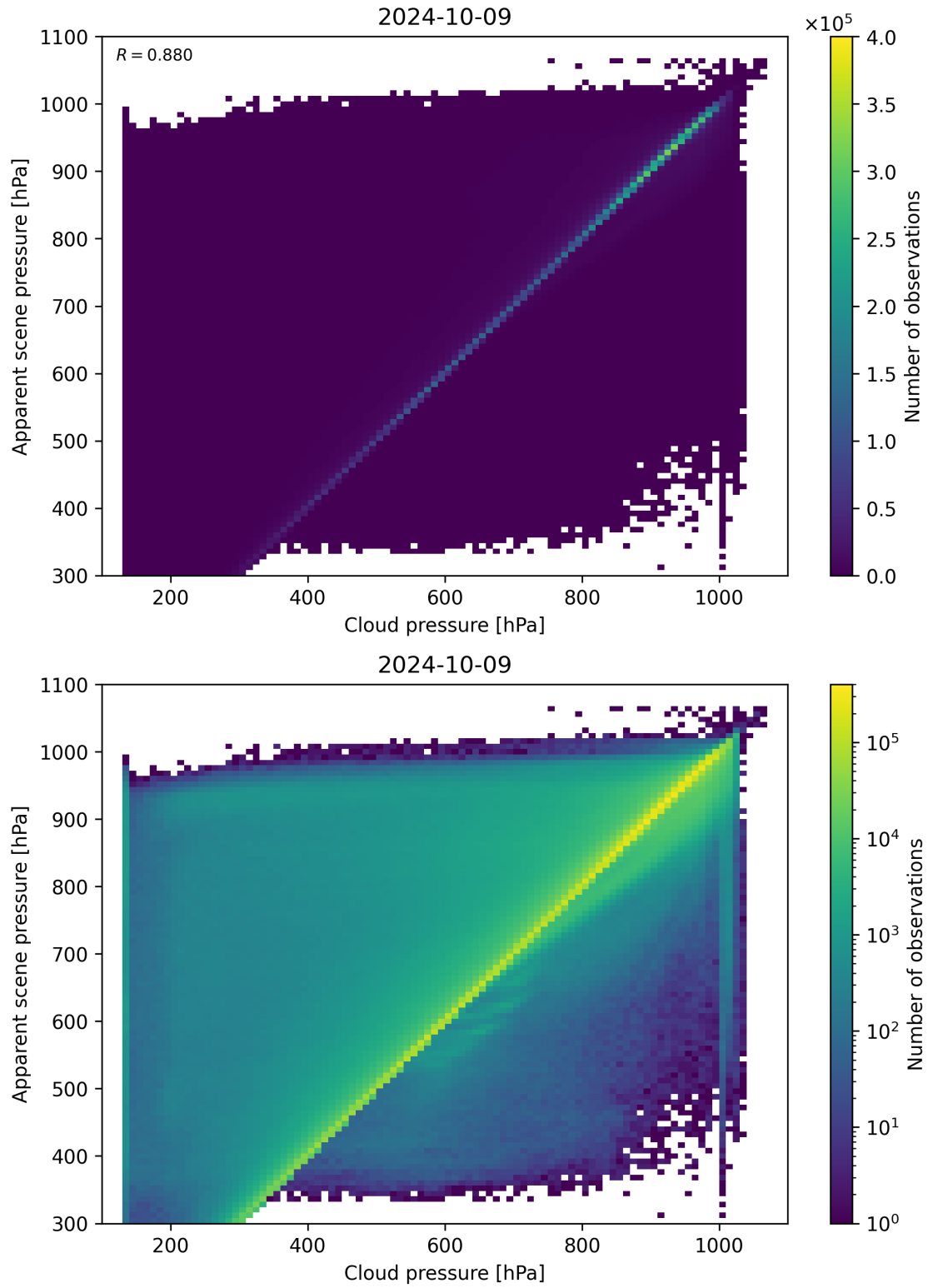
Figure 84: Scatter density plot of “Cloud pressure” against “Apparent scene pressure” for 2024-10-08 to 2024-10-10.
