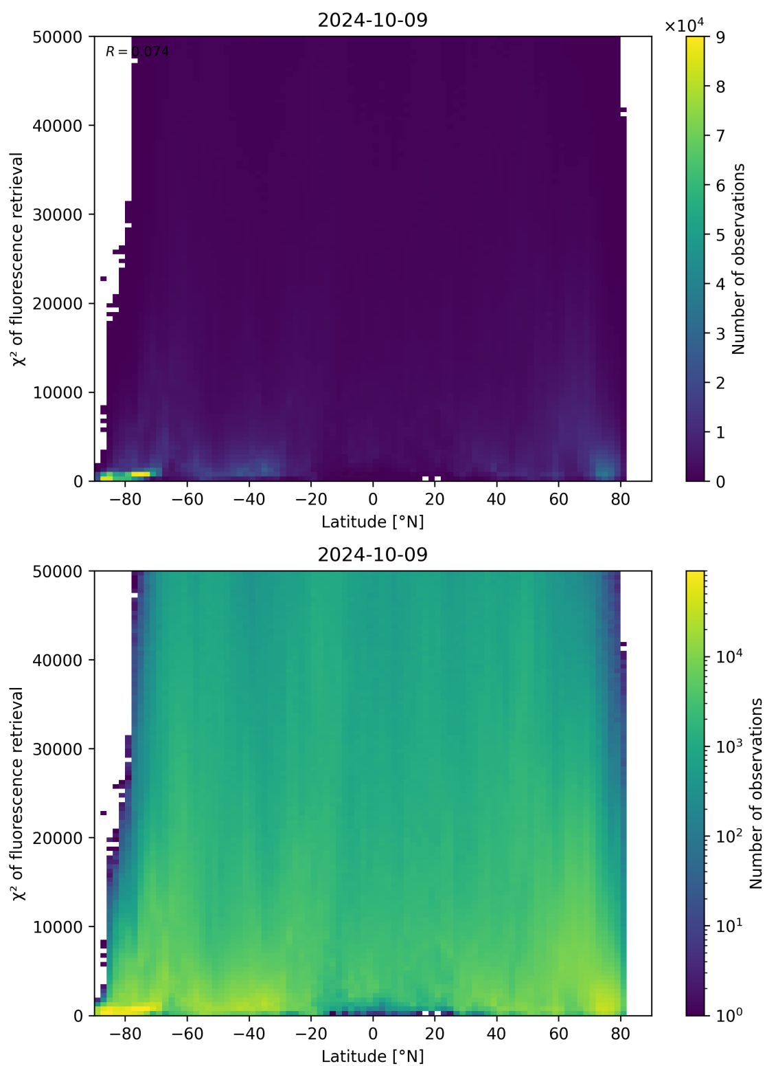
Figure 98: Scatter density plot of “Latitude” against “ \chi^2 of fluorescence retrieval” for 2024-10-08 to 2024-10-10.
