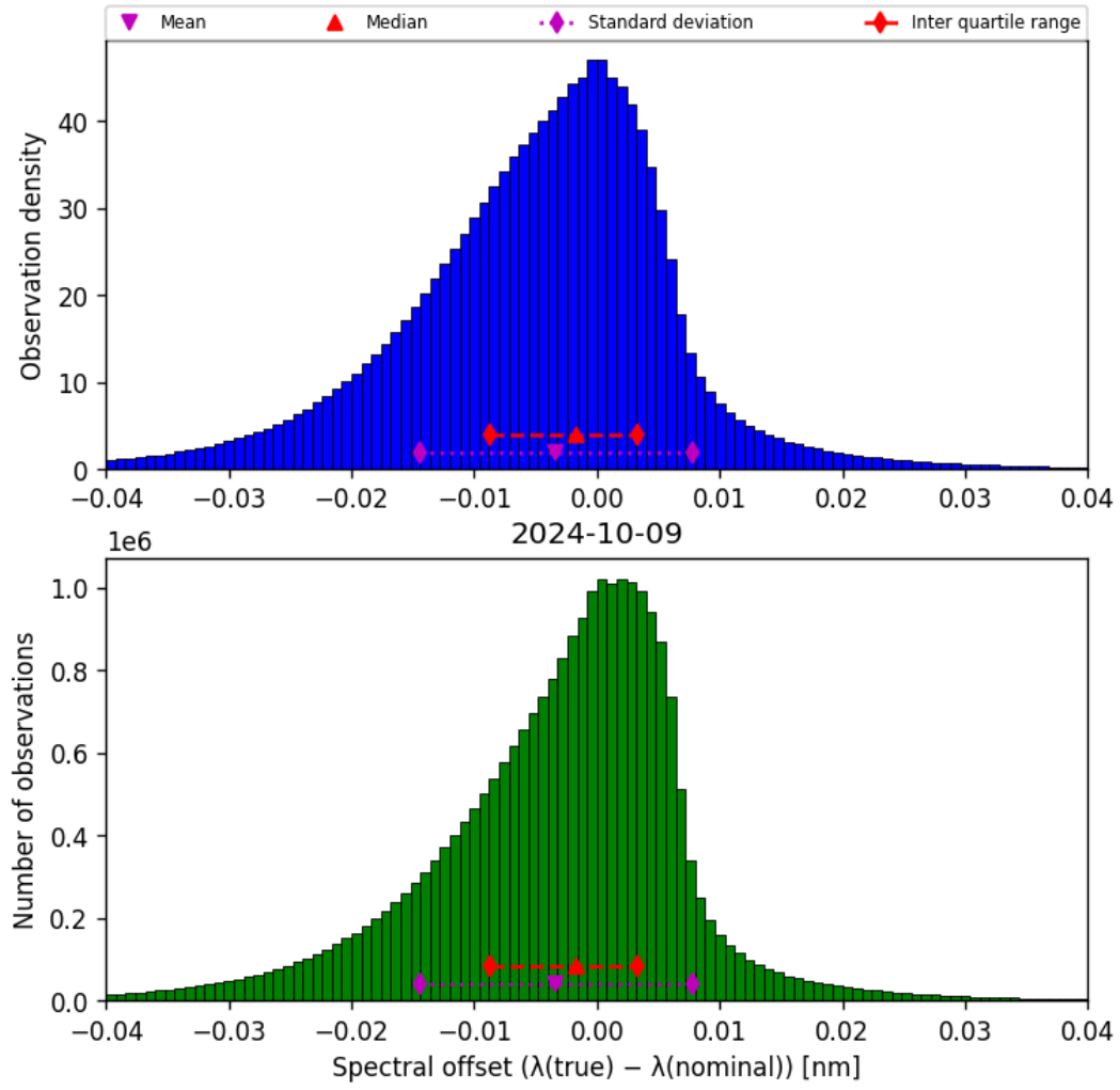
Figure 45: Histogram of “Spectral offset ( \lambda_{\text{true}} - \lambda_{\text{nominal}} )” for 2024-10-08 to 2024-10-10
