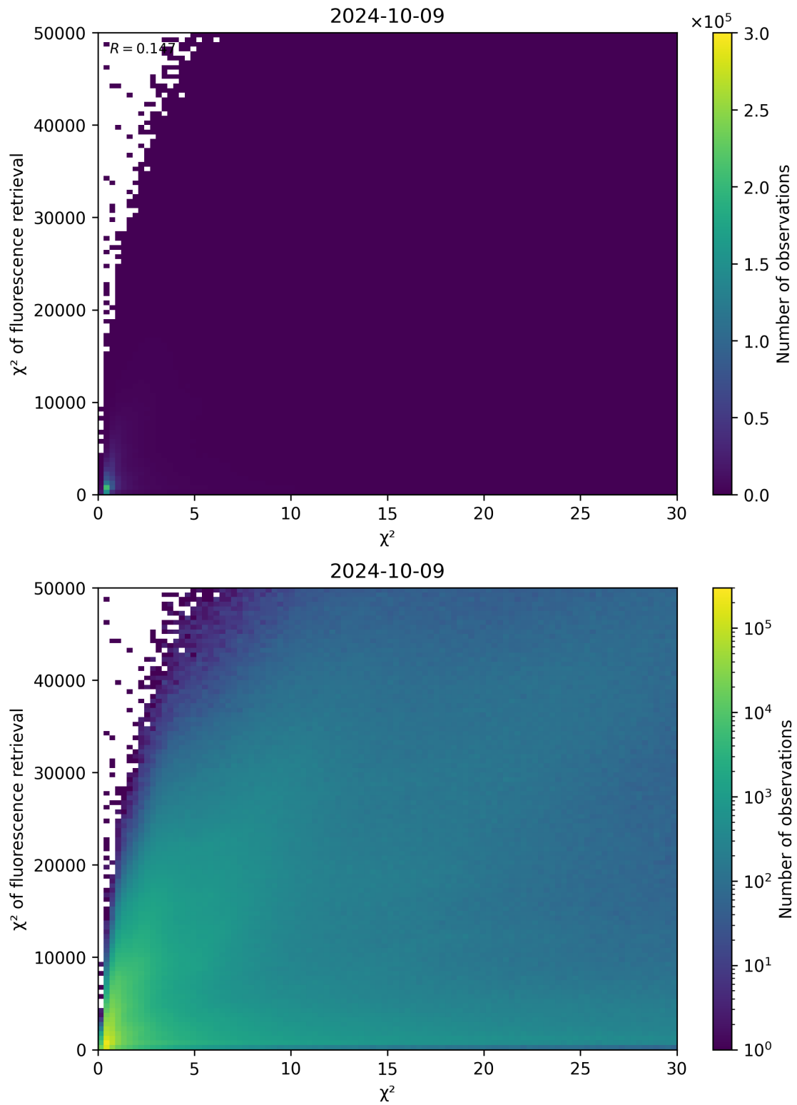
Figure 69: Scatter density plot of “ \chi^2 ” against “ \chi^2 of fluorescence retrieval” for 2024-10-08 to 2024-10-10.
