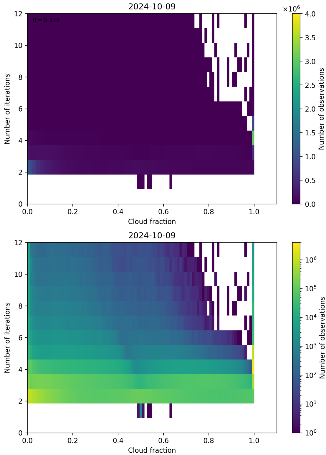
Figure 80: Scatter density plot of “Cloud fraction” against “Number of iterations” for 2024-10-08 to 2024-10-10.
