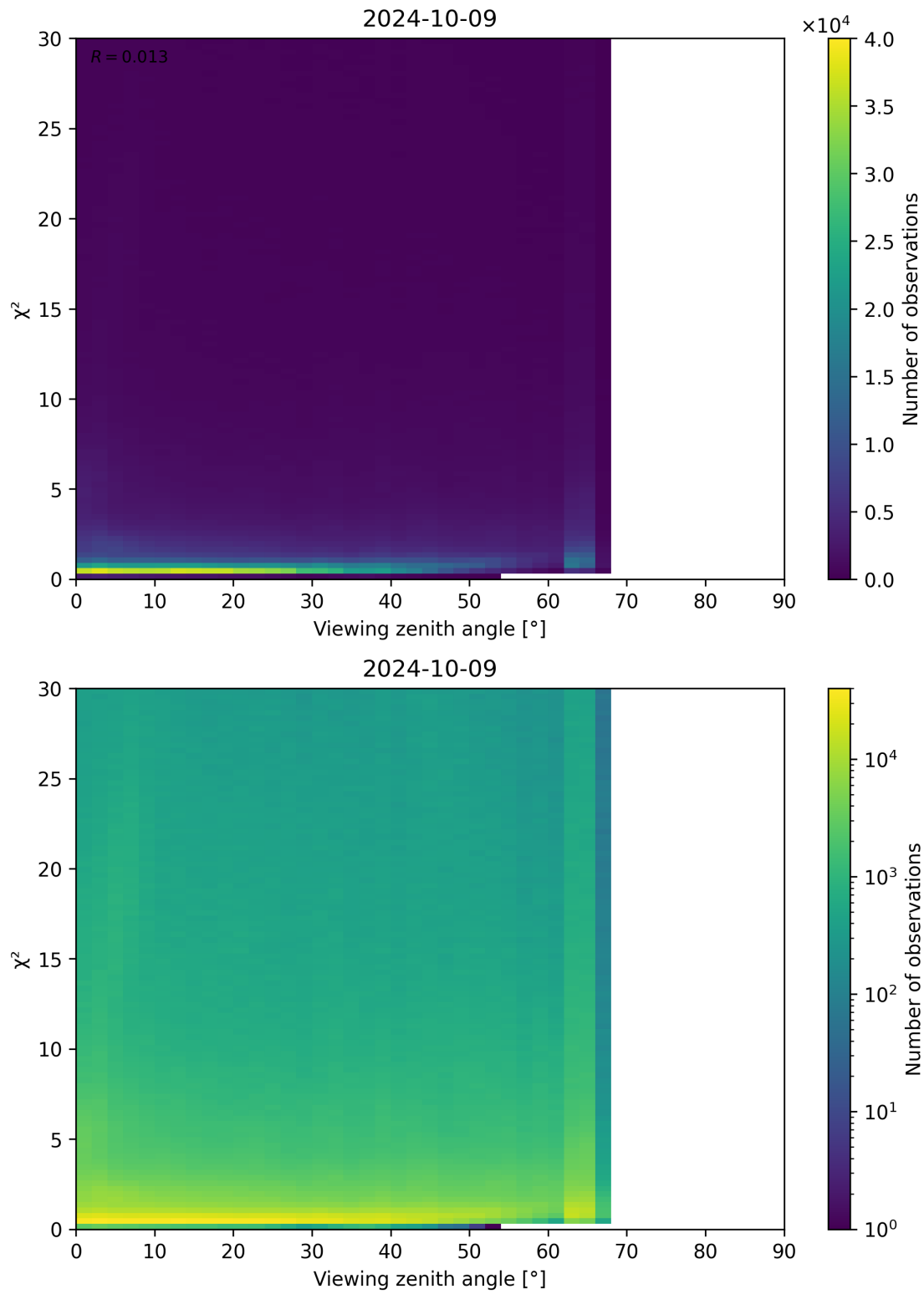
Figure 130: Scatter density plot of “Viewing zenith angle” against “ \chi^2 ” for 2024-10-08 to 2024-10-10.
