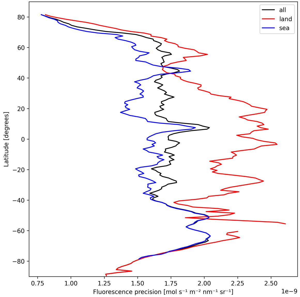
Figure 24: Zonal average of “Fluorescence precision” for 2024-10-08 to 2024-10-10.
