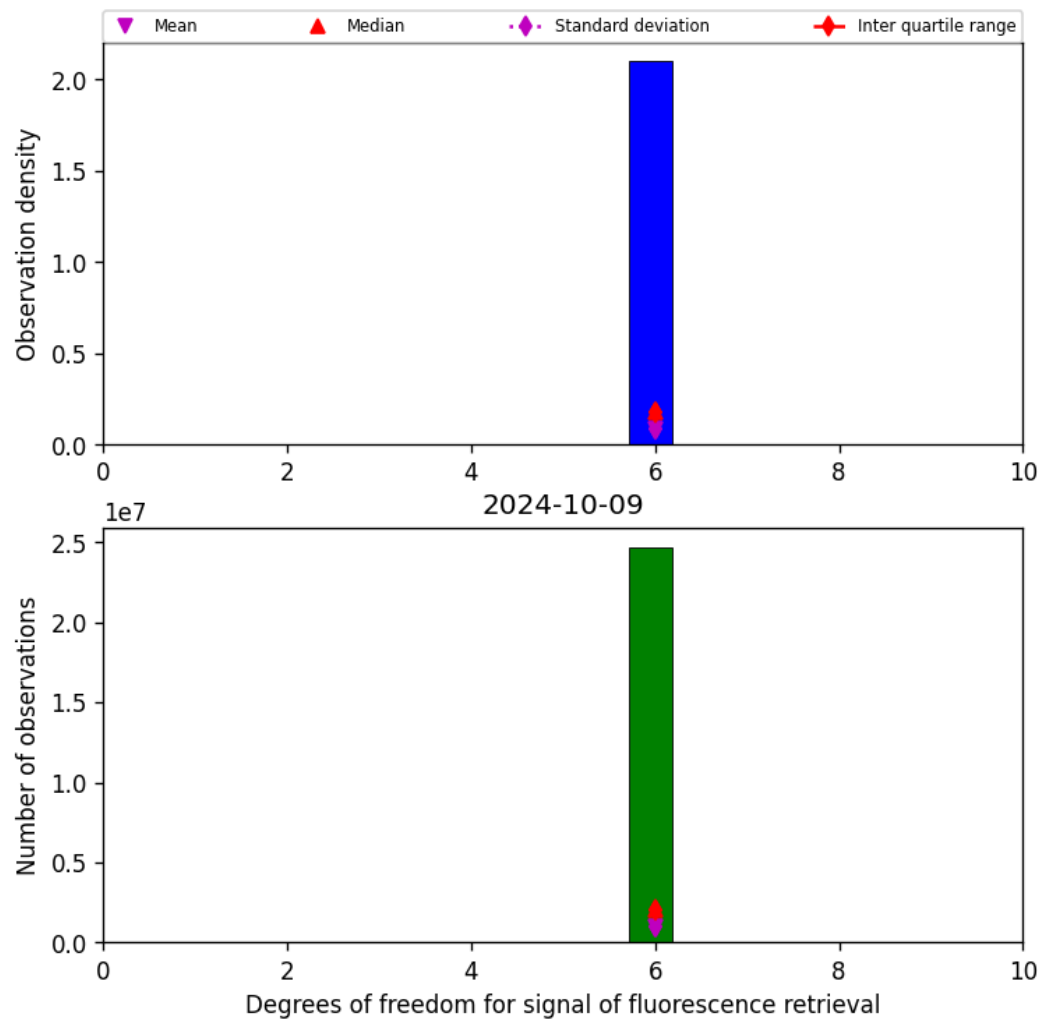
Figure 43: Histogram of "Degrees of freedom for signal of fluorescence retrieval" for 2024-10-08 to 2024-10-10
