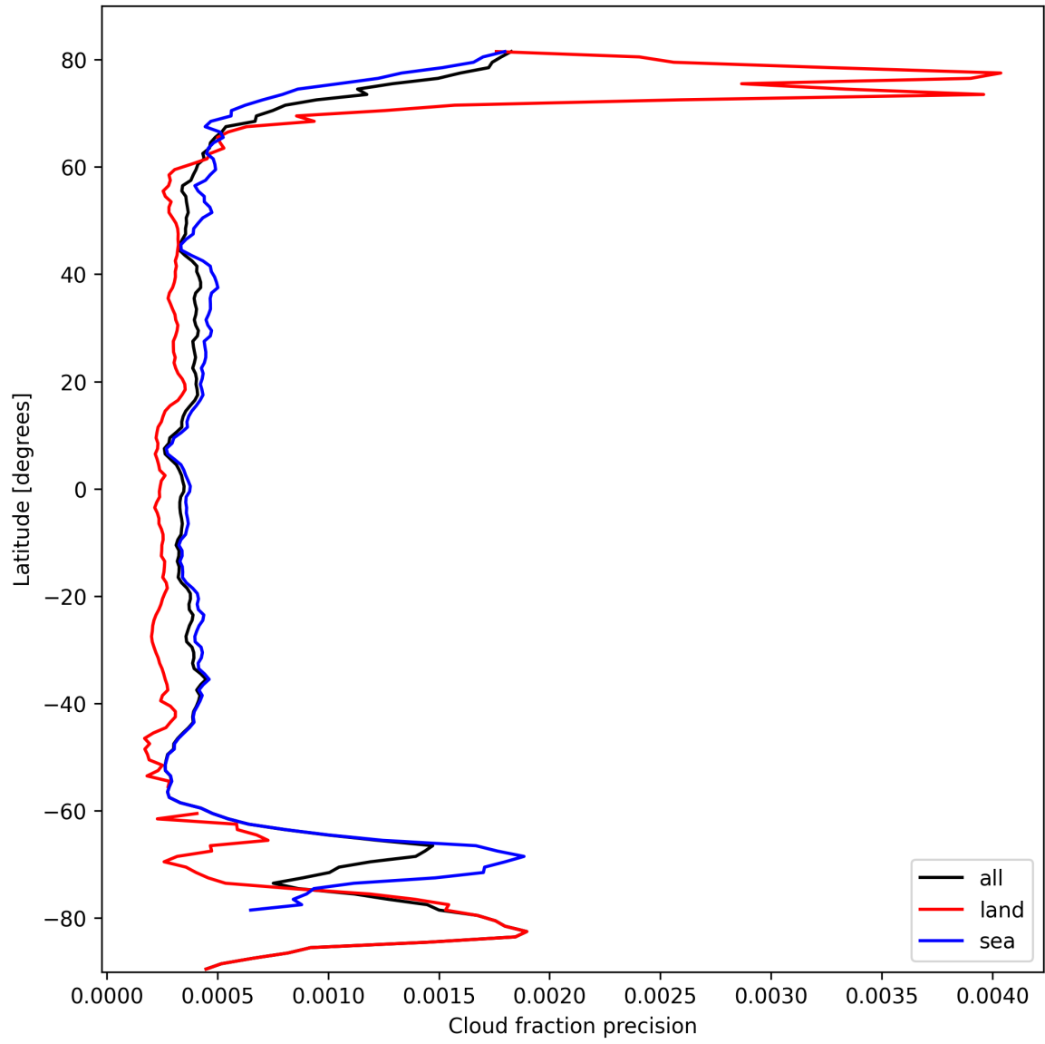
Figure 16: Zonal average of “Cloud fraction precision” for 2024-10-08 to 2024-10-10.
