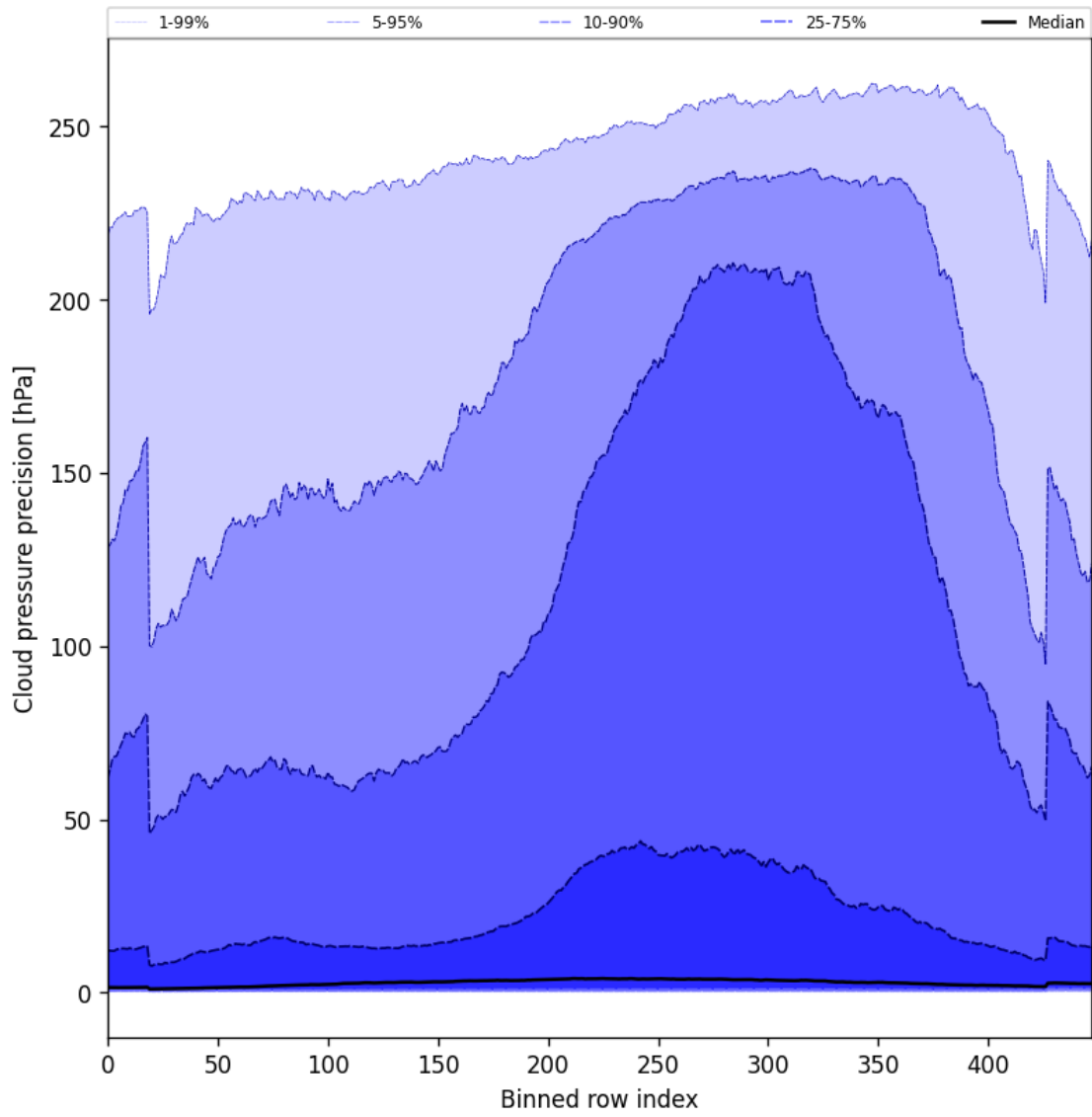
Figure 48: Along track statistics of “Cloud pressure precision” for 2024-10-08 to 2024-10-10
