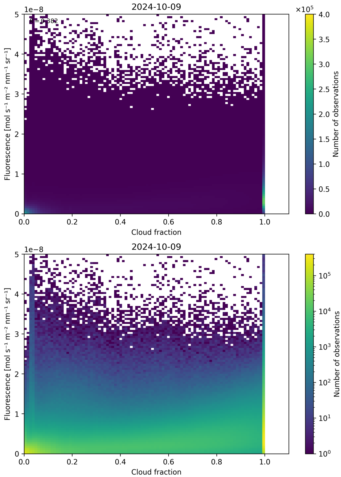
Figure 79: Scatter density plot of “Cloud fraction” against “Fluorescence” for 2024-10-08 to 2024-10-10.
