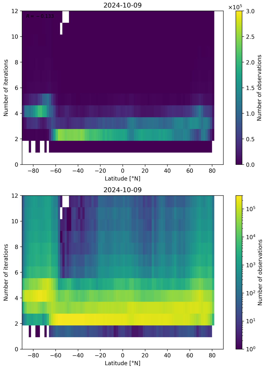
Figure 102: Scatter density plot of “Latitude” against “Number of iterations” for 2024-10-08 to 2024-10-10.
