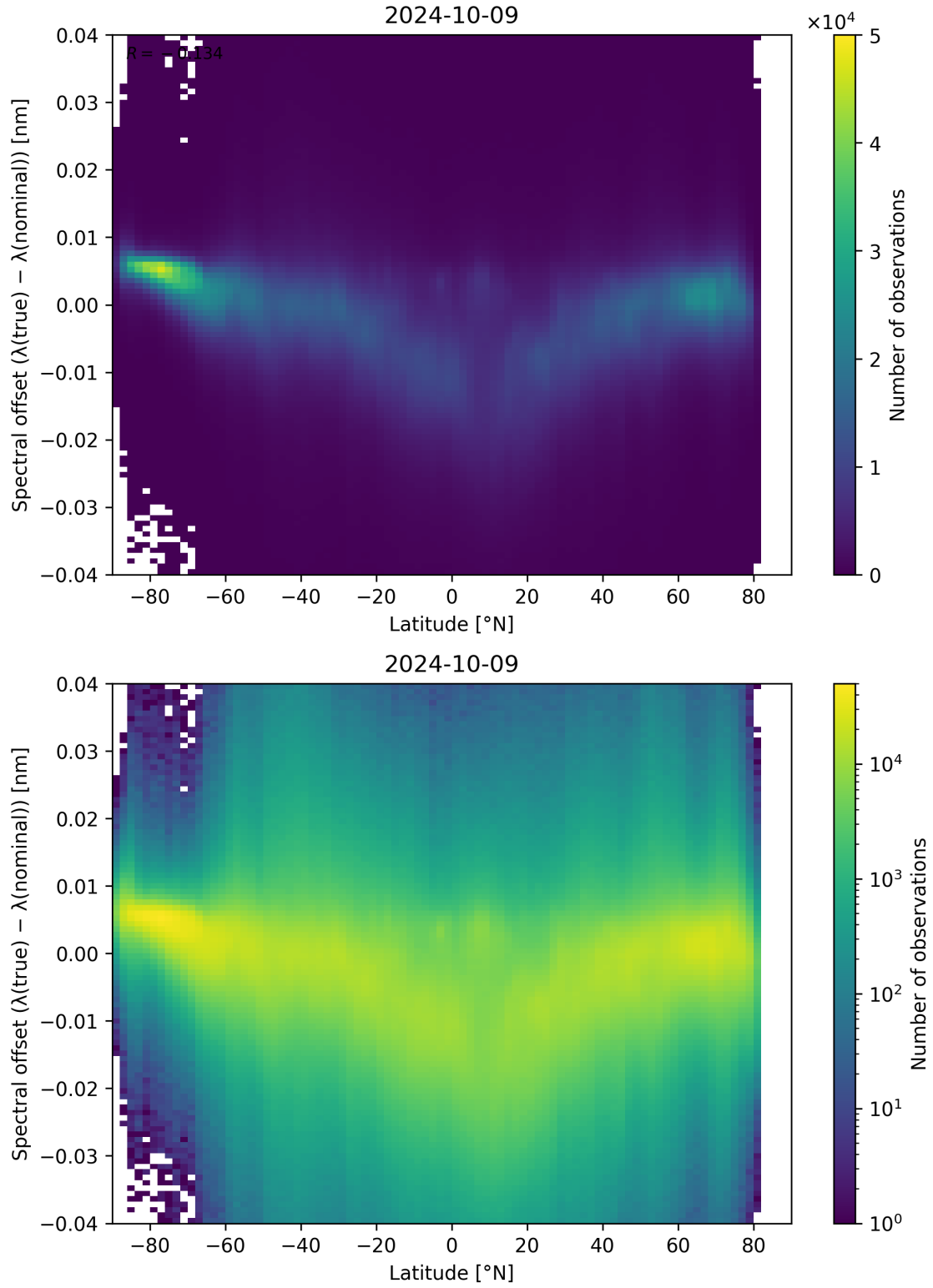
Figure 105: Scatter density plot of “Latitude” against “Spectral offset ( \lambda_{\text{true}} - \lambda_{\text{nominal}} )” for 2024-10-08 to 2024-10-10.
