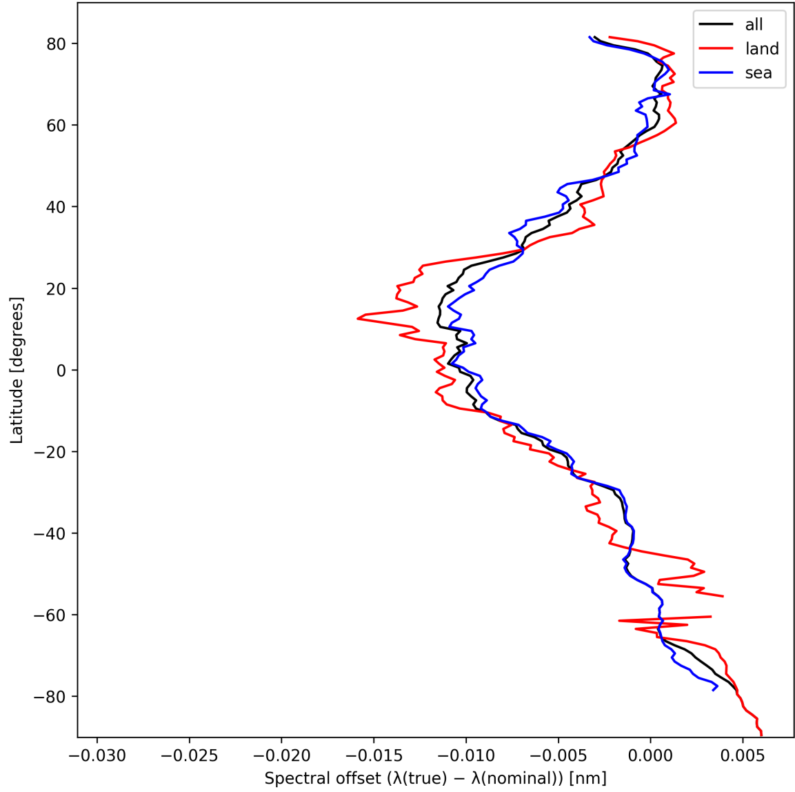
Figure 28: Zonal average of “Spectral offset ( \lambda_{\text{true}} - \lambda_{\text{nominal}} )” for 2024-10-08 to 2024-10-10.
