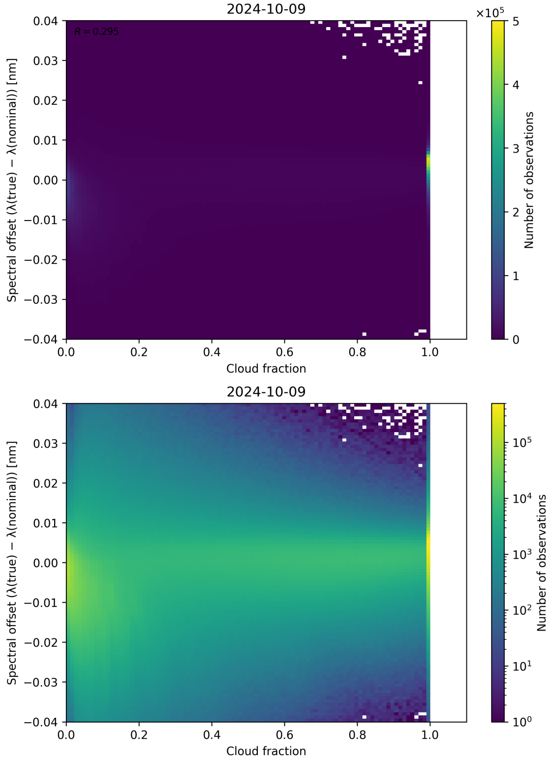
Figure 83: Scatter density plot of “Cloud fraction” against “Spectral offset ( \lambda_{\text{true}} - \lambda_{\text{nominal}} )” for 2024-10-08 to 2024-10-10.
