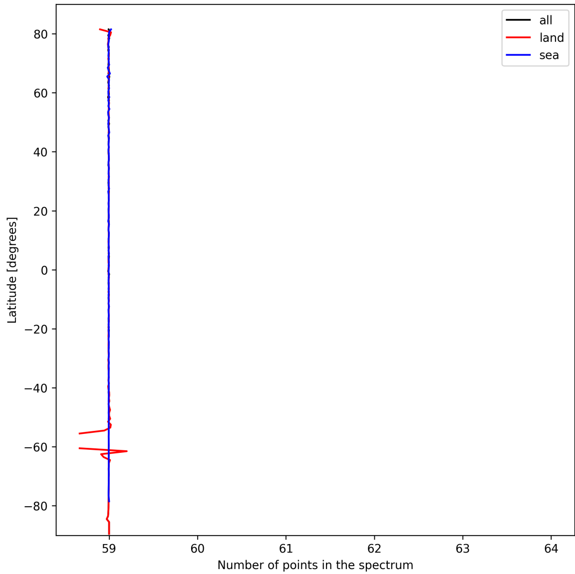
Figure 27: Zonal average of “Number of points in the spectrum” for 2024-10-08 to 2024-10-10.
