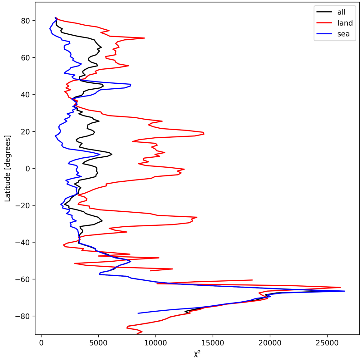
Figure 21: Zonal average of “ \chi^2 ” for 2024-10-08 to 2024-10-10.
