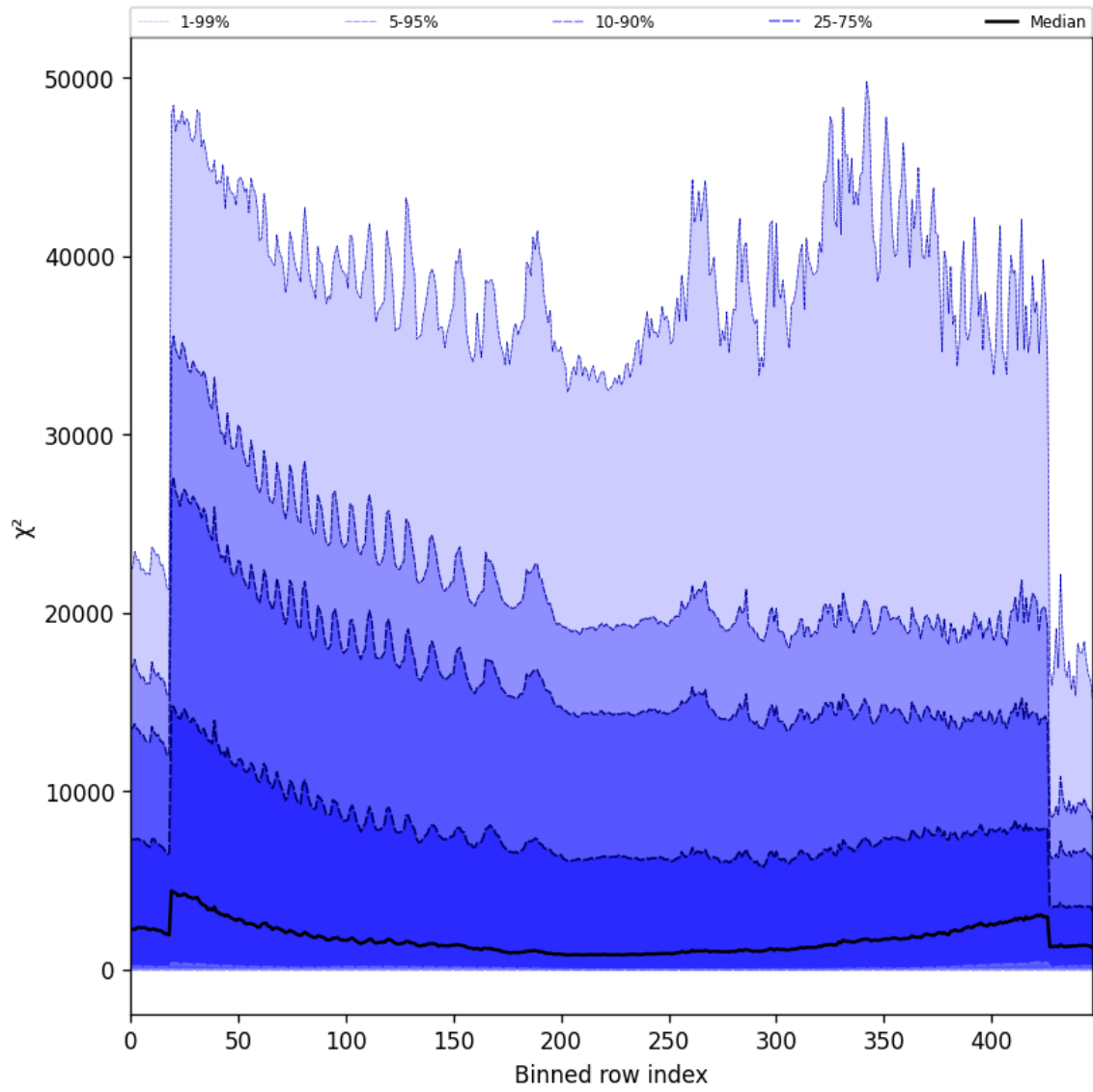
Figure 55: Along track statistics of “ \chi^2 ” for 2024-10-08 to 2024-10-10
