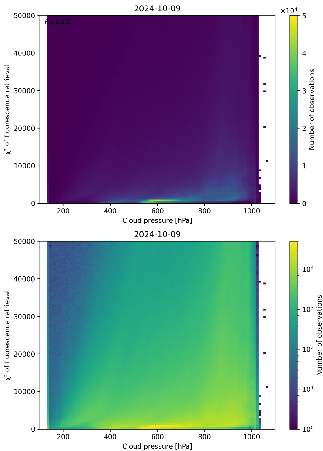
Figure 86: Scatter density plot of “Cloud pressure” against “ \chi^2 of fluorescence retrieval” for 2024-10-08 to 2024-10-10.
