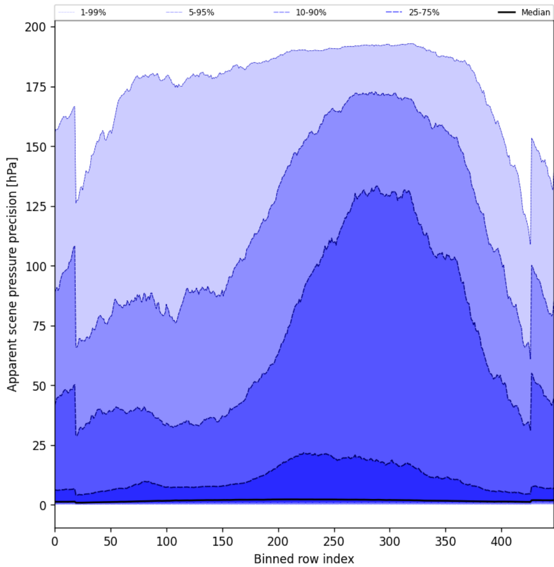
Figure 54: Along track statistics of “Apparent scene pressure precision” for 2024-10-08 to 2024-10-10
