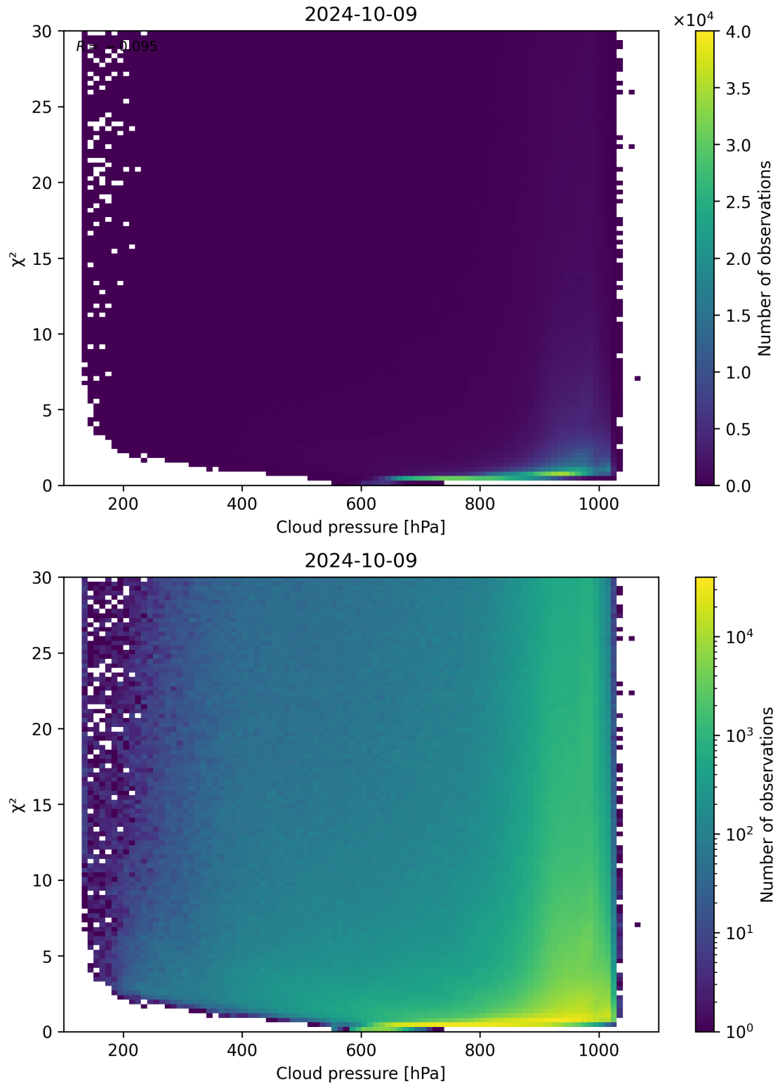
Figure 85: Scatter density plot of “Cloud pressure” against “ \chi^2 ” for 2024-10-08 to 2024-10-10.
