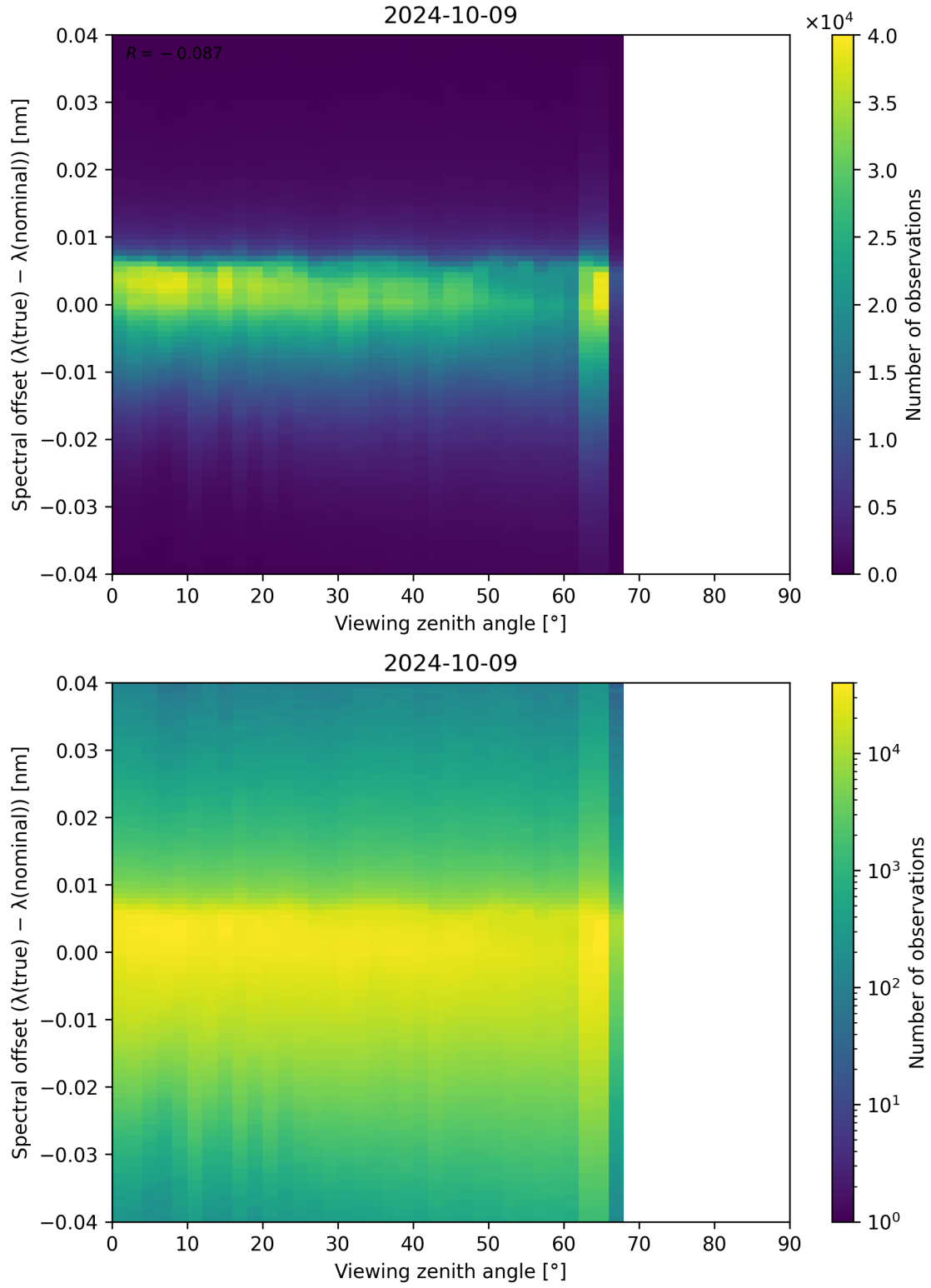
Figure 140: Scatter density plot of “Viewing zenith angle” against “Spectral offset ( \lambda_{\text{true}} - \lambda_{\text{nominal}} )” for 2024-10-08 to 2024-10-10.
