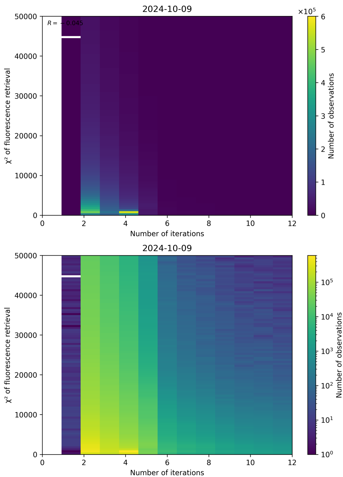
Figure 106: Scatter density plot of “Number of iterations” against “ \chi^2 of fluorescence retrieval” for 2024-10-08 to 2024-10-10.
