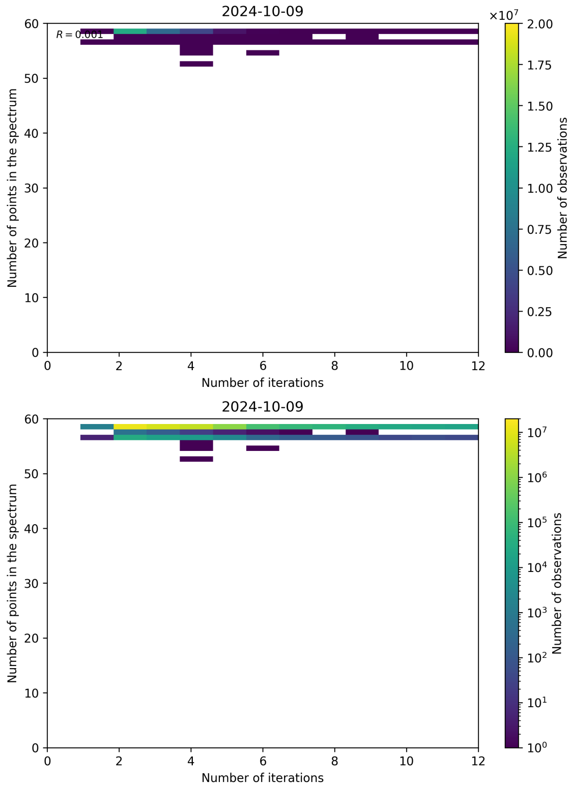
Figure 108: Scatter density plot of “Number of iterations” against “Number of points in the spectrum” for 2024-10-08 to 2024-10-10.
