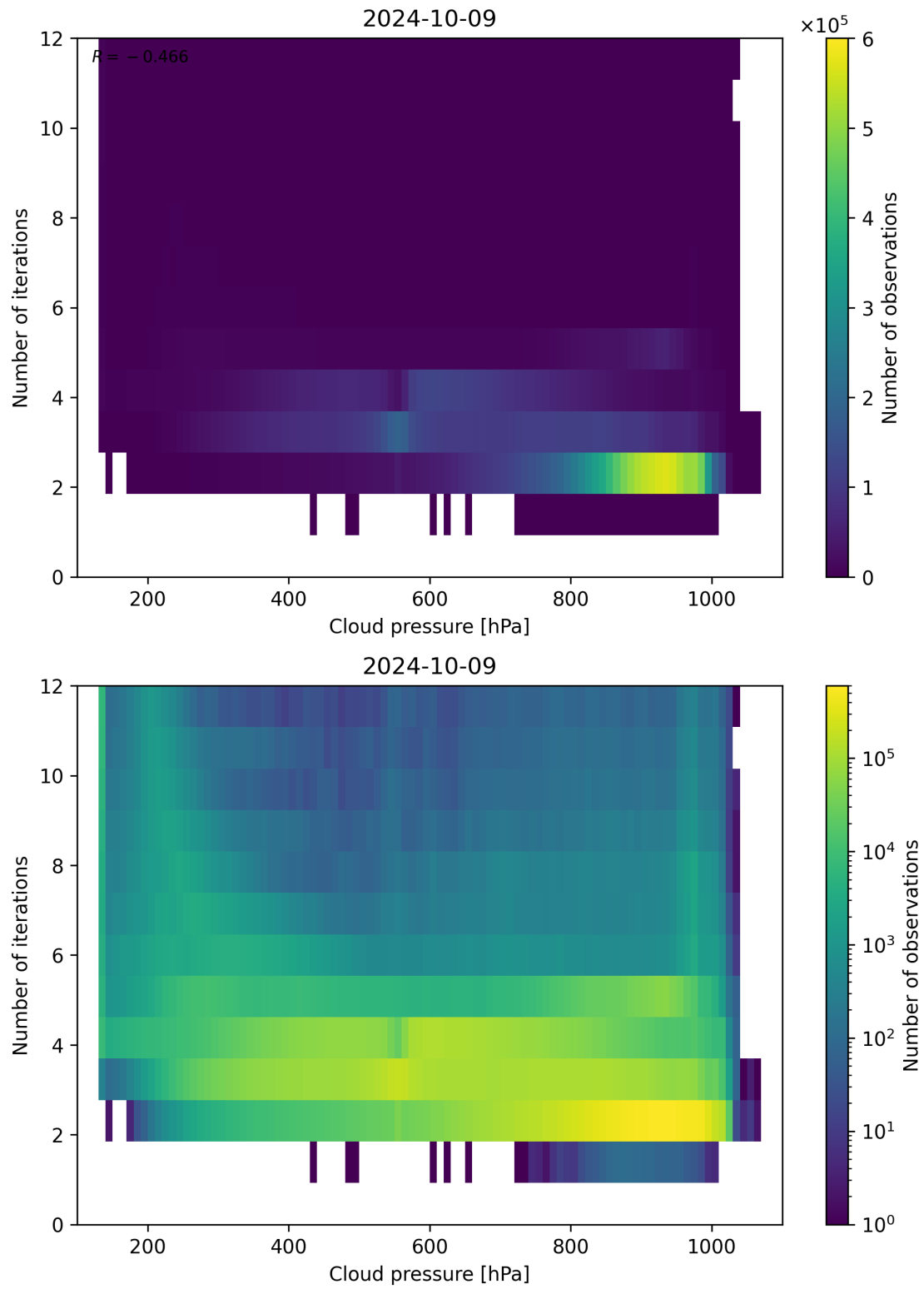
Figure 89: Scatter density plot of “Cloud pressure” against “Number of iterations” for 2024-10-08 to 2024-10-10.
