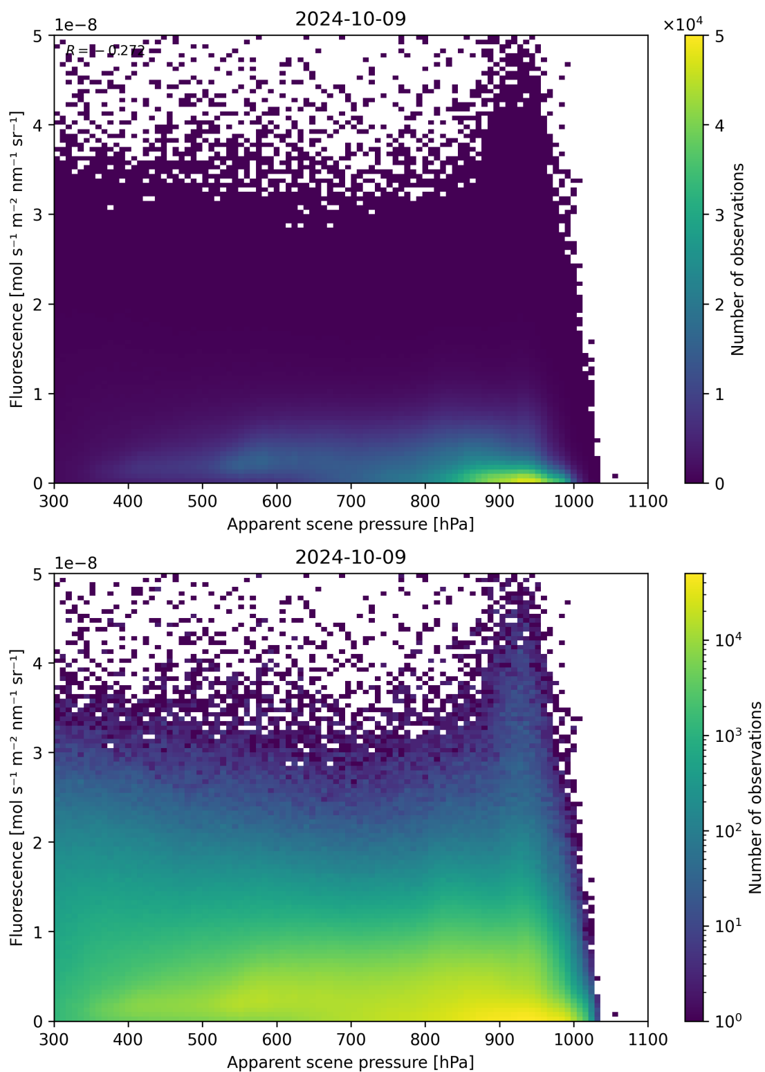
Figure 65: Scatter density plot of “Apparent scene pressure” against “Fluorescence” for 2024-10-08 to 2024-10-10.
