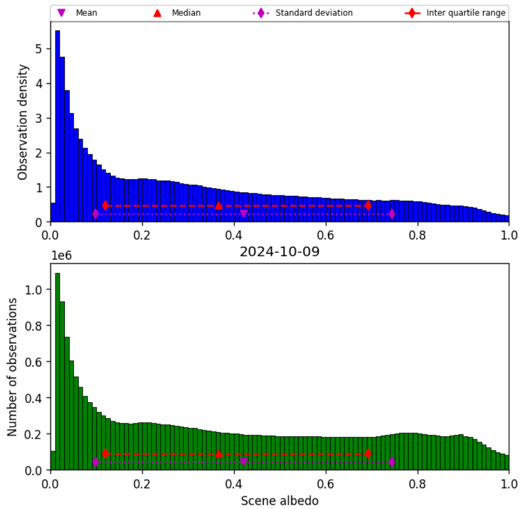
Figure 34: Histogram of “Scene albedo” for 2024-10-08 to 2024-10-10
