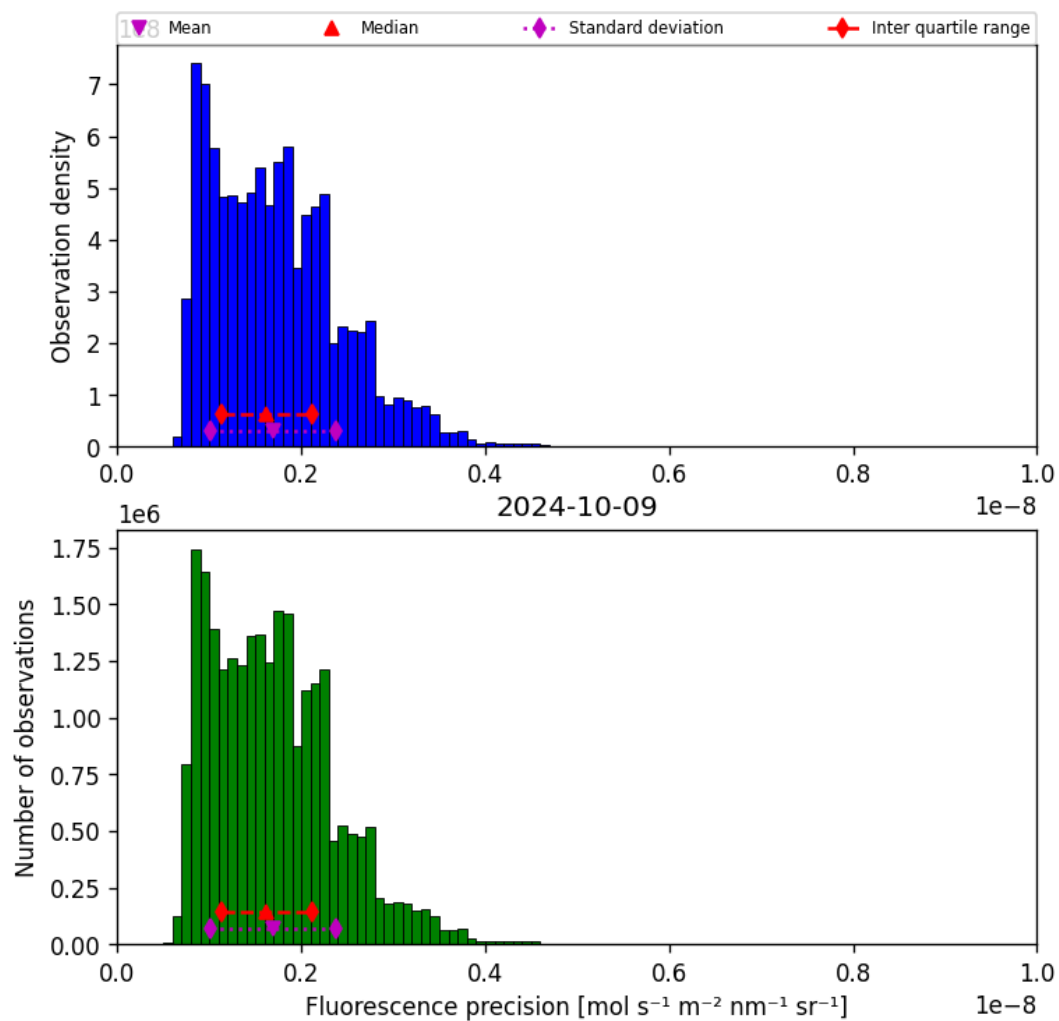
Figure 41: Histogram of “Fluorescence precision” for 2024-10-08 to 2024-10-10
