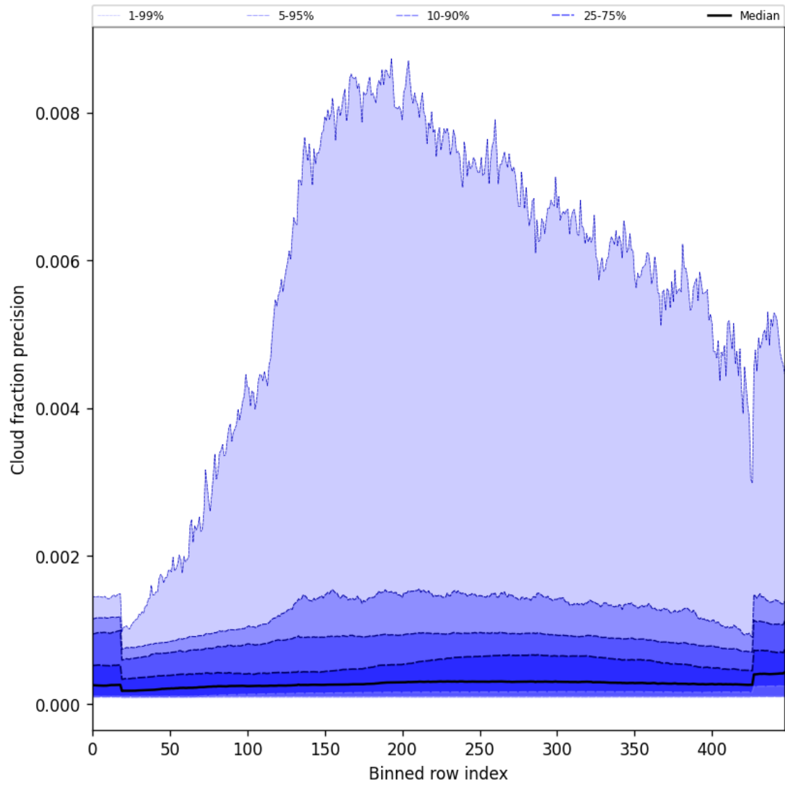
Figure 50: Along track statistics of “Cloud fraction precision” for 2024-10-08 to 2024-10-10
