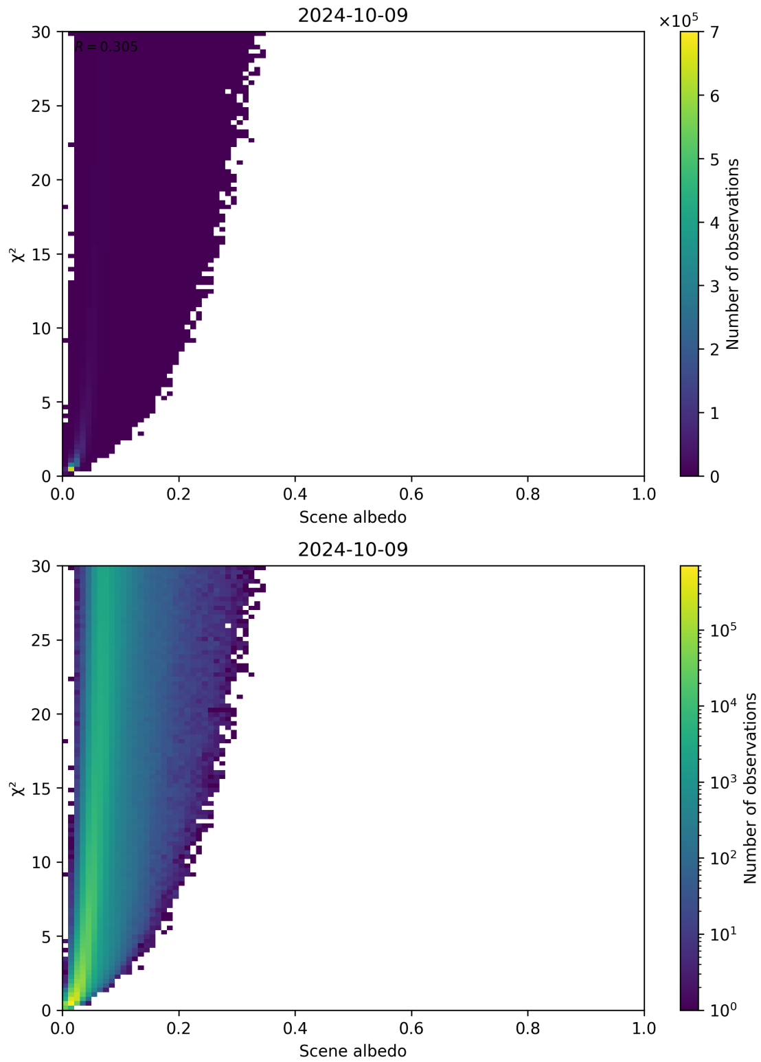
Figure 112: Scatter density plot of “Scene albedo” against “ \chi^2 ” for 2024-10-08 to 2024-10-10.
