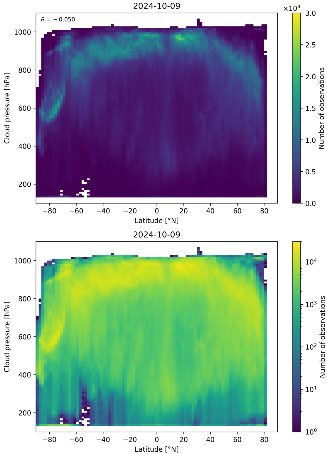
Figure 100: Scatter density plot of “Latitude” against “Cloud pressure” for 2024-10-08 to 2024-10-10.
