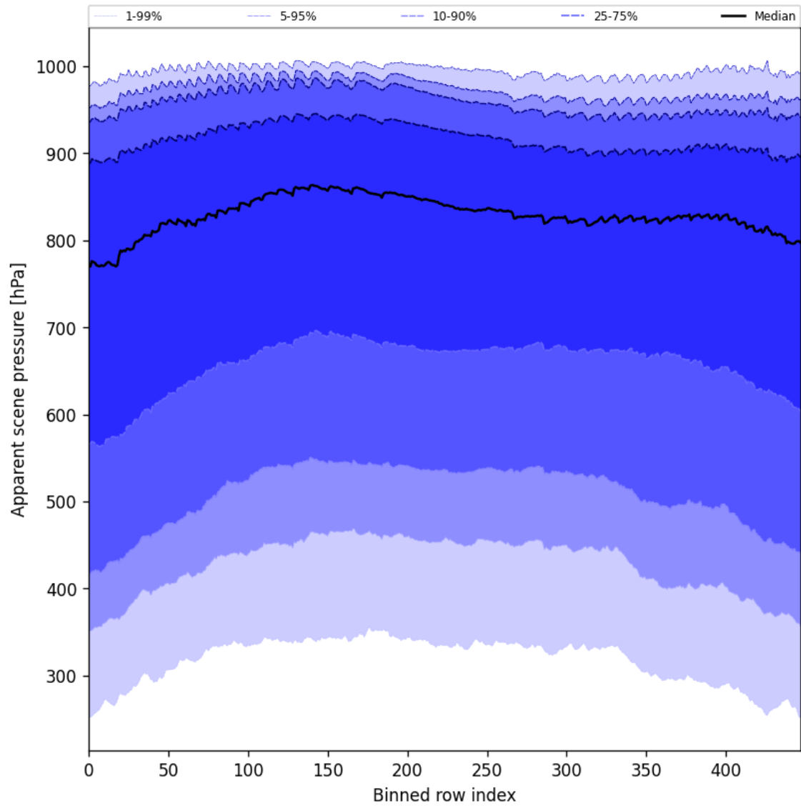
Figure 53: Along track statistics of “Apparent scene pressure” for 2024-10-08 to 2024-10-10
