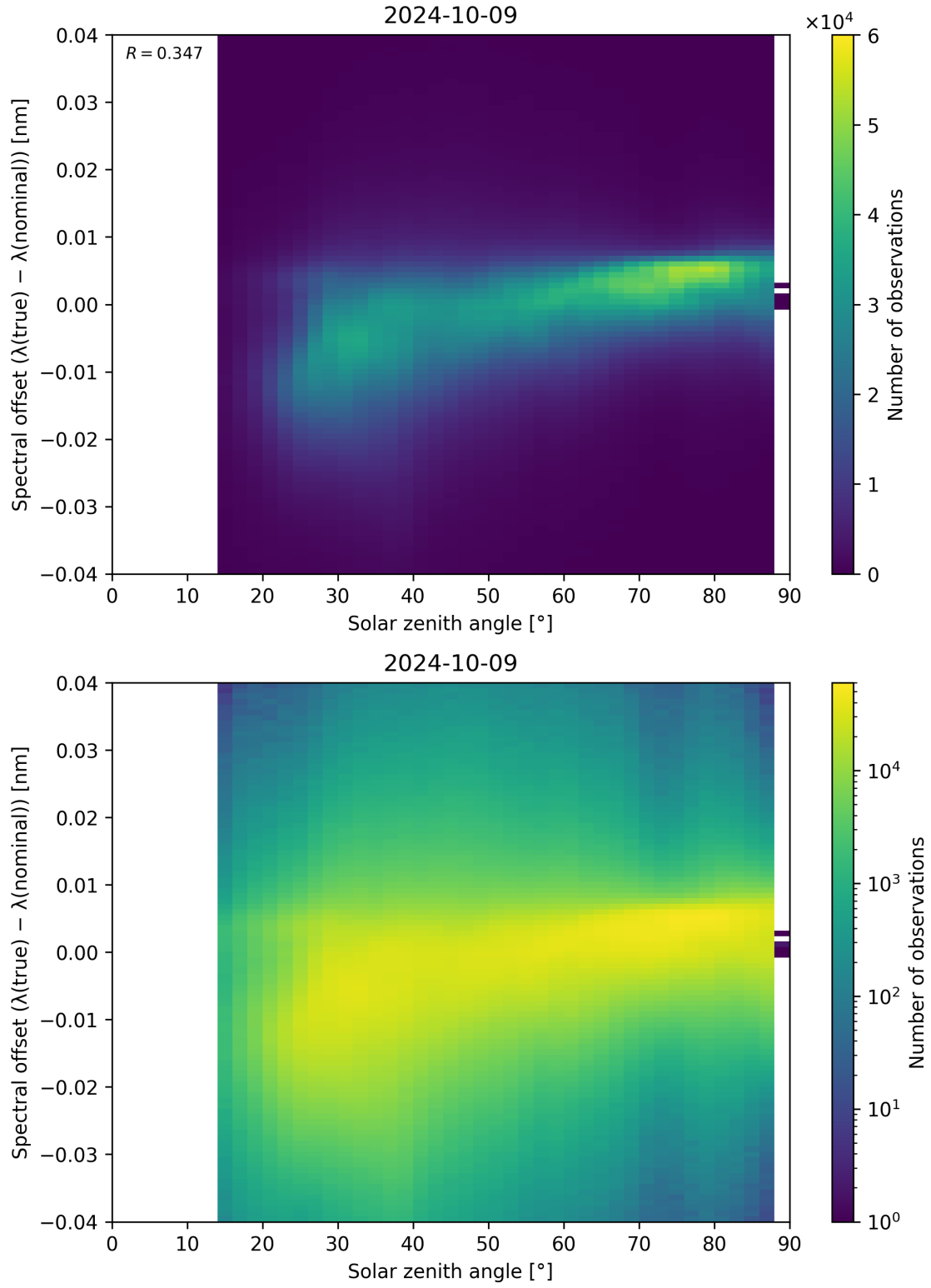
Figure 128: Scatter density plot of “Solar zenith angle” against “Spectral offset ( \lambda_{\text{true}} - \lambda_{\text{nominal}} )” for 2024-10-08 to 2024-10-10.
