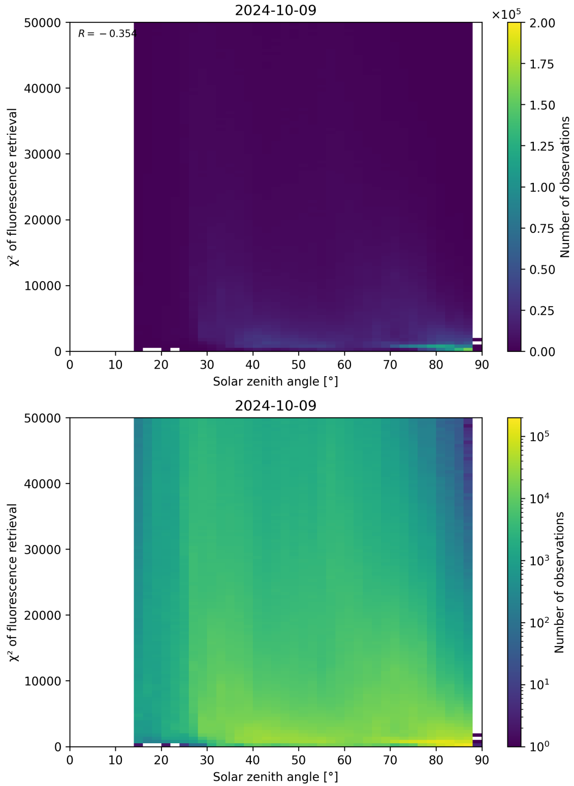
Figure 120: Scatter density plot of “Solar zenith angle” against “ \chi^2 of fluorescence retrieval” for 2024-10-08 to 2024-10-10.
