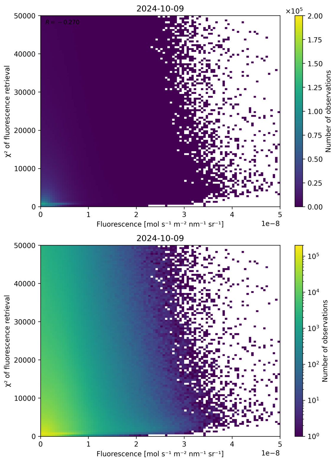
Figure 93: Scatter density plot of “Fluorescence” against “ \chi^2 of fluorescence retrieval” for 2024-10-08 to 2024-10-10.
