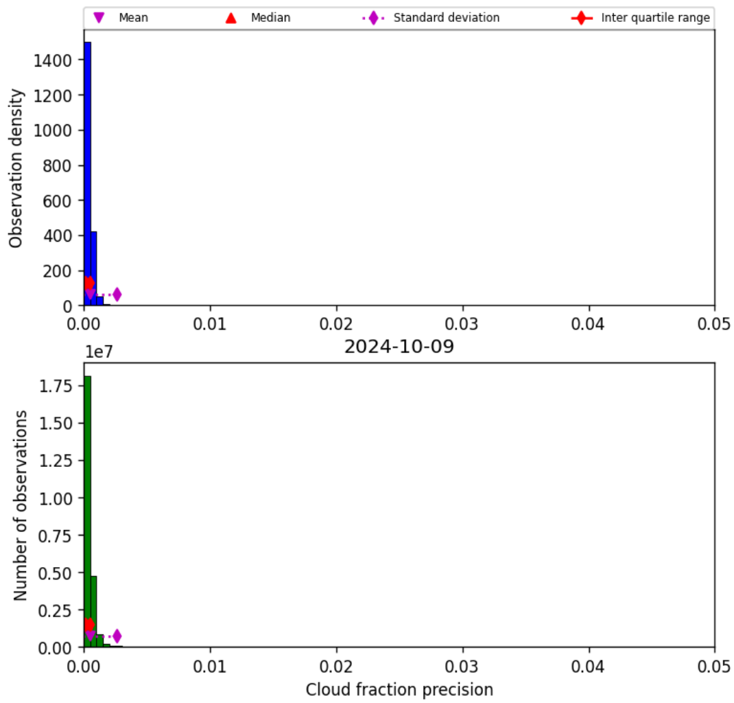
Figure 33: Histogram of “Cloud fraction precision” for 2024-10-08 to 2024-10-10
