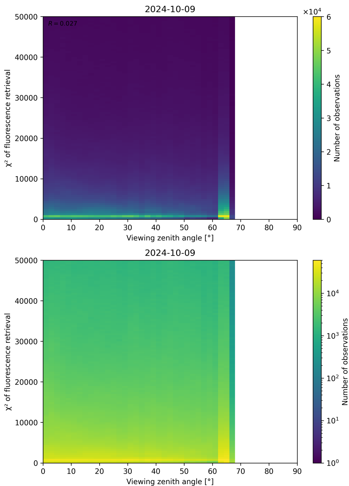
Figure 131: Scatter density plot of “Viewing zenith angle” against “ \chi^2 of fluorescence retrieval” for 2024-10-08 to 2024-10-10.
