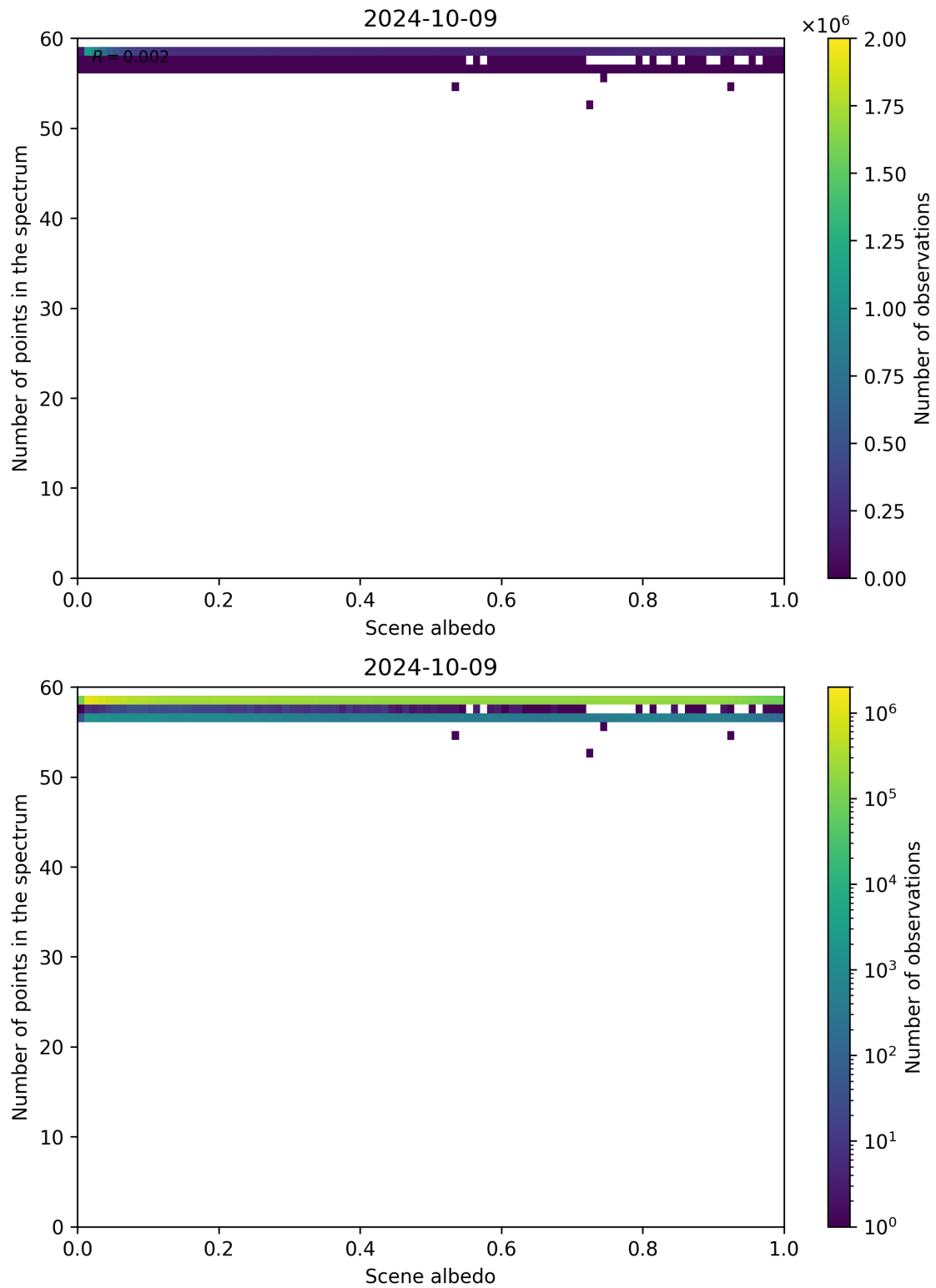
Figure 116: Scatter density plot of “Scene albedo” against “Number of points in the spectrum” for 2024-10-08 to 2024-10-10.
