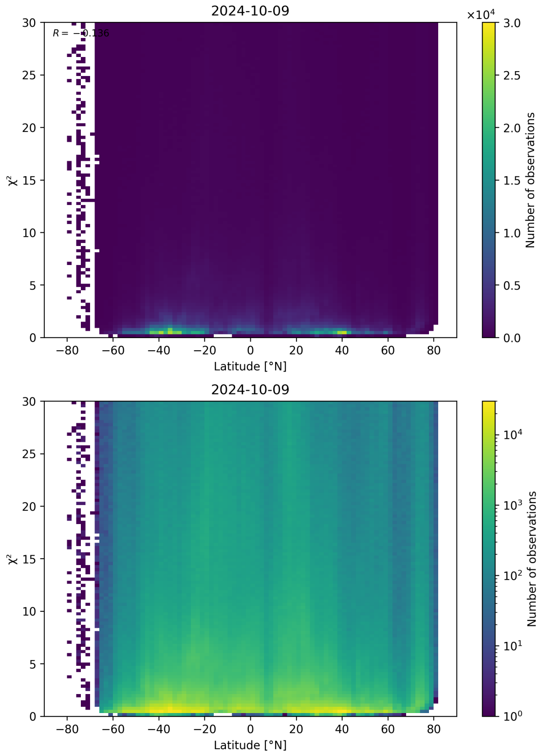
Figure 97: Scatter density plot of “Latitude” against “ \chi^2 ” for 2024-10-08 to 2024-10-10.
