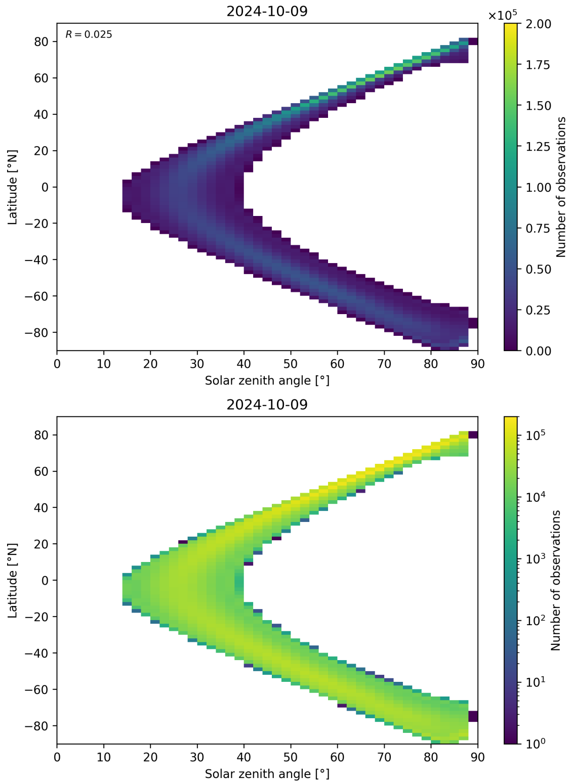
Figure 124: Scatter density plot of “Solar zenith angle” against “Latitude” for 2024-10-08 to 2024-10-10.
