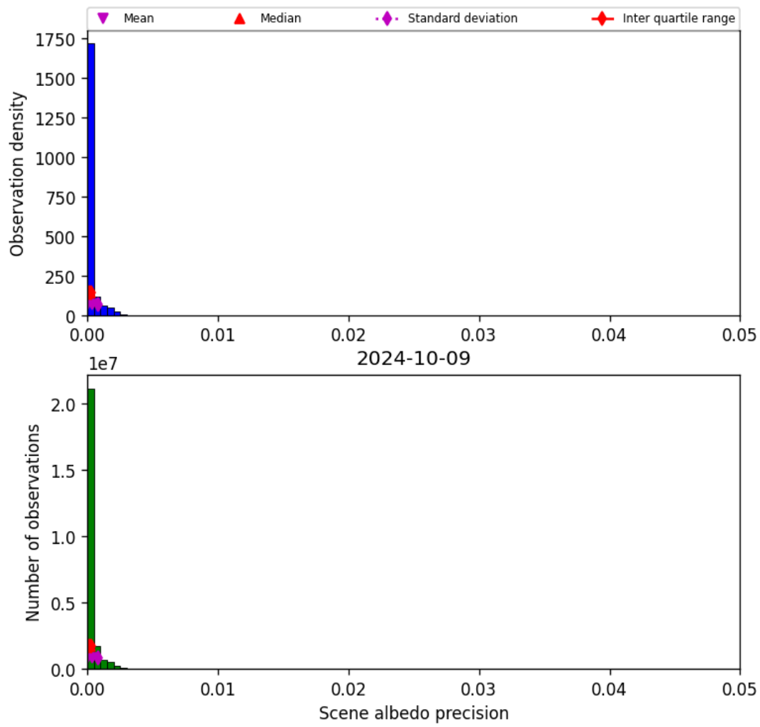
Figure 35: Histogram of “Scene albedo precision” for 2024-10-08 to 2024-10-10
