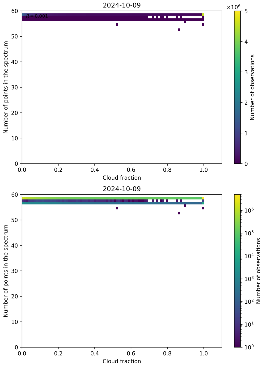
Figure 81: Scatter density plot of “Cloud fraction” against “Number of points in the spectrum” for 2024-10-08 to 2024-10-10.
