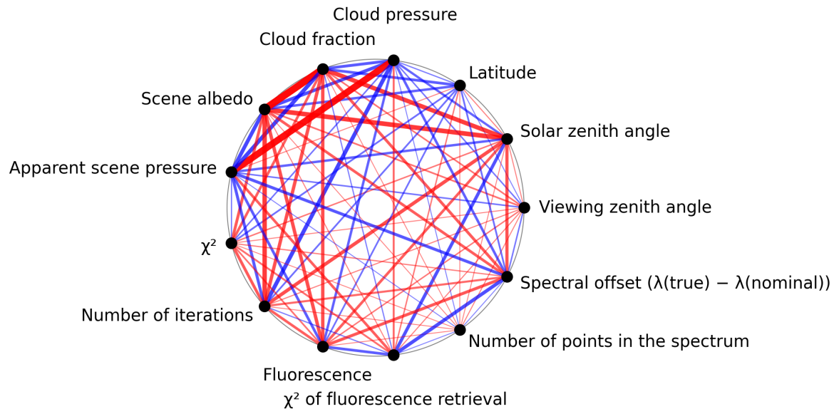
Figure 1: Map of correlation graph for 2024-10-08 to 2024-10-10.
