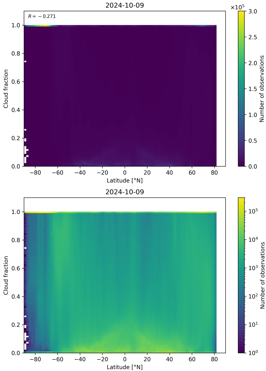
Figure 99: Scatter density plot of “Latitude” against “Cloud fraction” for 2024-10-08 to 2024-10-10.
