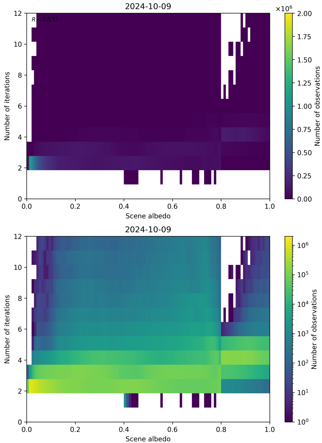
Figure 115: Scatter density plot of “Scene albedo” against “Number of iterations” for 2024-10-08 to 2024-10-10.
