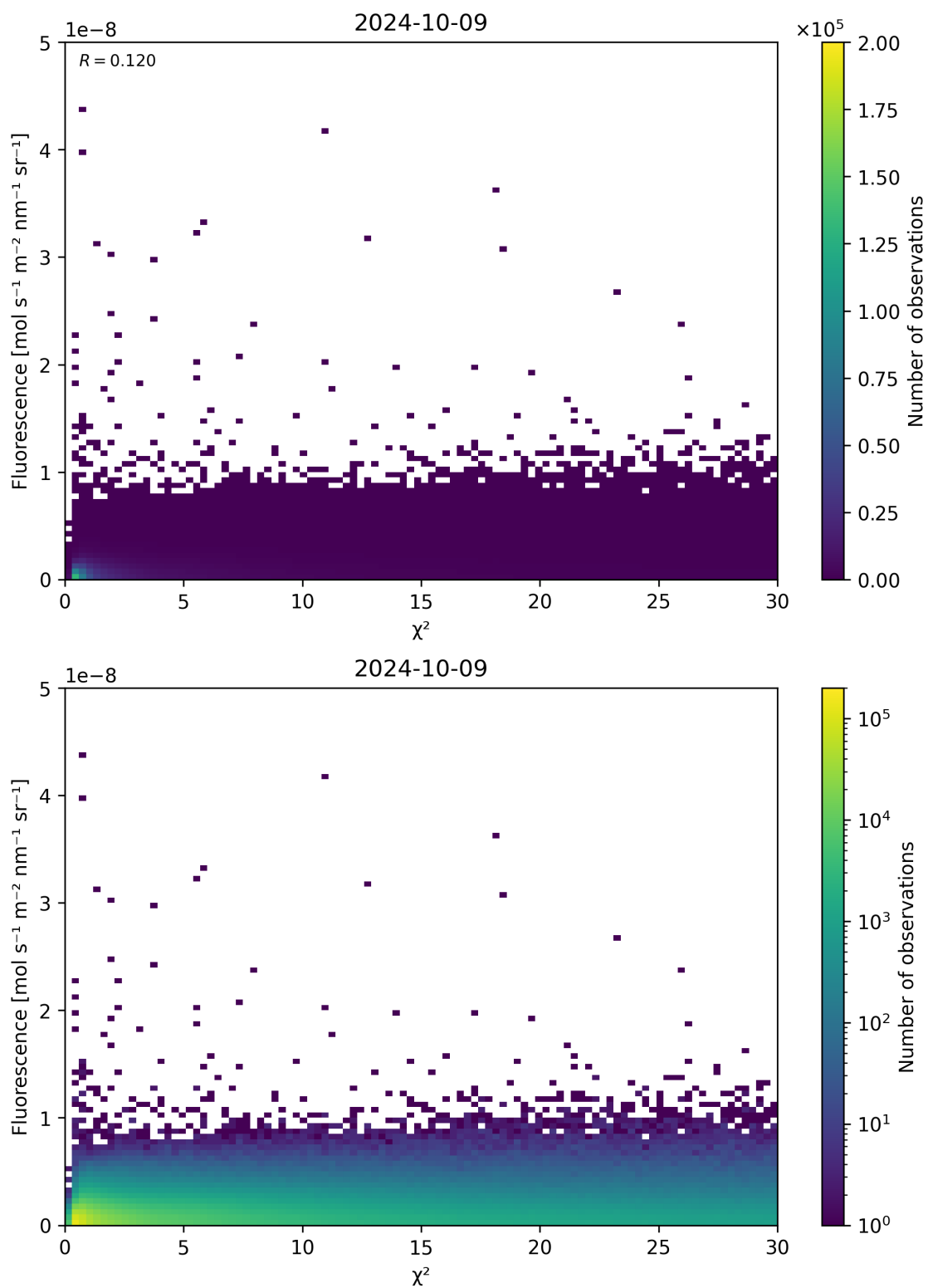
Figure 70: Scatter density plot of “ \chi^2 ” against “Fluorescence” for 2024-10-08 to 2024-10-10.
