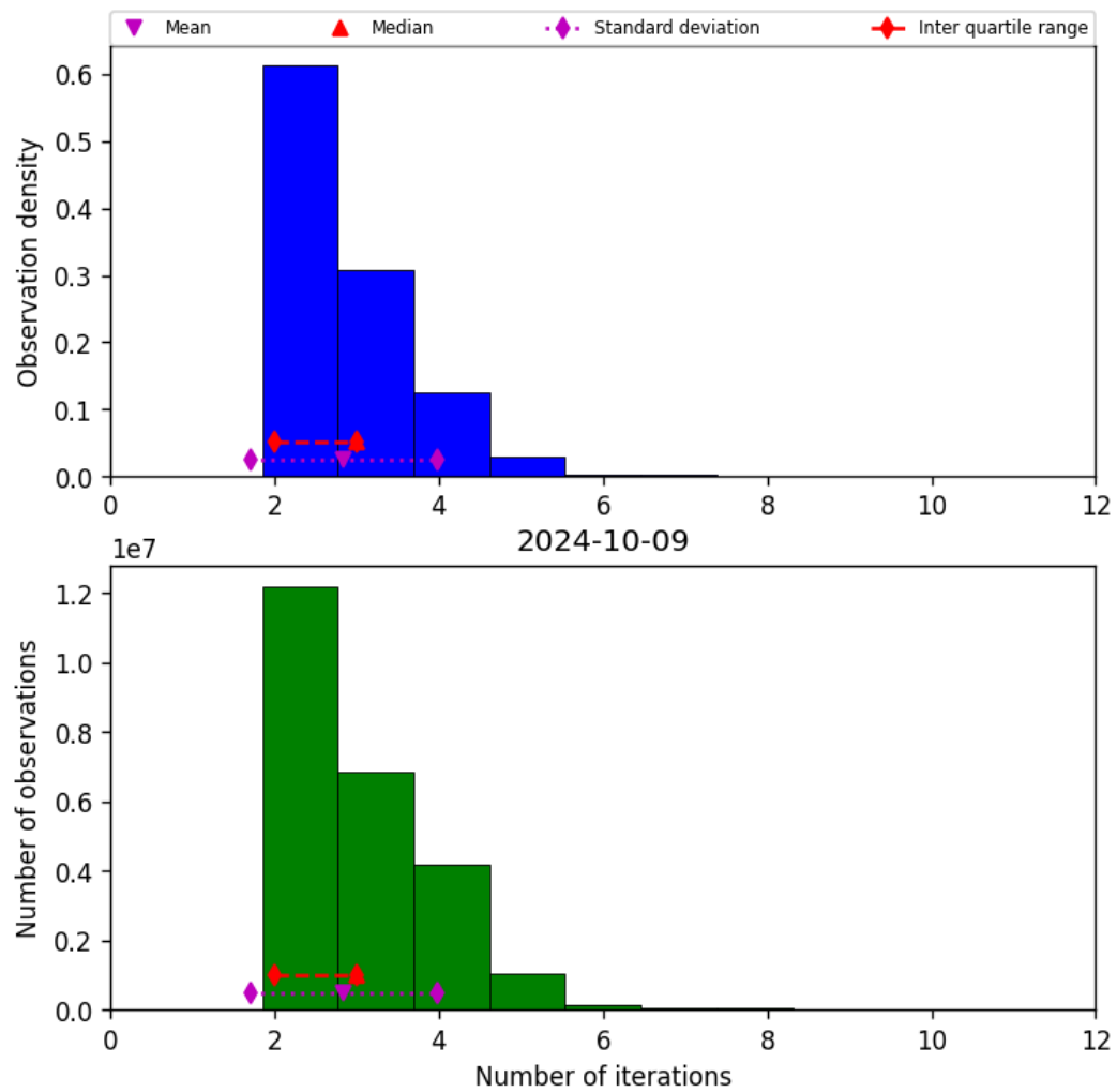
Figure 39: Histogram of “Number of iterations” for 2024-10-08 to 2024-10-10
