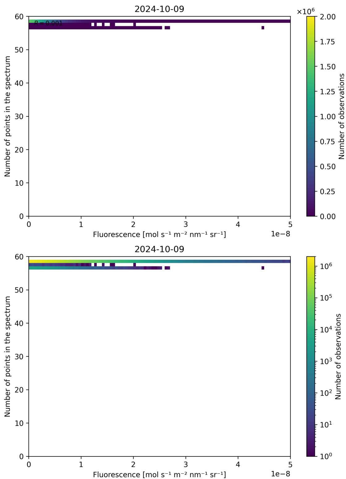
Figure 94: Scatter density plot of “Fluorescence” against “Number of points in the spectrum” for 2024-10-08 to 2024-10-10.
