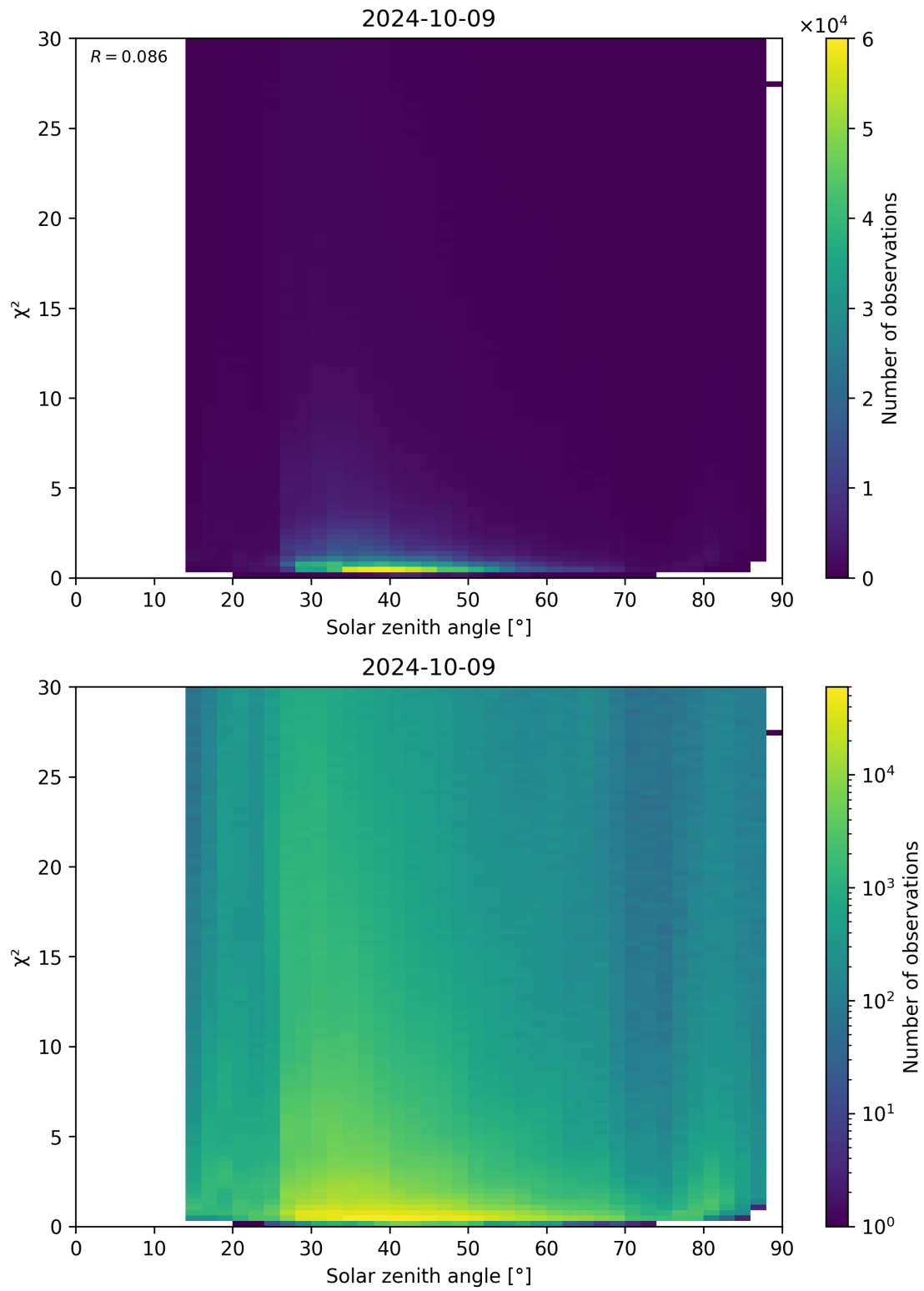
Figure 119: Scatter density plot of “Solar zenith angle” against “ \chi^2 ” for 2024-10-08 to 2024-10-10.
