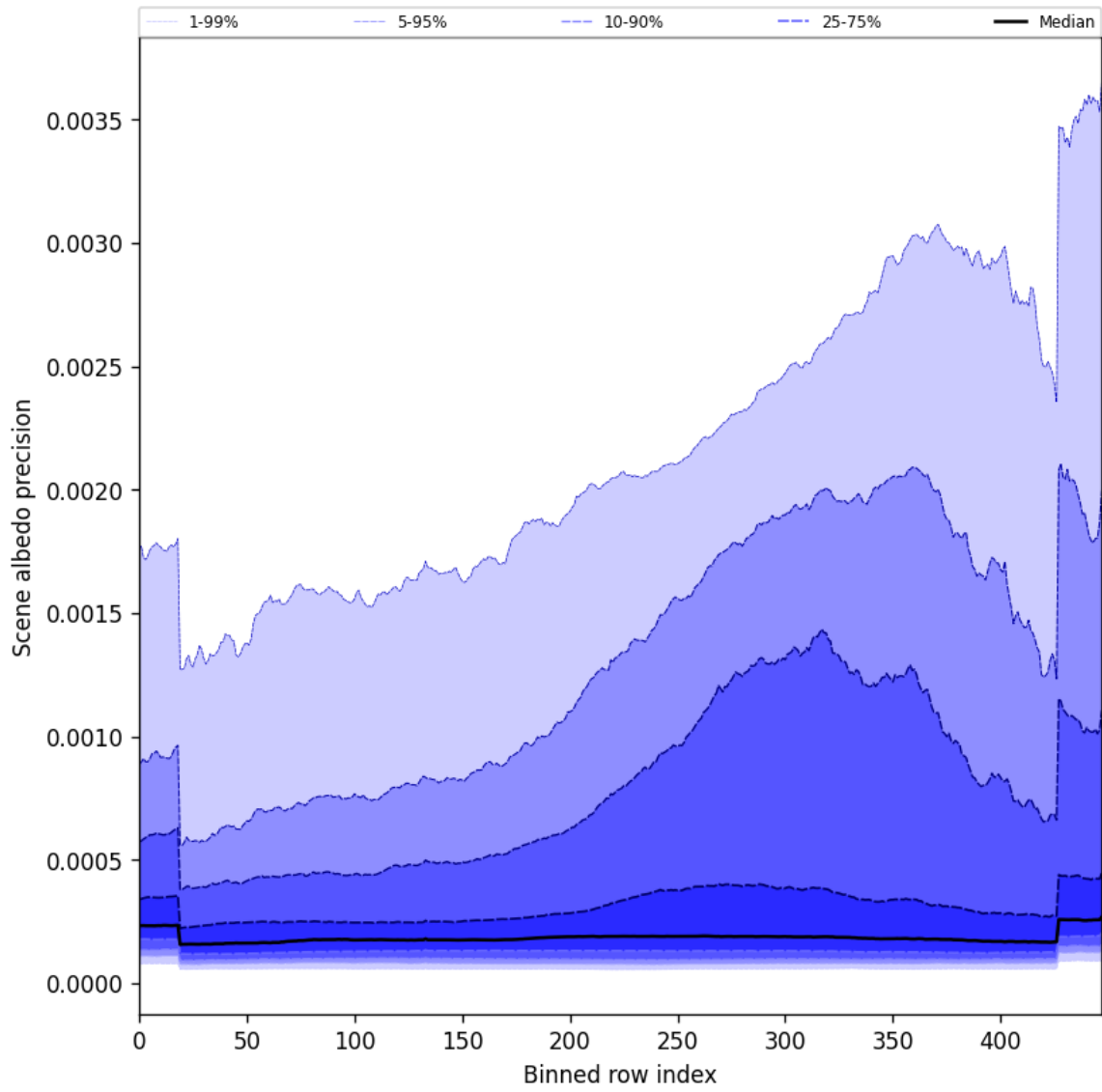
Figure 52: Along track statistics of “Scene albedo precision” for 2024-10-08 to 2024-10-10
