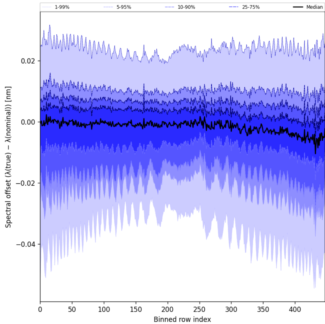
Figure 62: Along track statistics of “Spectral offset ( \lambda_{\text{true}} - \lambda_{\text{nominal}} )” for 2024-10-08 to 2024-10-10
