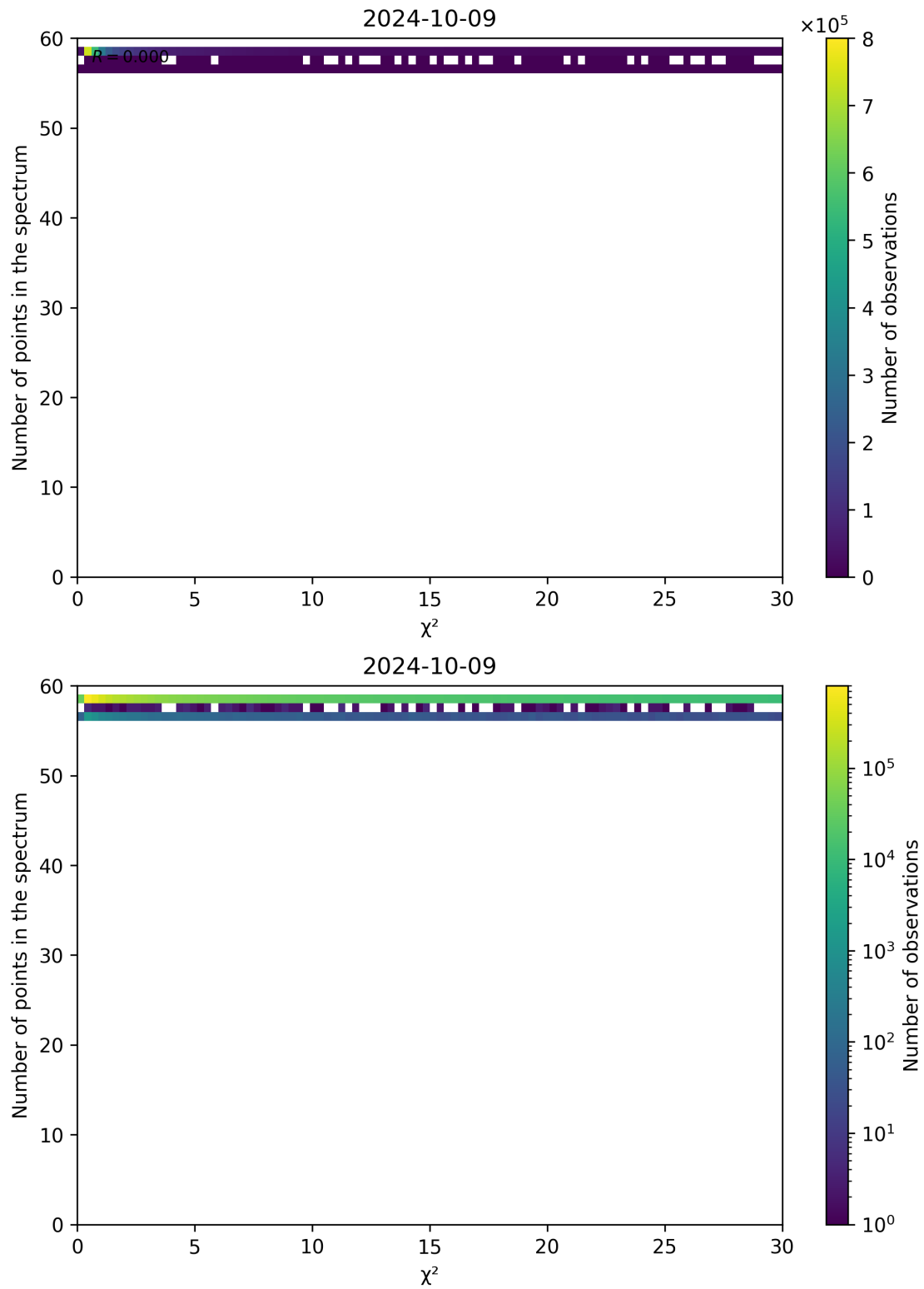
Figure 74: Scatter density plot of “ \chi^2 ” against “Number of points in the spectrum” for 2024-10-08 to 2024-10-10.
