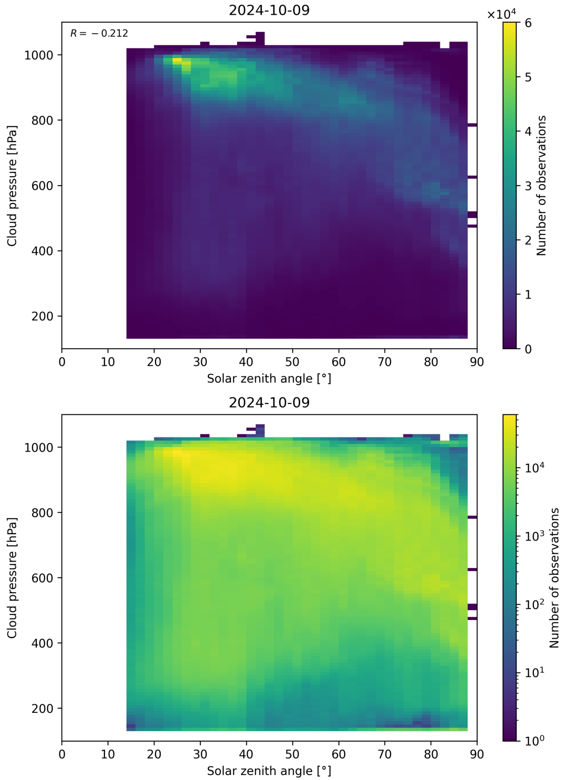
Figure 122: Scatter density plot of “Solar zenith angle” against “Cloud pressure” for 2024-10-08 to 2024-10-10.
