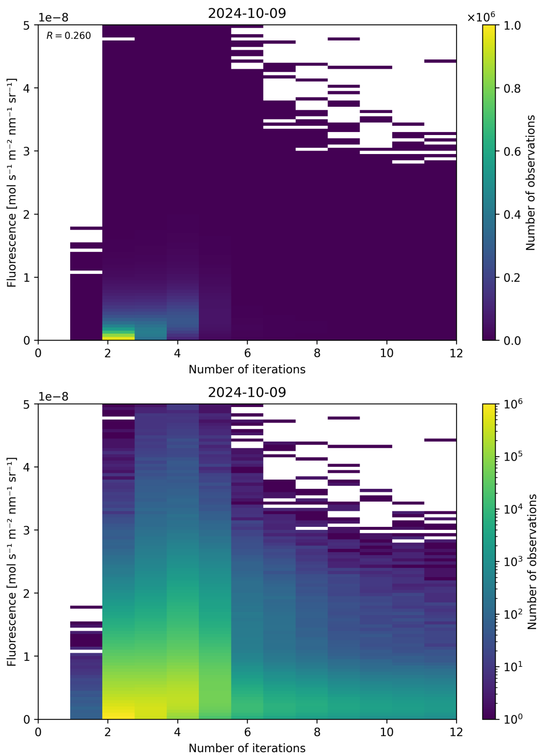
Figure 107: Scatter density plot of “Number of iterations” against “Fluorescence” for 2024-10-08 to 2024-10-10.
