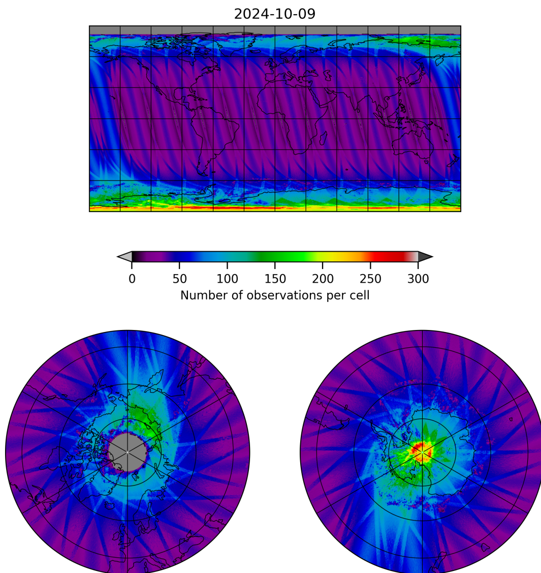
Figure 11: Map of the number of observations for 2024-10-08 to 2024-10-10
