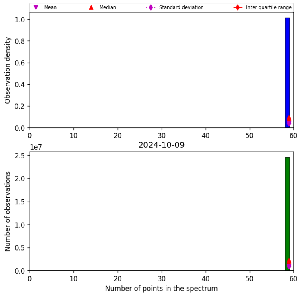
Figure 44: Histogram of “Number of points in the spectrum” for 2024-10-08 to 2024-10-10
