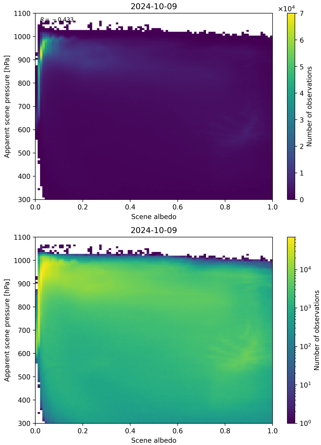
Figure 111: Scatter density plot of “Scene albedo” against “Apparent scene pressure” for 2024-10-08 to 2024-10-10.
