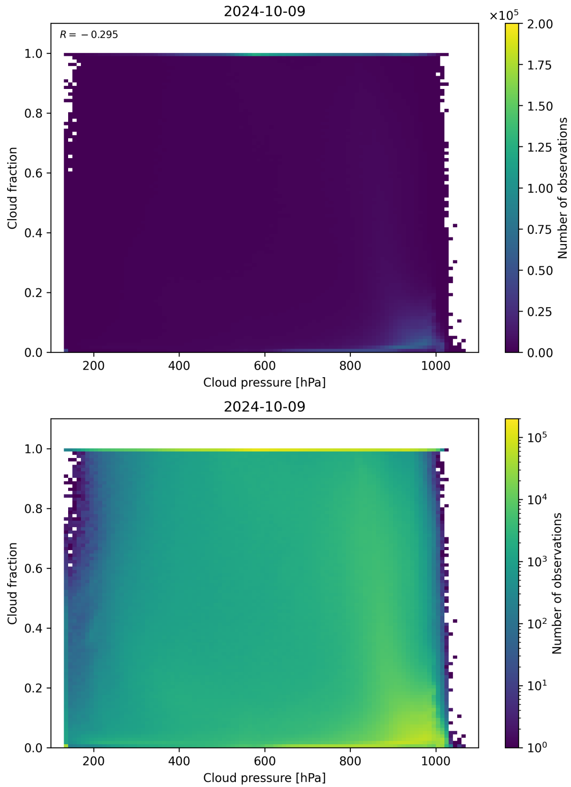
Figure 87: Scatter density plot of “Cloud pressure” against “Cloud fraction” for 2024-10-08 to 2024-10-10.
