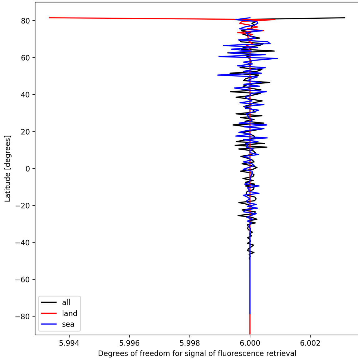
Figure 26: Zonal average of “Degrees of freedom for signal of fluorescence retrieval” for 2024-10-08 to 2024-10-10.
