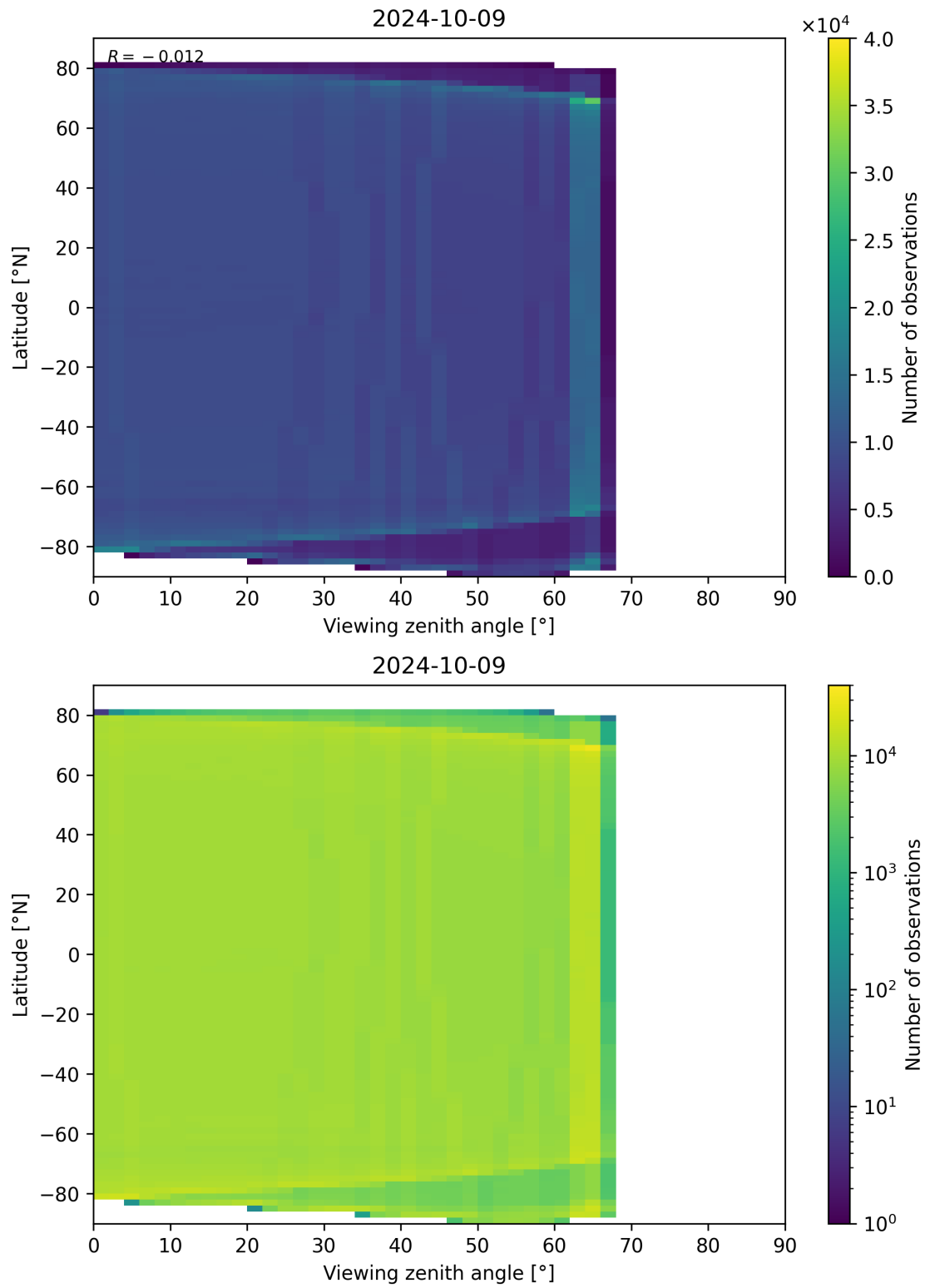
Figure 135: Scatter density plot of “Viewing zenith angle” against “Latitude” for 2024-10-08 to 2024-10-10.
