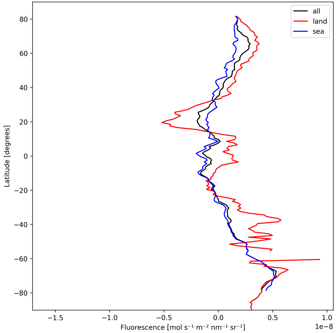
Figure 23: Zonal average of “Fluorescence” for 2024-10-08 to 2024-10-10.
