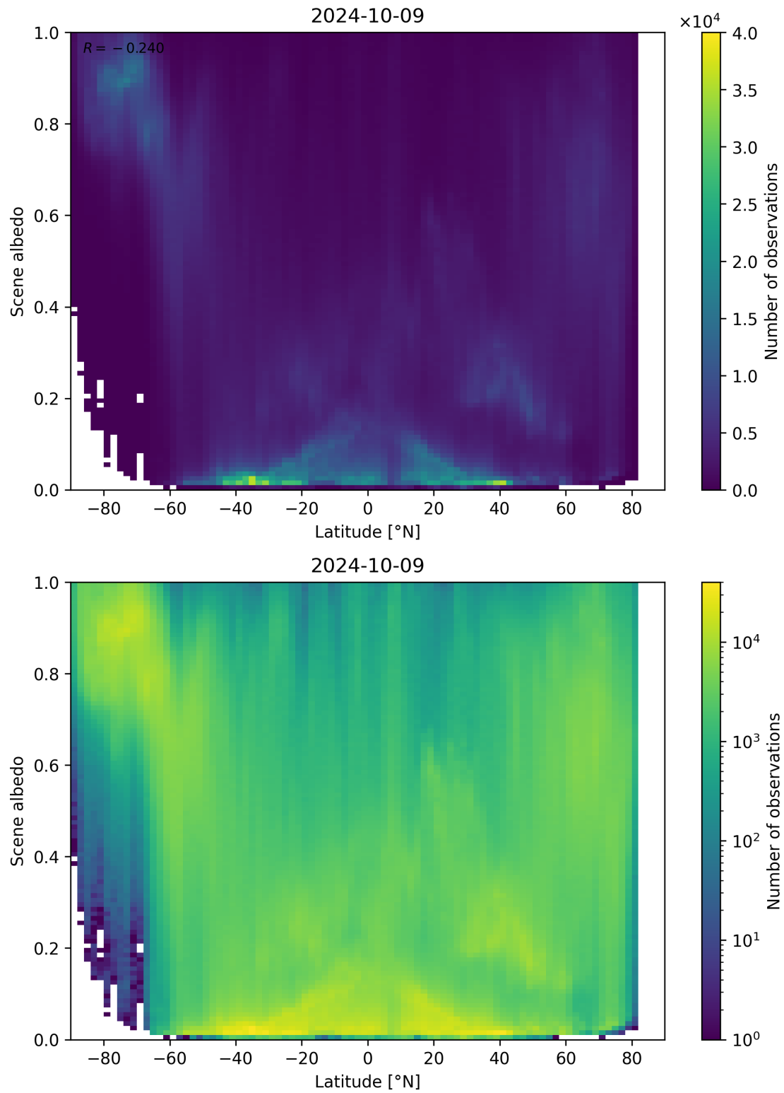
Figure 104: Scatter density plot of “Latitude” against “Scene albedo” for 2024-10-08 to 2024-10-10.
