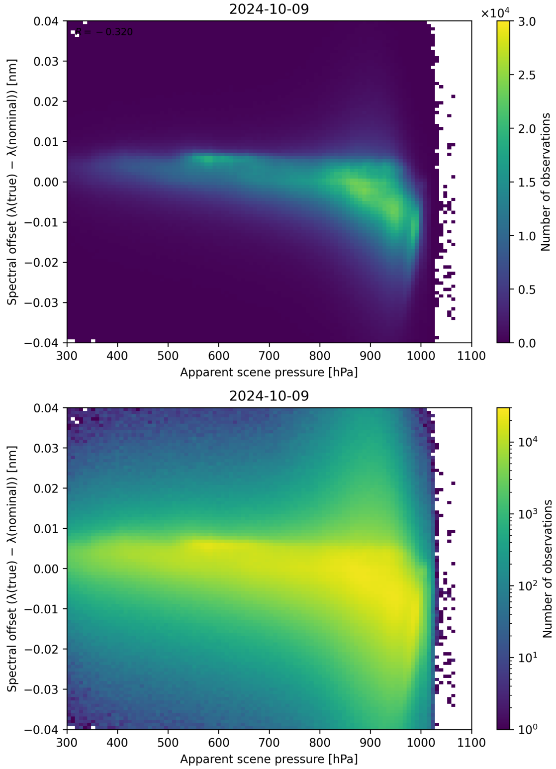
Figure 68: Scatter density plot of “Apparent scene pressure” against “Spectral offset ( \lambda_{\text{true}} - \lambda_{\text{nominal}} )” for 2024-10-08 to 2024-10-10.
