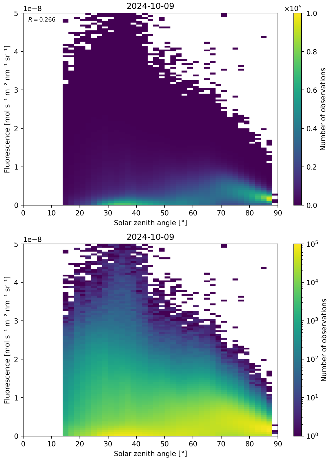
Figure 123: Scatter density plot of “Solar zenith angle” against “Fluorescence” for 2024-10-08 to 2024-10-10.
