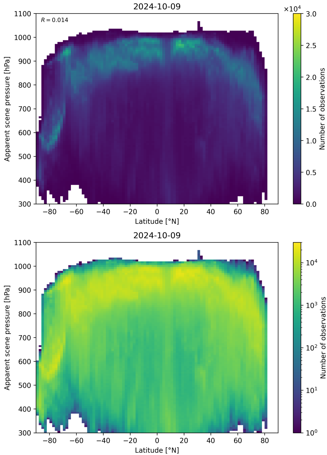
Figure 96: Scatter density plot of “Latitude” against “Apparent scene pressure” for 2024-10-08 to 2024-10-10.
