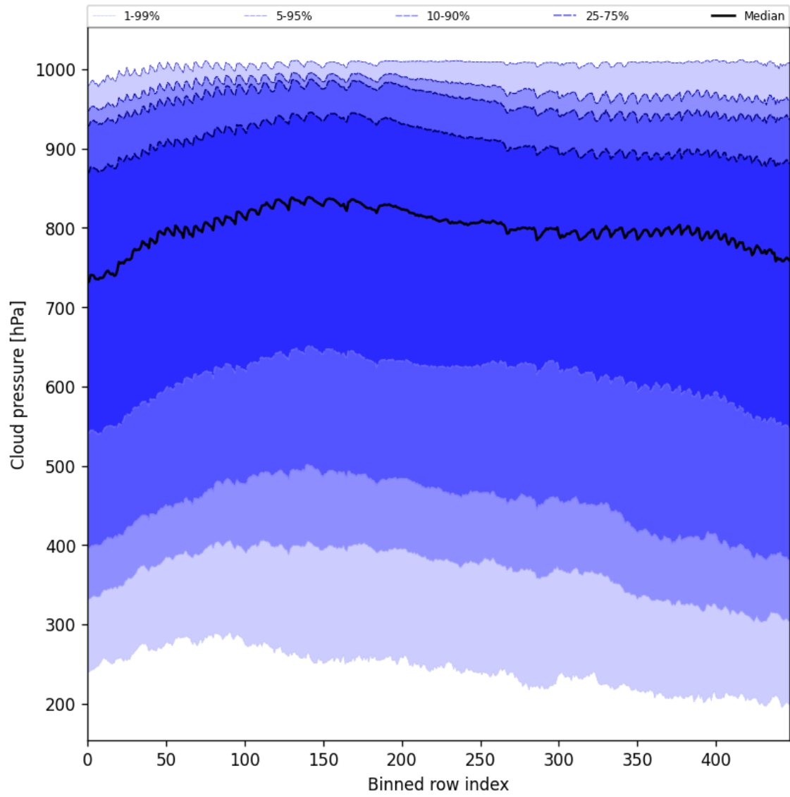
Figure 47: Along track statistics of “Cloud pressure” for 2024-10-08 to 2024-10-10
