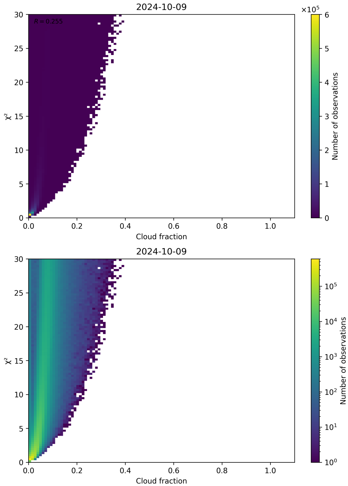
Figure 77: Scatter density plot of “Cloud fraction” against “ \chi^2 ” for 2024-10-08 to 2024-10-10.
