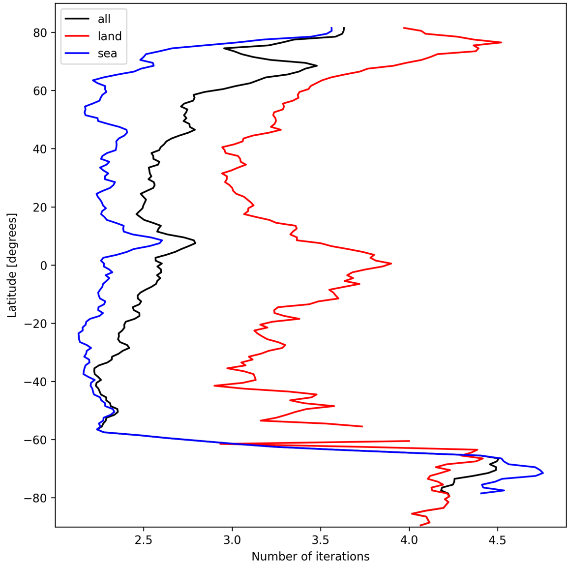
Figure 22: Zonal average of “Number of iterations” for 2024-10-08 to 2024-10-10.
