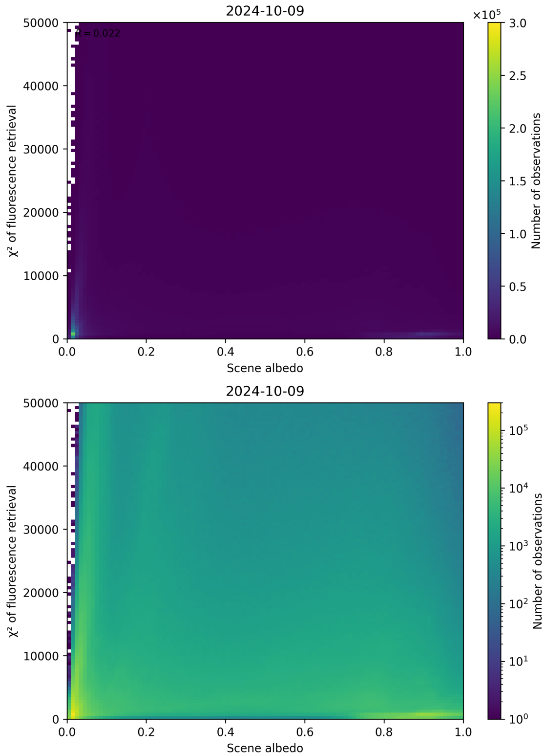
Figure 113: Scatter density plot of “Scene albedo” against “ \chi^2 of fluorescence retrieval” for 2024-10-08 to 2024-10-10.
