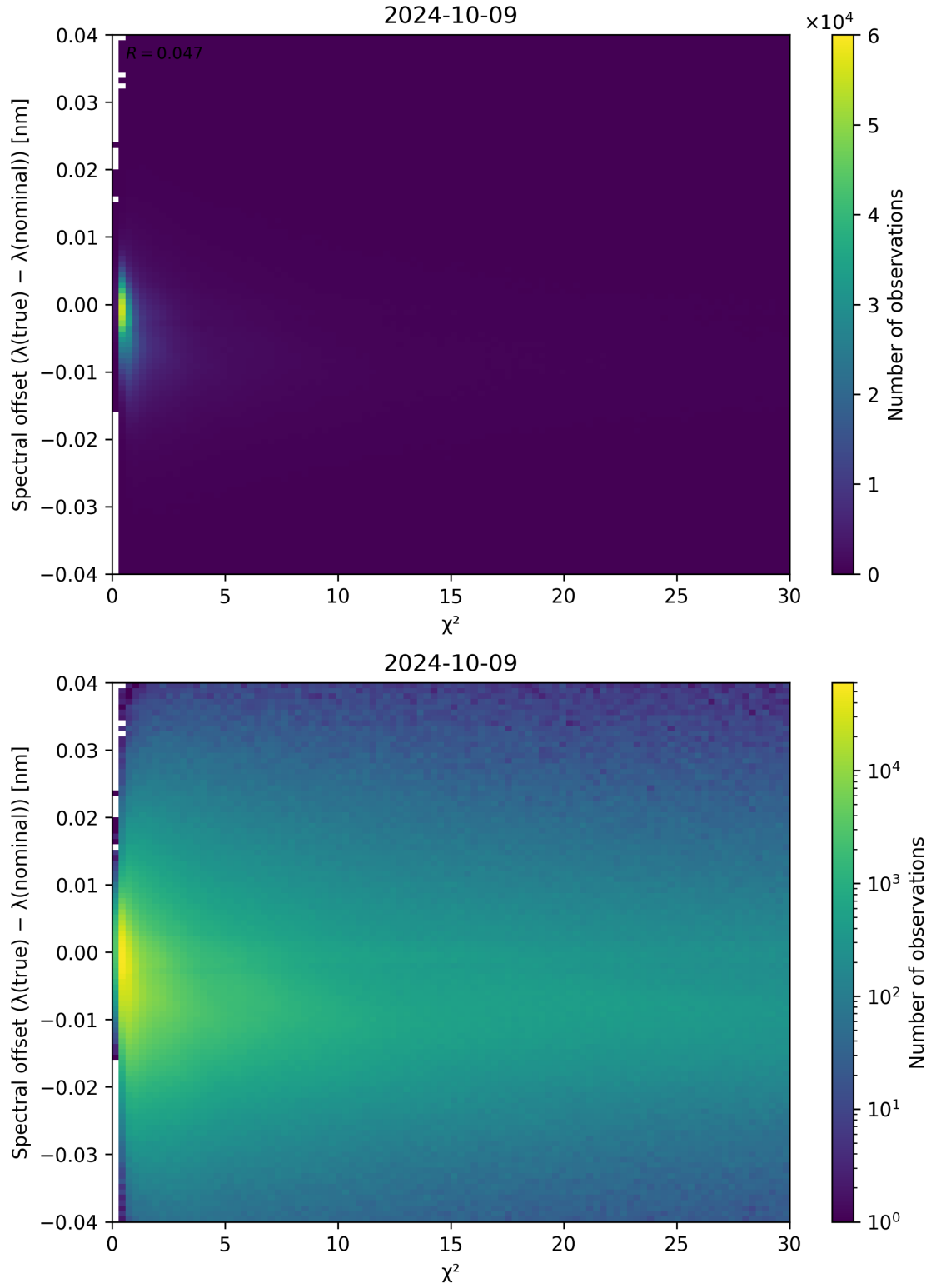
Figure 75: Scatter density plot of “ \chi^2 ” against “Spectral offset ( \lambda_{\text{true}} - \lambda_{\text{nominal}} )” for 2024-10-08 to 2024-10-10.
