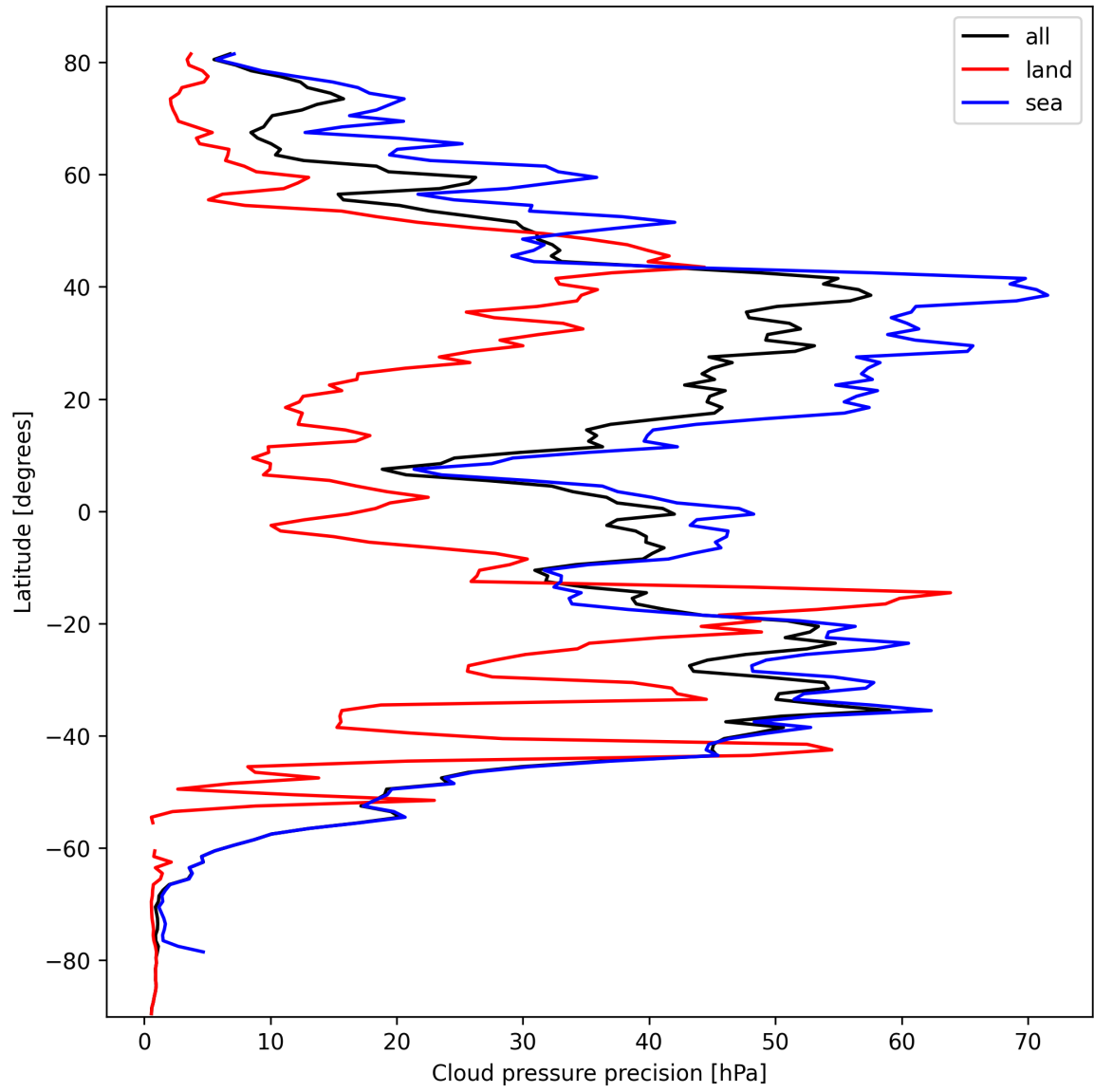
Figure 14: Zonal average of “Cloud pressure precision” for 2024-10-08 to 2024-10-10.
