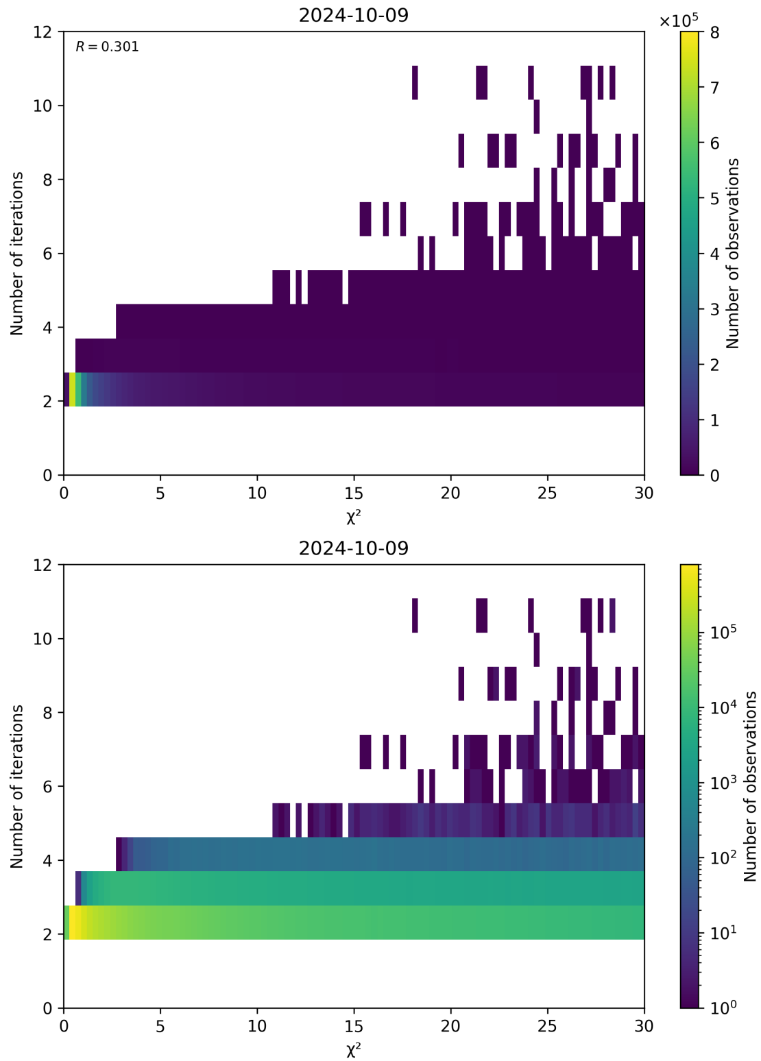
Figure 73: Scatter density plot of “ \chi^2 ” against “Number of iterations” for 2024-10-08 to 2024-10-10.
