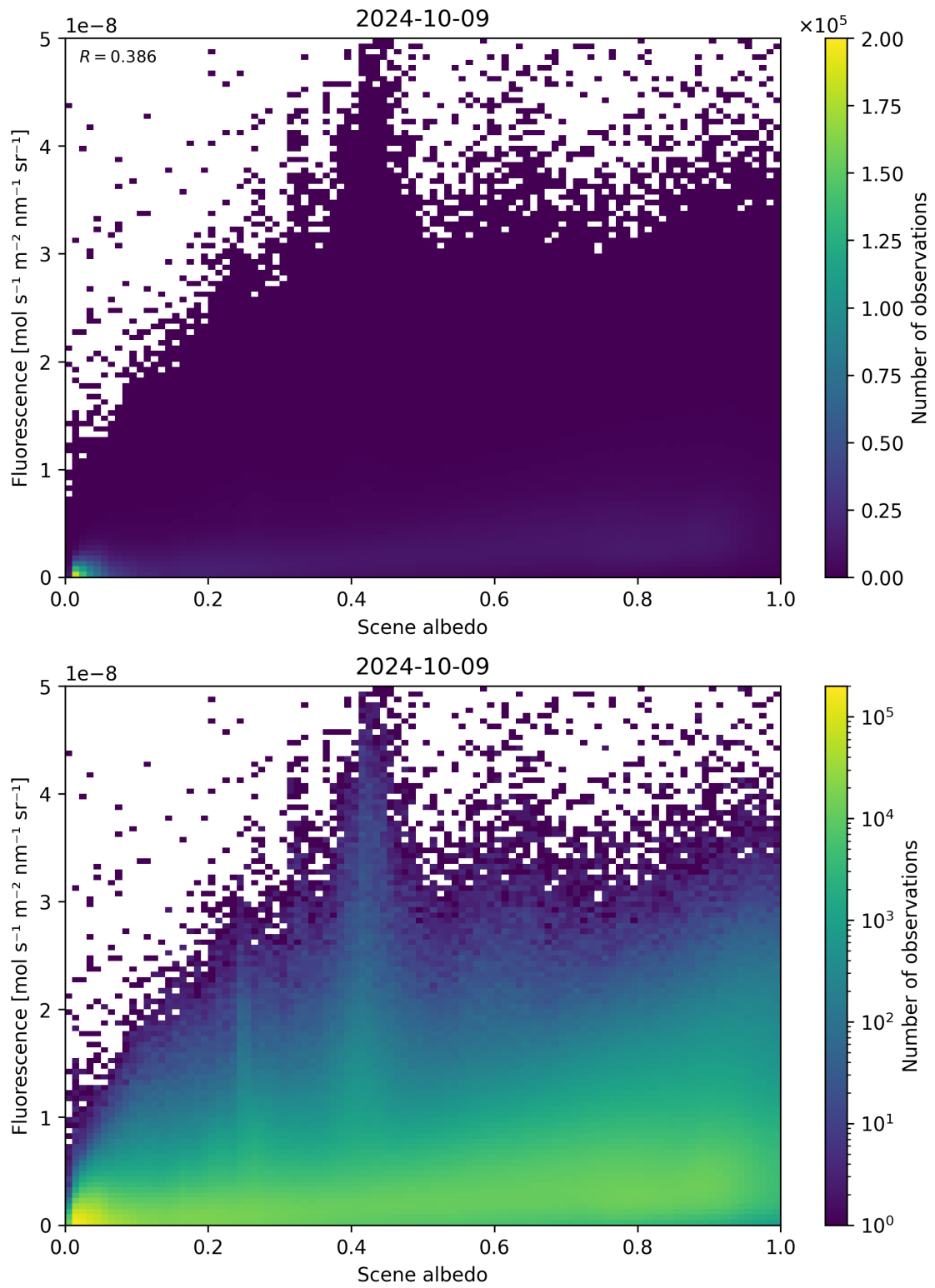
Figure 114: Scatter density plot of “Scene albedo” against “Fluorescence” for 2024-10-08 to 2024-10-10.
