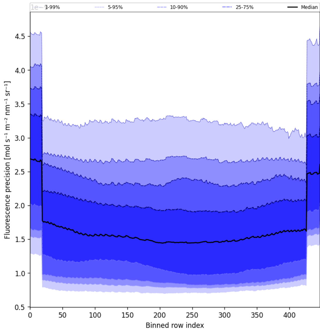
Figure 58: Along track statistics of “Fluorescence precision” for 2024-10-08 to 2024-10-10
