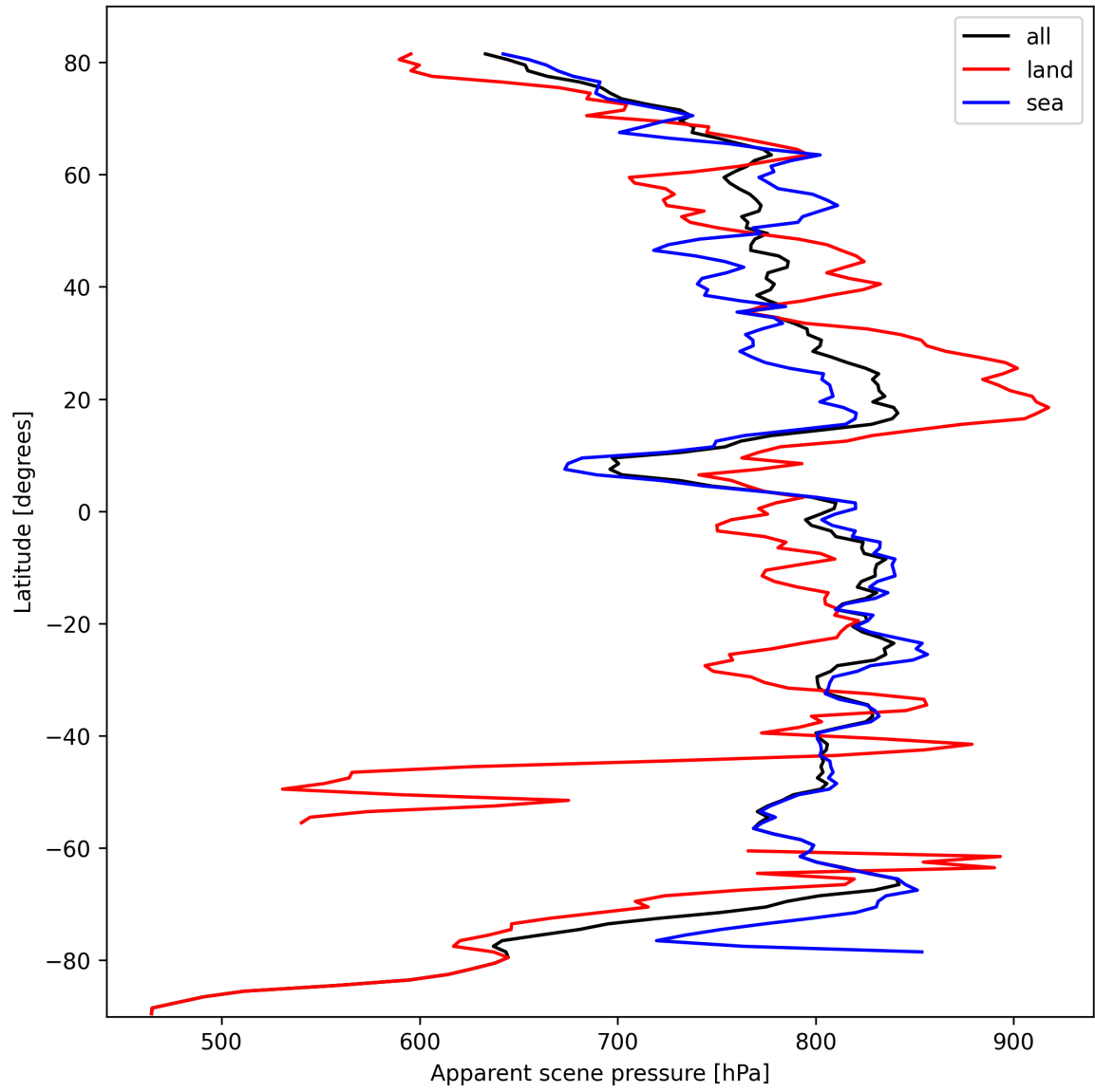
Figure 19: Zonal average of “Apparent scene pressure” for 2024-10-08 to 2024-10-10.
