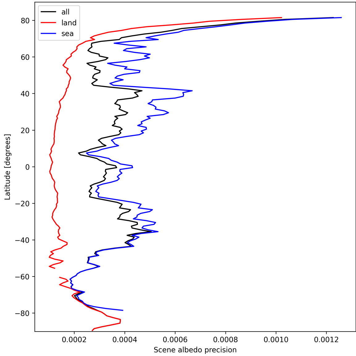
Figure 18: Zonal average of "Scene albedo precision" for 2024-10-08 to 2024-10-10.
