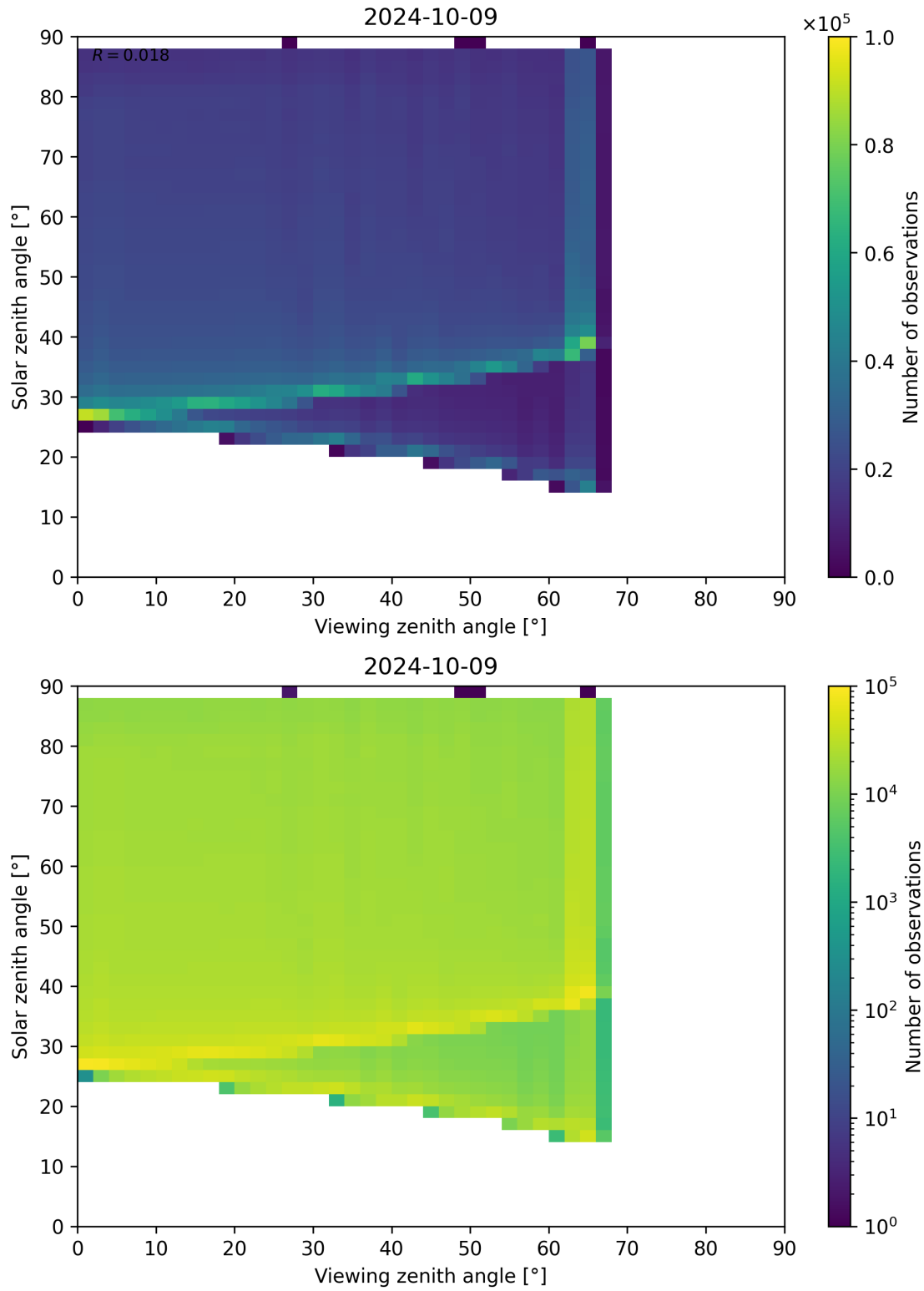
Figure 139: Scatter density plot of “Viewing zenith angle” against “Solar zenith angle” for 2024-10-08 to 2024-10-10.
