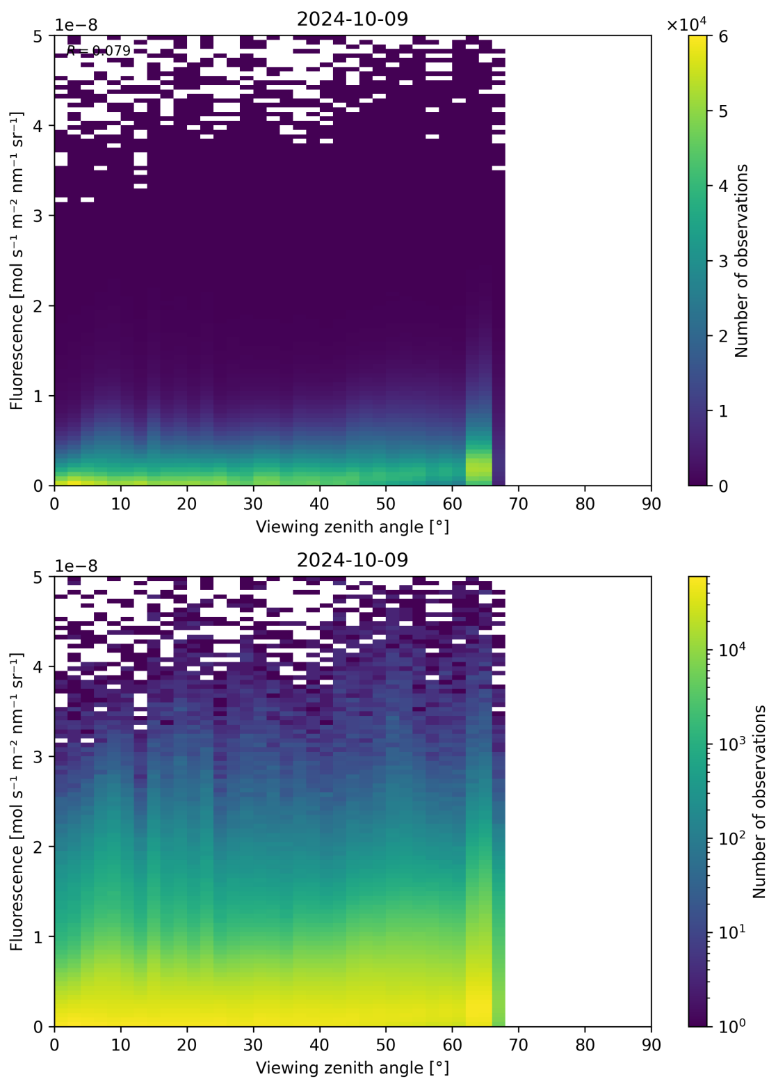
Figure 134: Scatter density plot of “Viewing zenith angle” against “Fluorescence” for 2024-10-08 to 2024-10-10.
