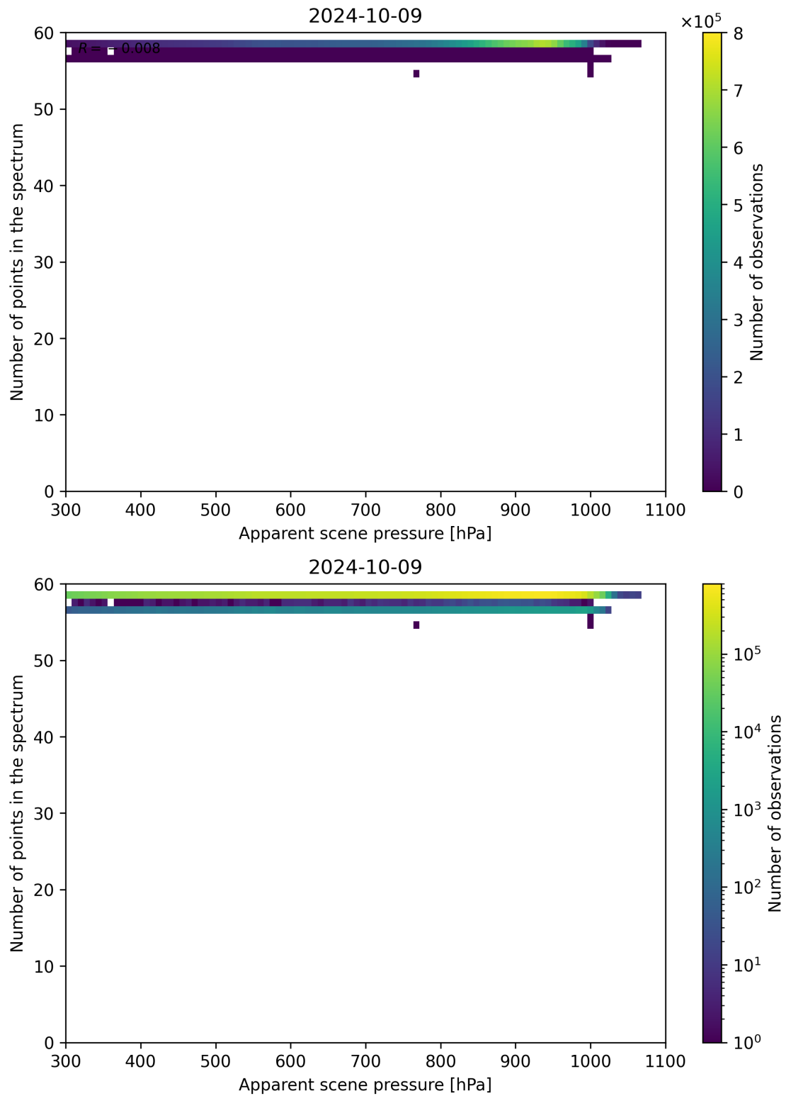
Figure 67: Scatter density plot of “Apparent scene pressure” against “Number of points in the spectrum” for 2024-10-08 to 2024-10-10.
