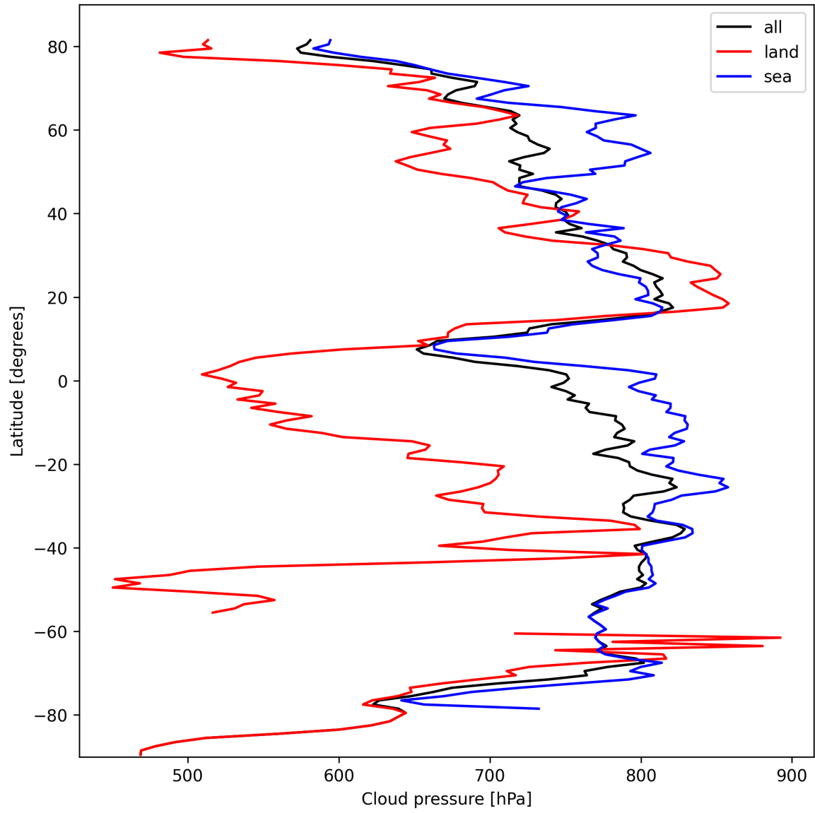
Figure 13: Zonal average of “Cloud pressure” for 2024-10-08 to 2024-10-10.
