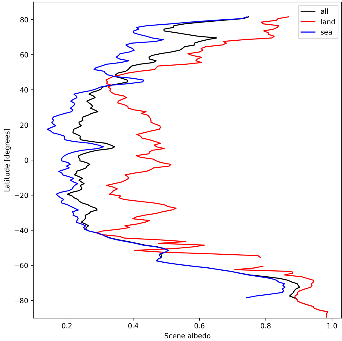
Figure 17: Zonal average of “Scene albedo” for 2024-10-08 to 2024-10-10.
