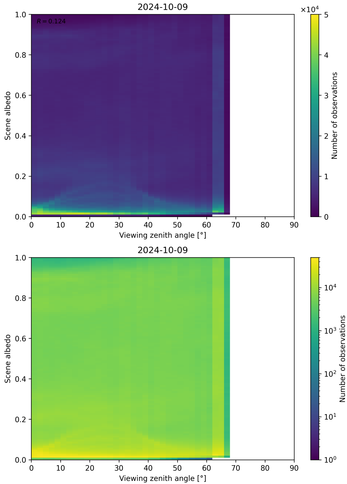
Figure 138: Scatter density plot of “Viewing zenith angle” against “Scene albedo” for 2024-10-08 to 2024-10-10.
