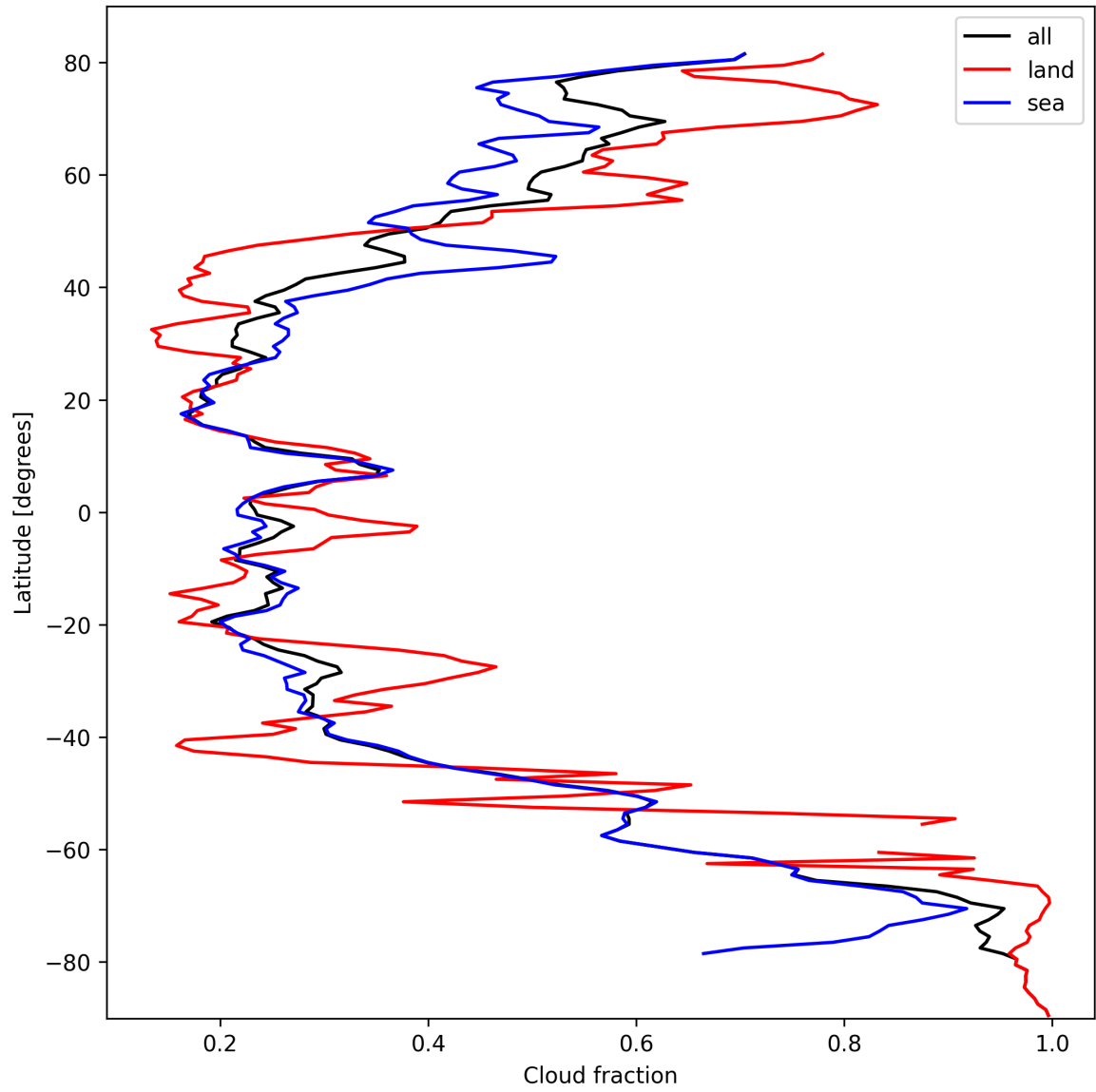
Figure 15: Zonal average of “Cloud fraction” for 2024-10-08 to 2024-10-10.
