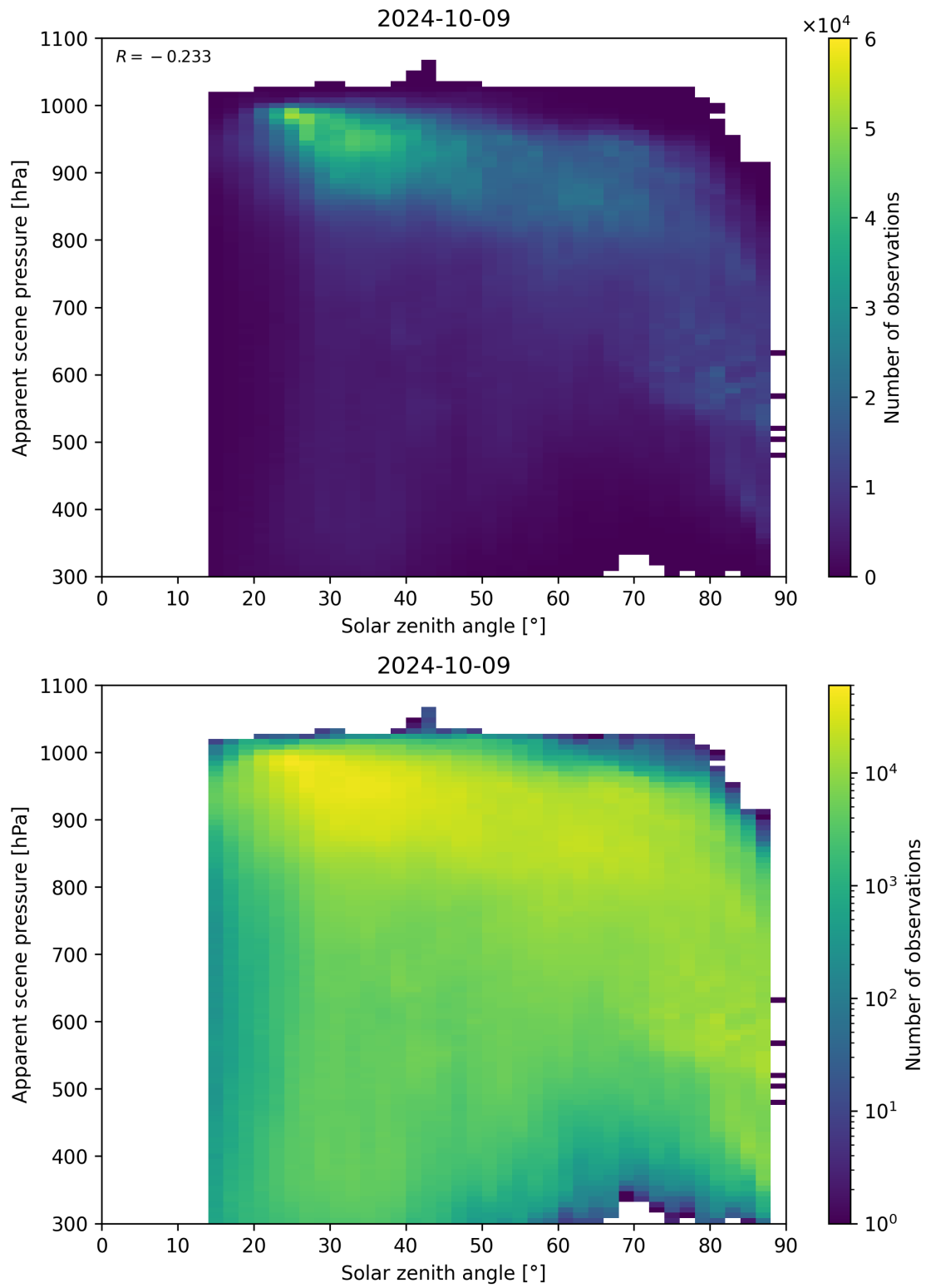
Figure 118: Scatter density plot of “Solar zenith angle” against “Apparent scene pressure” for 2024-10-08 to 2024-10-10.
