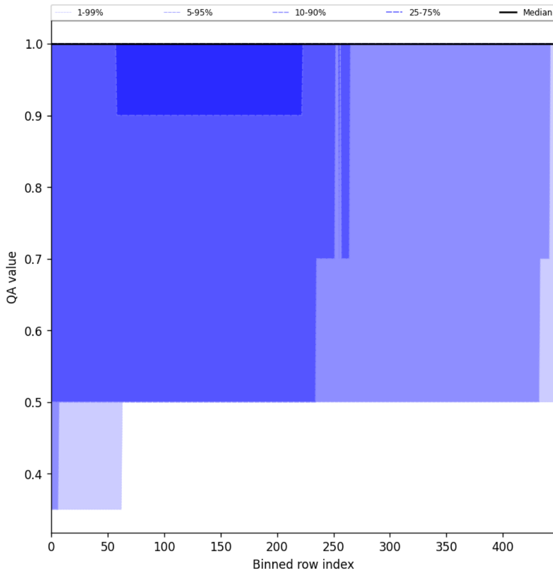
Figure 46: Along track statistics of “QA value” for 2024-10-08 to 2024-10-10
