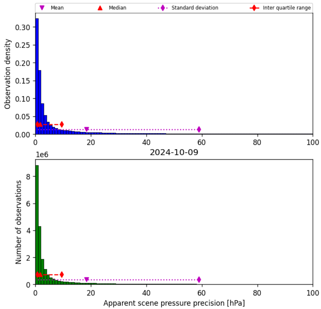
Figure 37: Histogram of “Apparent scene pressure precision” for 2024-10-08 to 2024-10-10
