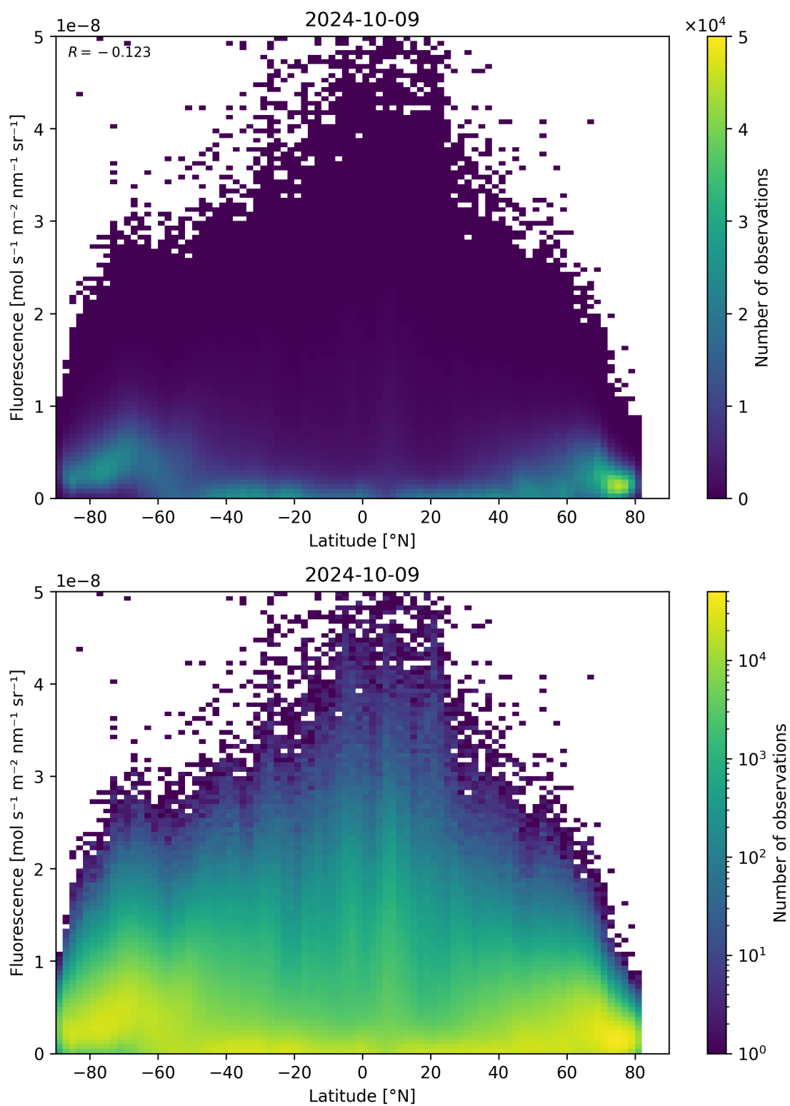
Figure 101: Scatter density plot of “Latitude” against “Fluorescence” for 2024-10-08 to 2024-10-10.
