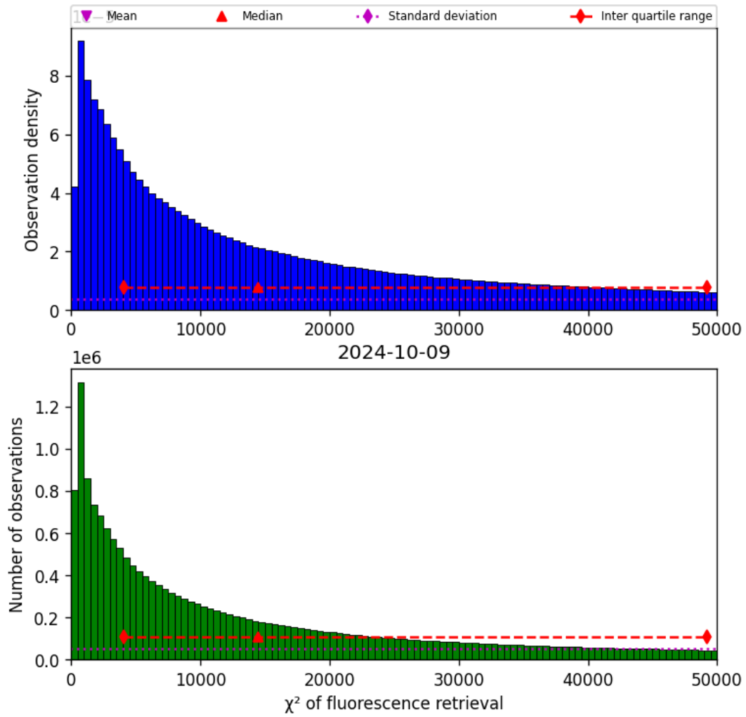
Figure 42: Histogram of “ \chi^2 of fluorescence retrieval” for 2024-10-08 to 2024-10-10
