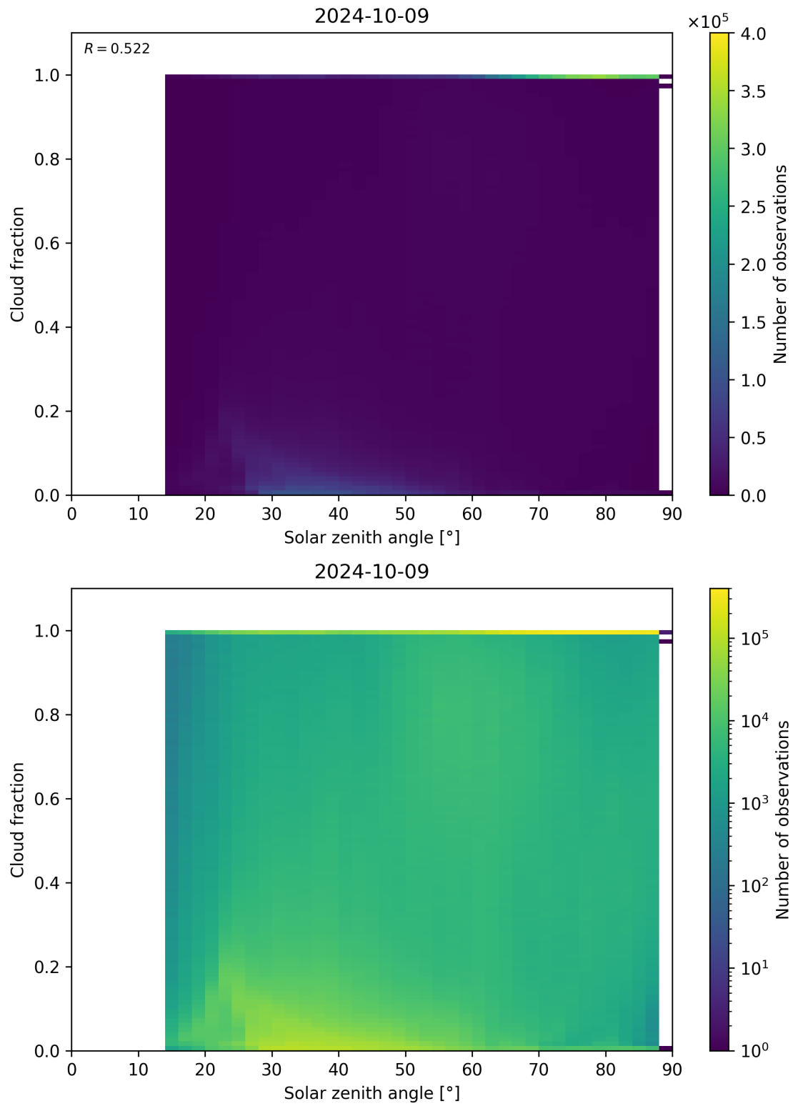
Figure 121: Scatter density plot of “Solar zenith angle” against “Cloud fraction” for 2024-10-08 to 2024-10-10.
