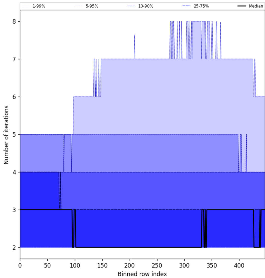
Figure 56: Along track statistics of “Number of iterations” for 2024-10-08 to 2024-10-10
