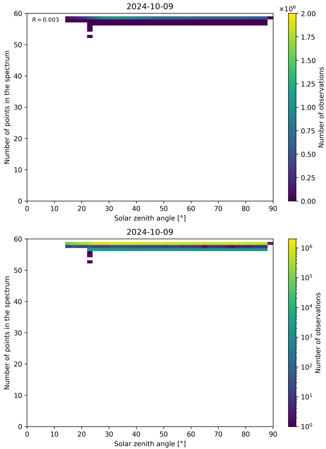
Figure 126: Scatter density plot of “Solar zenith angle” against “Number of points in the spectrum” for 2024-10-08 to 2024-10-10.
