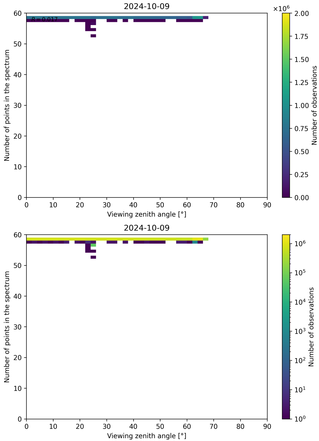
Figure 137: Scatter density plot of “Viewing zenith angle” against “Number of points in the spectrum” for 2024-10-08 to 2024-10-10.
