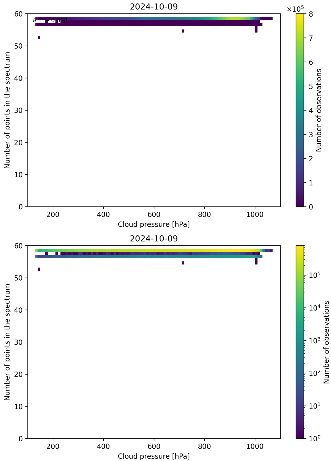
Figure 90: Scatter density plot of “Cloud pressure” against “Number of points in the spectrum” for 2024-10-08 to 2024-10-10.
