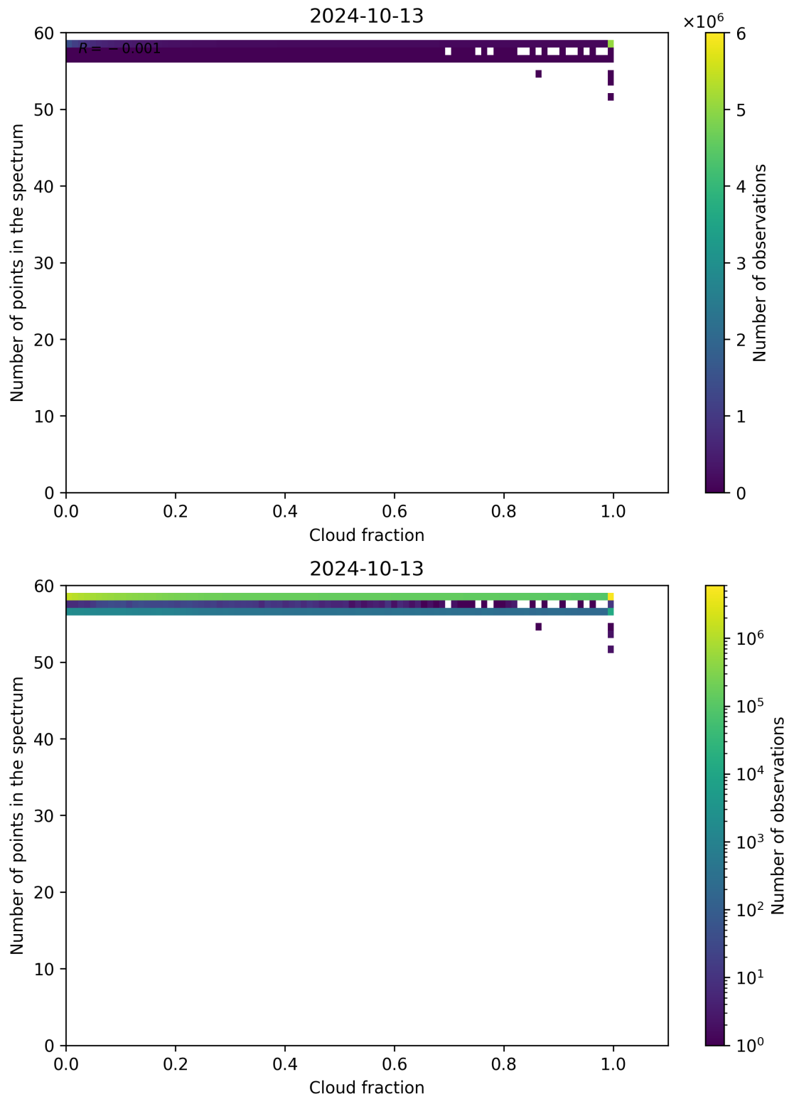
Figure 81: Scatter density plot of “Cloud fraction” against “Number of points in the spectrum” for 2024-10-12 to 2024-10-14.
