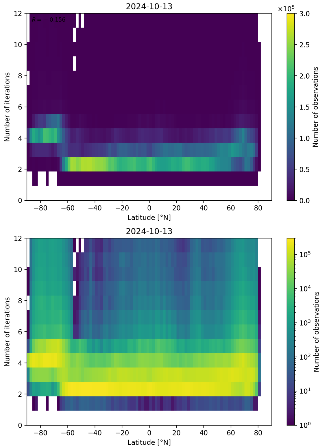
Figure 102: Scatter density plot of “Latitude” against “Number of iterations” for 2024-10-12 to 2024-10-14.
