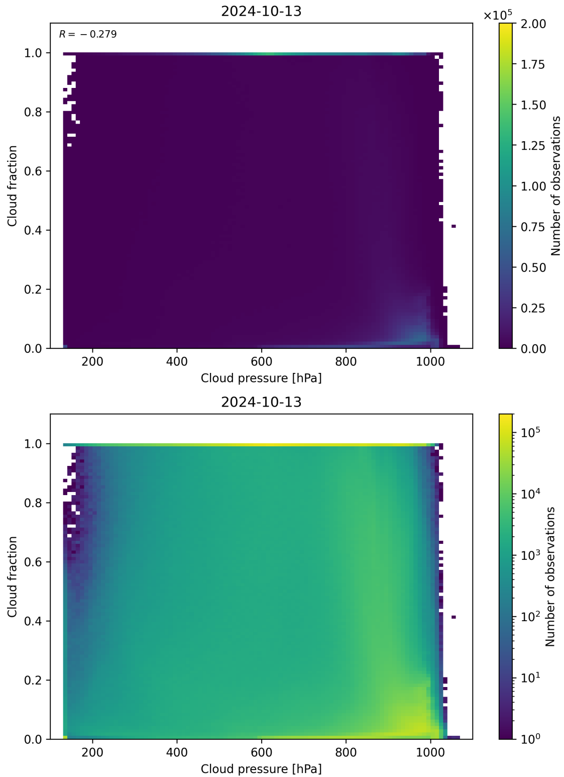
Figure 87: Scatter density plot of “Cloud pressure” against “Cloud fraction” for 2024-10-12 to 2024-10-14.
