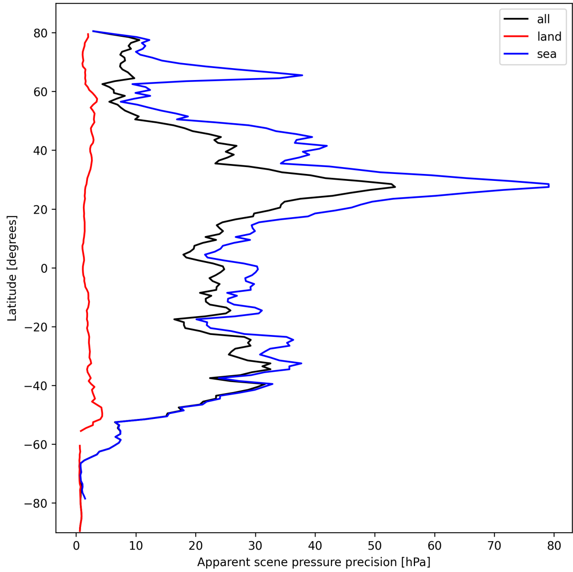
Figure 20: Zonal average of “Apparent scene pressure precision” for 2024-10-12 to 2024-10-14.
