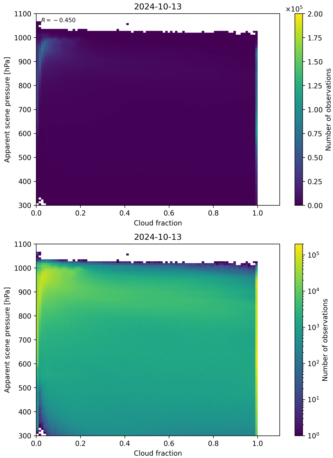
Figure 76: Scatter density plot of “Cloud fraction” against “Apparent scene pressure” for 2024-10-12 to 2024-10-14.
