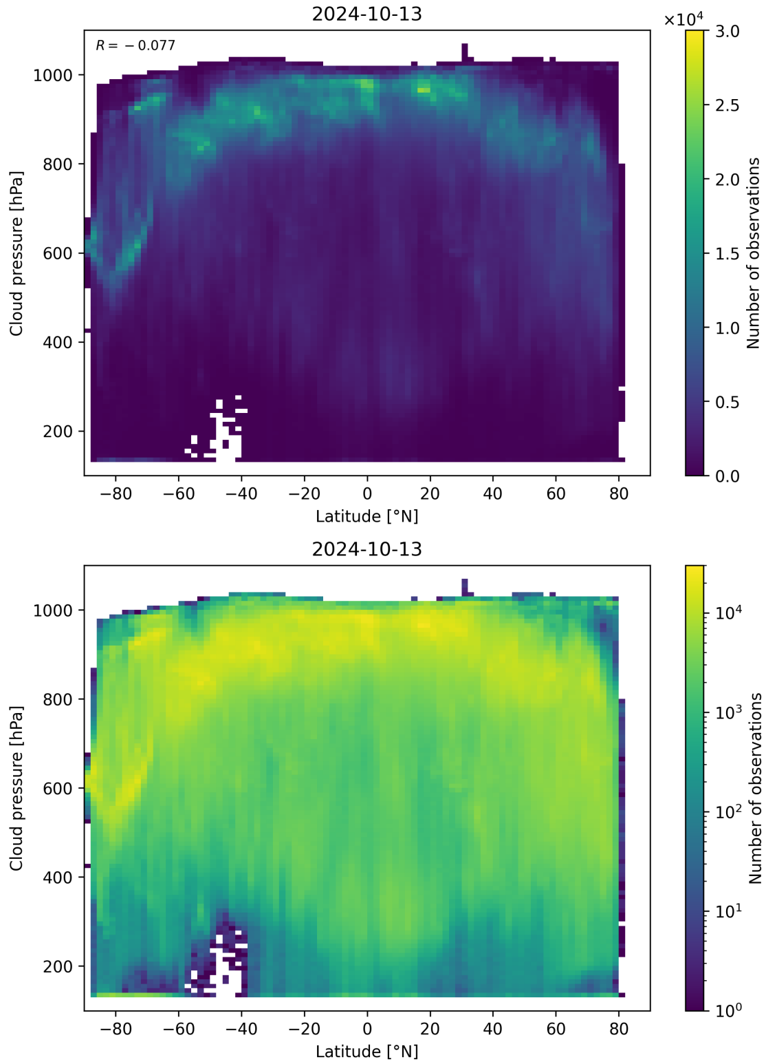
Figure 100: Scatter density plot of “Latitude” against “Cloud pressure” for 2024-10-12 to 2024-10-14.
