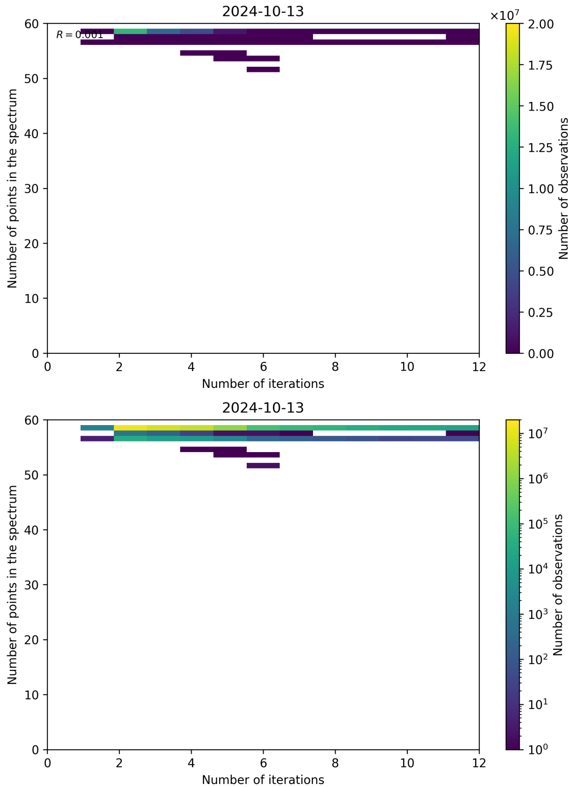
Figure 108: Scatter density plot of “Number of iterations” against “Number of points in the spectrum” for 2024-10-12 to 2024-10-14.
