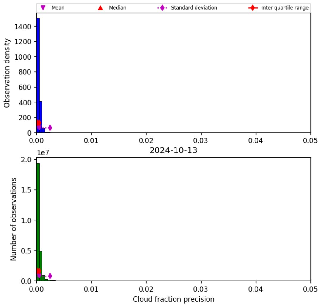
Figure 33: Histogram of “Cloud fraction precision” for 2024-10-12 to 2024-10-14
