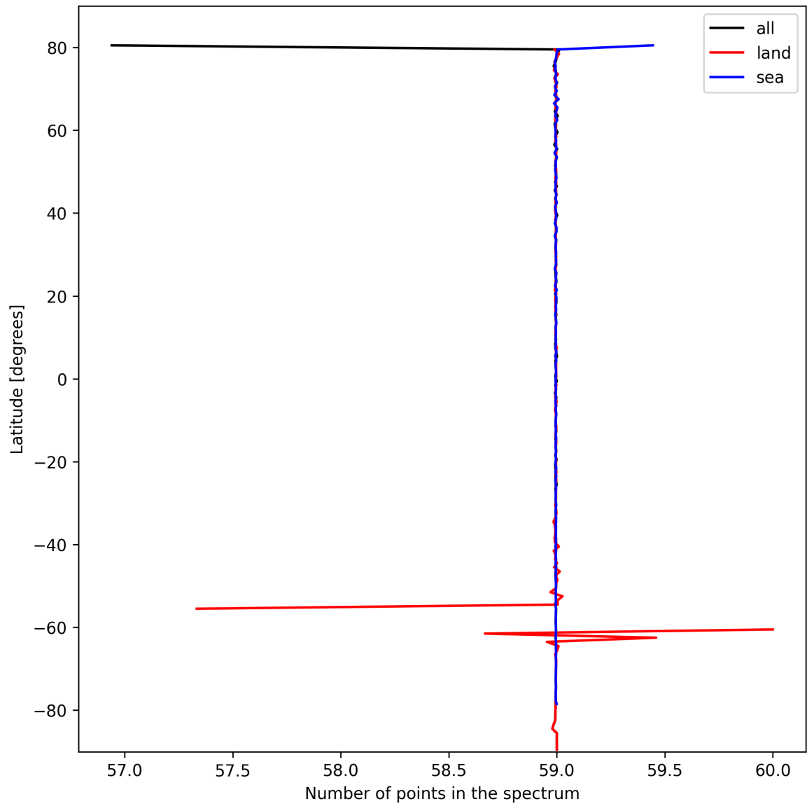
Figure 27: Zonal average of “Number of points in the spectrum” for 2024-10-12 to 2024-10-14.
