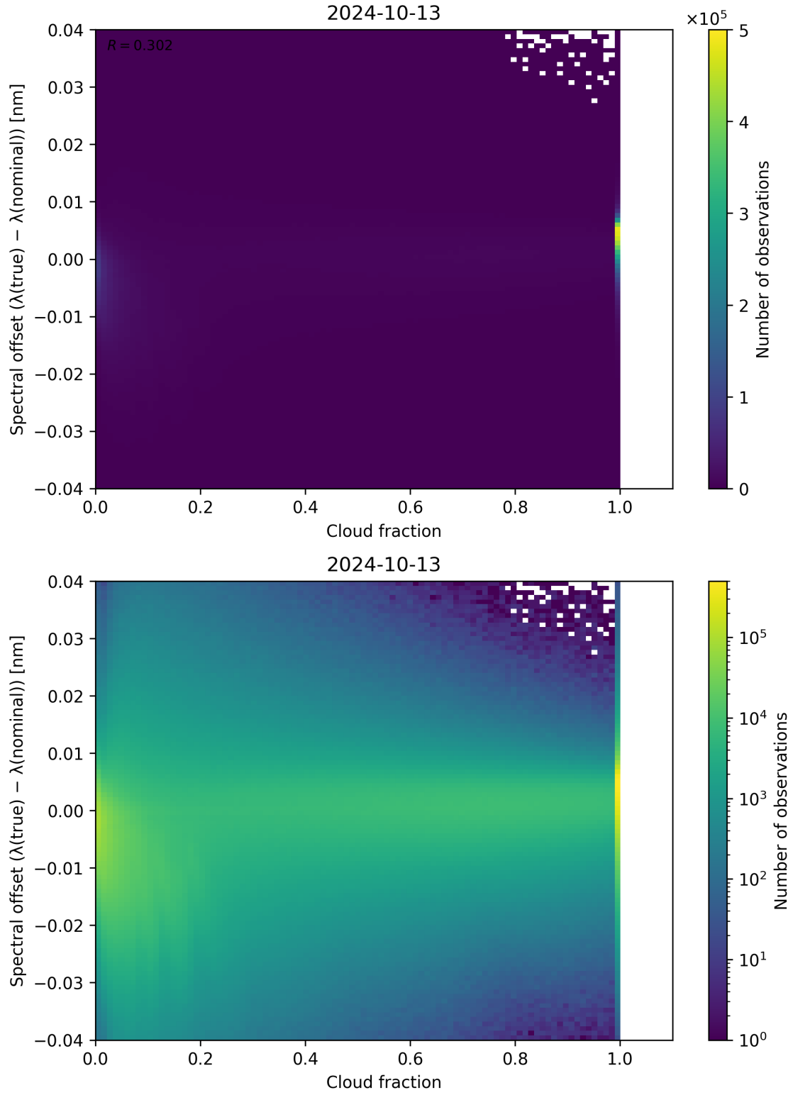
Figure 83: Scatter density plot of “Cloud fraction” against “Spectral offset ( \lambda_{\text{true}} - \lambda_{\text{nominal}} )” for 2024-10-12 to 2024-10-14.
