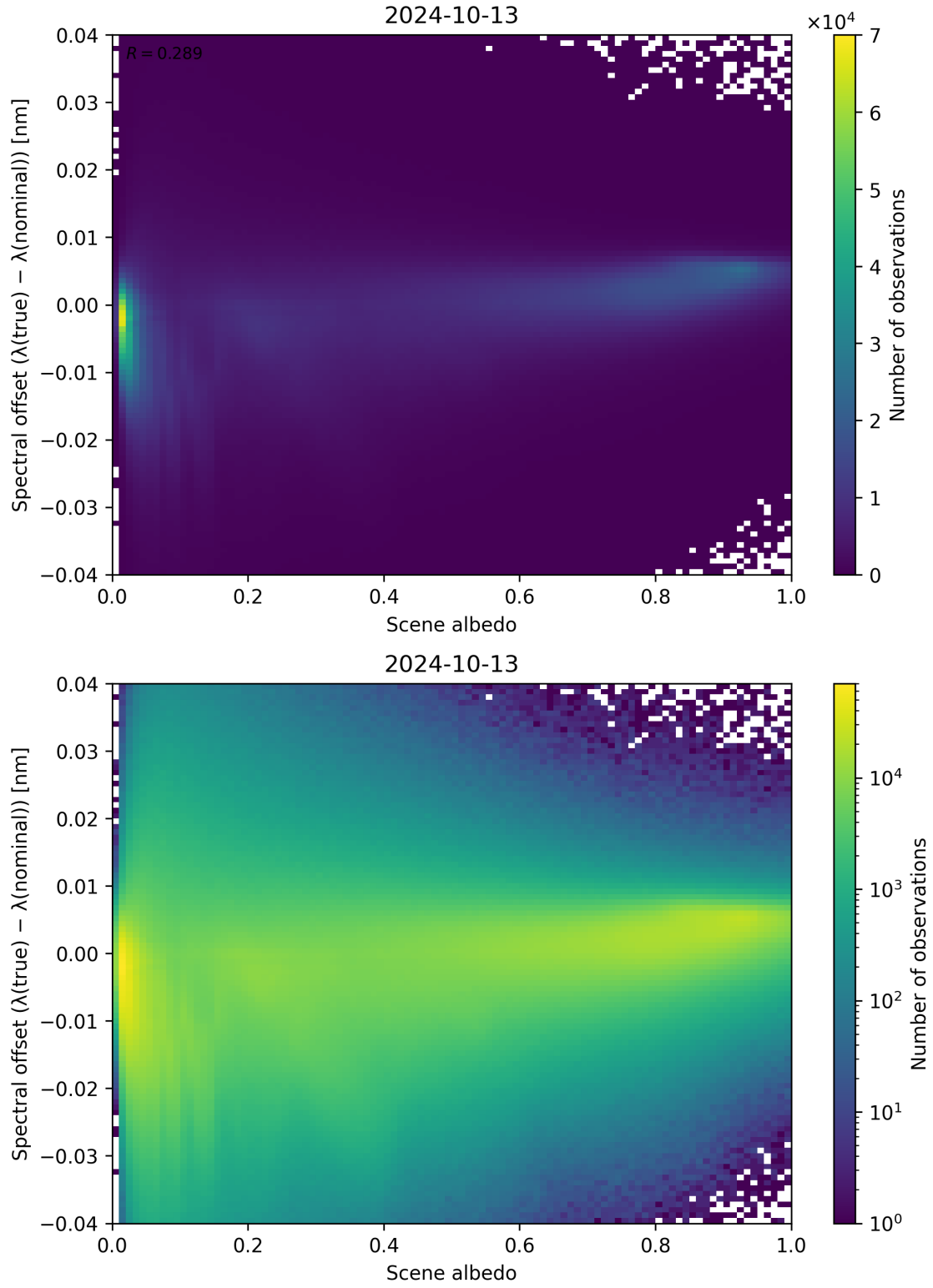
Figure 117: Scatter density plot of “Scene albedo” against “Spectral offset ( \lambda_{\text{true}} - \lambda_{\text{nominal}} )” for 2024-10-12 to 2024-10-14.
