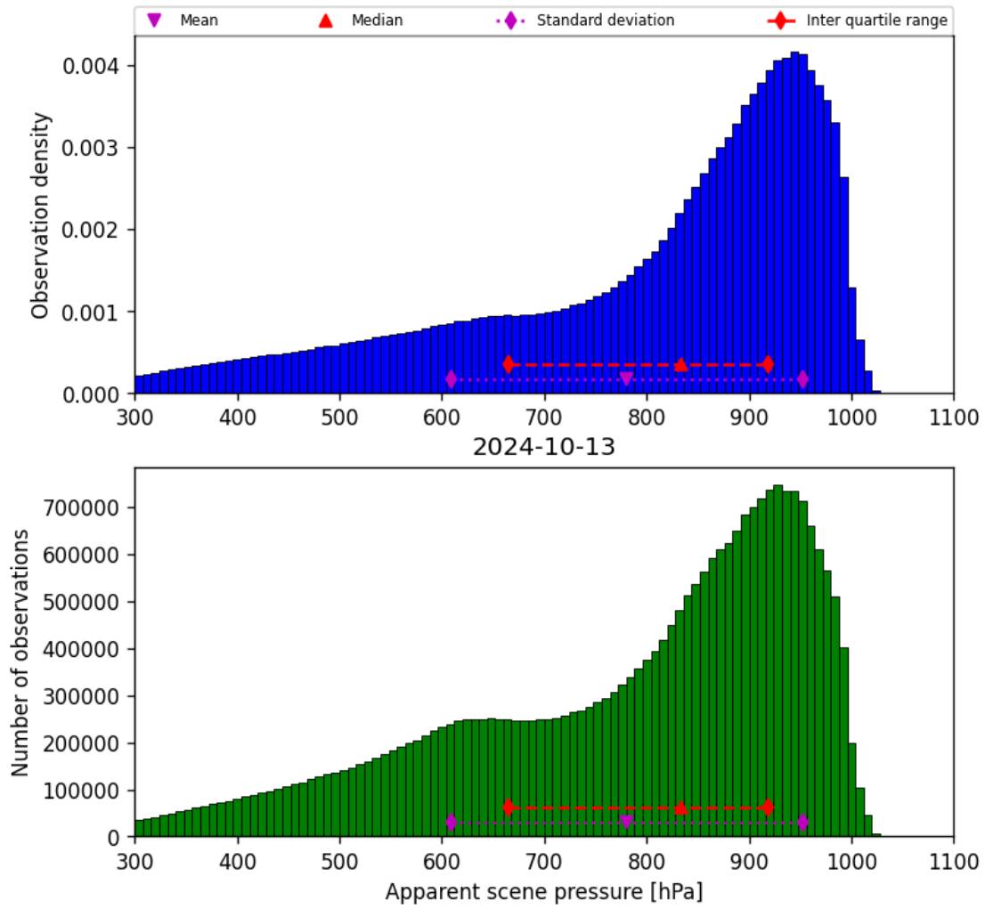
Figure 36: Histogram of “Apparent scene pressure” for 2024-10-12 to 2024-10-14
