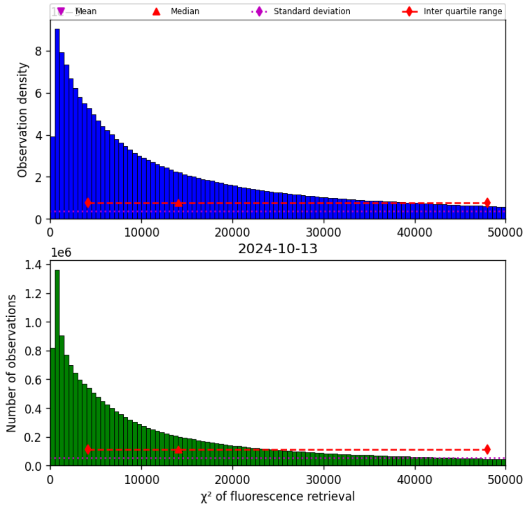
Figure 42: Histogram of “ \chi^2 of fluorescence retrieval” for 2024-10-12 to 2024-10-14
