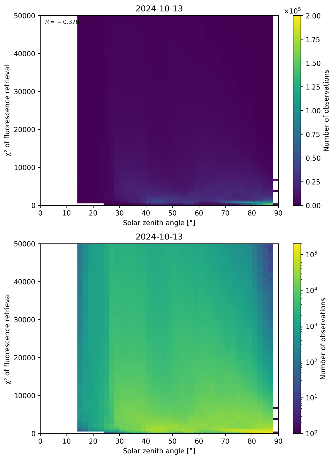
Figure 120: Scatter density plot of “Solar zenith angle” against “ \chi^2 of fluorescence retrieval” for 2024-10-12 to 2024-10-14.
