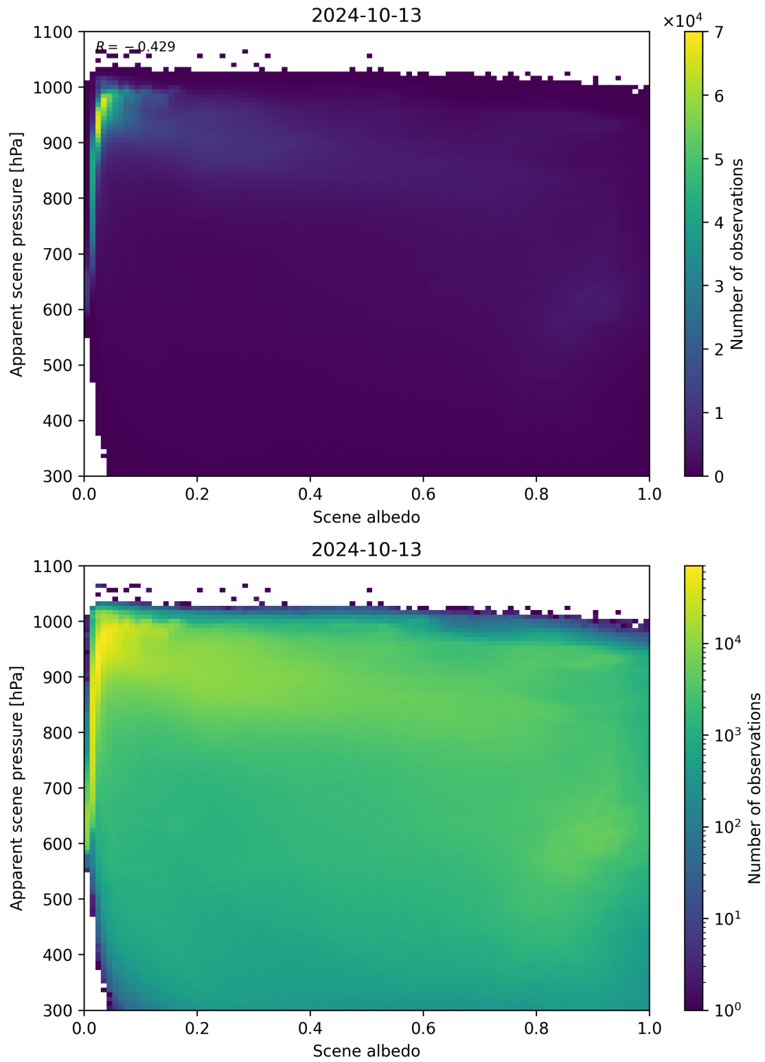
Figure 111: Scatter density plot of “Scene albedo” against “Apparent scene pressure” for 2024-10-12 to 2024-10-14.
