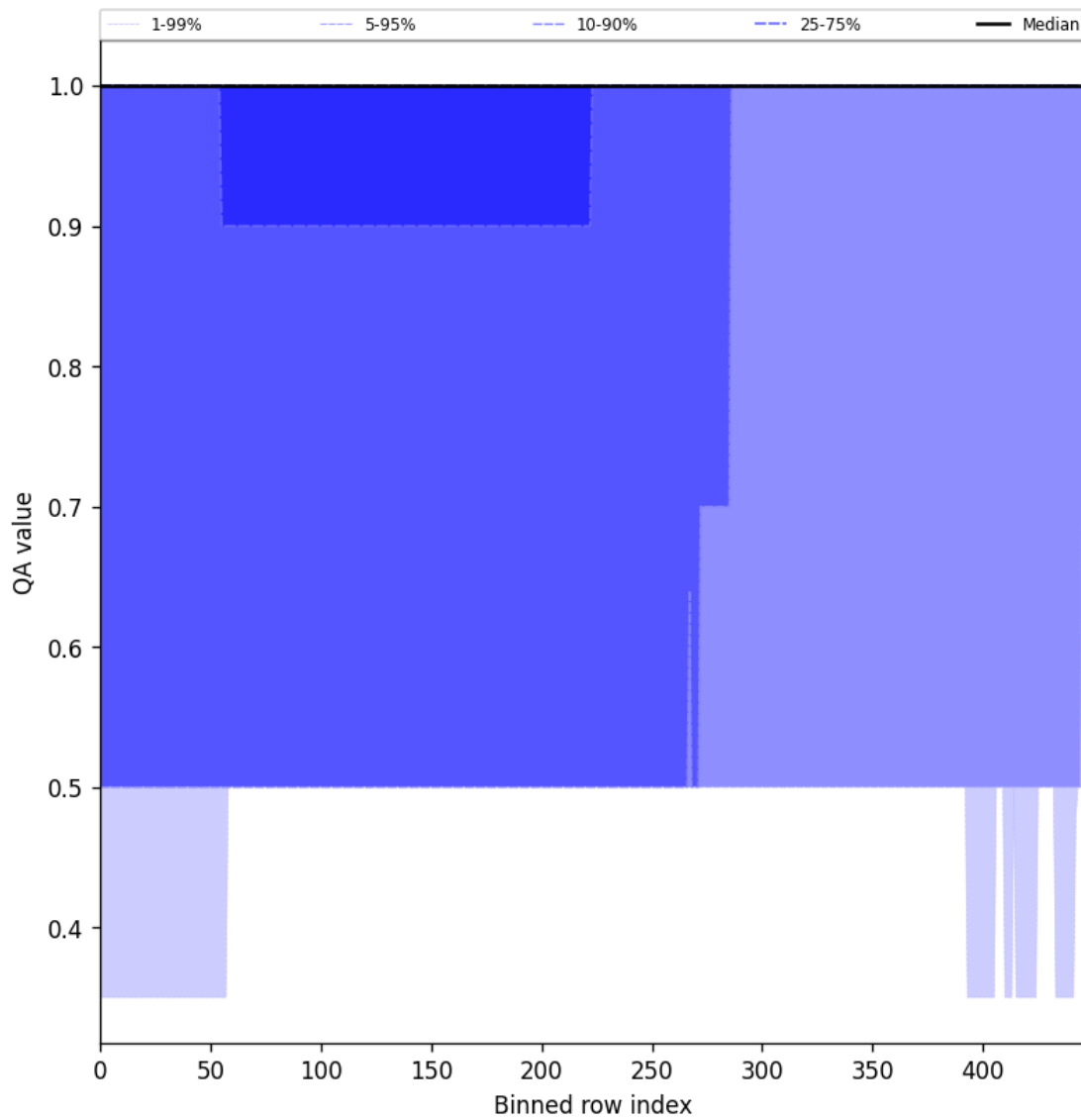
Figure 46: Along track statistics of “QA value” for 2024-10-12 to 2024-10-14
