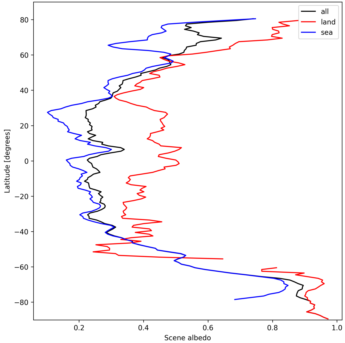
Figure 17: Zonal average of “Scene albedo” for 2024-10-12 to 2024-10-14.
