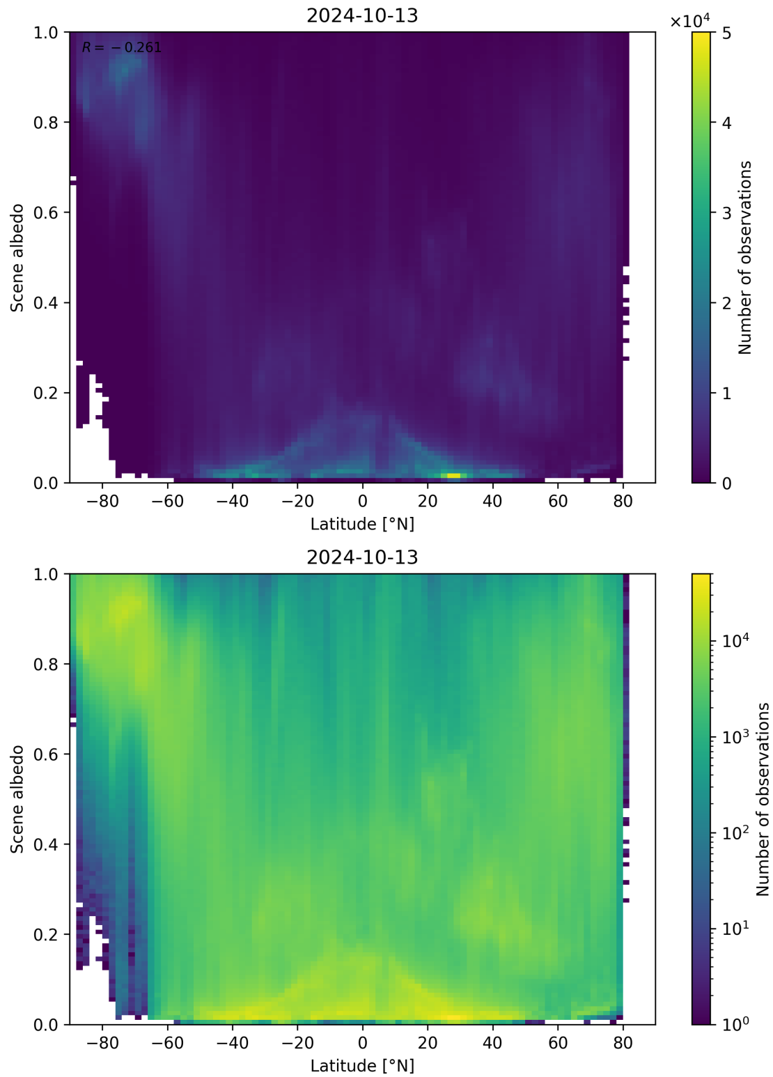
Figure 104: Scatter density plot of “Latitude” against “Scene albedo” for 2024-10-12 to 2024-10-14.
