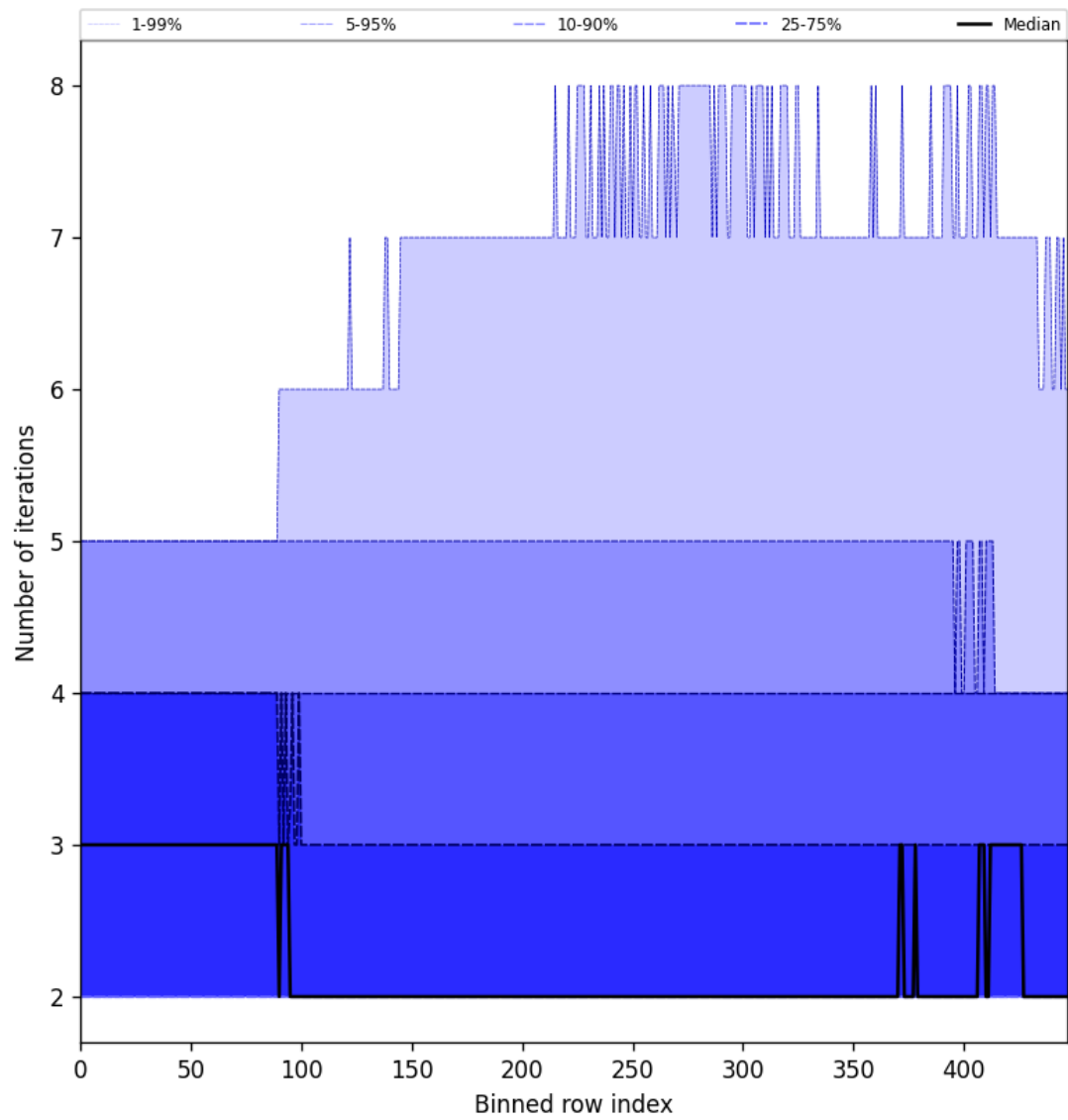
Figure 56: Along track statistics of “Number of iterations” for 2024-10-12 to 2024-10-14
