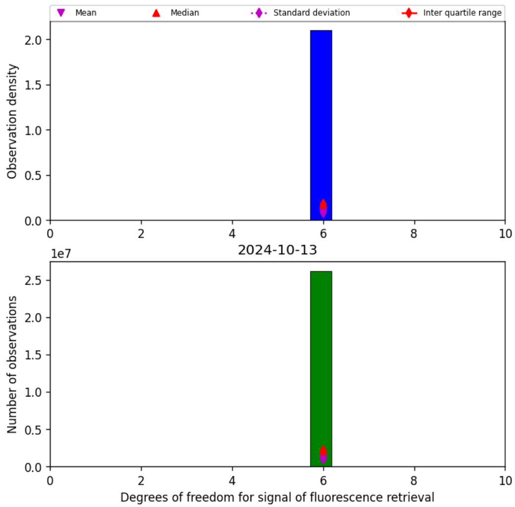
Figure 43: Histogram of "Degrees of freedom for signal of fluorescence retrieval" for 2024-10-12 to 2024-10-14
