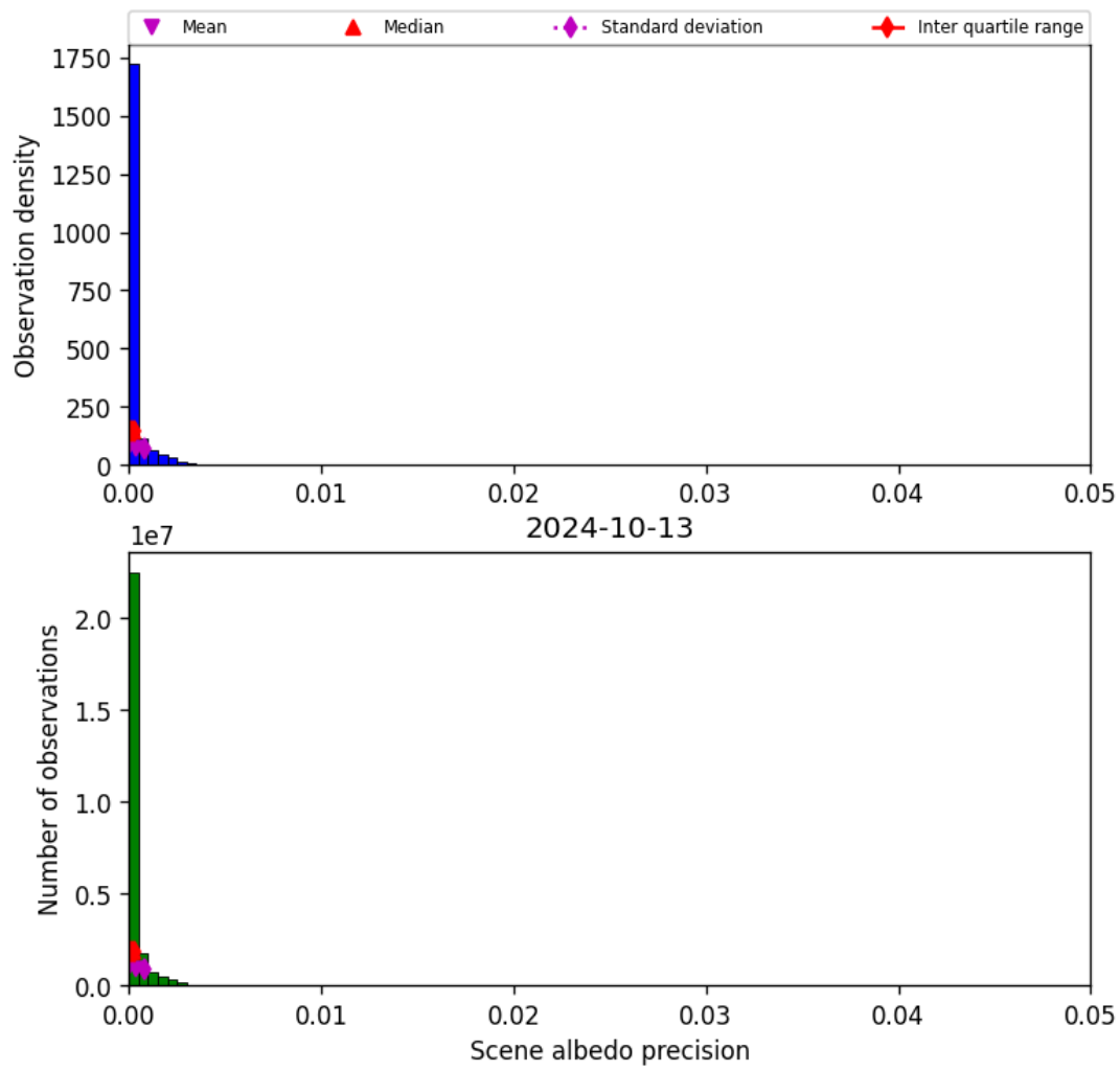
Figure 35: Histogram of “Scene albedo precision” for 2024-10-12 to 2024-10-14
