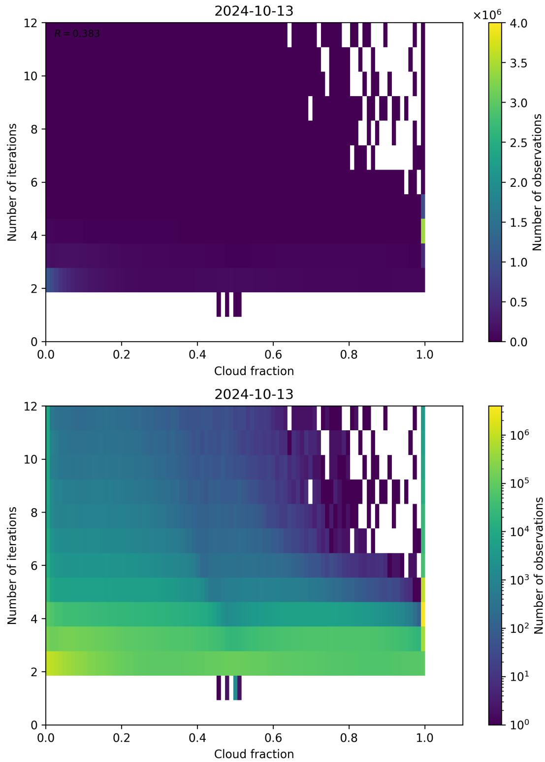
Figure 80: Scatter density plot of “Cloud fraction” against “Number of iterations” for 2024-10-12 to 2024-10-14.
