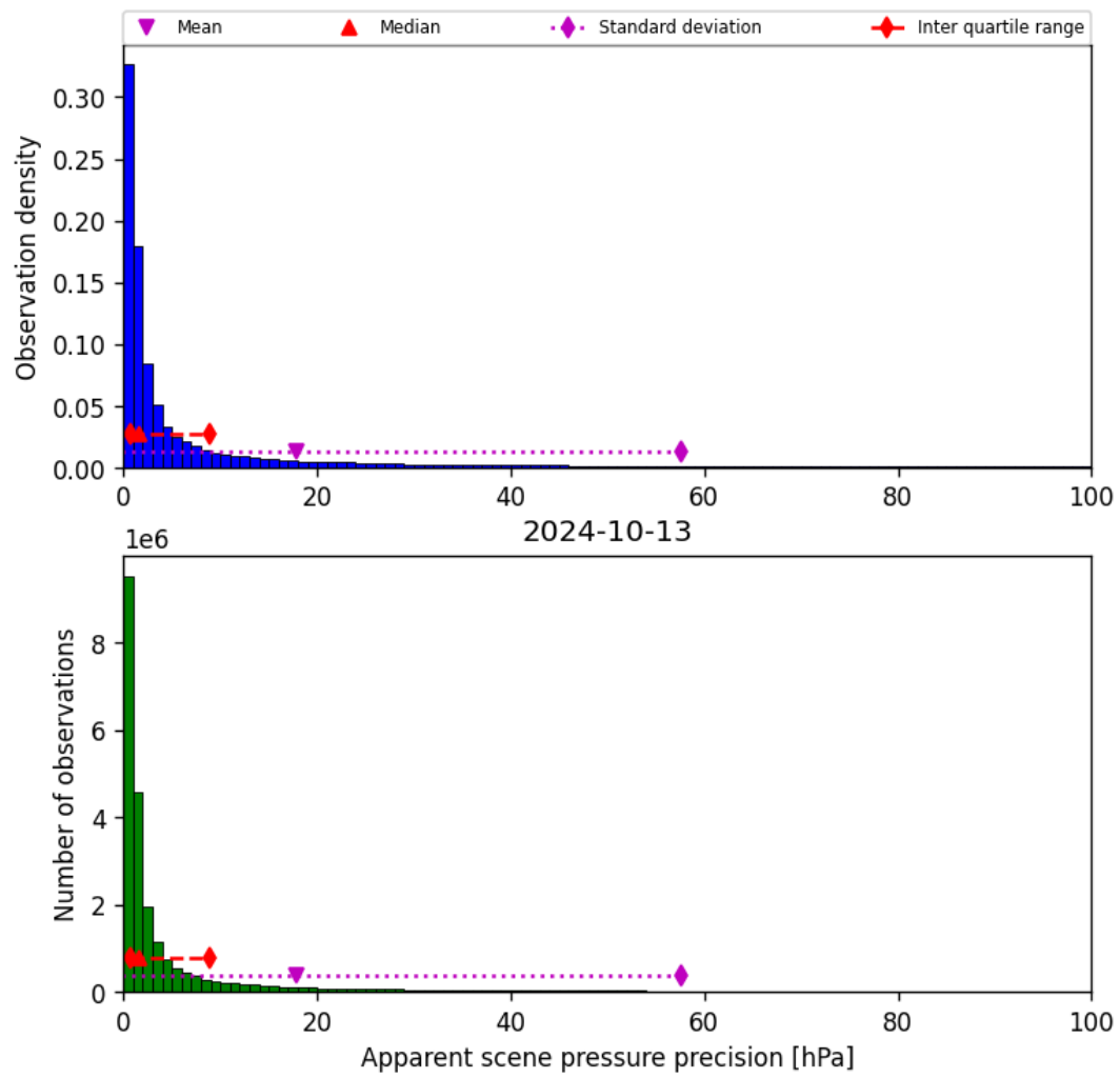
Figure 37: Histogram of “Apparent scene pressure precision” for 2024-10-12 to 2024-10-14
