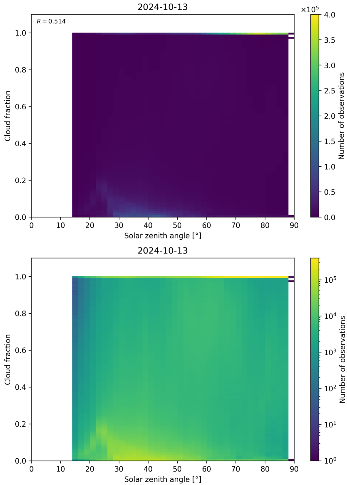
Figure 121: Scatter density plot of “Solar zenith angle” against “Cloud fraction” for 2024-10-12 to 2024-10-14.
