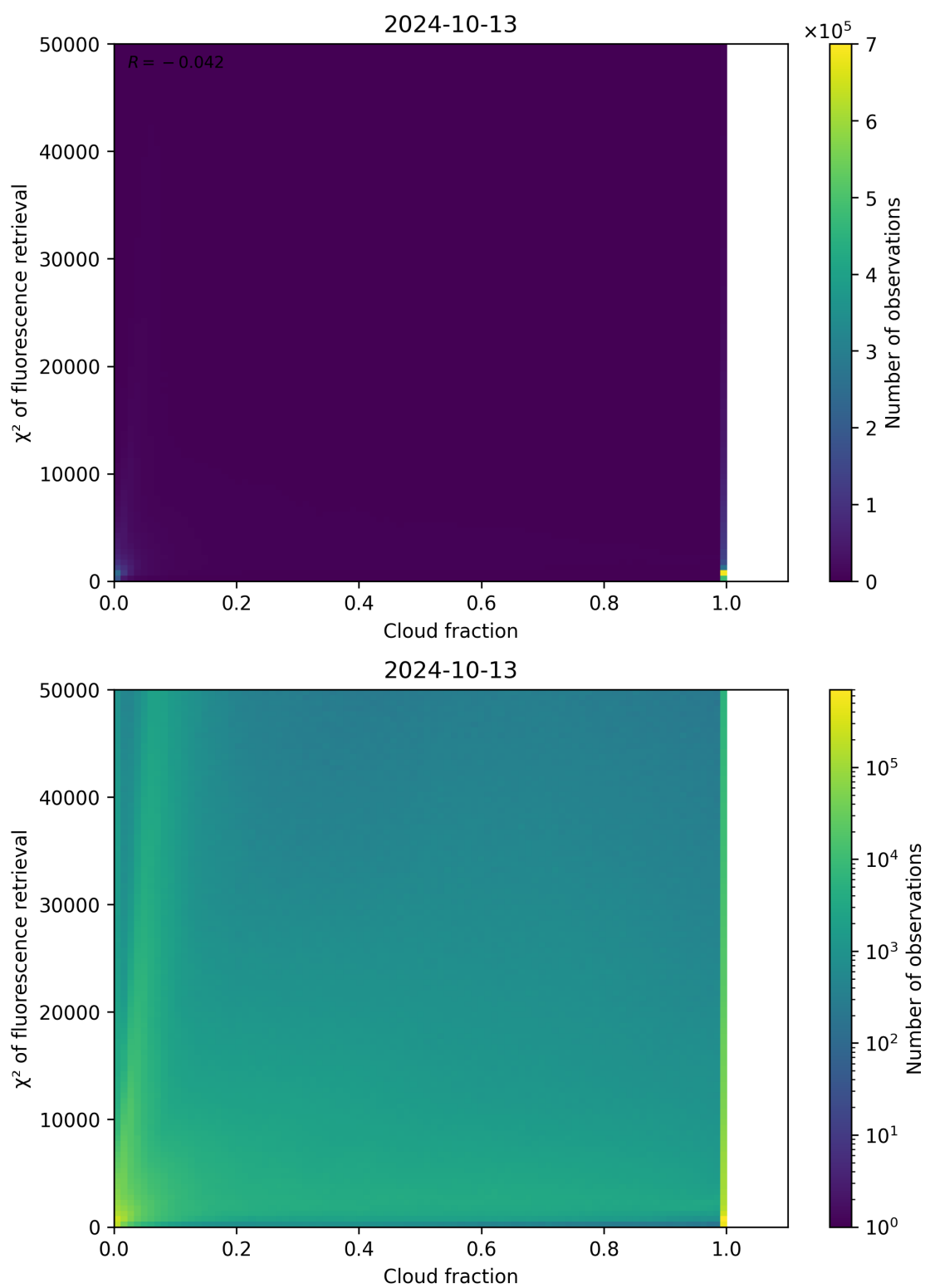
Figure 78: Scatter density plot of “Cloud fraction” against “ \chi^2 of fluorescence retrieval” for 2024-10-12 to 2024-10-14.
