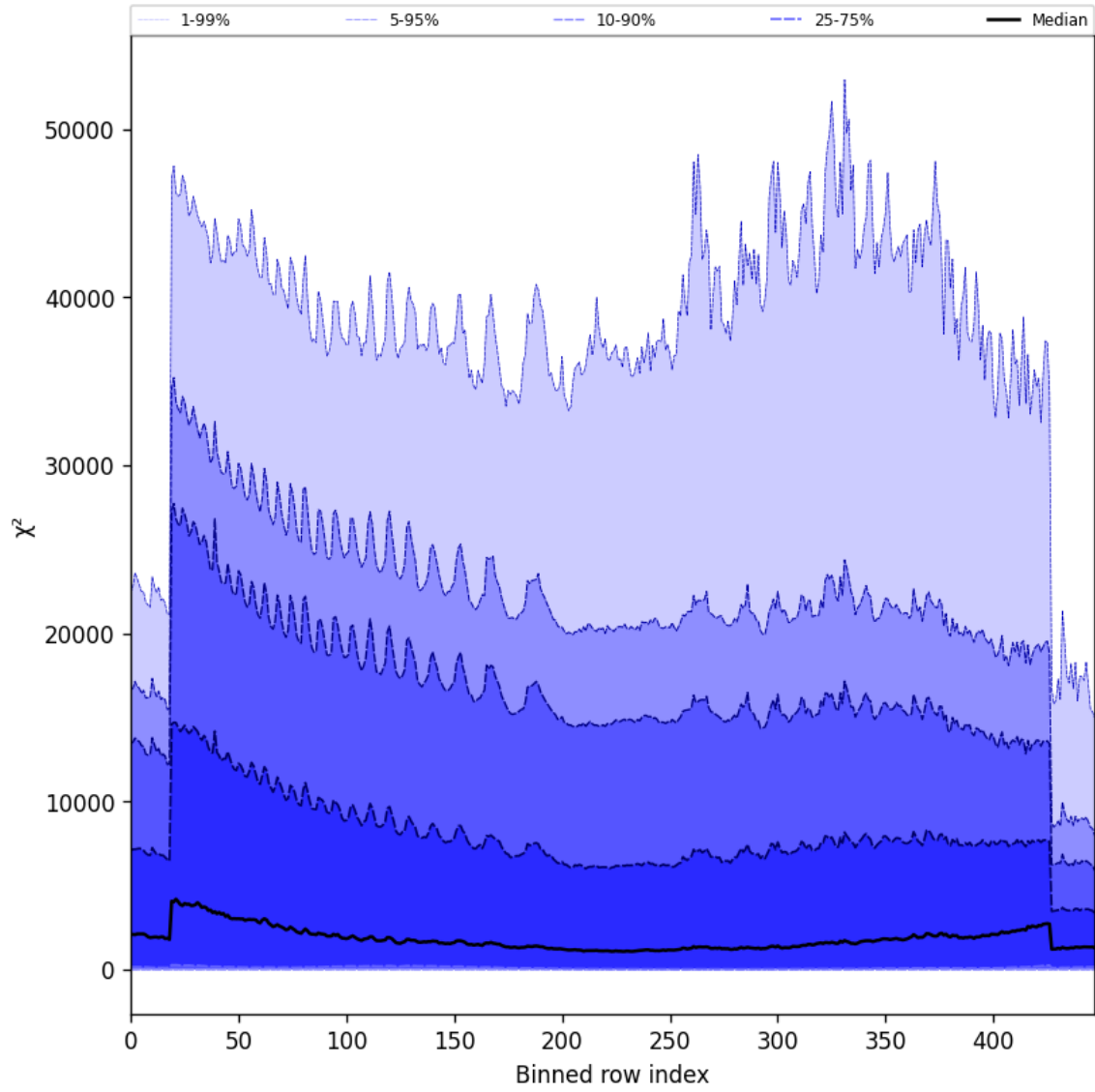
Figure 55: Along track statistics of “ \chi^2 ” for 2024-10-12 to 2024-10-14
