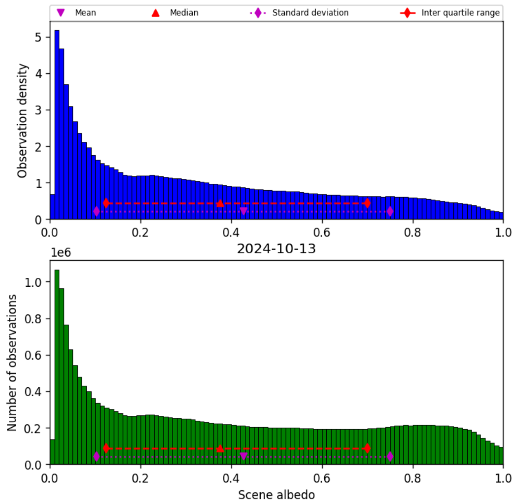
Figure 34: Histogram of “Scene albedo” for 2024-10-12 to 2024-10-14
