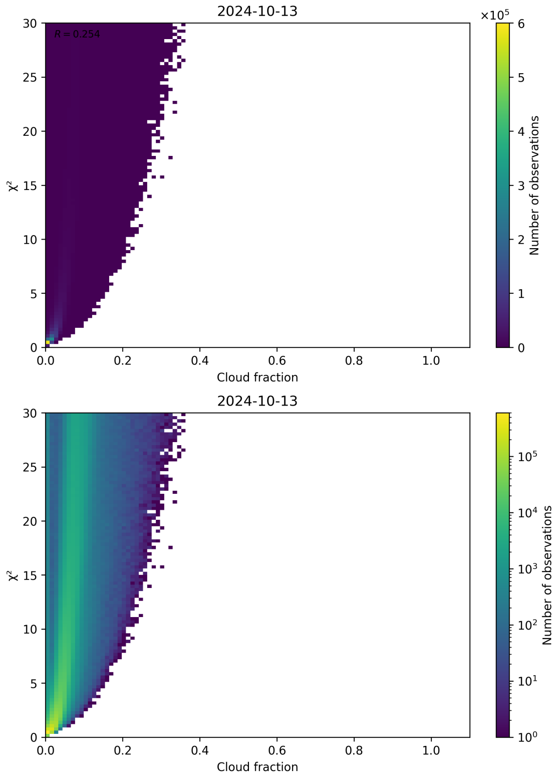
Figure 77: Scatter density plot of “Cloud fraction” against “ \chi^2 ” for 2024-10-12 to 2024-10-14.
