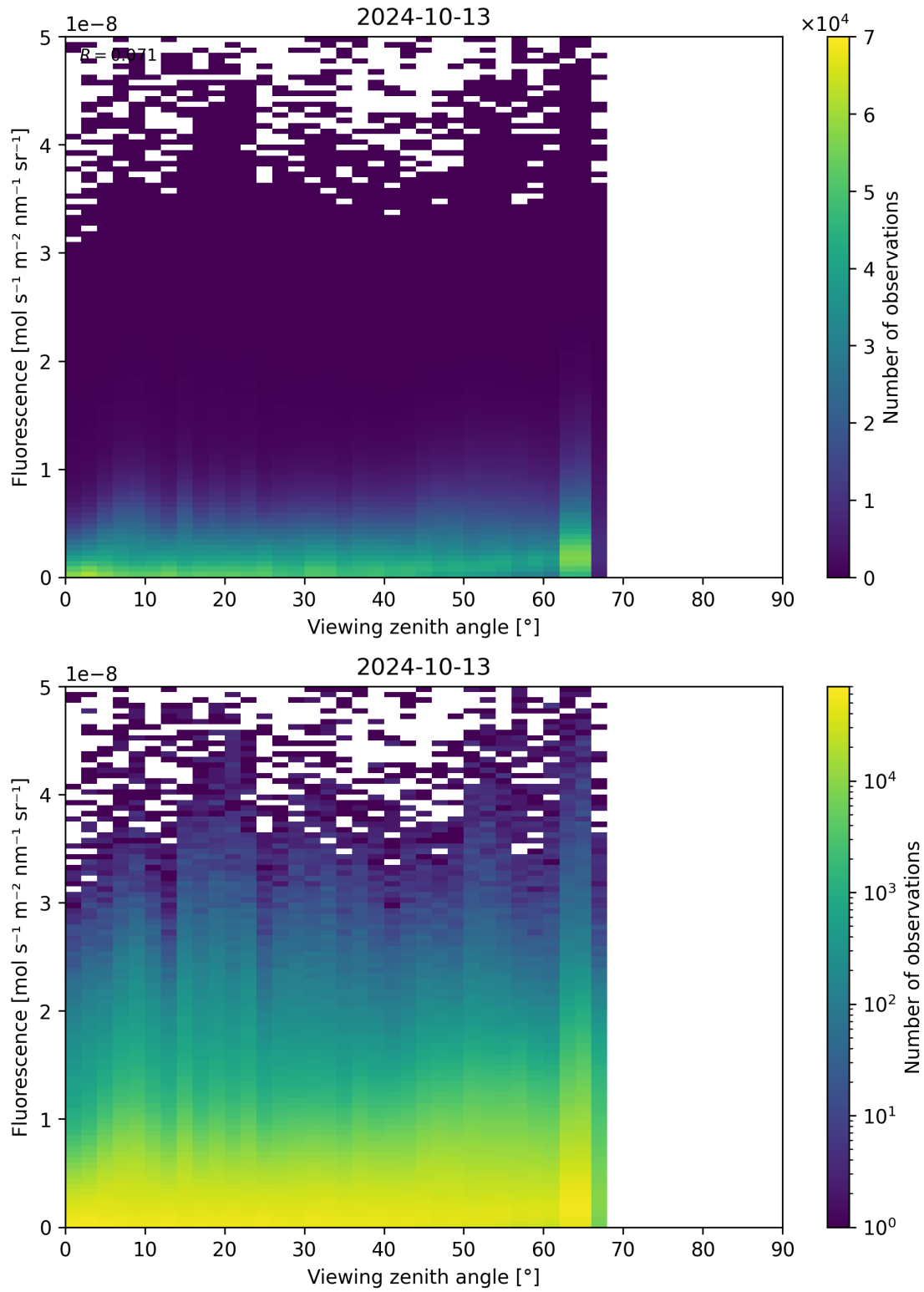
Figure 134: Scatter density plot of “Viewing zenith angle” against “Fluorescence” for 2024-10-12 to 2024-10-14.
