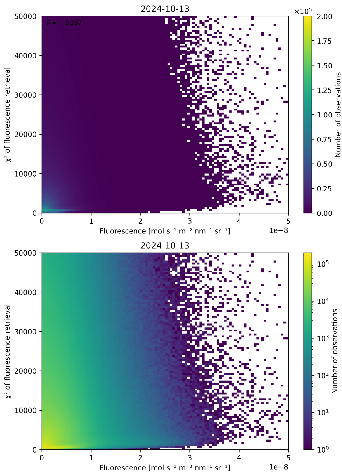
Figure 93: Scatter density plot of “Fluorescence” against “ \chi^2 of fluorescence retrieval” for 2024-10-12 to 2024-10-14.
