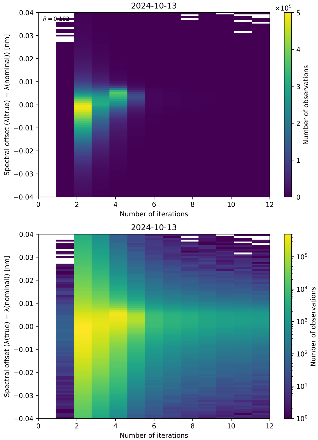
Figure 109: Scatter density plot of “Number of iterations” against “Spectral offset ( \lambda_{\text{true}} - \lambda_{\text{nominal}} )” for 2024-10-12 to 2024-10-14.
