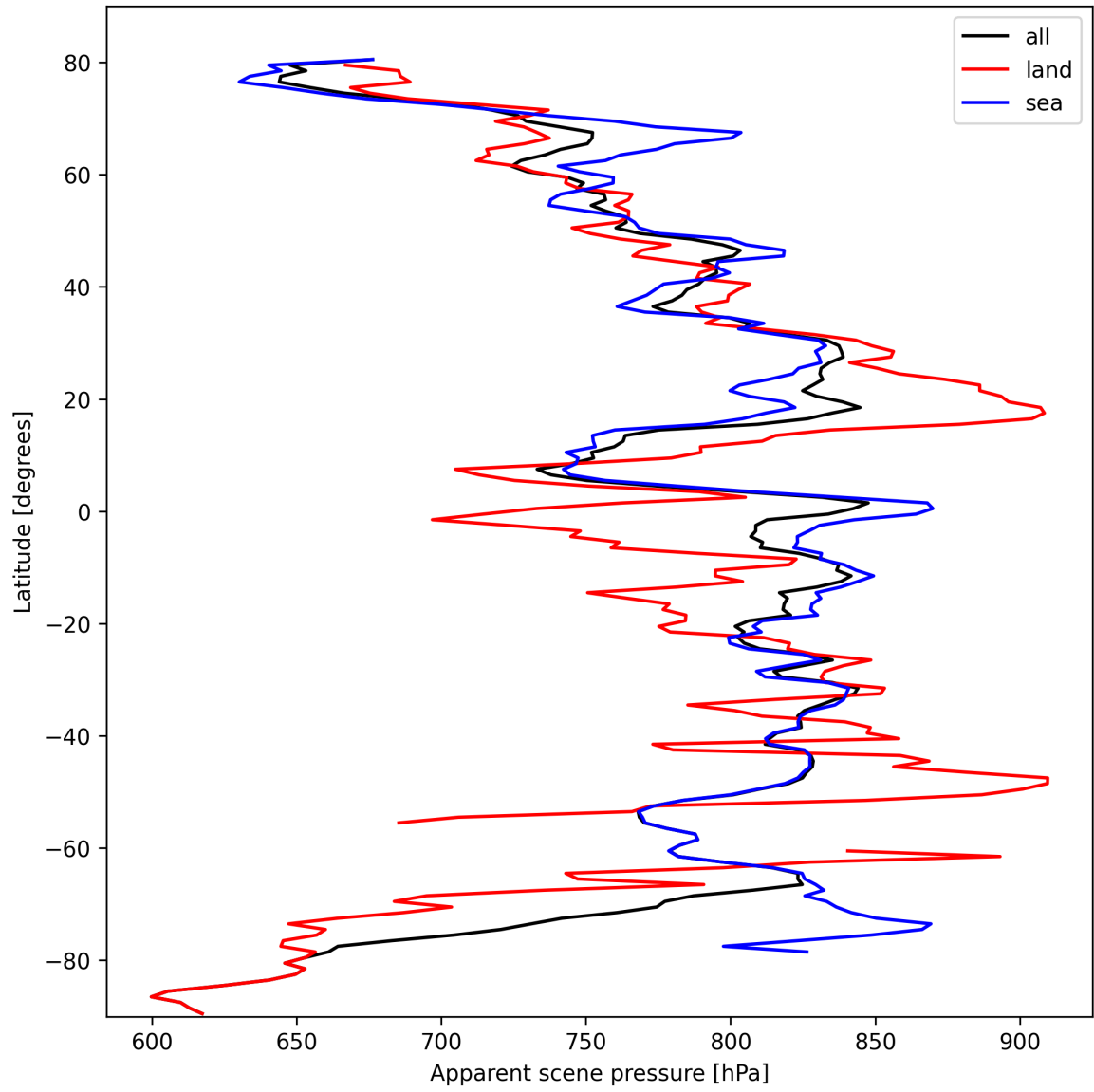
Figure 19: Zonal average of “Apparent scene pressure” for 2024-10-12 to 2024-10-14.
