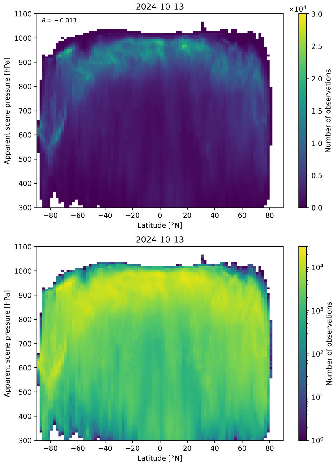
Figure 96: Scatter density plot of “Latitude” against “Apparent scene pressure” for 2024-10-12 to 2024-10-14.
