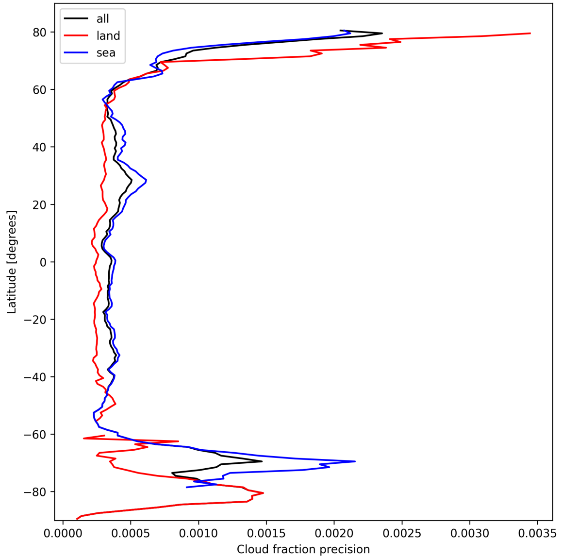
Figure 16: Zonal average of “Cloud fraction precision” for 2024-10-12 to 2024-10-14.
