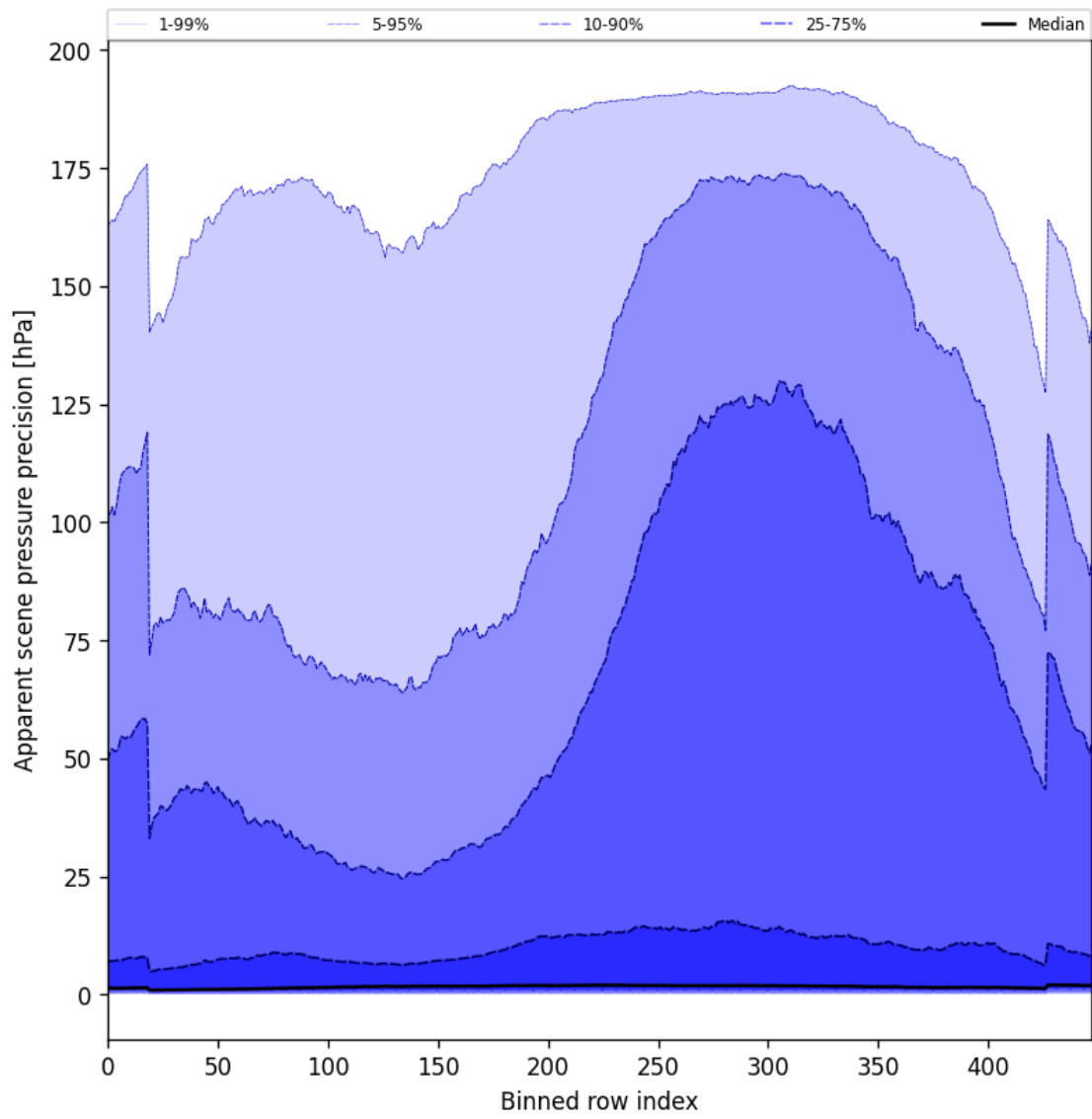
Figure 54: Along track statistics of “Apparent scene pressure precision” for 2024-10-12 to 2024-10-14
