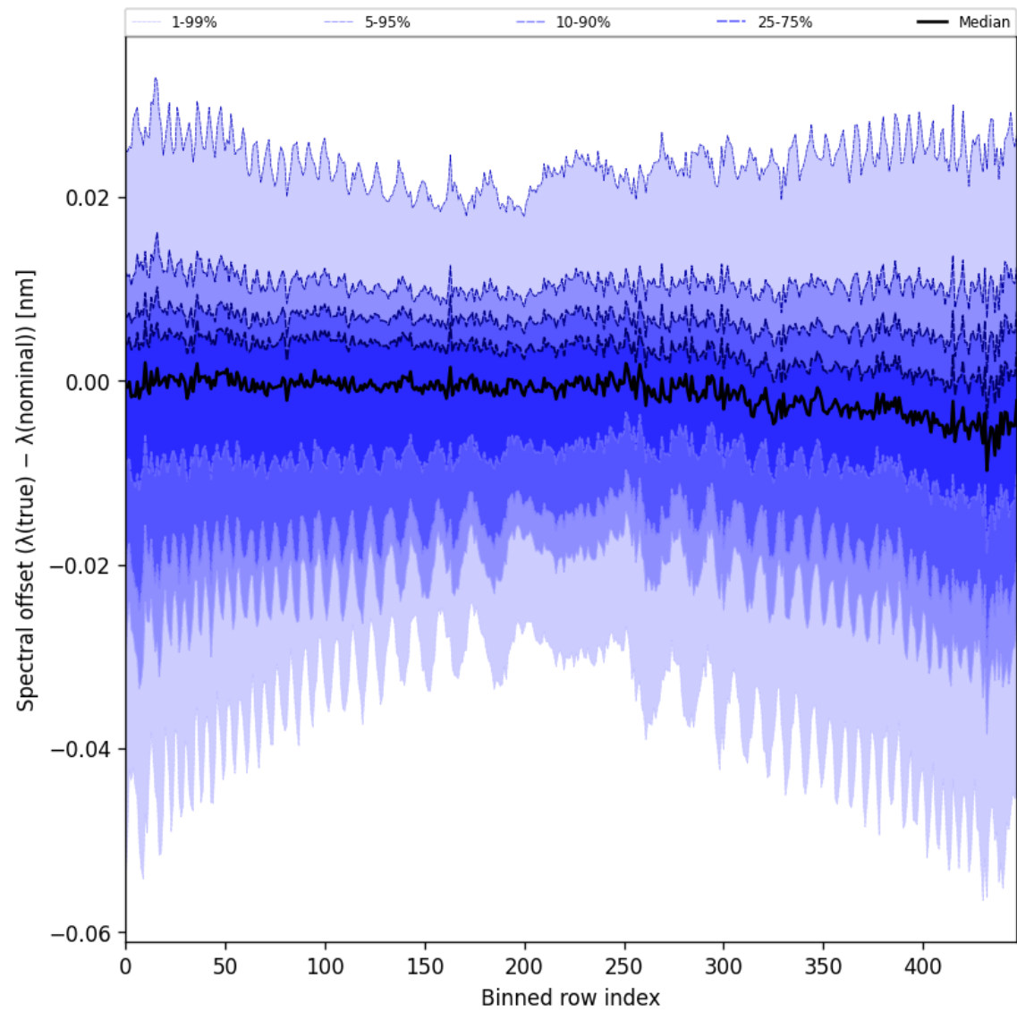
Figure 62: Along track statistics of “Spectral offset ( \lambda_{\text{true}} - \lambda_{\text{nominal}} )” for 2024-10-12 to 2024-10-14
