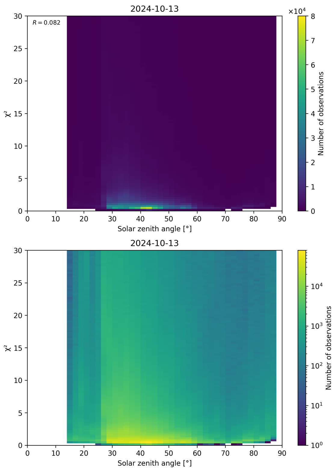
Figure 119: Scatter density plot of “Solar zenith angle” against “ \chi^2 ” for 2024-10-12 to 2024-10-14.
