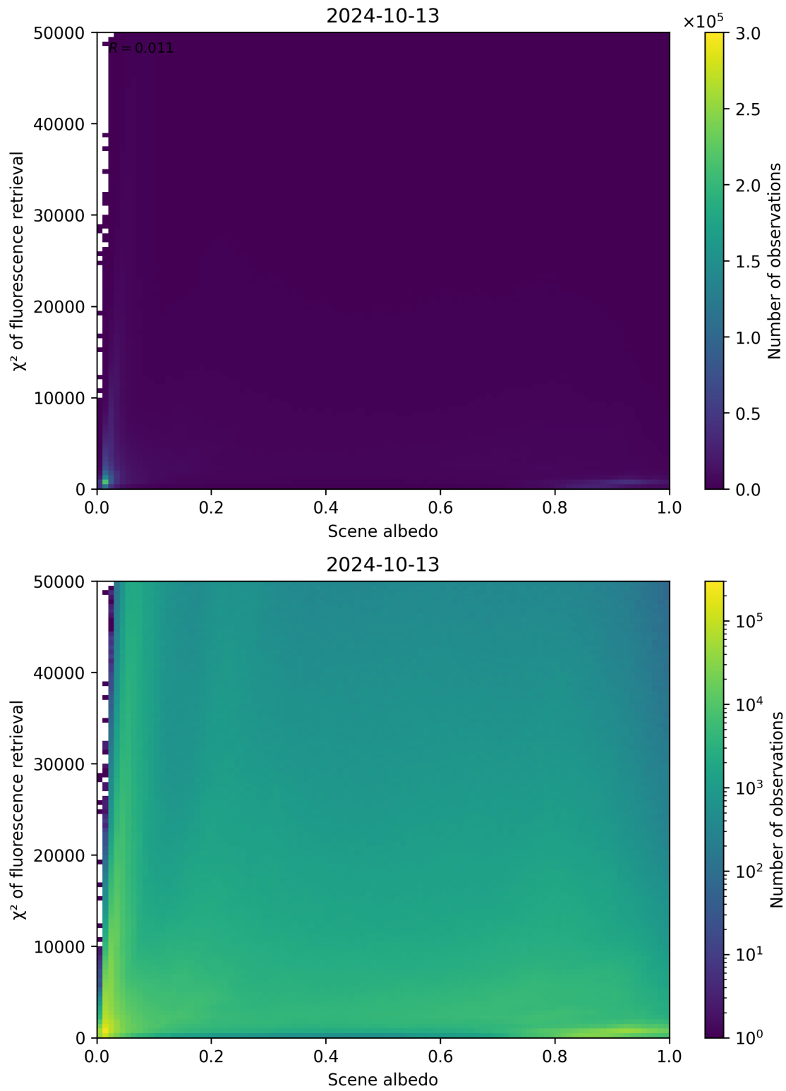
Figure 113: Scatter density plot of “Scene albedo” against “ \chi^2 of fluorescence retrieval” for 2024-10-12 to 2024-10-14.
