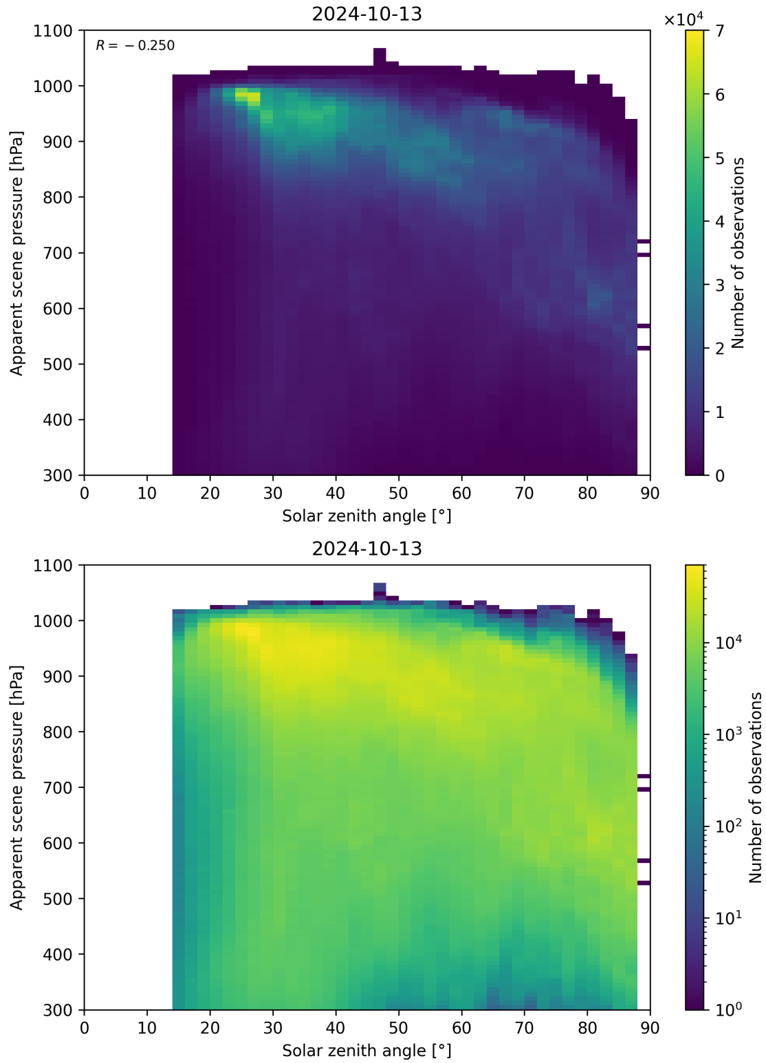
Figure 118: Scatter density plot of “Solar zenith angle” against “Apparent scene pressure” for 2024-10-12 to 2024-10-14.
