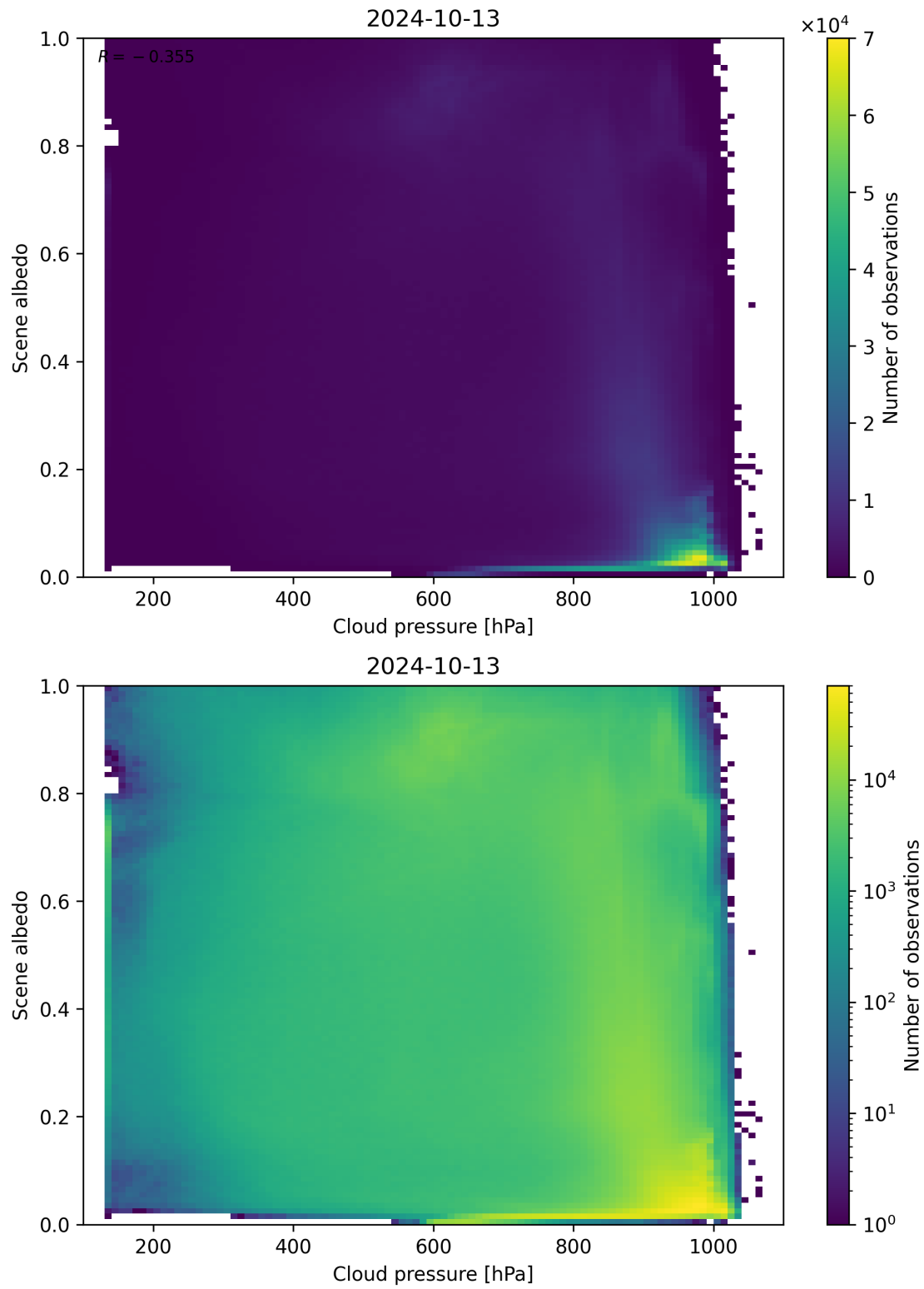
Figure 91: Scatter density plot of “Cloud pressure” against “Scene albedo” for 2024-10-12 to 2024-10-14.
