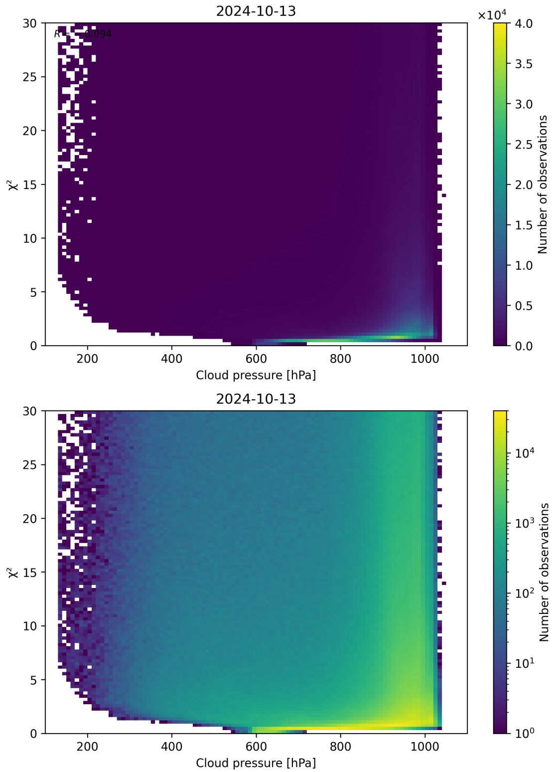
Figure 85: Scatter density plot of “Cloud pressure” against “ \chi^2 ” for 2024-10-12 to 2024-10-14.
