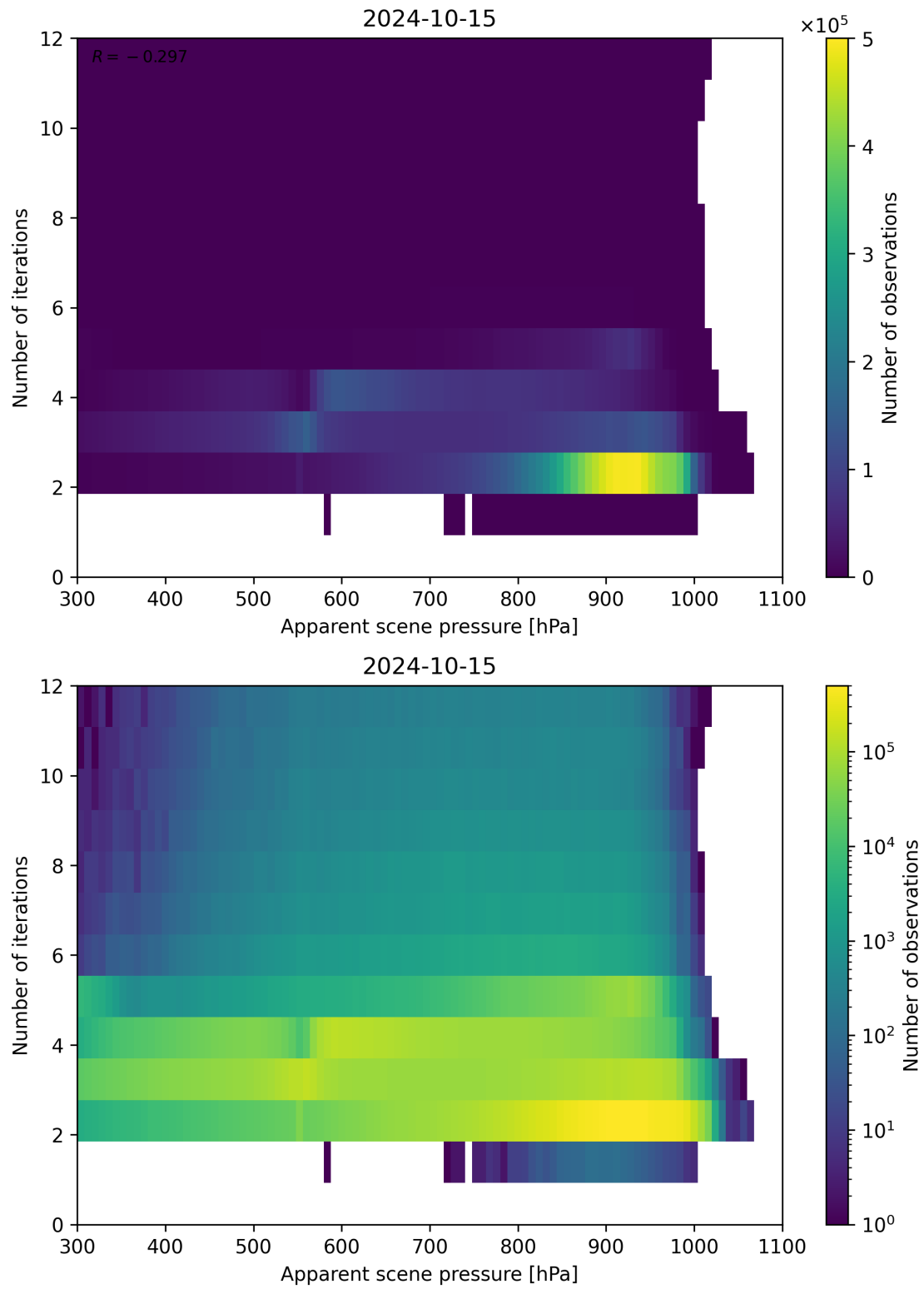
Figure 66: Scatter density plot of “Apparent scene pressure” against “Number of iterations” for 2024-10-14 to 2024-10-16.
