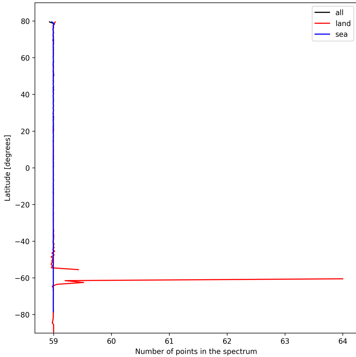
Figure 27: Zonal average of “Number of points in the spectrum” for 2024-10-14 to 2024-10-16.
