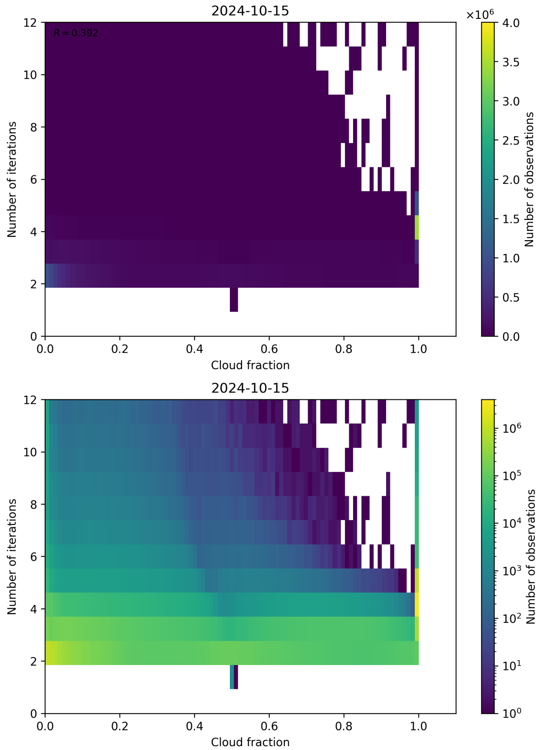
Figure 80: Scatter density plot of “Cloud fraction” against “Number of iterations” for 2024-10-14 to 2024-10-16.
