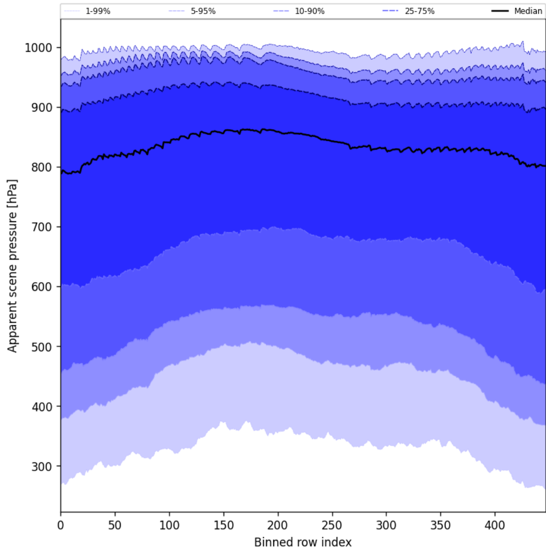
Figure 53: Along track statistics of “Apparent scene pressure” for 2024-10-14 to 2024-10-16
