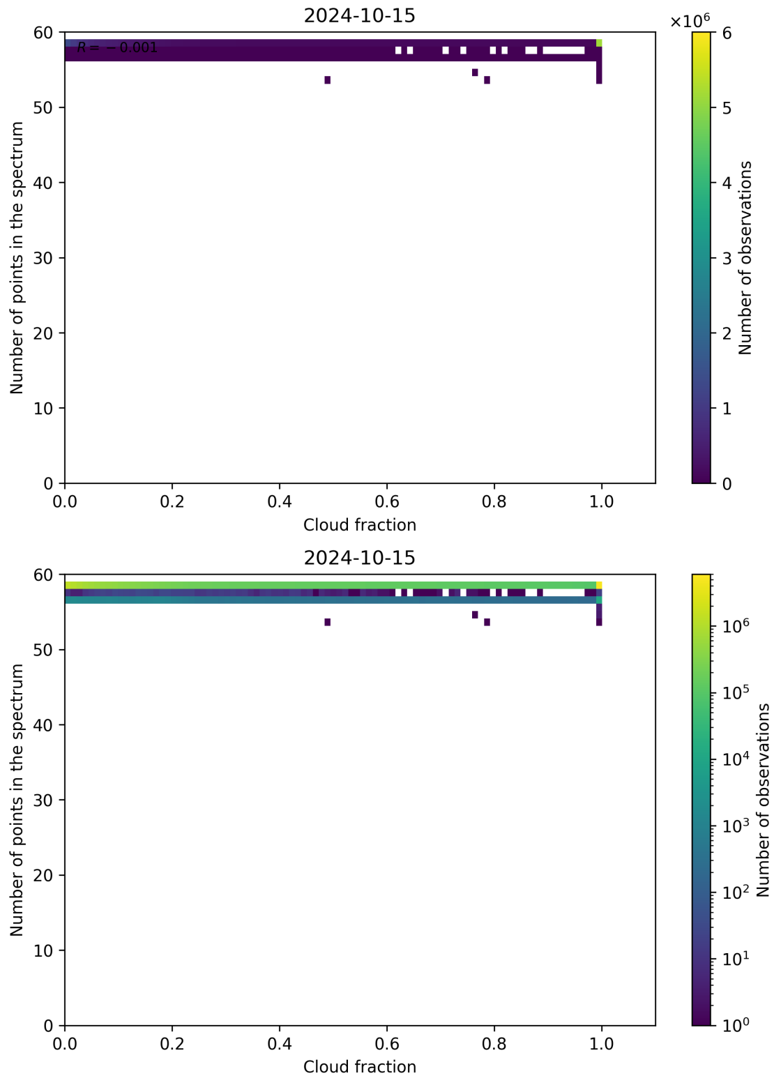
Figure 81: Scatter density plot of “Cloud fraction” against “Number of points in the spectrum” for 2024-10-14 to 2024-10-16.
