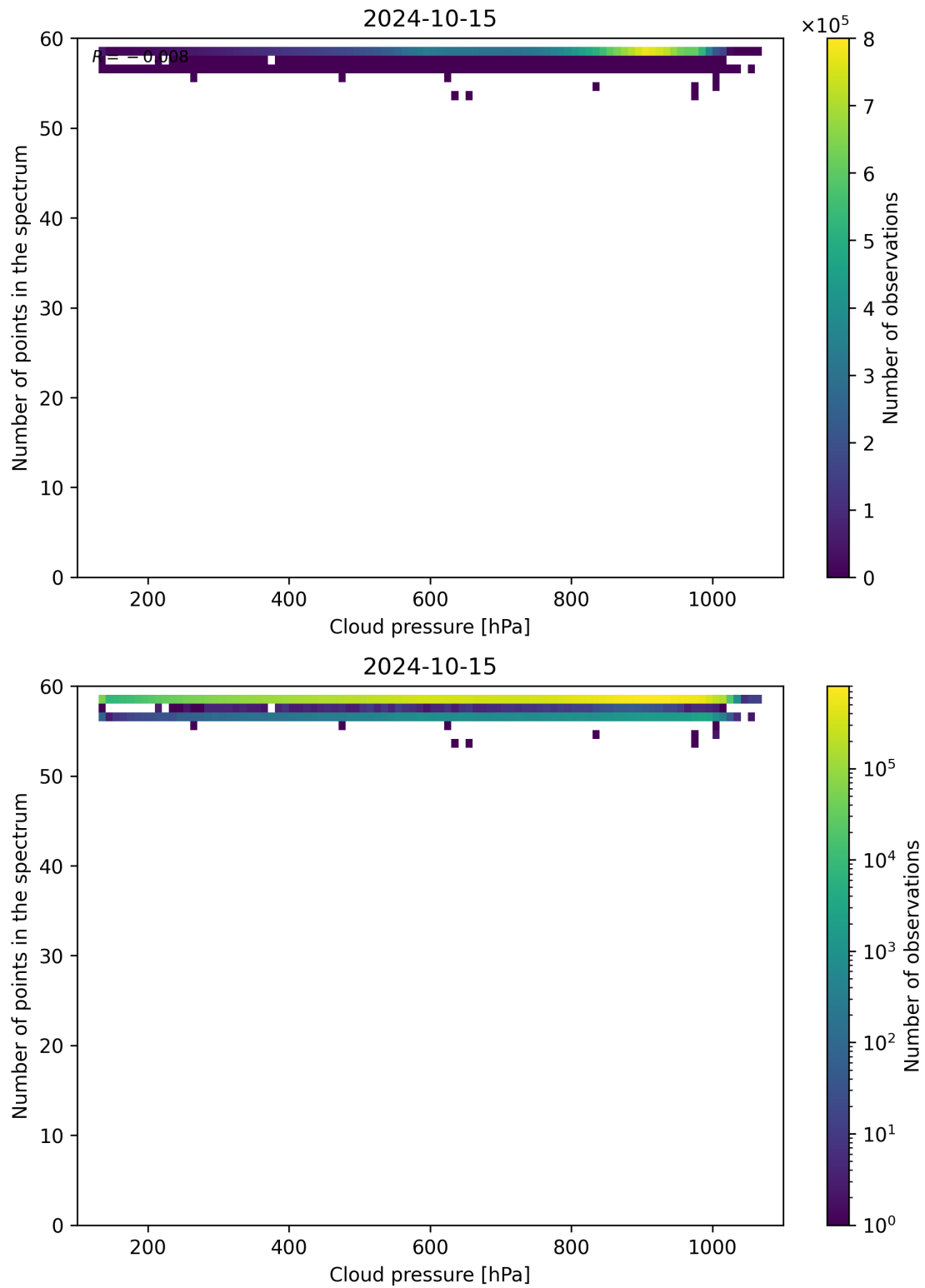
Figure 90: Scatter density plot of “Cloud pressure” against “Number of points in the spectrum” for 2024-10-14 to 2024-10-16.
