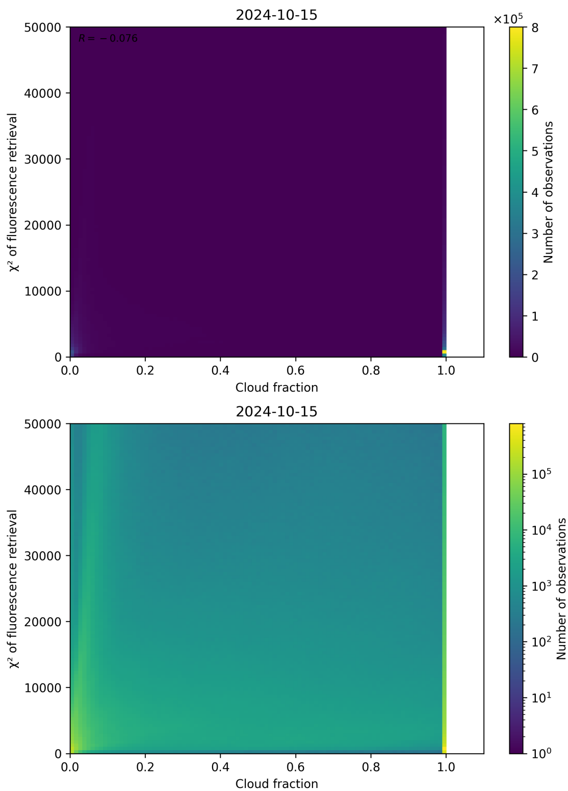
Figure 78: Scatter density plot of “Cloud fraction” against “ \chi^2 of fluorescence retrieval” for 2024-10-14 to 2024-10-16.
