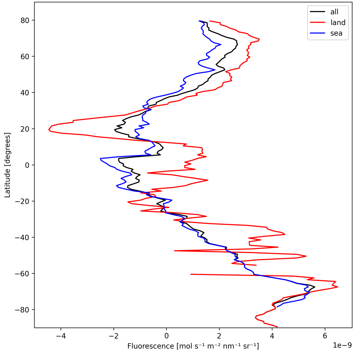
Figure 23: Zonal average of “Fluorescence” for 2024-10-14 to 2024-10-16.
