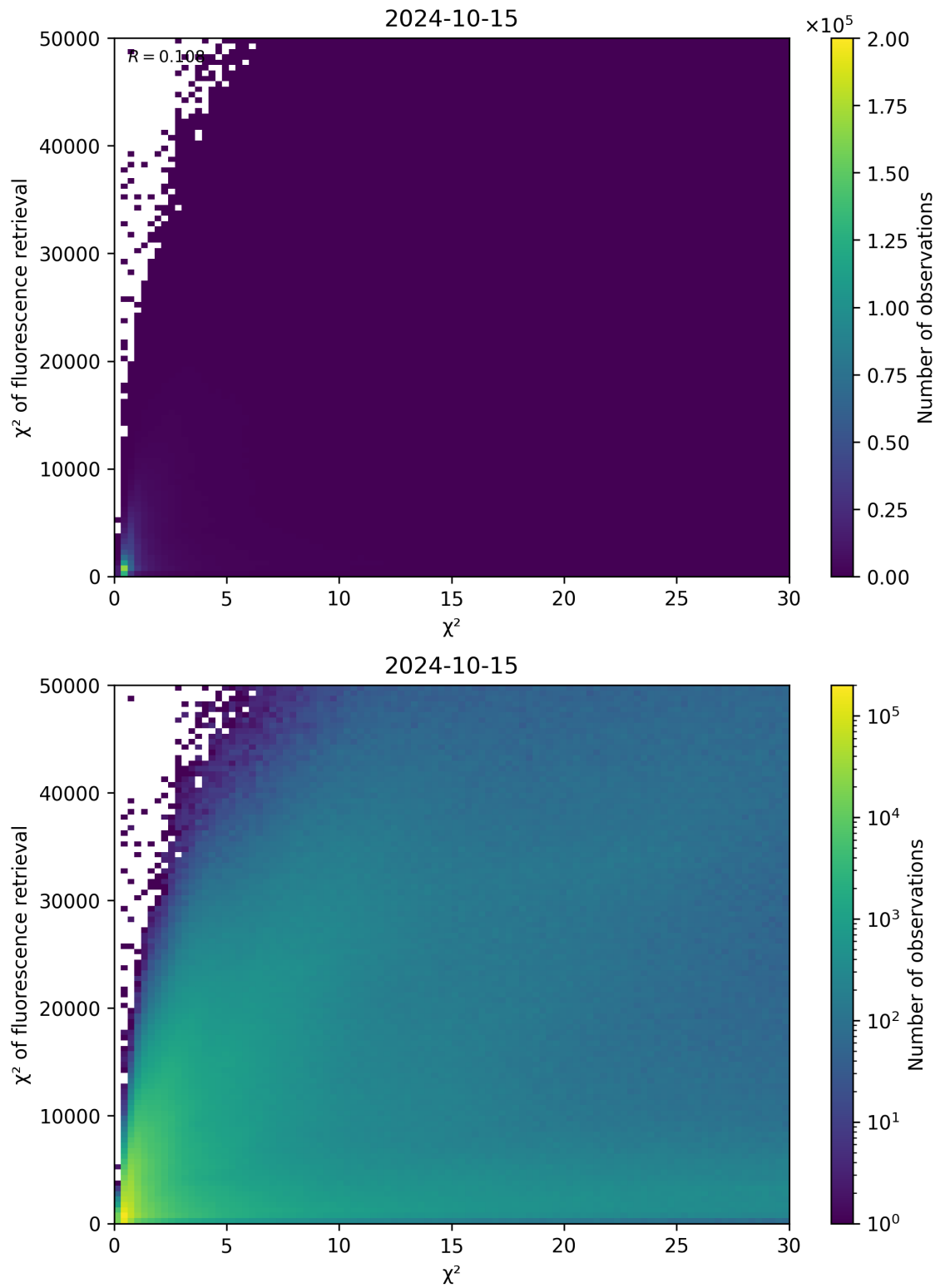
Figure 69: Scatter density plot of “ \chi^2 ” against “ \chi^2 of fluorescence retrieval” for 2024-10-14 to 2024-10-16.
