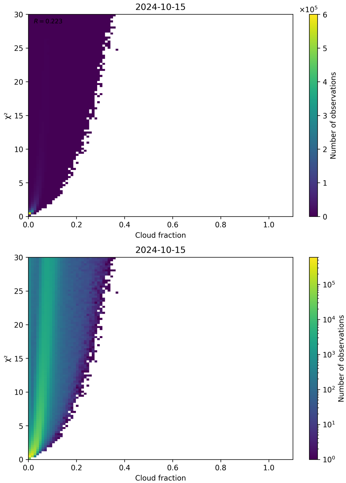
Figure 77: Scatter density plot of “Cloud fraction” against “ \chi^2 ” for 2024-10-14 to 2024-10-16.
