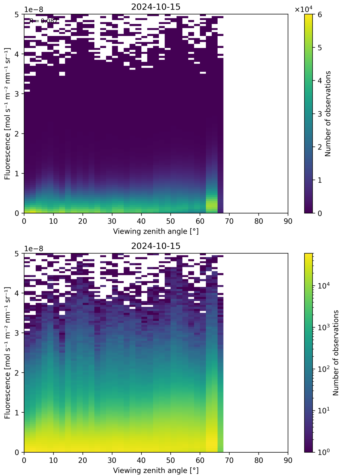
Figure 134: Scatter density plot of “Viewing zenith angle” against “Fluorescence” for 2024-10-14 to 2024-10-16.
