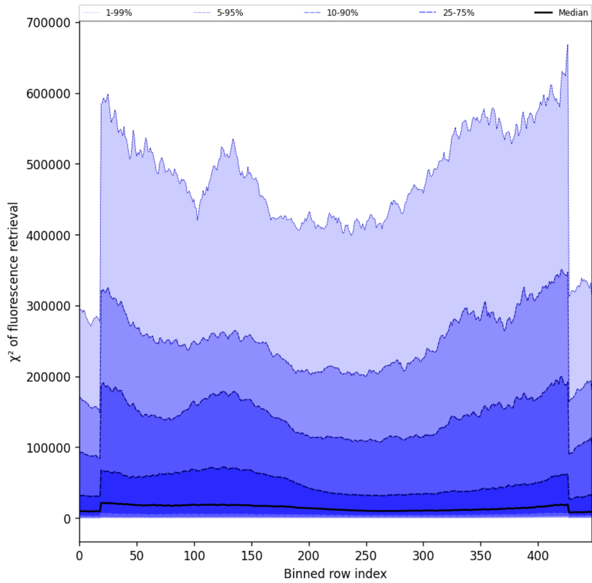
Figure 59: Along track statistics of “ \chi^2 of fluorescence retrieval” for 2024-10-14 to 2024-10-16
