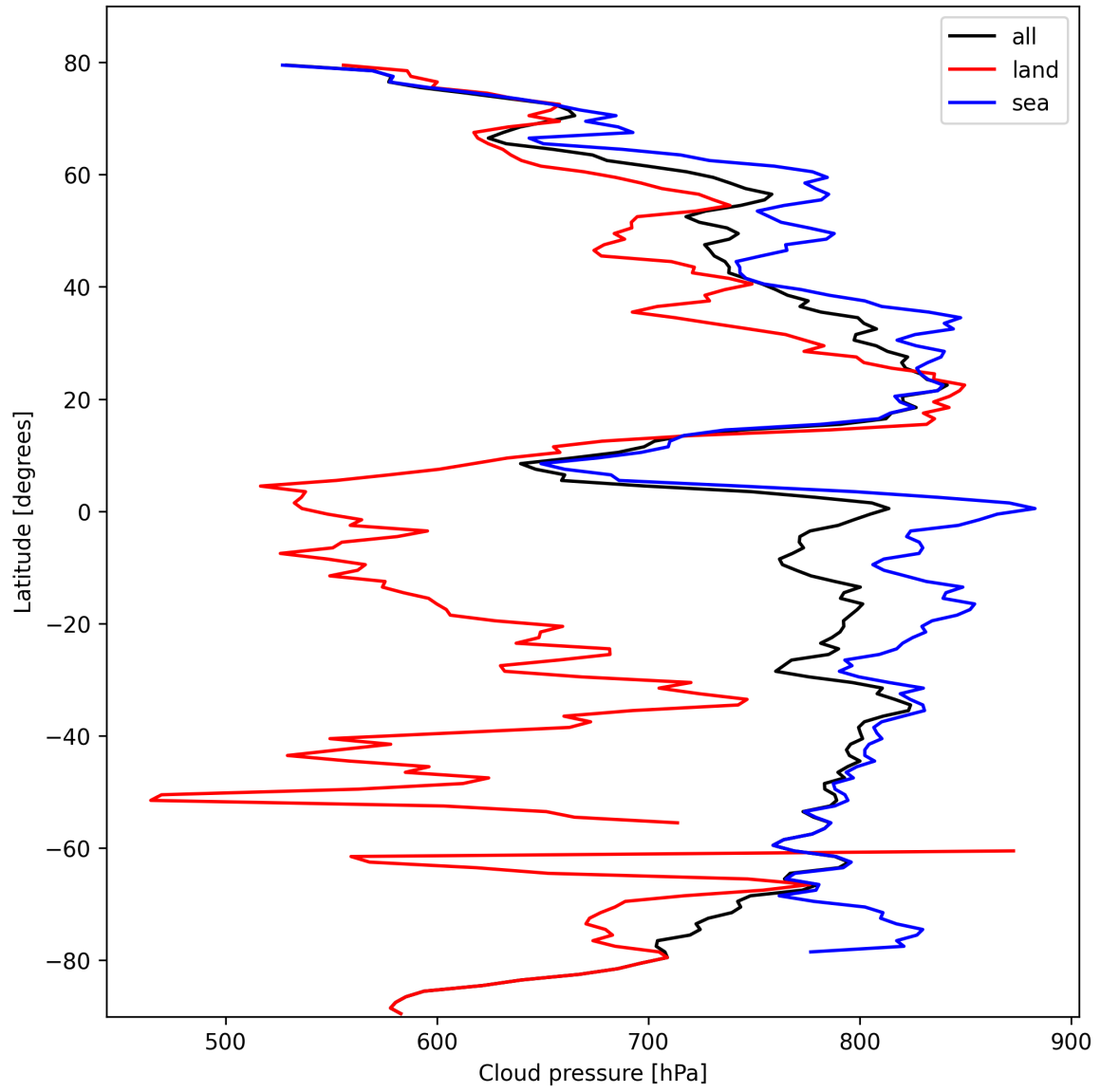
Figure 13: Zonal average of “Cloud pressure” for 2024-10-14 to 2024-10-16.
