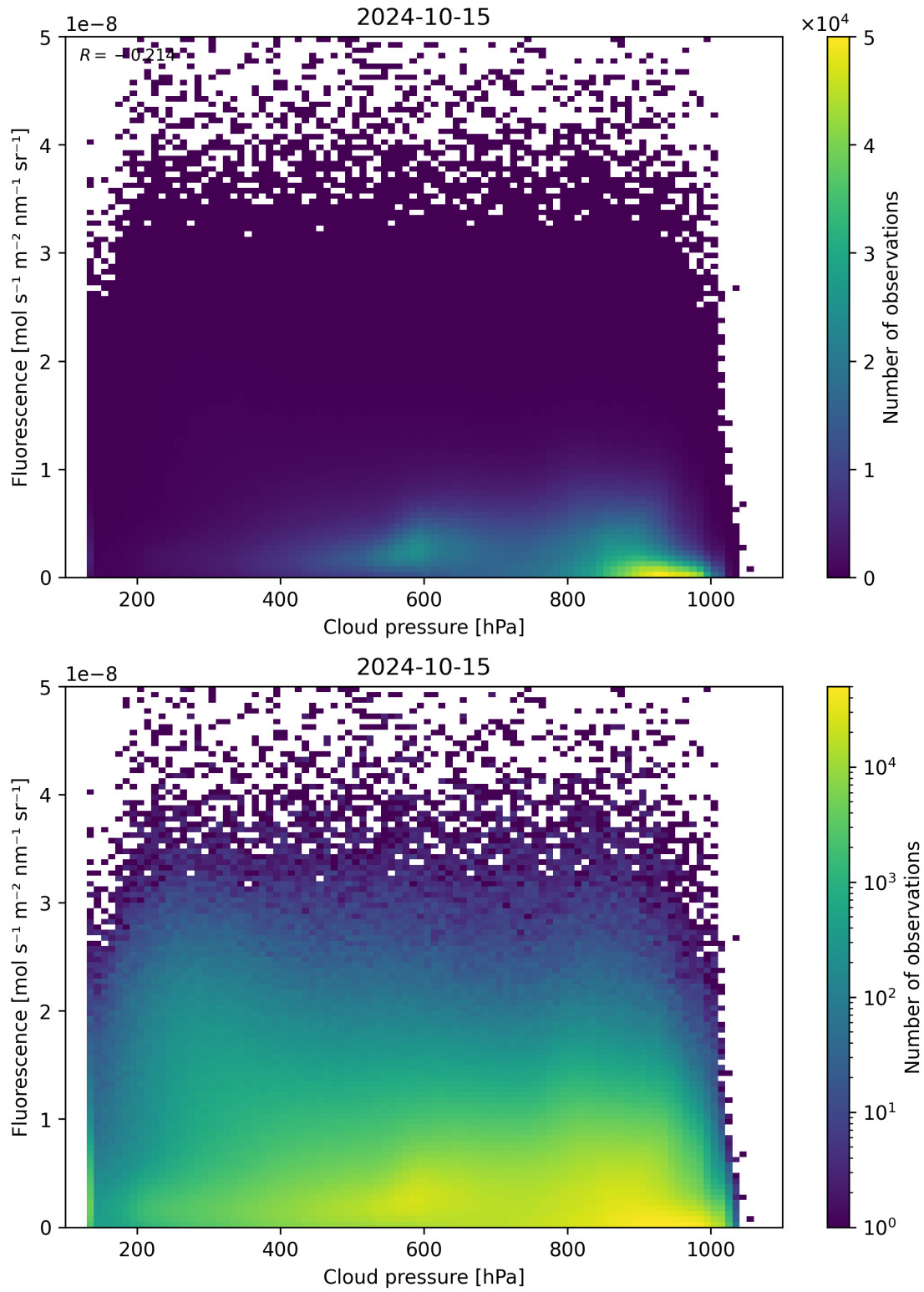
Figure 88: Scatter density plot of “Cloud pressure” against “Fluorescence” for 2024-10-14 to 2024-10-16.
