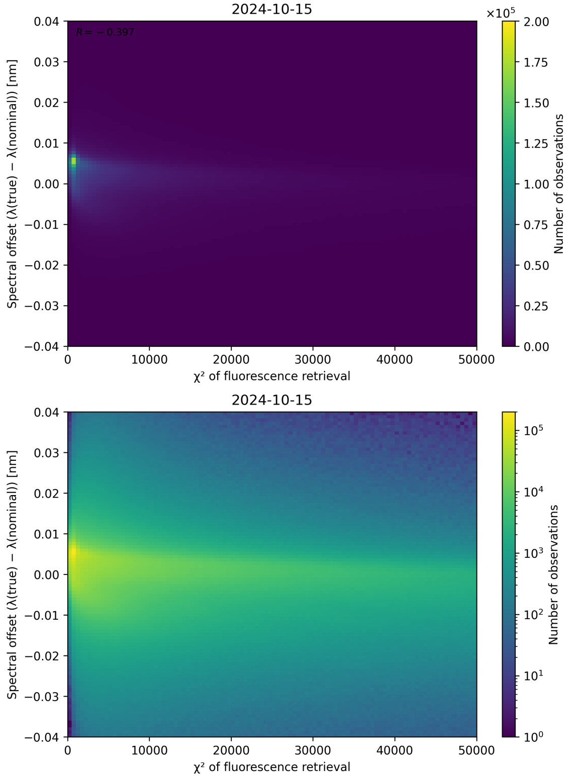
Figure 72: Scatter density plot of “ \chi^2 of fluorescence retrieval” against “Spectral offset ( \lambda_{\text{true}} - \lambda_{\text{nominal}} )” for 2024-10-14 to 2024-10-16.
