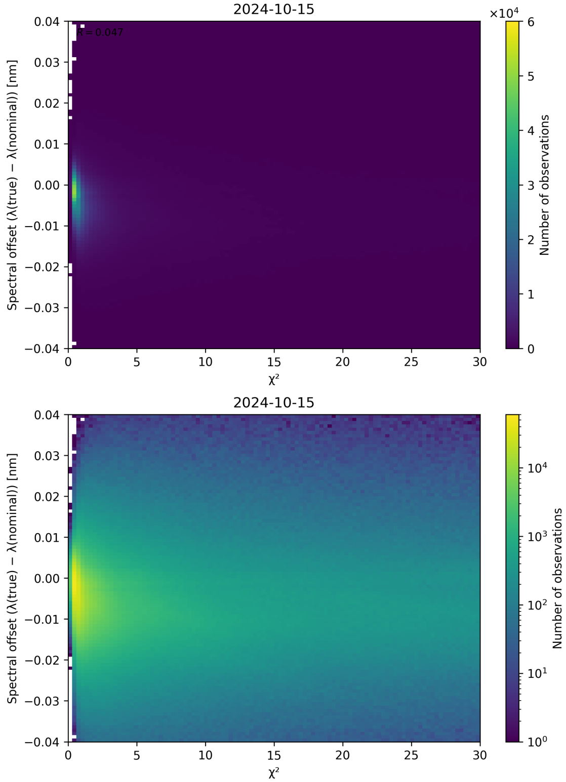
Figure 75: Scatter density plot of “ \chi^2 ” against “Spectral offset ( \lambda_{\text{true}} - \lambda_{\text{nominal}} )” for 2024-10-14 to 2024-10-16.
