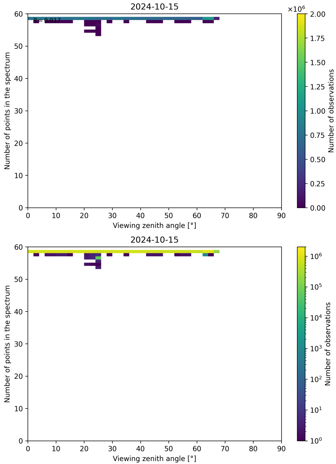
Figure 137: Scatter density plot of “Viewing zenith angle” against “Number of points in the spectrum” for 2024-10-14 to 2024-10-16.
