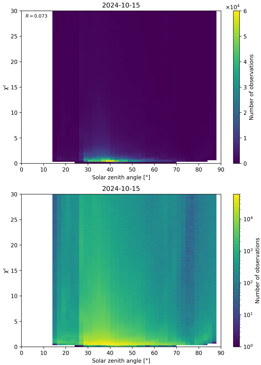
Figure 119: Scatter density plot of “Solar zenith angle” against “ \chi^2 ” for 2024-10-14 to 2024-10-16.
