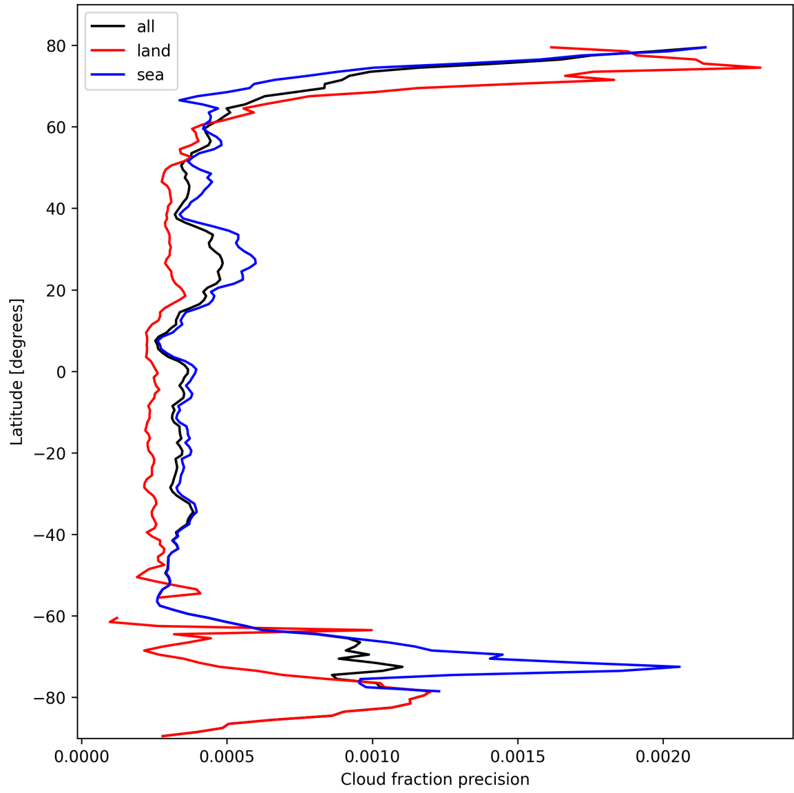
Figure 16: Zonal average of “Cloud fraction precision” for 2024-10-14 to 2024-10-16.
