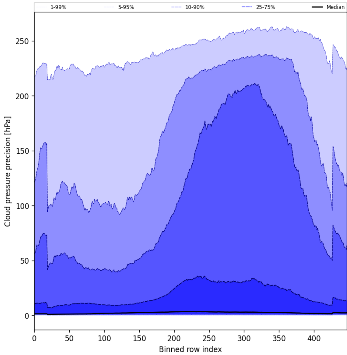
Figure 48: Along track statistics of “Cloud pressure precision” for 2024-10-14 to 2024-10-16
