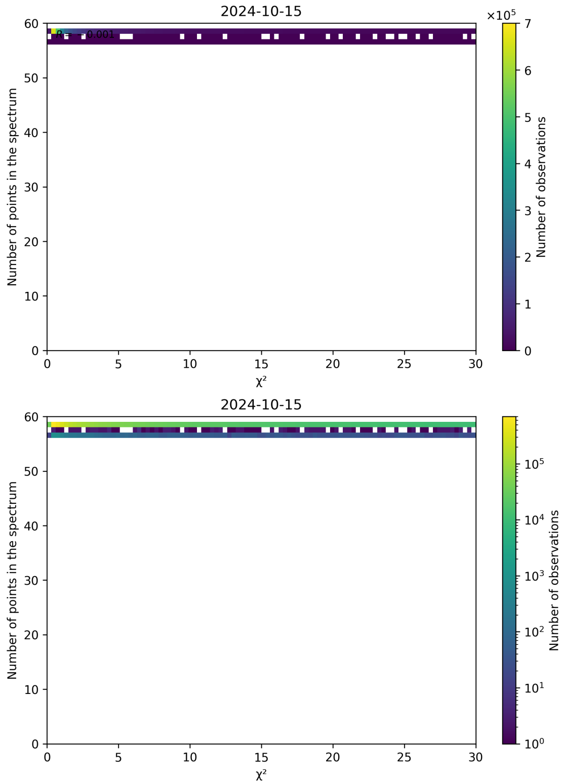
Figure 74: Scatter density plot of " \chi^2 " against "Number of points in the spectrum" for 2024-10-14 to 2024-10-16.
