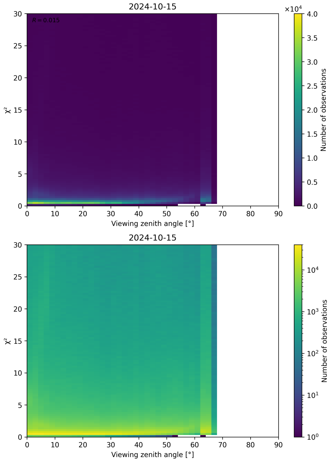
Figure 130: Scatter density plot of “Viewing zenith angle” against “ \chi^2 ” for 2024-10-14 to 2024-10-16.
