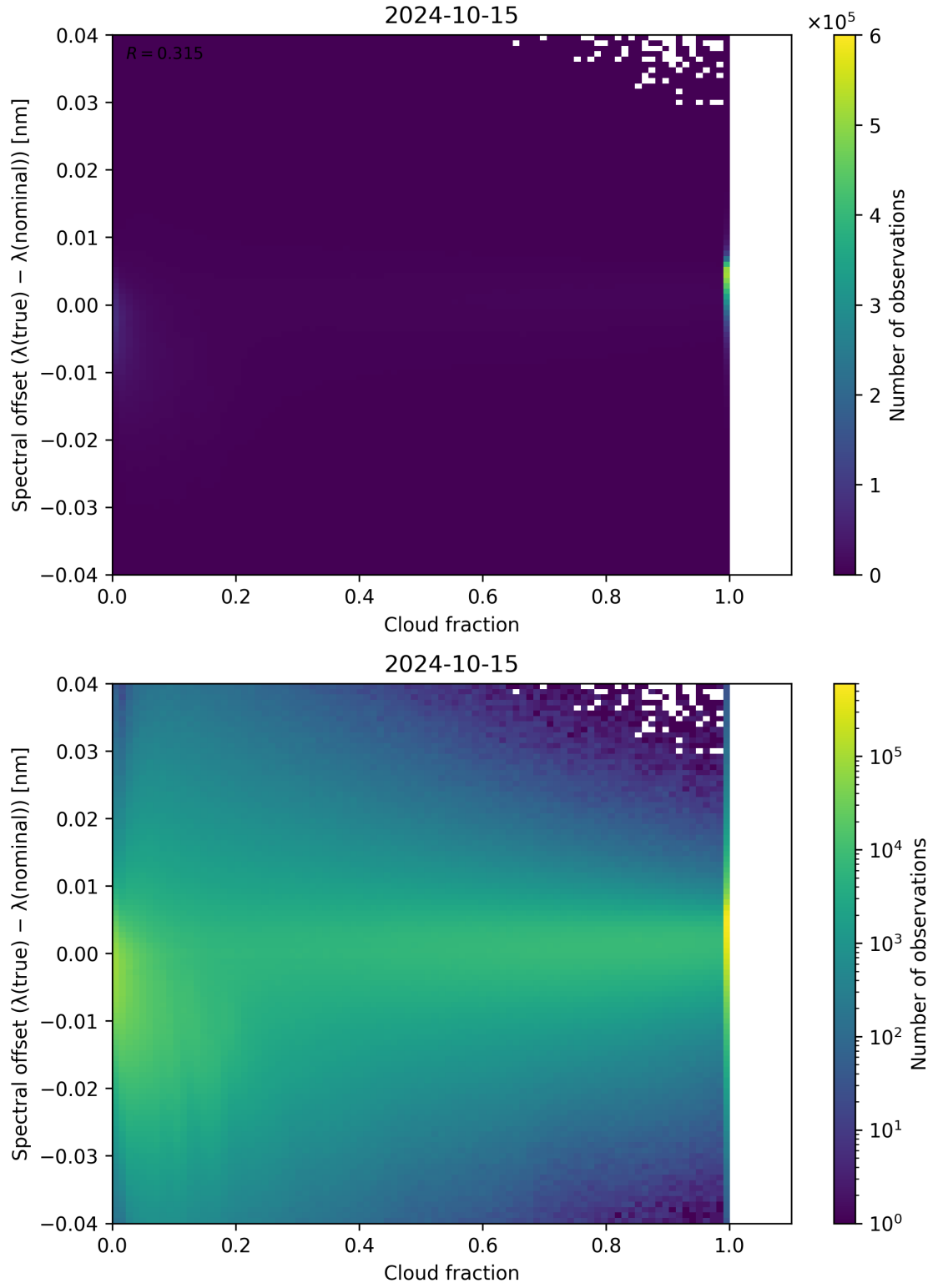
Figure 83: Scatter density plot of “Cloud fraction” against “Spectral offset ( \lambda_{\text{true}} - \lambda_{\text{nominal}} )” for 2024-10-14 to 2024-10-16.
