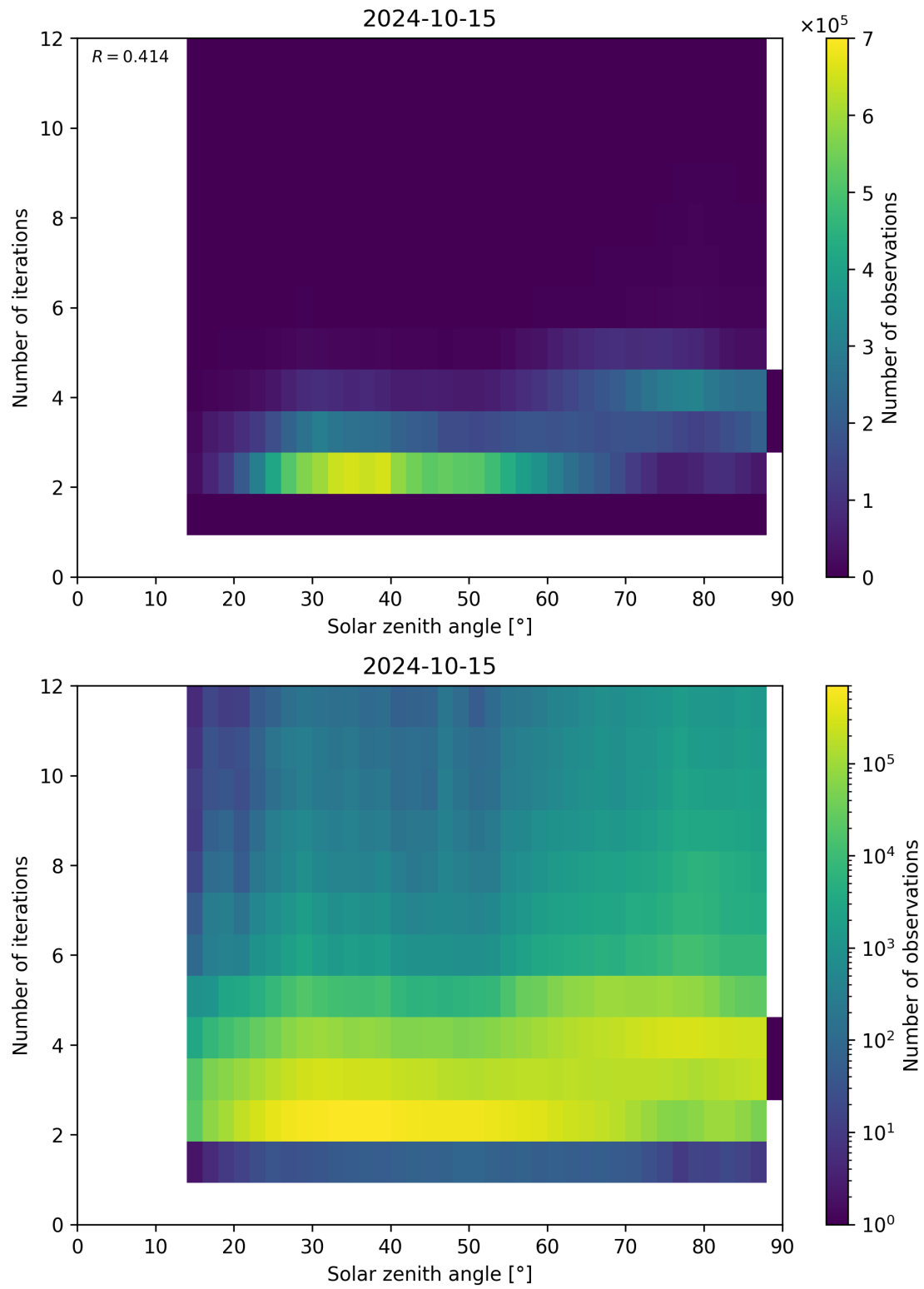
Figure 125: Scatter density plot of “Solar zenith angle” against “Number of iterations” for 2024-10-14 to 2024-10-16.
