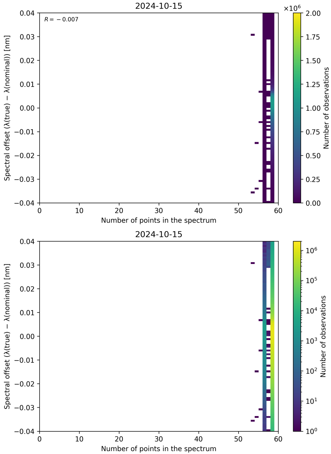
Figure 110: Scatter density plot of “Number of points in the spectrum” against “Spectral offset ( \lambda_{\text{true}} - \lambda_{\text{nominal}} )” for 2024-10-14 to 2024-10-16.
