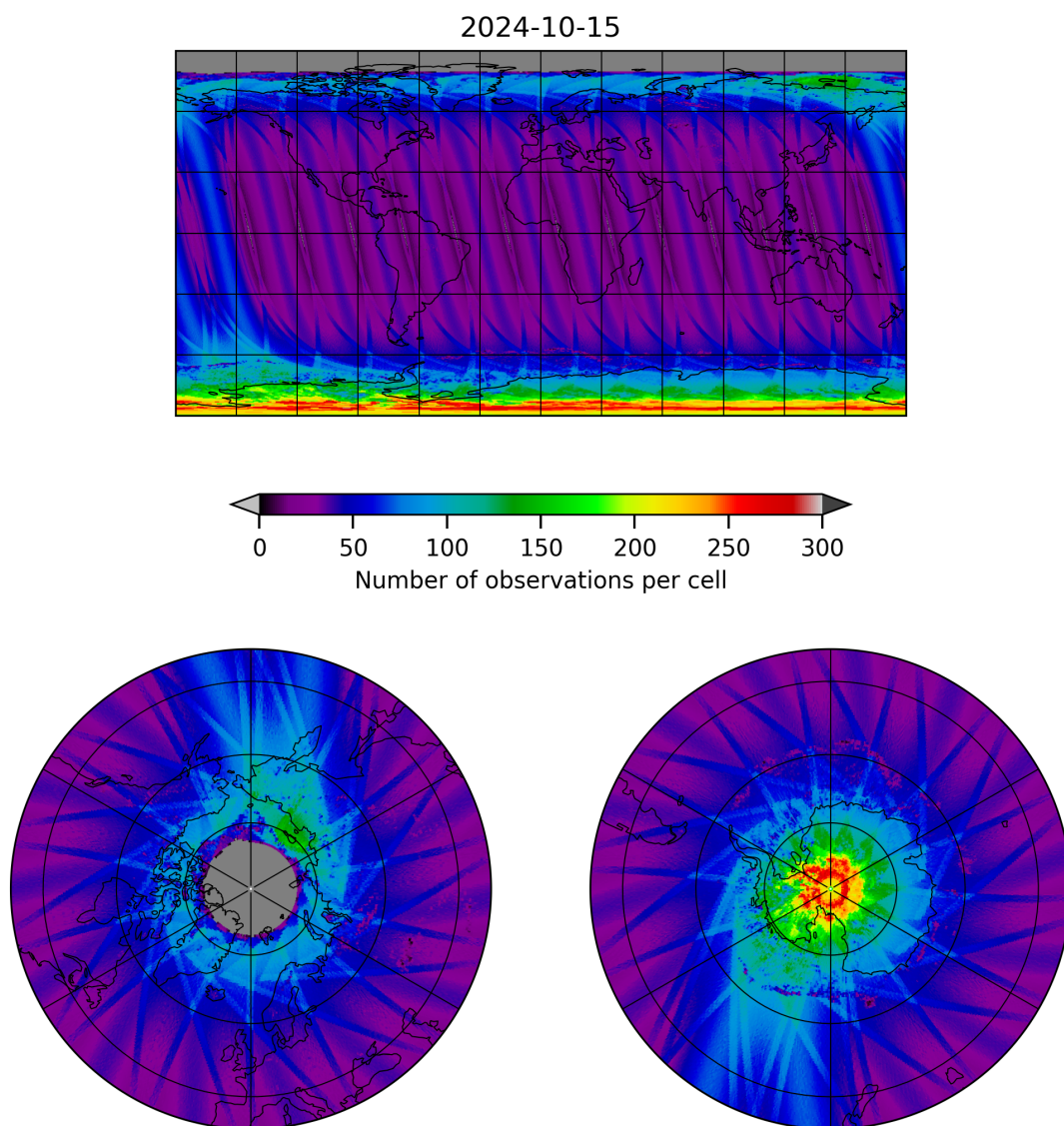
Figure 11: Map of the number of observations for 2024-10-14 to 2024-10-16
