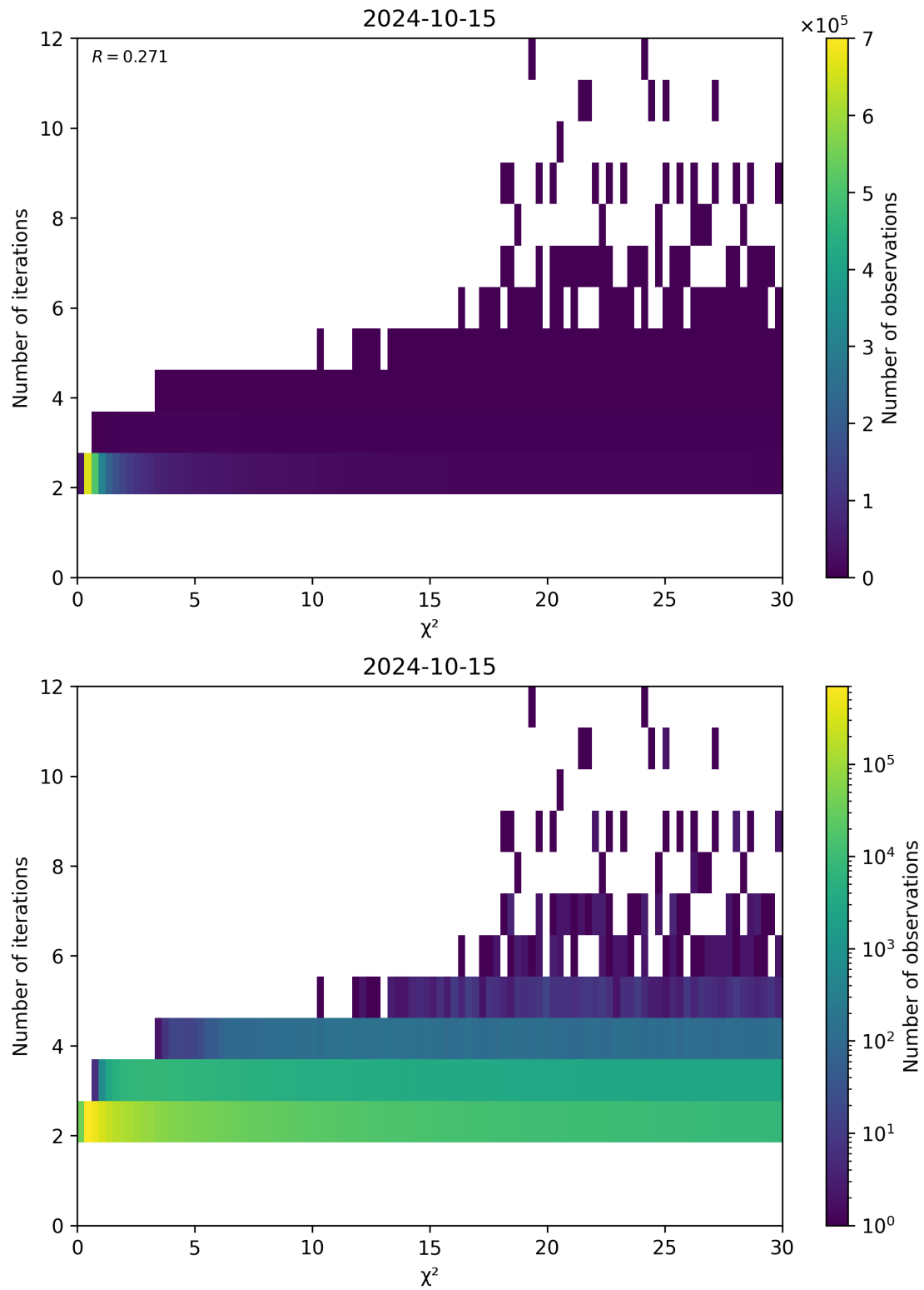
Figure 73: Scatter density plot of “ \chi^2 ” against “Number of iterations” for 2024-10-14 to 2024-10-16.
