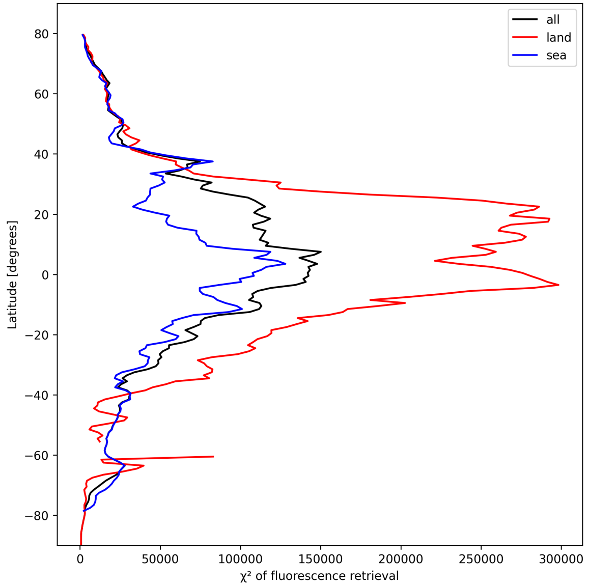
Figure 25: Zonal average of “ \chi^2 of fluorescence retrieval” for 2024-10-14 to 2024-10-16.
