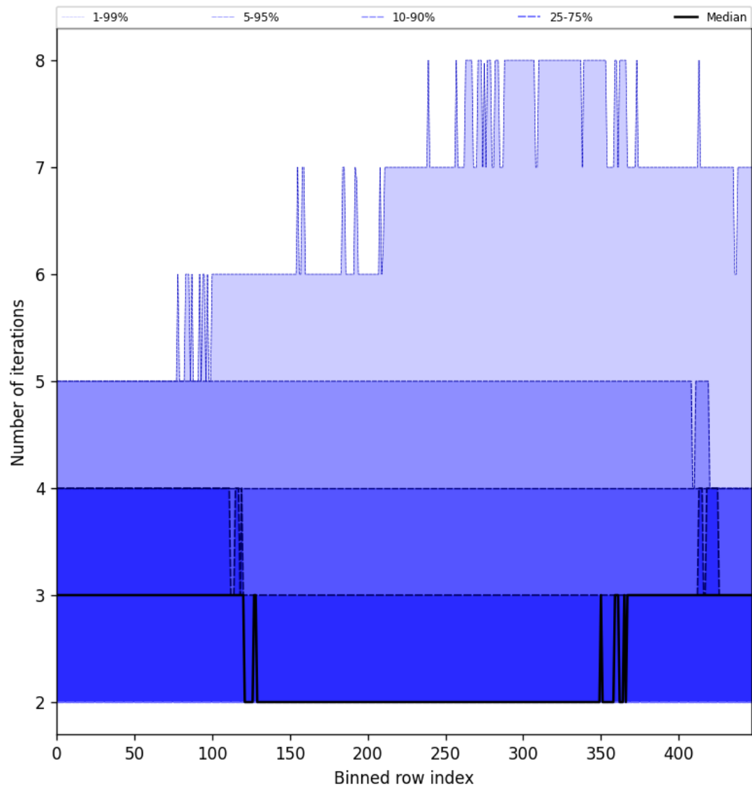
Figure 56: Along track statistics of “Number of iterations” for 2024-10-14 to 2024-10-16
