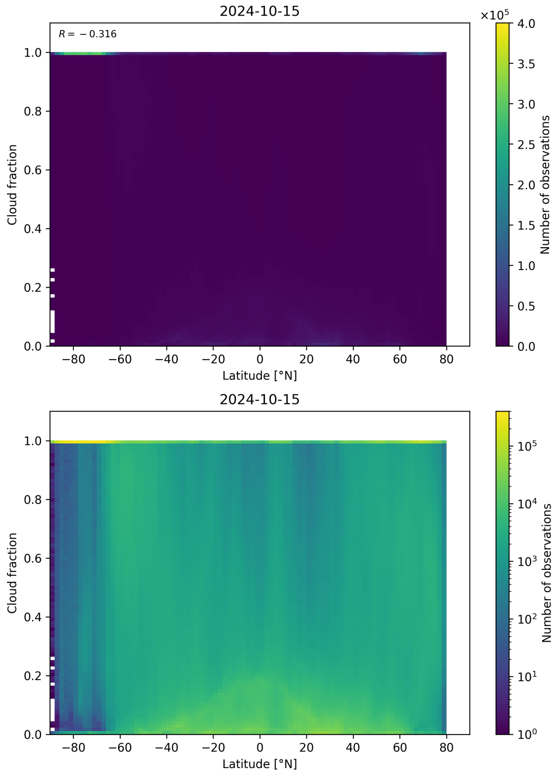
Figure 99: Scatter density plot of “Latitude” against “Cloud fraction” for 2024-10-14 to 2024-10-16.
