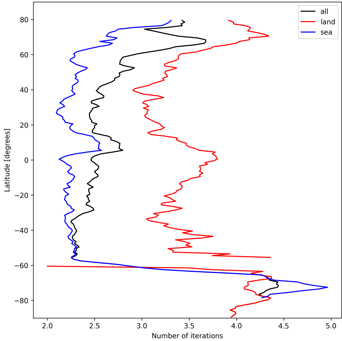
Figure 22: Zonal average of “Number of iterations” for 2024-10-14 to 2024-10-16.
