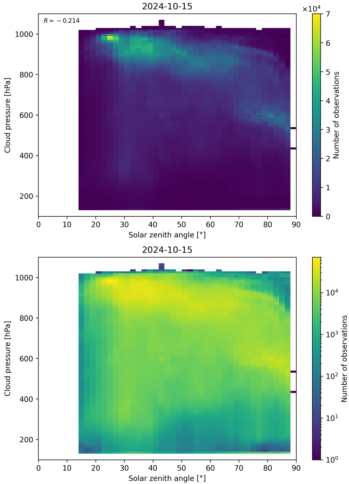
Figure 122: Scatter density plot of “Solar zenith angle” against “Cloud pressure” for 2024-10-14 to 2024-10-16.
