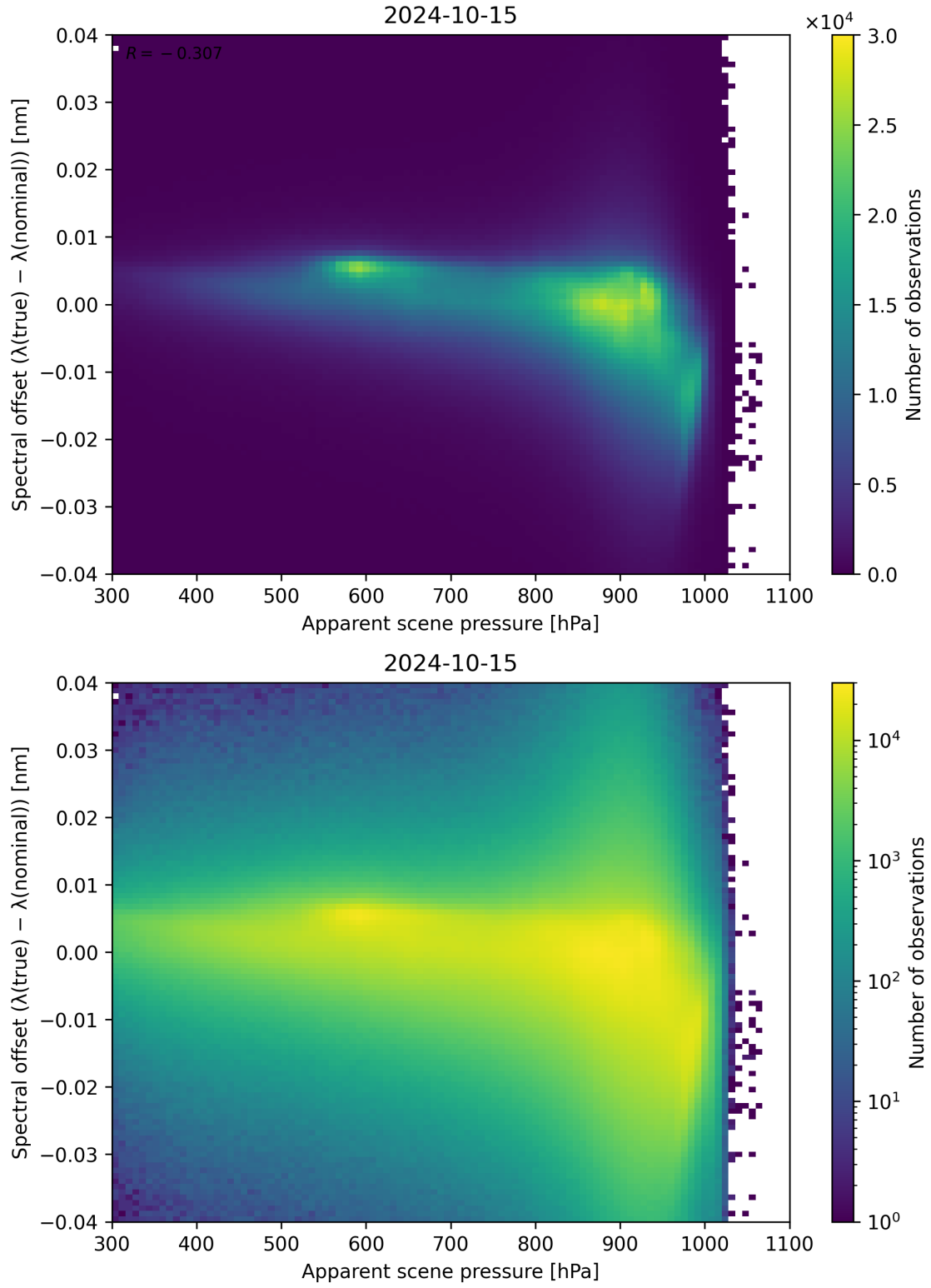
Figure 68: Scatter density plot of “Apparent scene pressure” against “Spectral offset ( \lambda_{\text{true}} - \lambda_{\text{nominal}} )” for 2024-10-14 to 2024-10-16.
