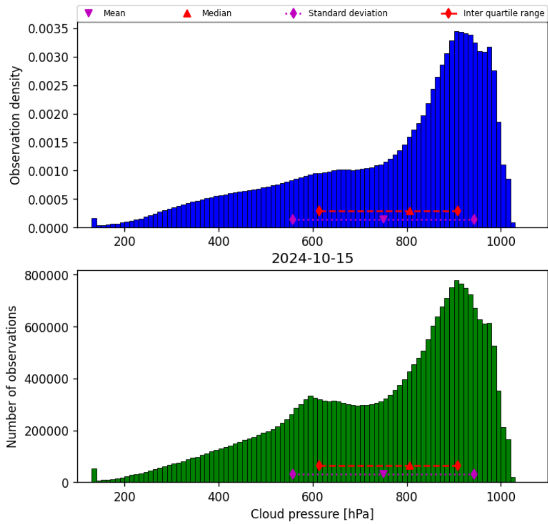
Figure 30: Histogram of “Cloud pressure” for 2024-10-14 to 2024-10-16
