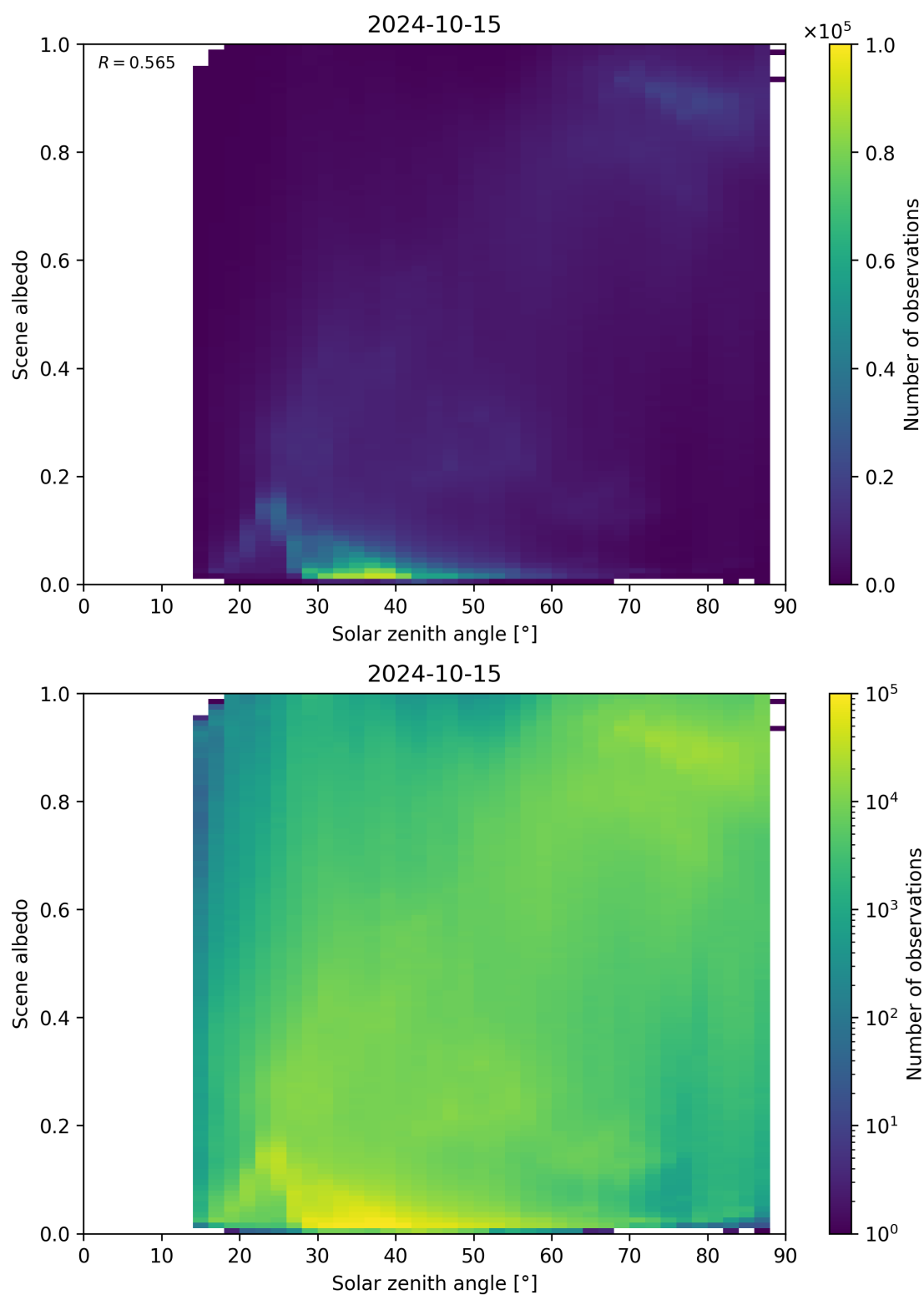
Figure 127: Scatter density plot of “Solar zenith angle” against “Scene albedo” for 2024-10-14 to 2024-10-16.
