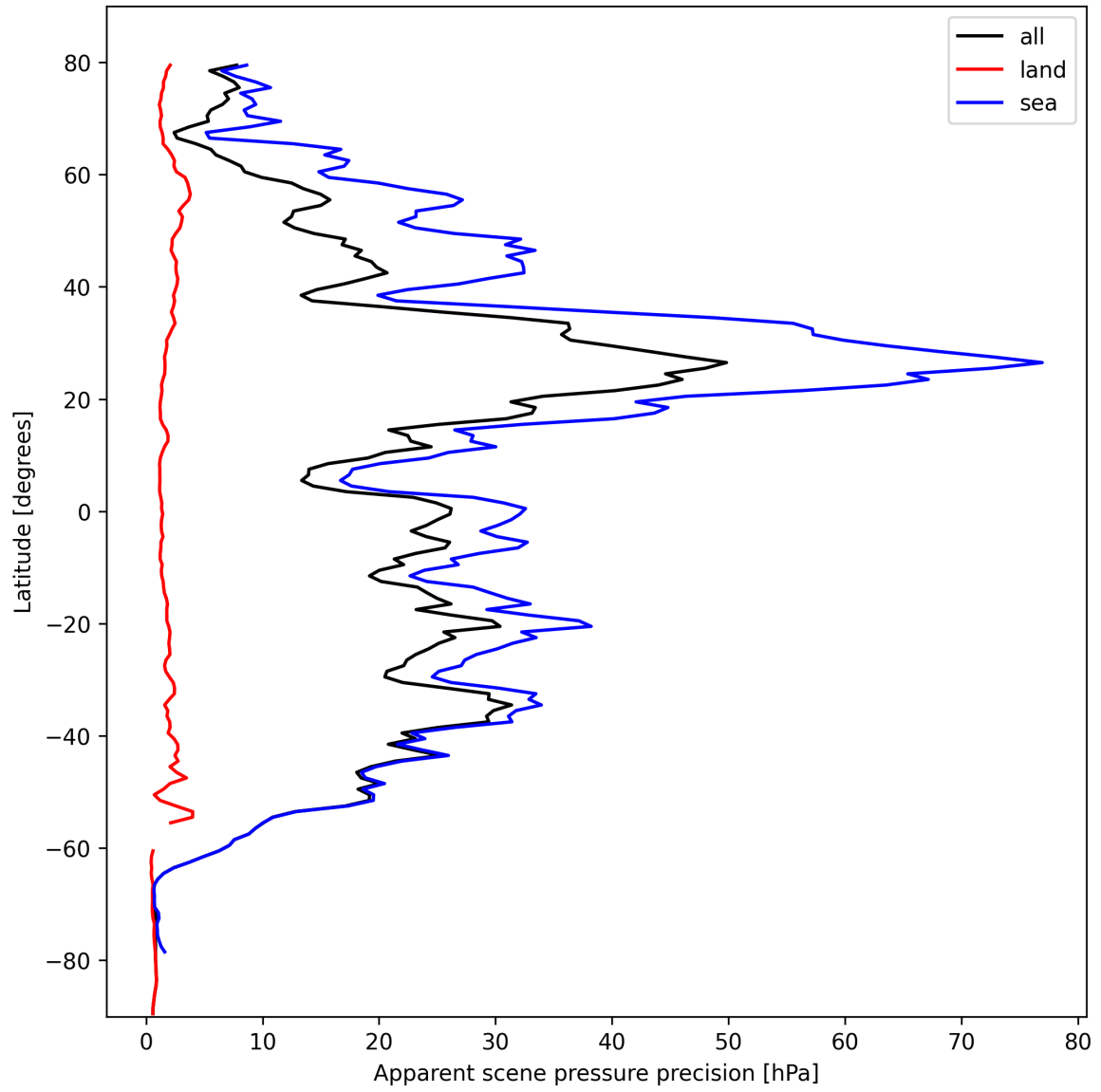
Figure 20: Zonal average of “Apparent scene pressure precision” for 2024-10-14 to 2024-10-16.
