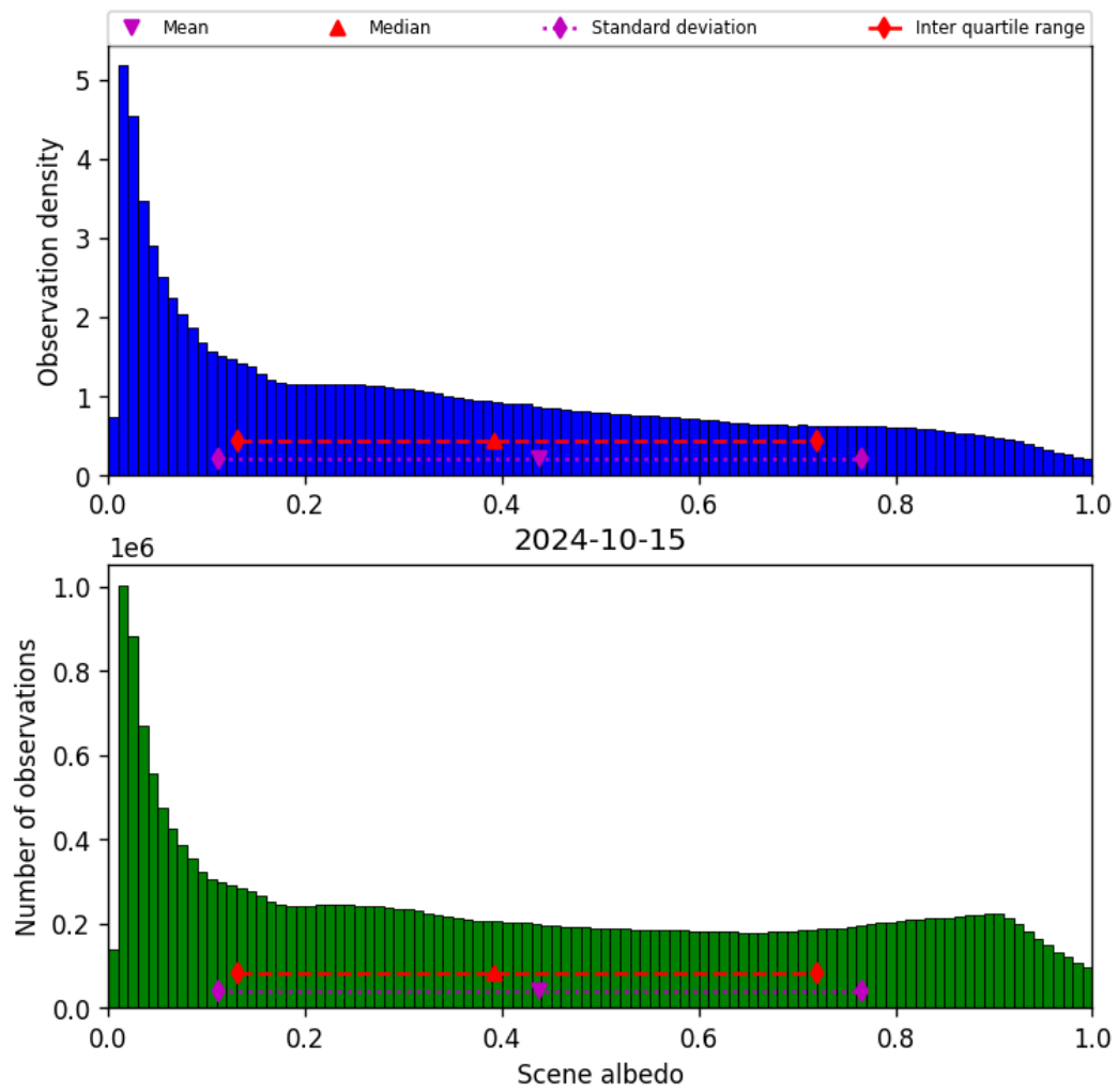
Figure 34: Histogram of “Scene albedo” for 2024-10-14 to 2024-10-16
