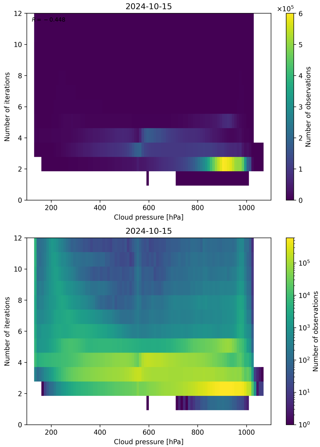
Figure 89: Scatter density plot of “Cloud pressure” against “Number of iterations” for 2024-10-14 to 2024-10-16.
