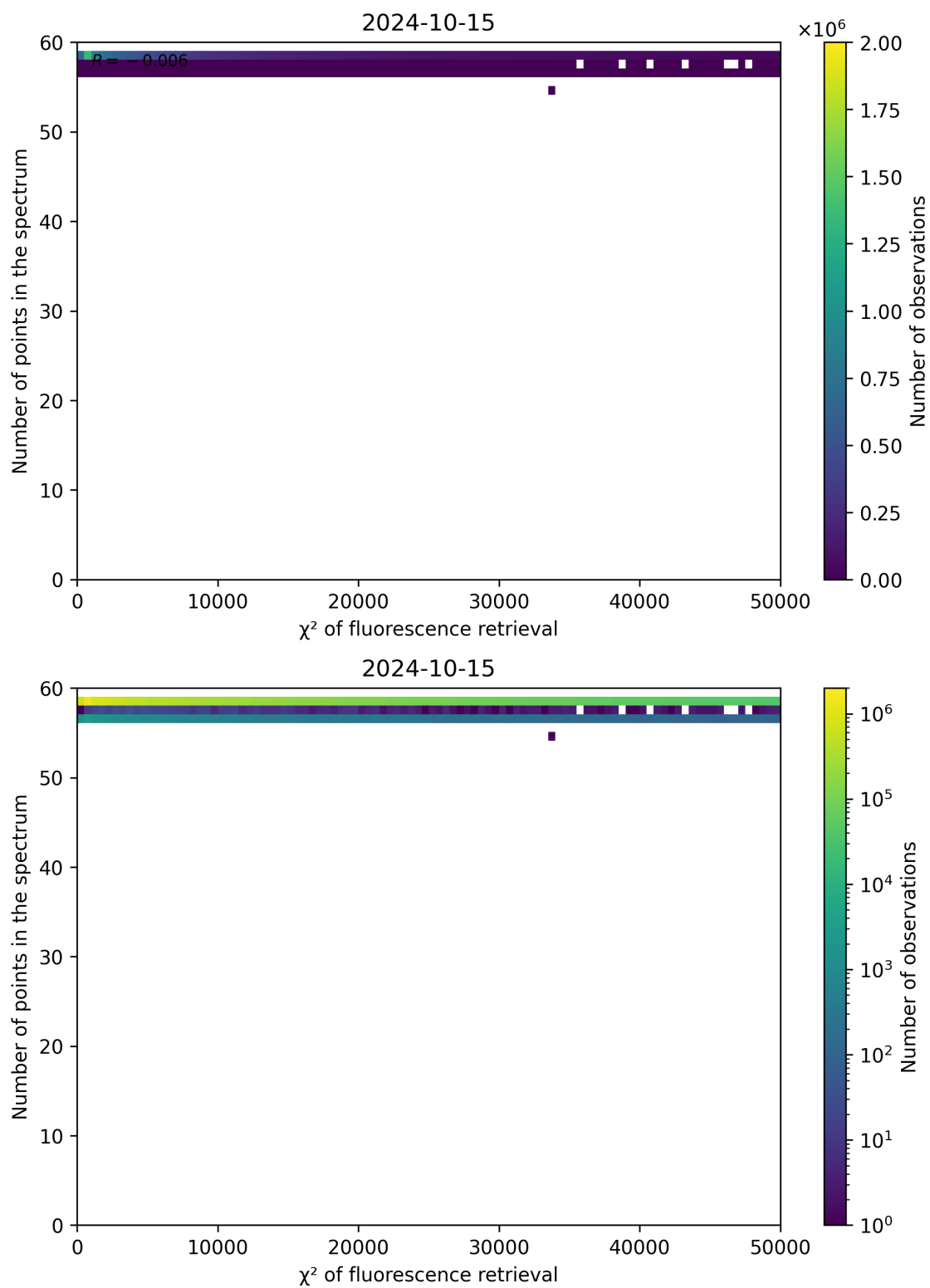
Figure 71: Scatter density plot of “ \chi^2 of fluorescence retrieval” against “Number of points in the spectrum” for 2024-10-14 to 2024-10-16.
