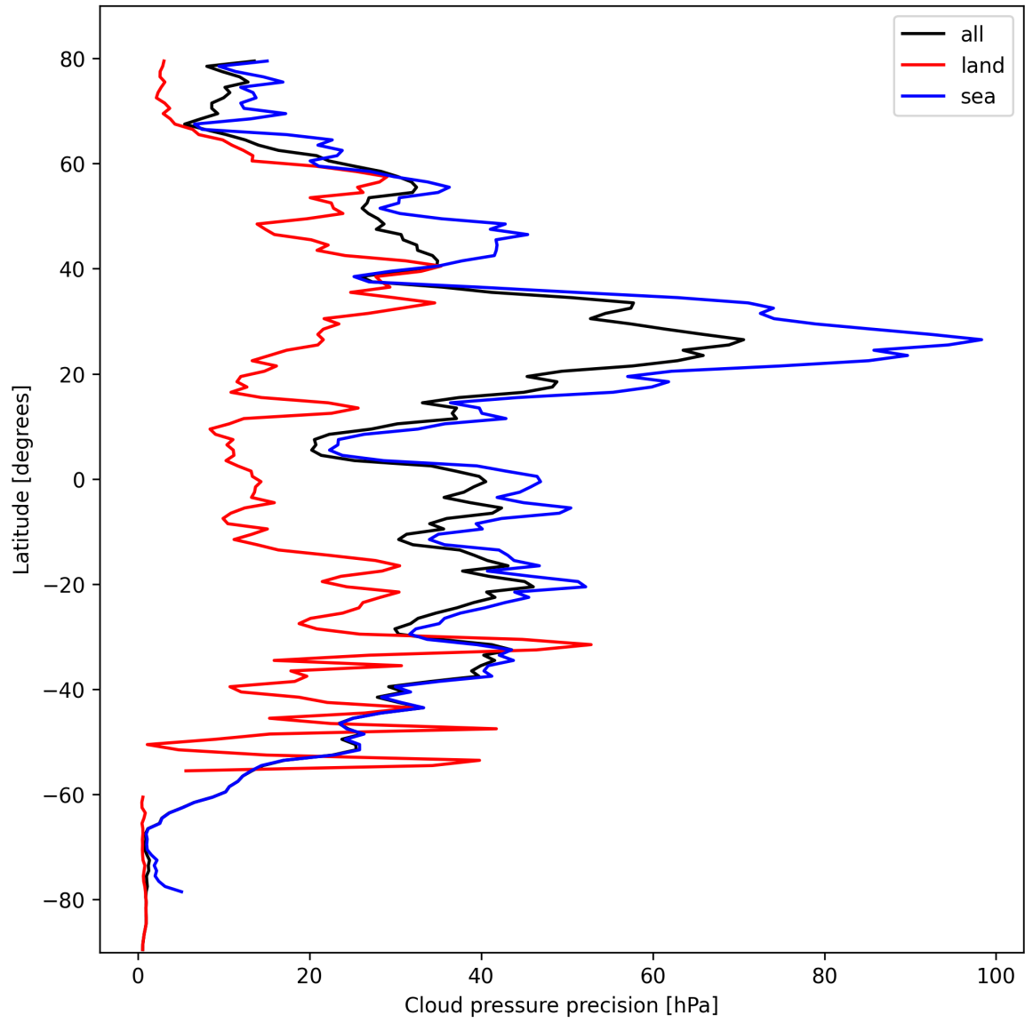
Figure 14: Zonal average of “Cloud pressure precision” for 2024-10-14 to 2024-10-16.
