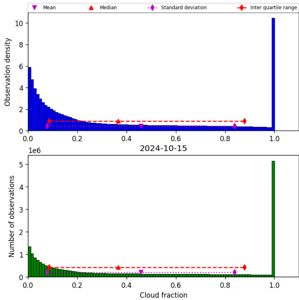
Figure 32: Histogram of “Cloud fraction” for 2024-10-14 to 2024-10-16
