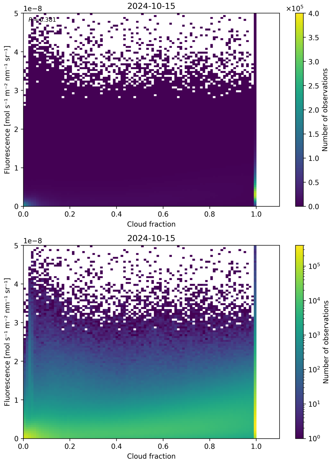
Figure 79: Scatter density plot of "Cloud fraction" against "Fluorescence" for 2024-10-14 to 2024-10-16.
