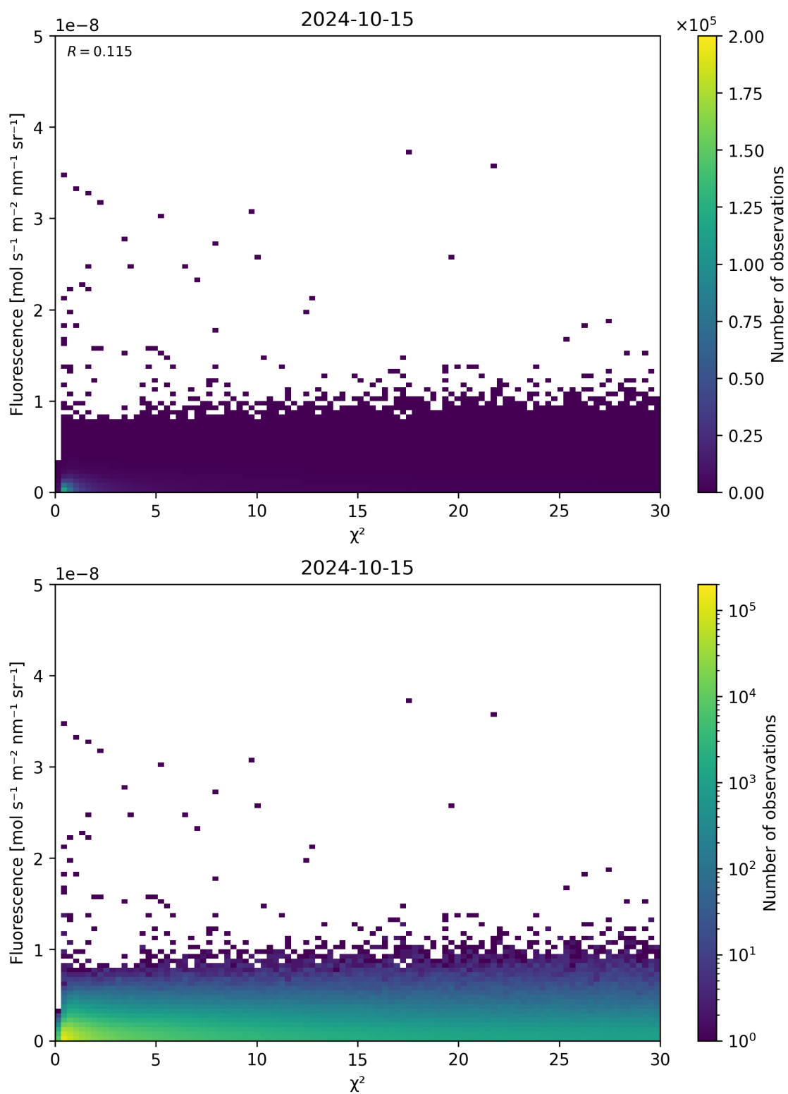
Figure 70: Scatter density plot of “ \chi^2 ” against “Fluorescence” for 2024-10-14 to 2024-10-16.
