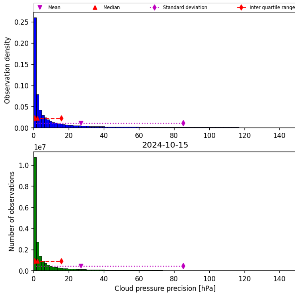
Figure 31: Histogram of “Cloud pressure precision” for 2024-10-14 to 2024-10-16
