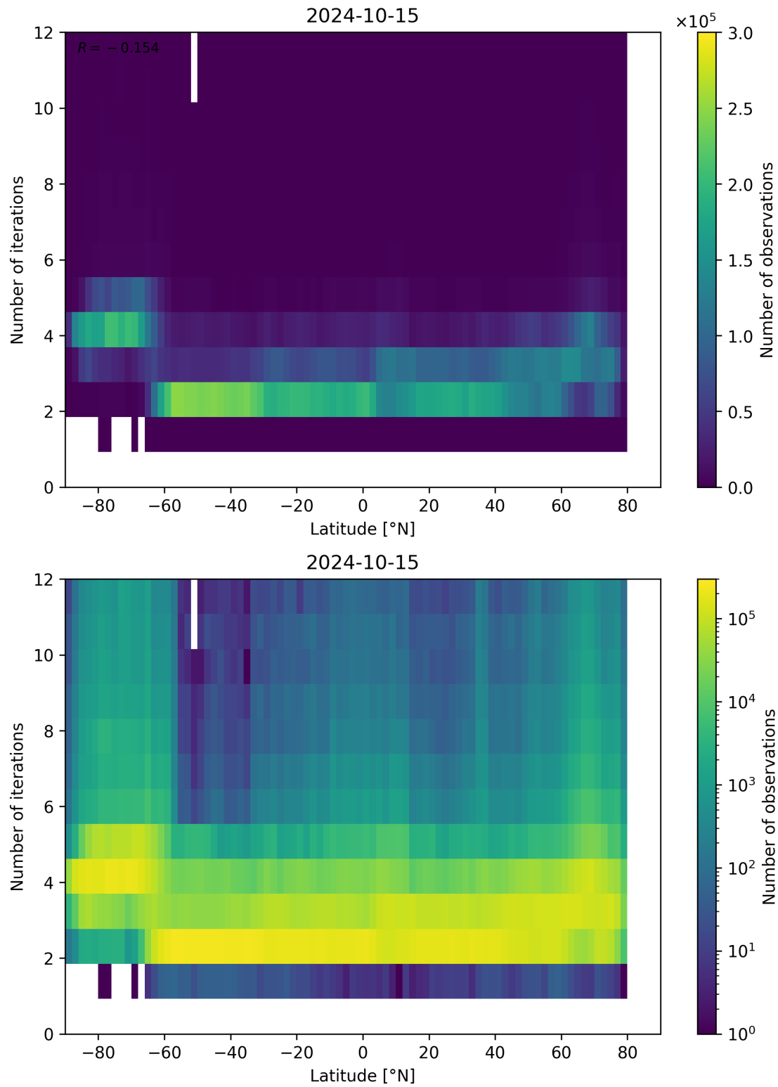
Figure 102: Scatter density plot of “Latitude” against “Number of iterations” for 2024-10-14 to 2024-10-16.
