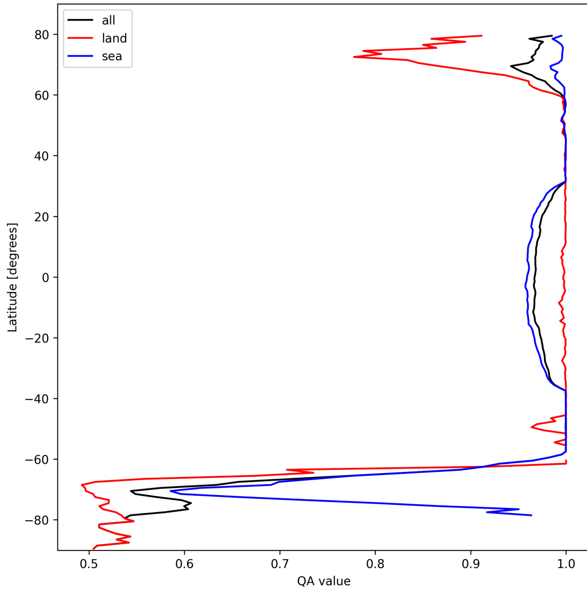
Figure 12: Zonal average of “QA value” for 2024-10-14 to 2024-10-16.
