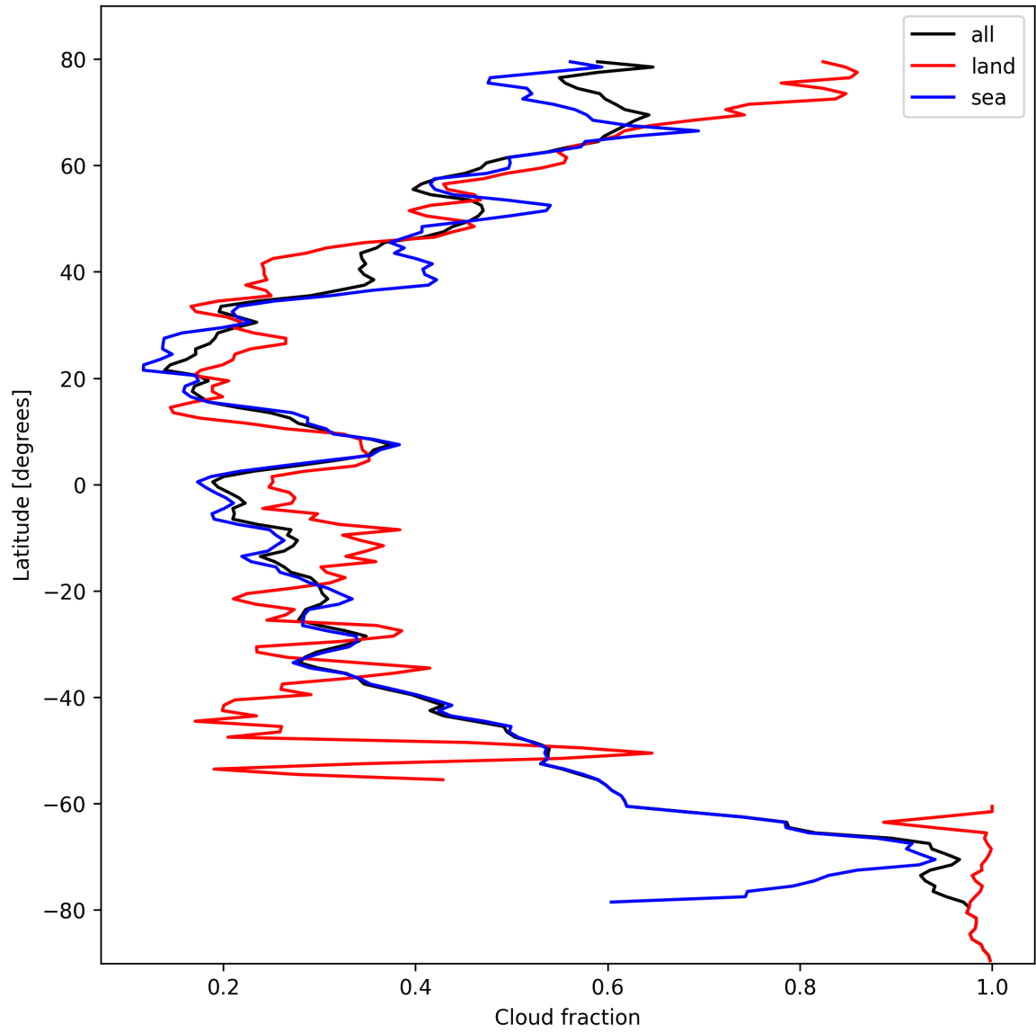
Figure 15: Zonal average of “Cloud fraction” for 2024-10-14 to 2024-10-16.
