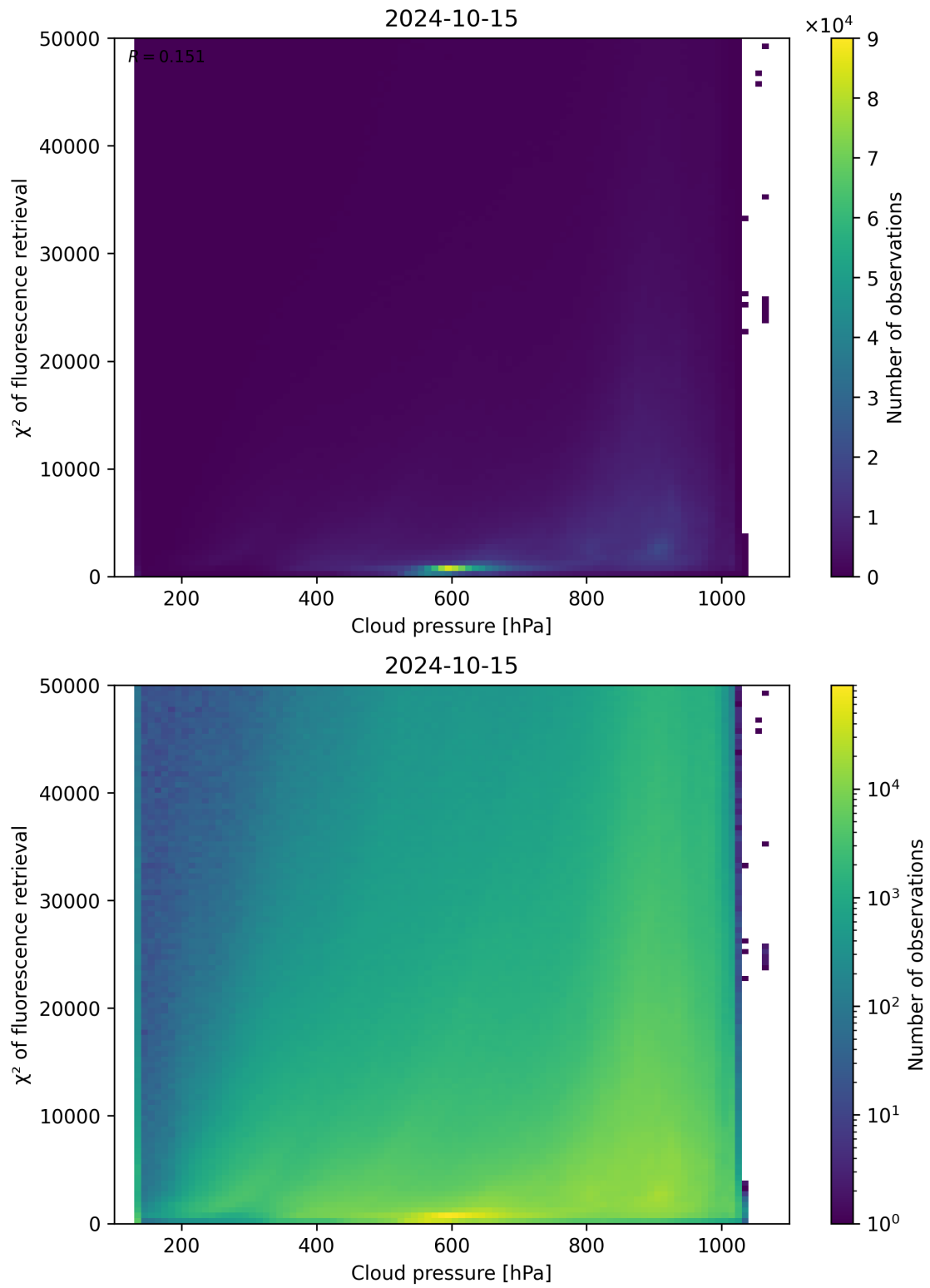
Figure 86: Scatter density plot of “Cloud pressure” against “ \chi^2 of fluorescence retrieval” for 2024-10-14 to 2024-10-16.
