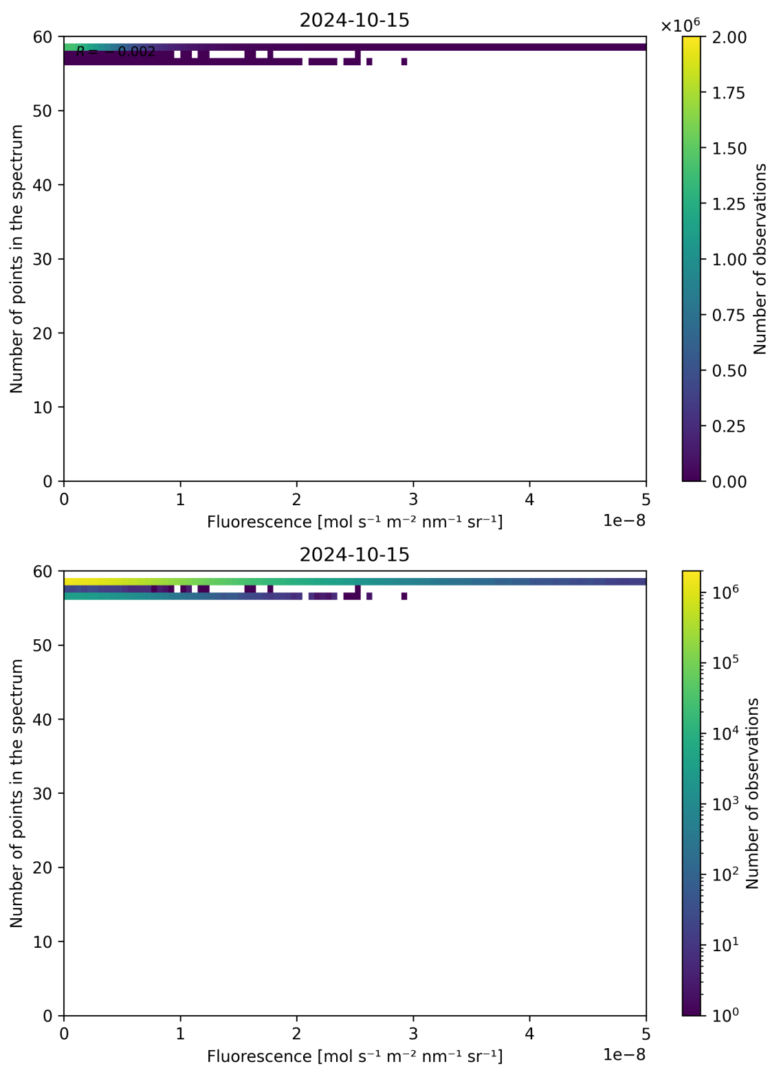
Figure 94: Scatter density plot of “Fluorescence” against “Number of points in the spectrum” for 2024-10-14 to 2024-10-16.
