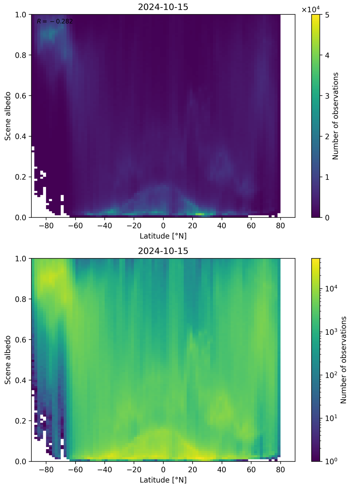
Figure 104: Scatter density plot of “Latitude” against “Scene albedo” for 2024-10-14 to 2024-10-16.
