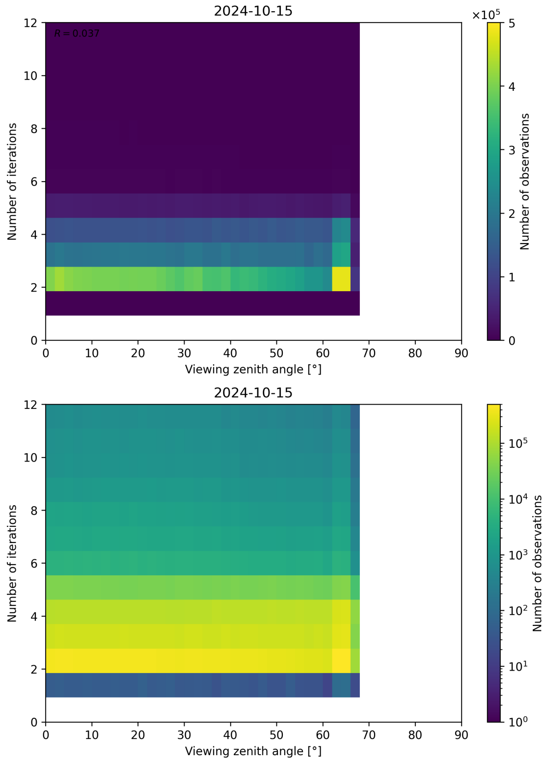
Figure 136: Scatter density plot of “Viewing zenith angle” against “Number of iterations” for 2024-10-14 to 2024-10-16.
