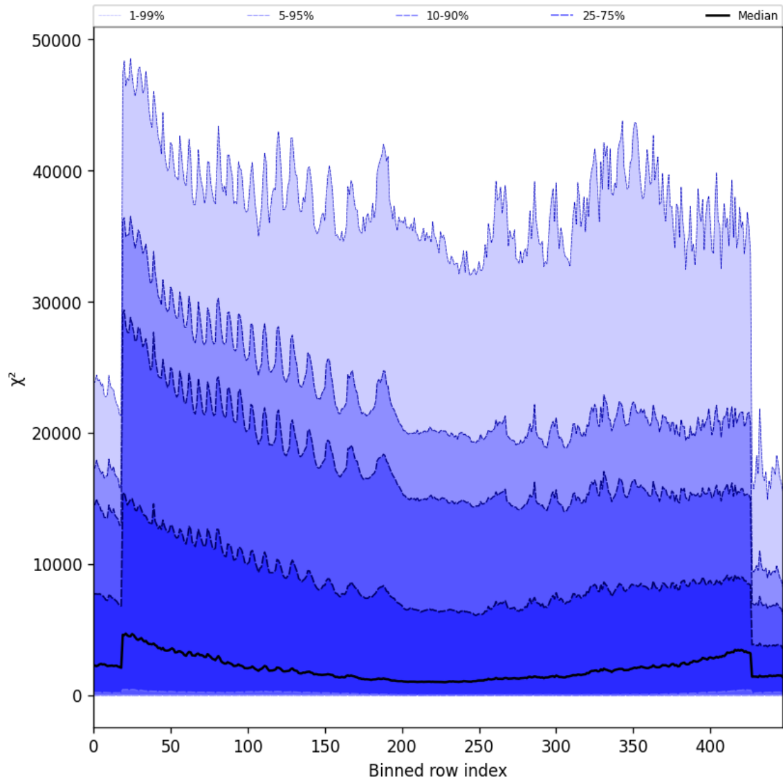
Figure 55: Along track statistics of “ \chi^2 ” for 2024-10-14 to 2024-10-16
