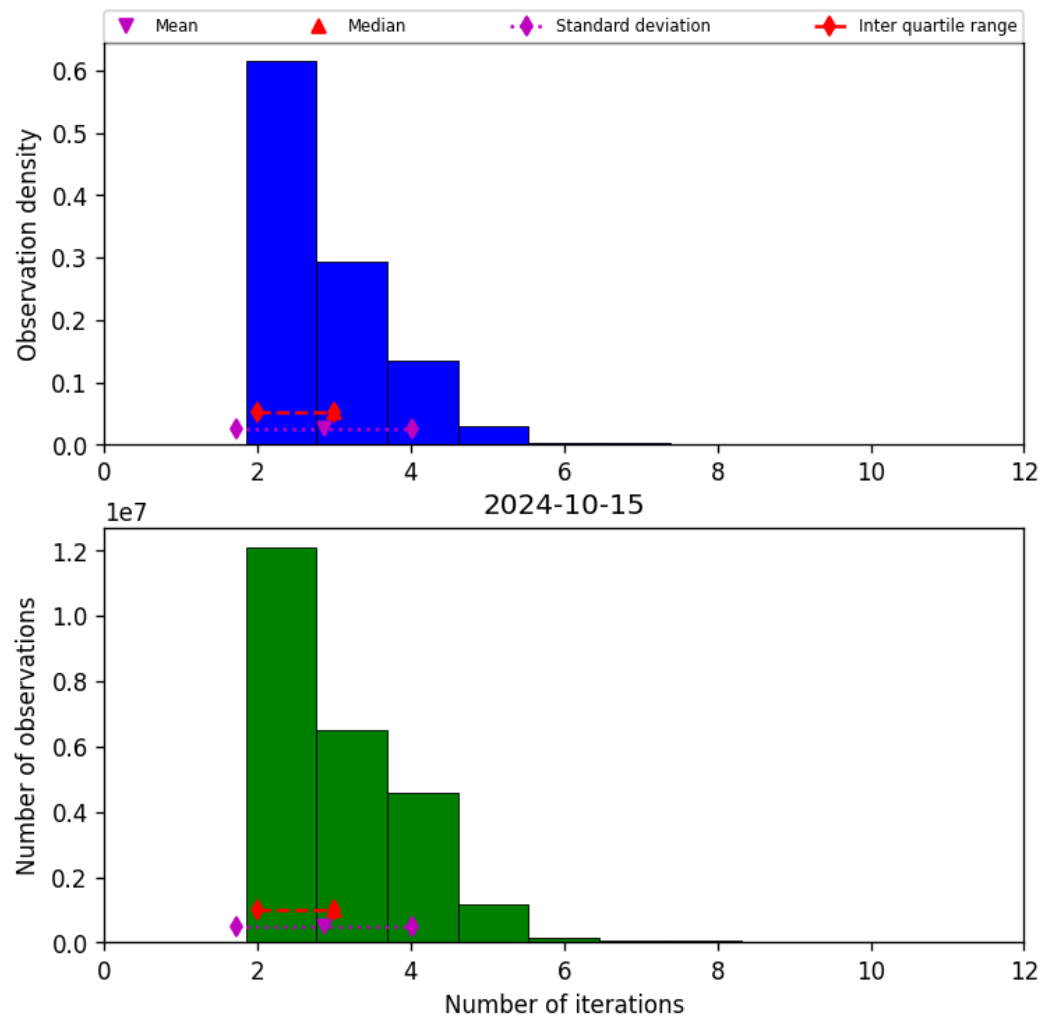
Figure 39: Histogram of “Number of iterations” for 2024-10-14 to 2024-10-16
