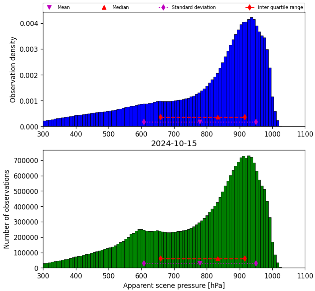
Figure 36: Histogram of "Apparent scene pressure" for 2024-10-14 to 2024-10-16
