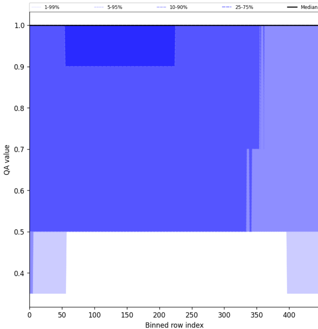
Figure 46: Along track statistics of “QA value” for 2024-10-14 to 2024-10-16
