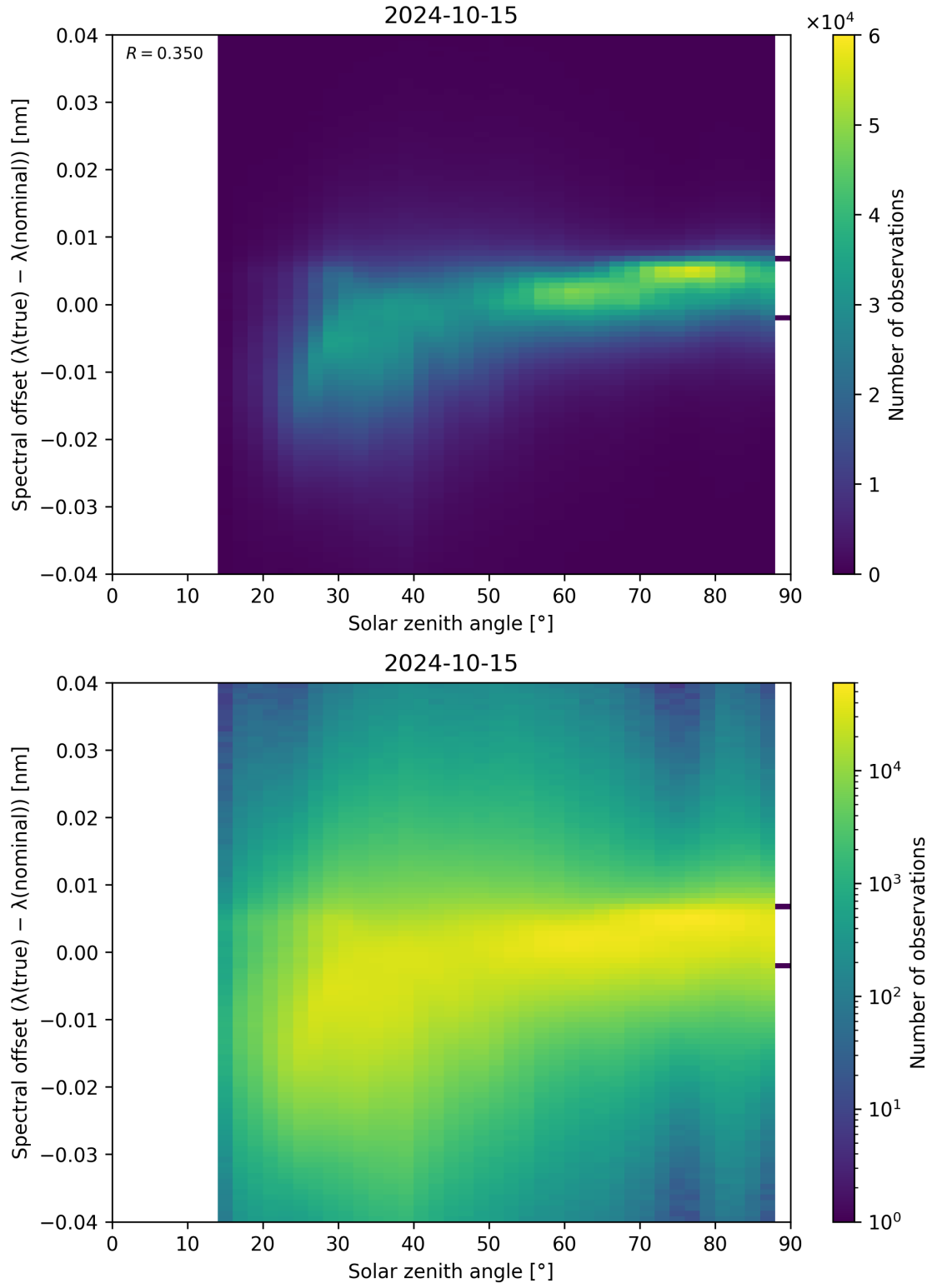
Figure 128: Scatter density plot of “Solar zenith angle” against “Spectral offset ( \lambda_{\text{true}} - \lambda_{\text{nominal}} )” for 2024-10-14 to 2024-10-16.
