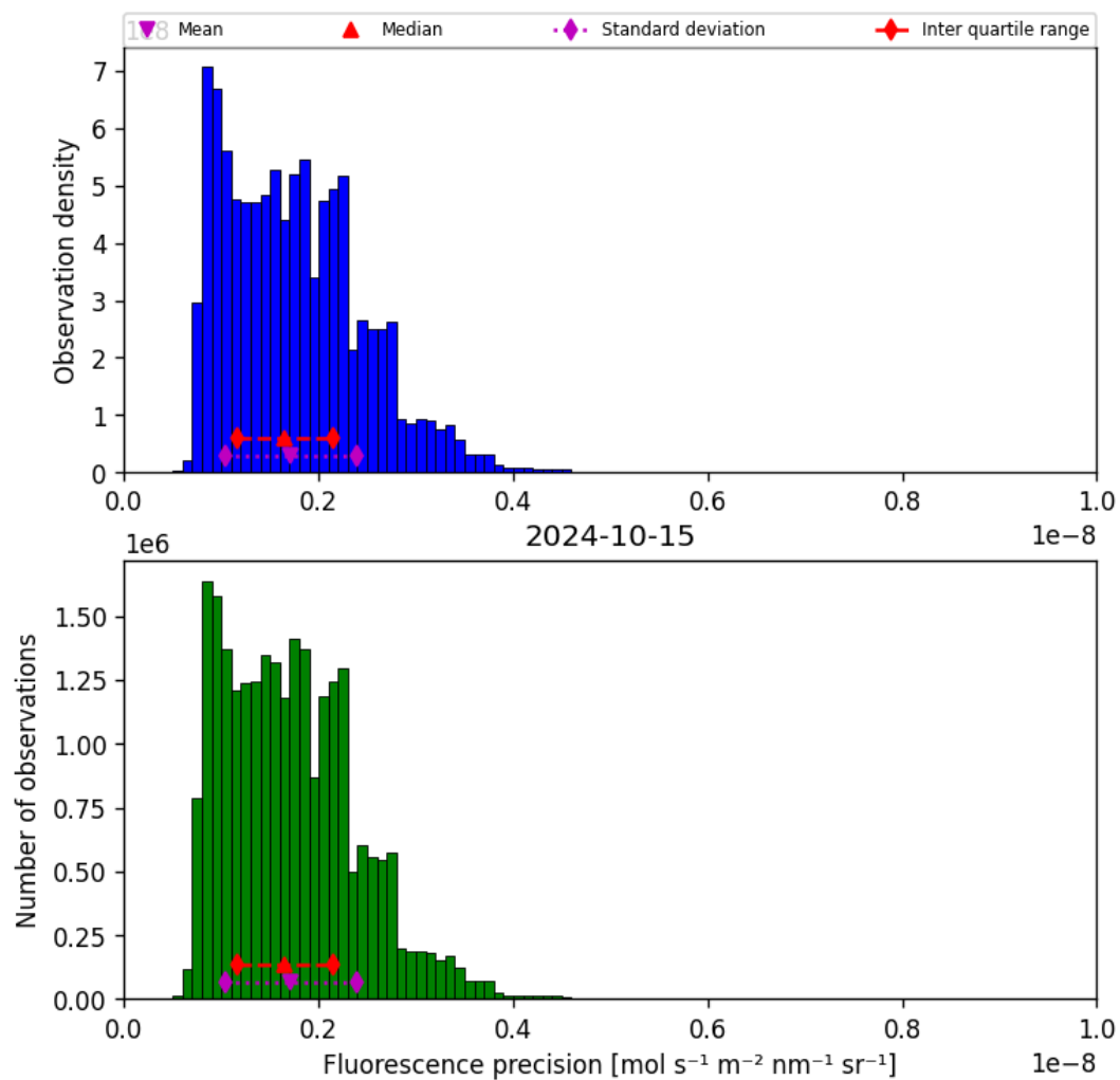
Figure 41: Histogram of “Fluorescence precision” for 2024-10-14 to 2024-10-16
