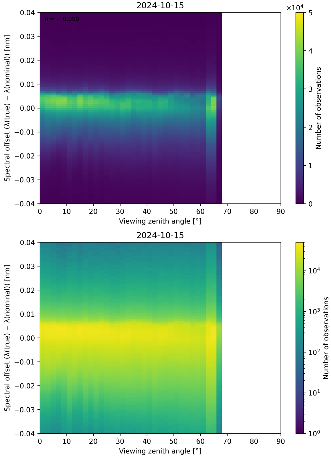
Figure 140: Scatter density plot of “Viewing zenith angle” against “Spectral offset ( \lambda_{\text{true}} - \lambda_{\text{nominal}} )” for 2024-10-14 to 2024-10-16.
