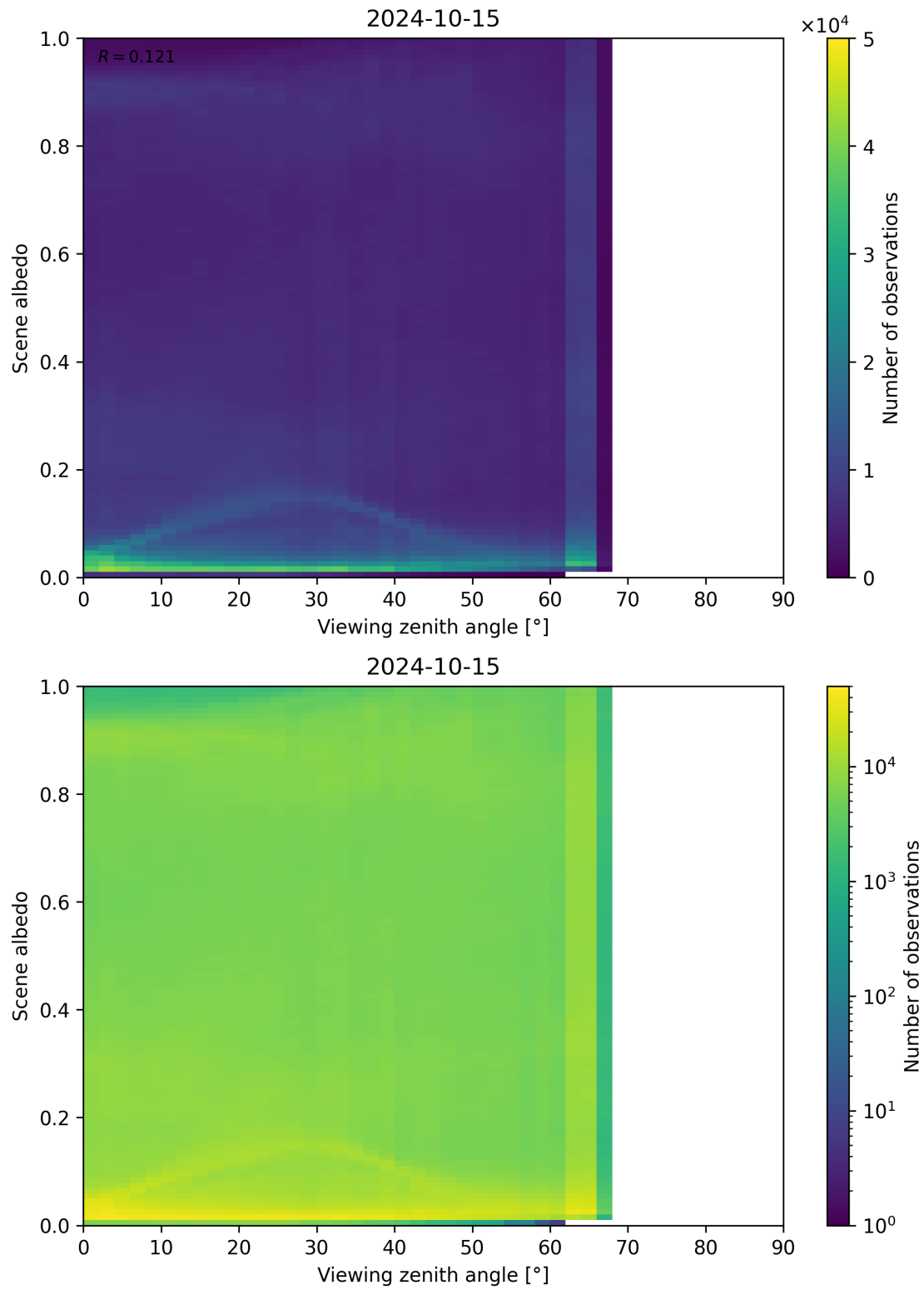
Figure 138: Scatter density plot of “Viewing zenith angle” against “Scene albedo” for 2024-10-14 to 2024-10-16.
