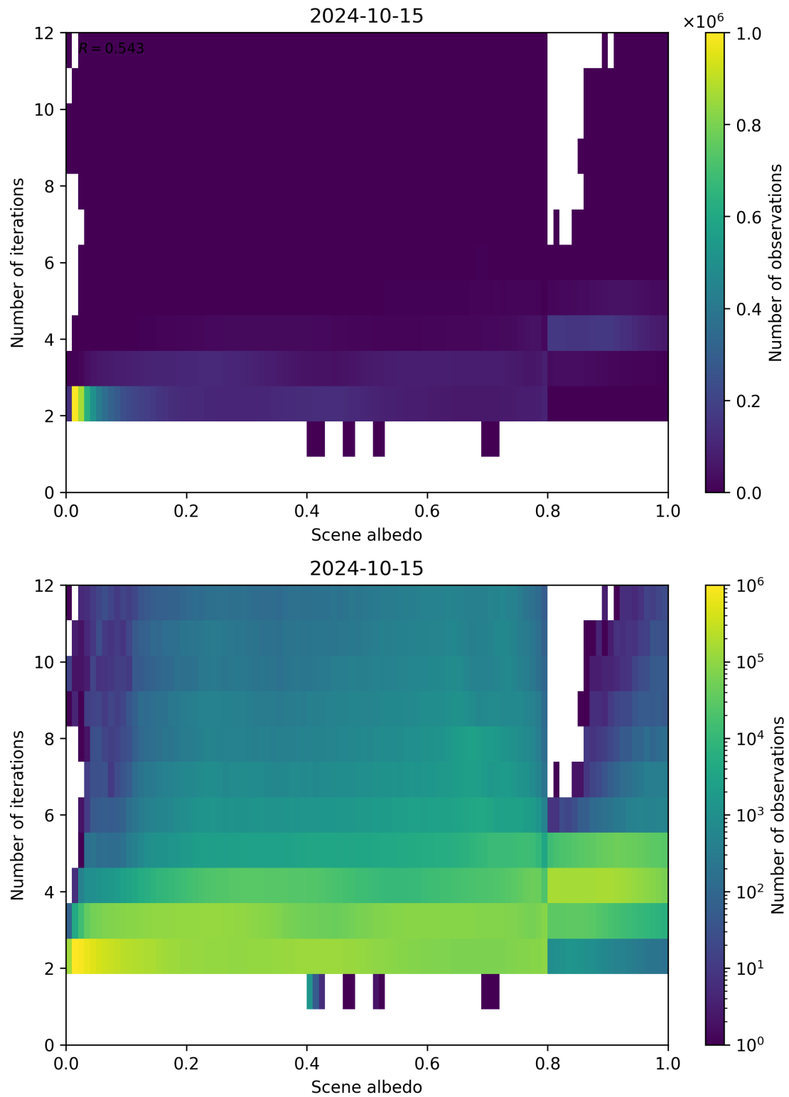
Figure 115: Scatter density plot of “Scene albedo” against “Number of iterations” for 2024-10-14 to 2024-10-16.
