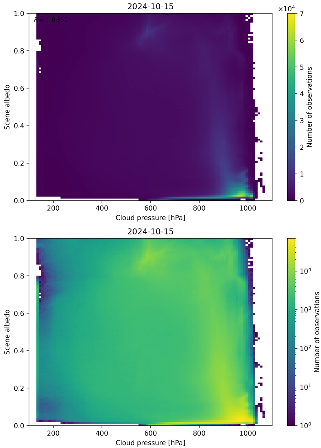
Figure 91: Scatter density plot of “Cloud pressure” against “Scene albedo” for 2024-10-14 to 2024-10-16.
