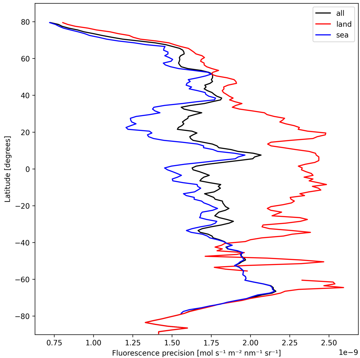
Figure 24: Zonal average of “Fluorescence precision” for 2024-10-14 to 2024-10-16.
