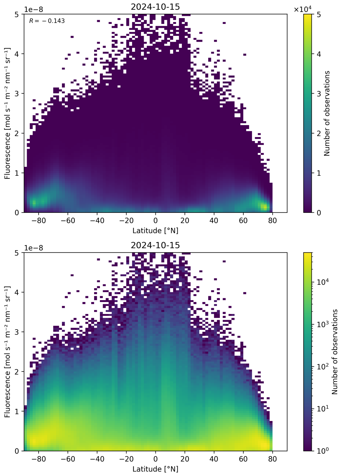
Figure 101: Scatter density plot of “Latitude” against “Fluorescence” for 2024-10-14 to 2024-10-16.
