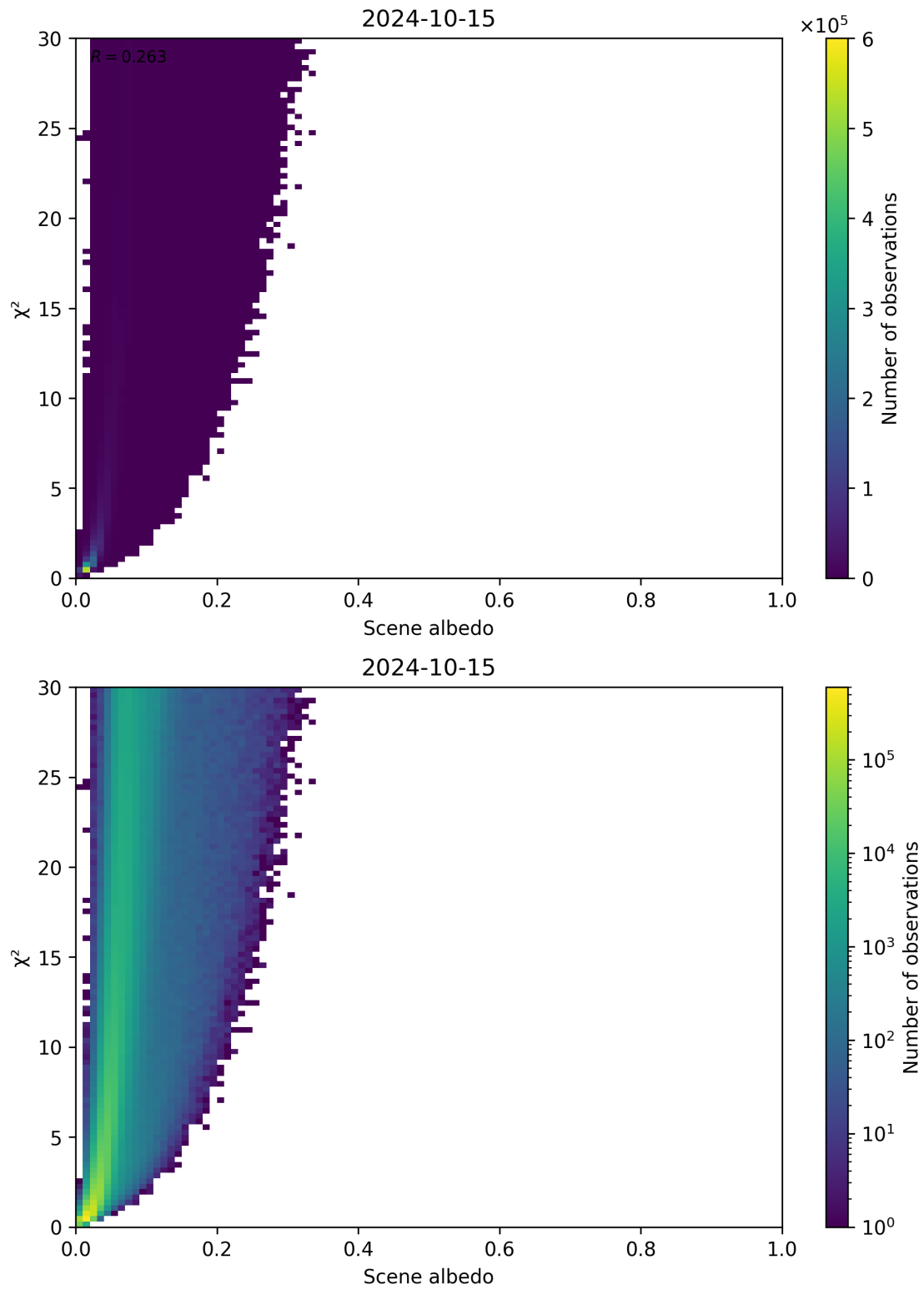
Figure 112: Scatter density plot of “Scene albedo” against “ \chi^2 ” for 2024-10-14 to 2024-10-16.
