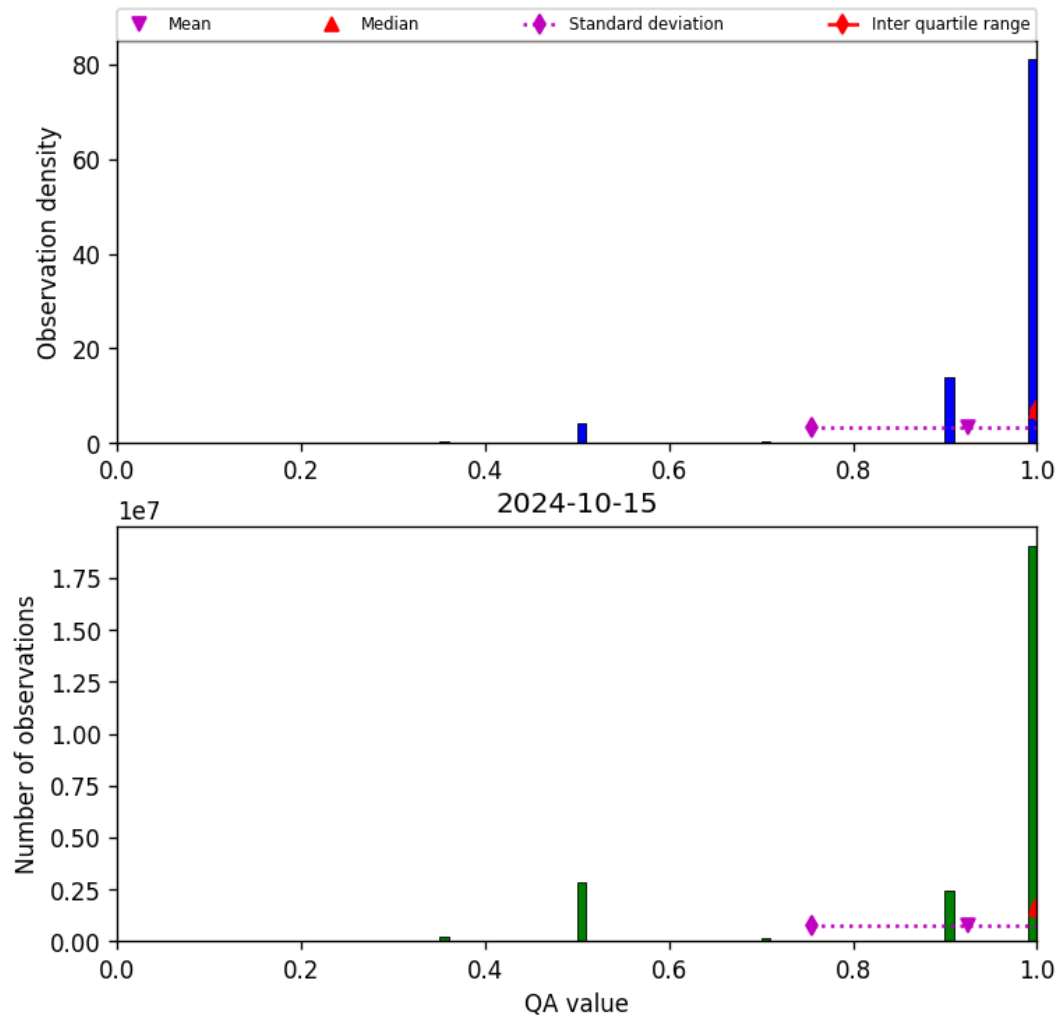
Figure 29: Histogram of “QA value” for 2024-10-14 to 2024-10-16
