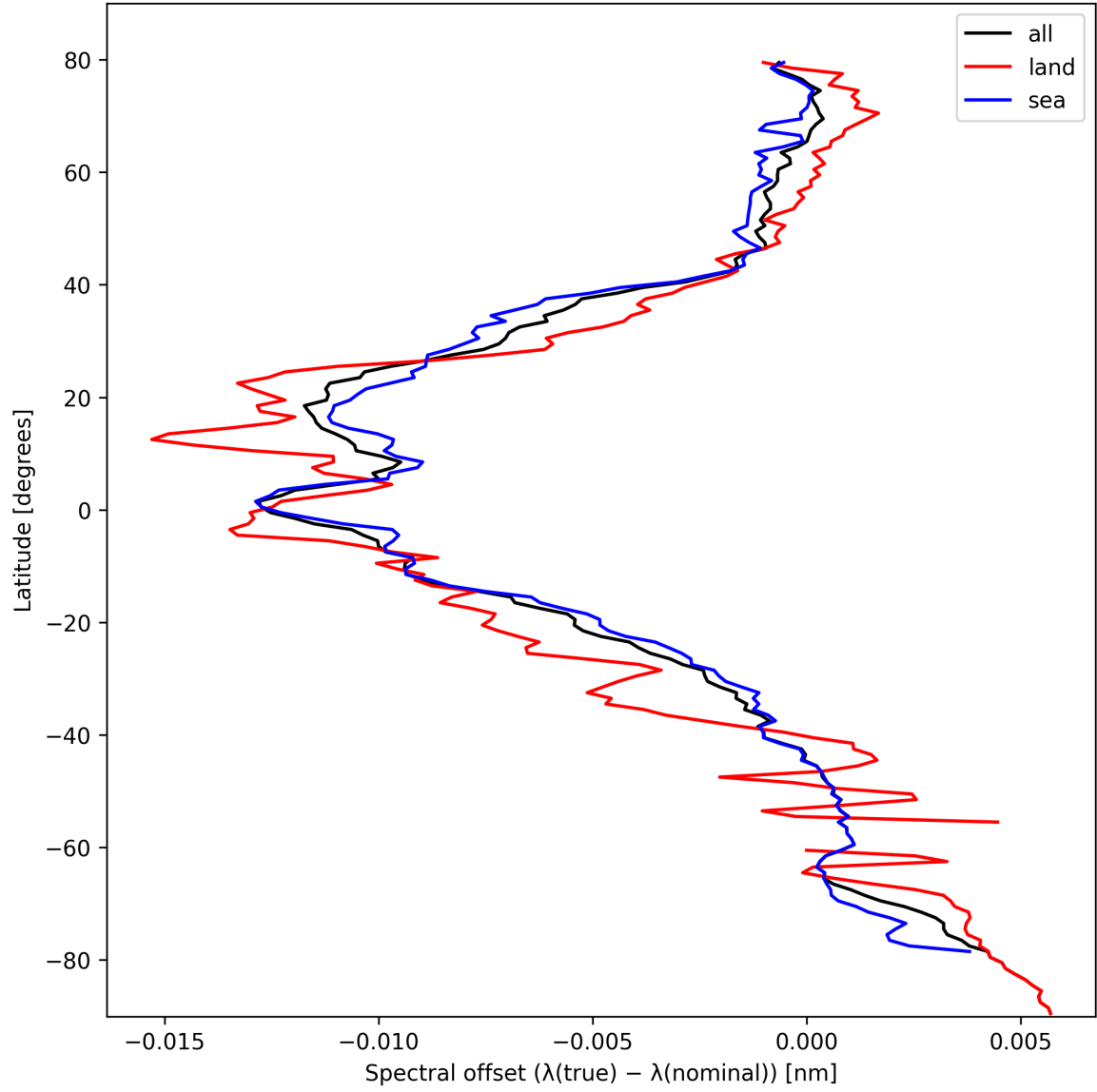
Figure 28: Zonal average of “Spectral offset ( \lambda_{\text{true}} - \lambda_{\text{nominal}} )” for 2024-10-14 to 2024-10-16.
