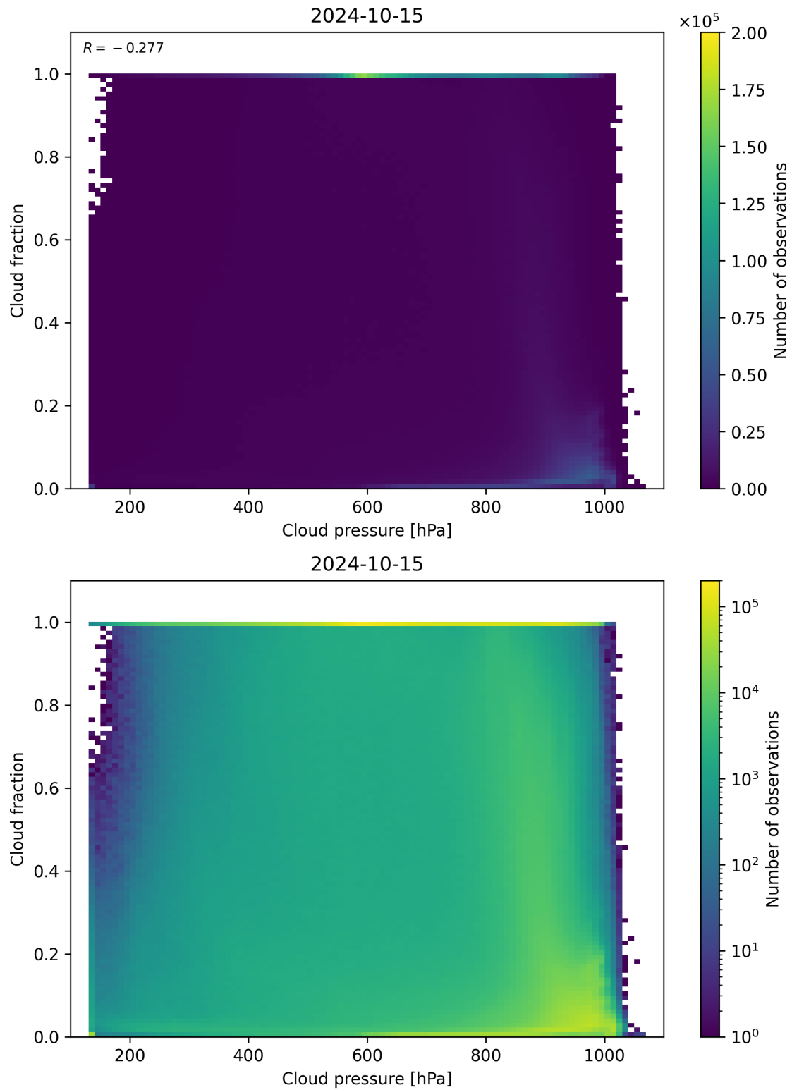
Figure 87: Scatter density plot of “Cloud pressure” against “Cloud fraction” for 2024-10-14 to 2024-10-16.
