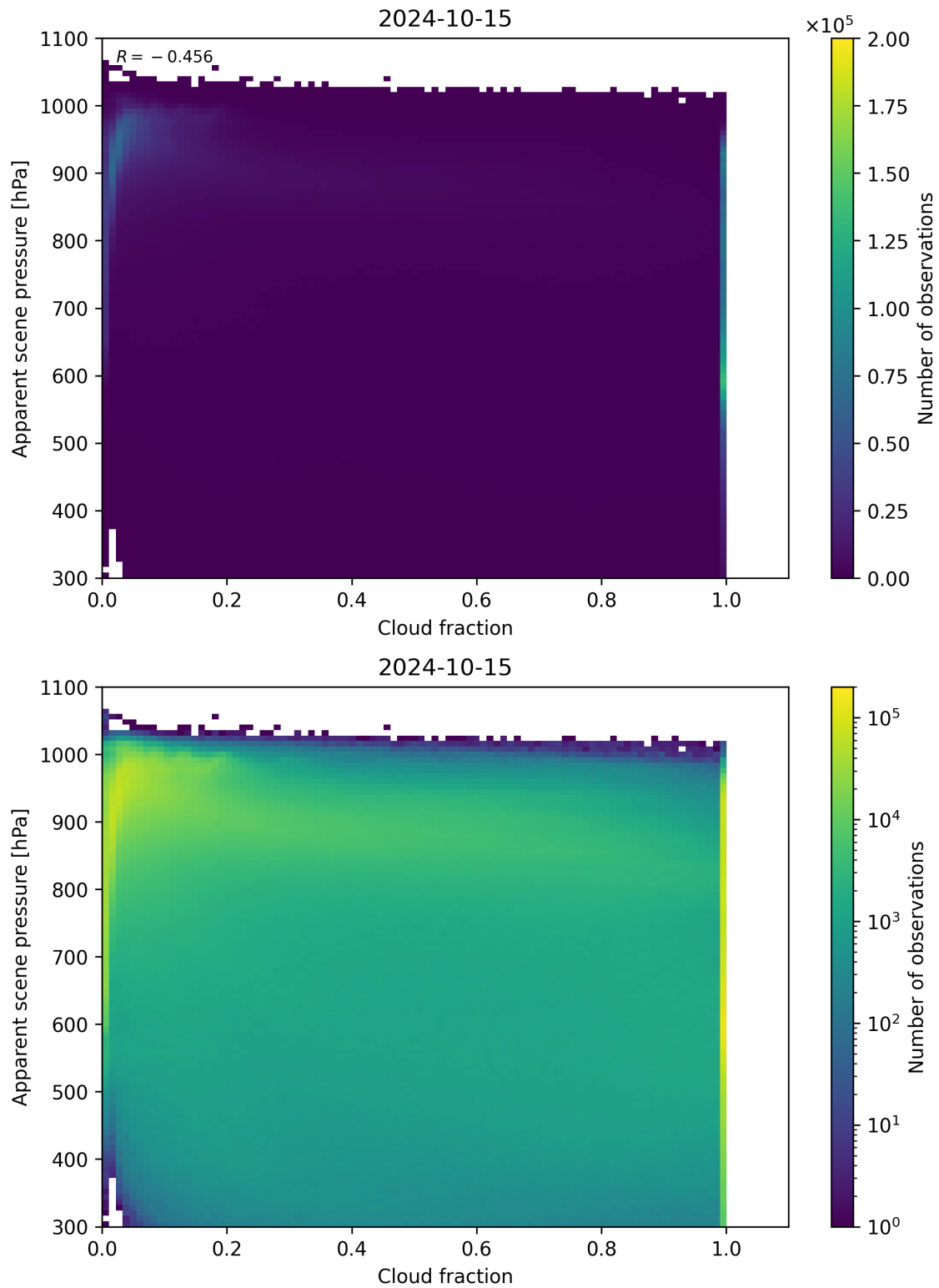
Figure 76: Scatter density plot of “Cloud fraction” against “Apparent scene pressure” for 2024-10-14 to 2024-10-16.
