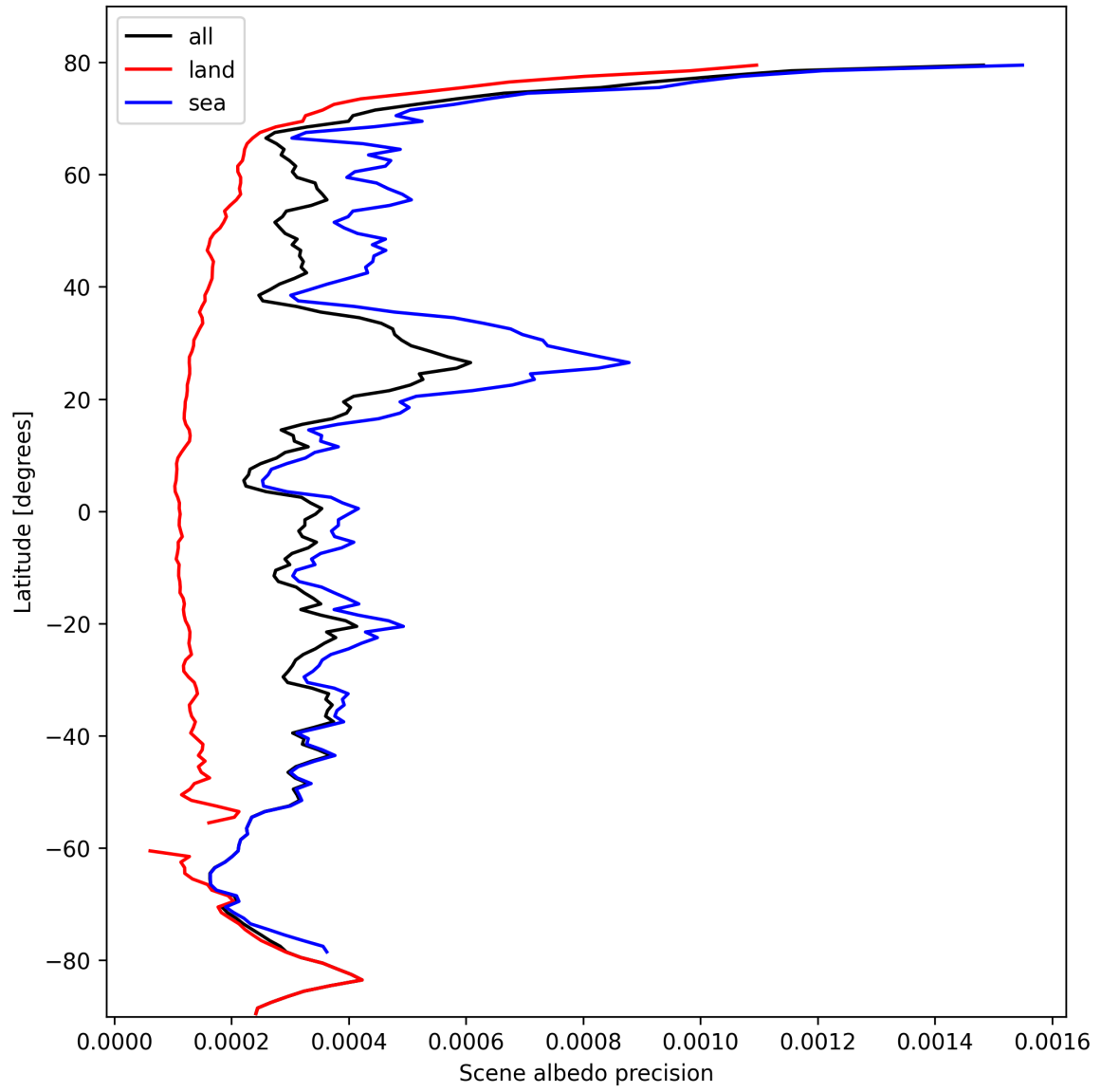
Figure 18: Zonal average of “Scene albedo precision” for 2024-10-14 to 2024-10-16.
