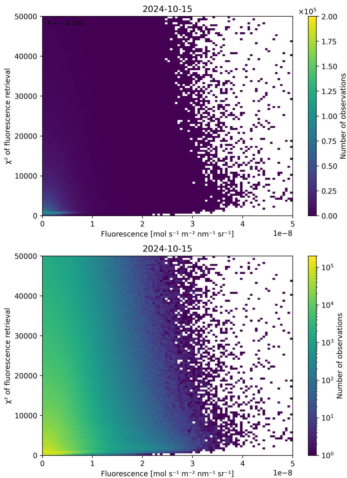
Figure 93: Scatter density plot of “Fluorescence” against “ \chi^2 of fluorescence retrieval” for 2024-10-14 to 2024-10-16.
