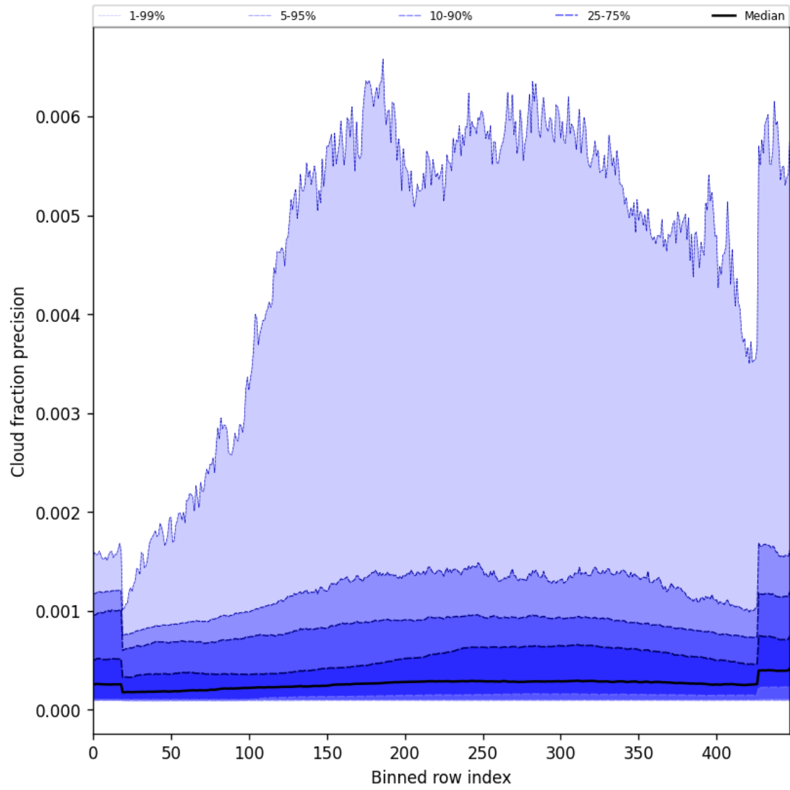
Figure 50: Along track statistics of “Cloud fraction precision” for 2024-10-14 to 2024-10-16
