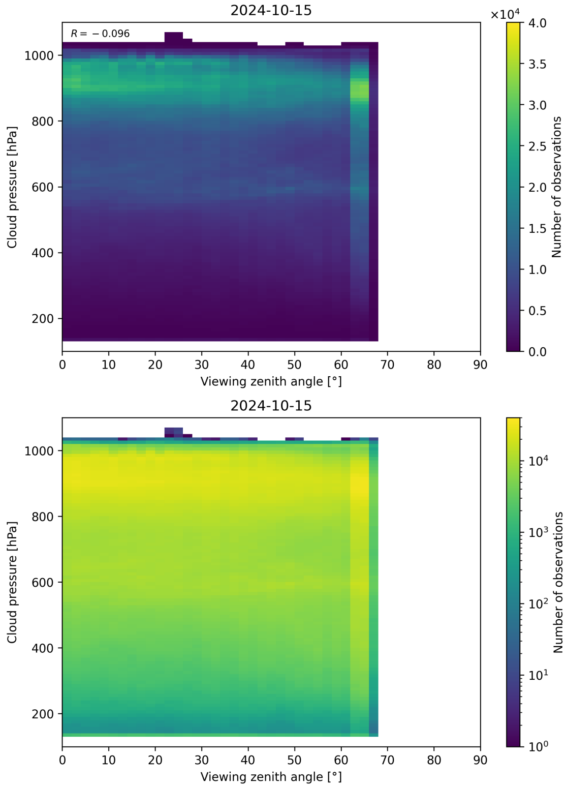
Figure 133: Scatter density plot of “Viewing zenith angle” against “Cloud pressure” for 2024-10-14 to 2024-10-16.
