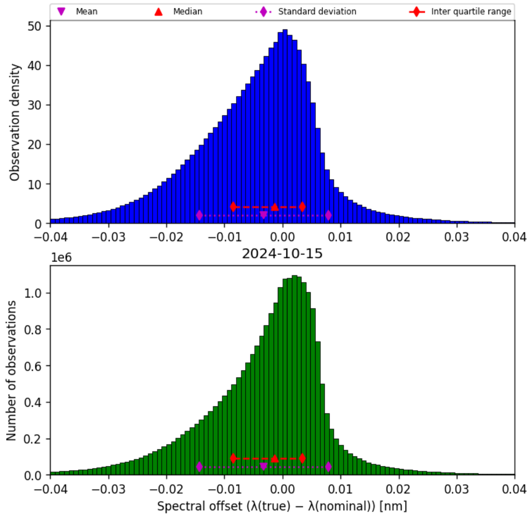
Figure 45: Histogram of “Spectral offset ( \lambda_{\text{true}} - \lambda_{\text{nominal}} )” for 2024-10-14 to 2024-10-16
