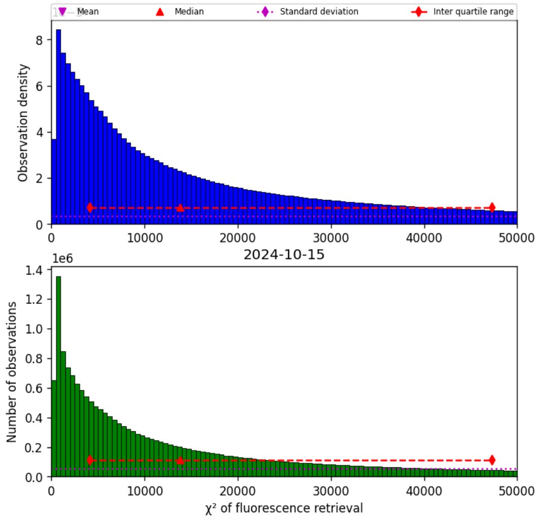
Figure 42: Histogram of “ \chi^2 of fluorescence retrieval” for 2024-10-14 to 2024-10-16
