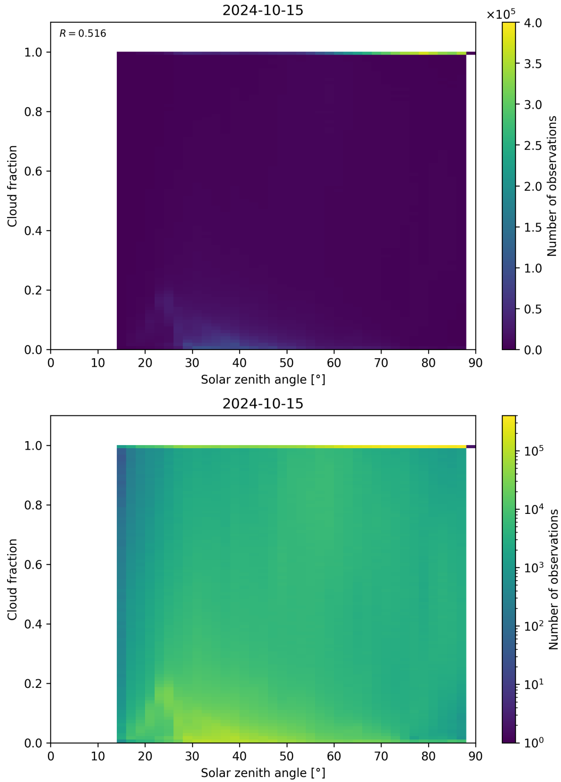
Figure 121: Scatter density plot of “Solar zenith angle” against “Cloud fraction” for 2024-10-14 to 2024-10-16.
