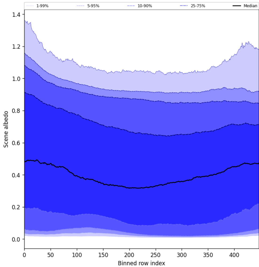
Figure 51: Along track statistics of “Scene albedo” for 2024-10-14 to 2024-10-16
