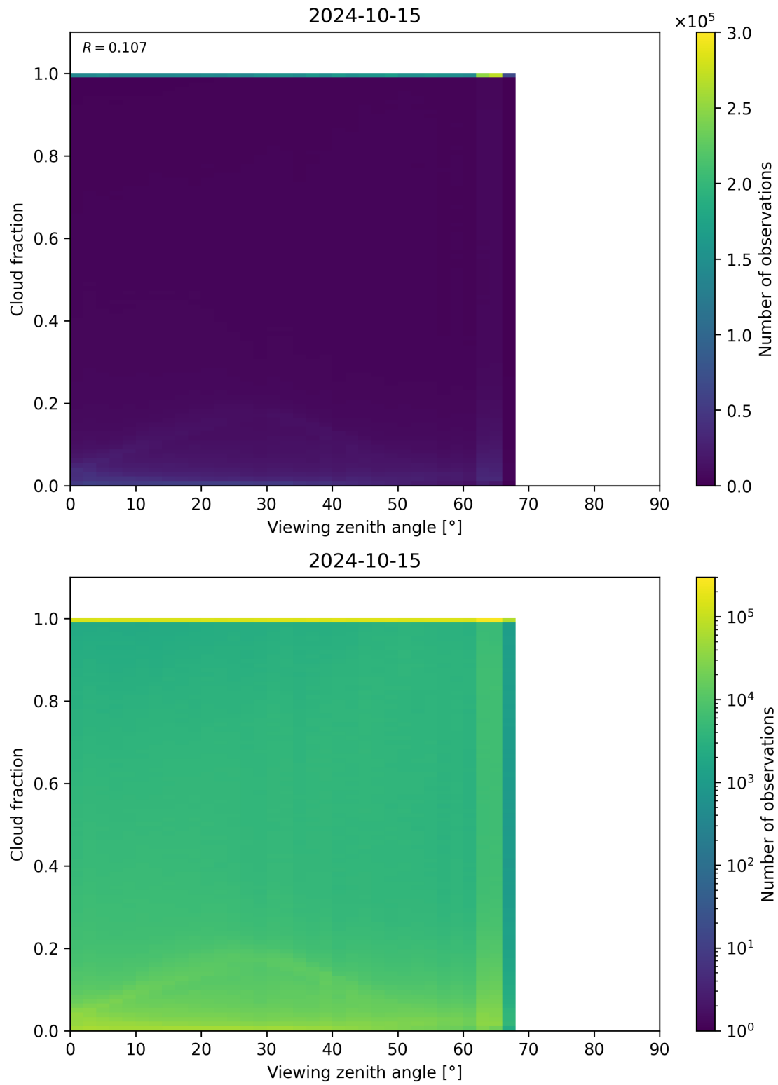
Figure 132: Scatter density plot of “Viewing zenith angle” against “Cloud fraction” for 2024-10-14 to 2024-10-16.
