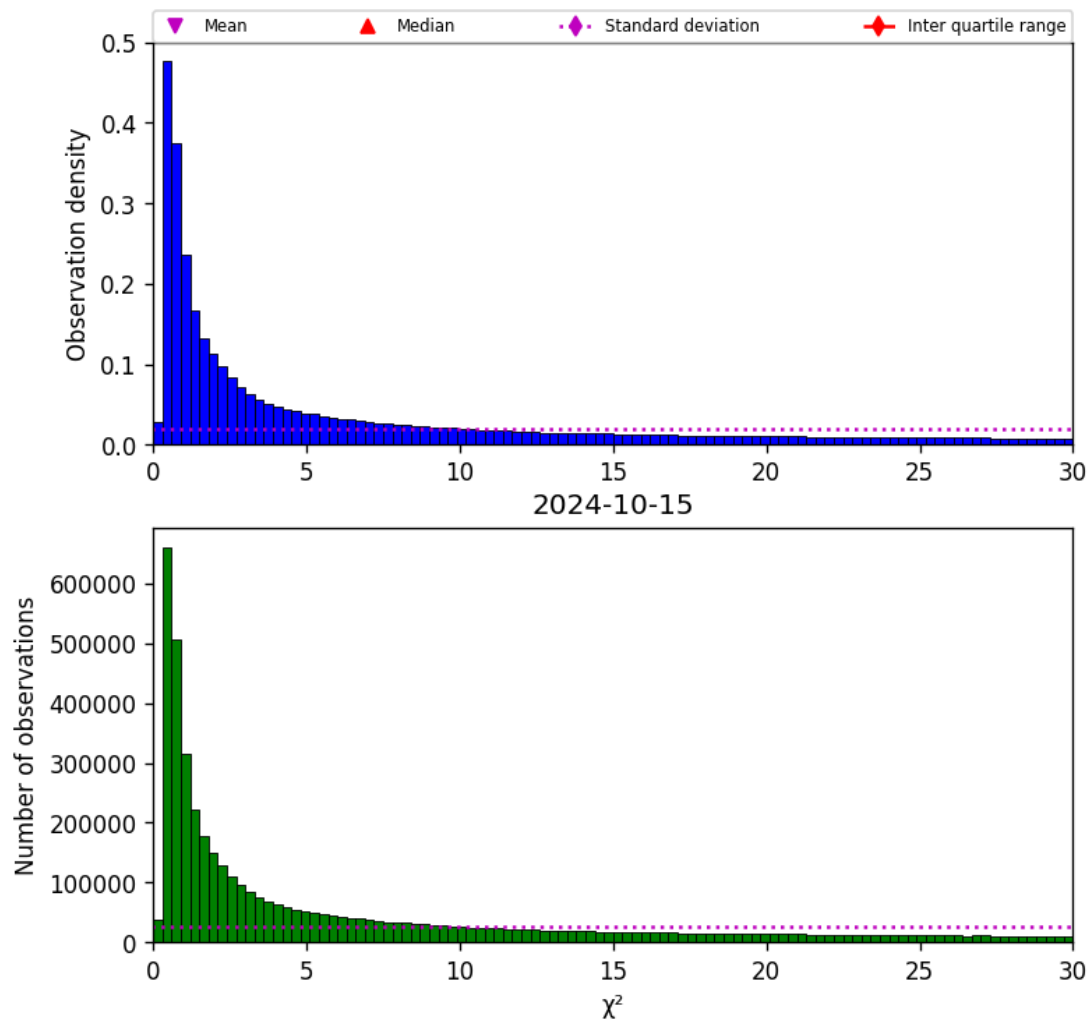
Figure 38: Histogram of “ \chi^2 ” for 2024-10-14 to 2024-10-16
