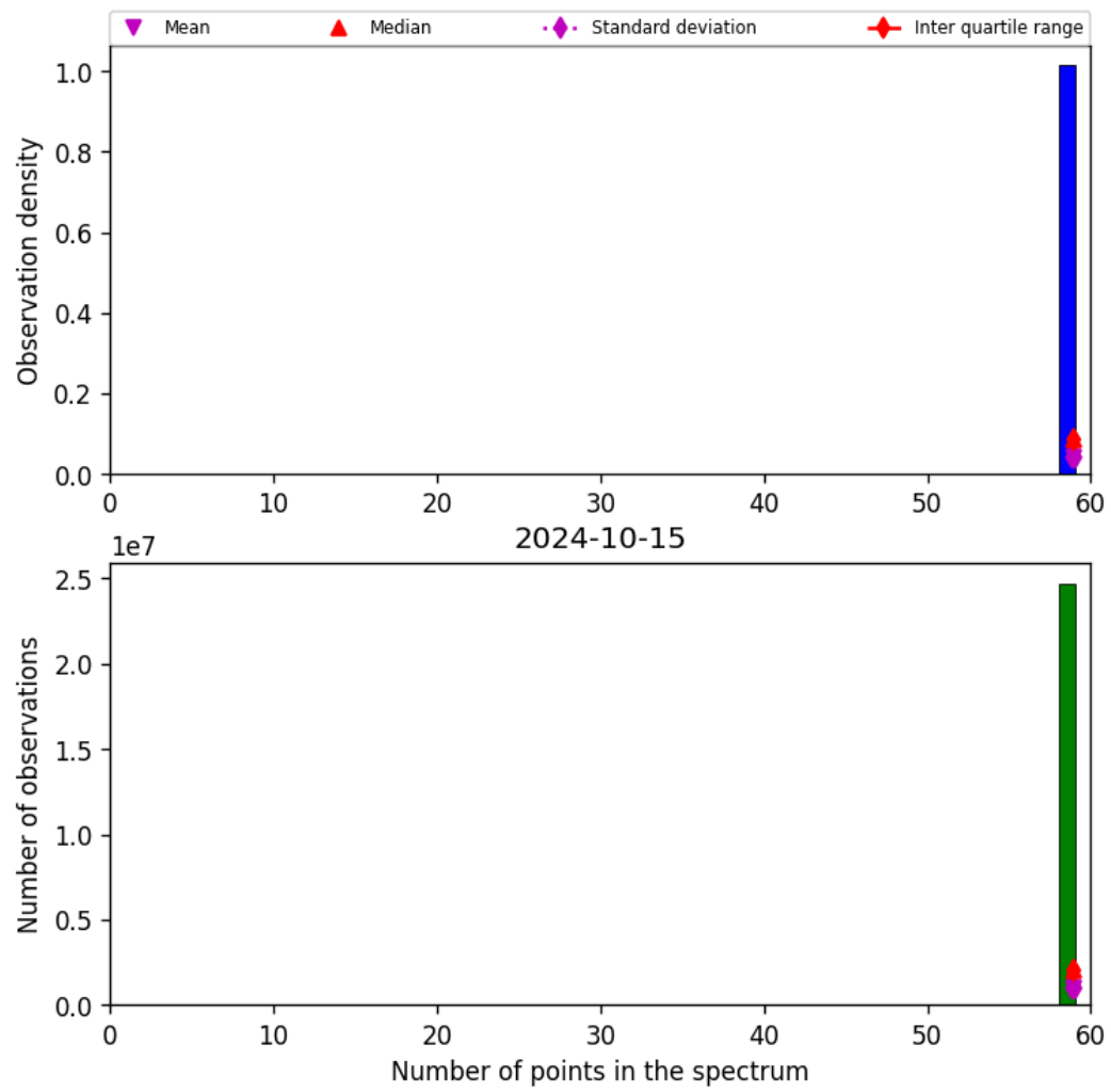
Figure 44: Histogram of “Number of points in the spectrum” for 2024-10-14 to 2024-10-16
