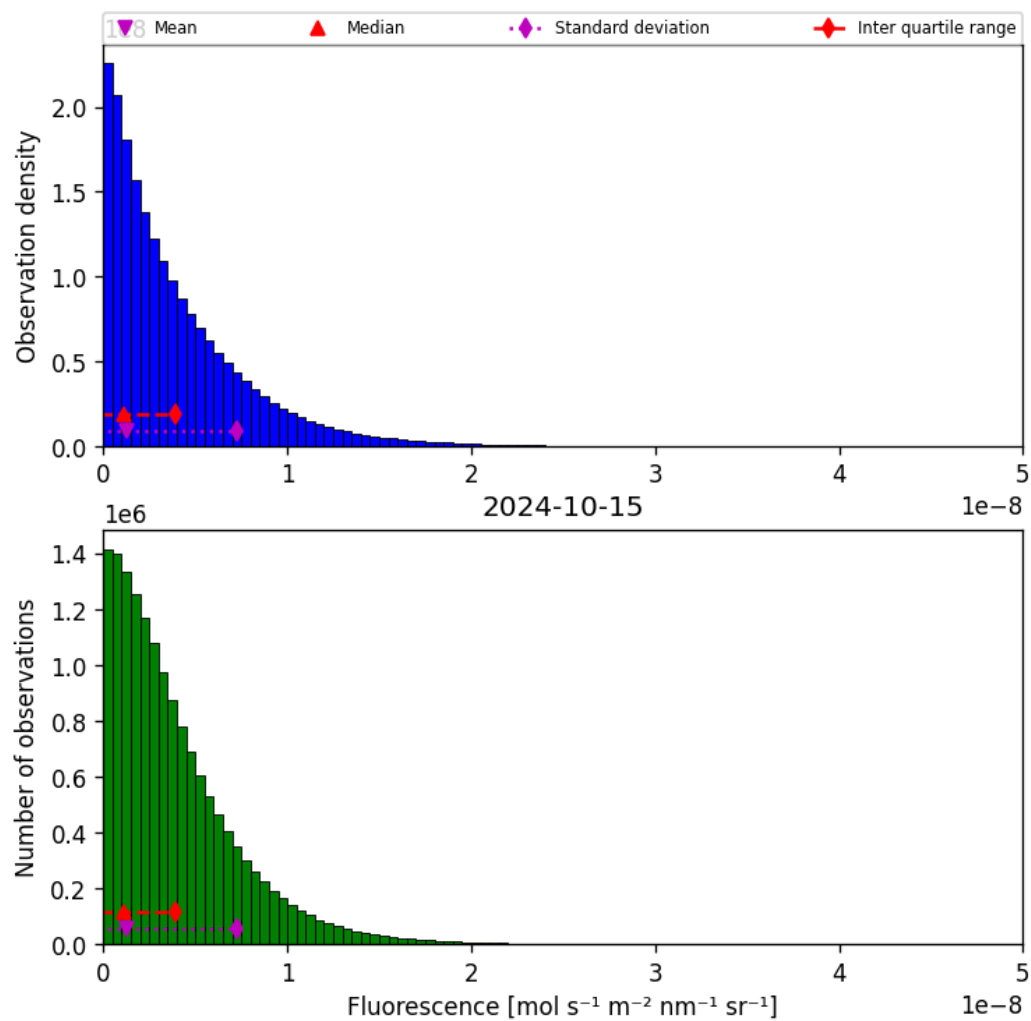
Figure 40: Histogram of “Fluorescence” for 2024-10-14 to 2024-10-16
