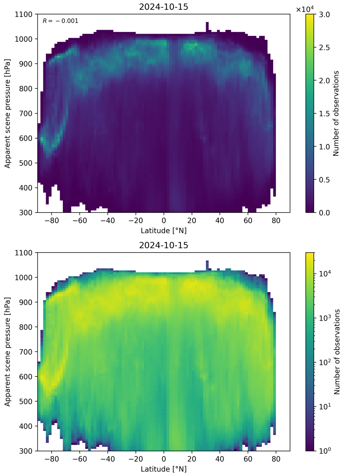
Figure 96: Scatter density plot of “Latitude” against “Apparent scene pressure” for 2024-10-14 to 2024-10-16.
