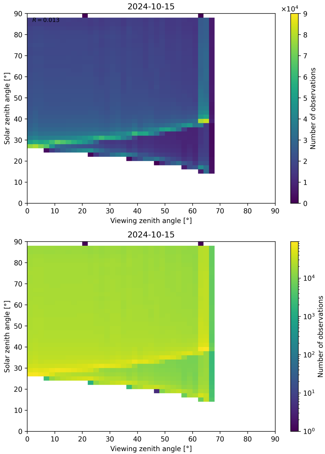
Figure 139: Scatter density plot of “Viewing zenith angle” against “Solar zenith angle” for 2024-10-14 to 2024-10-16.
