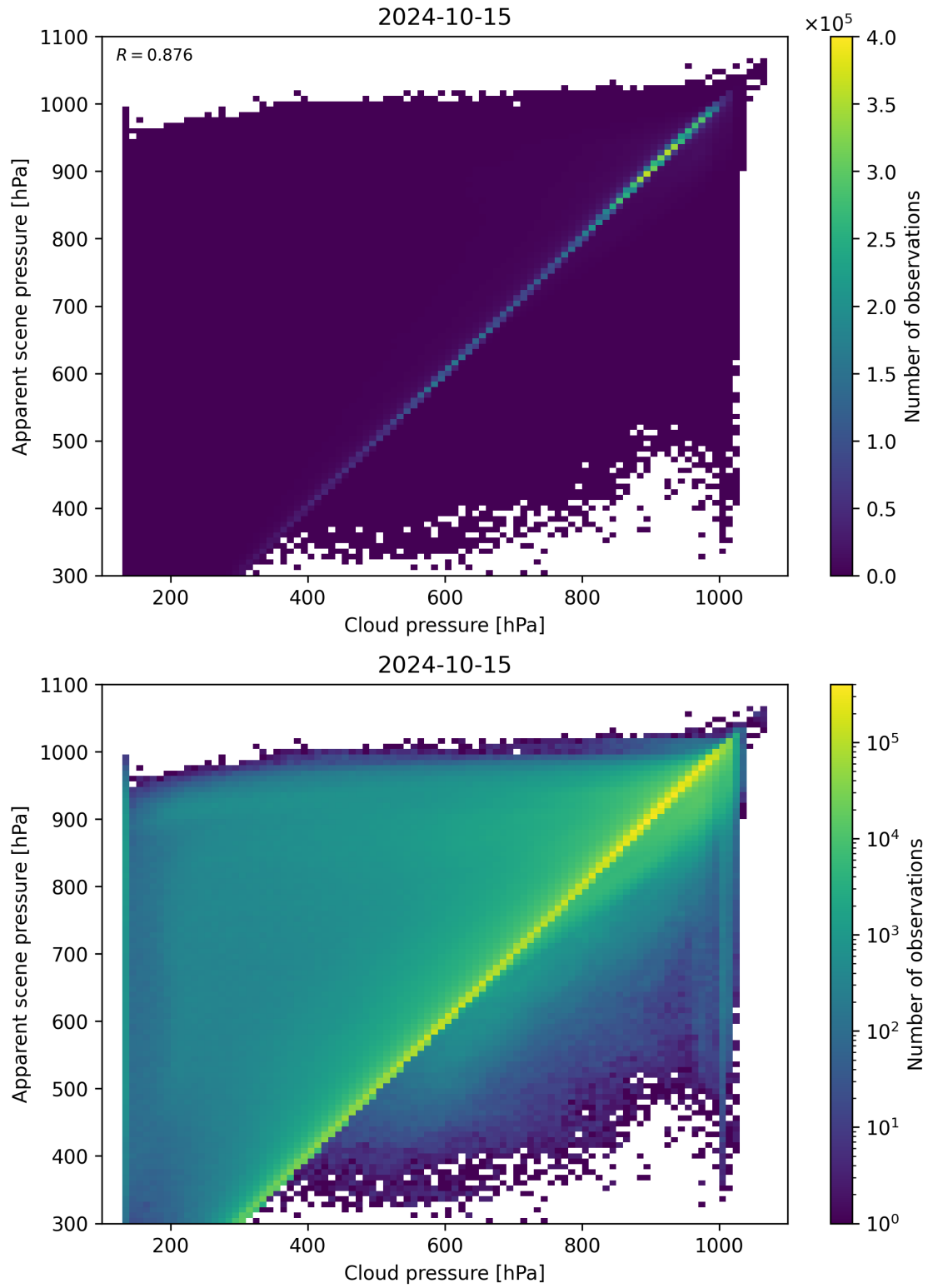
Figure 84: Scatter density plot of “Cloud pressure” against “Apparent scene pressure” for 2024-10-14 to 2024-10-16.
