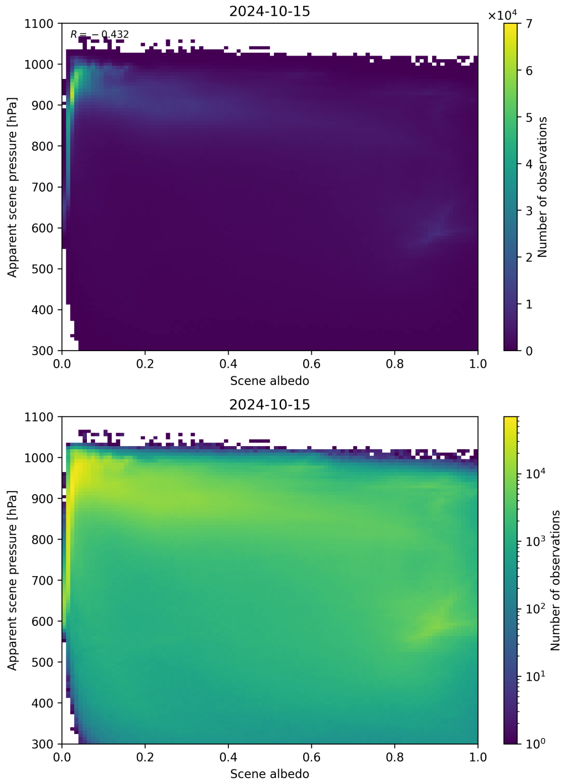
Figure 111: Scatter density plot of “Scene albedo” against “Apparent scene pressure” for 2024-10-14 to 2024-10-16.
