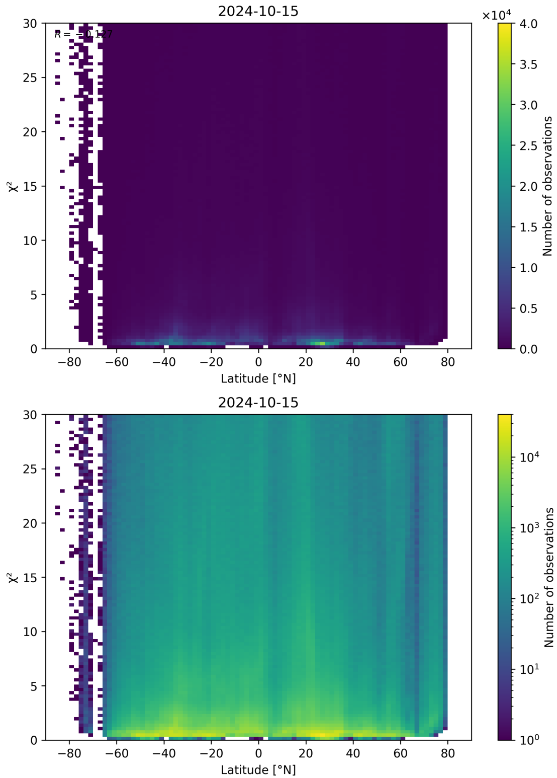
Figure 97: Scatter density plot of “Latitude” against “ \chi^2 ” for 2024-10-14 to 2024-10-16.
