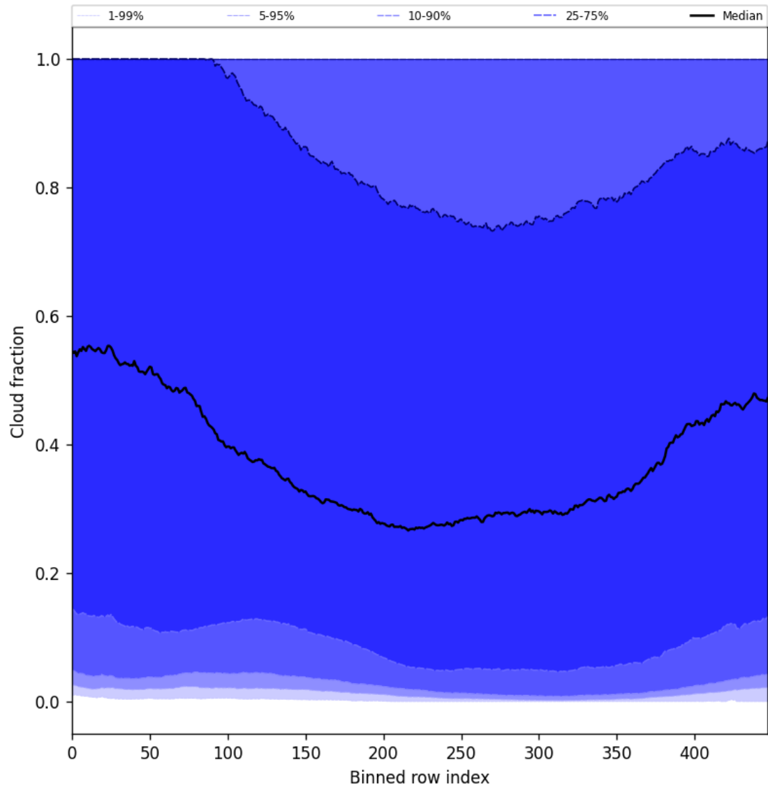
Figure 49: Along track statistics of “Cloud fraction” for 2024-10-14 to 2024-10-16
