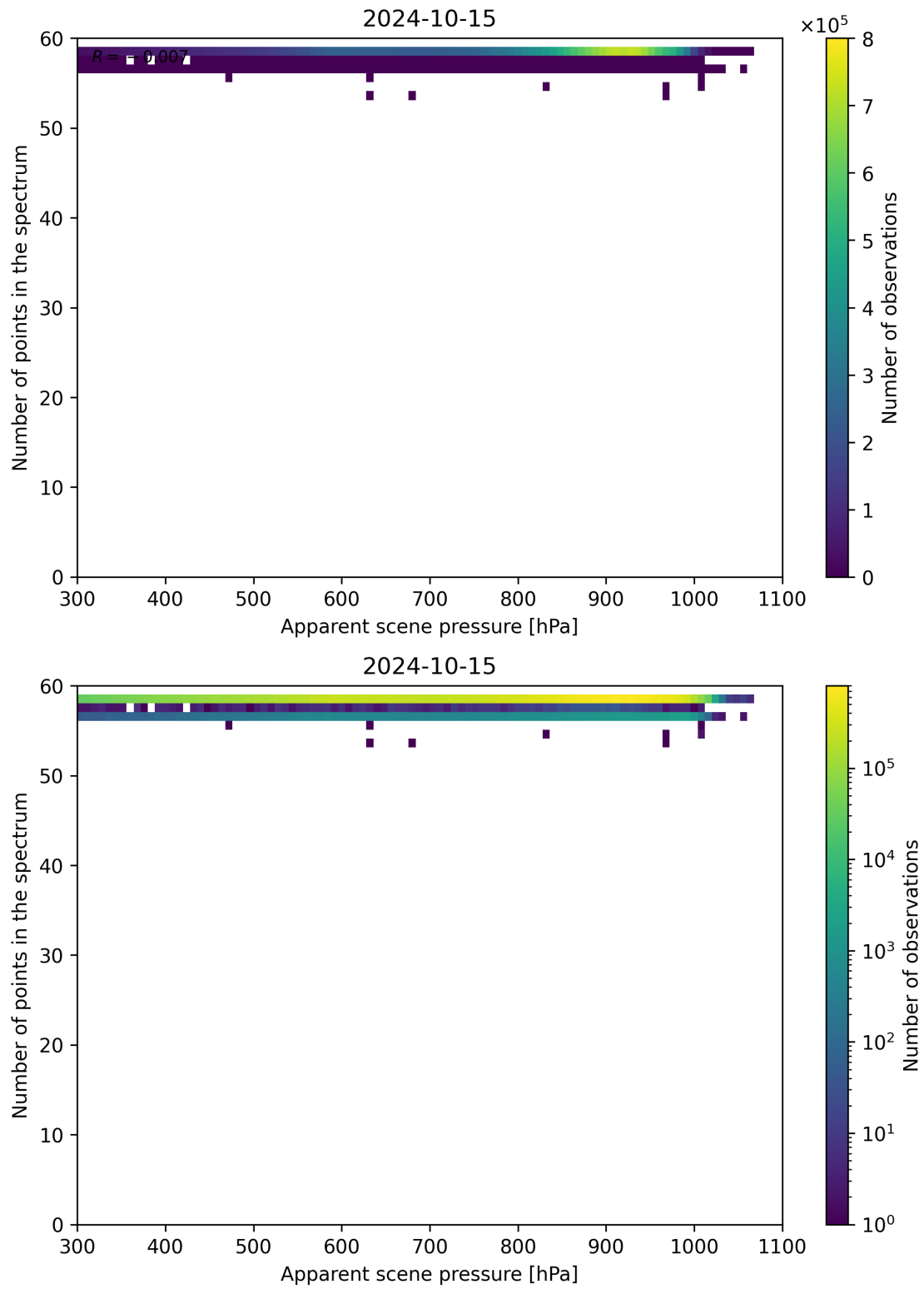
Figure 67: Scatter density plot of “Apparent scene pressure” against “Number of points in the spectrum” for 2024-10-14 to 2024-10-16.
