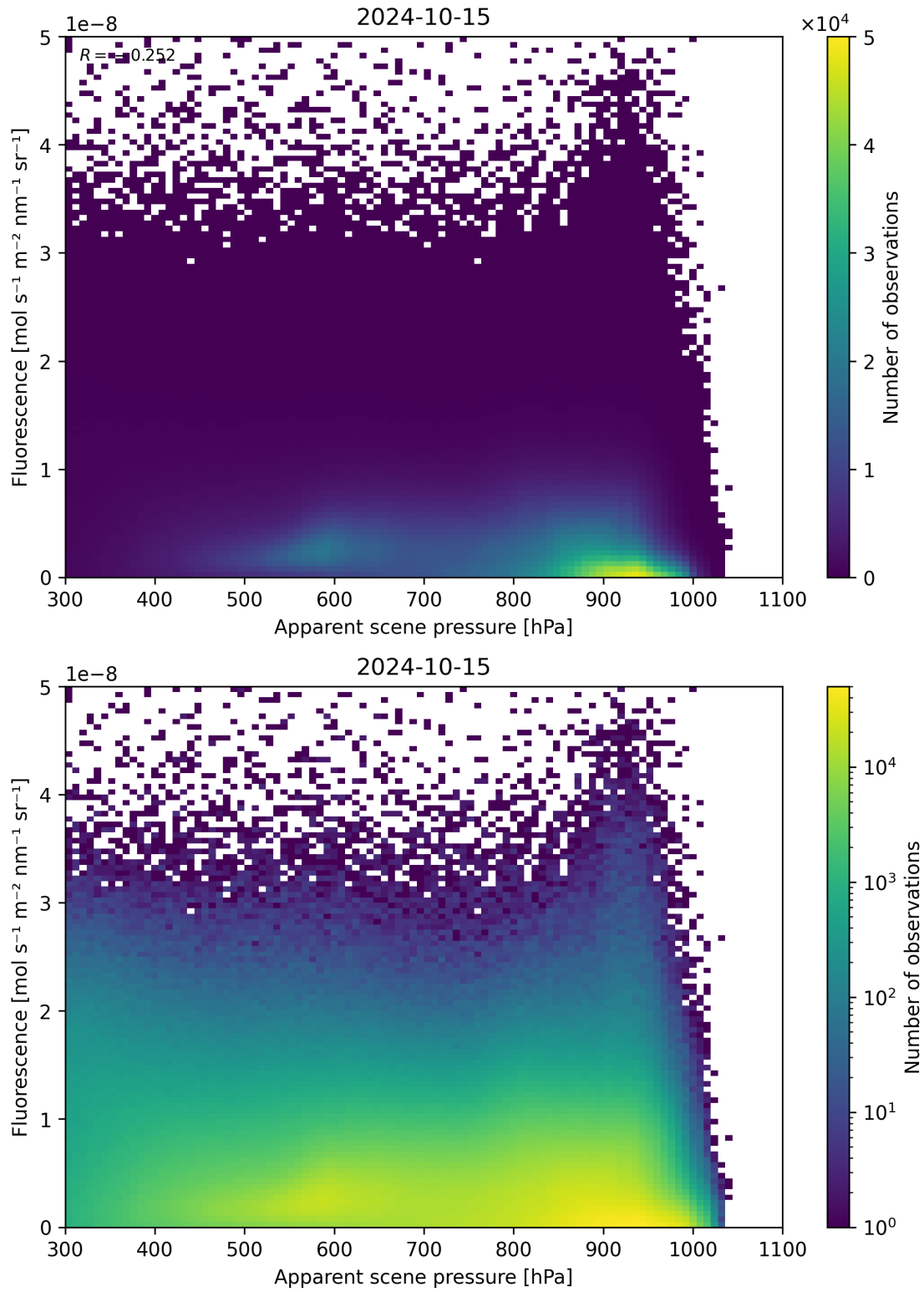
Figure 65: Scatter density plot of “Apparent scene pressure” against “Fluorescence” for 2024-10-14 to 2024-10-16.
