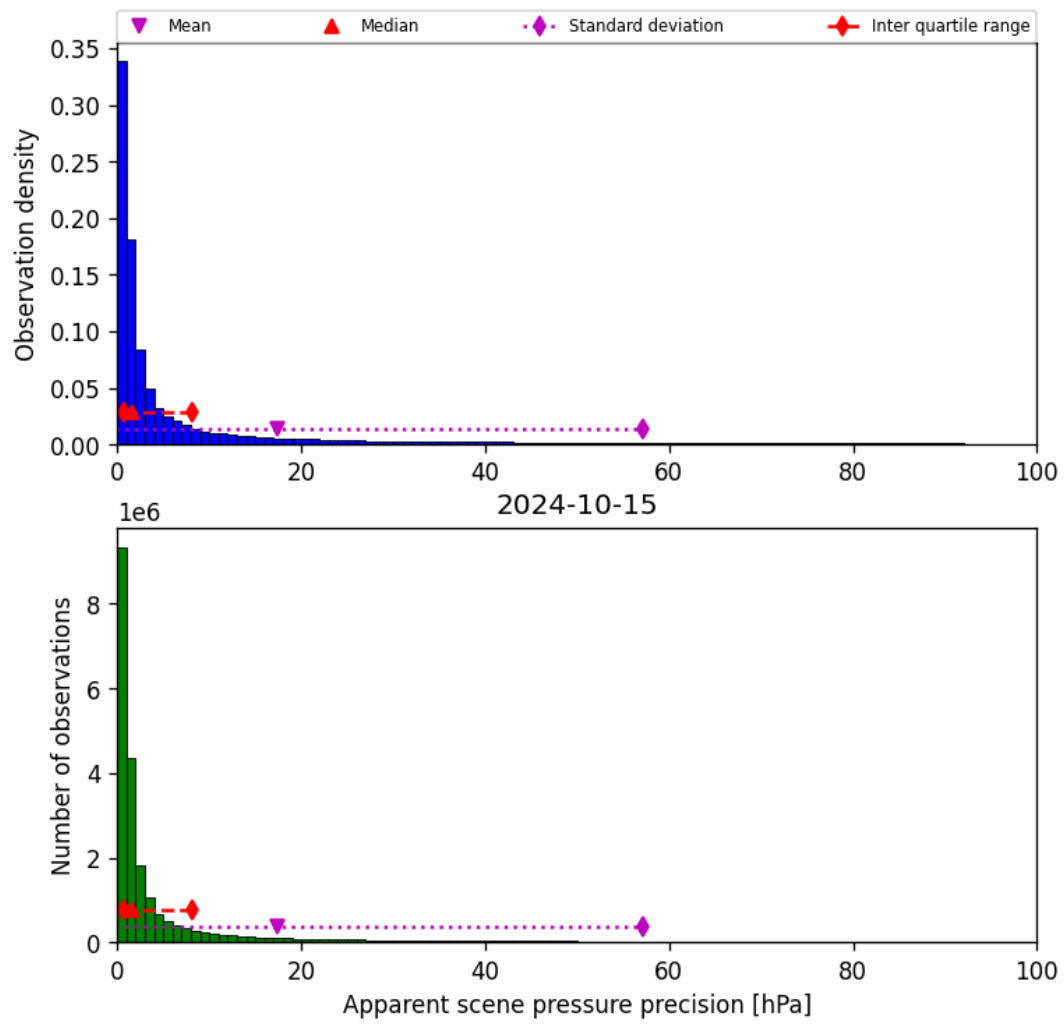
Figure 37: Histogram of “Apparent scene pressure precision” for 2024-10-14 to 2024-10-16
