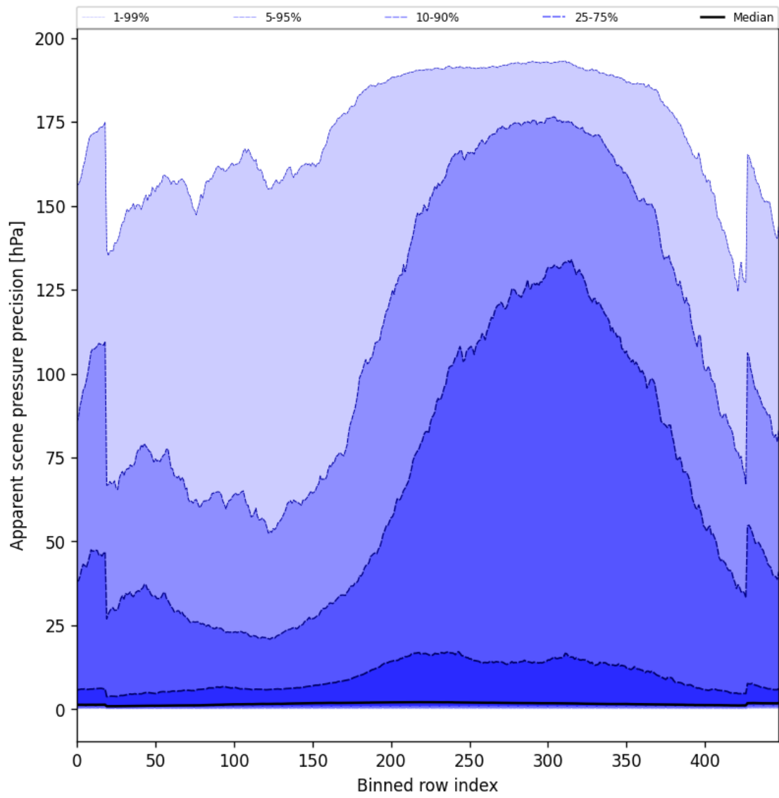
Figure 54: Along track statistics of “Apparent scene pressure precision” for 2024-10-14 to 2024-10-16
