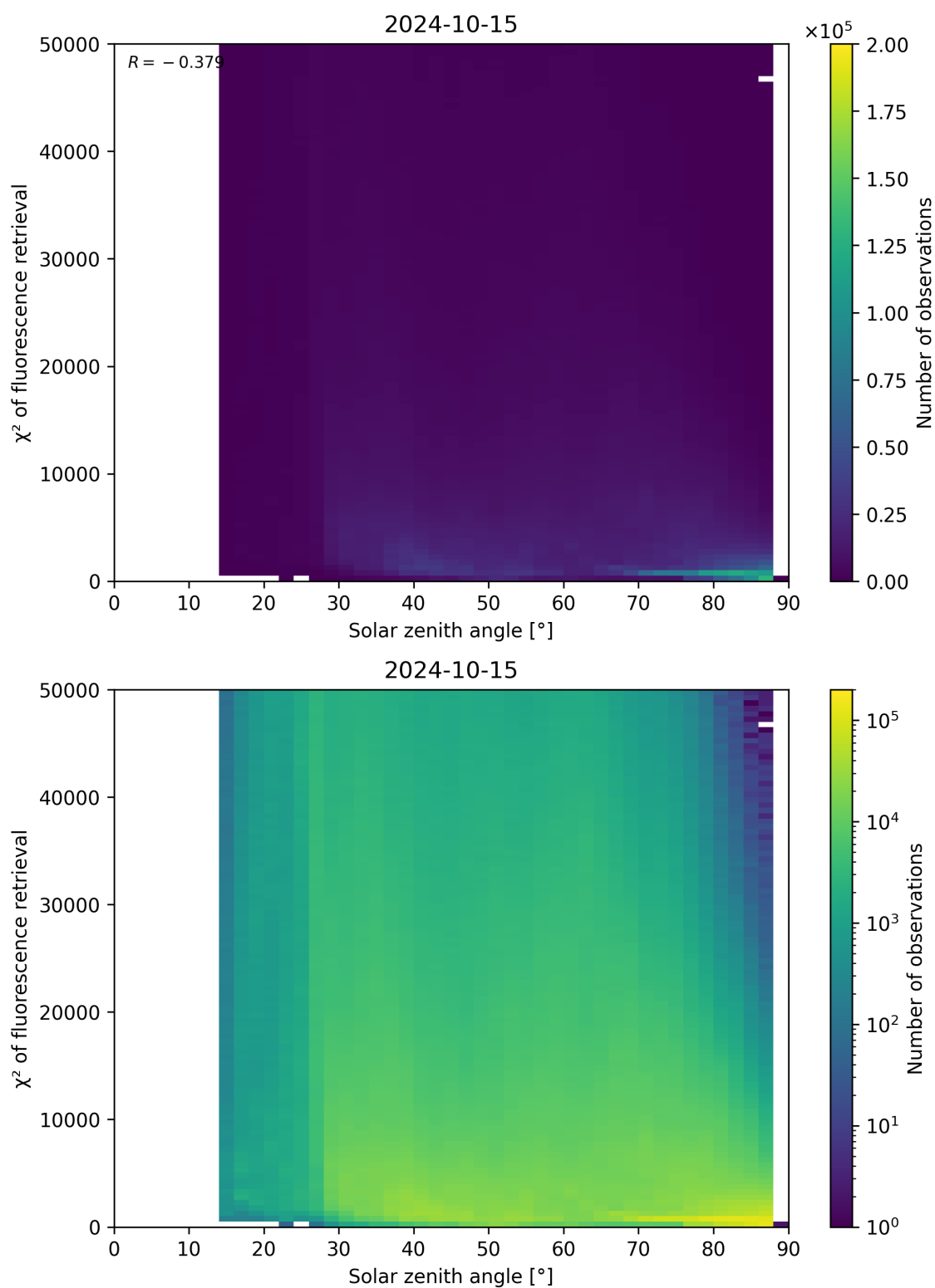
Figure 120: Scatter density plot of “Solar zenith angle” against “ \chi^2 of fluorescence retrieval” for 2024-10-14 to 2024-10-16.
