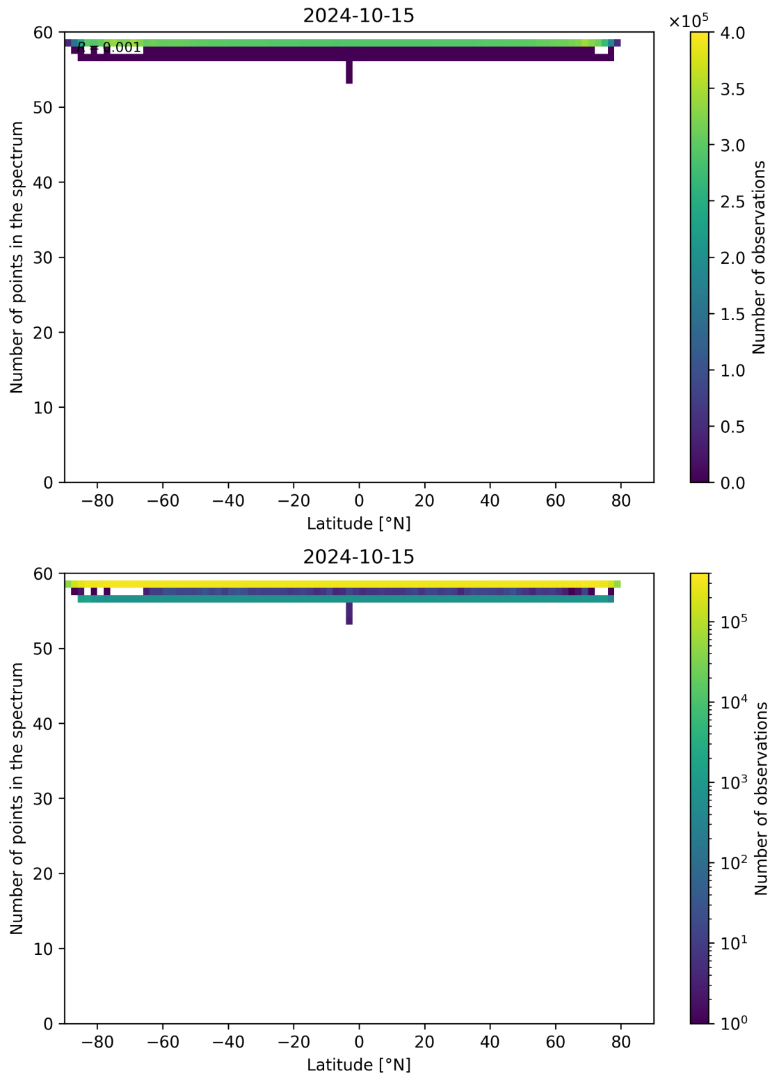
Figure 103: Scatter density plot of “Latitude” against “Number of points in the spectrum” for 2024-10-14 to 2024-10-16.
