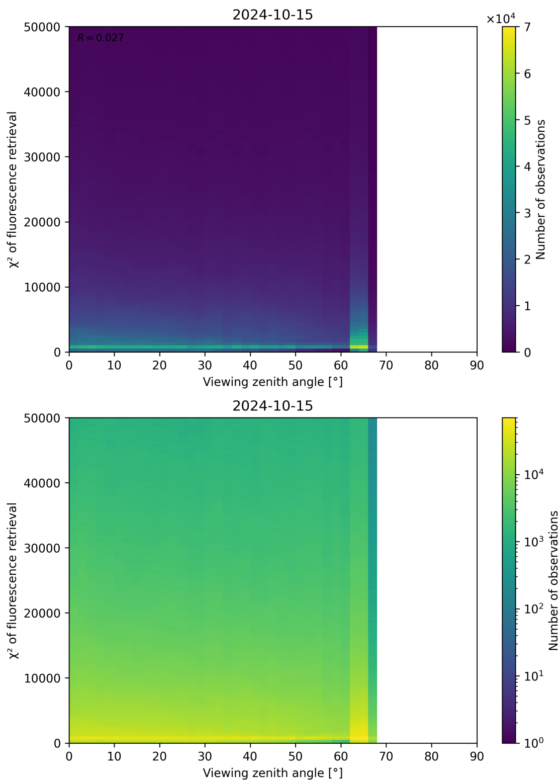
Figure 131: Scatter density plot of “Viewing zenith angle” against “ \chi^2 of fluorescence retrieval” for 2024-10-14 to 2024-10-16.
