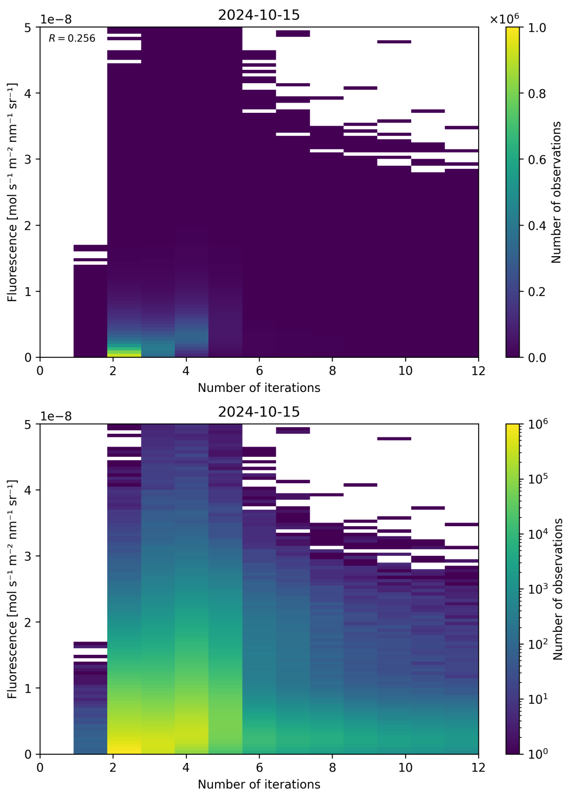
Figure 107: Scatter density plot of “Number of iterations” against “Fluorescence” for 2024-10-14 to 2024-10-16.
