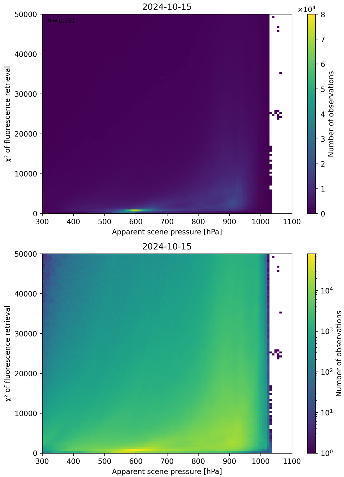
Figure 64: Scatter density plot of “Apparent scene pressure” against “ \chi^2 of fluorescence retrieval” for 2024-10-14 to 2024-10-16.
