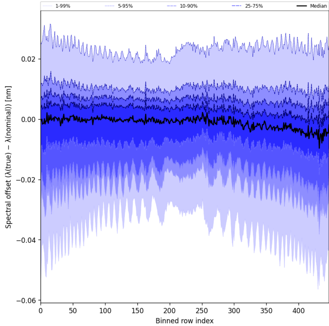
Figure 62: Along track statistics of “Spectral offset ( \lambda_{\text{true}} - \lambda_{\text{nominal}} )” for 2024-10-14 to 2024-10-16
