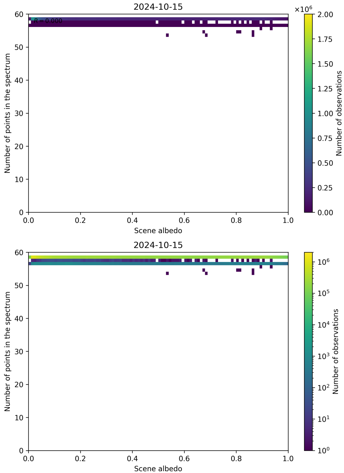
Figure 116: Scatter density plot of “Scene albedo” against “Number of points in the spectrum” for 2024-10-14 to 2024-10-16.
