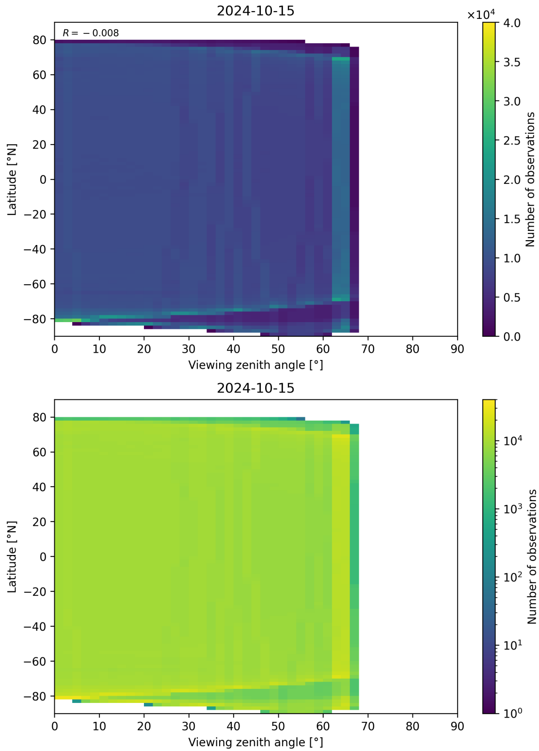
Figure 135: Scatter density plot of “Viewing zenith angle” against “Latitude” for 2024-10-14 to 2024-10-16.
