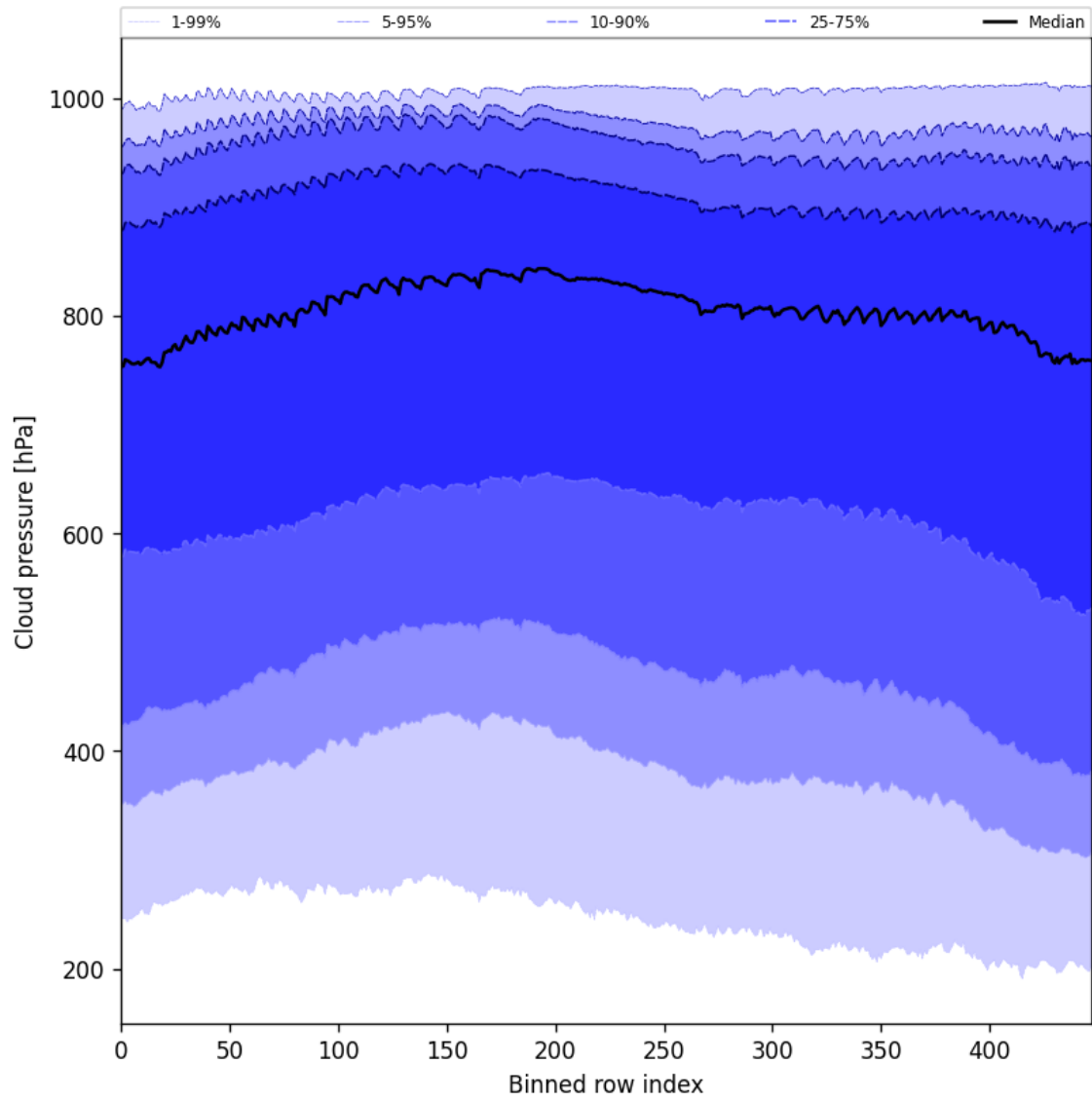
Figure 47: Along track statistics of "Cloud pressure" for 2024-10-14 to 2024-10-16
