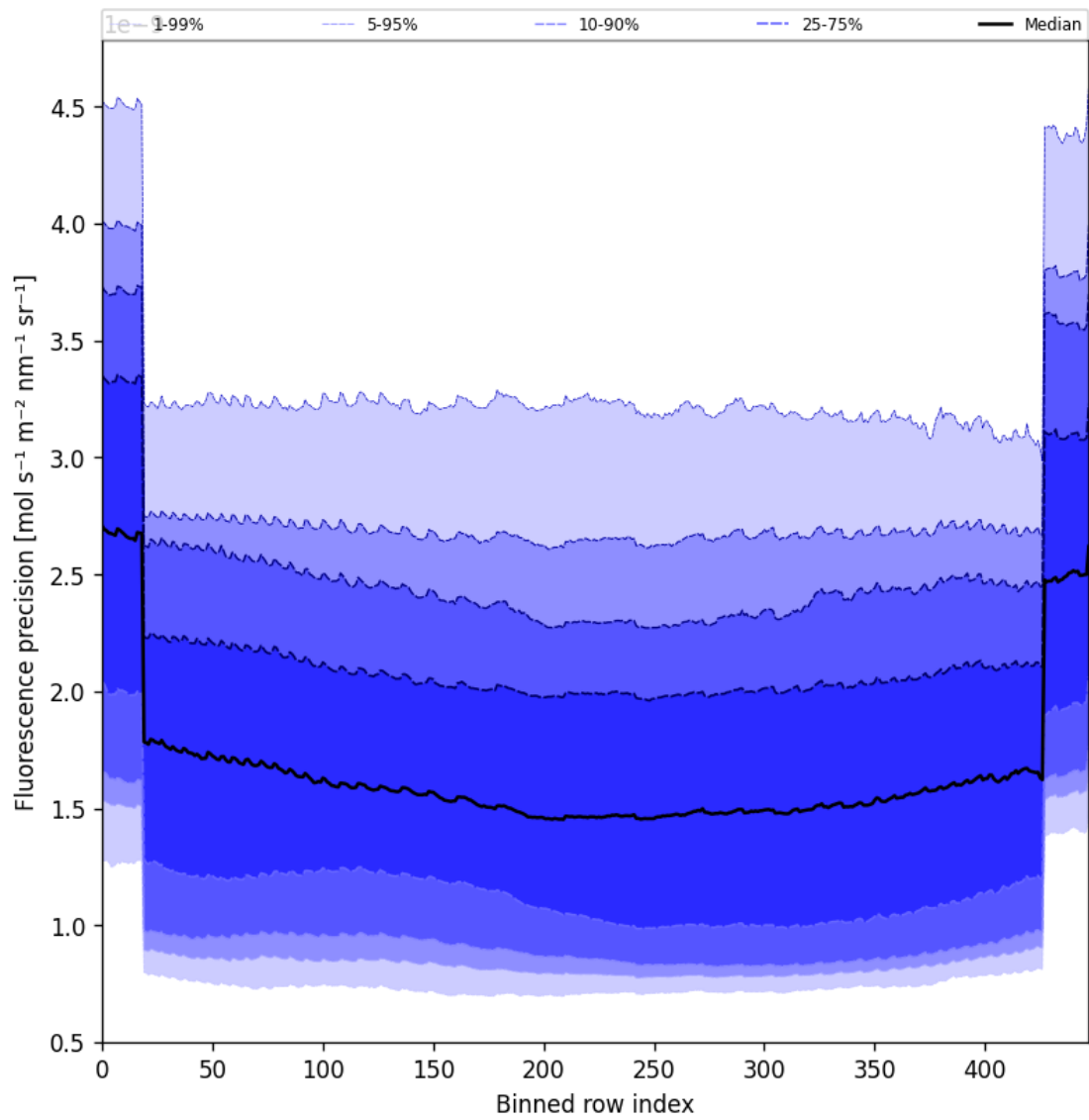
Figure 58: Along track statistics of “Fluorescence precision” for 2024-10-14 to 2024-10-16
