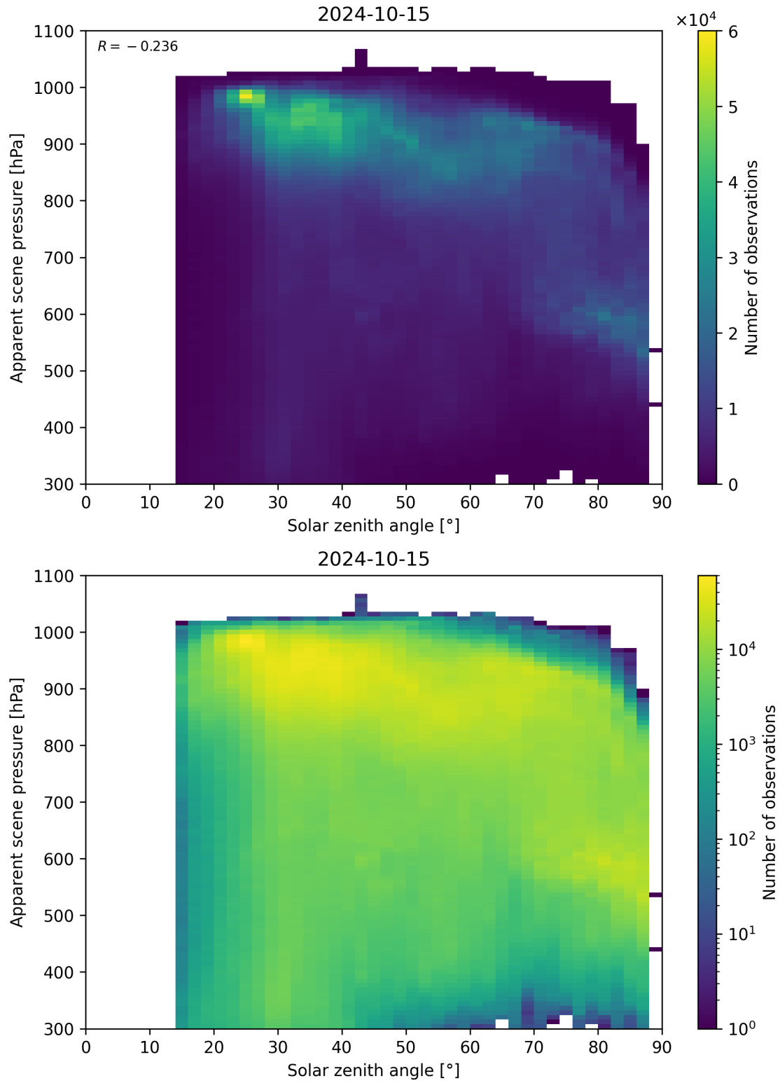
Figure 118: Scatter density plot of “Solar zenith angle” against “Apparent scene pressure” for 2024-10-14 to 2024-10-16.
