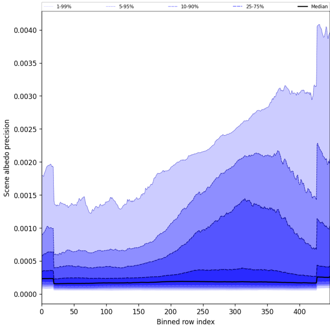
Figure 52: Along track statistics of “Scene albedo precision” for 2024-10-14 to 2024-10-16
