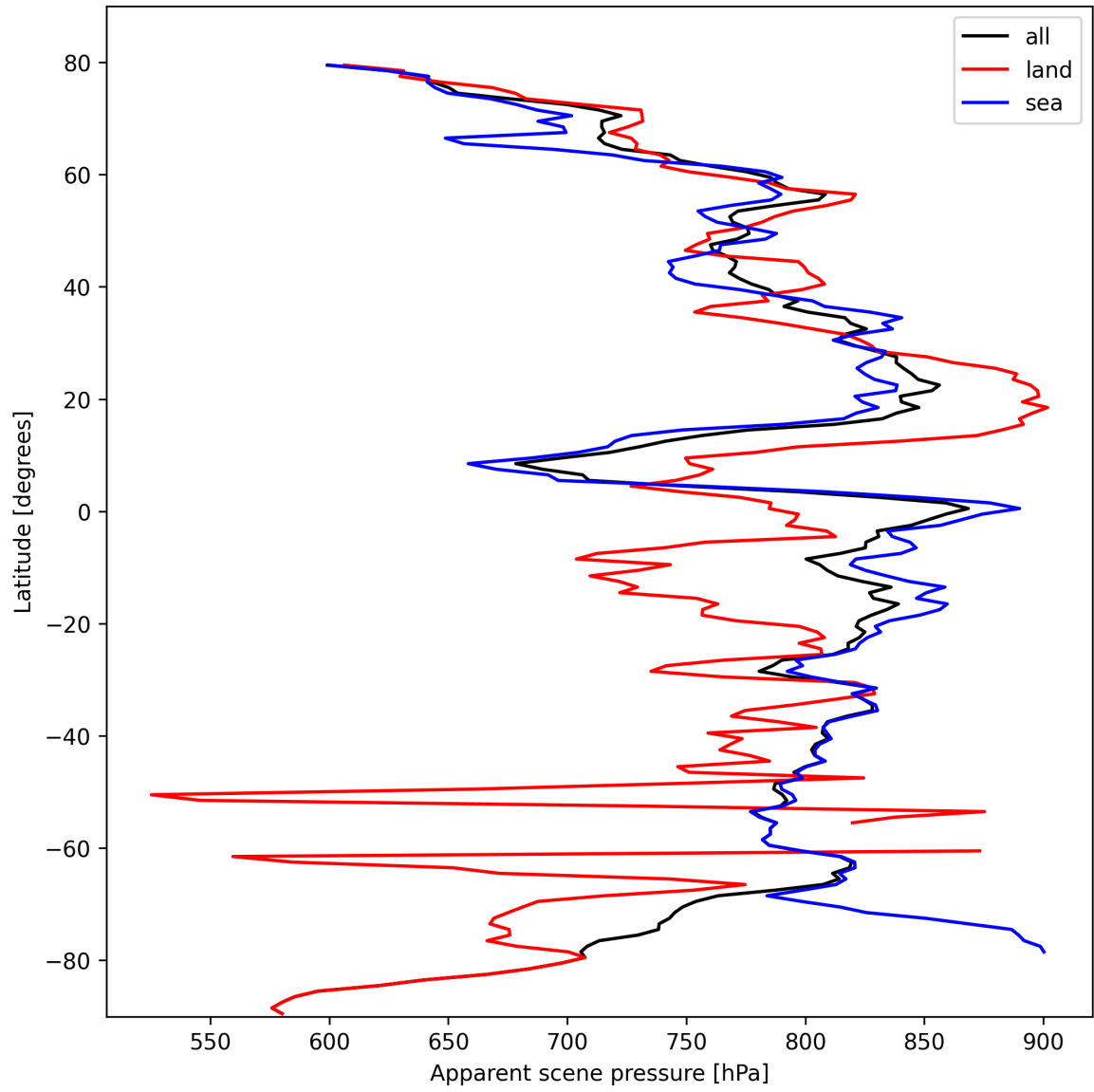
Figure 19: Zonal average of “Apparent scene pressure” for 2024-10-14 to 2024-10-16.
