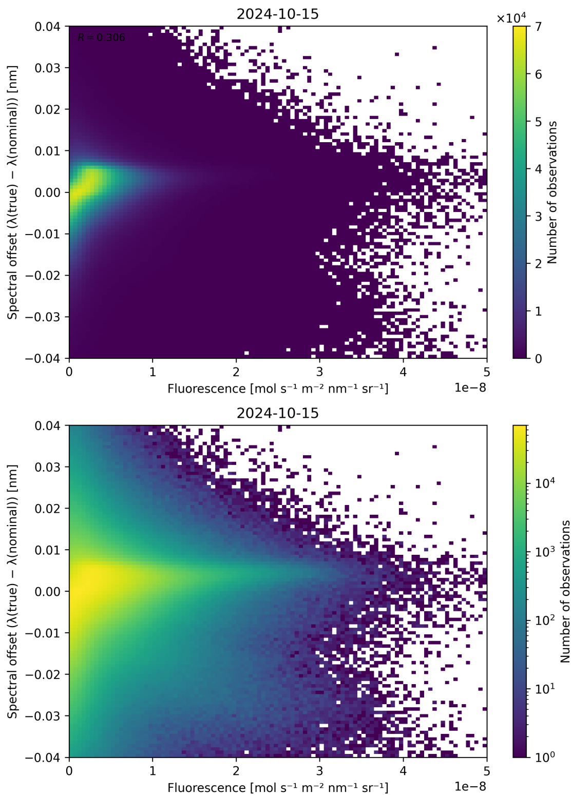
Figure 95: Scatter density plot of “Fluorescence” against “Spectral offset ( \lambda_{\text{true}} - \lambda_{\text{nominal}} )” for 2024-10-14 to 2024-10-16.
