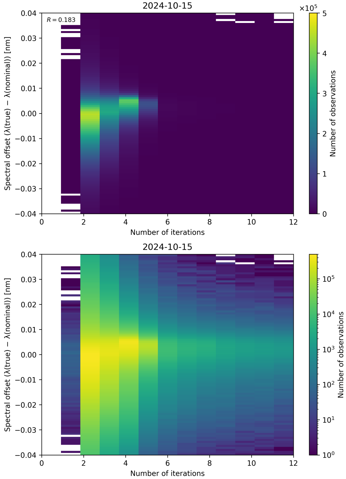
Figure 109: Scatter density plot of “Number of iterations” against “Spectral offset ( \lambda_{\text{true}} - \lambda_{\text{nominal}} )” for 2024-10-14 to 2024-10-16.
