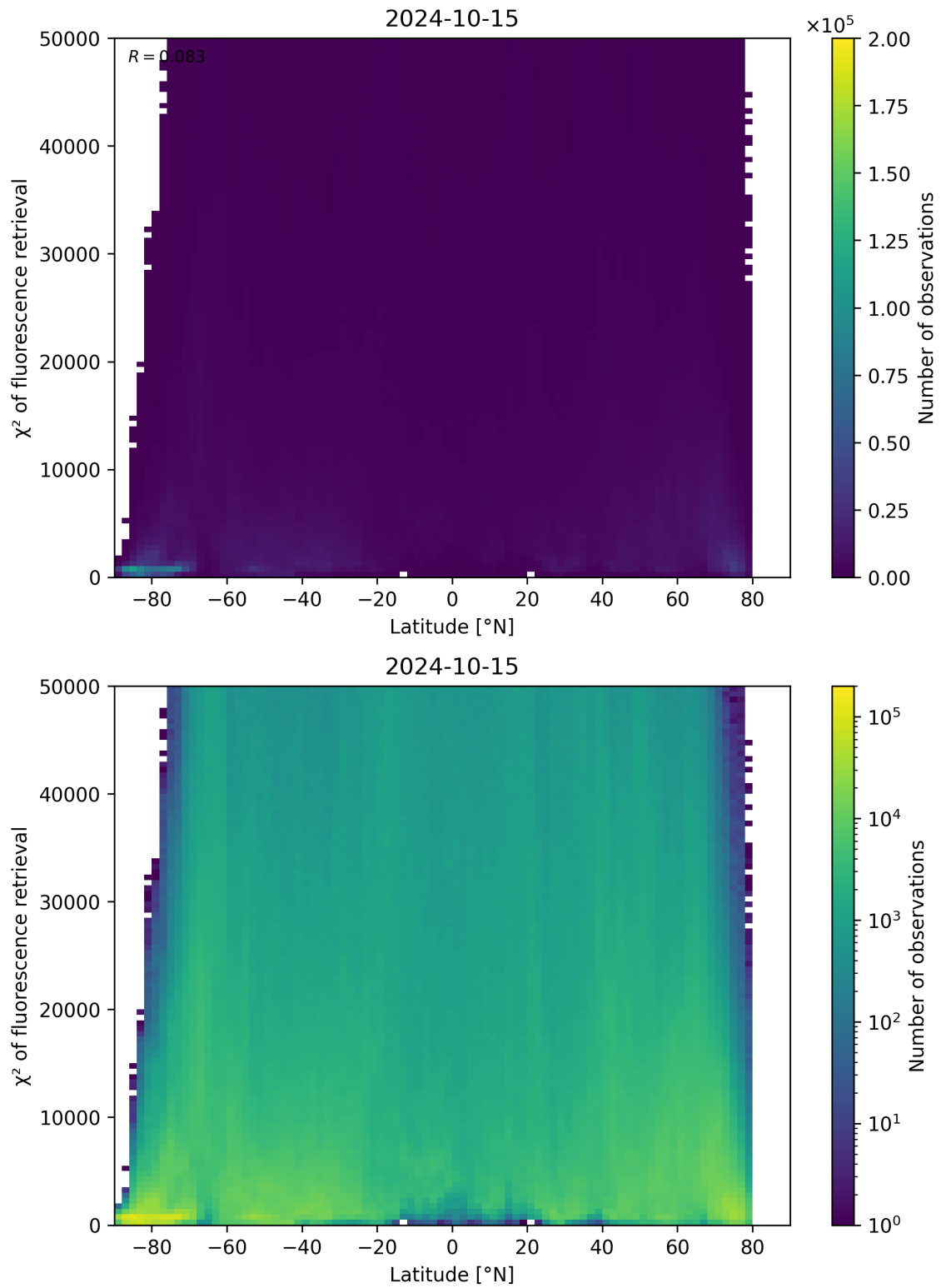
Figure 98: Scatter density plot of “Latitude” against “ \chi^2 of fluorescence retrieval” for 2024-10-14 to 2024-10-16.
