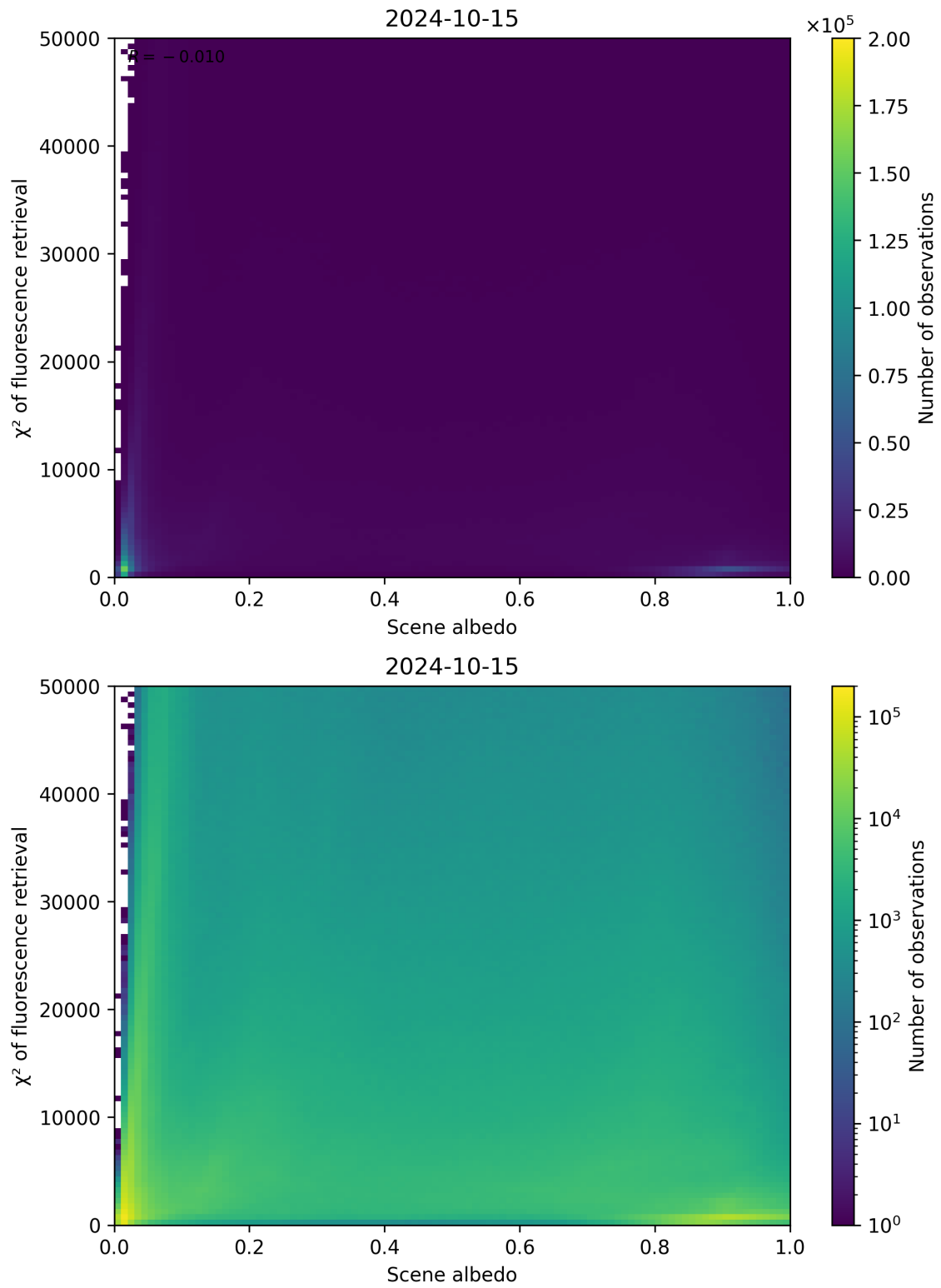
Figure 113: Scatter density plot of “Scene albedo” against “ \chi^2 of fluorescence retrieval” for 2024-10-14 to 2024-10-16.
