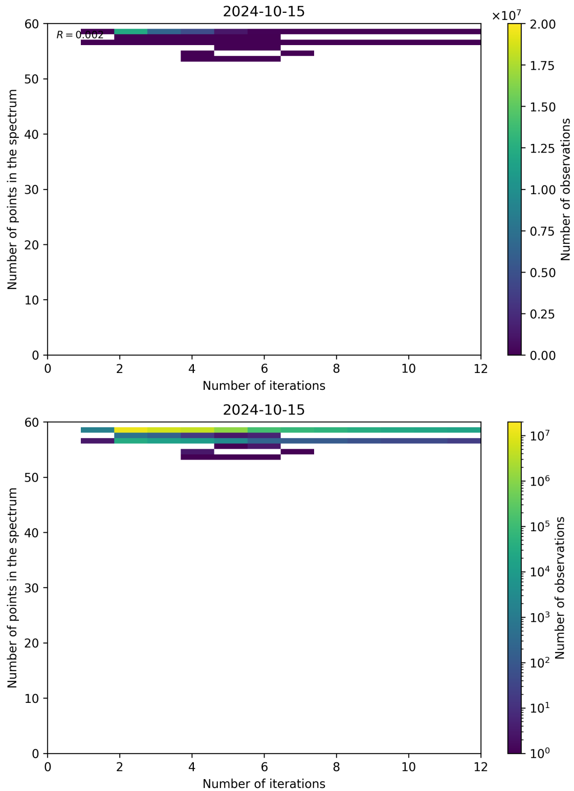
Figure 108: Scatter density plot of “Number of iterations” against “Number of points in the spectrum” for 2024-10-14 to 2024-10-16.
