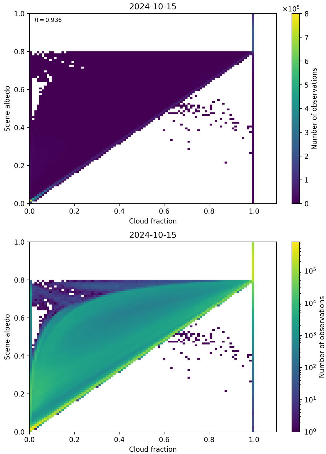
Figure 82: Scatter density plot of “Cloud fraction” against “Scene albedo” for 2024-10-14 to 2024-10-16.
