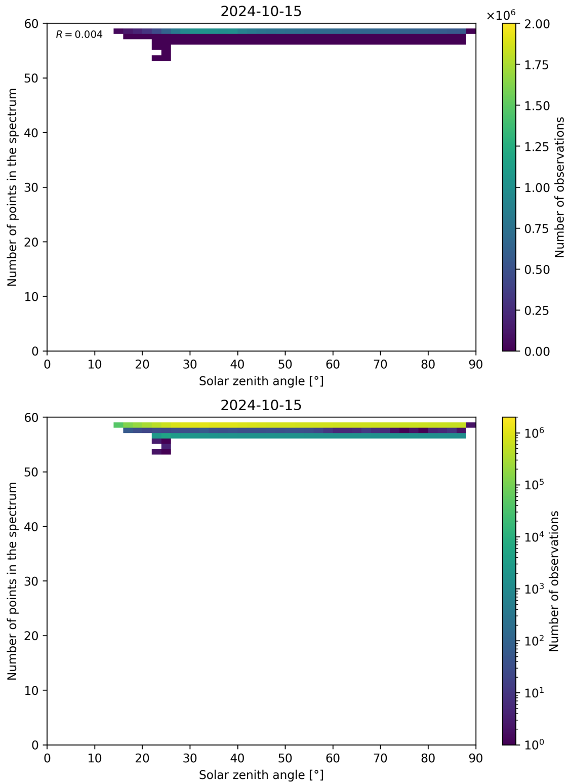
Figure 126: Scatter density plot of “Solar zenith angle” against “Number of points in the spectrum” for 2024-10-14 to 2024-10-16.
