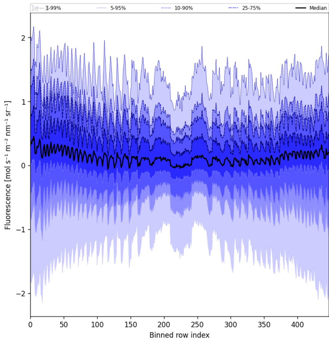
Figure 57: Along track statistics of "Fluorescence" for 2024-10-14 to 2024-10-16
