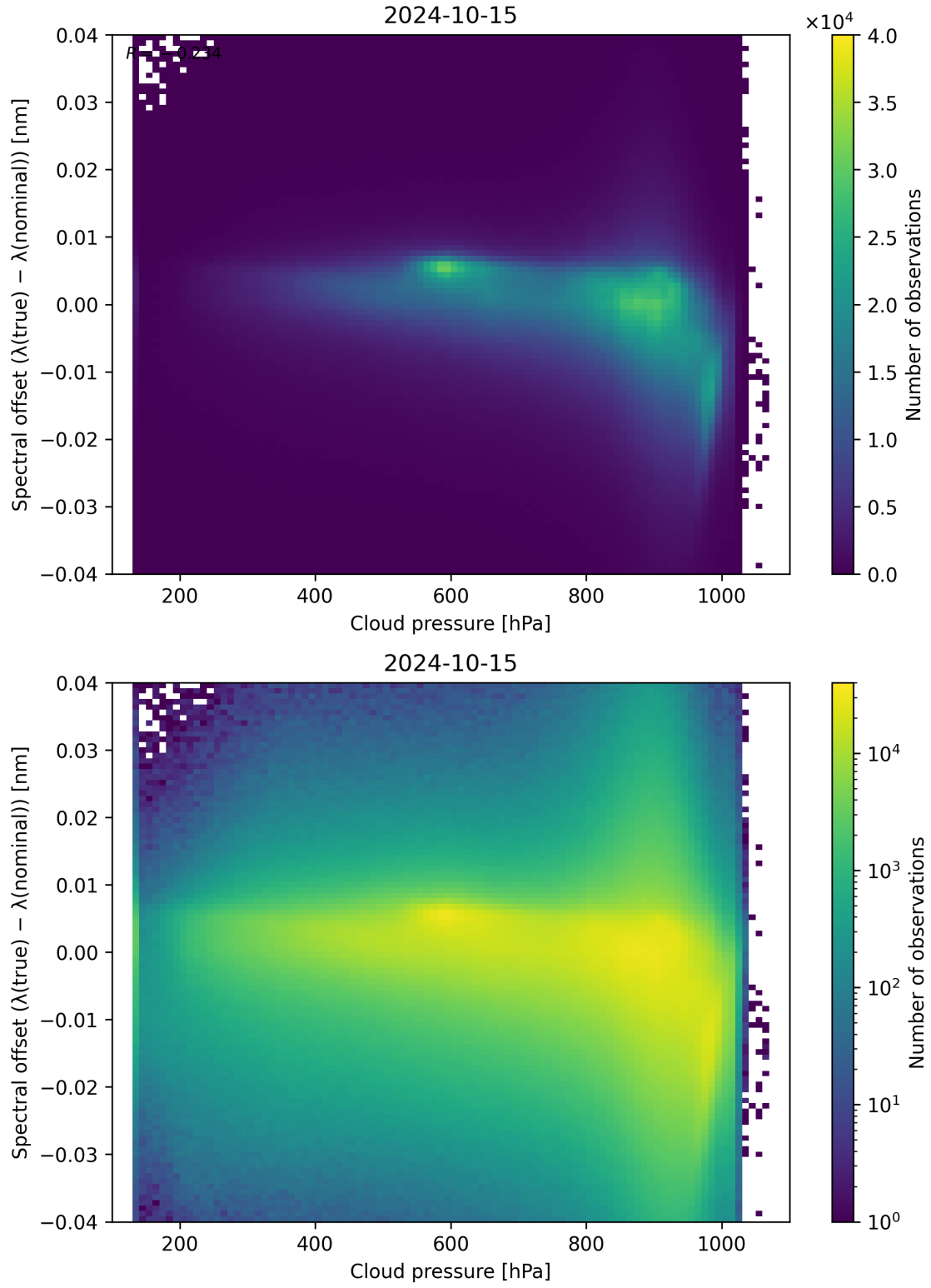
Figure 92: Scatter density plot of “Cloud pressure” against “Spectral offset ( \lambda_{\text{true}} - \lambda_{\text{nominal}} )” for 2024-10-14 to 2024-10-16.
