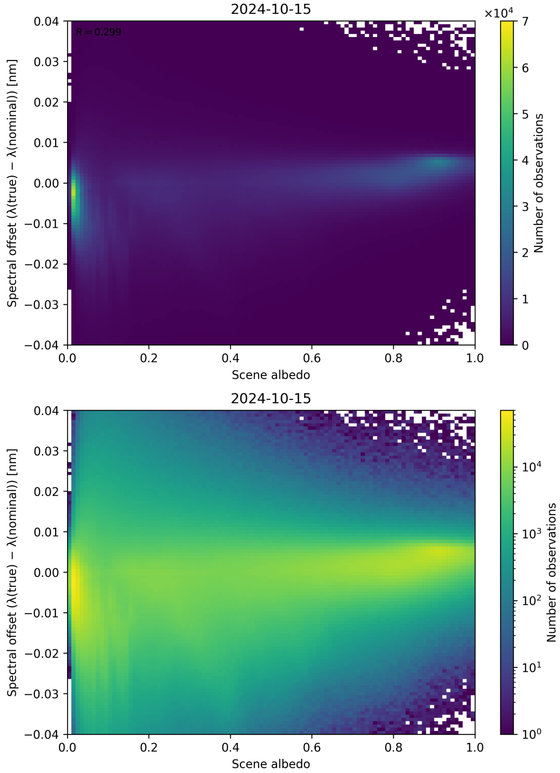
Figure 117: Scatter density plot of “Scene albedo” against “Spectral offset ( \lambda_{\text{true}} - \lambda_{\text{nominal}} )” for 2024-10-14 to 2024-10-16.
