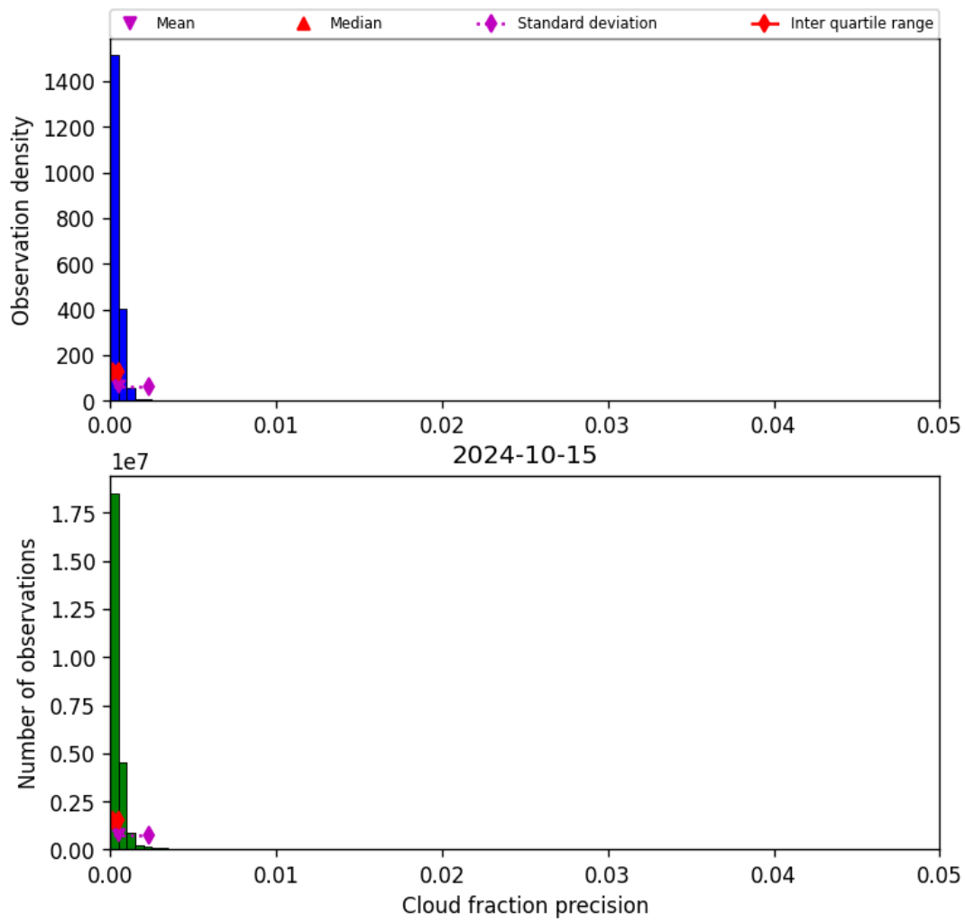
Figure 33: Histogram of “Cloud fraction precision” for 2024-10-14 to 2024-10-16
