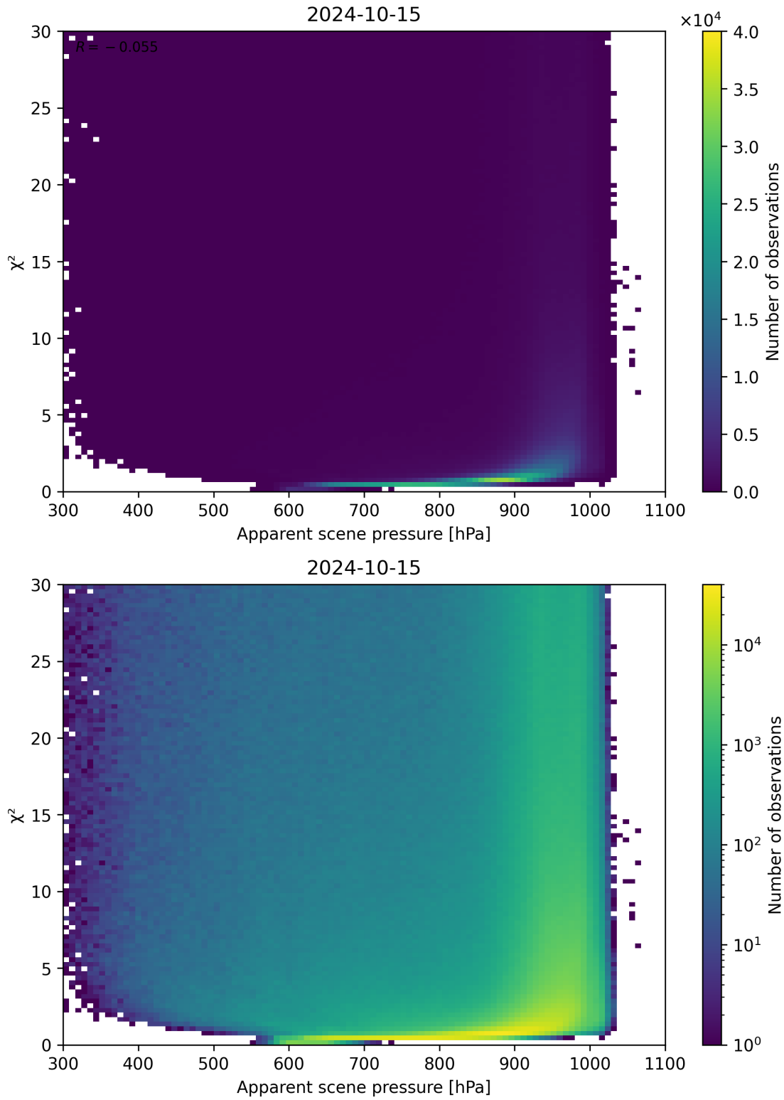
Figure 63: Scatter density plot of “Apparent scene pressure” against “ \chi^2 ” for 2024-10-14 to 2024-10-16.
