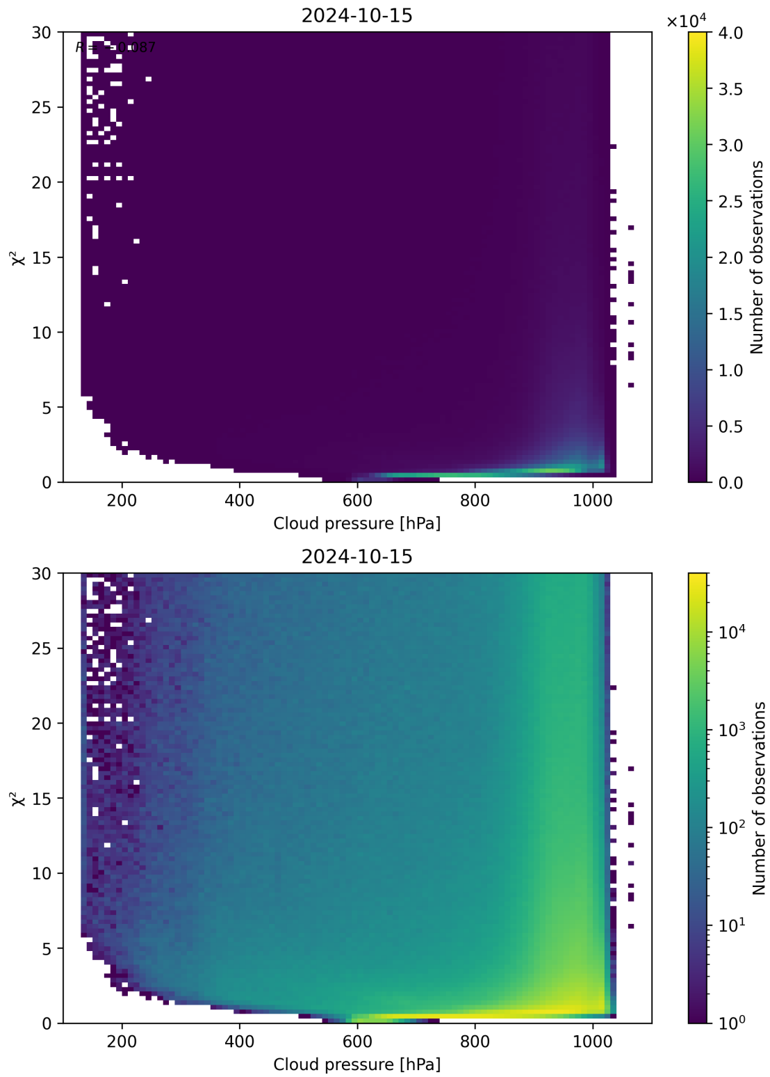
Figure 85: Scatter density plot of “Cloud pressure” against “ \chi^2 ” for 2024-10-14 to 2024-10-16.
