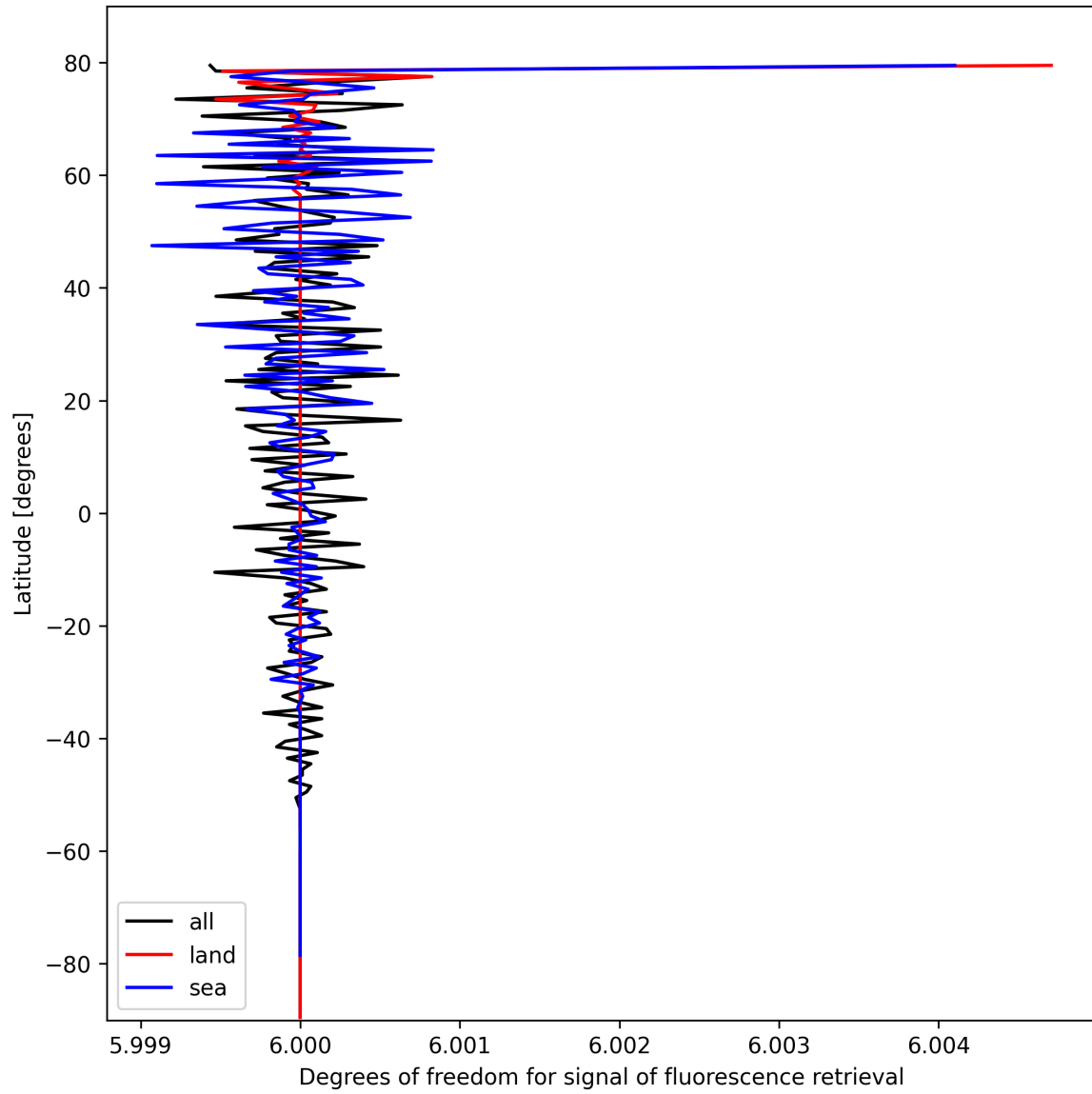
Figure 26: Zonal average of “Degrees of freedom for signal of fluorescence retrieval” for 2024-10-14 to 2024-10-16.
