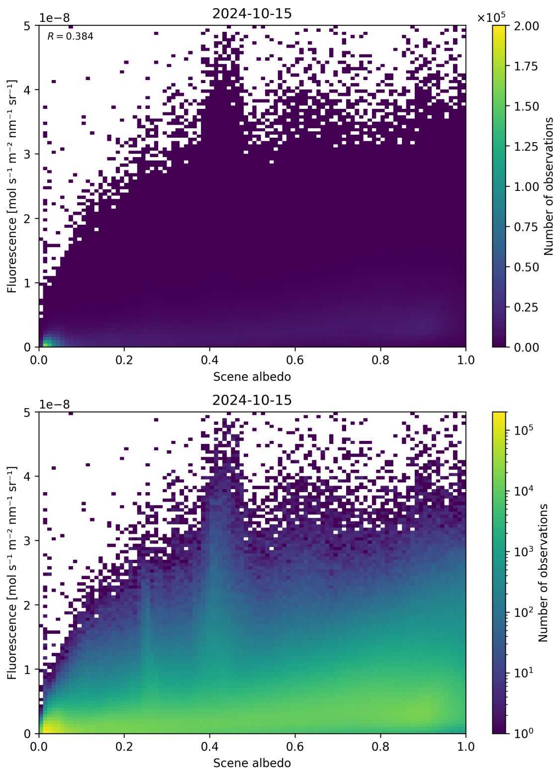
Figure 114: Scatter density plot of “Scene albedo” against “Fluorescence” for 2024-10-14 to 2024-10-16.
