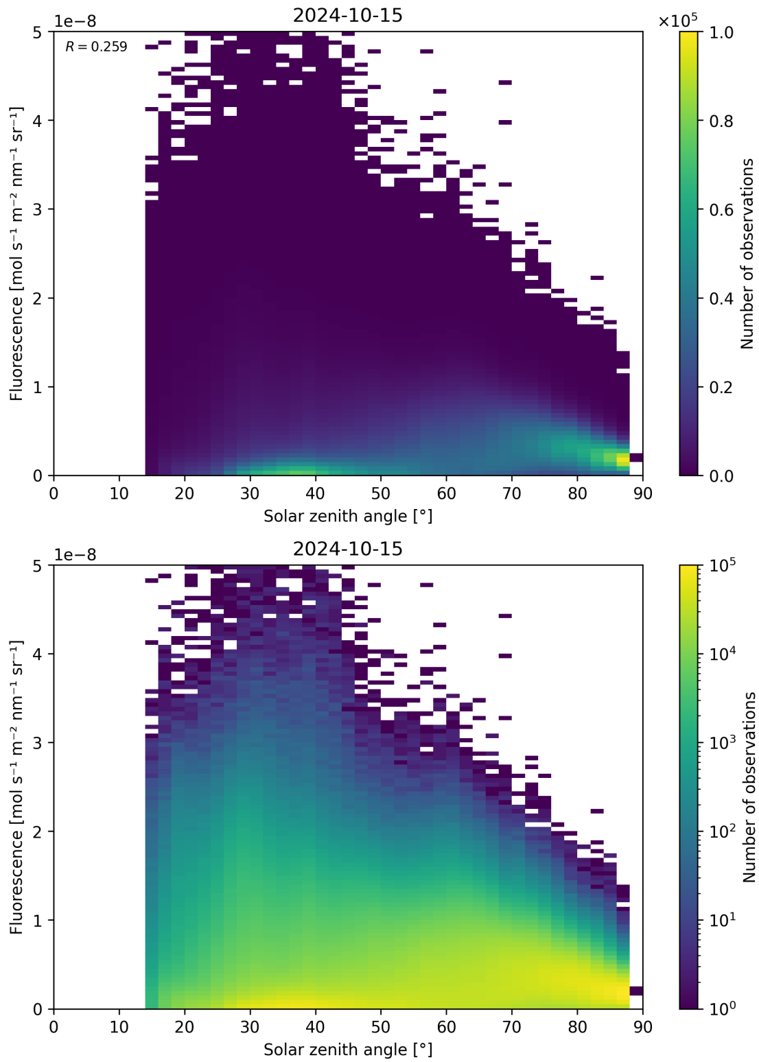
Figure 123: Scatter density plot of “Solar zenith angle” against “Fluorescence” for 2024-10-14 to 2024-10-16.
