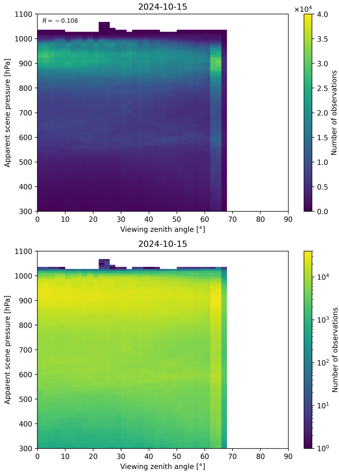
Figure 129: Scatter density plot of “Viewing zenith angle” against “Apparent scene pressure” for 2024-10-14 to 2024-10-16.
