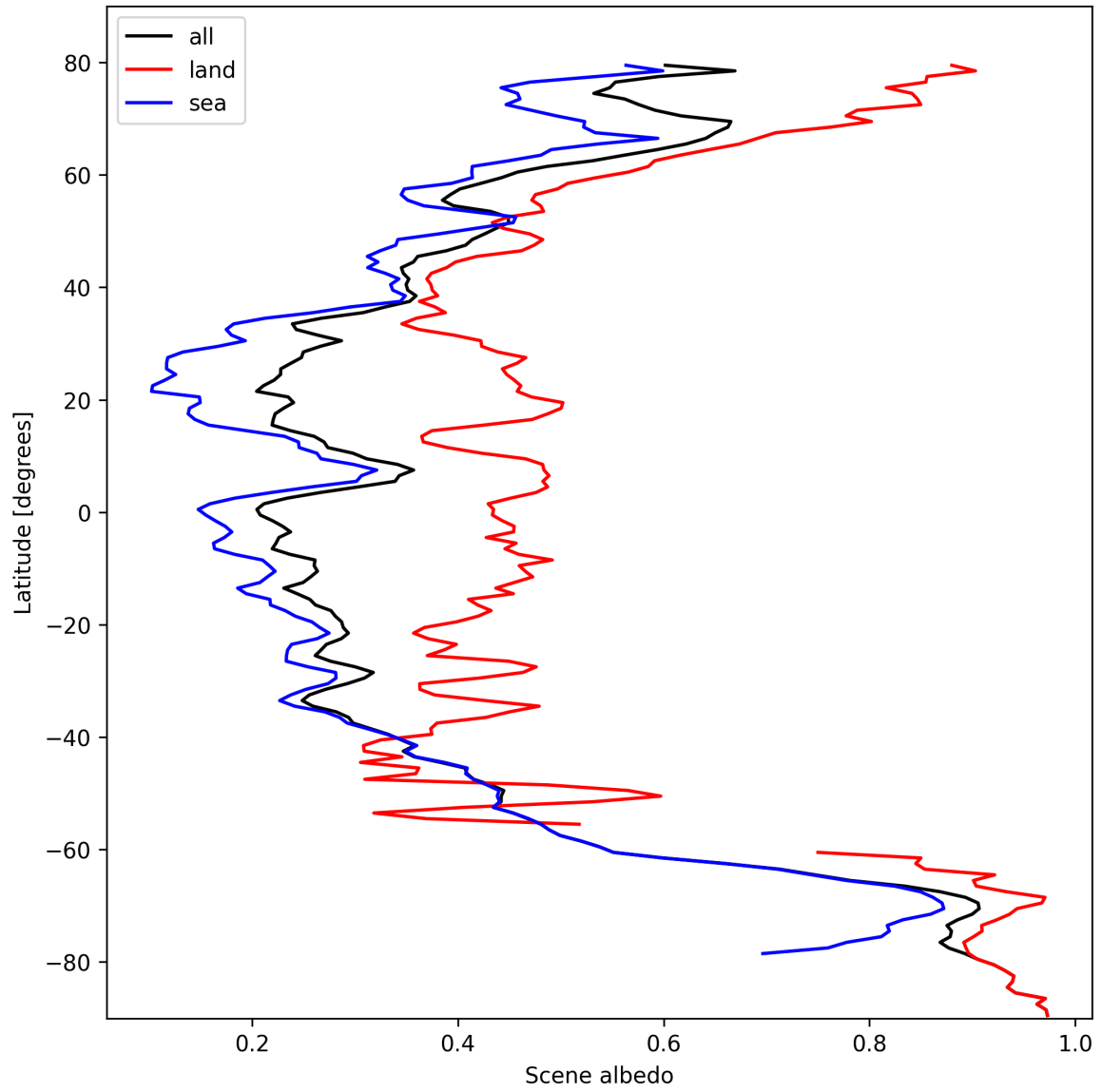
Figure 17: Zonal average of “Scene albedo” for 2024-10-14 to 2024-10-16.
