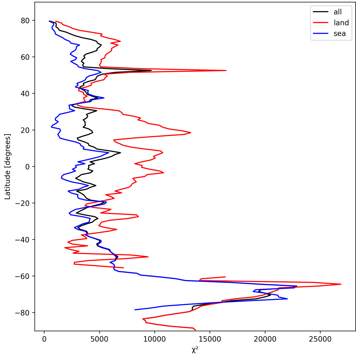
Figure 21: Zonal average of “ \chi^2 ” for 2024-10-14 to 2024-10-16.
