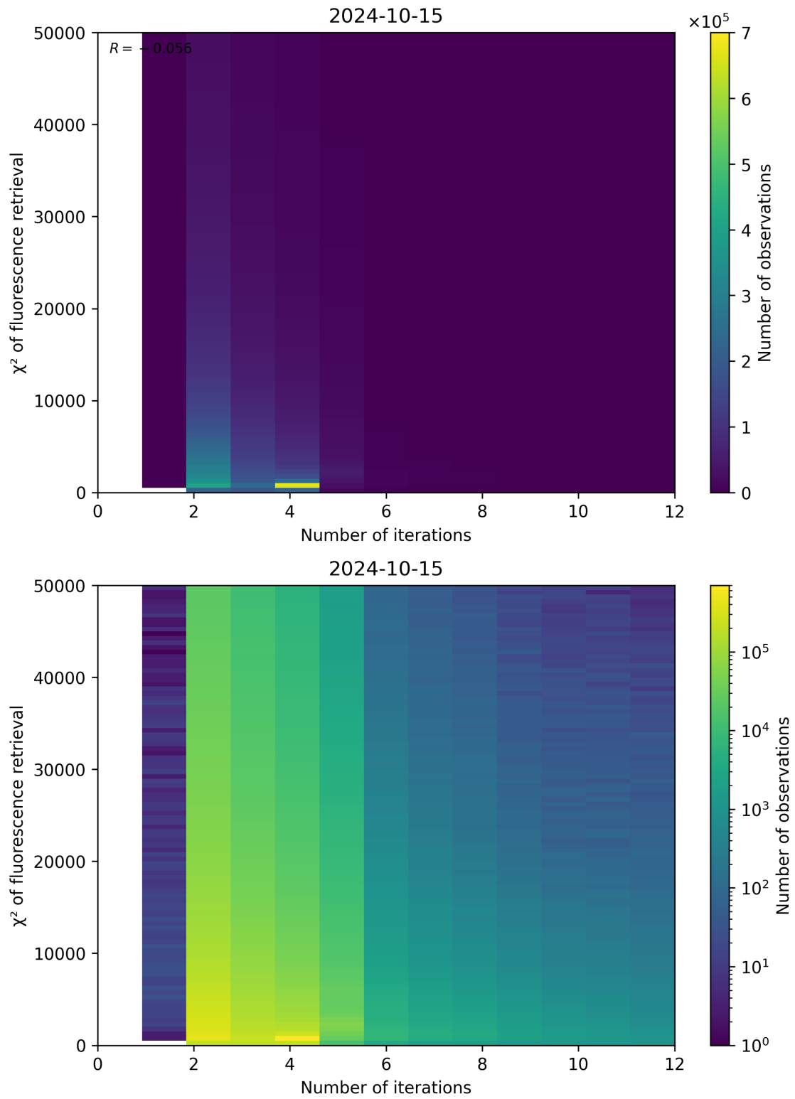
Figure 106: Scatter density plot of “Number of iterations” against “ \chi^2 of fluorescence retrieval” for 2024-10-14 to 2024-10-16.
