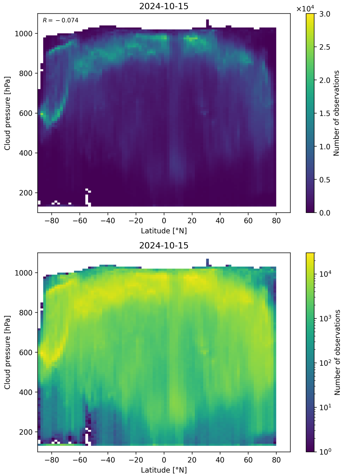
Figure 100: Scatter density plot of “Latitude” against “Cloud pressure” for 2024-10-14 to 2024-10-16.
