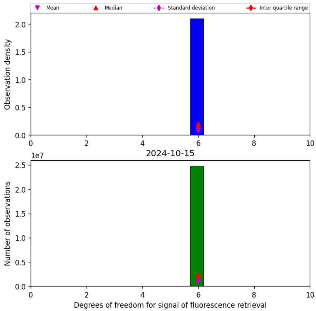
Figure 43: Histogram of “Degrees of freedom for signal of fluorescence retrieval” for 2024-10-14 to 2024-10-16
