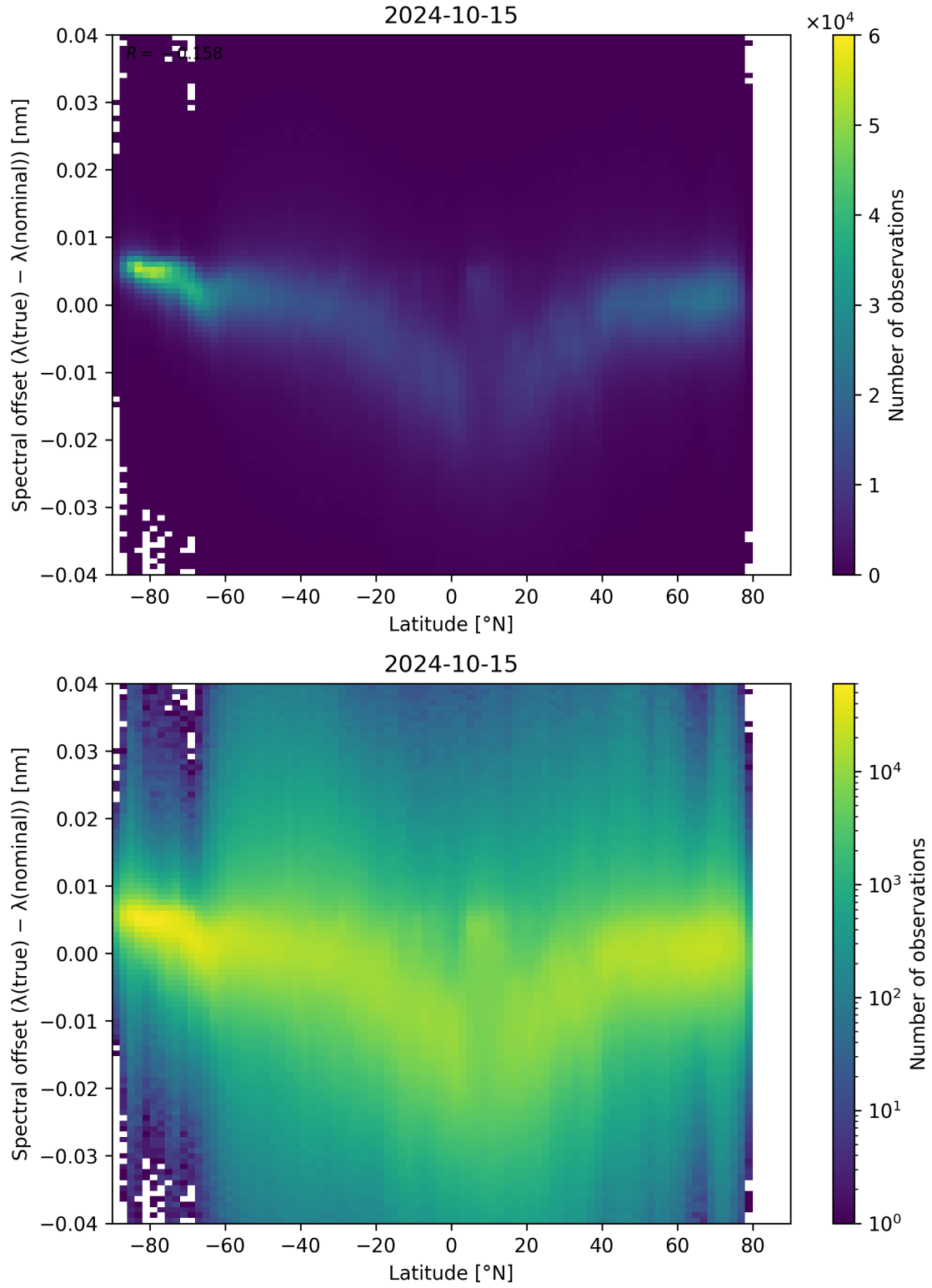
Figure 105: Scatter density plot of “Latitude” against “Spectral offset ( \lambda_{\text{true}} - \lambda_{\text{nominal}} )” for 2024-10-14 to 2024-10-16.
