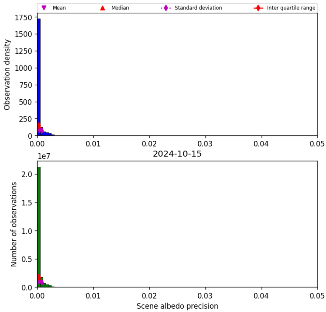
Figure 35: Histogram of “Scene albedo precision” for 2024-10-14 to 2024-10-16
