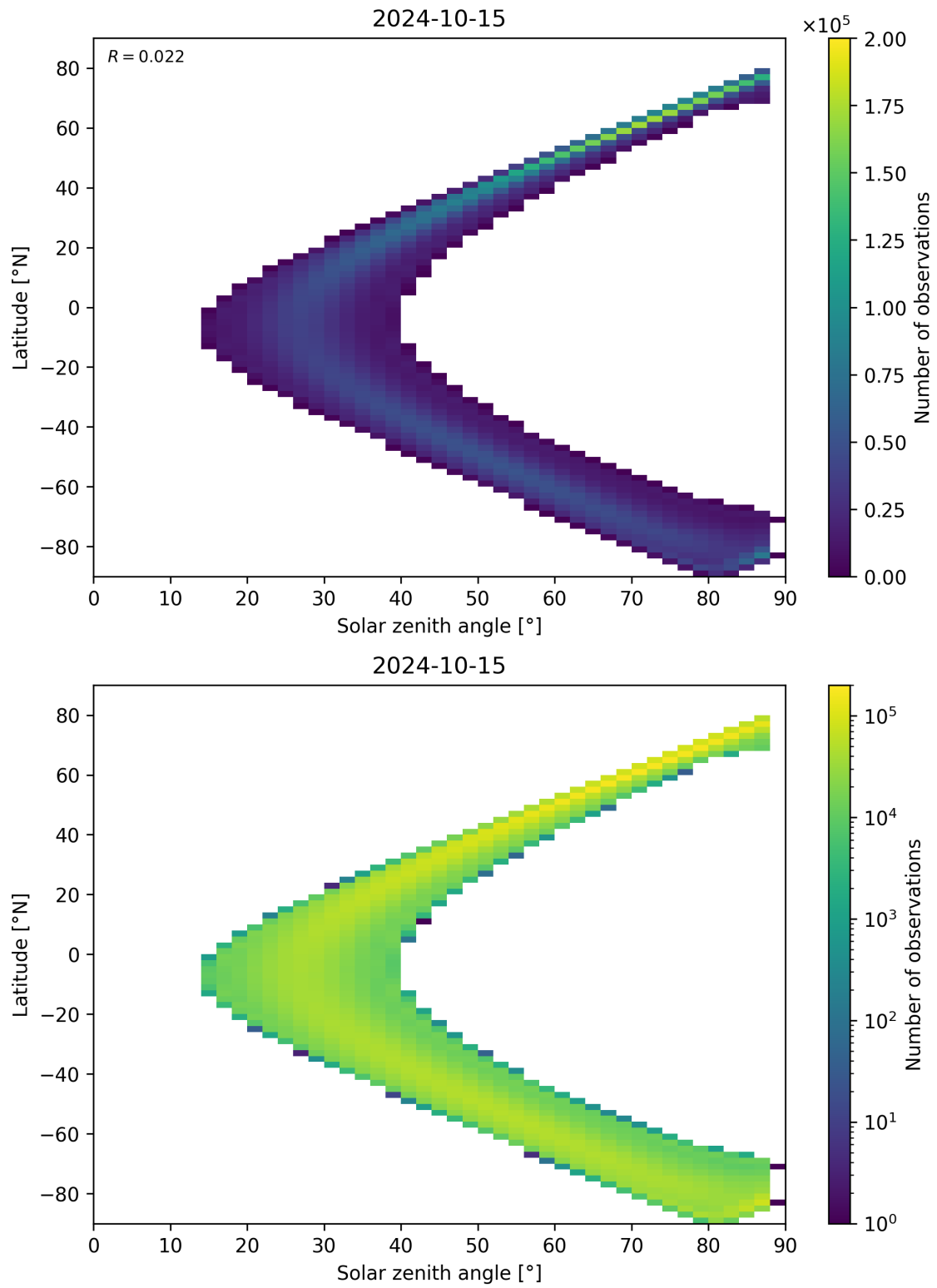
Figure 124: Scatter density plot of “Solar zenith angle” against “Latitude” for 2024-10-14 to 2024-10-16.
