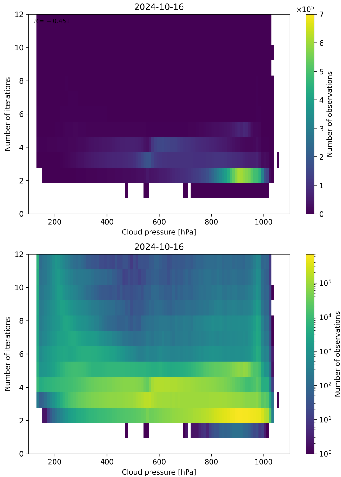
Figure 89: Scatter density plot of “Cloud pressure” against “Number of iterations” for 2024-10-15 to 2024-10-17.
