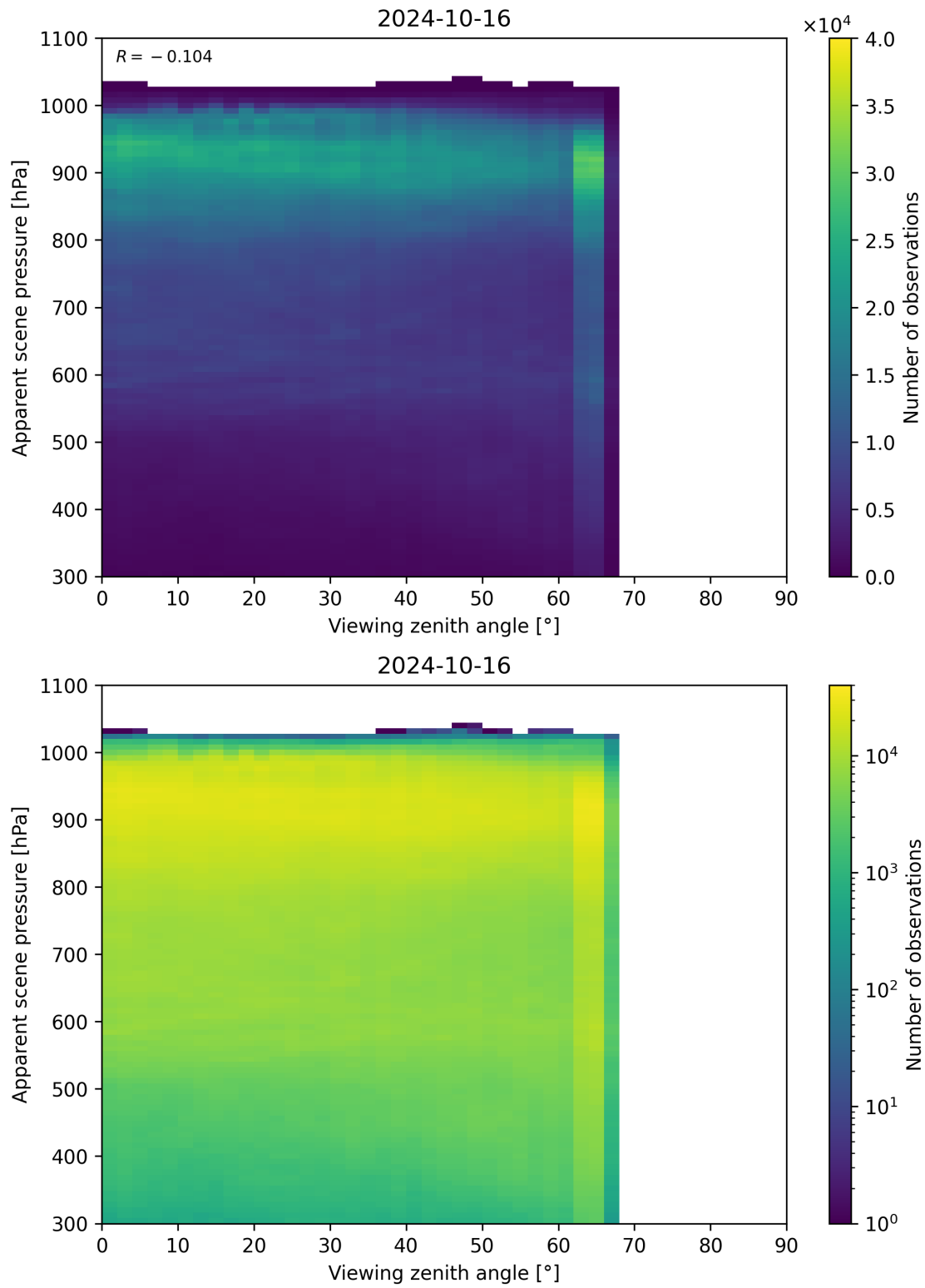
Figure 129: Scatter density plot of “Viewing zenith angle” against “Apparent scene pressure” for 2024-10-15 to 2024-10-17.
