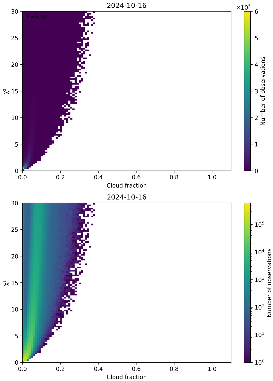
Figure 77: Scatter density plot of “Cloud fraction” against “ \chi^2 ” for 2024-10-15 to 2024-10-17.
