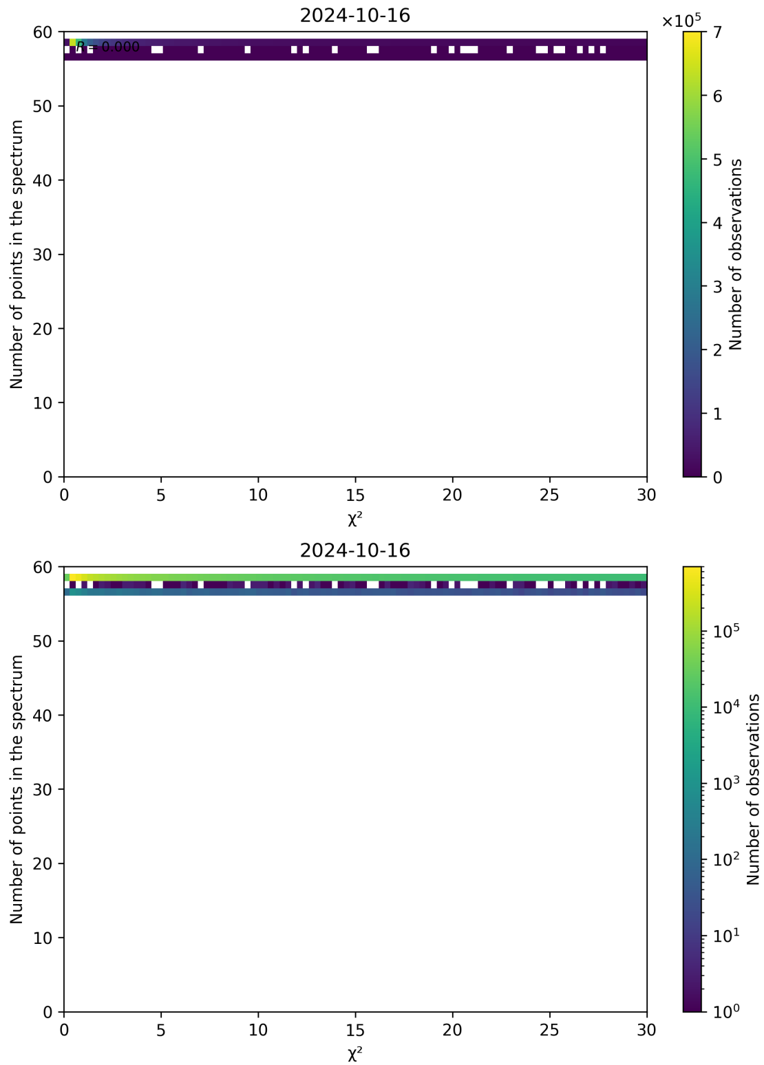
Figure 74: Scatter density plot of " \chi^2 " against "Number of points in the spectrum" for 2024-10-15 to 2024-10-17.
