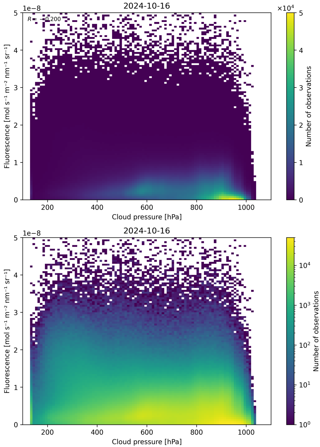
Figure 88: Scatter density plot of “Cloud pressure” against “Fluorescence” for 2024-10-15 to 2024-10-17.
