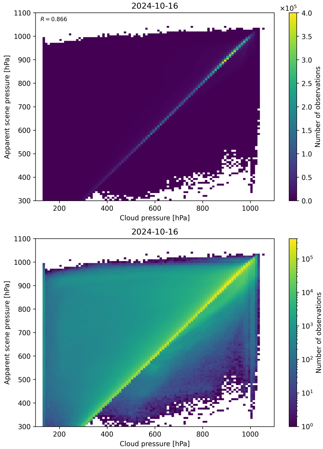
Figure 84: Scatter density plot of “Cloud pressure” against “Apparent scene pressure” for 2024-10-15 to 2024-10-17.
