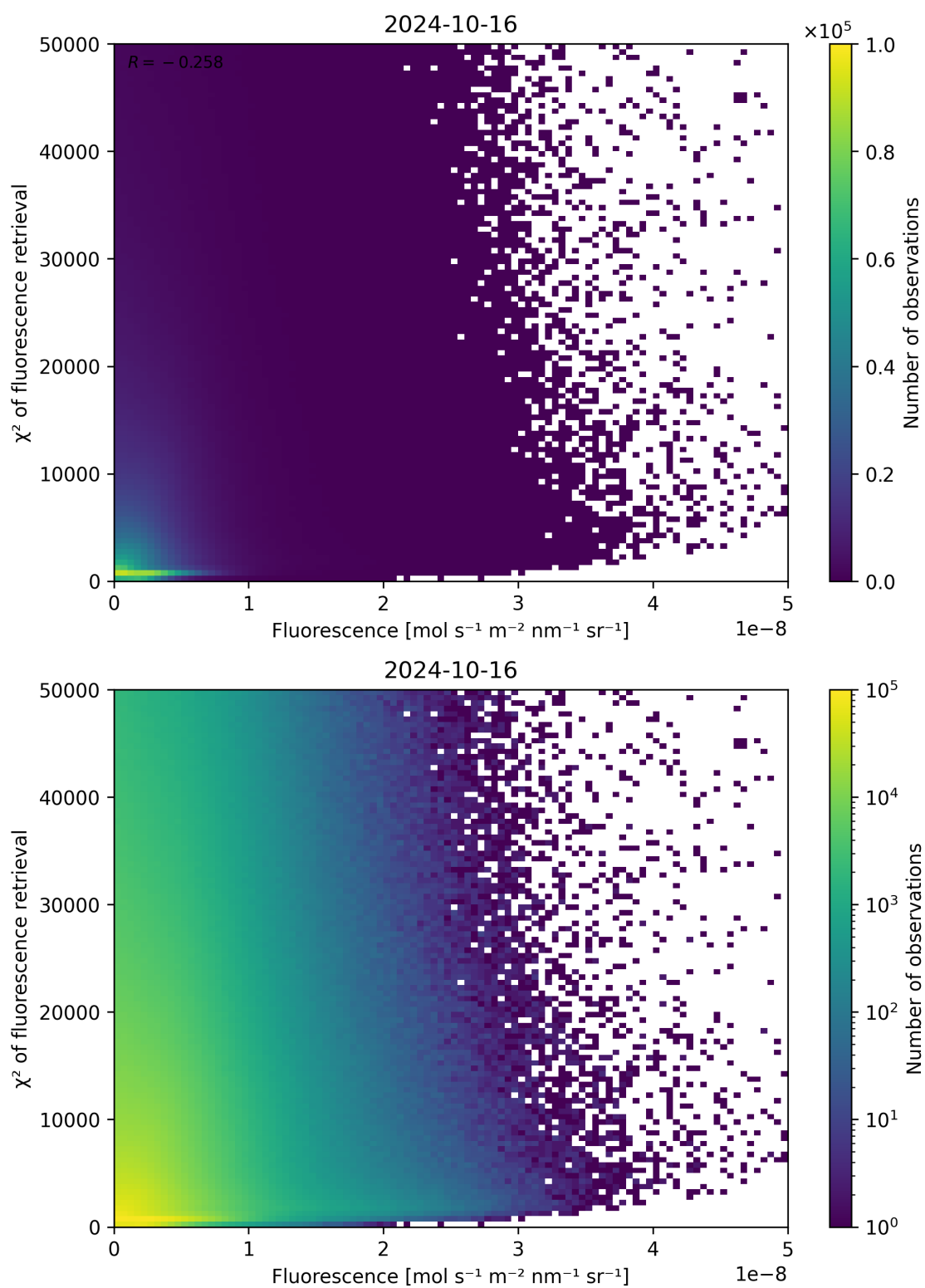
Figure 93: Scatter density plot of “Fluorescence” against “ \chi^2 of fluorescence retrieval” for 2024-10-15 to 2024-10-17.
