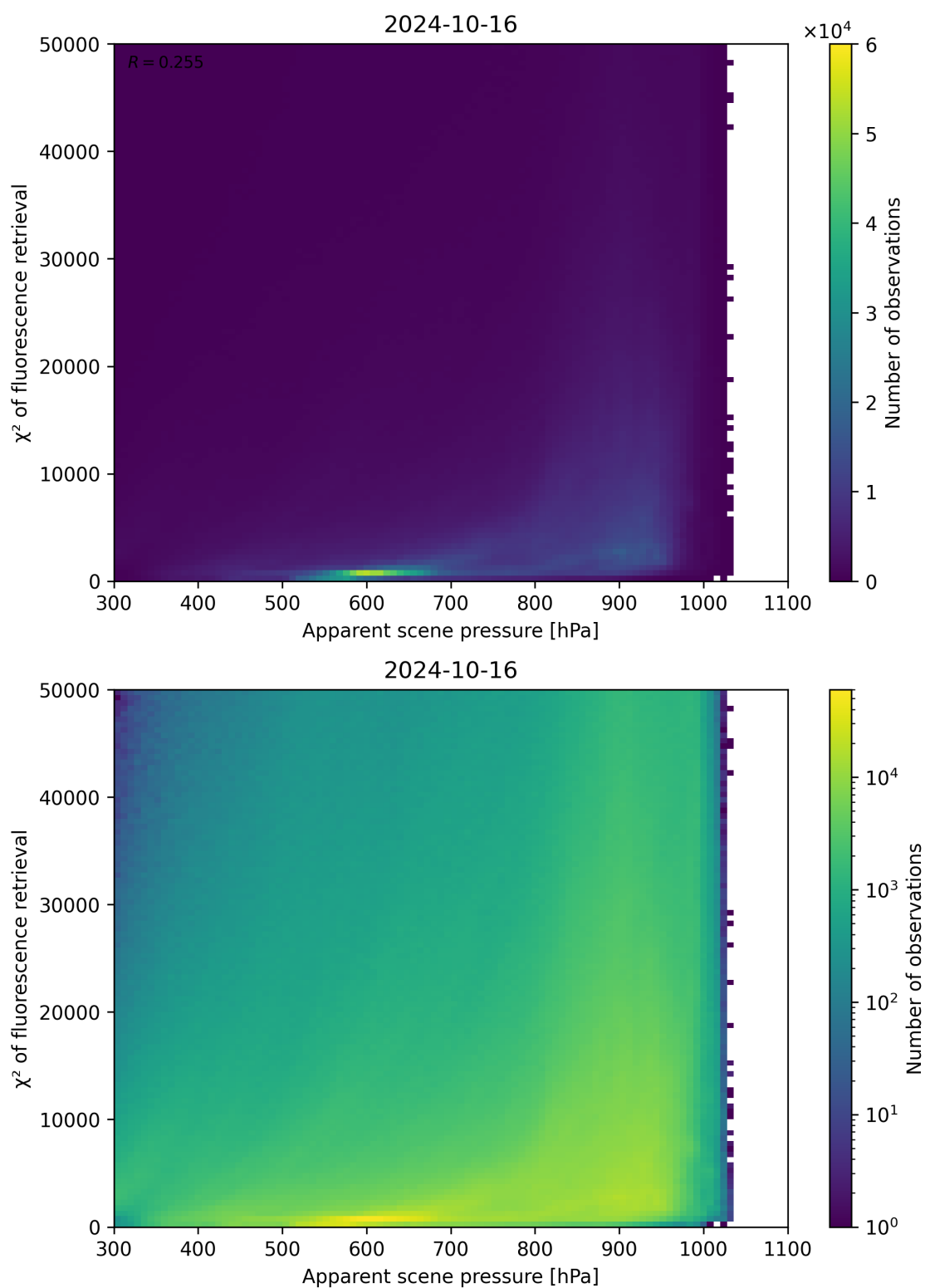
Figure 64: Scatter density plot of “Apparent scene pressure” against “ \chi^2 of fluorescence retrieval” for 2024-10-15 to 2024-10-17.
