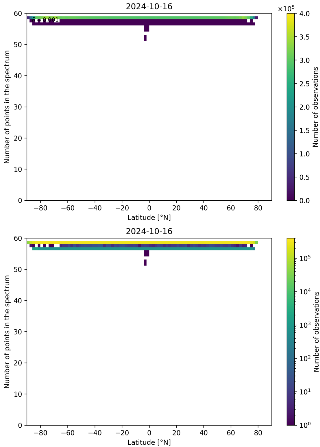
Figure 103: Scatter density plot of “Latitude” against “Number of points in the spectrum” for 2024-10-15 to 2024-10-17.
