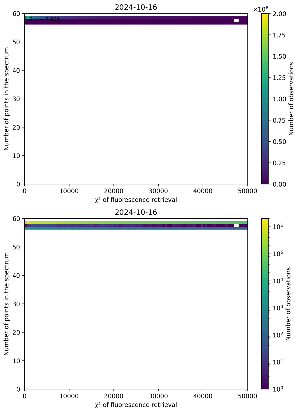
Figure 71: Scatter density plot of “ \chi^2 of fluorescence retrieval” against “Number of points in the spectrum” for 2024-10-15 to 2024-10-17.
