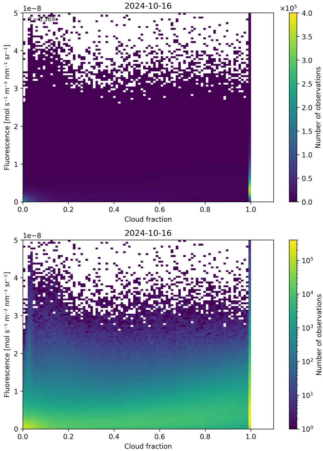
Figure 79: Scatter density plot of “Cloud fraction” against “Fluorescence” for 2024-10-15 to 2024-10-17.
