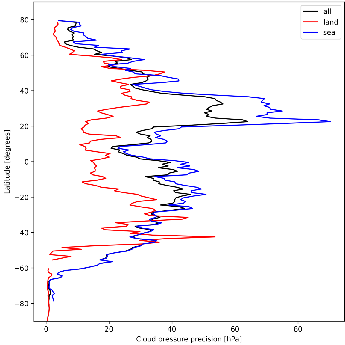
Figure 14: Zonal average of “Cloud pressure precision” for 2024-10-15 to 2024-10-17.
