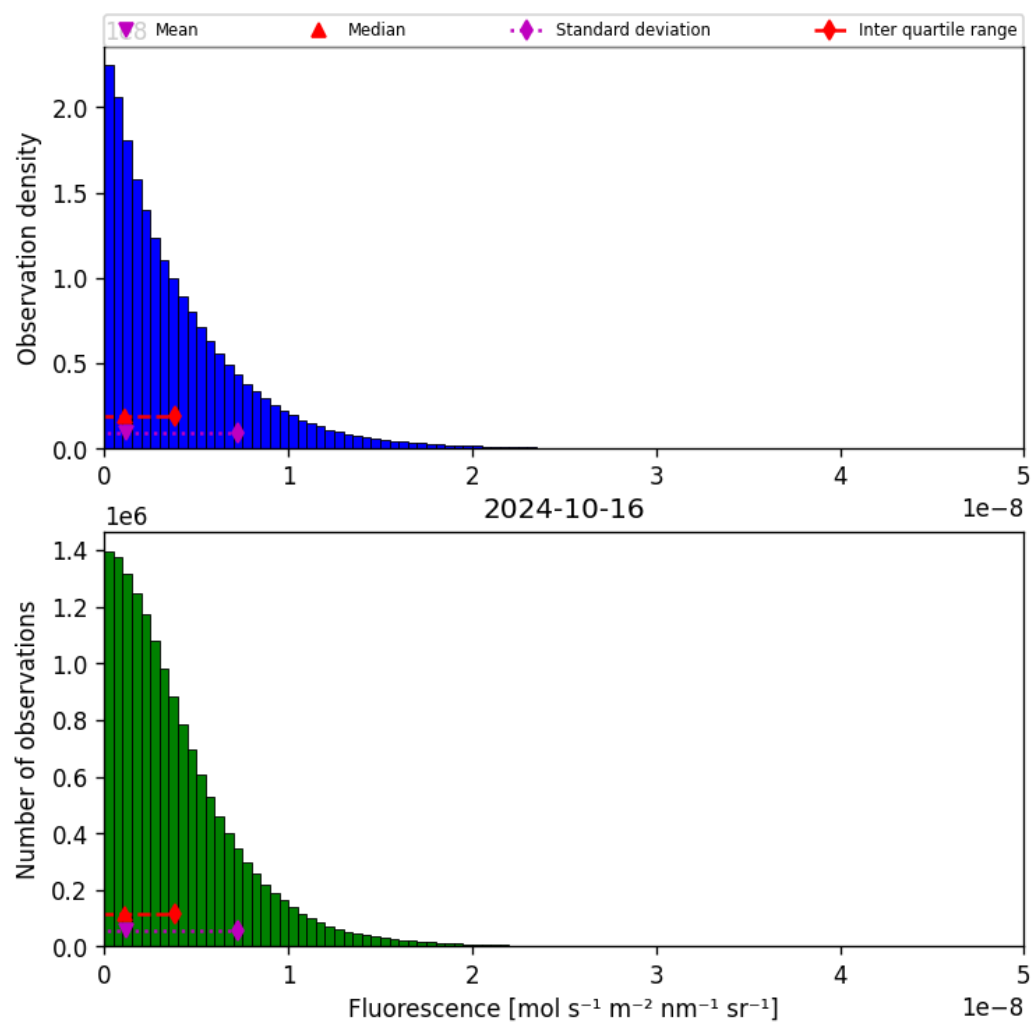
Figure 40: Histogram of “Fluorescence” for 2024-10-15 to 2024-10-17
