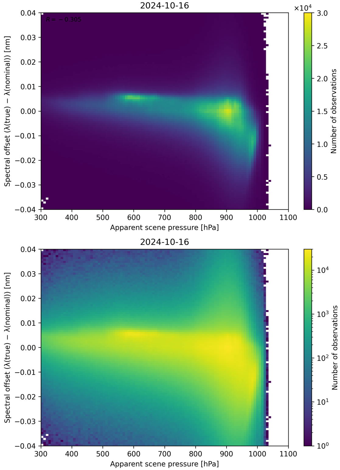
Figure 68: Scatter density plot of “Apparent scene pressure” against “Spectral offset ( \lambda_{\text{true}} - \lambda_{\text{nominal}} )” for 2024-10-15 to 2024-10-17.
