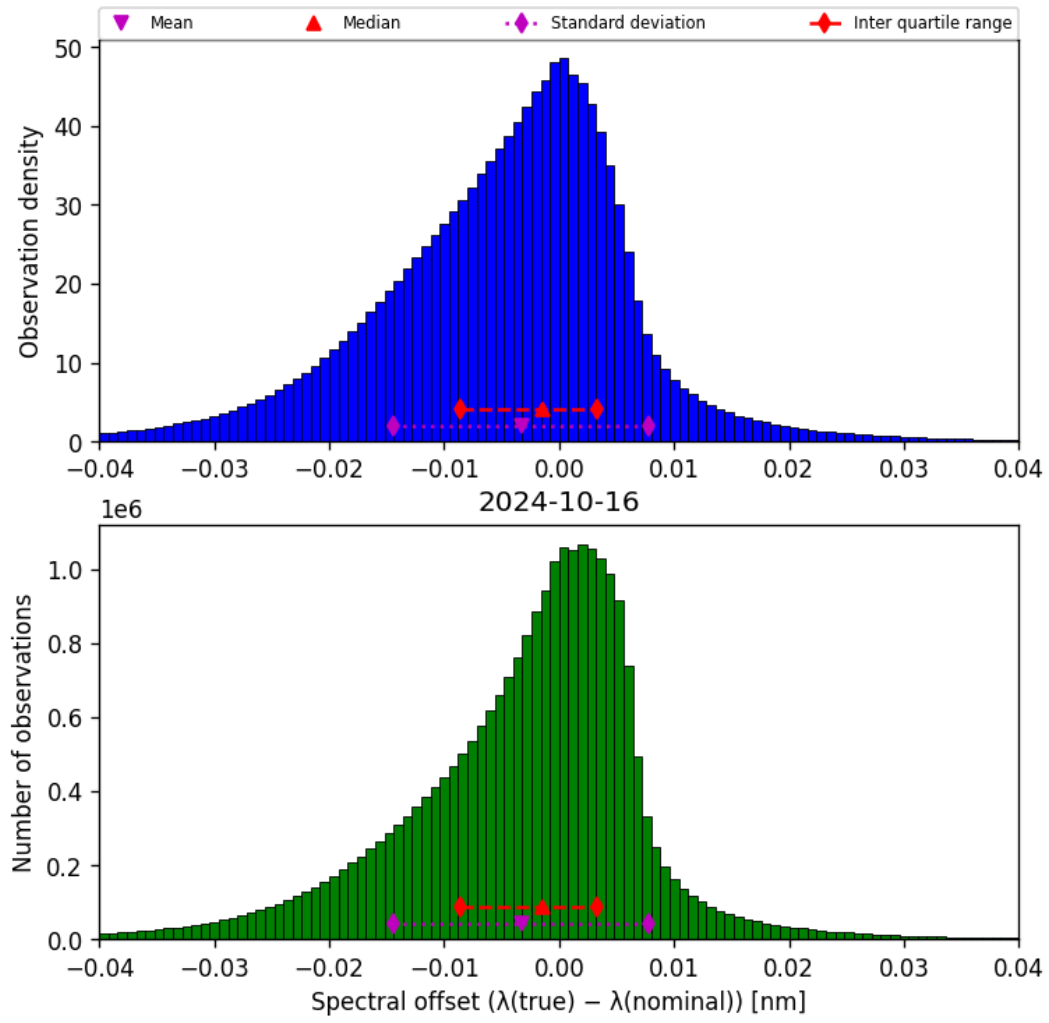
Figure 45: Histogram of “Spectral offset ( \lambda_{\text{true}} - \lambda_{\text{nominal}} )” for 2024-10-15 to 2024-10-17
