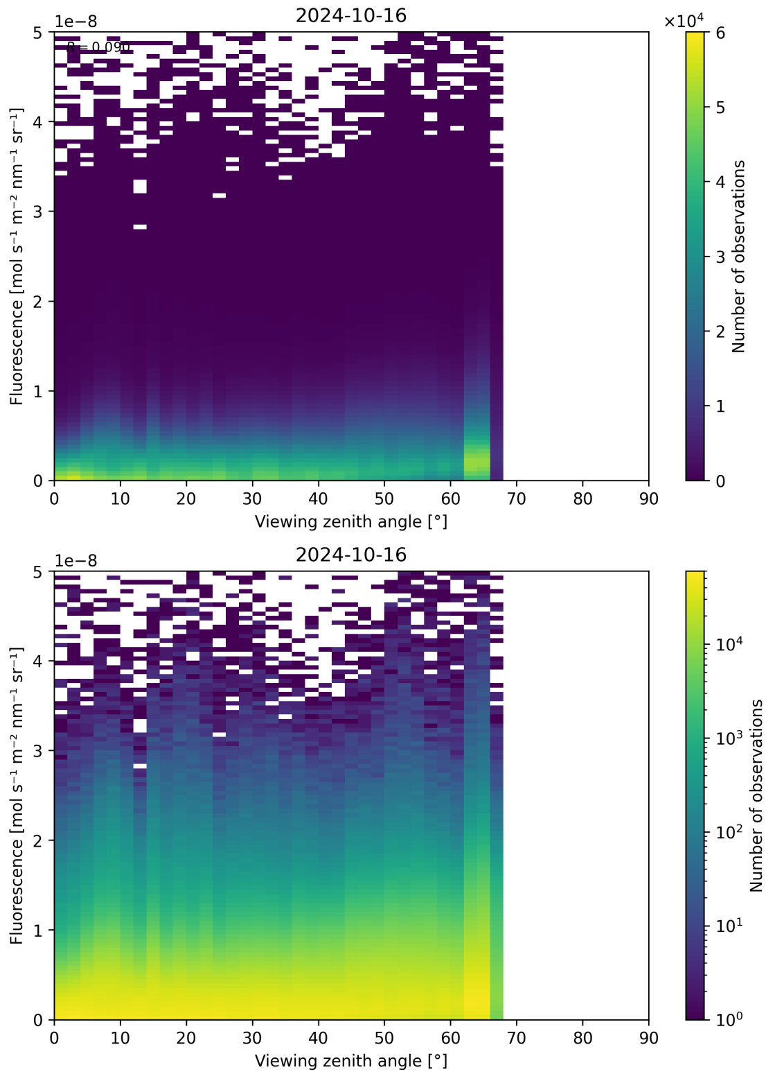
Figure 134: Scatter density plot of “Viewing zenith angle” against “Fluorescence” for 2024-10-15 to 2024-10-17.
