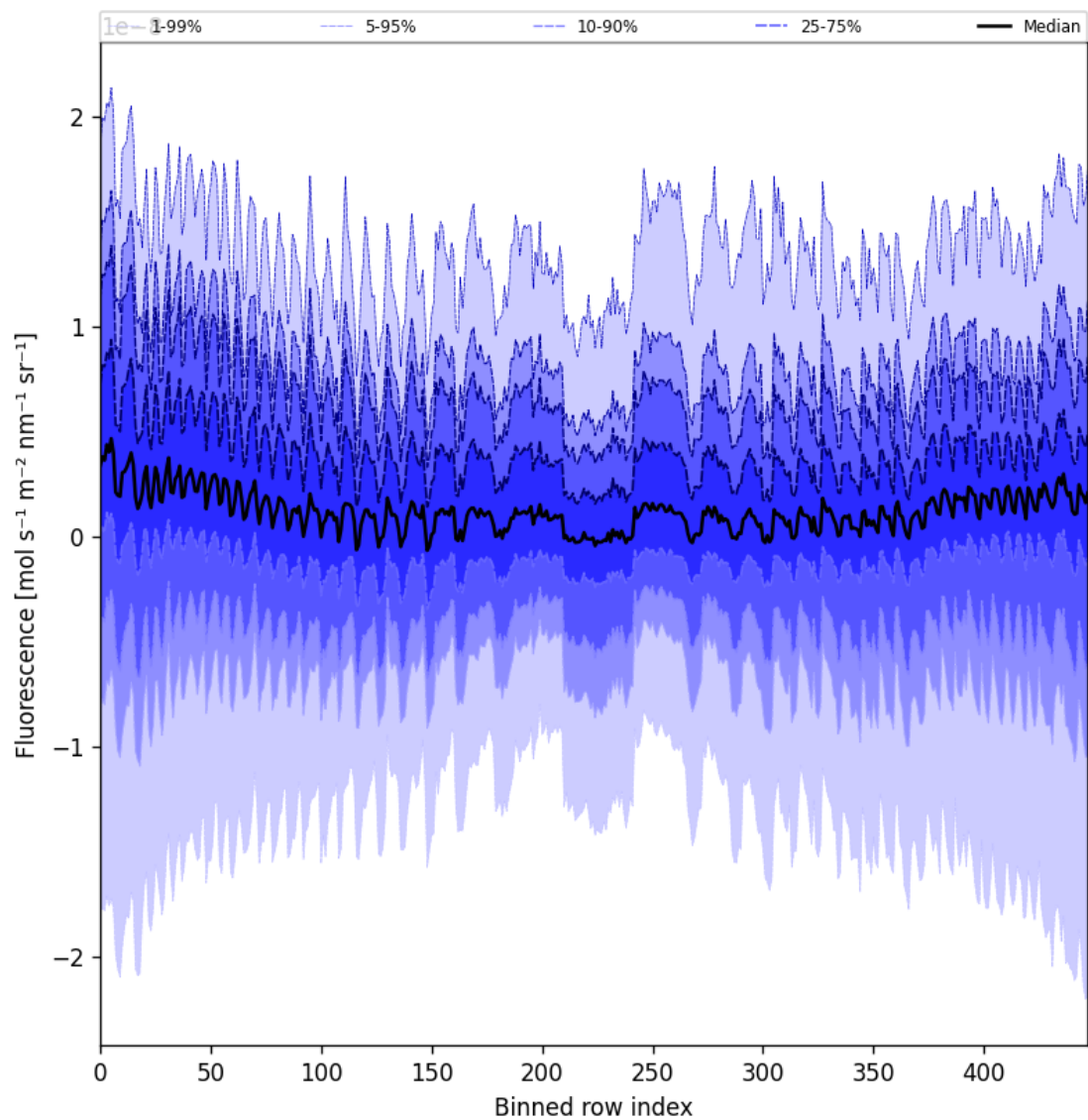
Figure 57: Along track statistics of “Fluorescence” for 2024-10-15 to 2024-10-17
