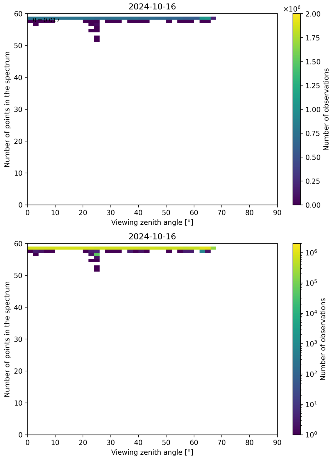
Figure 137: Scatter density plot of “Viewing zenith angle” against “Number of points in the spectrum” for 2024-10-15 to 2024-10-17.
