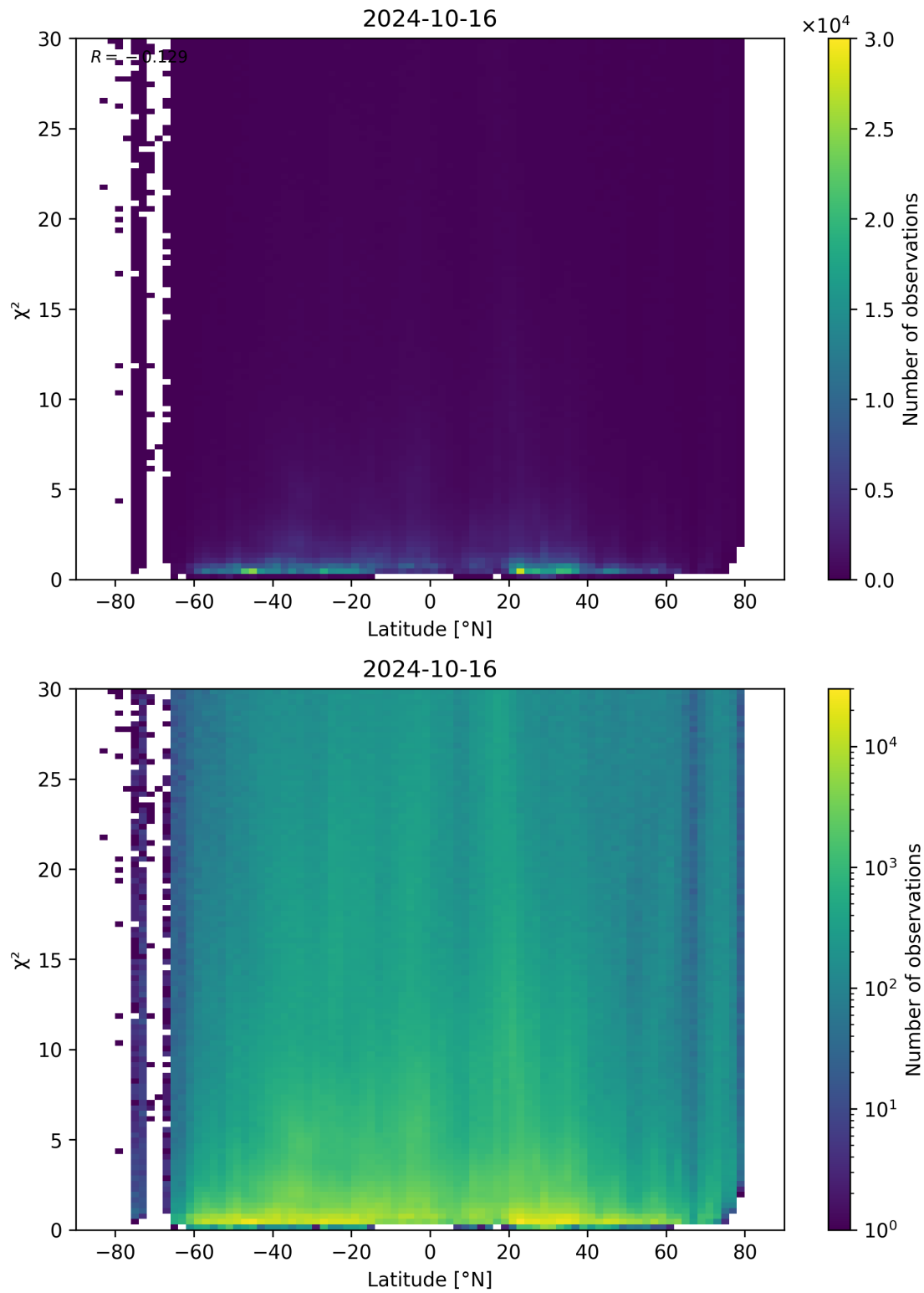
Figure 97: Scatter density plot of “Latitude” against “ \chi^2 ” for 2024-10-15 to 2024-10-17.
