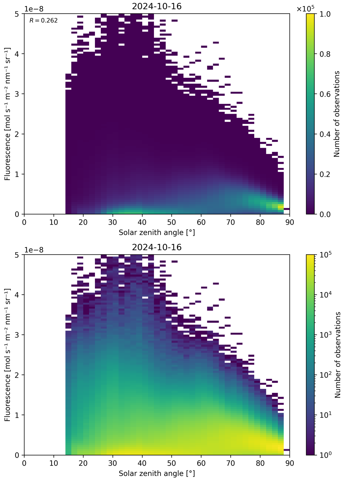
Figure 123: Scatter density plot of “Solar zenith angle” against “Fluorescence” for 2024-10-15 to 2024-10-17.
