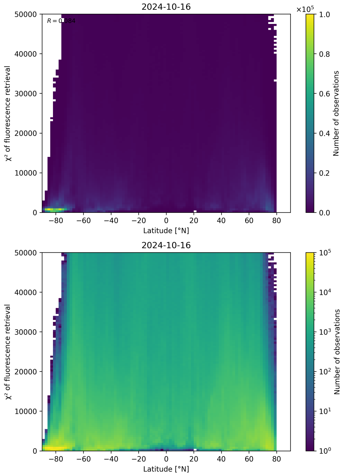
Figure 98: Scatter density plot of “Latitude” against “ \chi^2 of fluorescence retrieval” for 2024-10-15 to 2024-10-17.
