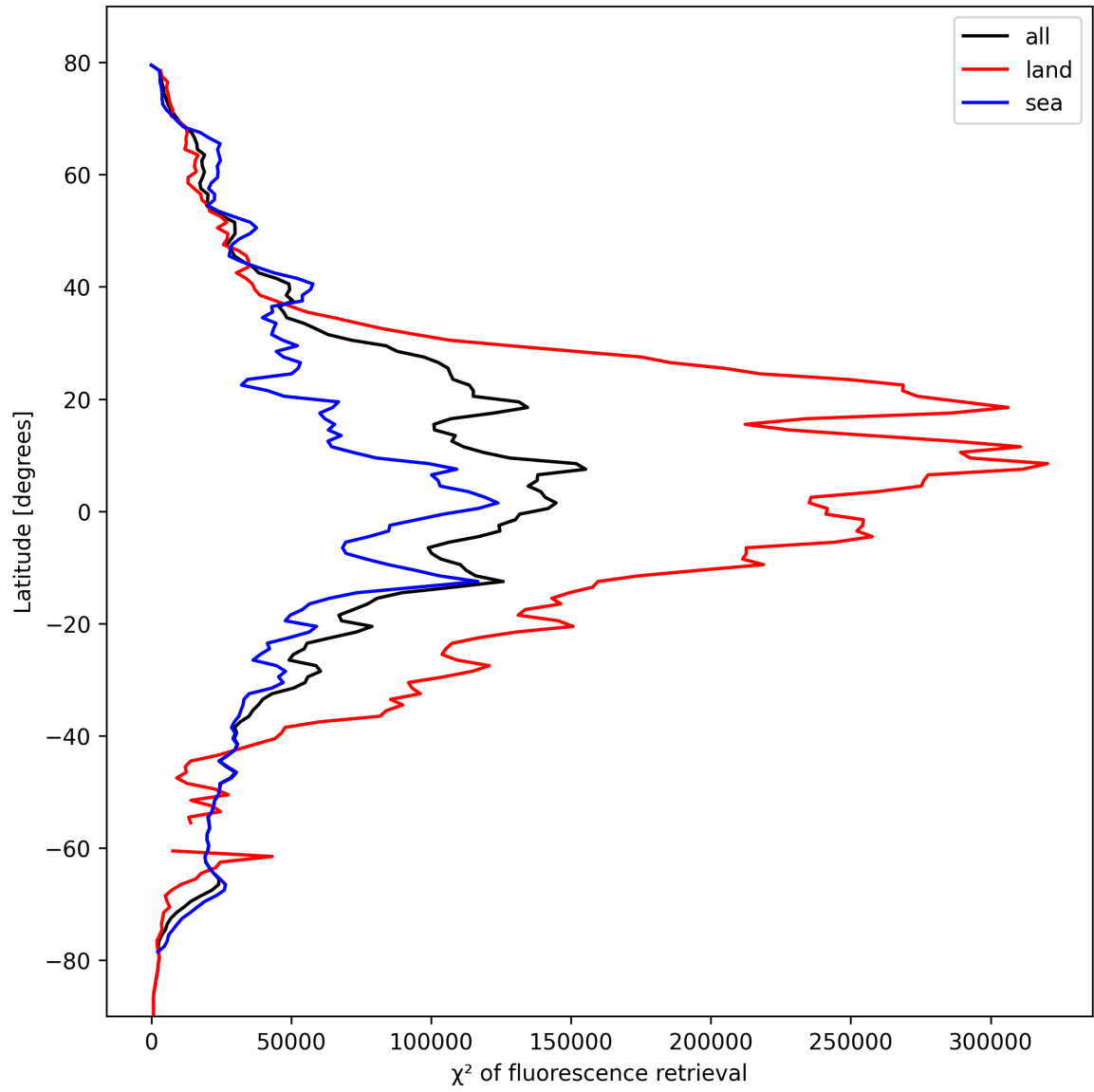
Figure 25: Zonal average of “ \chi^2 of fluorescence retrieval” for 2024-10-15 to 2024-10-17.
