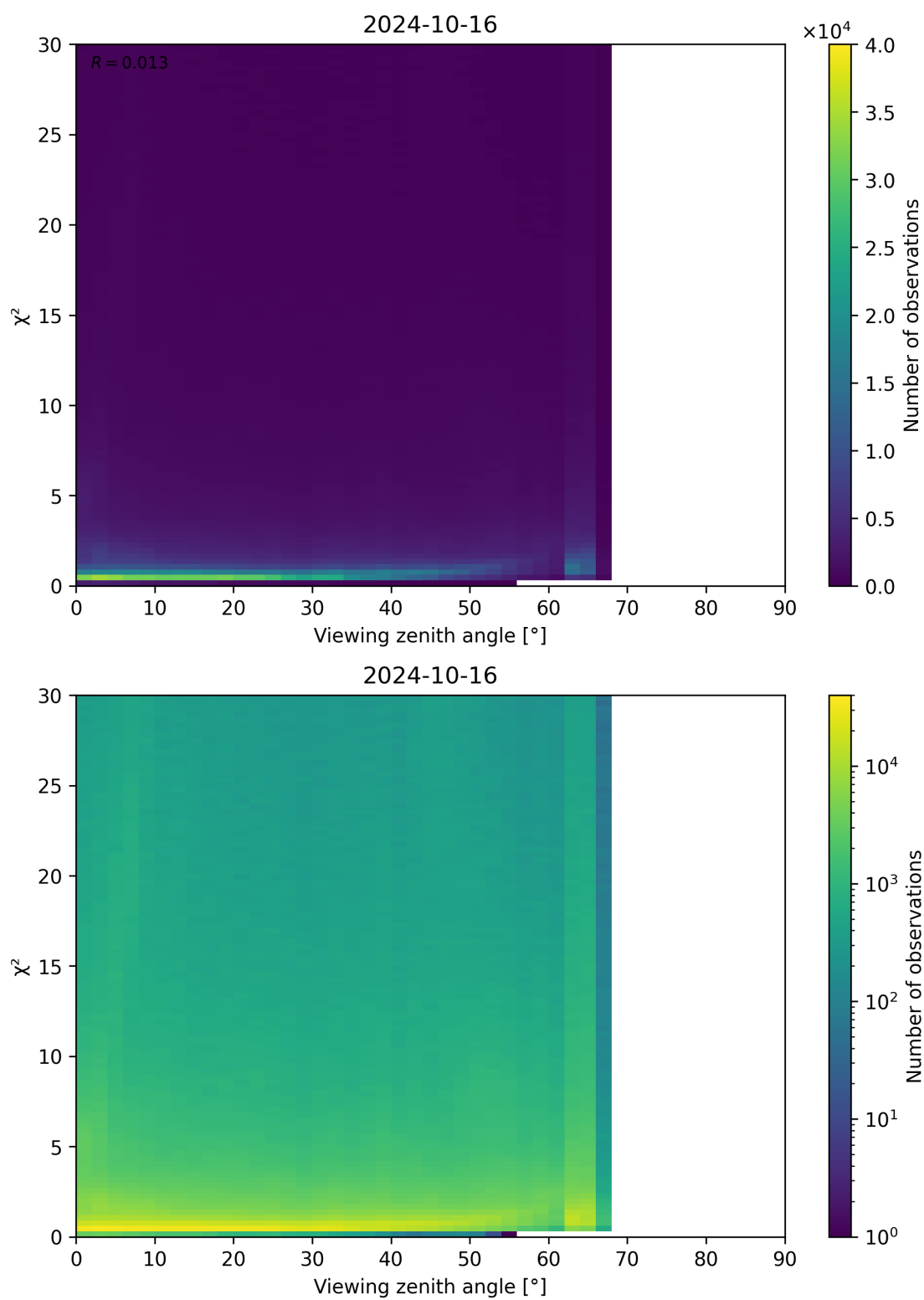
Figure 130: Scatter density plot of “Viewing zenith angle” against “ \chi^2 ” for 2024-10-15 to 2024-10-17.
