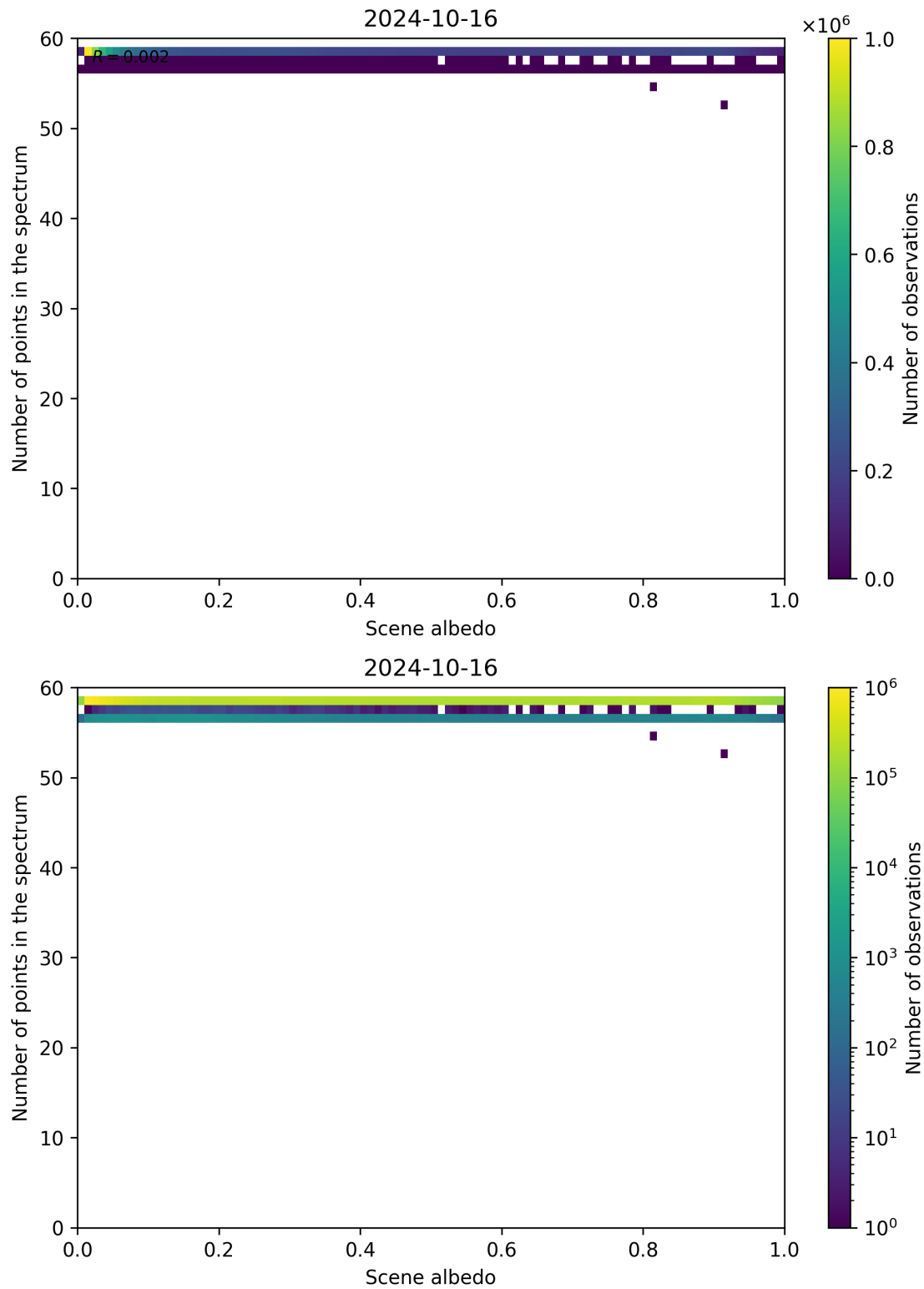
Figure 116: Scatter density plot of “Scene albedo” against “Number of points in the spectrum” for 2024-10-15 to 2024-10-17.
