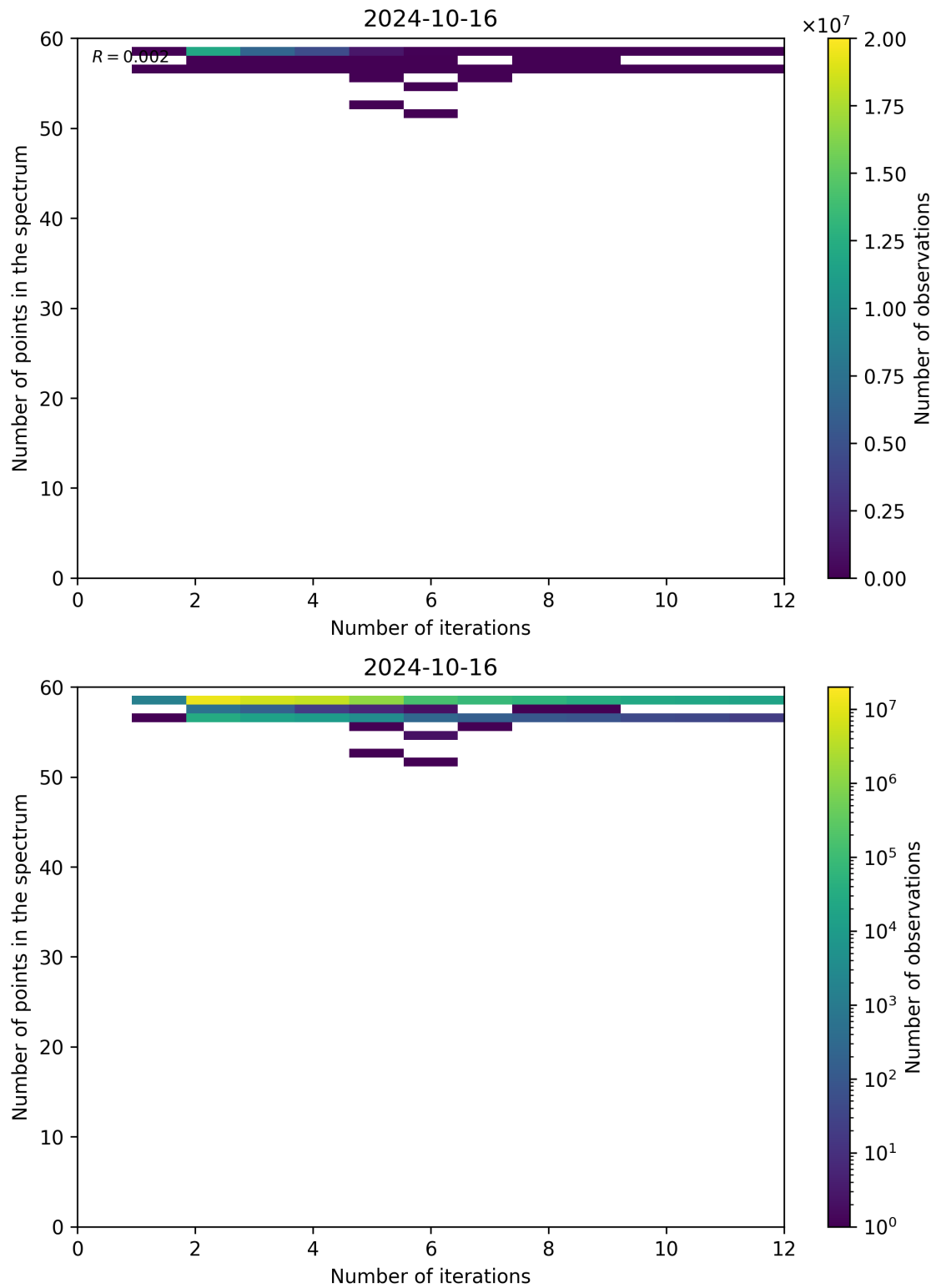
Figure 108: Scatter density plot of “Number of iterations” against “Number of points in the spectrum” for 2024-10-15 to 2024-10-17.
