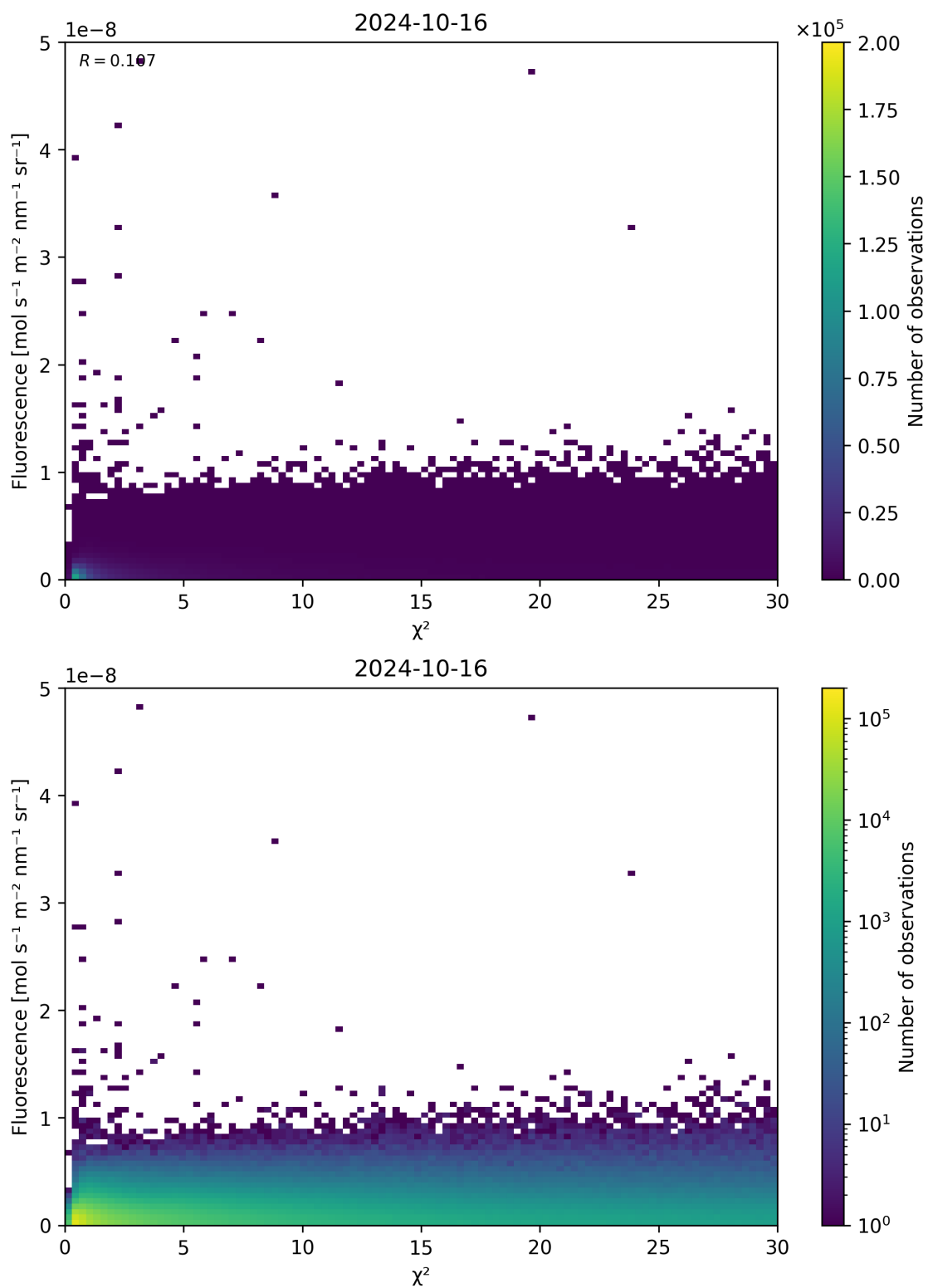
Figure 70: Scatter density plot of “ \chi^2 ” against “Fluorescence” for 2024-10-15 to 2024-10-17.
