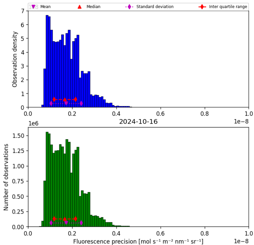
Figure 41: Histogram of “Fluorescence precision” for 2024-10-15 to 2024-10-17
