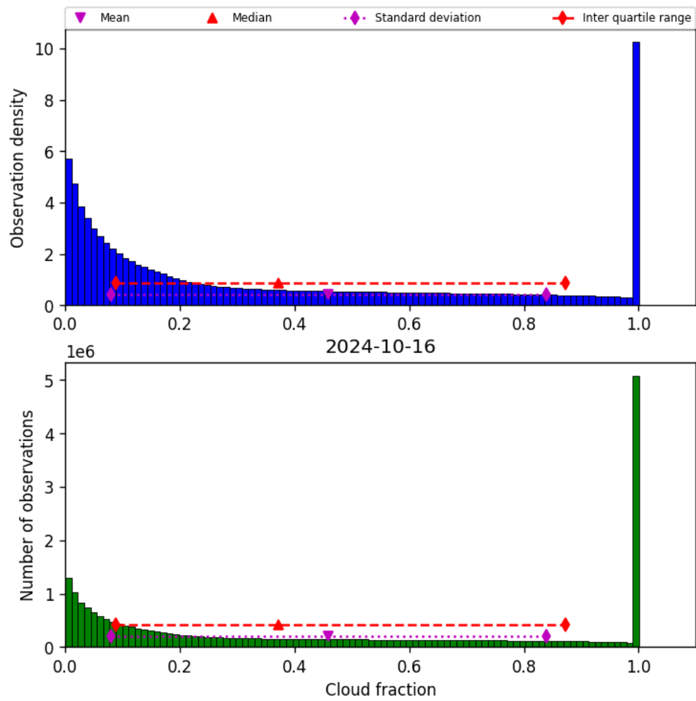
Figure 32: Histogram of “Cloud fraction” for 2024-10-15 to 2024-10-17
