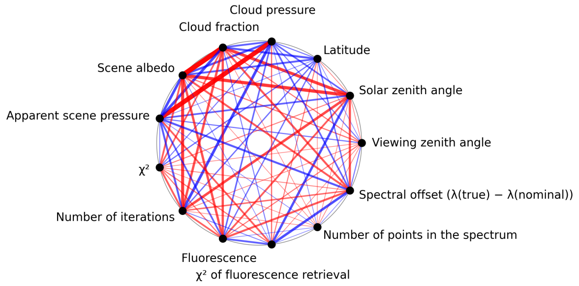
Figure 1: Map of correlation graph for 2024-10-15 to 2024-10-17.
