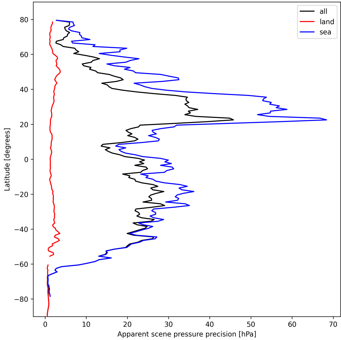
Figure 20: Zonal average of “Apparent scene pressure precision” for 2024-10-15 to 2024-10-17.
