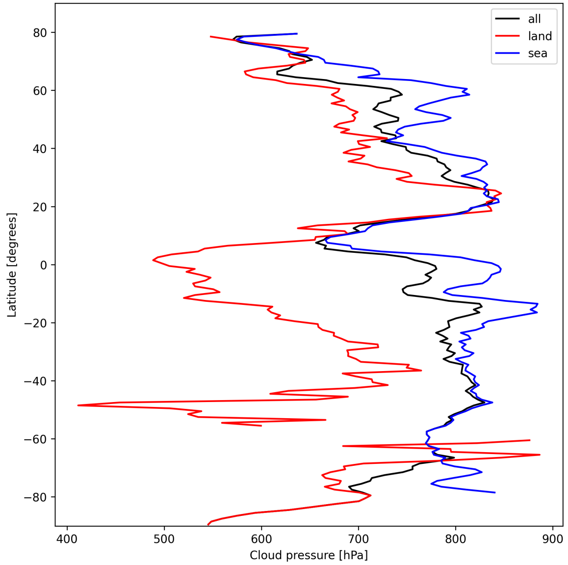
Figure 13: Zonal average of “Cloud pressure” for 2024-10-15 to 2024-10-17.
