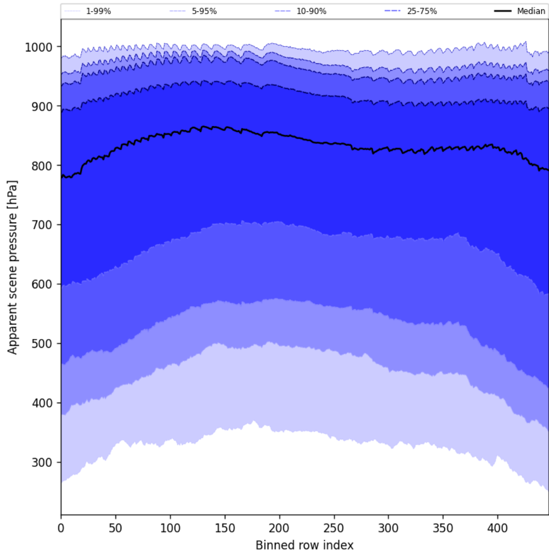
Figure 53: Along track statistics of “Apparent scene pressure” for 2024-10-15 to 2024-10-17
