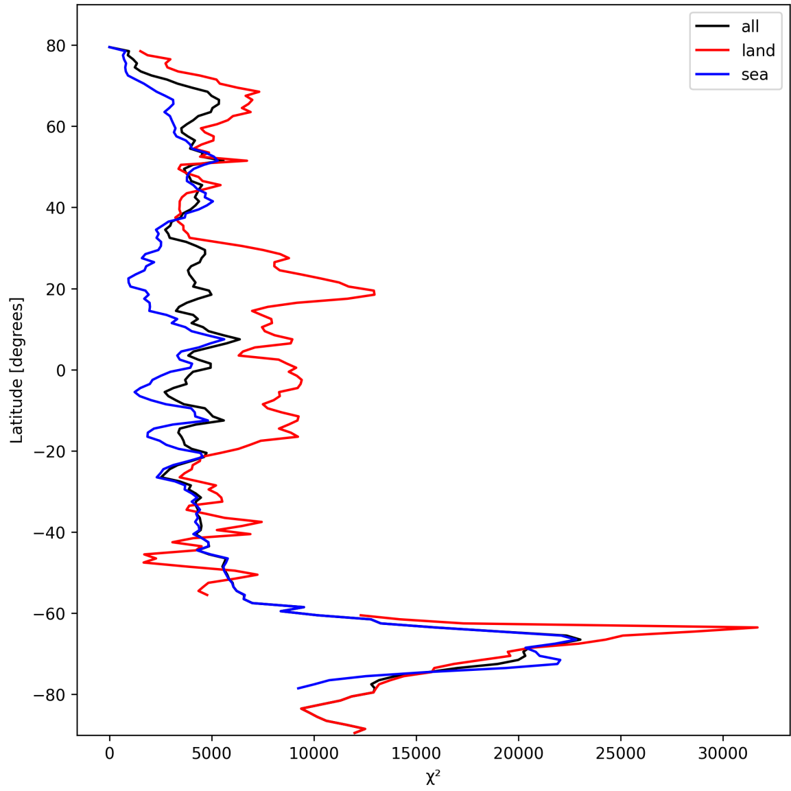
Figure 21: Zonal average of “ \chi^2 ” for 2024-10-15 to 2024-10-17.
