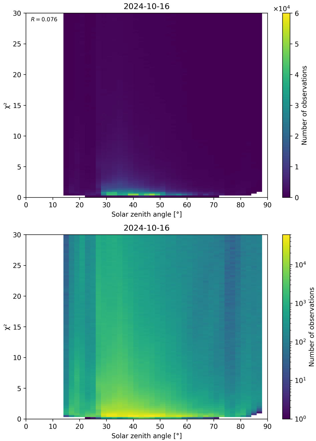
Figure 119: Scatter density plot of “Solar zenith angle” against “ \chi^2 ” for 2024-10-15 to 2024-10-17.
