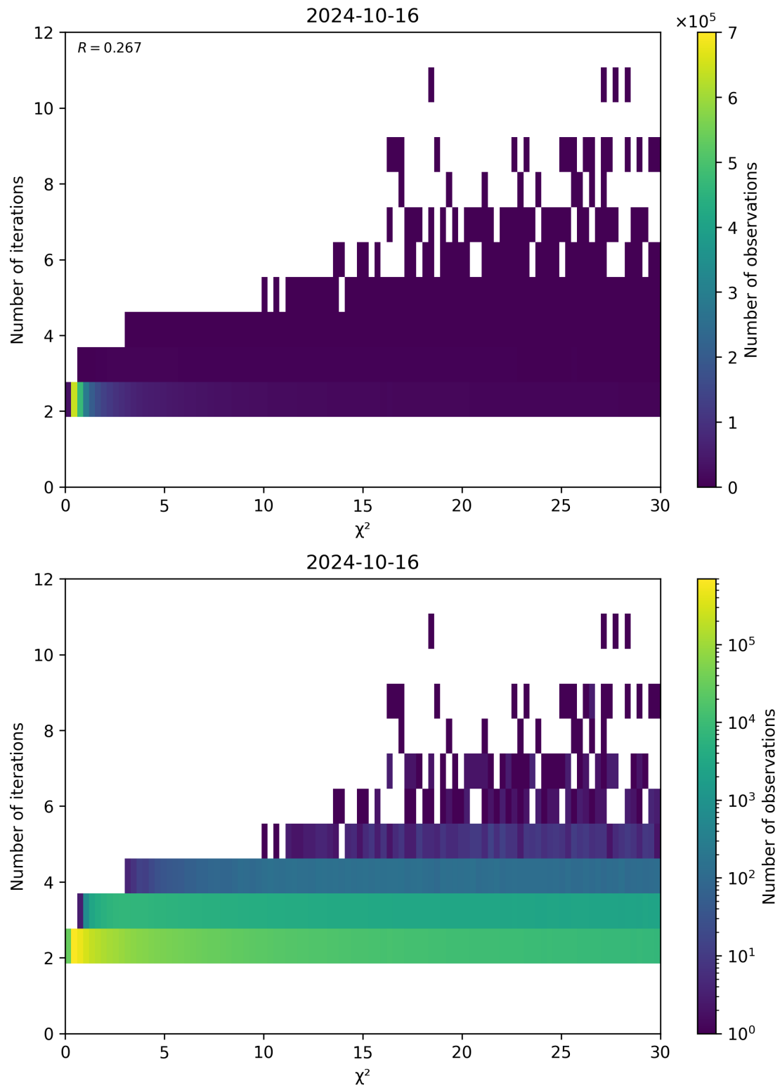
Figure 73: Scatter density plot of “ \chi^2 ” against “Number of iterations” for 2024-10-15 to 2024-10-17.
