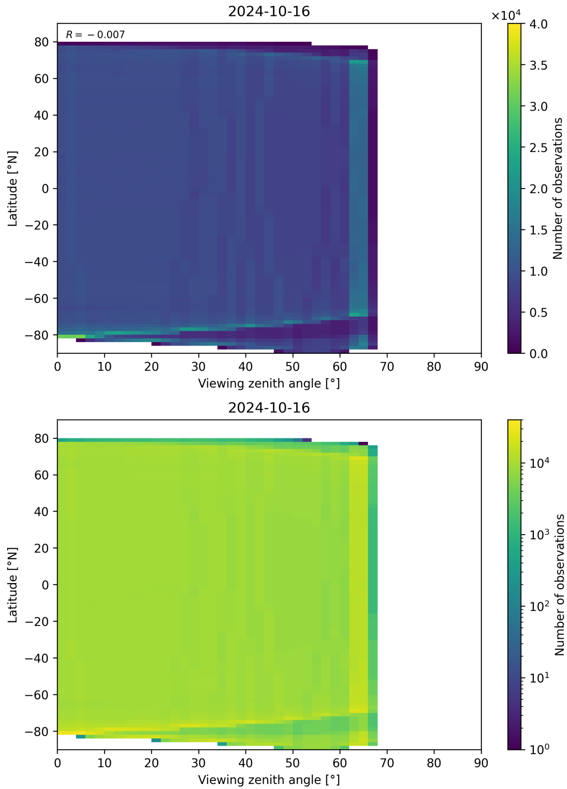
Figure 135: Scatter density plot of “Viewing zenith angle” against “Latitude” for 2024-10-15 to 2024-10-17.
