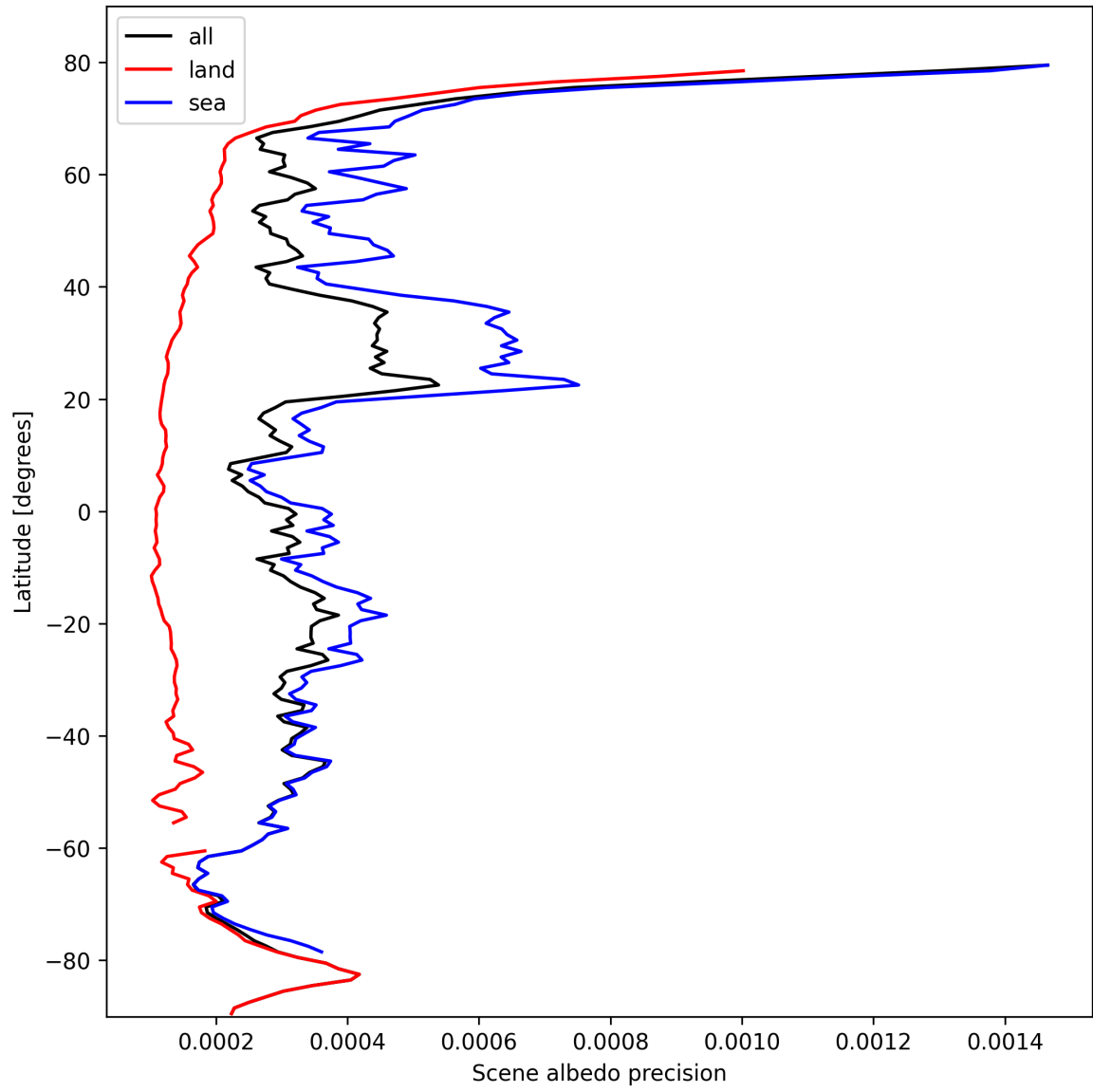
Figure 18: Zonal average of “Scene albedo precision” for 2024-10-15 to 2024-10-17.
