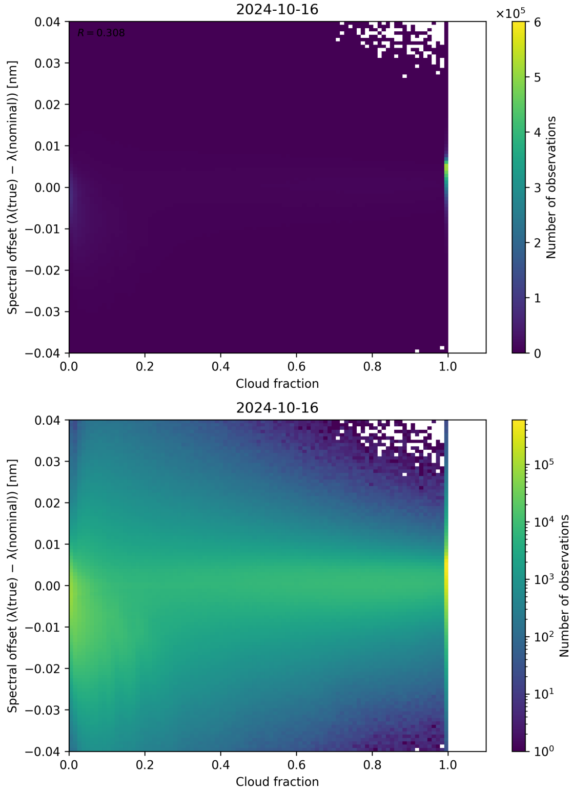
Figure 83: Scatter density plot of “Cloud fraction” against “Spectral offset ( \lambda_{\text{true}} - \lambda_{\text{nominal}} )” for 2024-10-15 to 2024-10-17.
