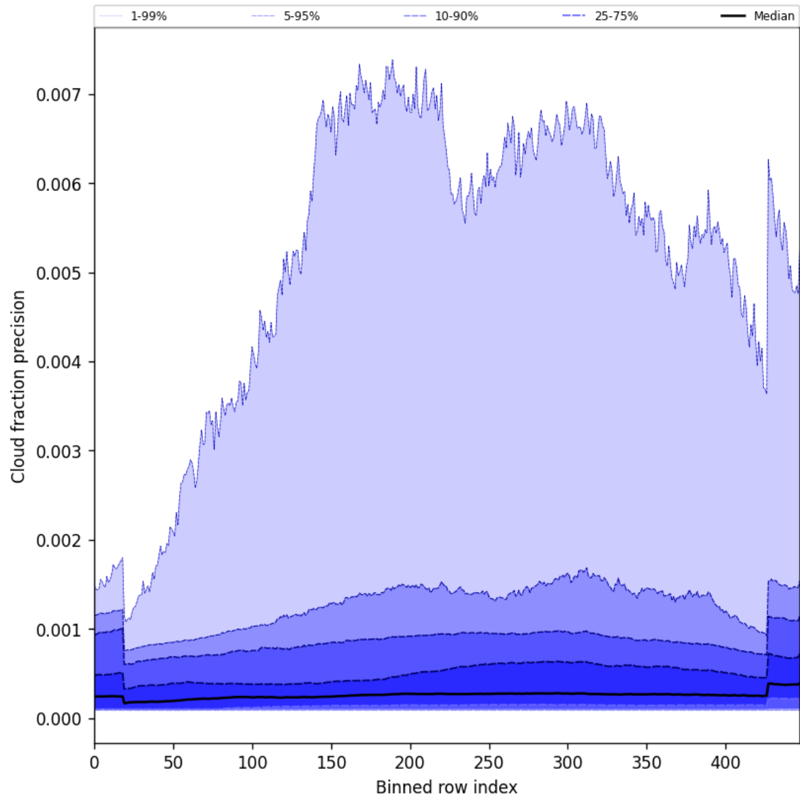
Figure 50: Along track statistics of “Cloud fraction precision” for 2024-10-15 to 2024-10-17
