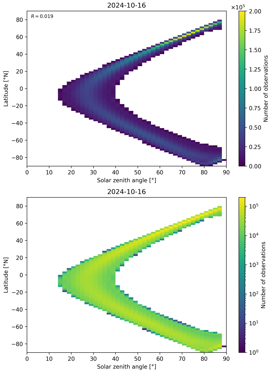
Figure 124: Scatter density plot of “Solar zenith angle” against “Latitude” for 2024-10-15 to 2024-10-17.
