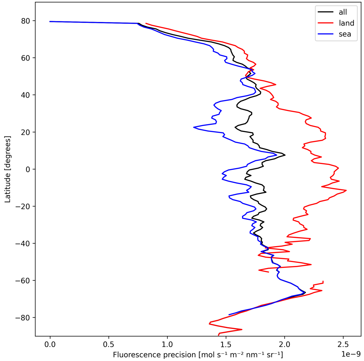
Figure 24: Zonal average of “Fluorescence precision” for 2024-10-15 to 2024-10-17.
