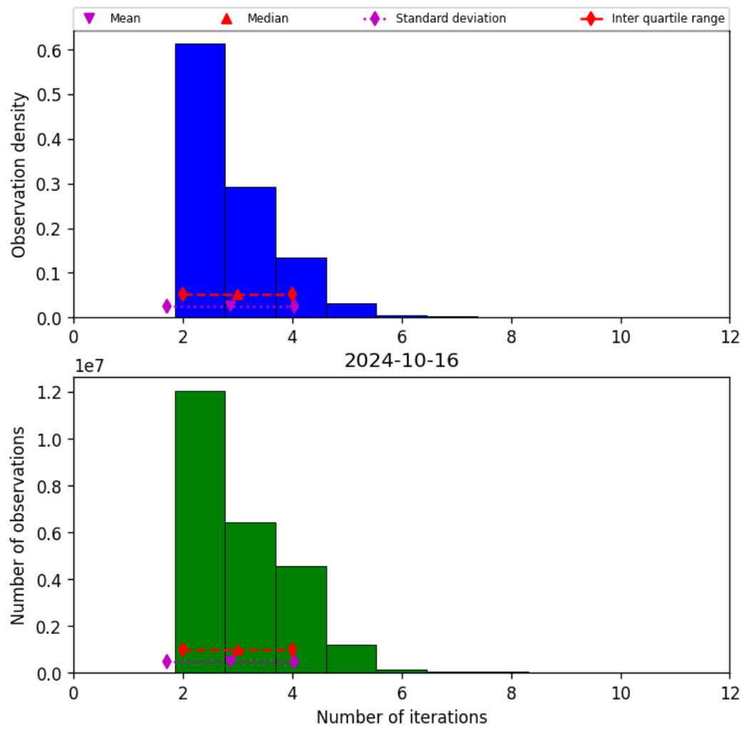
Figure 39: Histogram of “Number of iterations” for 2024-10-15 to 2024-10-17
