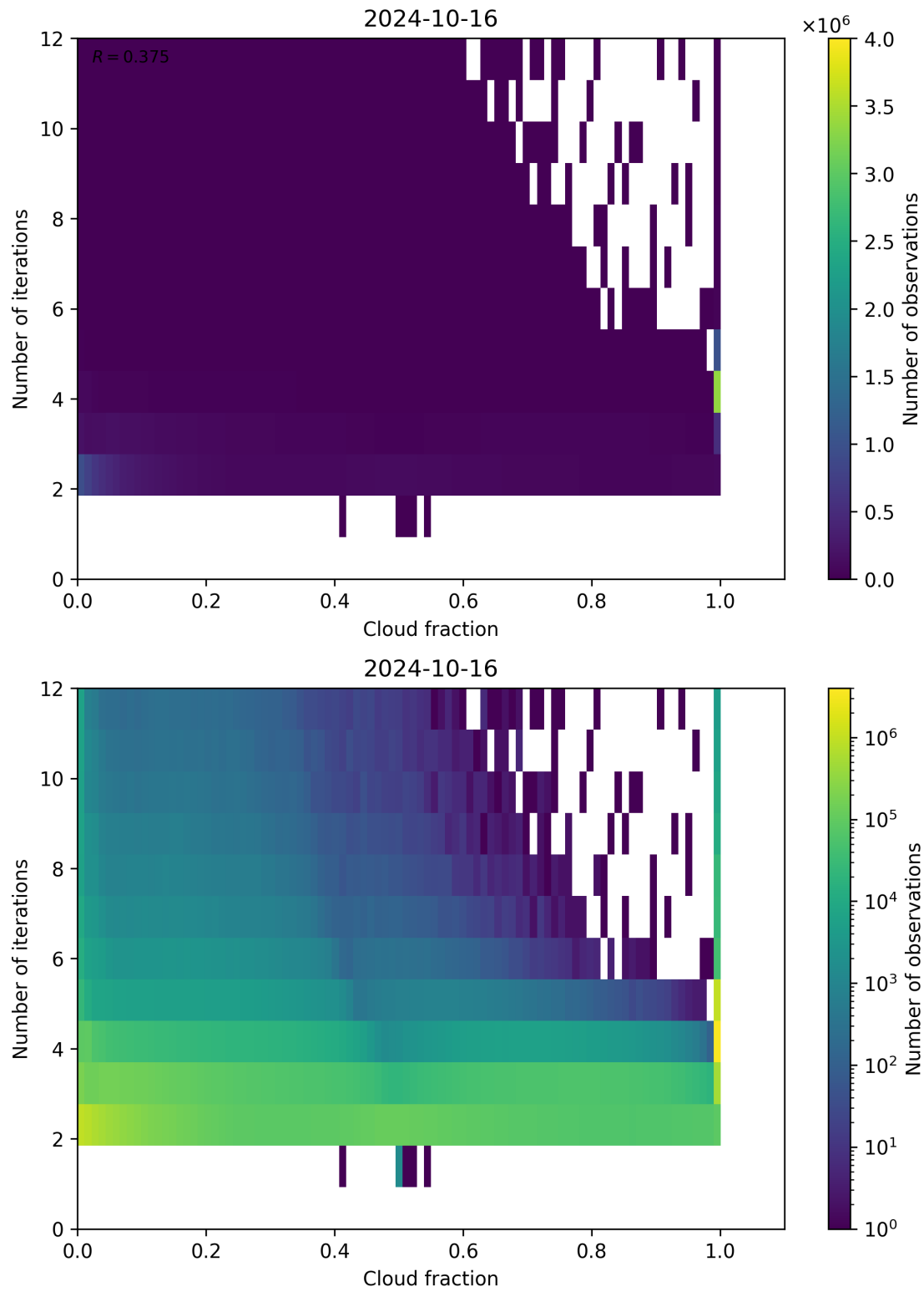
Figure 80: Scatter density plot of “Cloud fraction” against “Number of iterations” for 2024-10-15 to 2024-10-17.
