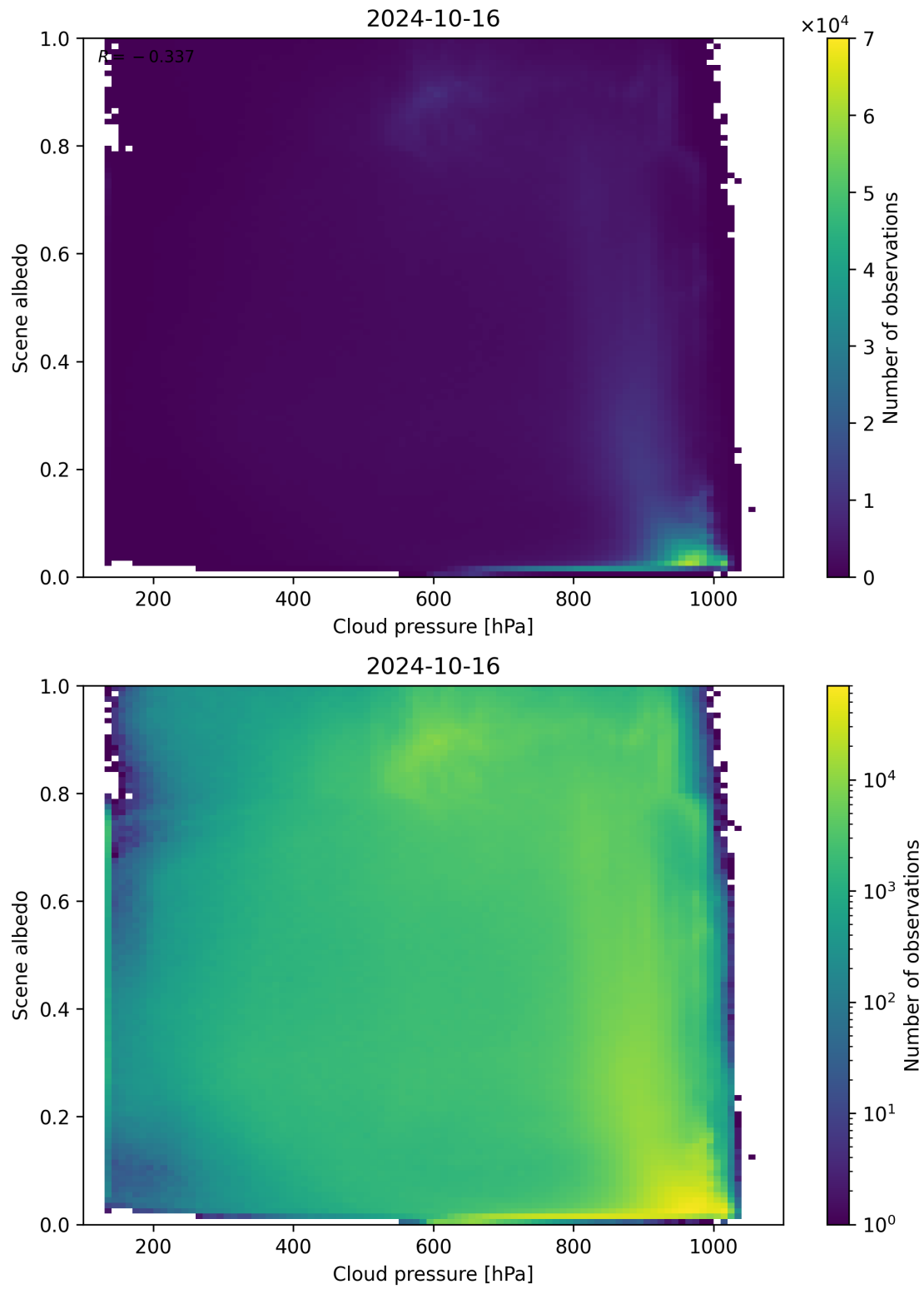
Figure 91: Scatter density plot of “Cloud pressure” against “Scene albedo” for 2024-10-15 to 2024-10-17.
