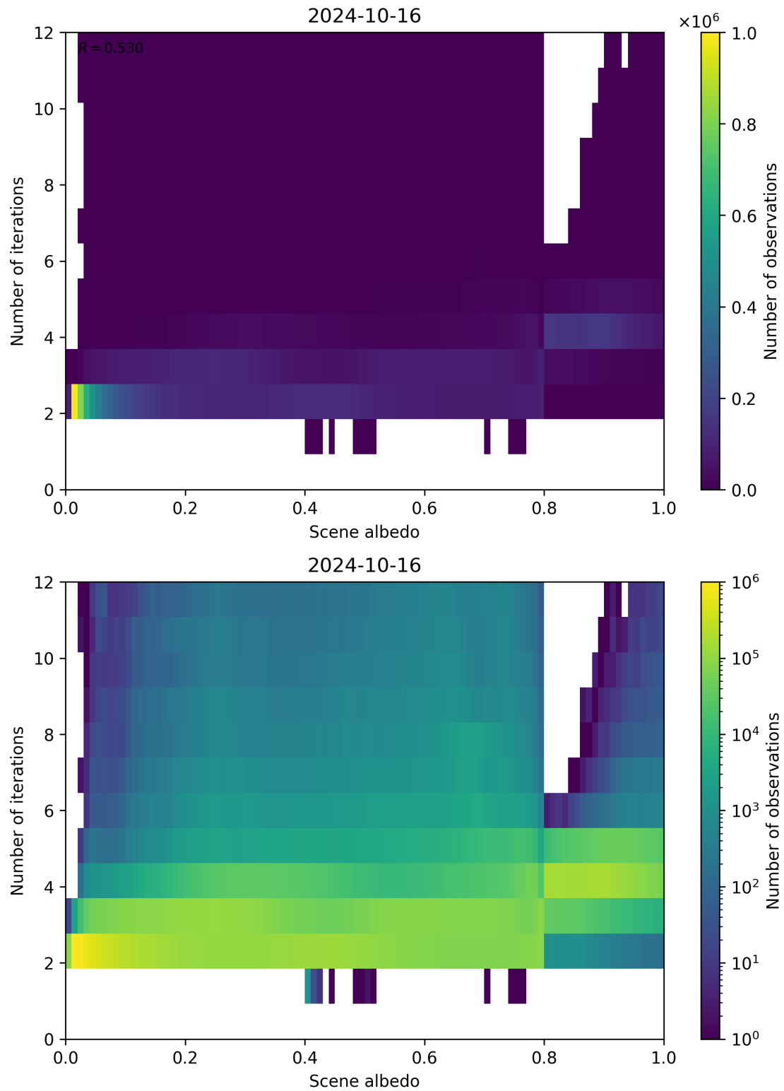
Figure 115: Scatter density plot of “Scene albedo” against “Number of iterations” for 2024-10-15 to 2024-10-17.
