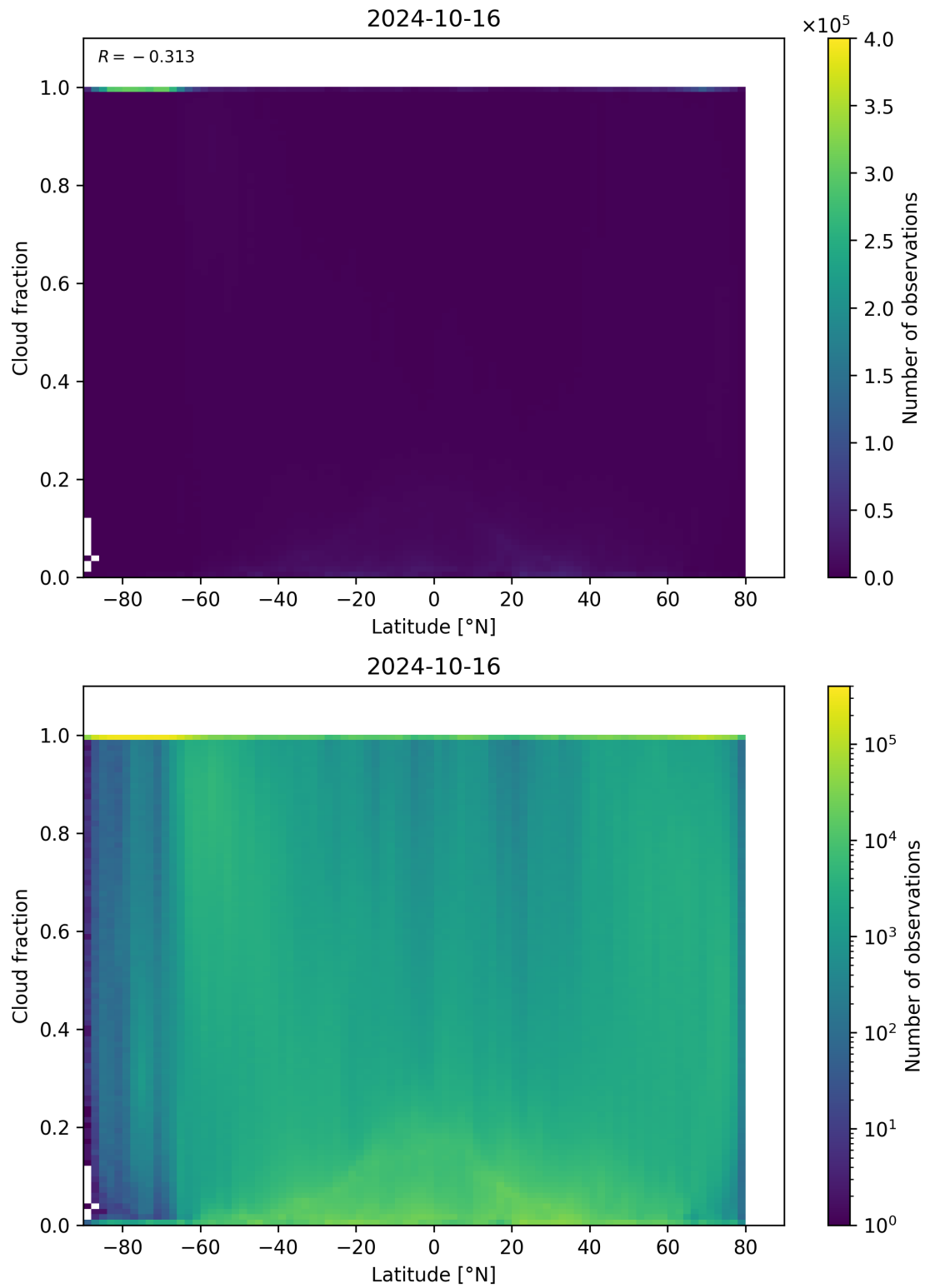
Figure 99: Scatter density plot of “Latitude” against “Cloud fraction” for 2024-10-15 to 2024-10-17.
