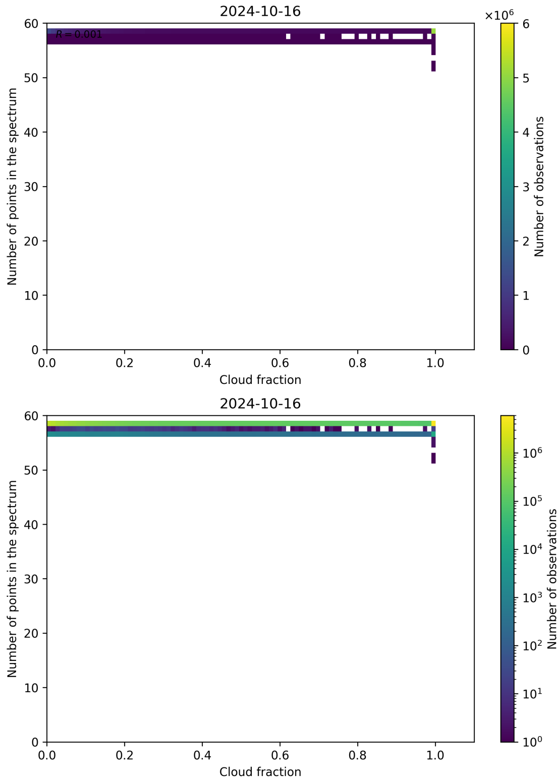
Figure 81: Scatter density plot of “Cloud fraction” against “Number of points in the spectrum” for 2024-10-15 to 2024-10-17.
