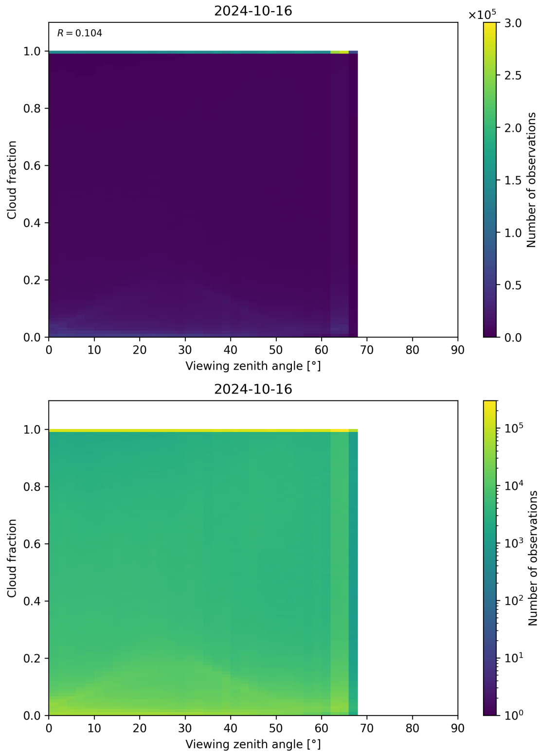
Figure 132: Scatter density plot of “Viewing zenith angle” against “Cloud fraction” for 2024-10-15 to 2024-10-17.
