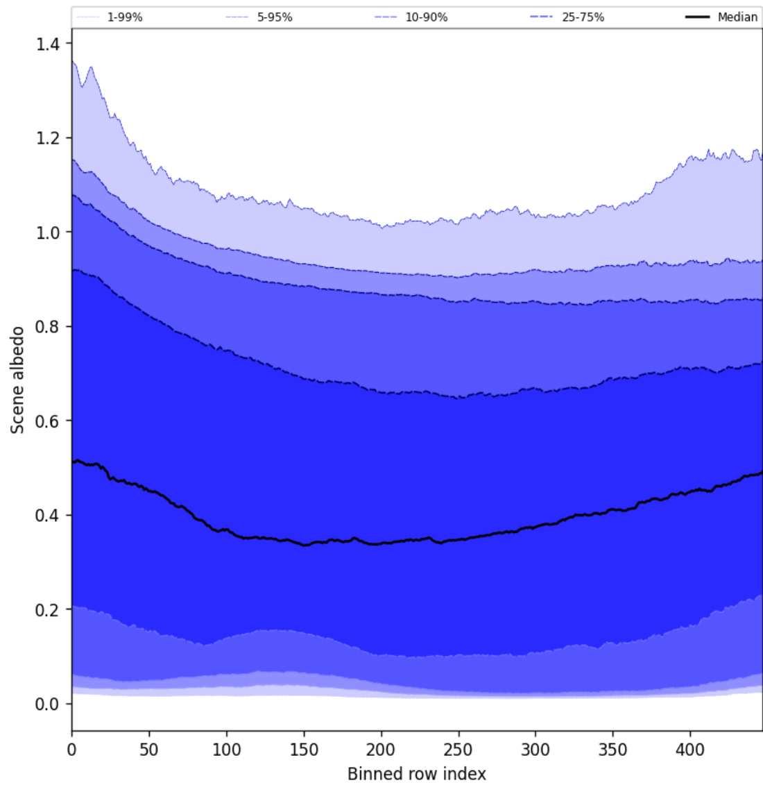
Figure 51: Along track statistics of “Scene albedo” for 2024-10-15 to 2024-10-17
