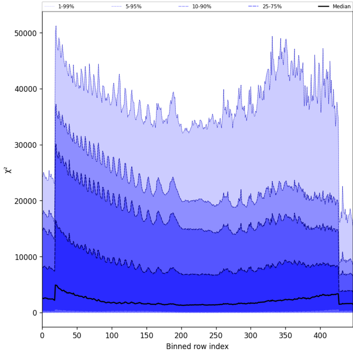
Figure 55: Along track statistics of “ \chi^2 ” for 2024-10-15 to 2024-10-17
