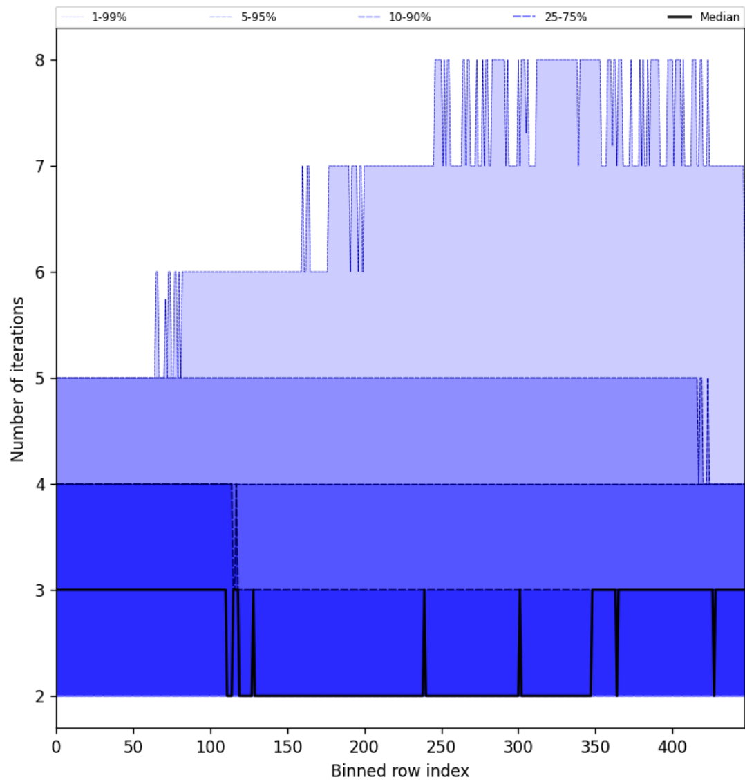
Figure 56: Along track statistics of “Number of iterations” for 2024-10-15 to 2024-10-17
