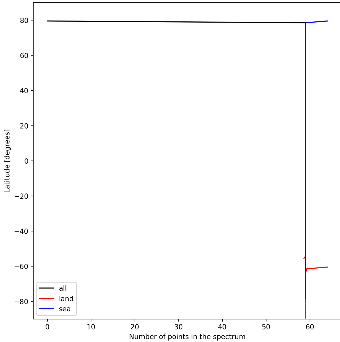
Figure 27: Zonal average of “Number of points in the spectrum” for 2024-10-15 to 2024-10-17.
