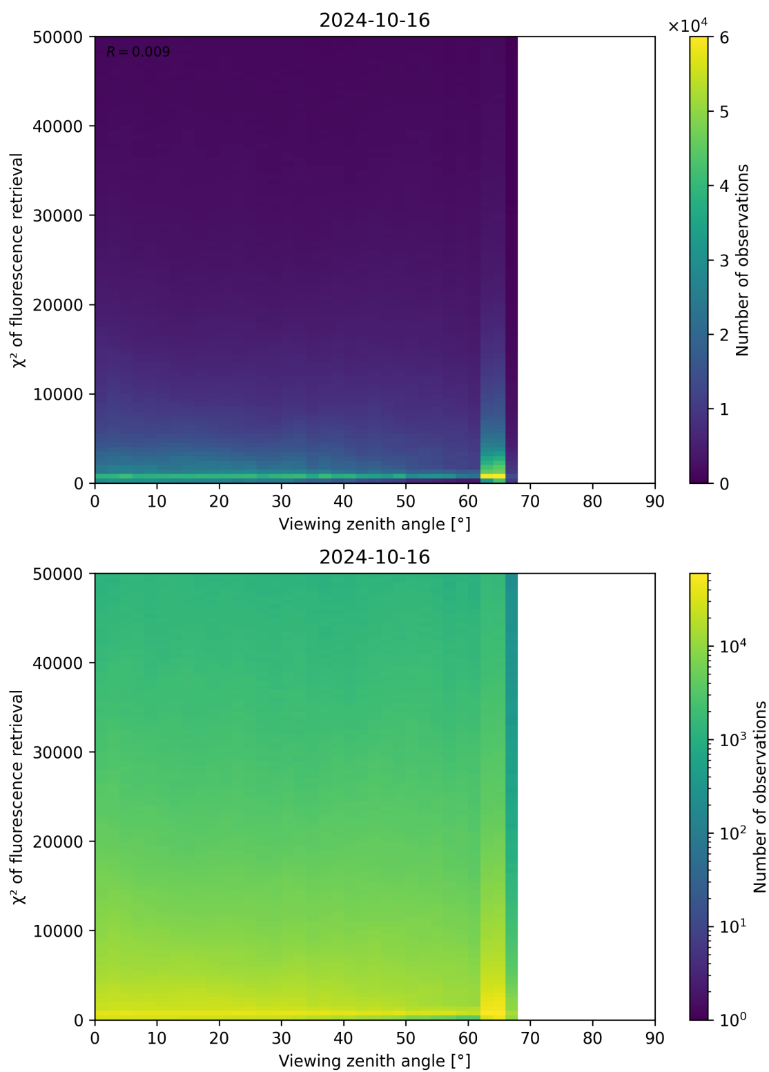
Figure 131: Scatter density plot of “Viewing zenith angle” against “ \chi^2 of fluorescence retrieval” for 2024-10-15 to 2024-10-17.
