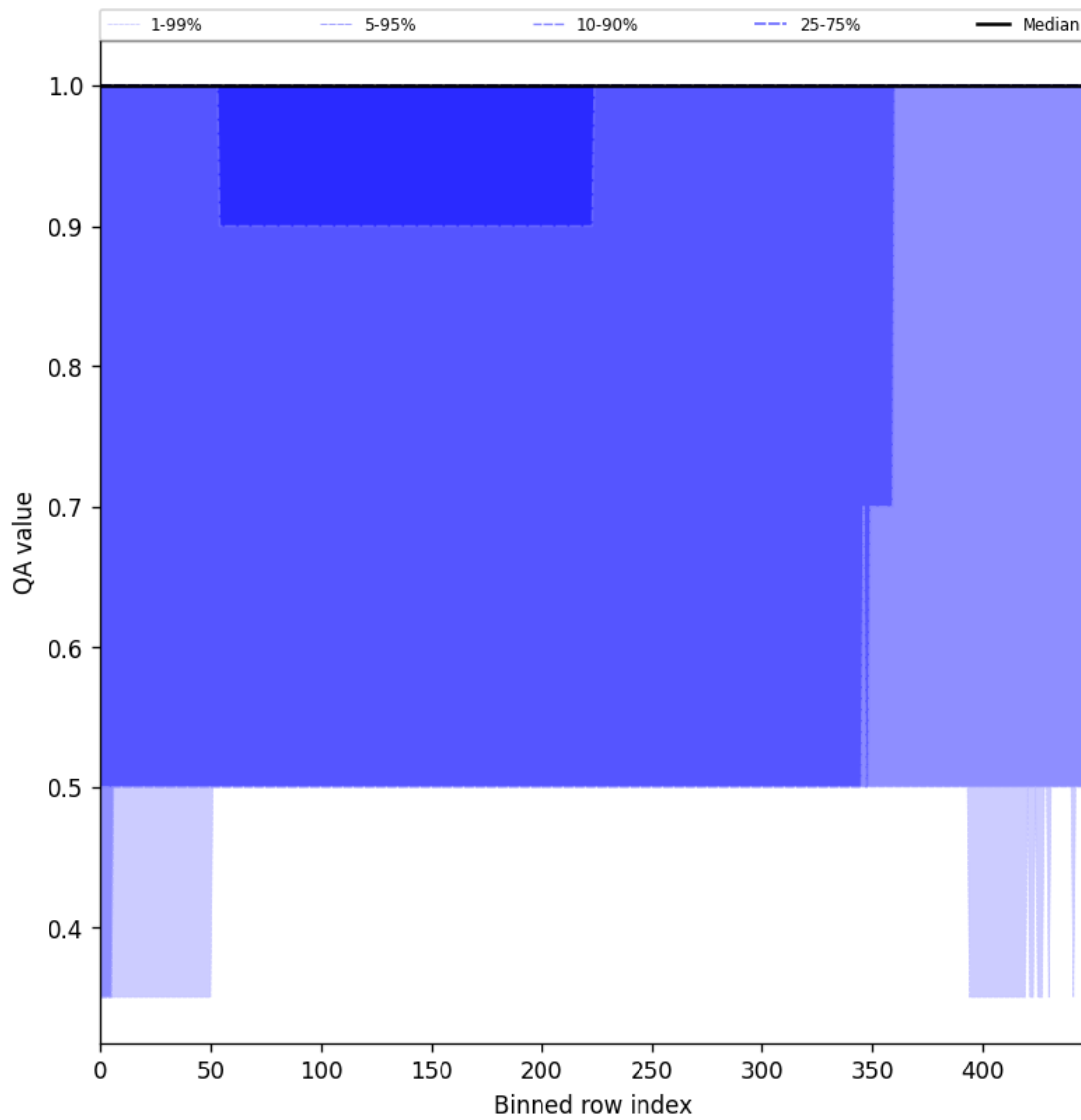
Figure 46: Along track statistics of “QA value” for 2024-10-15 to 2024-10-17
