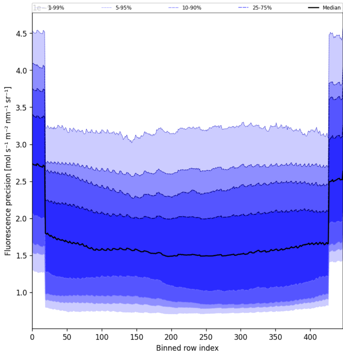
Figure 58: Along track statistics of “Fluorescence precision” for 2024-10-15 to 2024-10-17
