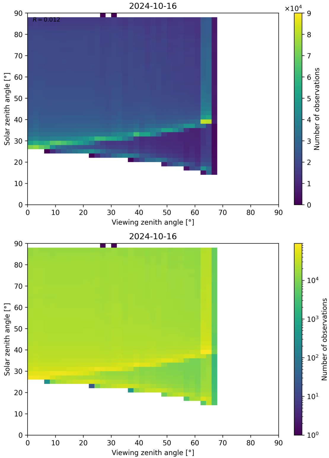
Figure 139: Scatter density plot of “Viewing zenith angle” against “Solar zenith angle” for 2024-10-15 to 2024-10-17.
