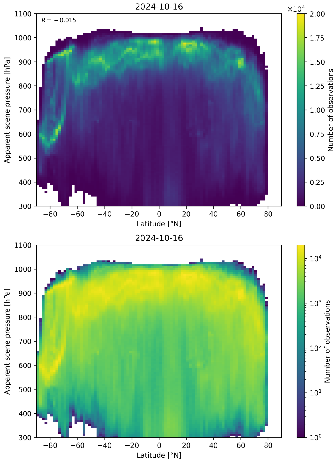
Figure 96: Scatter density plot of “Latitude” against “Apparent scene pressure” for 2024-10-15 to 2024-10-17.
