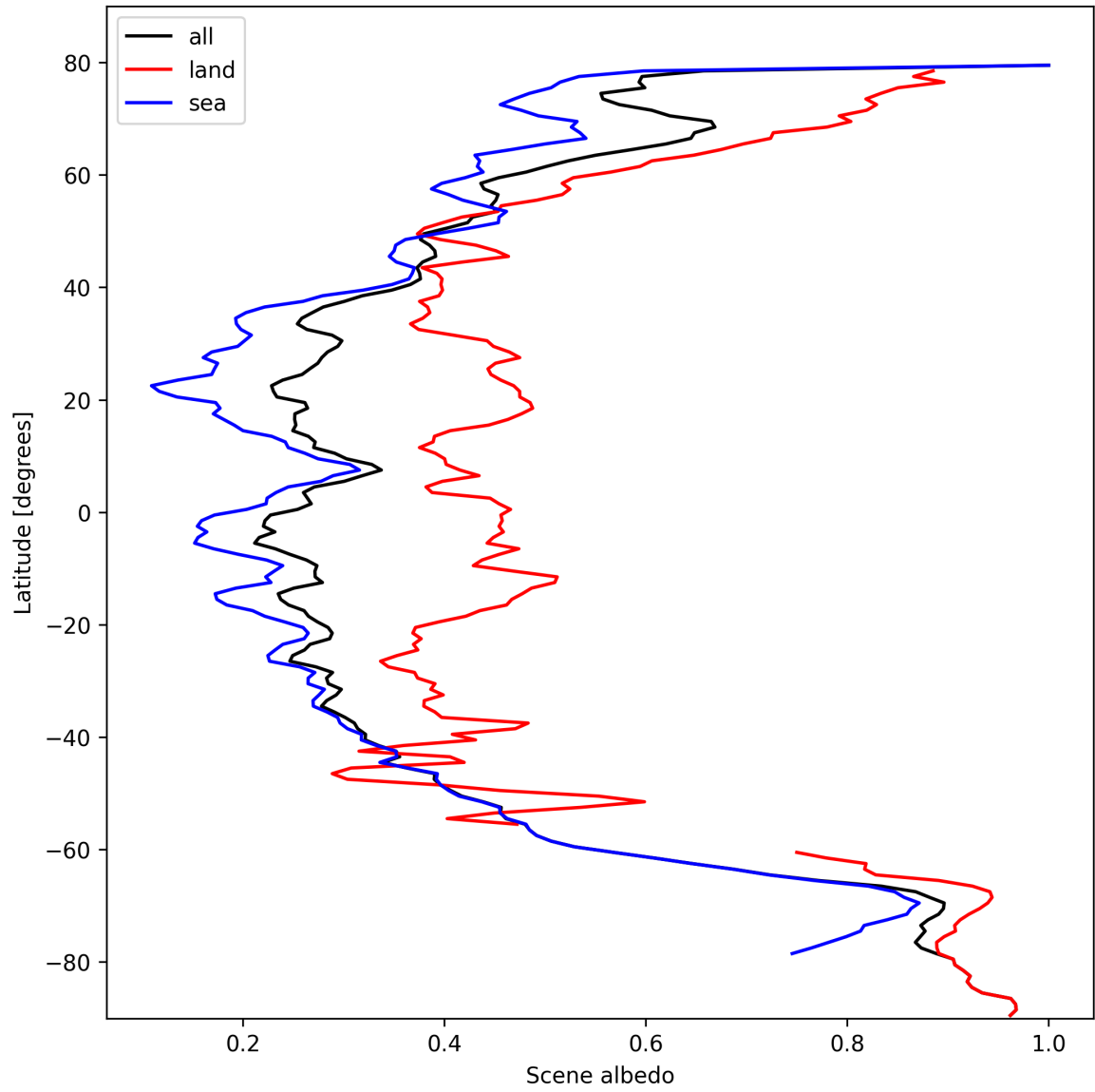
Figure 17: Zonal average of “Scene albedo” for 2024-10-15 to 2024-10-17.
