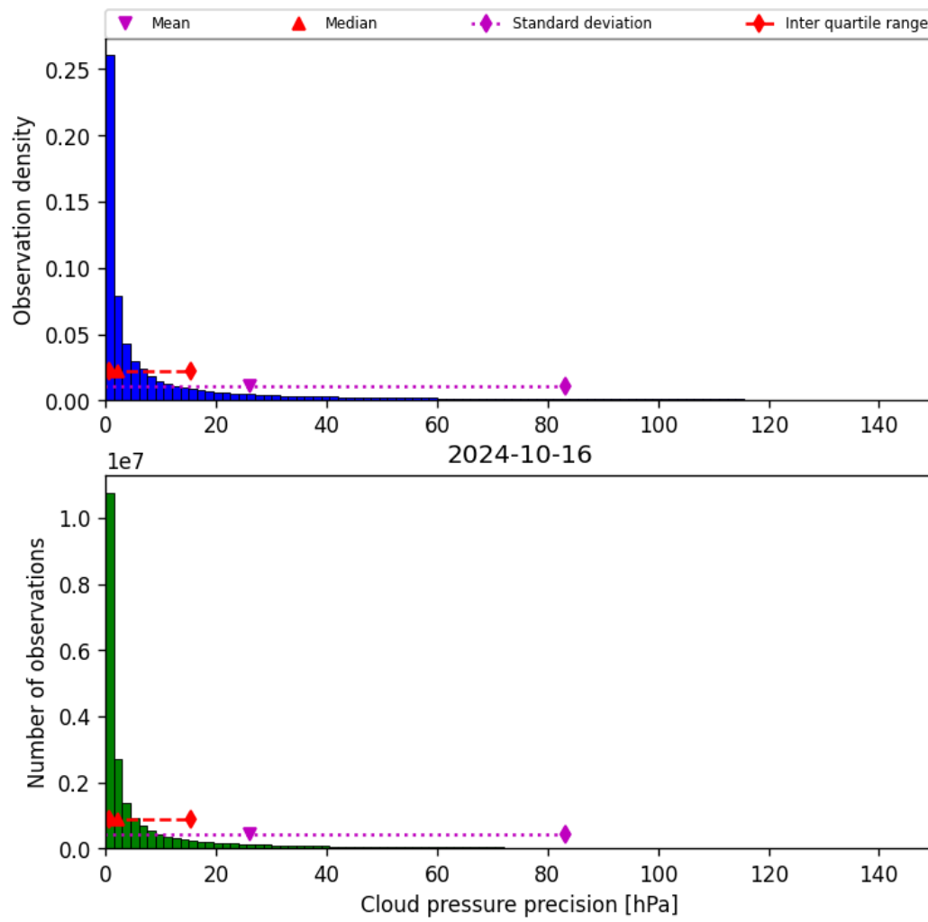
Figure 31: Histogram of “Cloud pressure precision” for 2024-10-15 to 2024-10-17
