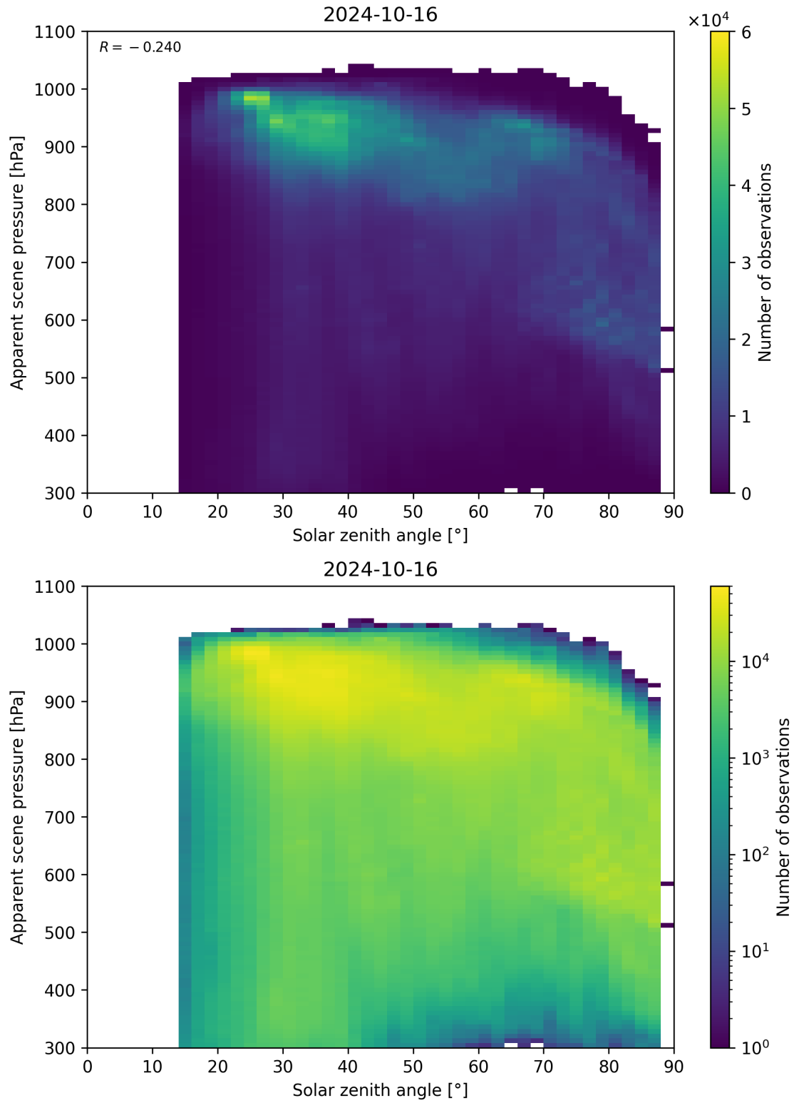
Figure 118: Scatter density plot of “Solar zenith angle” against “Apparent scene pressure” for 2024-10-15 to 2024-10-17.
