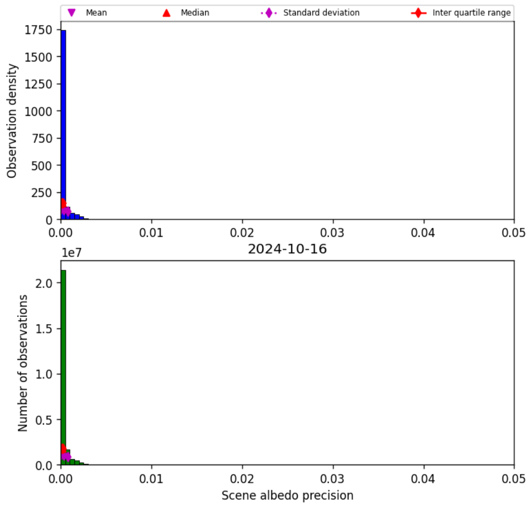
Figure 35: Histogram of “Scene albedo precision” for 2024-10-15 to 2024-10-17
