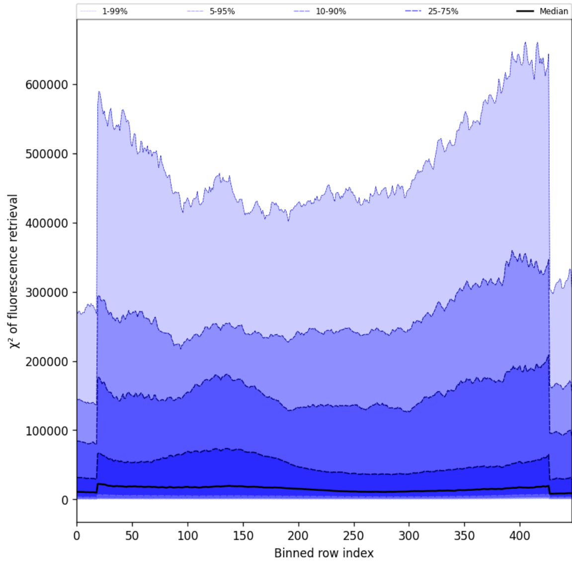
Figure 59: Along track statistics of “ \chi^2 of fluorescence retrieval” for 2024-10-15 to 2024-10-17
