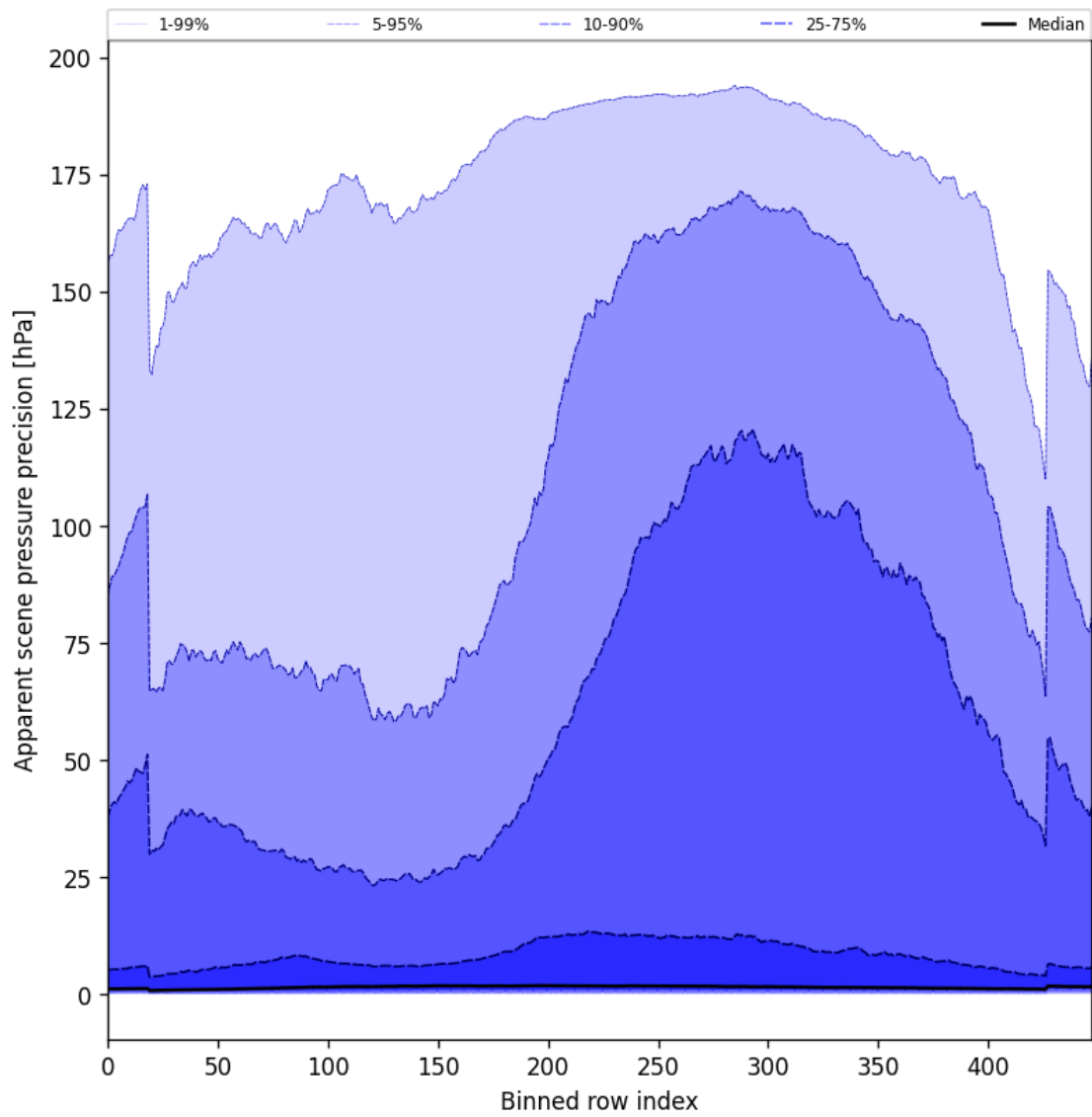
Figure 54: Along track statistics of “Apparent scene pressure precision” for 2024-10-15 to 2024-10-17
