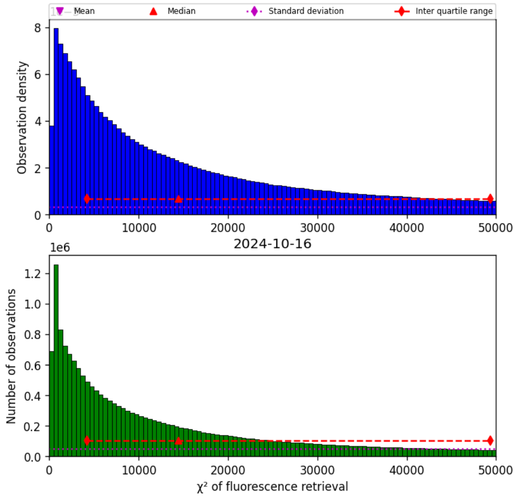
Figure 42: Histogram of “ \chi^2 of fluorescence retrieval” for 2024-10-15 to 2024-10-17
