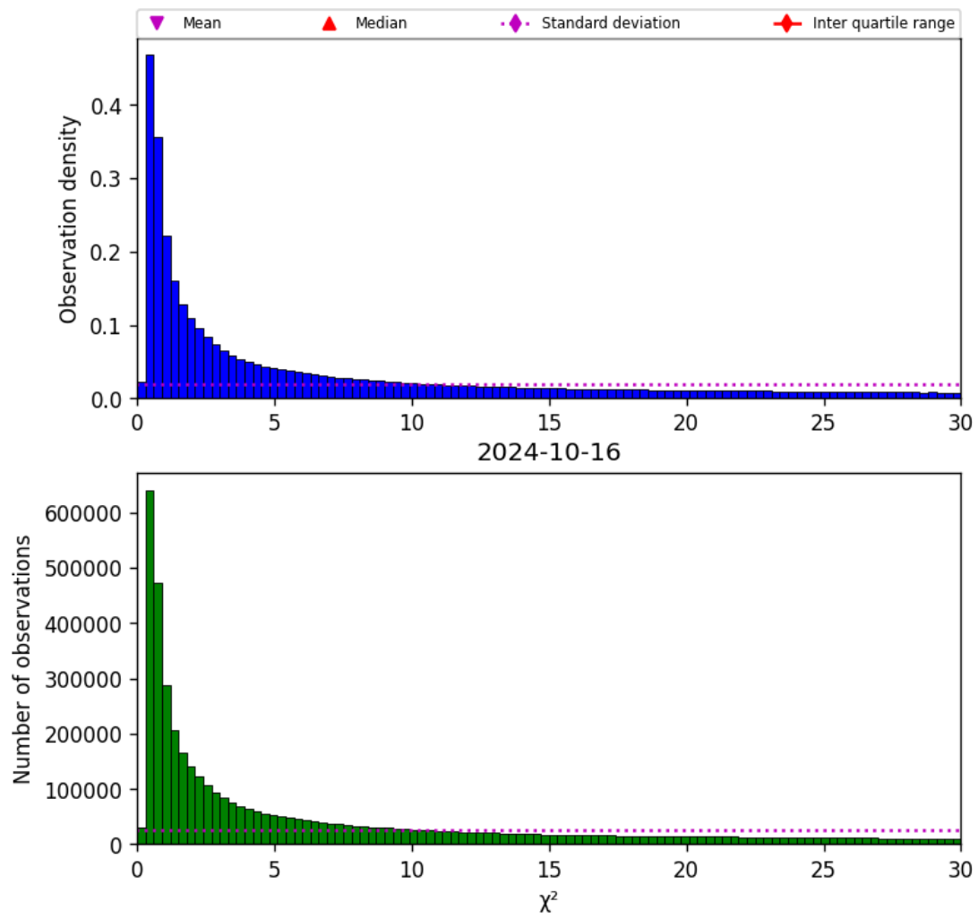
Figure 38: Histogram of “ \chi^2 ” for 2024-10-15 to 2024-10-17
