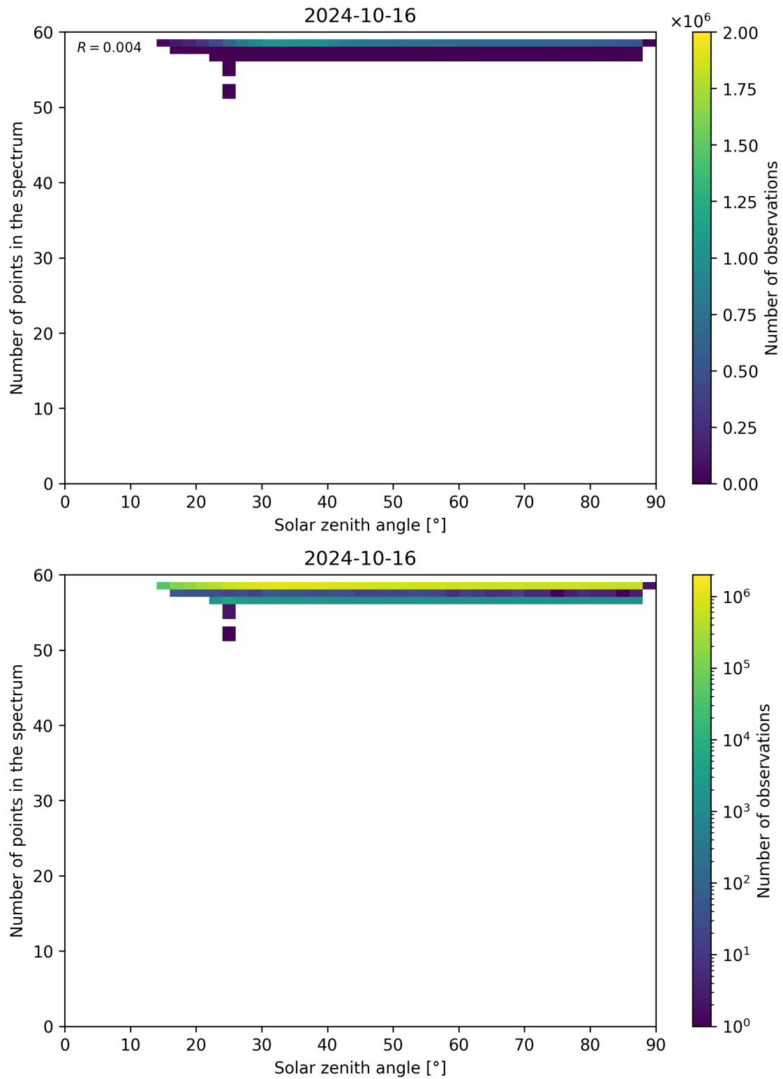
Figure 126: Scatter density plot of “Solar zenith angle” against “Number of points in the spectrum” for 2024-10-15 to 2024-10-17.
