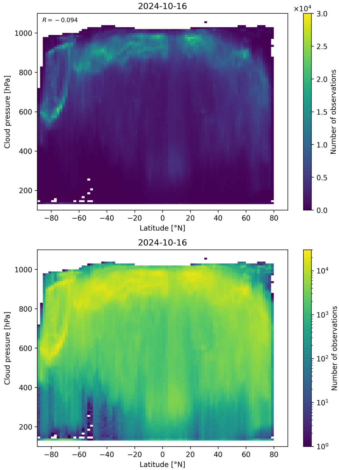
Figure 100: Scatter density plot of “Latitude” against “Cloud pressure” for 2024-10-15 to 2024-10-17.
