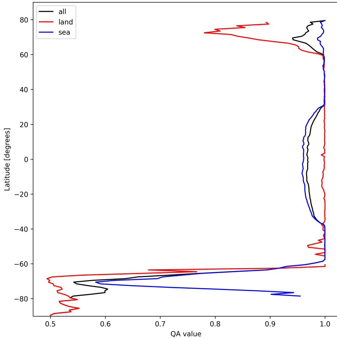
Figure 12: Zonal average of “QA value” for 2024-10-15 to 2024-10-17.
