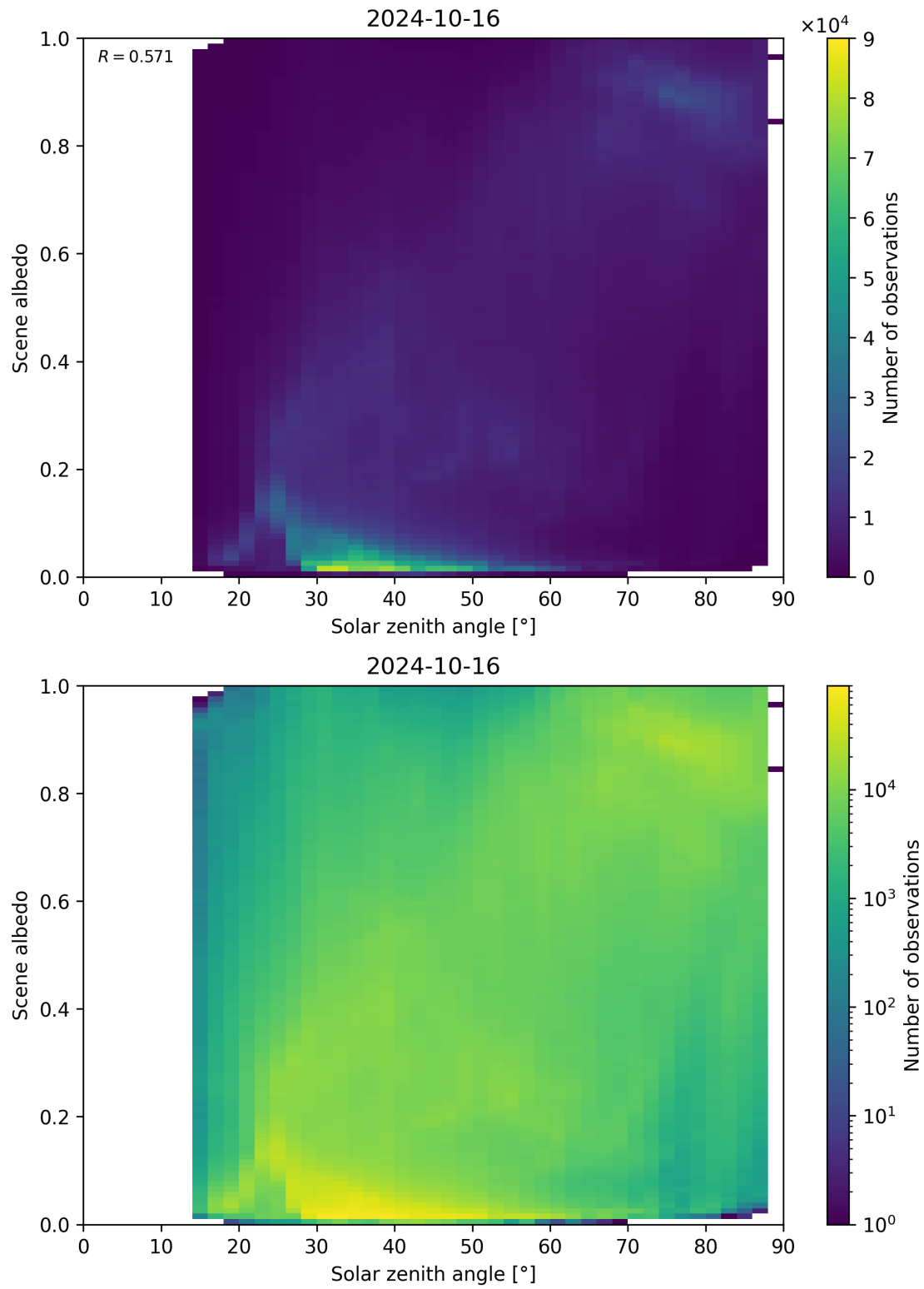
Figure 127: Scatter density plot of “Solar zenith angle” against “Scene albedo” for 2024-10-15 to 2024-10-17.
