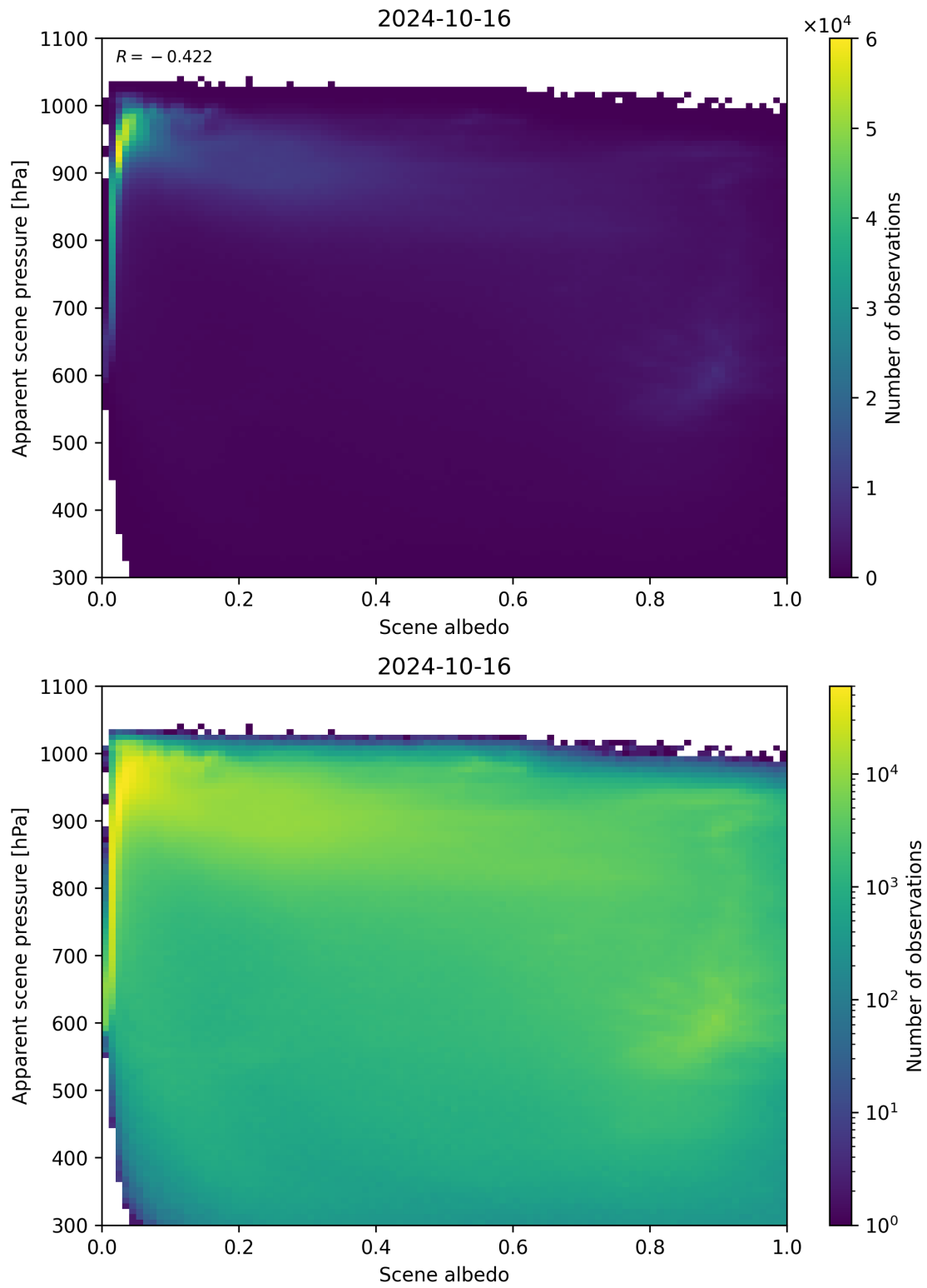
Figure 111: Scatter density plot of “Scene albedo” against “Apparent scene pressure” for 2024-10-15 to 2024-10-17.
