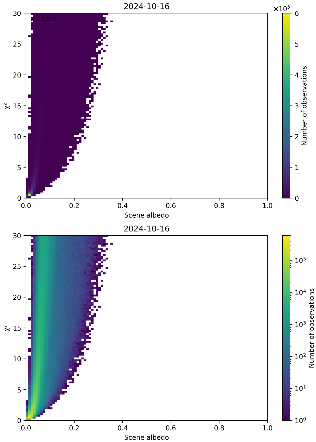
Figure 112: Scatter density plot of “Scene albedo” against “ \chi^2 ” for 2024-10-15 to 2024-10-17.
