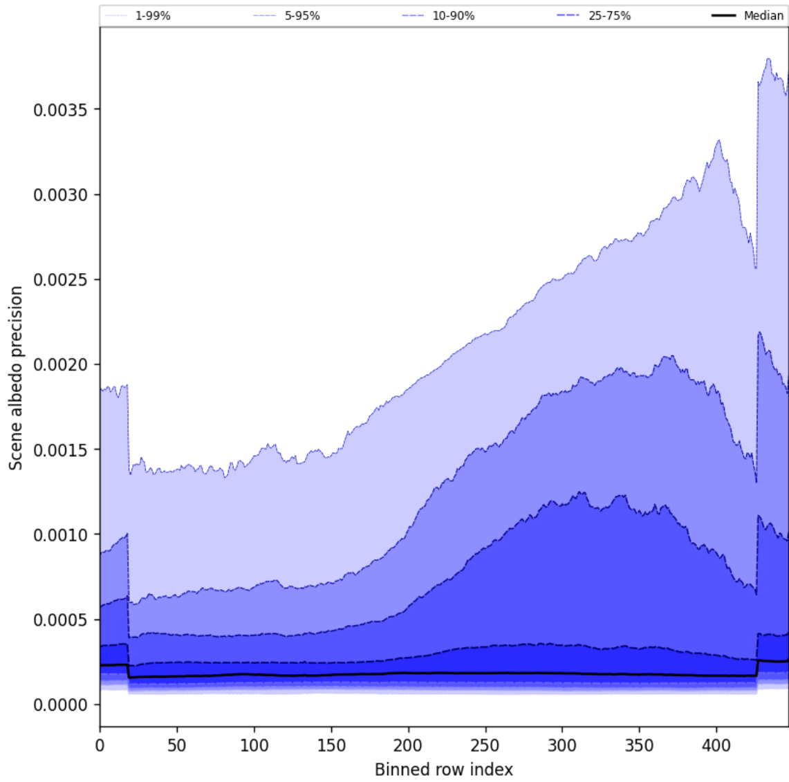
Figure 52: Along track statistics of “Scene albedo precision” for 2024-10-15 to 2024-10-17
