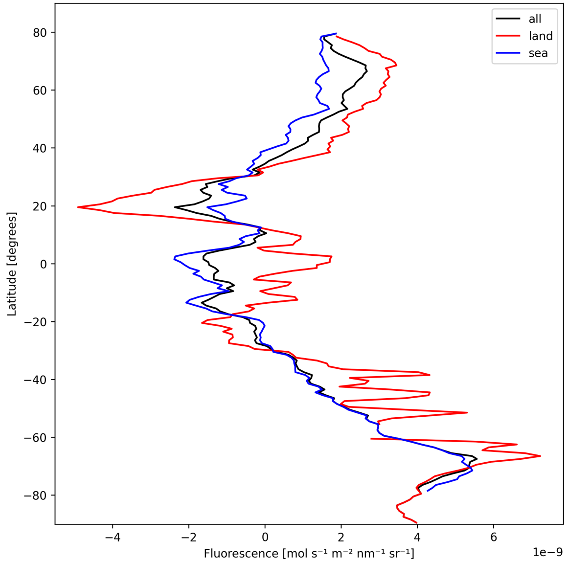
Figure 23: Zonal average of “Fluorescence” for 2024-10-15 to 2024-10-17.
