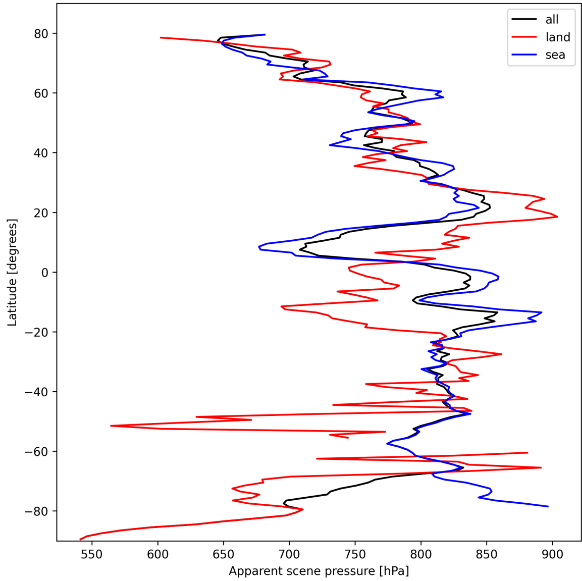
Figure 19: Zonal average of “Apparent scene pressure” for 2024-10-15 to 2024-10-17.
