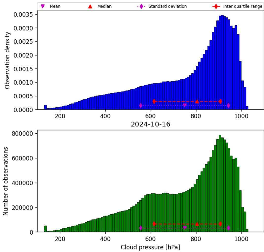
Figure 30: Histogram of “Cloud pressure” for 2024-10-15 to 2024-10-17
