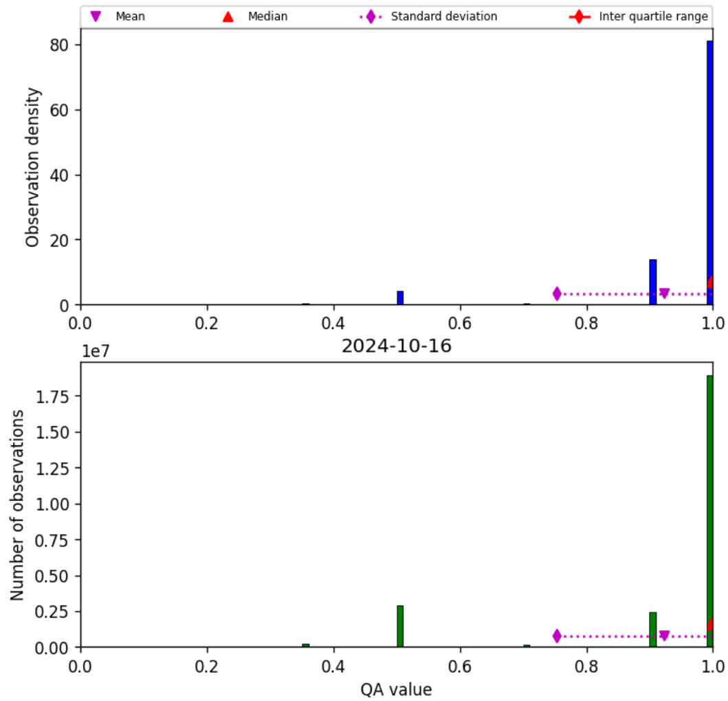
Figure 29: Histogram of “QA value” for 2024-10-15 to 2024-10-17
