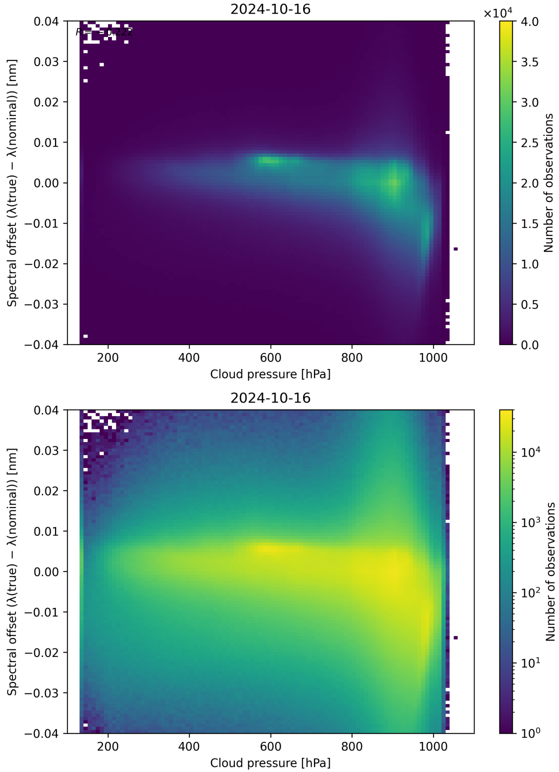
Figure 92: Scatter density plot of “Cloud pressure” against “Spectral offset ( \lambda_{\text{true}} - \lambda_{\text{nominal}} )” for 2024-10-15 to 2024-10-17.
