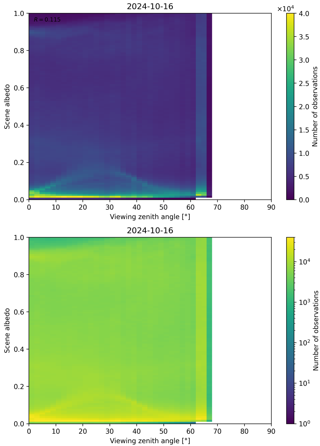
Figure 138: Scatter density plot of “Viewing zenith angle” against “Scene albedo” for 2024-10-15 to 2024-10-17.
