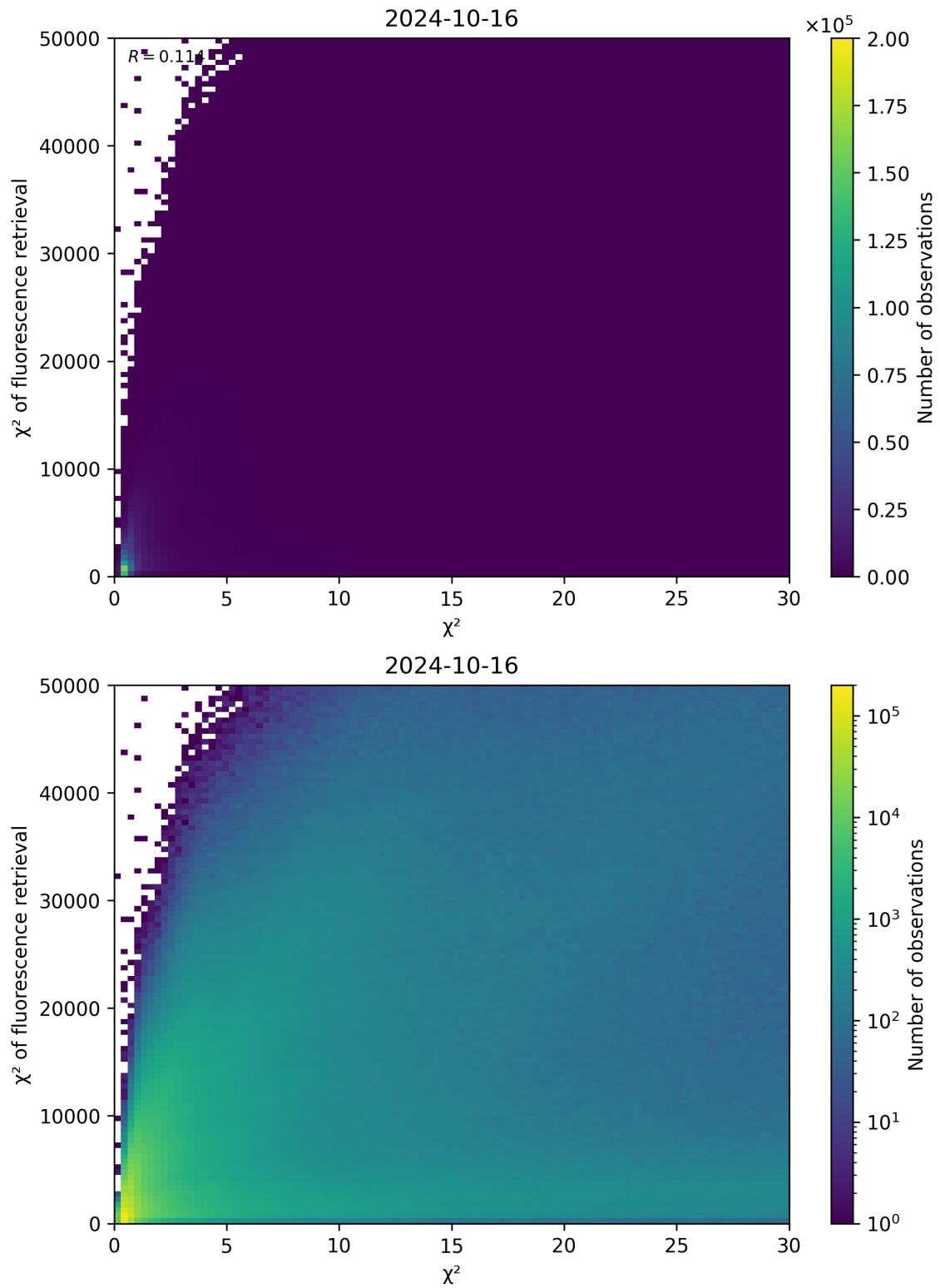
Figure 69: Scatter density plot of “ \chi^2 ” against “ \chi^2 of fluorescence retrieval” for 2024-10-15 to 2024-10-17.
