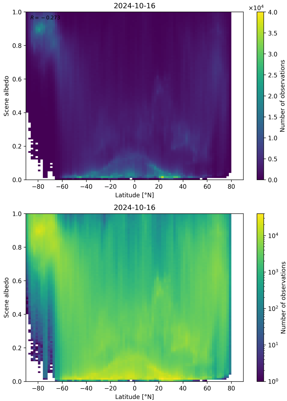
Figure 104: Scatter density plot of “Latitude” against “Scene albedo” for 2024-10-15 to 2024-10-17.
