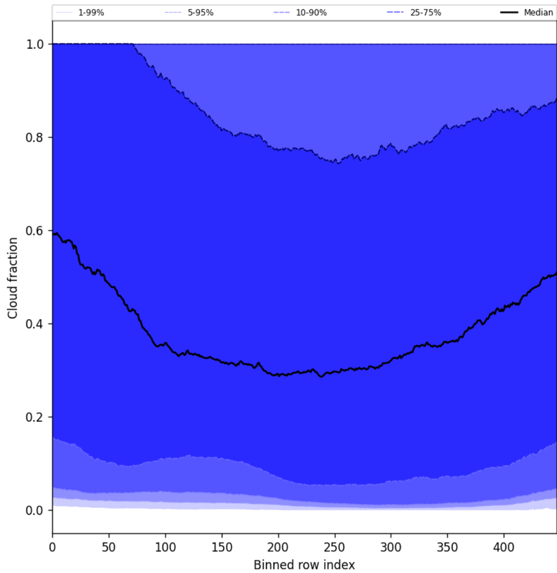
Figure 49: Along track statistics of “Cloud fraction” for 2024-10-15 to 2024-10-17
