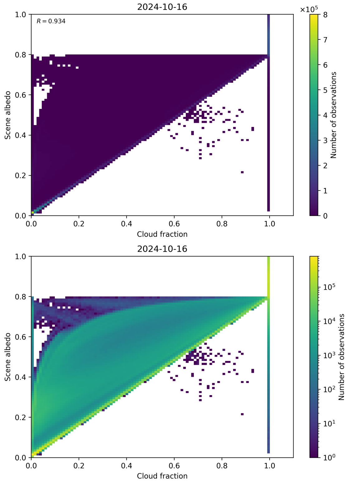
Figure 82: Scatter density plot of “Cloud fraction” against “Scene albedo” for 2024-10-15 to 2024-10-17.
