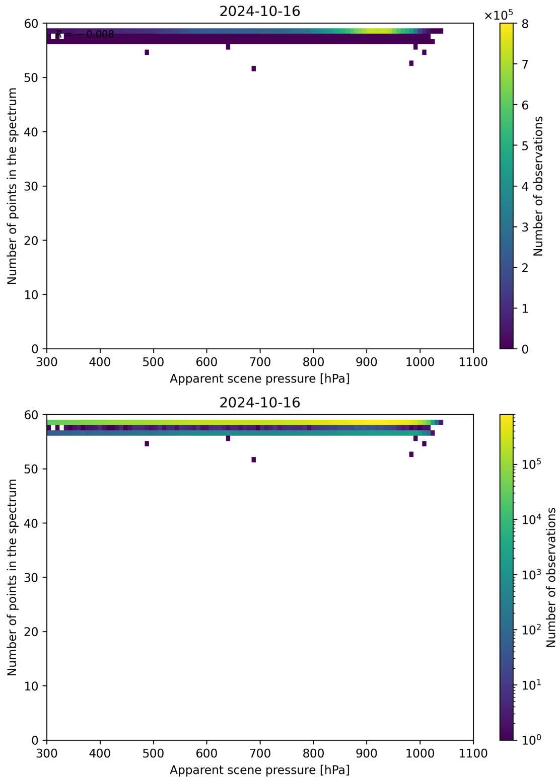
Figure 67: Scatter density plot of “Apparent scene pressure” against “Number of points in the spectrum” for 2024-10-15 to 2024-10-17.
