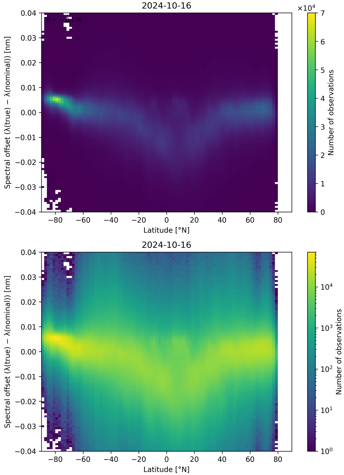
Figure 105: Scatter density plot of “Latitude” against “Spectral offset ( \lambda_{\text{true}} - \lambda_{\text{nominal}} )” for 2024-10-15 to 2024-10-17.
