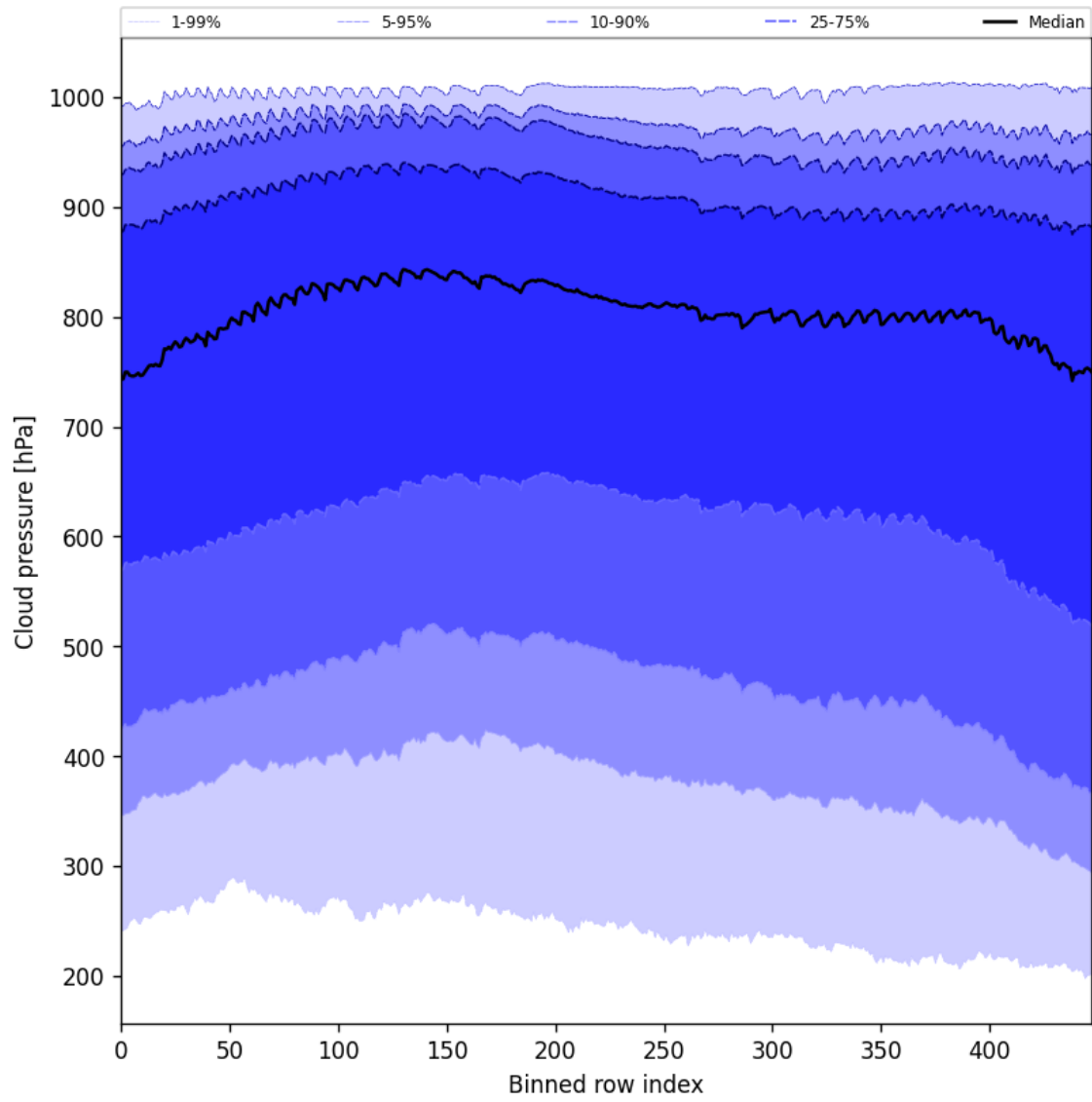
Figure 47: Along track statistics of “Cloud pressure” for 2024-10-15 to 2024-10-17
