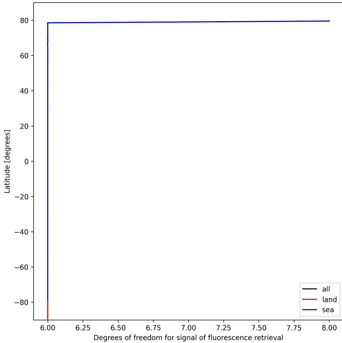
Figure 26: Zonal average of “Degrees of freedom for signal of fluorescence retrieval” for 2024-10-15 to 2024-10-17.
