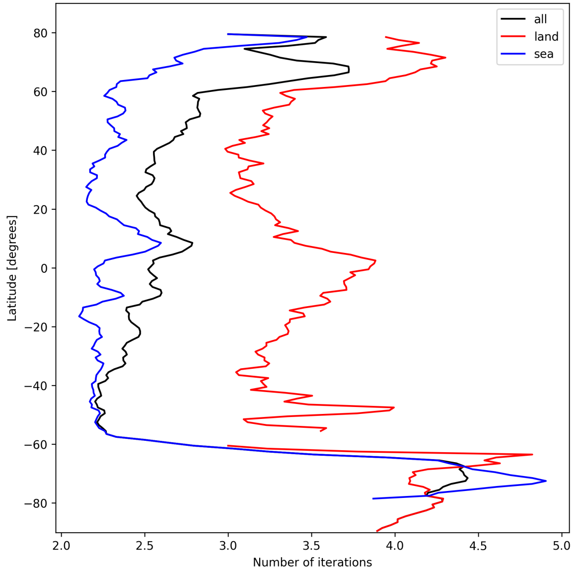
Figure 22: Zonal average of “Number of iterations” for 2024-10-15 to 2024-10-17.
