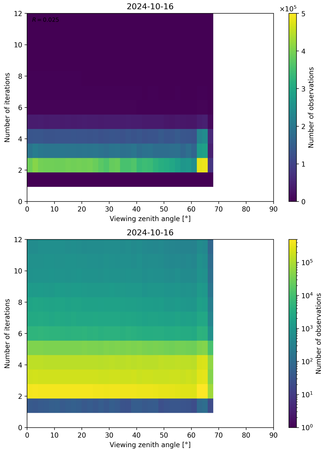
Figure 136: Scatter density plot of “Viewing zenith angle” against “Number of iterations” for 2024-10-15 to 2024-10-17.
