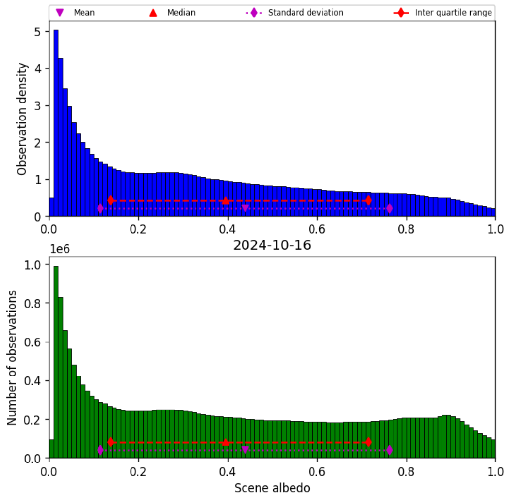
Figure 34: Histogram of “Scene albedo” for 2024-10-15 to 2024-10-17
