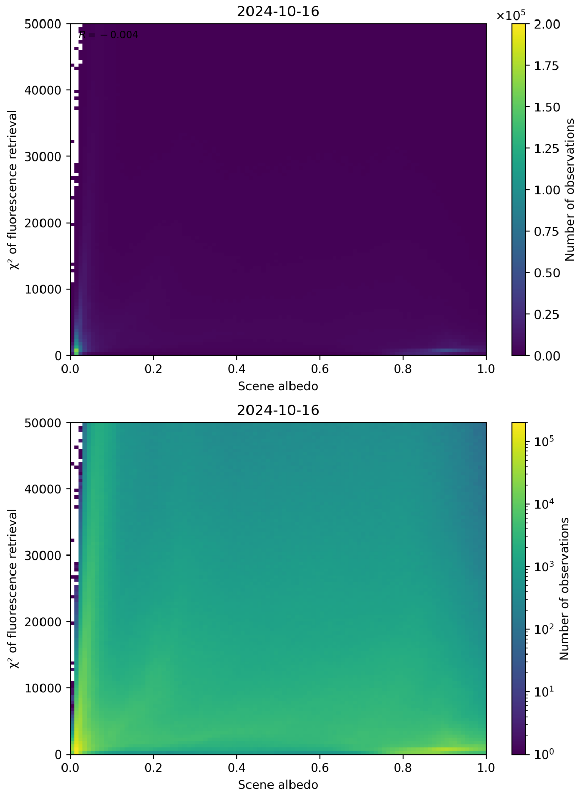
Figure 113: Scatter density plot of “Scene albedo” against “ \chi^2 of fluorescence retrieval” for 2024-10-15 to 2024-10-17.
