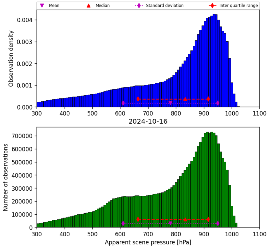
Figure 36: Histogram of “Apparent scene pressure” for 2024-10-15 to 2024-10-17
