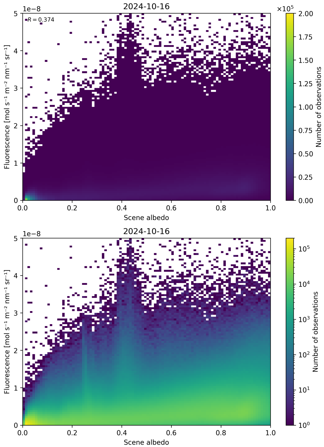
Figure 114: Scatter density plot of “Scene albedo” against “Fluorescence” for 2024-10-15 to 2024-10-17.
