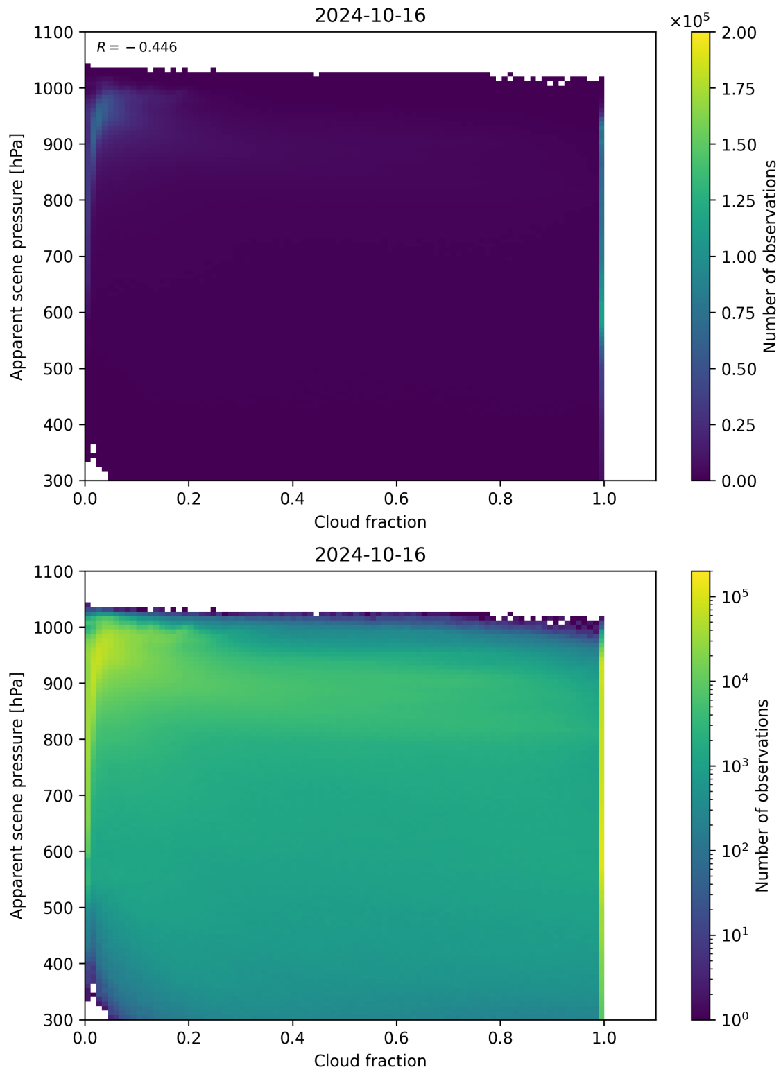
Figure 76: Scatter density plot of “Cloud fraction” against “Apparent scene pressure” for 2024-10-15 to 2024-10-17.
