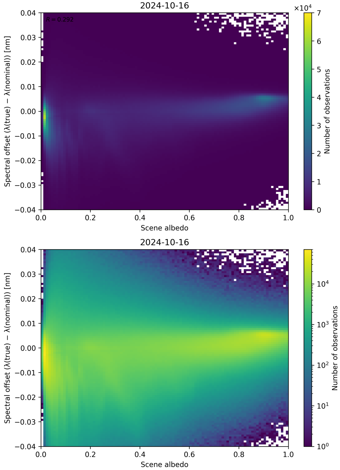
Figure 117: Scatter density plot of “Scene albedo” against “Spectral offset ( \lambda_{\text{true}} - \lambda_{\text{nominal}} )” for 2024-10-15 to 2024-10-17.
