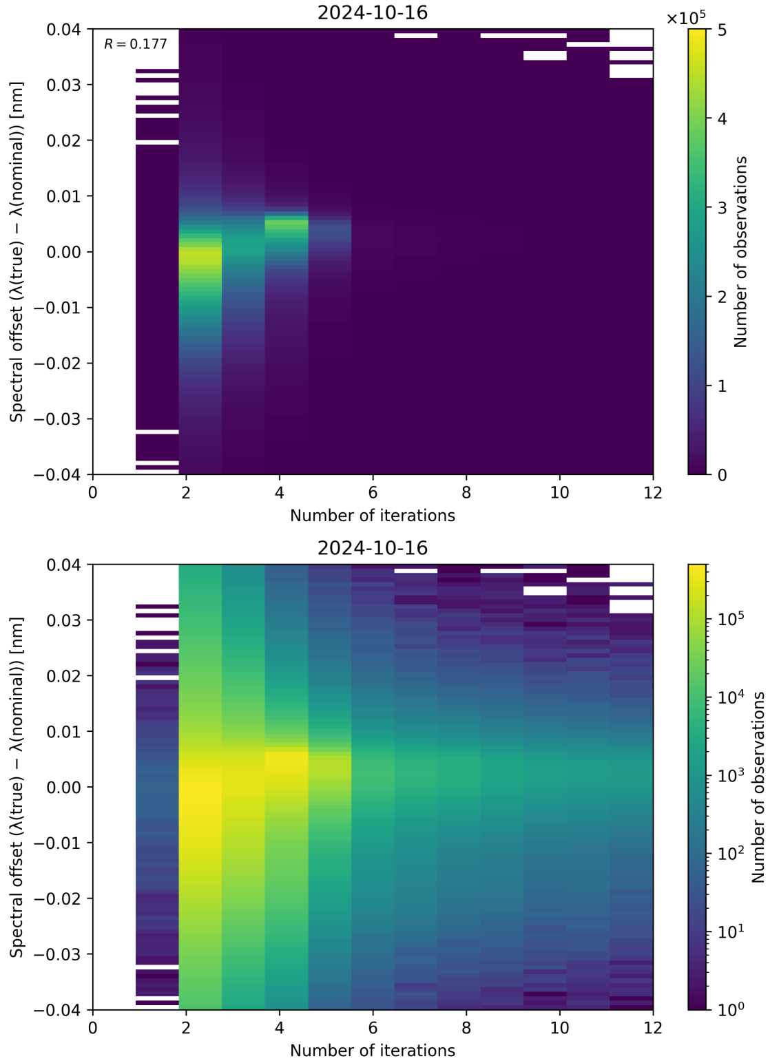
Figure 109: Scatter density plot of “Number of iterations” against “Spectral offset ( \lambda_{\text{true}} - \lambda_{\text{nominal}} )” for 2024-10-15 to 2024-10-17.
