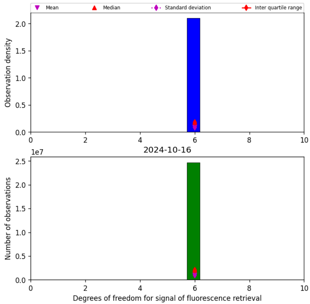
Figure 43: Histogram of “Degrees of freedom for signal of fluorescence retrieval” for 2024-10-15 to 2024-10-17
