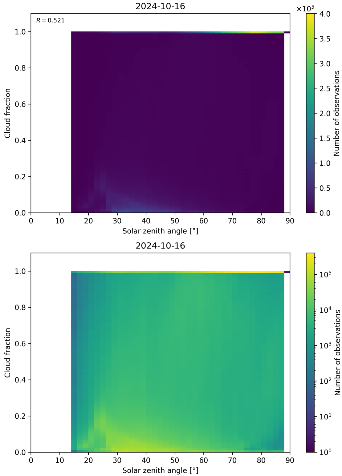
Figure 121: Scatter density plot of “Solar zenith angle” against “Cloud fraction” for 2024-10-15 to 2024-10-17.
