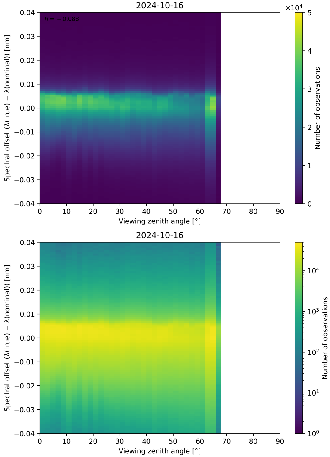
Figure 140: Scatter density plot of “Viewing zenith angle” against “Spectral offset ( \lambda_{\text{true}} - \lambda_{\text{nominal}} )” for 2024-10-15 to 2024-10-17.
