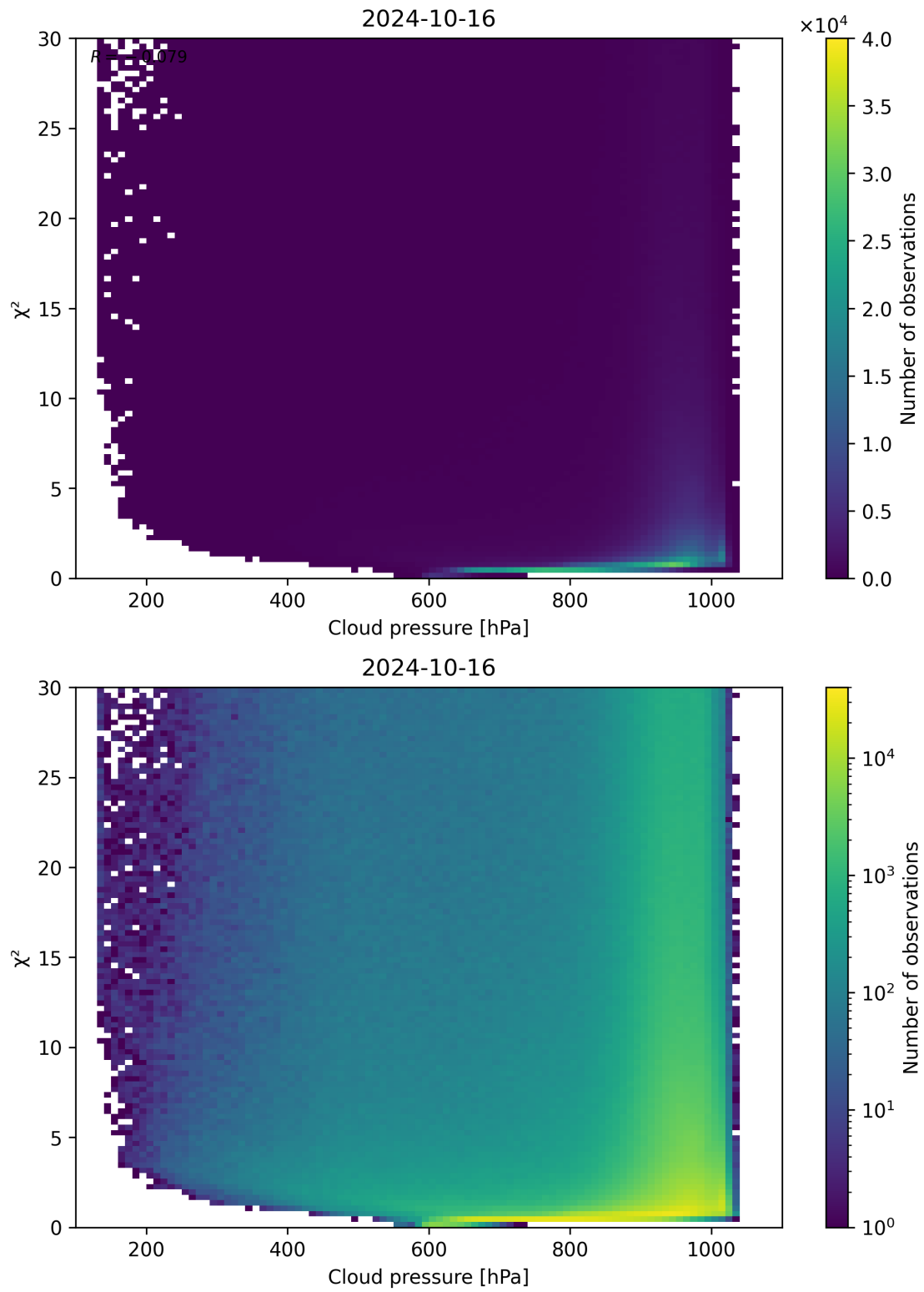
Figure 85: Scatter density plot of “Cloud pressure” against “ \chi^2 ” for 2024-10-15 to 2024-10-17.
