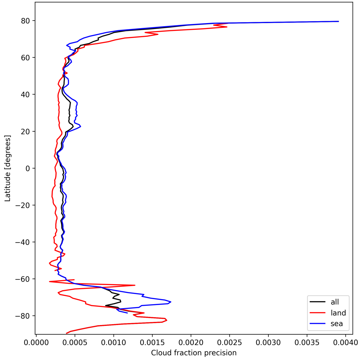
Figure 16: Zonal average of “Cloud fraction precision” for 2024-10-15 to 2024-10-17.
