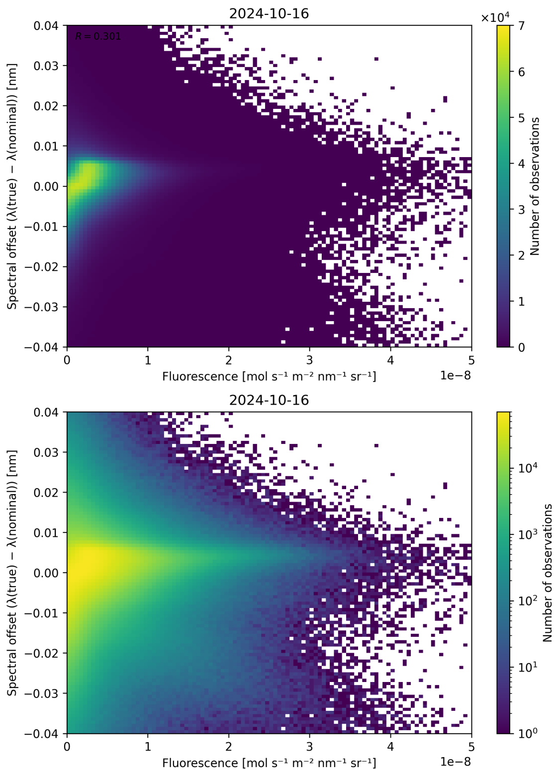
Figure 95: Scatter density plot of “Fluorescence” against “Spectral offset ( \lambda_{\text{true}} - \lambda_{\text{nominal}} )” for 2024-10-15 to 2024-10-17.
