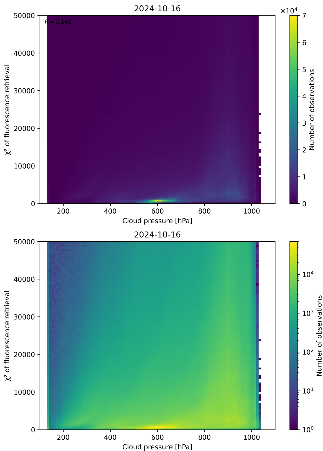
Figure 86: Scatter density plot of “Cloud pressure” against “ \chi^2 of fluorescence retrieval” for 2024-10-15 to 2024-10-17.
