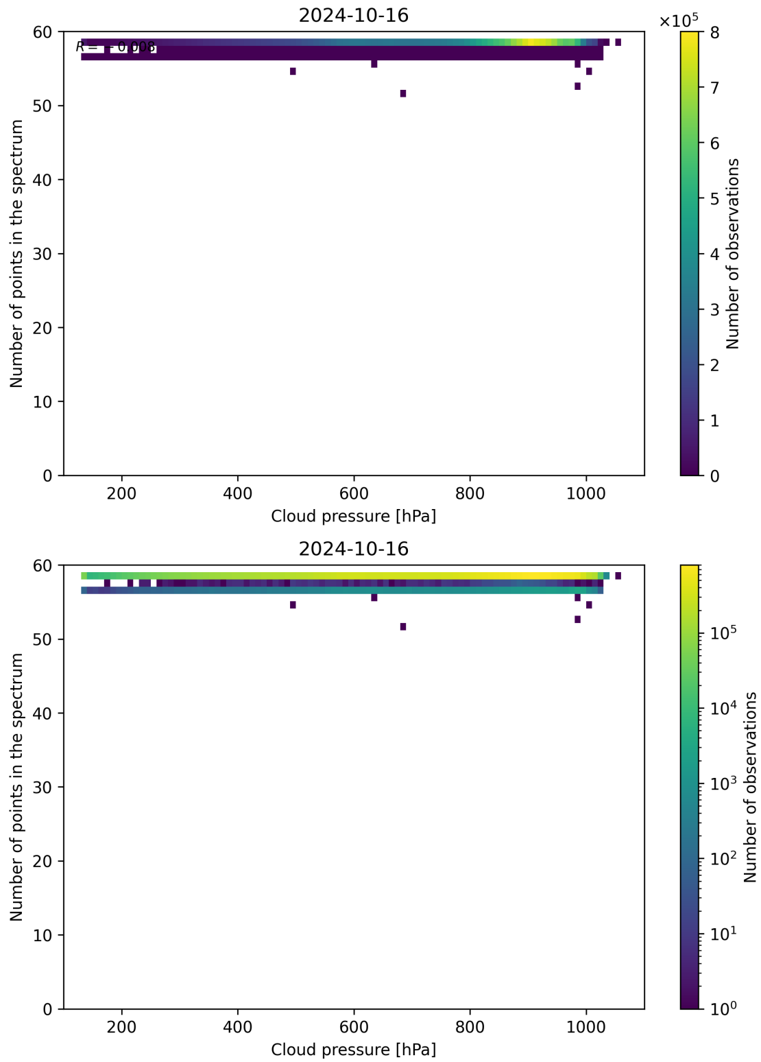
Figure 90: Scatter density plot of “Cloud pressure” against “Number of points in the spectrum” for 2024-10-15 to 2024-10-17.
