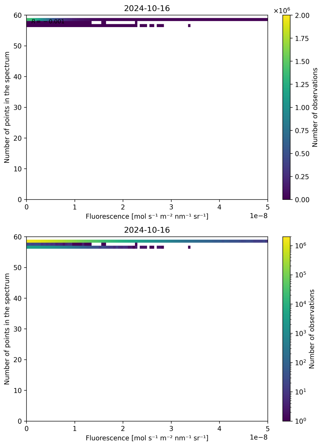
Figure 94: Scatter density plot of “Fluorescence” against “Number of points in the spectrum” for 2024-10-15 to 2024-10-17.
