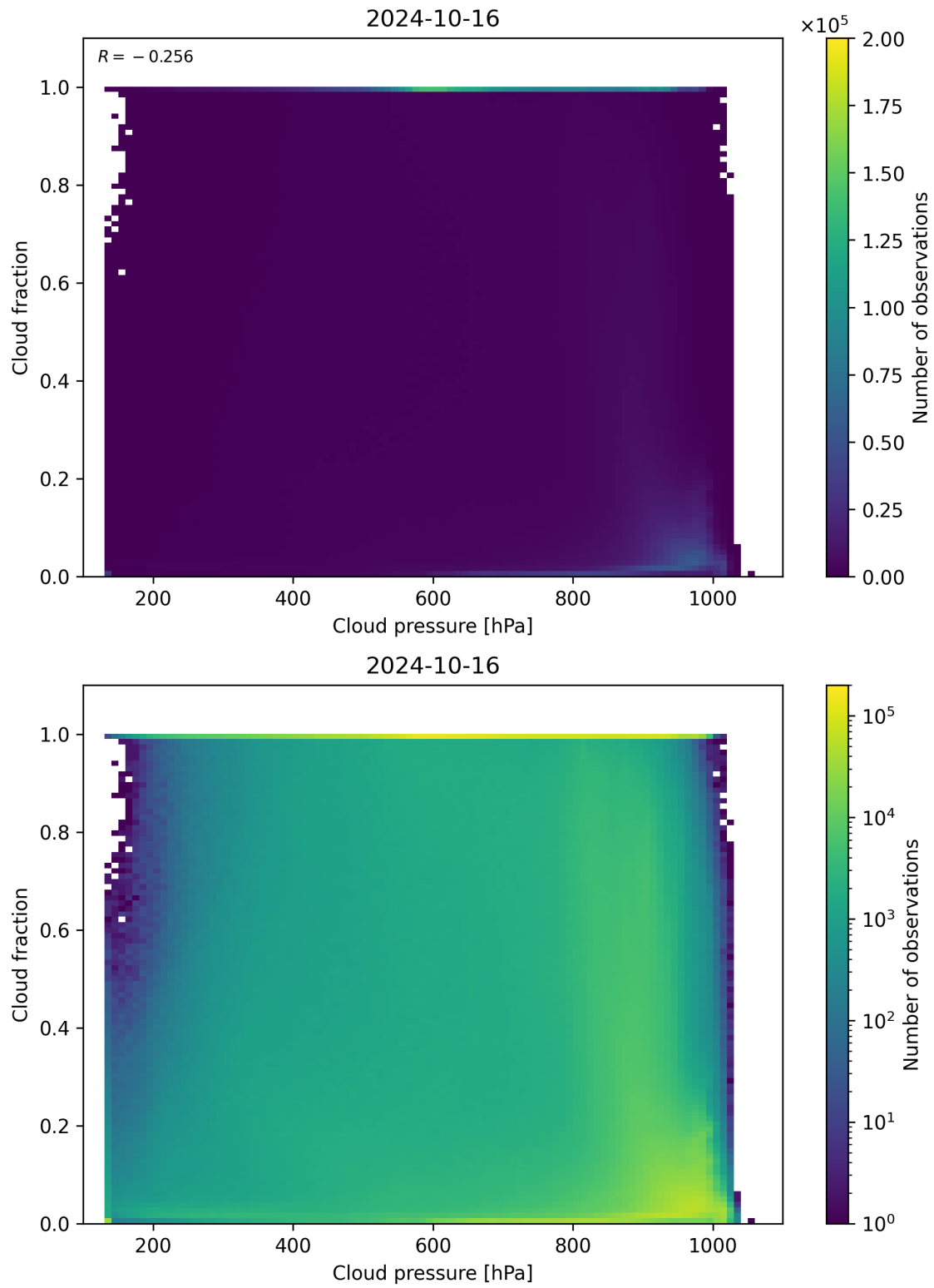
Figure 87: Scatter density plot of “Cloud pressure” against “Cloud fraction” for 2024-10-15 to 2024-10-17.
