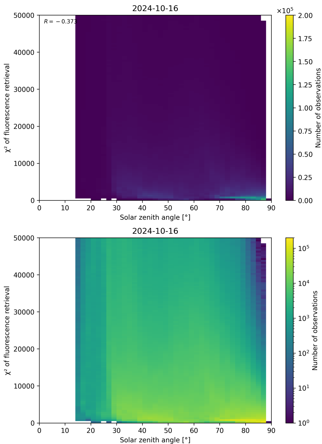
Figure 120: Scatter density plot of “Solar zenith angle” against “ \chi^2 of fluorescence retrieval” for 2024-10-15 to 2024-10-17.
