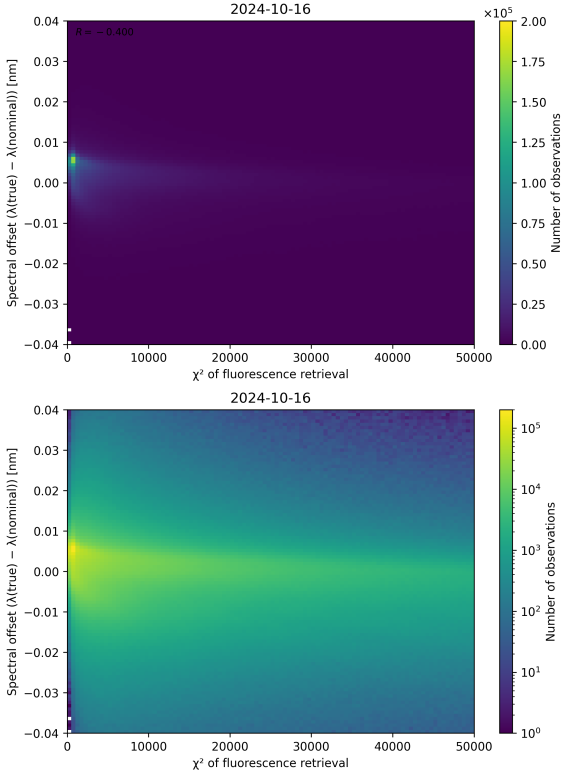
Figure 72: Scatter density plot of “ \chi^2 of fluorescence retrieval” against “Spectral offset ( \lambda_{\text{true}} - \lambda_{\text{nominal}} )” for 2024-10-15 to 2024-10-17.
