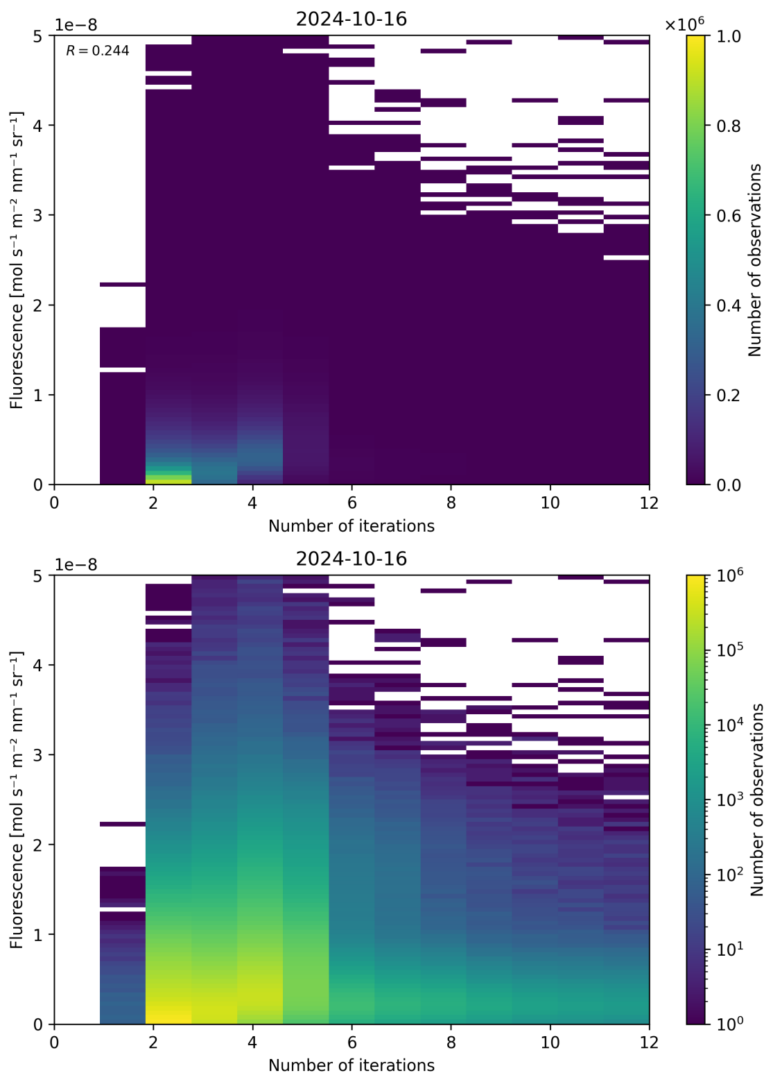
Figure 107: Scatter density plot of “Number of iterations” against “Fluorescence” for 2024-10-15 to 2024-10-17.
