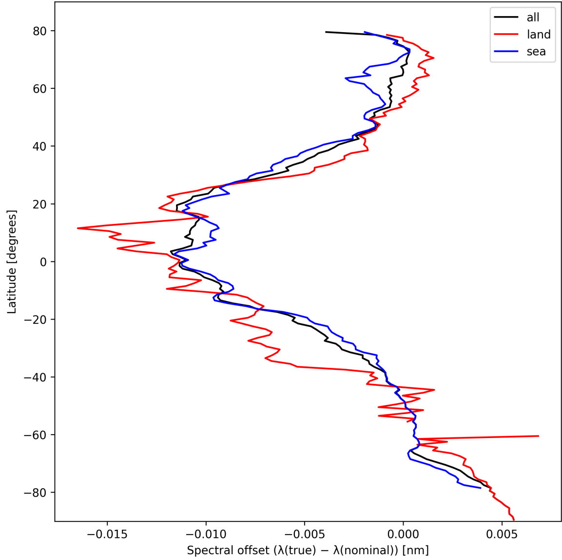
Figure 28: Zonal average of “Spectral offset ( \lambda_{\text{true}} - \lambda_{\text{nominal}} )” for 2024-10-15 to 2024-10-17.
