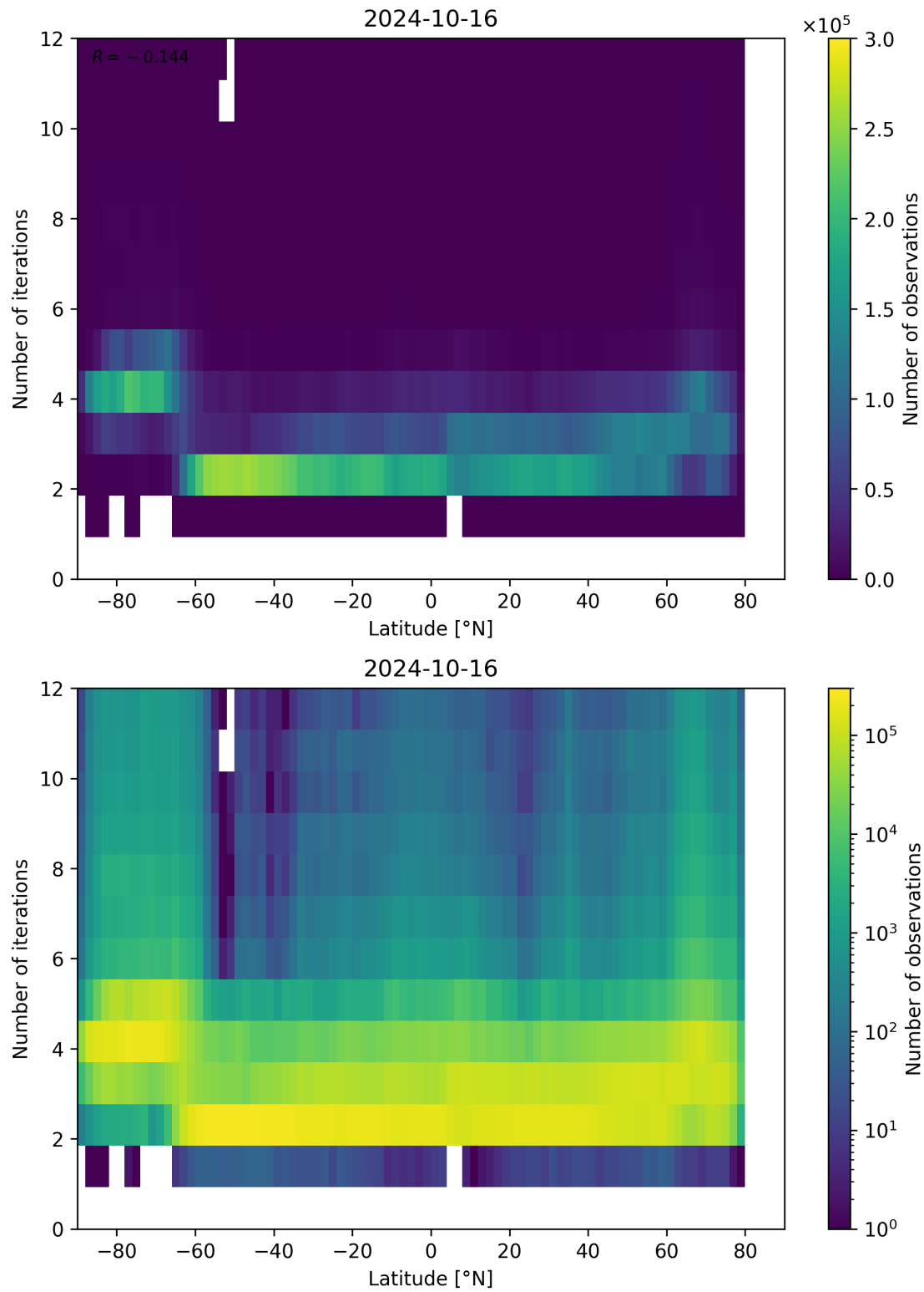
Figure 102: Scatter density plot of “Latitude” against “Number of iterations” for 2024-10-15 to 2024-10-17.
