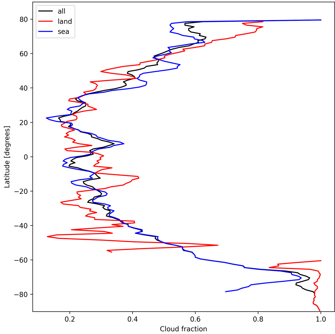
Figure 15: Zonal average of “Cloud fraction” for 2024-10-15 to 2024-10-17.
