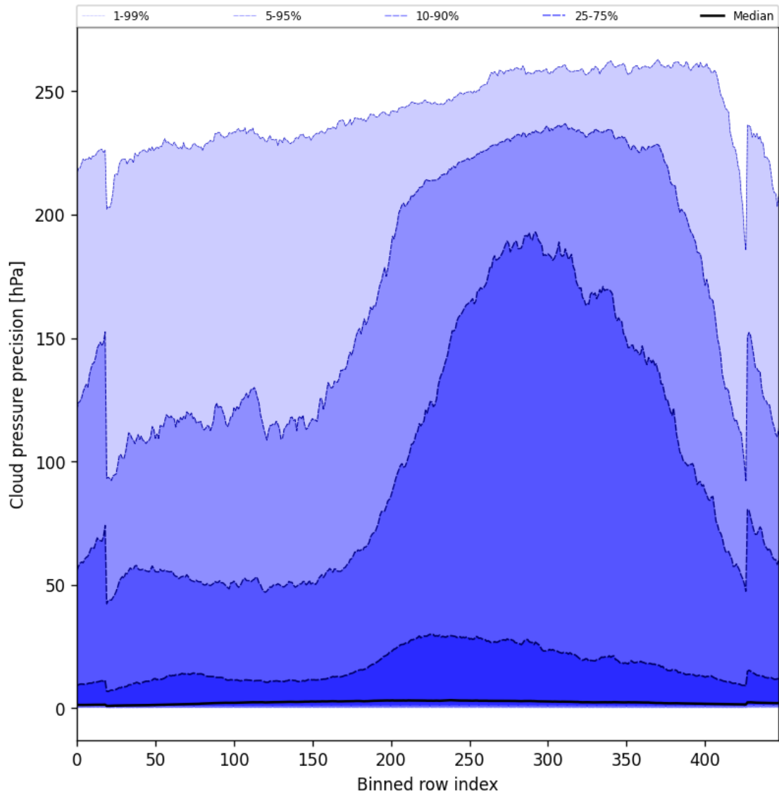
Figure 48: Along track statistics of “Cloud pressure precision” for 2024-10-15 to 2024-10-17
