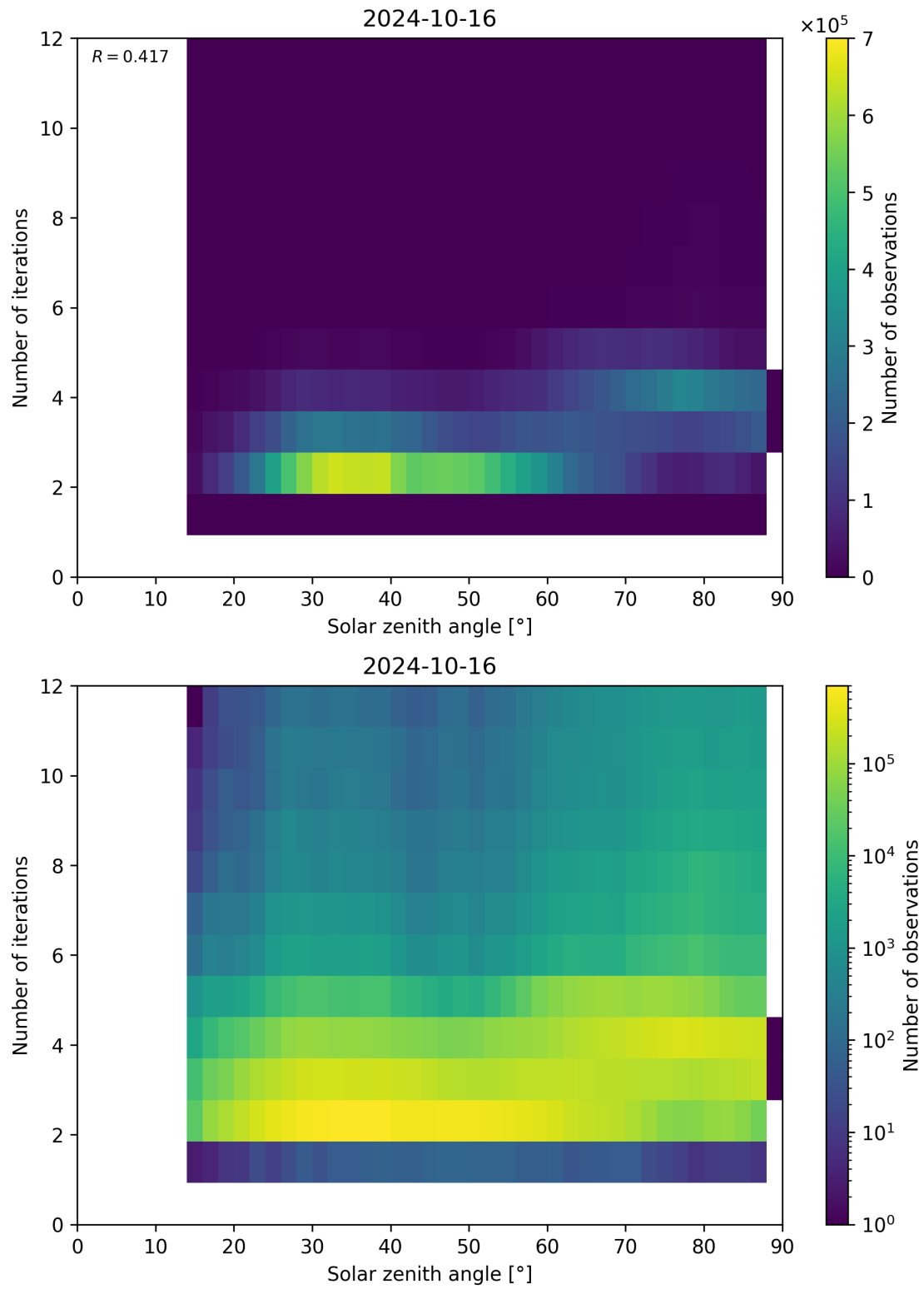
Figure 125: Scatter density plot of “Solar zenith angle” against “Number of iterations” for 2024-10-15 to 2024-10-17.
