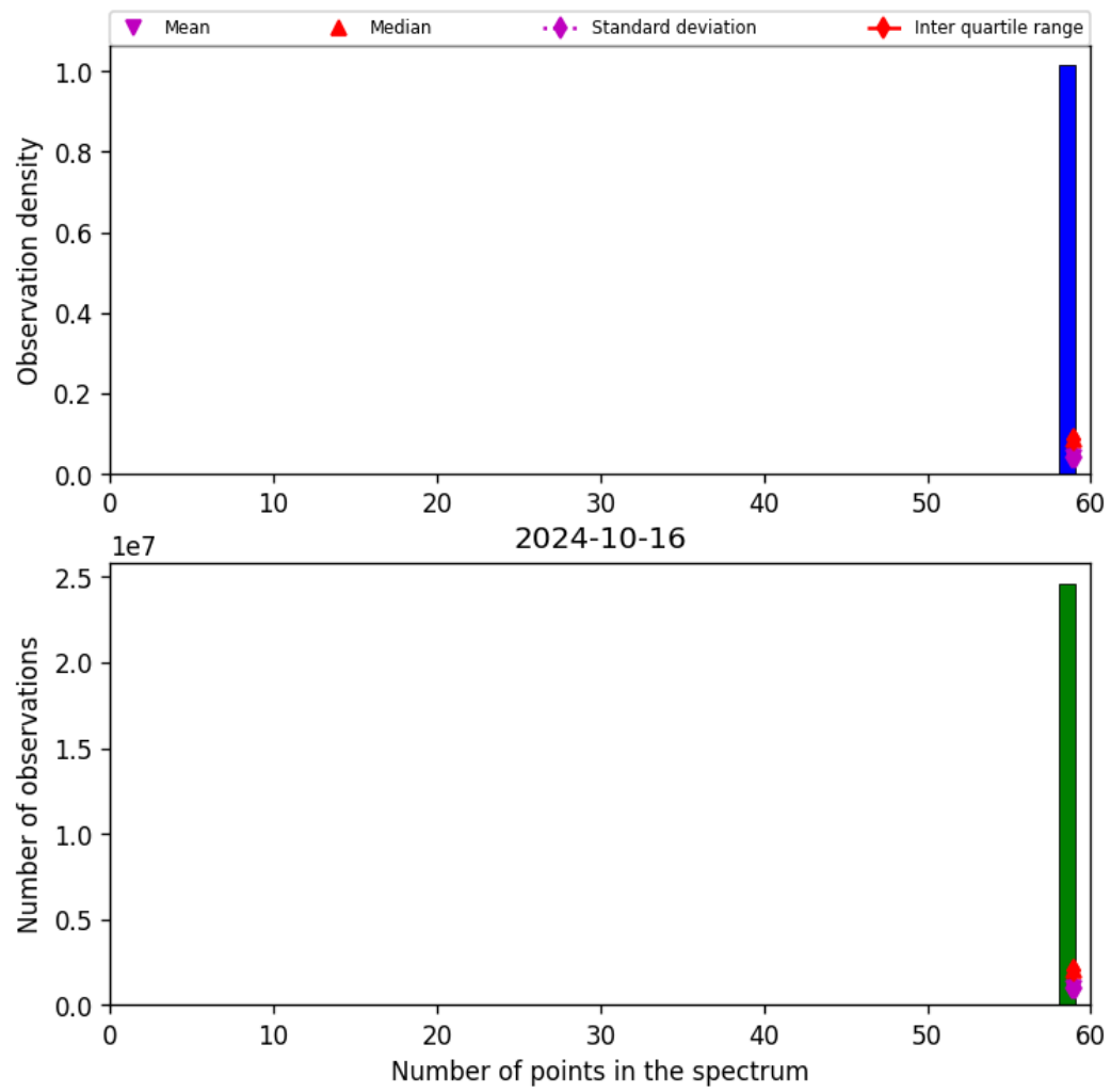
Figure 44: Histogram of “Number of points in the spectrum” for 2024-10-15 to 2024-10-17
