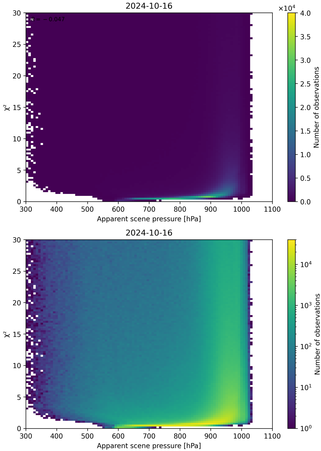
Figure 63: Scatter density plot of “Apparent scene pressure” against “ \chi^2 ” for 2024-10-15 to 2024-10-17.
