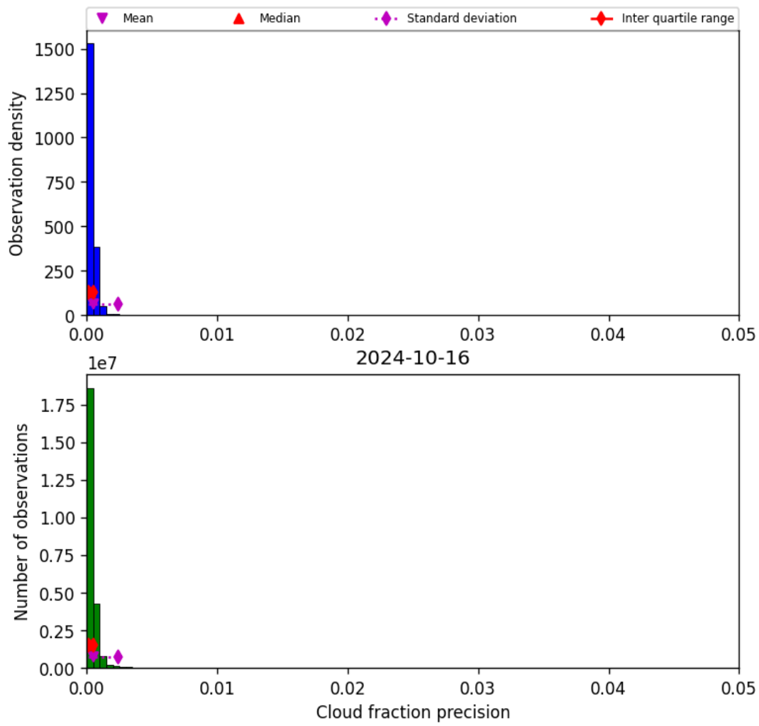
Figure 33: Histogram of “Cloud fraction precision” for 2024-10-15 to 2024-10-17
