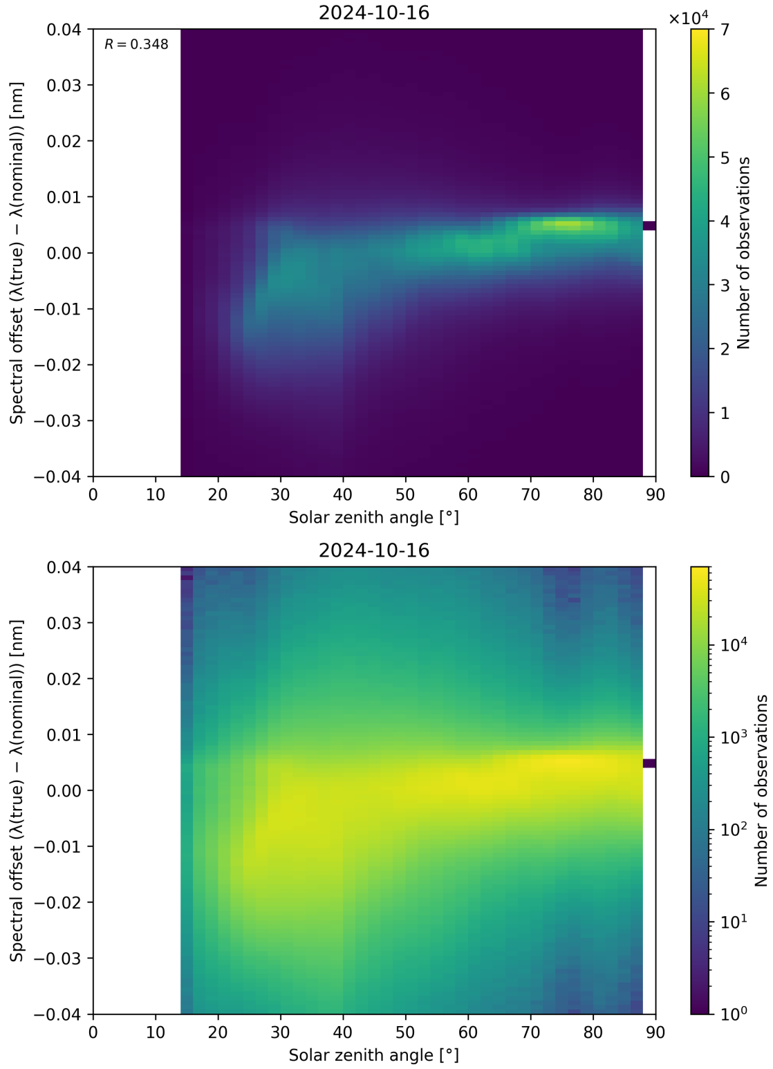
Figure 128: Scatter density plot of “Solar zenith angle” against “Spectral offset ( \lambda_{\text{true}} - \lambda_{\text{nominal}} )” for 2024-10-15 to 2024-10-17.
