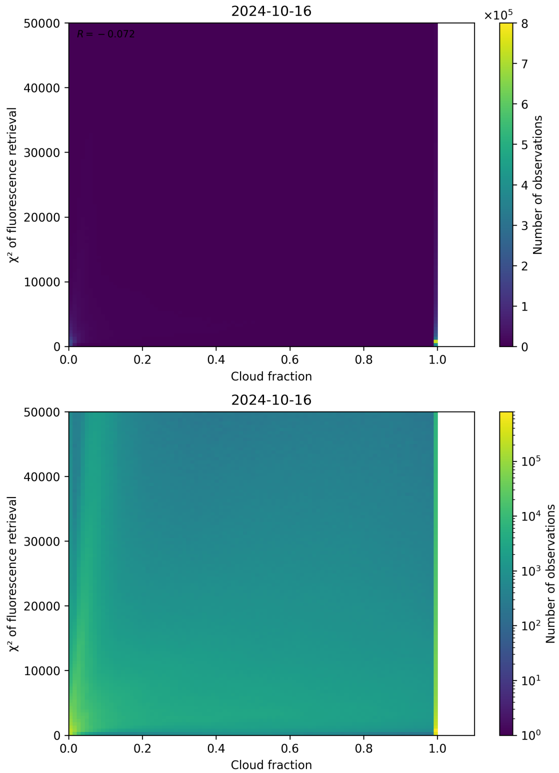
Figure 78: Scatter density plot of “Cloud fraction” against “ \chi^2 of fluorescence retrieval” for 2024-10-15 to 2024-10-17.
