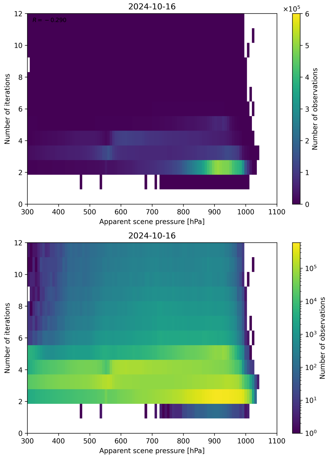
Figure 66: Scatter density plot of “Apparent scene pressure” against “Number of iterations” for 2024-10-15 to 2024-10-17.
