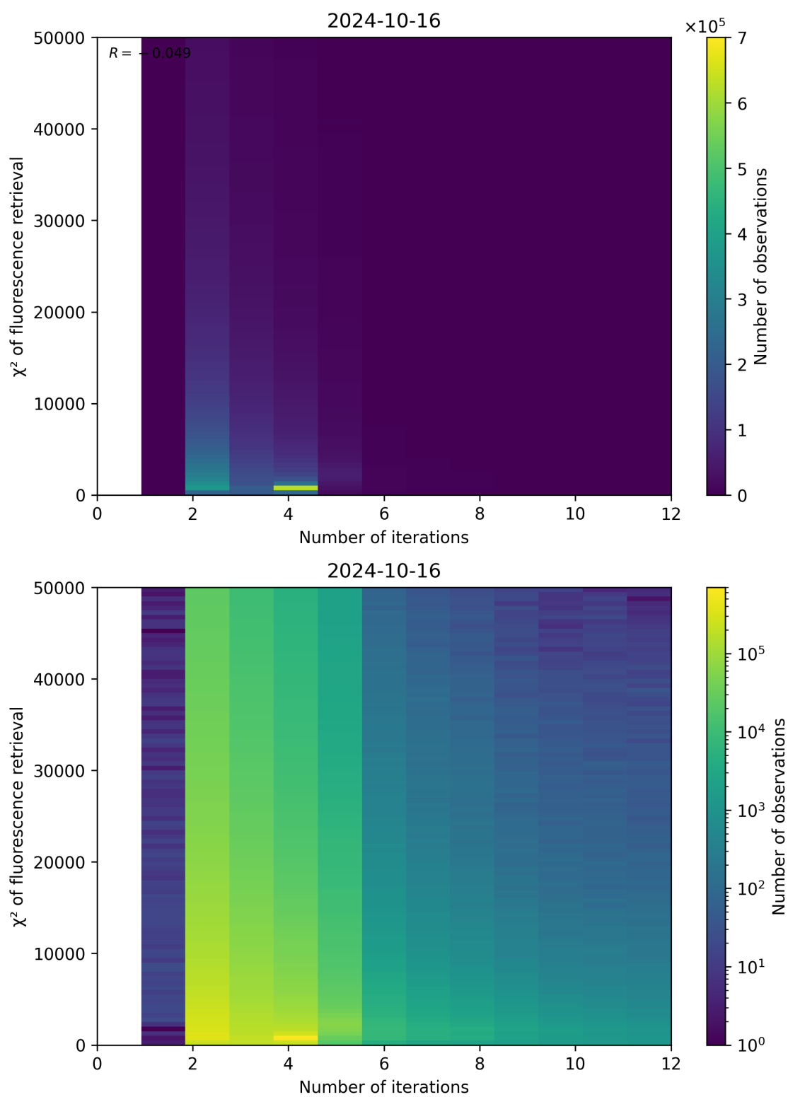
Figure 106: Scatter density plot of “Number of iterations” against “ \chi^2 of fluorescence retrieval” for 2024-10-15 to 2024-10-17.
