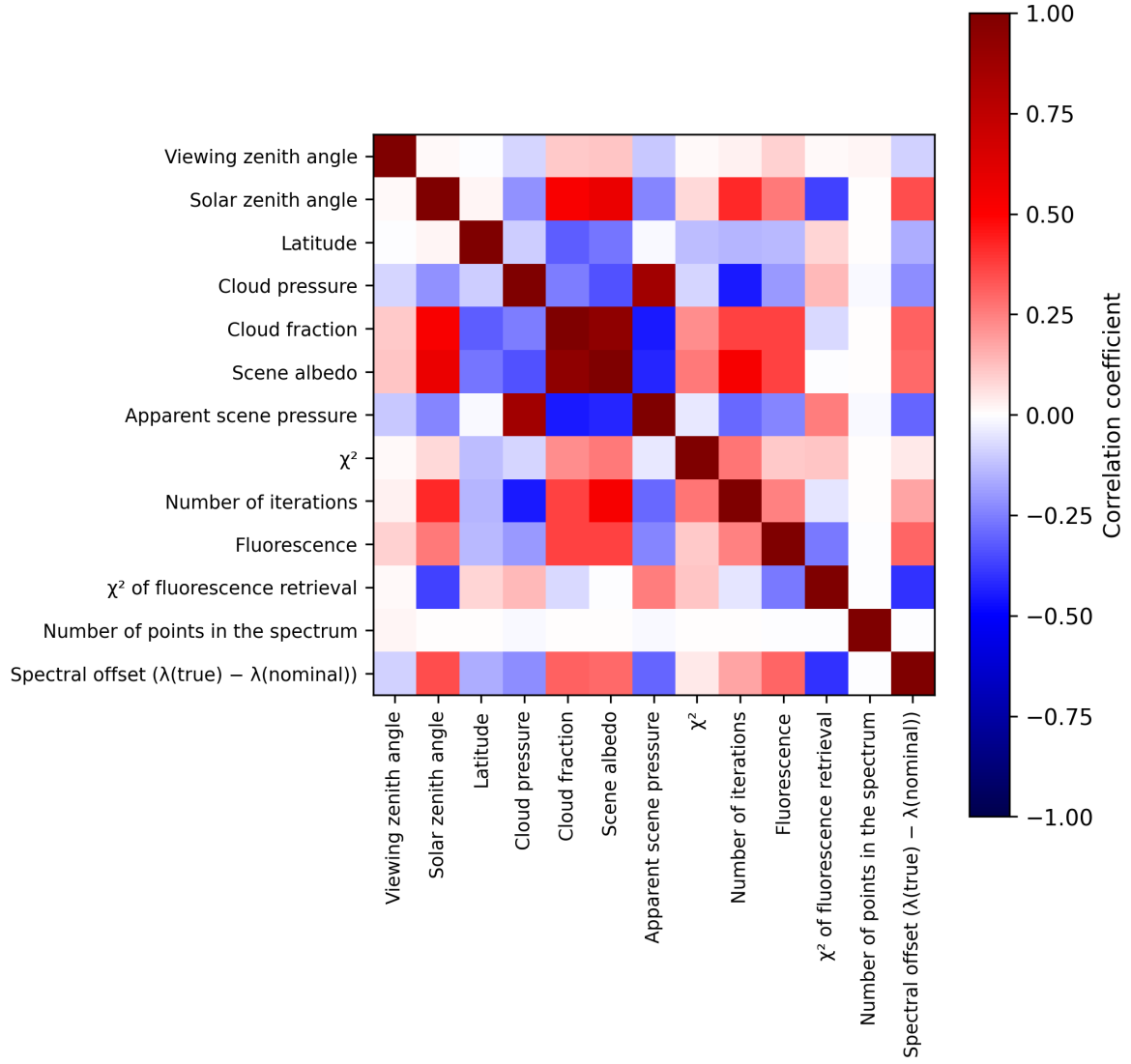
Figure 2: Map of correlation matrix for 2024-10-15 to 2024-10-17.
