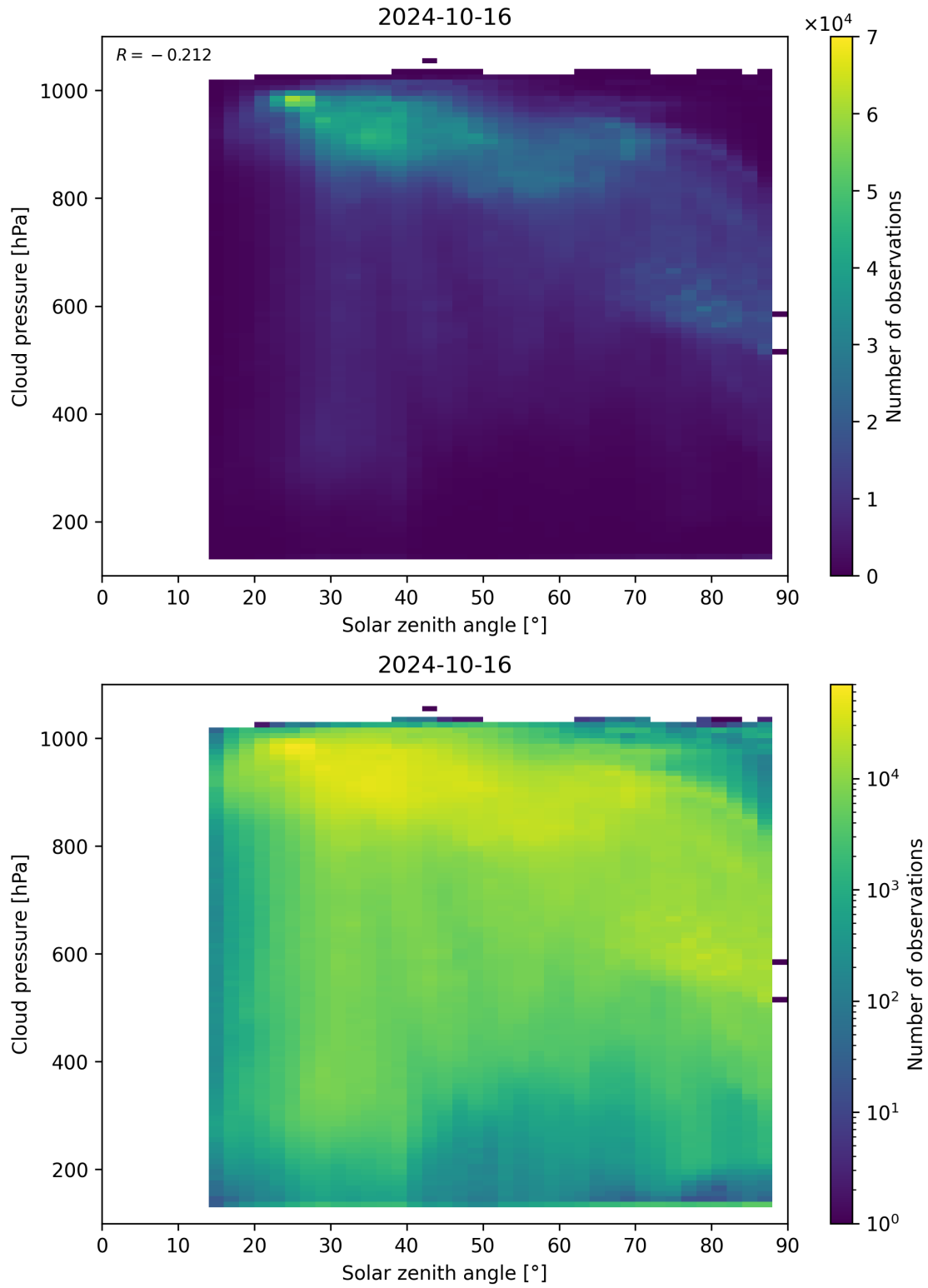
Figure 122: Scatter density plot of “Solar zenith angle” against “Cloud pressure” for 2024-10-15 to 2024-10-17.
