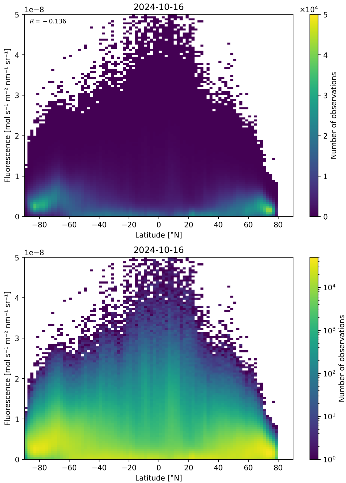
Figure 101: Scatter density plot of “Latitude” against “Fluorescence” for 2024-10-15 to 2024-10-17.
