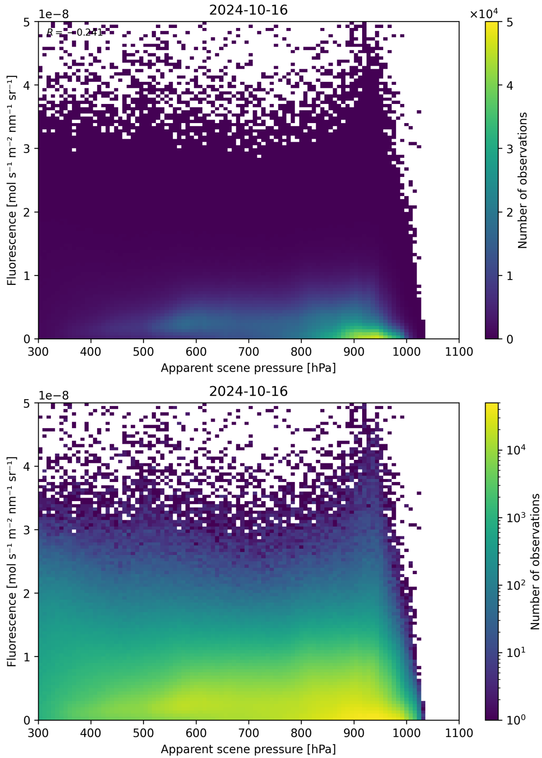
Figure 65: Scatter density plot of “Apparent scene pressure” against “Fluorescence” for 2024-10-15 to 2024-10-17.
