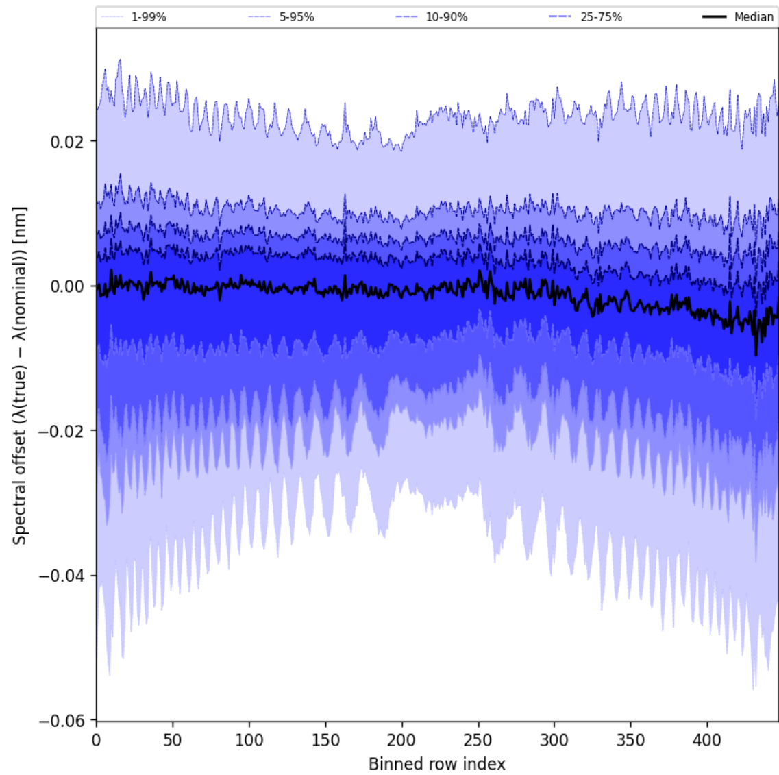
Figure 62: Along track statistics of “Spectral offset ( \lambda_{\text{true}} - \lambda_{\text{nominal}} )” for 2024-10-15 to 2024-10-17
