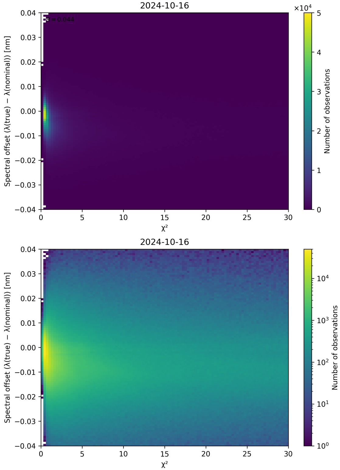
Figure 75: Scatter density plot of “ \chi^2 ” against “Spectral offset ( \lambda_{\text{true}} - \lambda_{\text{nominal}} )” for 2024-10-15 to 2024-10-17.
