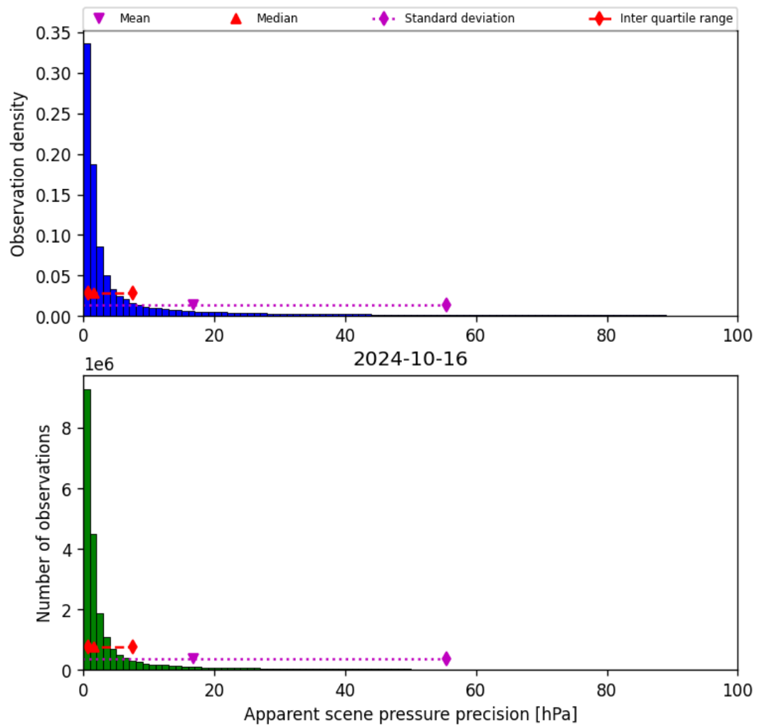
Figure 37: Histogram of “Apparent scene pressure precision” for 2024-10-15 to 2024-10-17
