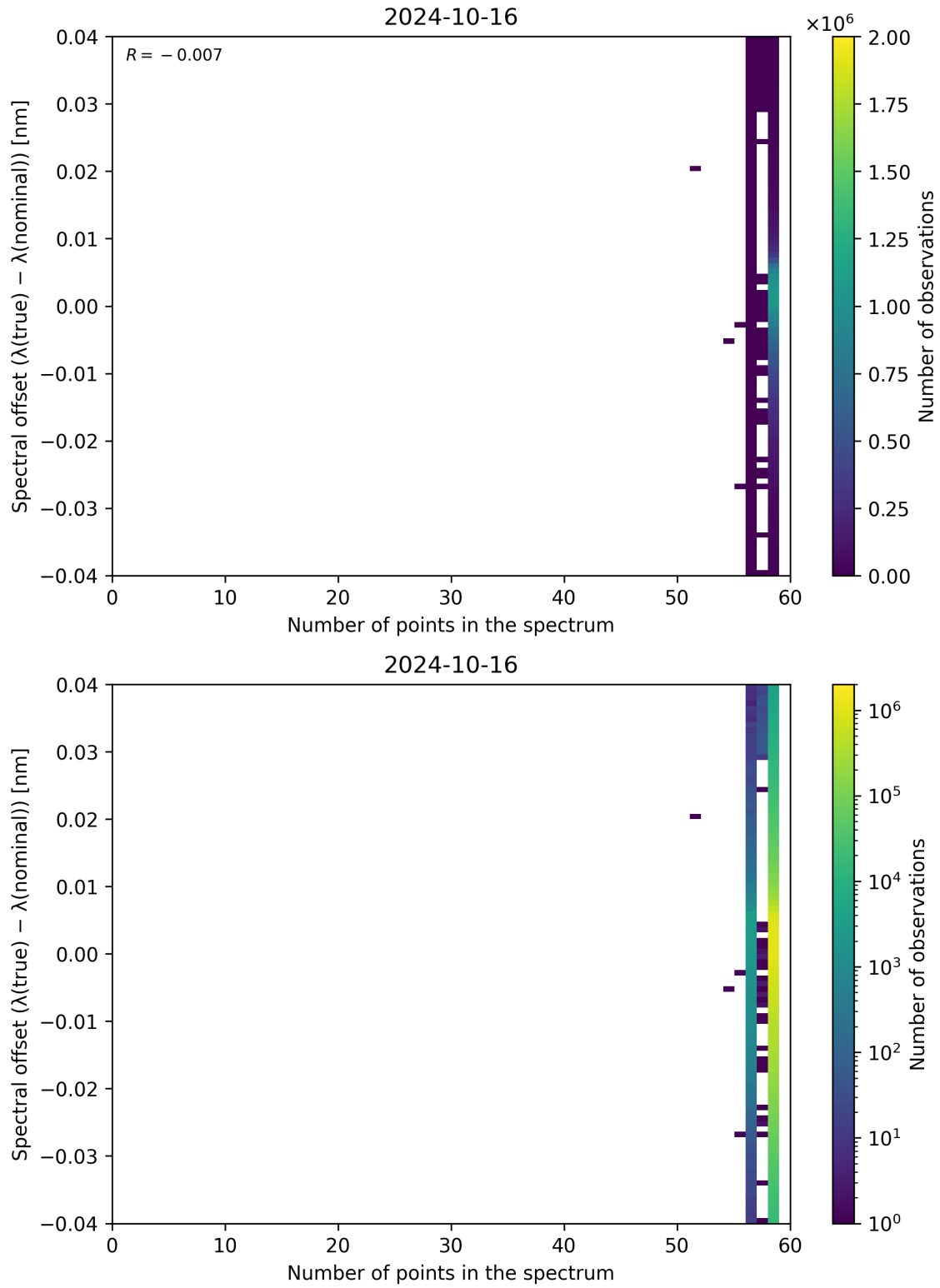
Figure 110: Scatter density plot of “Number of points in the spectrum” against “Spectral offset ( \lambda_{\text{true}} - \lambda_{\text{nominal}} )” for 2024-10-15 to 2024-10-17.
