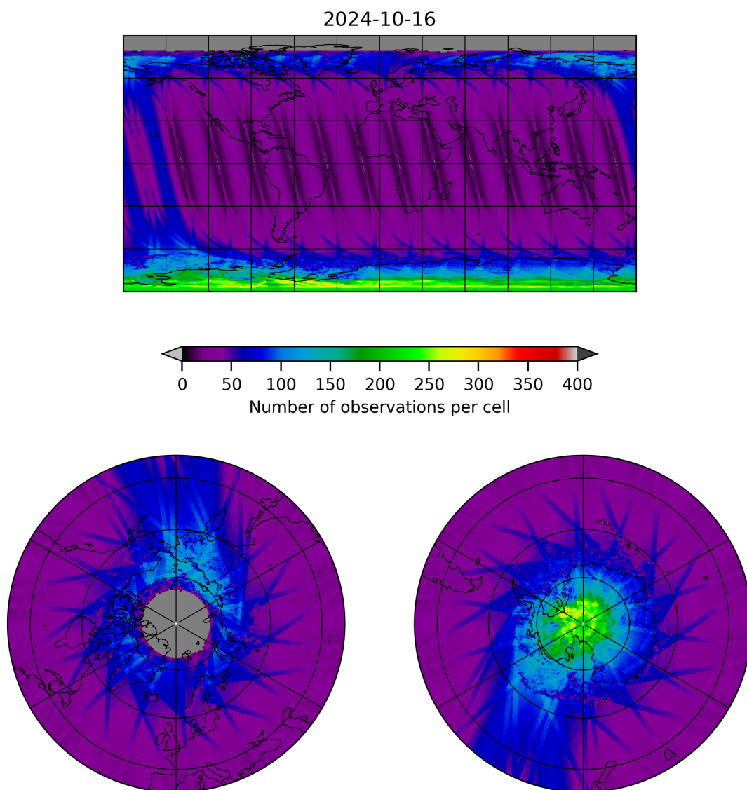
Figure 11: Map of the number of observations for 2024-10-15 to 2024-10-17
