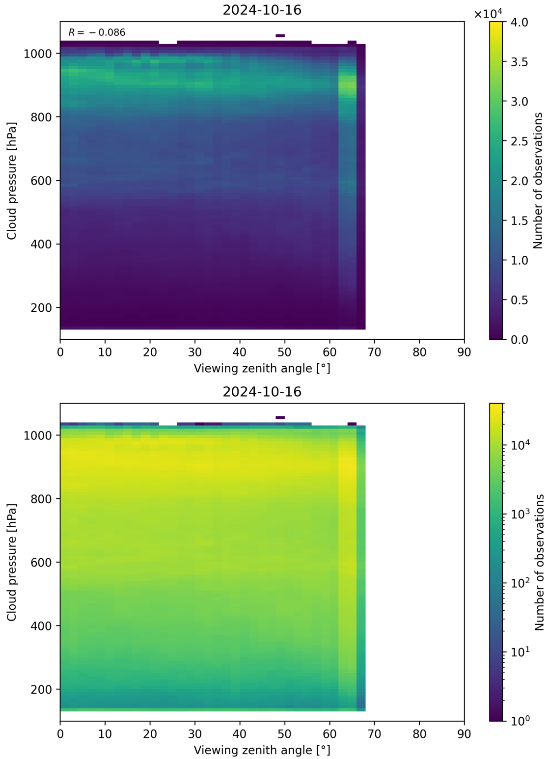
Figure 133: Scatter density plot of “Viewing zenith angle” against “Cloud pressure” for 2024-10-15 to 2024-10-17.
