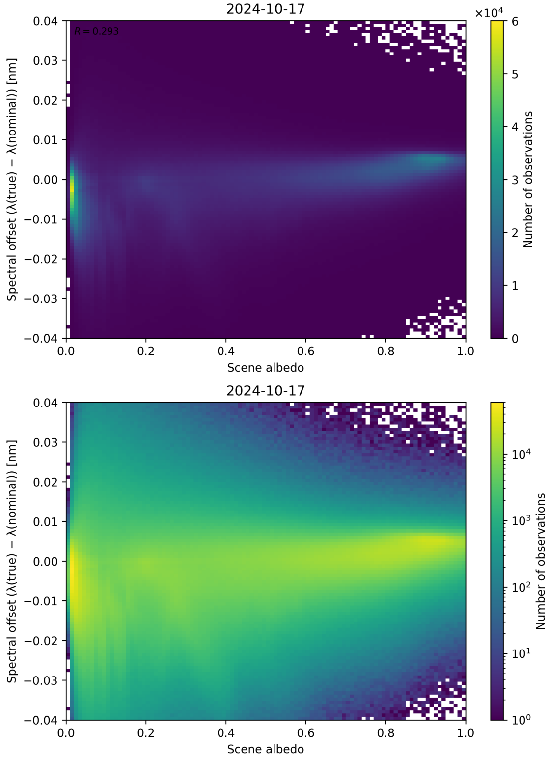
Figure 117: Scatter density plot of “Scene albedo” against “Spectral offset ( \lambda_{\text{true}} - \lambda_{\text{nominal}} )” for 2024-10-16 to 2024-10-18.
