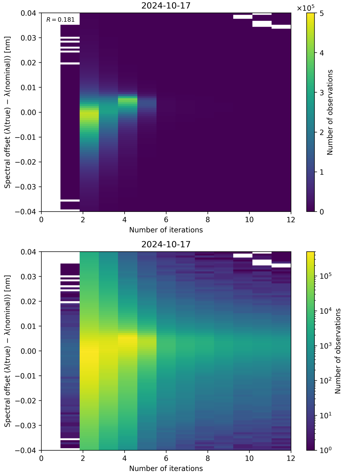
Figure 109: Scatter density plot of “Number of iterations” against “Spectral offset ( \lambda_{\text{true}} - \lambda_{\text{nominal}} )” for 2024-10-16 to 2024-10-18.
