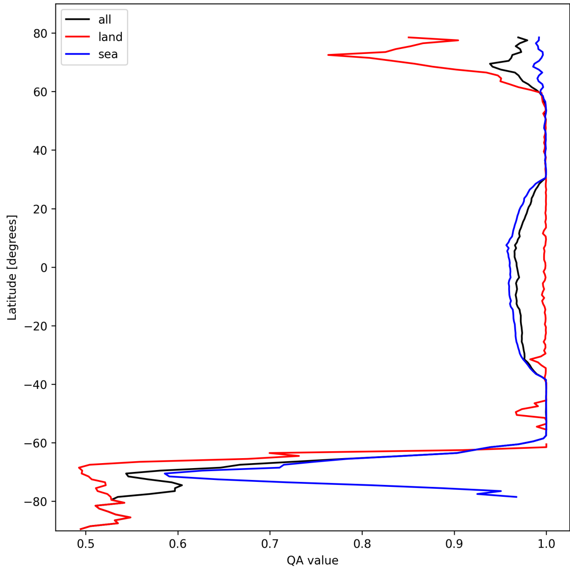
Figure 12: Zonal average of “QA value” for 2024-10-16 to 2024-10-18.
