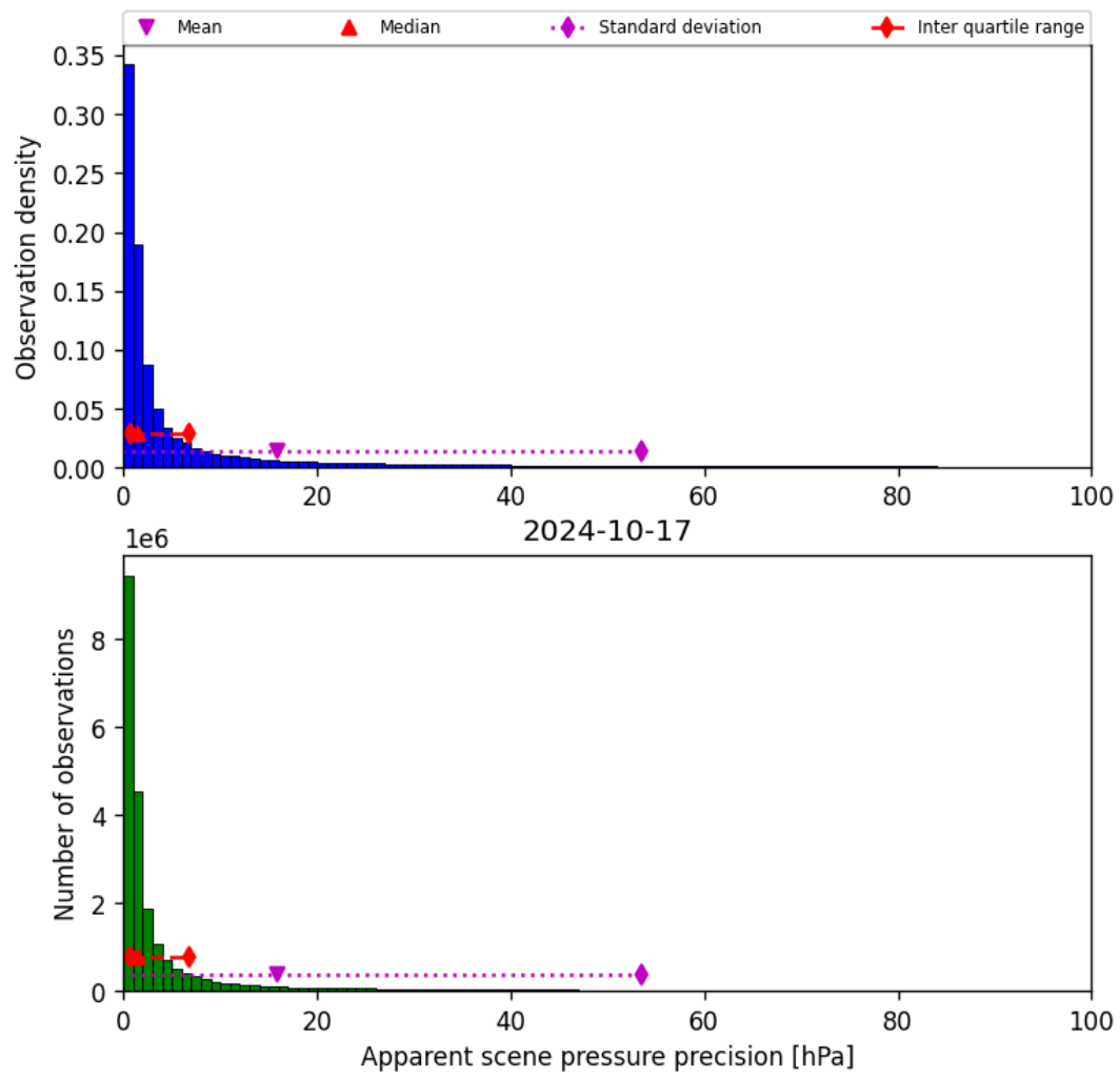
Figure 37: Histogram of “Apparent scene pressure precision” for 2024-10-16 to 2024-10-18
