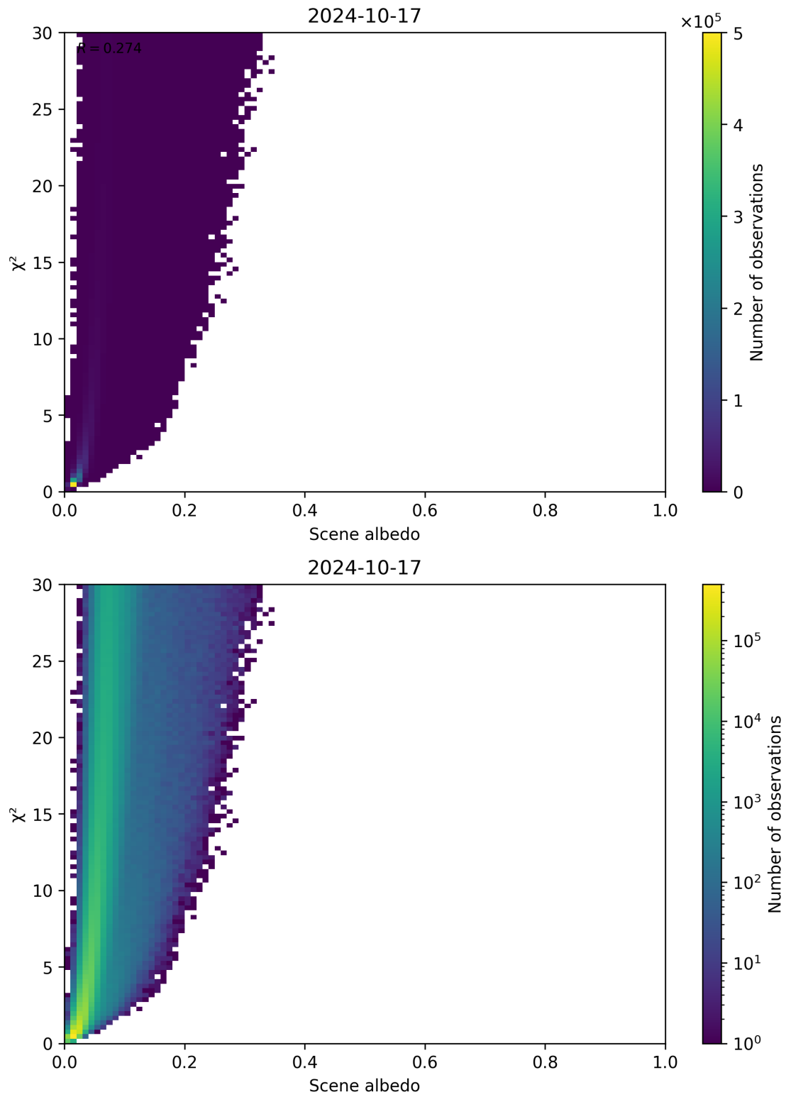
Figure 112: Scatter density plot of “Scene albedo” against “ \chi^2 ” for 2024-10-16 to 2024-10-18.
