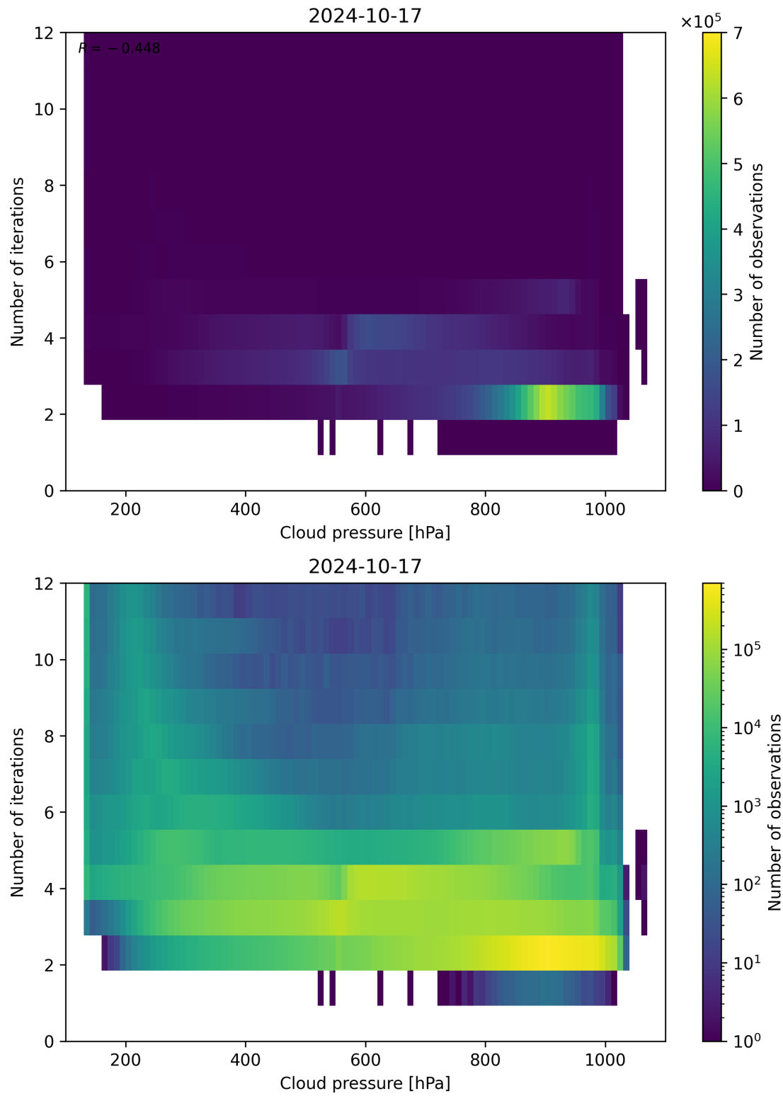
Figure 89: Scatter density plot of “Cloud pressure” against “Number of iterations” for 2024-10-16 to 2024-10-18.
