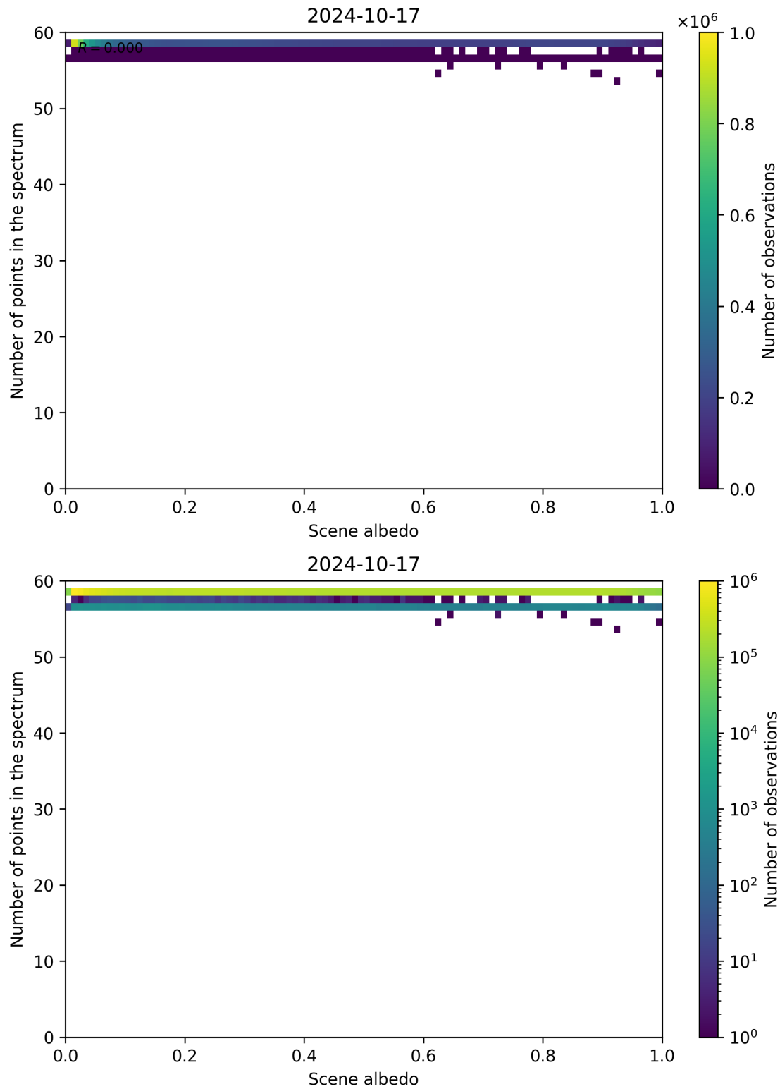
Figure 116: Scatter density plot of “Scene albedo” against “Number of points in the spectrum” for 2024-10-16 to 2024-10-18.
