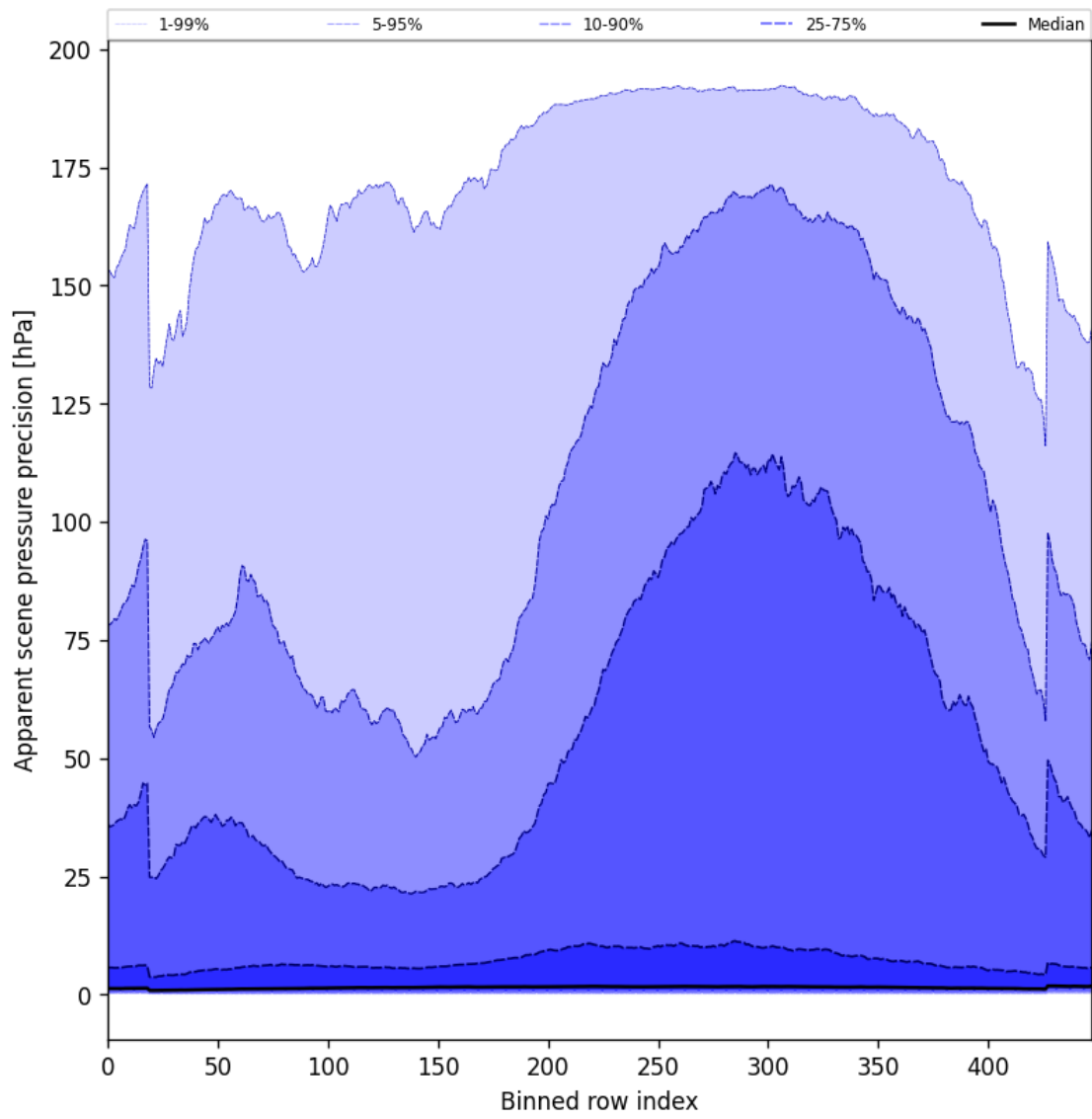
Figure 54: Along track statistics of “Apparent scene pressure precision” for 2024-10-16 to 2024-10-18
