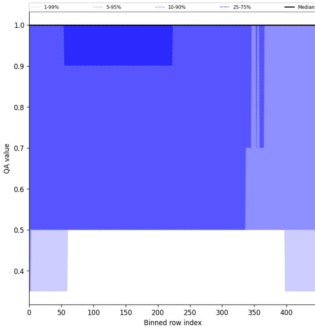
Figure 46: Along track statistics of “QA value” for 2024-10-16 to 2024-10-18
