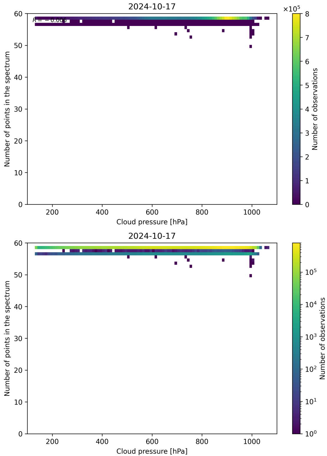
Figure 90: Scatter density plot of “Cloud pressure” against “Number of points in the spectrum” for 2024-10-16 to 2024-10-18.
