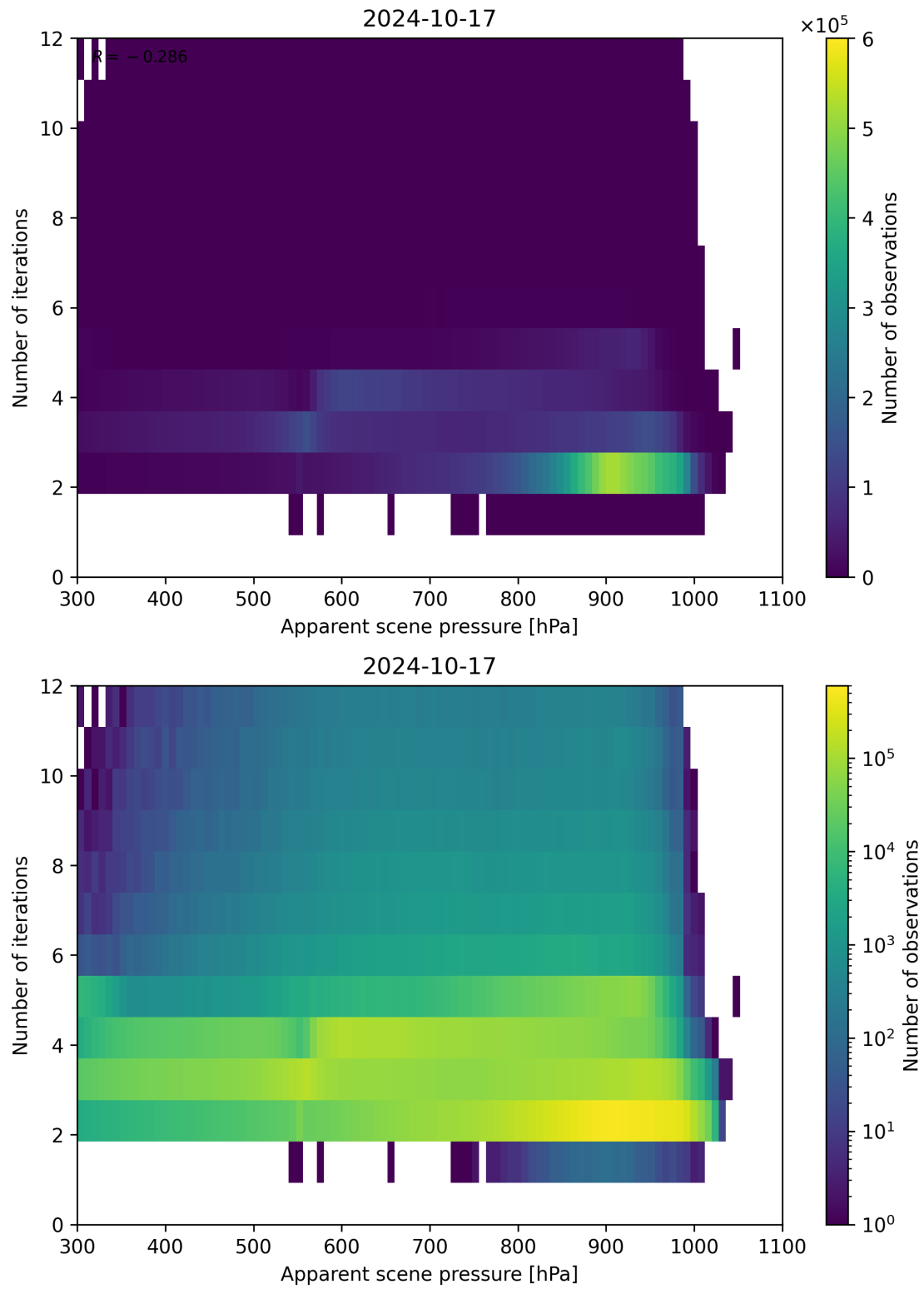
Figure 66: Scatter density plot of “Apparent scene pressure” against “Number of iterations” for 2024-10-16 to 2024-10-18.
