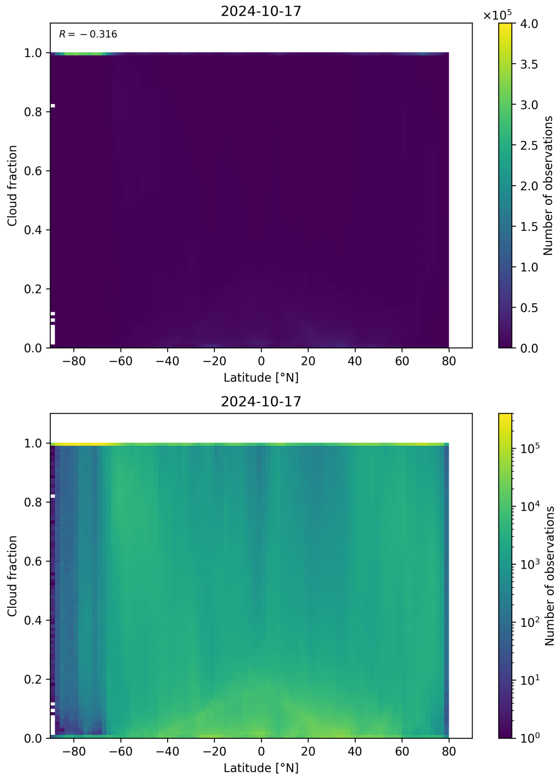
Figure 99: Scatter density plot of “Latitude” against “Cloud fraction” for 2024-10-16 to 2024-10-18.
