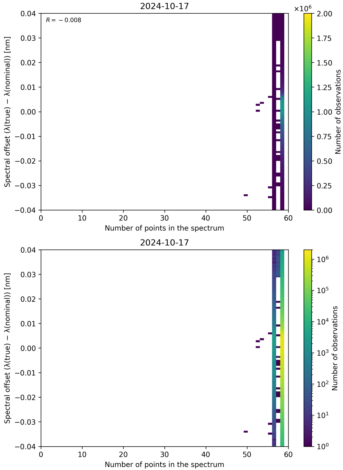
Figure 110: Scatter density plot of “Number of points in the spectrum” against “Spectral offset ( \lambda_{\text{true}} - \lambda_{\text{nominal}} )” for 2024-10-16 to 2024-10-18.
