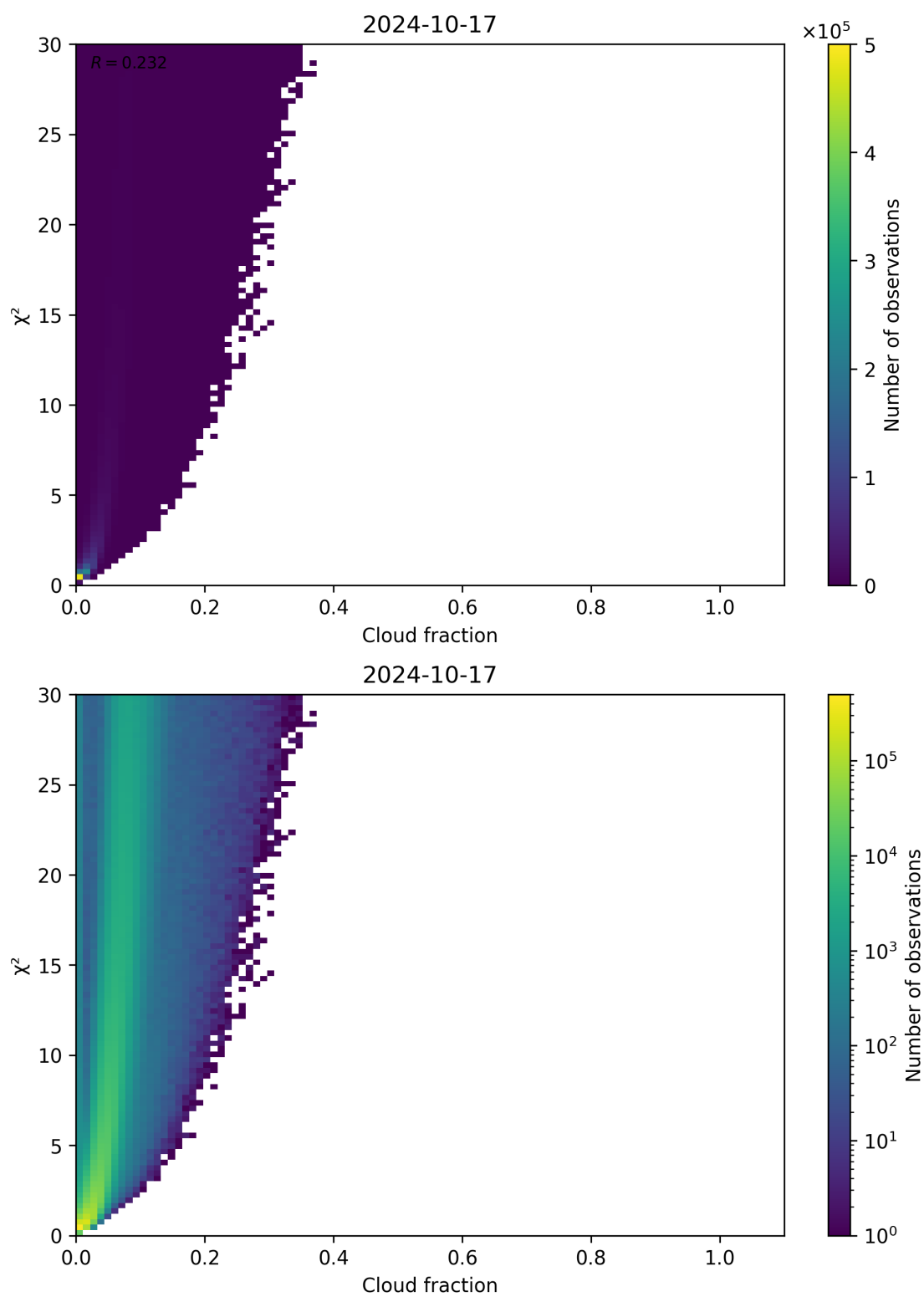
Figure 77: Scatter density plot of “Cloud fraction” against “ \chi^2 ” for 2024-10-16 to 2024-10-18.
