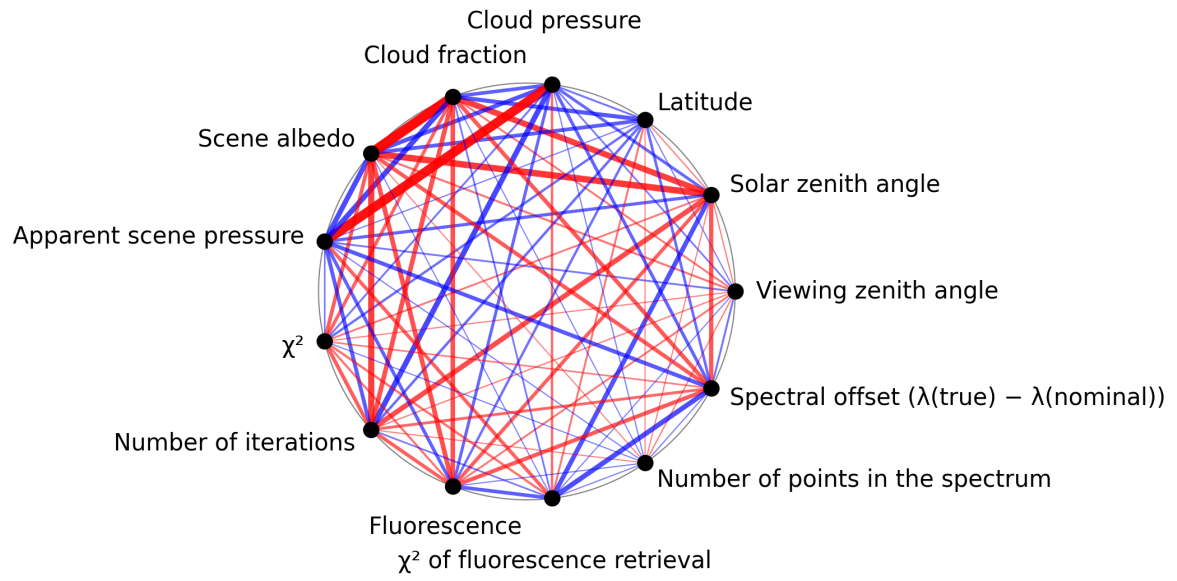
Figure 1: Map of correlation graph for 2024-10-16 to 2024-10-18.
