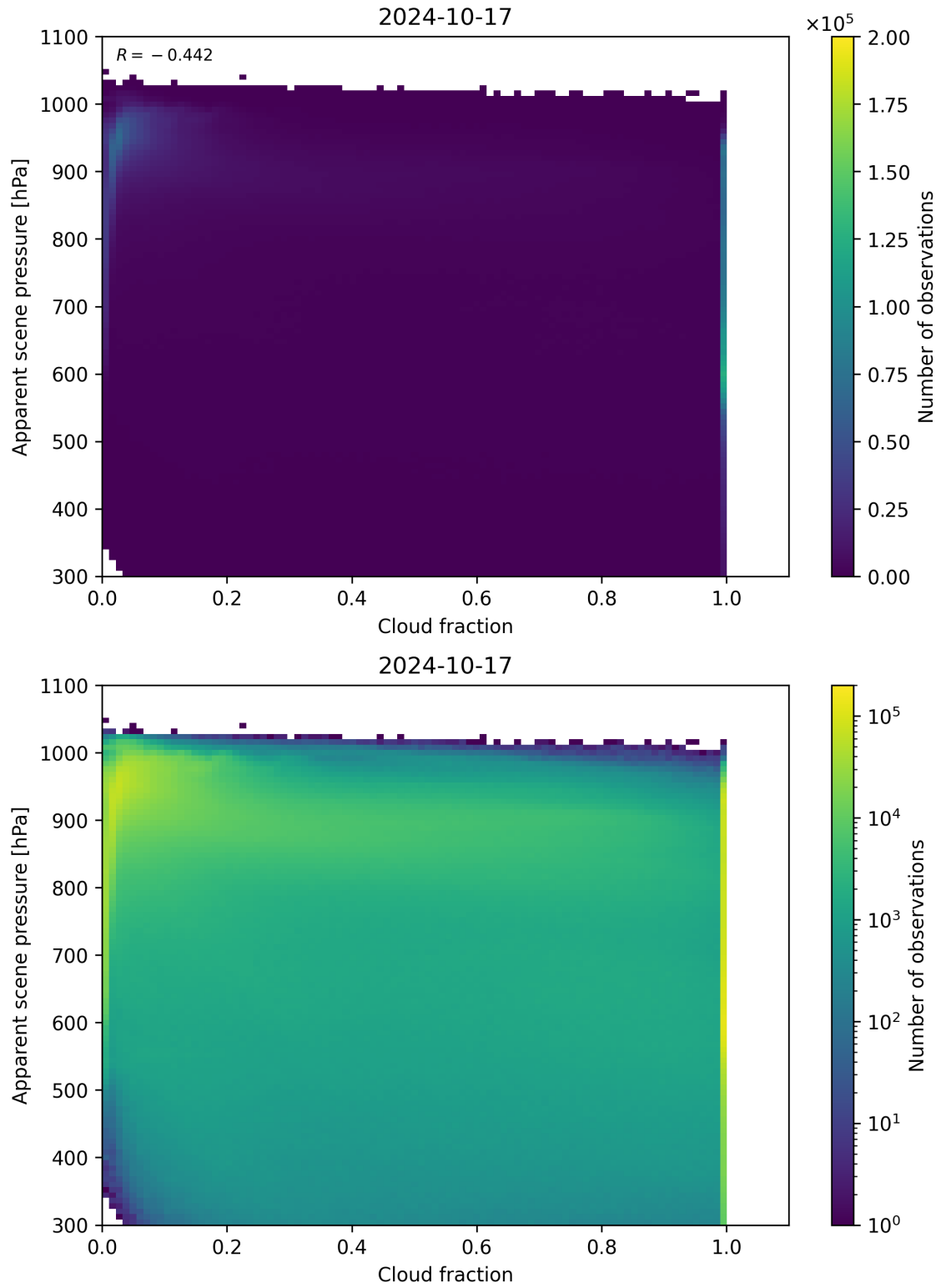
Figure 76: Scatter density plot of “Cloud fraction” against “Apparent scene pressure” for 2024-10-16 to 2024-10-18.
