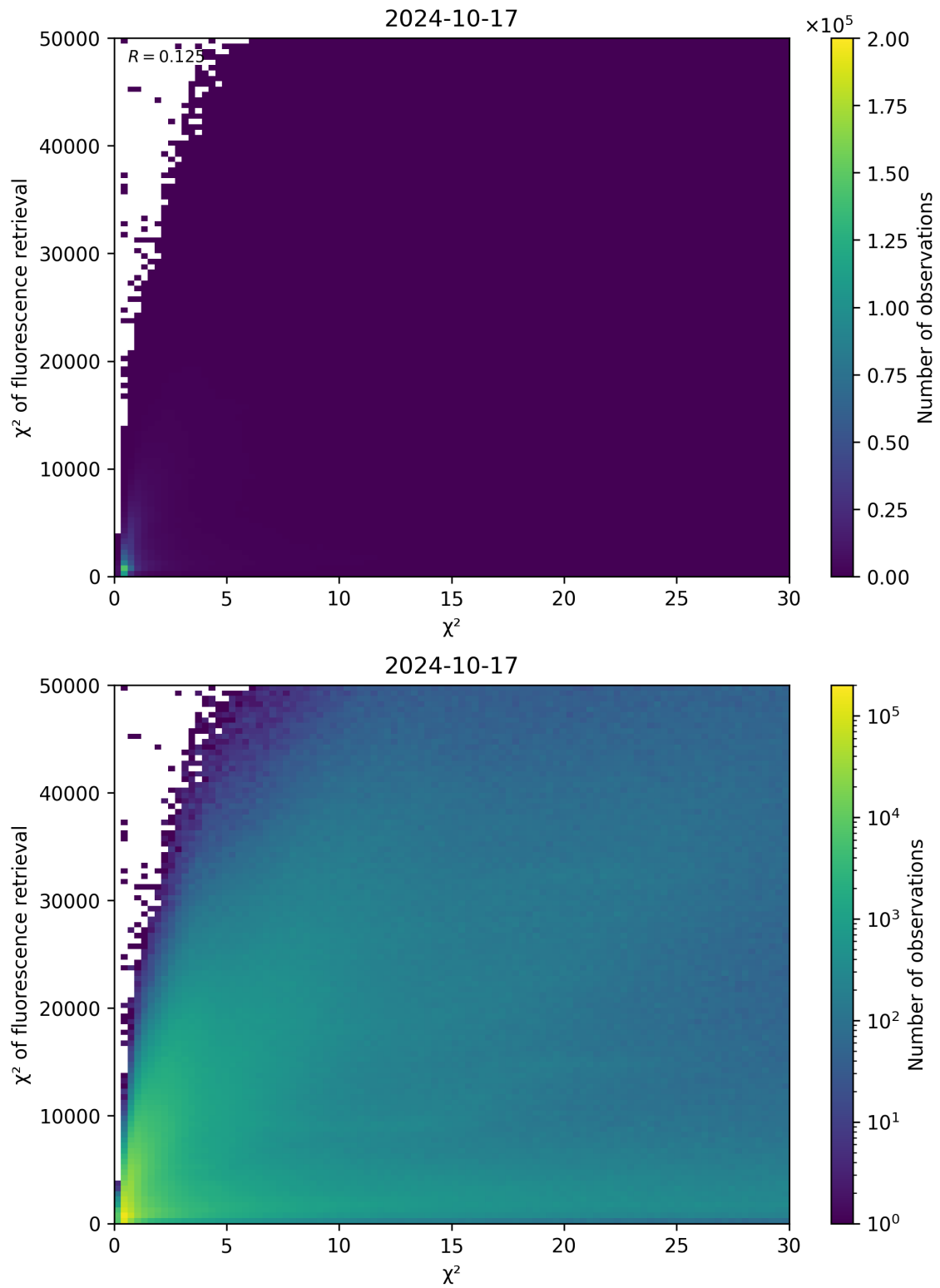
Figure 69: Scatter density plot of “ \chi^2 ” against “ \chi^2 of fluorescence retrieval” for 2024-10-16 to 2024-10-18.
