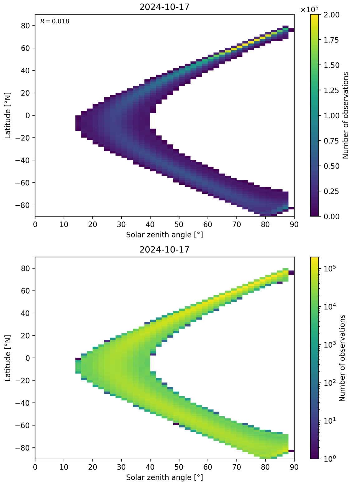
Figure 124: Scatter density plot of “Solar zenith angle” against “Latitude” for 2024-10-16 to 2024-10-18.
