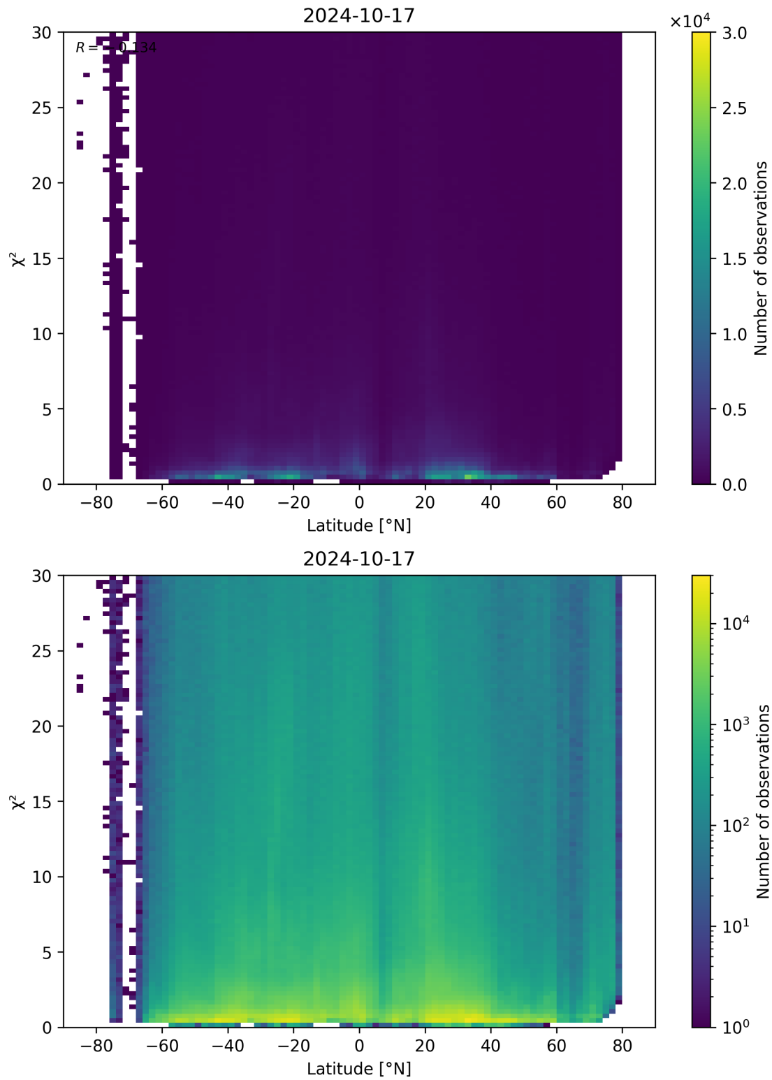
Figure 97: Scatter density plot of “Latitude” against “ \chi^2 ” for 2024-10-16 to 2024-10-18.
