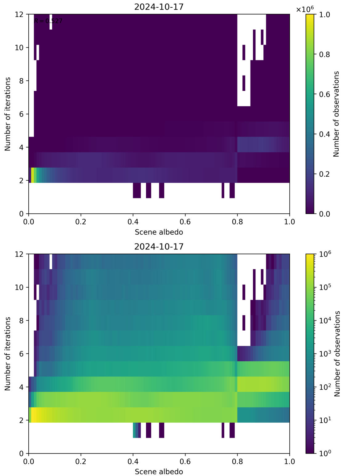
Figure 115: Scatter density plot of “Scene albedo” against “Number of iterations” for 2024-10-16 to 2024-10-18.
