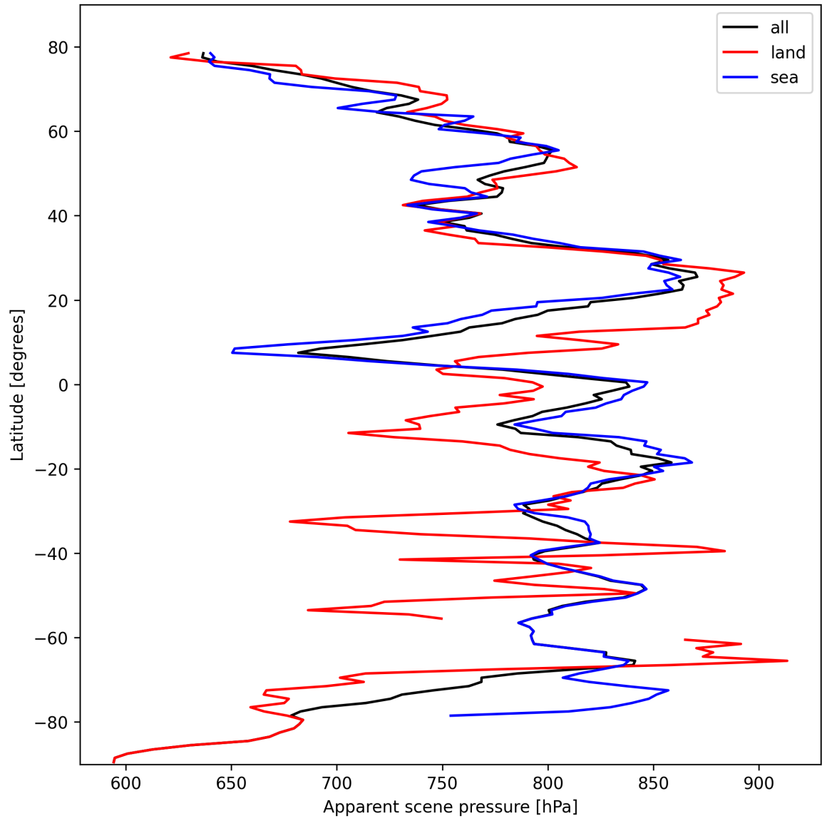
Figure 19: Zonal average of “Apparent scene pressure” for 2024-10-16 to 2024-10-18.
