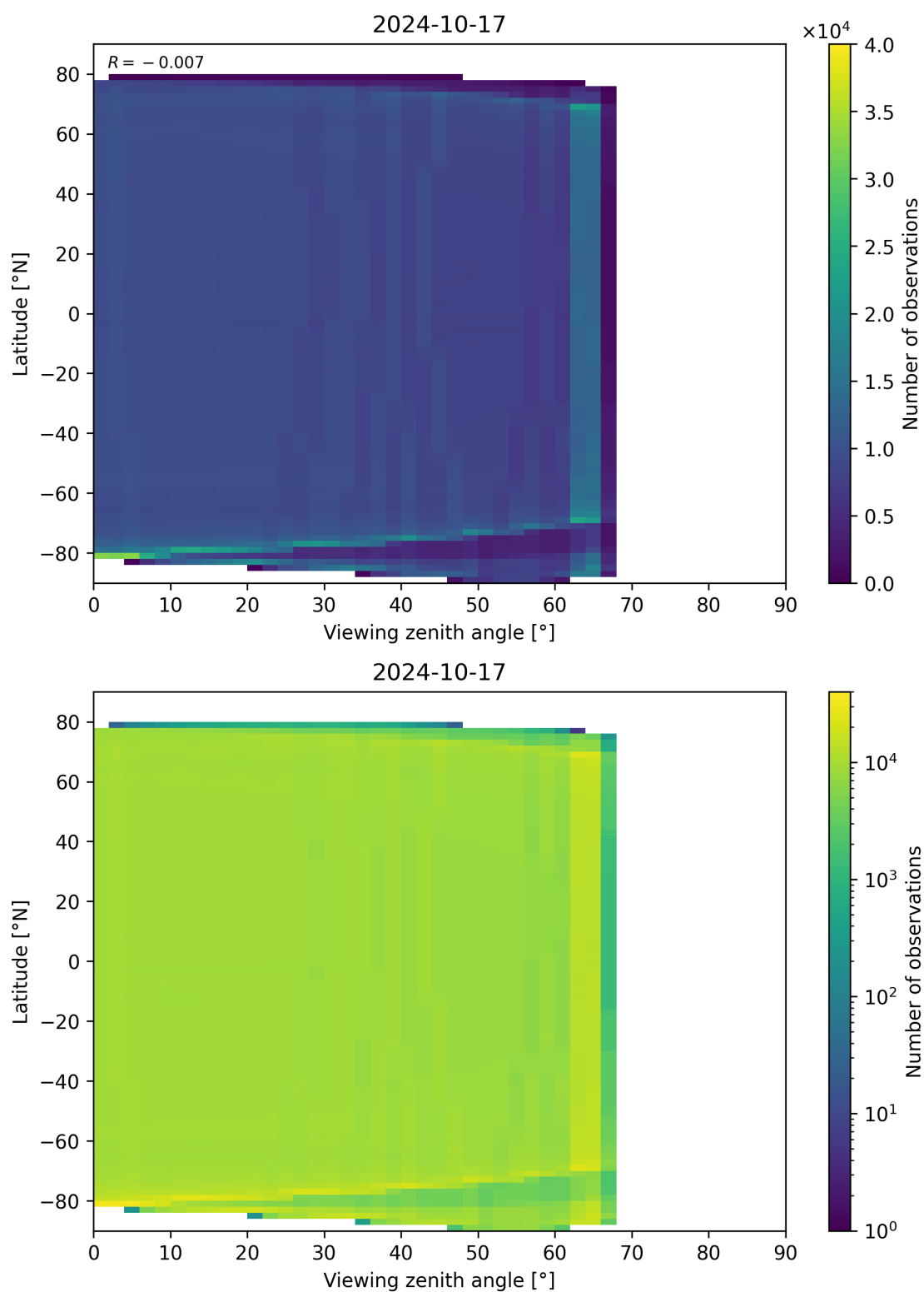
Figure 135: Scatter density plot of “Viewing zenith angle” against “Latitude” for 2024-10-16 to 2024-10-18.
