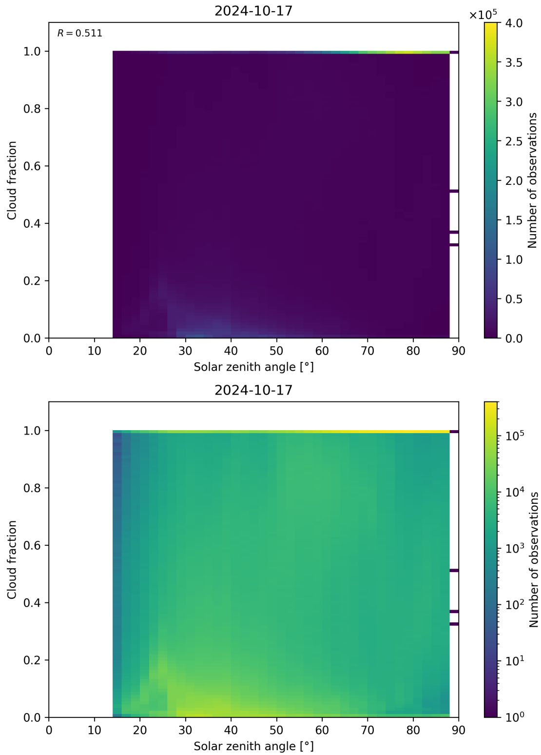
Figure 121: Scatter density plot of “Solar zenith angle” against “Cloud fraction” for 2024-10-16 to 2024-10-18.
