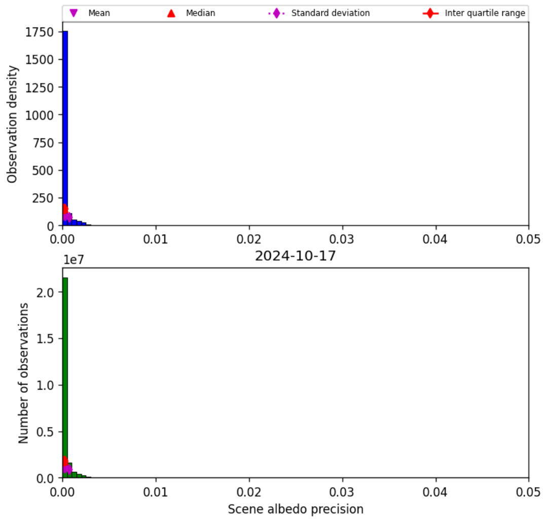
Figure 35: Histogram of “Scene albedo precision” for 2024-10-16 to 2024-10-18
