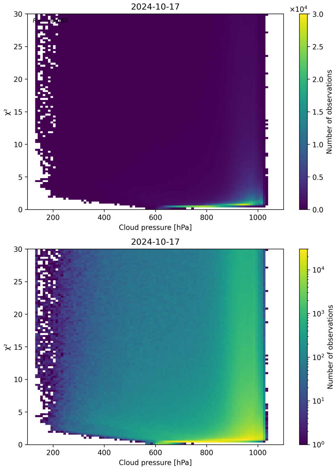
Figure 85: Scatter density plot of “Cloud pressure” against “ \chi^2 ” for 2024-10-16 to 2024-10-18.
