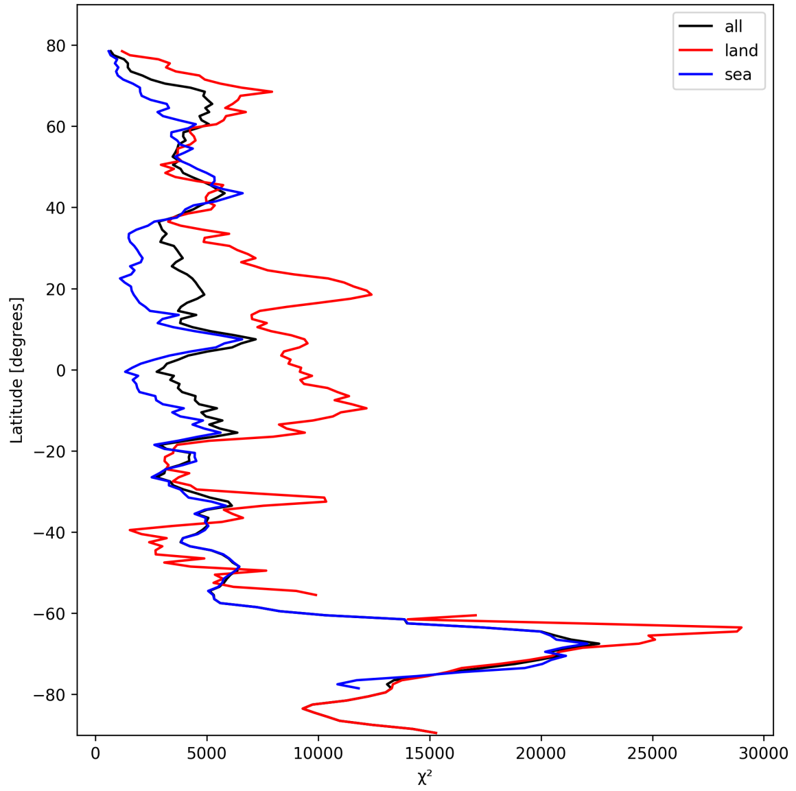
Figure 21: Zonal average of “ \chi^2 ” for 2024-10-16 to 2024-10-18.
