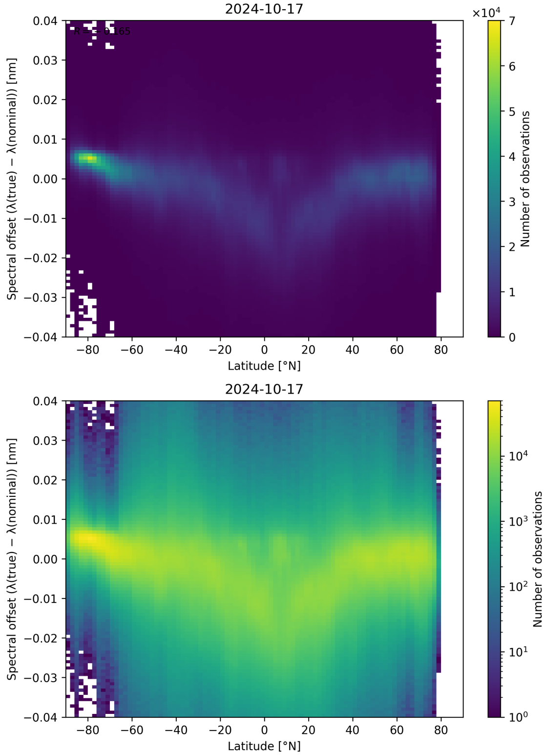
Figure 105: Scatter density plot of “Latitude” against “Spectral offset ( \lambda_{\text{true}} - \lambda_{\text{nominal}} )” for 2024-10-16 to 2024-10-18.
