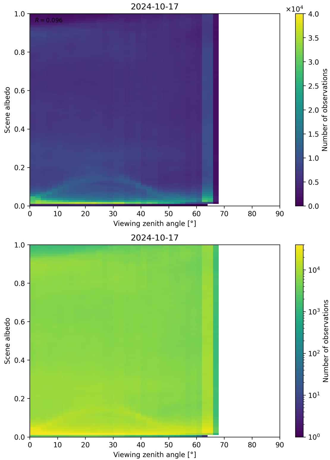
Figure 138: Scatter density plot of “Viewing zenith angle” against “Scene albedo” for 2024-10-16 to 2024-10-18.
