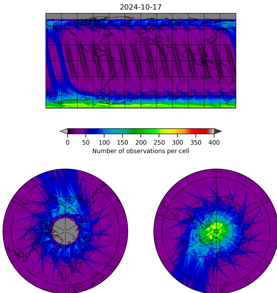
Figure 11: Map of the number of observations for 2024-10-16 to 2024-10-18
