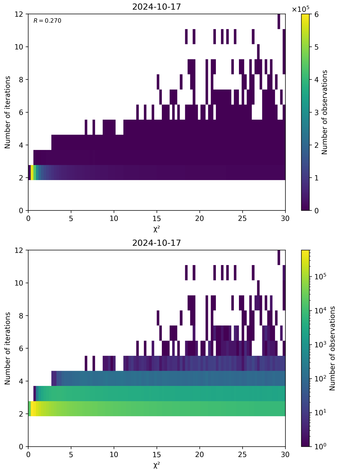
Figure 73: Scatter density plot of “ \chi^2 ” against “Number of iterations” for 2024-10-16 to 2024-10-18.
