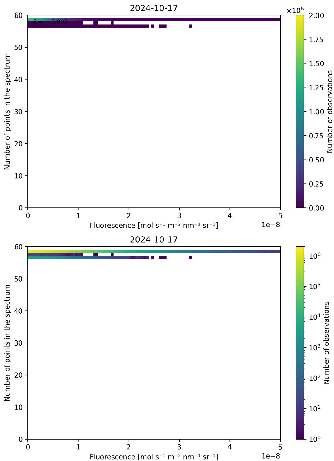
Figure 94: Scatter density plot of “Fluorescence” against “Number of points in the spectrum” for 2024-10-16 to 2024-10-18.
