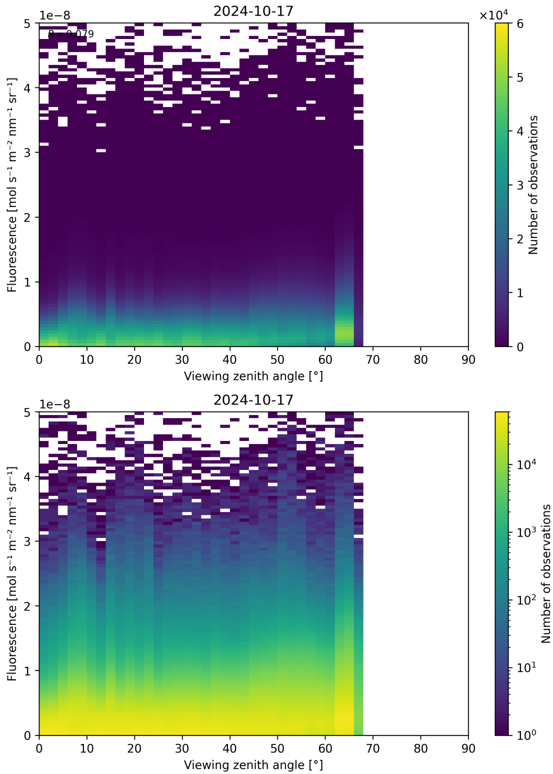
Figure 134: Scatter density plot of “Viewing zenith angle” against “Fluorescence” for 2024-10-16 to 2024-10-18.
