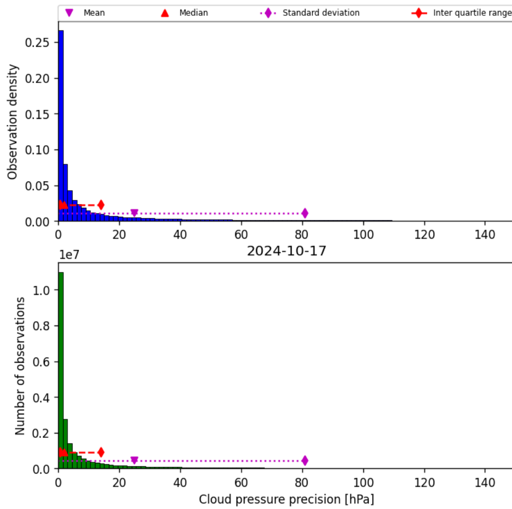
Figure 31: Histogram of “Cloud pressure precision” for 2024-10-16 to 2024-10-18
