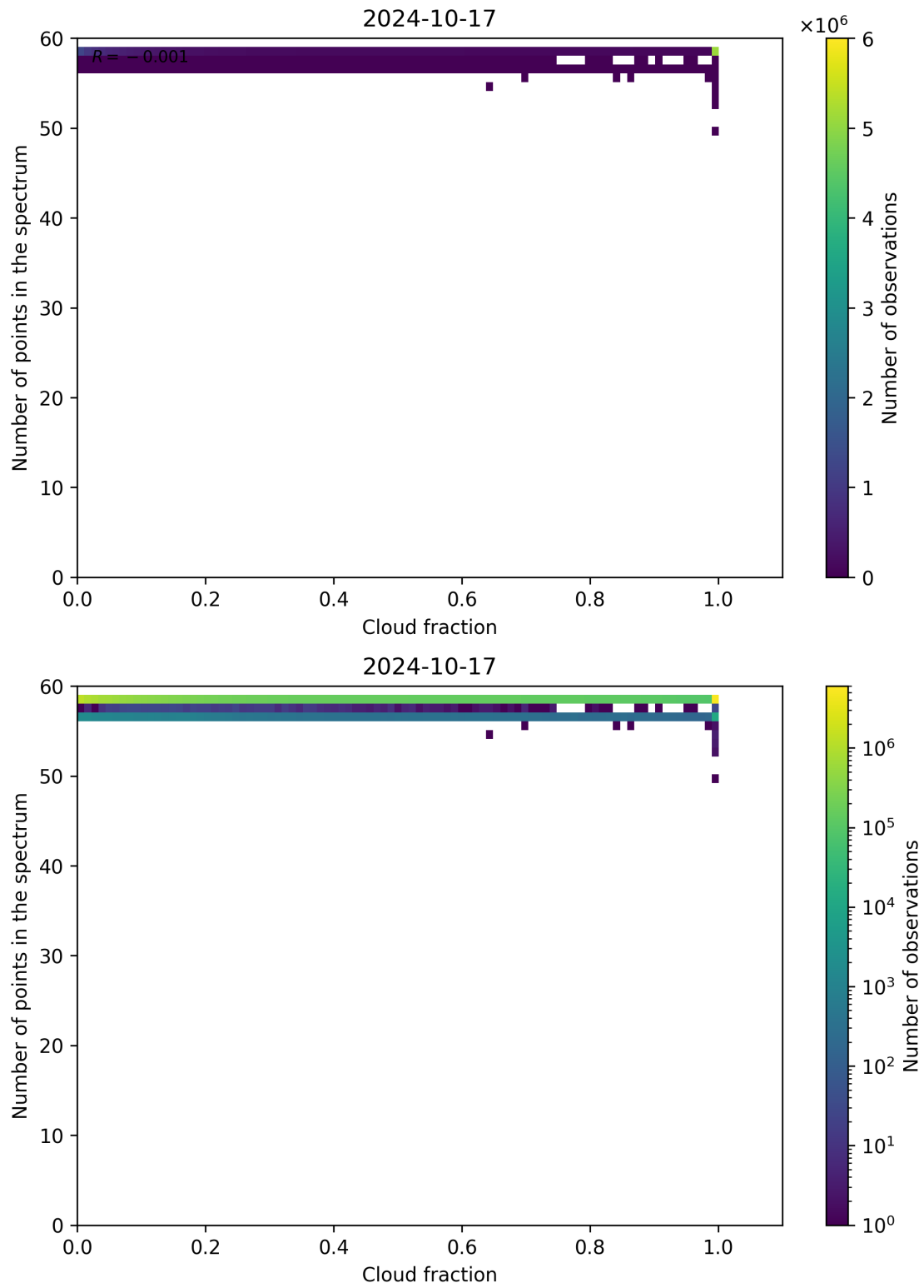
Figure 81: Scatter density plot of “Cloud fraction” against “Number of points in the spectrum” for 2024-10-16 to 2024-10-18.
