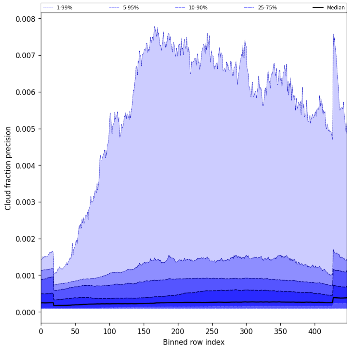
Figure 50: Along track statistics of “Cloud fraction precision” for 2024-10-16 to 2024-10-18
