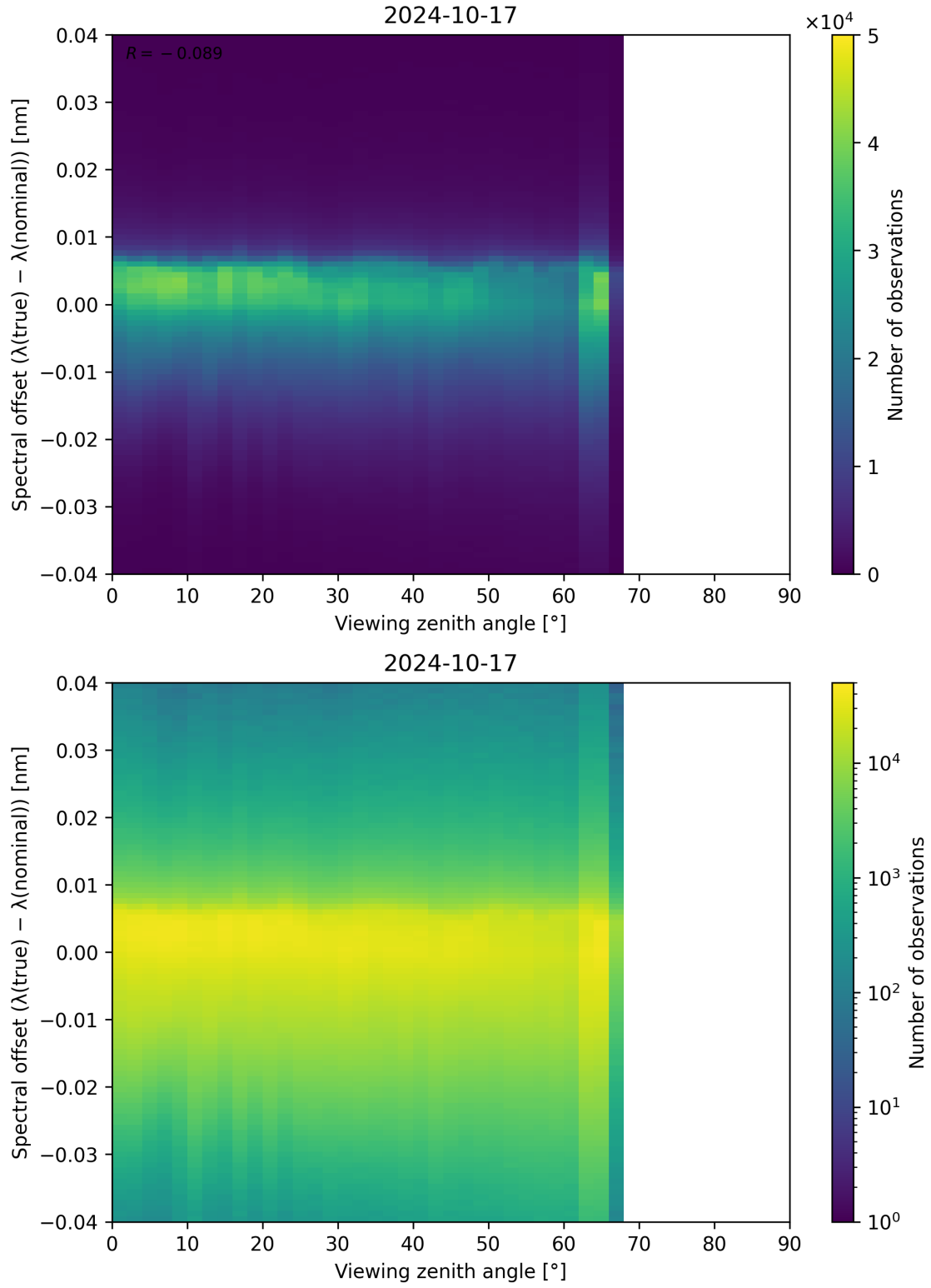
Figure 140: Scatter density plot of “Viewing zenith angle” against “Spectral offset ( \lambda_{\text{true}} - \lambda_{\text{nominal}} )” for 2024-10-16 to 2024-10-18.
