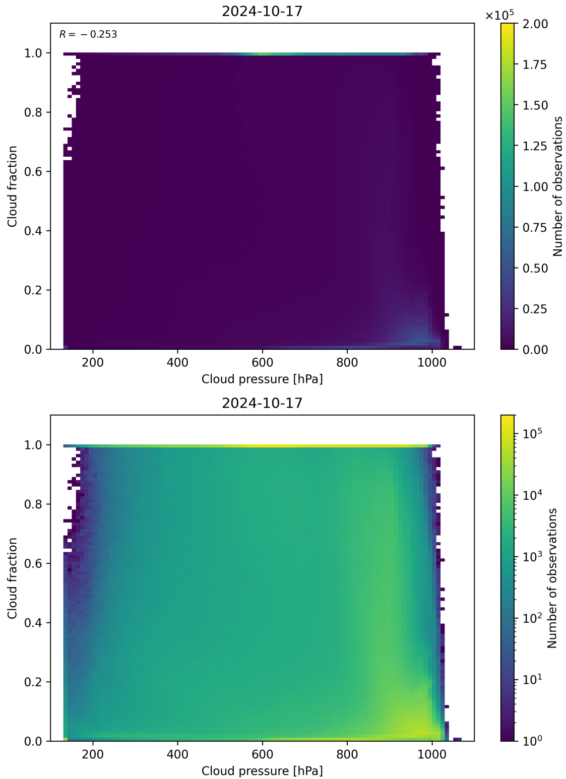
Figure 87: Scatter density plot of “Cloud pressure” against “Cloud fraction” for 2024-10-16 to 2024-10-18.
