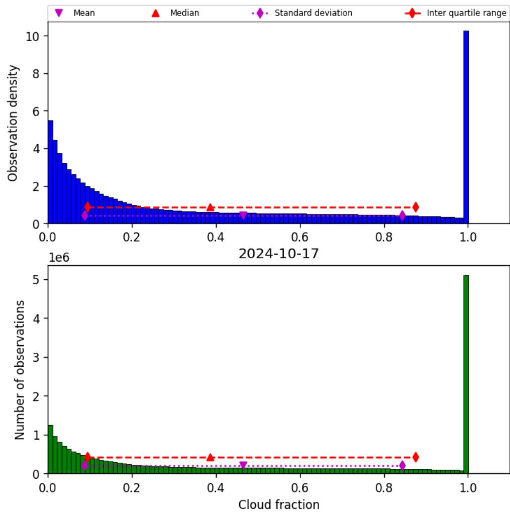
Figure 32: Histogram of “Cloud fraction” for 2024-10-16 to 2024-10-18
