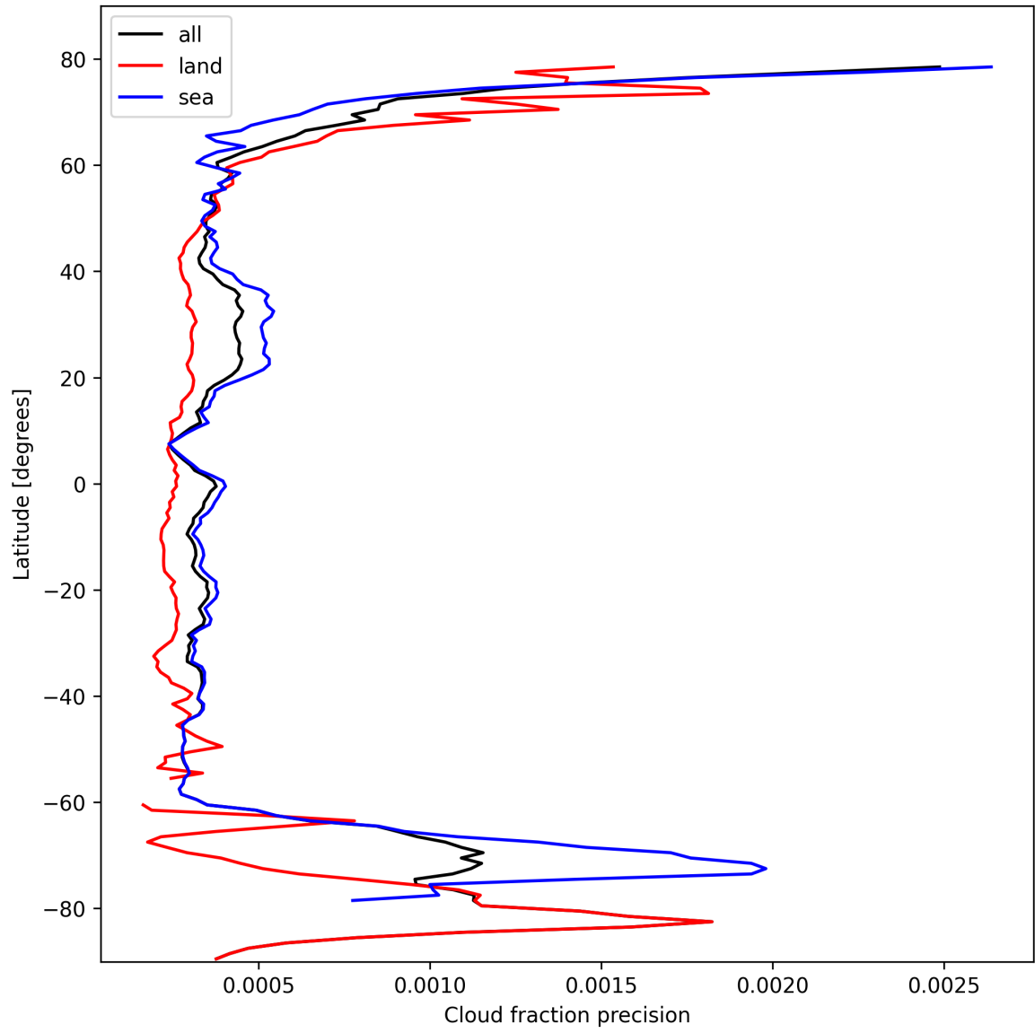
Figure 16: Zonal average of “Cloud fraction precision” for 2024-10-16 to 2024-10-18.
