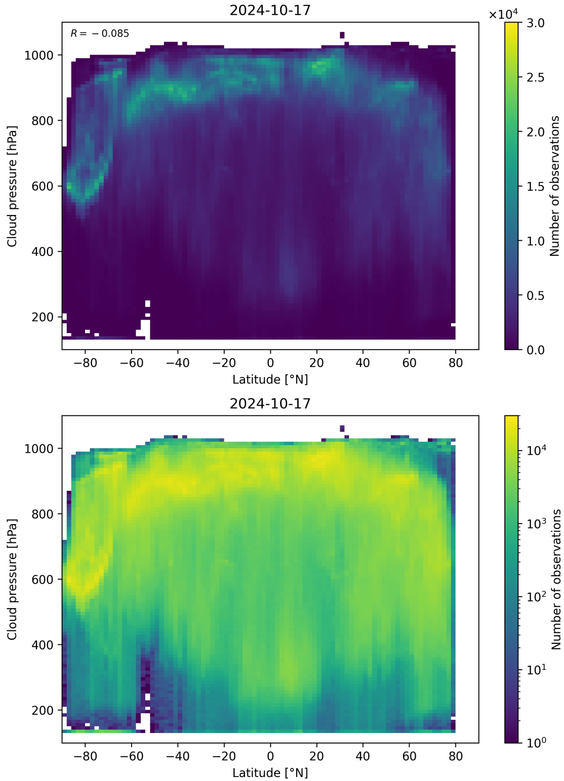
Figure 100: Scatter density plot of “Latitude” against “Cloud pressure” for 2024-10-16 to 2024-10-18.
