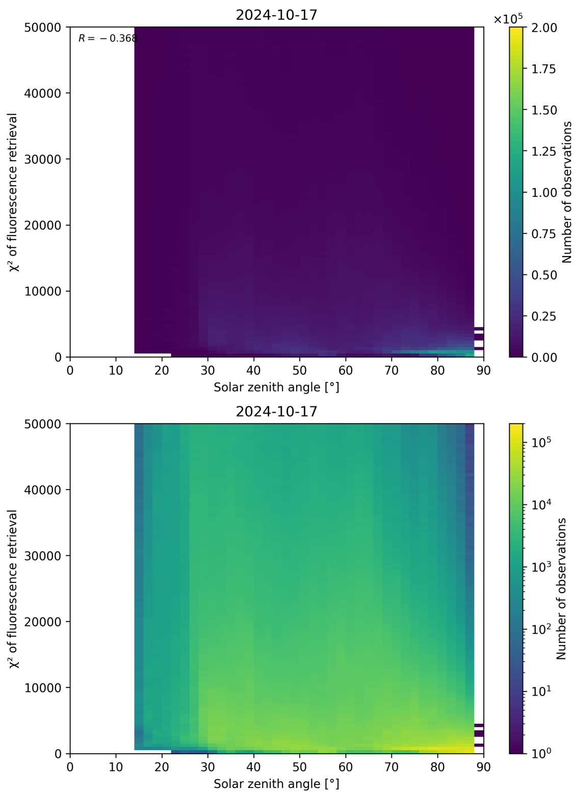
Figure 120: Scatter density plot of “Solar zenith angle” against “ \chi^2 of fluorescence retrieval” for 2024-10-16 to 2024-10-18.
