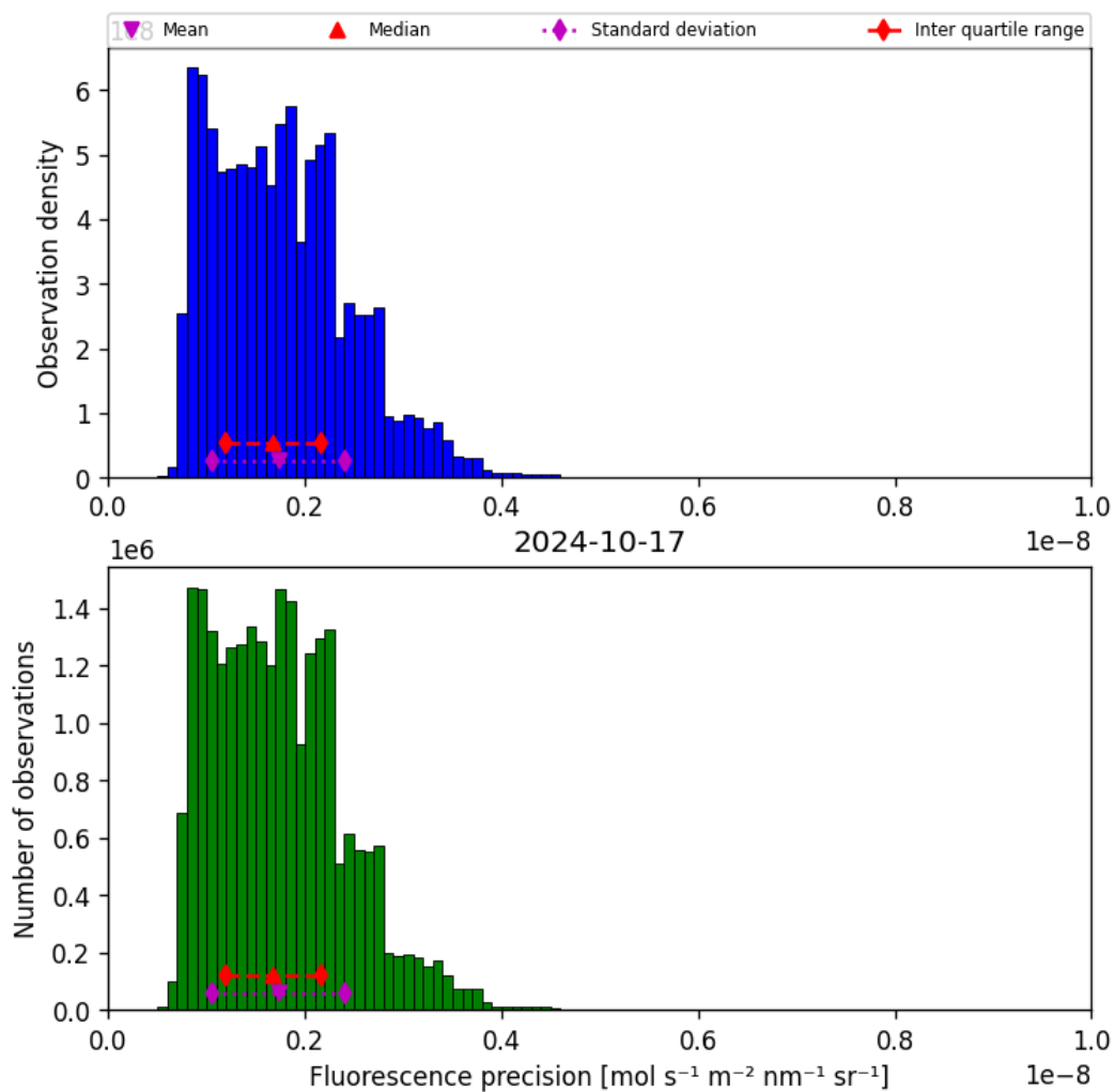
Figure 41: Histogram of “Fluorescence precision” for 2024-10-16 to 2024-10-18
