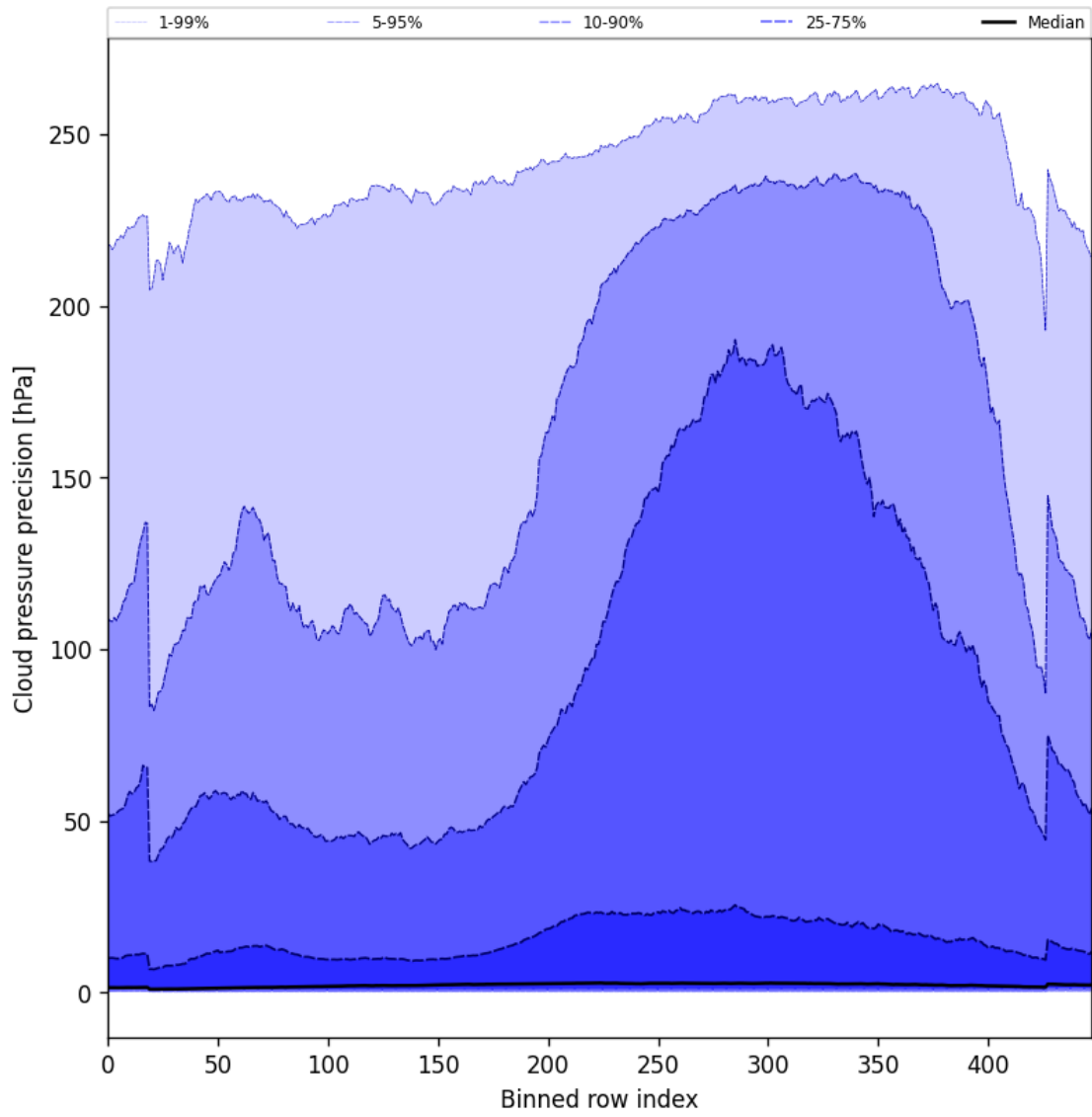
Figure 48: Along track statistics of “Cloud pressure precision” for 2024-10-16 to 2024-10-18
