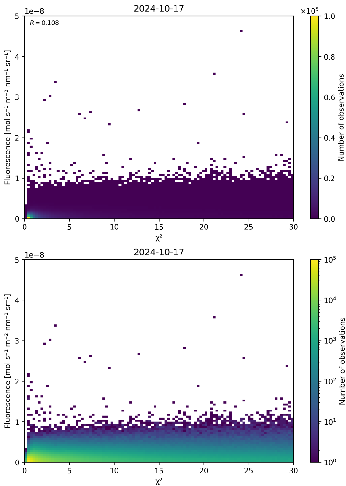
Figure 70: Scatter density plot of “ \chi^2 ” against “Fluorescence” for 2024-10-16 to 2024-10-18.
