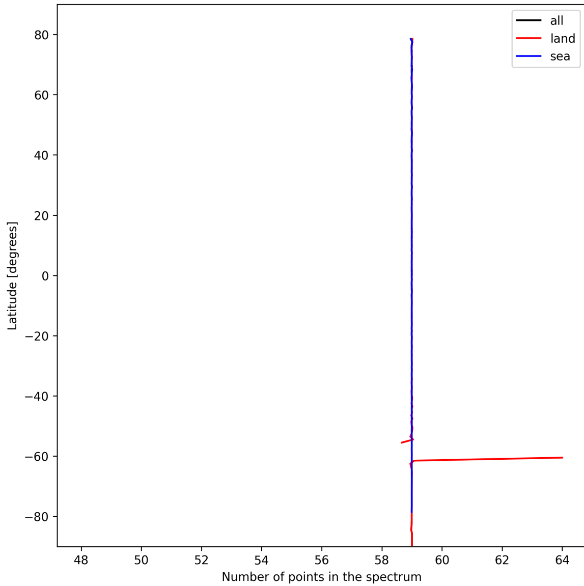
Figure 27: Zonal average of “Number of points in the spectrum” for 2024-10-16 to 2024-10-18.
