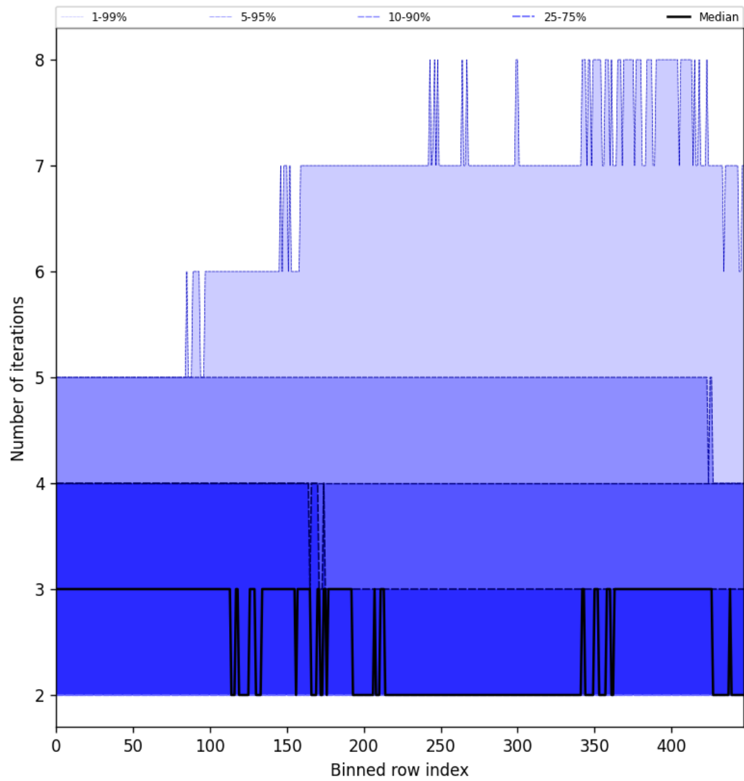
Figure 56: Along track statistics of “Number of iterations” for 2024-10-16 to 2024-10-18
