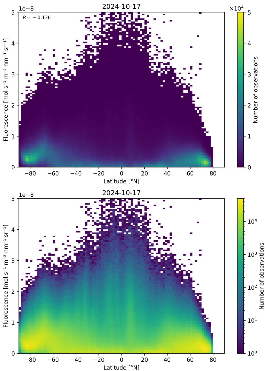
Figure 101: Scatter density plot of “Latitude” against “Fluorescence” for 2024-10-16 to 2024-10-18.
