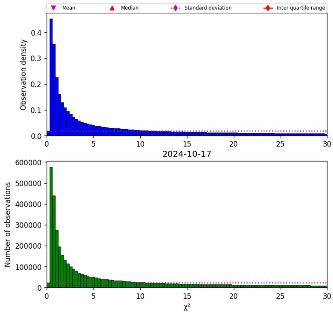
Figure 38: Histogram of “ \chi^2 ” for 2024-10-16 to 2024-10-18
