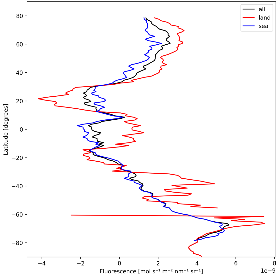
Figure 23: Zonal average of “Fluorescence” for 2024-10-16 to 2024-10-18.
