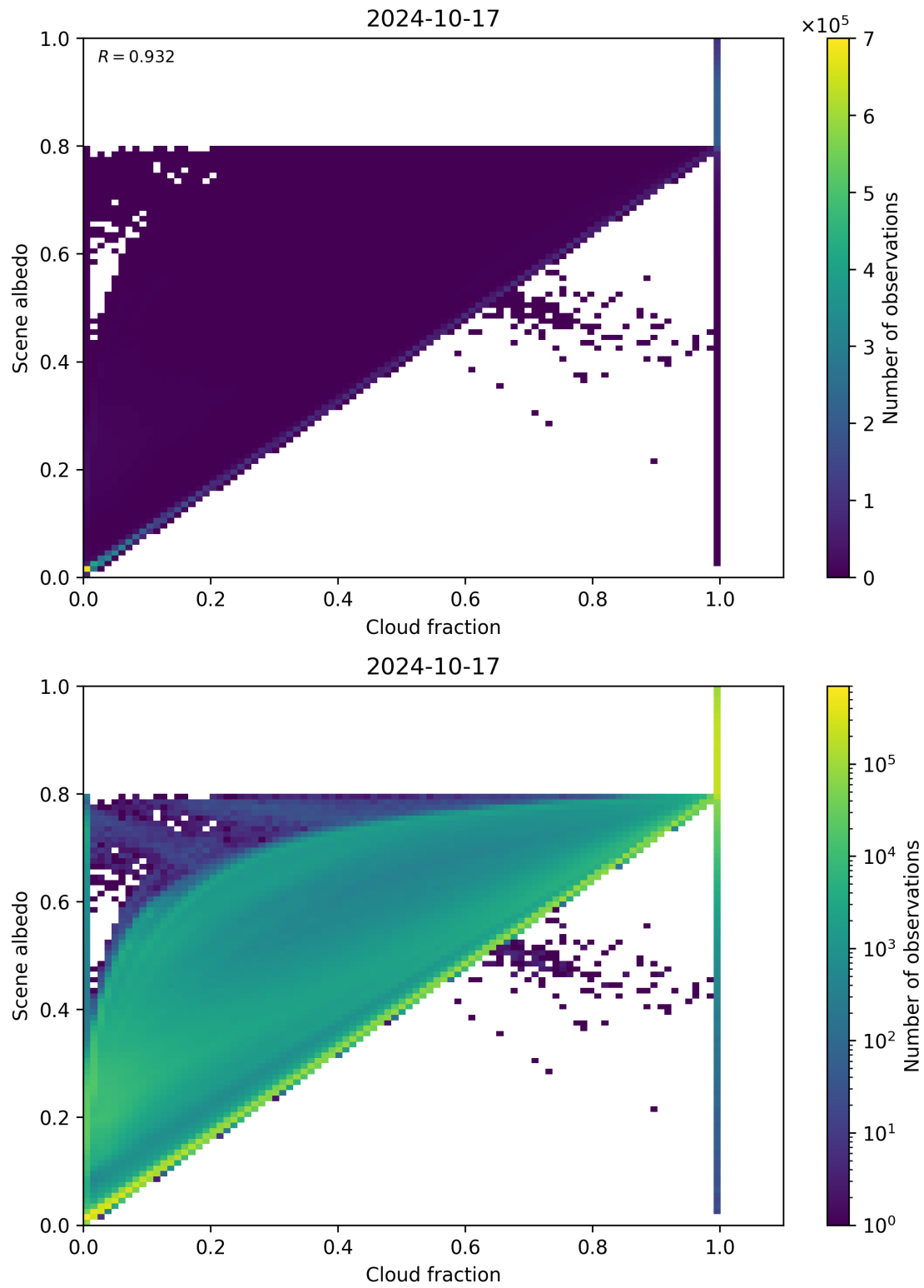
Figure 82: Scatter density plot of “Cloud fraction” against “Scene albedo” for 2024-10-16 to 2024-10-18.
