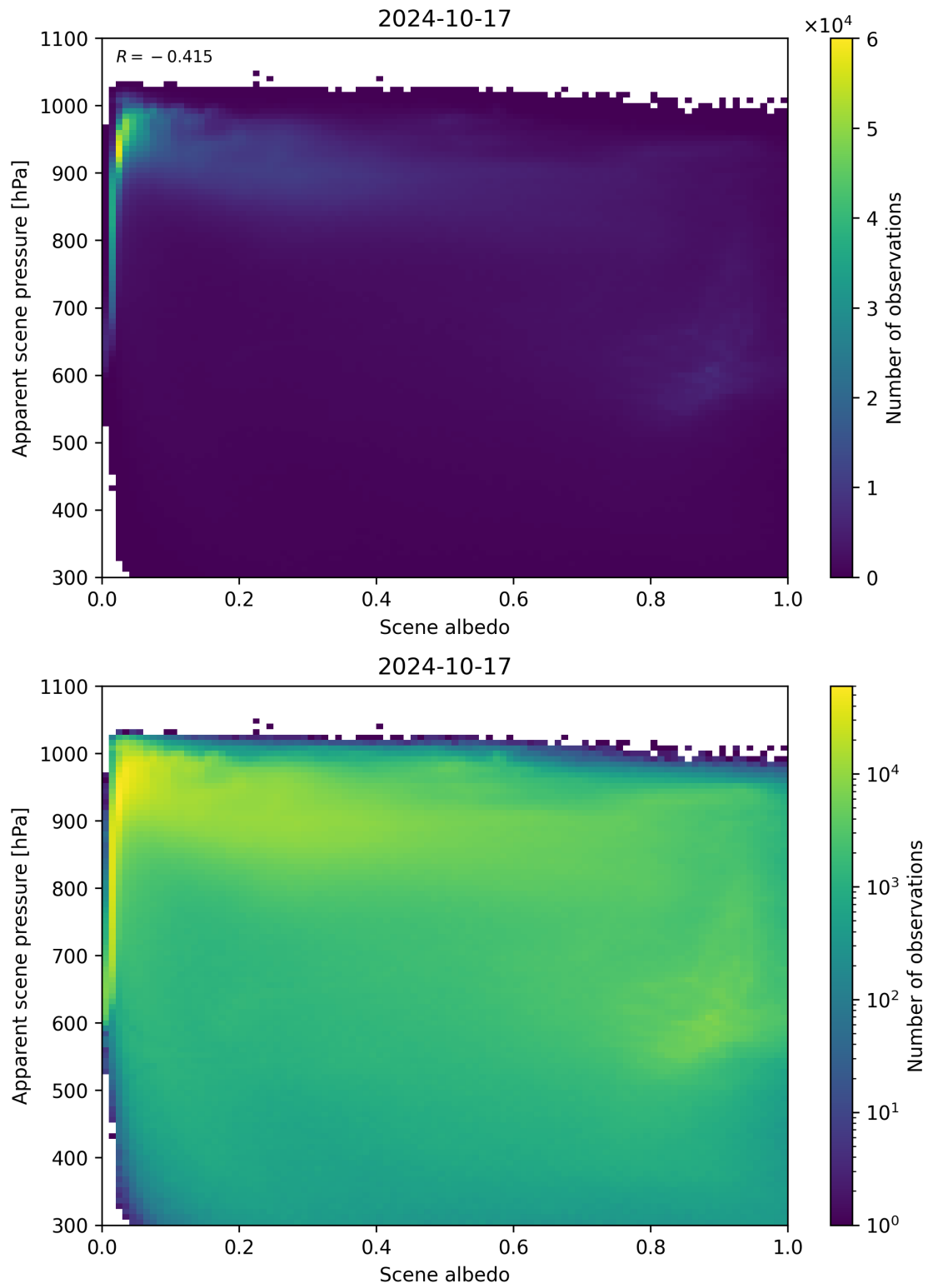
Figure 111: Scatter density plot of “Scene albedo” against “Apparent scene pressure” for 2024-10-16 to 2024-10-18.
