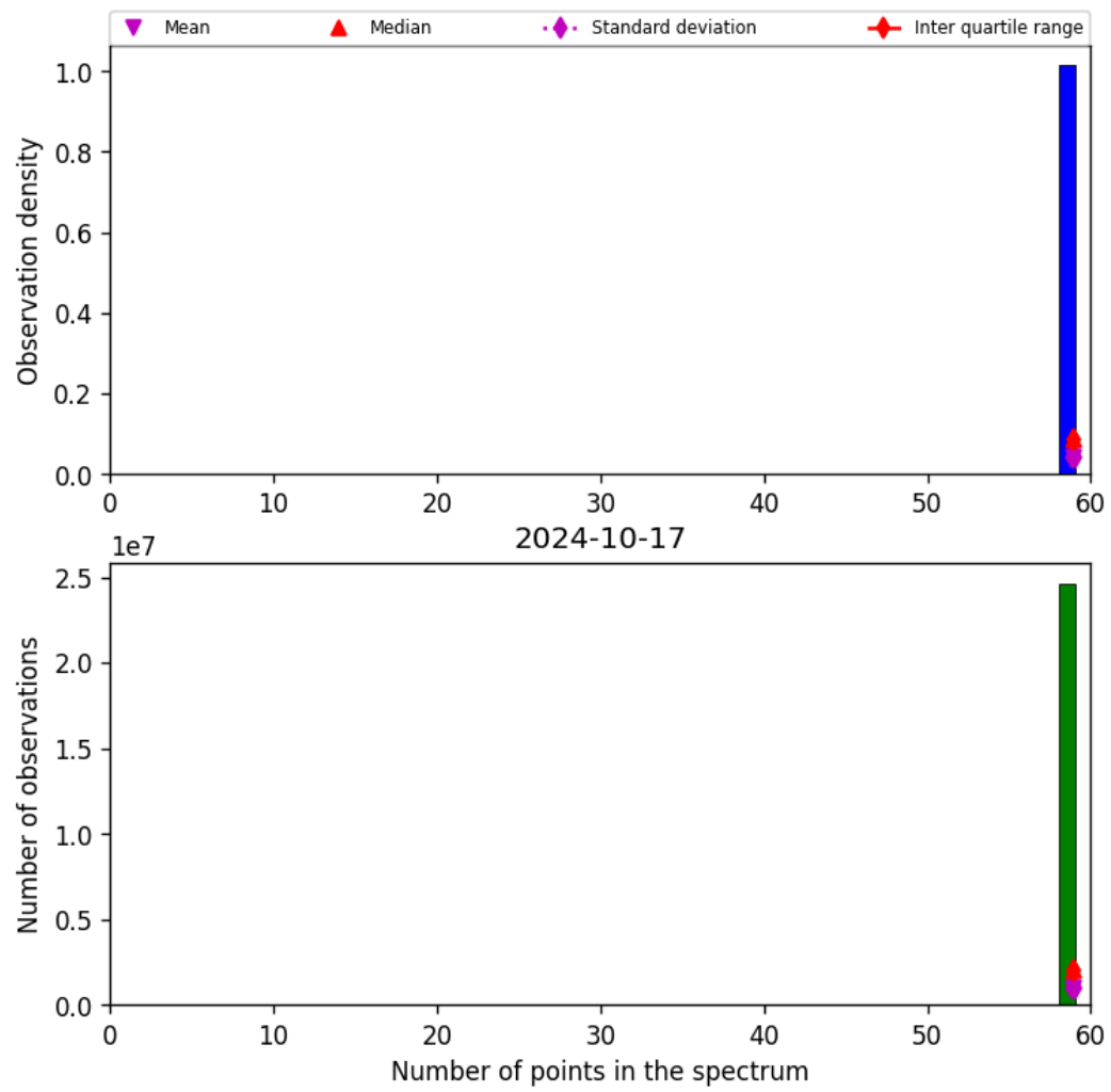
Figure 44: Histogram of “Number of points in the spectrum” for 2024-10-16 to 2024-10-18
