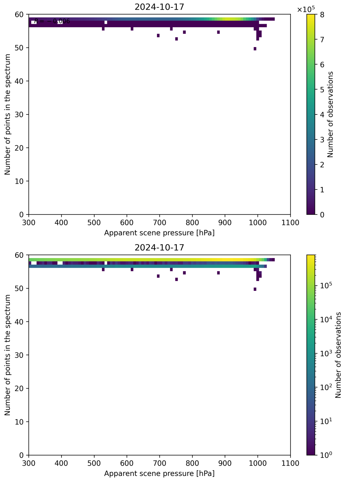
Figure 67: Scatter density plot of “Apparent scene pressure” against “Number of points in the spectrum” for 2024-10-16 to 2024-10-18.
