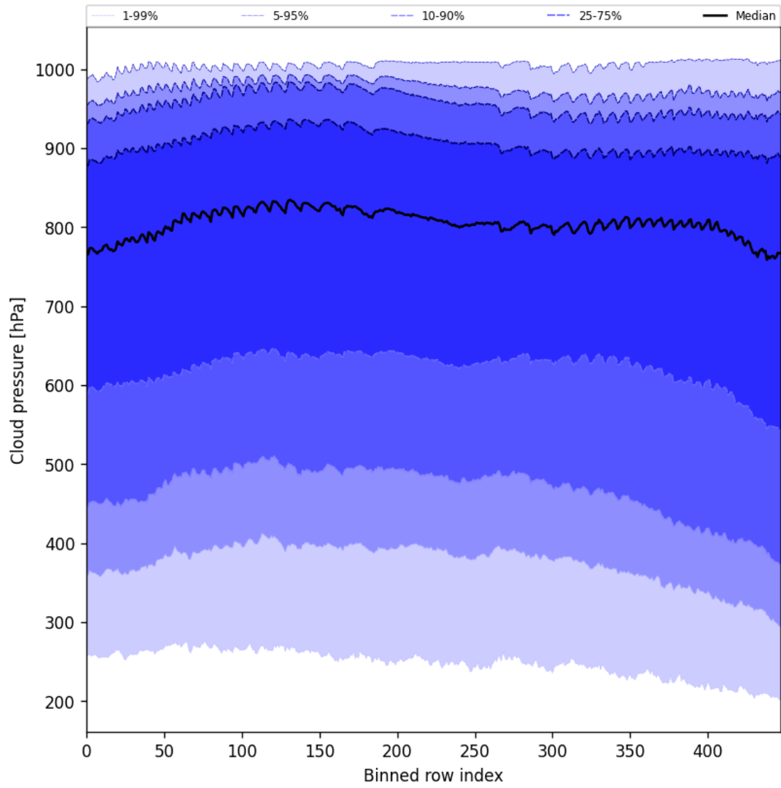
Figure 47: Along track statistics of “Cloud pressure” for 2024-10-16 to 2024-10-18
