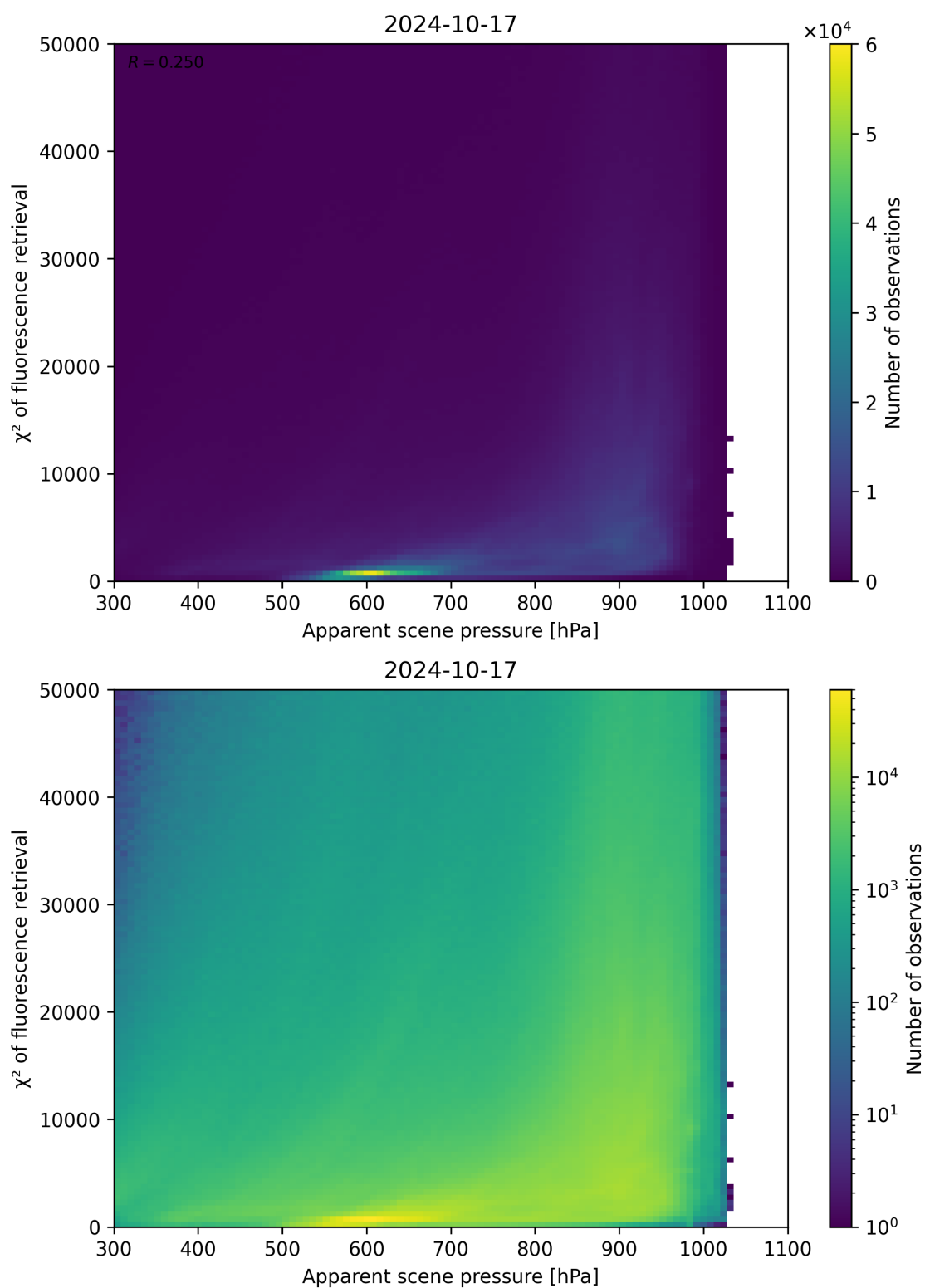
Figure 64: Scatter density plot of “Apparent scene pressure” against “ \chi^2 of fluorescence retrieval” for 2024-10-16 to 2024-10-18.
