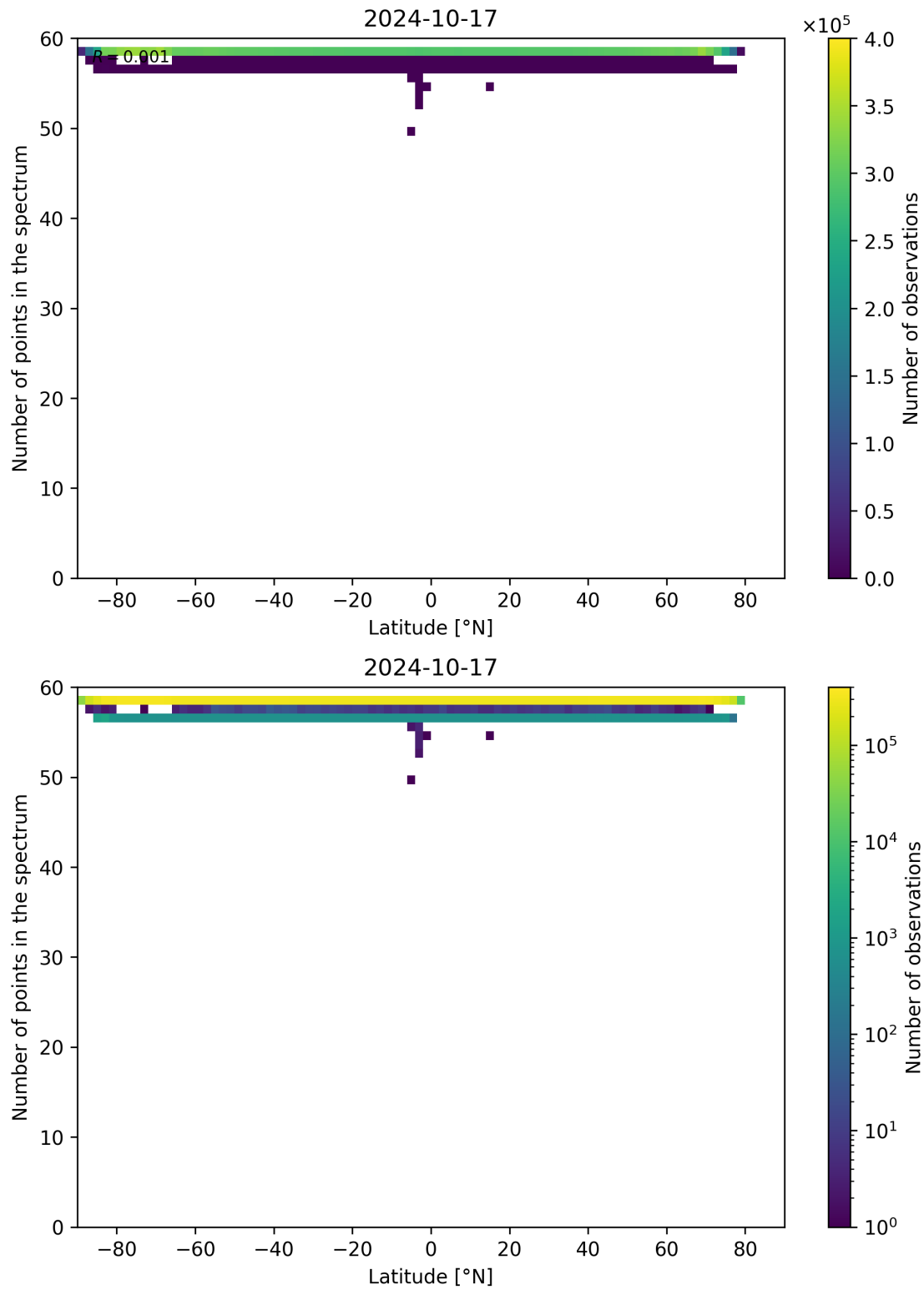
Figure 103: Scatter density plot of “Latitude” against “Number of points in the spectrum” for 2024-10-16 to 2024-10-18.
