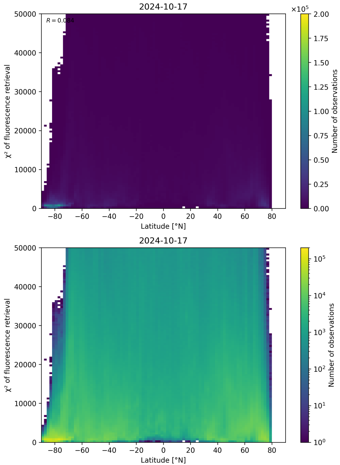
Figure 98: Scatter density plot of “Latitude” against “ \chi^2 of fluorescence retrieval” for 2024-10-16 to 2024-10-18.
