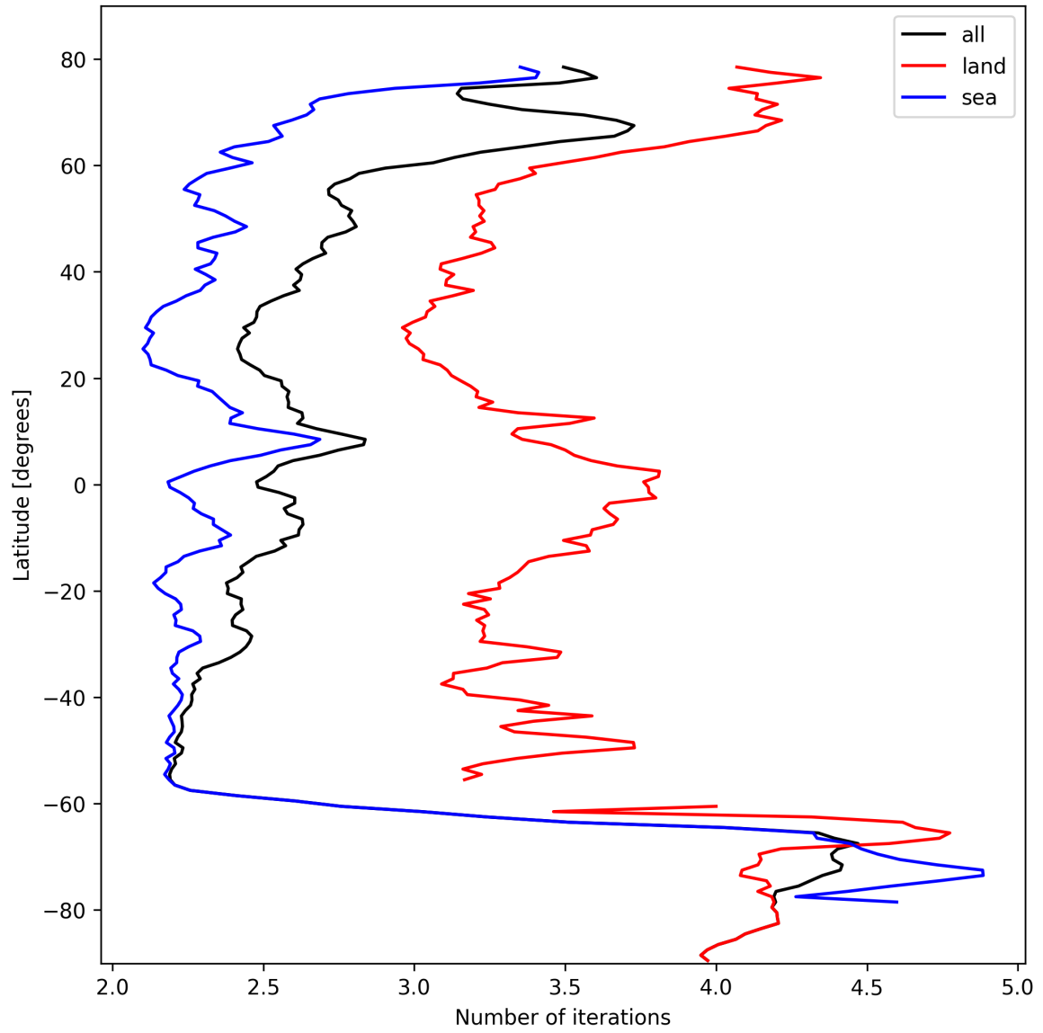
Figure 22: Zonal average of “Number of iterations” for 2024-10-16 to 2024-10-18.
