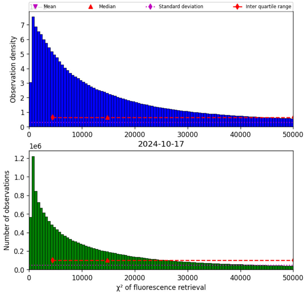
Figure 42: Histogram of “ \chi^2 of fluorescence retrieval” for 2024-10-16 to 2024-10-18
