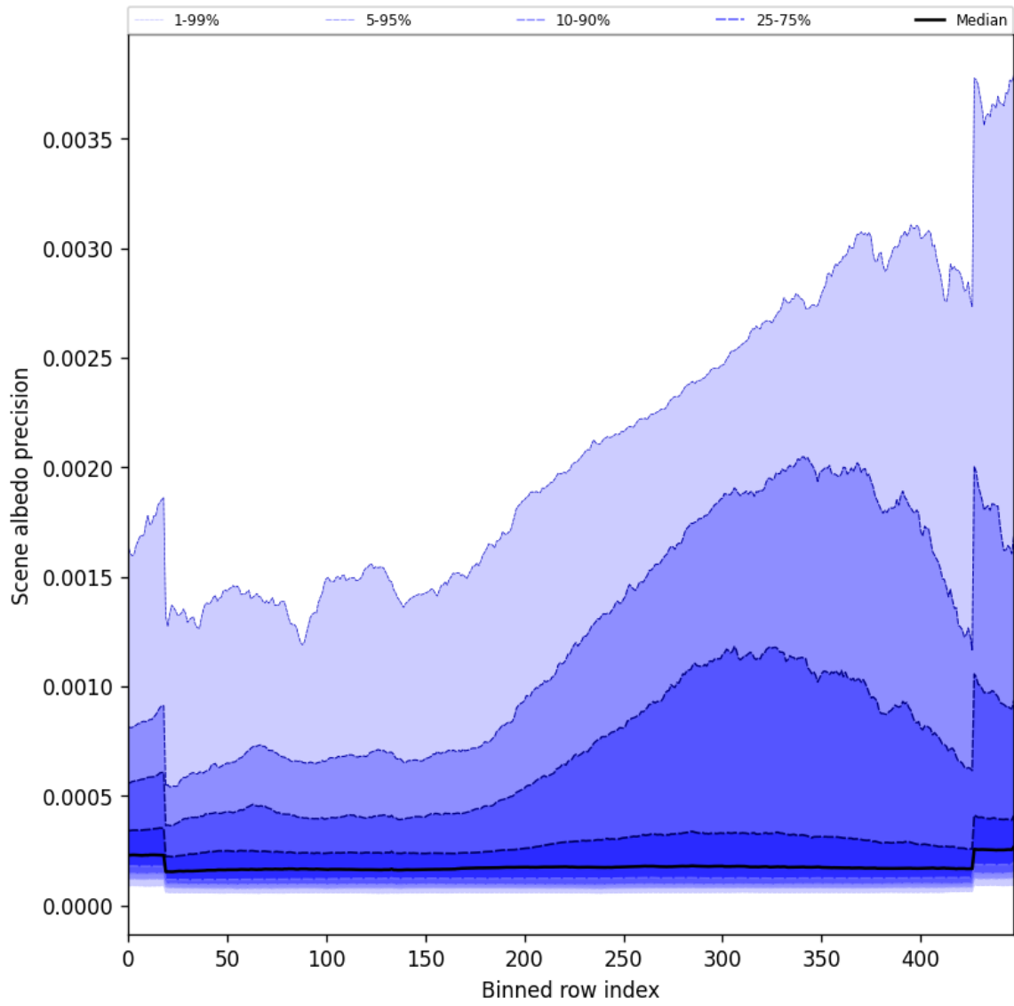
Figure 52: Along track statistics of “Scene albedo precision” for 2024-10-16 to 2024-10-18
