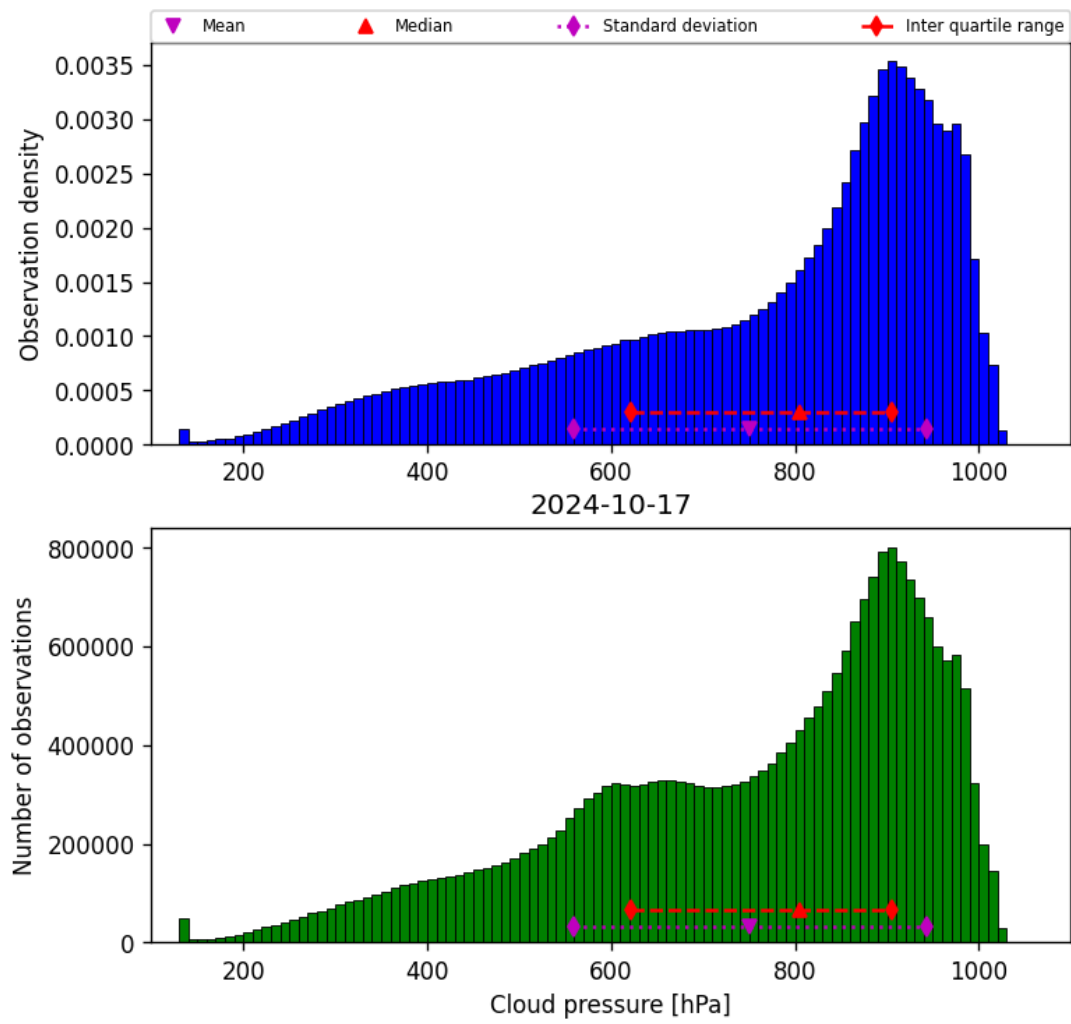
Figure 30: Histogram of “Cloud pressure” for 2024-10-16 to 2024-10-18
