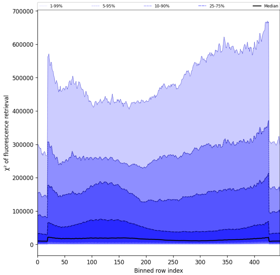
Figure 59: Along track statistics of “ \chi^2 of fluorescence retrieval” for 2024-10-16 to 2024-10-18
