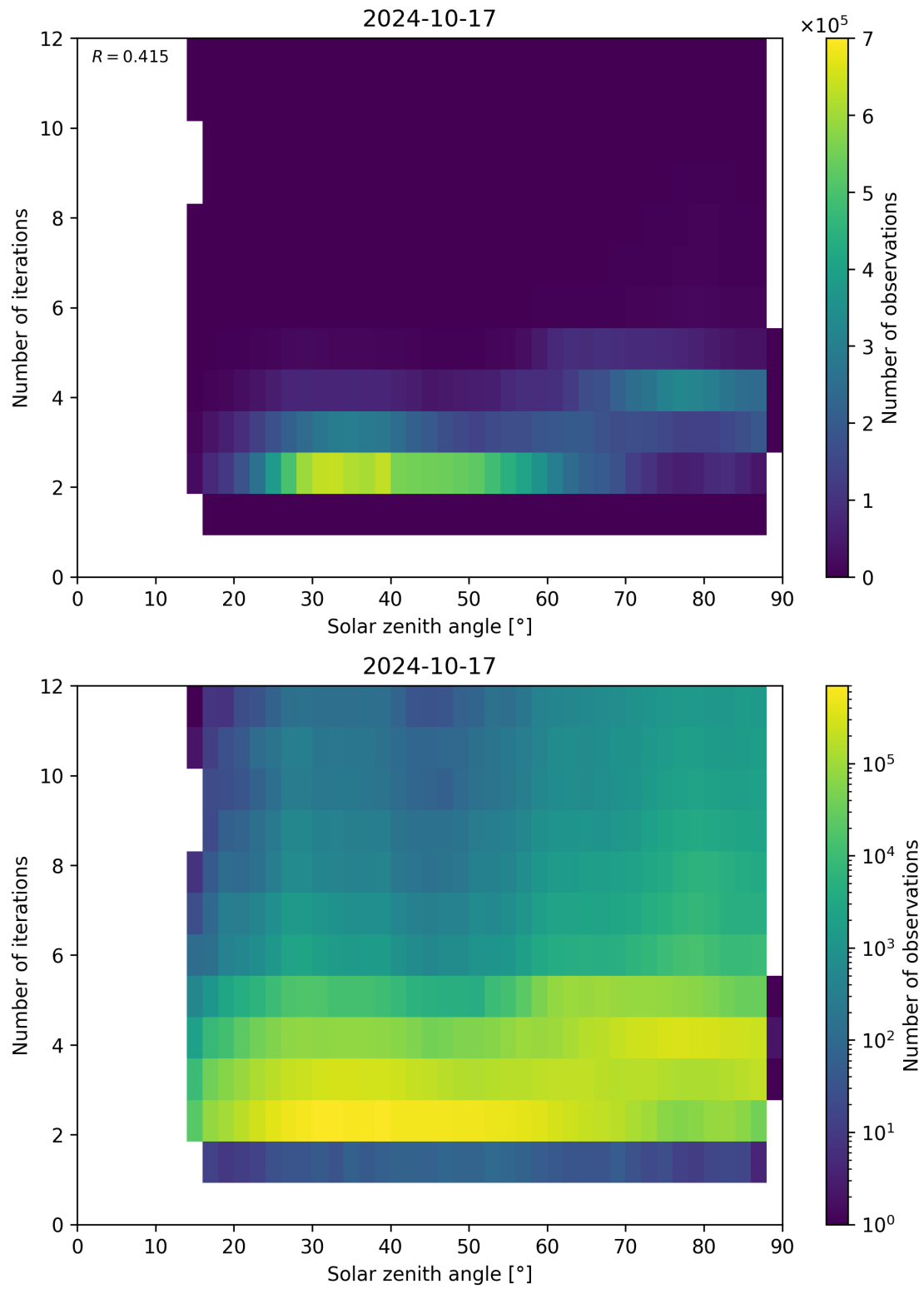
Figure 125: Scatter density plot of “Solar zenith angle” against “Number of iterations” for 2024-10-16 to 2024-10-18.
