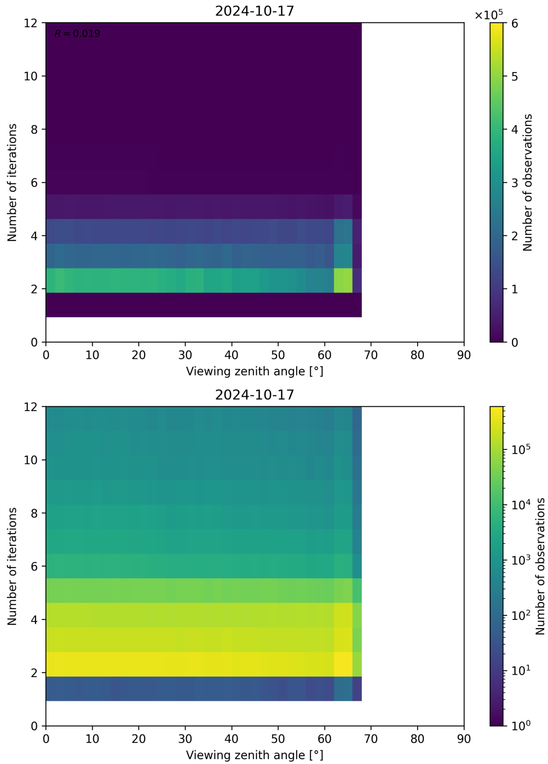
Figure 136: Scatter density plot of “Viewing zenith angle” against “Number of iterations” for 2024-10-16 to 2024-10-18.
