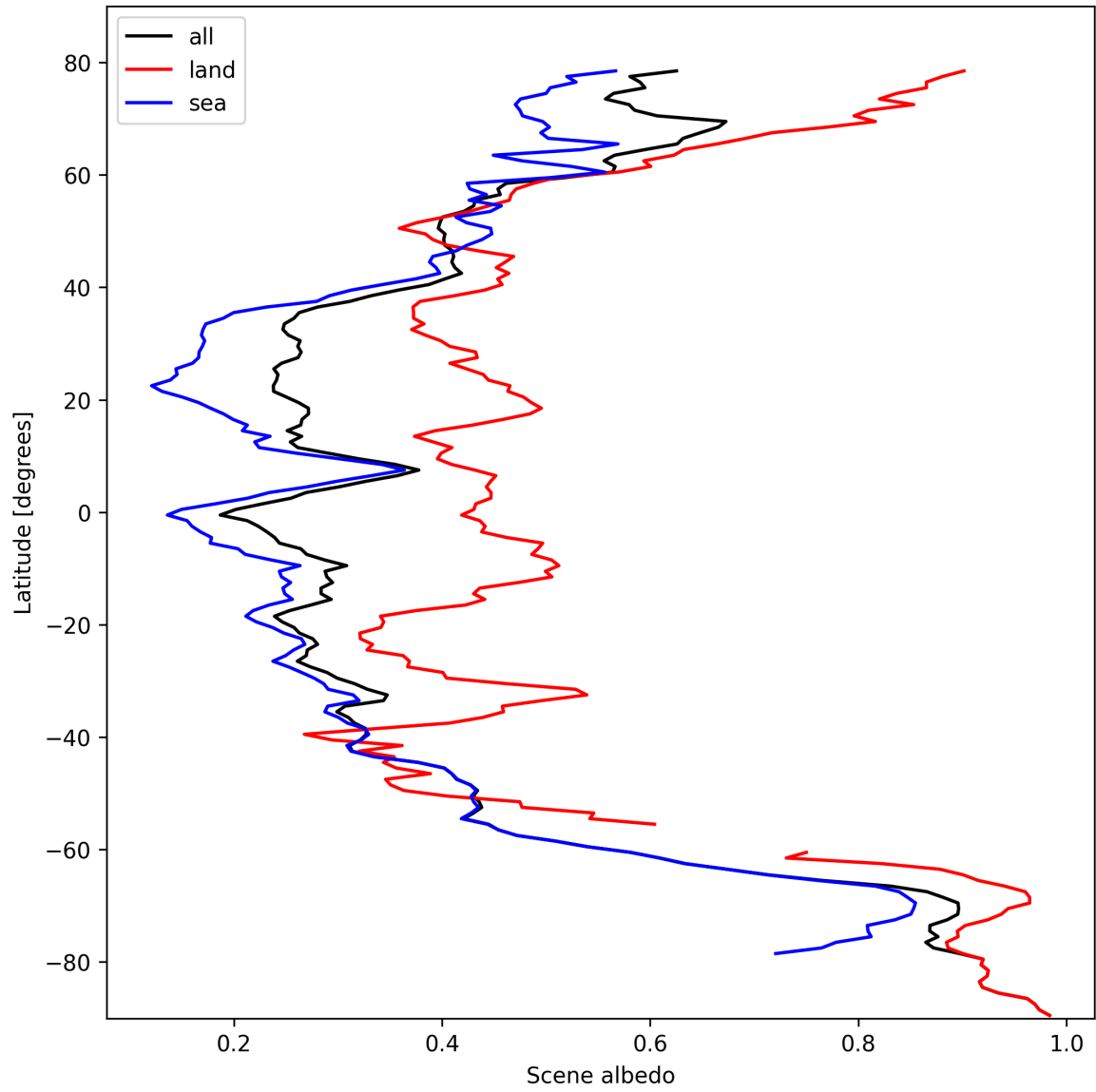
Figure 17: Zonal average of “Scene albedo” for 2024-10-16 to 2024-10-18.
