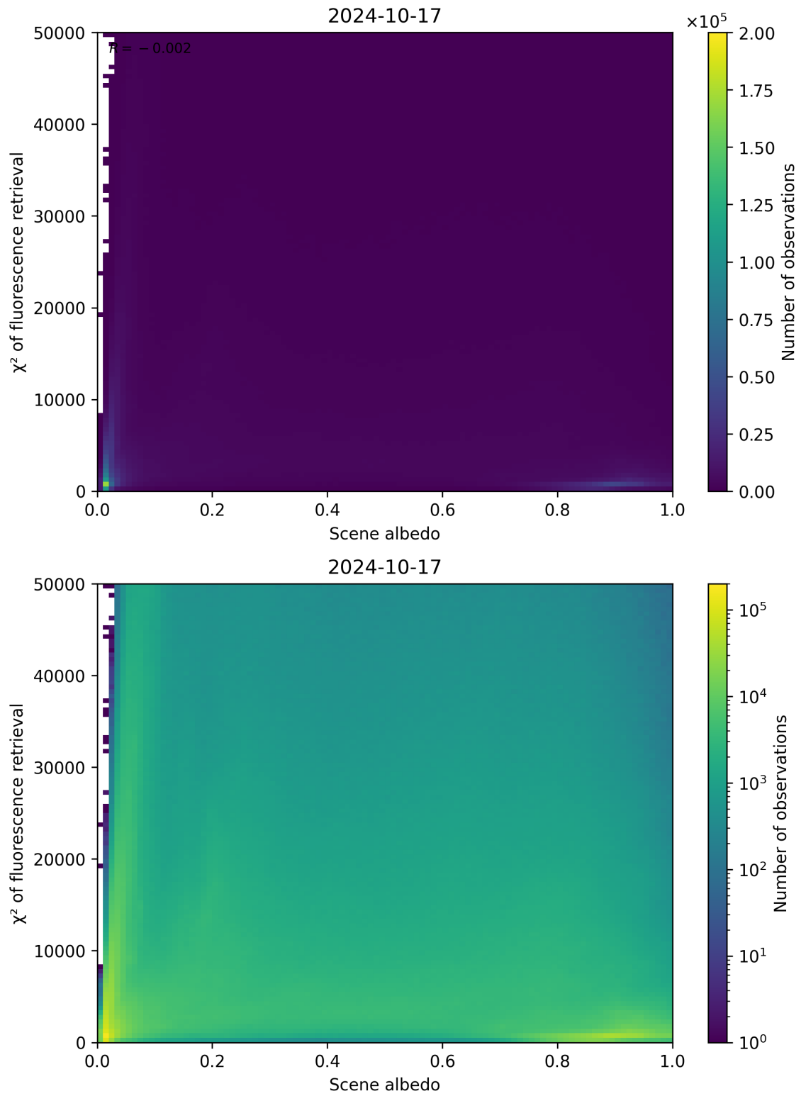
Figure 113: Scatter density plot of “Scene albedo” against “ \chi^2 of fluorescence retrieval” for 2024-10-16 to 2024-10-18.
