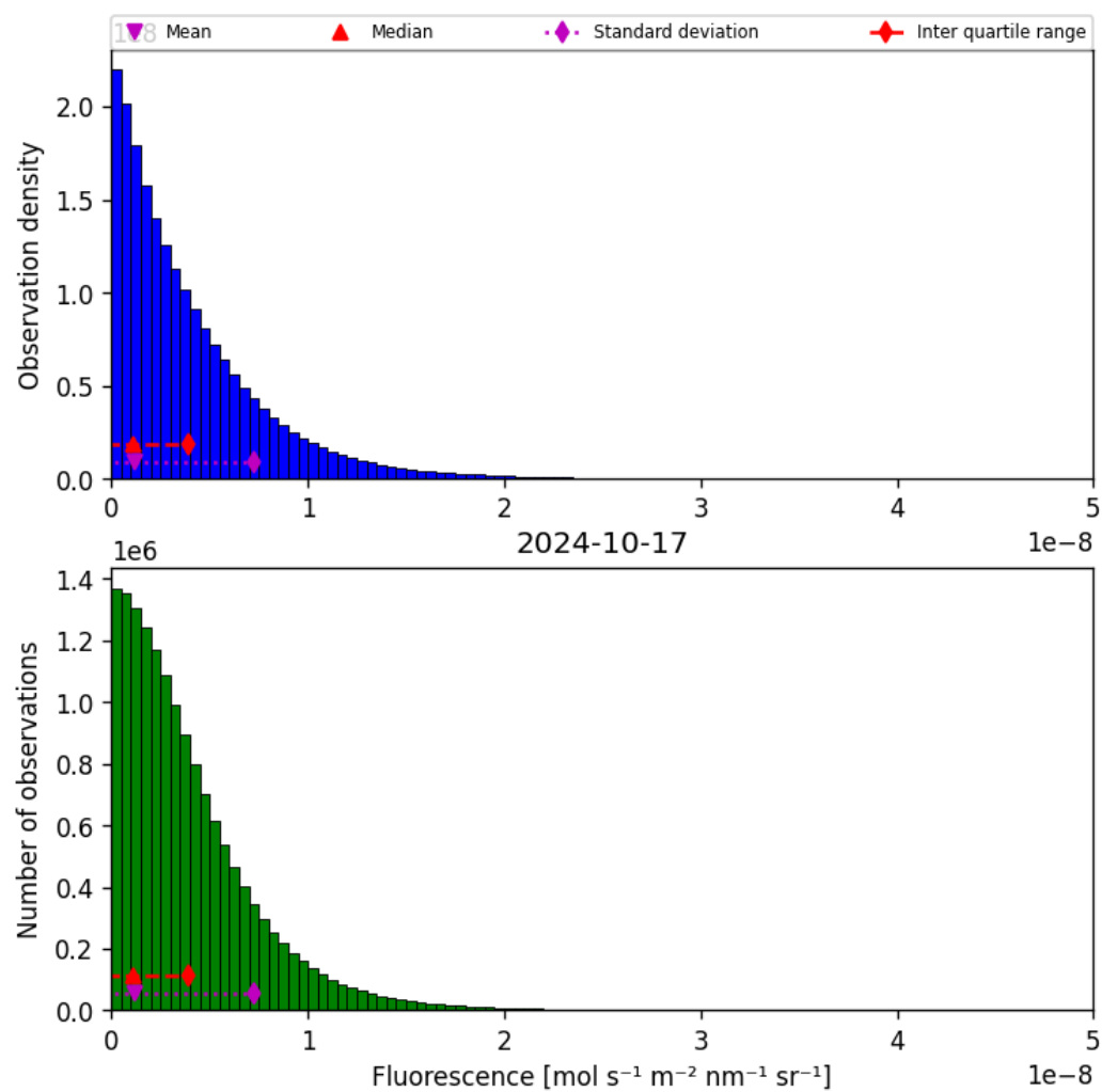
Figure 40: Histogram of “Fluorescence” for 2024-10-16 to 2024-10-18
