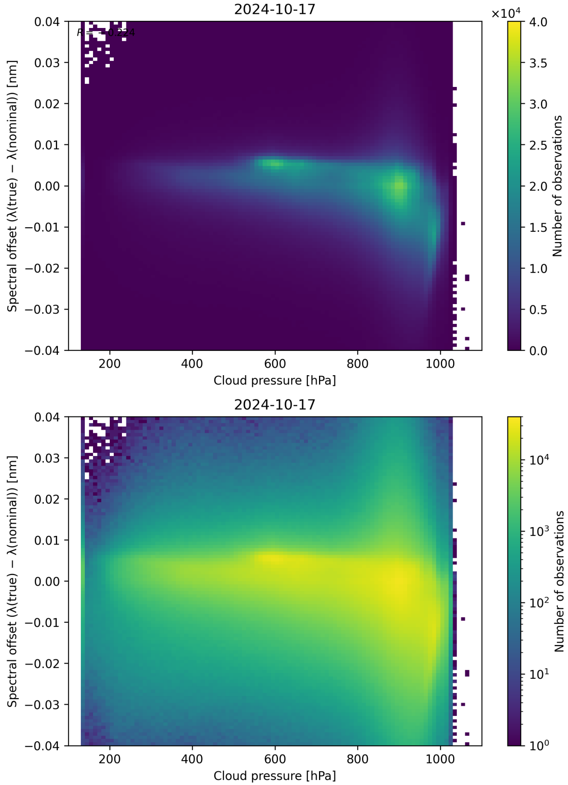
Figure 92: Scatter density plot of “Cloud pressure” against “Spectral offset ( \lambda_{\text{true}} - \lambda_{\text{nominal}} )” for 2024-10-16 to 2024-10-18.
