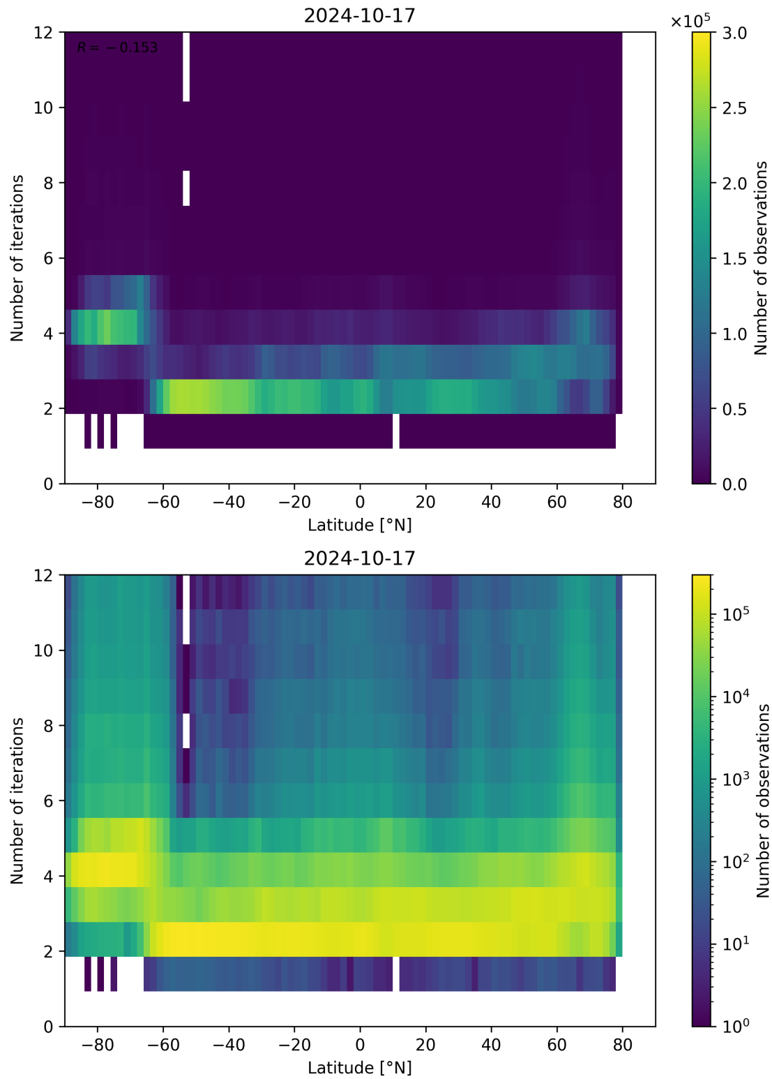
Figure 102: Scatter density plot of “Latitude” against “Number of iterations” for 2024-10-16 to 2024-10-18.
