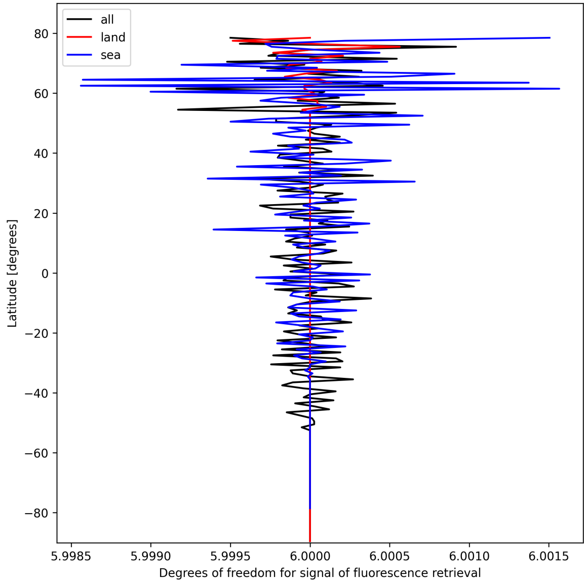
Figure 26: Zonal average of “Degrees of freedom for signal of fluorescence retrieval” for 2024-10-16 to 2024-10-18.
