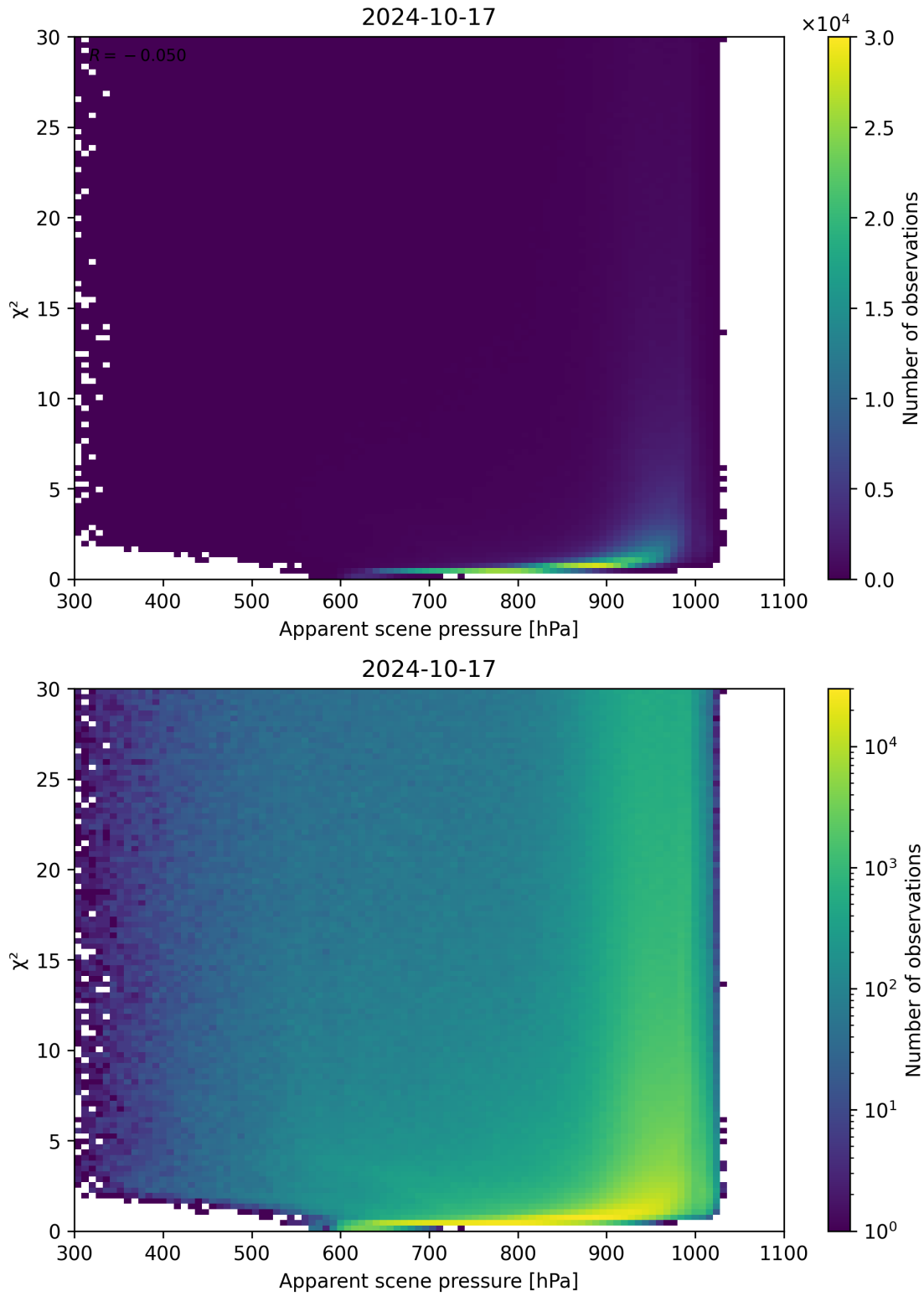
Figure 63: Scatter density plot of “Apparent scene pressure” against “ \chi^2 ” for 2024-10-16 to 2024-10-18.
