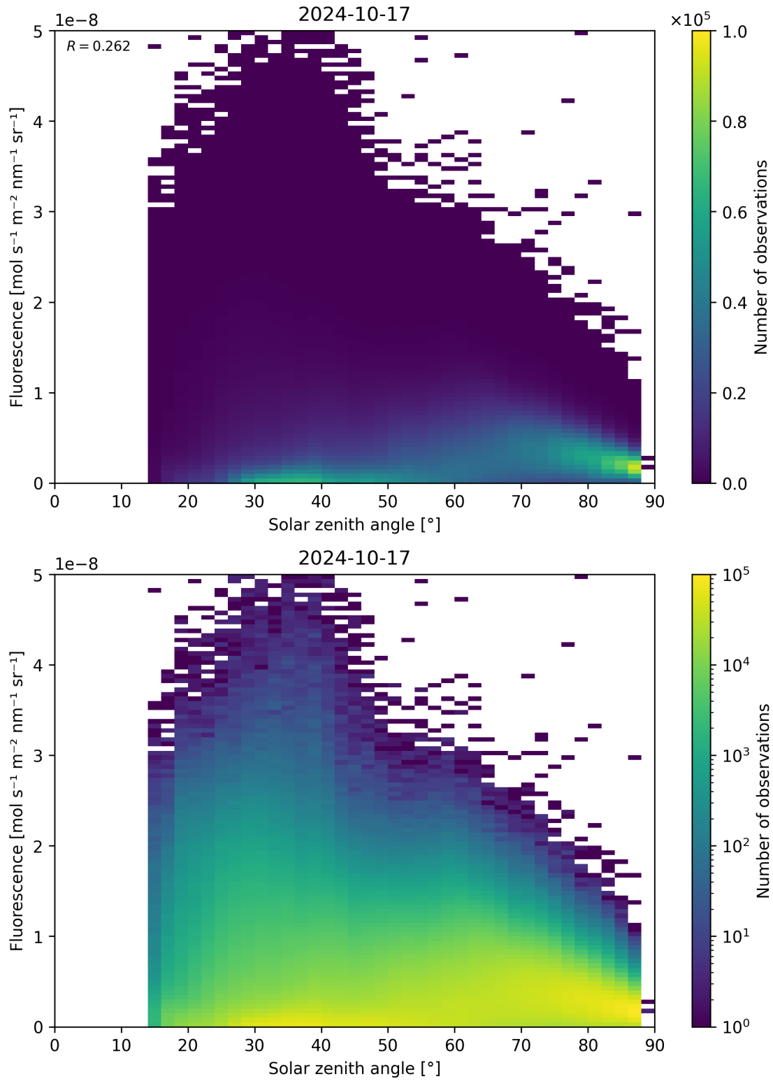
Figure 123: Scatter density plot of “Solar zenith angle” against “Fluorescence” for 2024-10-16 to 2024-10-18.
