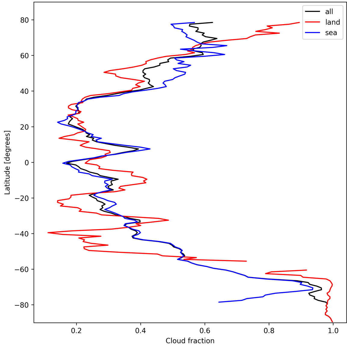
Figure 15: Zonal average of “Cloud fraction” for 2024-10-16 to 2024-10-18.
