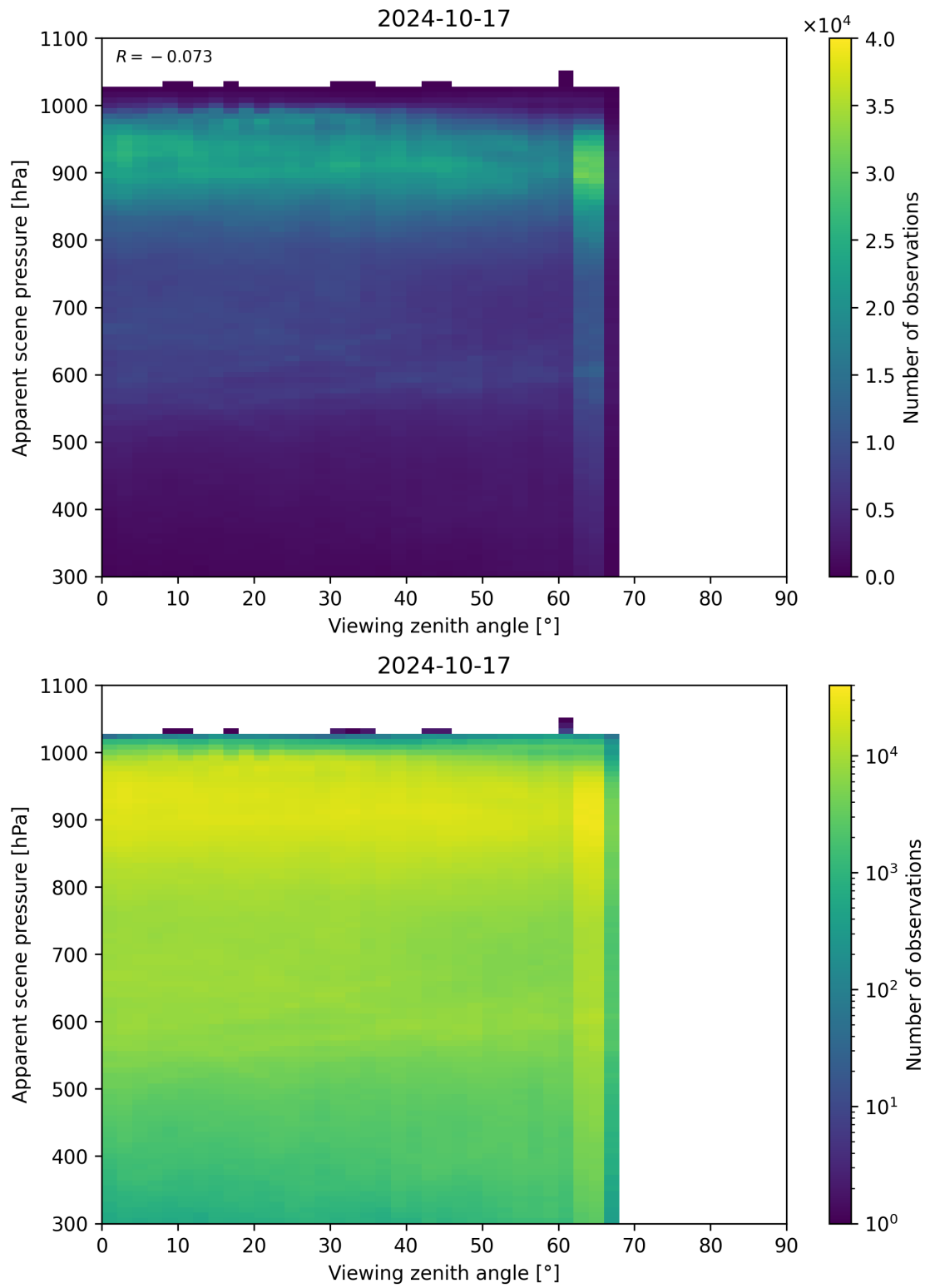
Figure 129: Scatter density plot of “Viewing zenith angle” against “Apparent scene pressure” for 2024-10-16 to 2024-10-18.
