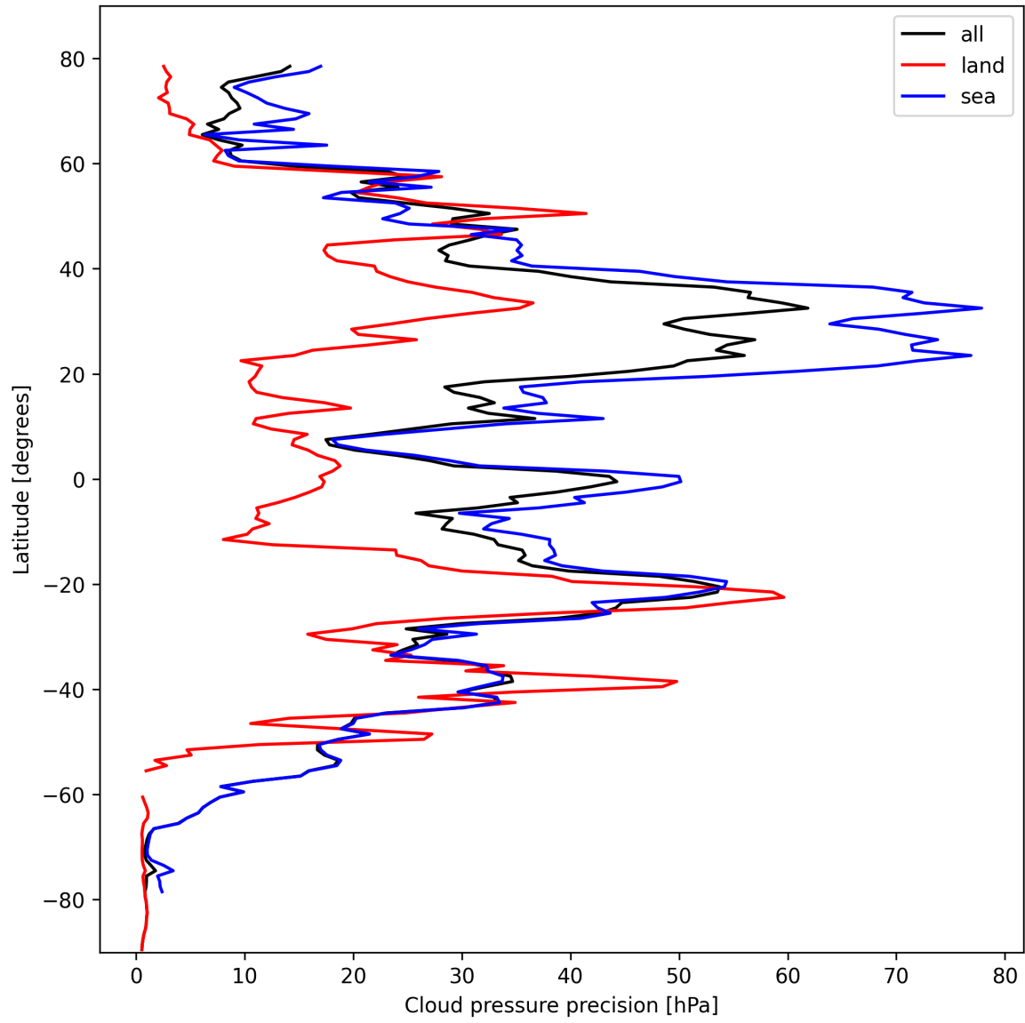
Figure 14: Zonal average of “Cloud pressure precision” for 2024-10-16 to 2024-10-18.
