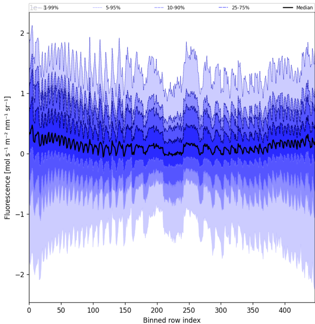
Figure 57: Along track statistics of “Fluorescence” for 2024-10-16 to 2024-10-18
