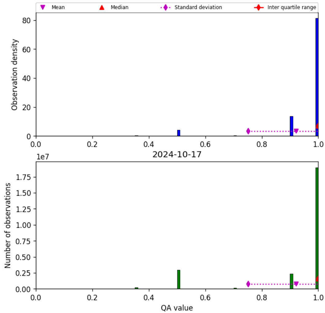
Figure 29: Histogram of “QA value” for 2024-10-16 to 2024-10-18
