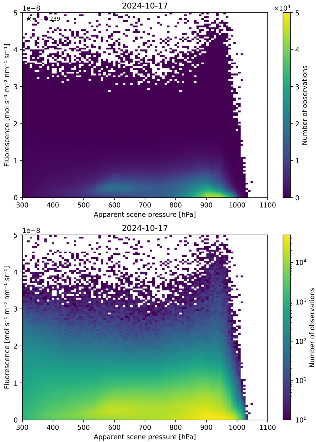
Figure 65: Scatter density plot of “Apparent scene pressure” against “Fluorescence” for 2024-10-16 to 2024-10-18.
