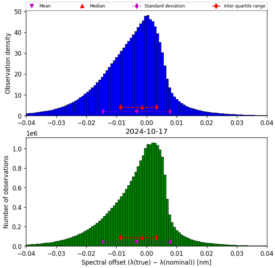
Figure 45: Histogram of “Spectral offset ( \lambda_{\text{true}} - \lambda_{\text{nominal}} )” for 2024-10-16 to 2024-10-18
