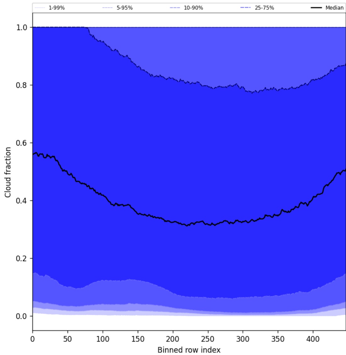
Figure 49: Along track statistics of “Cloud fraction” for 2024-10-16 to 2024-10-18
