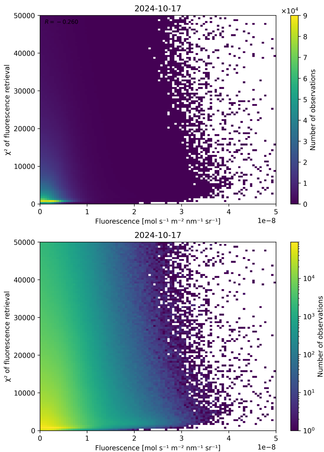
Figure 93: Scatter density plot of “Fluorescence” against “ \chi^2 of fluorescence retrieval” for 2024-10-16 to 2024-10-18.
