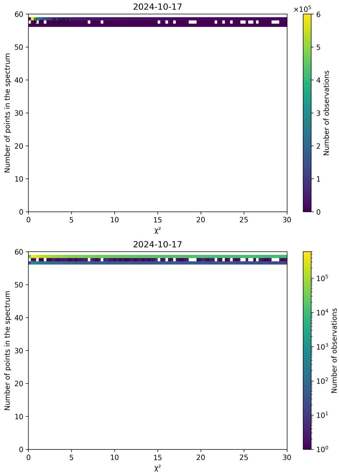
Figure 74: Scatter density plot of " \chi^2 " against "Number of points in the spectrum" for 2024-10-16 to 2024-10-18.
