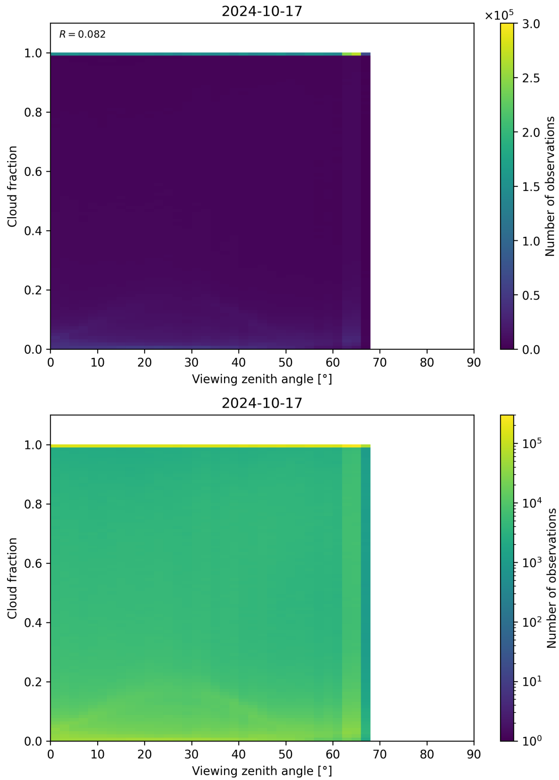
Figure 132: Scatter density plot of “Viewing zenith angle” against “Cloud fraction” for 2024-10-16 to 2024-10-18.
