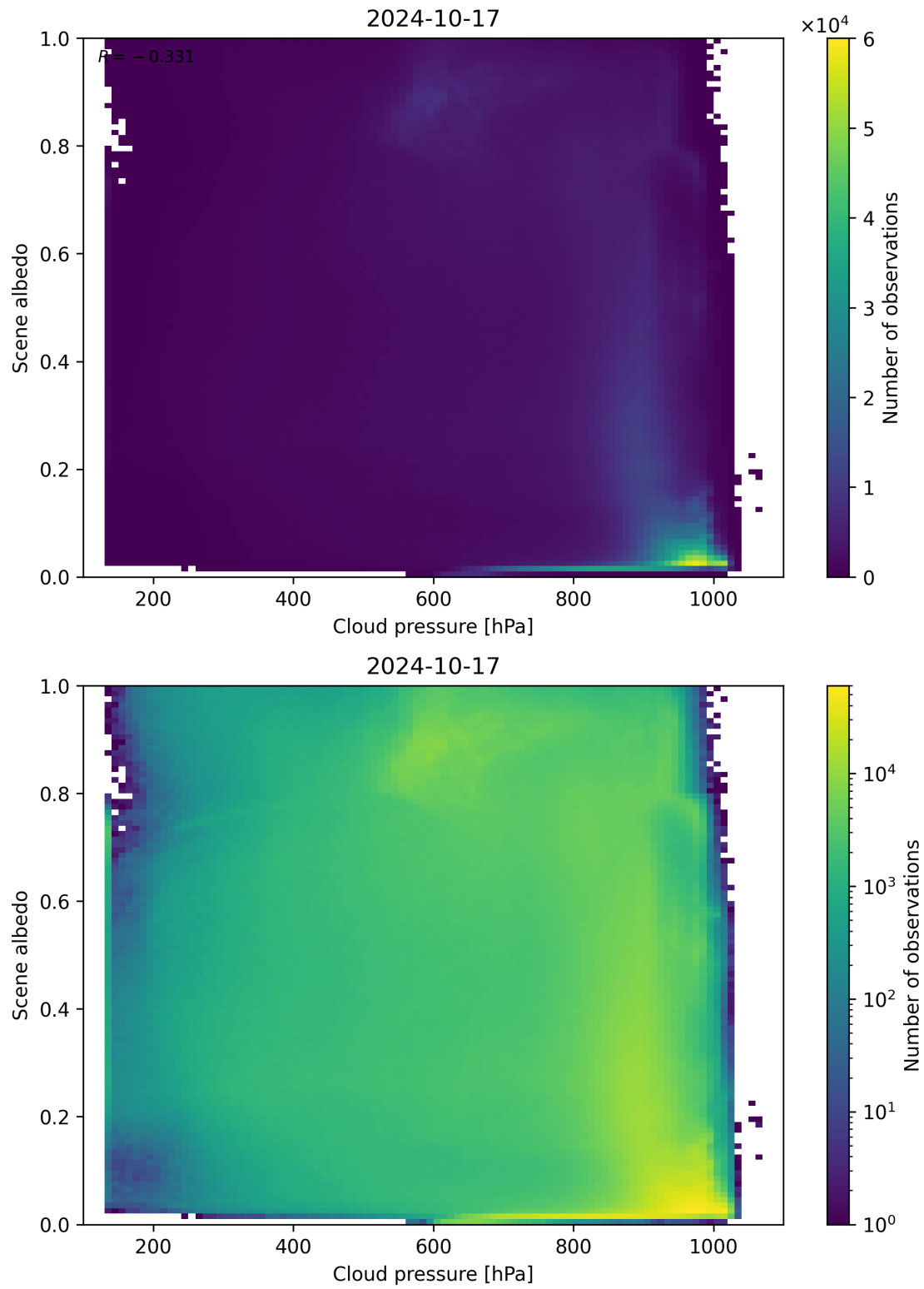
Figure 91: Scatter density plot of “Cloud pressure” against “Scene albedo” for 2024-10-16 to 2024-10-18.
