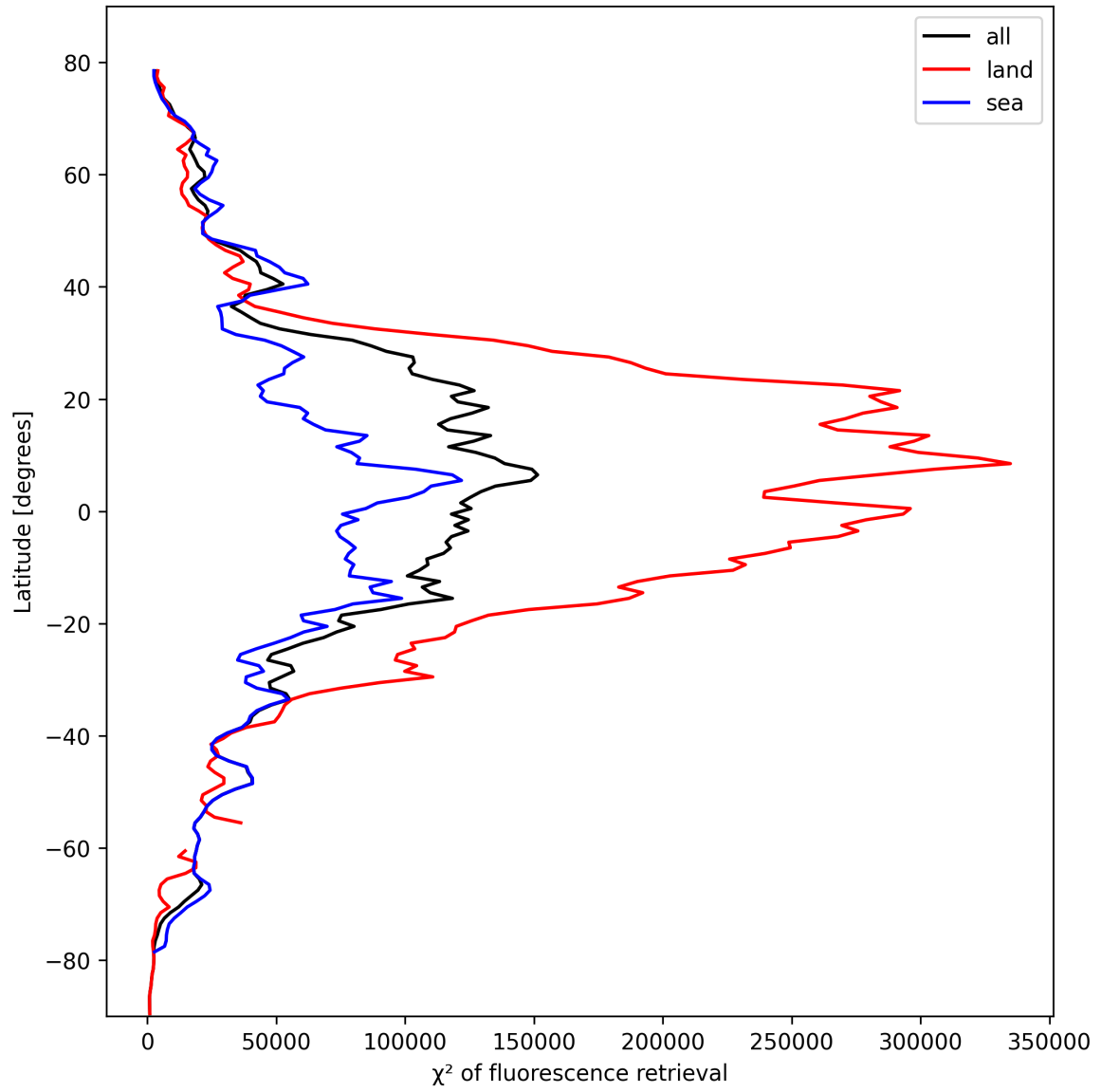
Figure 25: Zonal average of “ \chi^2 of fluorescence retrieval” for 2024-10-16 to 2024-10-18.
