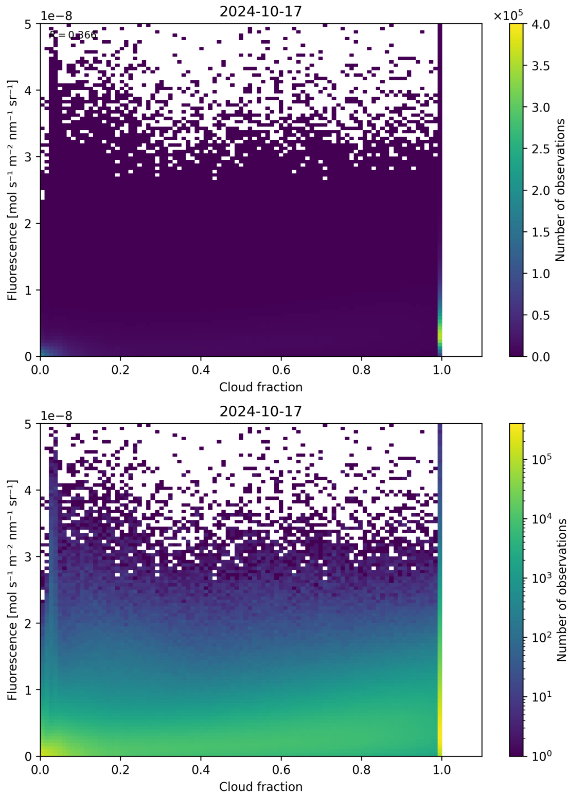
Figure 79: Scatter density plot of “Cloud fraction” against “Fluorescence” for 2024-10-16 to 2024-10-18.
