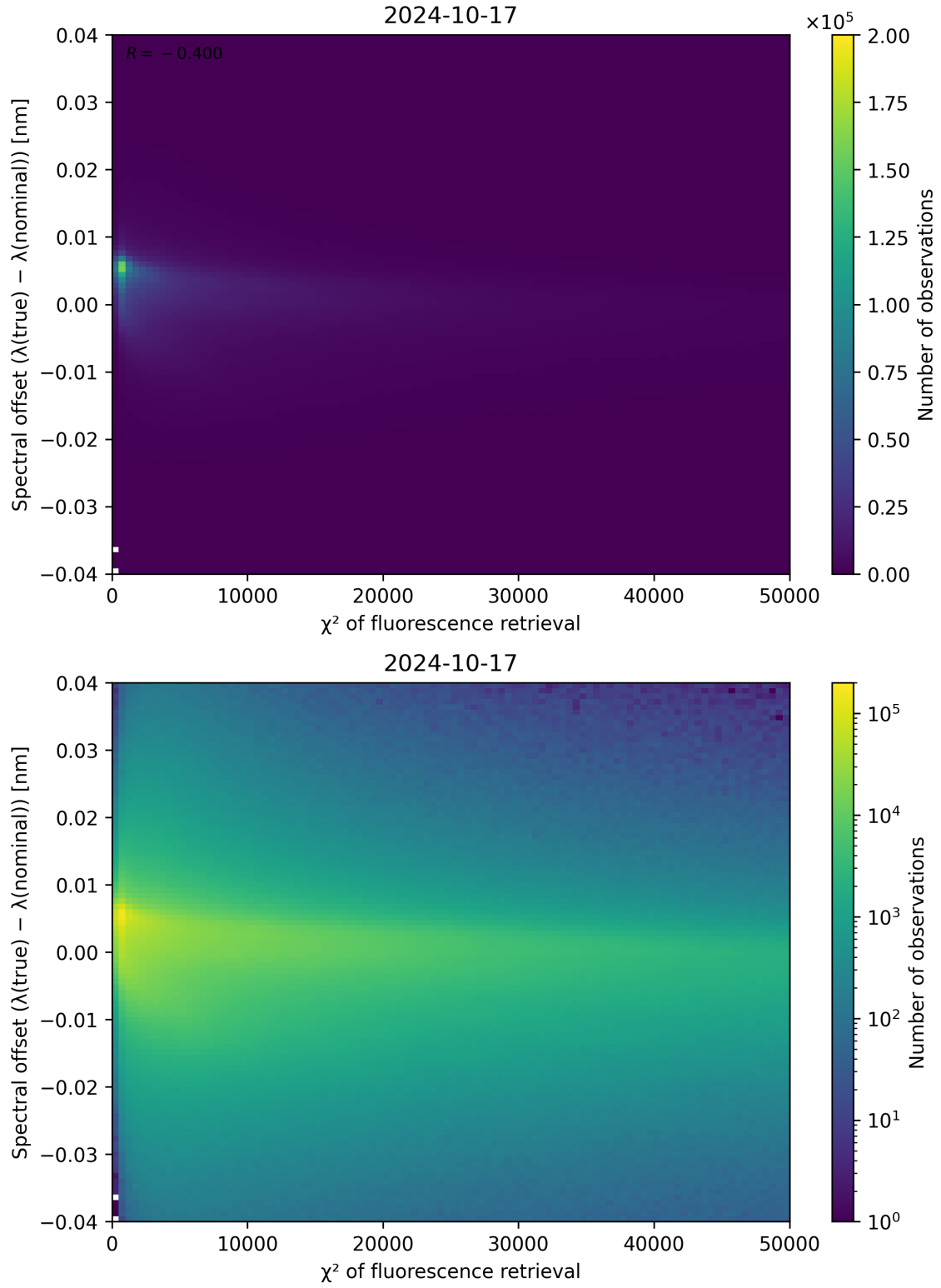
Figure 72: Scatter density plot of “ \chi^2 of fluorescence retrieval” against “Spectral offset ( \lambda_{\text{true}} - \lambda_{\text{nominal}} )” for 2024-10-16 to 2024-10-18.
