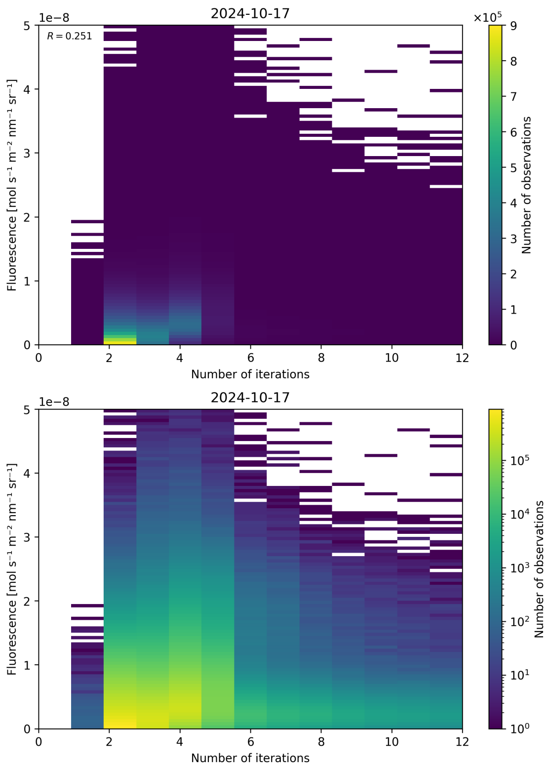
Figure 107: Scatter density plot of “Number of iterations” against “Fluorescence” for 2024-10-16 to 2024-10-18.
