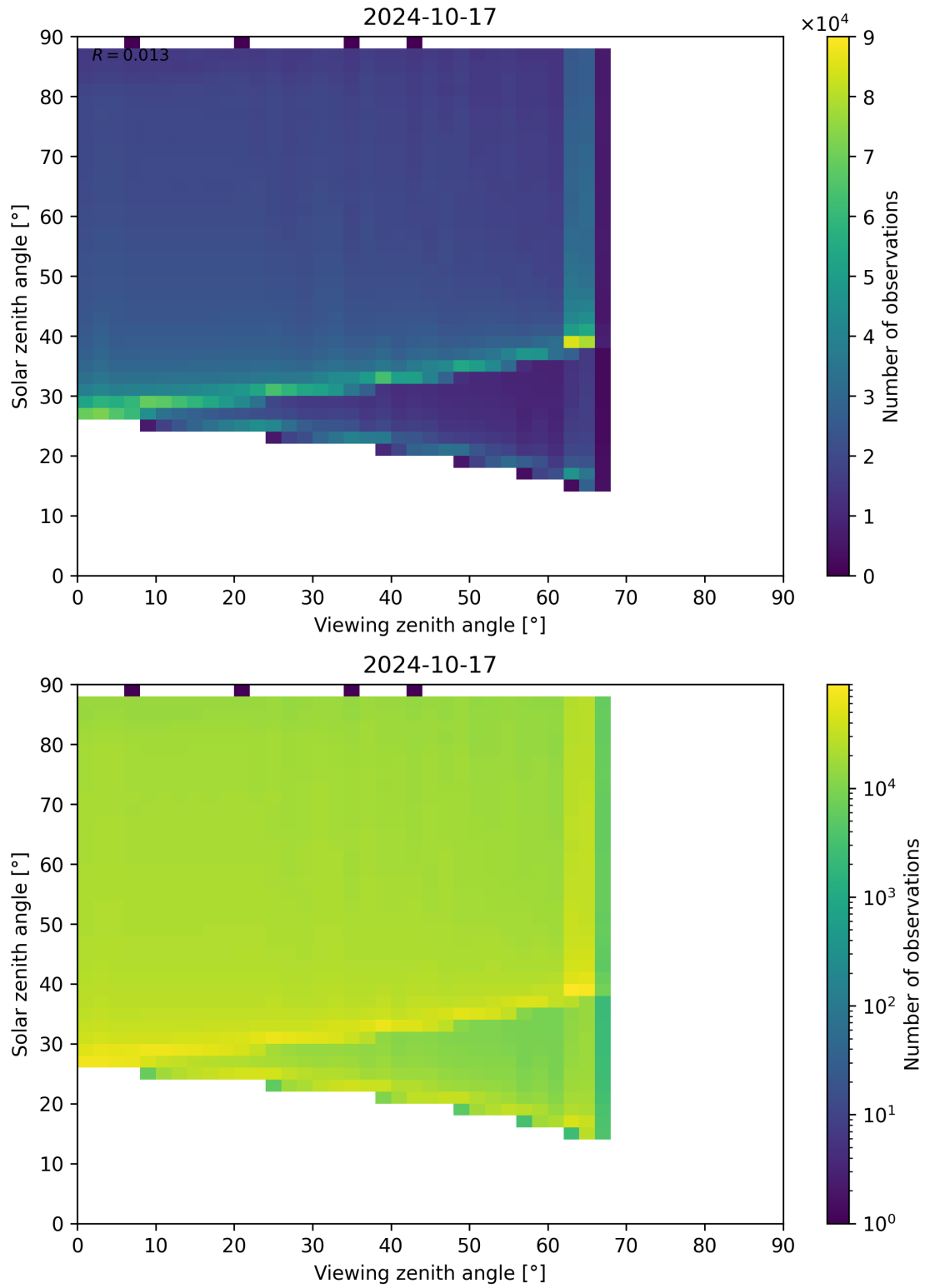
Figure 139: Scatter density plot of “Viewing zenith angle” against “Solar zenith angle” for 2024-10-16 to 2024-10-18.
