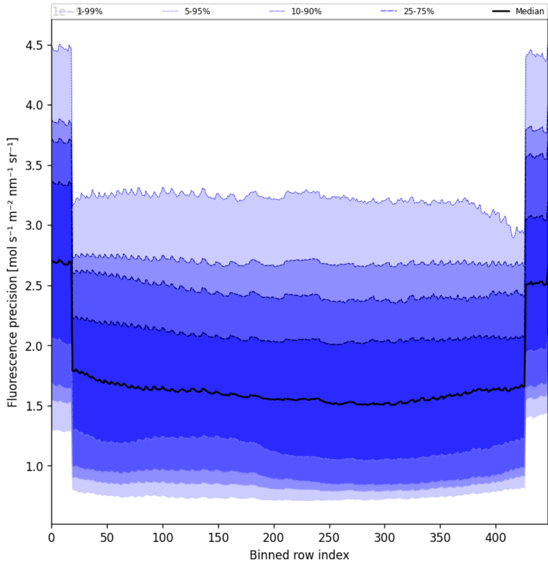
Figure 58: Along track statistics of “Fluorescence precision” for 2024-10-16 to 2024-10-18
