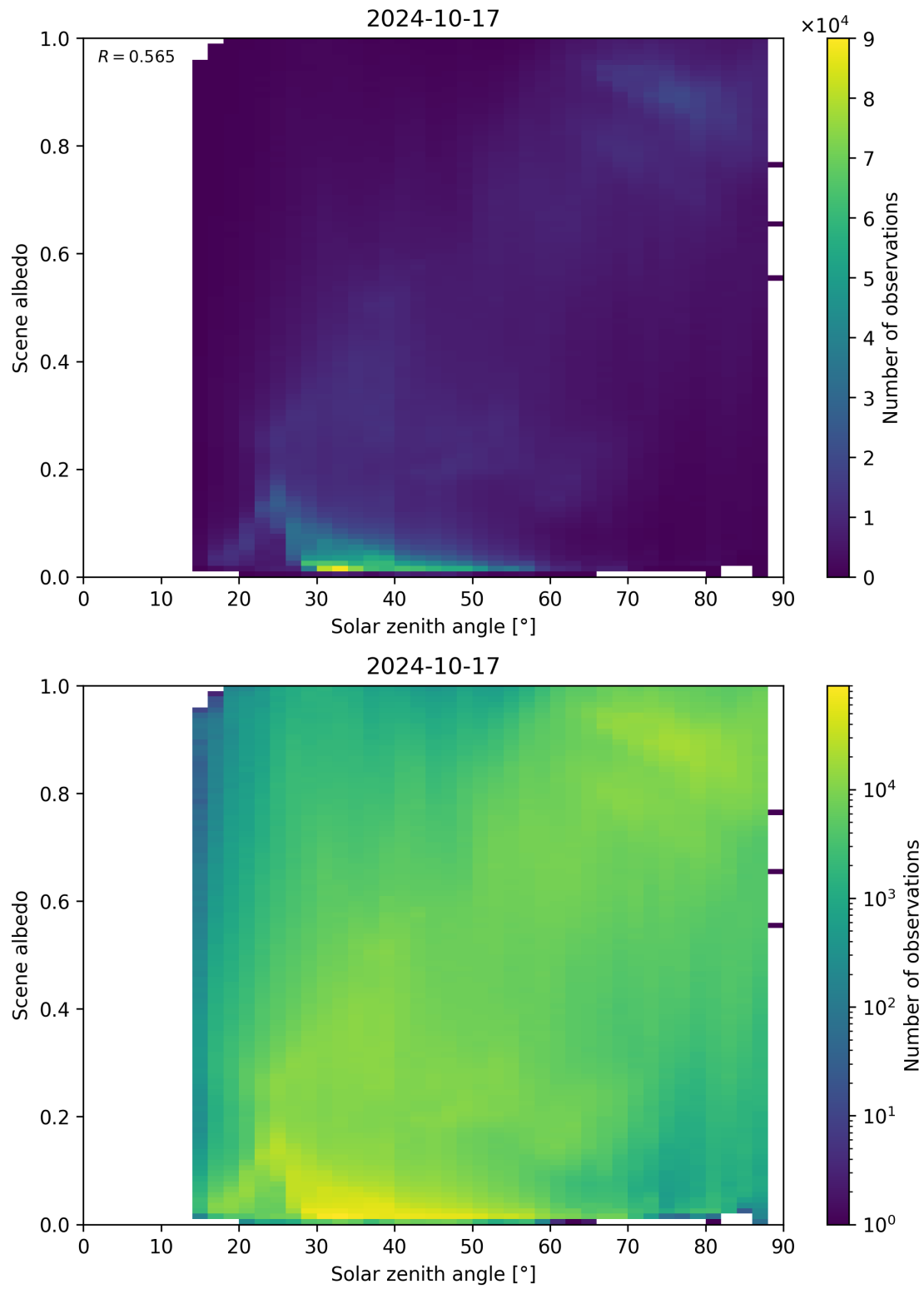
Figure 127: Scatter density plot of “Solar zenith angle” against “Scene albedo” for 2024-10-16 to 2024-10-18.
