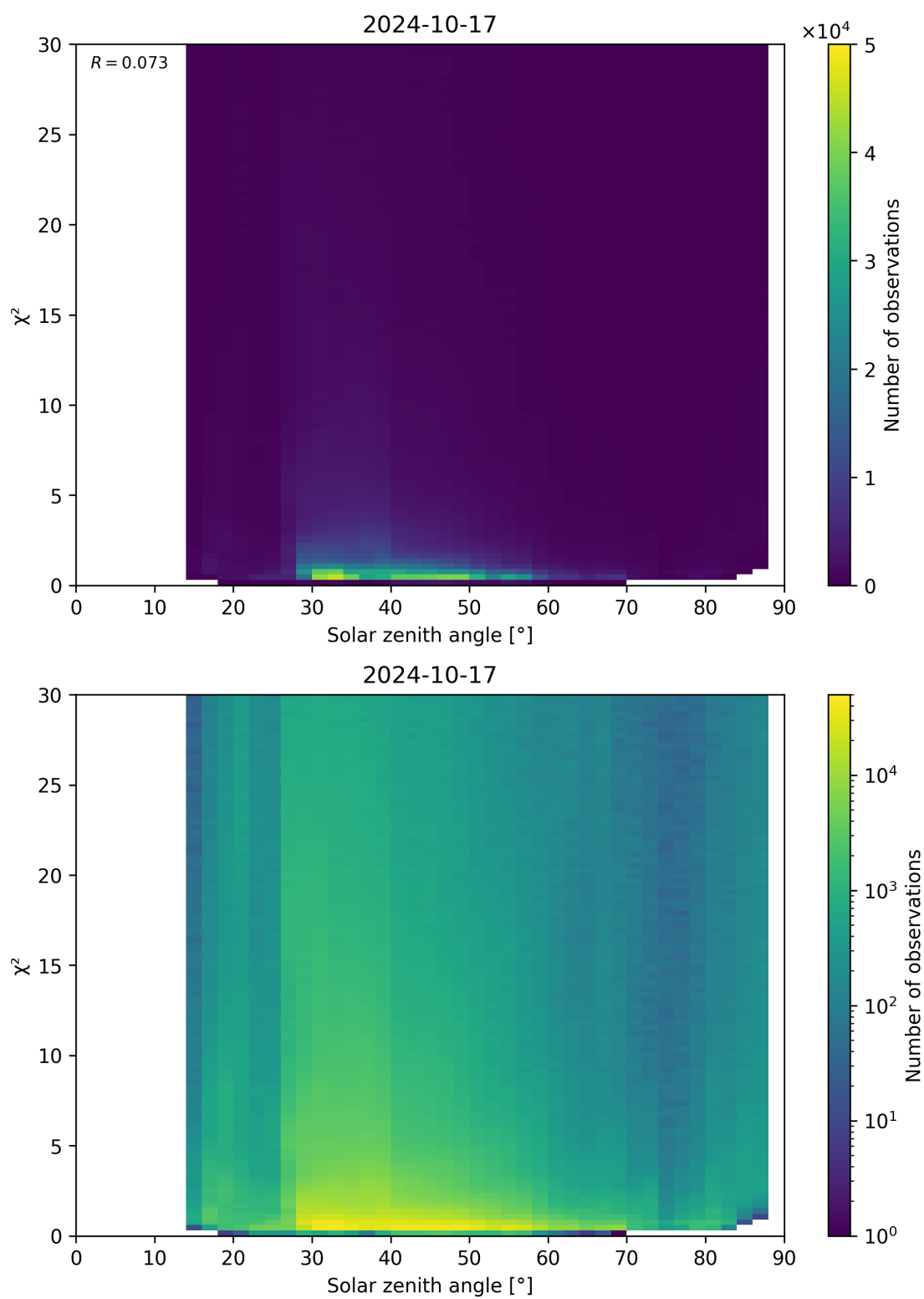
Figure 119: Scatter density plot of “Solar zenith angle” against “ \chi^2 ” for 2024-10-16 to 2024-10-18.
