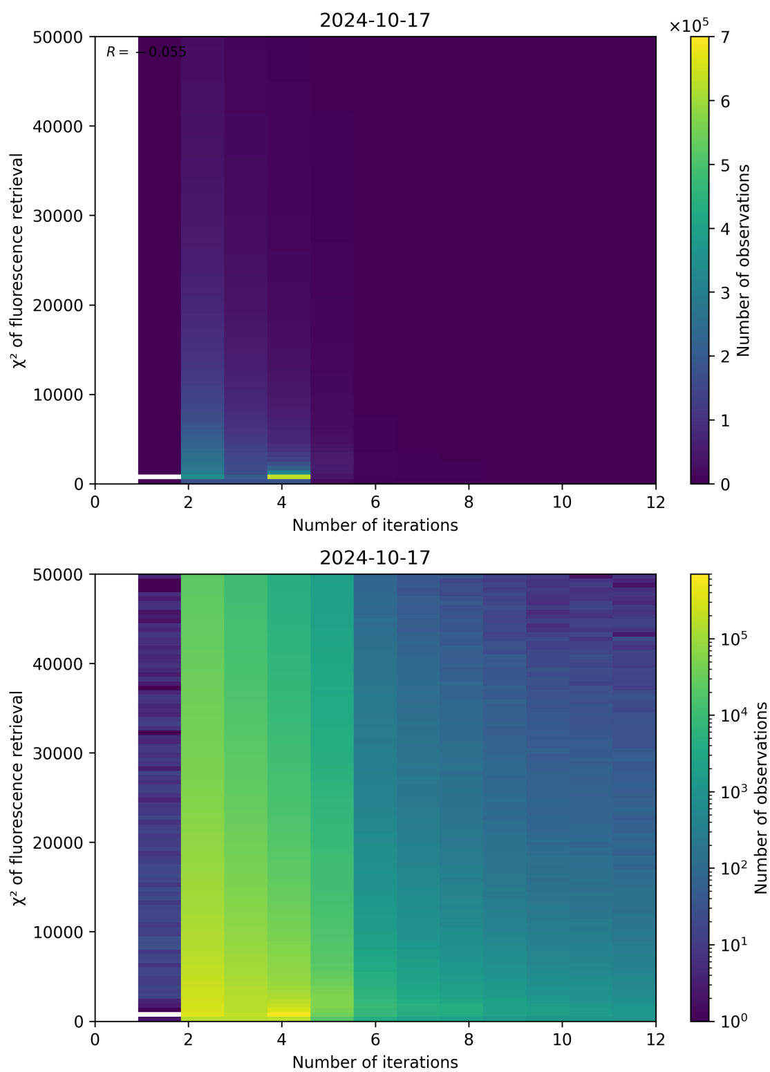
Figure 106: Scatter density plot of “Number of iterations” against “ \chi^2 of fluorescence retrieval” for 2024-10-16 to 2024-10-18.
