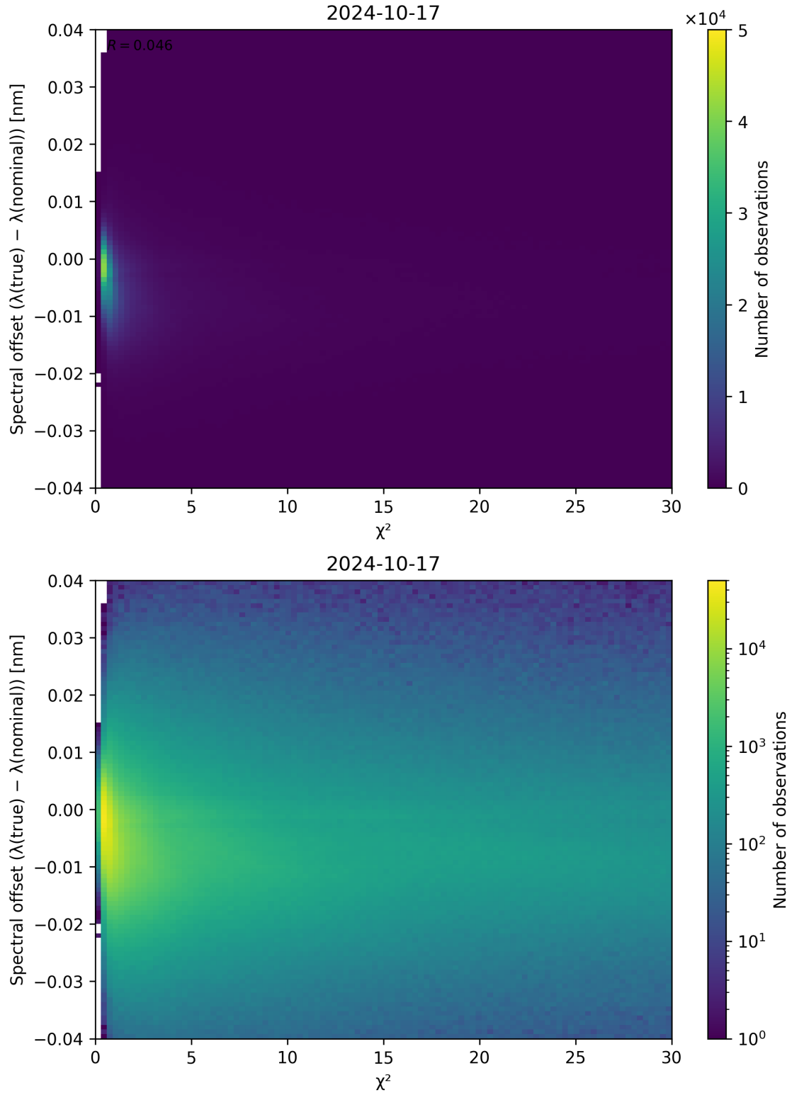
Figure 75: Scatter density plot of “ \chi^2 ” against “Spectral offset ( \lambda_{\text{true}} - \lambda_{\text{nominal}} )” for 2024-10-16 to 2024-10-18.
