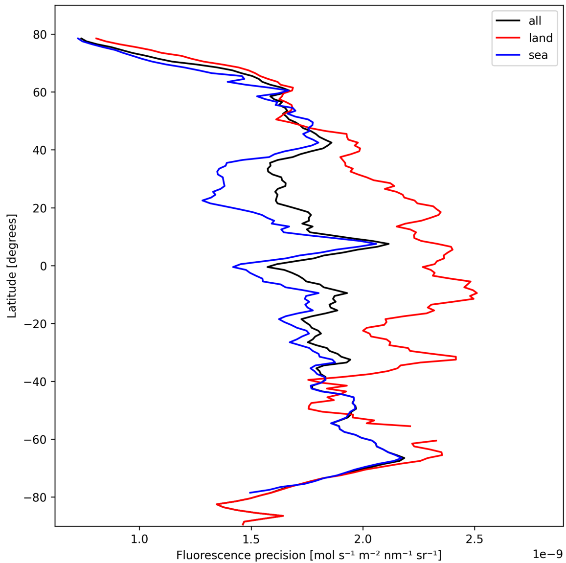
Figure 24: Zonal average of “Fluorescence precision” for 2024-10-16 to 2024-10-18.
