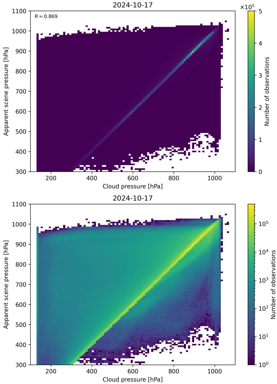
Figure 84: Scatter density plot of “Cloud pressure” against “Apparent scene pressure” for 2024-10-16 to 2024-10-18.
