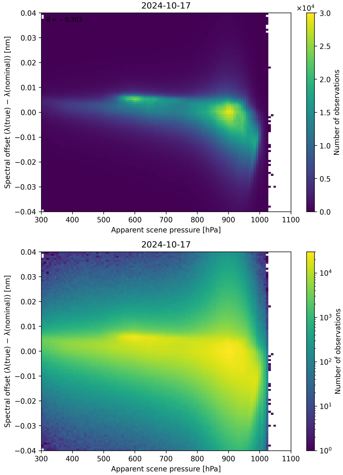
Figure 68: Scatter density plot of “Apparent scene pressure” against “Spectral offset ( \lambda_{\text{true}} - \lambda_{\text{nominal}} )” for 2024-10-16 to 2024-10-18.
