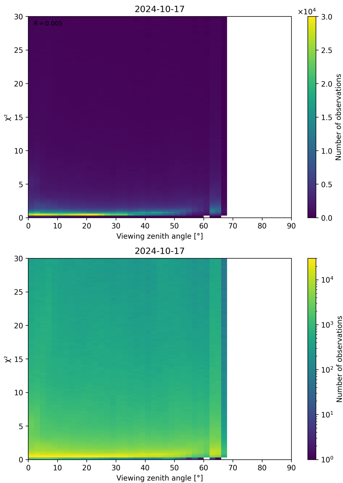
Figure 130: Scatter density plot of “Viewing zenith angle” against “ \chi^2 ” for 2024-10-16 to 2024-10-18.
