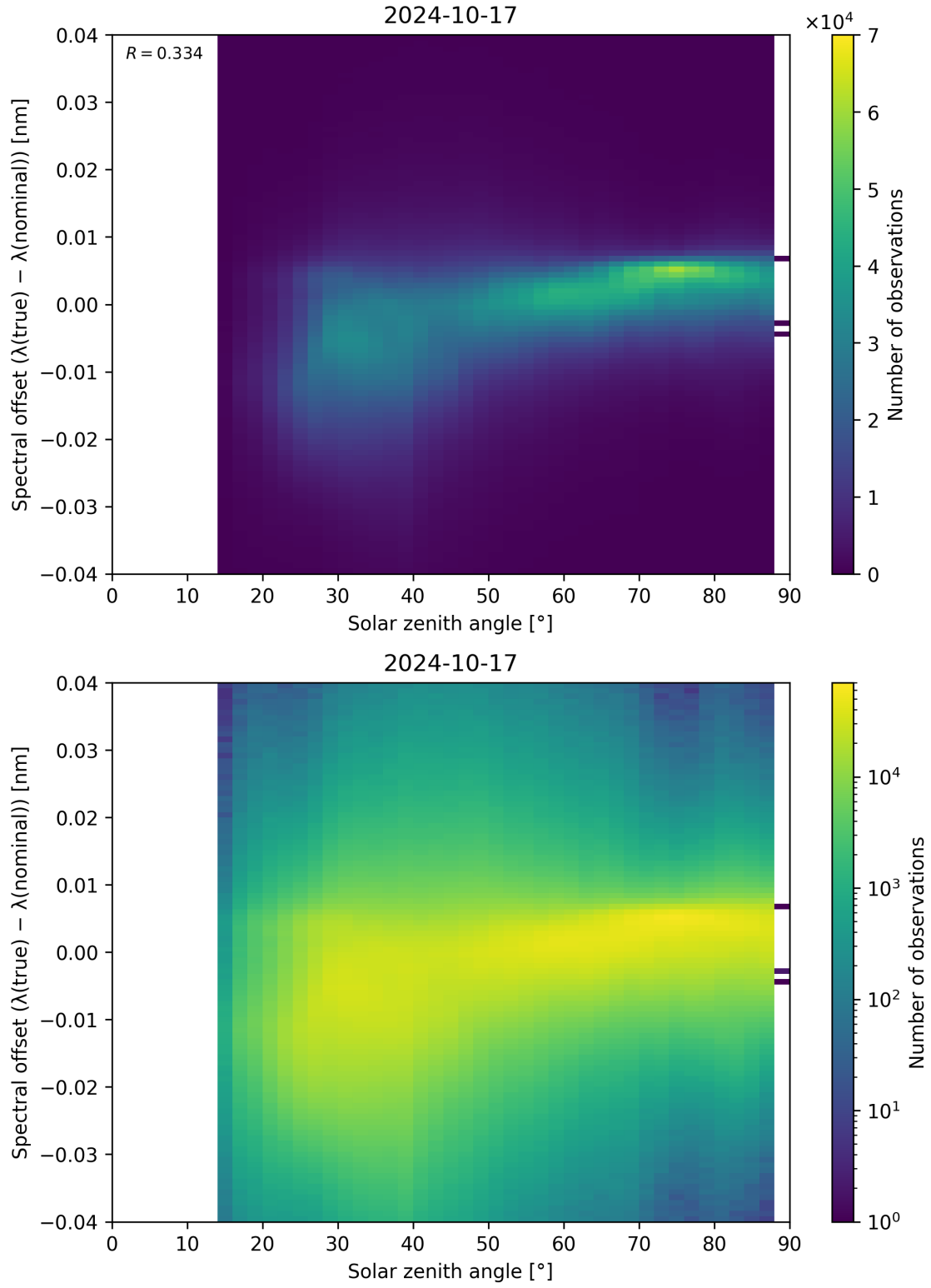
Figure 128: Scatter density plot of “Solar zenith angle” against “Spectral offset ( \lambda_{\text{true}} - \lambda_{\text{nominal}} )” for 2024-10-16 to 2024-10-18.
