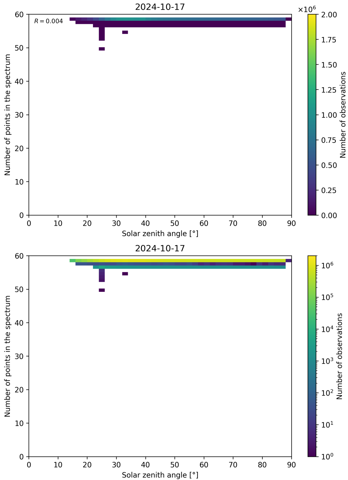
Figure 126: Scatter density plot of “Solar zenith angle” against “Number of points in the spectrum” for 2024-10-16 to 2024-10-18.
