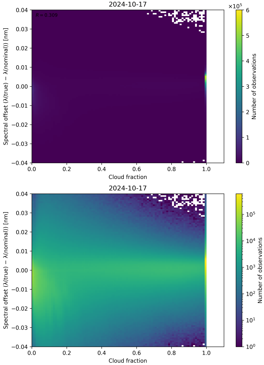
Figure 83: Scatter density plot of “Cloud fraction” against “Spectral offset ( \lambda_{\text{true}} - \lambda_{\text{nominal}} )” for 2024-10-16 to 2024-10-18.
