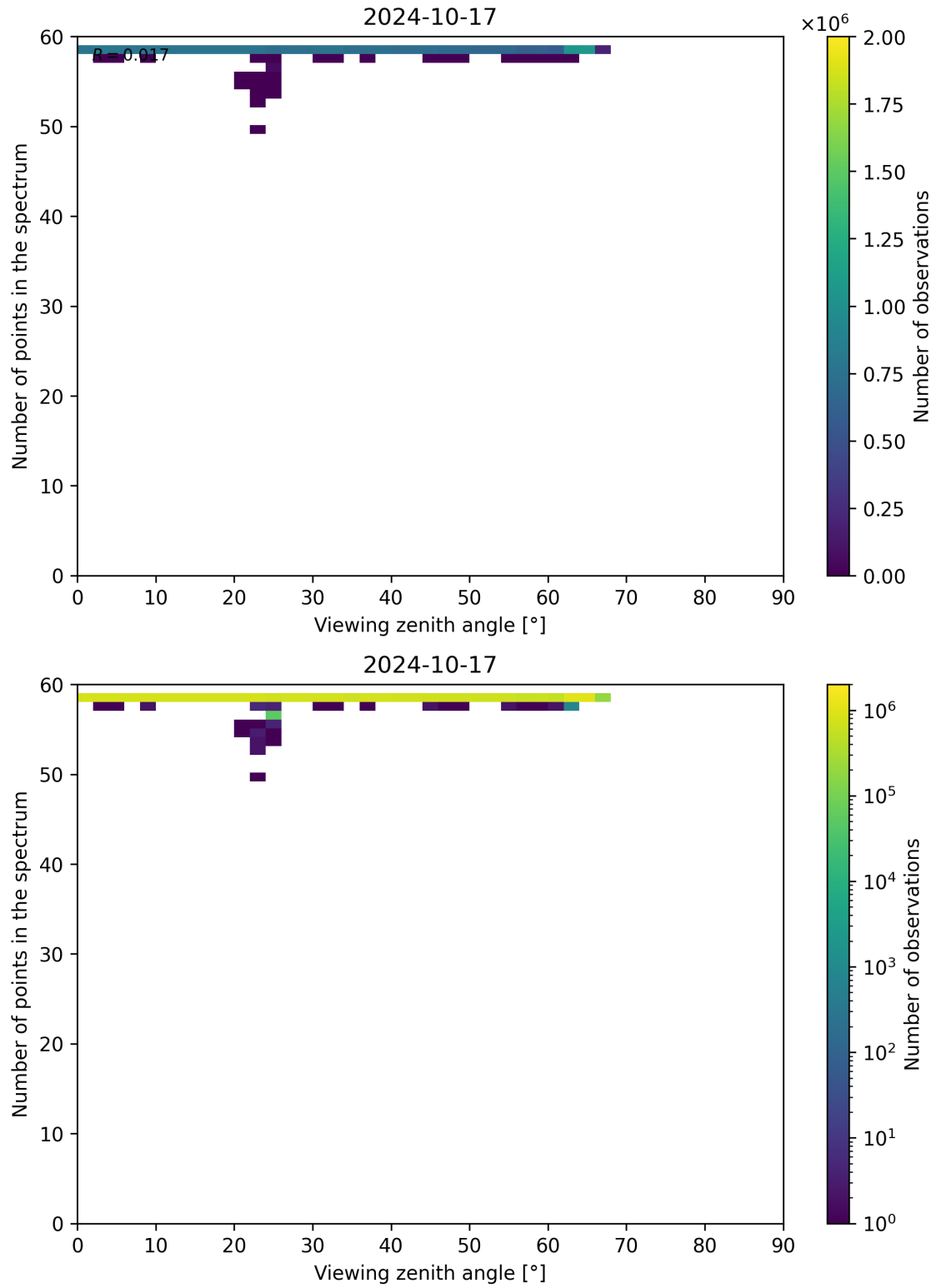
Figure 137: Scatter density plot of “Viewing zenith angle” against “Number of points in the spectrum” for 2024-10-16 to 2024-10-18.
