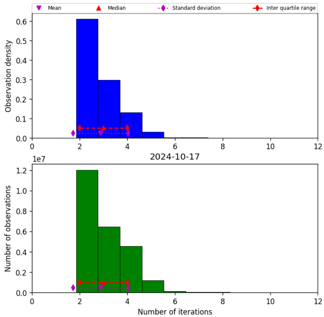
Figure 39: Histogram of “Number of iterations” for 2024-10-16 to 2024-10-18
