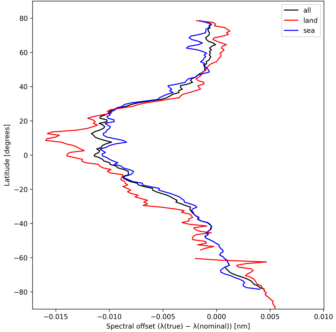
Figure 28: Zonal average of “Spectral offset ( \lambda_{\text{true}} - \lambda_{\text{nominal}} )” for 2024-10-16 to 2024-10-18.
