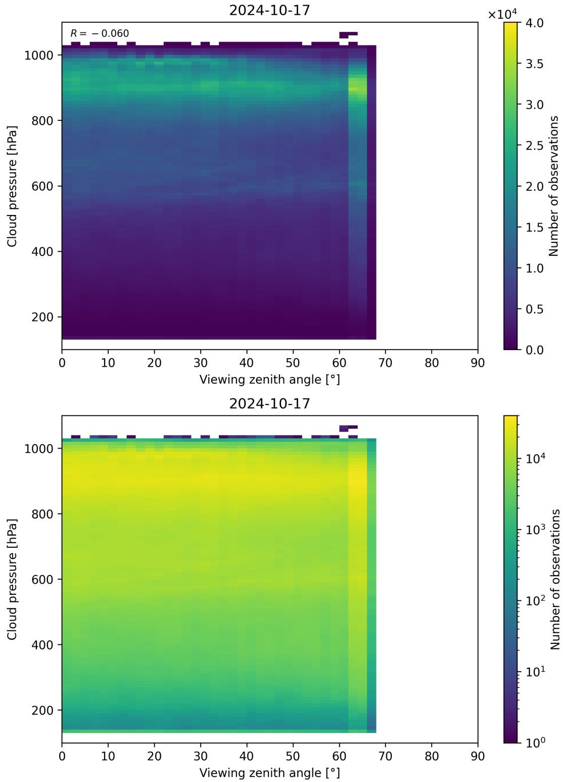
Figure 133: Scatter density plot of “Viewing zenith angle” against “Cloud pressure” for 2024-10-16 to 2024-10-18.
