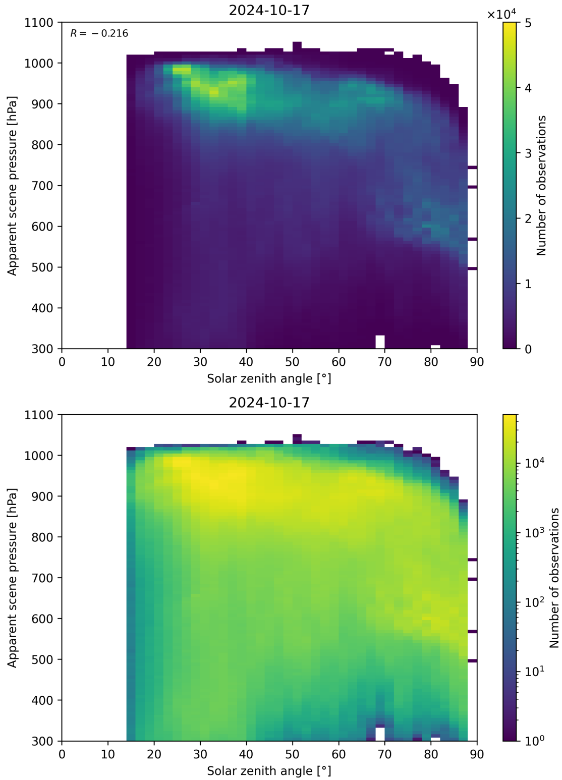
Figure 118: Scatter density plot of “Solar zenith angle” against “Apparent scene pressure” for 2024-10-16 to 2024-10-18.
