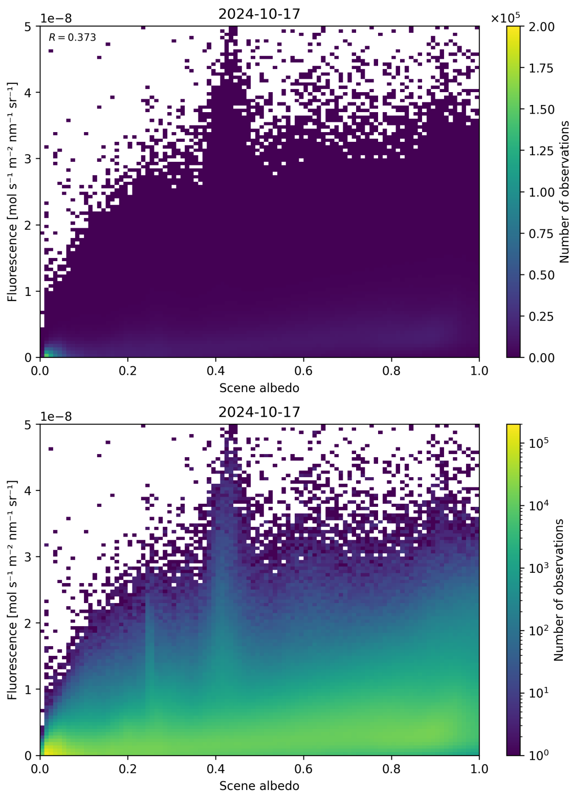
Figure 114: Scatter density plot of “Scene albedo” against “Fluorescence” for 2024-10-16 to 2024-10-18.
