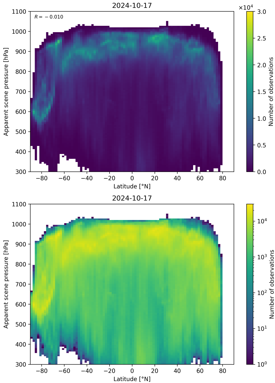
Figure 96: Scatter density plot of “Latitude” against “Apparent scene pressure” for 2024-10-16 to 2024-10-18.
