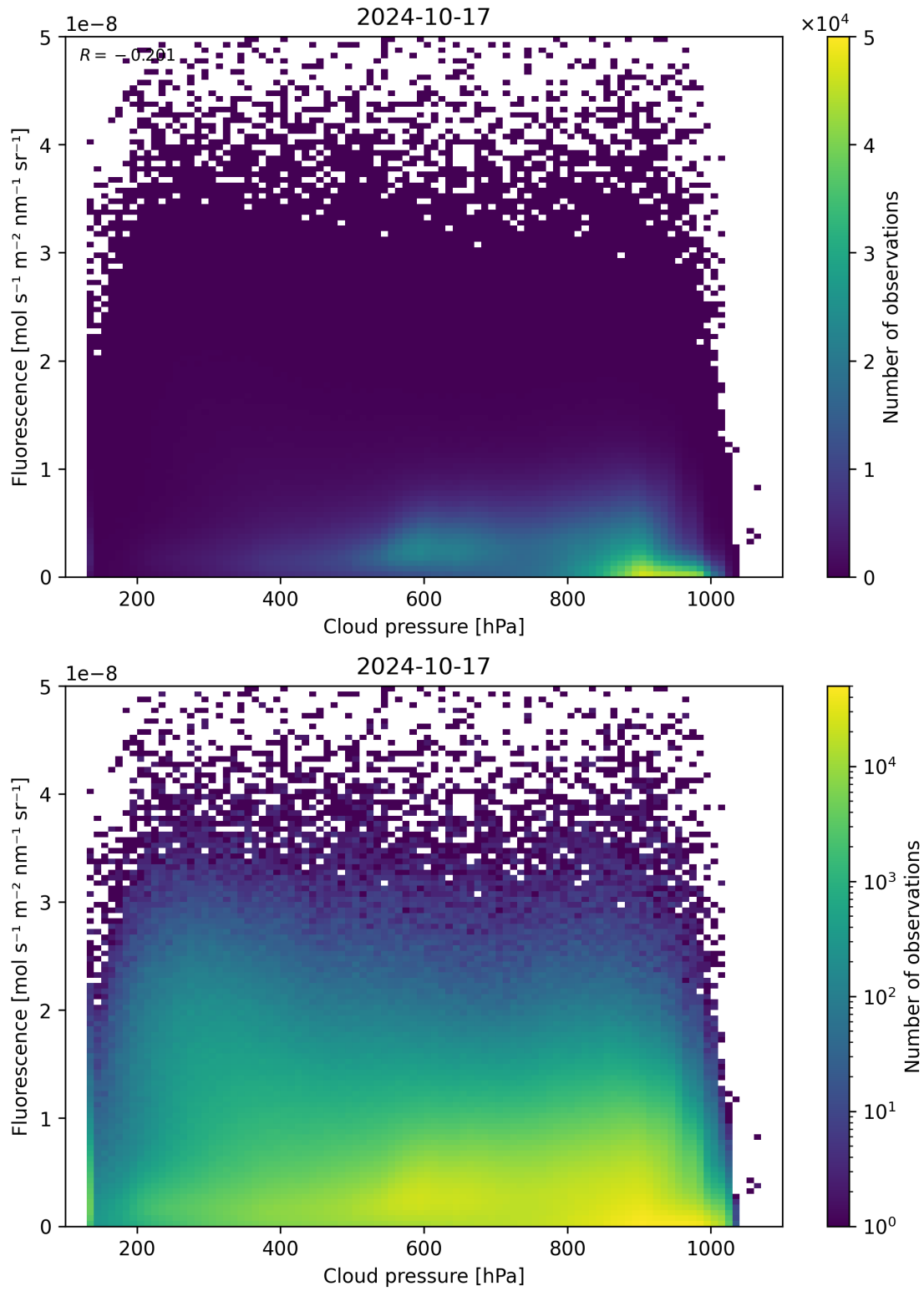
Figure 88: Scatter density plot of “Cloud pressure” against “Fluorescence” for 2024-10-16 to 2024-10-18.
