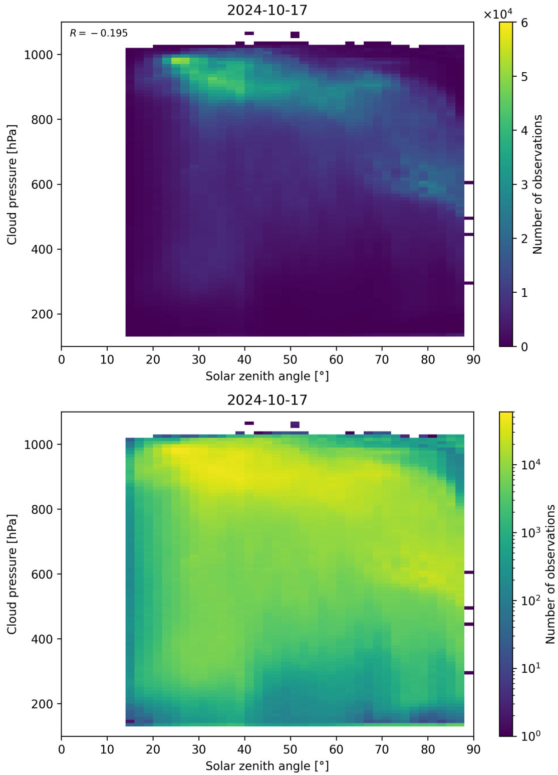
Figure 122: Scatter density plot of “Solar zenith angle” against “Cloud pressure” for 2024-10-16 to 2024-10-18.
