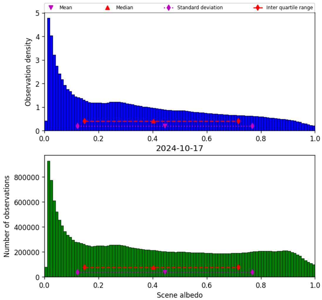
Figure 34: Histogram of “Scene albedo” for 2024-10-16 to 2024-10-18
