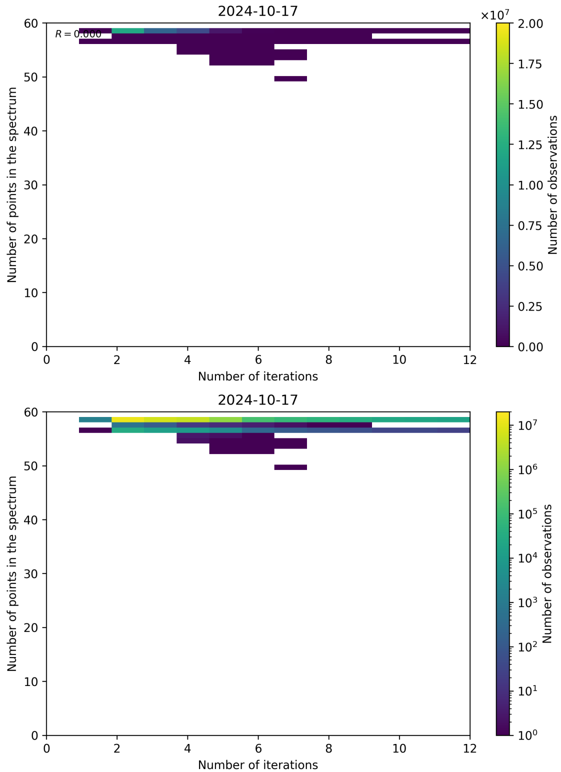
Figure 108: Scatter density plot of “Number of iterations” against “Number of points in the spectrum” for 2024-10-16 to 2024-10-18.
