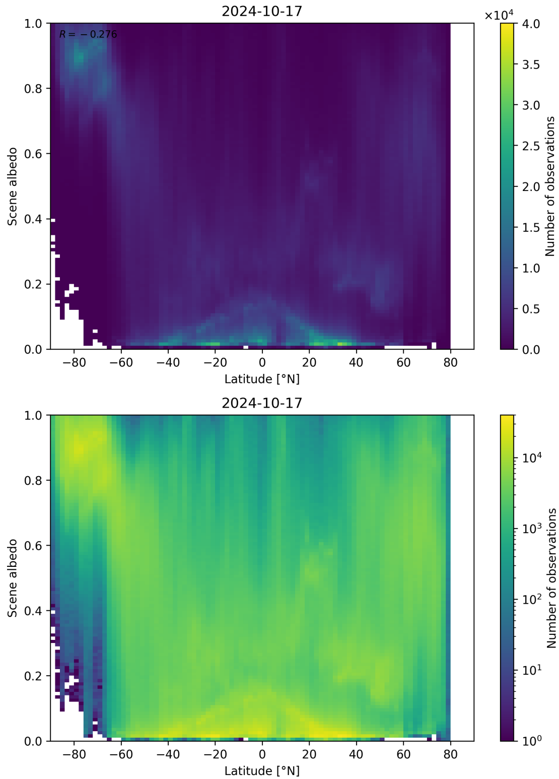
Figure 104: Scatter density plot of “Latitude” against “Scene albedo” for 2024-10-16 to 2024-10-18.
