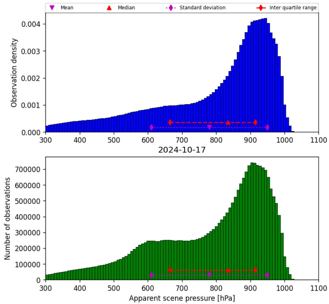
Figure 36: Histogram of “Apparent scene pressure” for 2024-10-16 to 2024-10-18
