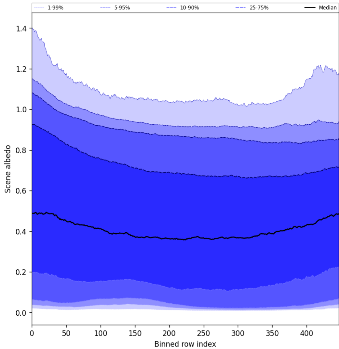
Figure 51: Along track statistics of “Scene albedo” for 2024-10-16 to 2024-10-18
