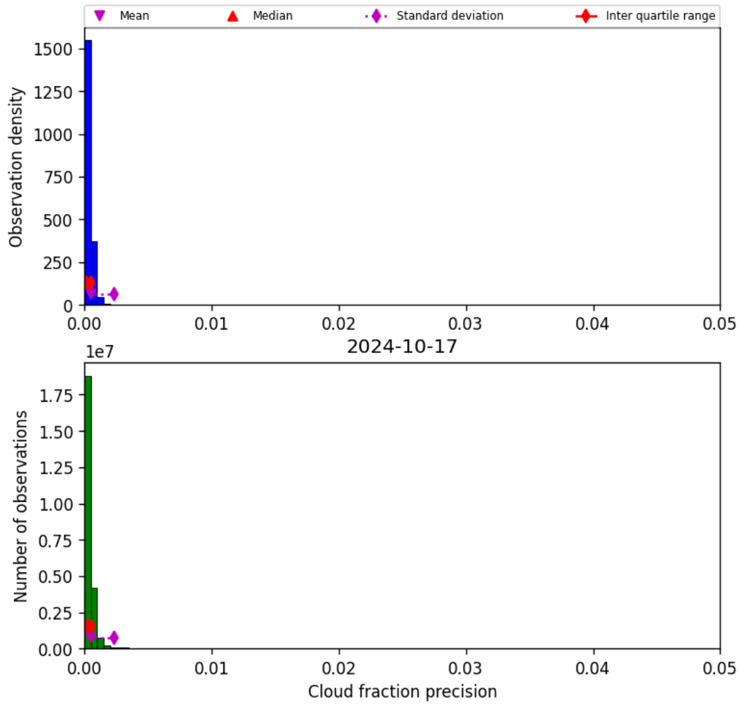
Figure 33: Histogram of “Cloud fraction precision” for 2024-10-16 to 2024-10-18
