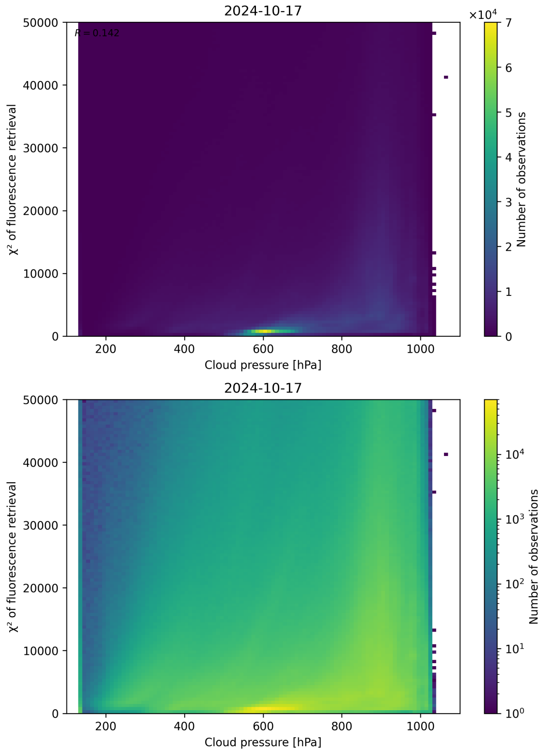
Figure 86: Scatter density plot of “Cloud pressure” against “ \chi^2 of fluorescence retrieval” for 2024-10-16 to 2024-10-18.
