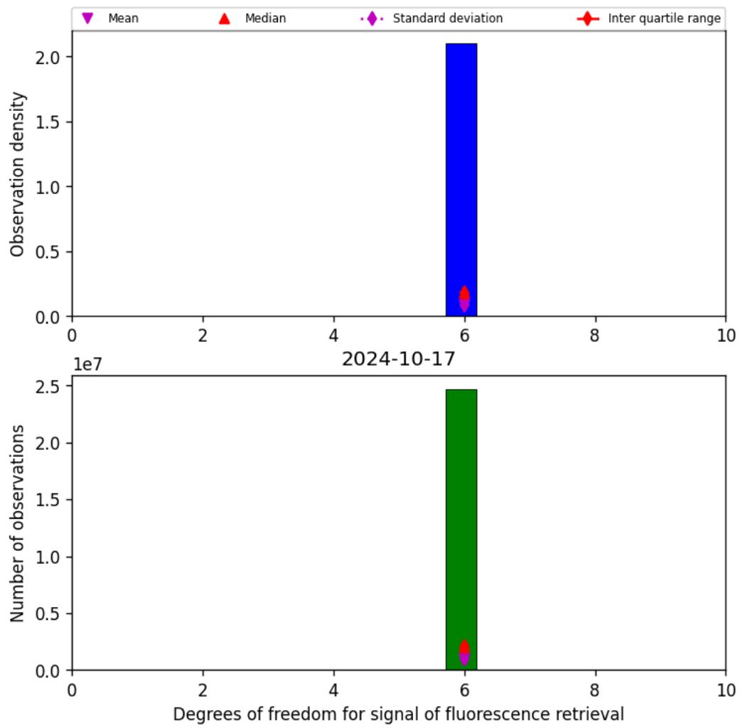
Figure 43: Histogram of “Degrees of freedom for signal of fluorescence retrieval” for 2024-10-16 to 2024-10-18
