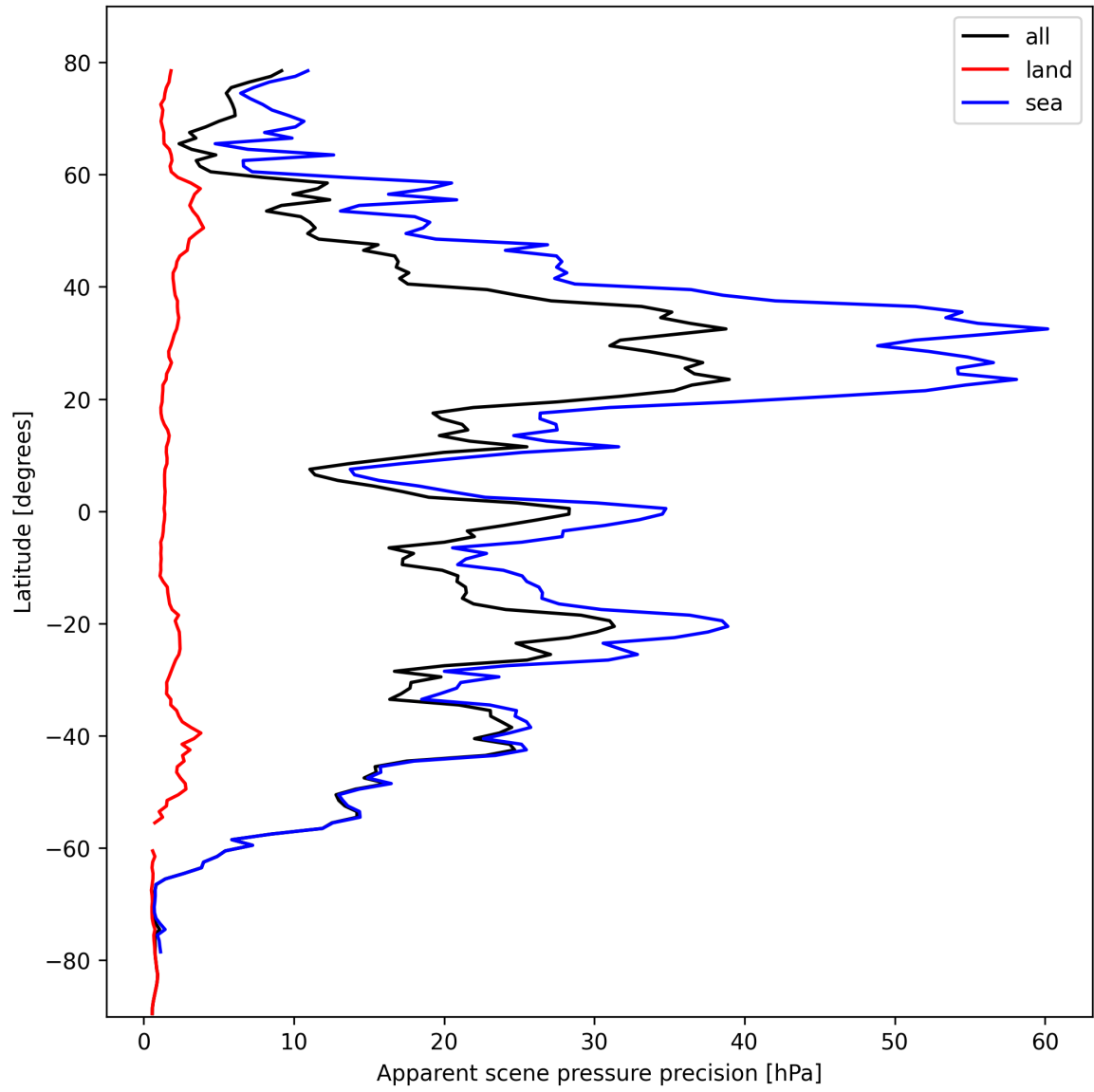
Figure 20: Zonal average of “Apparent scene pressure precision” for 2024-10-16 to 2024-10-18.
