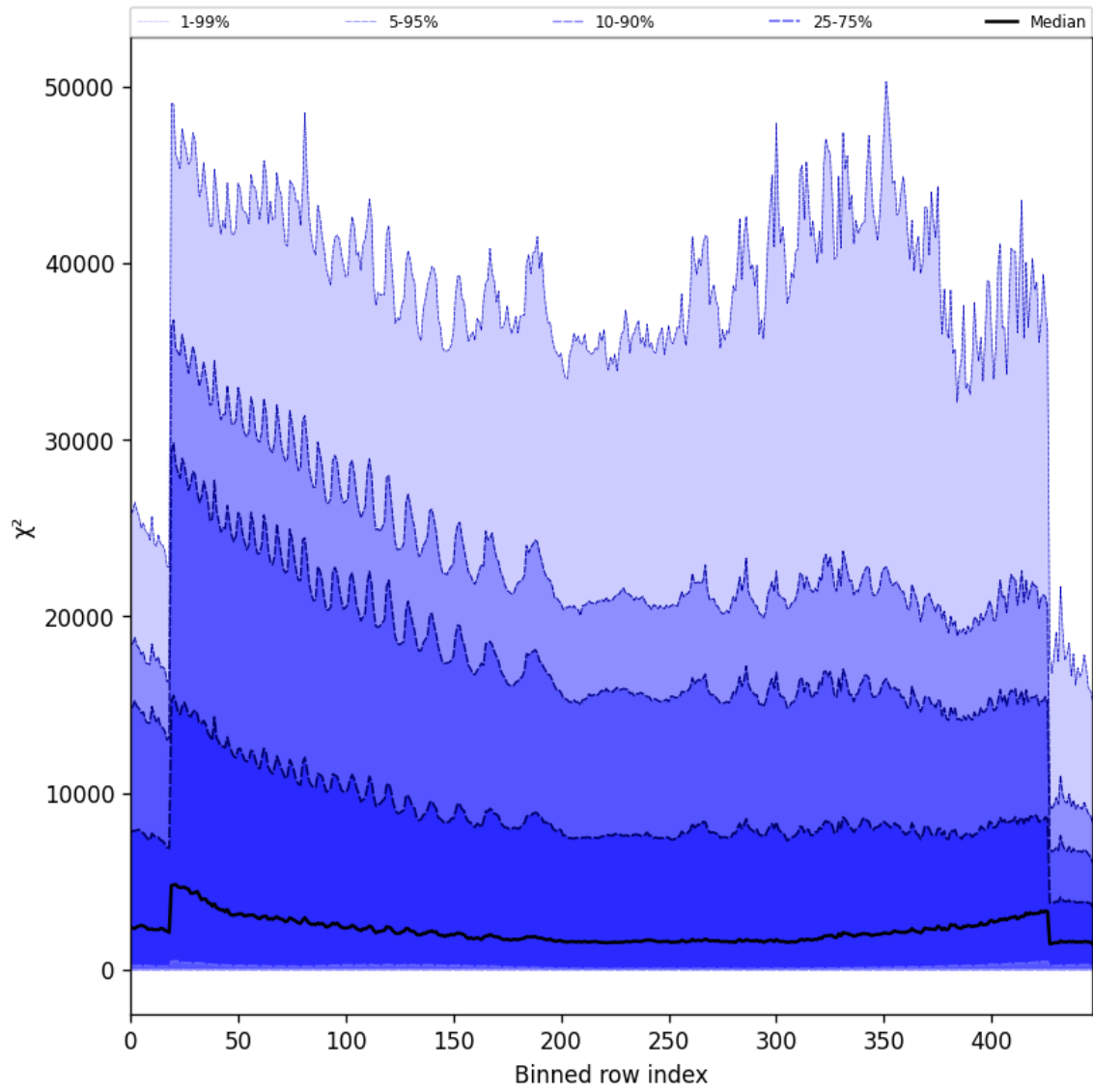
Figure 55: Along track statistics of “ \chi^2 ” for 2024-10-16 to 2024-10-18
