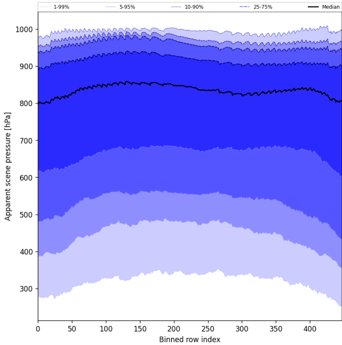
Figure 53: Along track statistics of “Apparent scene pressure” for 2024-10-16 to 2024-10-18
