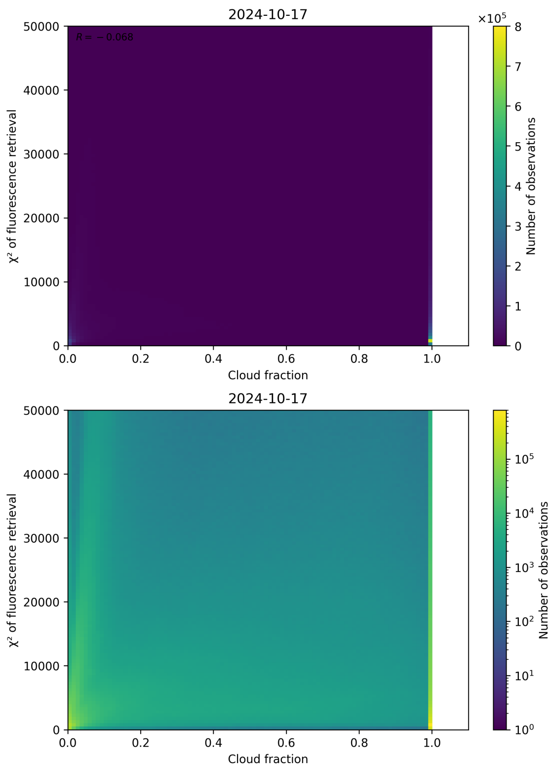
Figure 78: Scatter density plot of “Cloud fraction” against “ \chi^2 of fluorescence retrieval” for 2024-10-16 to 2024-10-18.
