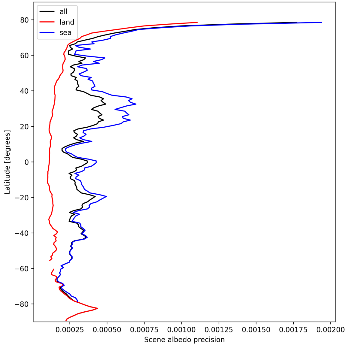
Figure 18: Zonal average of “Scene albedo precision” for 2024-10-16 to 2024-10-18.
