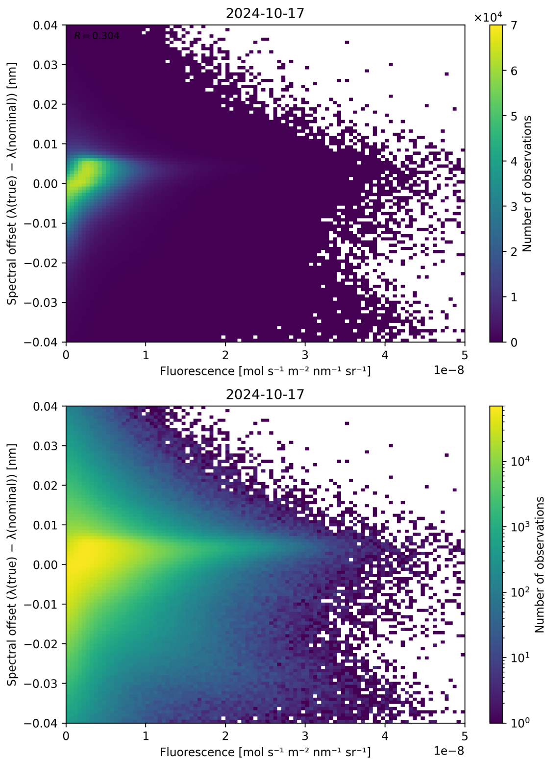
Figure 95: Scatter density plot of “Fluorescence” against “Spectral offset ( \lambda_{\text{true}} - \lambda_{\text{nominal}} )” for 2024-10-16 to 2024-10-18.
