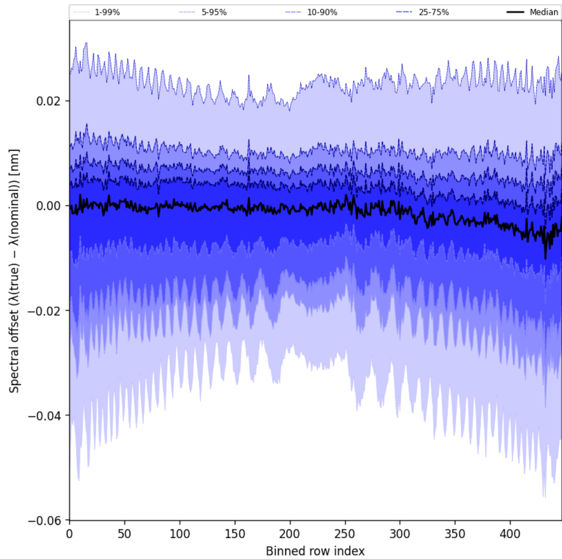
Figure 62: Along track statistics of “Spectral offset ( \lambda_{\text{true}} - \lambda_{\text{nominal}} )” for 2024-10-16 to 2024-10-18
