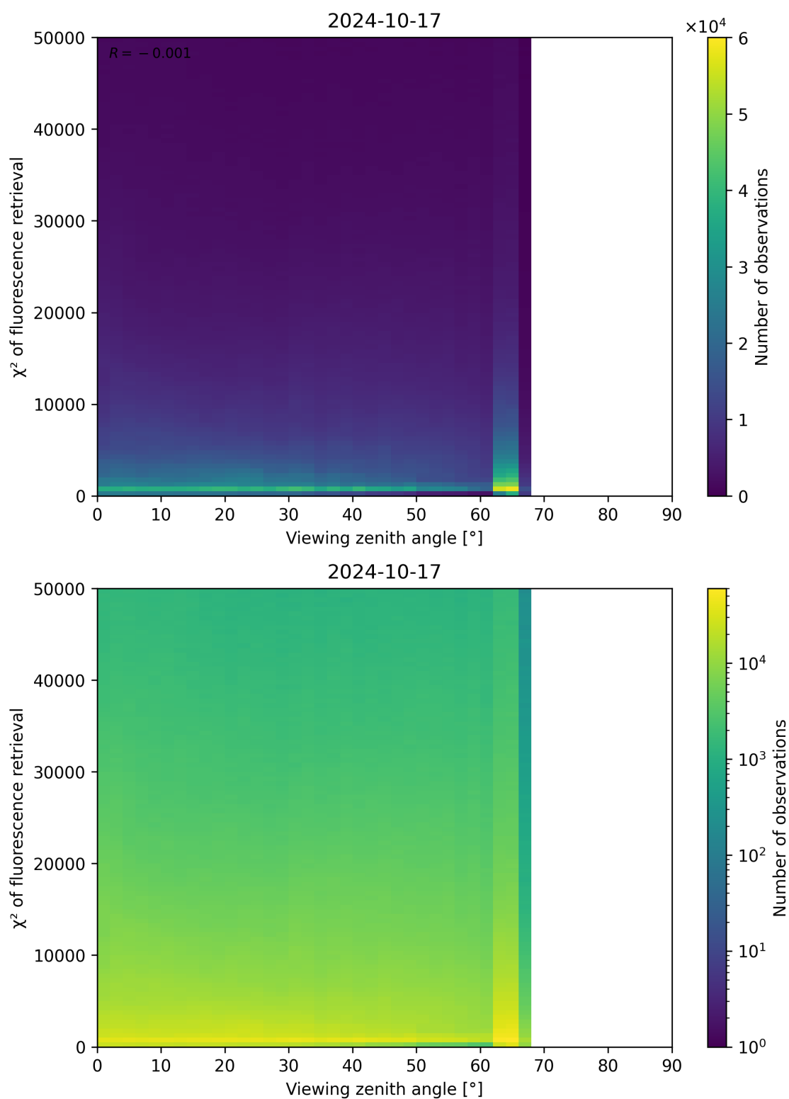
Figure 131: Scatter density plot of “Viewing zenith angle” against “ \chi^2 of fluorescence retrieval” for 2024-10-16 to 2024-10-18.
