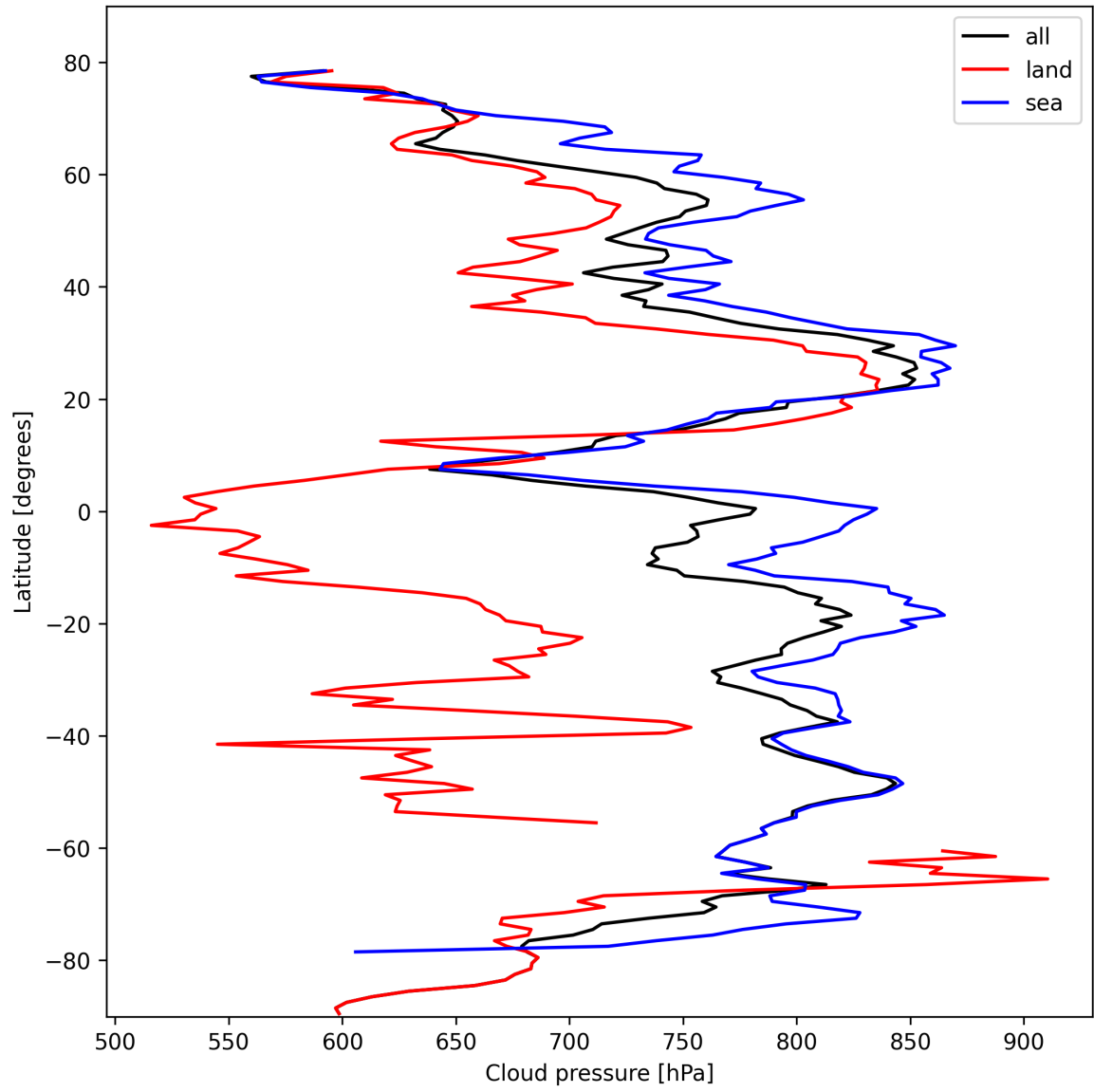
Figure 13: Zonal average of “Cloud pressure” for 2024-10-16 to 2024-10-18.
