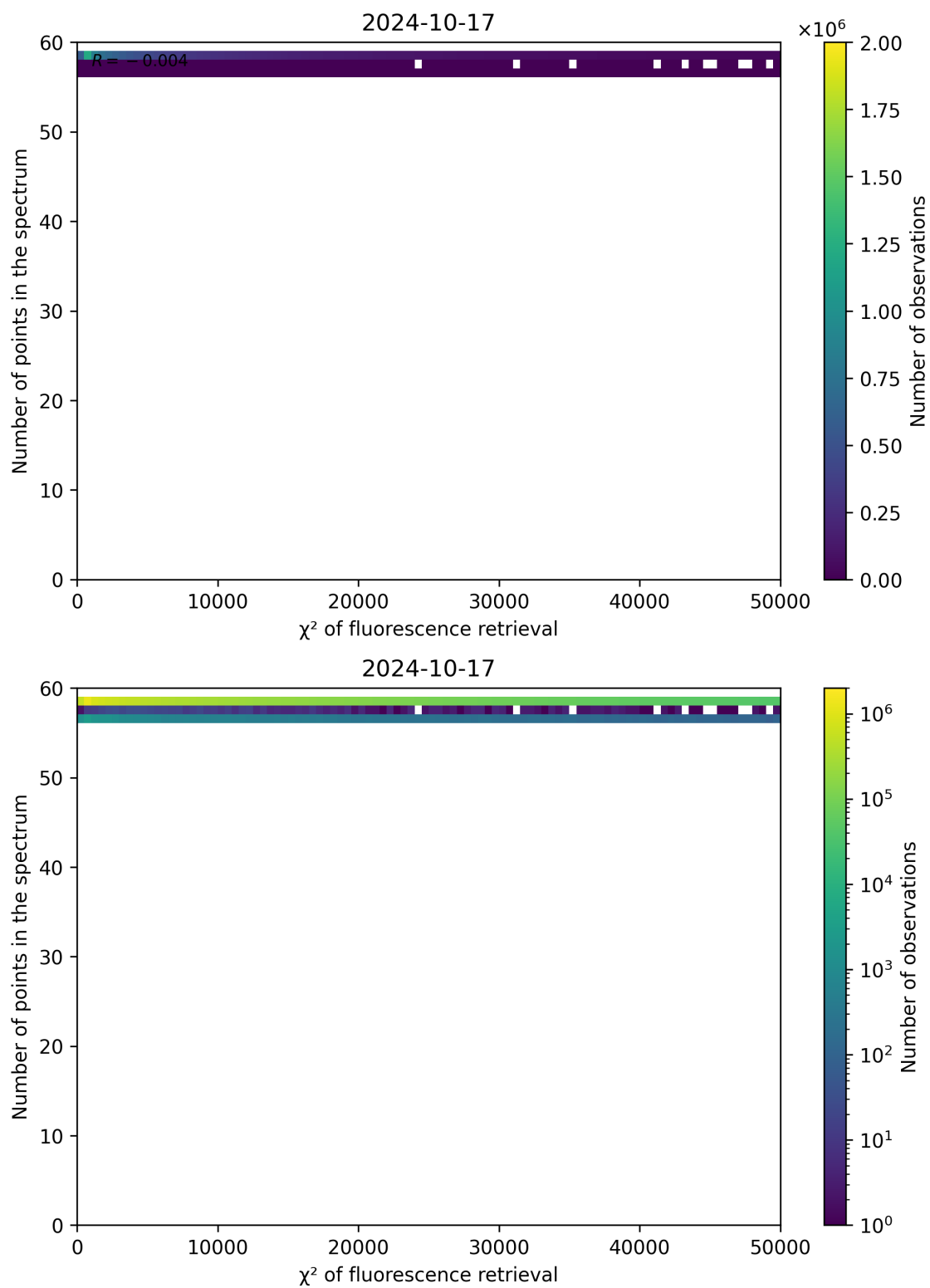
Figure 71: Scatter density plot of “ \chi^2 of fluorescence retrieval” against “Number of points in the spectrum” for 2024-10-16 to 2024-10-18.
