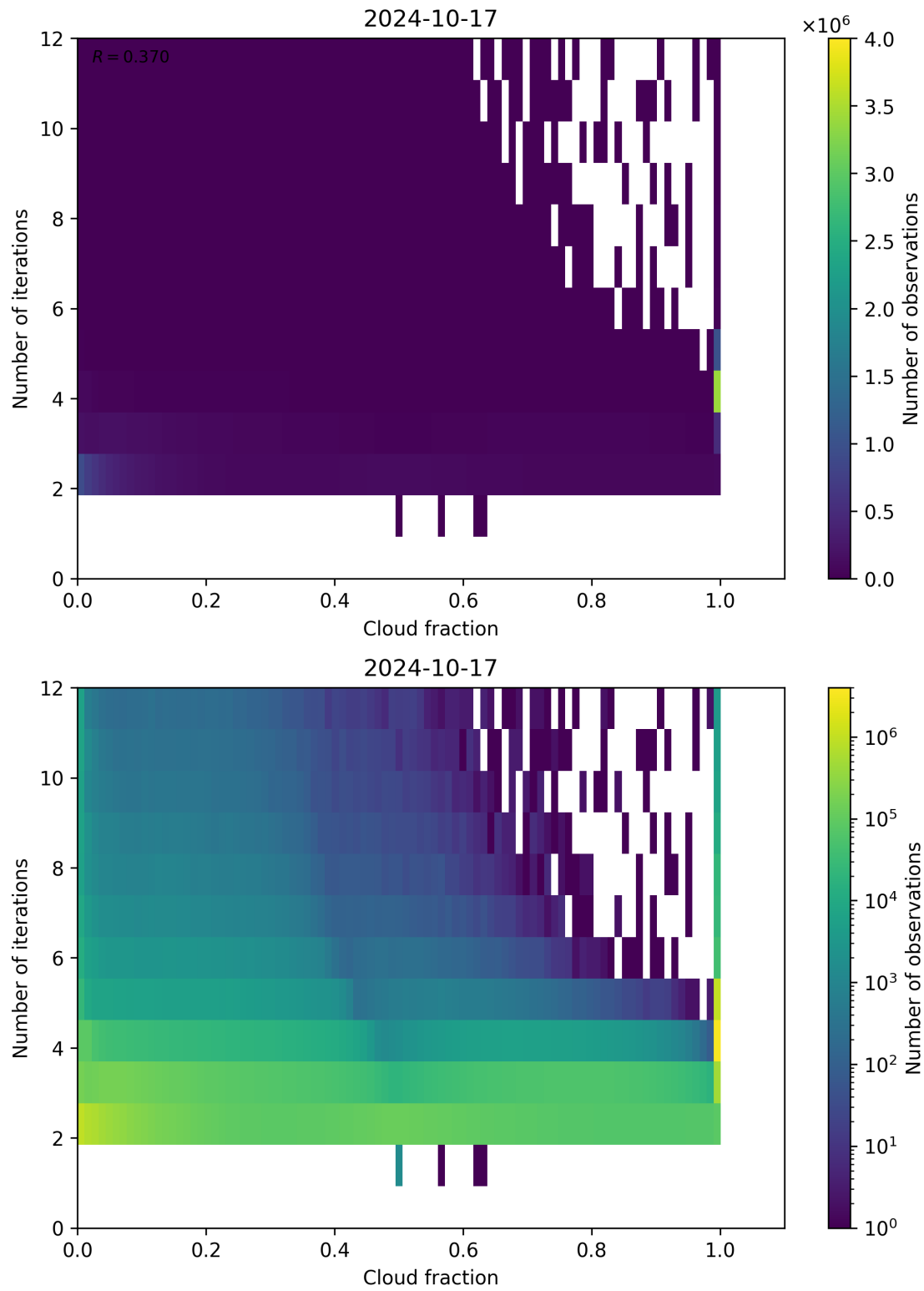
Figure 80: Scatter density plot of “Cloud fraction” against “Number of iterations” for 2024-10-16 to 2024-10-18.
