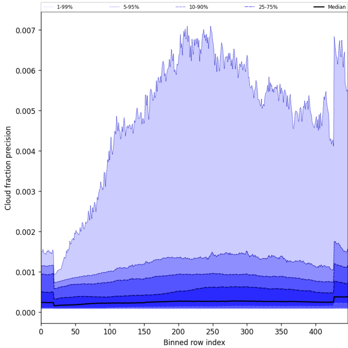
Figure 50: Along track statistics of “Cloud fraction precision” for 2024-10-17 to 2024-10-19
