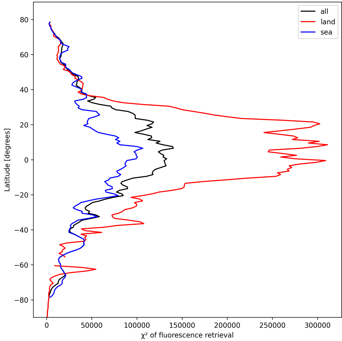
Figure 25: Zonal average of “ \chi^2 of fluorescence retrieval” for 2024-10-17 to 2024-10-19.
