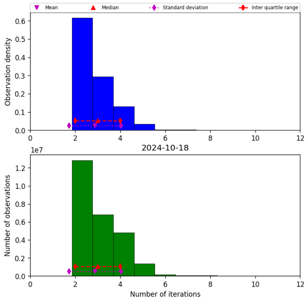
Figure 39: Histogram of “Number of iterations” for 2024-10-17 to 2024-10-19
