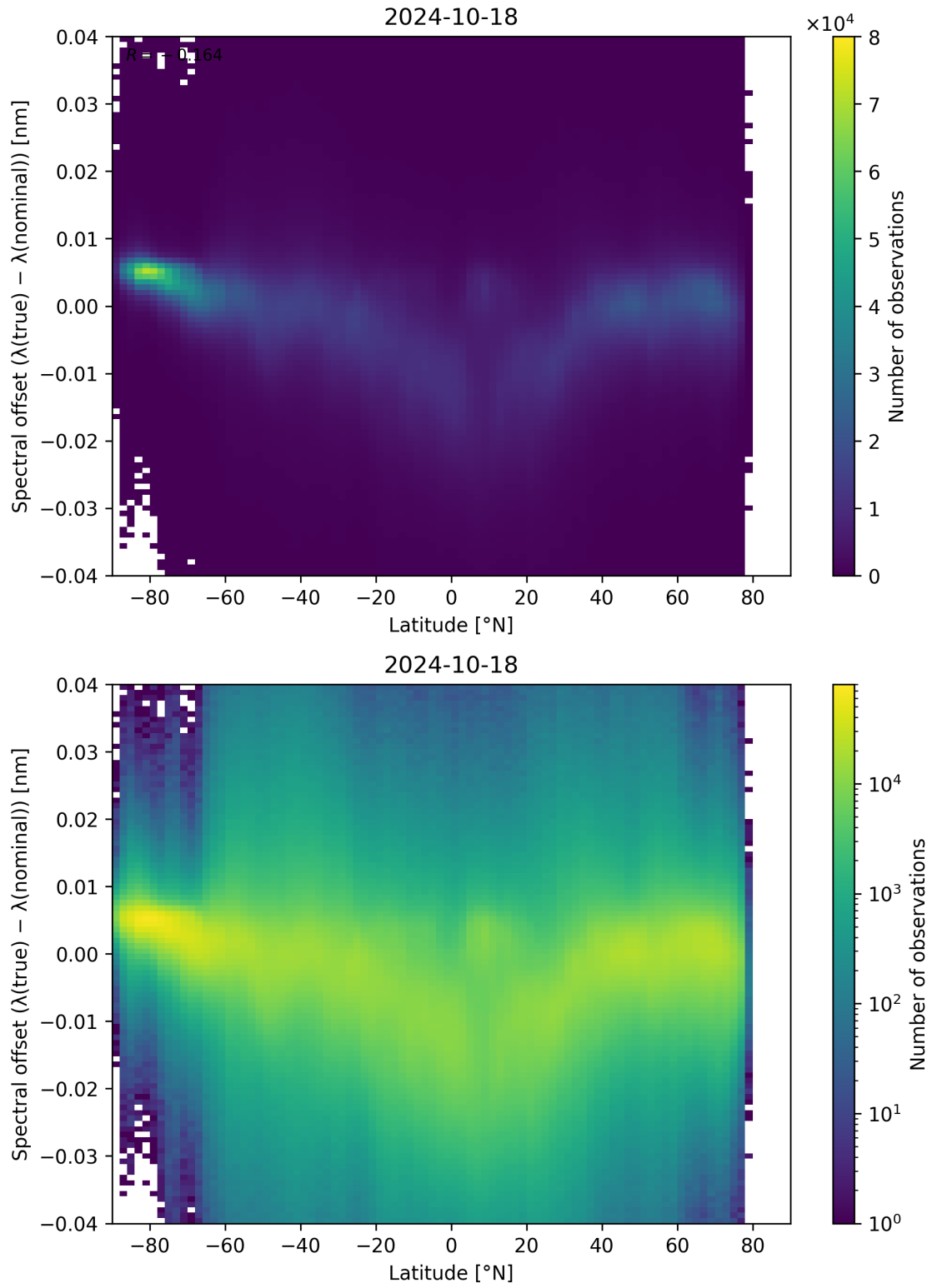
Figure 105: Scatter density plot of “Latitude” against “Spectral offset ( \lambda_{\text{true}} - \lambda_{\text{nominal}} )” for 2024-10-17 to 2024-10-19.
