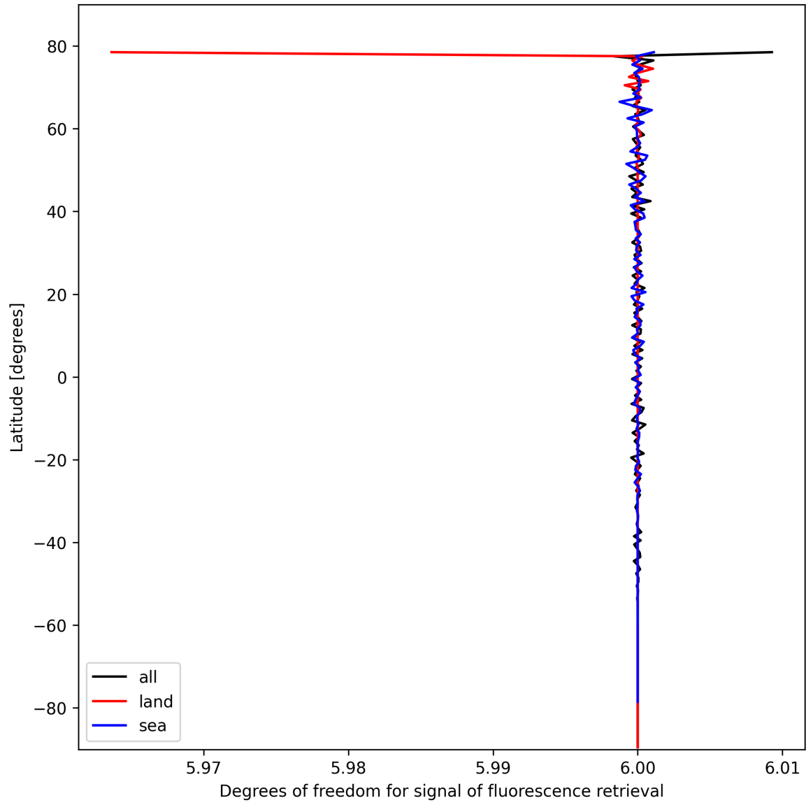
Figure 26: Zonal average of “Degrees of freedom for signal of fluorescence retrieval” for 2024-10-17 to 2024-10-19.
