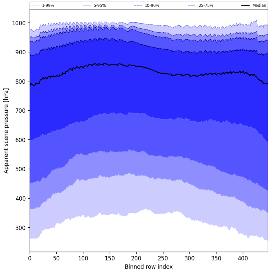
Figure 53: Along track statistics of “Apparent scene pressure” for 2024-10-17 to 2024-10-19
