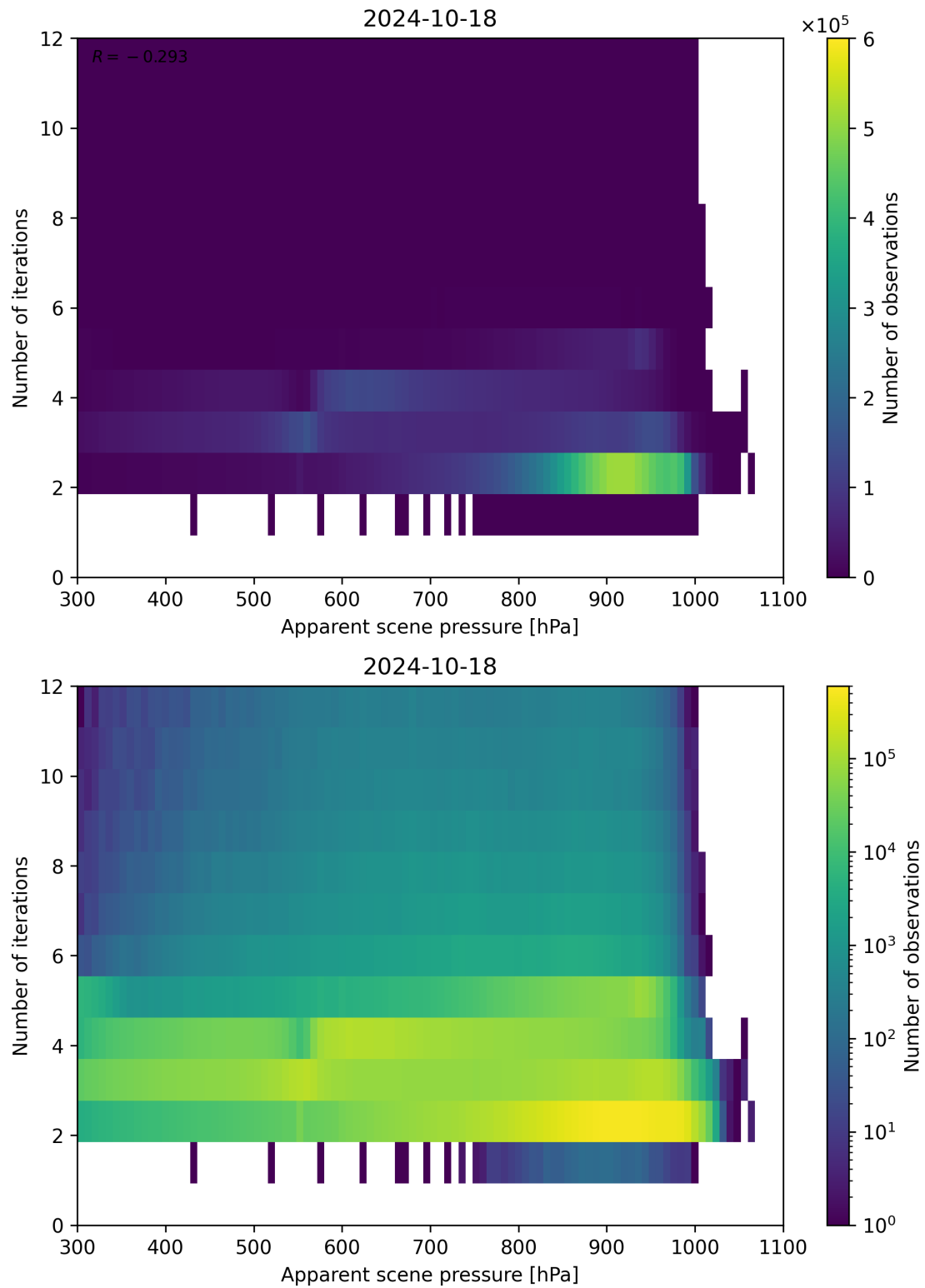
Figure 66: Scatter density plot of “Apparent scene pressure” against “Number of iterations” for 2024-10-17 to 2024-10-19.
