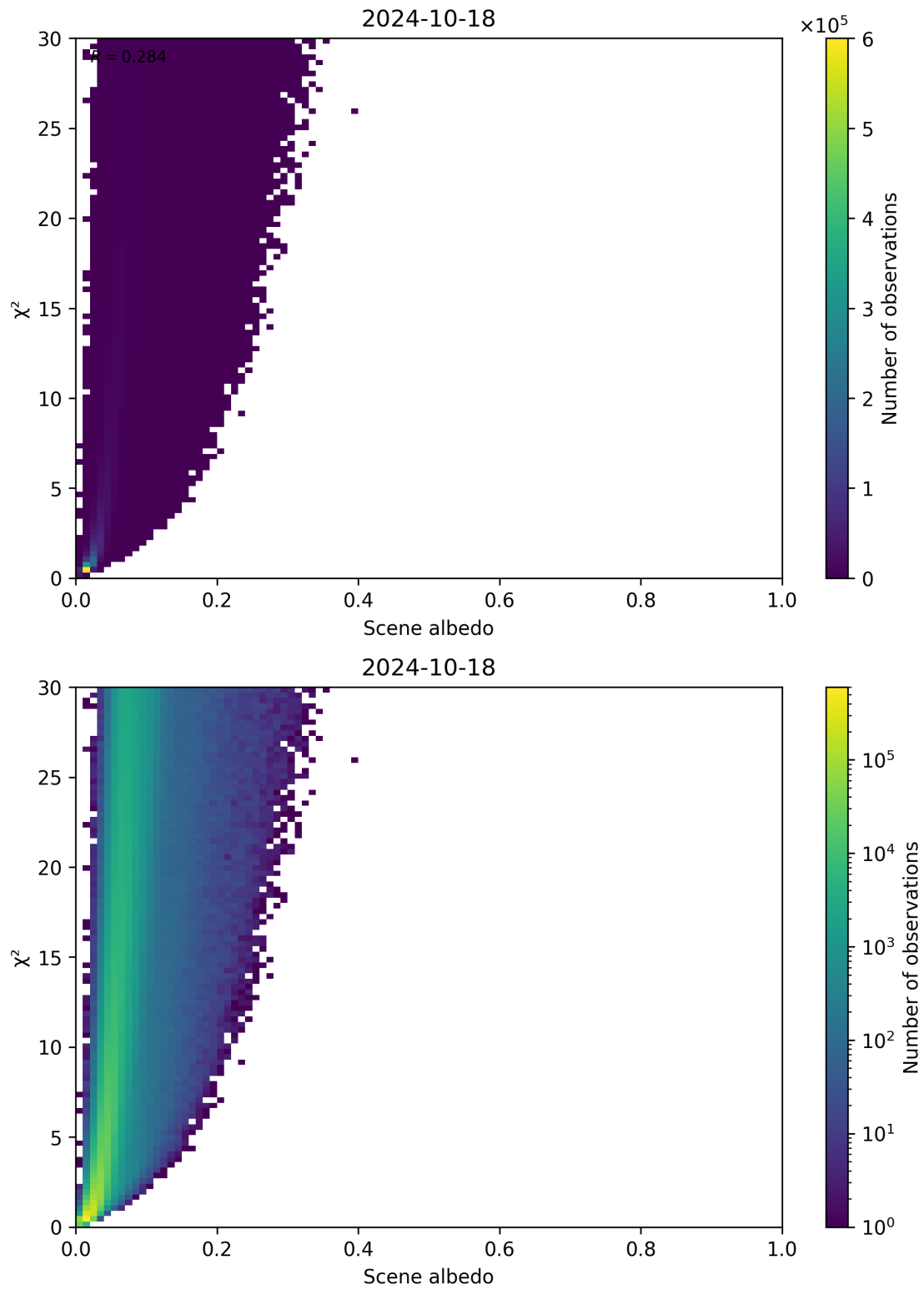
Figure 112: Scatter density plot of “Scene albedo” against “ \chi^2 ” for 2024-10-17 to 2024-10-19.
