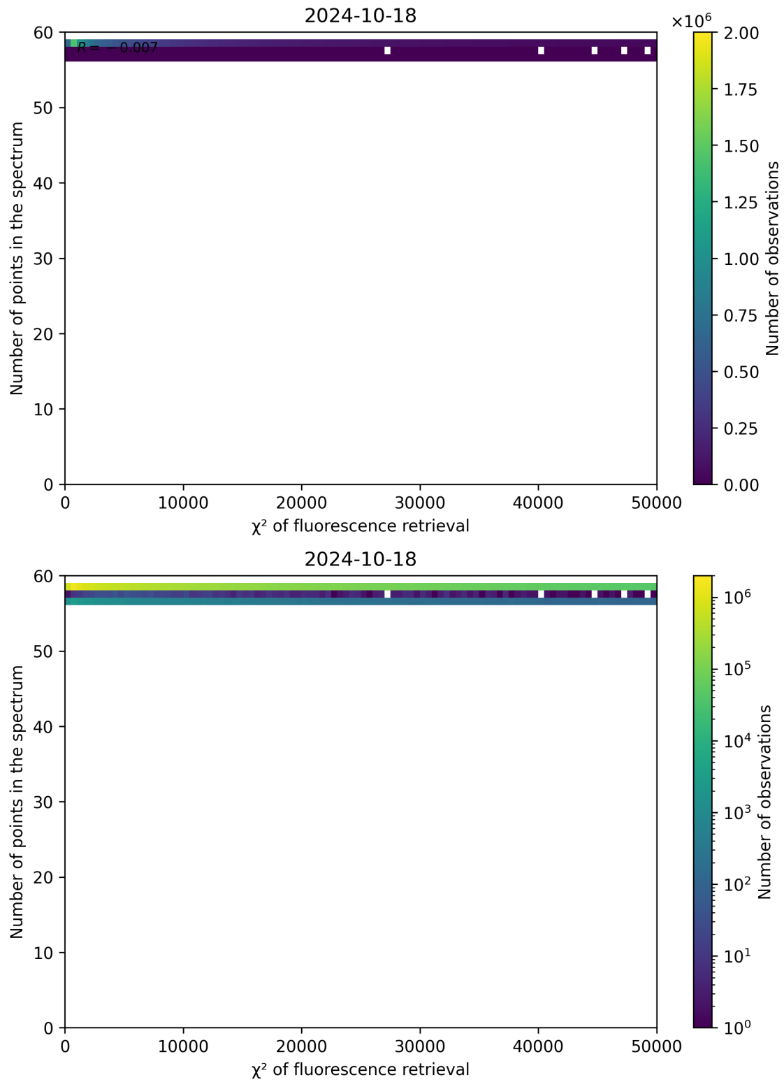
Figure 71: Scatter density plot of “ \chi^2 of fluorescence retrieval” against “Number of points in the spectrum” for 2024-10-17 to 2024-10-19.
