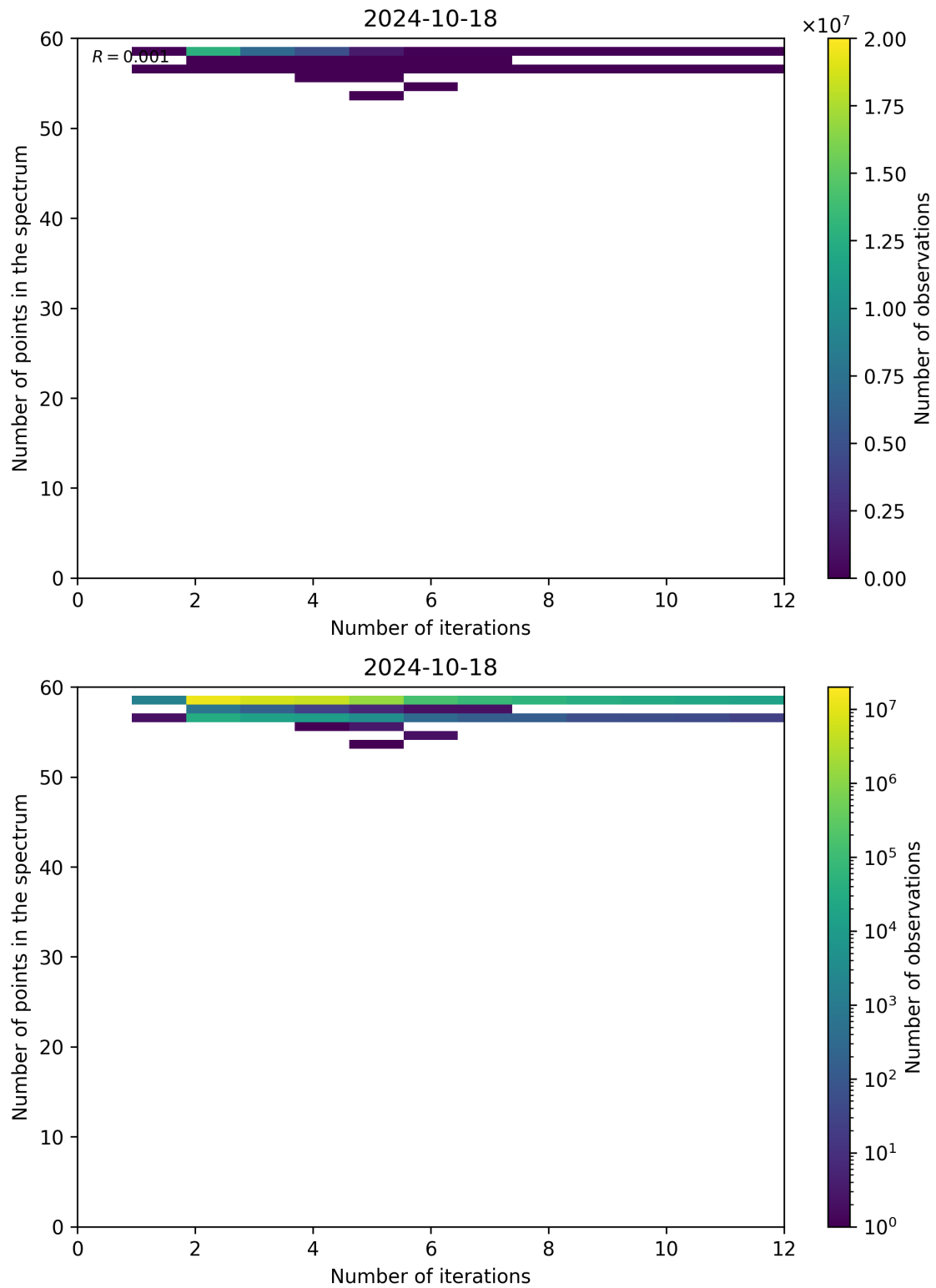
Figure 108: Scatter density plot of “Number of iterations” against “Number of points in the spectrum” for 2024-10-17 to 2024-10-19.
