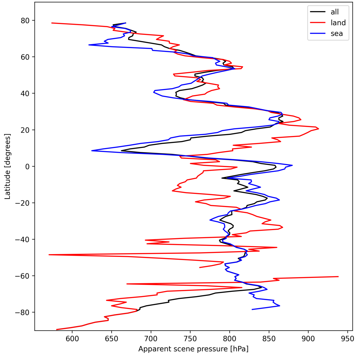
Figure 19: Zonal average of “Apparent scene pressure” for 2024-10-17 to 2024-10-19.
