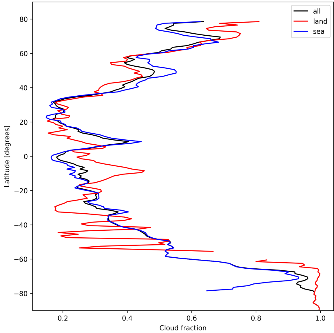
Figure 15: Zonal average of “Cloud fraction” for 2024-10-17 to 2024-10-19.
