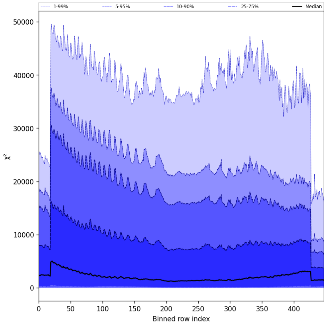
Figure 55: Along track statistics of “ \chi^2 ” for 2024-10-17 to 2024-10-19
