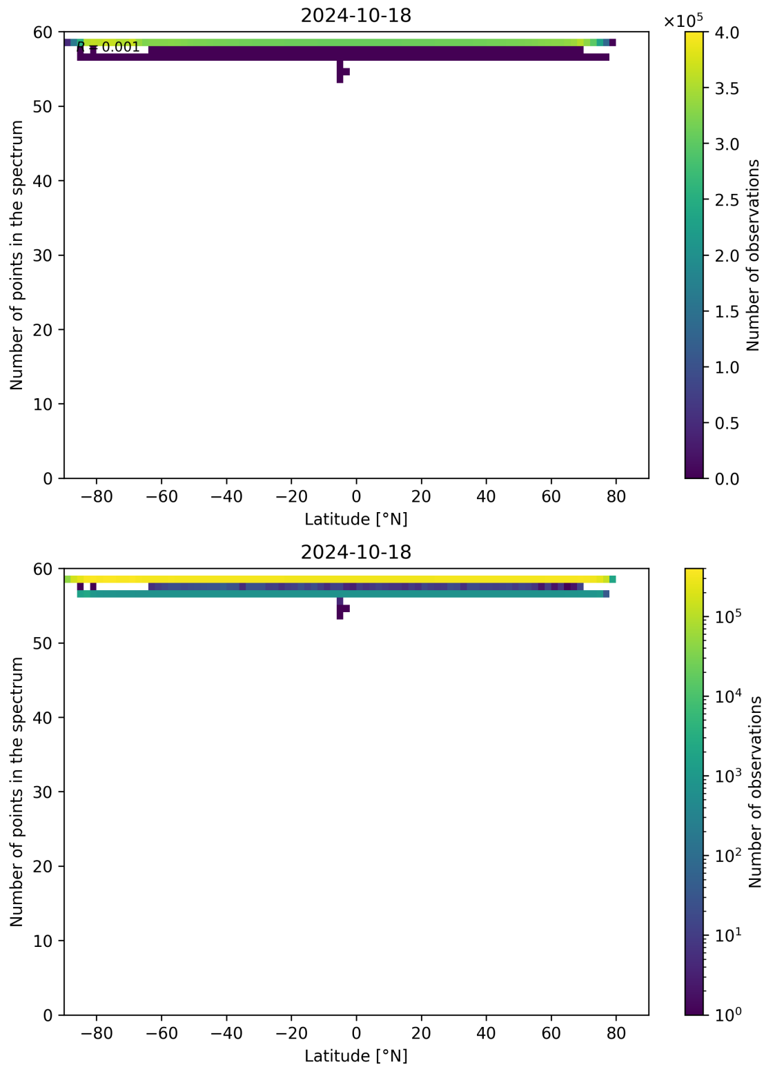
Figure 103: Scatter density plot of “Latitude” against “Number of points in the spectrum” for 2024-10-17 to 2024-10-19.
