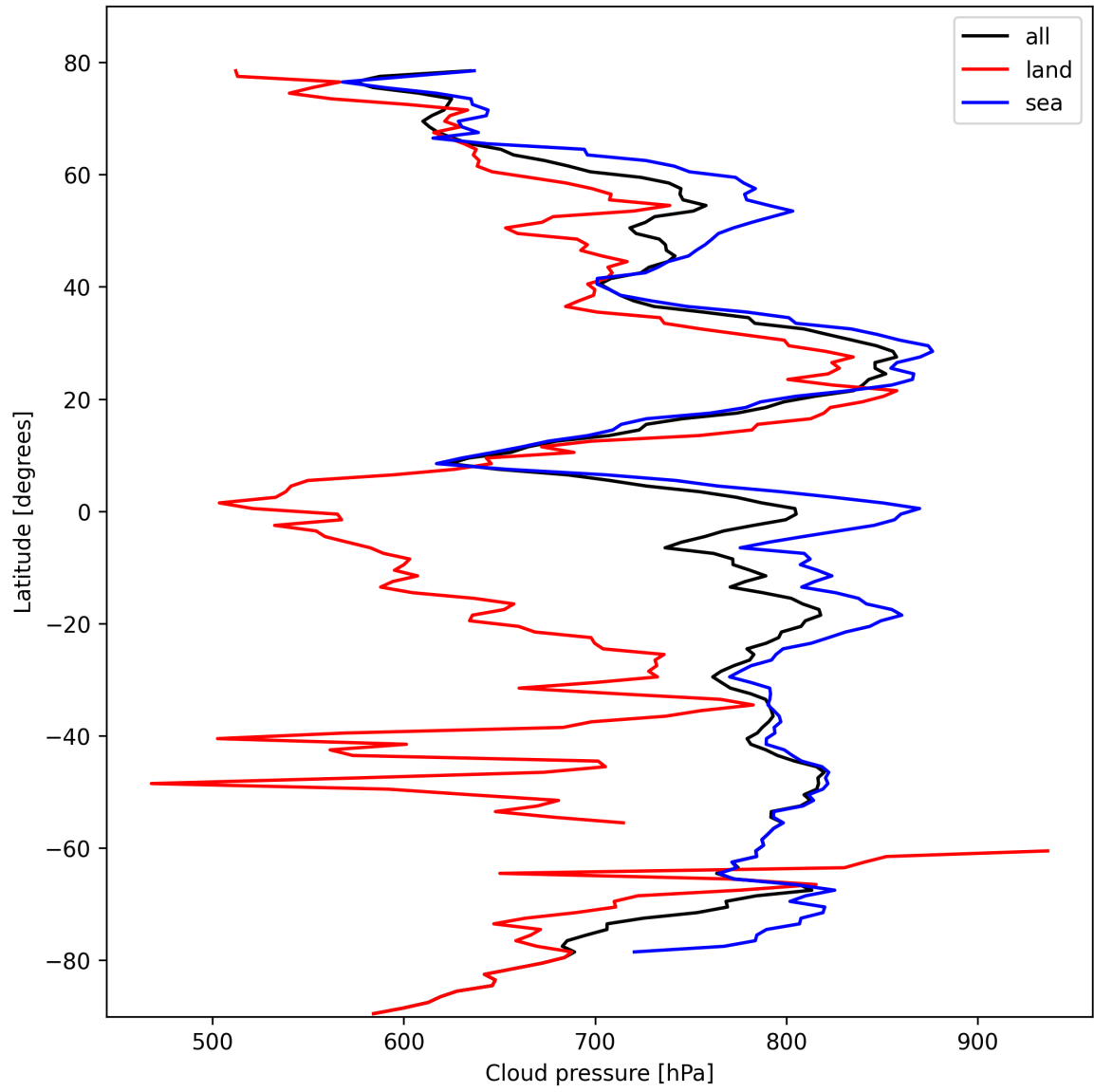
Figure 13: Zonal average of “Cloud pressure” for 2024-10-17 to 2024-10-19.
