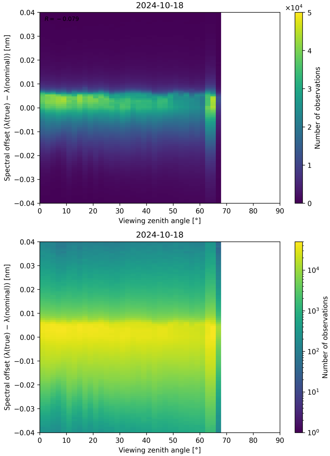
Figure 140: Scatter density plot of “Viewing zenith angle” against “Spectral offset ( \lambda_{\text{true}} - \lambda_{\text{nominal}} )” for 2024-10-17 to 2024-10-19.
