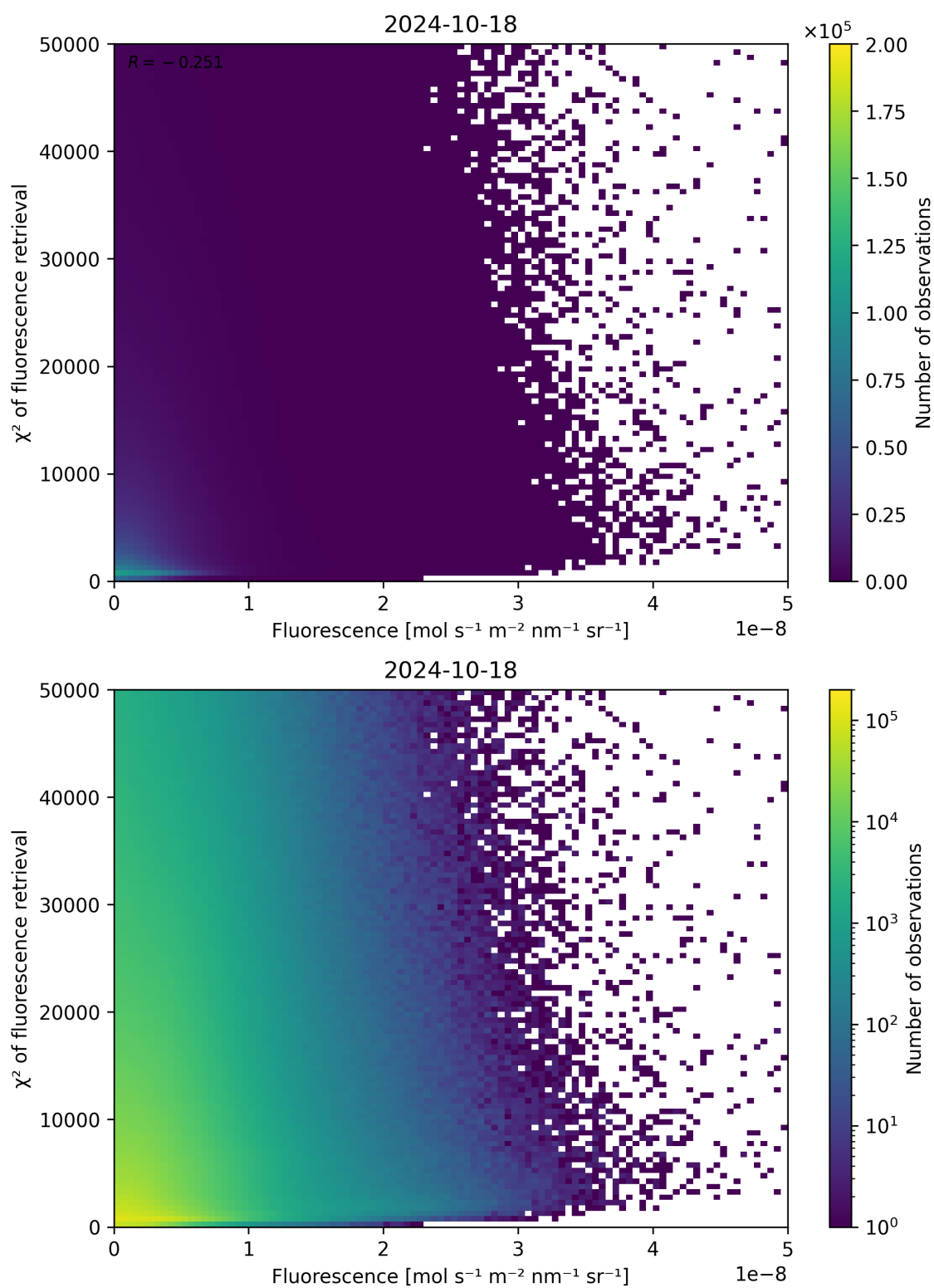
Figure 93: Scatter density plot of “Fluorescence” against “ \chi^2 of fluorescence retrieval” for 2024-10-17 to 2024-10-19.
