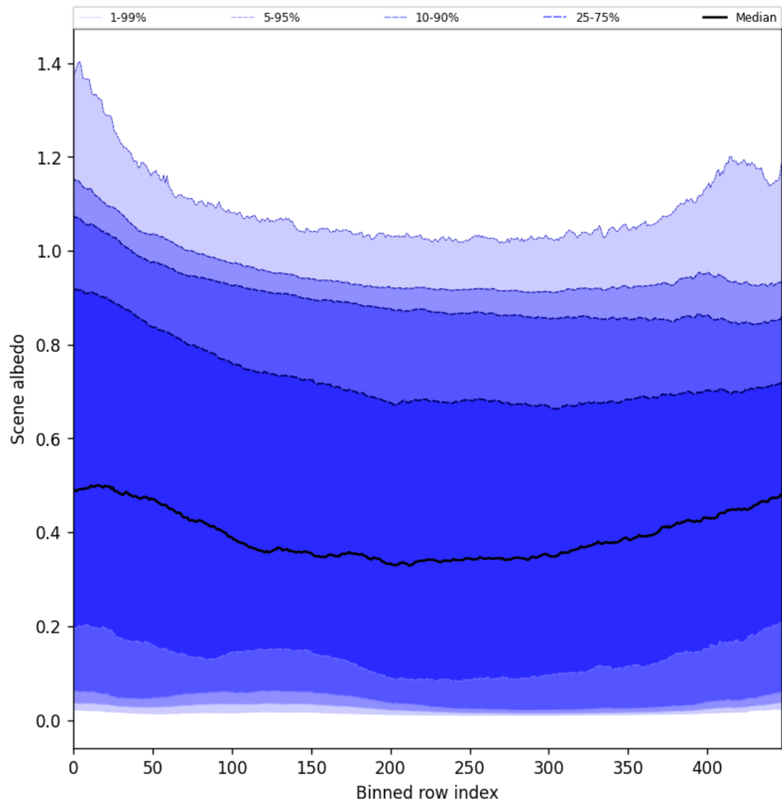
Figure 51: Along track statistics of “Scene albedo” for 2024-10-17 to 2024-10-19
