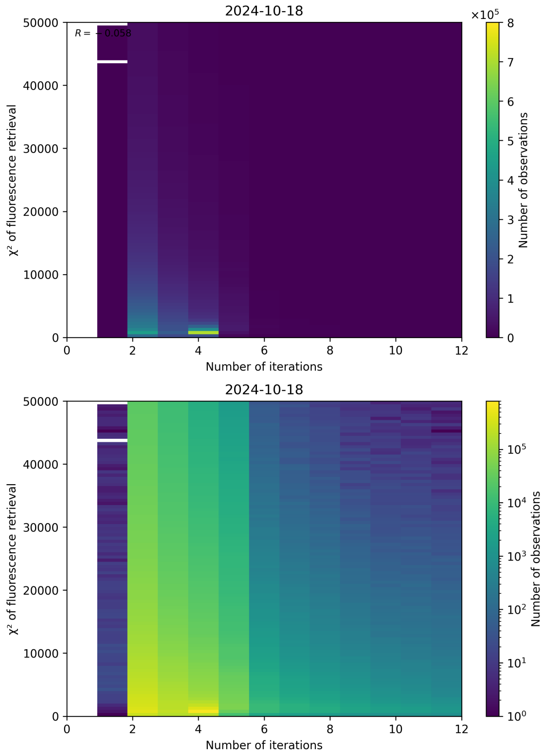
Figure 106: Scatter density plot of “Number of iterations” against “ \chi^2 of fluorescence retrieval” for 2024-10-17 to 2024-10-19.
