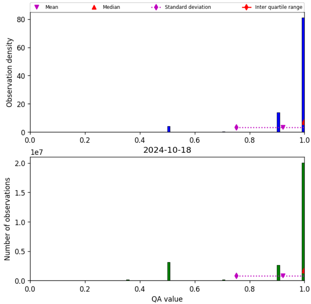
Figure 29: Histogram of “QA value” for 2024-10-17 to 2024-10-19
