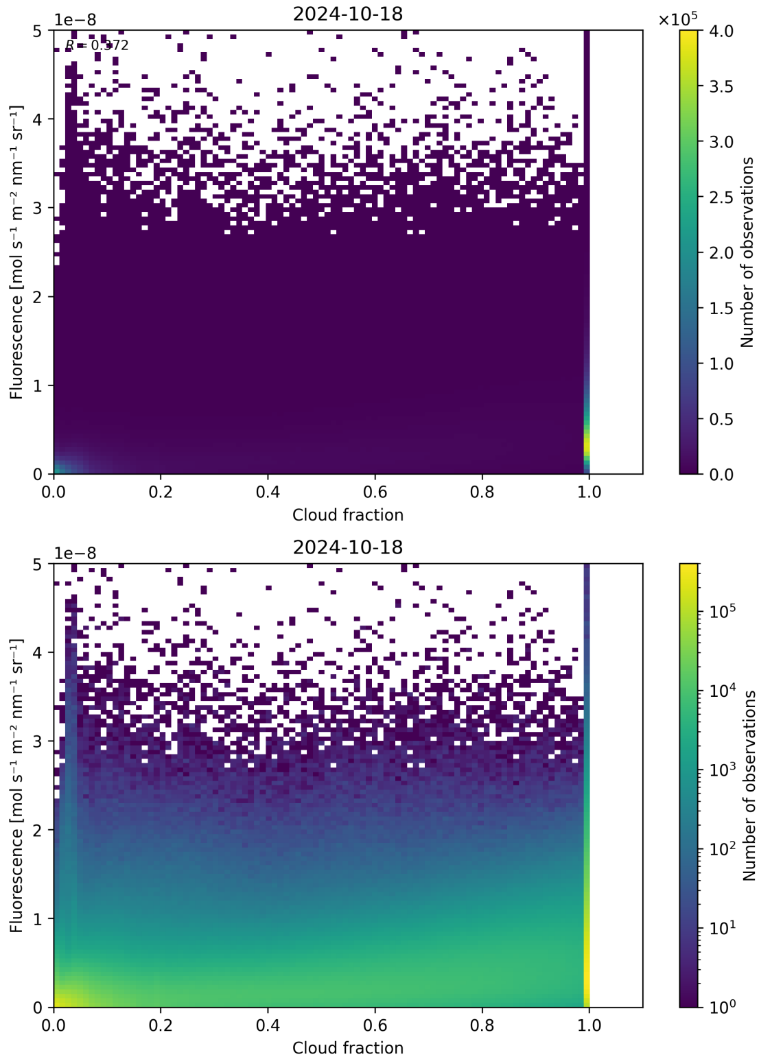
Figure 79: Scatter density plot of “Cloud fraction” against “Fluorescence” for 2024-10-17 to 2024-10-19.
