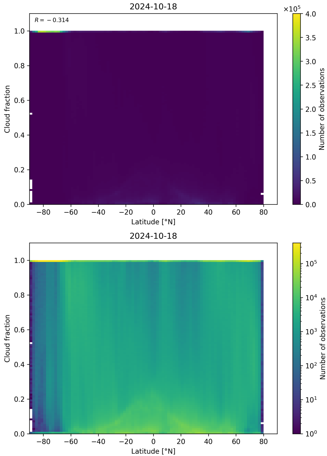
Figure 99: Scatter density plot of “Latitude” against “Cloud fraction” for 2024-10-17 to 2024-10-19.
