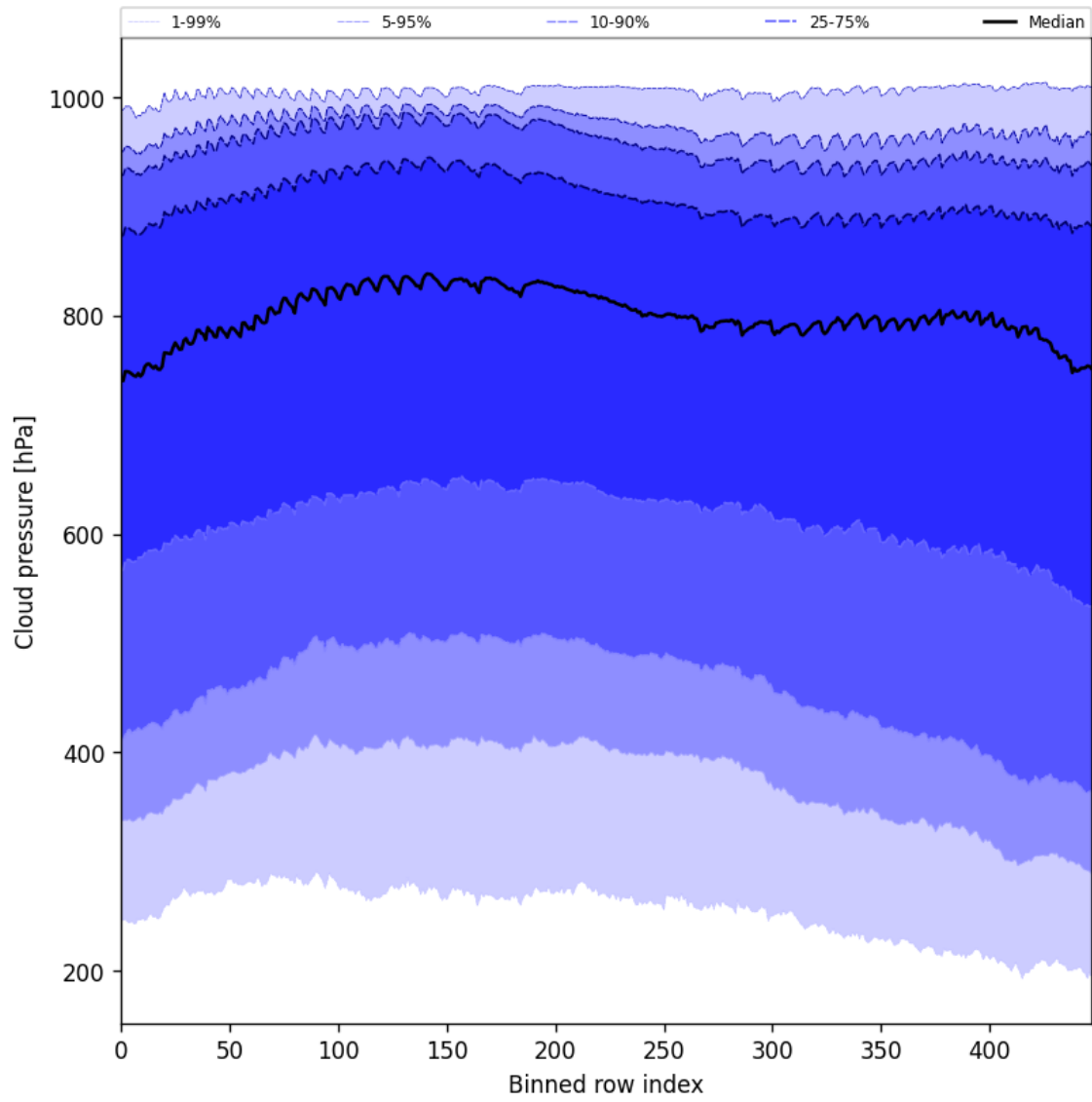
Figure 47: Along track statistics of “Cloud pressure” for 2024-10-17 to 2024-10-19
