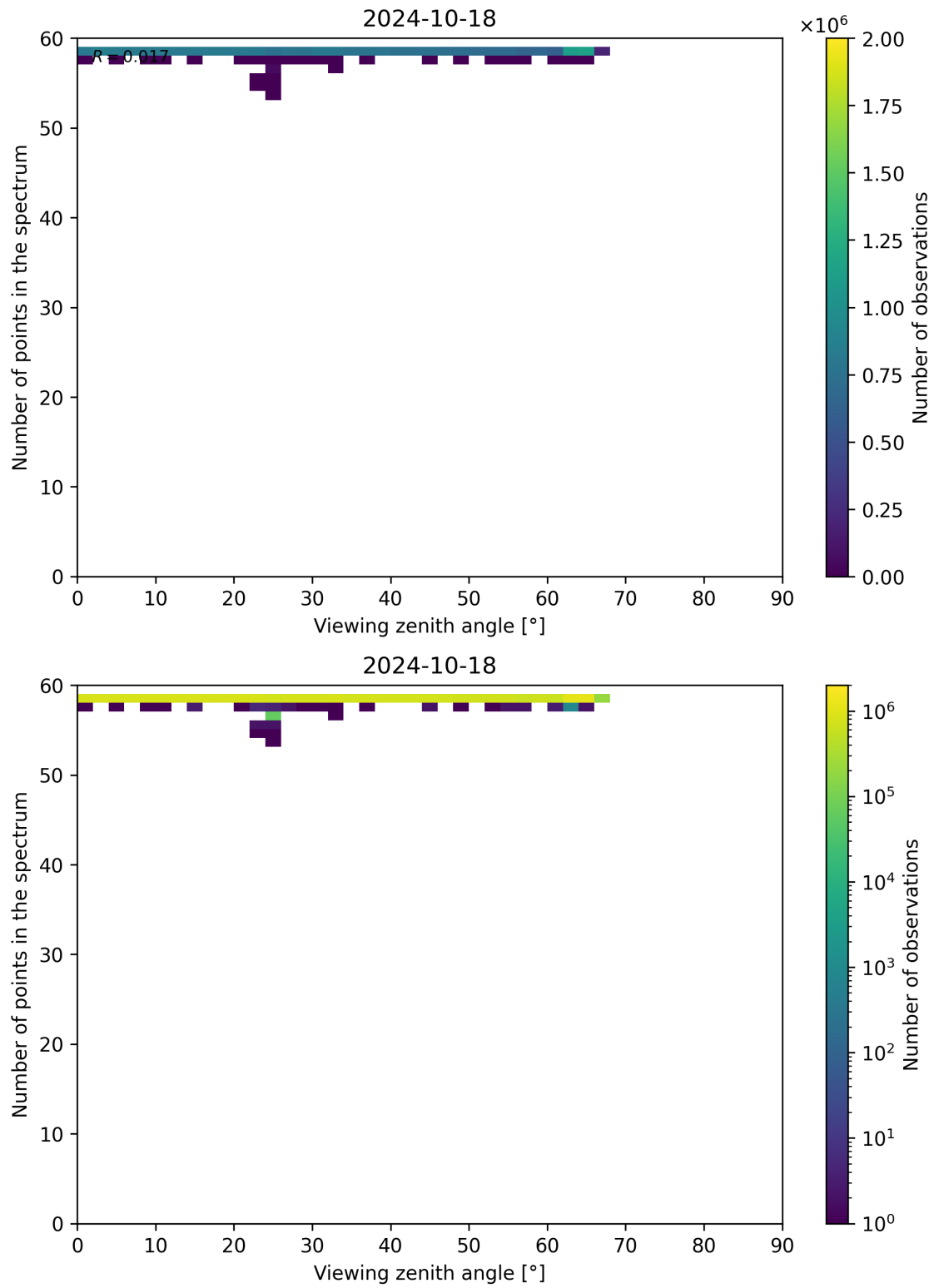
Figure 137: Scatter density plot of “Viewing zenith angle” against “Number of points in the spectrum” for 2024-10-17 to 2024-10-19.
