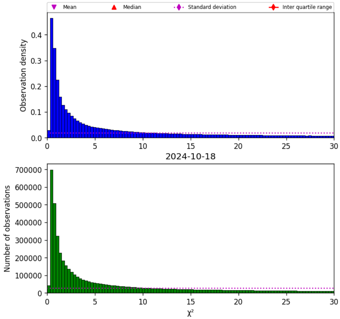
Figure 38: Histogram of " \chi^2 " for 2024-10-17 to 2024-10-19
