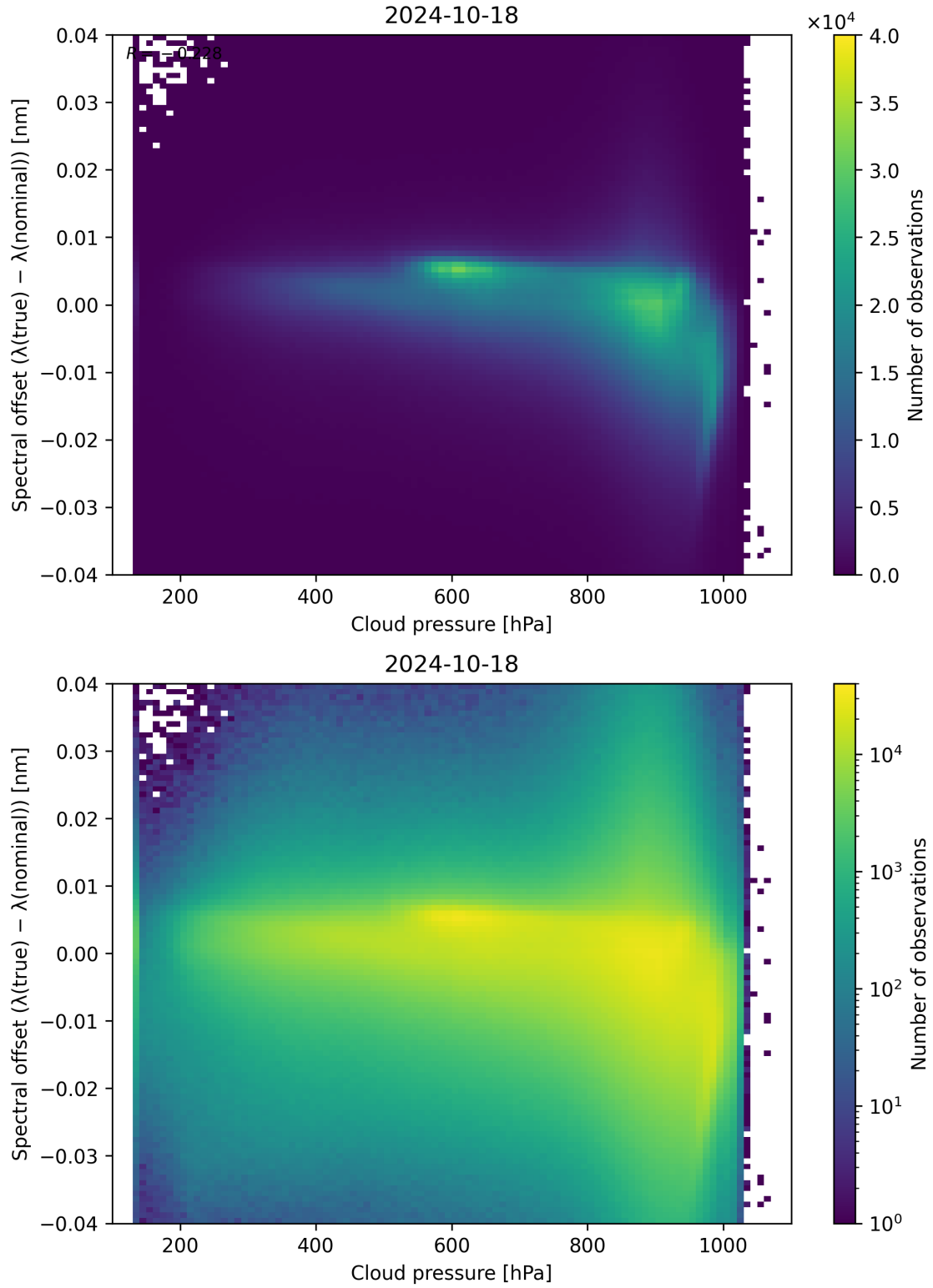
Figure 92: Scatter density plot of “Cloud pressure” against “Spectral offset ( \lambda_{\text{true}} - \lambda_{\text{nominal}} )” for 2024-10-17 to 2024-10-19.
