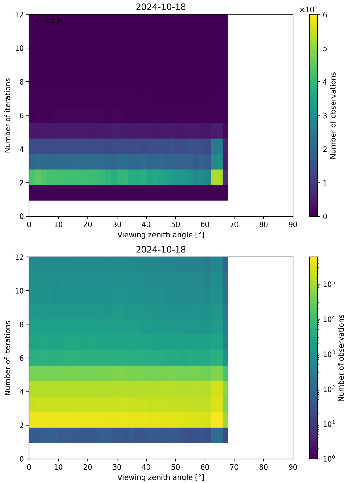
Figure 136: Scatter density plot of “Viewing zenith angle” against “Number of iterations” for 2024-10-17 to 2024-10-19.
