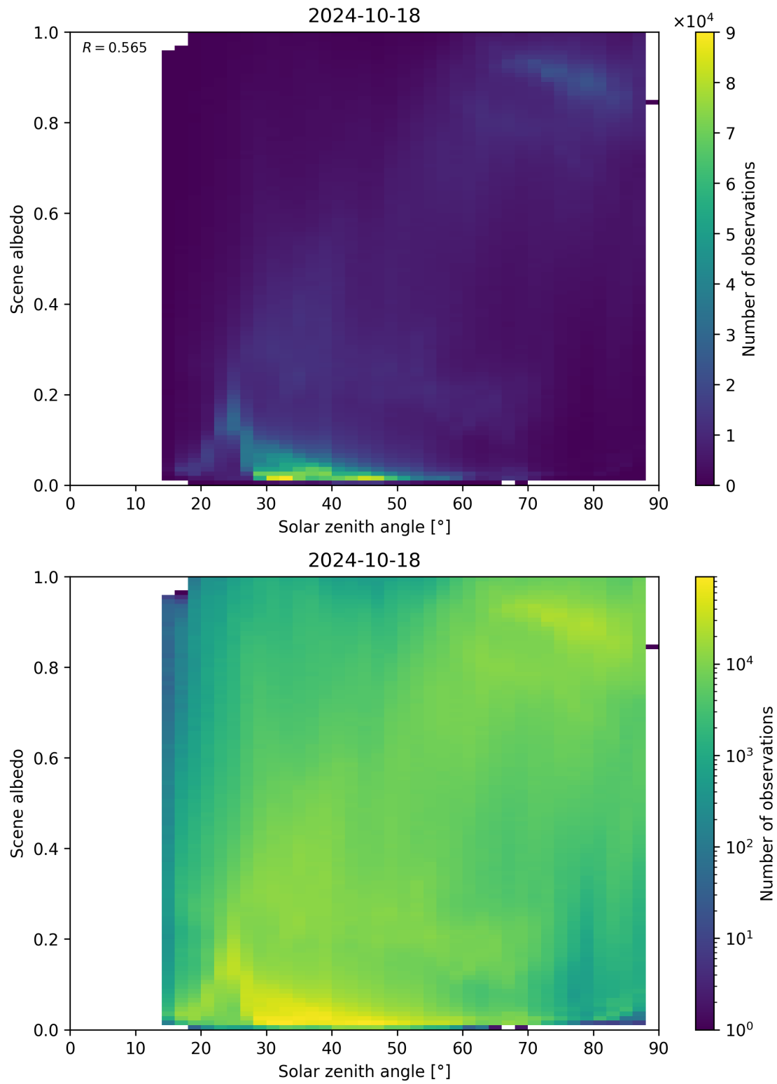
Figure 127: Scatter density plot of “Solar zenith angle” against “Scene albedo” for 2024-10-17 to 2024-10-19.
