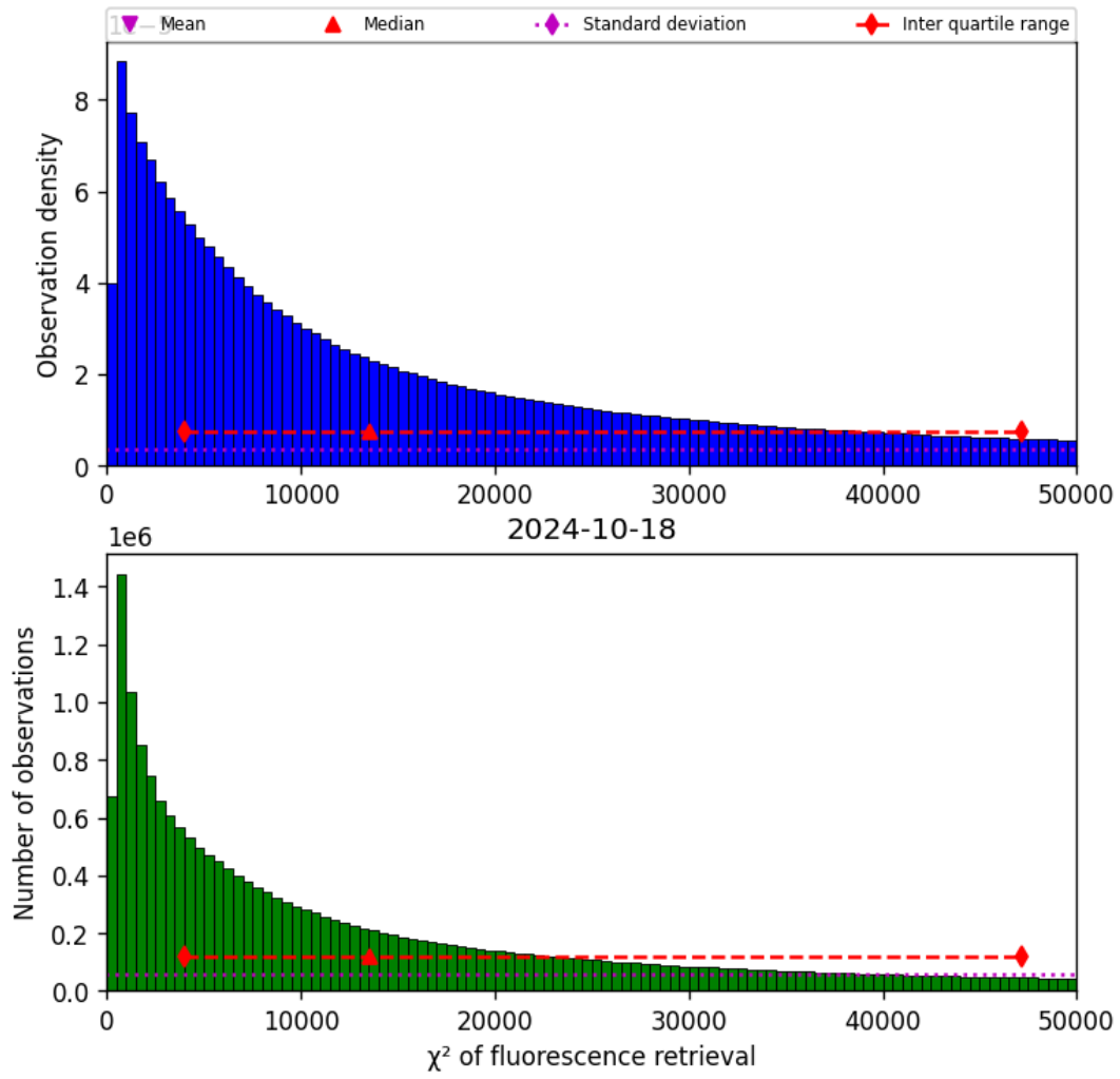
Figure 42: Histogram of “ \chi^2 of fluorescence retrieval” for 2024-10-17 to 2024-10-19
