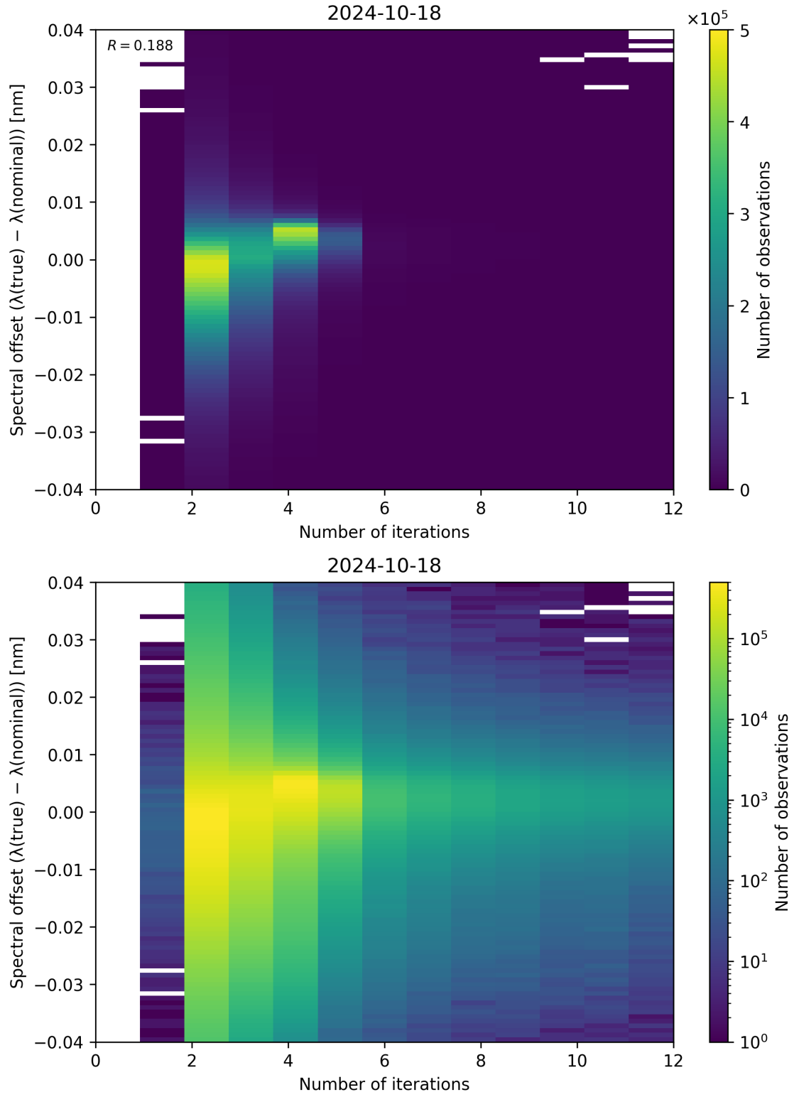
Figure 109: Scatter density plot of “Number of iterations” against “Spectral offset ( \lambda_{\text{true}} - \lambda_{\text{nominal}} )” for 2024-10-17 to 2024-10-19.
