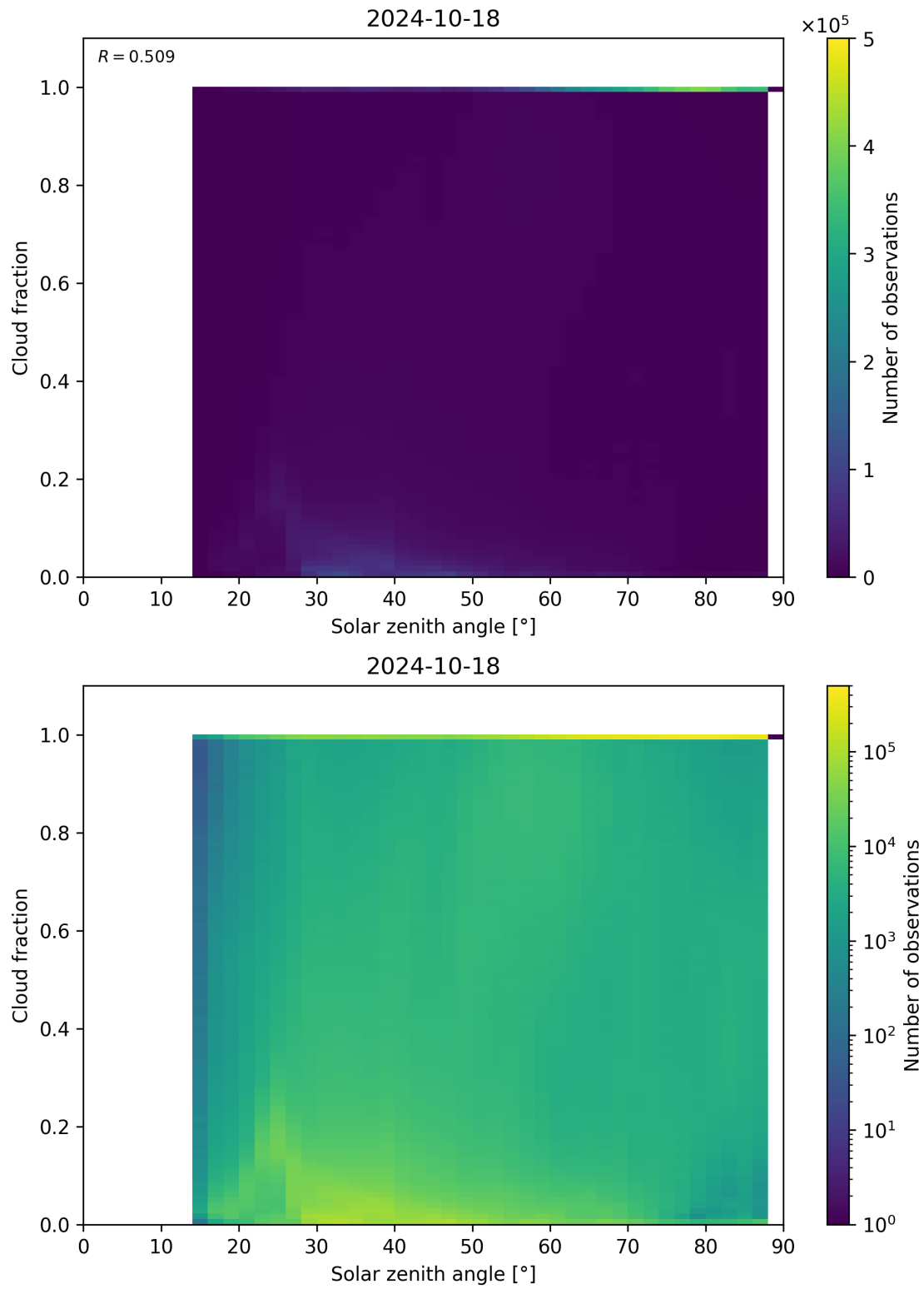
Figure 121: Scatter density plot of “Solar zenith angle” against “Cloud fraction” for 2024-10-17 to 2024-10-19.
