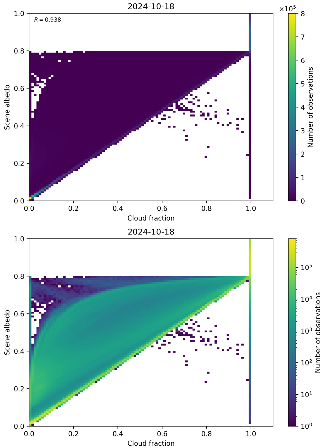
Figure 82: Scatter density plot of “Cloud fraction” against “Scene albedo” for 2024-10-17 to 2024-10-19.
