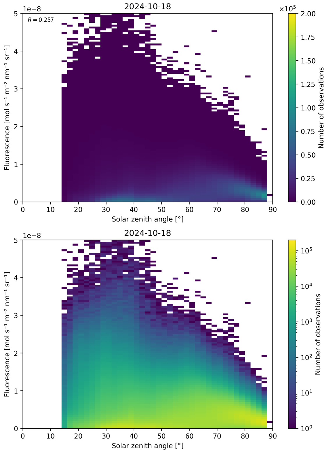
Figure 123: Scatter density plot of “Solar zenith angle” against “Fluorescence” for 2024-10-17 to 2024-10-19.
