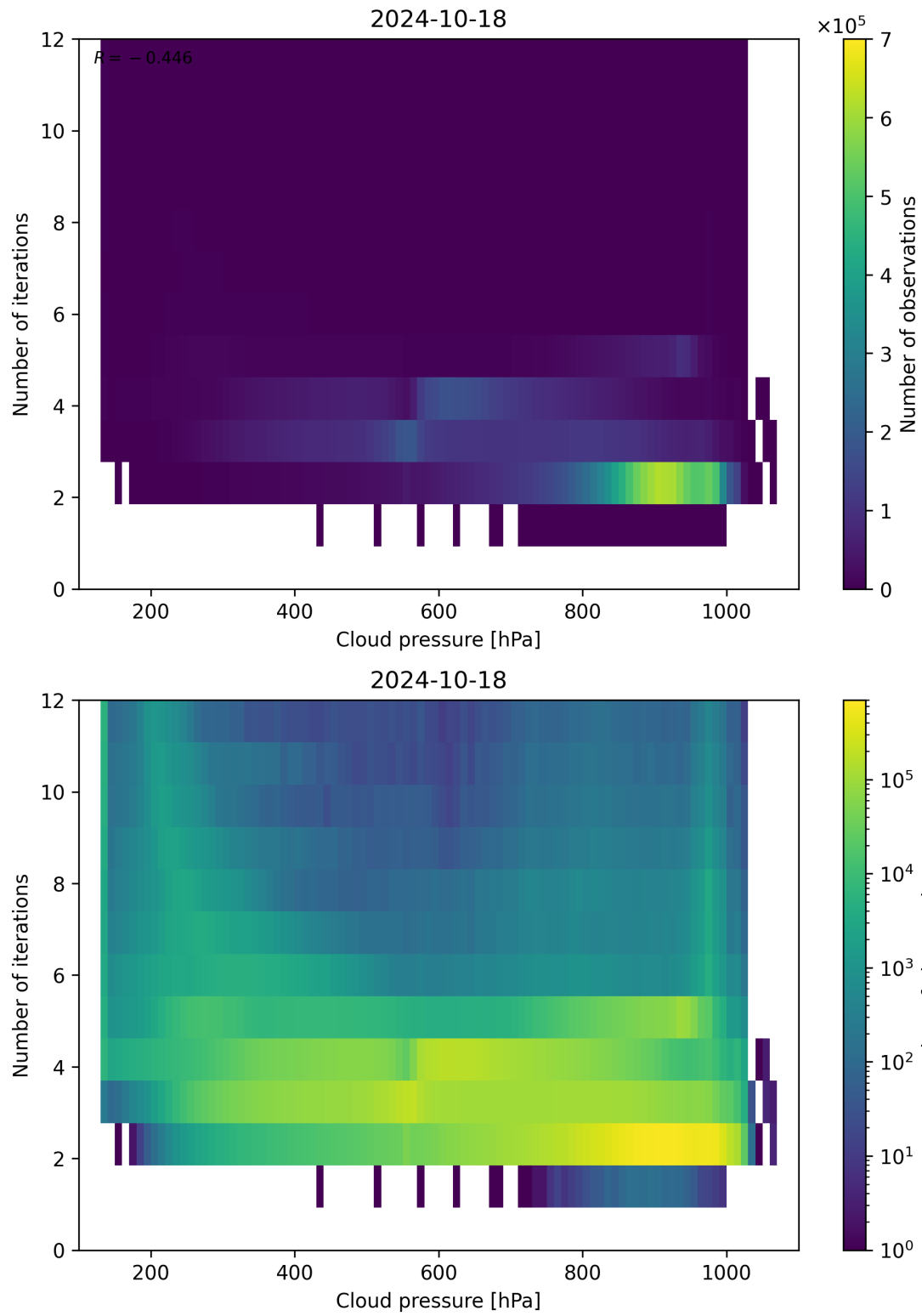
Figure 89: Scatter density plot of “Cloud pressure” against “Number of iterations” for 2024-10-17 to 2024-10-19.
