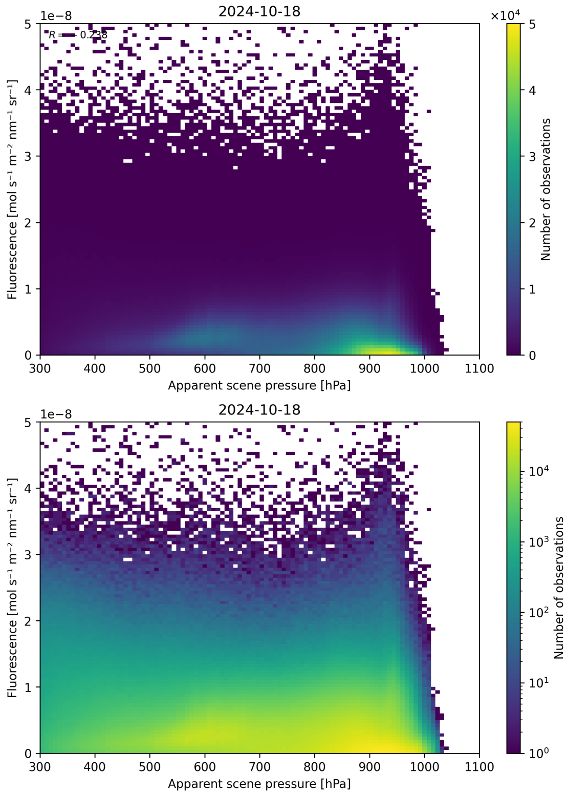
Figure 65: Scatter density plot of “Apparent scene pressure” against “Fluorescence” for 2024-10-17 to 2024-10-19.
