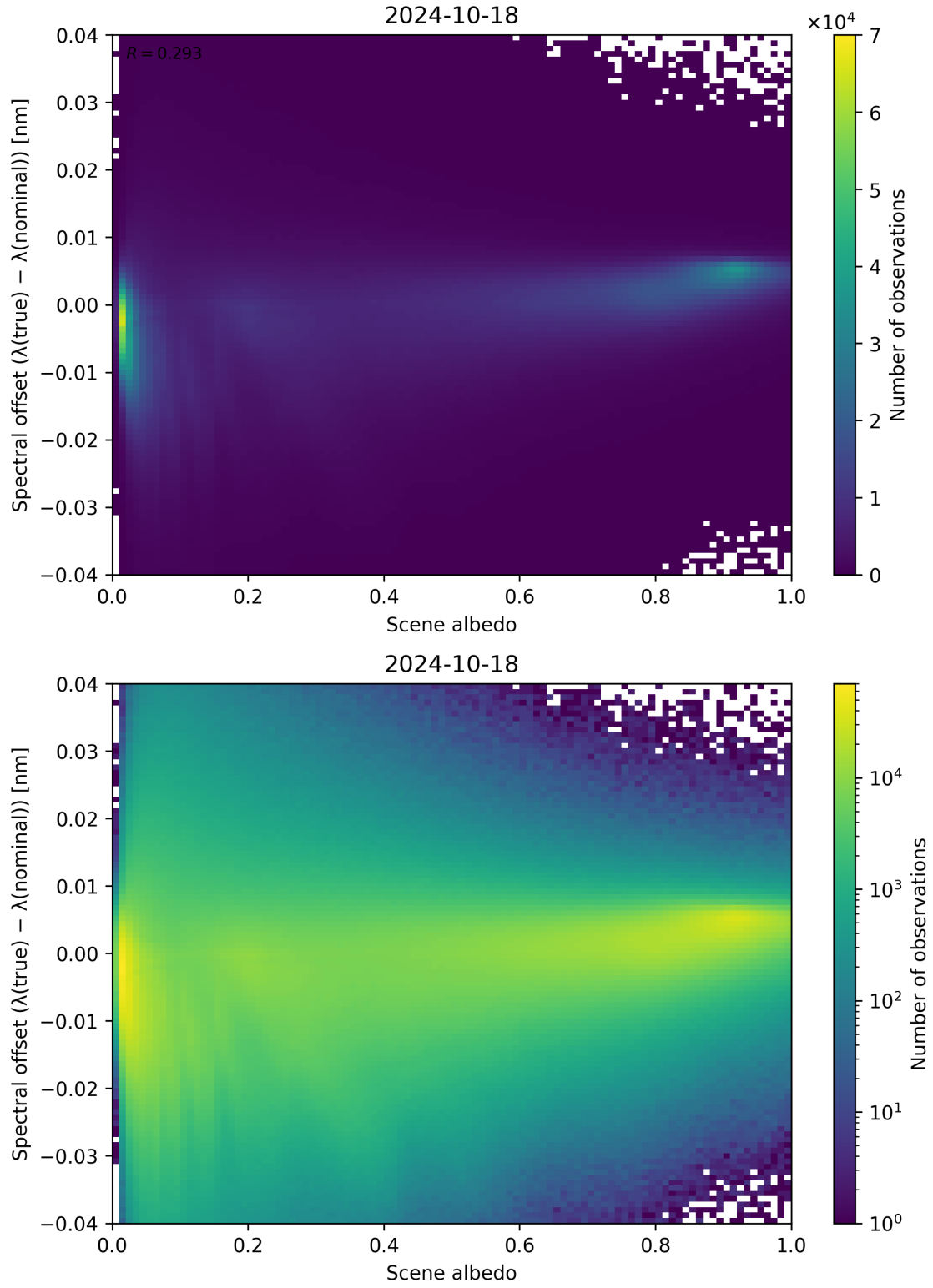
Figure 117: Scatter density plot of “Scene albedo” against “Spectral offset ( \lambda_{\text{true}} - \lambda_{\text{nominal}} )” for 2024-10-17 to 2024-10-19.
