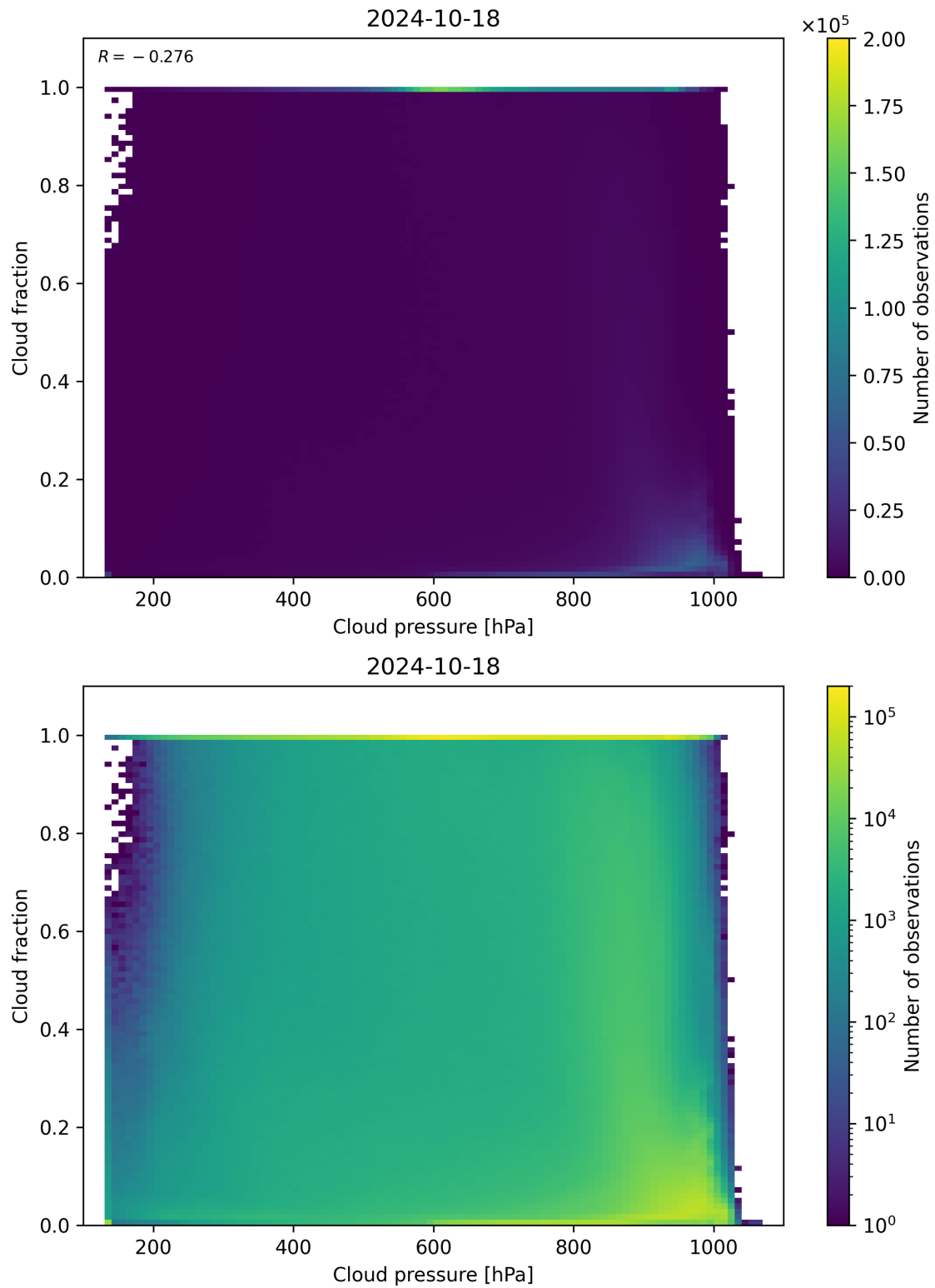
Figure 87: Scatter density plot of “Cloud pressure” against “Cloud fraction” for 2024-10-17 to 2024-10-19.
