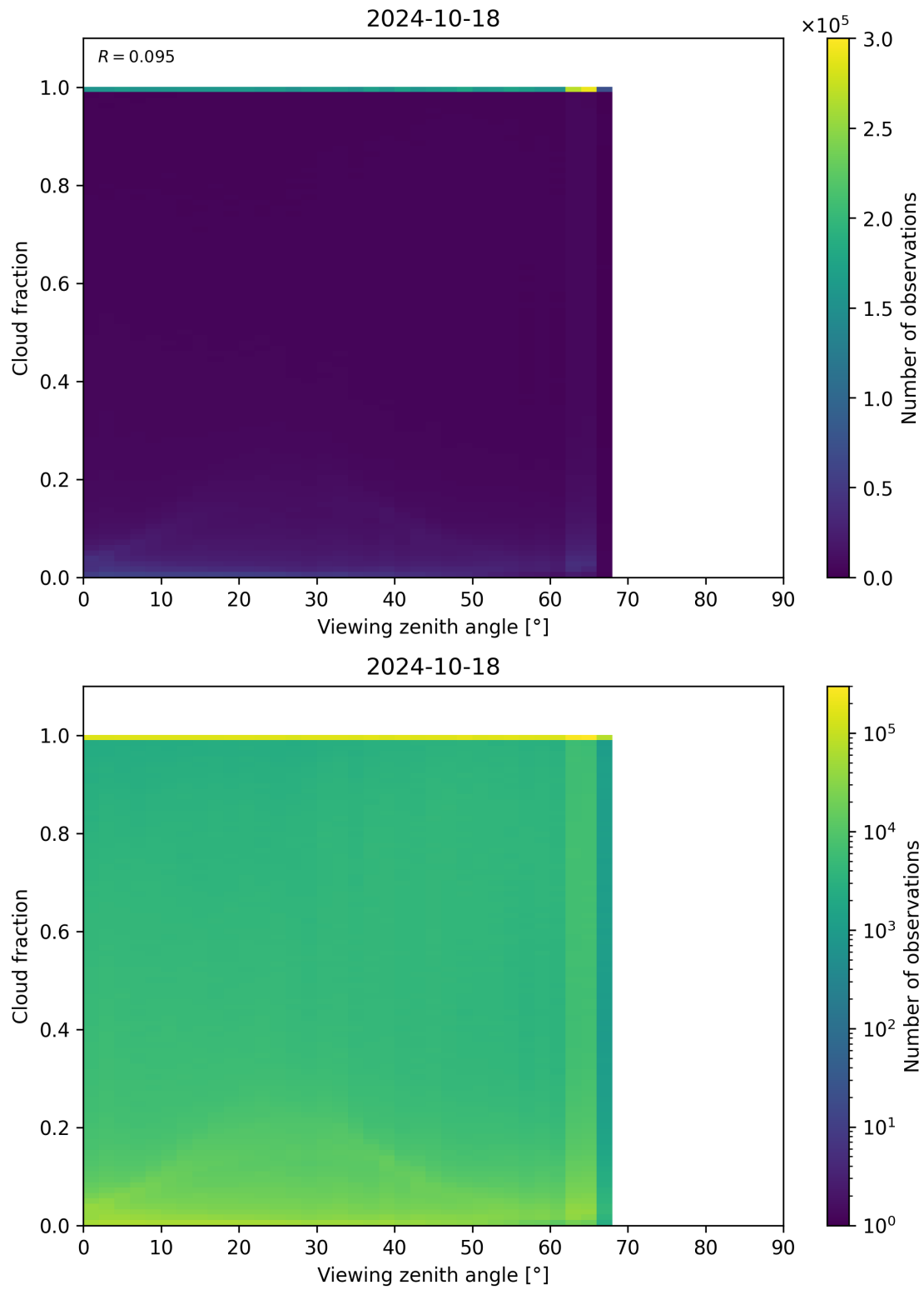
Figure 132: Scatter density plot of “Viewing zenith angle” against “Cloud fraction” for 2024-10-17 to 2024-10-19.
