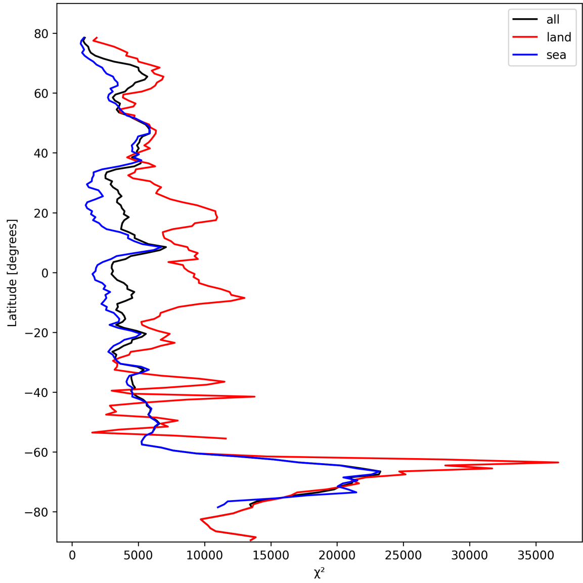
Figure 21: Zonal average of “ \chi^2 ” for 2024-10-17 to 2024-10-19.
