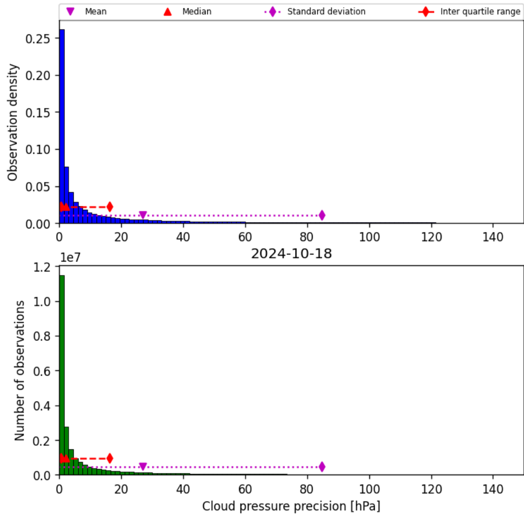
Figure 31: Histogram of “Cloud pressure precision” for 2024-10-17 to 2024-10-19
