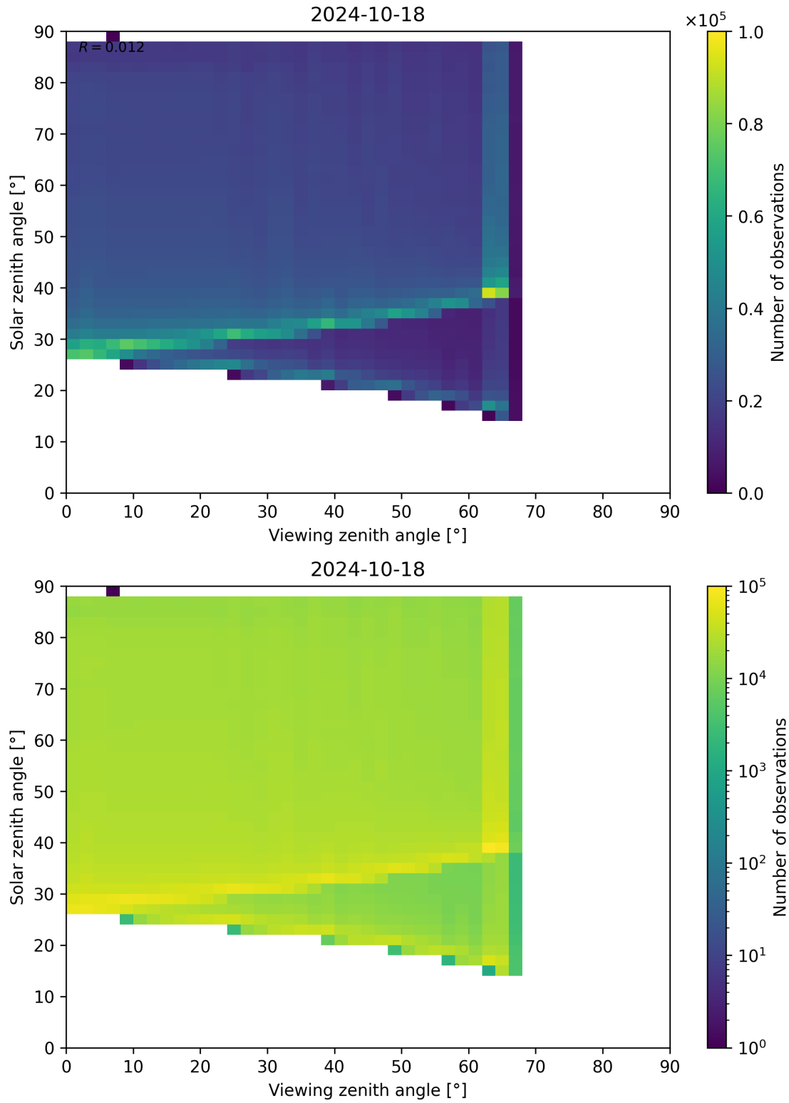
Figure 139: Scatter density plot of “Viewing zenith angle” against “Solar zenith angle” for 2024-10-17 to 2024-10-19.
