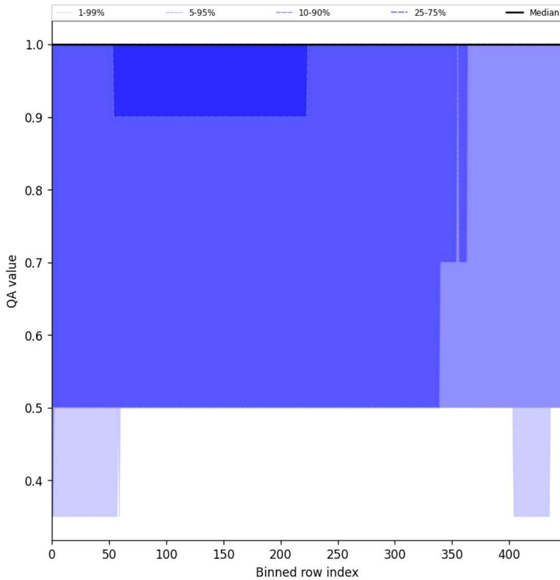
Figure 46: Along track statistics of “QA value” for 2024-10-17 to 2024-10-19
