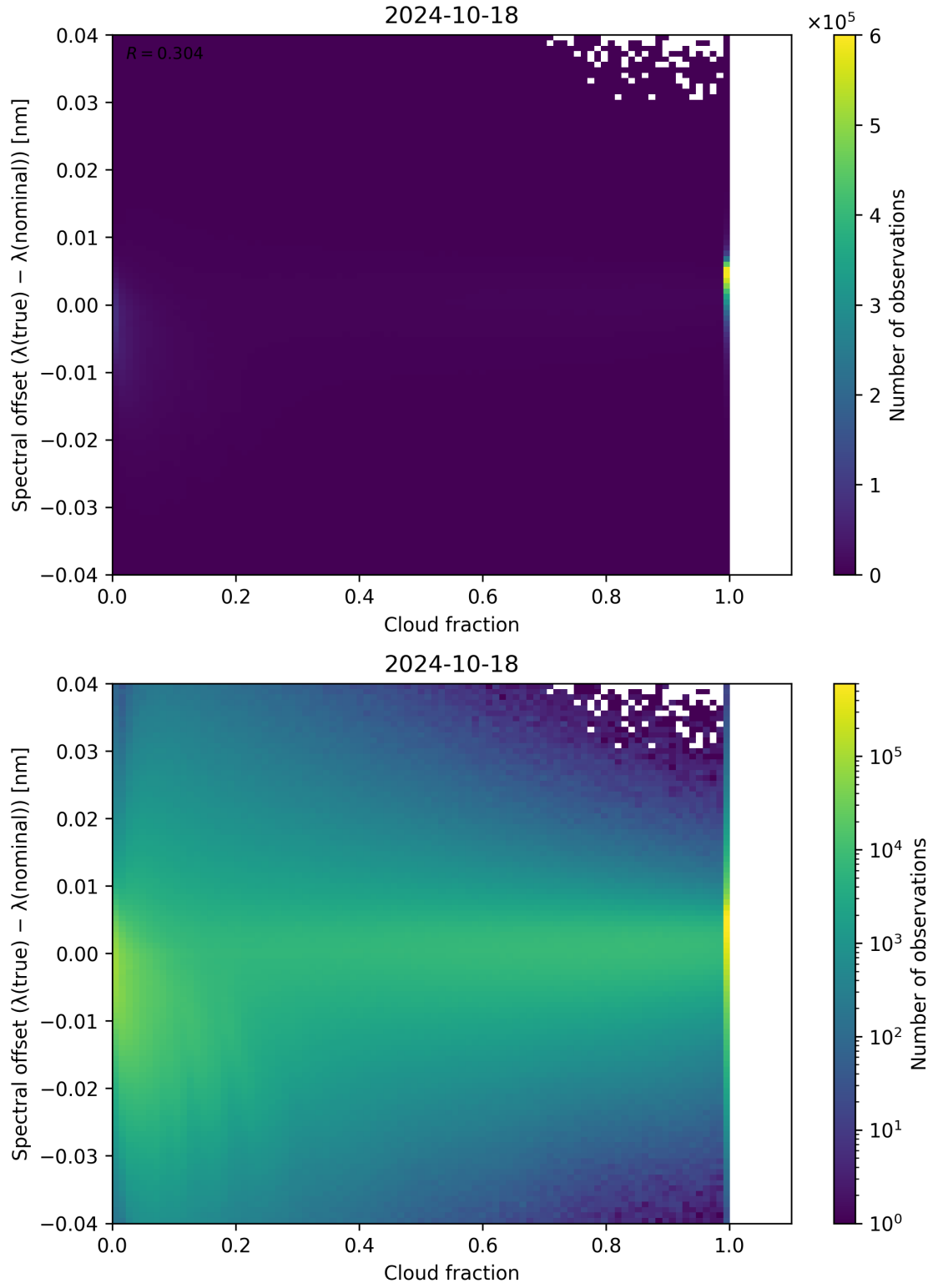
Figure 83: Scatter density plot of “Cloud fraction” against “Spectral offset ( \lambda_{\text{true}} - \lambda_{\text{nominal}} )” for 2024-10-17 to 2024-10-19.
