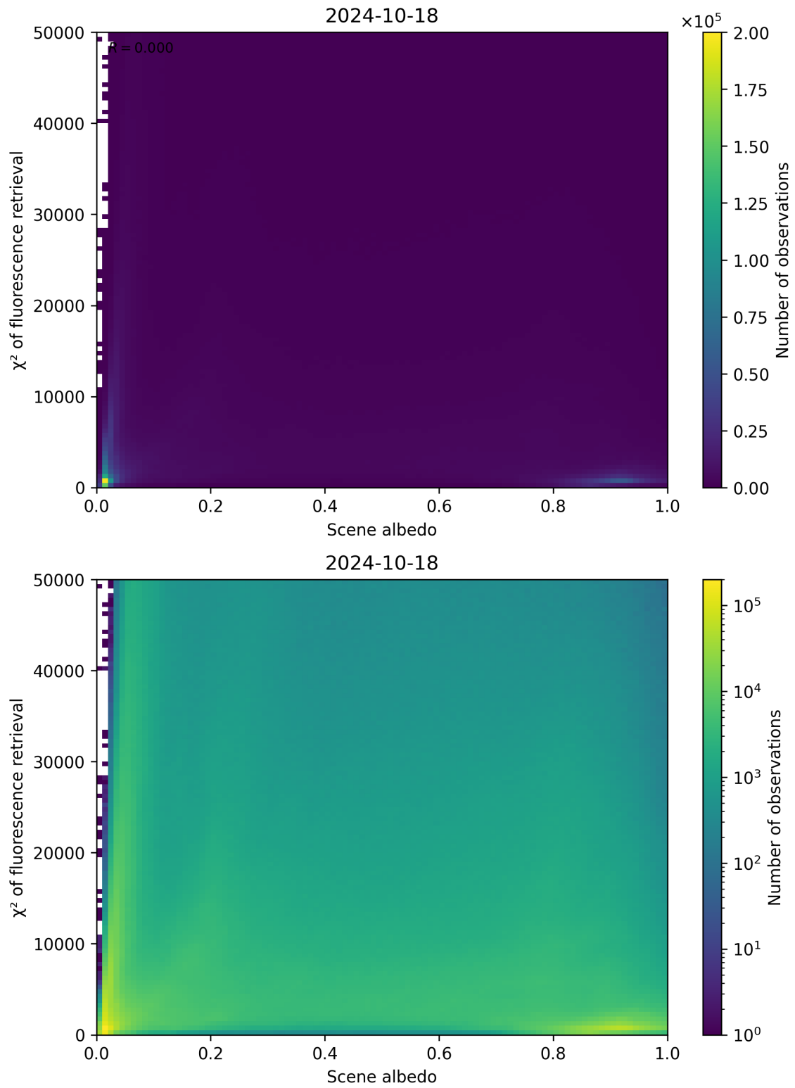
Figure 113: Scatter density plot of “Scene albedo” against “ \chi^2 of fluorescence retrieval” for 2024-10-17 to 2024-10-19.
