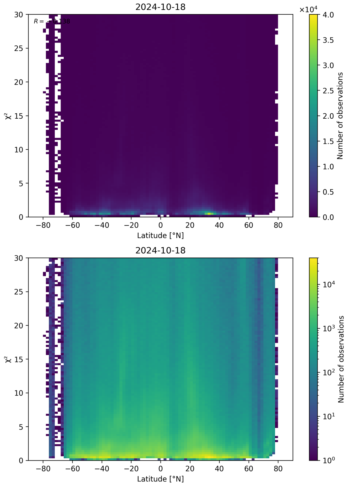
Figure 97: Scatter density plot of “Latitude” against “ \chi^2 ” for 2024-10-17 to 2024-10-19.
