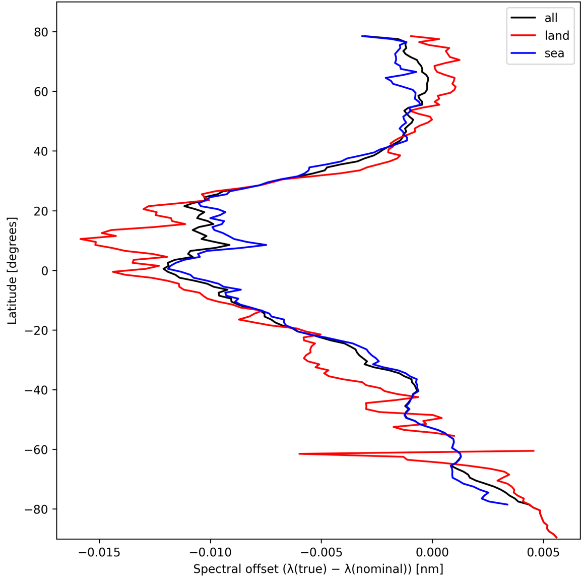
Figure 28: Zonal average of “Spectral offset ( \lambda_{\text{true}} - \lambda_{\text{nominal}} )” for 2024-10-17 to 2024-10-19.
