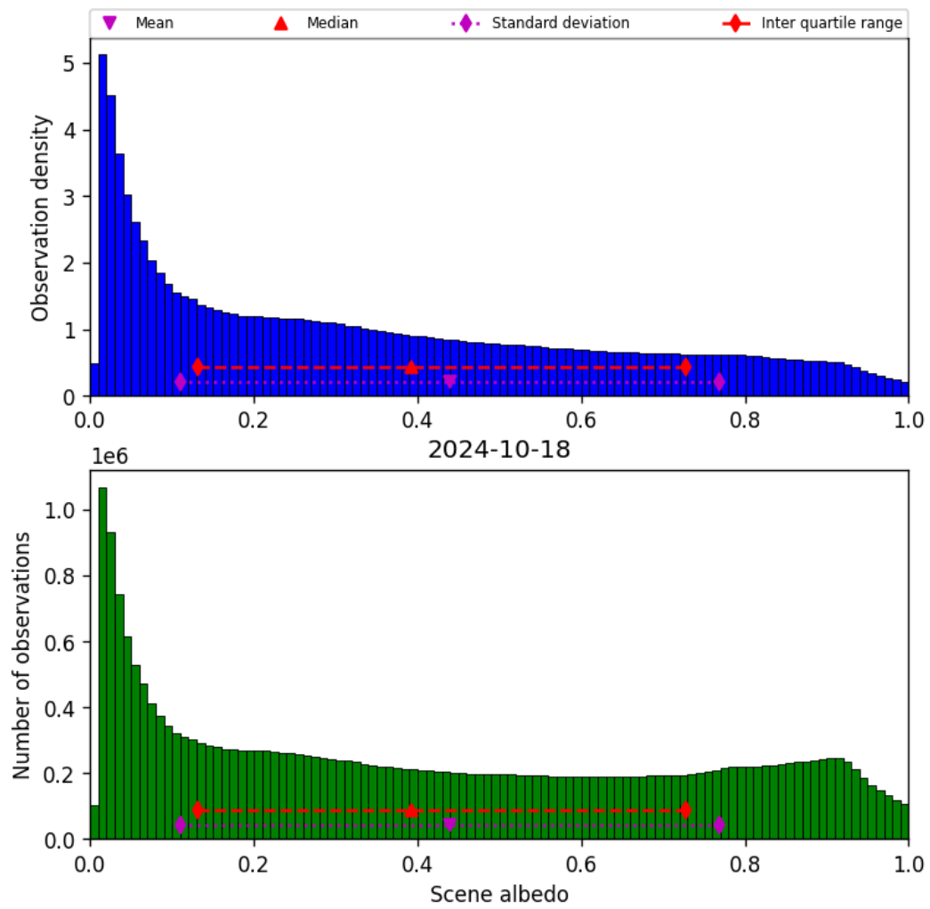
Figure 34: Histogram of “Scene albedo” for 2024-10-17 to 2024-10-19
