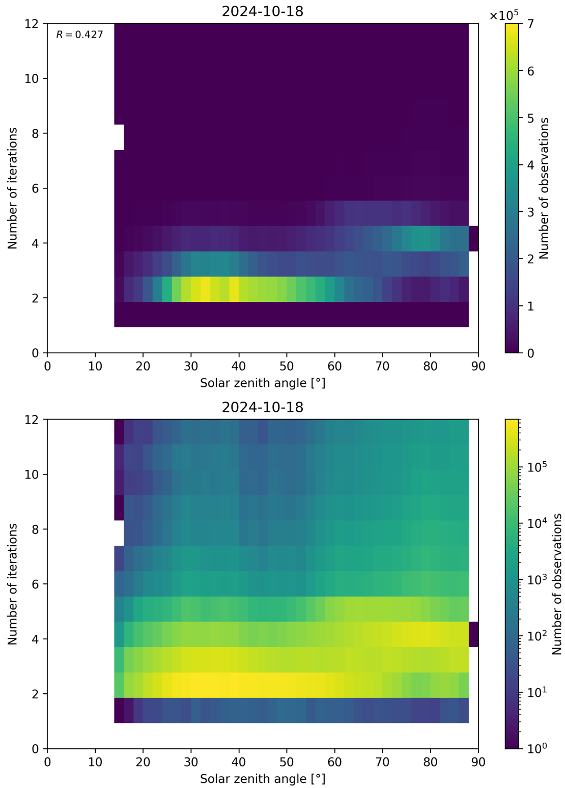
Figure 125: Scatter density plot of “Solar zenith angle” against “Number of iterations” for 2024-10-17 to 2024-10-19.
