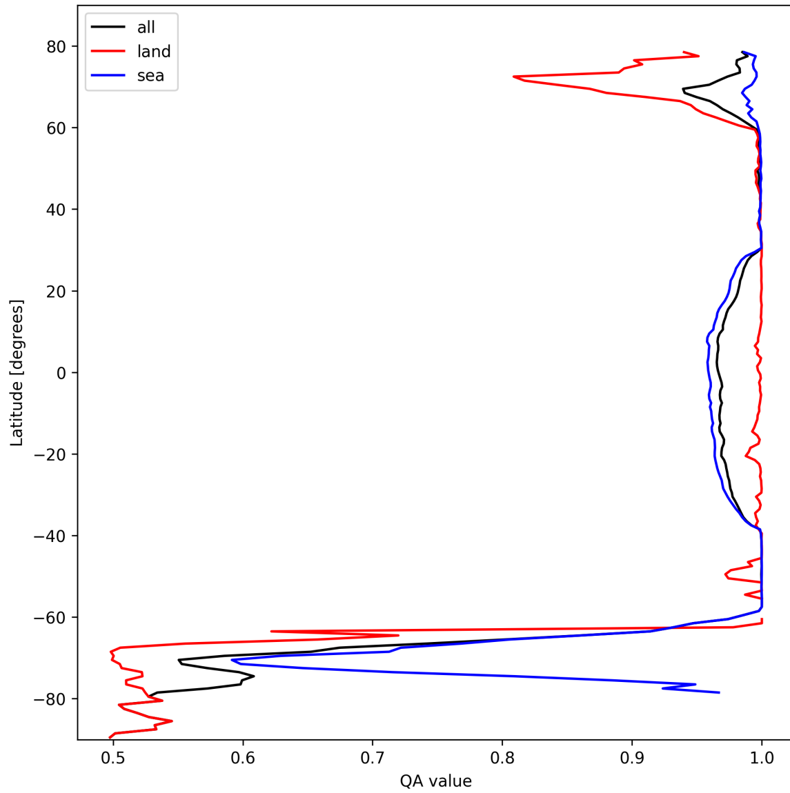
Figure 12: Zonal average of “QA value” for 2024-10-17 to 2024-10-19.
