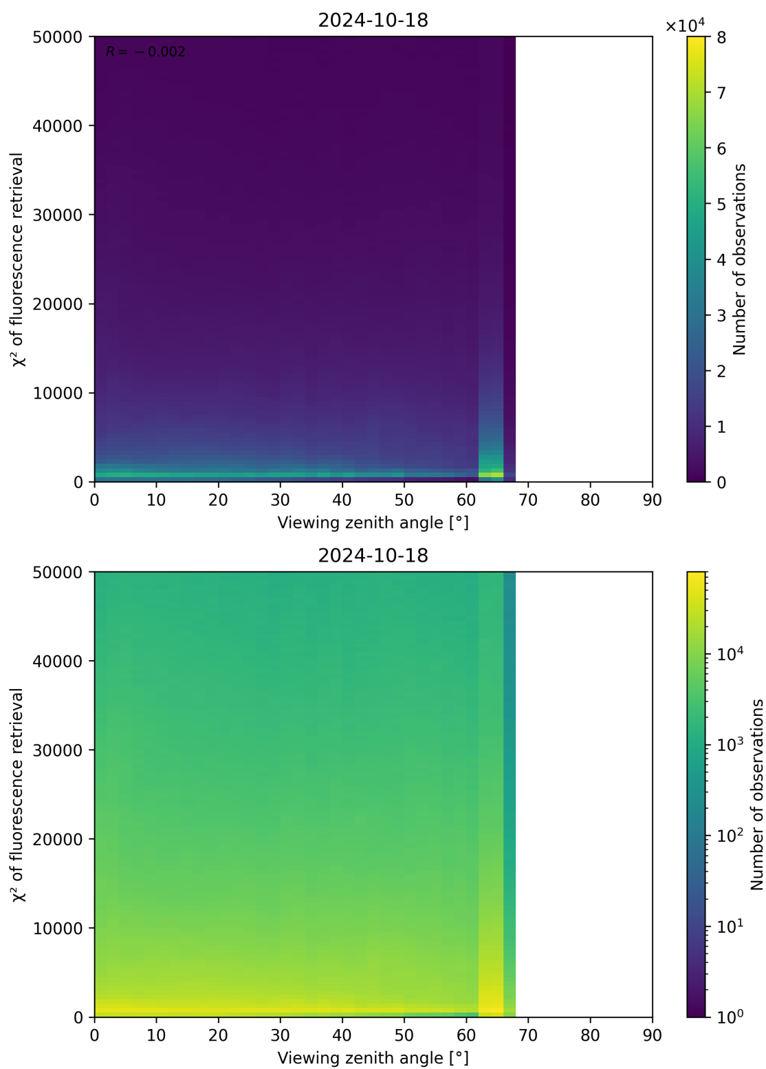
Figure 131: Scatter density plot of “Viewing zenith angle” against “ \chi^2 of fluorescence retrieval” for 2024-10-17 to 2024-10-19.
