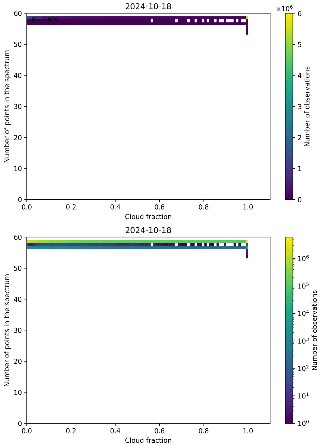
Figure 81: Scatter density plot of “Cloud fraction” against “Number of points in the spectrum” for 2024-10-17 to 2024-10-19.
