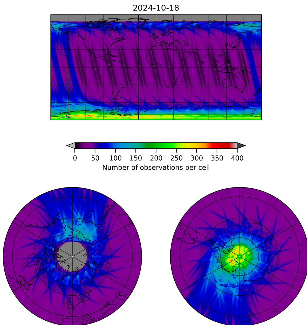
Figure 11: Map of the number of observations for 2024-10-17 to 2024-10-19
