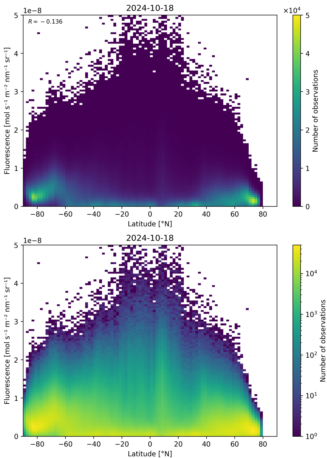
Figure 101: Scatter density plot of “Latitude” against “Fluorescence” for 2024-10-17 to 2024-10-19.
