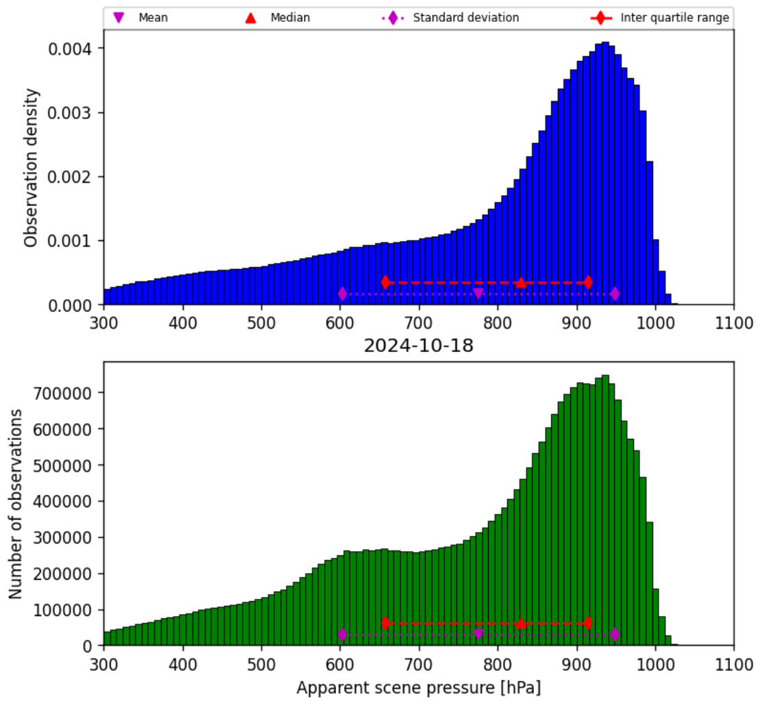
Figure 36: Histogram of “Apparent scene pressure” for 2024-10-17 to 2024-10-19
