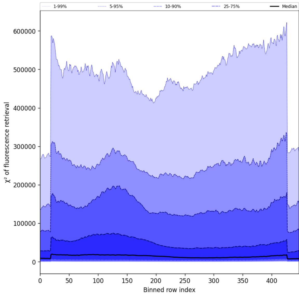
Figure 59: Along track statistics of “ \chi^2 of fluorescence retrieval” for 2024-10-17 to 2024-10-19
