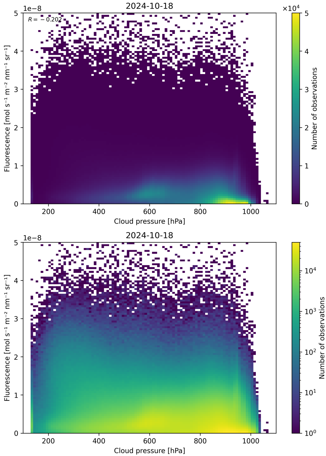
Figure 88: Scatter density plot of “Cloud pressure” against “Fluorescence” for 2024-10-17 to 2024-10-19.
