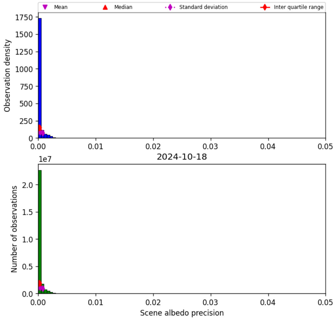
Figure 35: Histogram of “Scene albedo precision” for 2024-10-17 to 2024-10-19
