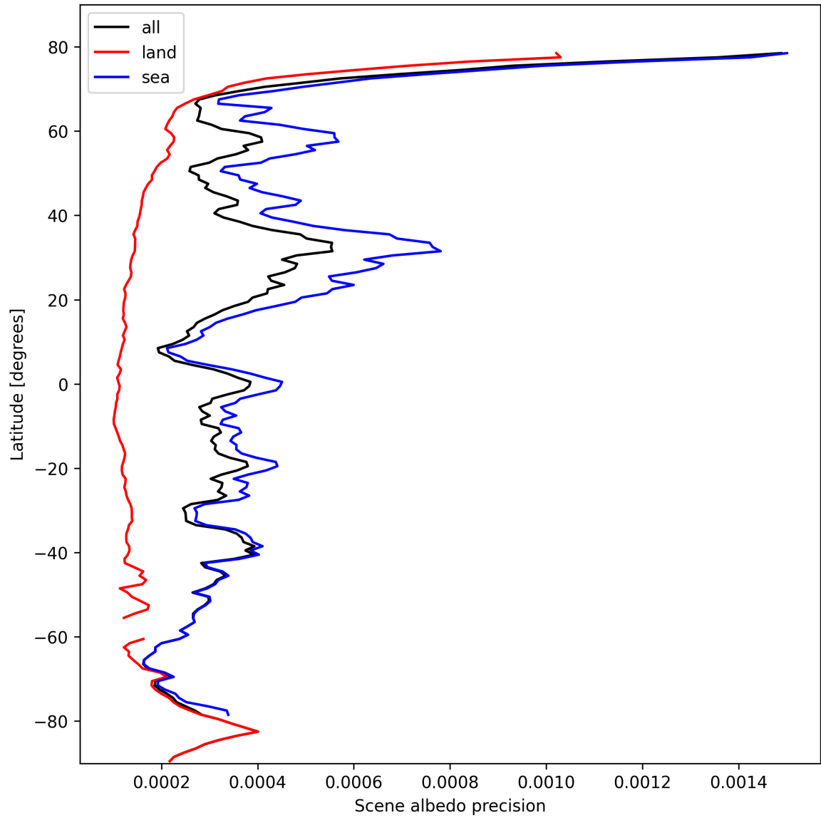
Figure 18: Zonal average of "Scene albedo precision" for 2024-10-17 to 2024-10-19.
