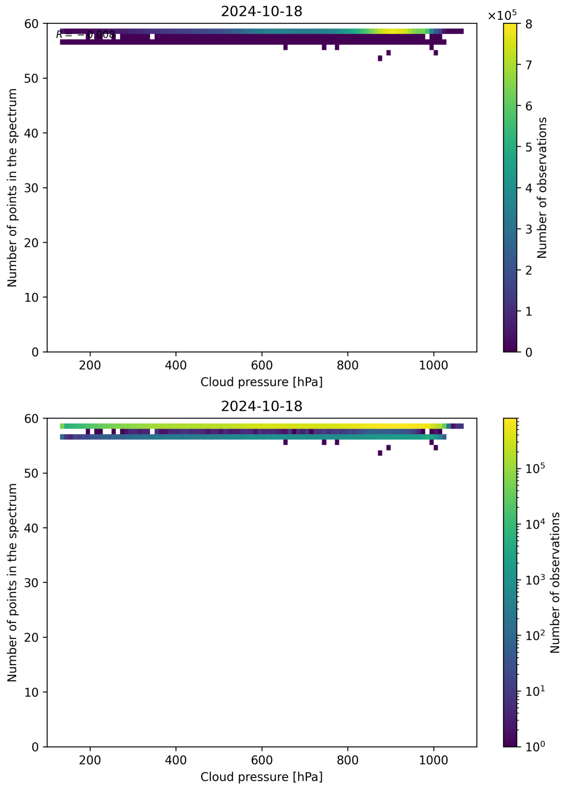
Figure 90: Scatter density plot of “Cloud pressure” against “Number of points in the spectrum” for 2024-10-17 to 2024-10-19.
