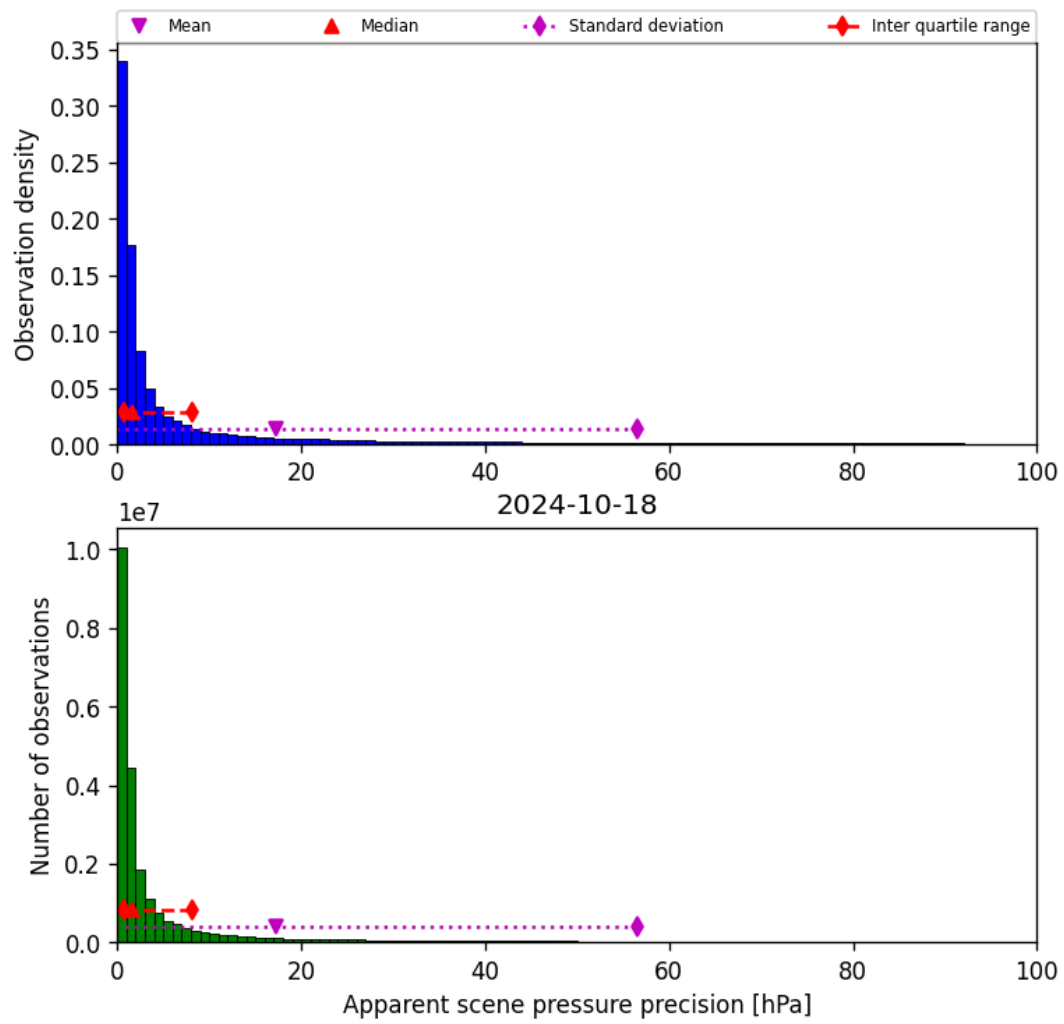
Figure 37: Histogram of “Apparent scene pressure precision” for 2024-10-17 to 2024-10-19
