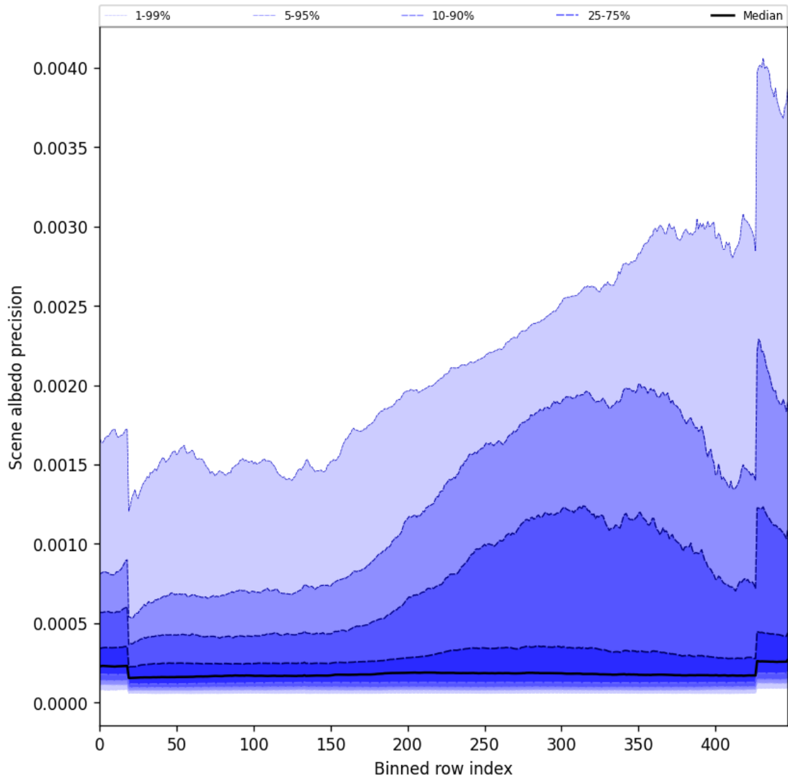
Figure 52: Along track statistics of “Scene albedo precision” for 2024-10-17 to 2024-10-19
