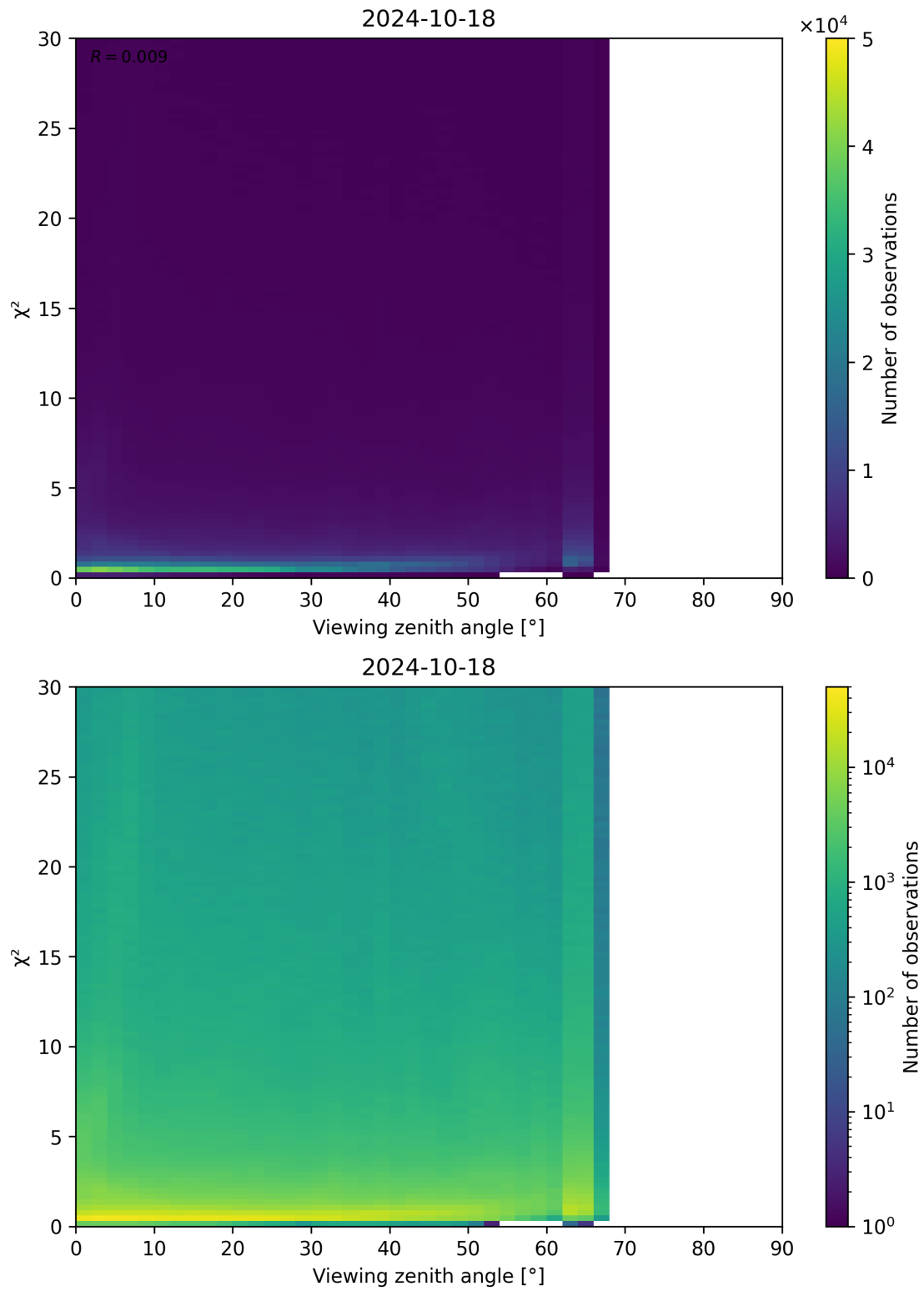
Figure 130: Scatter density plot of “Viewing zenith angle” against “ \chi^2 ” for 2024-10-17 to 2024-10-19.
