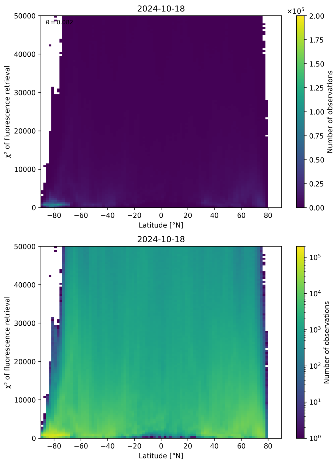
Figure 98: Scatter density plot of “Latitude” against “ \chi^2 of fluorescence retrieval” for 2024-10-17 to 2024-10-19.
