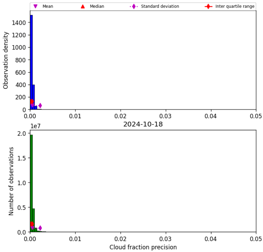
Figure 33: Histogram of “Cloud fraction precision” for 2024-10-17 to 2024-10-19
