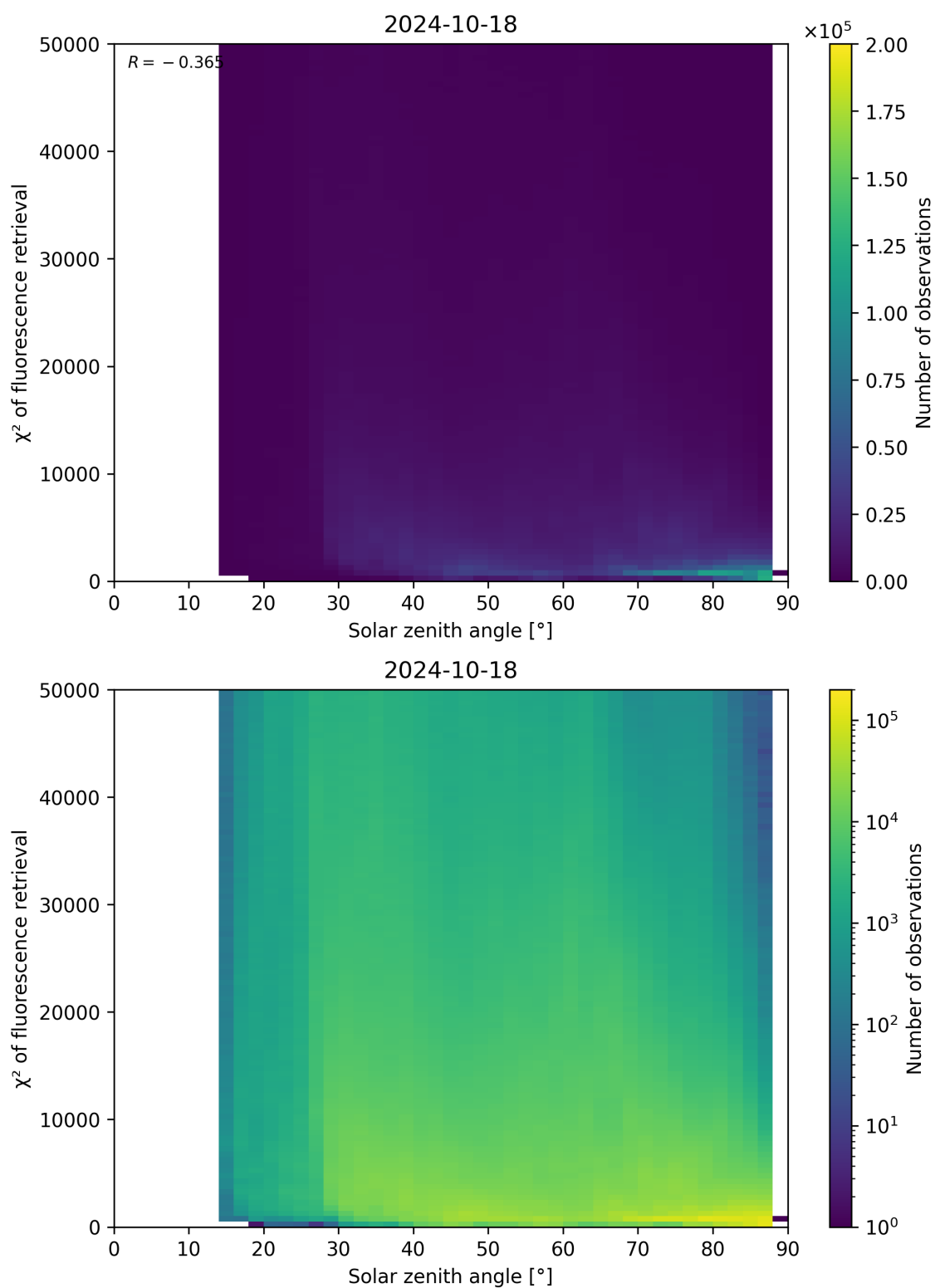
Figure 120: Scatter density plot of “Solar zenith angle” against “ \chi^2 of fluorescence retrieval” for 2024-10-17 to 2024-10-19.
