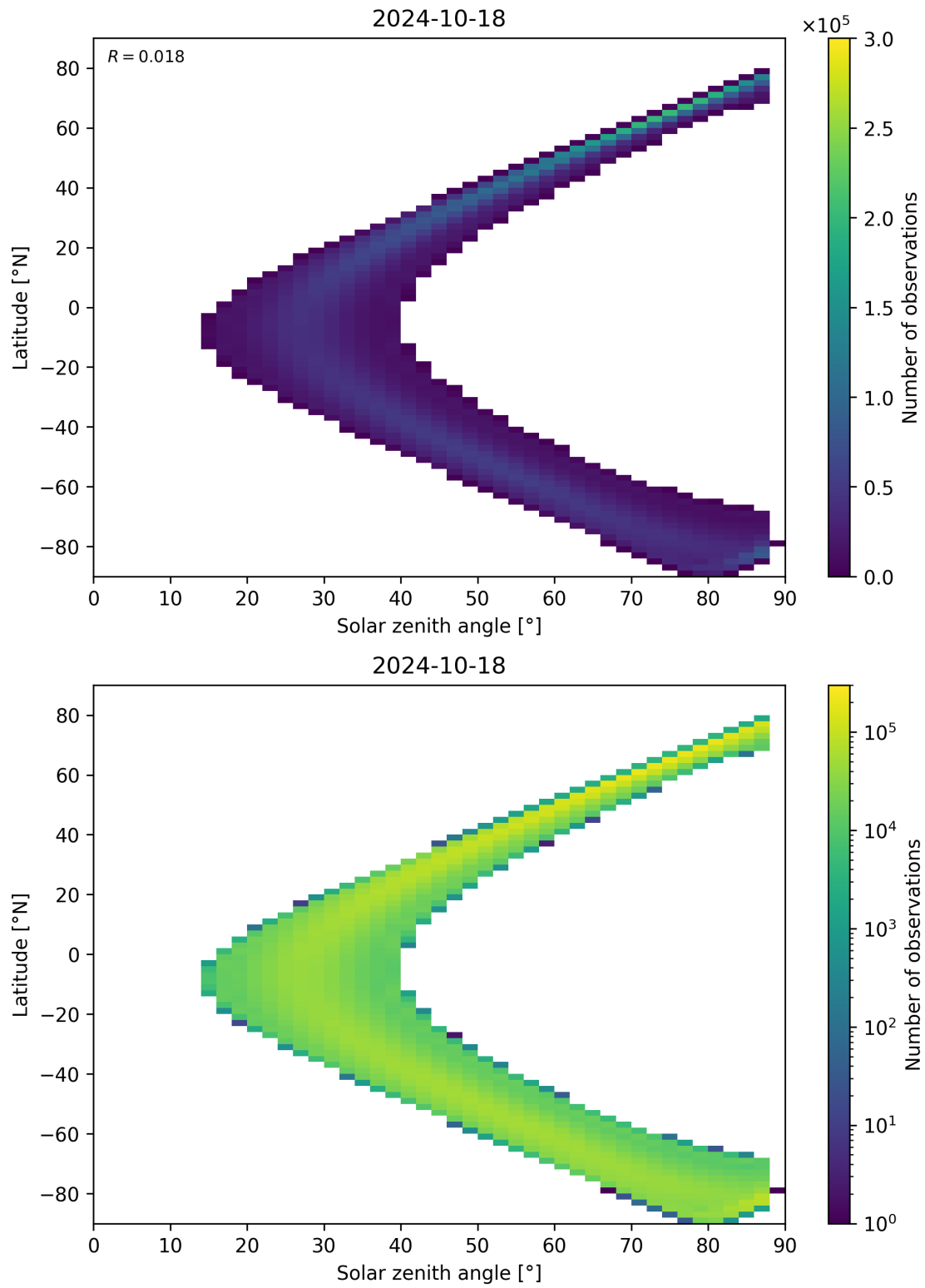
Figure 124: Scatter density plot of “Solar zenith angle” against “Latitude” for 2024-10-17 to 2024-10-19.
