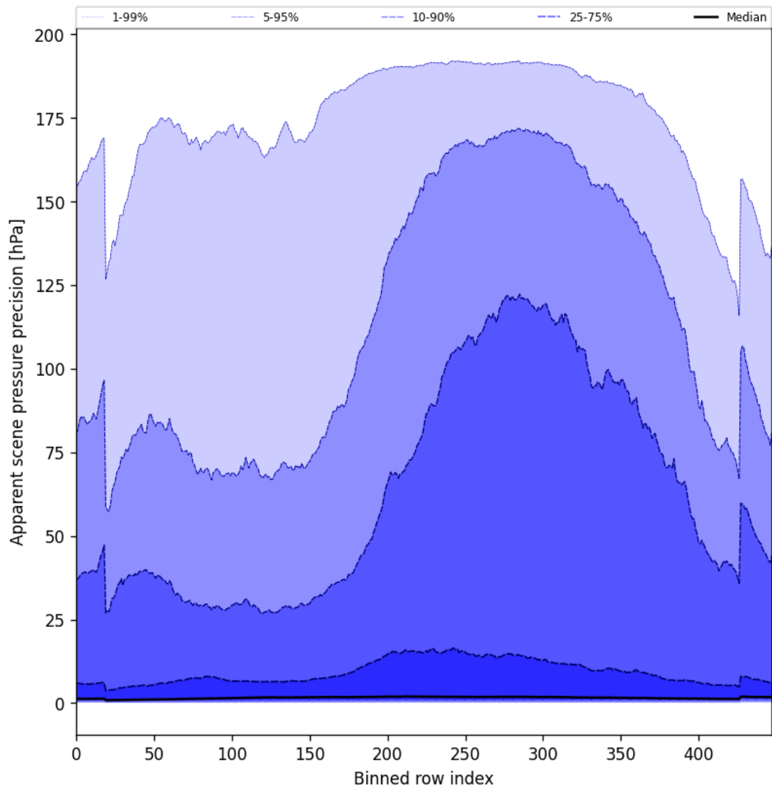
Figure 54: Along track statistics of “Apparent scene pressure precision” for 2024-10-17 to 2024-10-19
