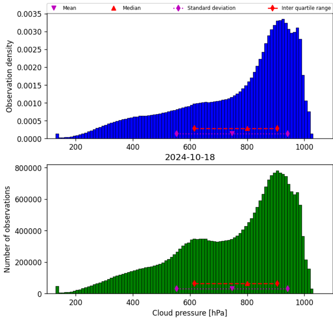
Figure 30: Histogram of “Cloud pressure” for 2024-10-17 to 2024-10-19
