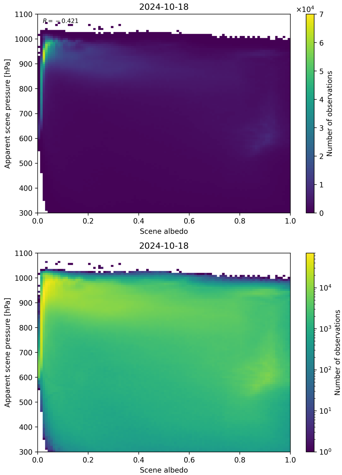
Figure 111: Scatter density plot of “Scene albedo” against “Apparent scene pressure” for 2024-10-17 to 2024-10-19.
