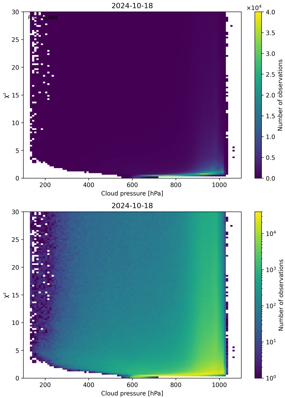
Figure 85: Scatter density plot of “Cloud pressure” against “ \chi^2 ” for 2024-10-17 to 2024-10-19.
