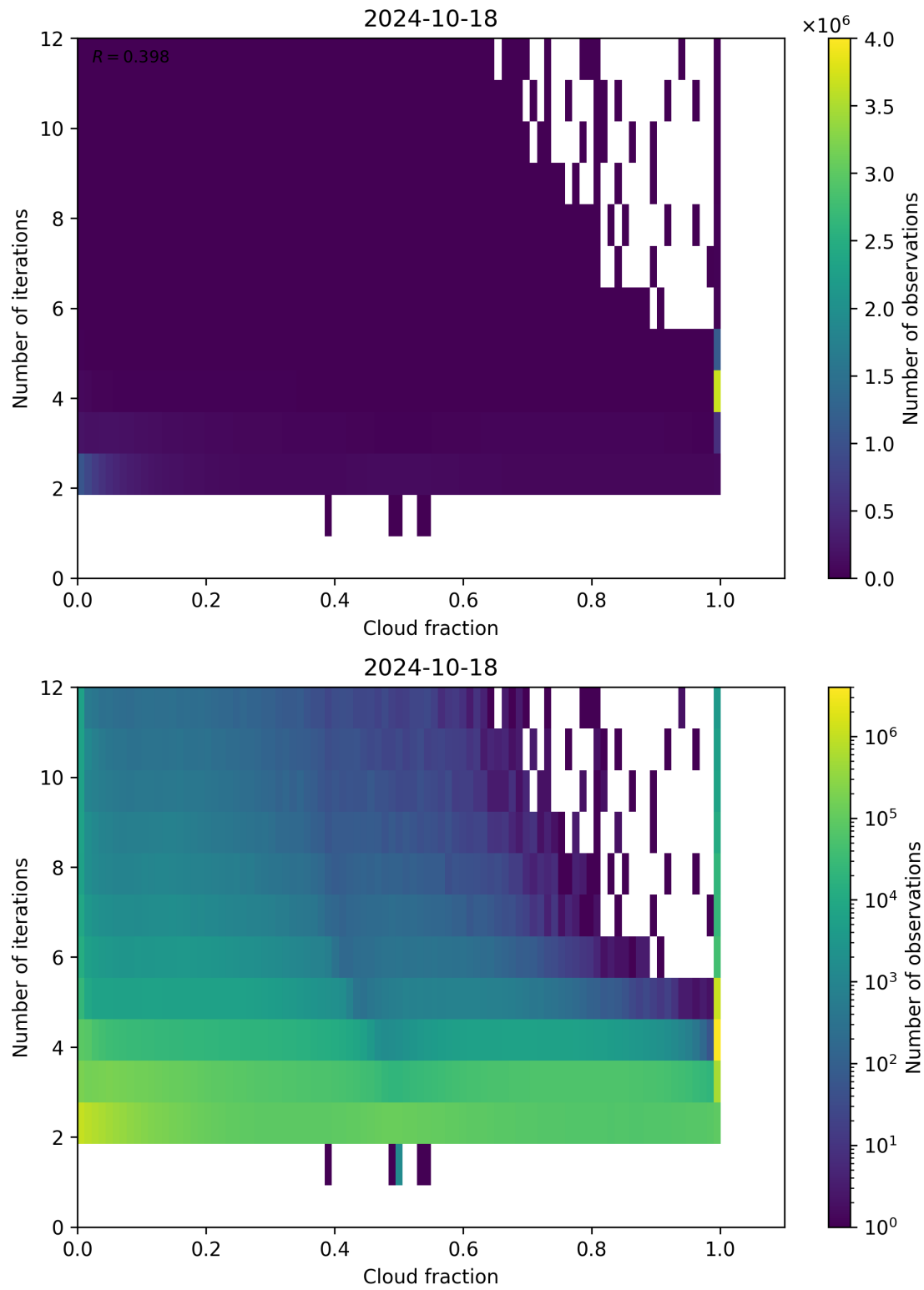
Figure 80: Scatter density plot of “Cloud fraction” against “Number of iterations” for 2024-10-17 to 2024-10-19.
