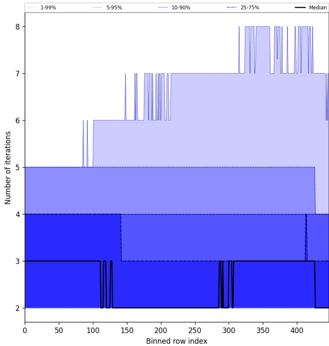
Figure 56: Along track statistics of “Number of iterations” for 2024-10-17 to 2024-10-19
