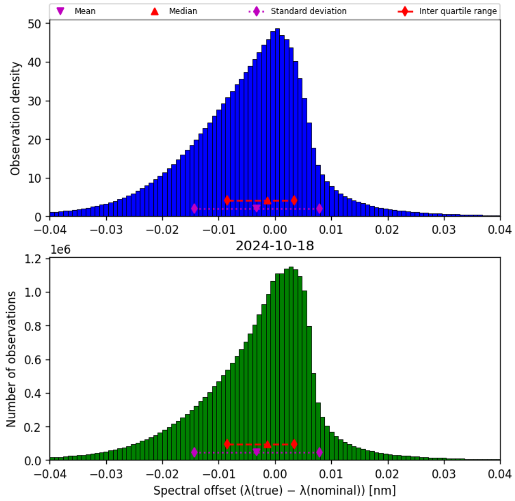
Figure 45: Histogram of “Spectral offset ( \lambda_{\text{true}} - \lambda_{\text{nominal}} )” for 2024-10-17 to 2024-10-19
