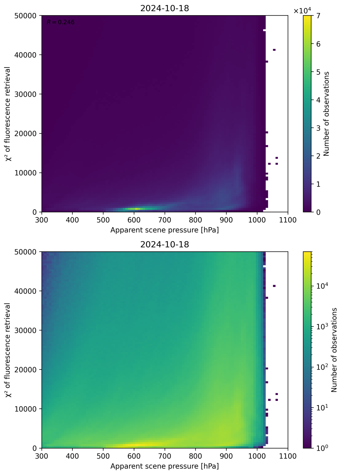
Figure 64: Scatter density plot of “Apparent scene pressure” against “ \chi^2 of fluorescence retrieval” for 2024-10-17 to 2024-10-19.
