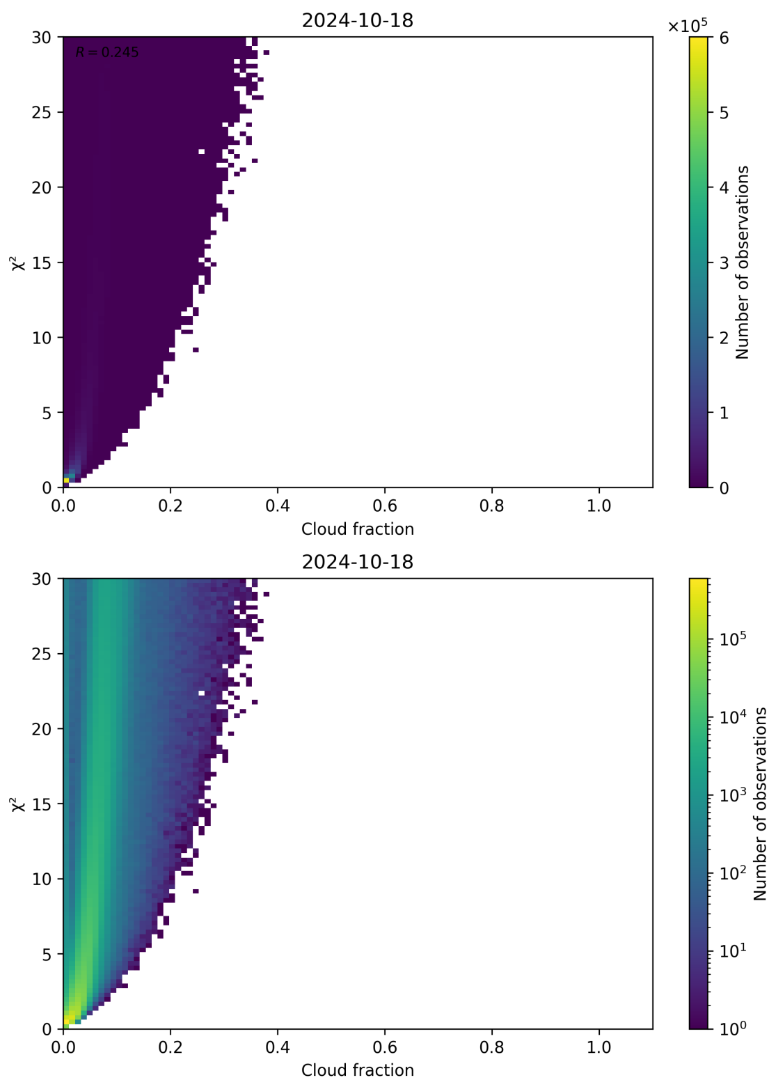
Figure 77: Scatter density plot of “Cloud fraction” against “ \chi^2 ” for 2024-10-17 to 2024-10-19.
