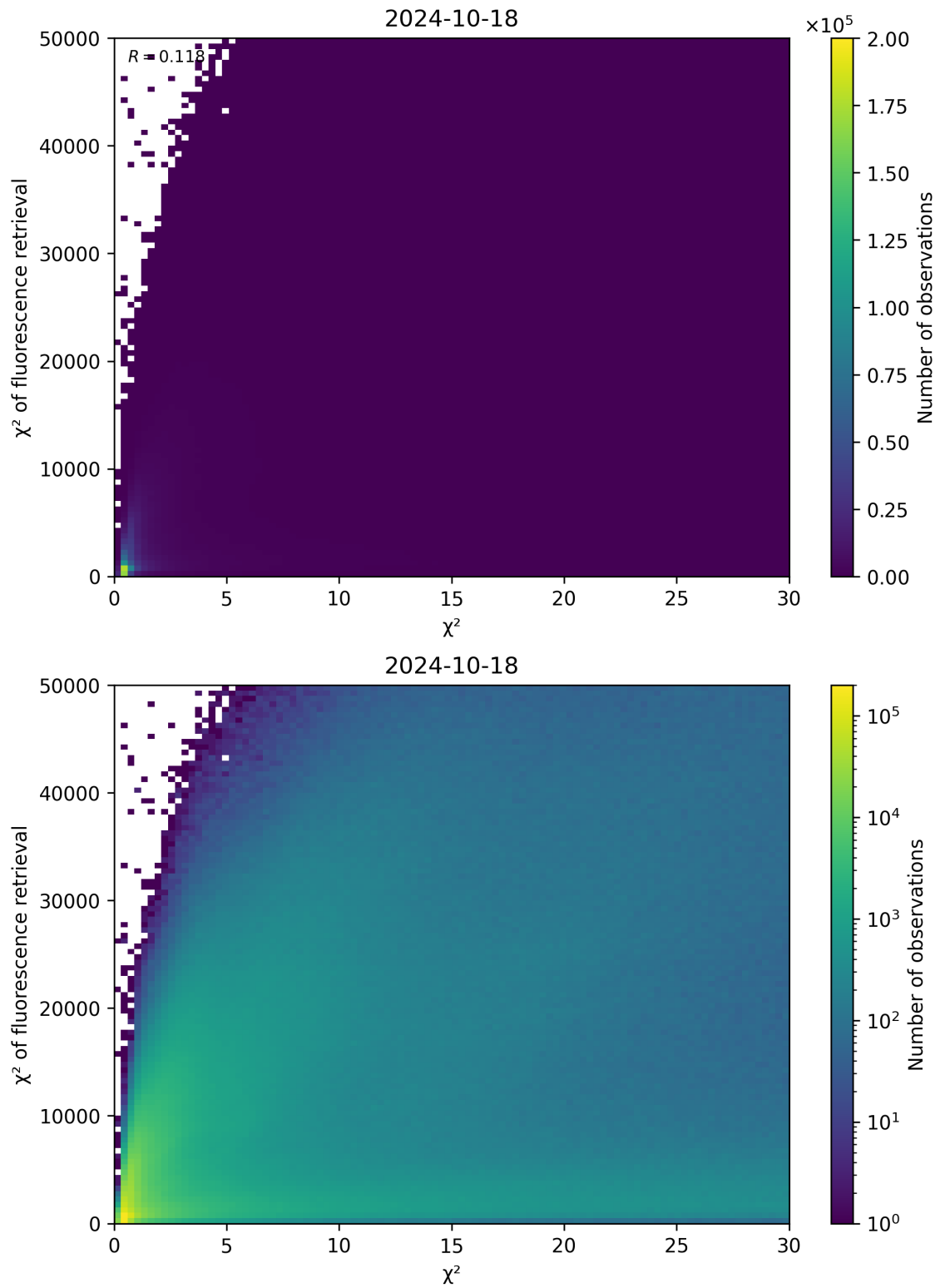
Figure 69: Scatter density plot of “ \chi^2 ” against “ \chi^2 of fluorescence retrieval” for 2024-10-17 to 2024-10-19.
