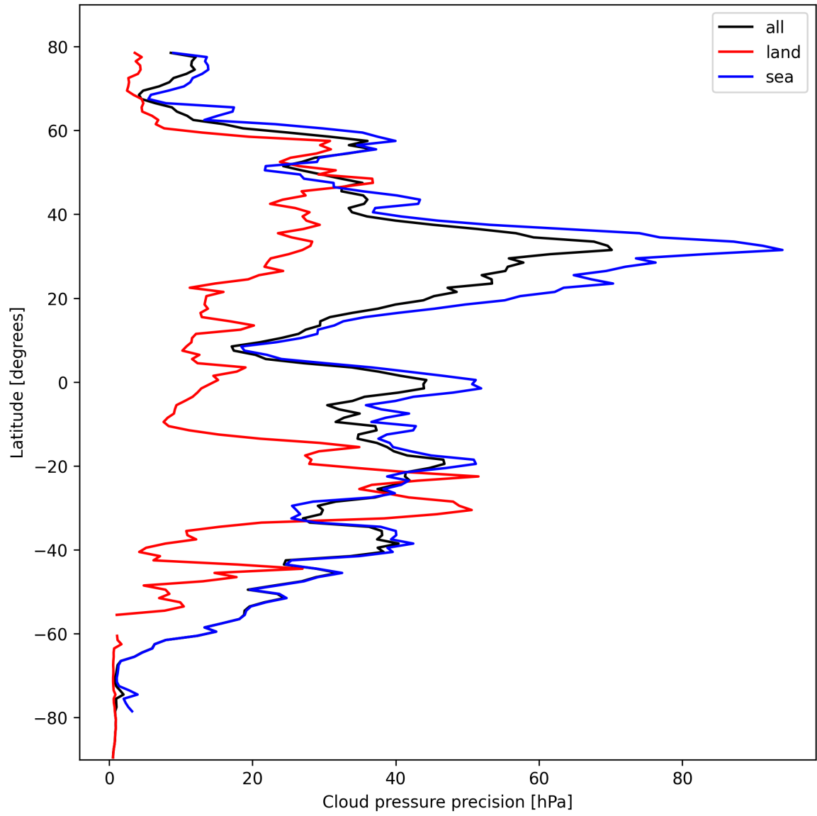
Figure 14: Zonal average of “Cloud pressure precision” for 2024-10-17 to 2024-10-19.
