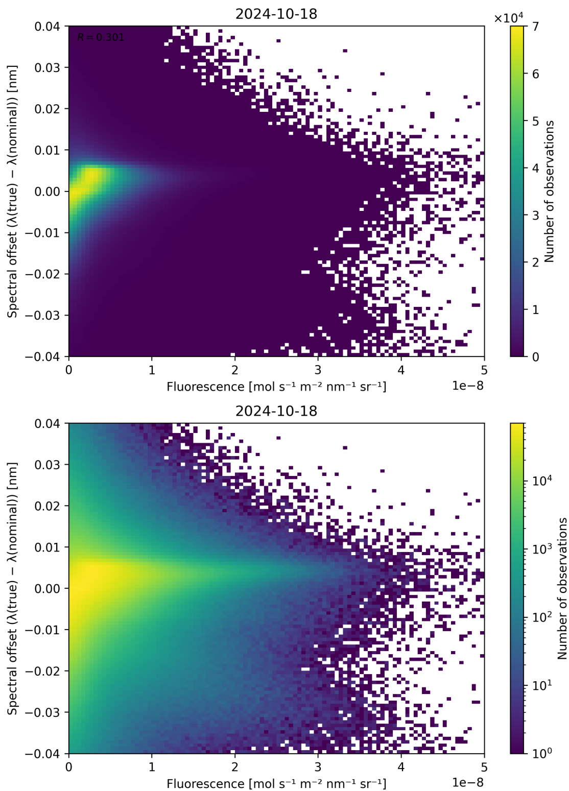
Figure 95: Scatter density plot of “Fluorescence” against “Spectral offset ( \lambda_{\text{true}} - \lambda_{\text{nominal}} )” for 2024-10-17 to 2024-10-19.
