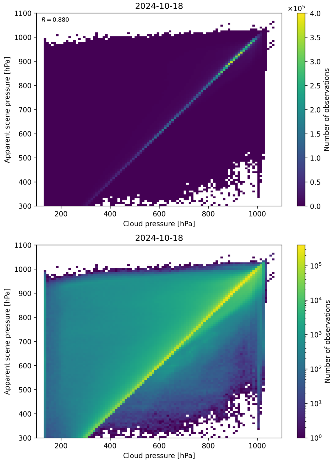
Figure 84: Scatter density plot of “Cloud pressure” against “Apparent scene pressure” for 2024-10-17 to 2024-10-19.
