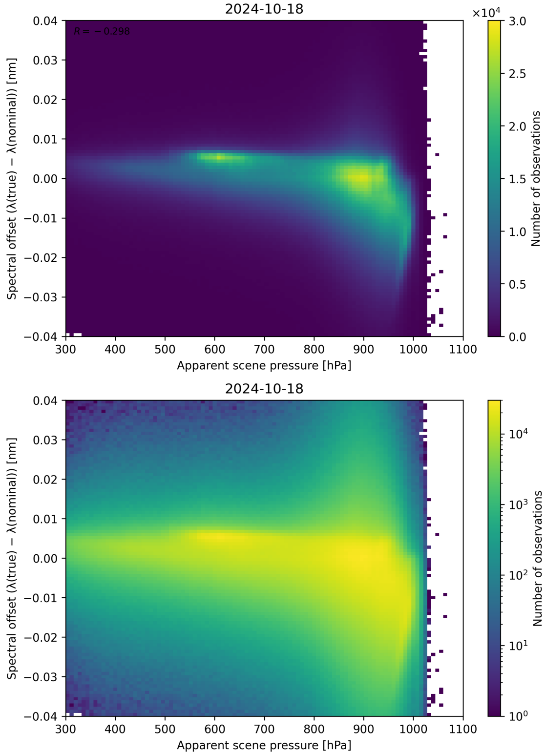
Figure 68: Scatter density plot of “Apparent scene pressure” against “Spectral offset ( \lambda_{\text{true}} - \lambda_{\text{nominal}} )” for 2024-10-17 to 2024-10-19.
