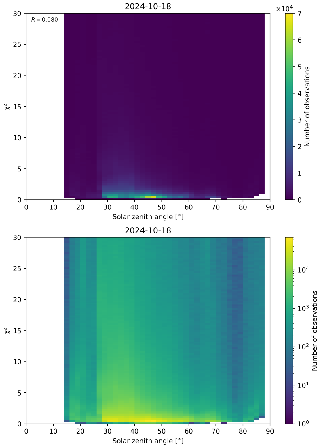
Figure 119: Scatter density plot of “Solar zenith angle” against “ \chi^2 ” for 2024-10-17 to 2024-10-19.
