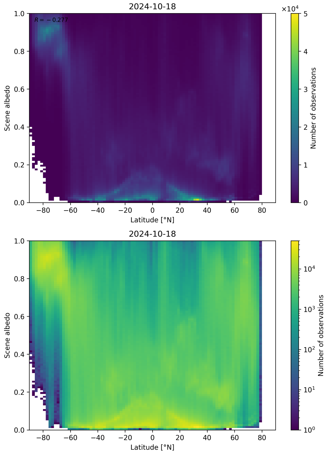
Figure 104: Scatter density plot of “Latitude” against “Scene albedo” for 2024-10-17 to 2024-10-19.
