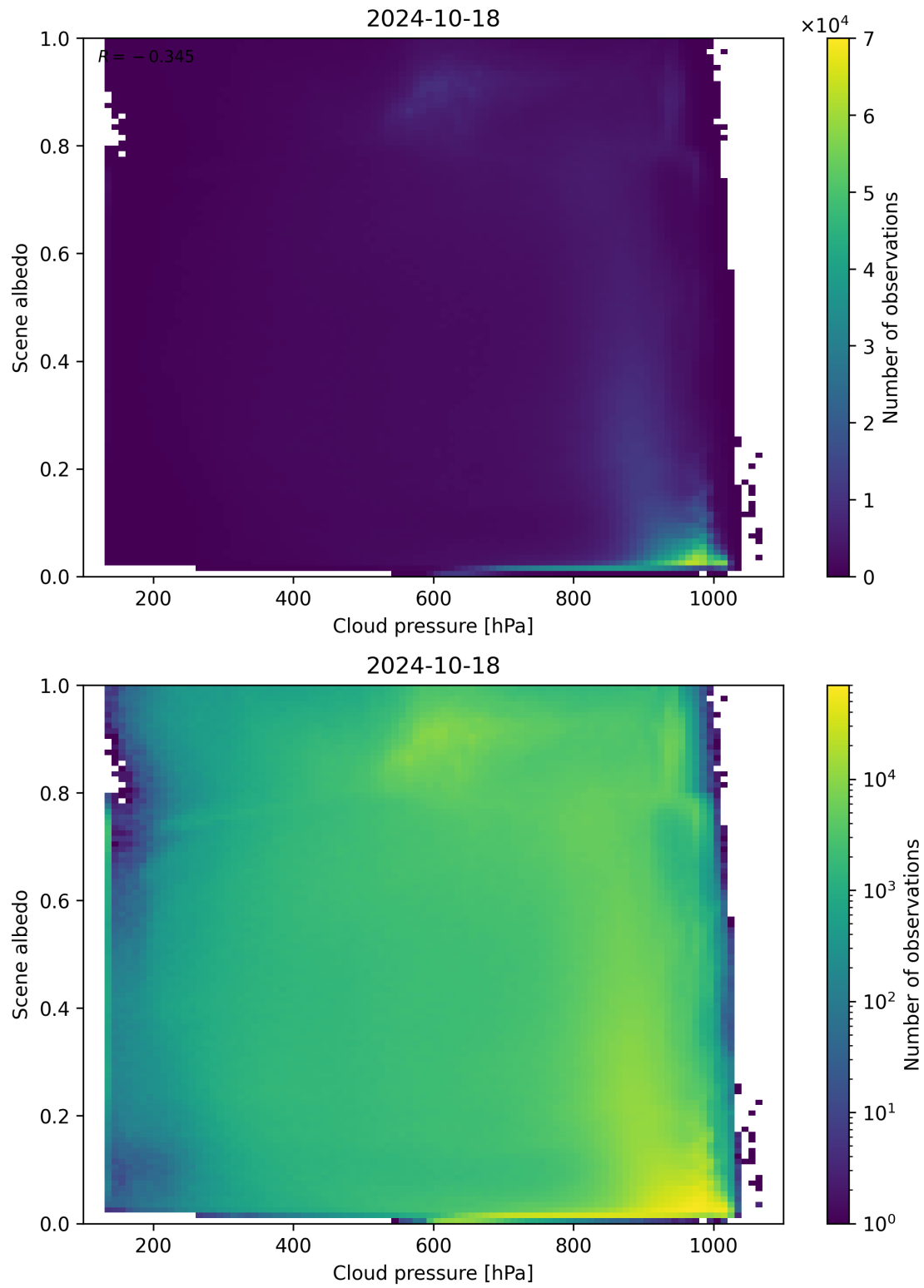
Figure 91: Scatter density plot of “Cloud pressure” against “Scene albedo” for 2024-10-17 to 2024-10-19.
