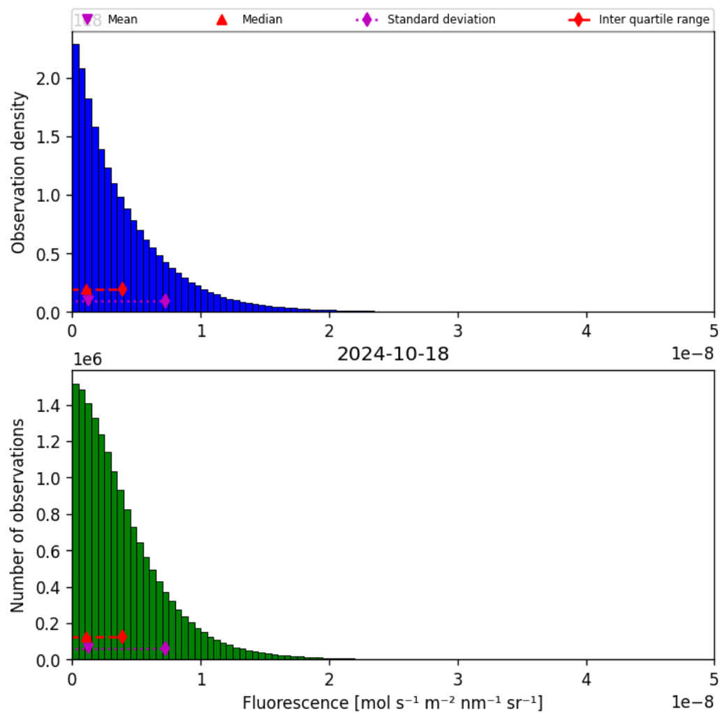
Figure 40: Histogram of “Fluorescence” for 2024-10-17 to 2024-10-19
