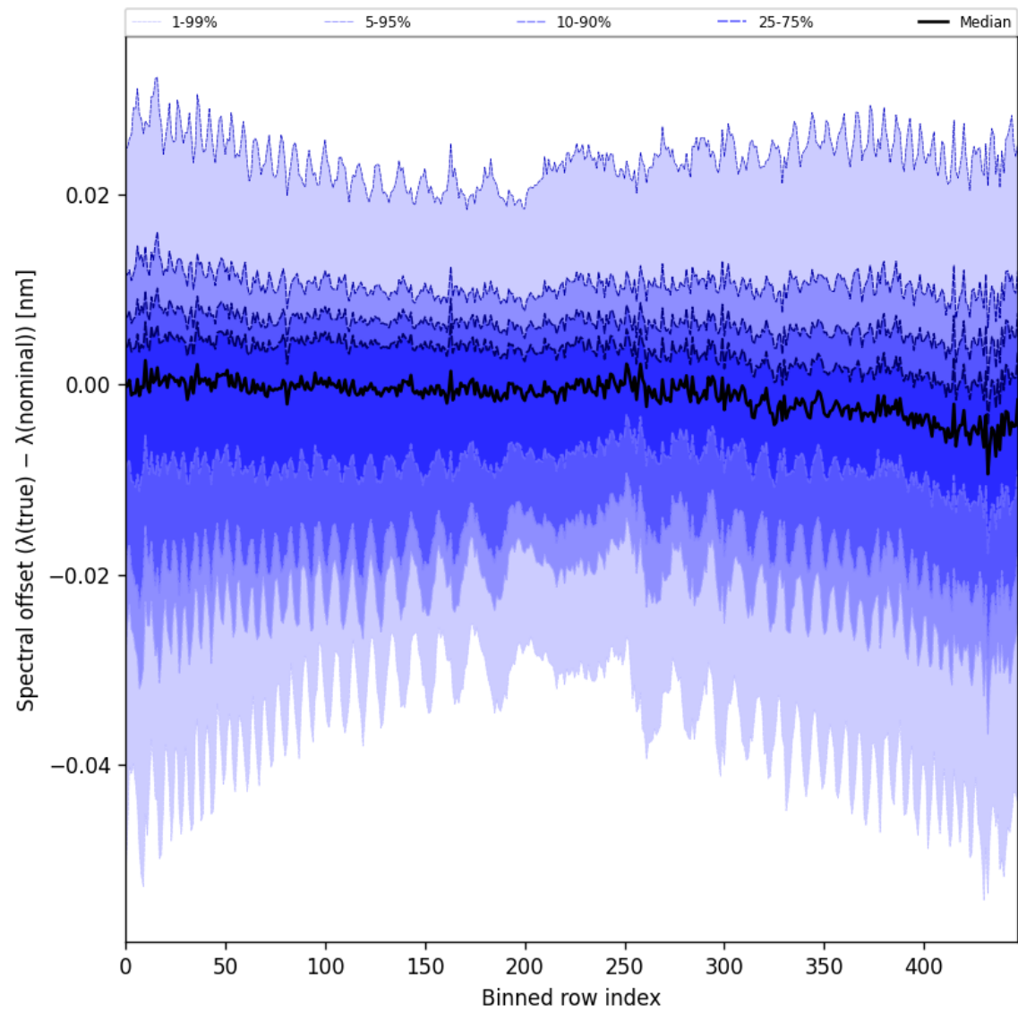
Figure 62: Along track statistics of “Spectral offset ( \lambda_{\text{true}} - \lambda_{\text{nominal}} )” for 2024-10-17 to 2024-10-19
