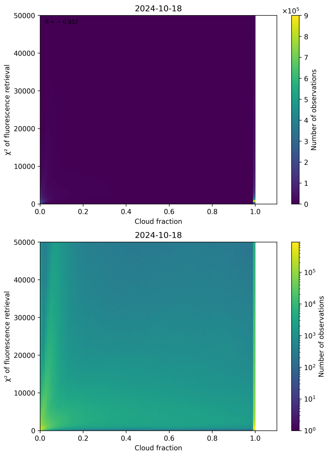
Figure 78: Scatter density plot of “Cloud fraction” against “ \chi^2 of fluorescence retrieval” for 2024-10-17 to 2024-10-19.
