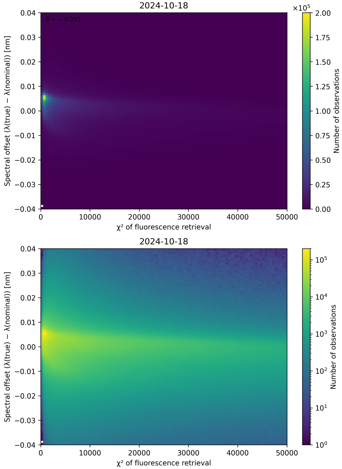
Figure 72: Scatter density plot of “ \chi^2 of fluorescence retrieval” against “Spectral offset ( \lambda_{\text{true}} - \lambda_{\text{nominal}} )” for 2024-10-17 to 2024-10-19.
