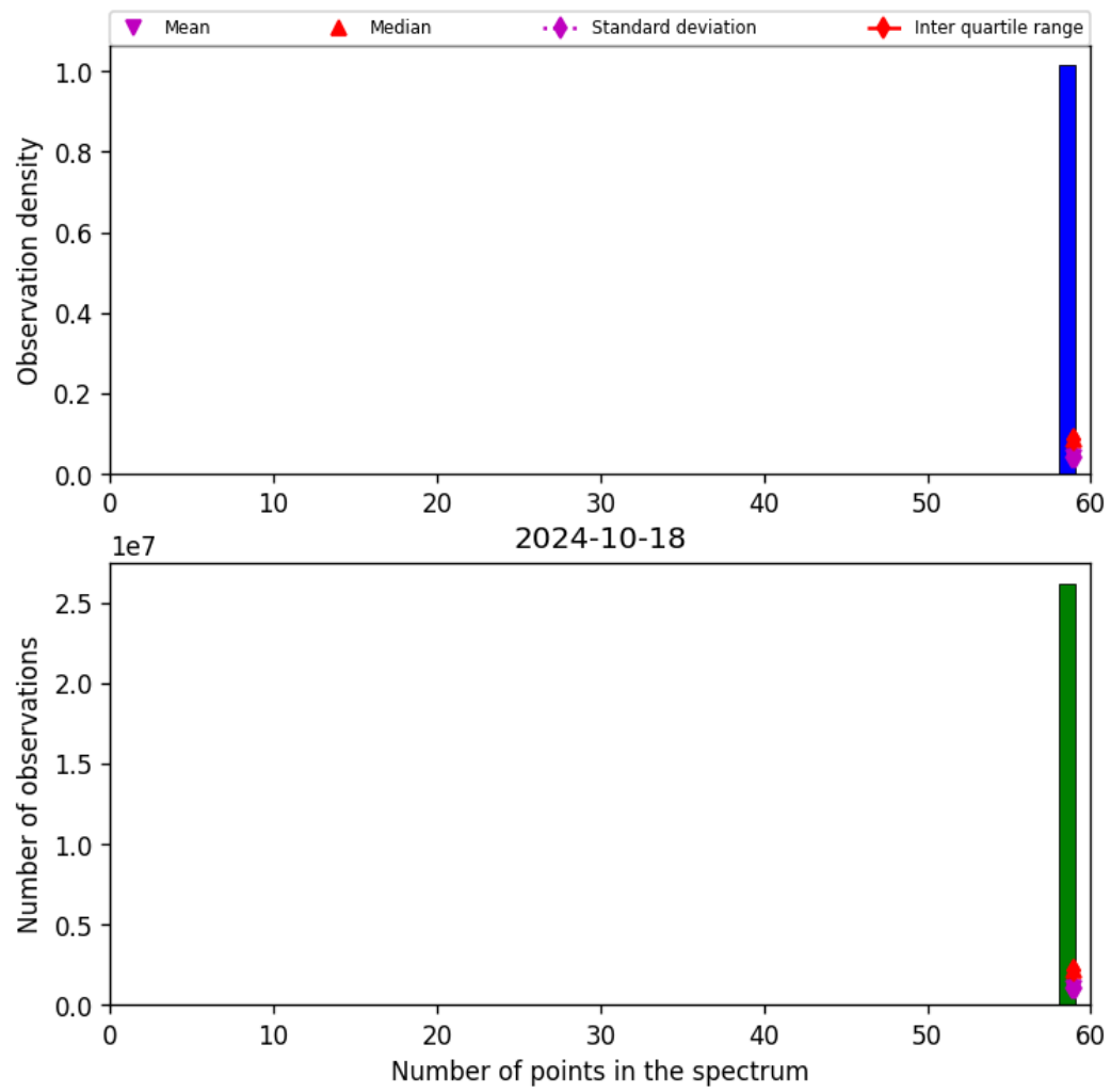
Figure 44: Histogram of “Number of points in the spectrum” for 2024-10-17 to 2024-10-19
