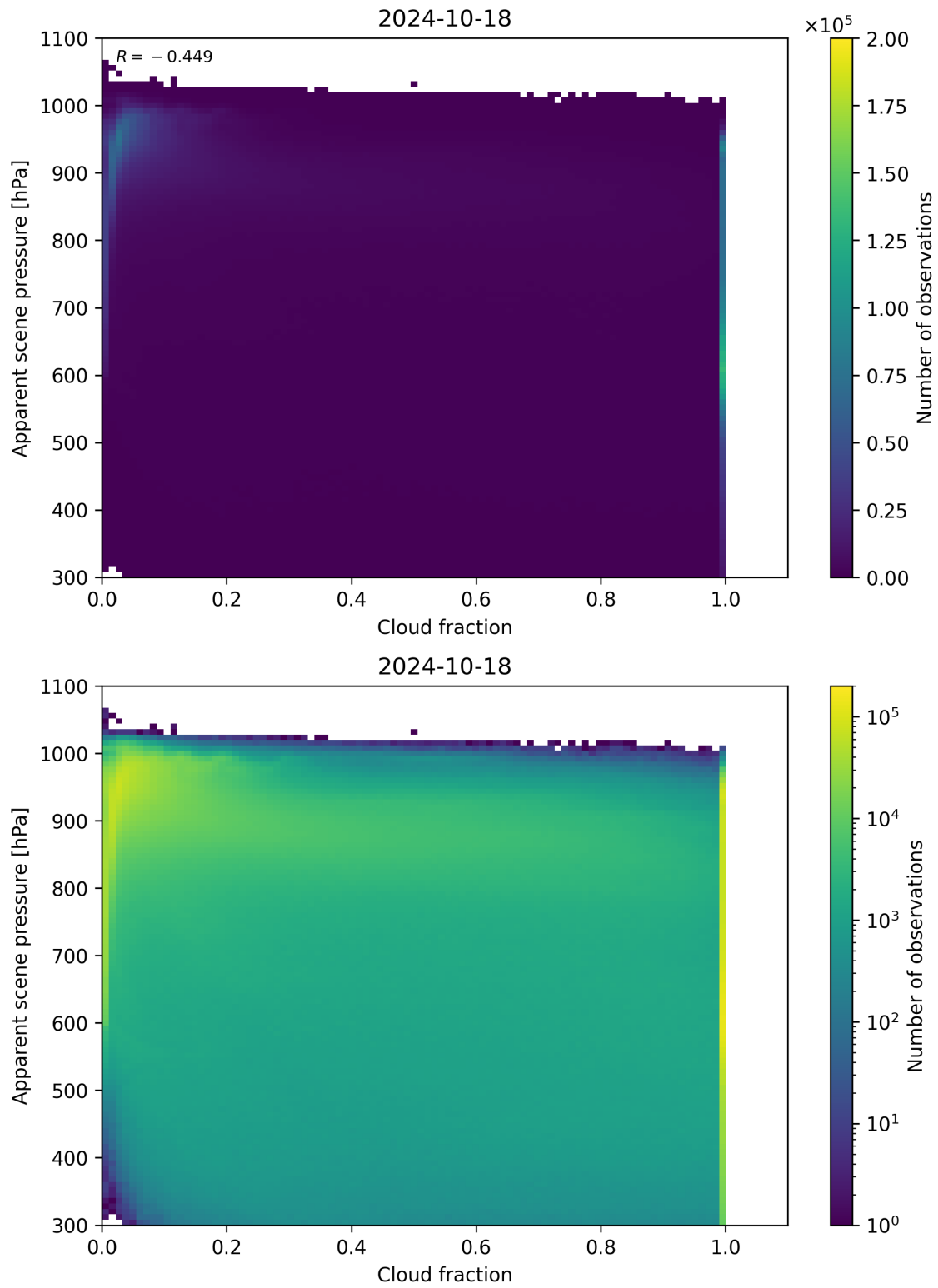
Figure 76: Scatter density plot of “Cloud fraction” against “Apparent scene pressure” for 2024-10-17 to 2024-10-19.
