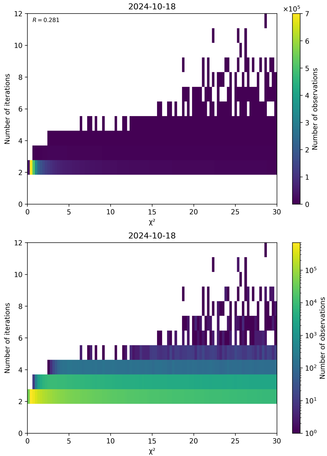
Figure 73: Scatter density plot of “ \chi^2 ” against “Number of iterations” for 2024-10-17 to 2024-10-19.
