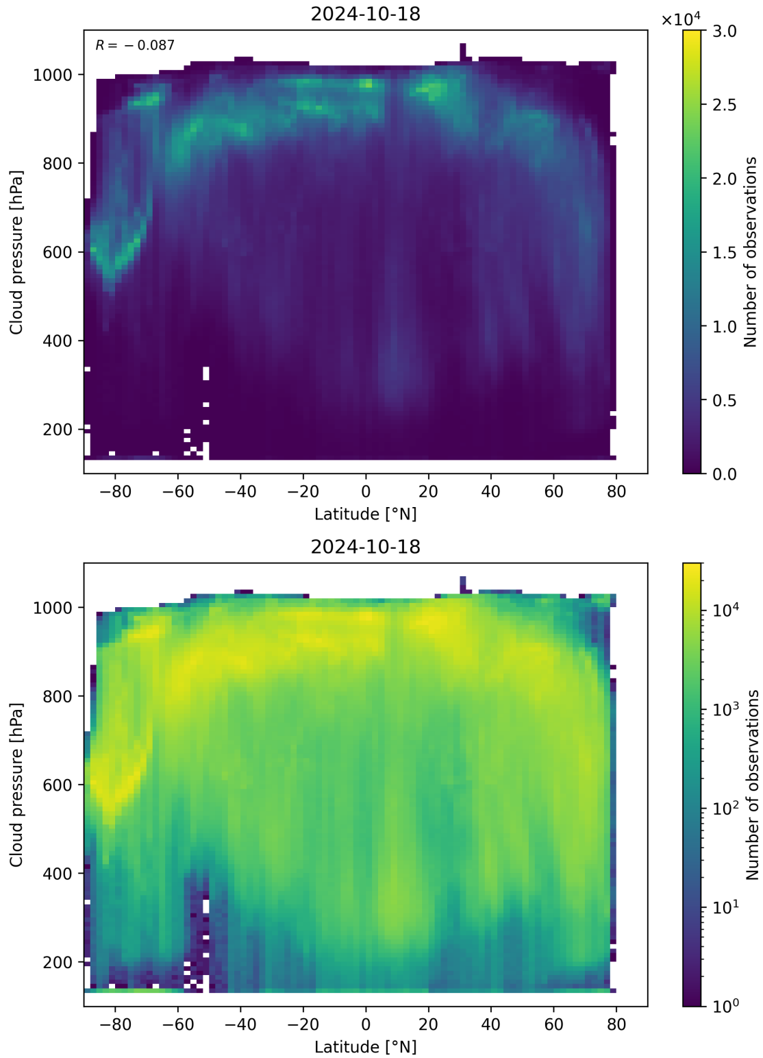
Figure 100: Scatter density plot of “Latitude” against “Cloud pressure” for 2024-10-17 to 2024-10-19.
