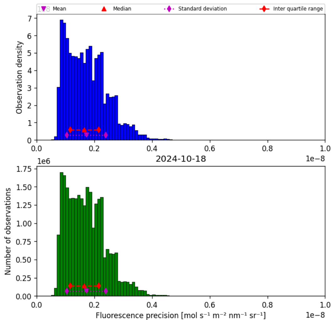
Figure 41: Histogram of “Fluorescence precision” for 2024-10-17 to 2024-10-19
