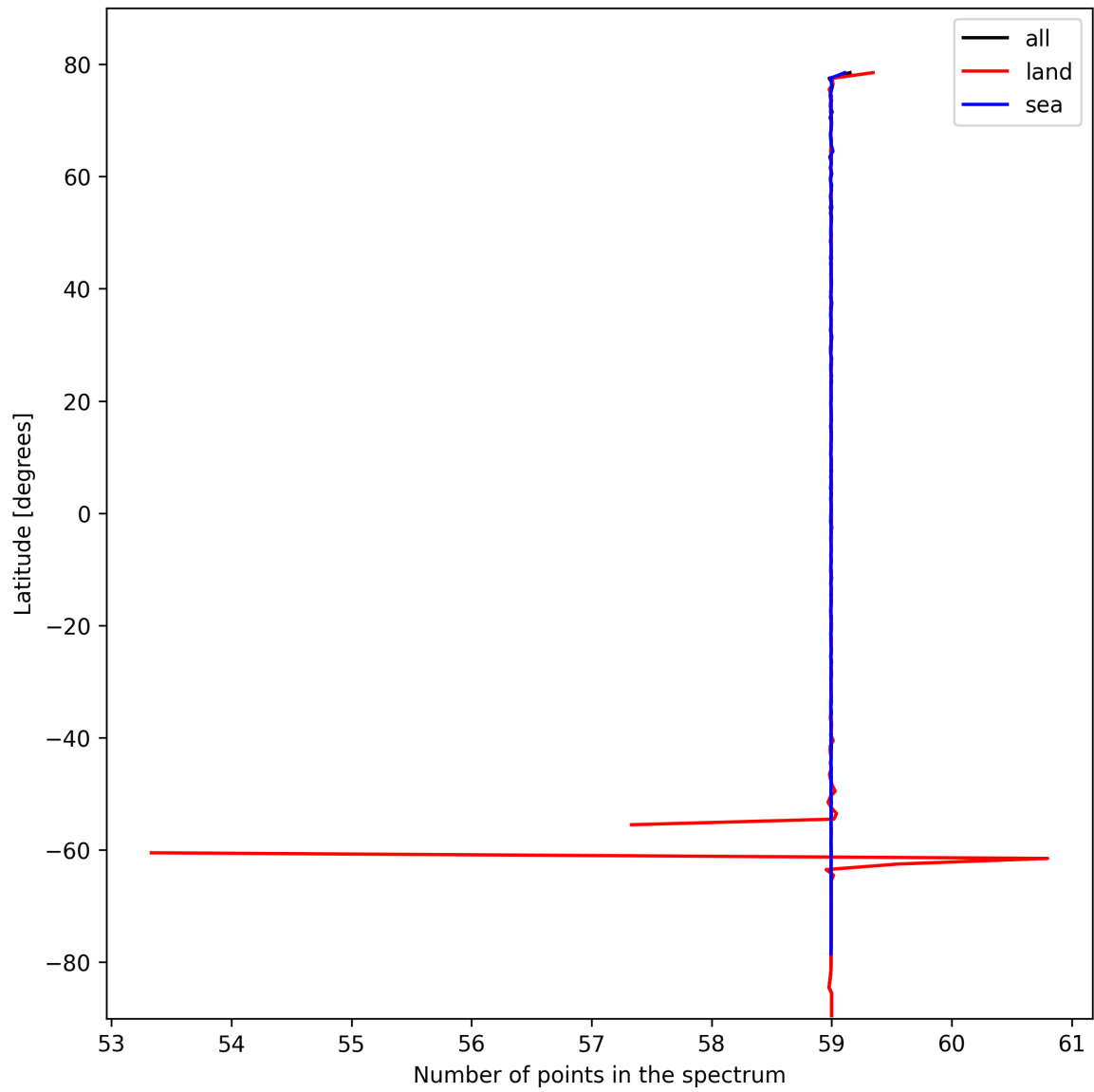
Figure 27: Zonal average of “Number of points in the spectrum” for 2024-10-17 to 2024-10-19.
