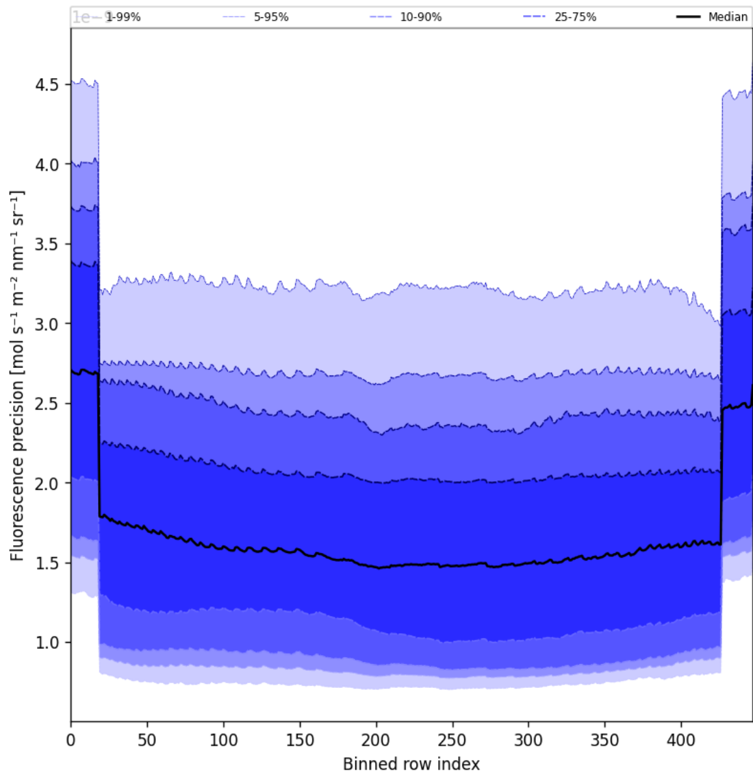
Figure 58: Along track statistics of “Fluorescence precision” for 2024-10-17 to 2024-10-19
