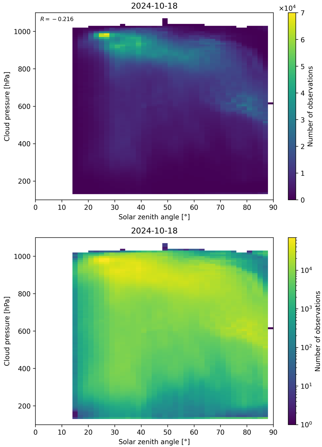
Figure 122: Scatter density plot of “Solar zenith angle” against “Cloud pressure” for 2024-10-17 to 2024-10-19.
