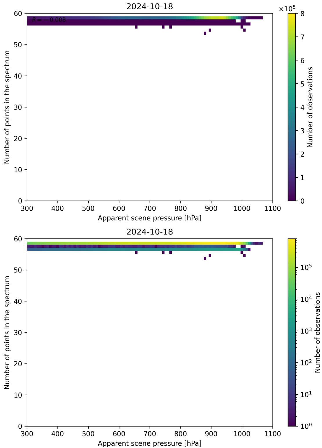
Figure 67: Scatter density plot of “Apparent scene pressure” against “Number of points in the spectrum” for 2024-10-17 to 2024-10-19.
