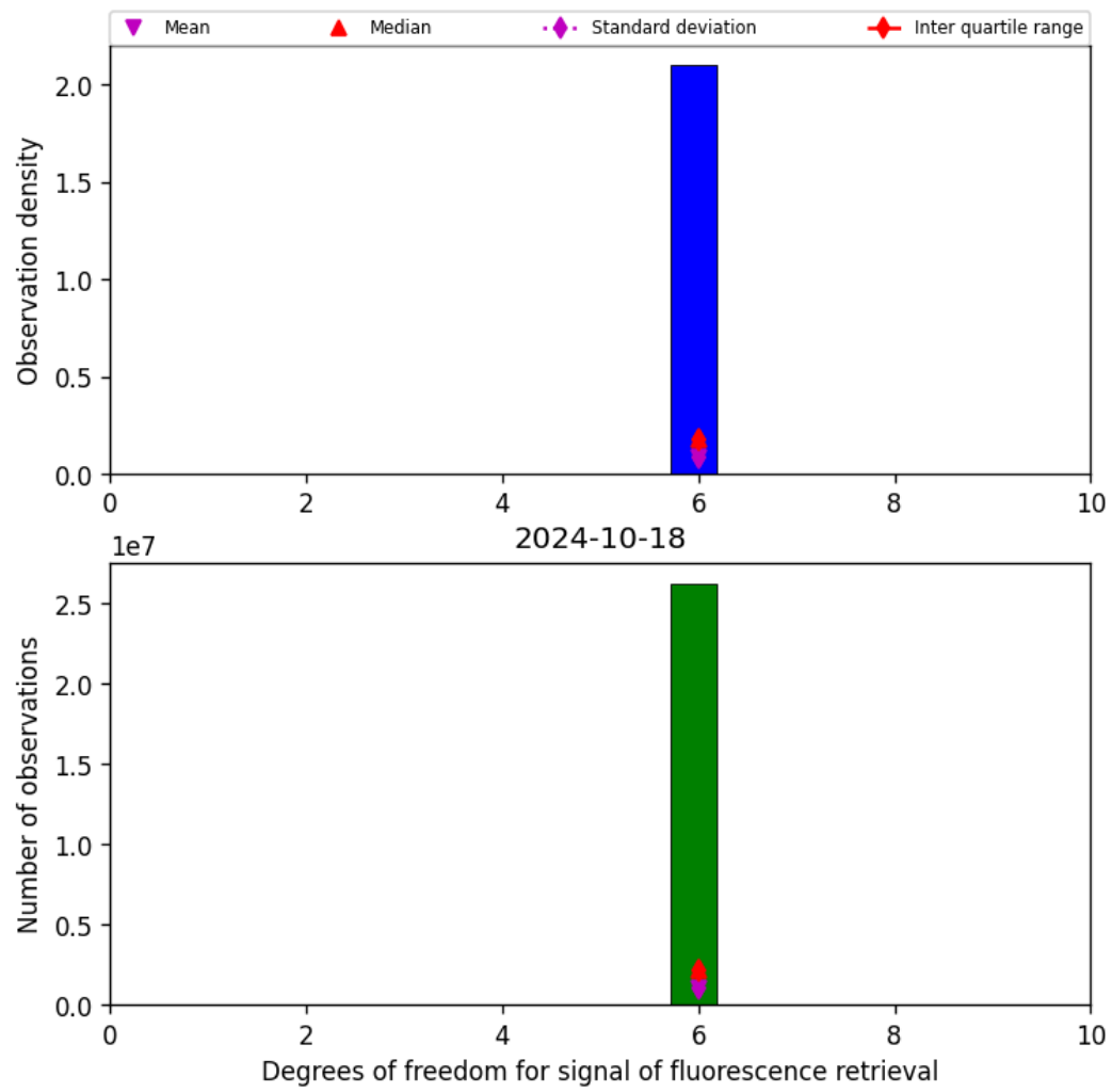
Figure 43: Histogram of "Degrees of freedom for signal of fluorescence retrieval" for 2024-10-17 to 2024-10-19
