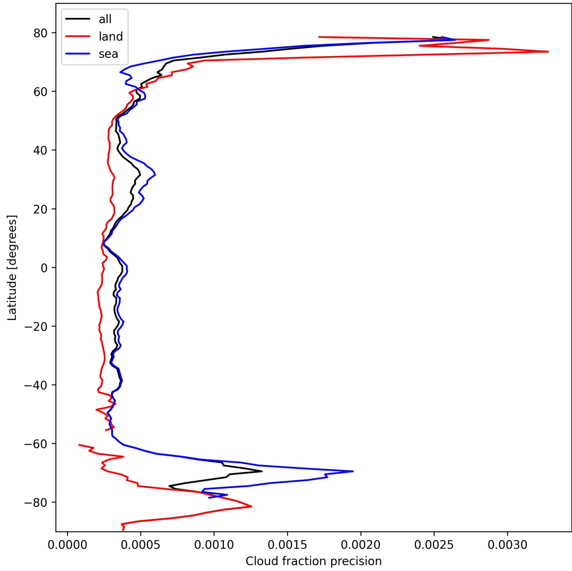
Figure 16: Zonal average of “Cloud fraction precision” for 2024-10-17 to 2024-10-19.
