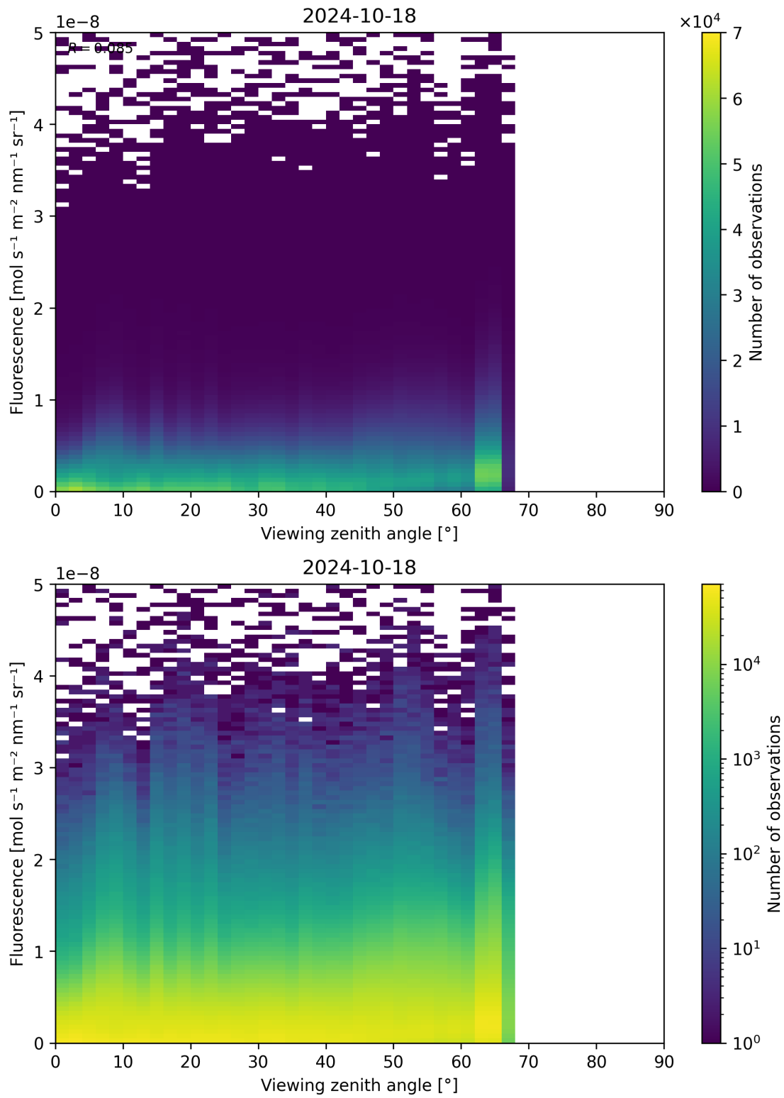
Figure 134: Scatter density plot of “Viewing zenith angle” against “Fluorescence” for 2024-10-17 to 2024-10-19.
