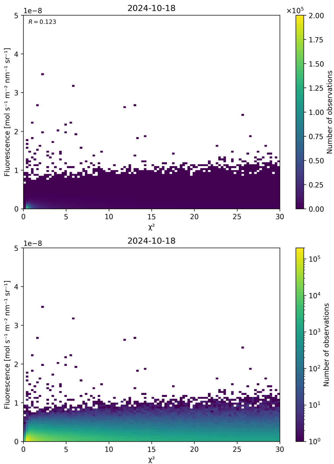
Figure 70: Scatter density plot of “ \chi^2 ” against “Fluorescence” for 2024-10-17 to 2024-10-19.
