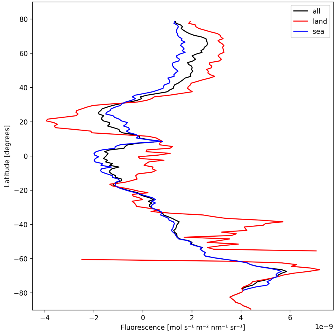
Figure 23: Zonal average of “Fluorescence” for 2024-10-17 to 2024-10-19.
