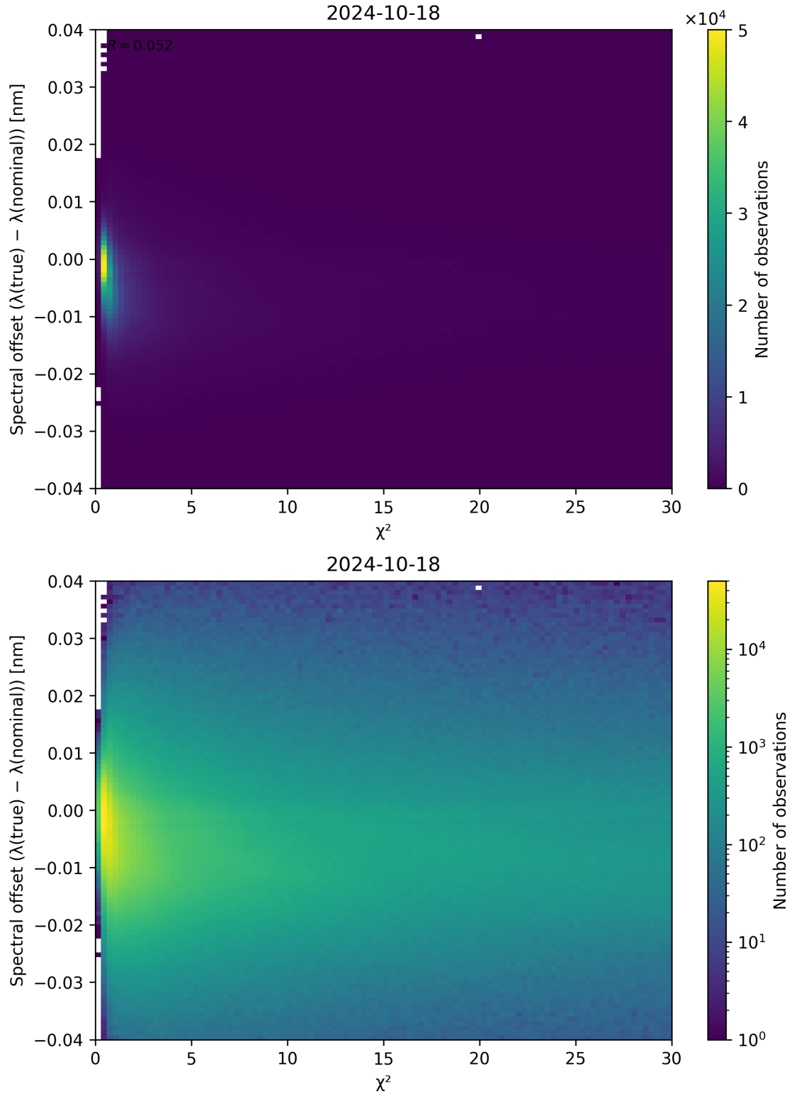
Figure 75: Scatter density plot of “ \chi^2 ” against “Spectral offset ( \lambda_{\text{true}} - \lambda_{\text{nominal}} )” for 2024-10-17 to 2024-10-19.
