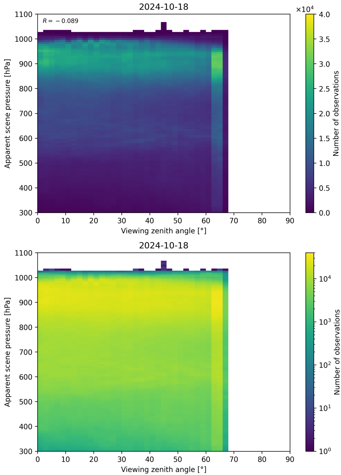
Figure 129: Scatter density plot of “Viewing zenith angle” against “Apparent scene pressure” for 2024-10-17 to 2024-10-19.
