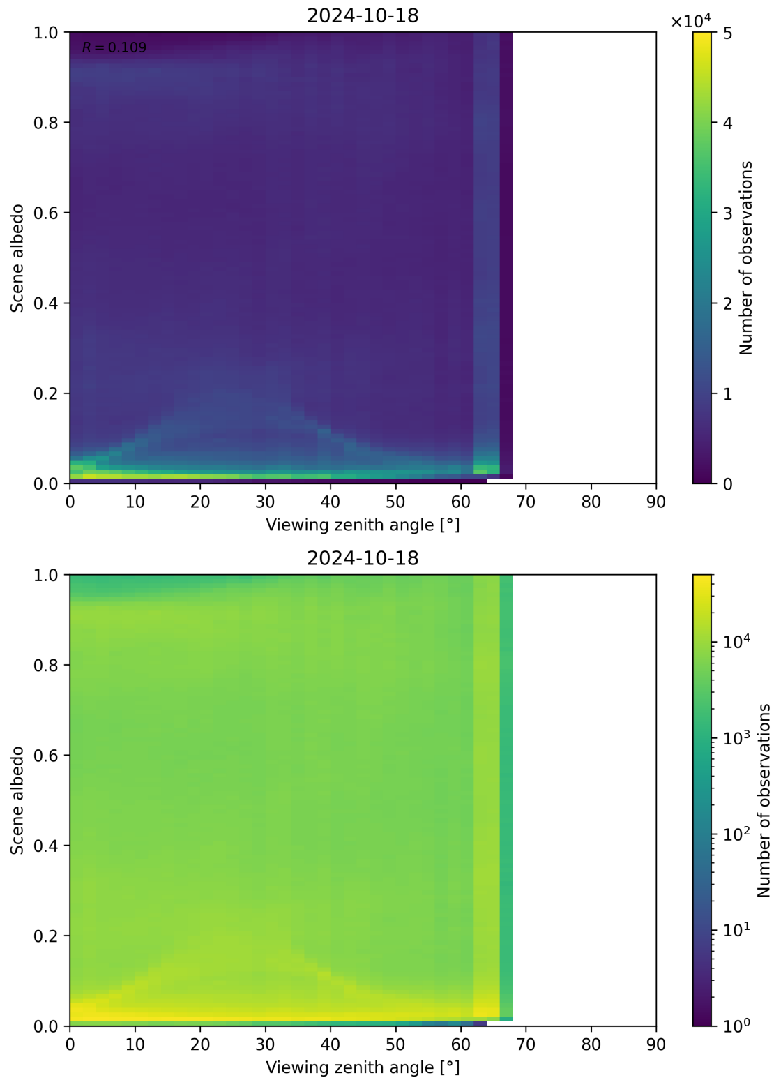
Figure 138: Scatter density plot of “Viewing zenith angle” against “Scene albedo” for 2024-10-17 to 2024-10-19.
