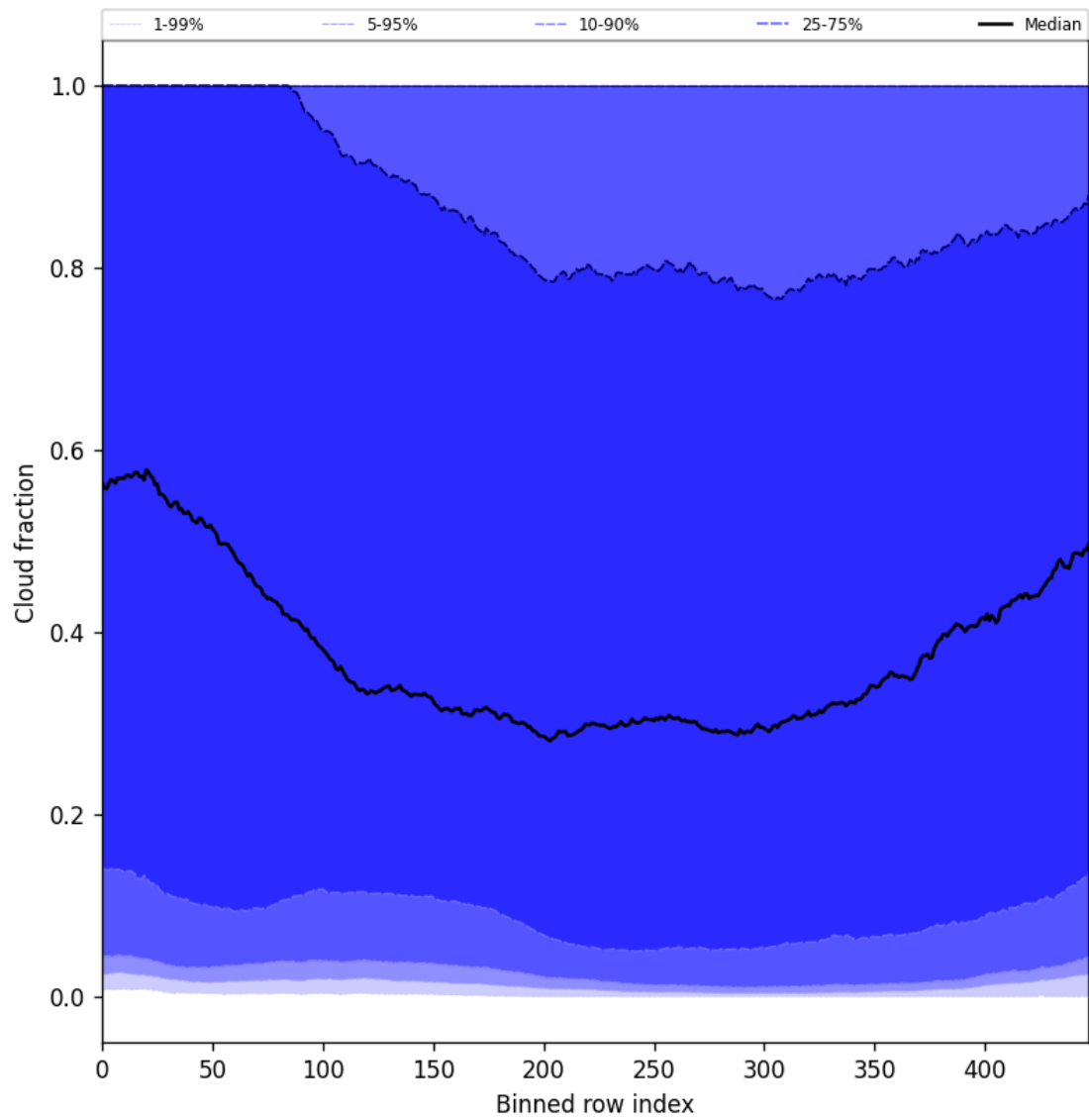
Figure 49: Along track statistics of “Cloud fraction” for 2024-10-17 to 2024-10-19
