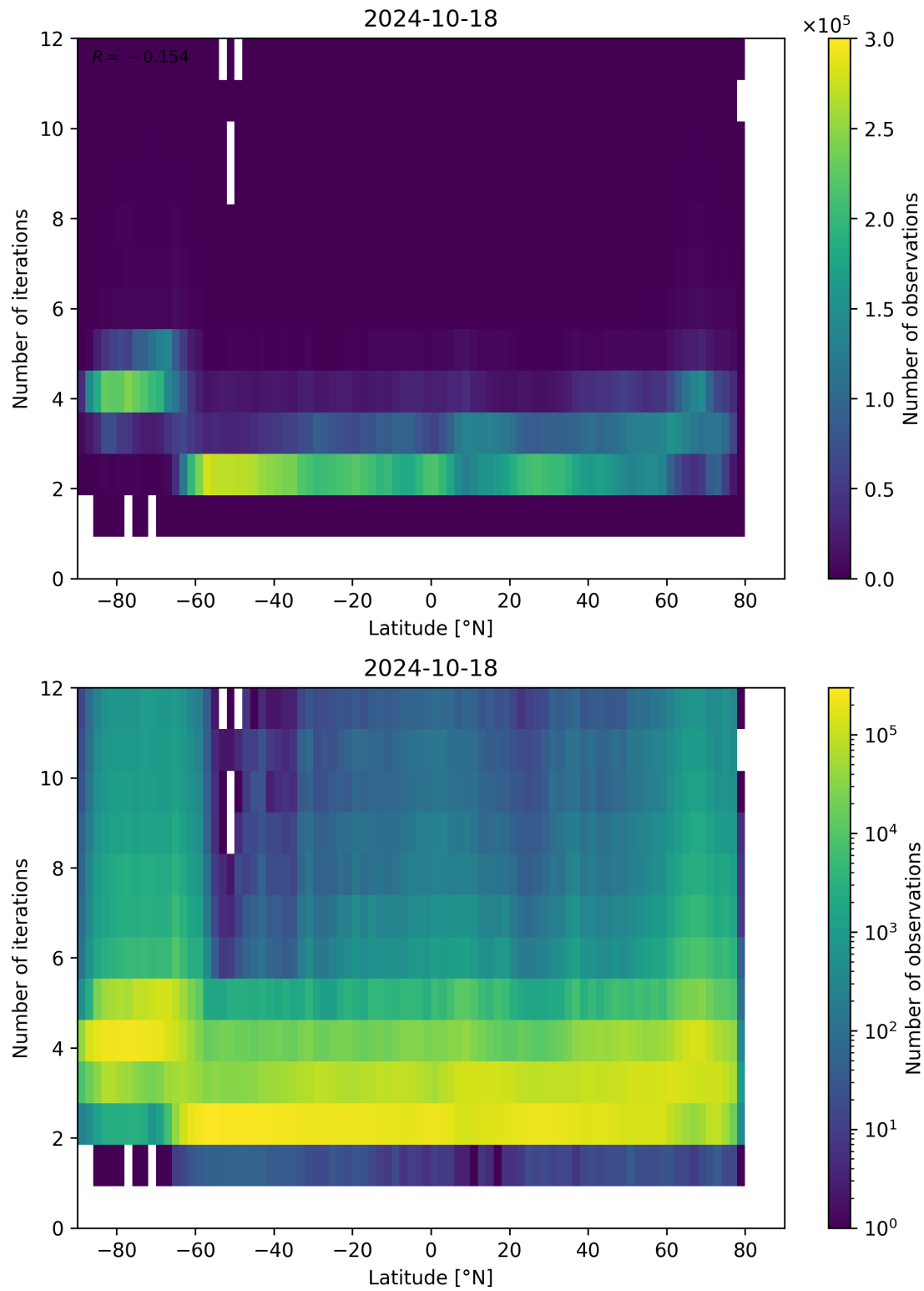
Figure 102: Scatter density plot of “Latitude” against “Number of iterations” for 2024-10-17 to 2024-10-19.
