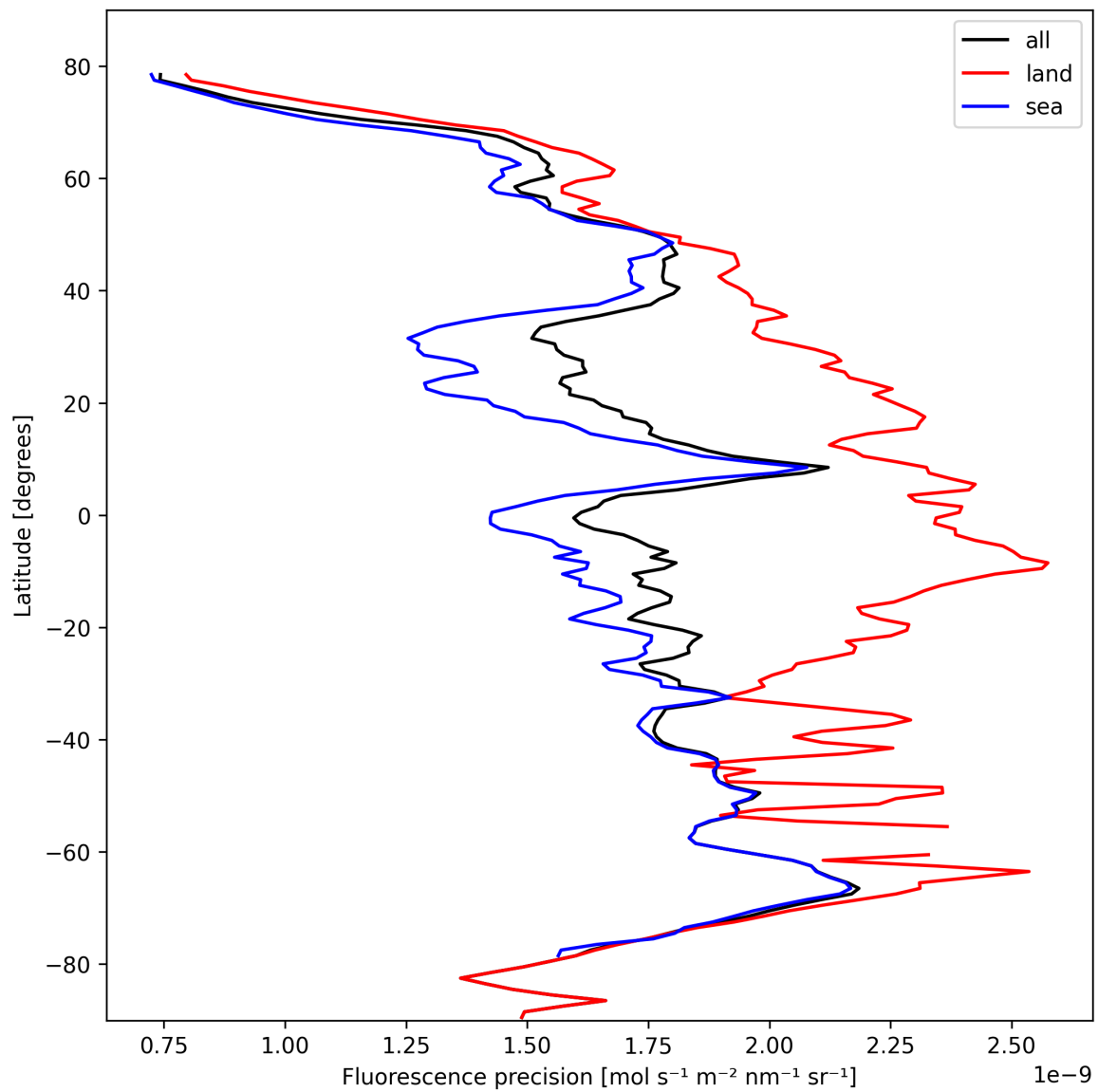
Figure 24: Zonal average of “Fluorescence precision” for 2024-10-17 to 2024-10-19.
