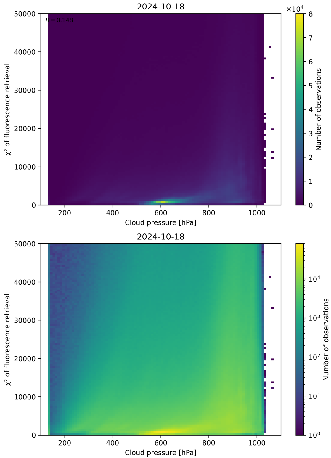
Figure 86: Scatter density plot of “Cloud pressure” against “ \chi^2 of fluorescence retrieval” for 2024-10-17 to 2024-10-19.
