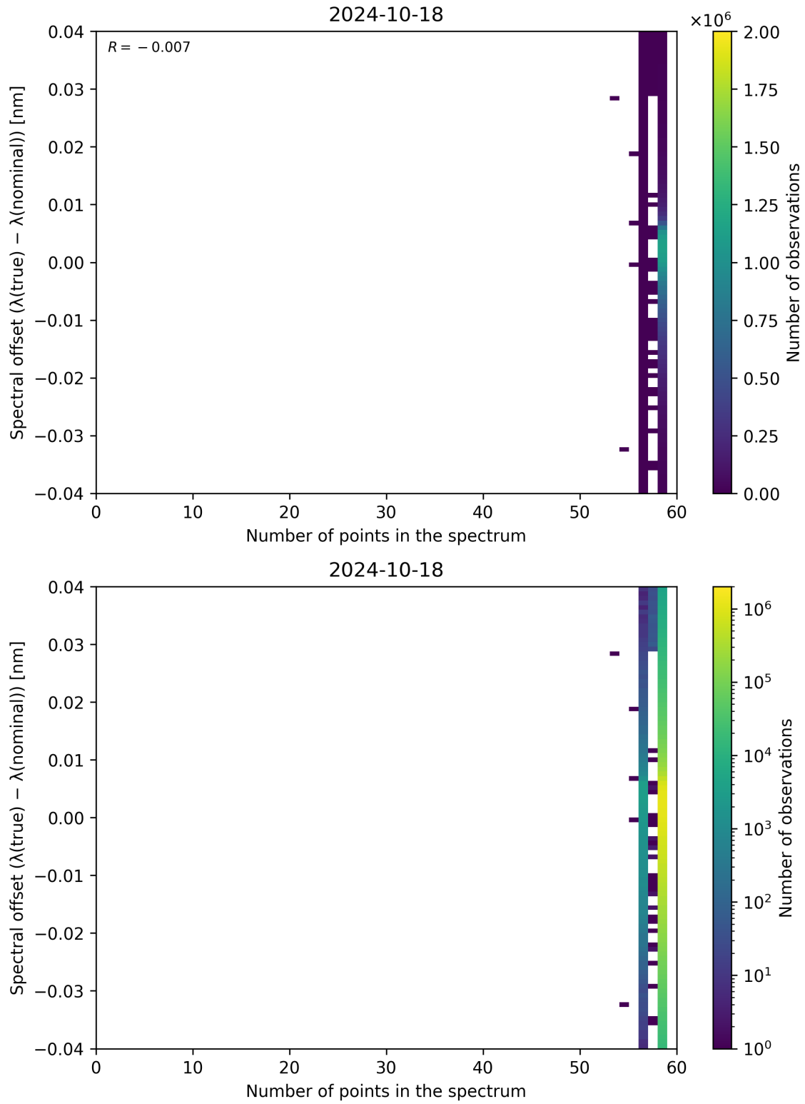
Figure 110: Scatter density plot of “Number of points in the spectrum” against “Spectral offset ( \lambda_{\text{true}} - \lambda_{\text{nominal}} )” for 2024-10-17 to 2024-10-19.
