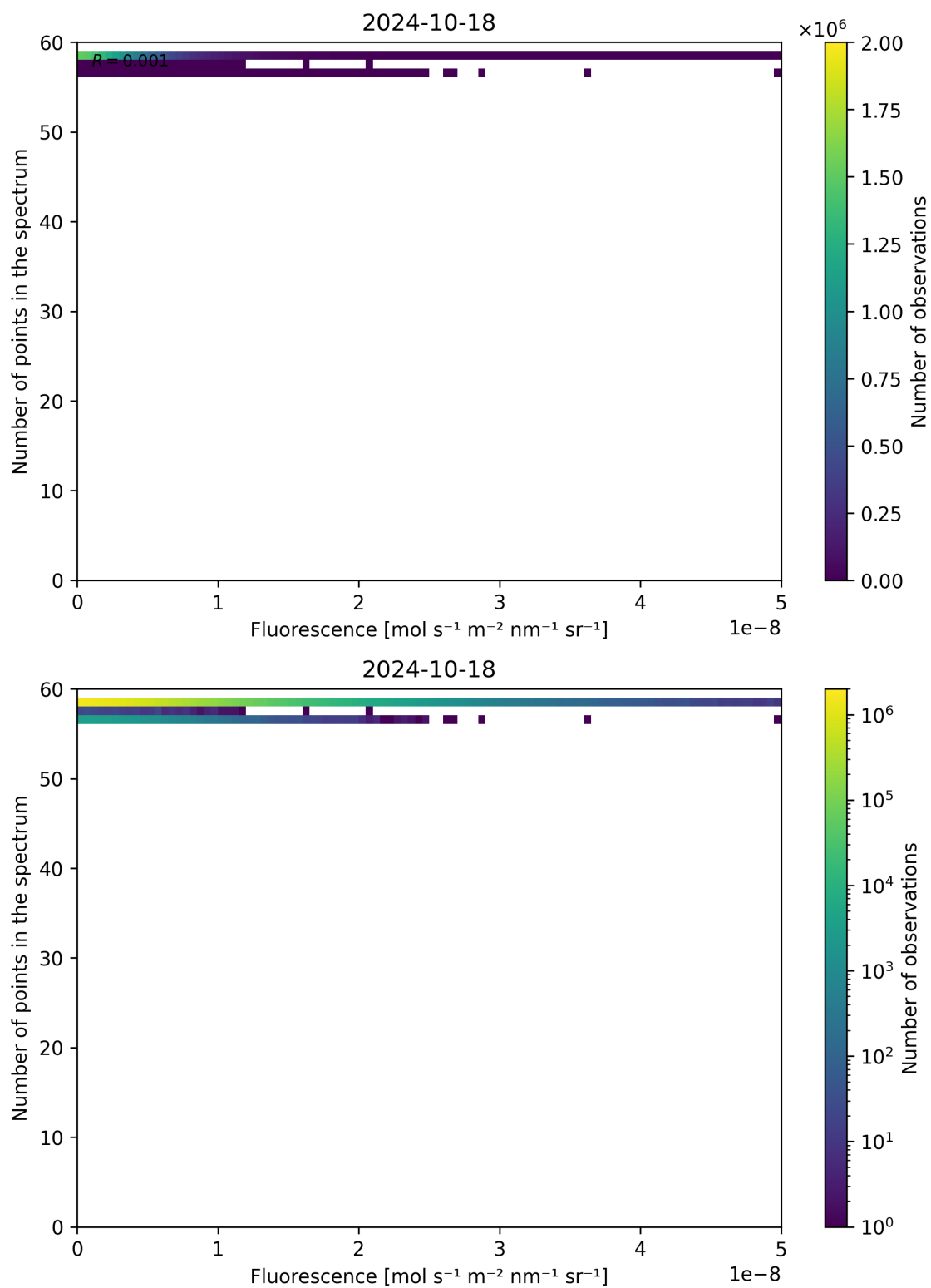
Figure 94: Scatter density plot of “Fluorescence” against “Number of points in the spectrum” for 2024-10-17 to 2024-10-19.
