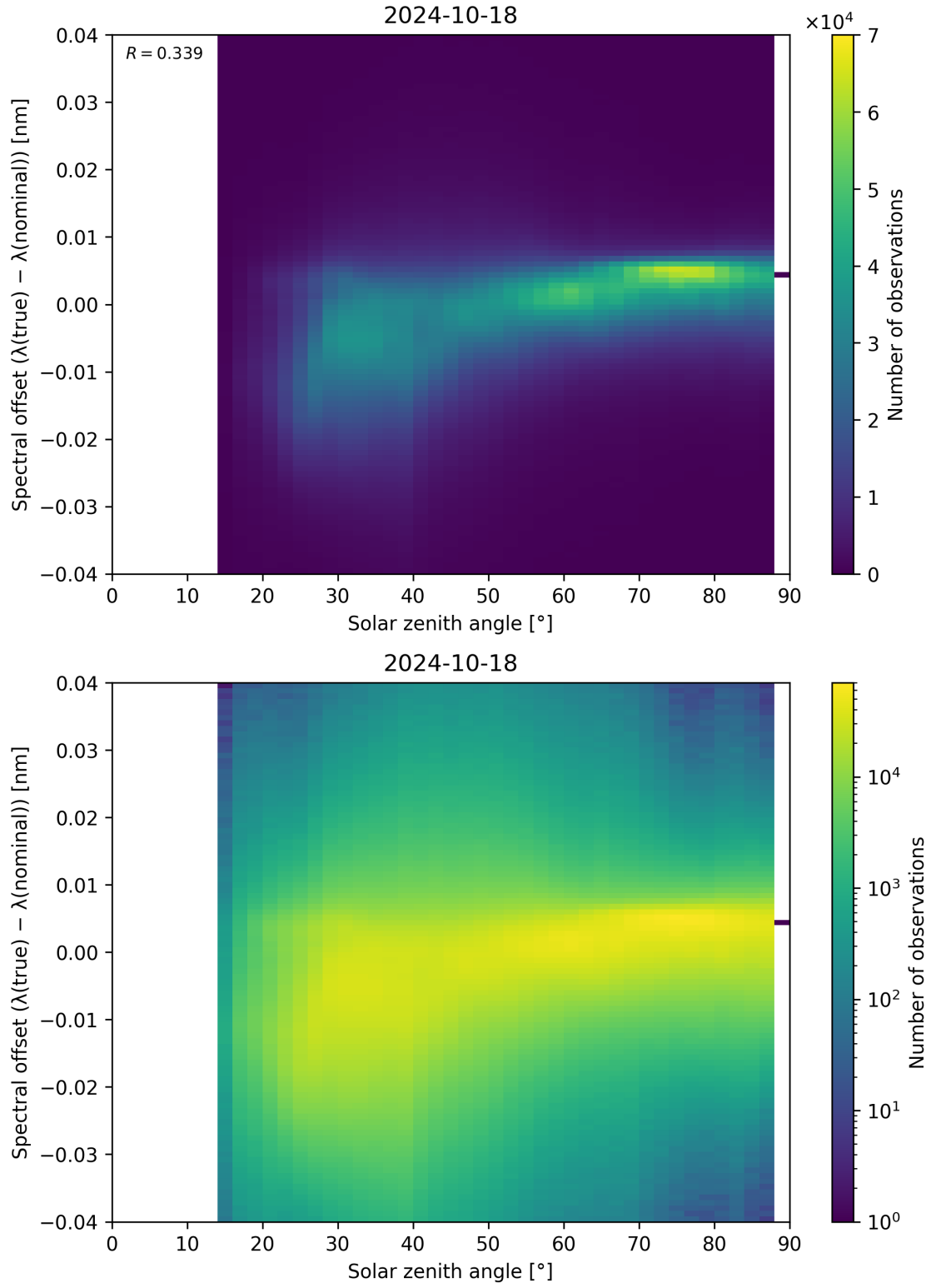
Figure 128: Scatter density plot of “Solar zenith angle” against “Spectral offset ( \lambda_{\text{true}} - \lambda_{\text{nominal}} )” for 2024-10-17 to 2024-10-19.
