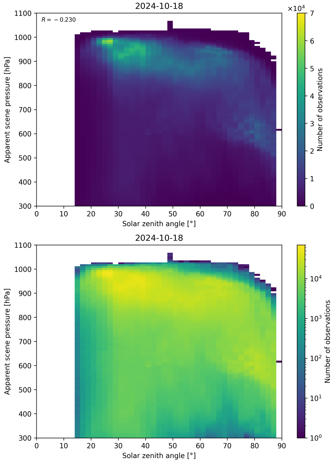
Figure 118: Scatter density plot of “Solar zenith angle” against “Apparent scene pressure” for 2024-10-17 to 2024-10-19.
