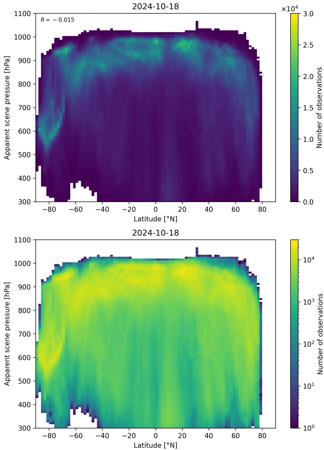
Figure 96: Scatter density plot of “Latitude” against “Apparent scene pressure” for 2024-10-17 to 2024-10-19.
