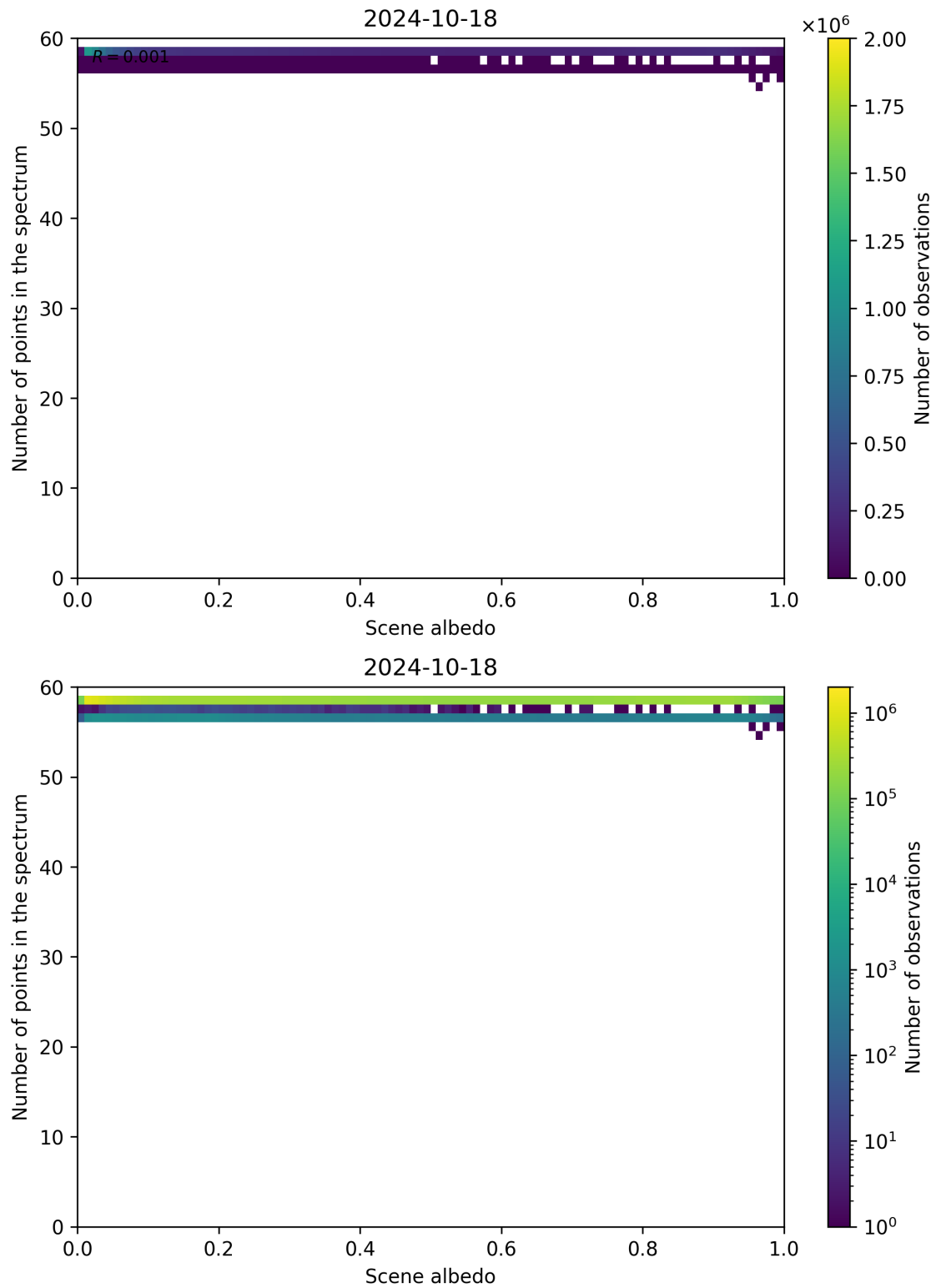
Figure 116: Scatter density plot of “Scene albedo” against “Number of points in the spectrum” for 2024-10-17 to 2024-10-19.
