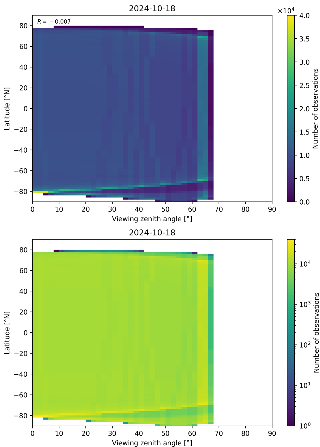
Figure 135: Scatter density plot of “Viewing zenith angle” against “Latitude” for 2024-10-17 to 2024-10-19.
