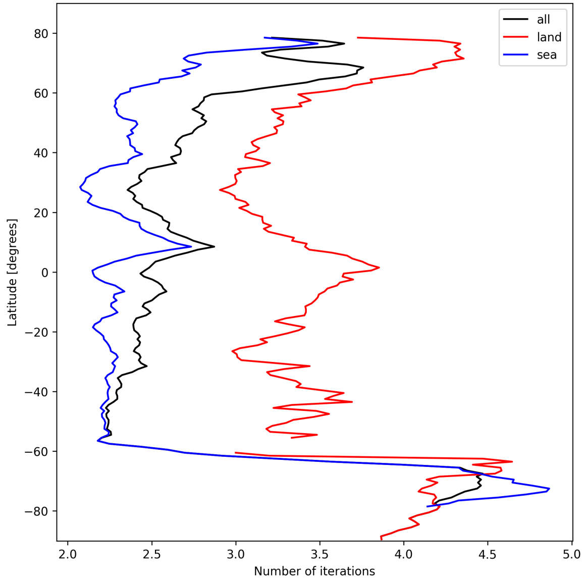
Figure 22: Zonal average of “Number of iterations” for 2024-10-17 to 2024-10-19.
