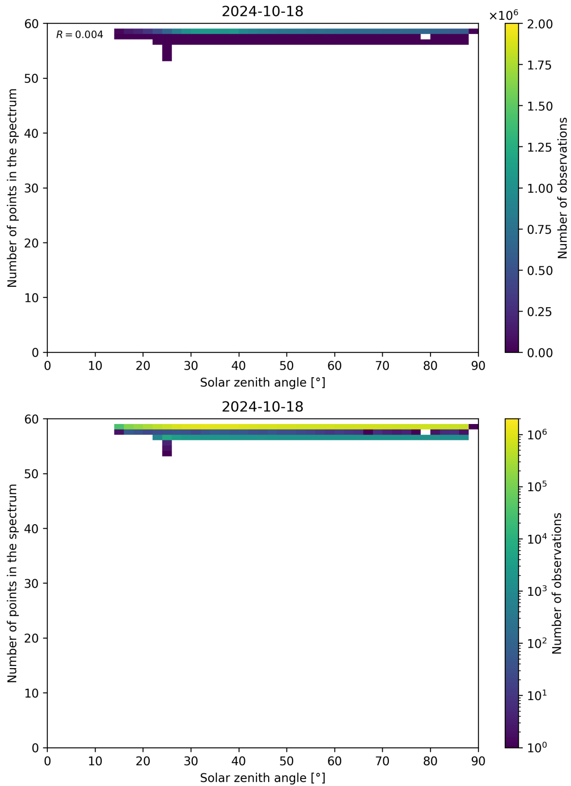
Figure 126: Scatter density plot of “Solar zenith angle” against “Number of points in the spectrum” for 2024-10-17 to 2024-10-19.
