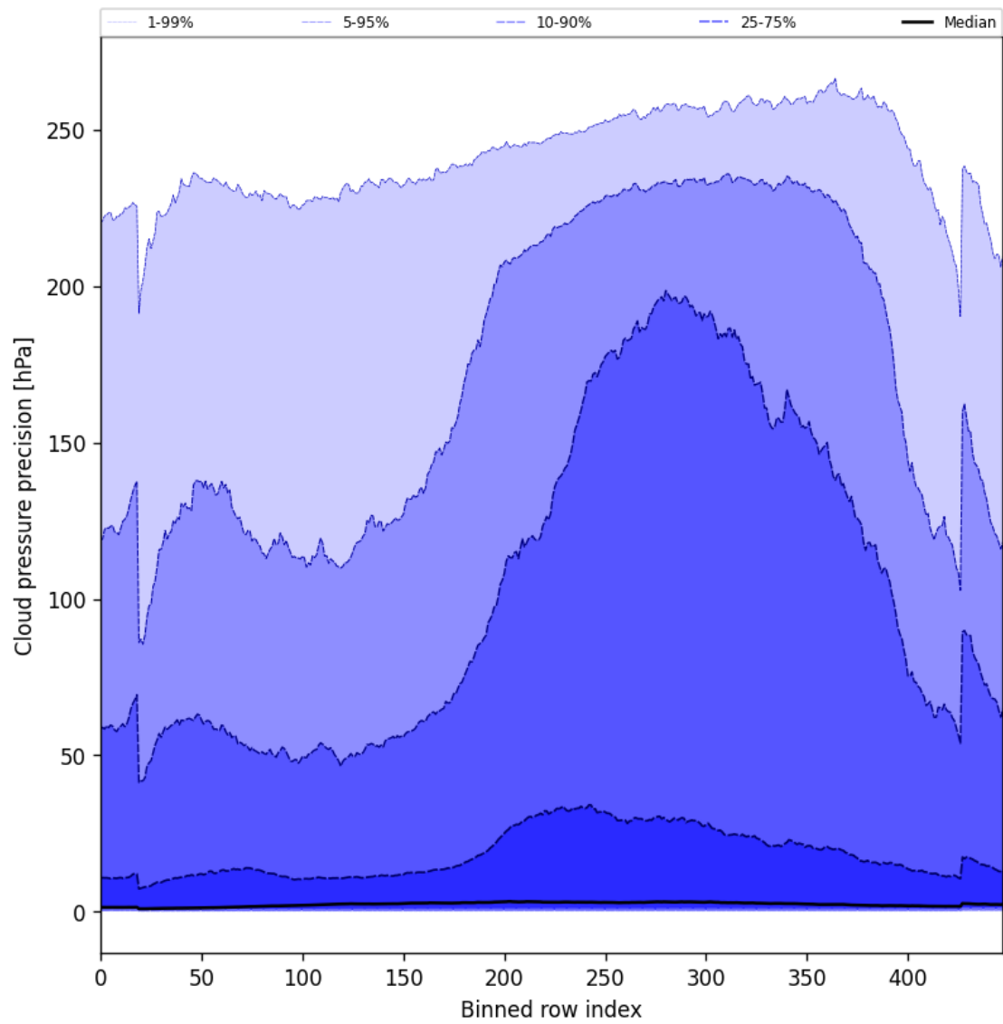
Figure 48: Along track statistics of “Cloud pressure precision” for 2024-10-17 to 2024-10-19
