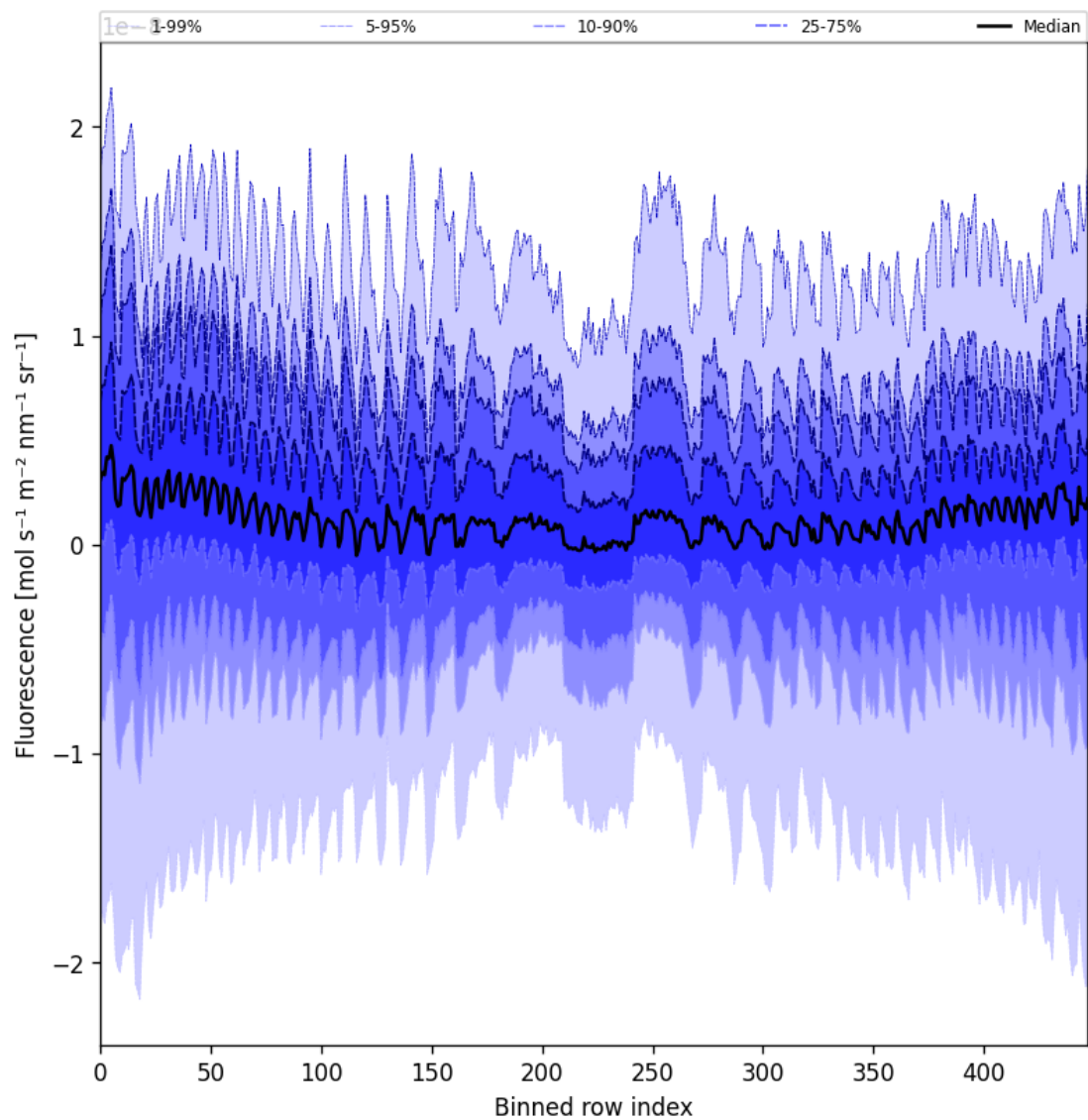
Figure 57: Along track statistics of “Fluorescence” for 2024-10-17 to 2024-10-19
