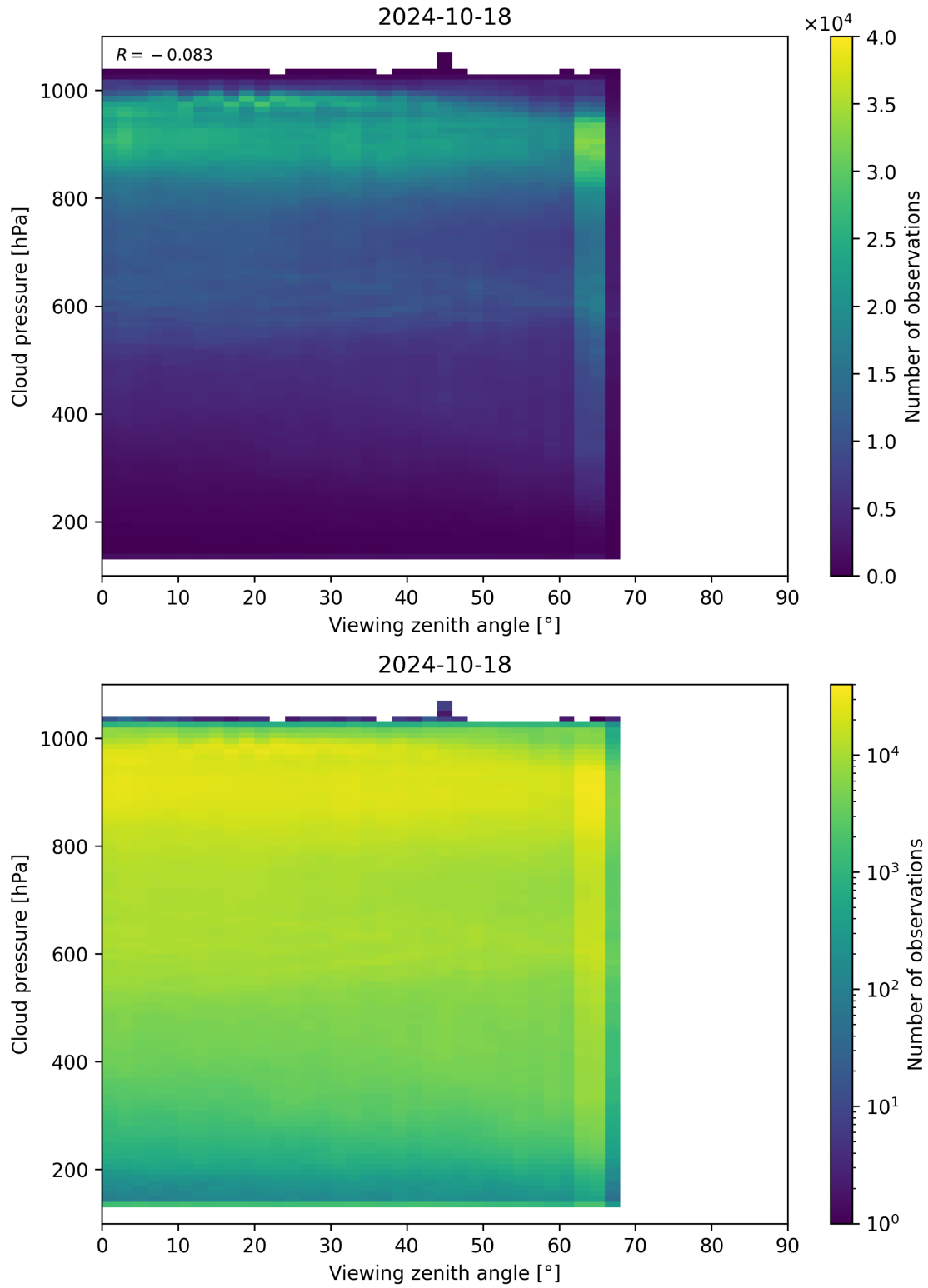
Figure 133: Scatter density plot of “Viewing zenith angle” against “Cloud pressure” for 2024-10-17 to 2024-10-19.
