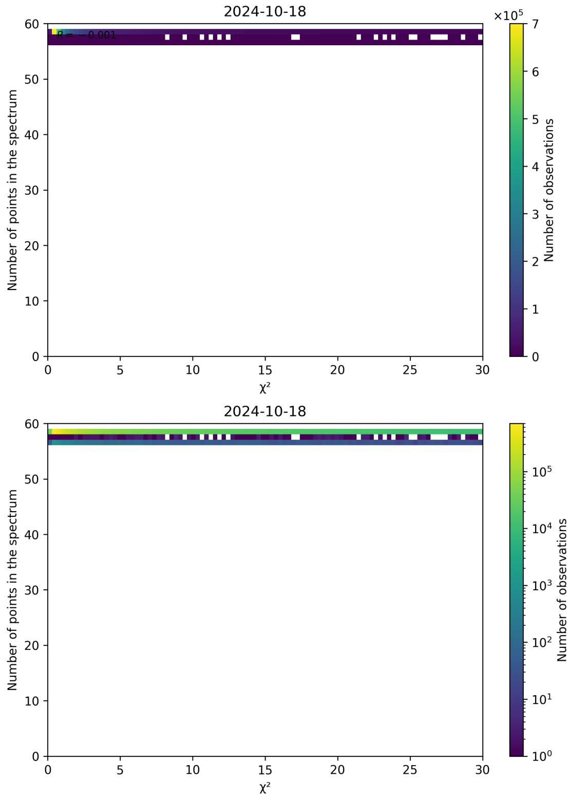
Figure 74: Scatter density plot of " \chi^2 " against "Number of points in the spectrum" for 2024-10-17 to 2024-10-19.
