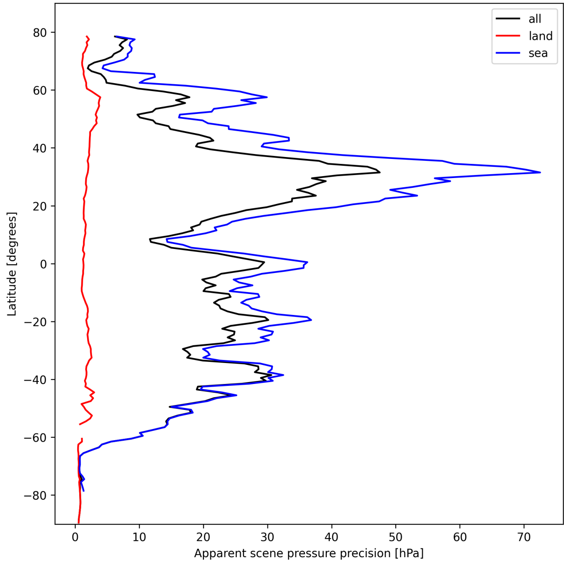
Figure 20: Zonal average of “Apparent scene pressure precision” for 2024-10-17 to 2024-10-19.
