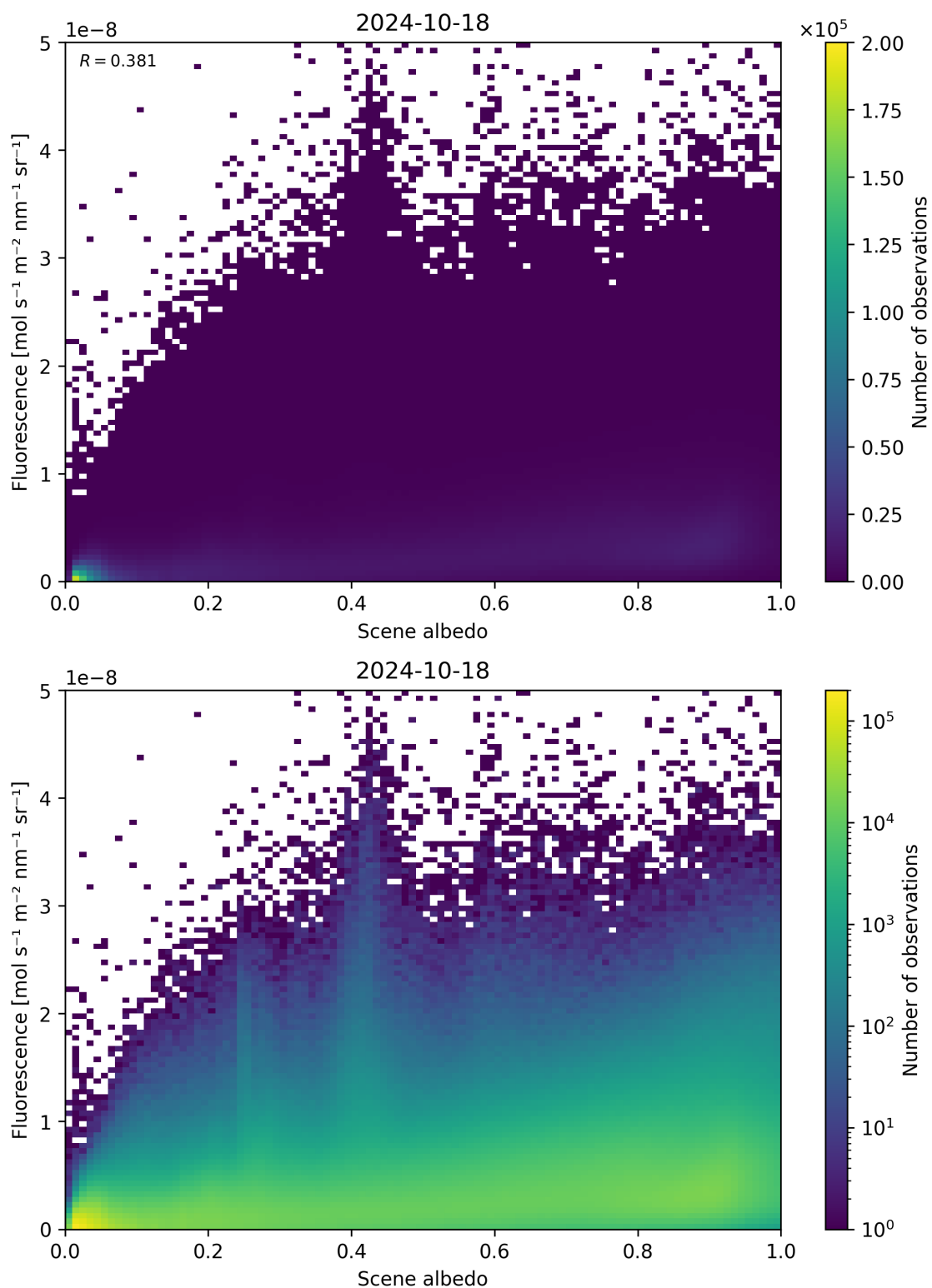
Figure 114: Scatter density plot of “Scene albedo” against “Fluorescence” for 2024-10-17 to 2024-10-19.
