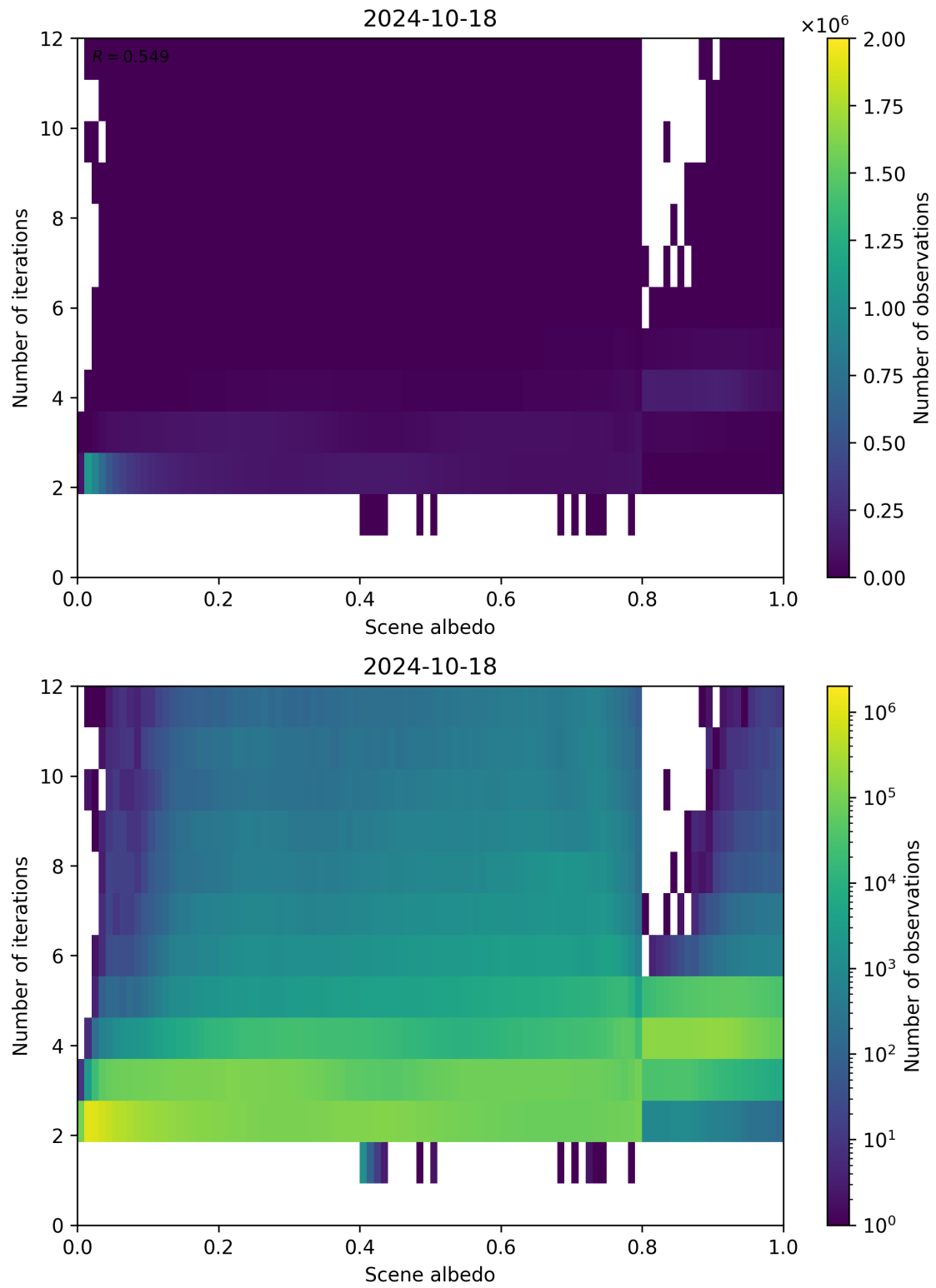
Figure 115: Scatter density plot of “Scene albedo” against “Number of iterations” for 2024-10-17 to 2024-10-19.
