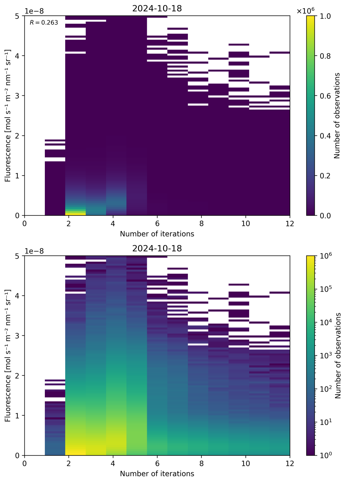
Figure 107: Scatter density plot of “Number of iterations” against “Fluorescence” for 2024-10-17 to 2024-10-19.
