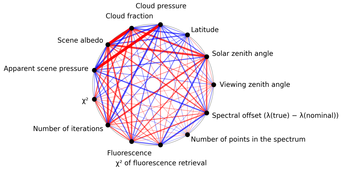
Figure 1: Map of correlation graph for 2024-10-17 to 2024-10-19.
