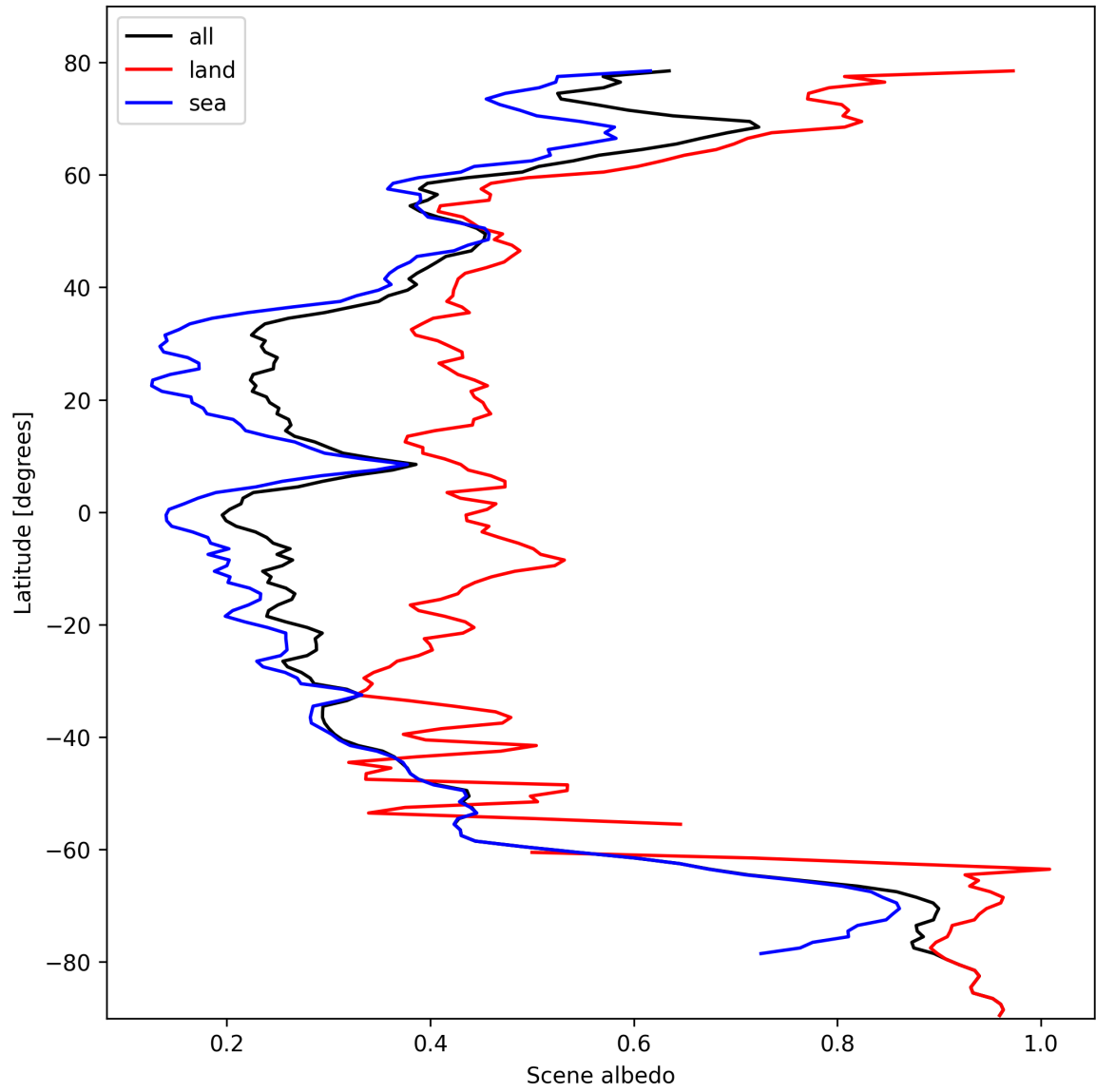
Figure 17: Zonal average of “Scene albedo” for 2024-10-17 to 2024-10-19.
