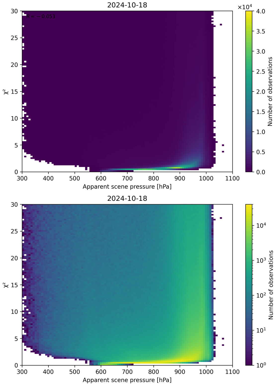
Figure 63: Scatter density plot of “Apparent scene pressure” against “ \chi^2 ” for 2024-10-17 to 2024-10-19.
