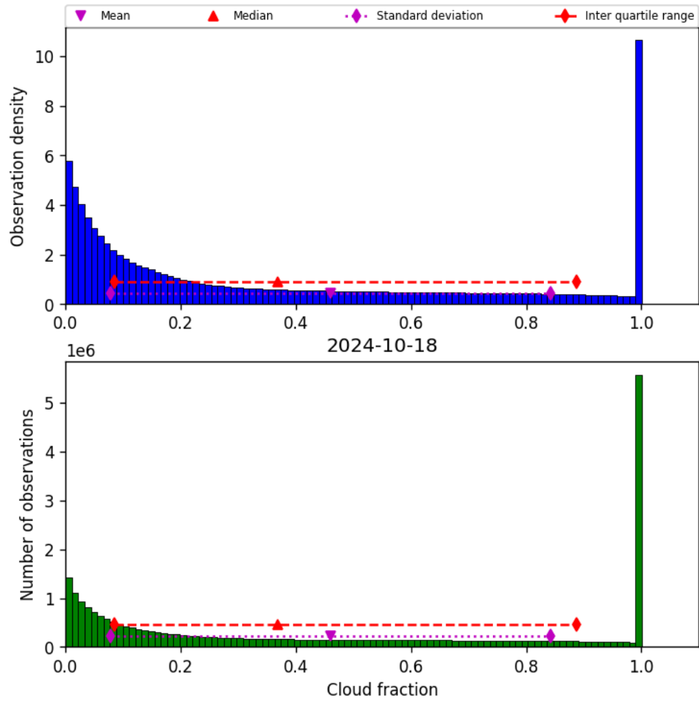
Figure 32: Histogram of “Cloud fraction” for 2024-10-17 to 2024-10-19
