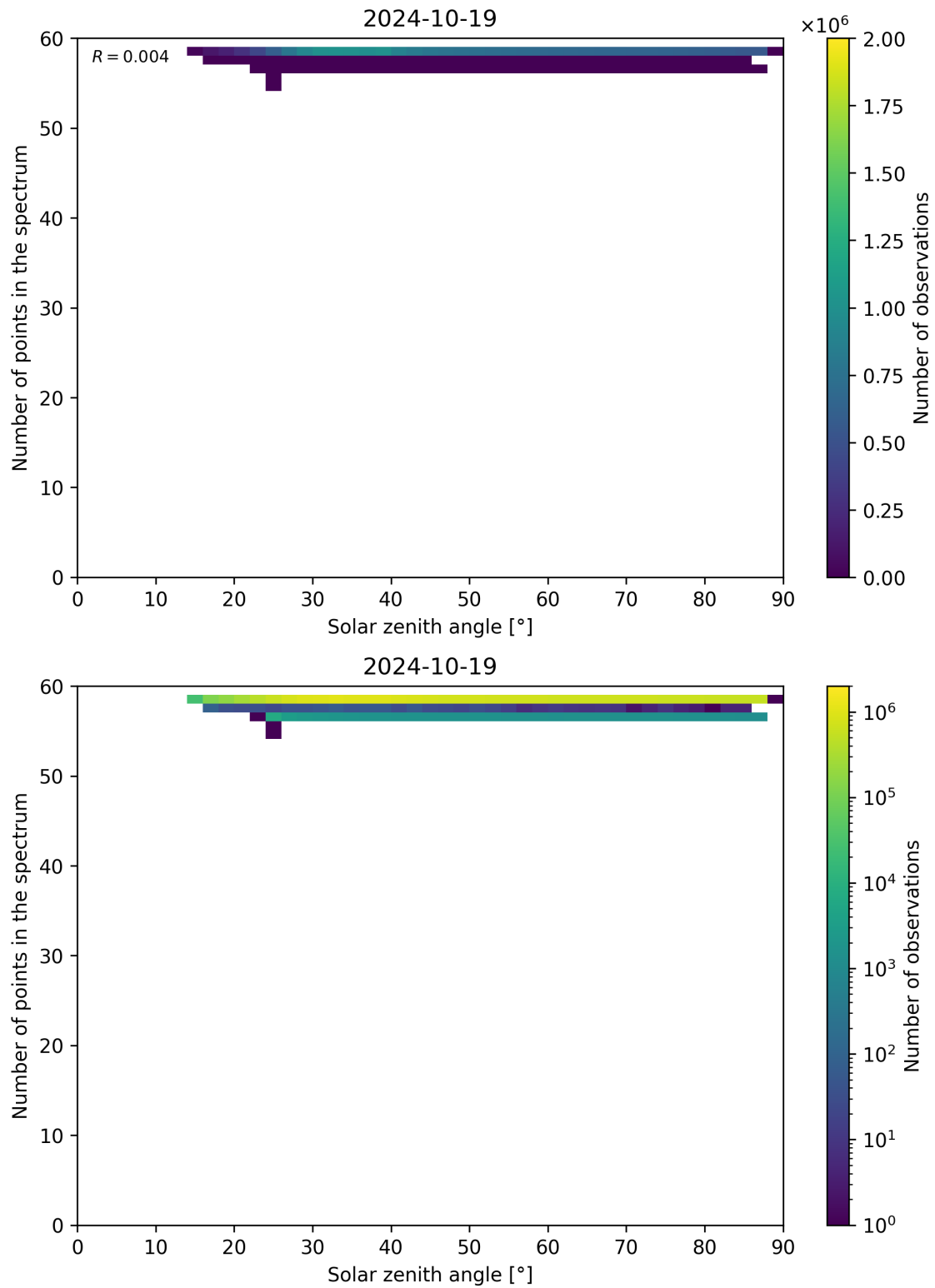
Figure 126: Scatter density plot of “Solar zenith angle” against “Number of points in the spectrum” for 2024-10-19 to 2024-10-20.
