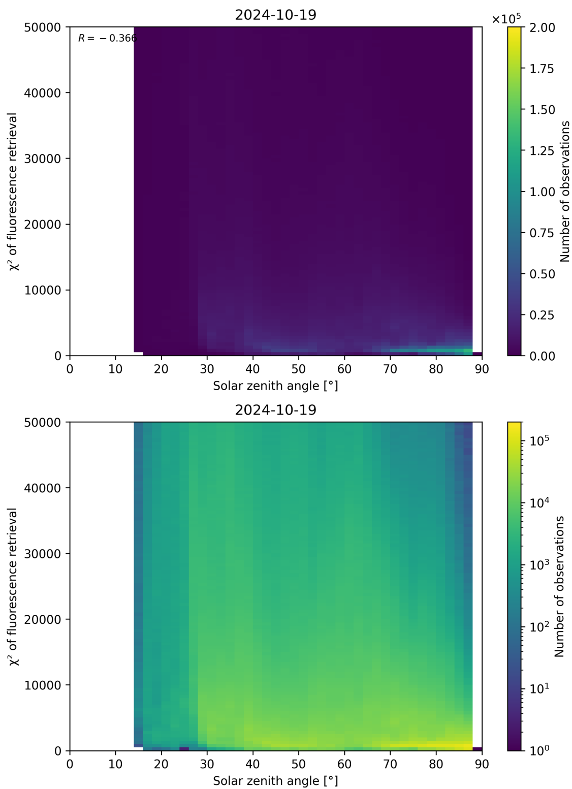
Figure 120: Scatter density plot of “Solar zenith angle” against “ \chi^2 of fluorescence retrieval” for 2024-10-19 to 2024-10-20.
