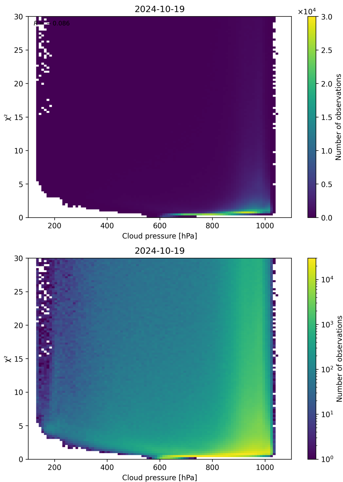
Figure 85: Scatter density plot of “Cloud pressure” against “ \chi^2 ” for 2024-10-19 to 2024-10-20.
