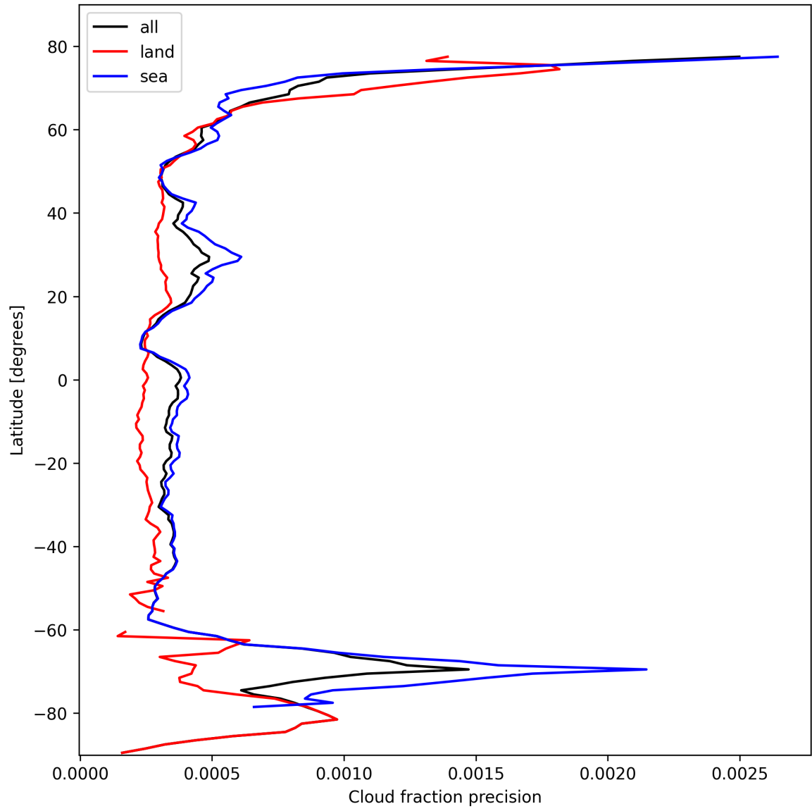
Figure 16: Zonal average of “Cloud fraction precision” for 2024-10-19 to 2024-10-20.
