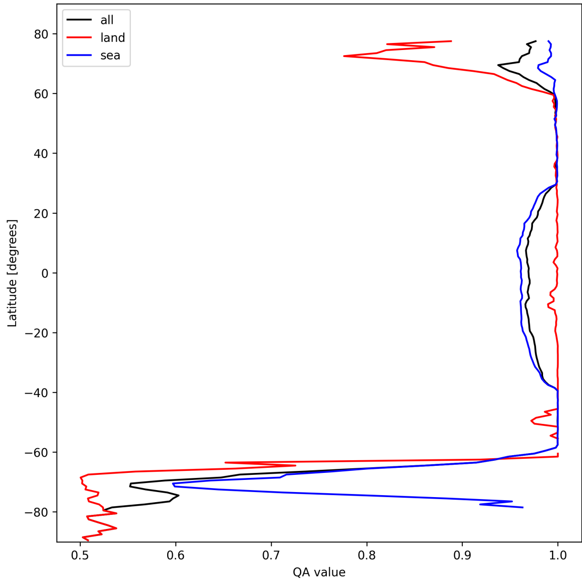
Figure 12: Zonal average of “QA value” for 2024-10-19 to 2024-10-20.
