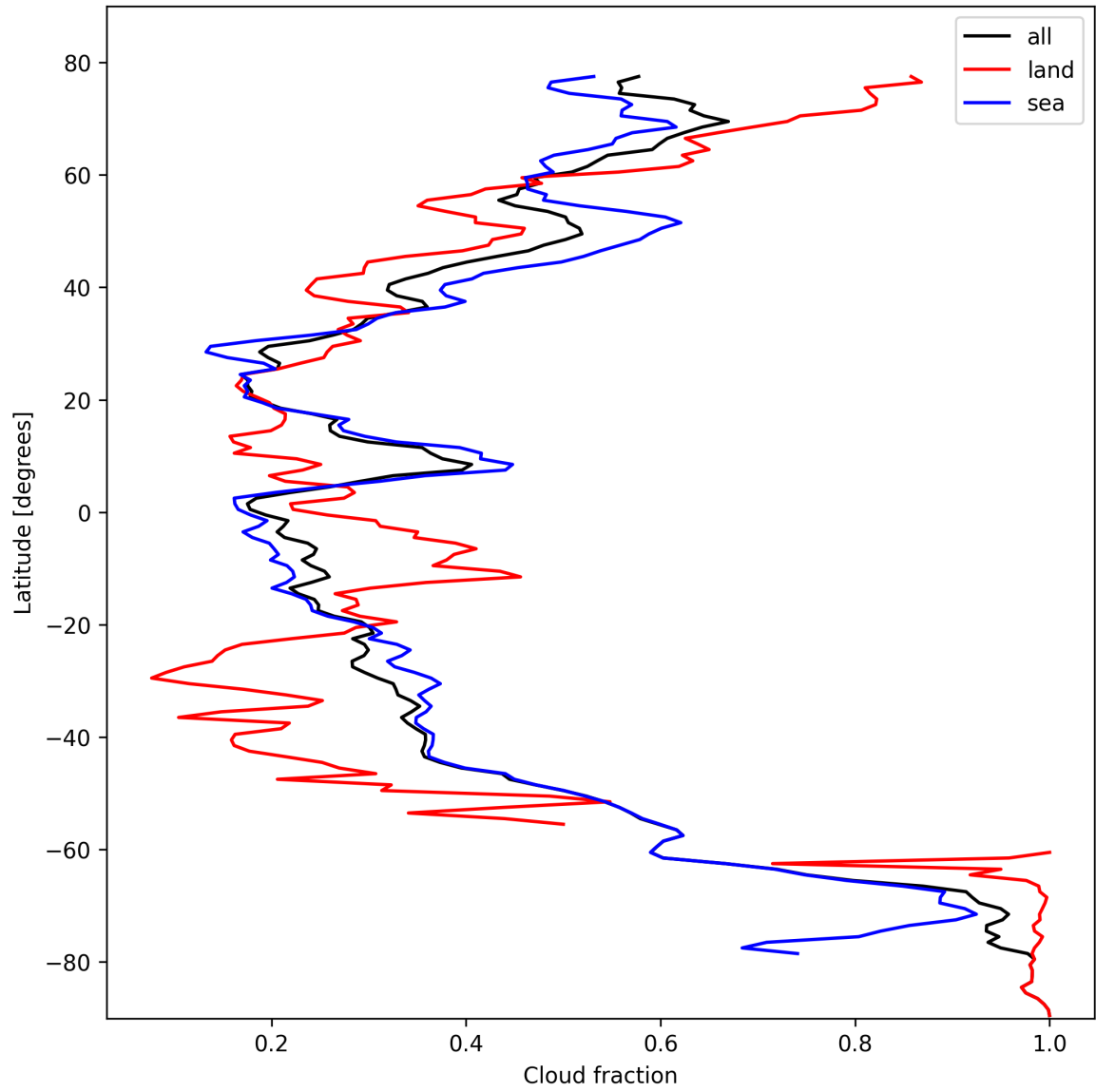
Figure 15: Zonal average of “Cloud fraction” for 2024-10-19 to 2024-10-20.
