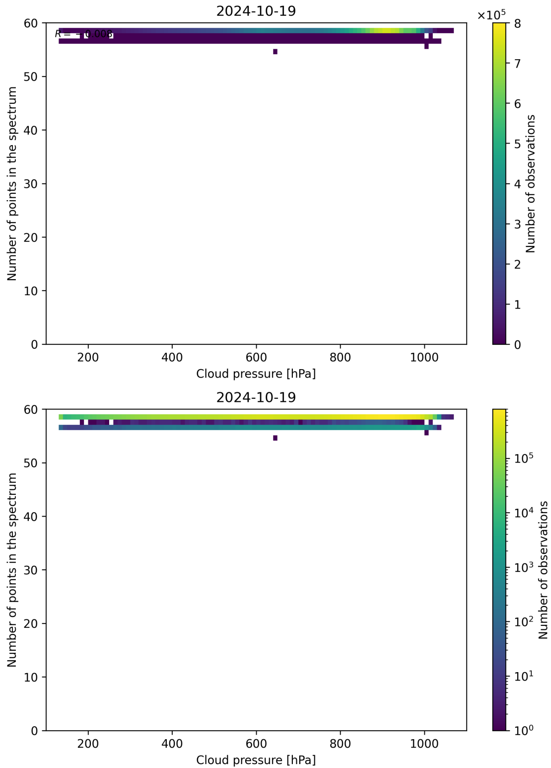
Figure 90: Scatter density plot of “Cloud pressure” against “Number of points in the spectrum” for 2024-10-19 to 2024-10-20.
