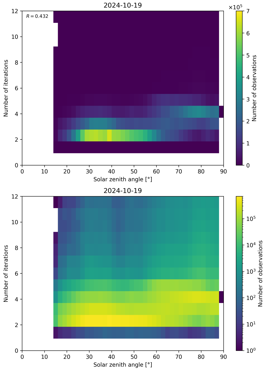
Figure 125: Scatter density plot of “Solar zenith angle” against “Number of iterations” for 2024-10-19 to 2024-10-20.
