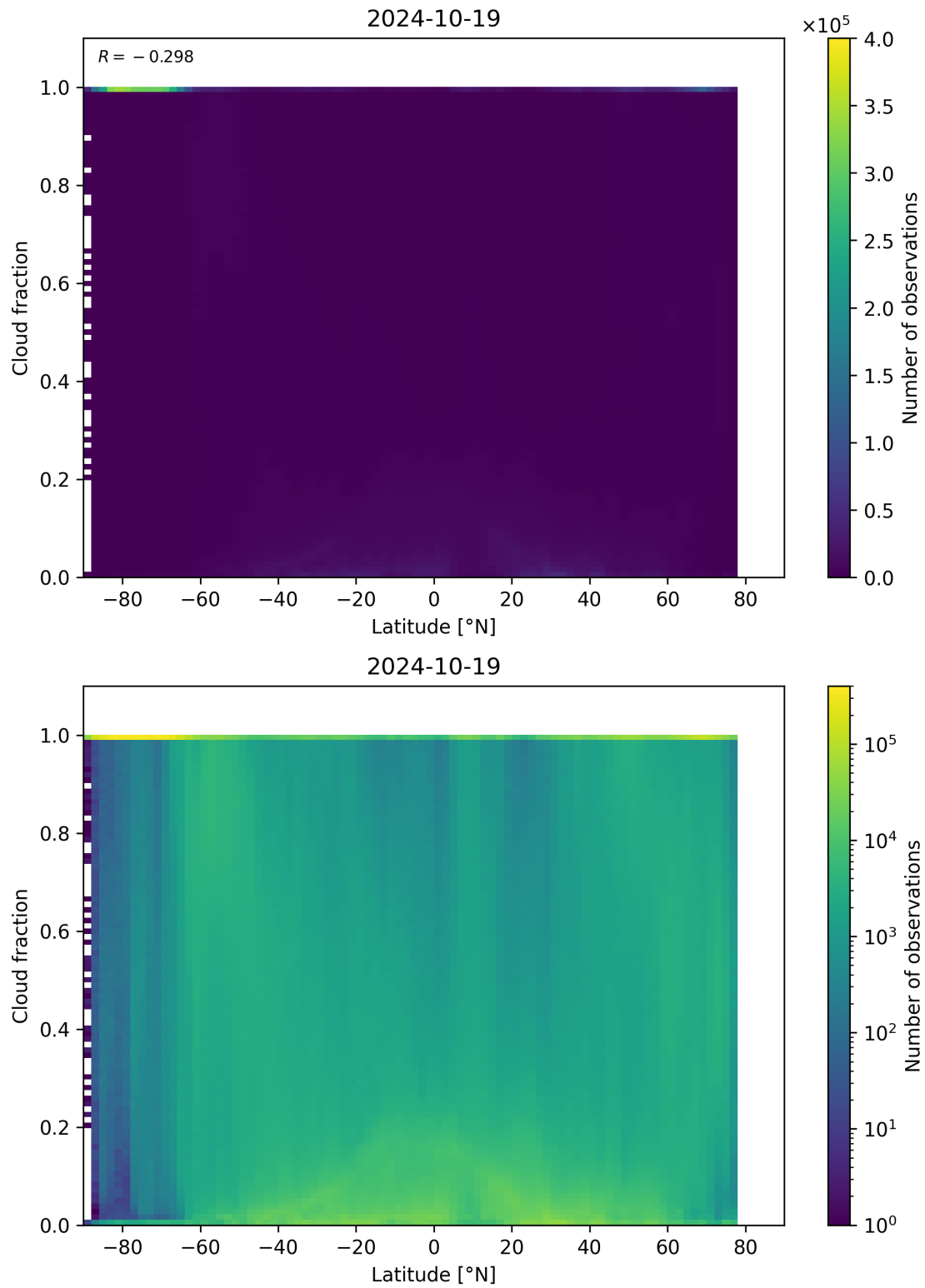
Figure 99: Scatter density plot of “Latitude” against “Cloud fraction” for 2024-10-19 to 2024-10-20.
