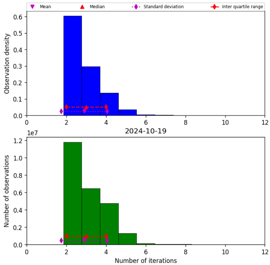
Figure 39: Histogram of “Number of iterations” for 2024-10-19 to 2024-10-20
