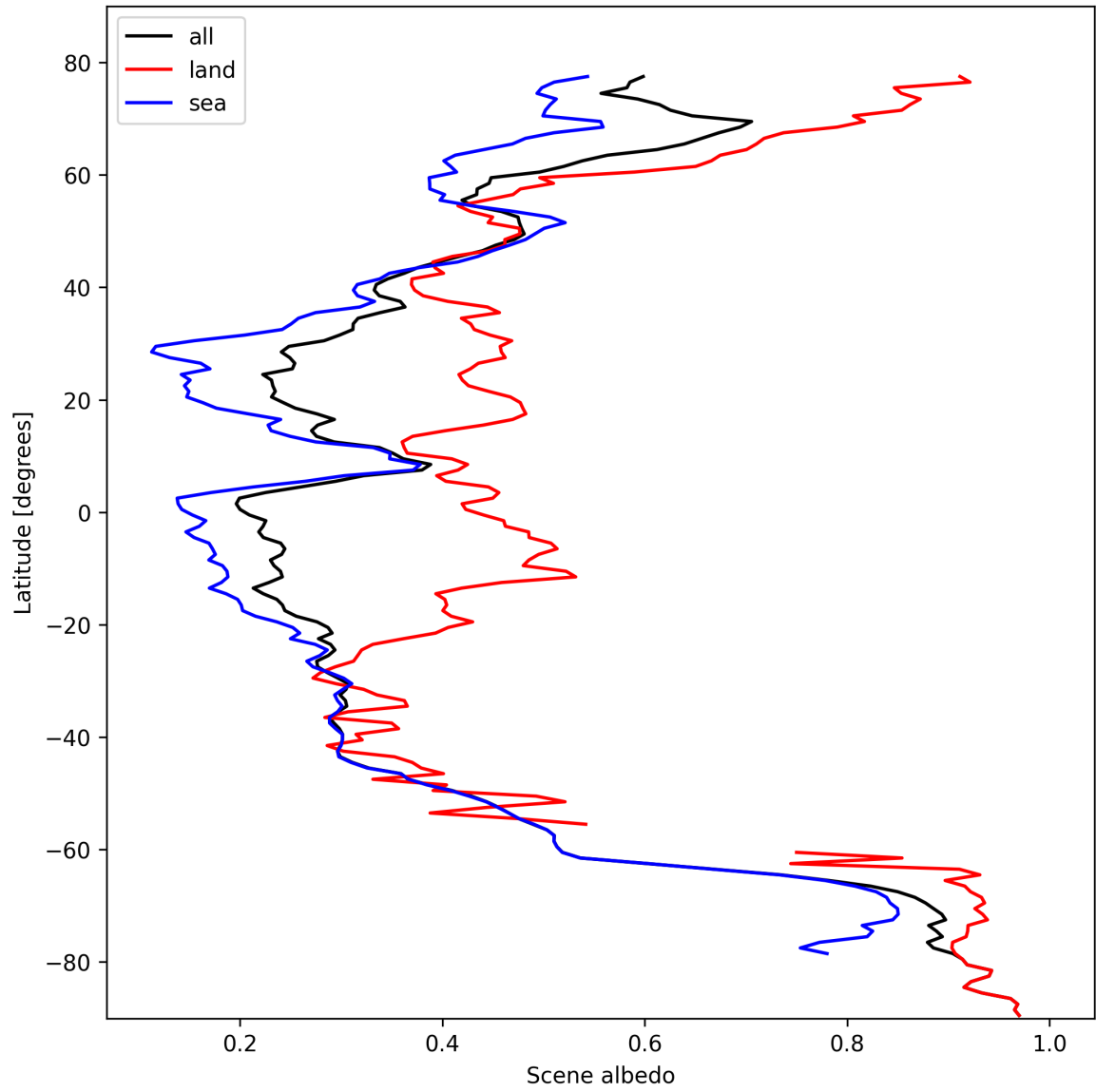
Figure 17: Zonal average of “Scene albedo” for 2024-10-19 to 2024-10-20.
