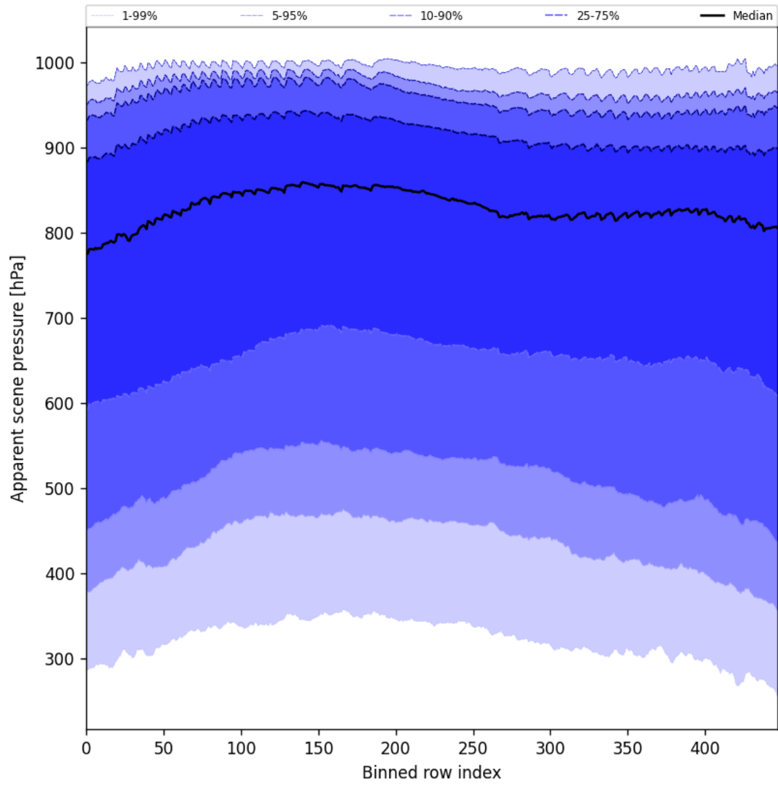
Figure 53: Along track statistics of “Apparent scene pressure” for 2024-10-19 to 2024-10-20
