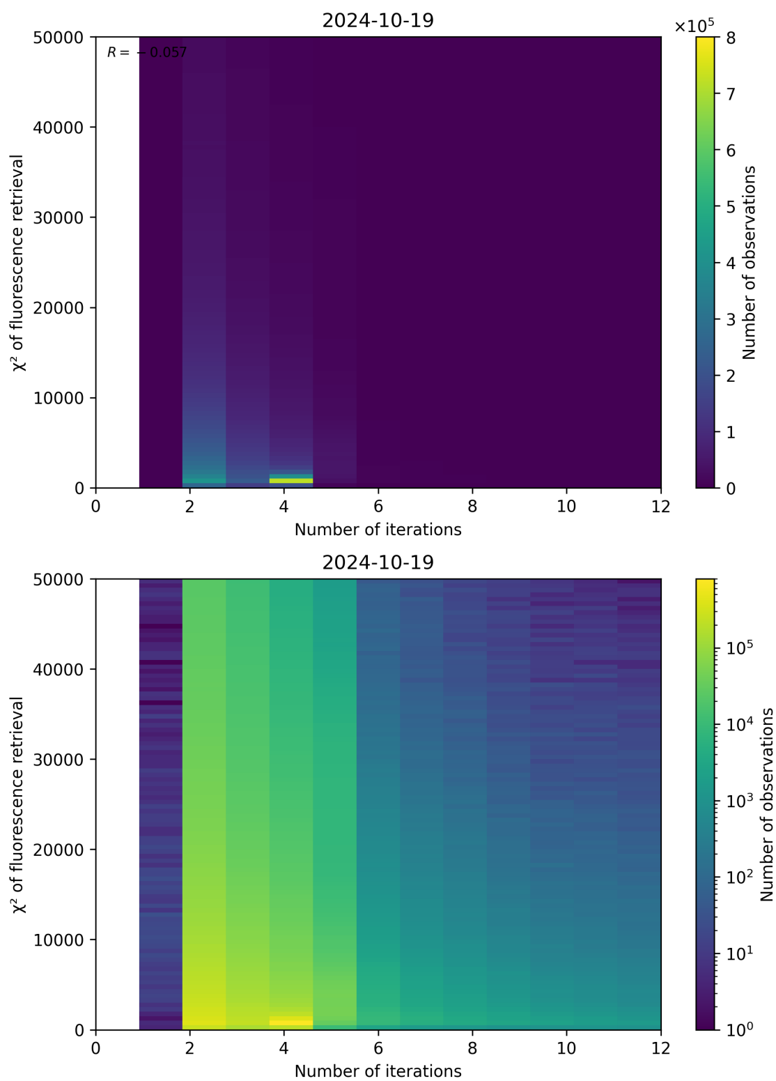
Figure 106: Scatter density plot of “Number of iterations” against “ \chi^2 of fluorescence retrieval” for 2024-10-19 to 2024-10-20.
