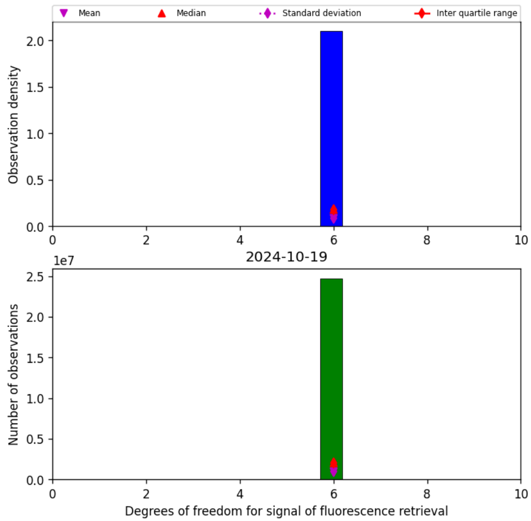
Figure 43: Histogram of “Degrees of freedom for signal of fluorescence retrieval” for 2024-10-19 to 2024-10-20
