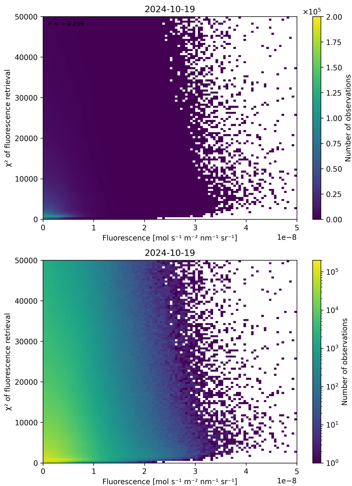
Figure 93: Scatter density plot of “Fluorescence” against “ \chi^2 of fluorescence retrieval” for 2024-10-19 to 2024-10-20.
