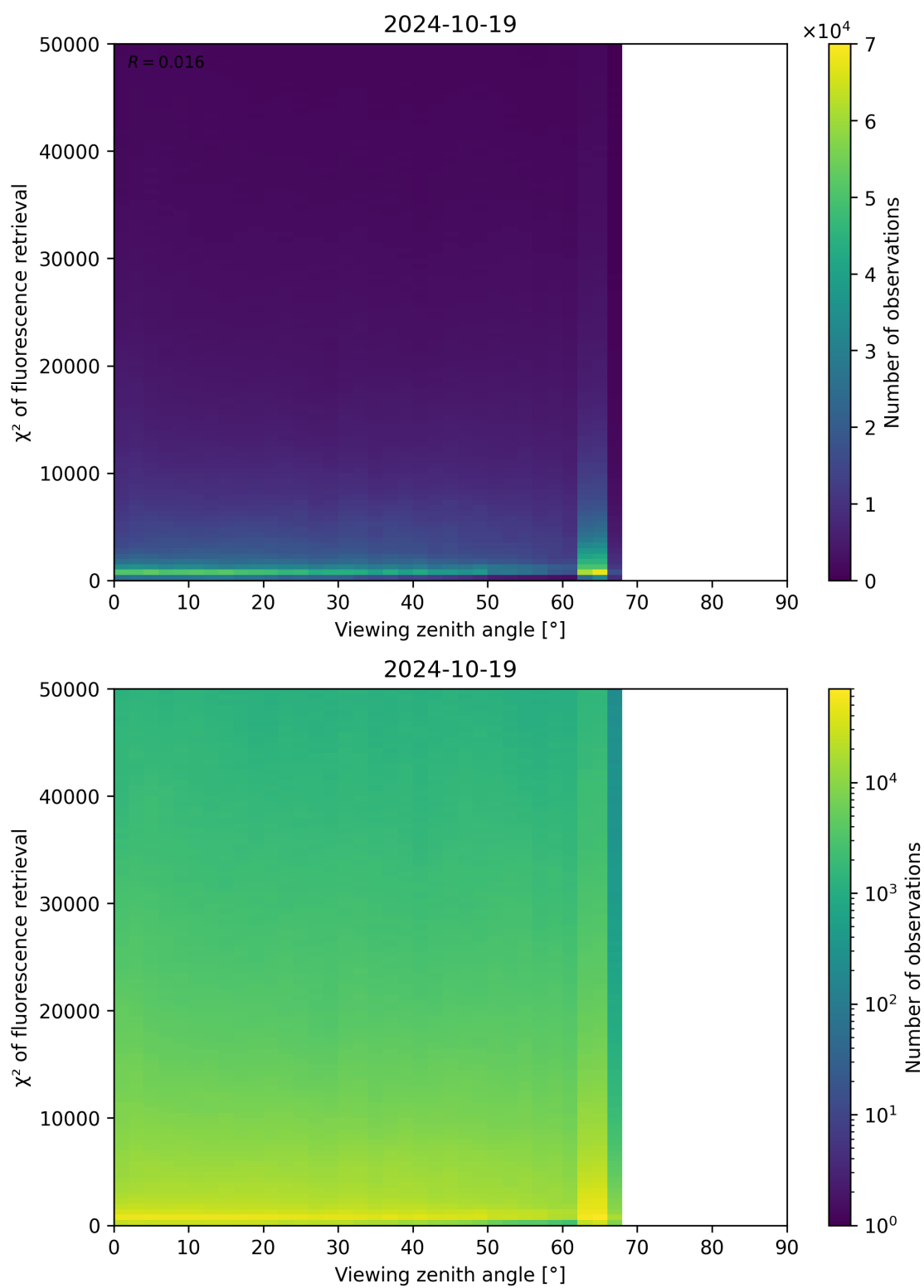
Figure 131: Scatter density plot of “Viewing zenith angle” against “ \chi^2 of fluorescence retrieval” for 2024-10-19 to 2024-10-20.
