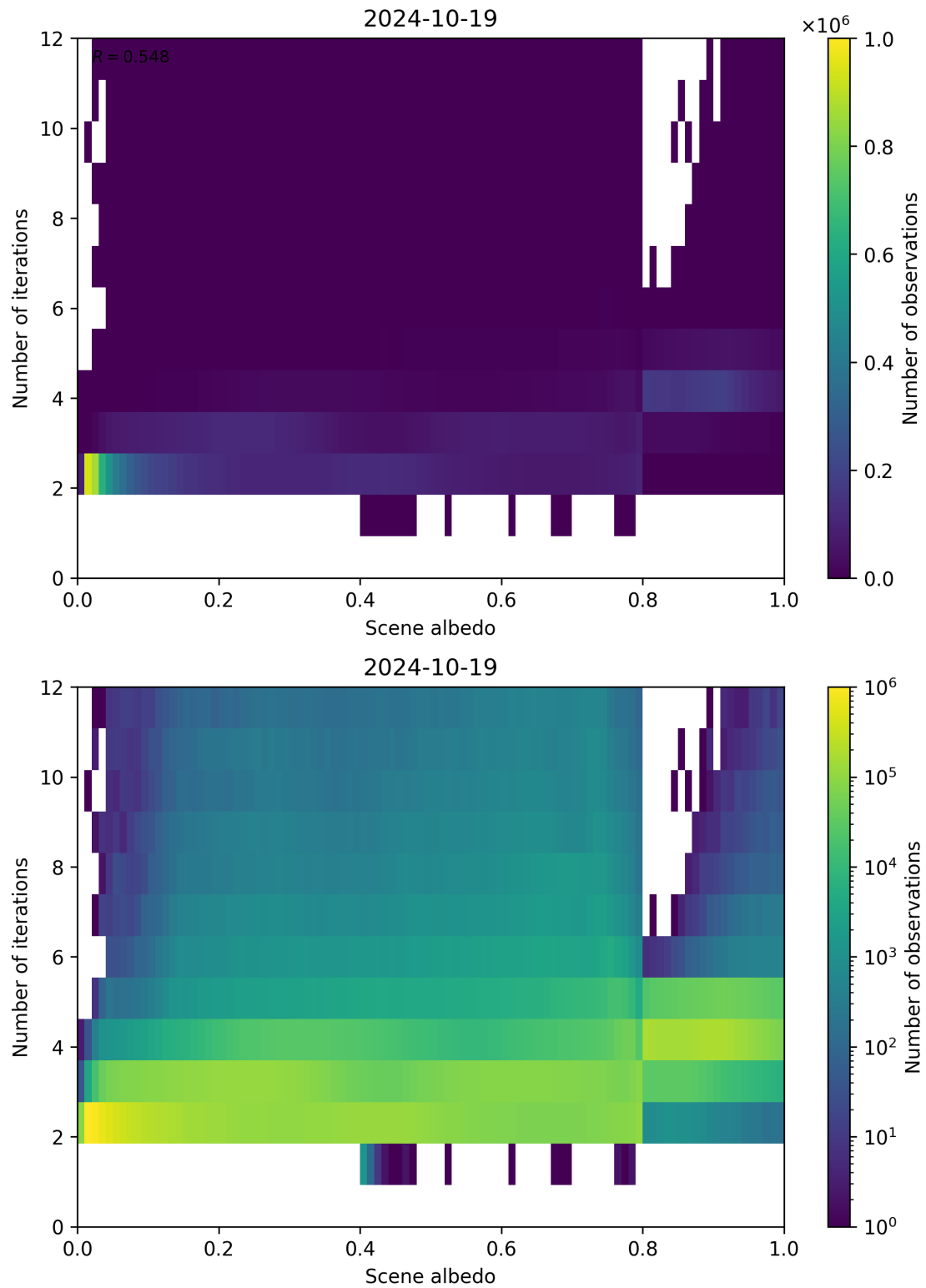
Figure 115: Scatter density plot of “Scene albedo” against “Number of iterations” for 2024-10-19 to 2024-10-20.
