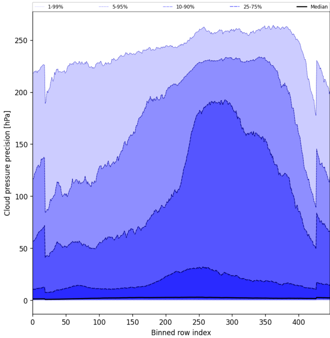
Figure 48: Along track statistics of “Cloud pressure precision” for 2024-10-19 to 2024-10-20
