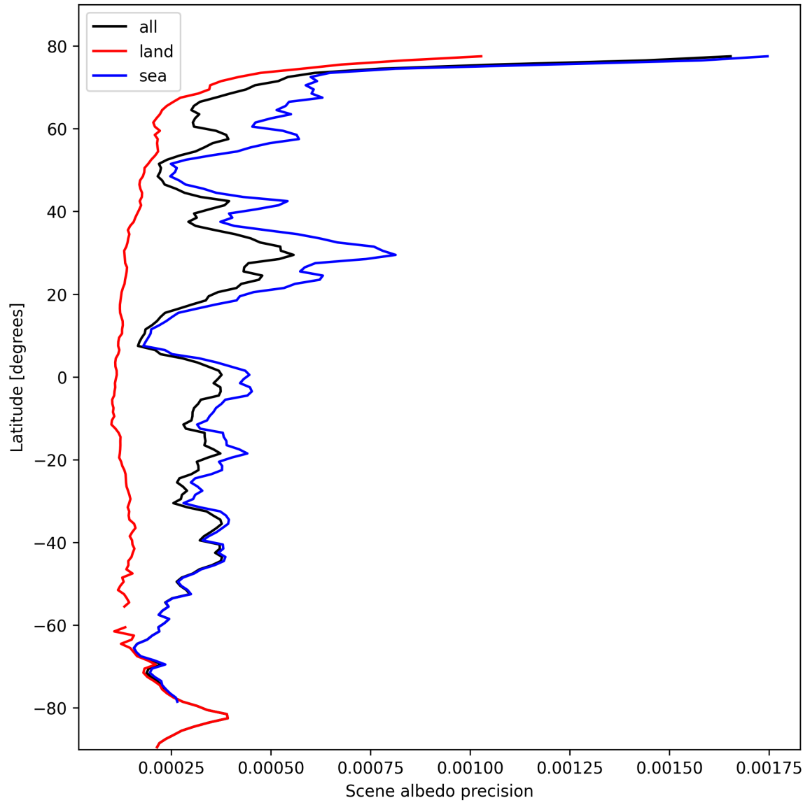
Figure 18: Zonal average of “Scene albedo precision” for 2024-10-19 to 2024-10-20.
