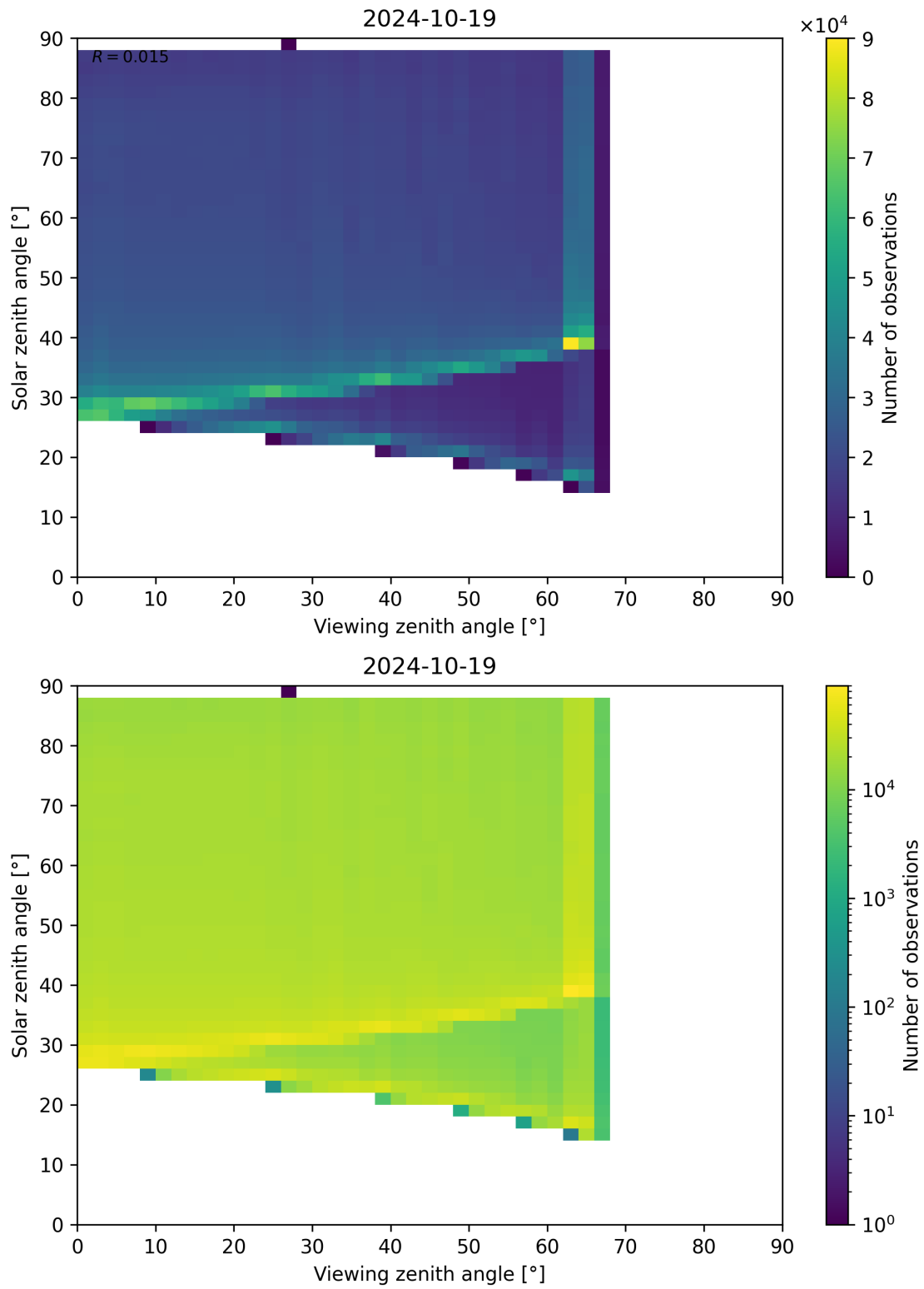
Figure 139: Scatter density plot of “Viewing zenith angle” against “Solar zenith angle” for 2024-10-19 to 2024-10-20.
