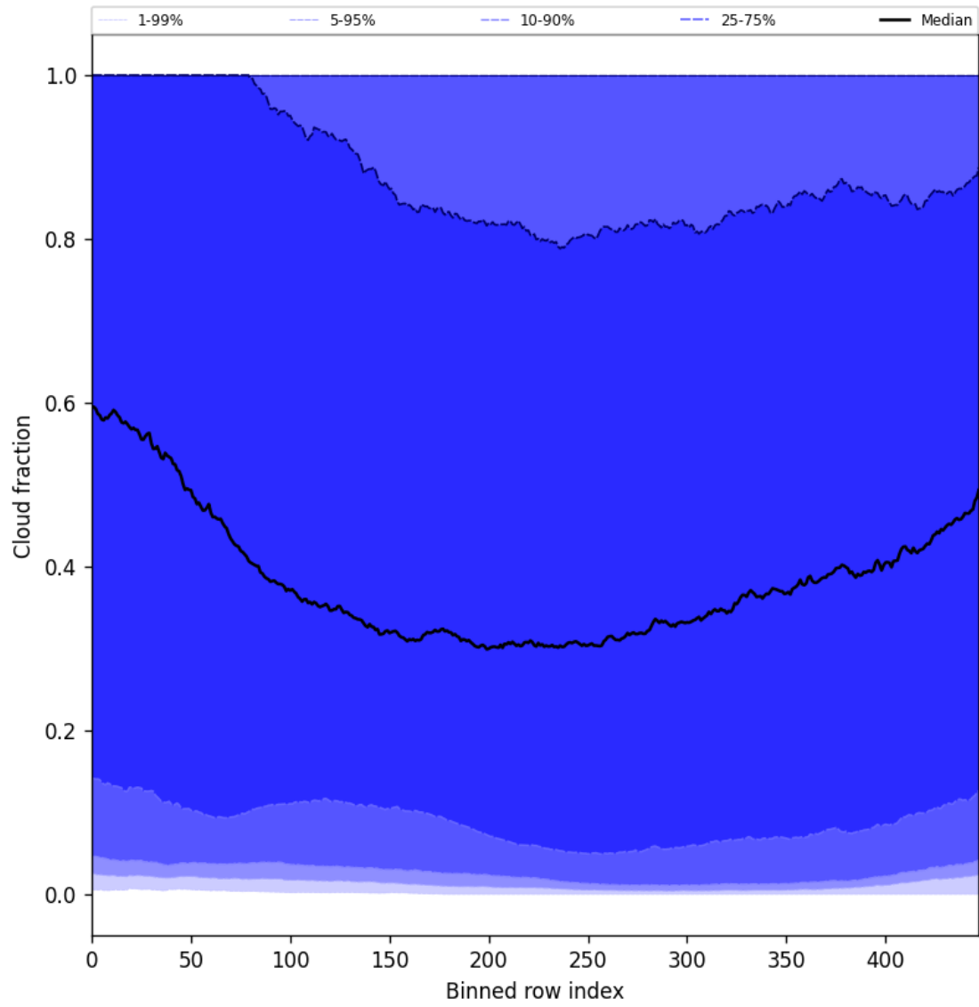
Figure 49: Along track statistics of “Cloud fraction” for 2024-10-19 to 2024-10-20
