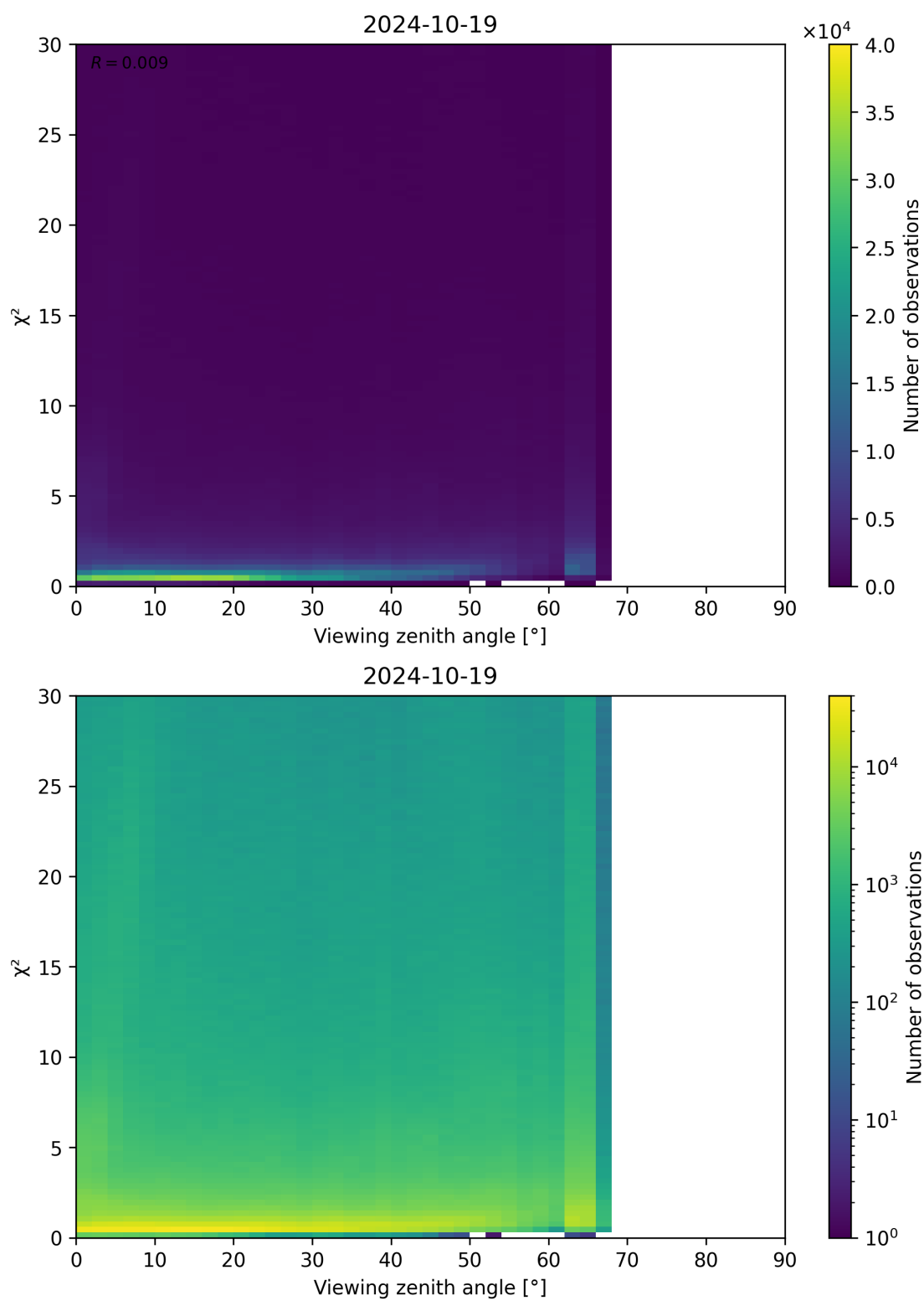
Figure 130: Scatter density plot of “Viewing zenith angle” against “ \chi^2 ” for 2024-10-19 to 2024-10-20.
