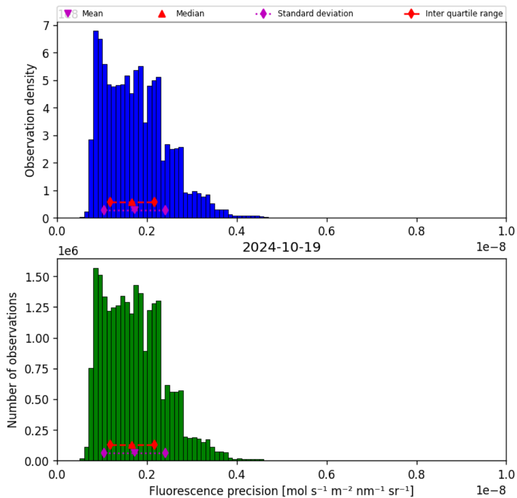
Figure 41: Histogram of “Fluorescence precision” for 2024-10-19 to 2024-10-20
