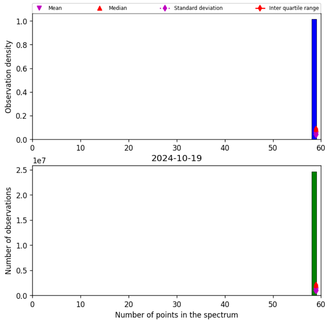
Figure 44: Histogram of “Number of points in the spectrum” for 2024-10-19 to 2024-10-20
