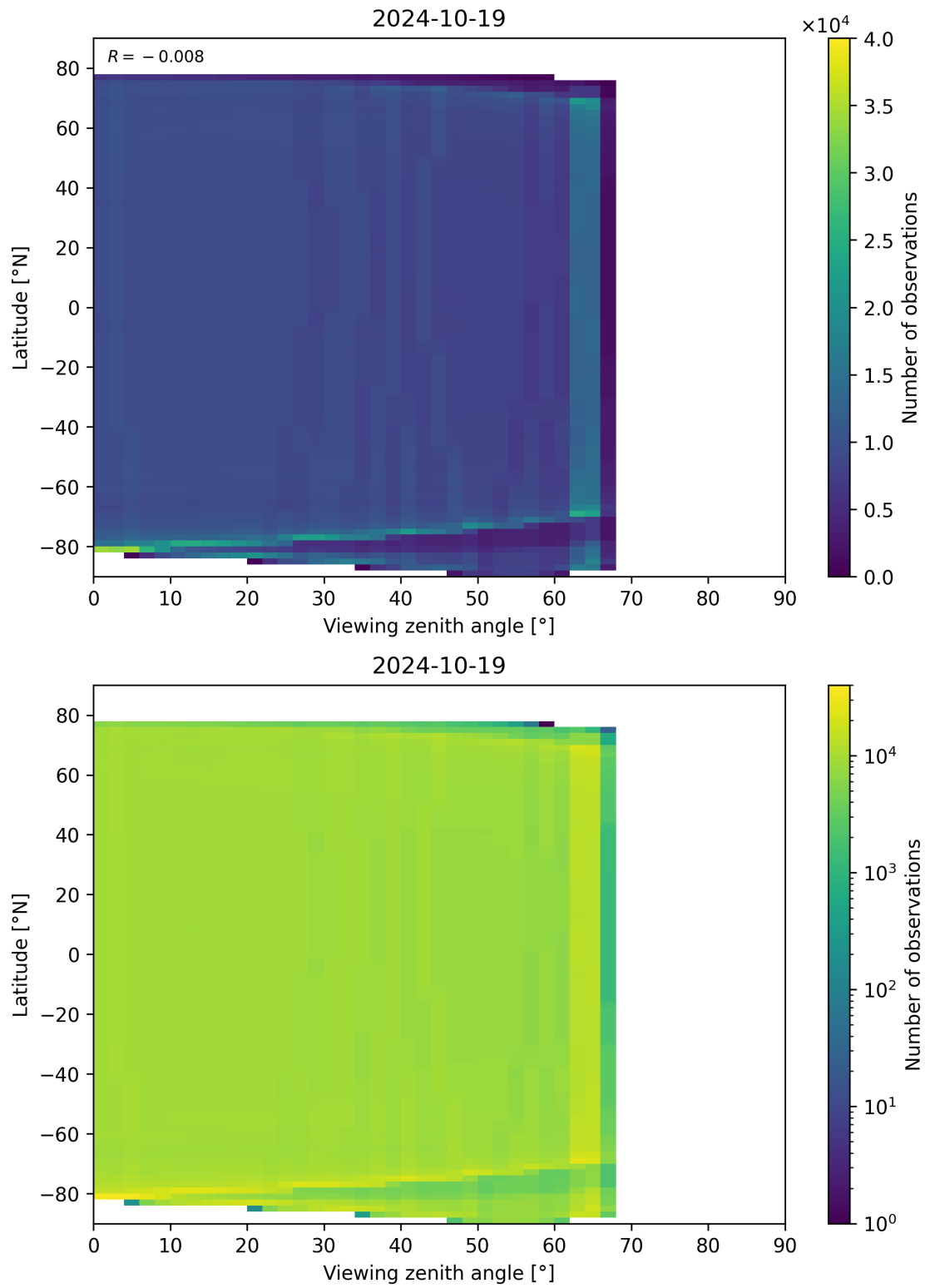
Figure 135: Scatter density plot of “Viewing zenith angle” against “Latitude” for 2024-10-19 to 2024-10-20.
