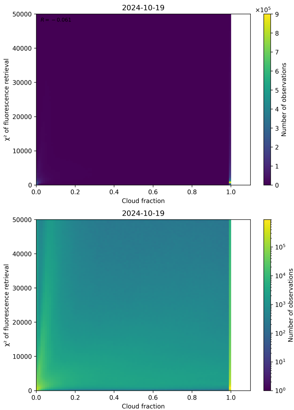
Figure 78: Scatter density plot of “Cloud fraction” against “ \chi^2 of fluorescence retrieval” for 2024-10-19 to 2024-10-20.
