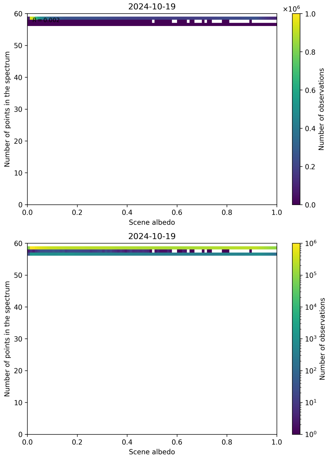
Figure 116: Scatter density plot of “Scene albedo” against “Number of points in the spectrum” for 2024-10-19 to 2024-10-20.
