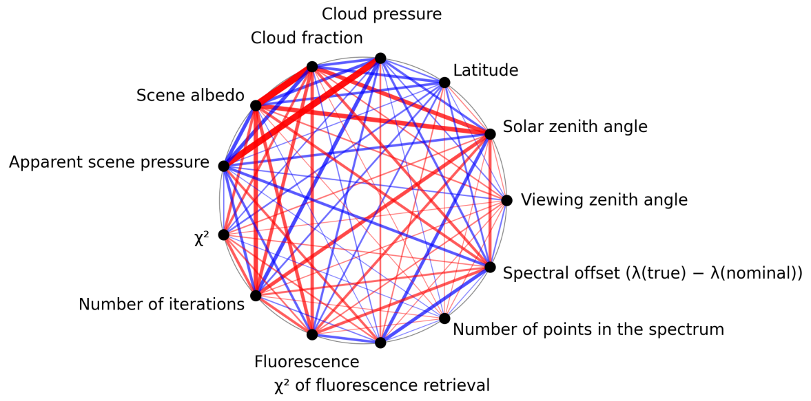
Figure 1: Map of correlation graph for 2024-10-19 to 2024-10-20.
