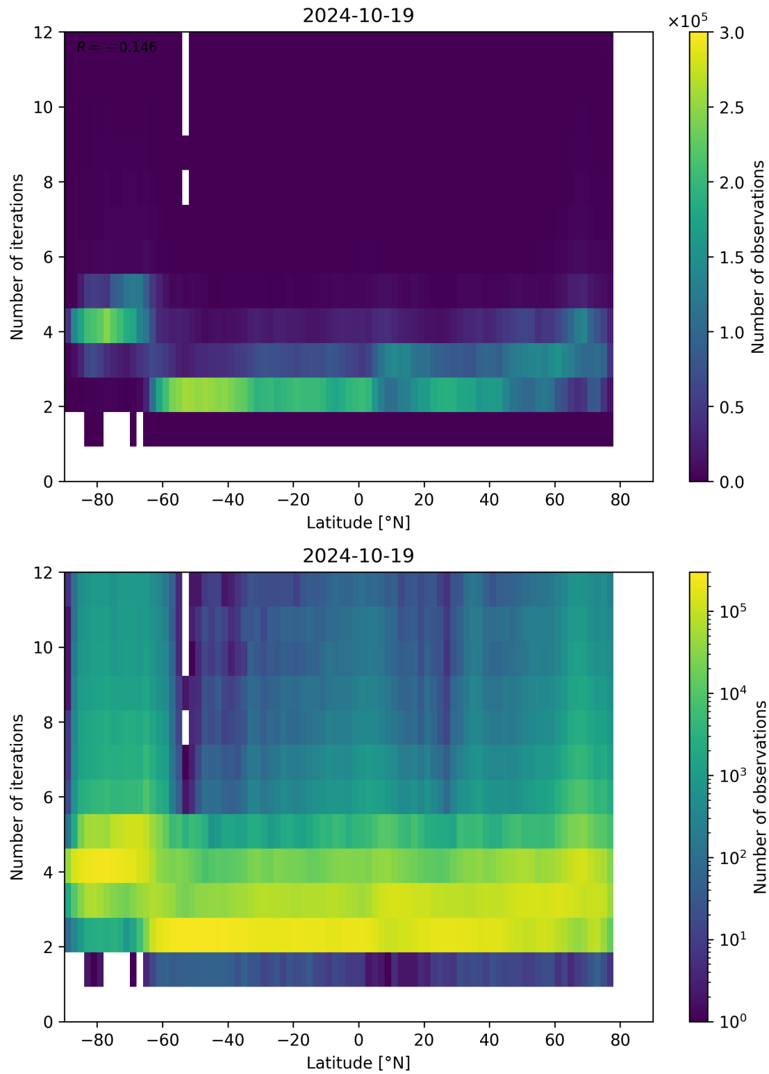
Figure 102: Scatter density plot of “Latitude” against “Number of iterations” for 2024-10-19 to 2024-10-20.
