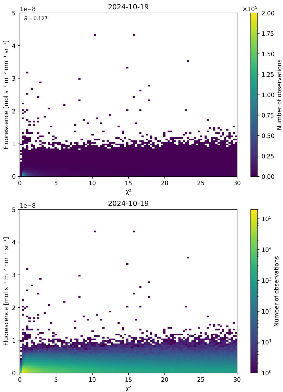
Figure 70: Scatter density plot of “ \chi^2 ” against “Fluorescence” for 2024-10-19 to 2024-10-20.
