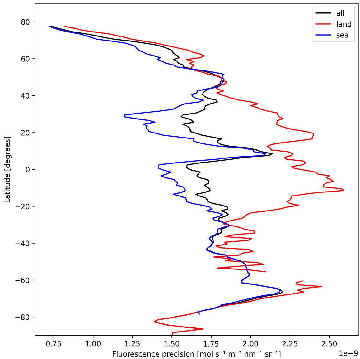
Figure 24: Zonal average of “Fluorescence precision” for 2024-10-19 to 2024-10-20.
