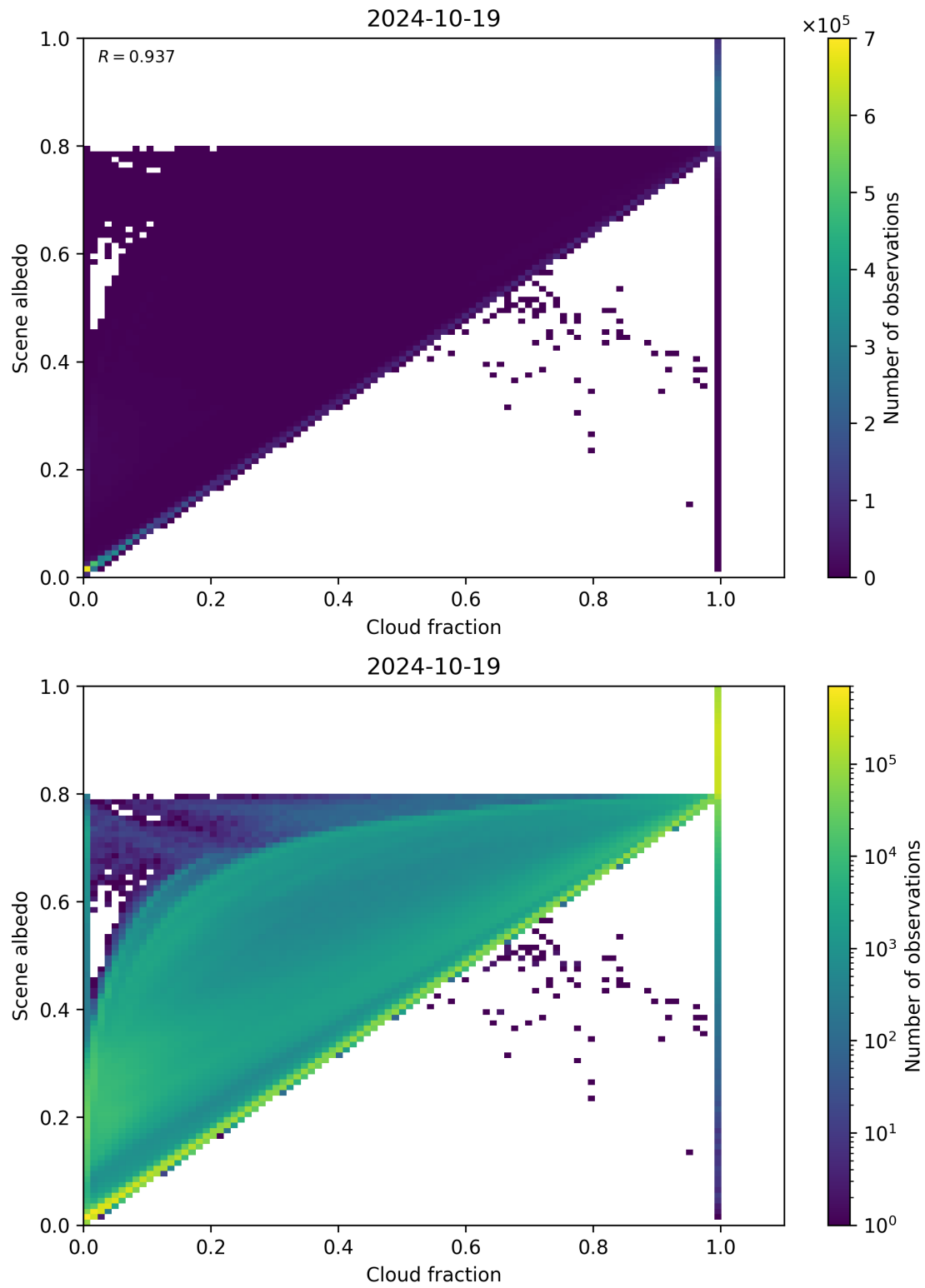
Figure 82: Scatter density plot of “Cloud fraction” against “Scene albedo” for 2024-10-19 to 2024-10-20.
