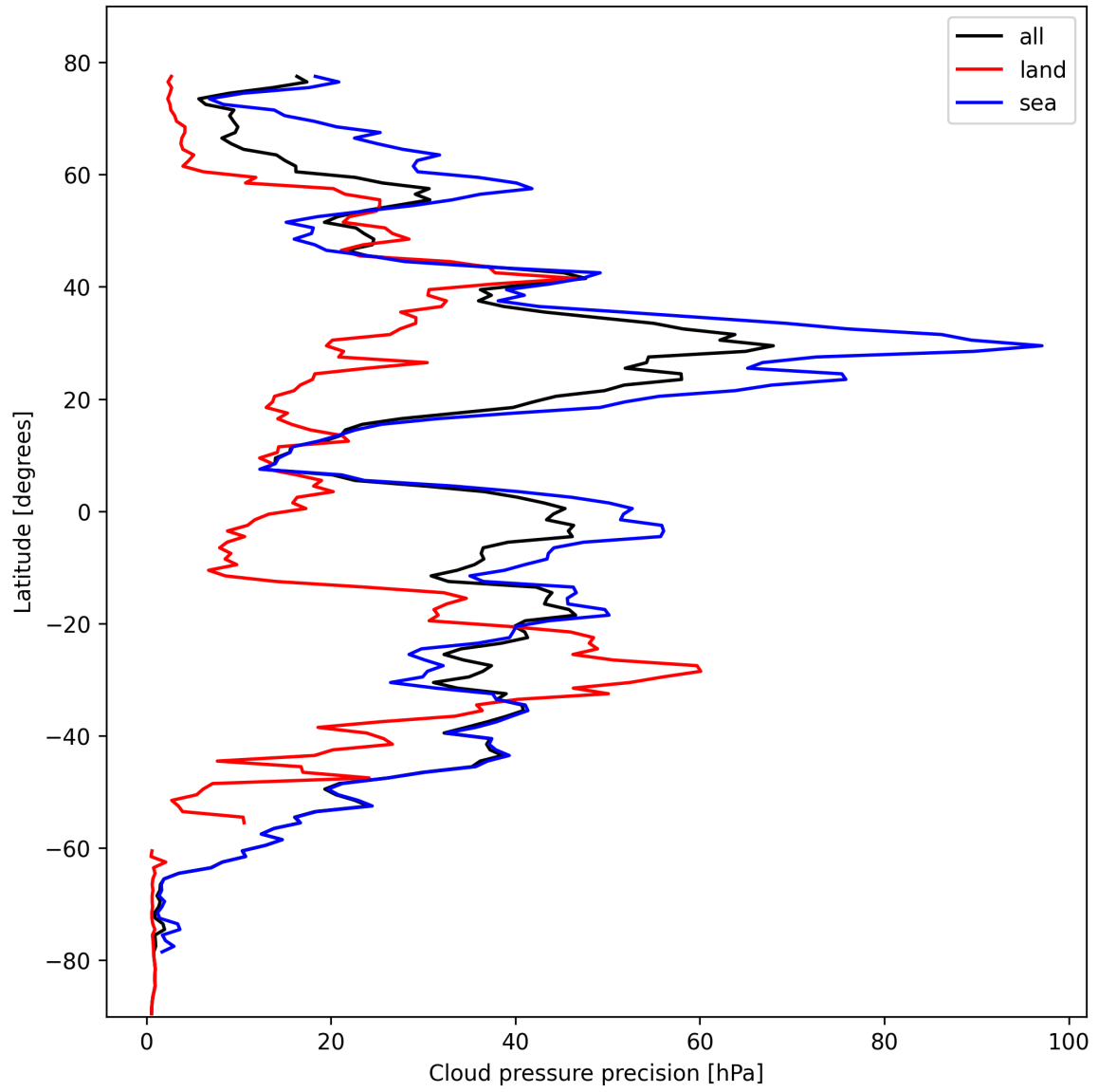
Figure 14: Zonal average of “Cloud pressure precision” for 2024-10-19 to 2024-10-20.
