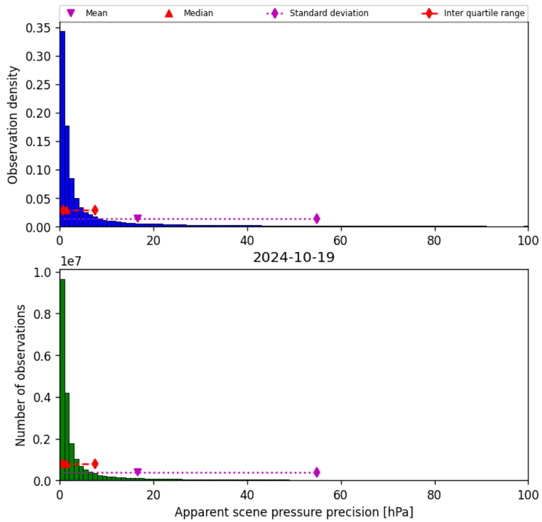
Figure 37: Histogram of “Apparent scene pressure precision” for 2024-10-19 to 2024-10-20
