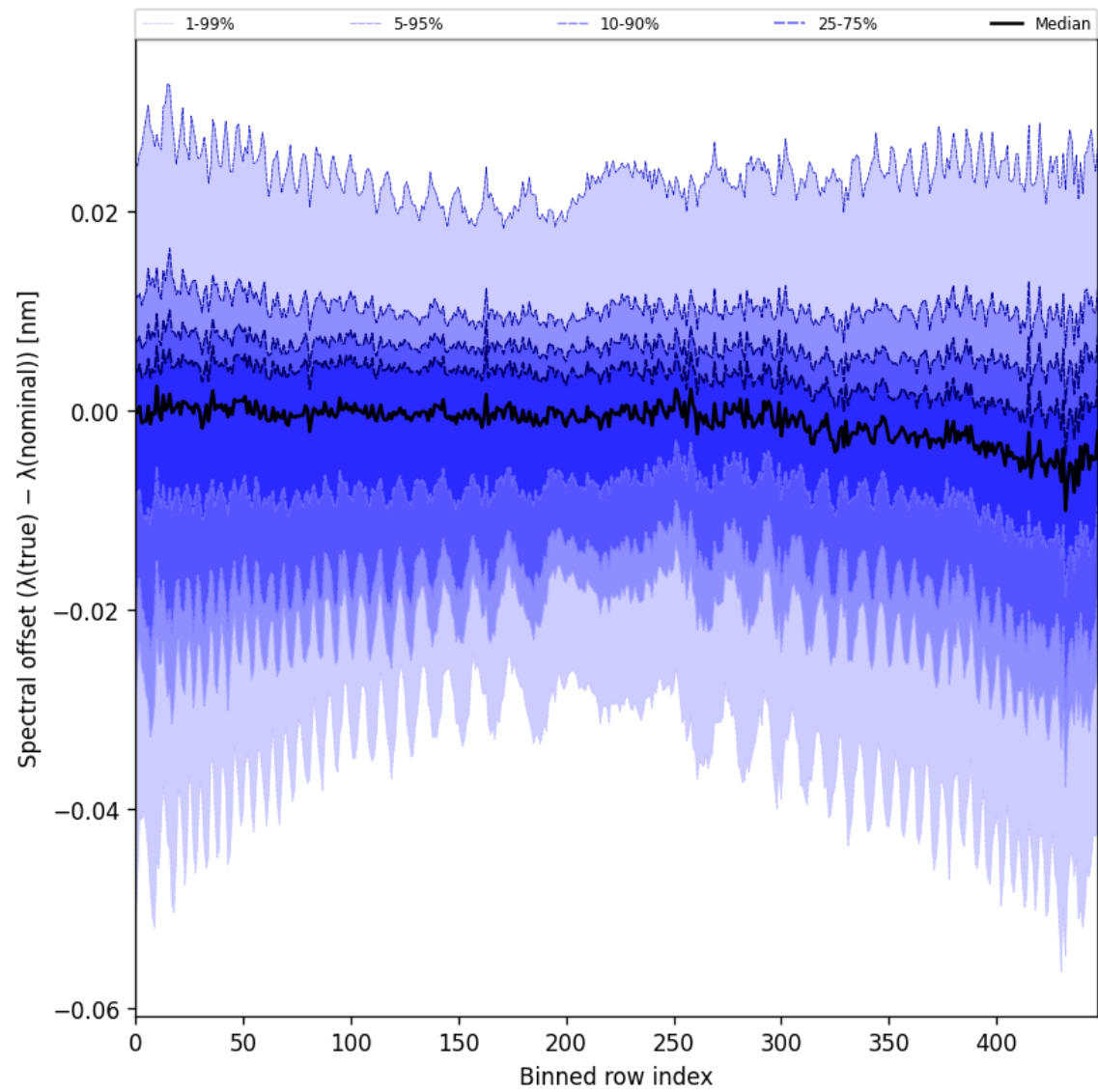
Figure 62: Along track statistics of “Spectral offset ( \lambda_{\text{true}} - \lambda_{\text{nominal}} )” for 2024-10-19 to 2024-10-20
