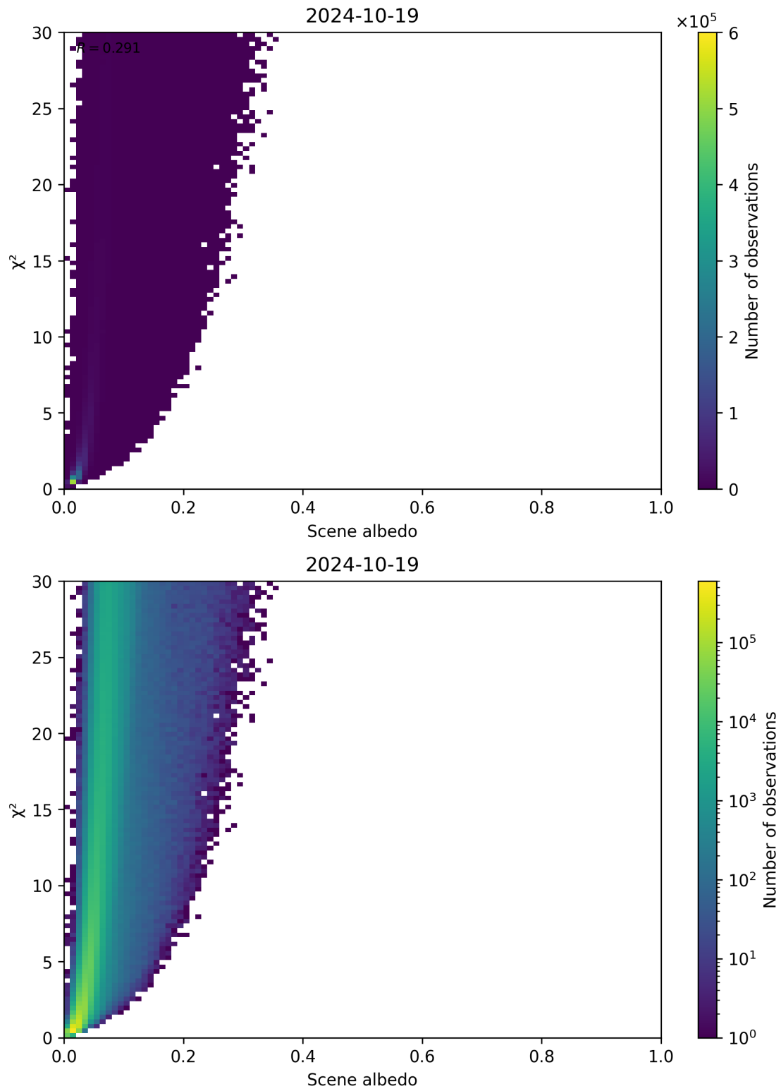
Figure 112: Scatter density plot of “Scene albedo” against “ \chi^2 ” for 2024-10-19 to 2024-10-20.
