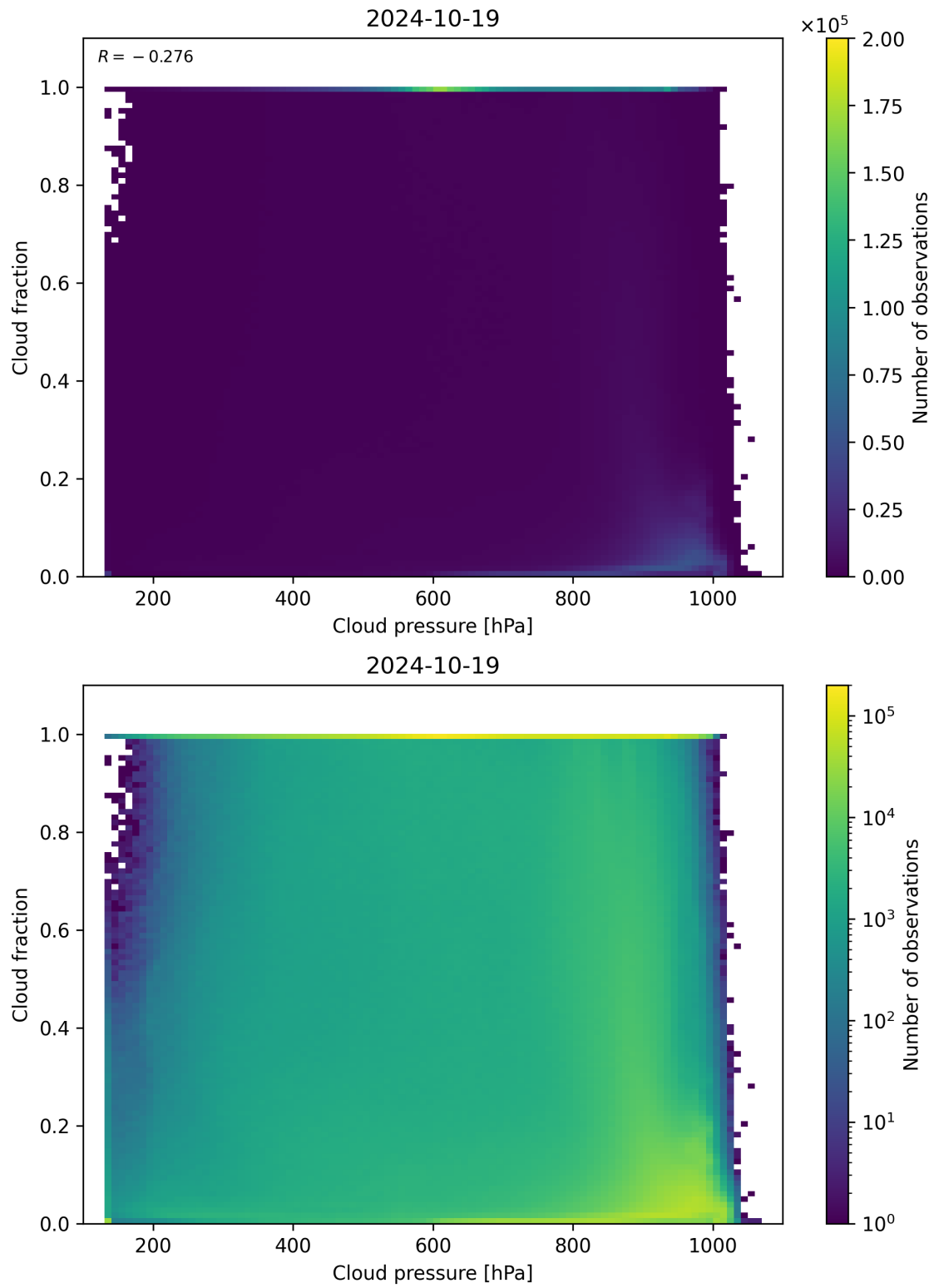
Figure 87: Scatter density plot of “Cloud pressure” against “Cloud fraction” for 2024-10-19 to 2024-10-20.
