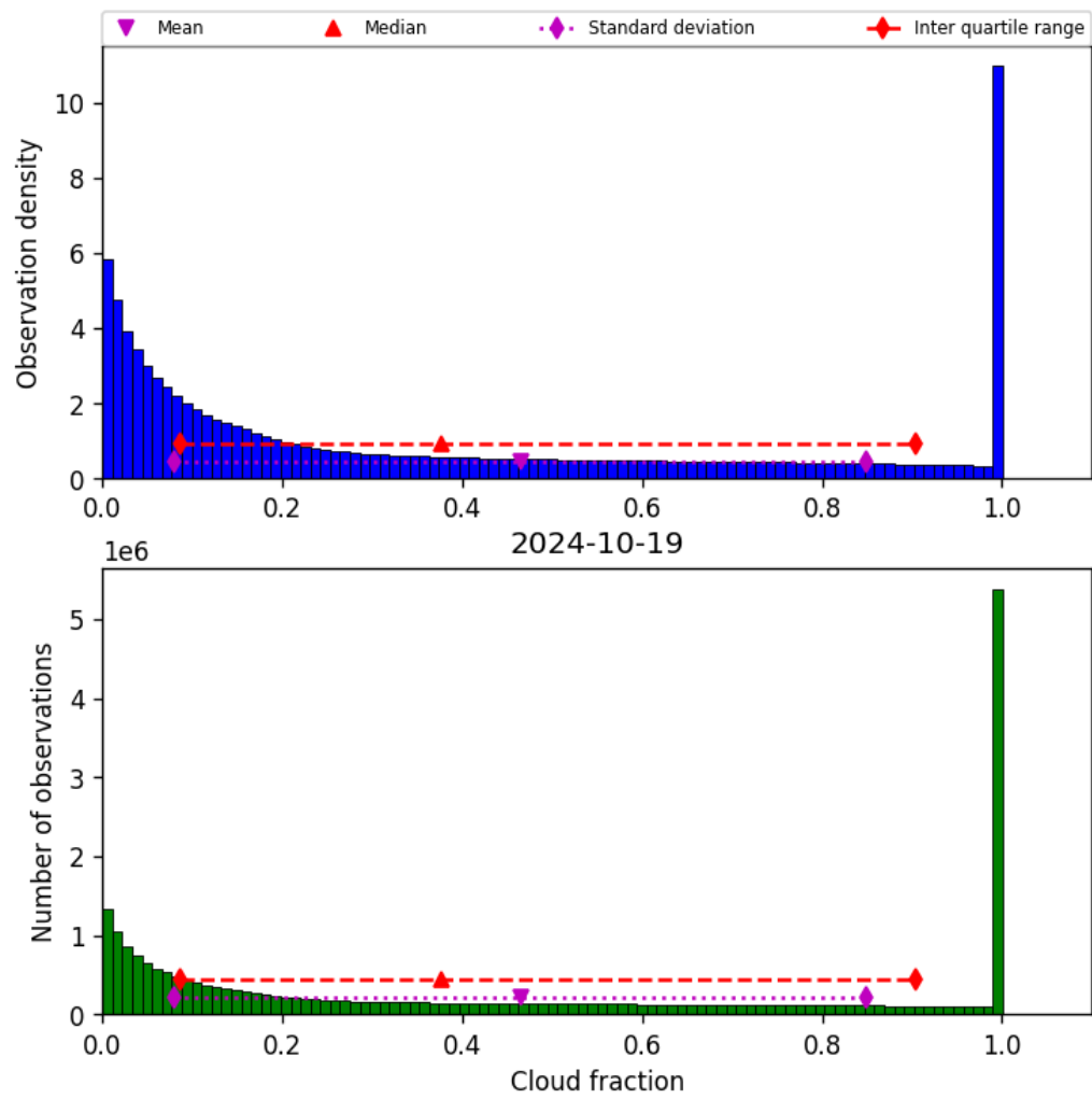
Figure 32: Histogram of “Cloud fraction” for 2024-10-19 to 2024-10-20
