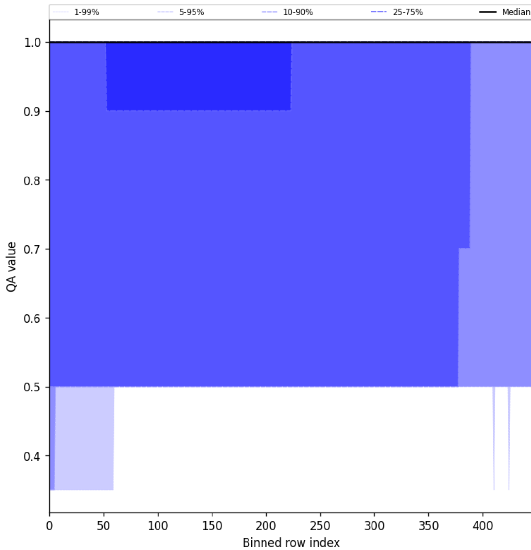
Figure 46: Along track statistics of “QA value” for 2024-10-19 to 2024-10-20
