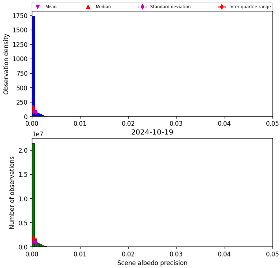
Figure 35: Histogram of “Scene albedo precision” for 2024-10-19 to 2024-10-20
