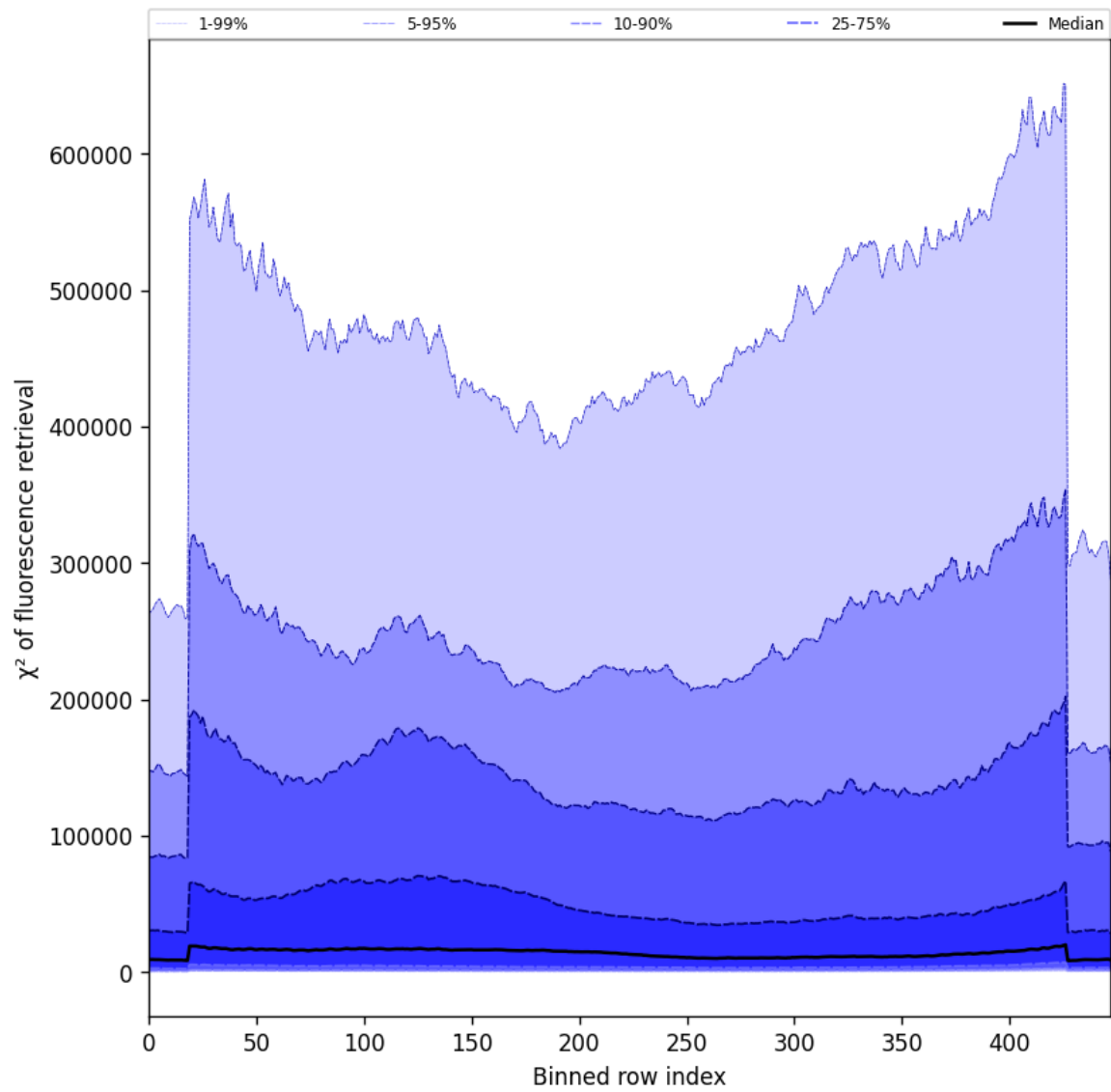
Figure 59: Along track statistics of “ \chi^2 of fluorescence retrieval” for 2024-10-19 to 2024-10-20
