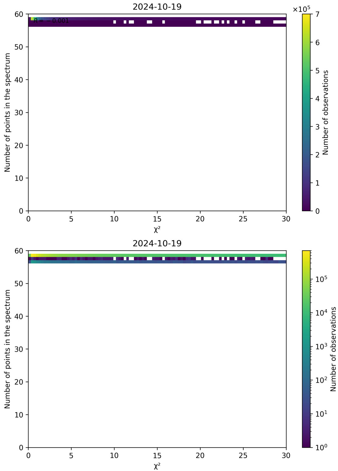
Figure 74: Scatter density plot of “ \chi^2 ” against “Number of points in the spectrum” for 2024-10-19 to 2024-10-20.
