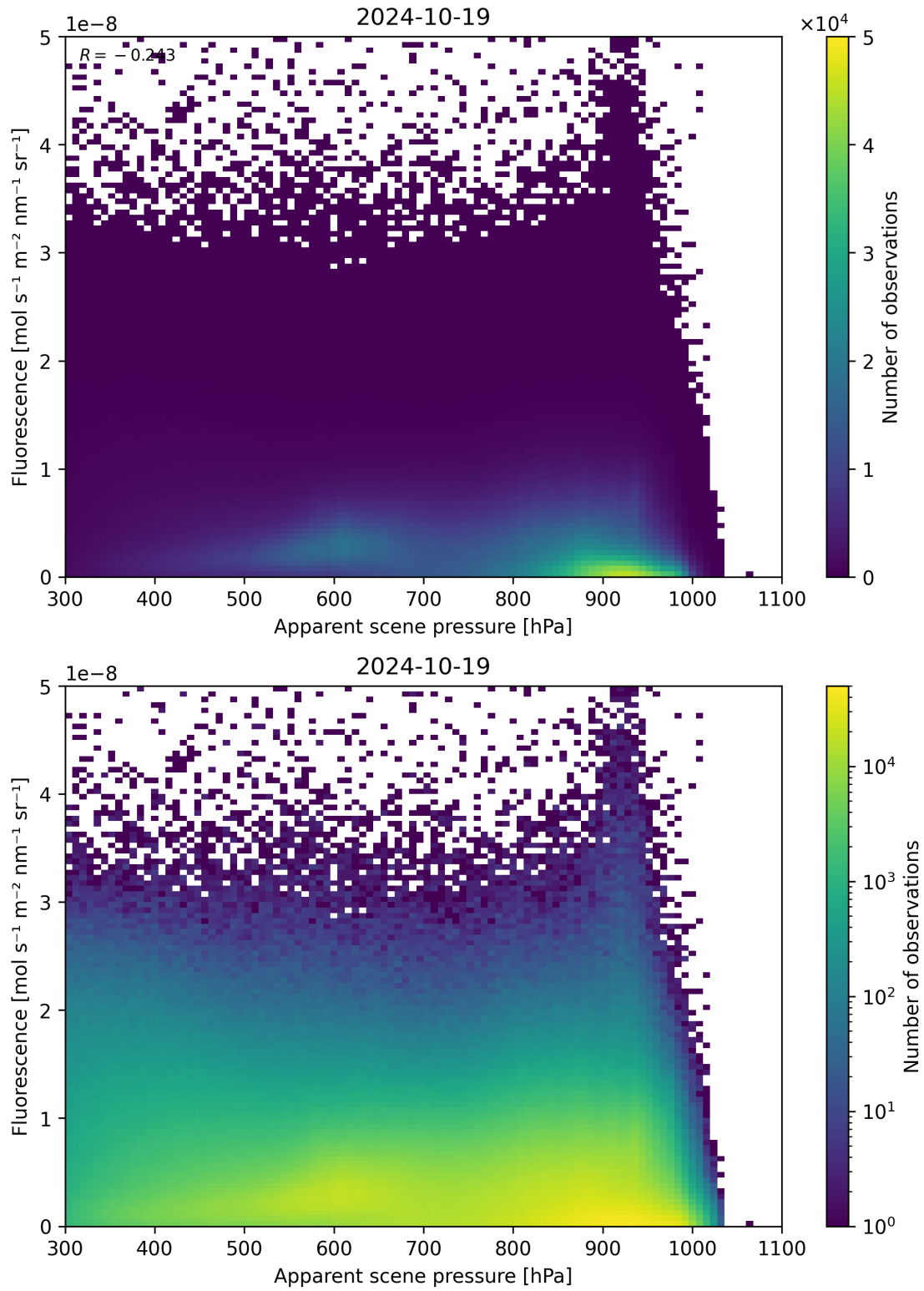
Figure 65: Scatter density plot of “Apparent scene pressure” against “Fluorescence” for 2024-10-19 to 2024-10-20.
