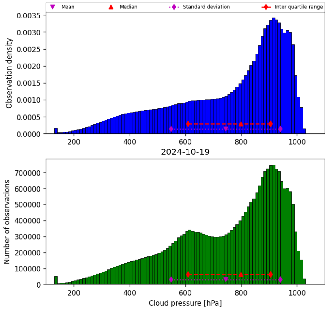
Figure 30: Histogram of “Cloud pressure” for 2024-10-19 to 2024-10-20
