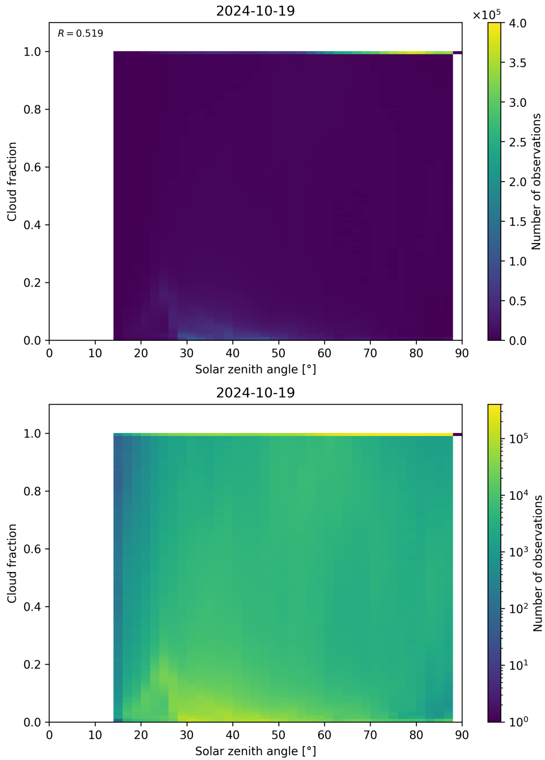
Figure 121: Scatter density plot of “Solar zenith angle” against “Cloud fraction” for 2024-10-19 to 2024-10-20.
