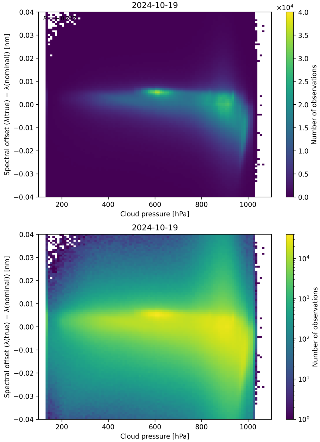
Figure 92: Scatter density plot of “Cloud pressure” against “Spectral offset ( \lambda_{\text{true}} - \lambda_{\text{nominal}} )” for 2024-10-19 to 2024-10-20.
