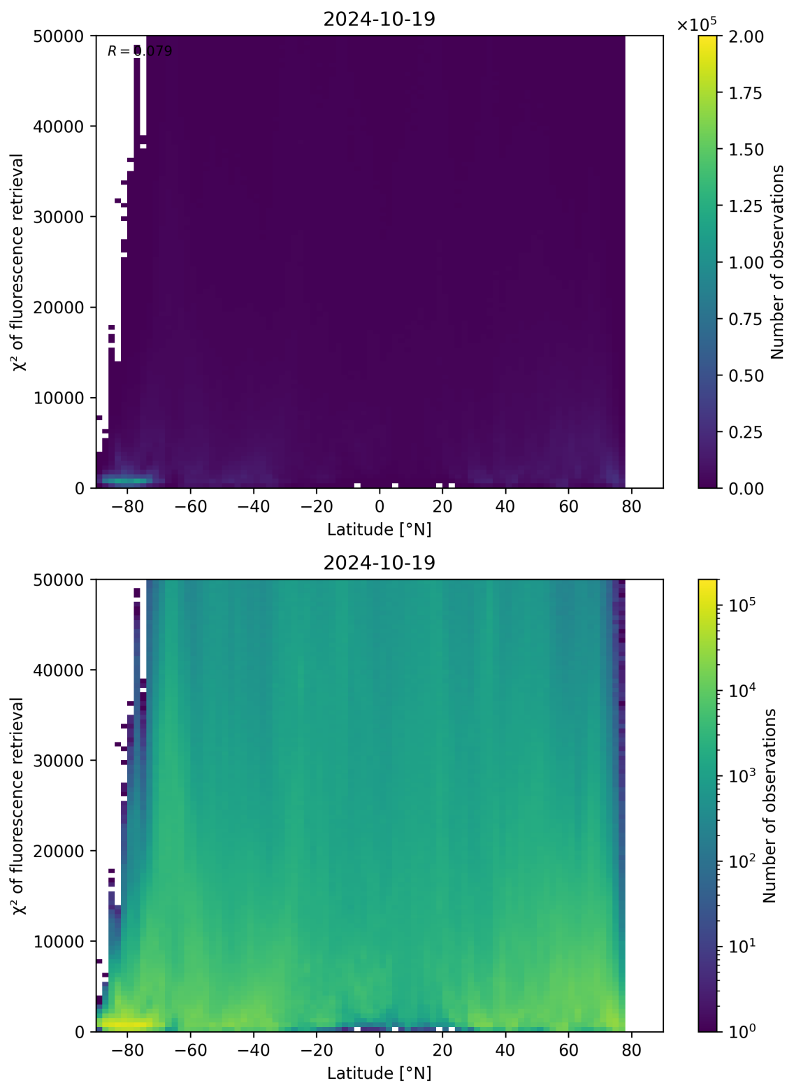
Figure 98: Scatter density plot of “Latitude” against “ \chi^2 of fluorescence retrieval” for 2024-10-19 to 2024-10-20.
