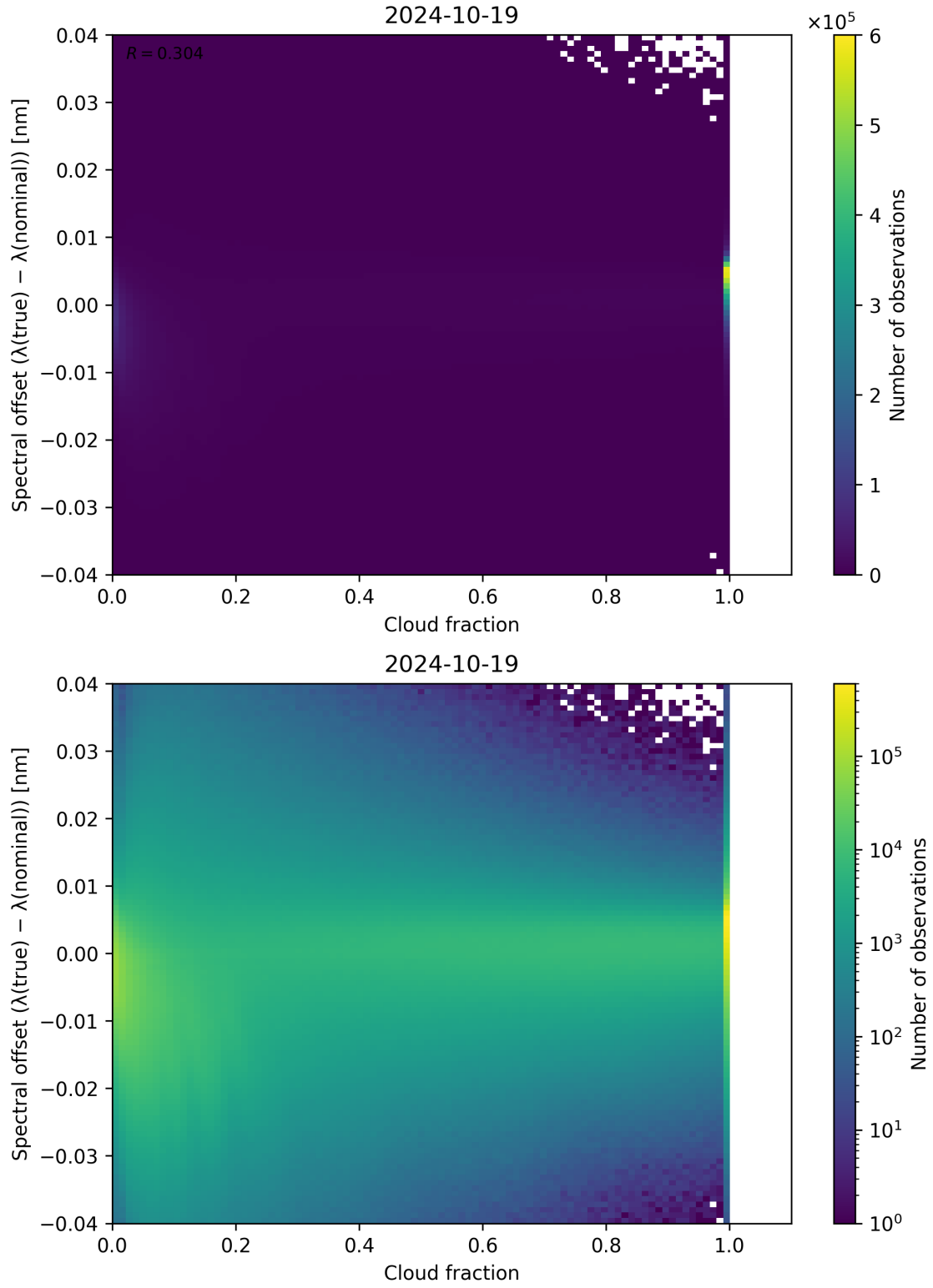
Figure 83: Scatter density plot of “Cloud fraction” against “Spectral offset ( \lambda_{\text{true}} - \lambda_{\text{nominal}} )” for 2024-10-19 to 2024-10-20.
