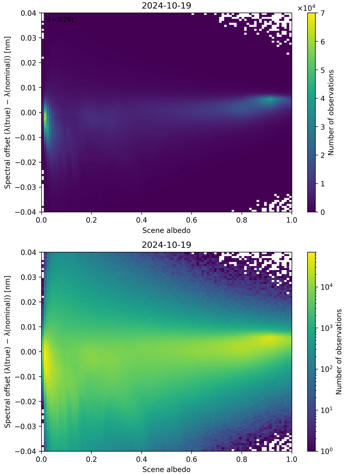
Figure 117: Scatter density plot of “Scene albedo” against “Spectral offset ( \lambda_{\text{true}} - \lambda_{\text{nominal}} )” for 2024-10-19 to 2024-10-20.
