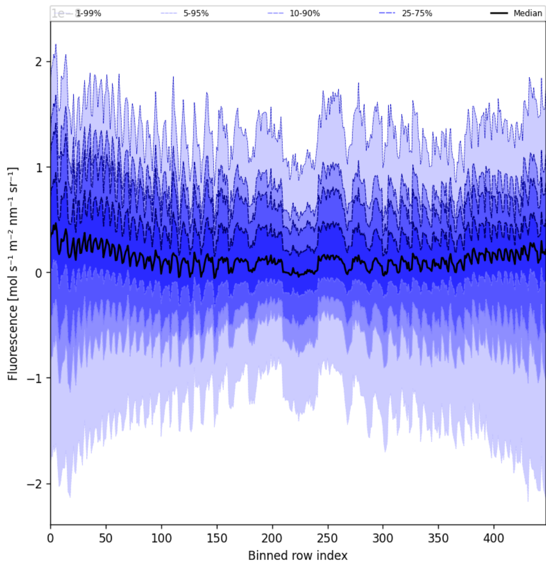
Figure 57: Along track statistics of “Fluorescence” for 2024-10-19 to 2024-10-20
