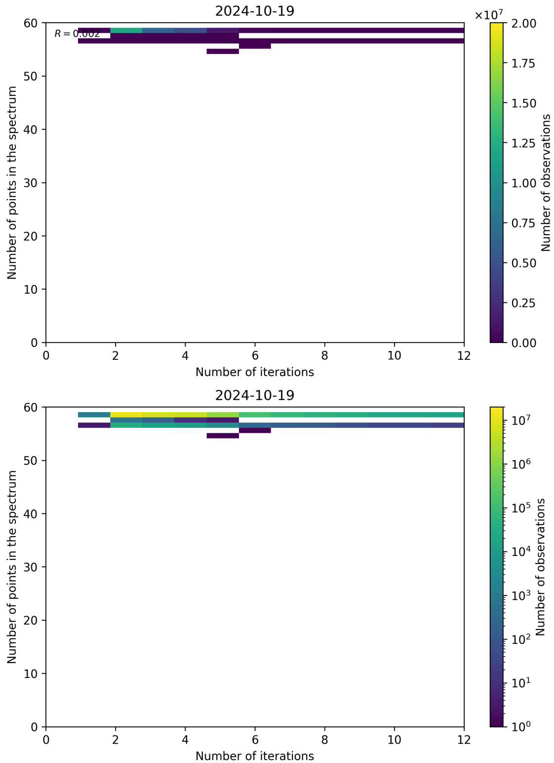
Figure 108: Scatter density plot of “Number of iterations” against “Number of points in the spectrum” for 2024-10-19 to 2024-10-20.
