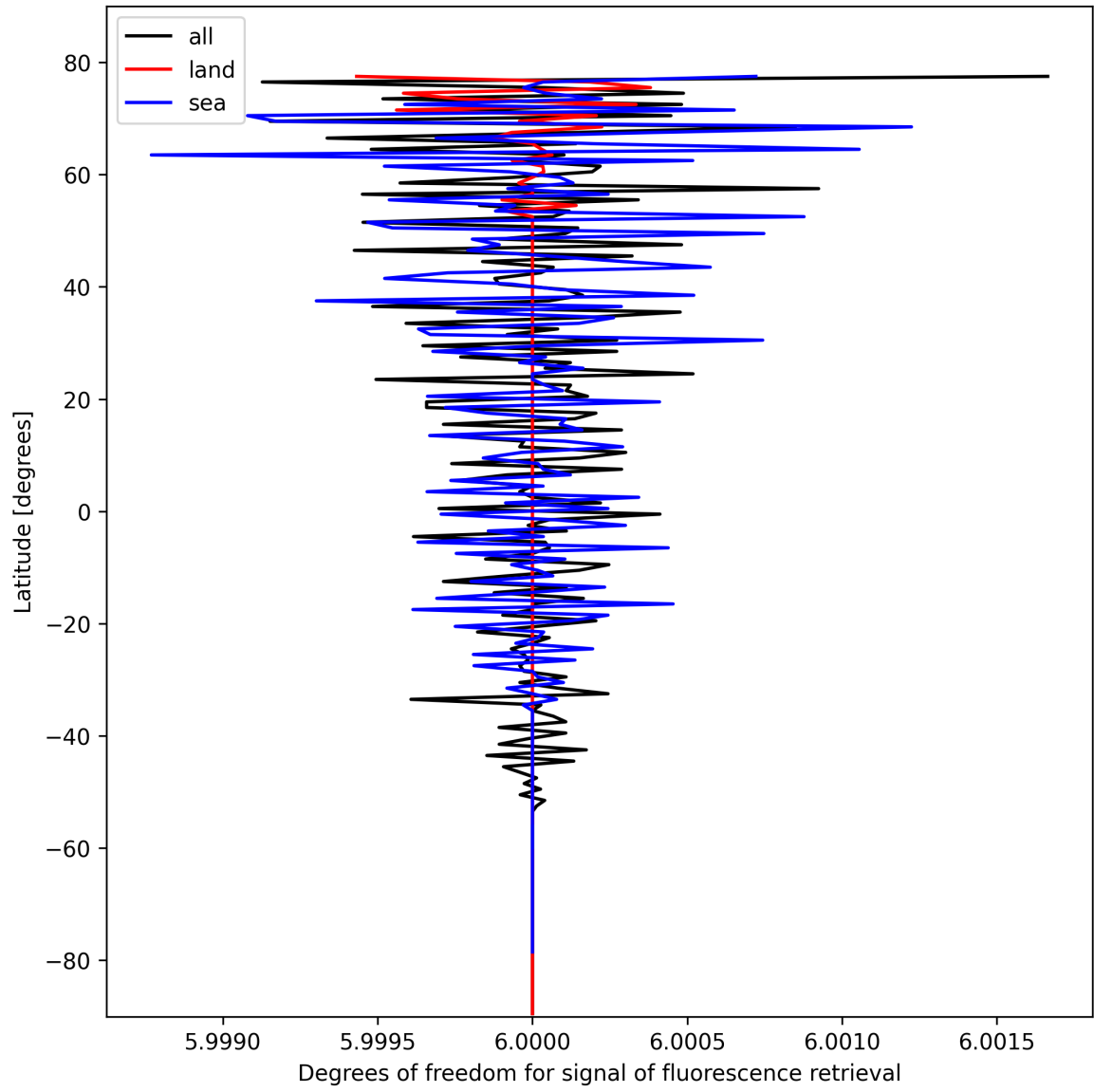
Figure 26: Zonal average of “Degrees of freedom for signal of fluorescence retrieval” for 2024-10-19 to 2024-10-20.
