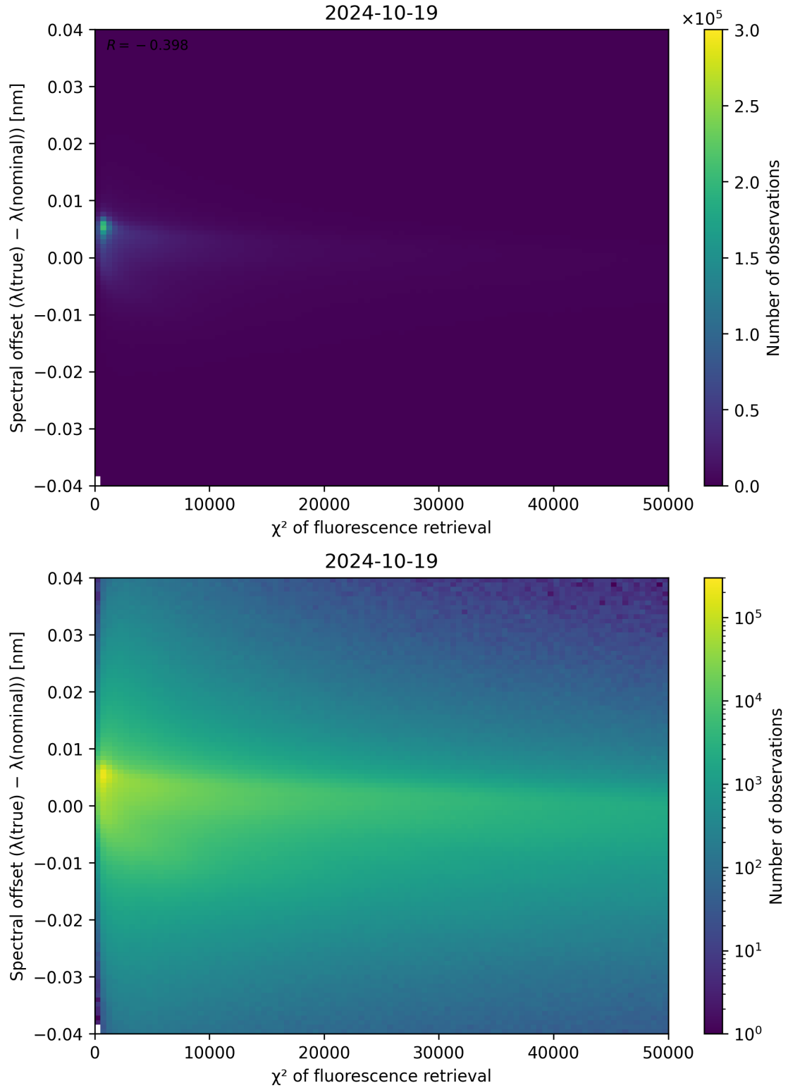
Figure 72: Scatter density plot of “ \chi^2 of fluorescence retrieval” against “Spectral offset ( \lambda_{\text{true}} - \lambda_{\text{nominal}} )” for 2024-10-19 to 2024-10-20.
