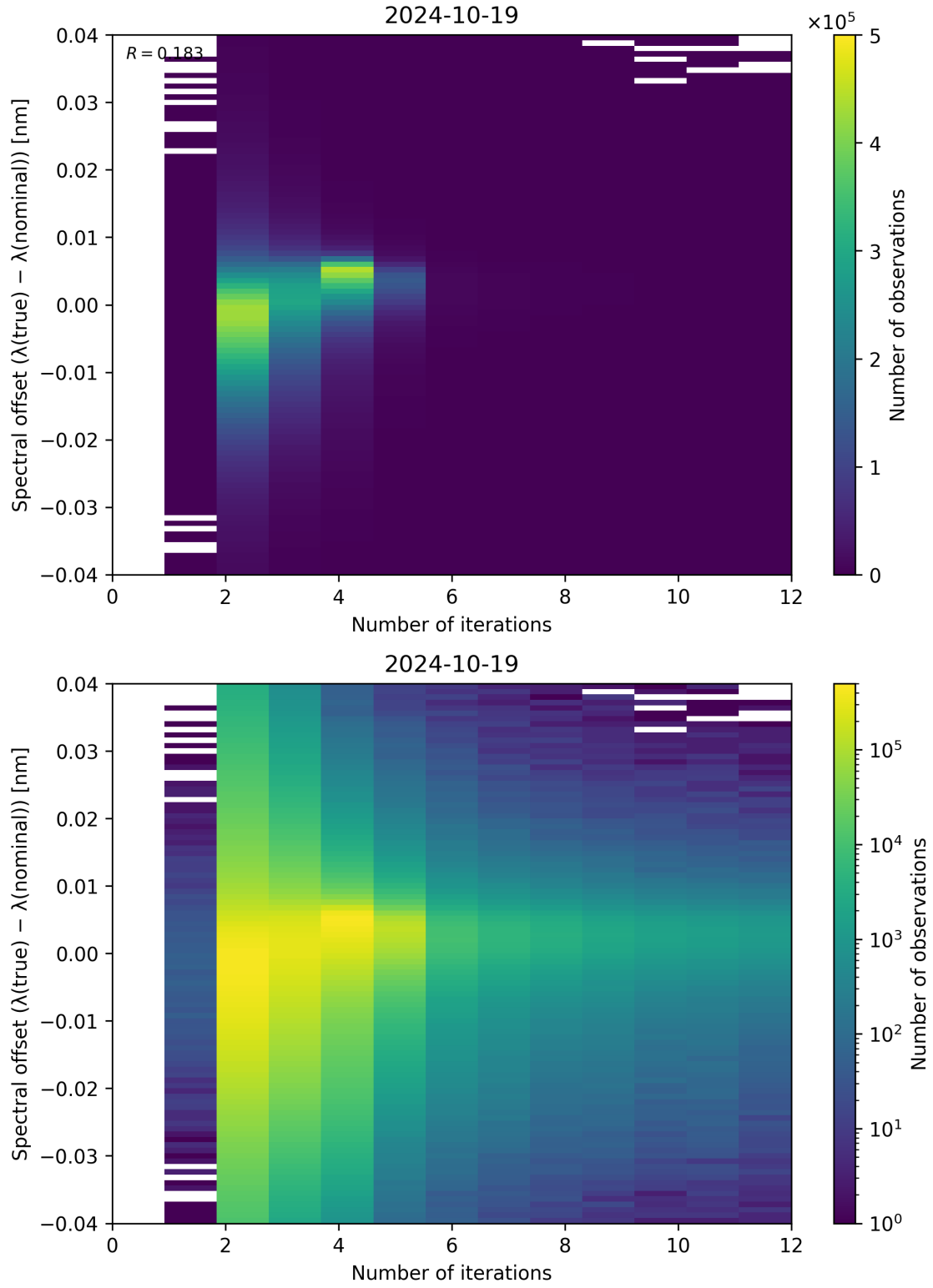
Figure 109: Scatter density plot of “Number of iterations” against “Spectral offset ( \lambda_{\text{true}} - \lambda_{\text{nominal}} )” for 2024-10-19 to 2024-10-20.
