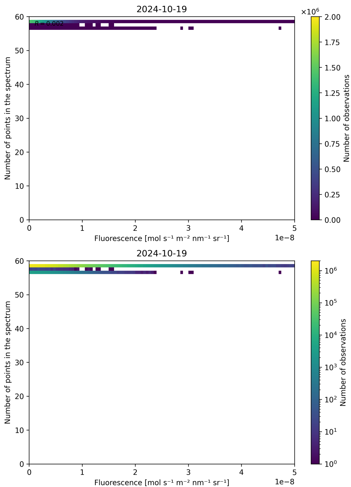
Figure 94: Scatter density plot of “Fluorescence” against “Number of points in the spectrum” for 2024-10-19 to 2024-10-20.
