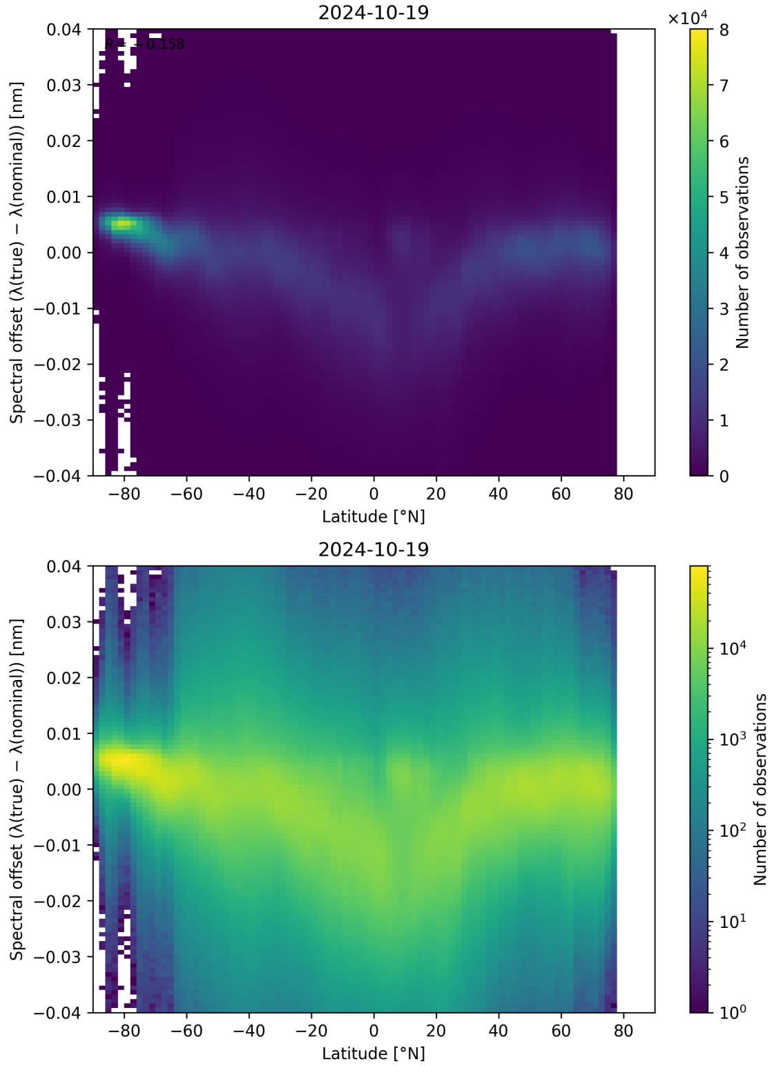
Figure 105: Scatter density plot of “Latitude” against “Spectral offset ( \lambda_{\text{true}} - \lambda_{\text{nominal}} )” for 2024-10-19 to 2024-10-20.
