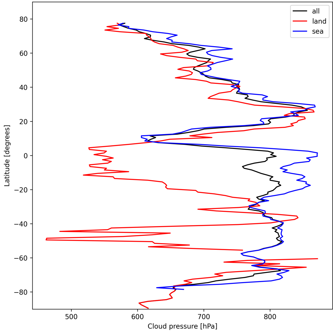
Figure 13: Zonal average of “Cloud pressure” for 2024-10-19 to 2024-10-20.
