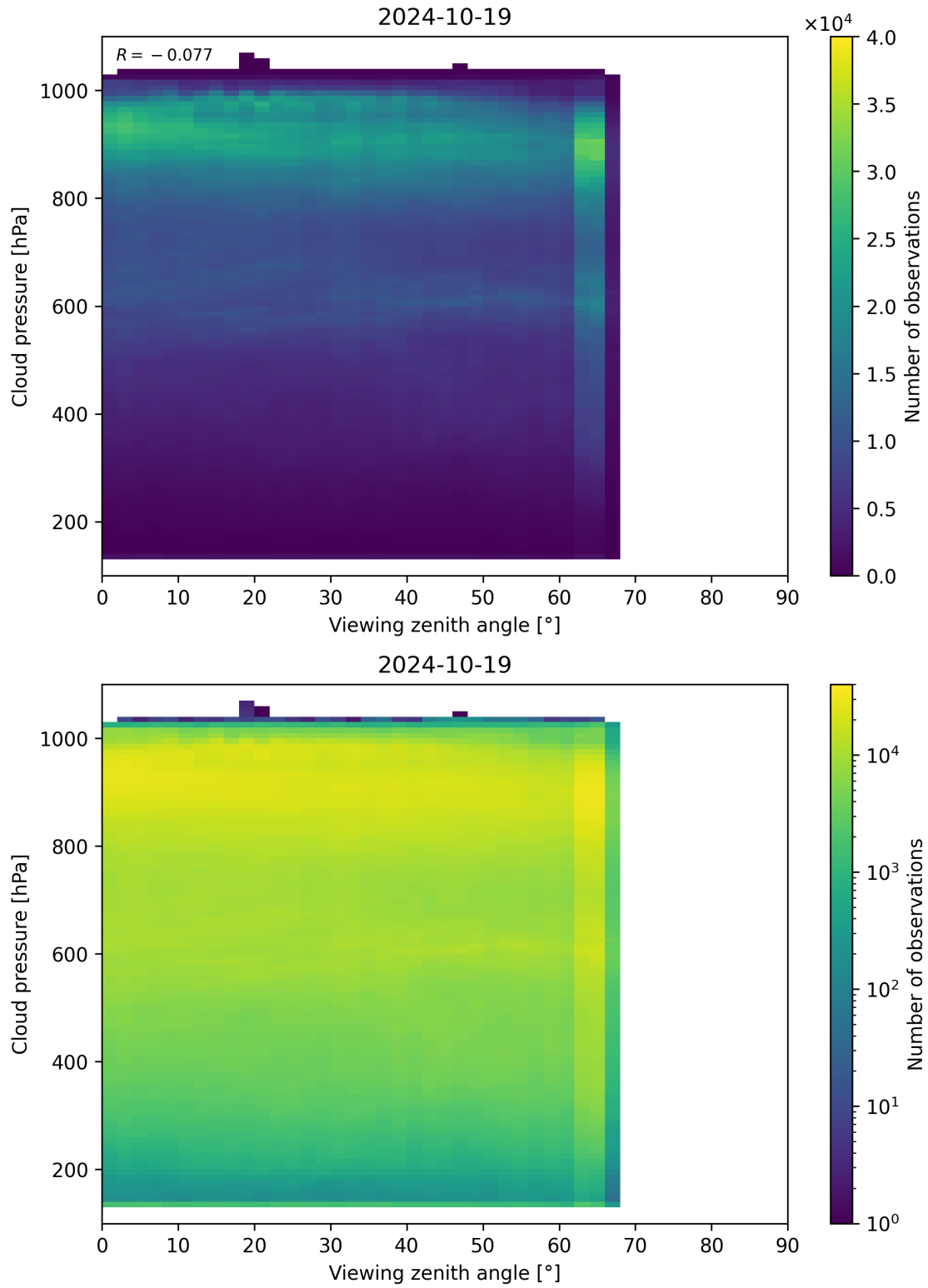
Figure 133: Scatter density plot of “Viewing zenith angle” against “Cloud pressure” for 2024-10-19 to 2024-10-20.
