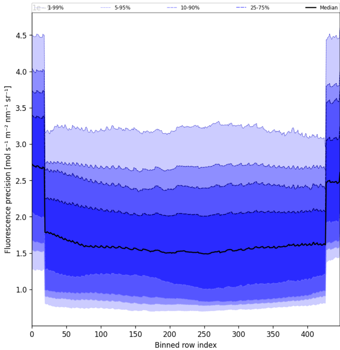
Figure 58: Along track statistics of “Fluorescence precision” for 2024-10-19 to 2024-10-20
