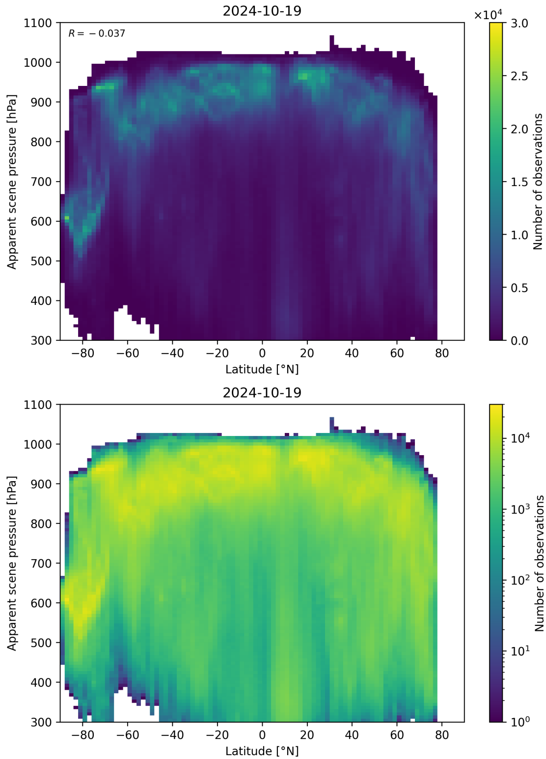
Figure 96: Scatter density plot of “Latitude” against “Apparent scene pressure” for 2024-10-19 to 2024-10-20.
