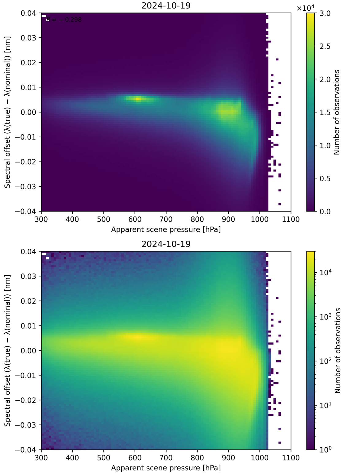
Figure 68: Scatter density plot of “Apparent scene pressure” against “Spectral offset ( \lambda_{\text{true}} - \lambda_{\text{nominal}} )” for 2024-10-19 to 2024-10-20.
