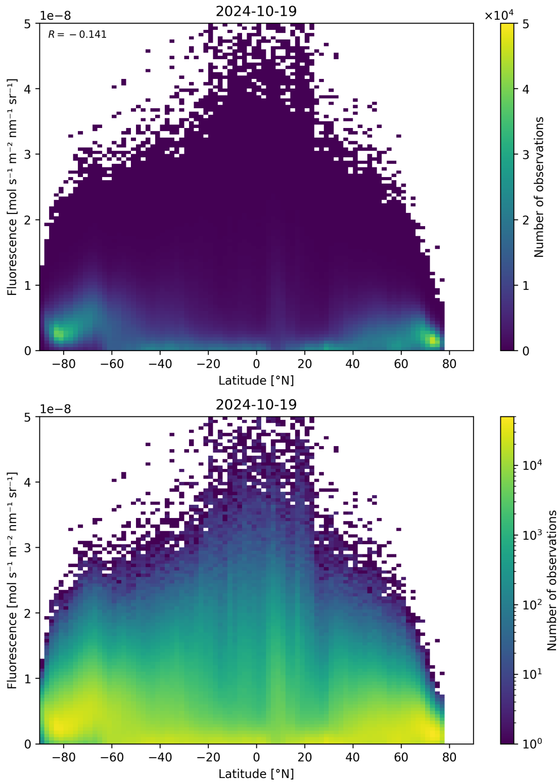
Figure 101: Scatter density plot of “Latitude” against “Fluorescence” for 2024-10-19 to 2024-10-20.
