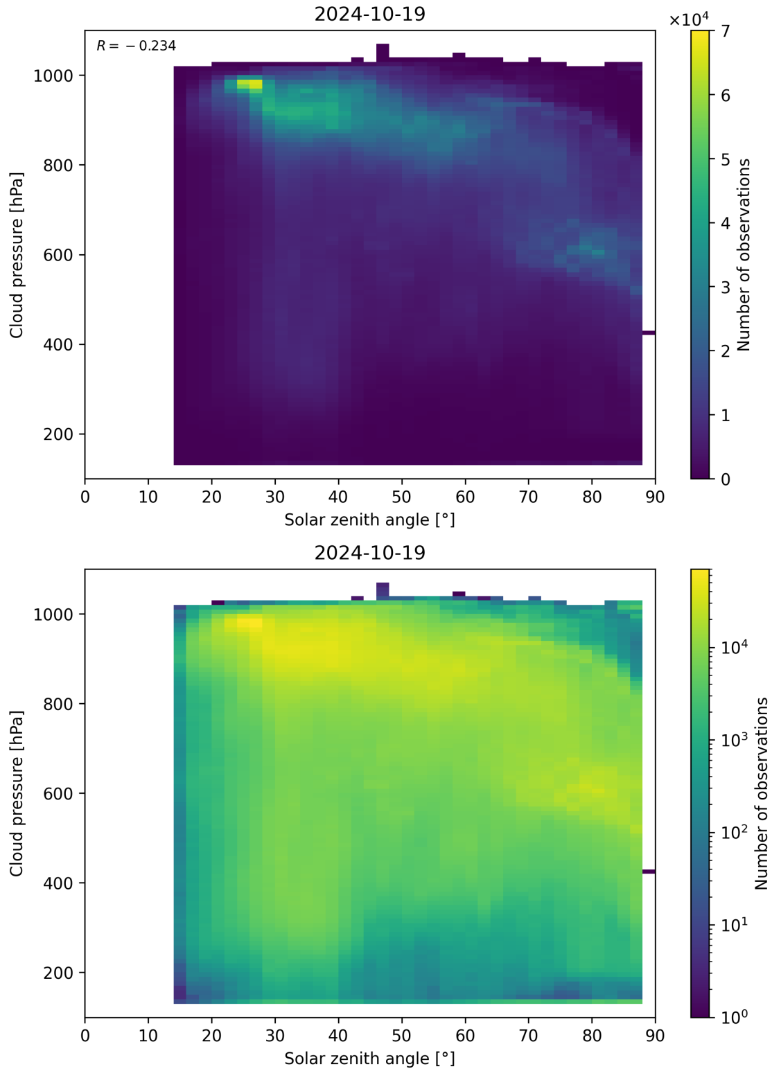
Figure 122: Scatter density plot of “Solar zenith angle” against “Cloud pressure” for 2024-10-19 to 2024-10-20.
