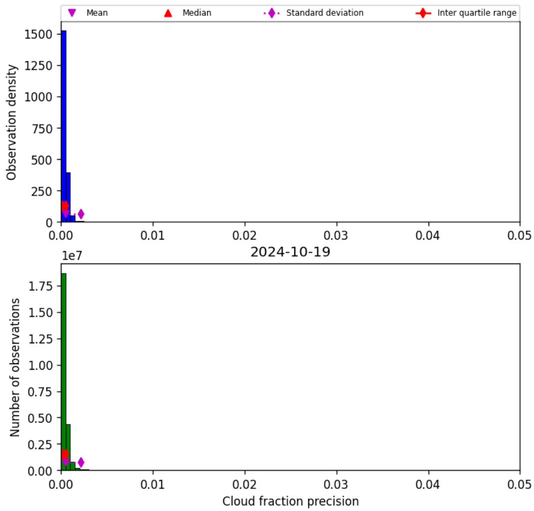
Figure 33: Histogram of “Cloud fraction precision” for 2024-10-19 to 2024-10-20
