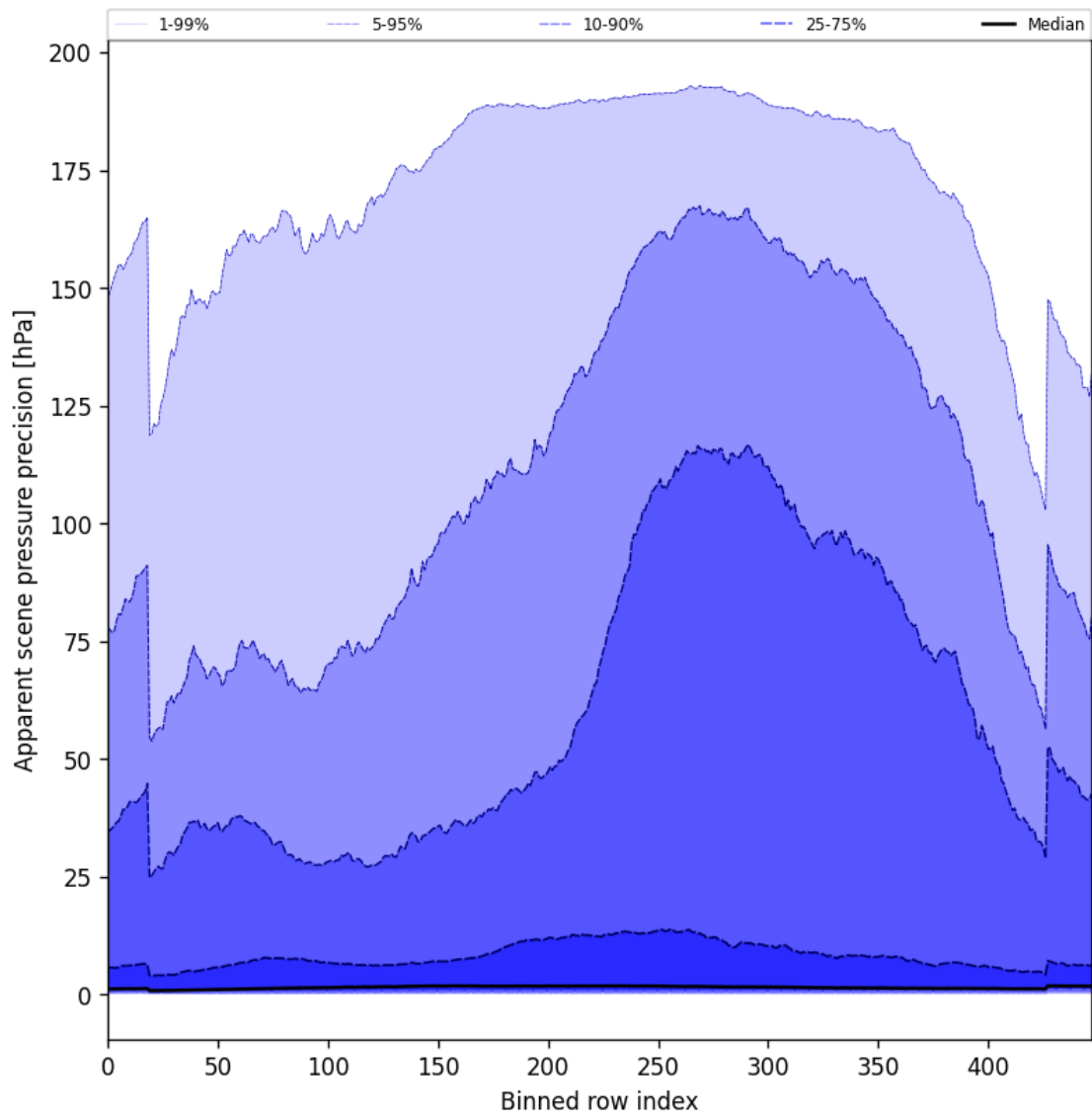
Figure 54: Along track statistics of “Apparent scene pressure precision” for 2024-10-19 to 2024-10-20
