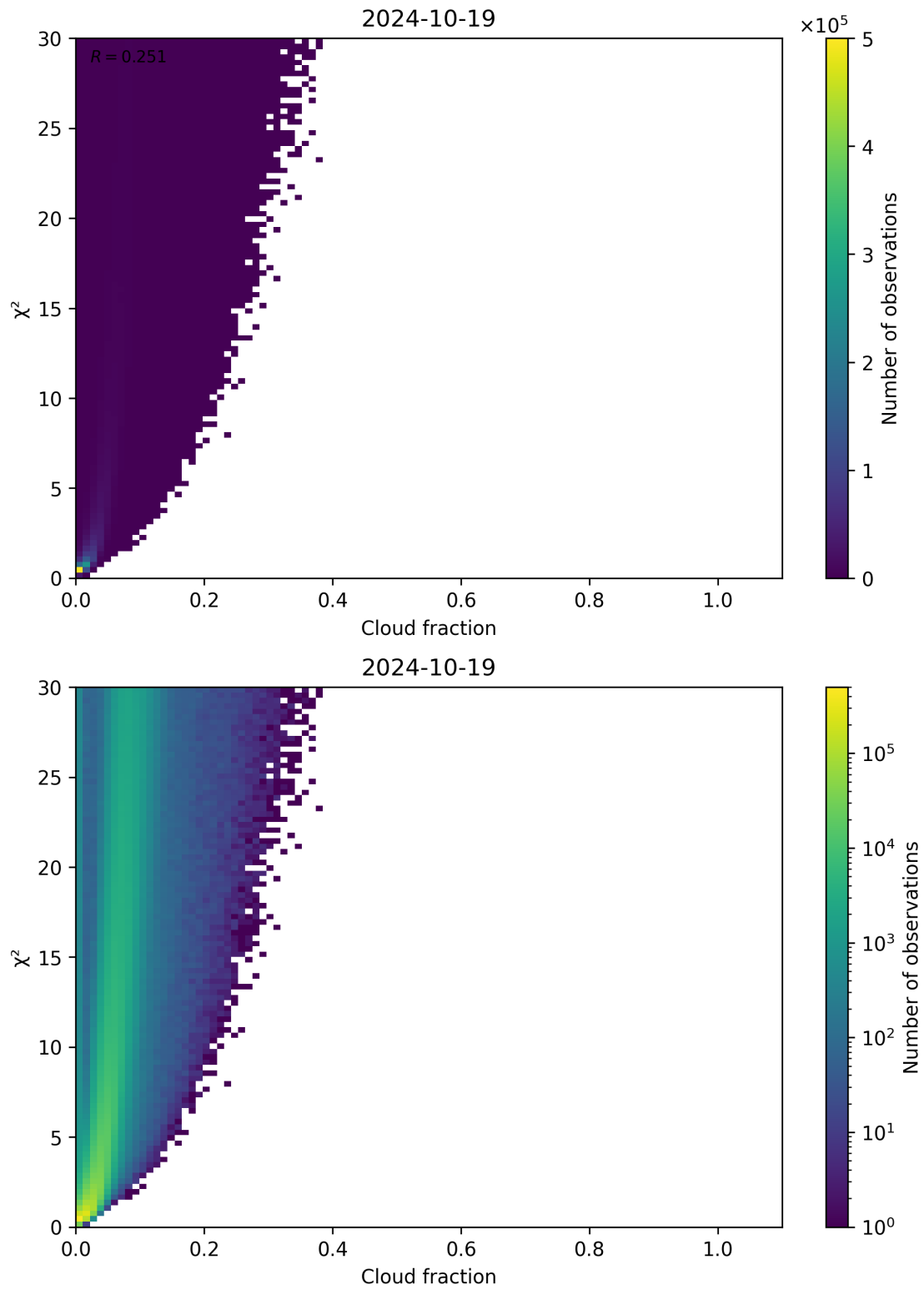
Figure 77: Scatter density plot of “Cloud fraction” against “ \chi^2 ” for 2024-10-19 to 2024-10-20.
