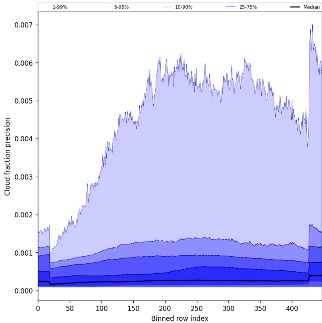
Figure 50: Along track statistics of “Cloud fraction precision” for 2024-10-19 to 2024-10-20
