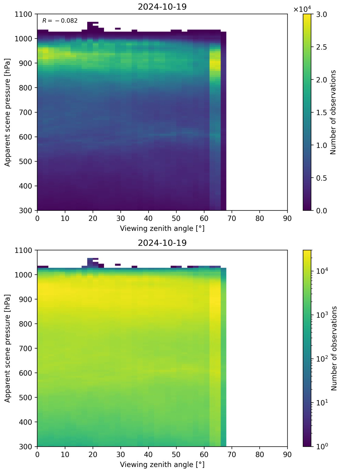
Figure 129: Scatter density plot of “Viewing zenith angle” against “Apparent scene pressure” for 2024-10-19 to 2024-10-20.
