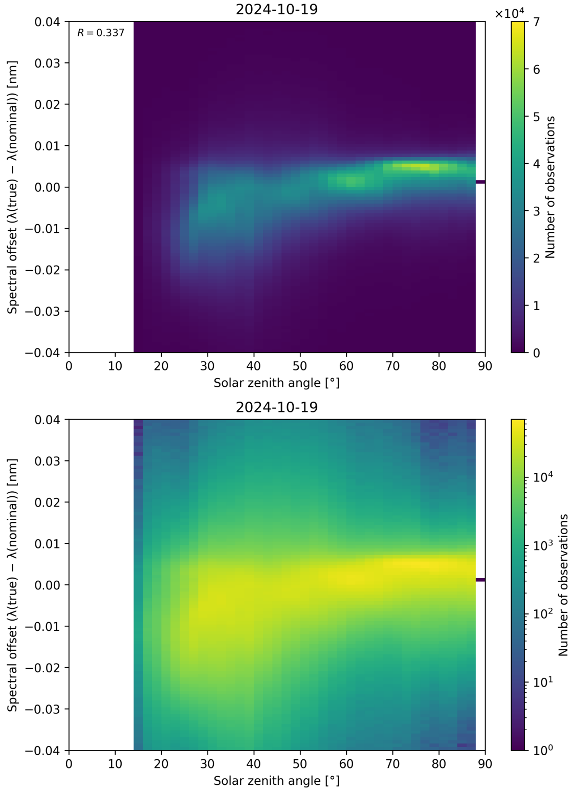
Figure 128: Scatter density plot of “Solar zenith angle” against “Spectral offset ( \lambda_{\text{true}} - \lambda_{\text{nominal}} )” for 2024-10-19 to 2024-10-20.
