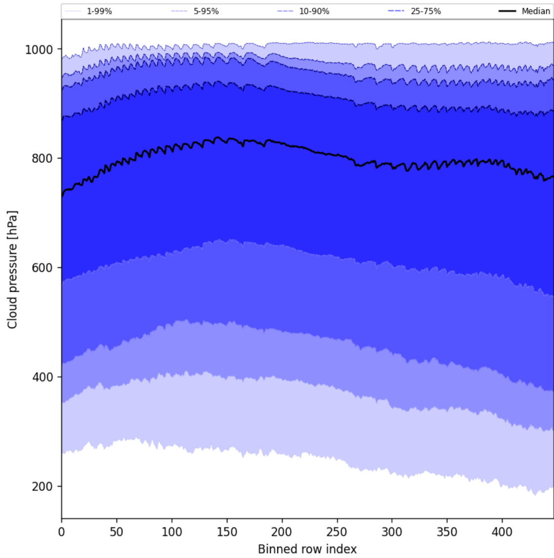
Figure 47: Along track statistics of “Cloud pressure” for 2024-10-19 to 2024-10-20
