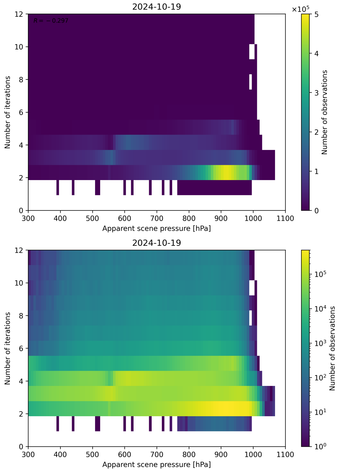
Figure 66: Scatter density plot of “Apparent scene pressure” against “Number of iterations” for 2024-10-19 to 2024-10-20.
