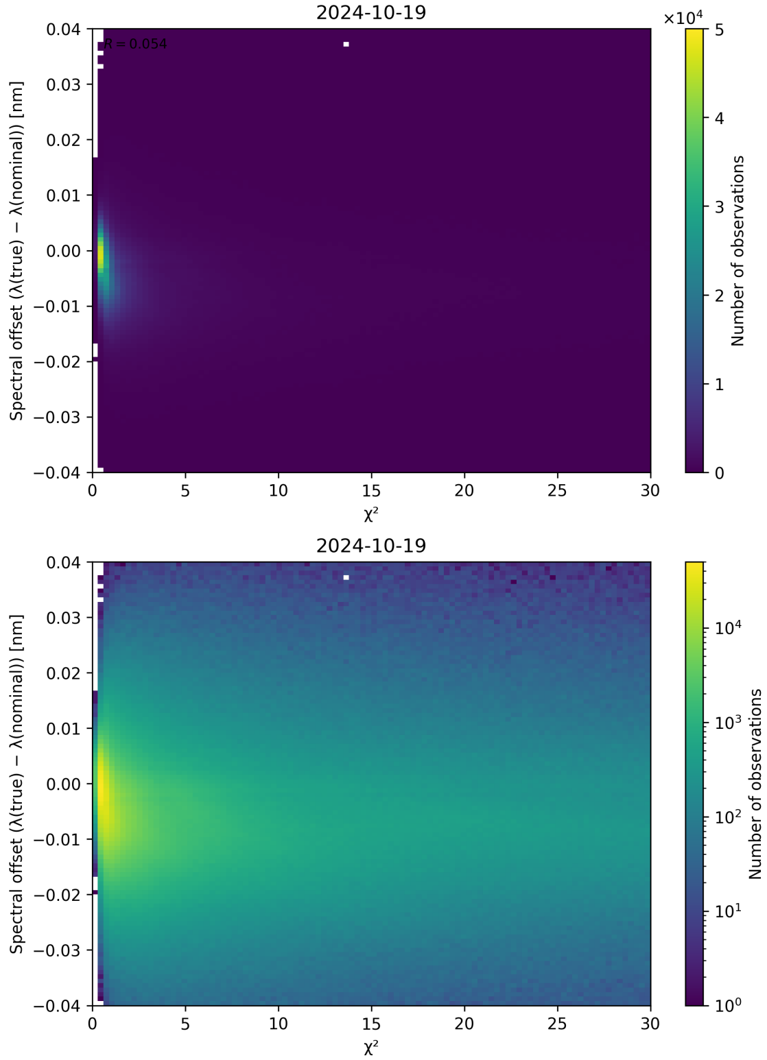
Figure 75: Scatter density plot of “ \chi^2 ” against “Spectral offset ( \lambda_{\text{true}} - \lambda_{\text{nominal}} )” for 2024-10-19 to 2024-10-20.
