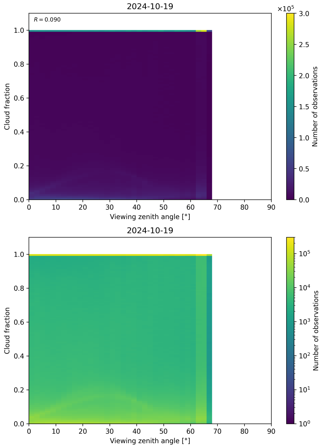
Figure 132: Scatter density plot of “Viewing zenith angle” against “Cloud fraction” for 2024-10-19 to 2024-10-20.
