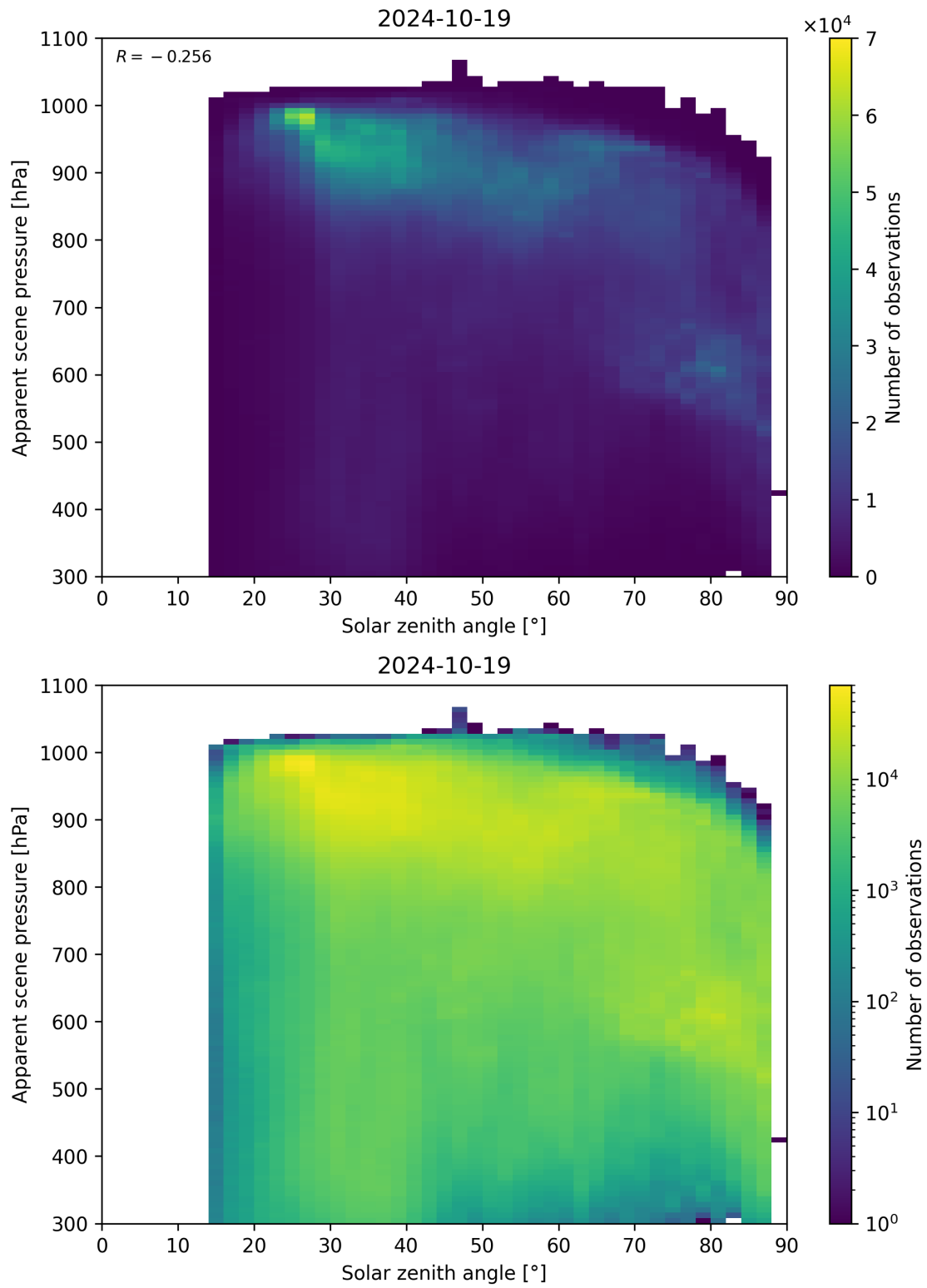
Figure 118: Scatter density plot of “Solar zenith angle” against “Apparent scene pressure” for 2024-10-19 to 2024-10-20.
