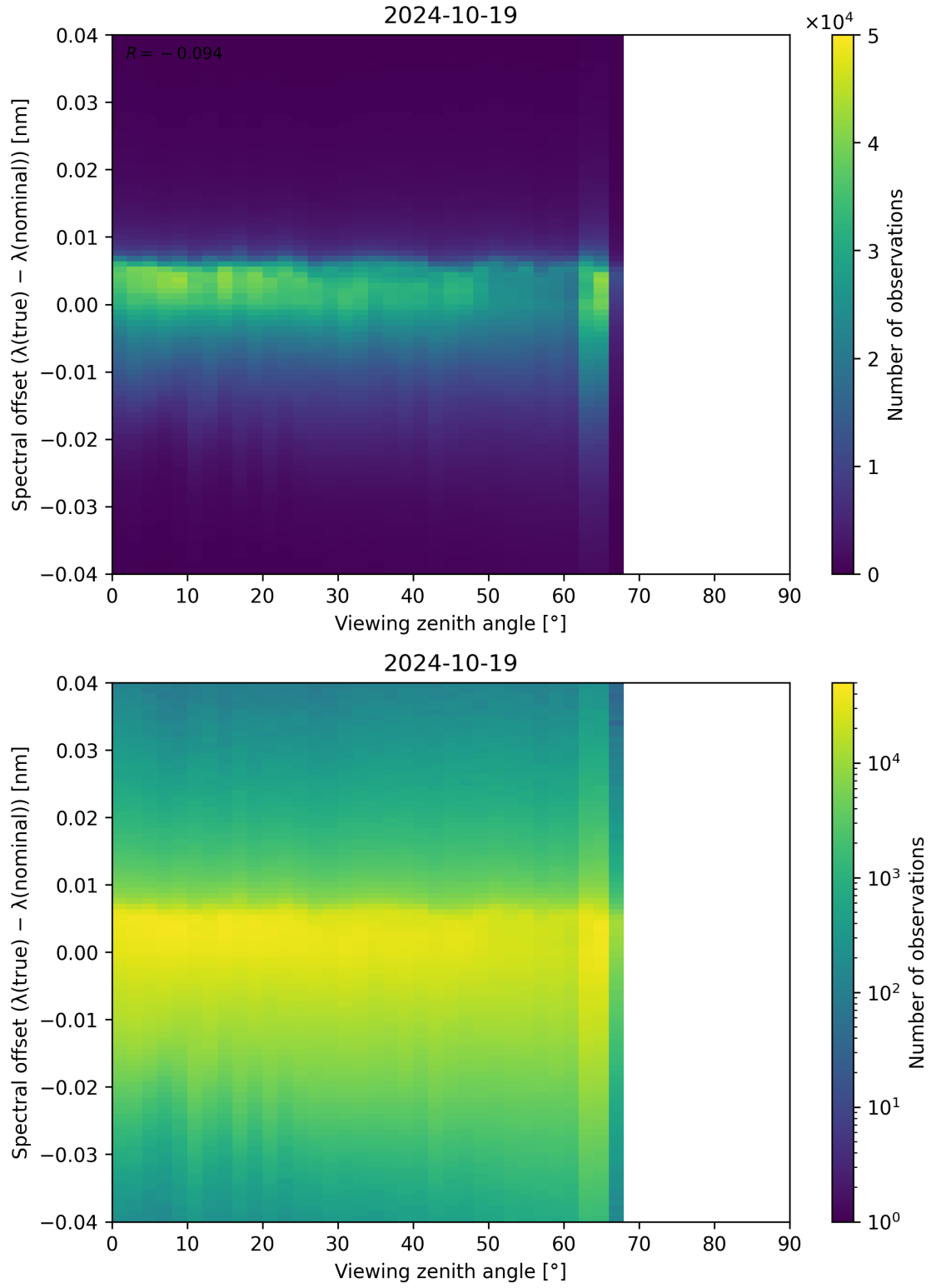
Figure 140: Scatter density plot of “Viewing zenith angle” against “Spectral offset ( \lambda_{\text{true}} - \lambda_{\text{nominal}} )” for 2024-10-19 to 2024-10-20.
