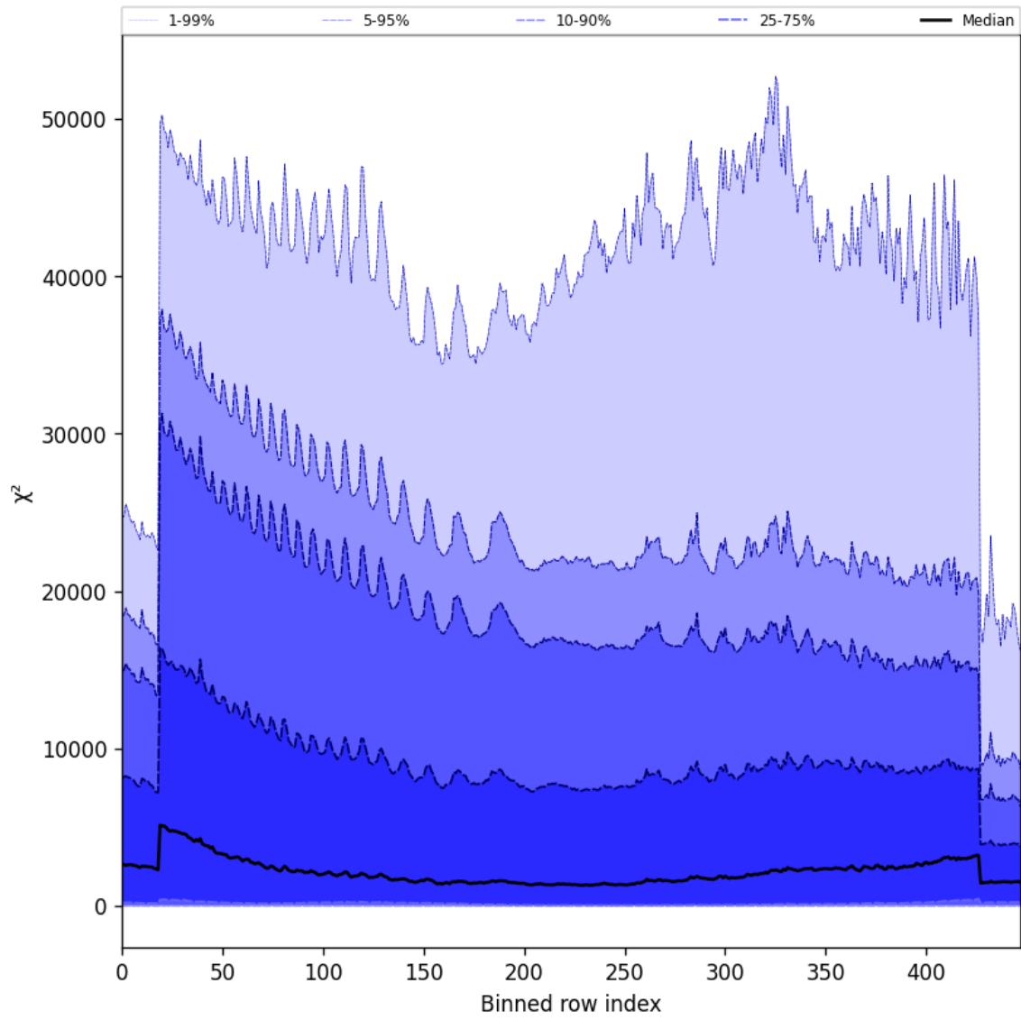
Figure 55: Along track statistics of “ \chi^2 ” for 2024-10-19 to 2024-10-20
