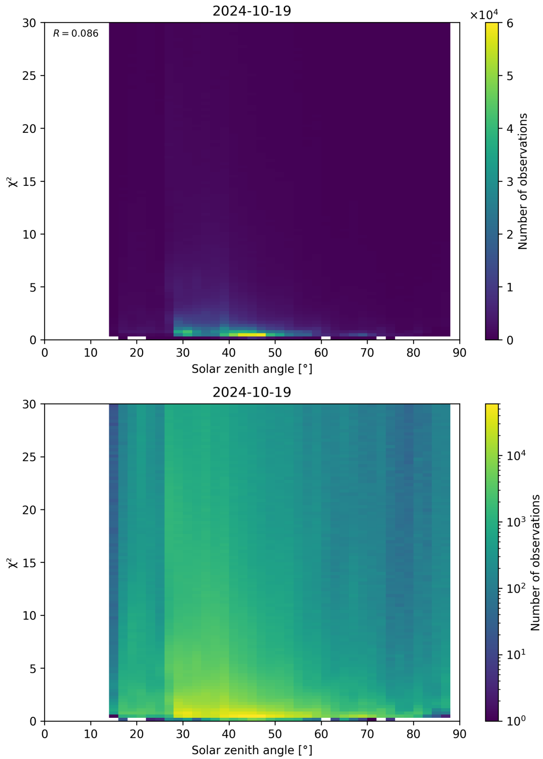
Figure 119: Scatter density plot of “Solar zenith angle” against “ \chi^2 ” for 2024-10-19 to 2024-10-20.
