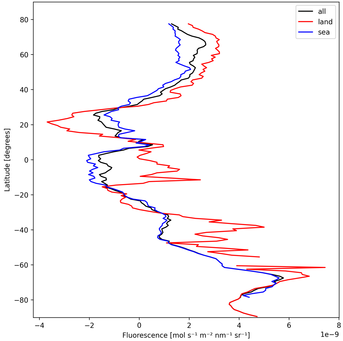
Figure 23: Zonal average of “Fluorescence” for 2024-10-19 to 2024-10-20.
