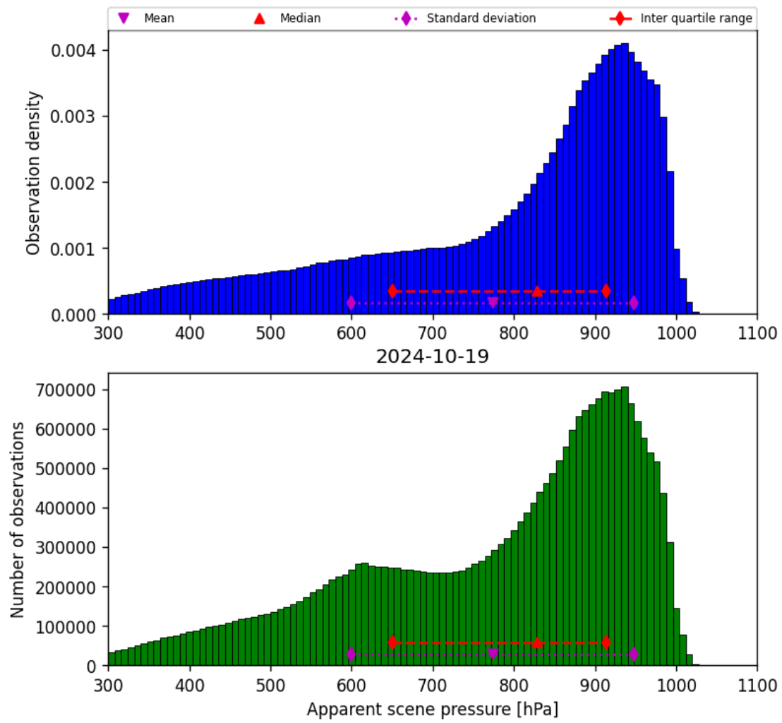
Figure 36: Histogram of “Apparent scene pressure” for 2024-10-19 to 2024-10-20
