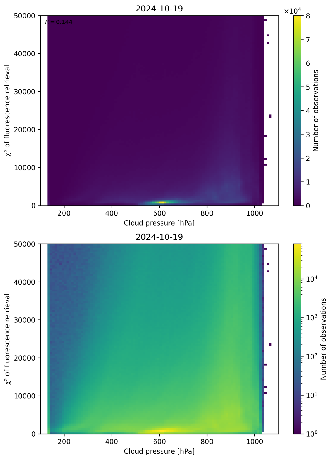
Figure 86: Scatter density plot of “Cloud pressure” against “ \chi^2 of fluorescence retrieval” for 2024-10-19 to 2024-10-20.
