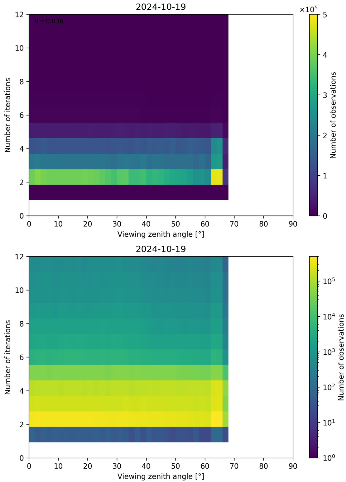
Figure 136: Scatter density plot of “Viewing zenith angle” against “Number of iterations” for 2024-10-19 to 2024-10-20.
