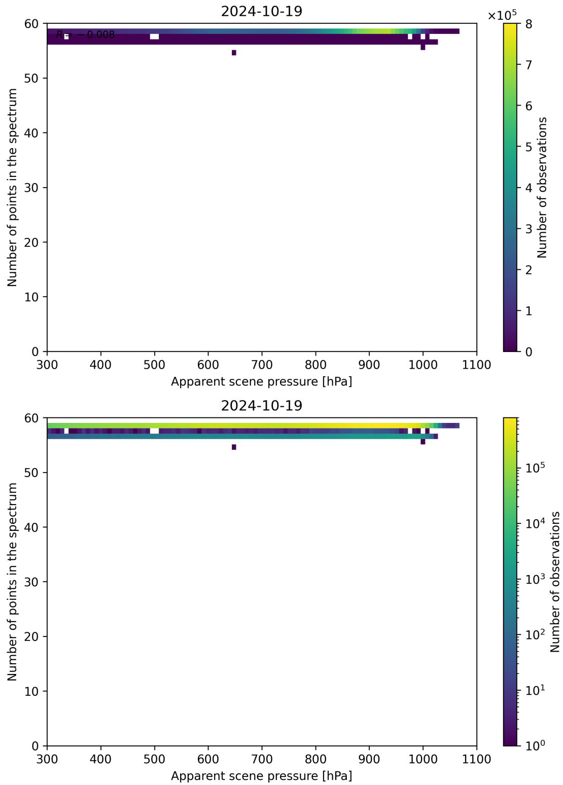
Figure 67: Scatter density plot of “Apparent scene pressure” against “Number of points in the spectrum” for 2024-10-19 to 2024-10-20.
