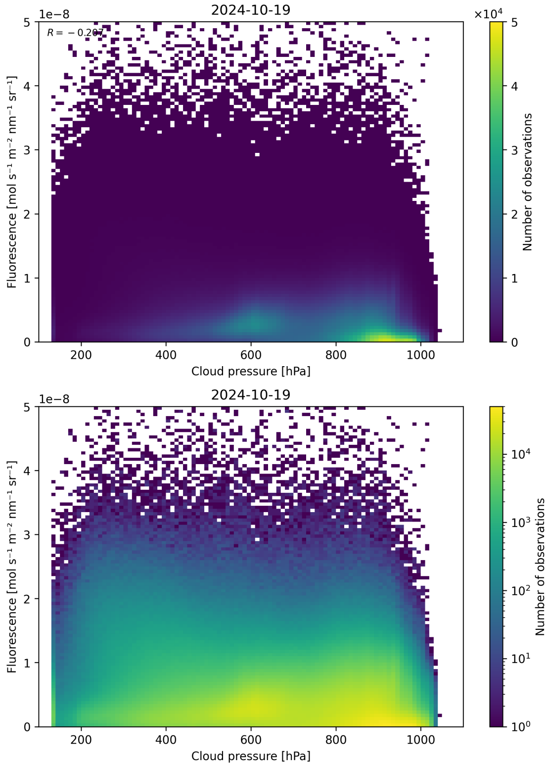
Figure 88: Scatter density plot of “Cloud pressure” against “Fluorescence” for 2024-10-19 to 2024-10-20.
