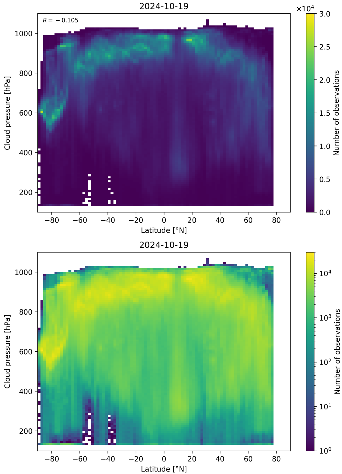
Figure 100: Scatter density plot of “Latitude” against “Cloud pressure” for 2024-10-19 to 2024-10-20.
