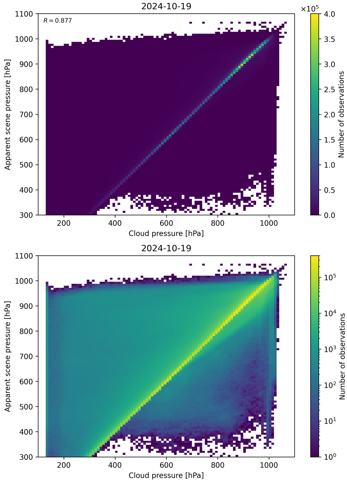
Figure 84: Scatter density plot of “Cloud pressure” against “Apparent scene pressure” for 2024-10-19 to 2024-10-20.
