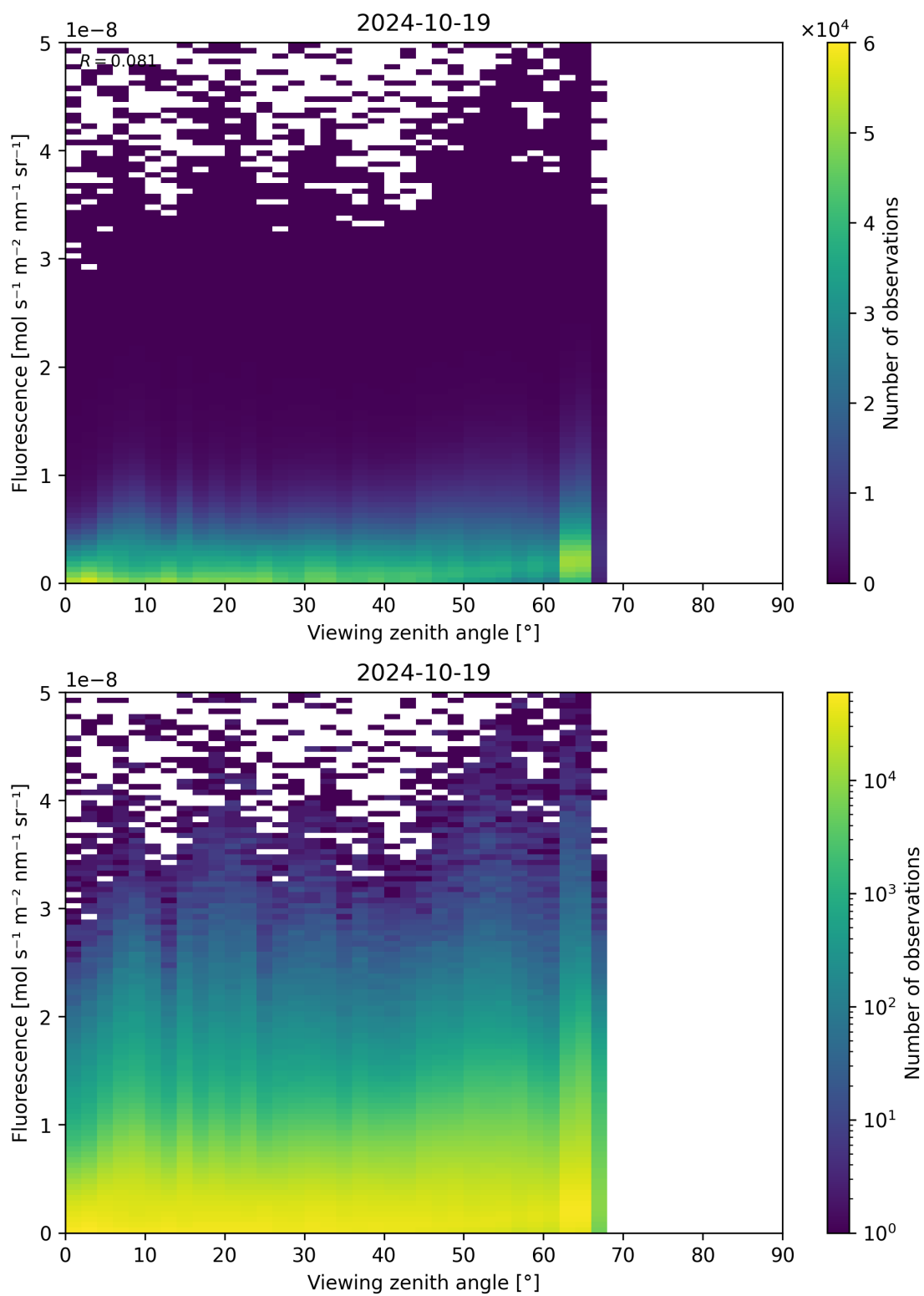
Figure 134: Scatter density plot of “Viewing zenith angle” against “Fluorescence” for 2024-10-19 to 2024-10-20.
