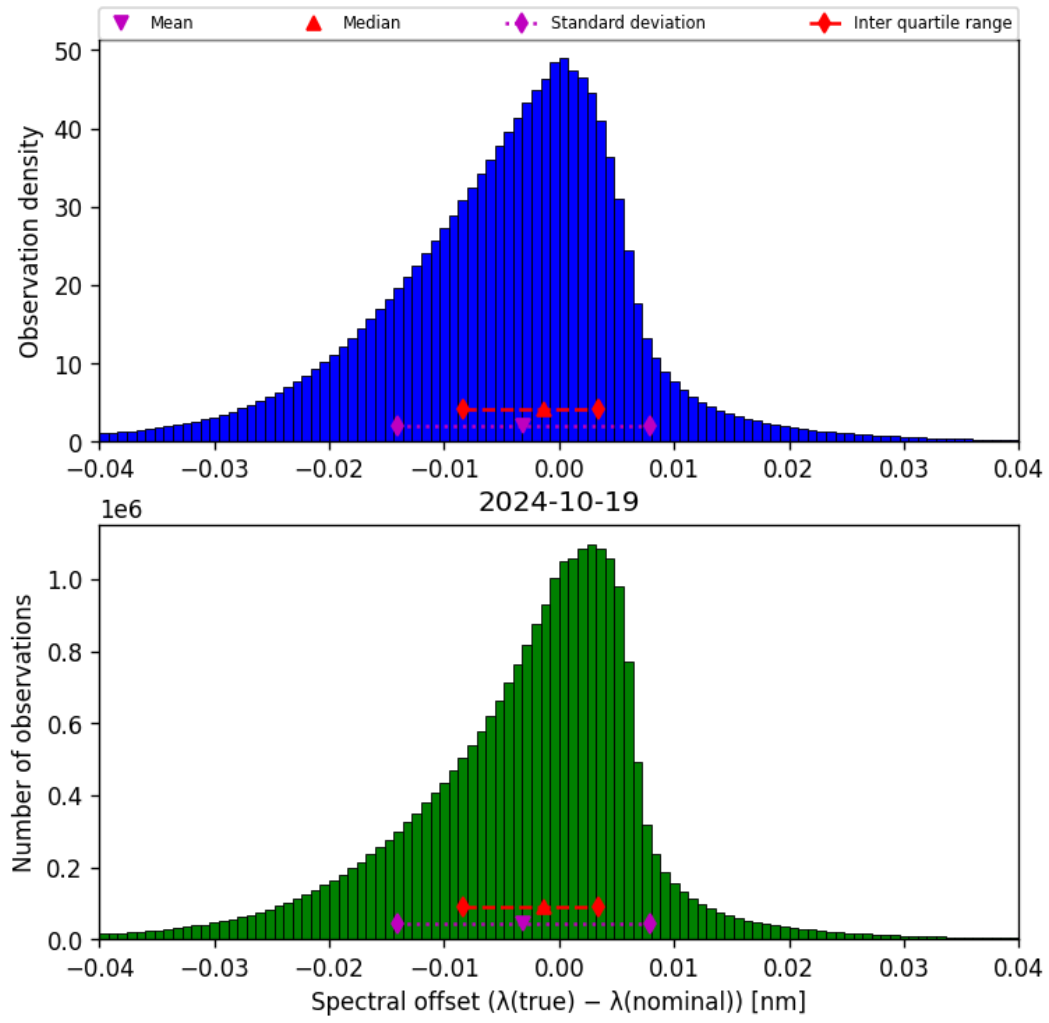
Figure 45: Histogram of “Spectral offset ( \lambda_{\text{true}} - \lambda_{\text{nominal}} )” for 2024-10-19 to 2024-10-20
