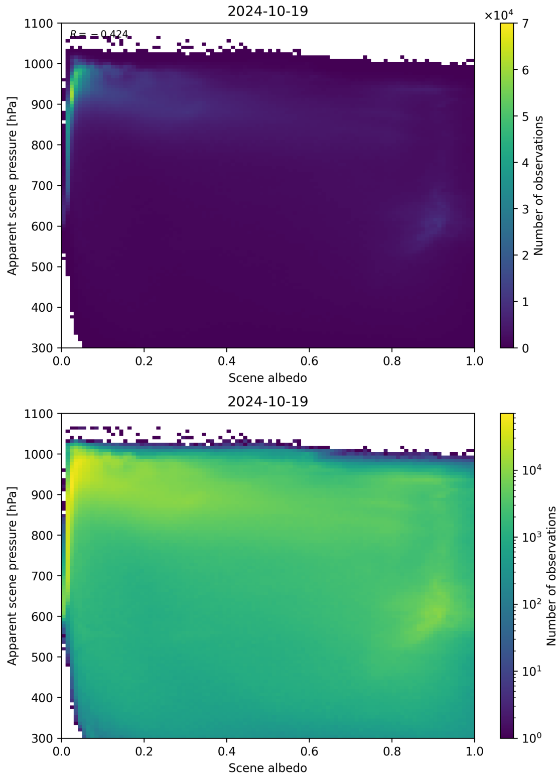
Figure 111: Scatter density plot of “Scene albedo” against “Apparent scene pressure” for 2024-10-19 to 2024-10-20.
