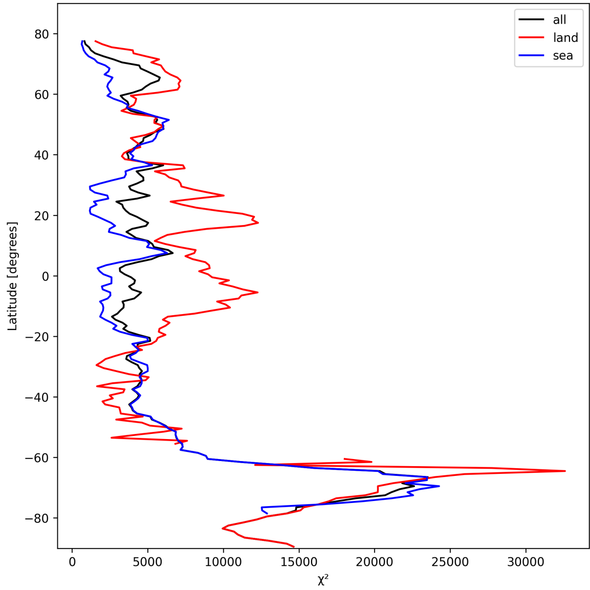
Figure 21: Zonal average of “ \chi^2 ” for 2024-10-19 to 2024-10-20.
