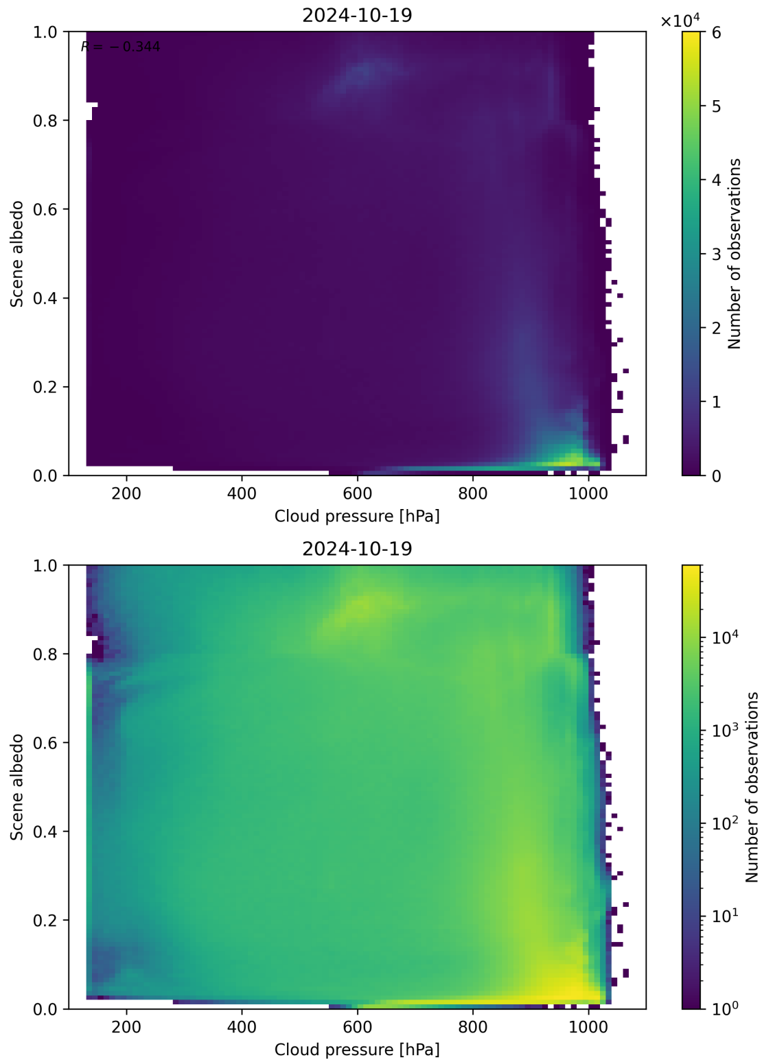
Figure 91: Scatter density plot of “Cloud pressure” against “Scene albedo” for 2024-10-19 to 2024-10-20.
