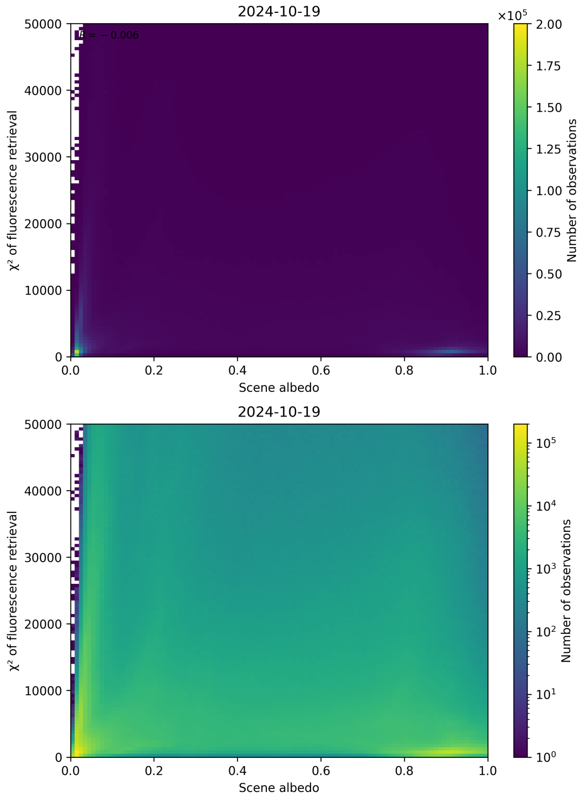
Figure 113: Scatter density plot of “Scene albedo” against “ \chi^2 of fluorescence retrieval” for 2024-10-19 to 2024-10-20.
