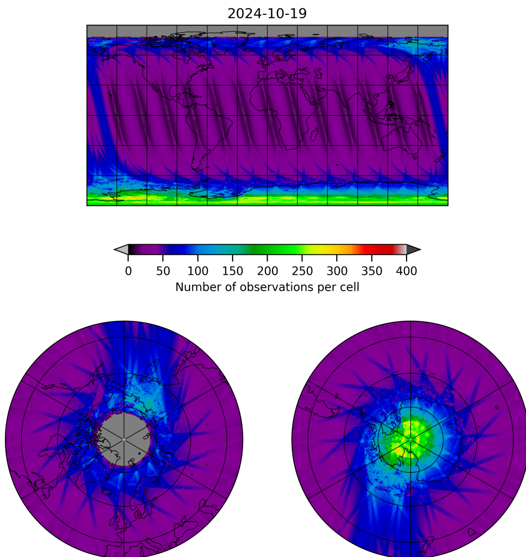
Figure 11: Map of the number of observations for 2024-10-19 to 2024-10-20
