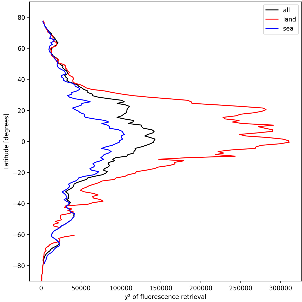
Figure 25: Zonal average of “ \chi^2 of fluorescence retrieval” for 2024-10-19 to 2024-10-20.
