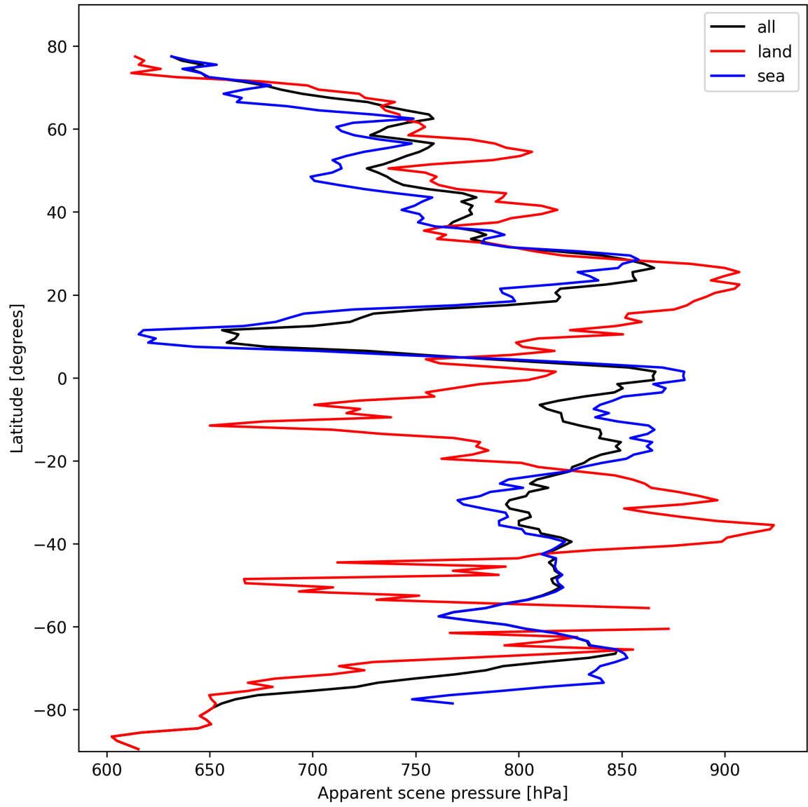
Figure 19: Zonal average of “Apparent scene pressure” for 2024-10-19 to 2024-10-20.
