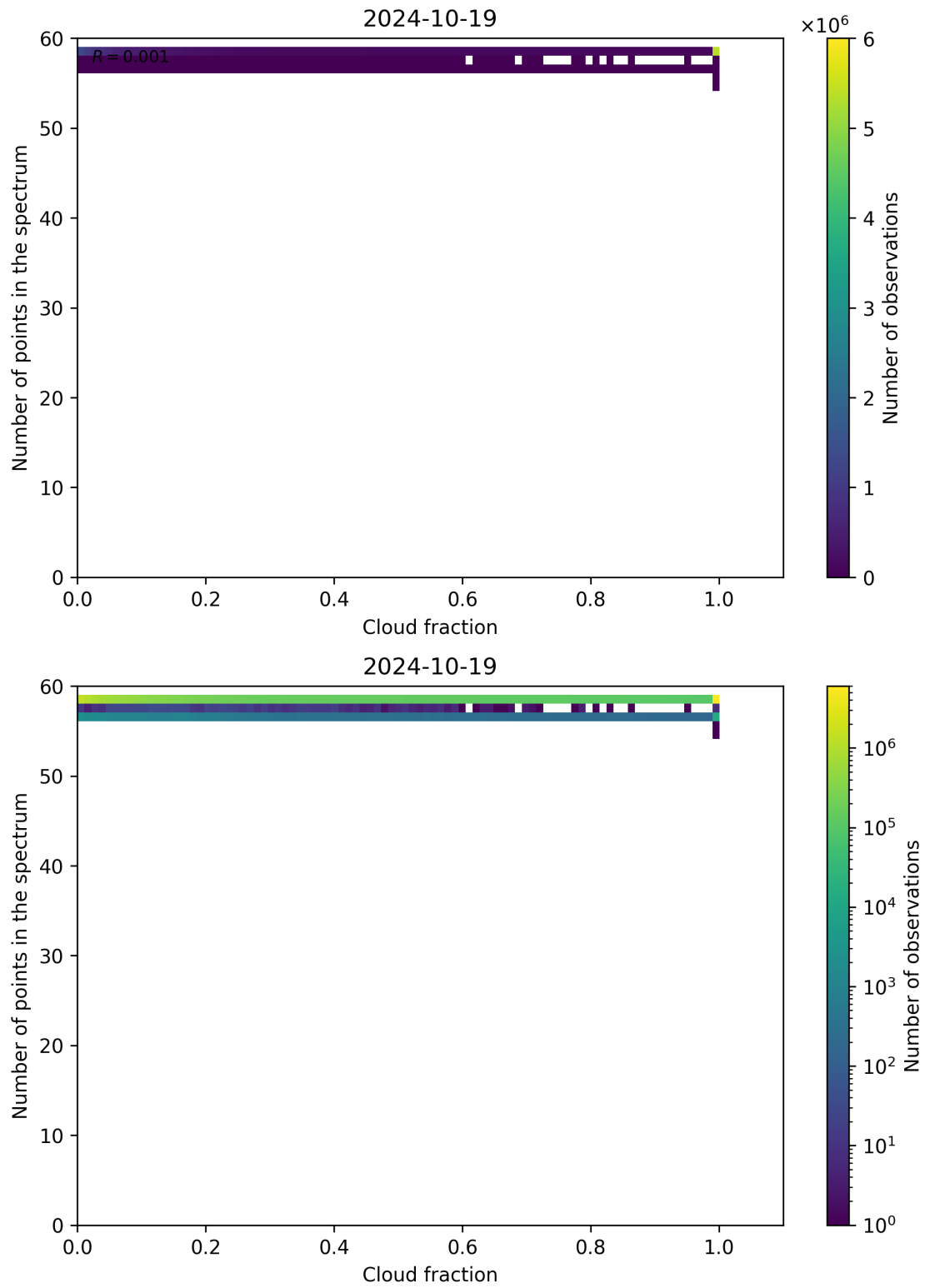
Figure 81: Scatter density plot of “Cloud fraction” against “Number of points in the spectrum” for 2024-10-19 to 2024-10-20.
