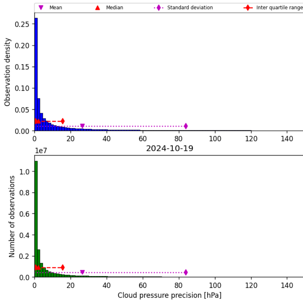
Figure 31: Histogram of “Cloud pressure precision” for 2024-10-19 to 2024-10-20
