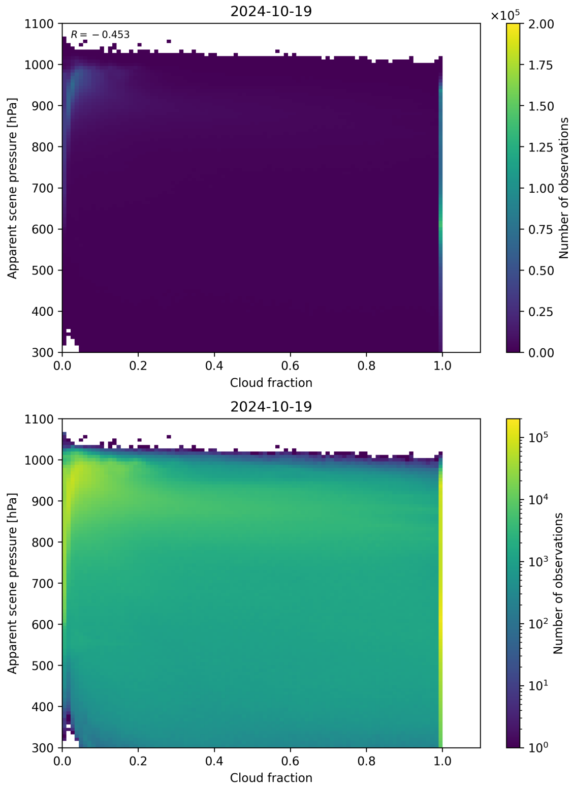
Figure 76: Scatter density plot of “Cloud fraction” against “Apparent scene pressure” for 2024-10-19 to 2024-10-20.
