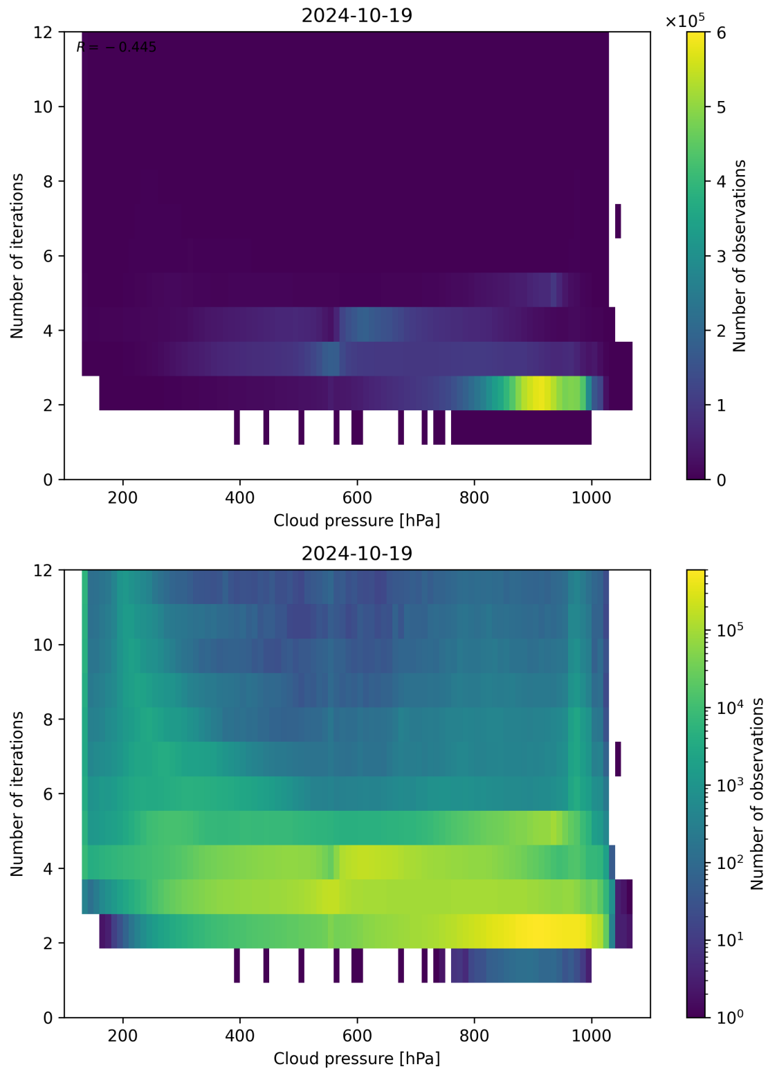
Figure 89: Scatter density plot of “Cloud pressure” against “Number of iterations” for 2024-10-19 to 2024-10-20.
