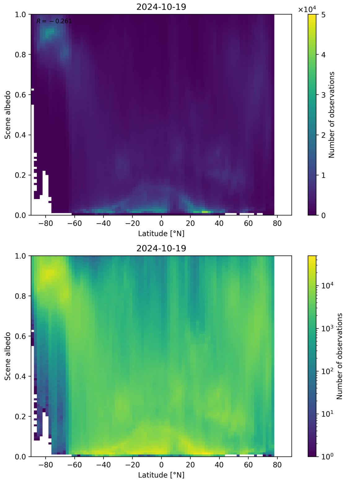
Figure 104: Scatter density plot of “Latitude” against “Scene albedo” for 2024-10-19 to 2024-10-20.
