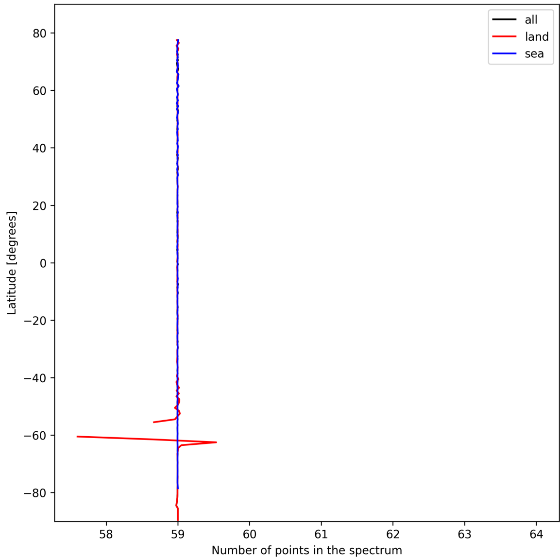
Figure 27: Zonal average of “Number of points in the spectrum” for 2024-10-19 to 2024-10-20.
