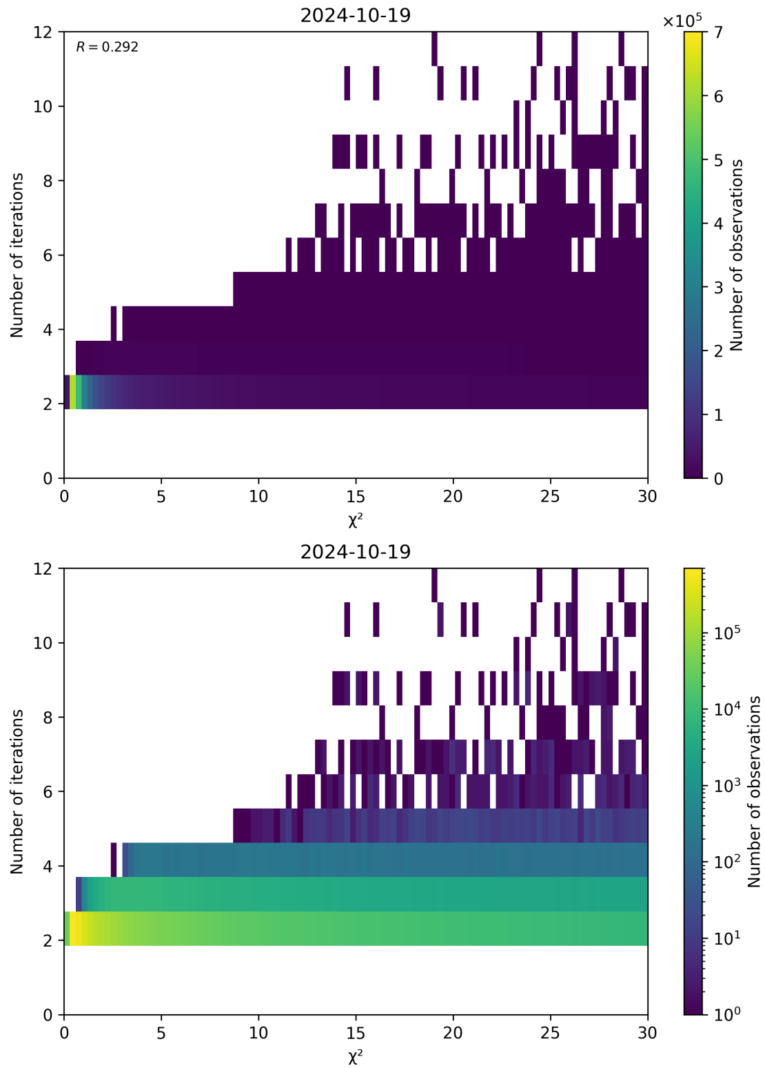
Figure 73: Scatter density plot of “ \chi^2 ” against “Number of iterations” for 2024-10-19 to 2024-10-20.
