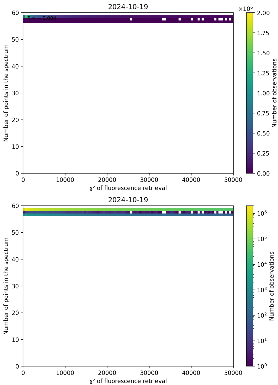
Figure 71: Scatter density plot of " \chi^2 of fluorescence retrieval" against "Number of points in the spectrum" for 2024-10-19 to 2024-10-20.
