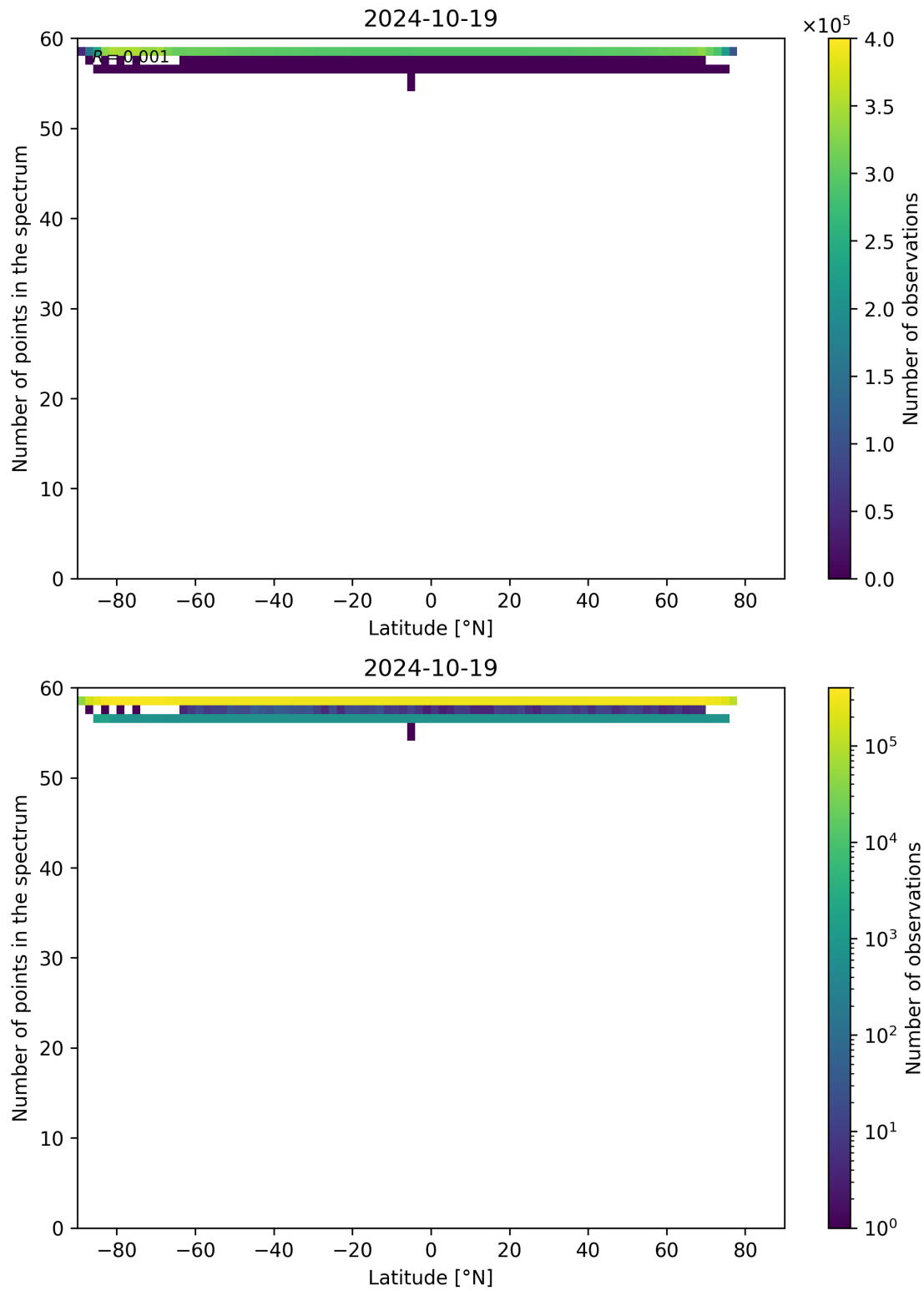
Figure 103: Scatter density plot of “Latitude” against “Number of points in the spectrum” for 2024-10-19 to 2024-10-20.
