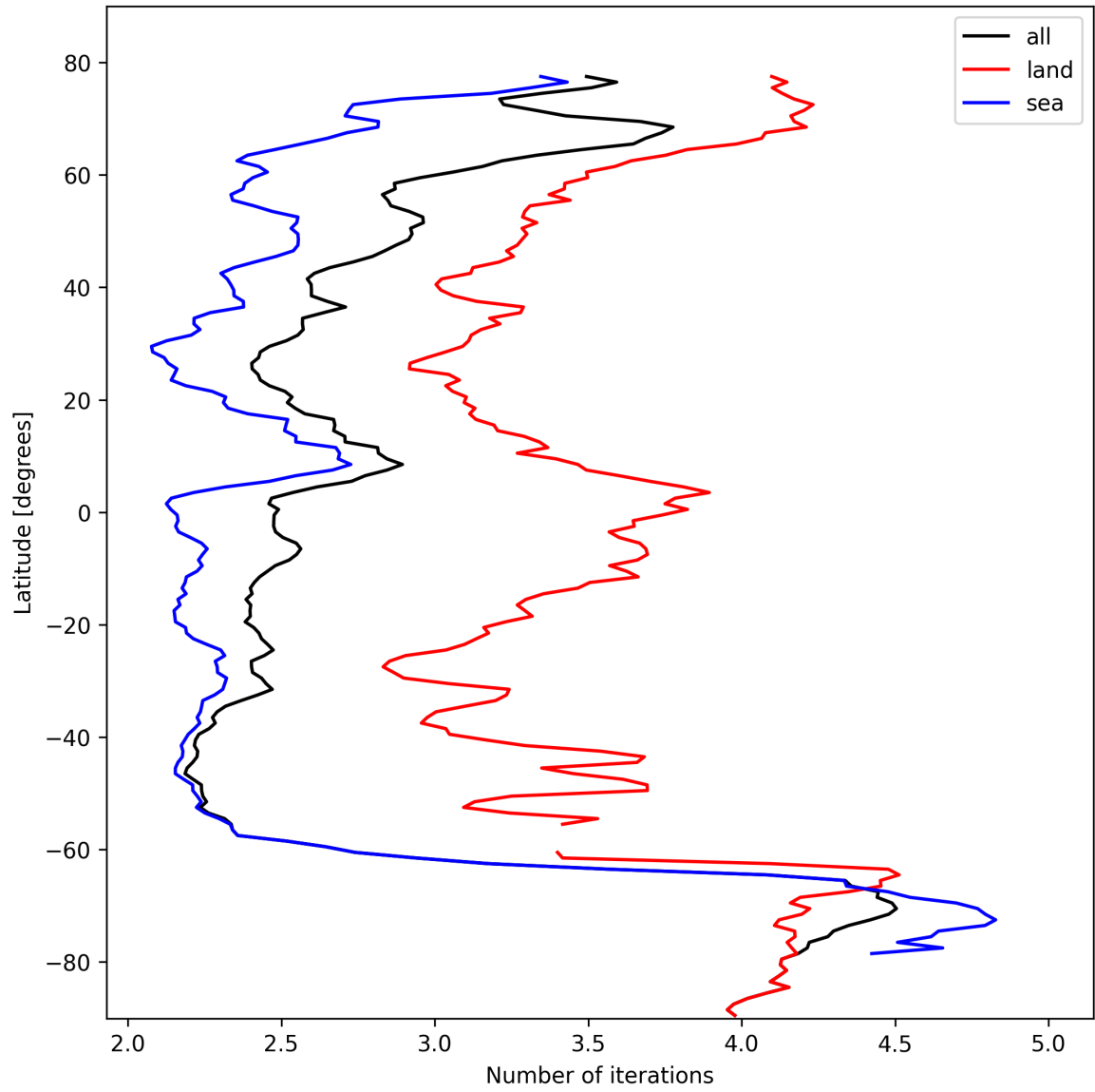
Figure 22: Zonal average of “Number of iterations” for 2024-10-19 to 2024-10-20.
