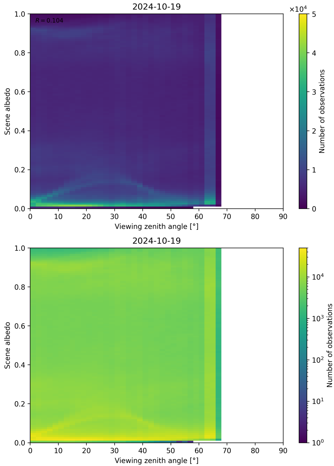
Figure 138: Scatter density plot of “Viewing zenith angle” against “Scene albedo” for 2024-10-19 to 2024-10-20.
