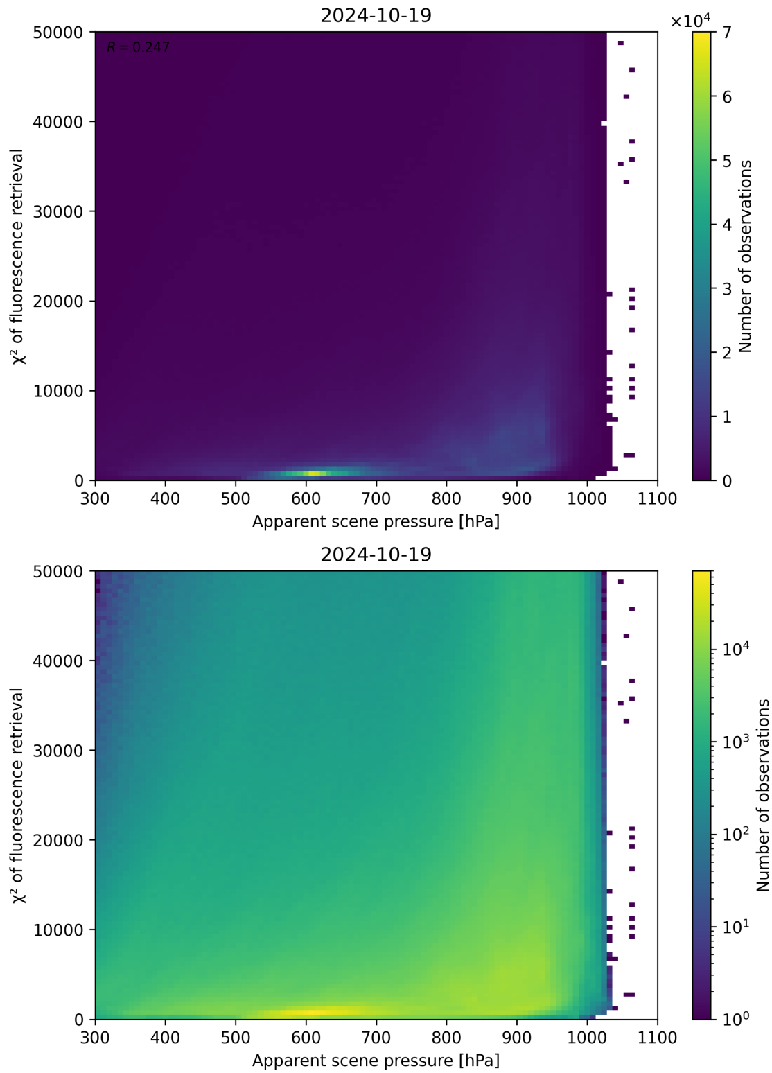
Figure 64: Scatter density plot of “Apparent scene pressure” against “ \chi^2 of fluorescence retrieval” for 2024-10-19 to 2024-10-20.
