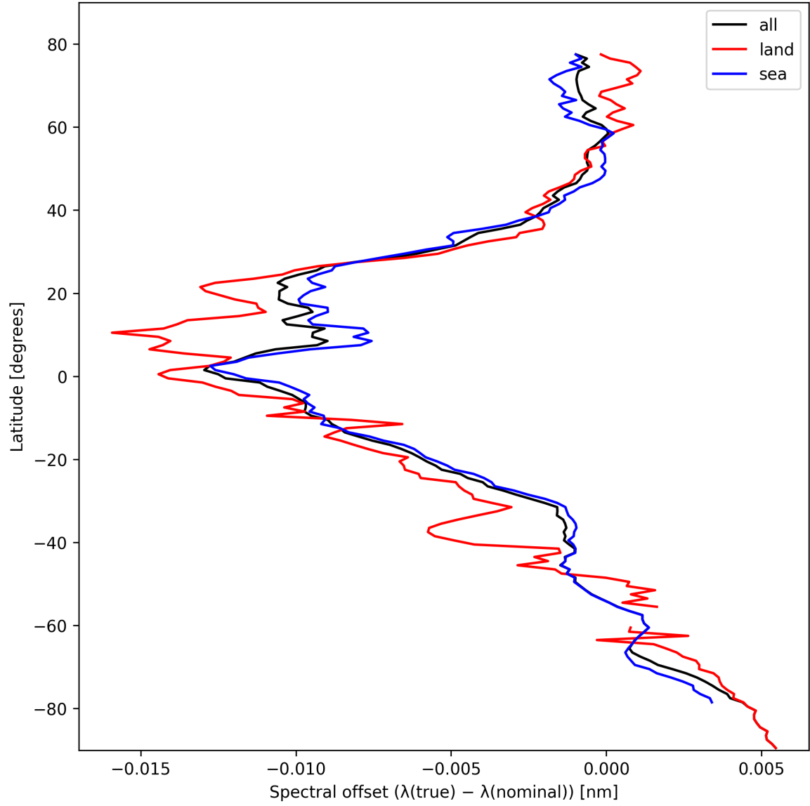
Figure 28: Zonal average of “Spectral offset ( \lambda_{\text{true}} - \lambda_{\text{nominal}} )” for 2024-10-19 to 2024-10-20.
