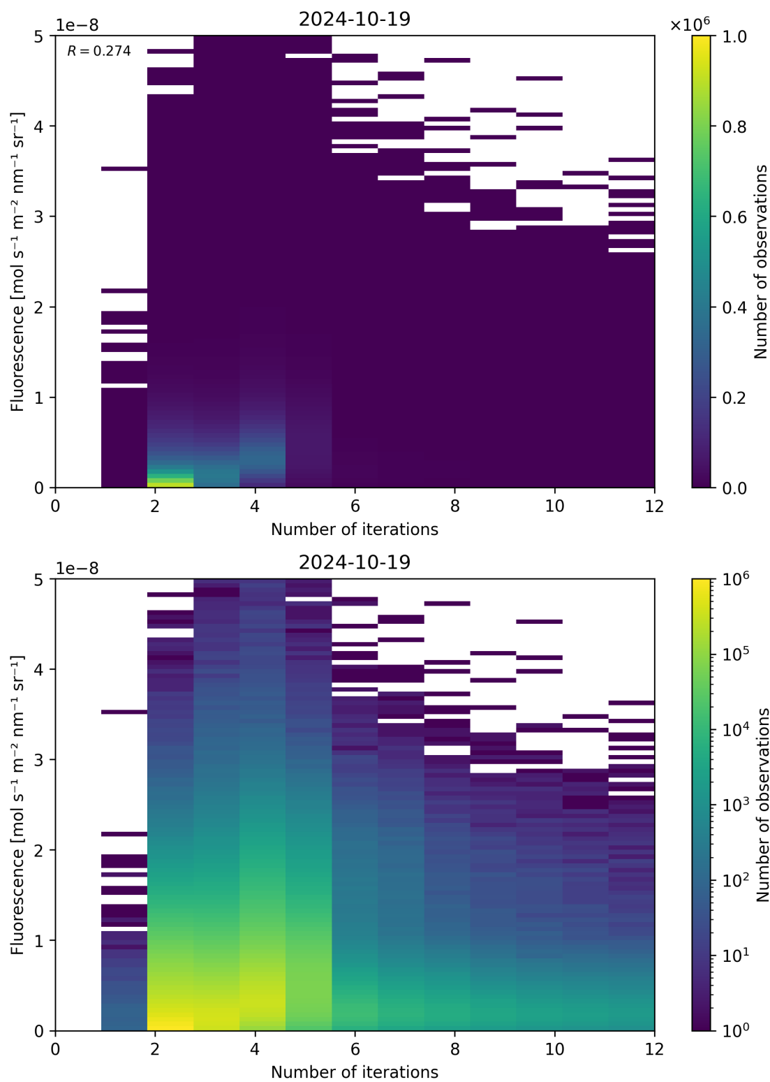
Figure 107: Scatter density plot of “Number of iterations” against “Fluorescence” for 2024-10-19 to 2024-10-20.
