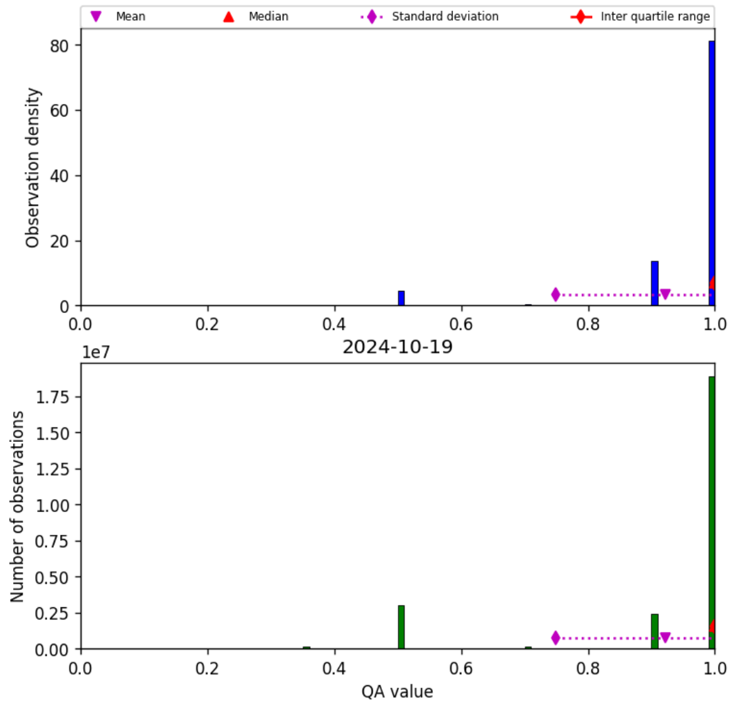
Figure 29: Histogram of “QA value” for 2024-10-19 to 2024-10-20
