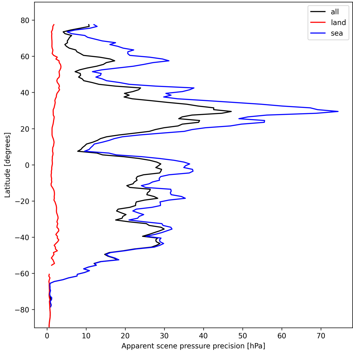
Figure 20: Zonal average of “Apparent scene pressure precision” for 2024-10-19 to 2024-10-20.
