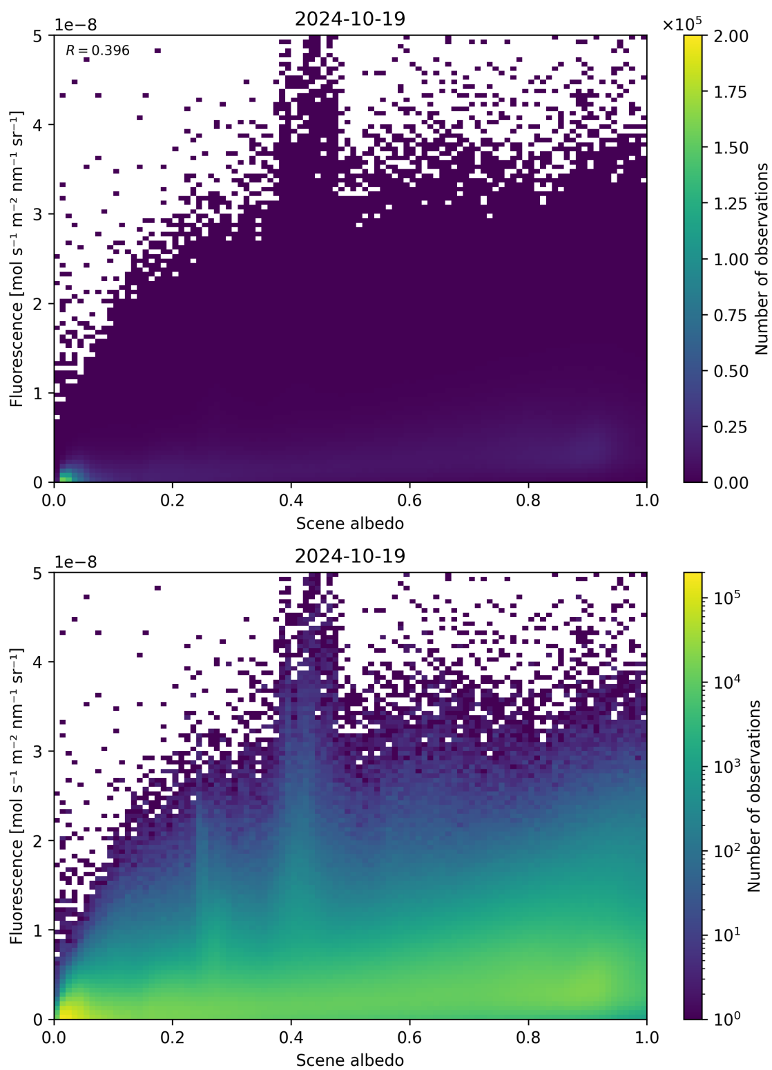
Figure 114: Scatter density plot of “Scene albedo” against “Fluorescence” for 2024-10-19 to 2024-10-20.
