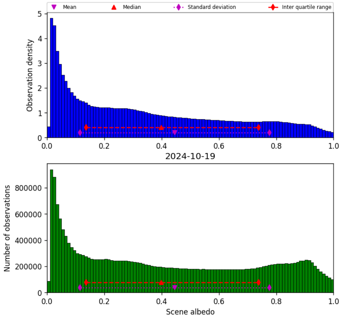
Figure 34: Histogram of “Scene albedo” for 2024-10-19 to 2024-10-20
