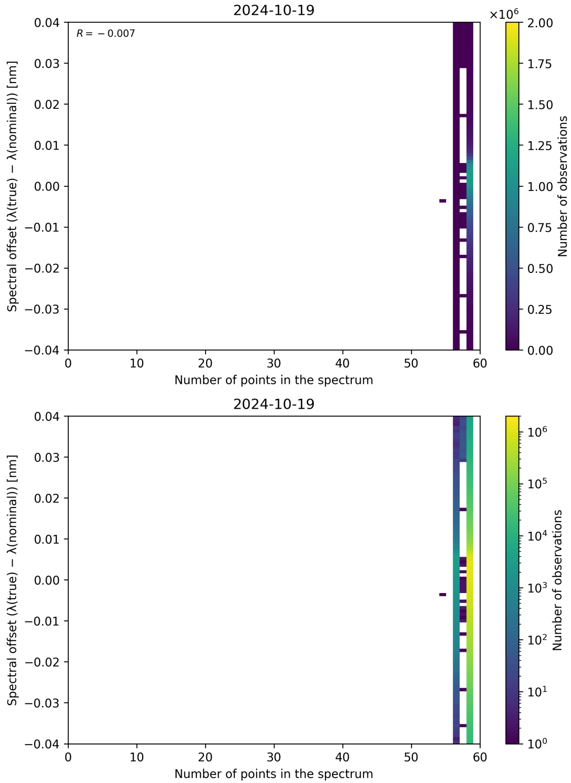
Figure 110: Scatter density plot of “Number of points in the spectrum” against “Spectral offset ( \lambda_{\text{true}} - \lambda_{\text{nominal}} )” for 2024-10-19 to 2024-10-20.
