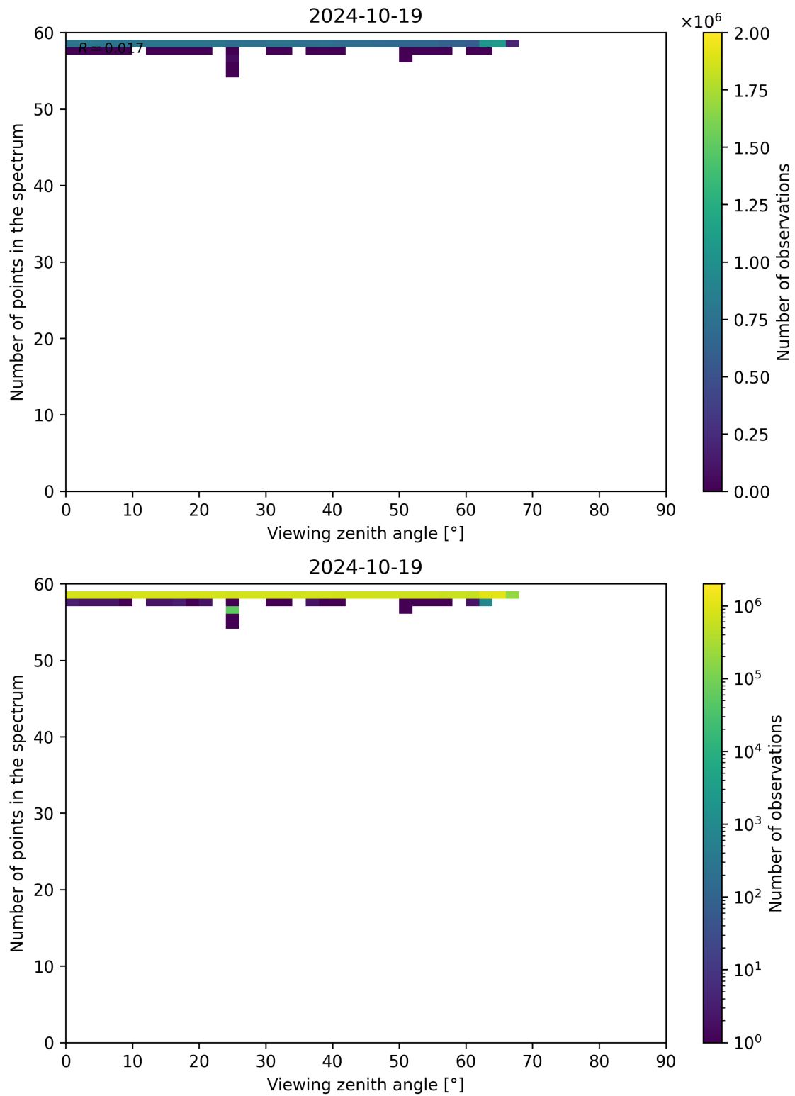
Figure 137: Scatter density plot of “Viewing zenith angle” against “Number of points in the spectrum” for 2024-10-19 to 2024-10-20.
