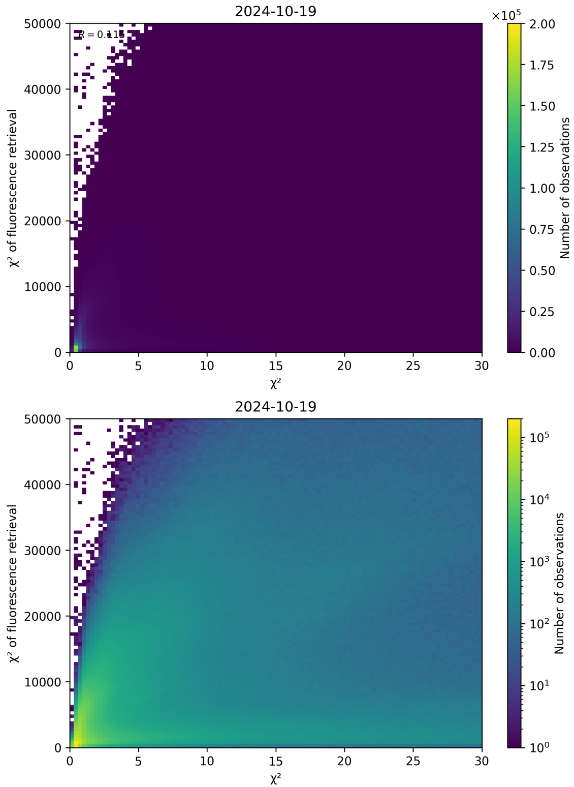
Figure 69: Scatter density plot of “ \chi^2 ” against “ \chi^2 of fluorescence retrieval” for 2024-10-19 to 2024-10-20.
