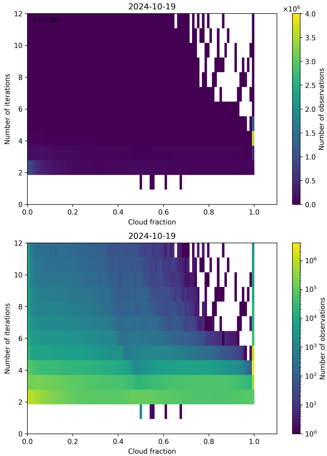
Figure 80: Scatter density plot of “Cloud fraction” against “Number of iterations” for 2024-10-19 to 2024-10-20.
