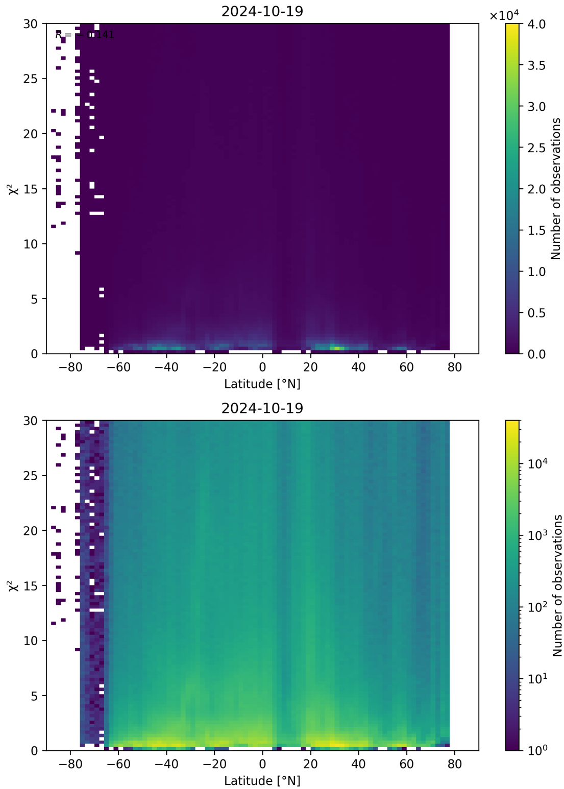
Figure 97: Scatter density plot of “Latitude” against “ \chi^2 ” for 2024-10-19 to 2024-10-20.
