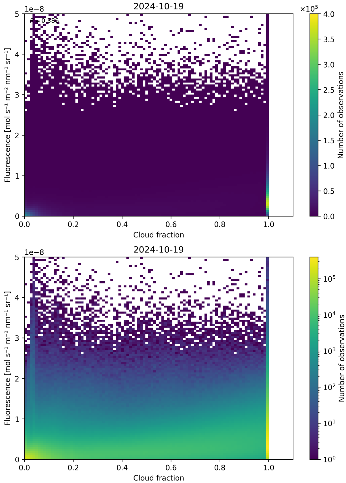
Figure 79: Scatter density plot of “Cloud fraction” against “Fluorescence” for 2024-10-19 to 2024-10-20.
