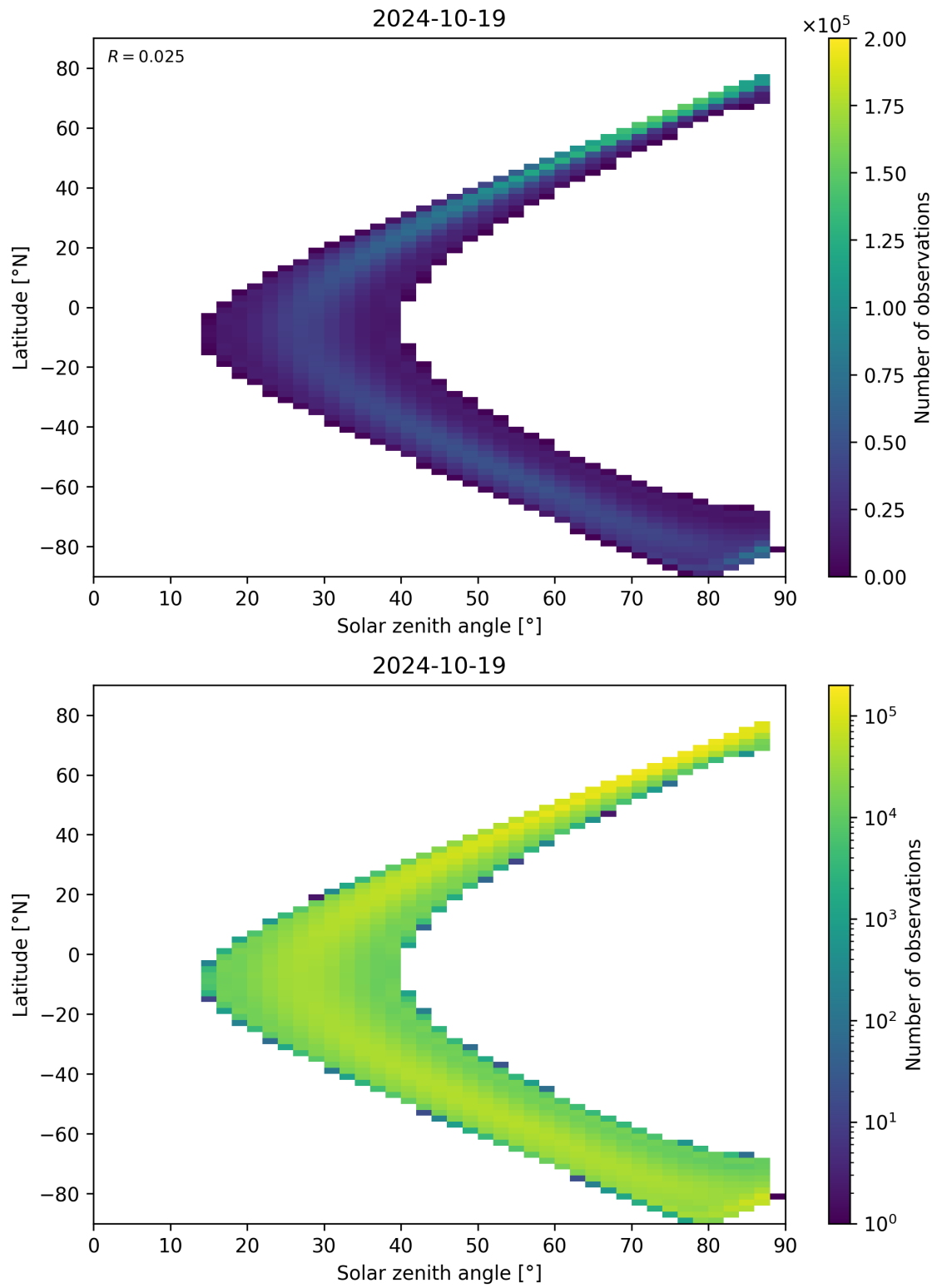
Figure 124: Scatter density plot of “Solar zenith angle” against “Latitude” for 2024-10-19 to 2024-10-20.
