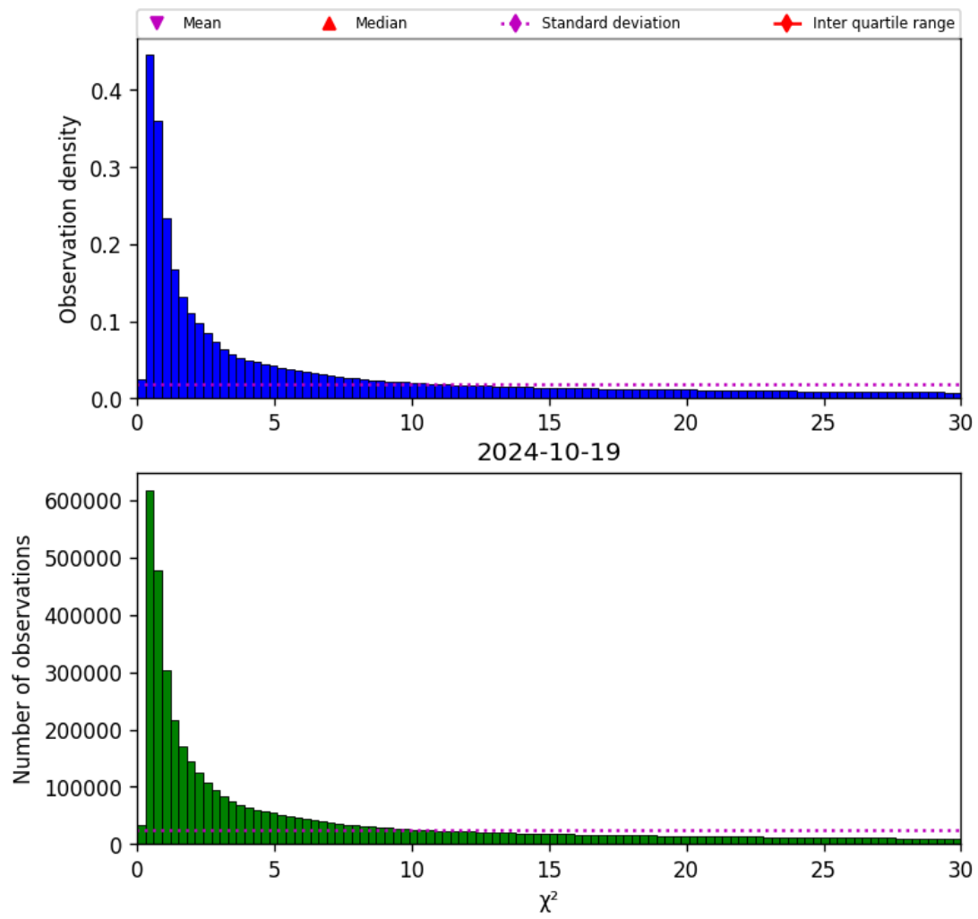
Figure 38: Histogram of “ \chi^2 ” for 2024-10-19 to 2024-10-20
