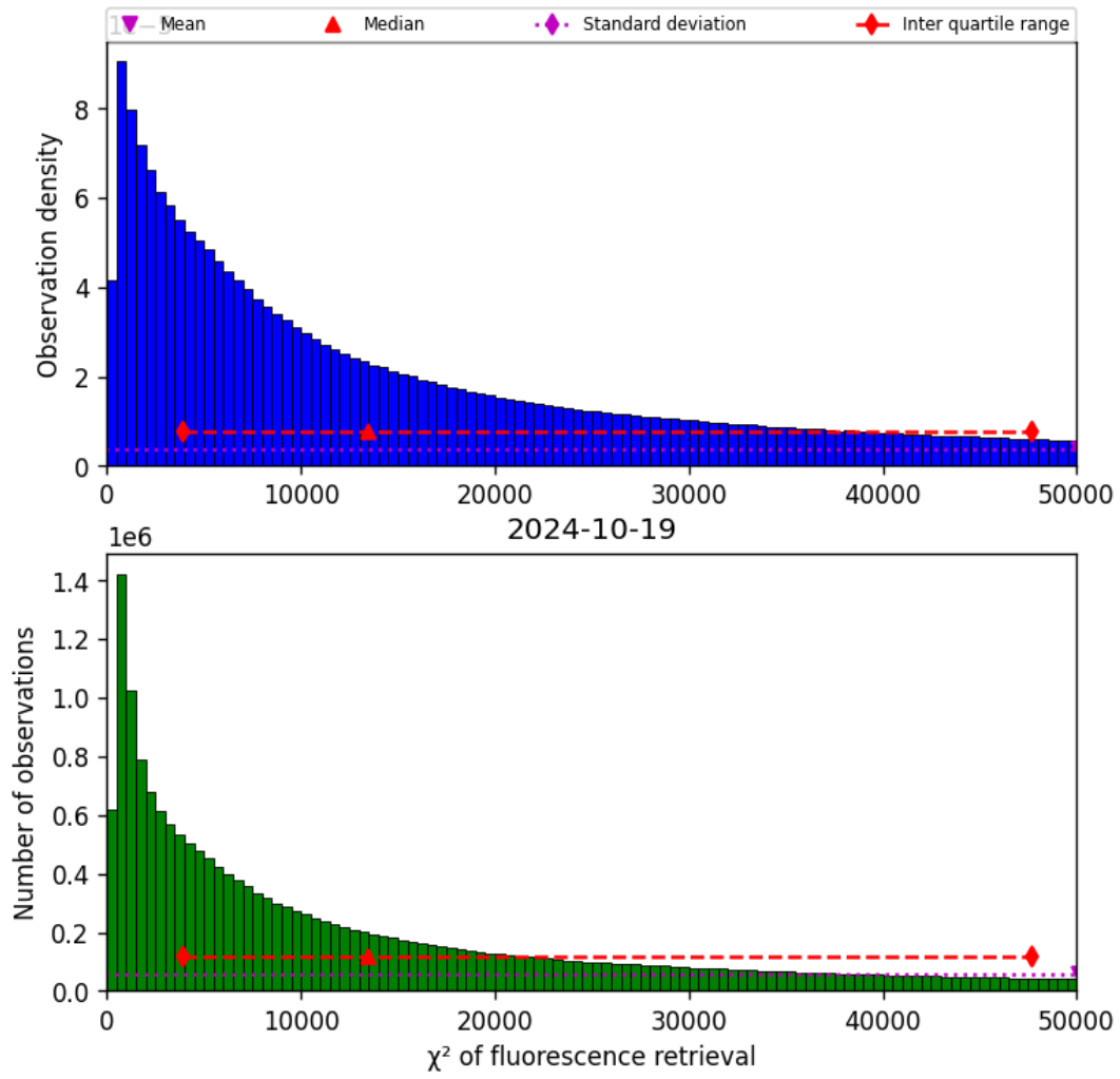
Figure 42: Histogram of “ \chi^2 of fluorescence retrieval” for 2024-10-19 to 2024-10-20
