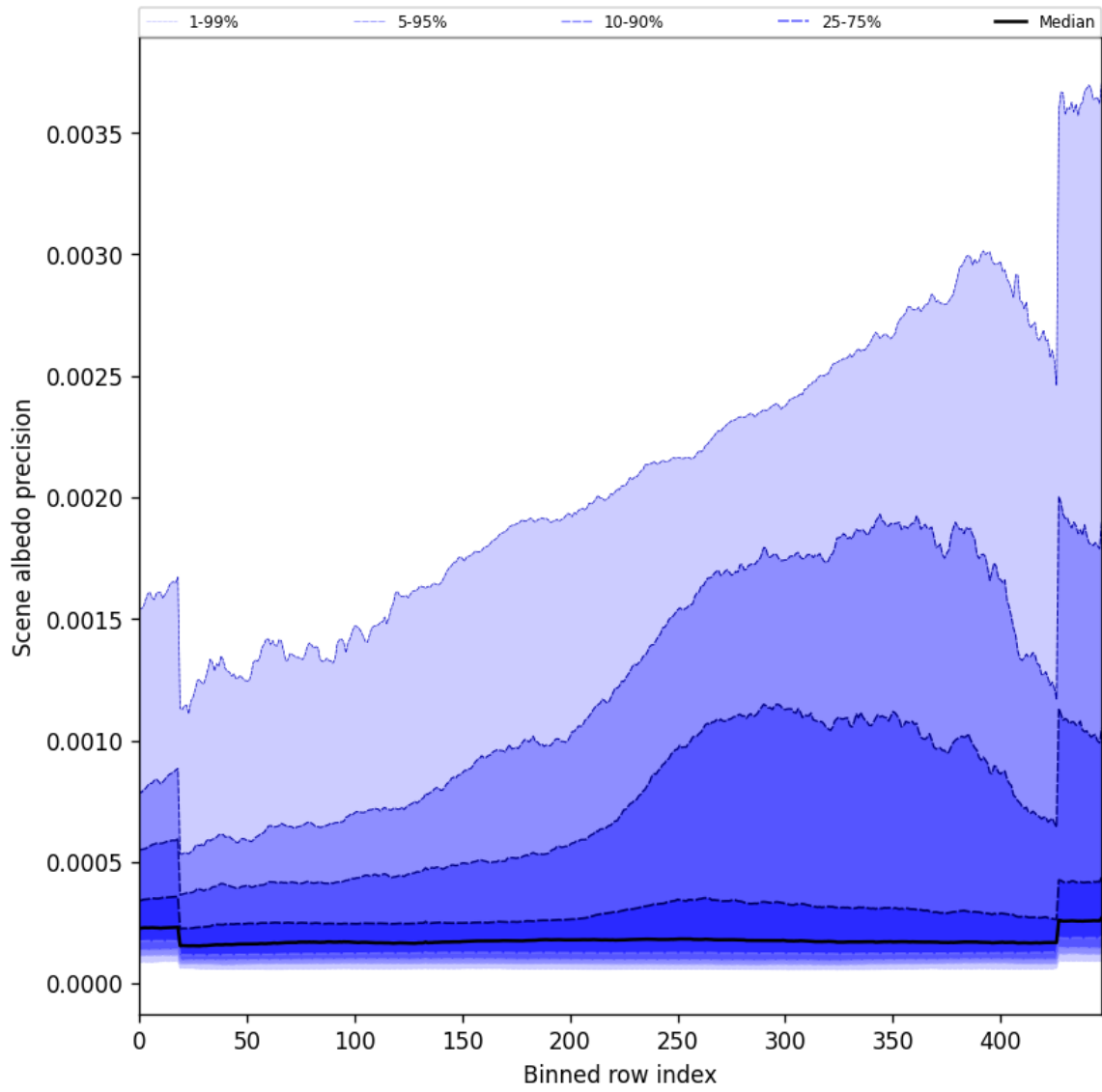
Figure 52: Along track statistics of “Scene albedo precision” for 2024-10-19 to 2024-10-20
