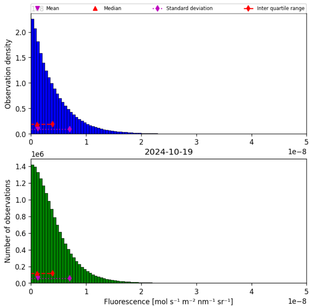
Figure 40: Histogram of “Fluorescence” for 2024-10-19 to 2024-10-20
