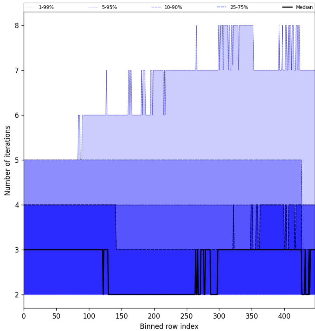
Figure 56: Along track statistics of “Number of iterations” for 2024-10-19 to 2024-10-20
