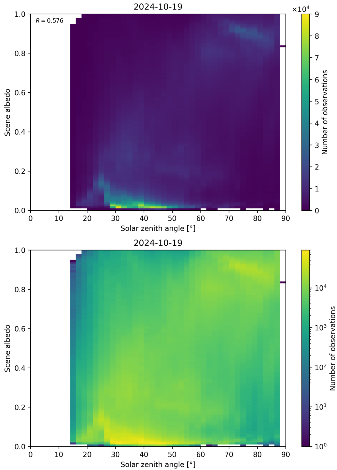
Figure 127: Scatter density plot of “Solar zenith angle” against “Scene albedo” for 2024-10-19 to 2024-10-20.
