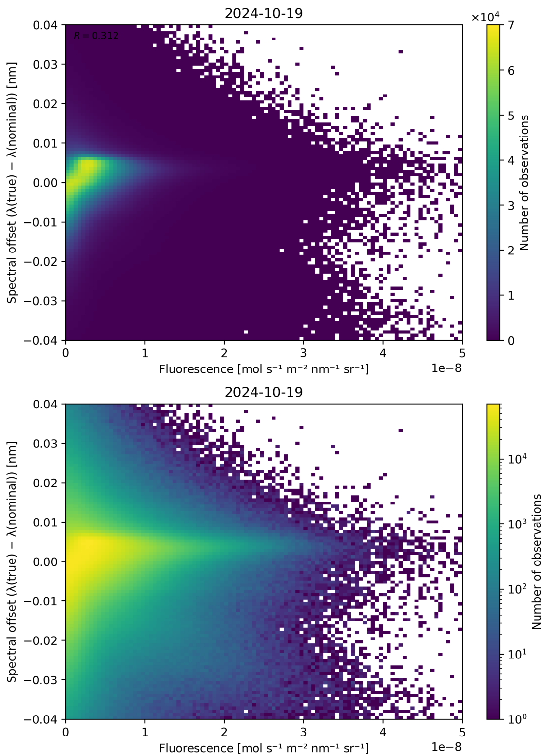
Figure 95: Scatter density plot of “Fluorescence” against “Spectral offset ( \lambda_{\text{true}} - \lambda_{\text{nominal}} )” for 2024-10-19 to 2024-10-20.
