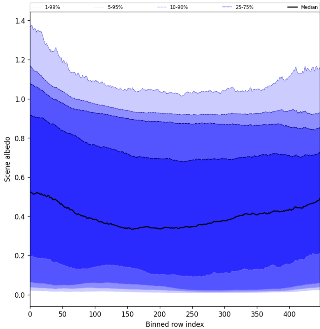
Figure 51: Along track statistics of “Scene albedo” for 2024-10-19 to 2024-10-20
