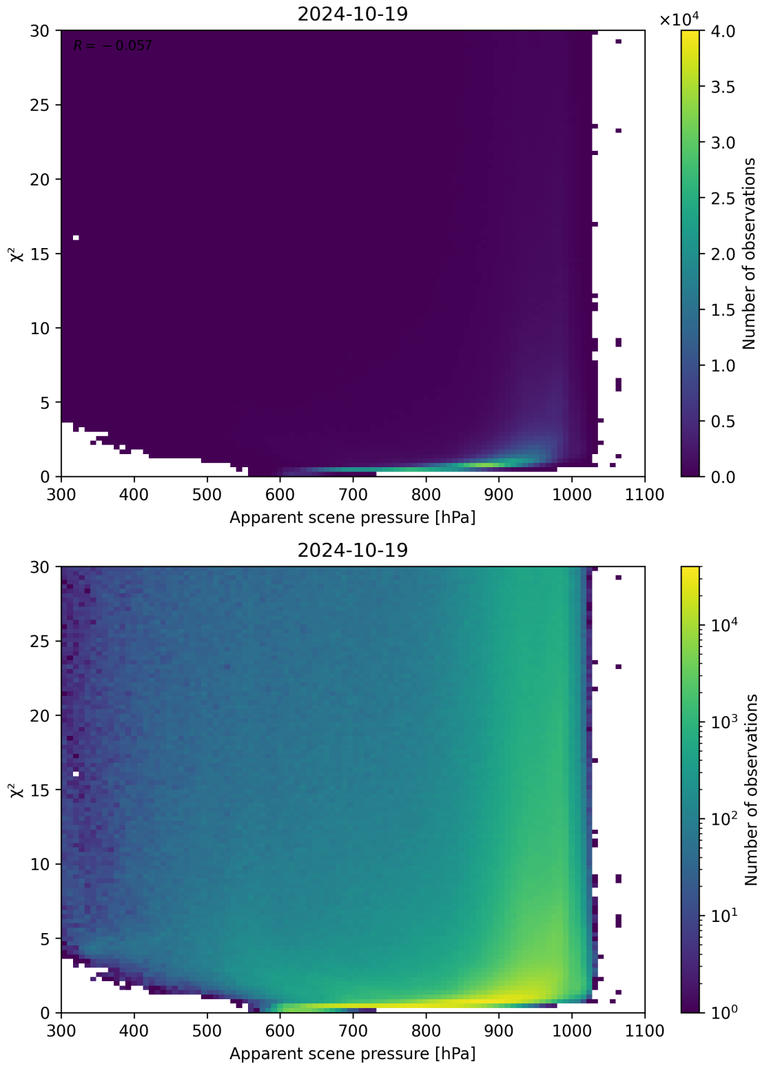
Figure 63: Scatter density plot of “Apparent scene pressure” against “ \chi^2 ” for 2024-10-19 to 2024-10-20.
