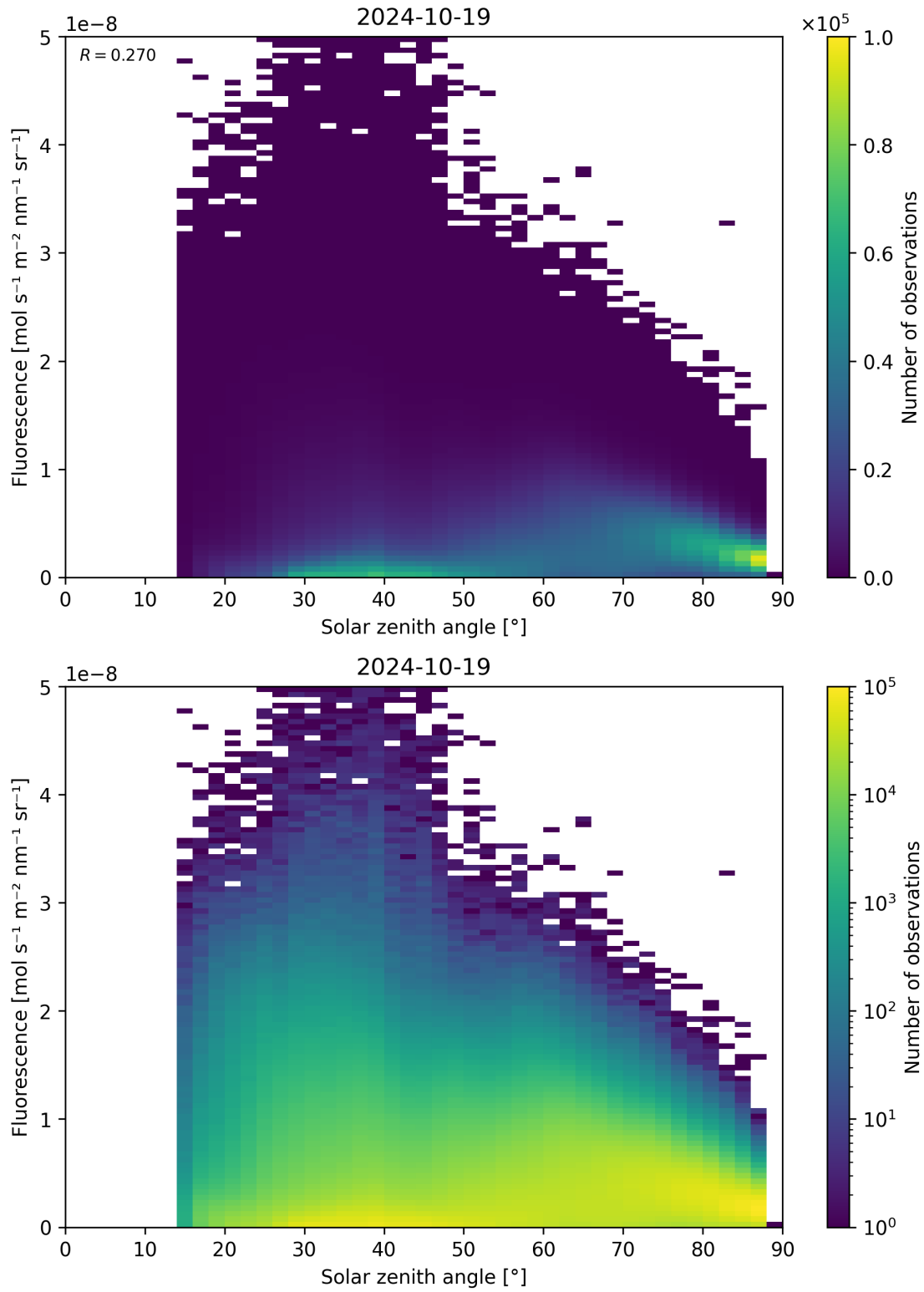
Figure 123: Scatter density plot of “Solar zenith angle” against “Fluorescence” for 2024-10-19 to 2024-10-20.
