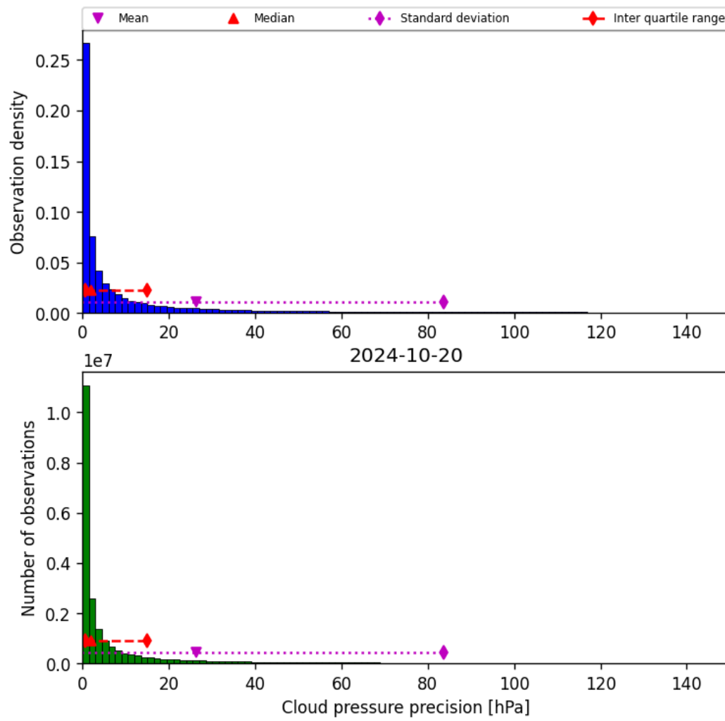
Figure 31: Histogram of “Cloud pressure precision” for 2024-10-19 to 2024-10-21
