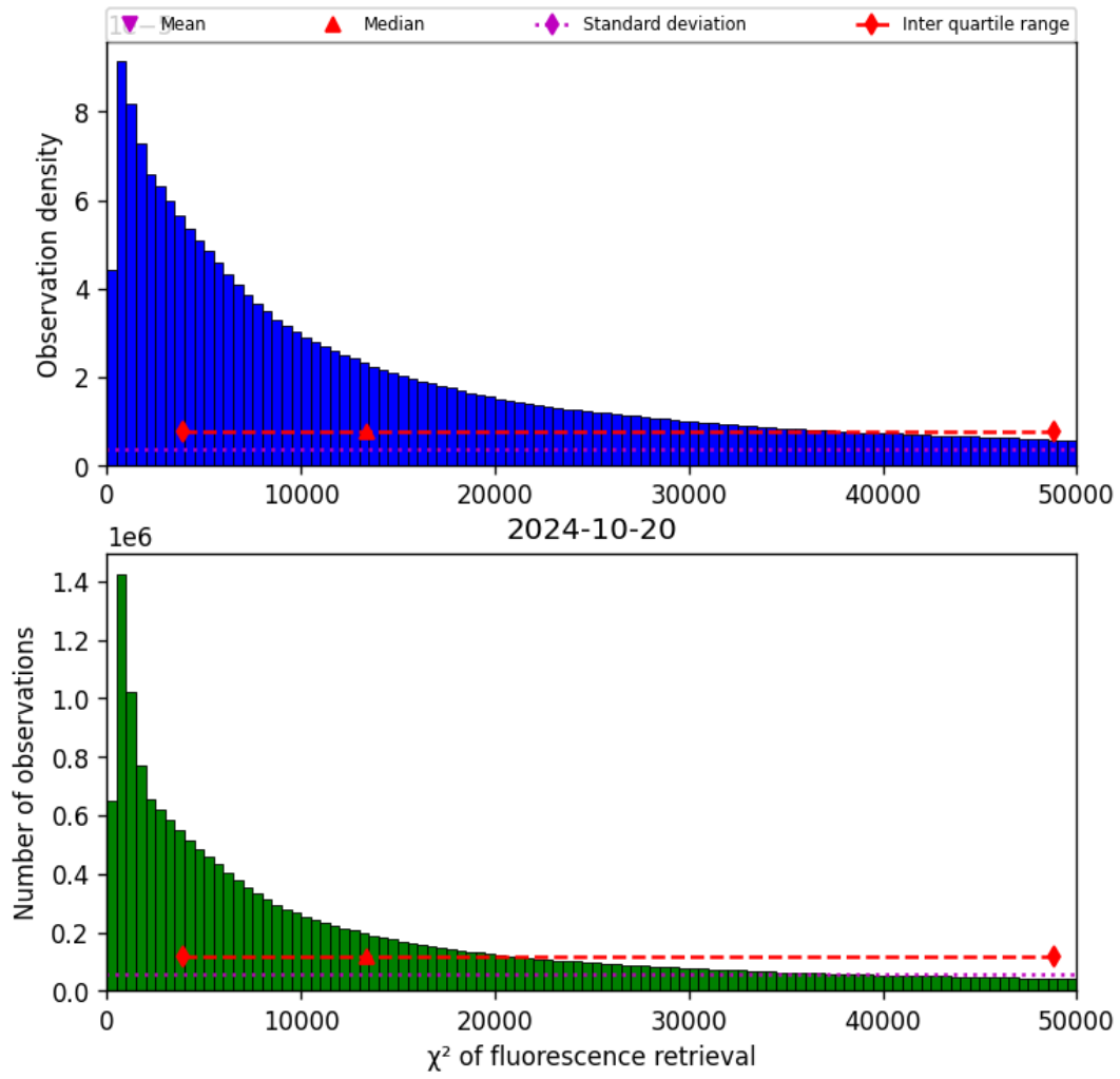
Figure 42: Histogram of “ \chi^2 of fluorescence retrieval” for 2024-10-19 to 2024-10-21
