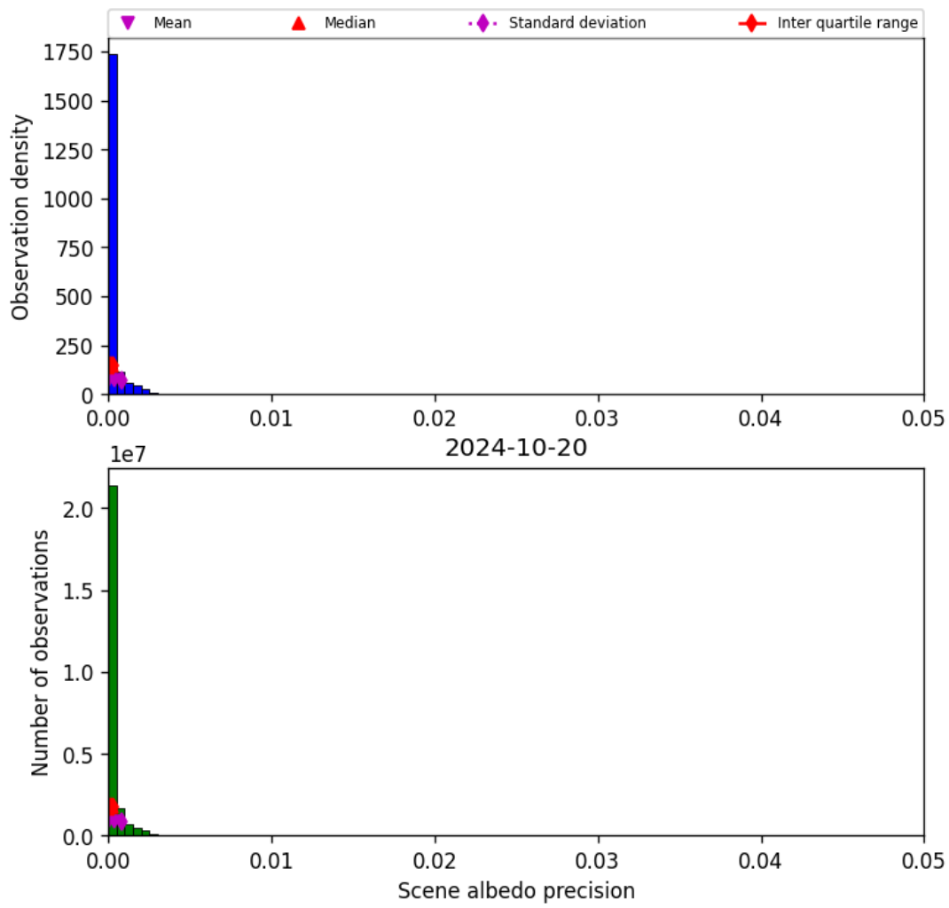
Figure 35: Histogram of “Scene albedo precision” for 2024-10-19 to 2024-10-21
