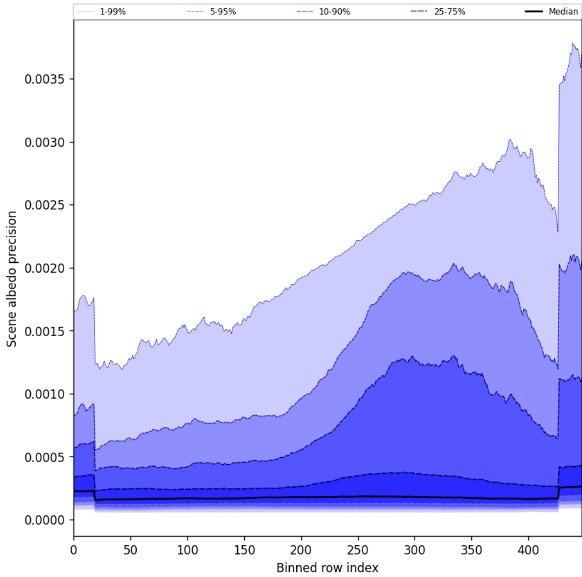
Figure 52: Along track statistics of “Scene albedo precision” for 2024-10-19 to 2024-10-21
