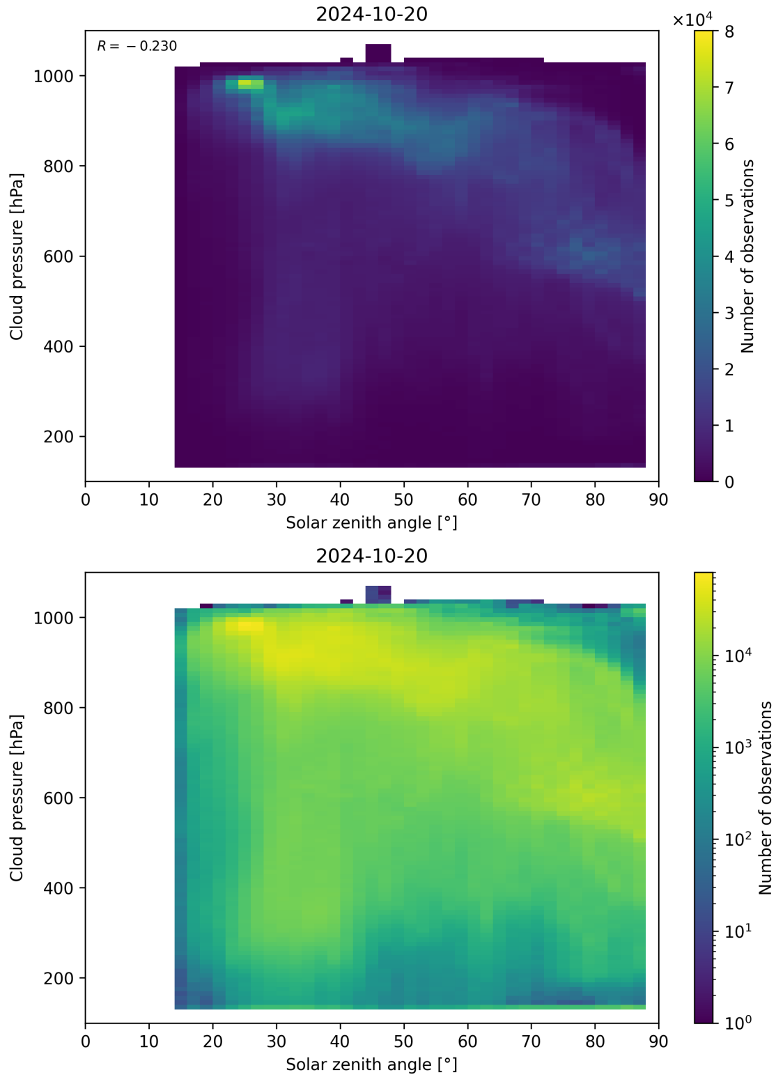
Figure 122: Scatter density plot of “Solar zenith angle” against “Cloud pressure” for 2024-10-19 to 2024-10-21.
