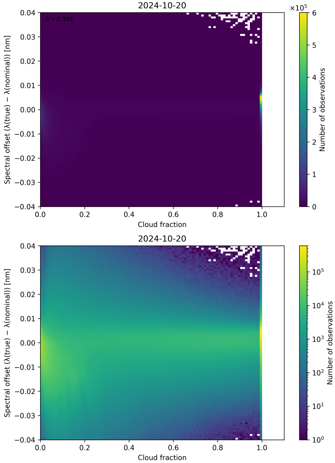
Figure 83: Scatter density plot of “Cloud fraction” against “Spectral offset ( \lambda_{\text{true}} - \lambda_{\text{nominal}} )” for 2024-10-19 to 2024-10-21.
