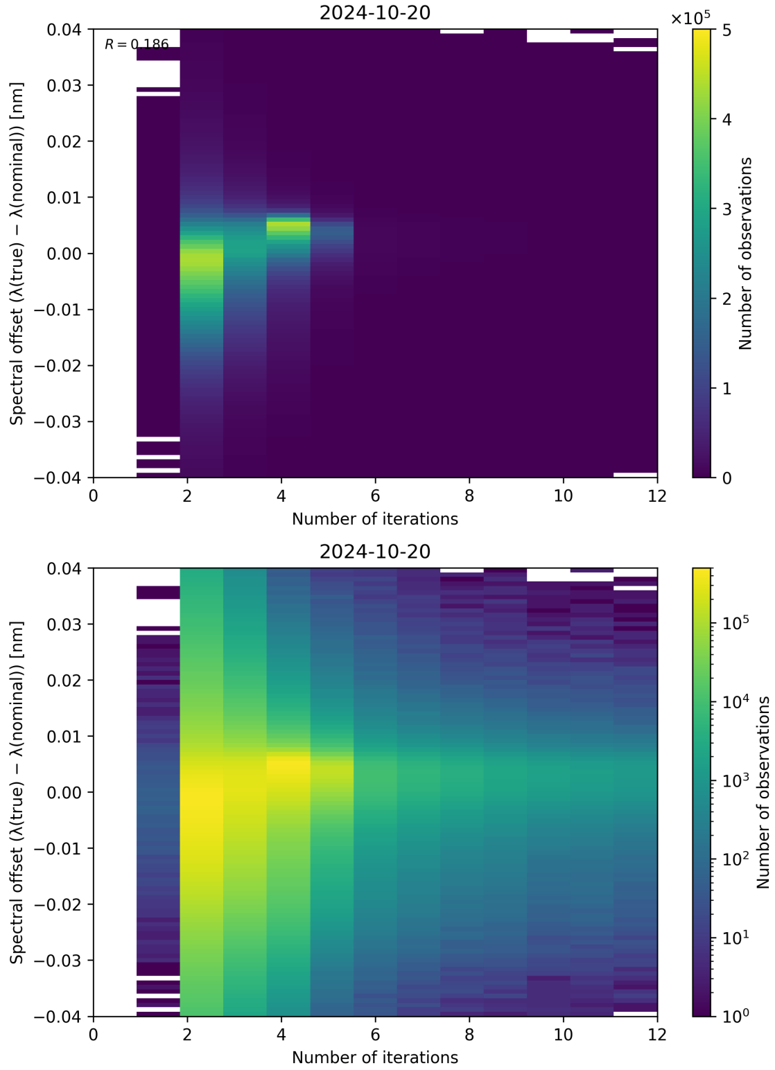
Figure 109: Scatter density plot of “Number of iterations” against “Spectral offset ( \lambda_{\text{true}} - \lambda_{\text{nominal}} )” for 2024-10-19 to 2024-10-21.
