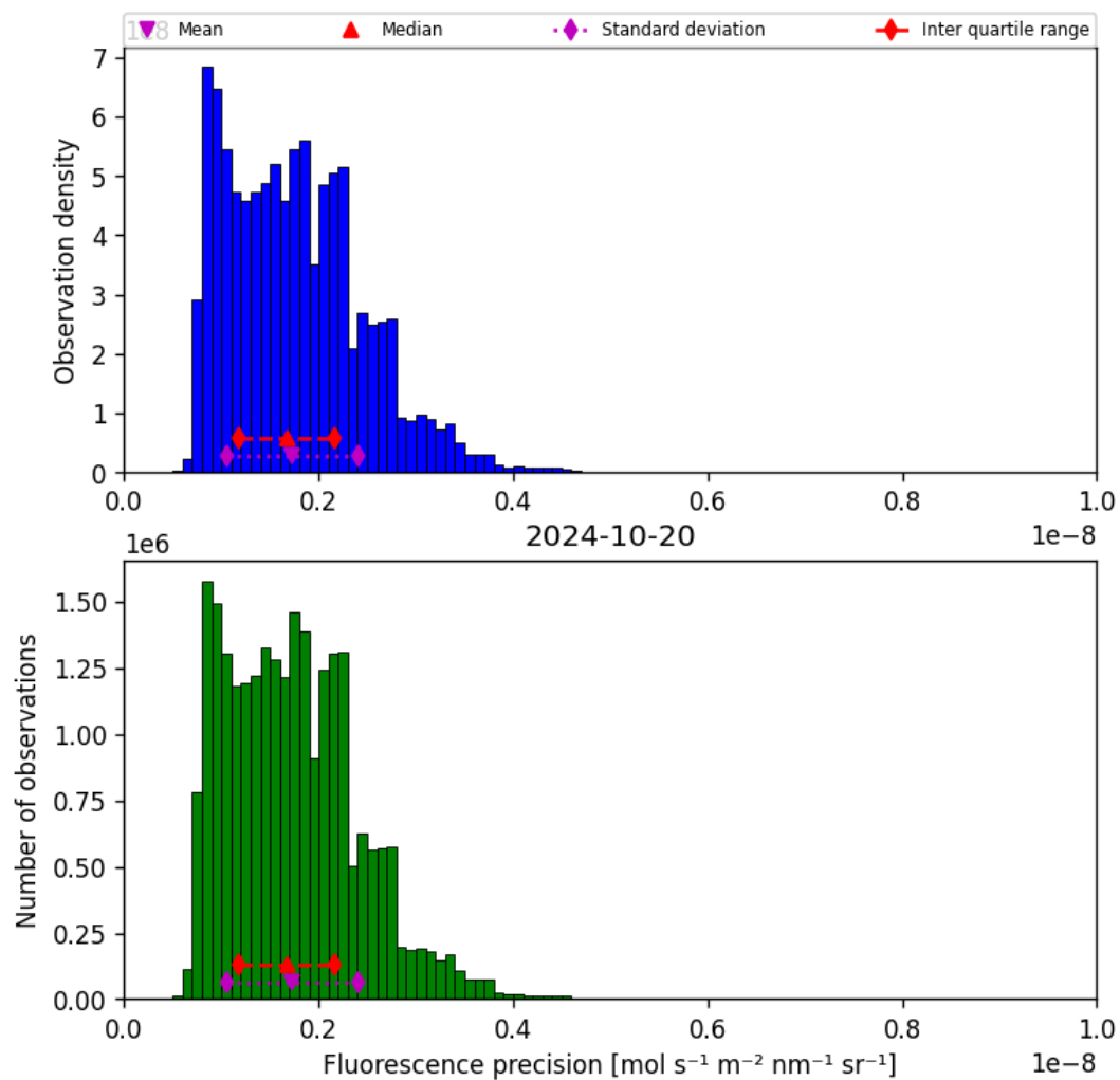
Figure 41: Histogram of “Fluorescence precision” for 2024-10-19 to 2024-10-21
