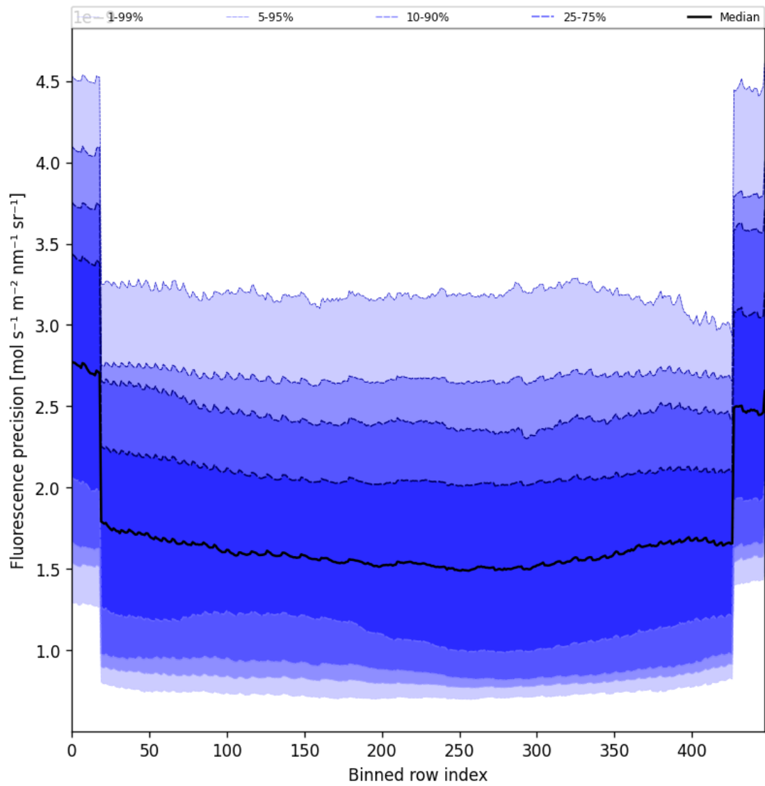
Figure 58: Along track statistics of “Fluorescence precision” for 2024-10-19 to 2024-10-21
