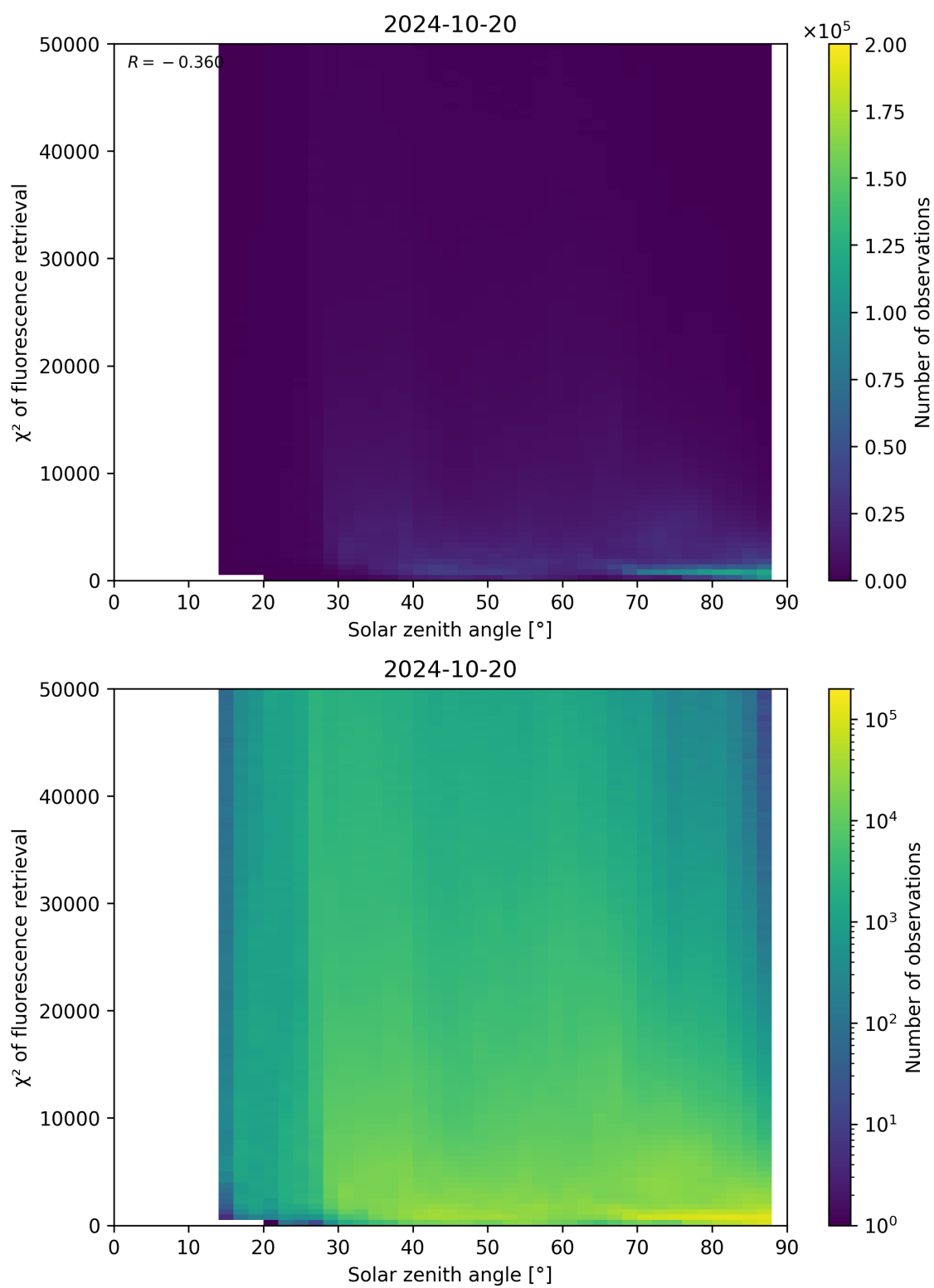
Figure 120: Scatter density plot of “Solar zenith angle” against “ \chi^2 of fluorescence retrieval” for 2024-10-19 to 2024-10-21.
