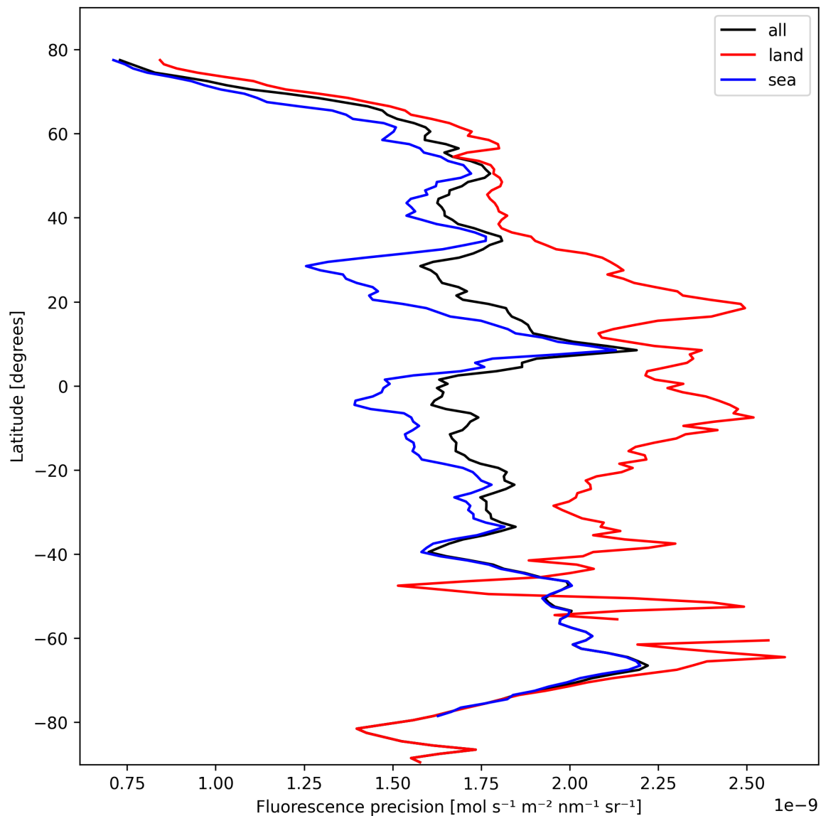
Figure 24: Zonal average of “Fluorescence precision” for 2024-10-19 to 2024-10-21.
