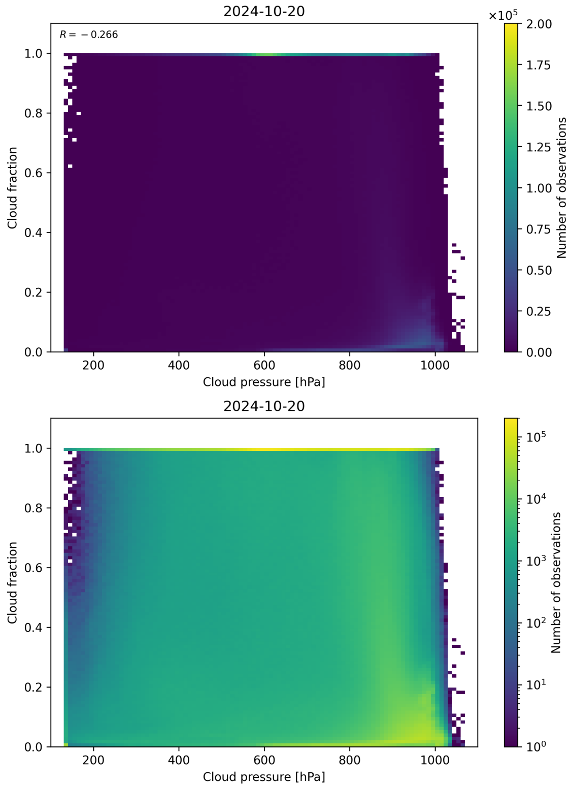
Figure 87: Scatter density plot of “Cloud pressure” against “Cloud fraction” for 2024-10-19 to 2024-10-21.
