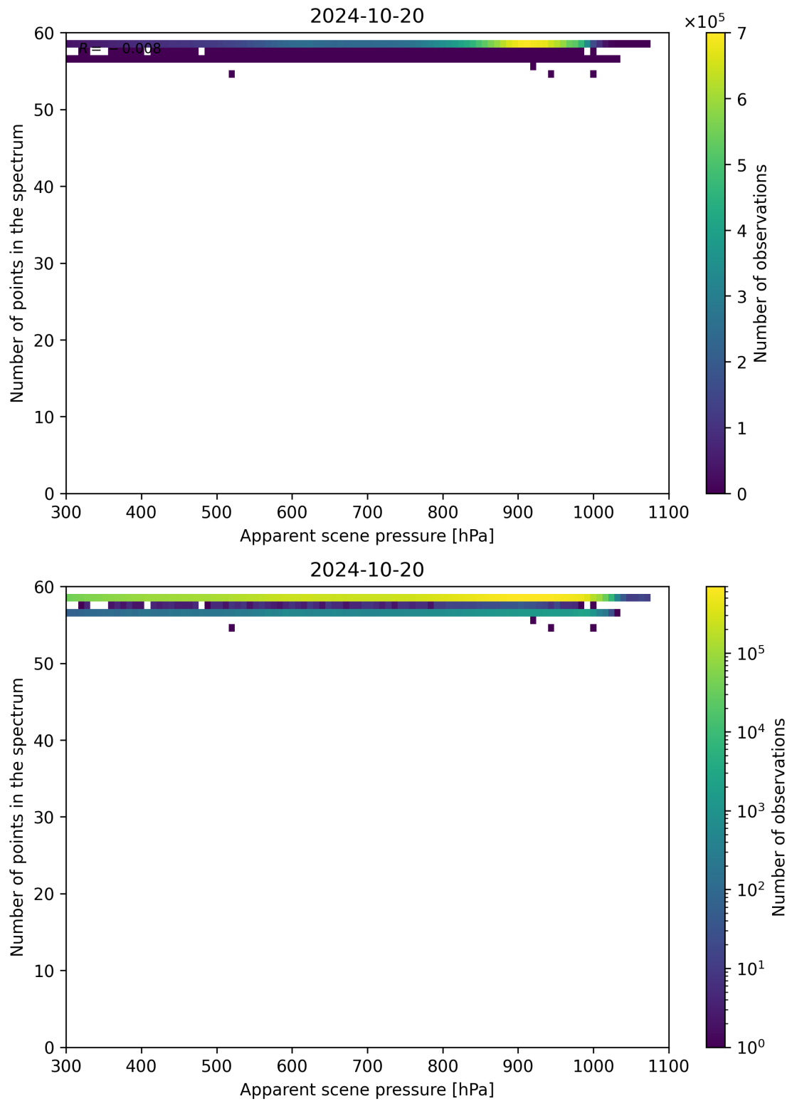
Figure 67: Scatter density plot of “Apparent scene pressure” against “Number of points in the spectrum” for 2024-10-19 to 2024-10-21.
