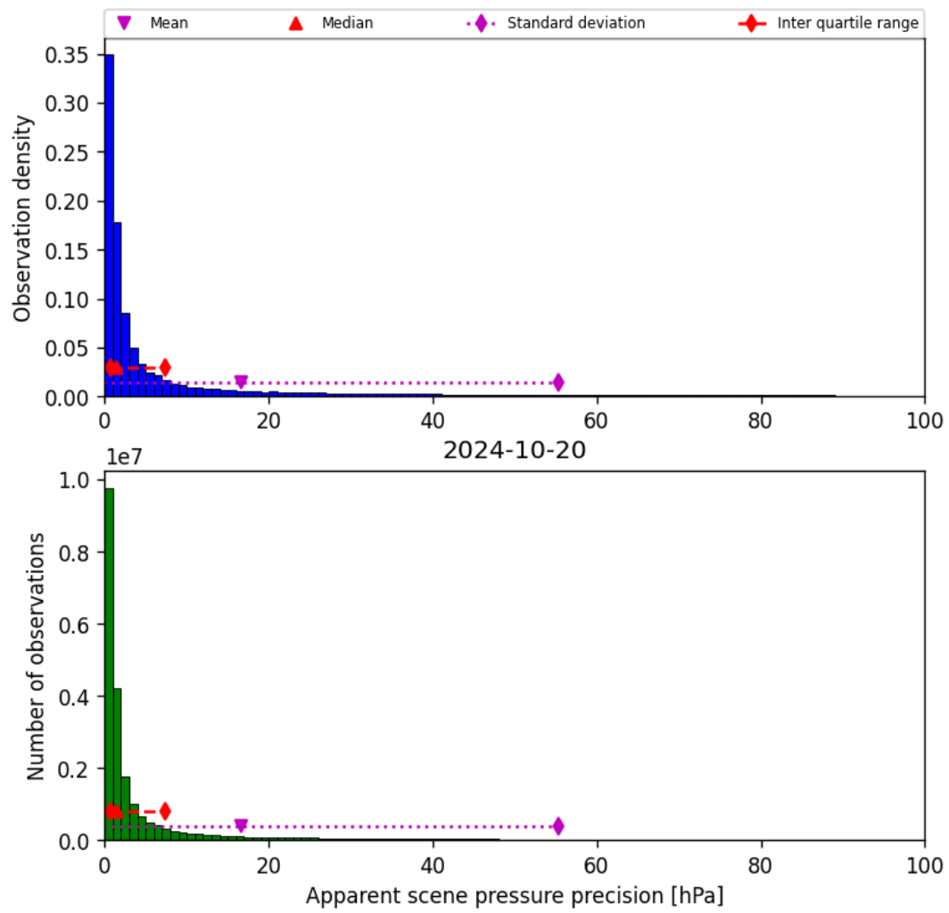
Figure 37: Histogram of “Apparent scene pressure precision” for 2024-10-19 to 2024-10-21
