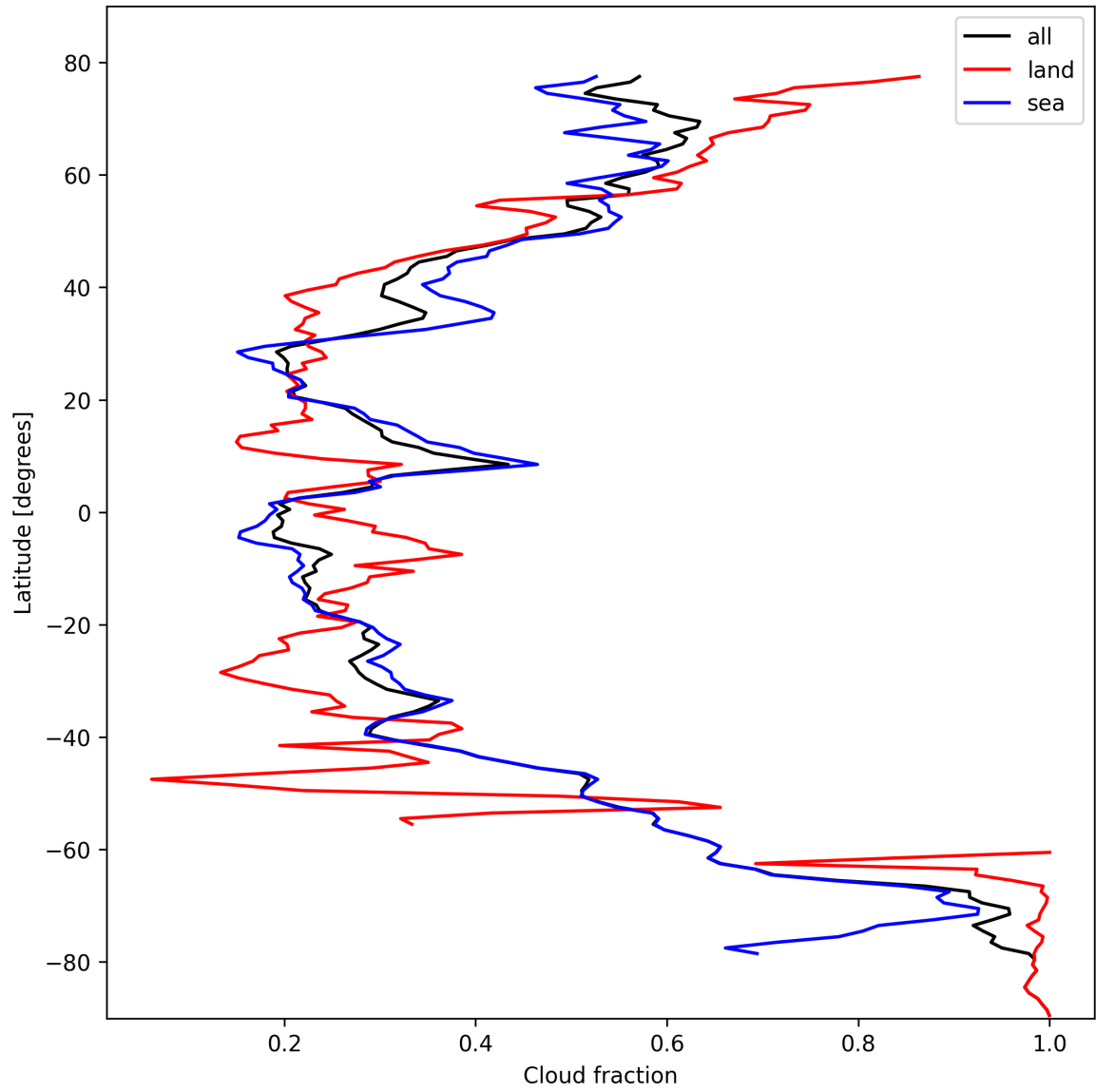
Figure 15: Zonal average of “Cloud fraction” for 2024-10-19 to 2024-10-21.
