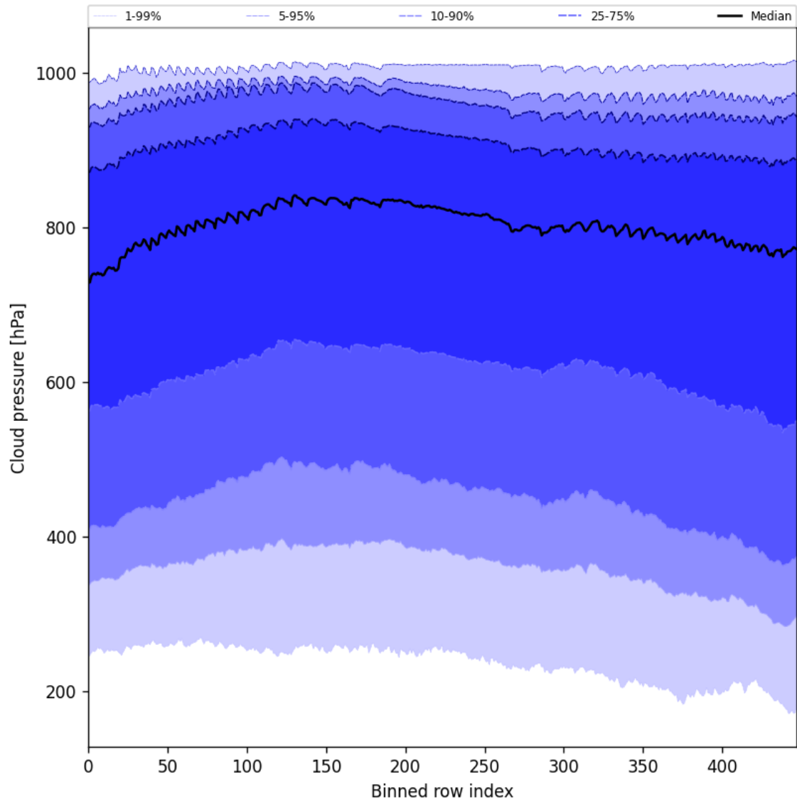
Figure 47: Along track statistics of “Cloud pressure” for 2024-10-19 to 2024-10-21
