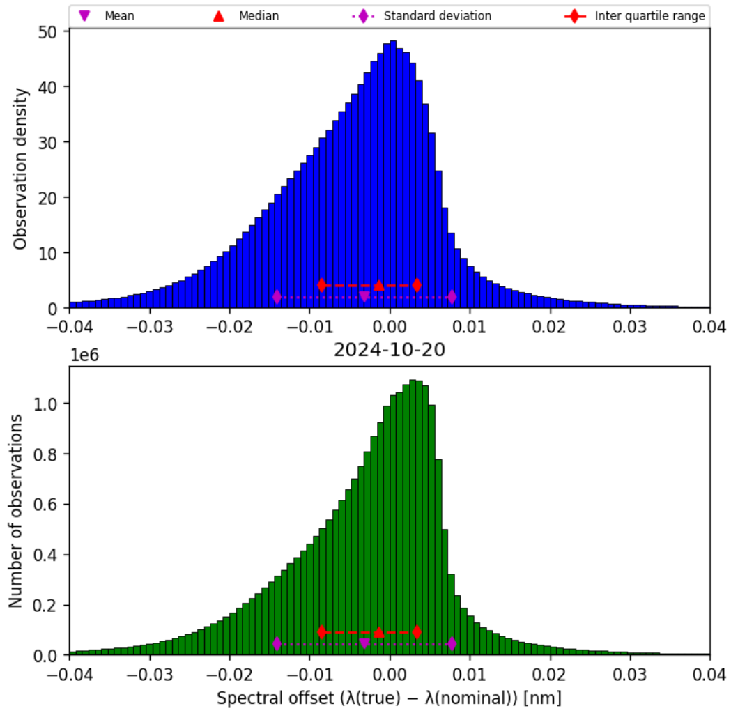
Figure 45: Histogram of “Spectral offset ( \lambda_{\text{true}} - \lambda_{\text{nominal}} )” for 2024-10-19 to 2024-10-21
