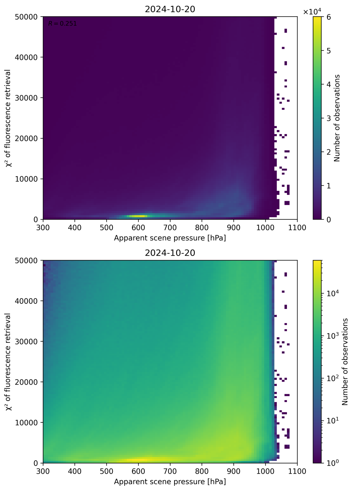
Figure 64: Scatter density plot of “Apparent scene pressure” against “ \chi^2 of fluorescence retrieval” for 2024-10-19 to 2024-10-21.
