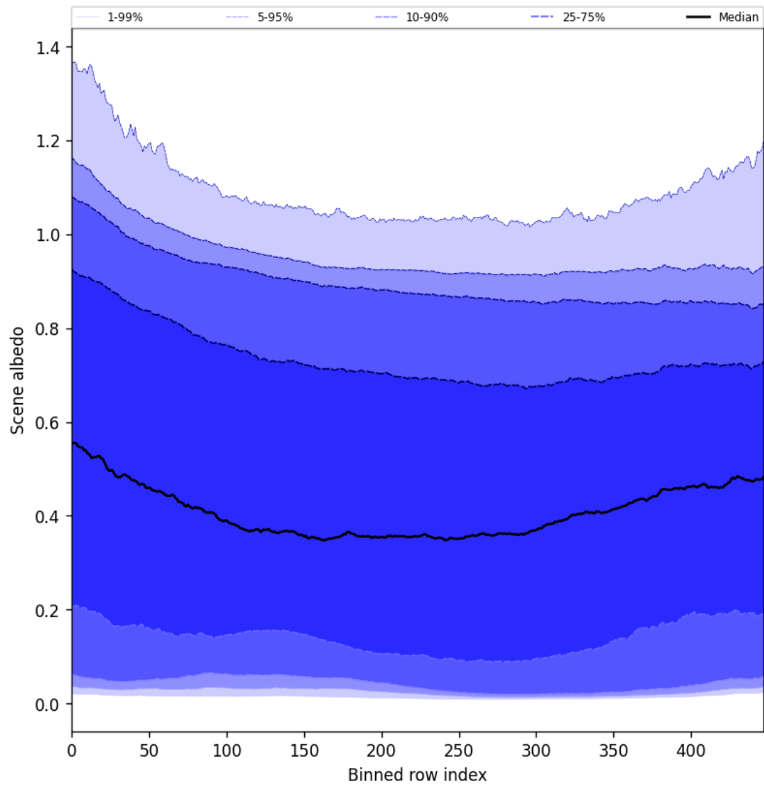
Figure 51: Along track statistics of “Scene albedo” for 2024-10-19 to 2024-10-21
