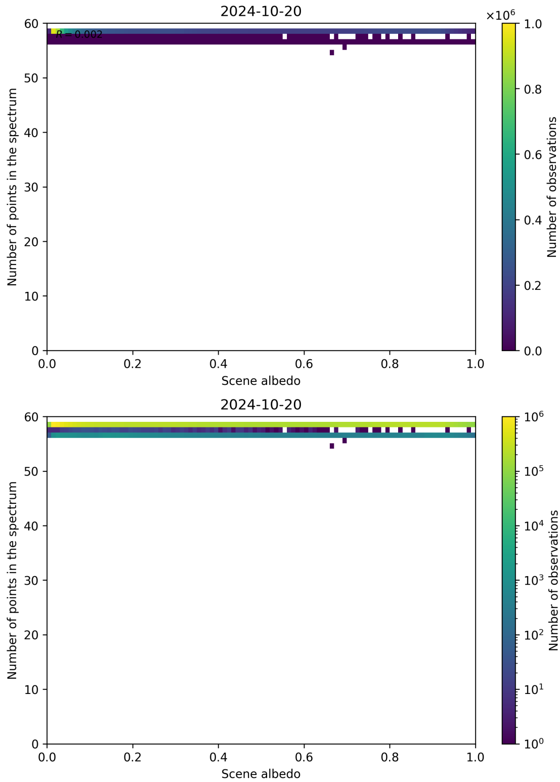
Figure 116: Scatter density plot of “Scene albedo” against “Number of points in the spectrum” for 2024-10-19 to 2024-10-21.
