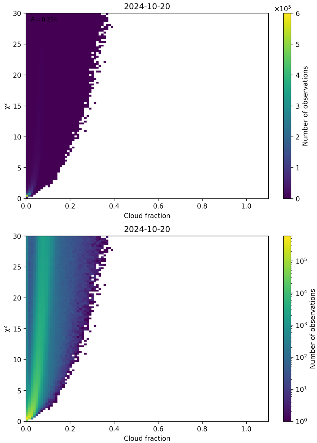
Figure 77: Scatter density plot of “Cloud fraction” against “ \chi^2 ” for 2024-10-19 to 2024-10-21.
