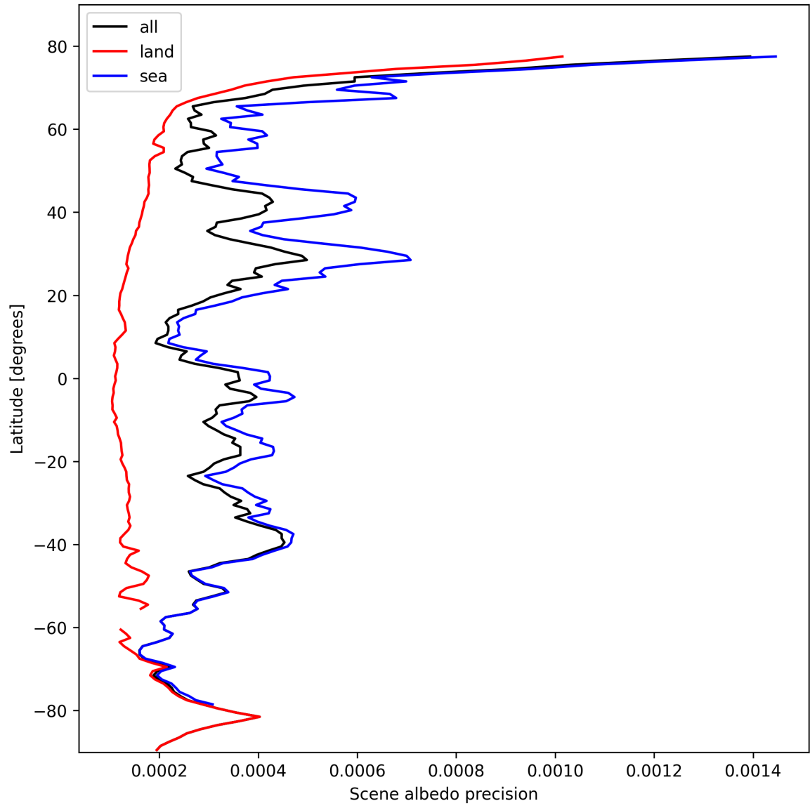
Figure 18: Zonal average of “Scene albedo precision” for 2024-10-19 to 2024-10-21.
