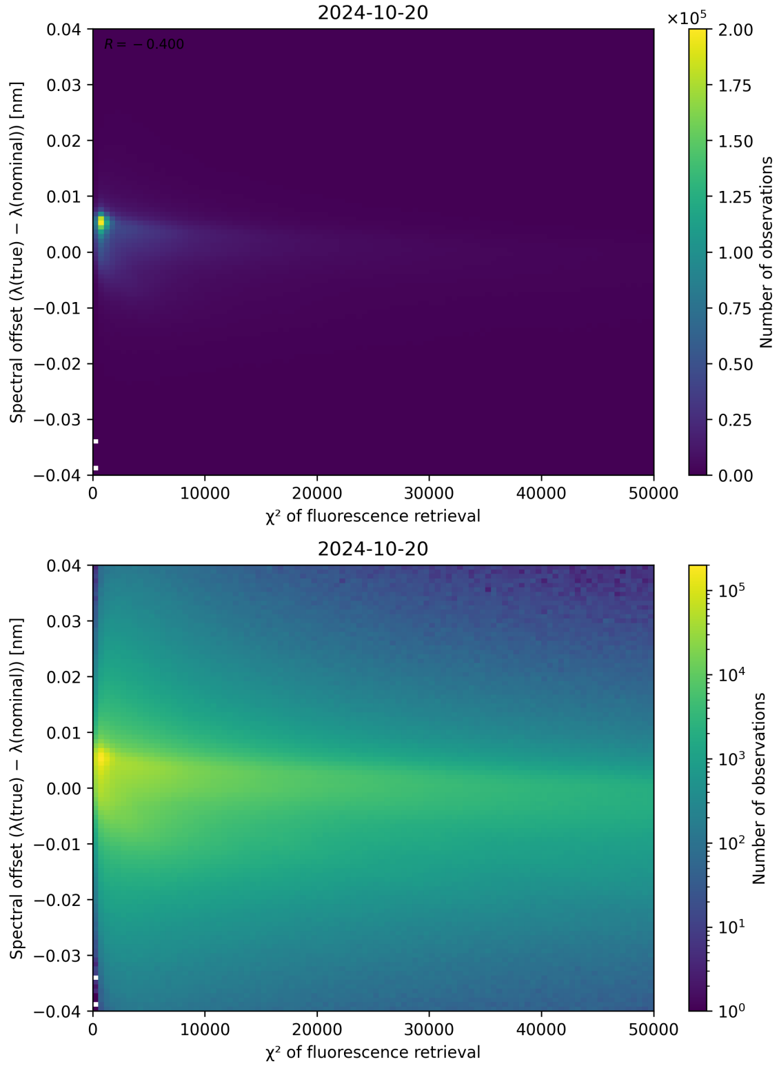
Figure 72: Scatter density plot of “ \chi^2 of fluorescence retrieval” against “Spectral offset ( \lambda_{\text{true}} - \lambda_{\text{nominal}} )” for 2024-10-19 to 2024-10-21.
