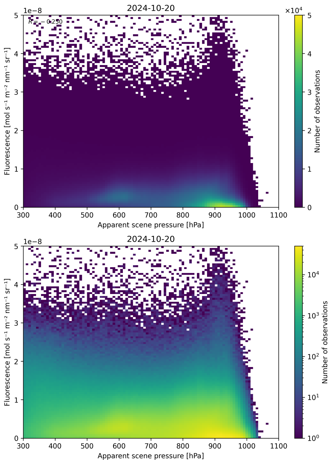
Figure 65: Scatter density plot of “Apparent scene pressure” against “Fluorescence” for 2024-10-19 to 2024-10-21.
