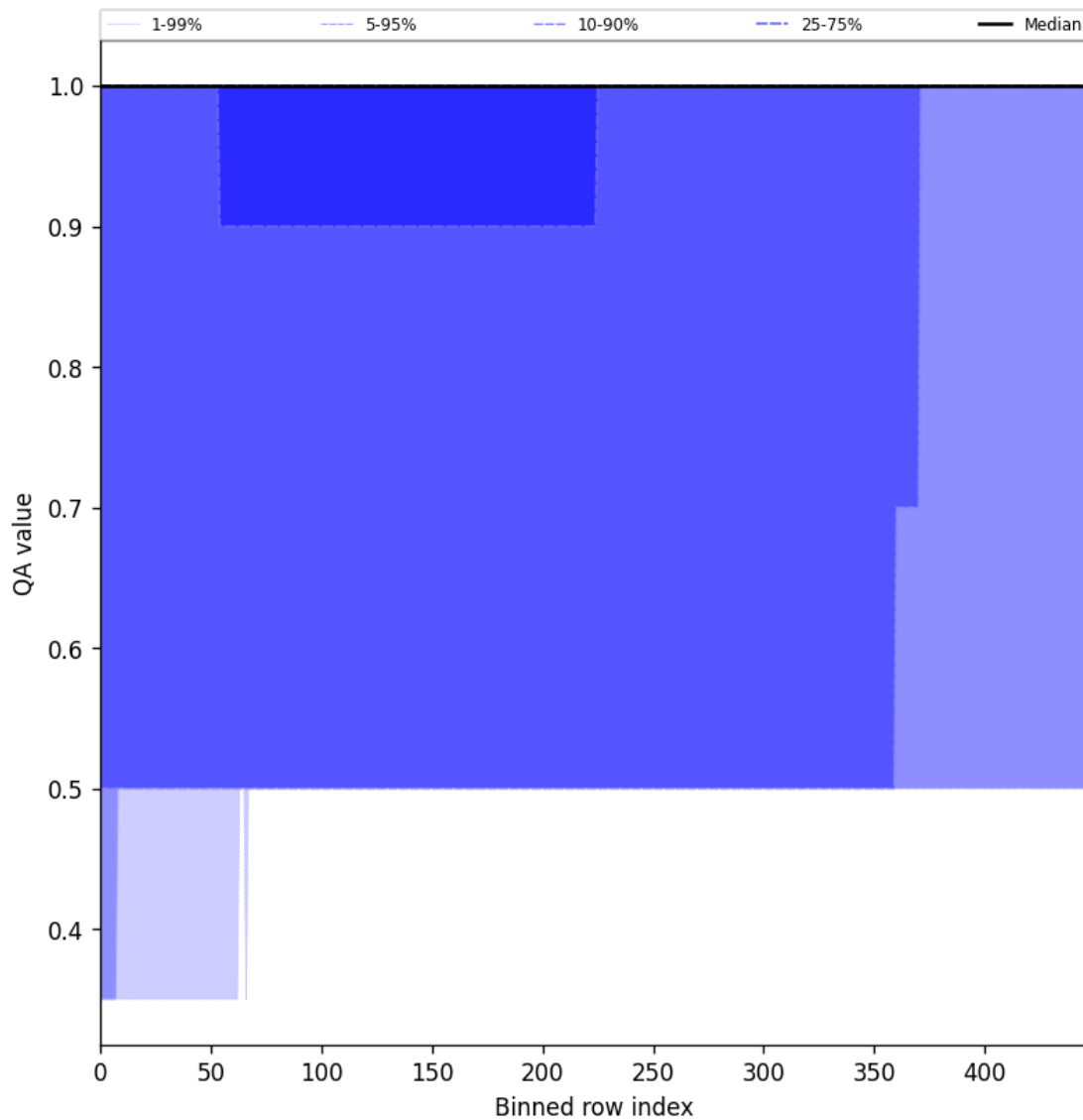
Figure 46: Along track statistics of “QA value” for 2024-10-19 to 2024-10-21
