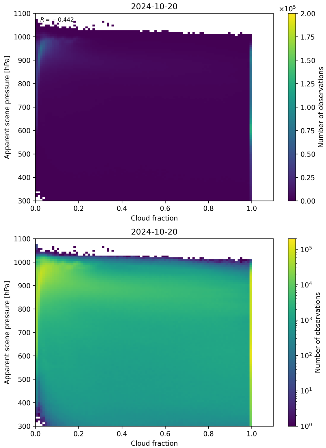
Figure 76: Scatter density plot of “Cloud fraction” against “Apparent scene pressure” for 2024-10-19 to 2024-10-21.
