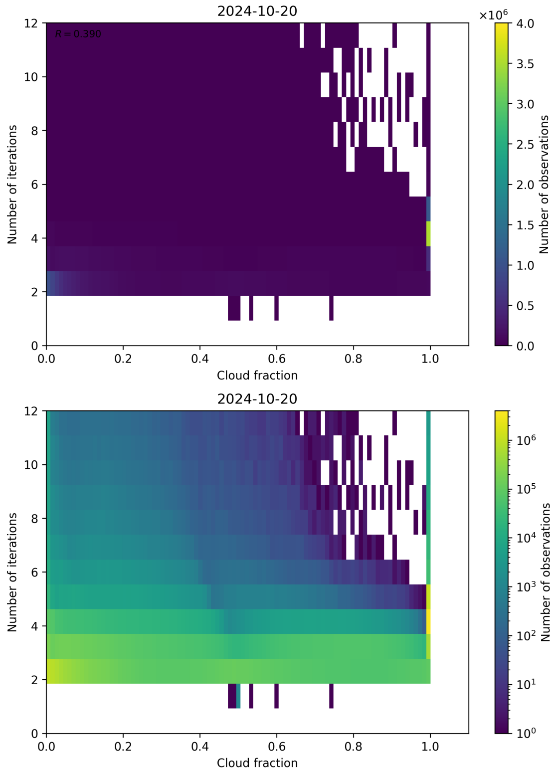
Figure 80: Scatter density plot of “Cloud fraction” against “Number of iterations” for 2024-10-19 to 2024-10-21.
