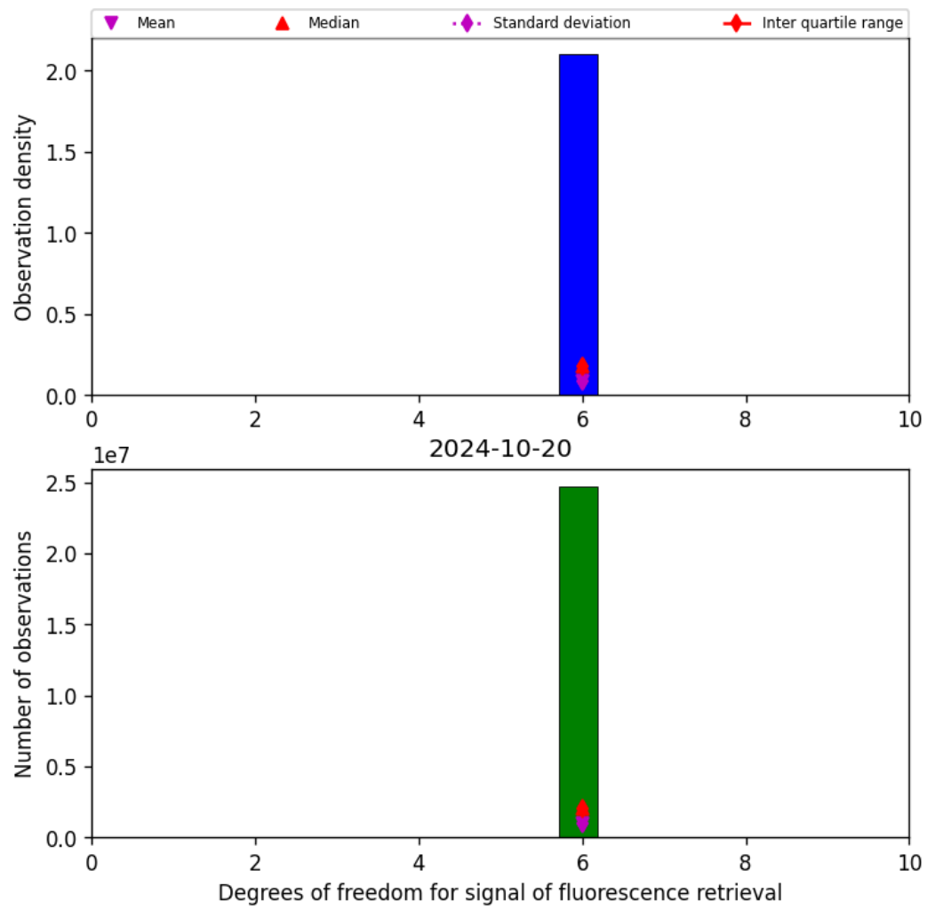
Figure 43: Histogram of "Degrees of freedom for signal of fluorescence retrieval" for 2024-10-19 to 2024-10-21
