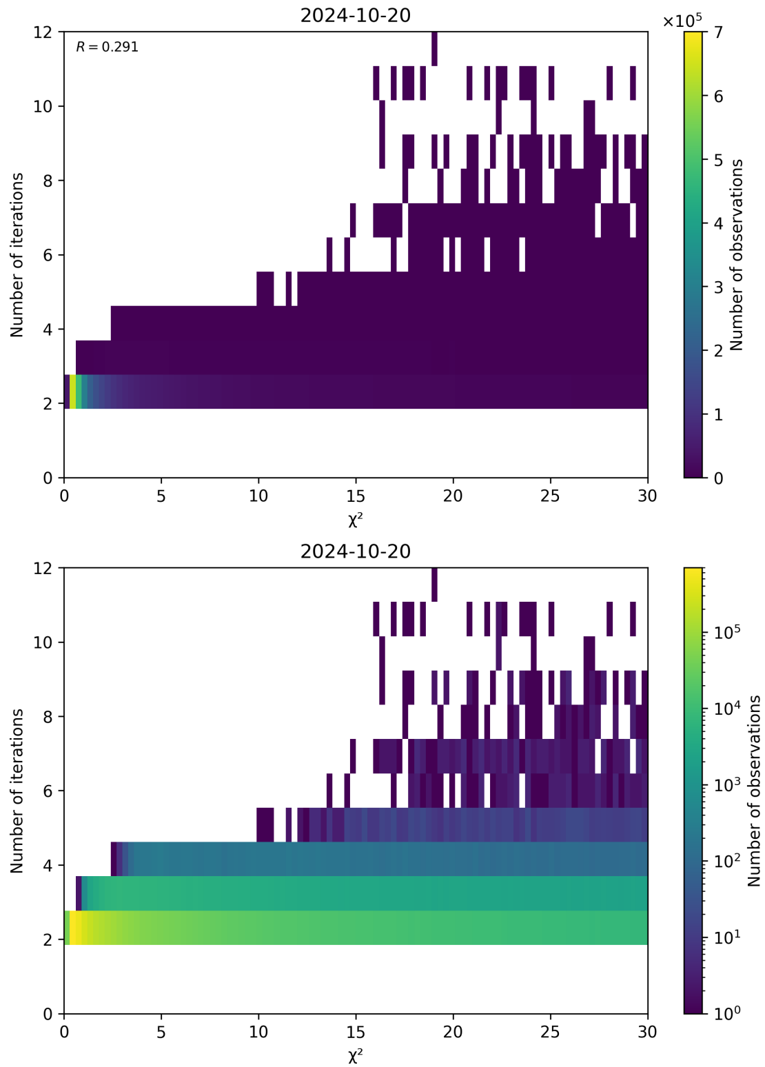
Figure 73: Scatter density plot of “ \chi^2 ” against “Number of iterations” for 2024-10-19 to 2024-10-21.
