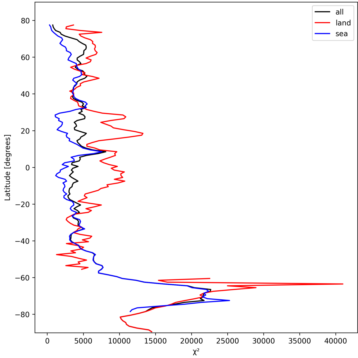
Figure 21: Zonal average of “ \chi^2 ” for 2024-10-19 to 2024-10-21.
