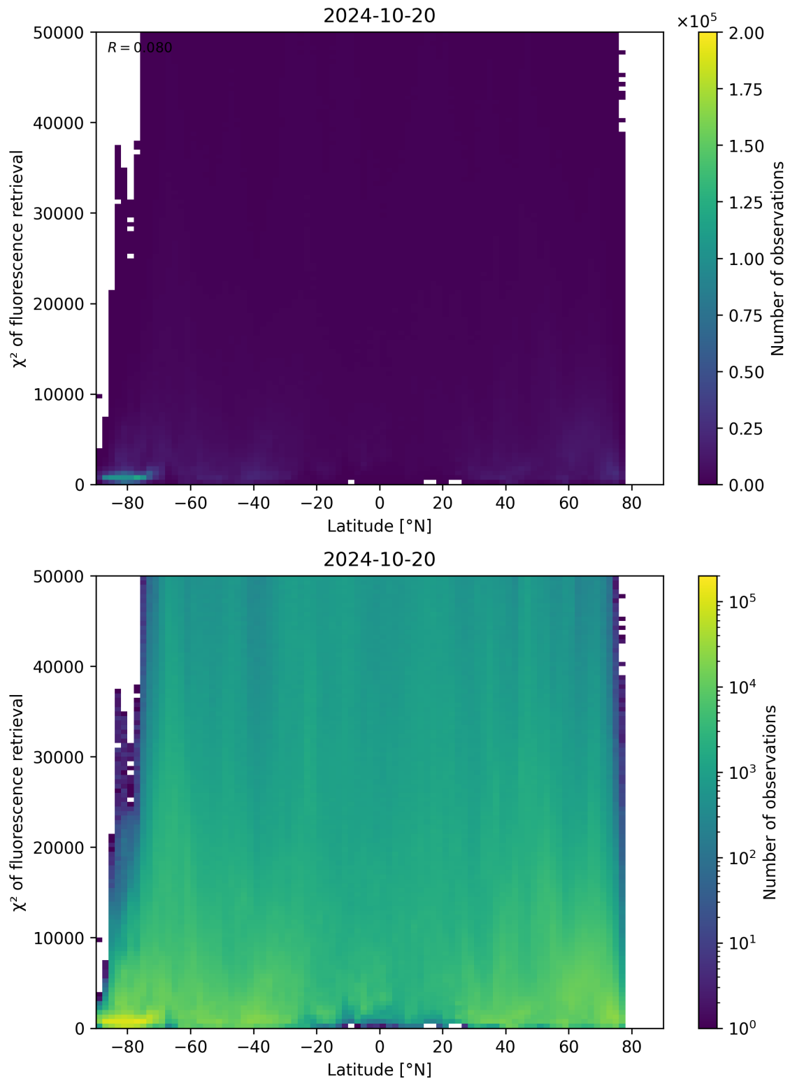
Figure 98: Scatter density plot of “Latitude” against “ \chi^2 of fluorescence retrieval” for 2024-10-19 to 2024-10-21.
