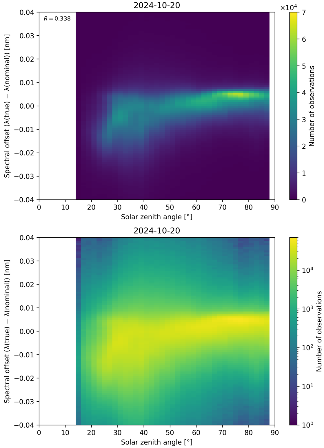
Figure 128: Scatter density plot of “Solar zenith angle” against “Spectral offset ( \lambda_{\text{true}} - \lambda_{\text{nominal}} )” for 2024-10-19 to 2024-10-21.
