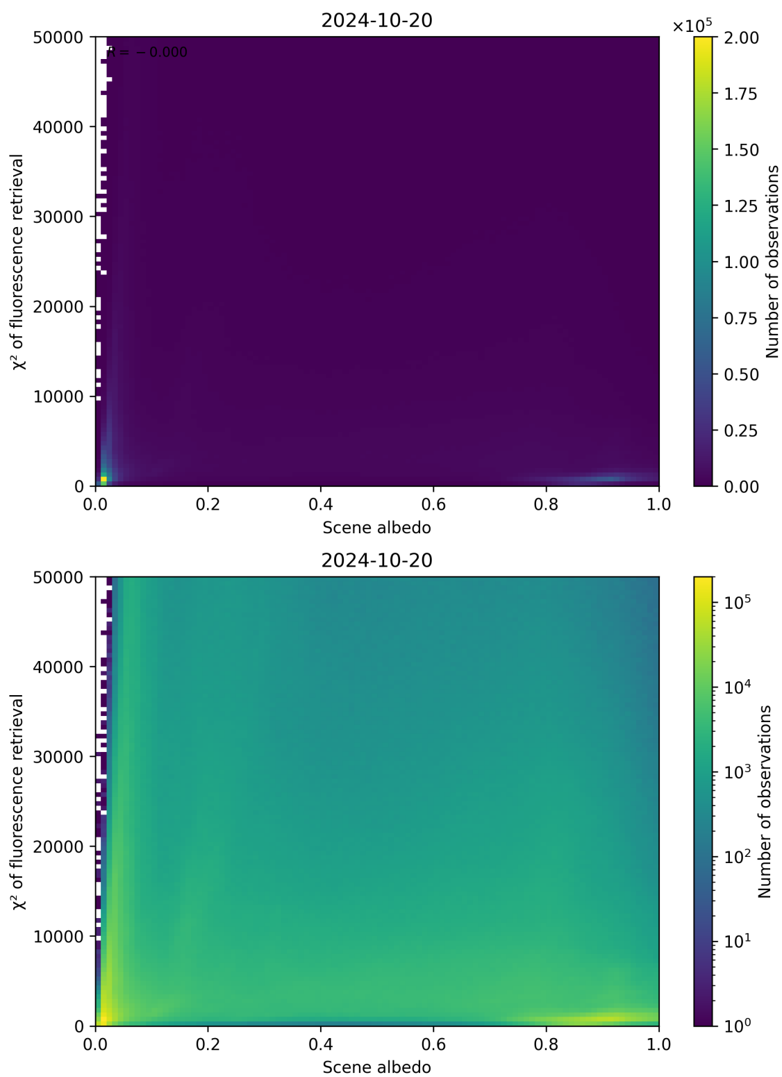
Figure 113: Scatter density plot of “Scene albedo” against “ \chi^2 of fluorescence retrieval” for 2024-10-19 to 2024-10-21.
