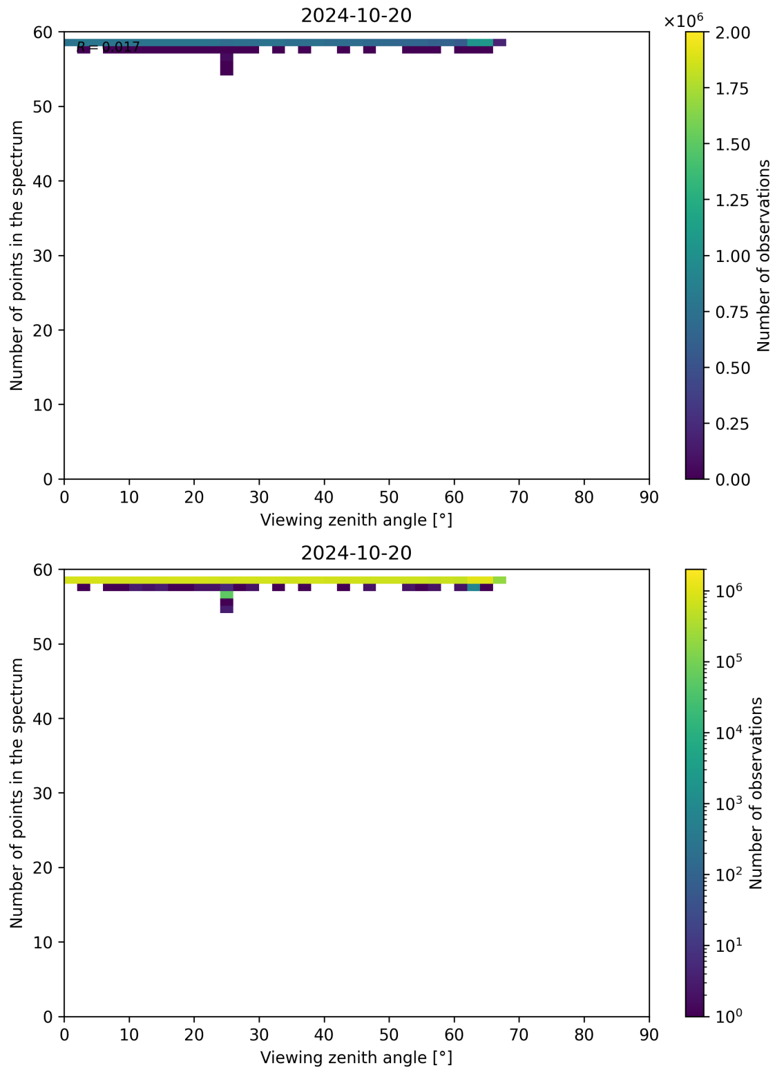
Figure 137: Scatter density plot of “Viewing zenith angle” against “Number of points in the spectrum” for 2024-10-19 to 2024-10-21.
