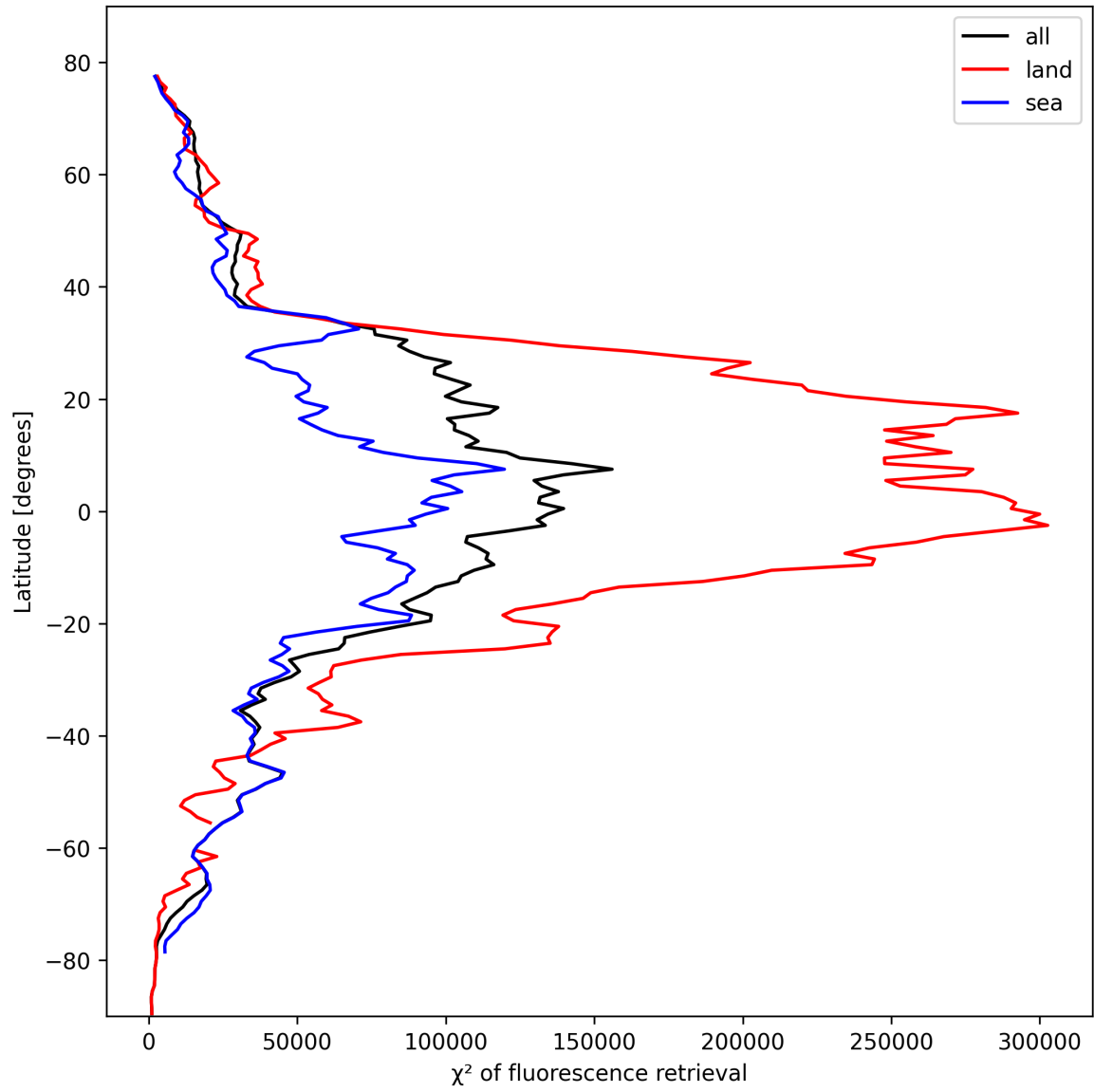
Figure 25: Zonal average of “ \chi^2 of fluorescence retrieval” for 2024-10-19 to 2024-10-21.
