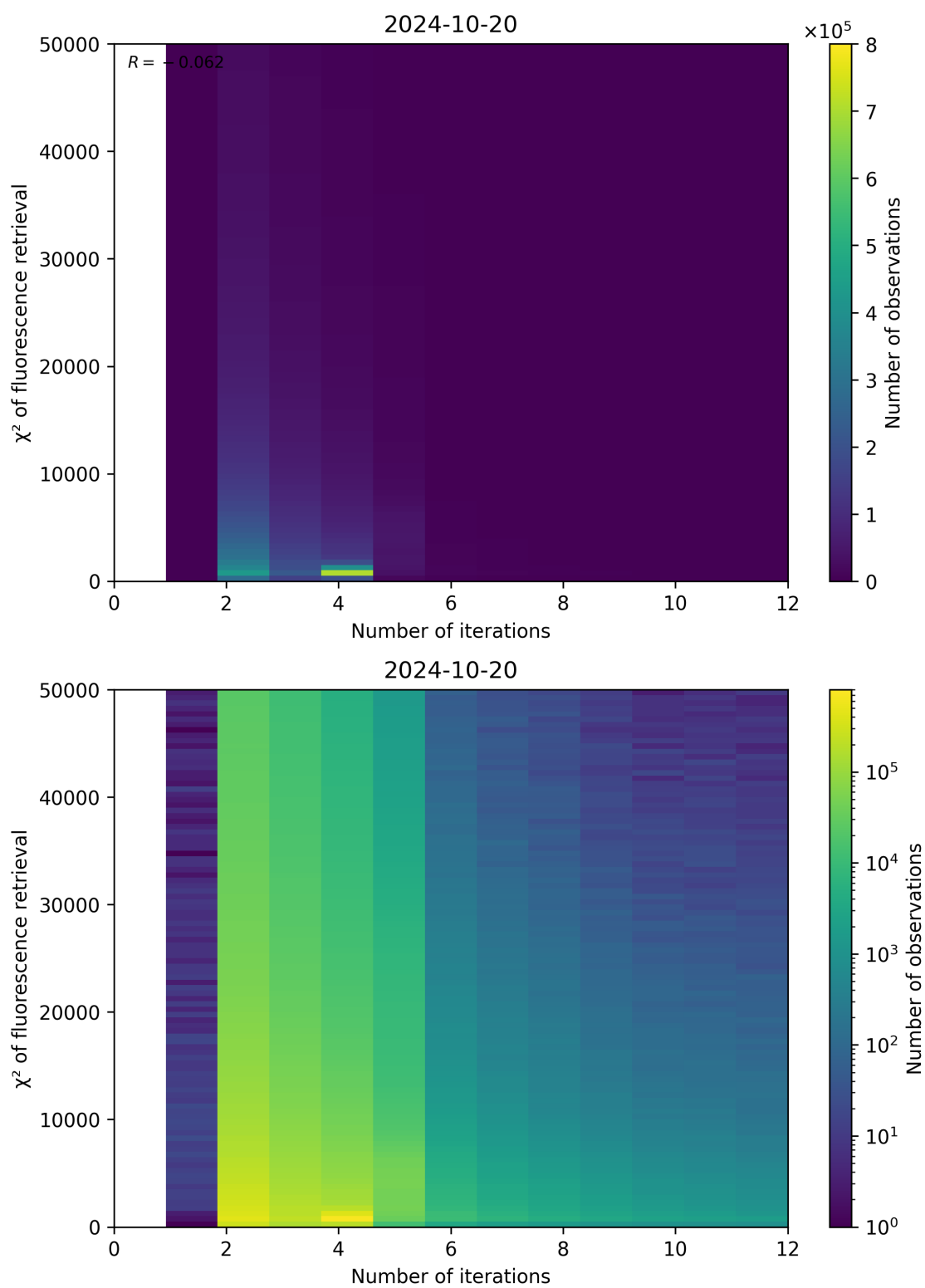
Figure 106: Scatter density plot of “Number of iterations” against “ \chi^2 of fluorescence retrieval” for 2024-10-19 to 2024-10-21.
