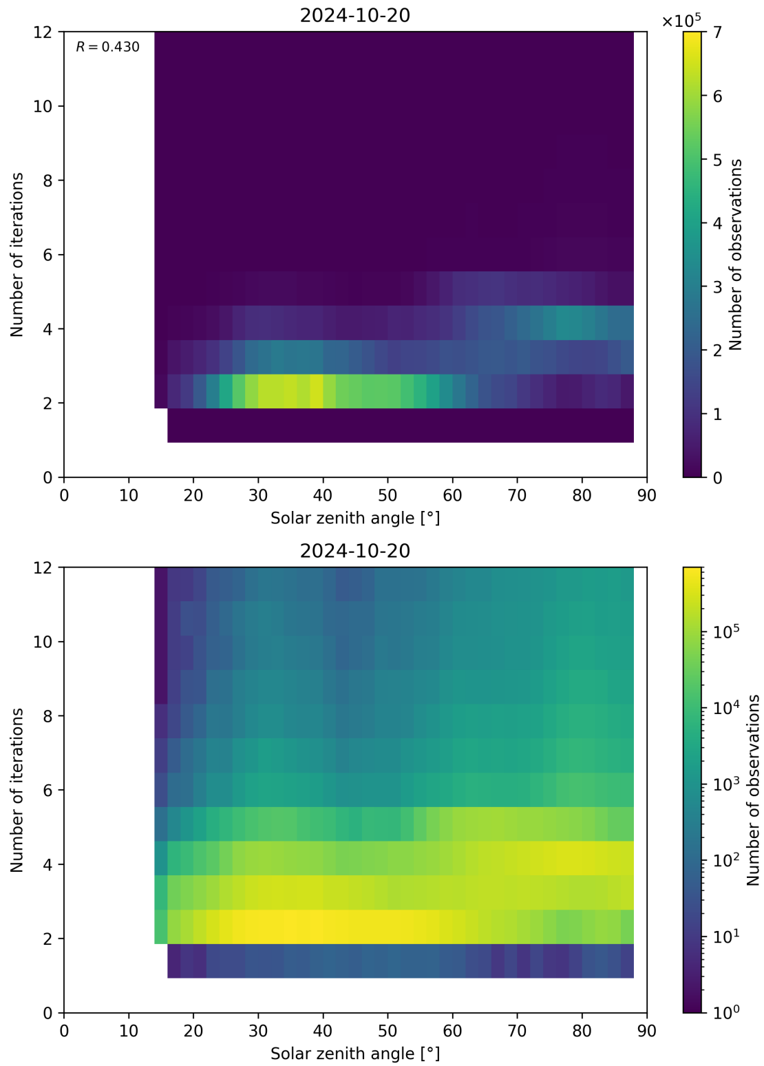
Figure 125: Scatter density plot of “Solar zenith angle” against “Number of iterations” for 2024-10-19 to 2024-10-21.
