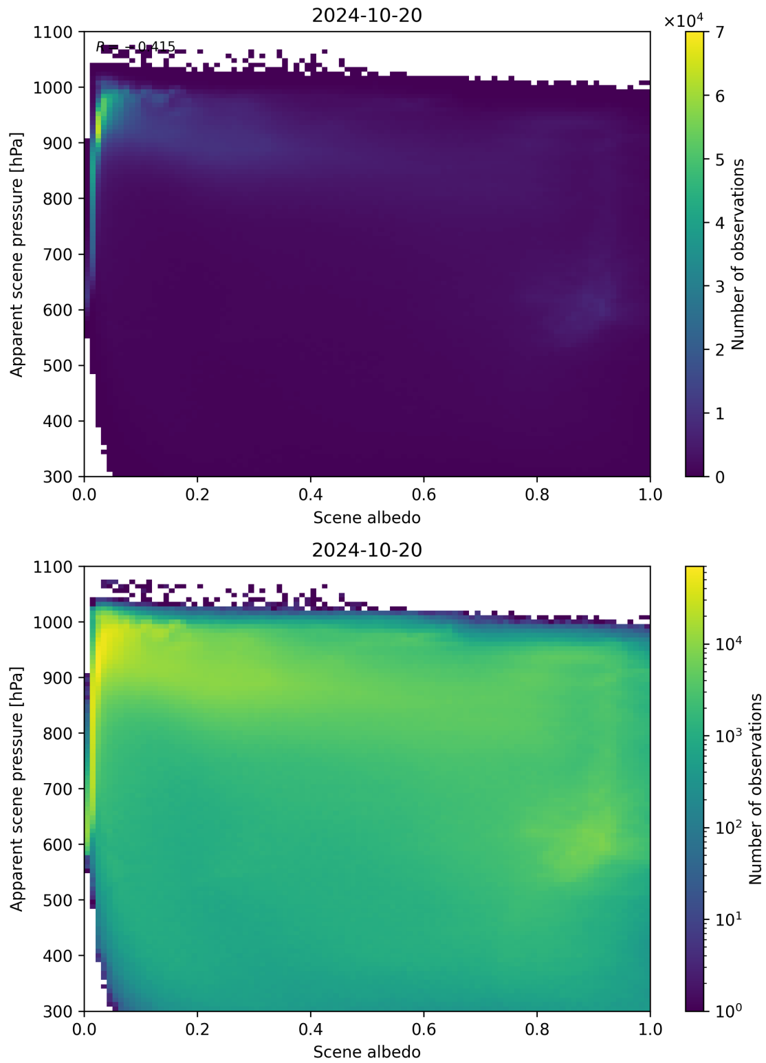
Figure 111: Scatter density plot of “Scene albedo” against “Apparent scene pressure” for 2024-10-19 to 2024-10-21.
