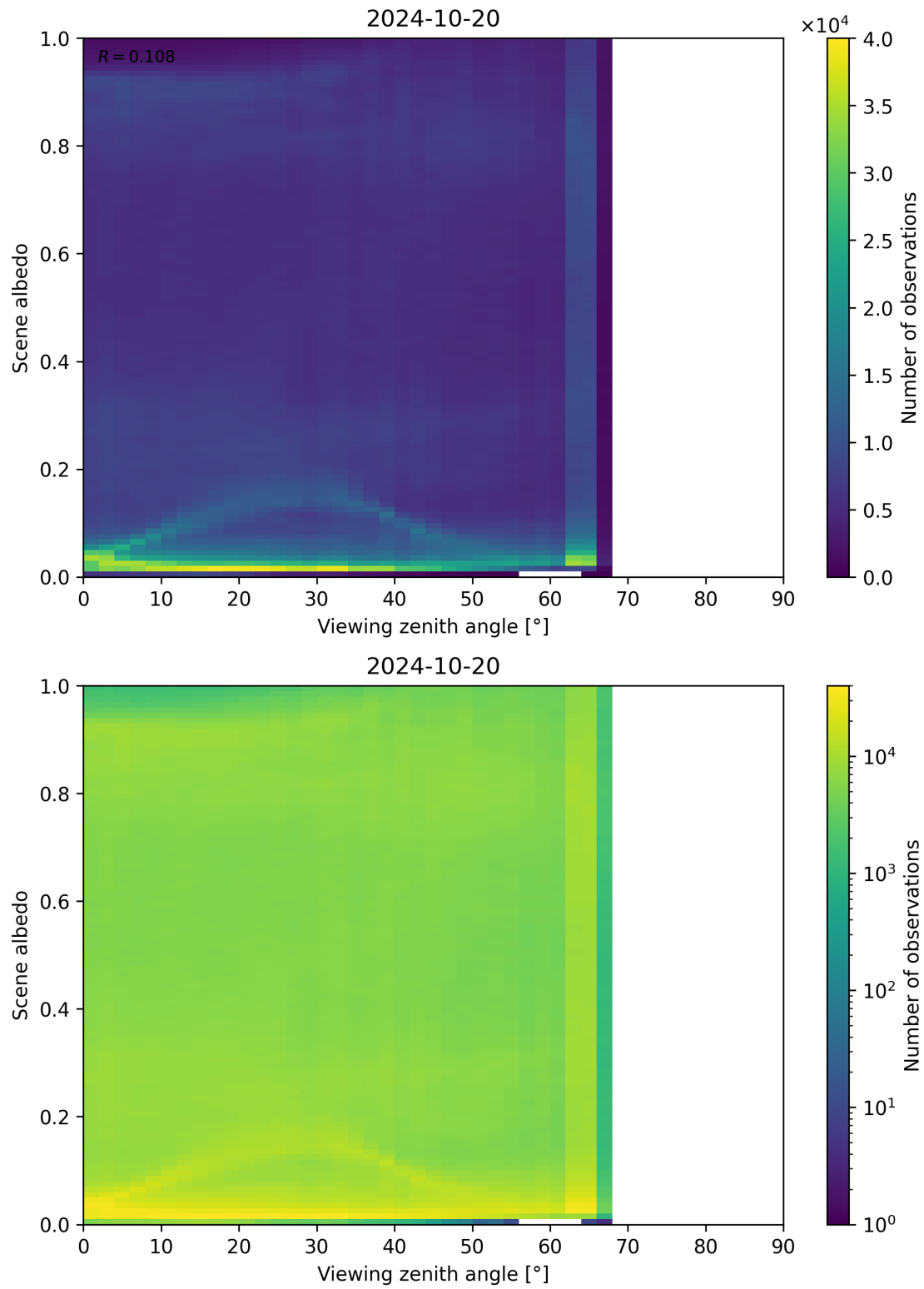
Figure 138: Scatter density plot of “Viewing zenith angle” against “Scene albedo” for 2024-10-19 to 2024-10-21.
