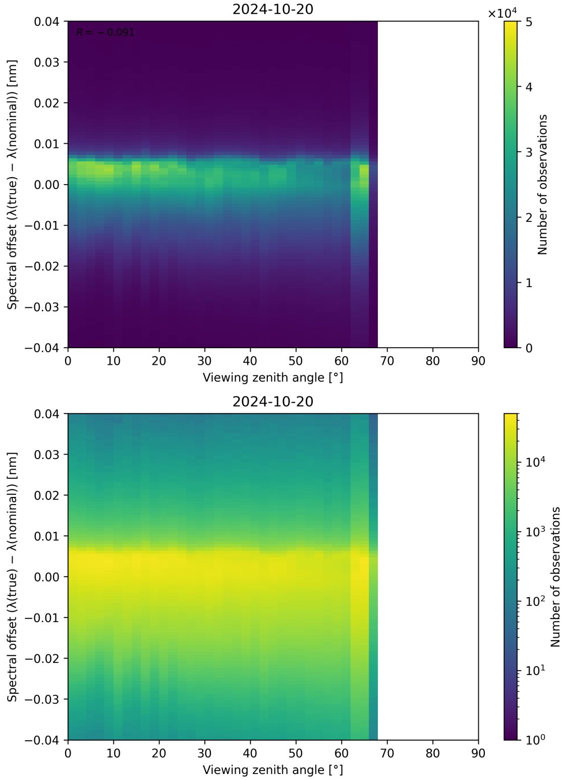
Figure 140: Scatter density plot of “Viewing zenith angle” against “Spectral offset ( \lambda_{\text{true}} - \lambda_{\text{nominal}} )” for 2024-10-19 to 2024-10-21.
