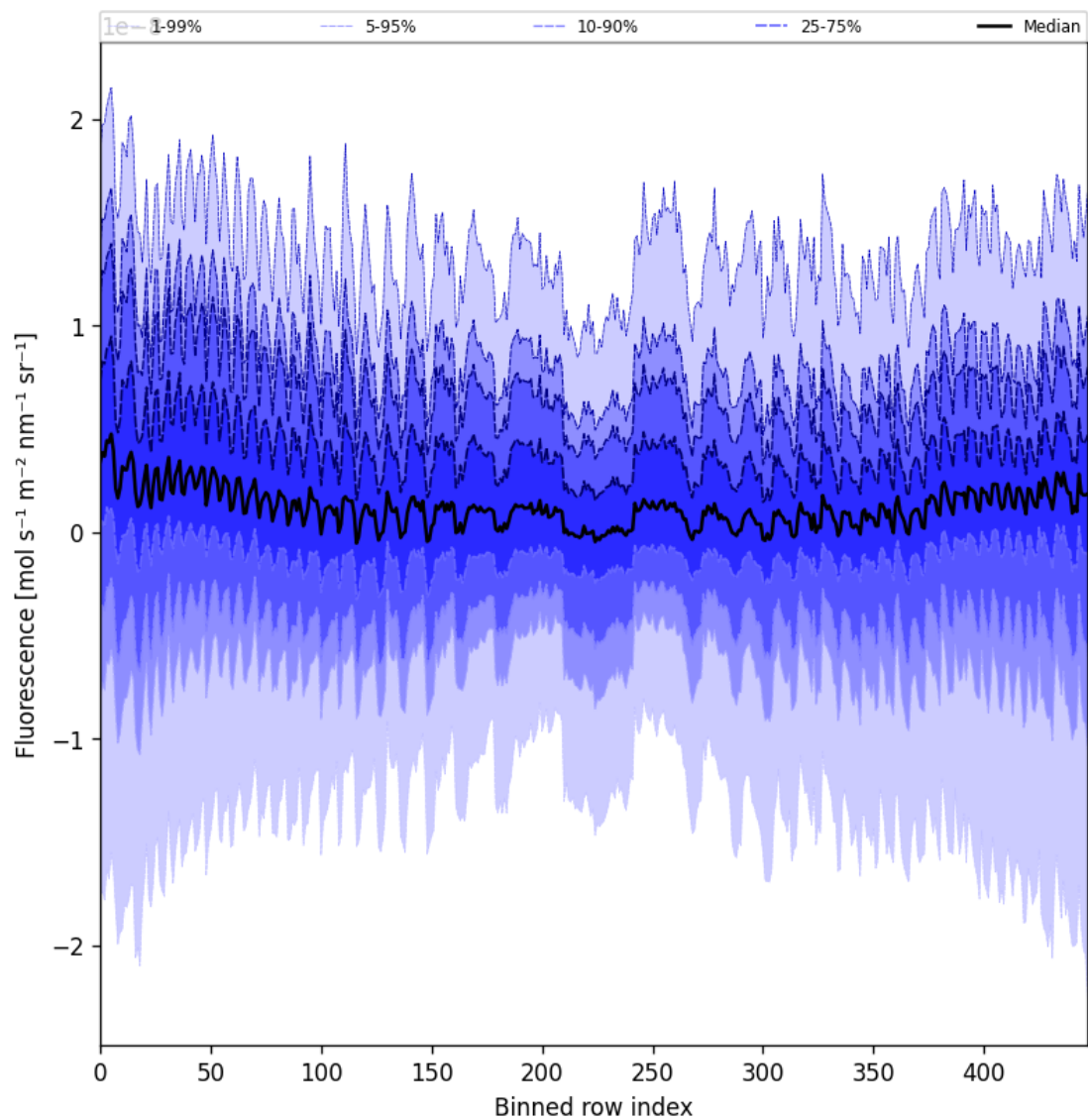
Figure 57: Along track statistics of “Fluorescence” for 2024-10-19 to 2024-10-21
