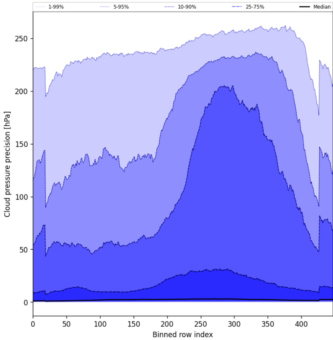
Figure 48: Along track statistics of “Cloud pressure precision” for 2024-10-19 to 2024-10-21
