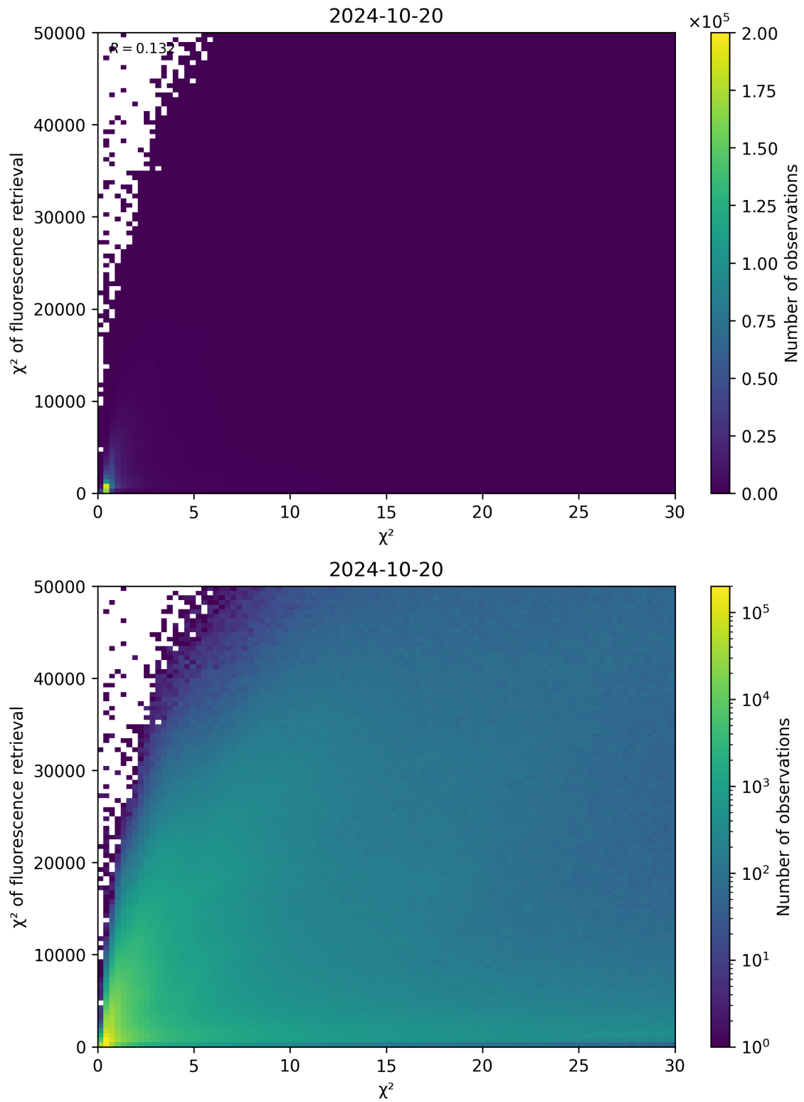
Figure 69: Scatter density plot of “ \chi^2 ” against “ \chi^2 of fluorescence retrieval” for 2024-10-19 to 2024-10-21.
