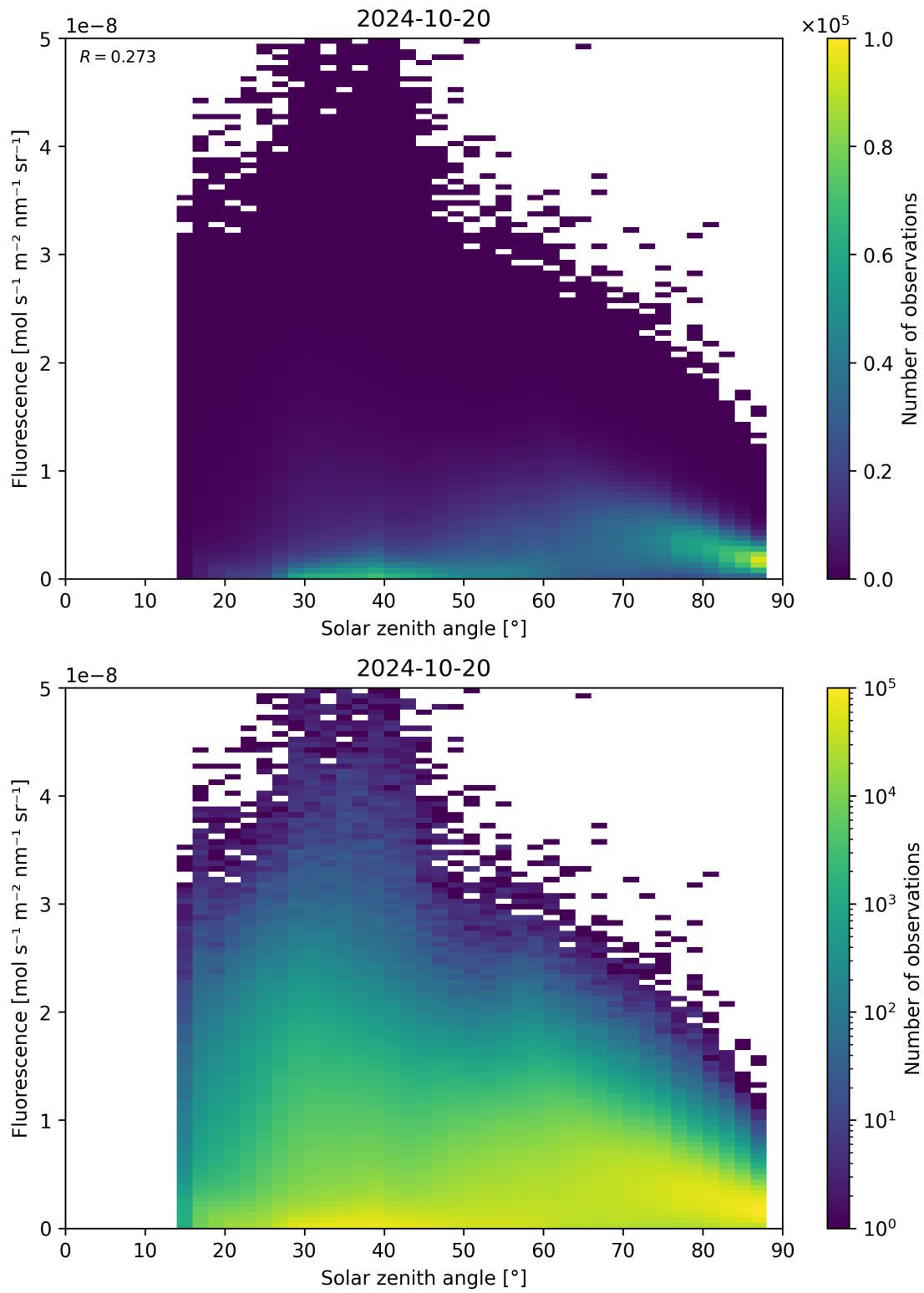
Figure 123: Scatter density plot of “Solar zenith angle” against “Fluorescence” for 2024-10-19 to 2024-10-21.
