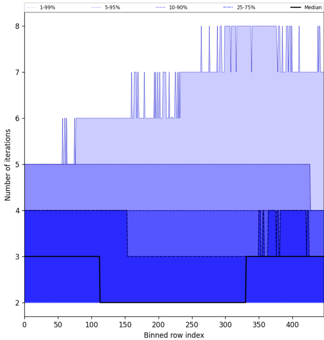
Figure 56: Along track statistics of “Number of iterations” for 2024-10-19 to 2024-10-21
