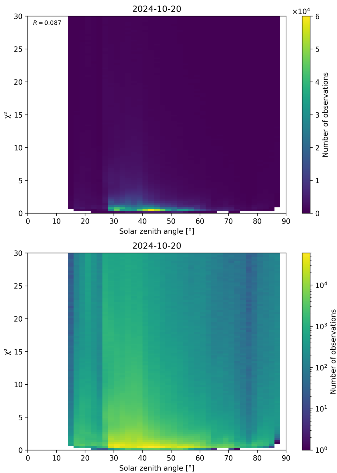
Figure 119: Scatter density plot of “Solar zenith angle” against “ \chi^2 ” for 2024-10-19 to 2024-10-21.
