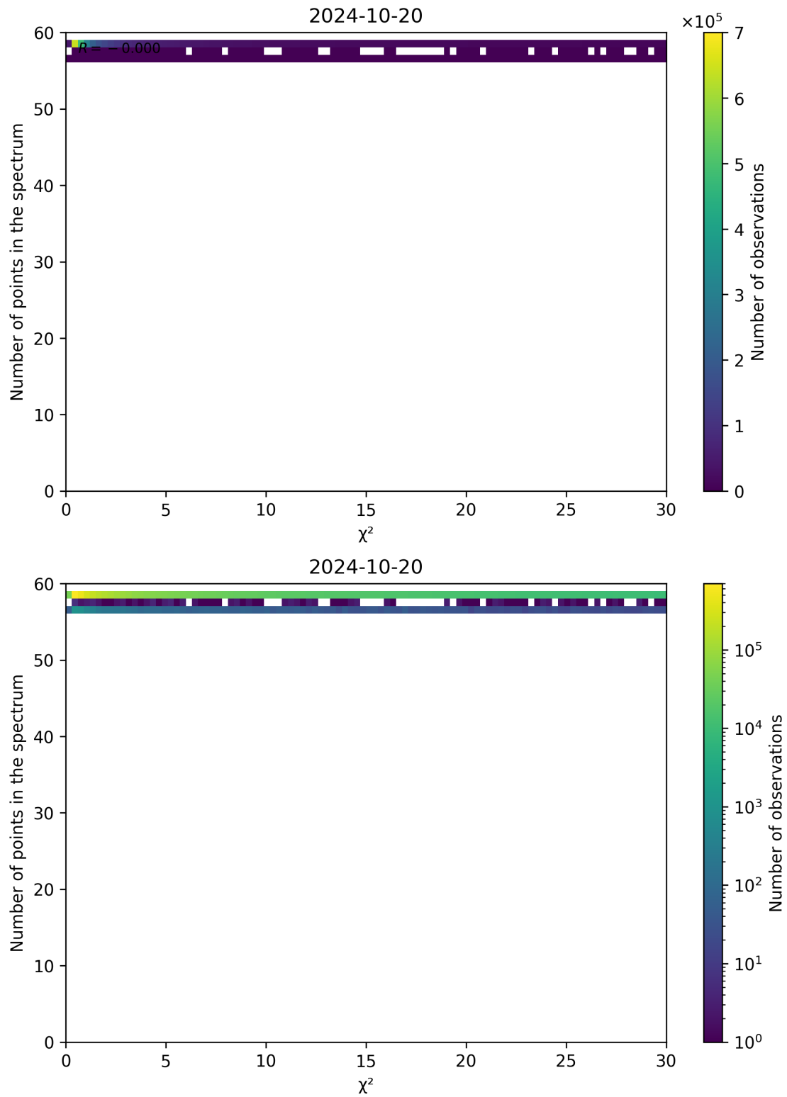
Figure 74: Scatter density plot of " \chi^2 " against "Number of points in the spectrum" for 2024-10-19 to 2024-10-21.
