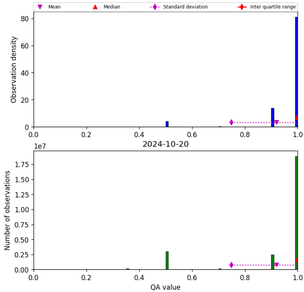
Figure 29: Histogram of “QA value” for 2024-10-19 to 2024-10-21
