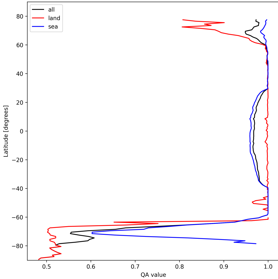
Figure 12: Zonal average of “QA value” for 2024-10-19 to 2024-10-21.
