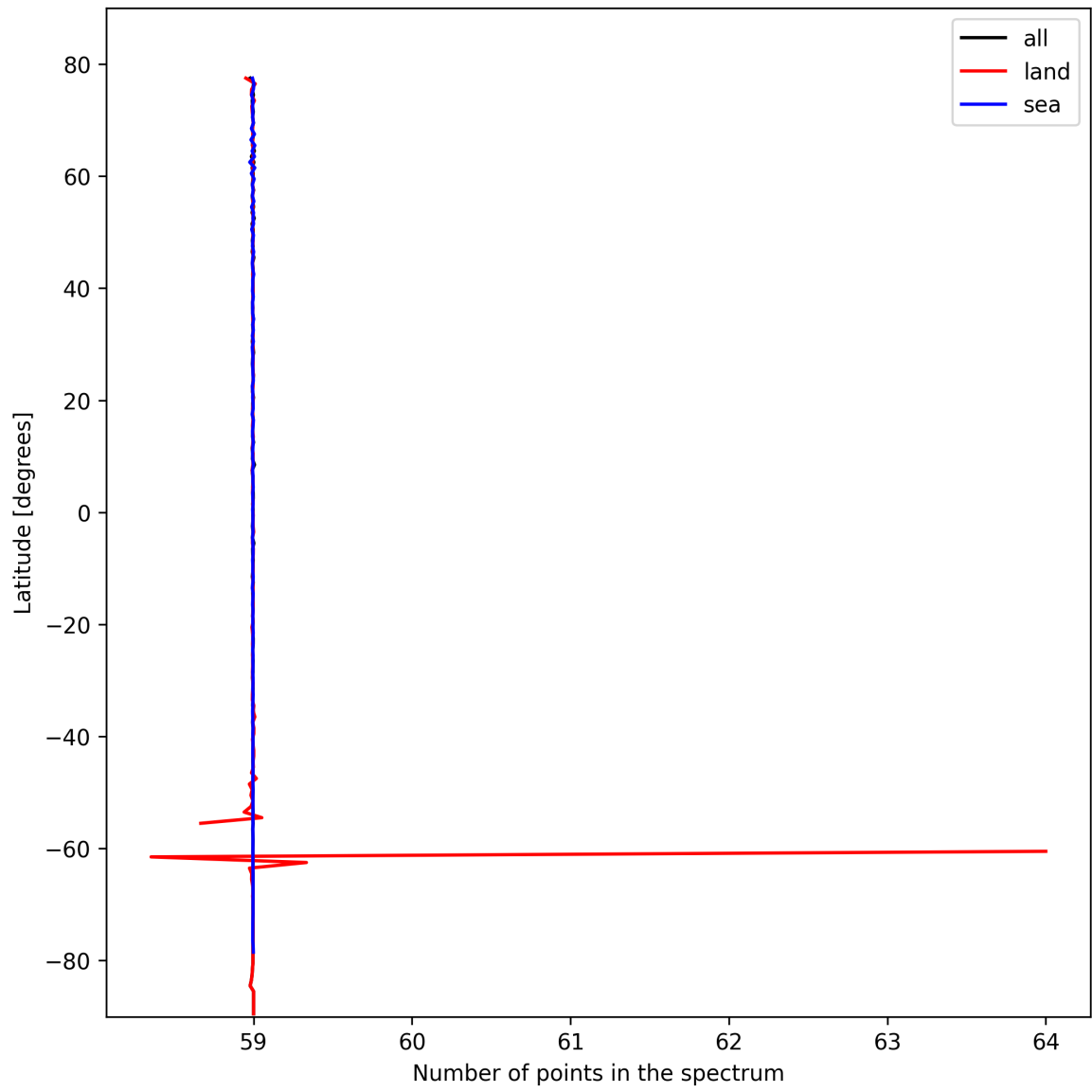
Figure 27: Zonal average of “Number of points in the spectrum” for 2024-10-19 to 2024-10-21.
