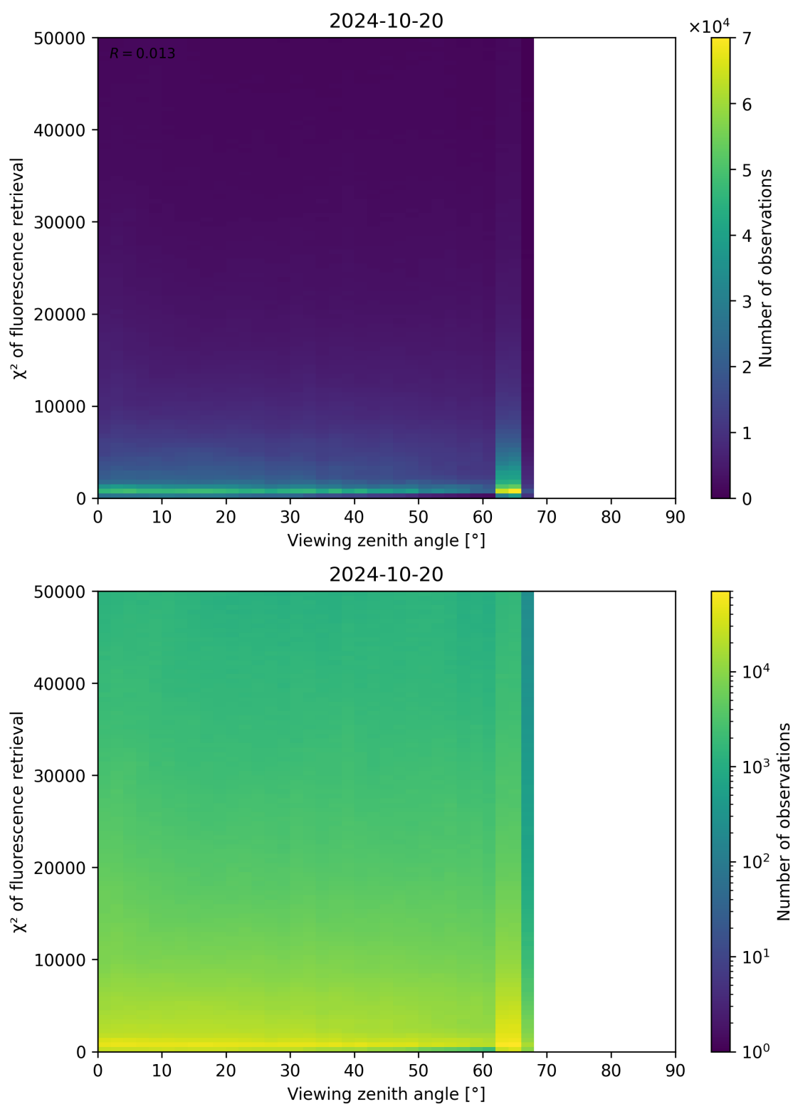
Figure 131: Scatter density plot of “Viewing zenith angle” against “ \chi^2 of fluorescence retrieval” for 2024-10-19 to 2024-10-21.
