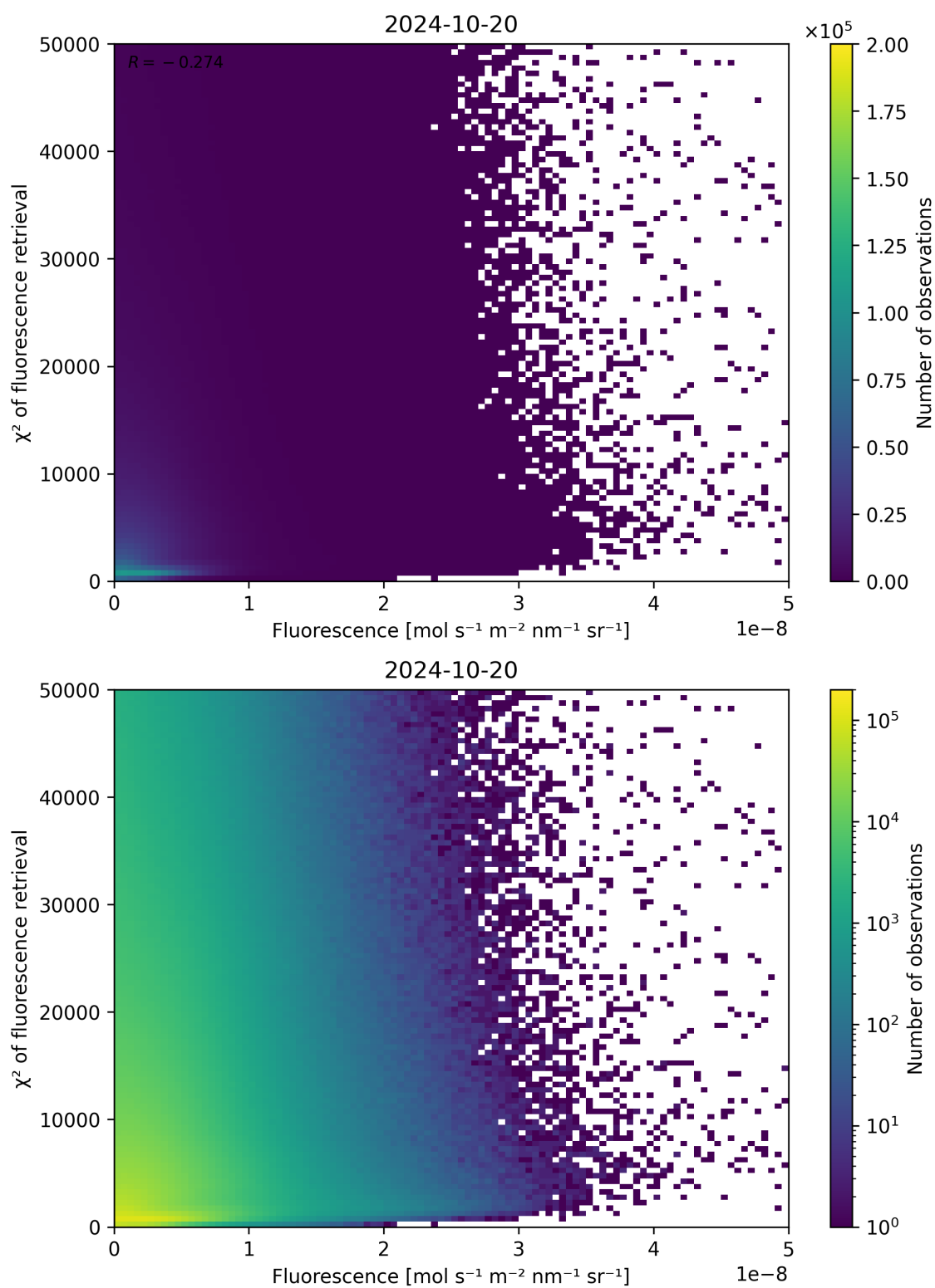
Figure 93: Scatter density plot of “Fluorescence” against “ \chi^2 of fluorescence retrieval” for 2024-10-19 to 2024-10-21.
