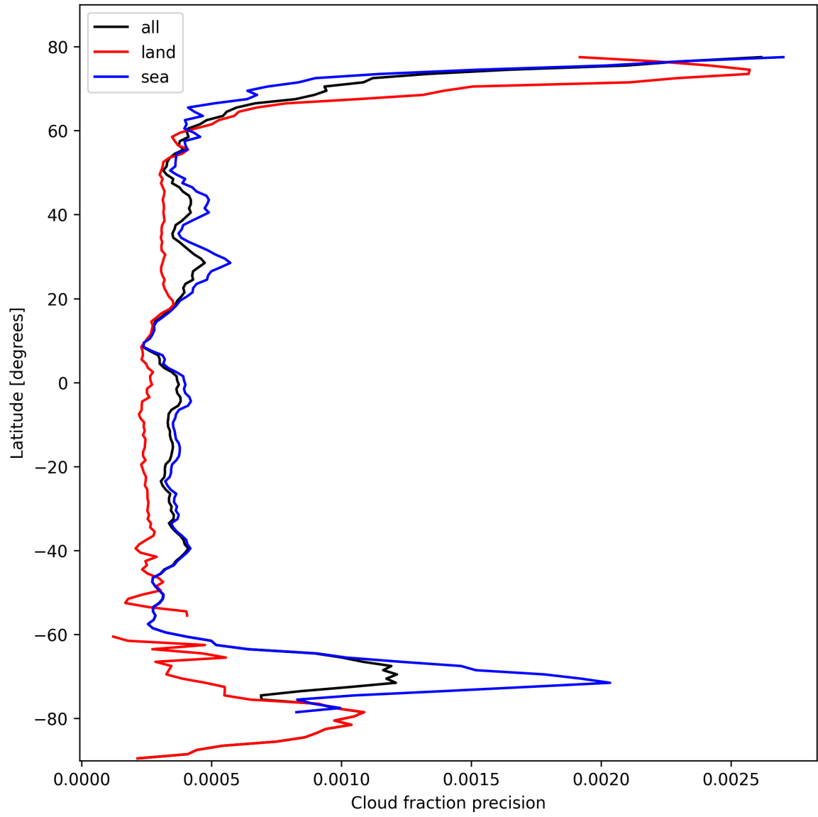
Figure 16: Zonal average of “Cloud fraction precision” for 2024-10-19 to 2024-10-21.
