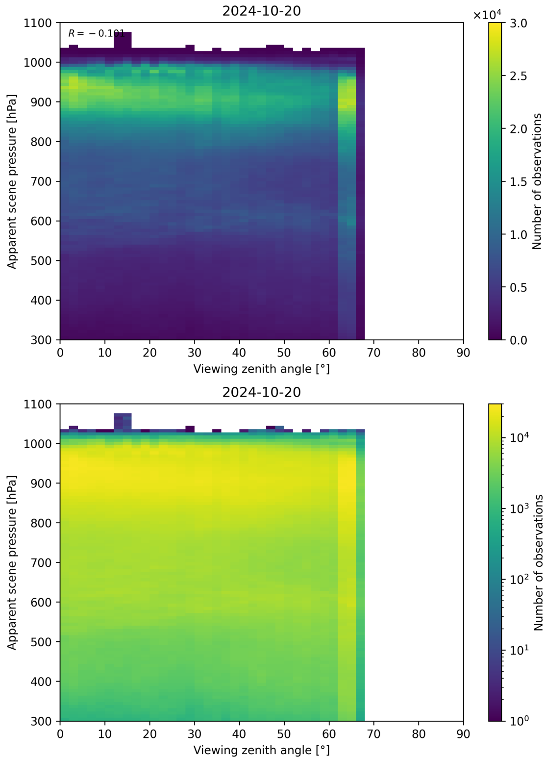
Figure 129: Scatter density plot of “Viewing zenith angle” against “Apparent scene pressure” for 2024-10-19 to 2024-10-21.
