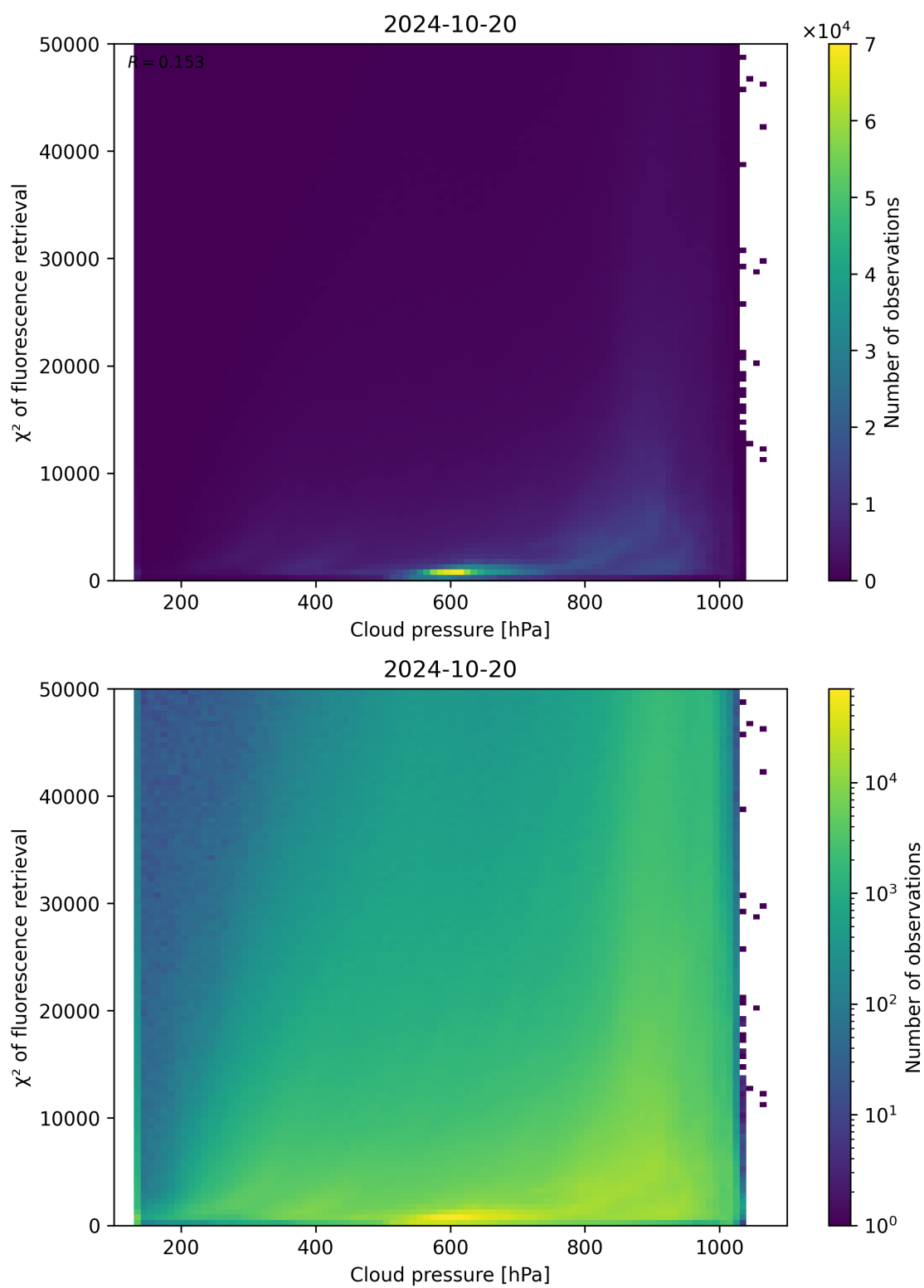
Figure 86: Scatter density plot of “Cloud pressure” against “ \chi^2 of fluorescence retrieval” for 2024-10-19 to 2024-10-21.
