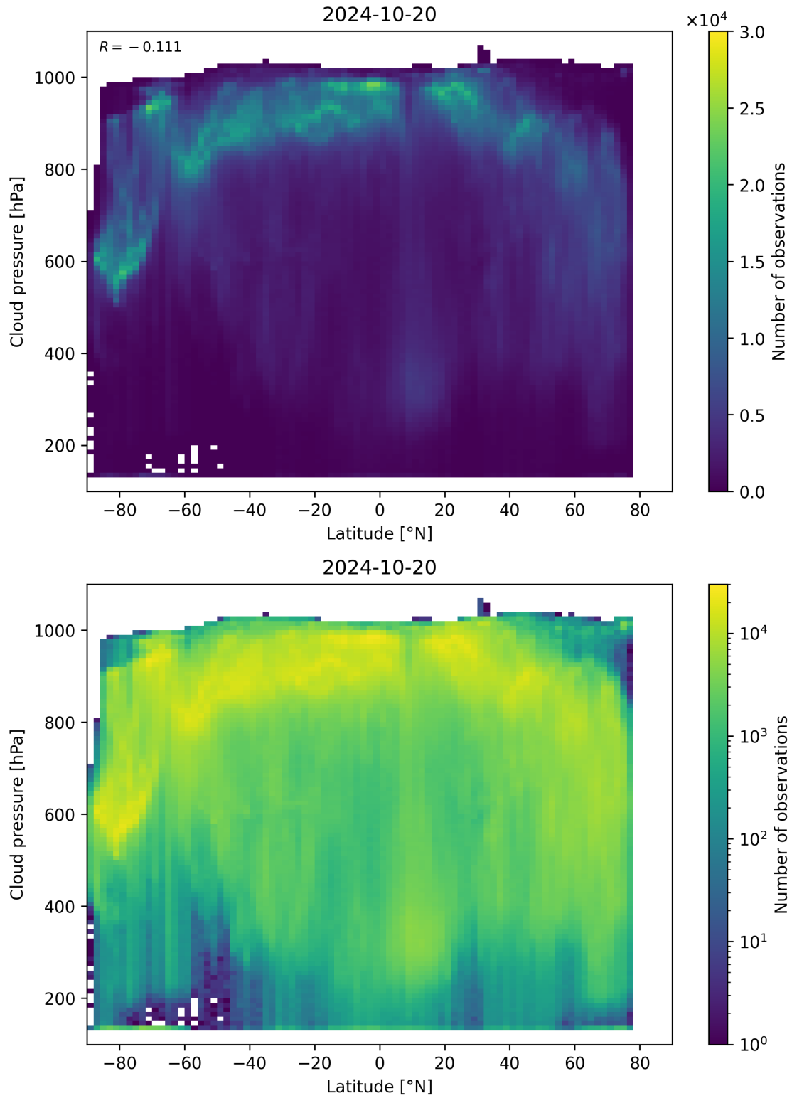
Figure 100: Scatter density plot of “Latitude” against “Cloud pressure” for 2024-10-19 to 2024-10-21.
