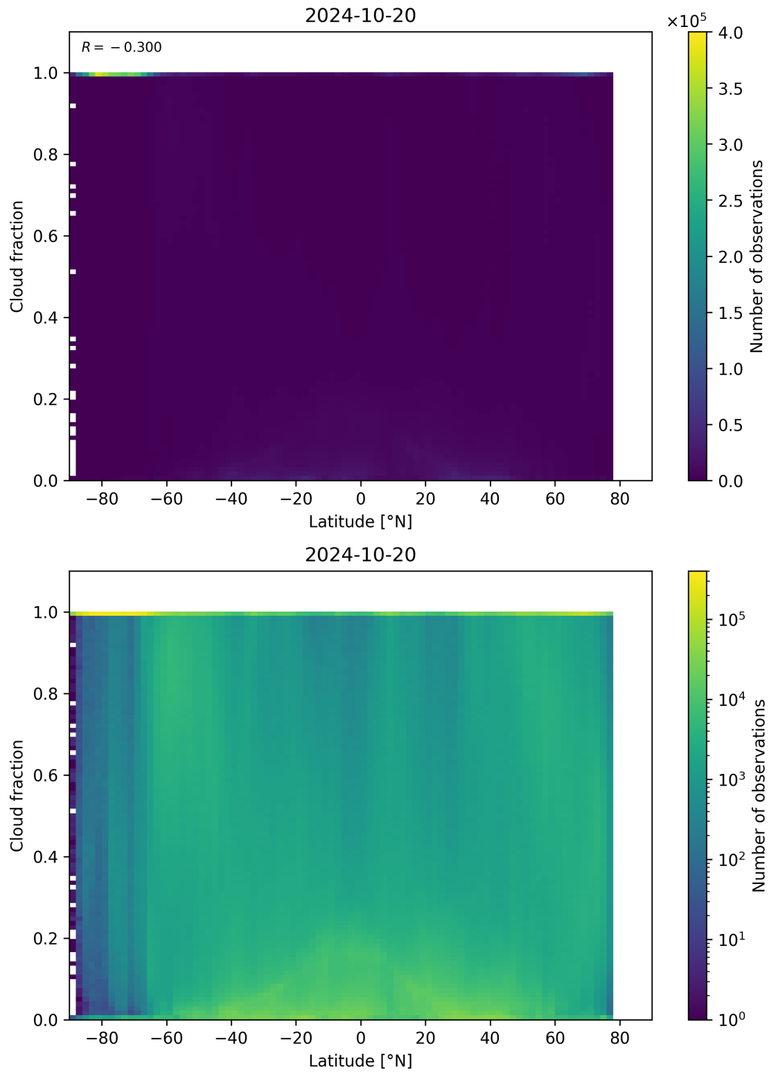
Figure 99: Scatter density plot of “Latitude” against “Cloud fraction” for 2024-10-19 to 2024-10-21.
