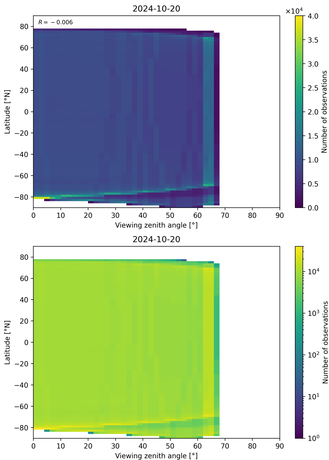
Figure 135: Scatter density plot of “Viewing zenith angle” against “Latitude” for 2024-10-19 to 2024-10-21.
