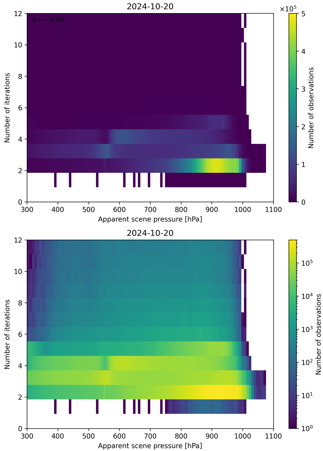
Figure 66: Scatter density plot of “Apparent scene pressure” against “Number of iterations” for 2024-10-19 to 2024-10-21.
