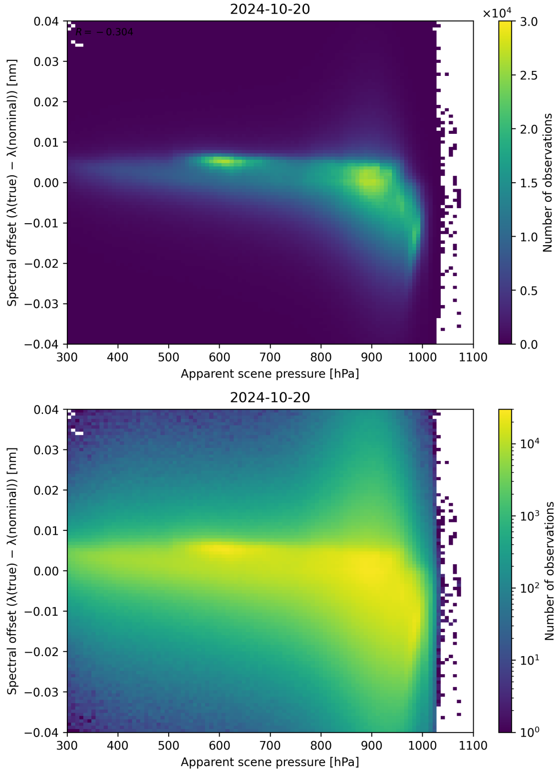
Figure 68: Scatter density plot of “Apparent scene pressure” against “Spectral offset ( \lambda_{\text{true}} - \lambda_{\text{nominal}} )” for 2024-10-19 to 2024-10-21.
