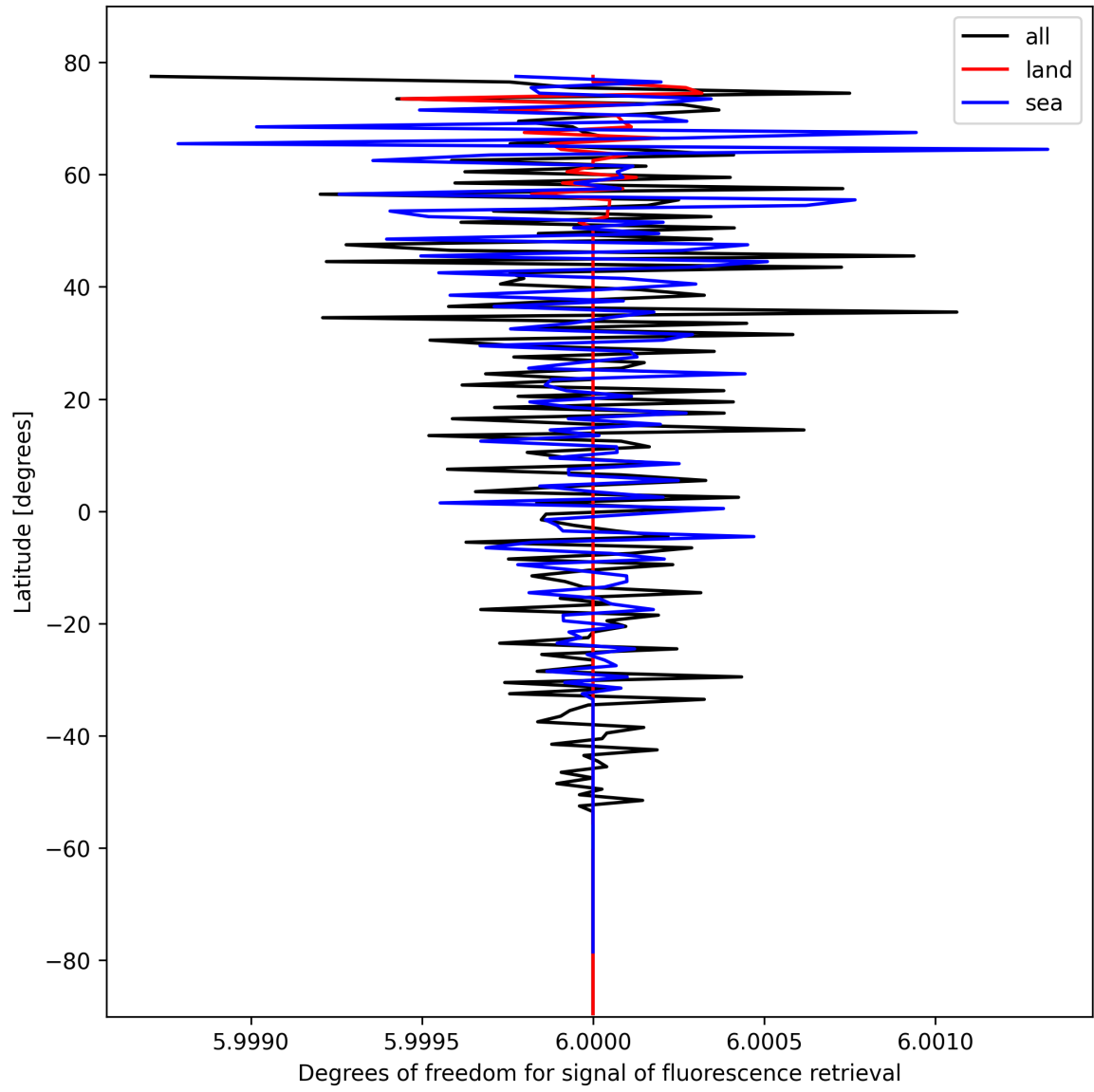
Figure 26: Zonal average of “Degrees of freedom for signal of fluorescence retrieval” for 2024-10-19 to 2024-10-21.
