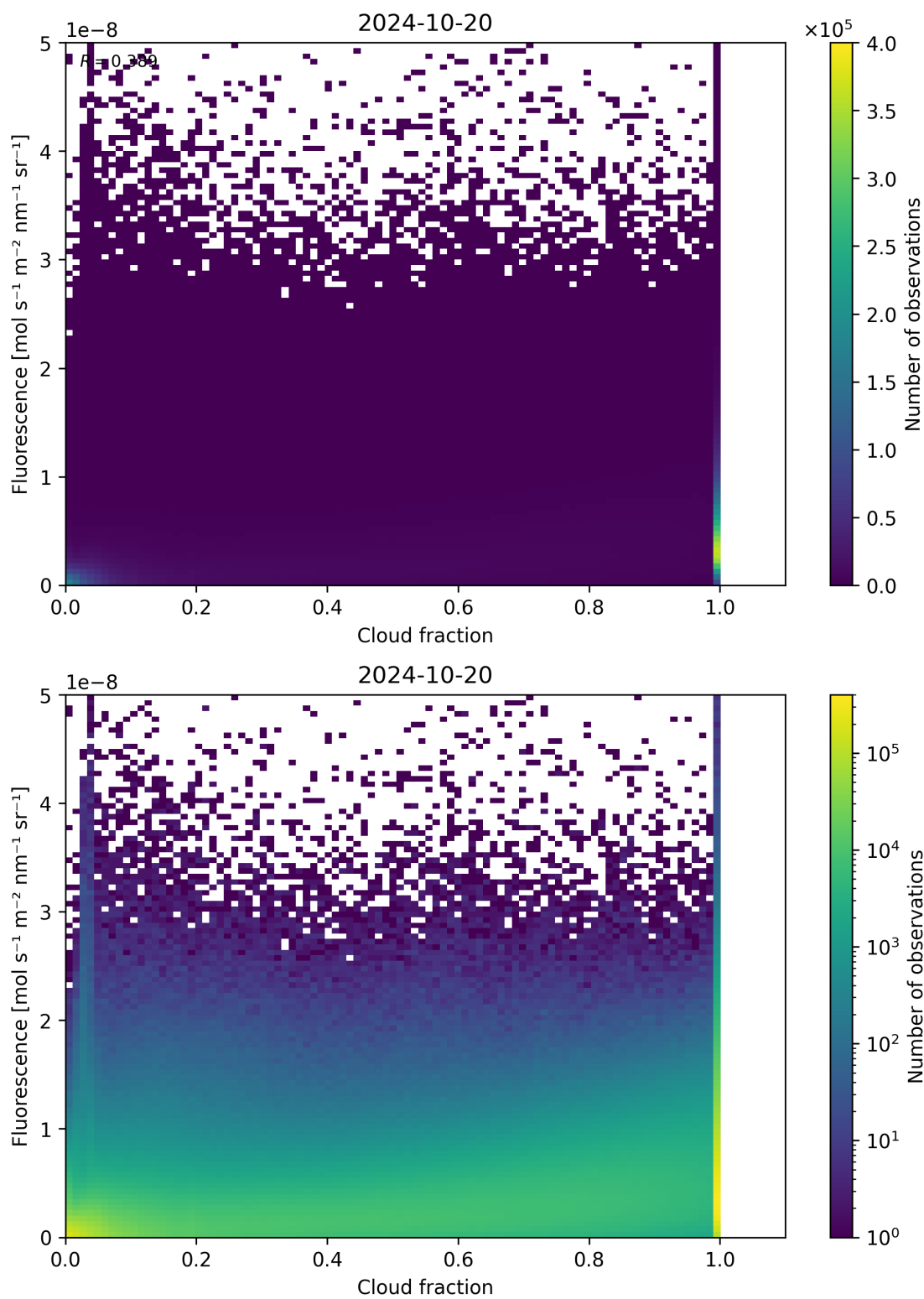
Figure 79: Scatter density plot of “Cloud fraction” against “Fluorescence” for 2024-10-19 to 2024-10-21.
