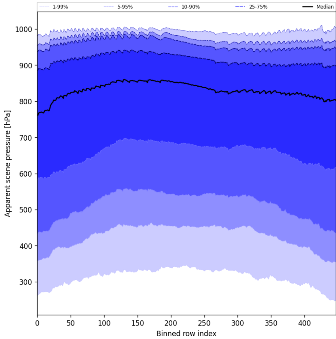
Figure 53: Along track statistics of “Apparent scene pressure” for 2024-10-19 to 2024-10-21
