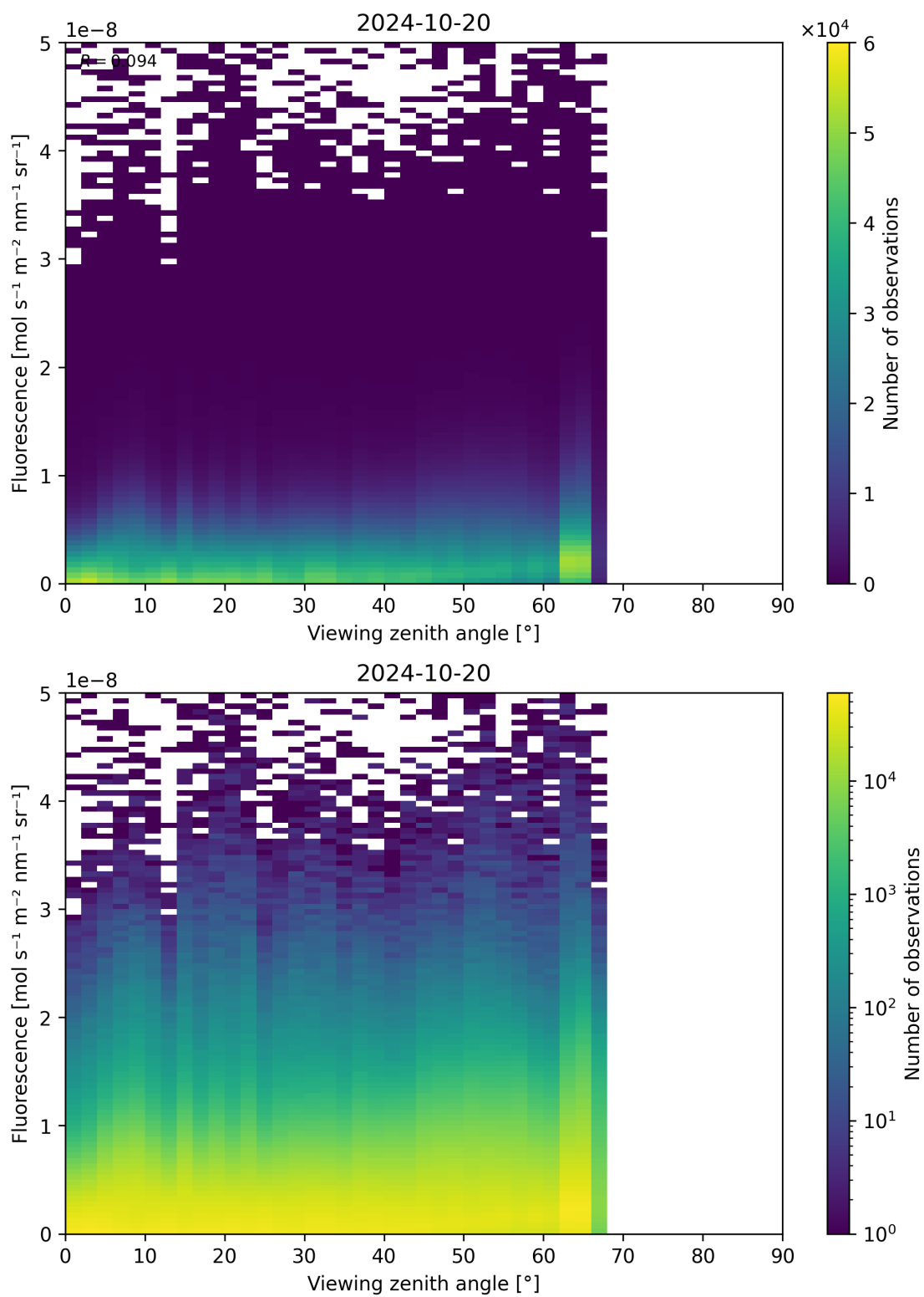
Figure 134: Scatter density plot of “Viewing zenith angle” against “Fluorescence” for 2024-10-19 to 2024-10-21.
