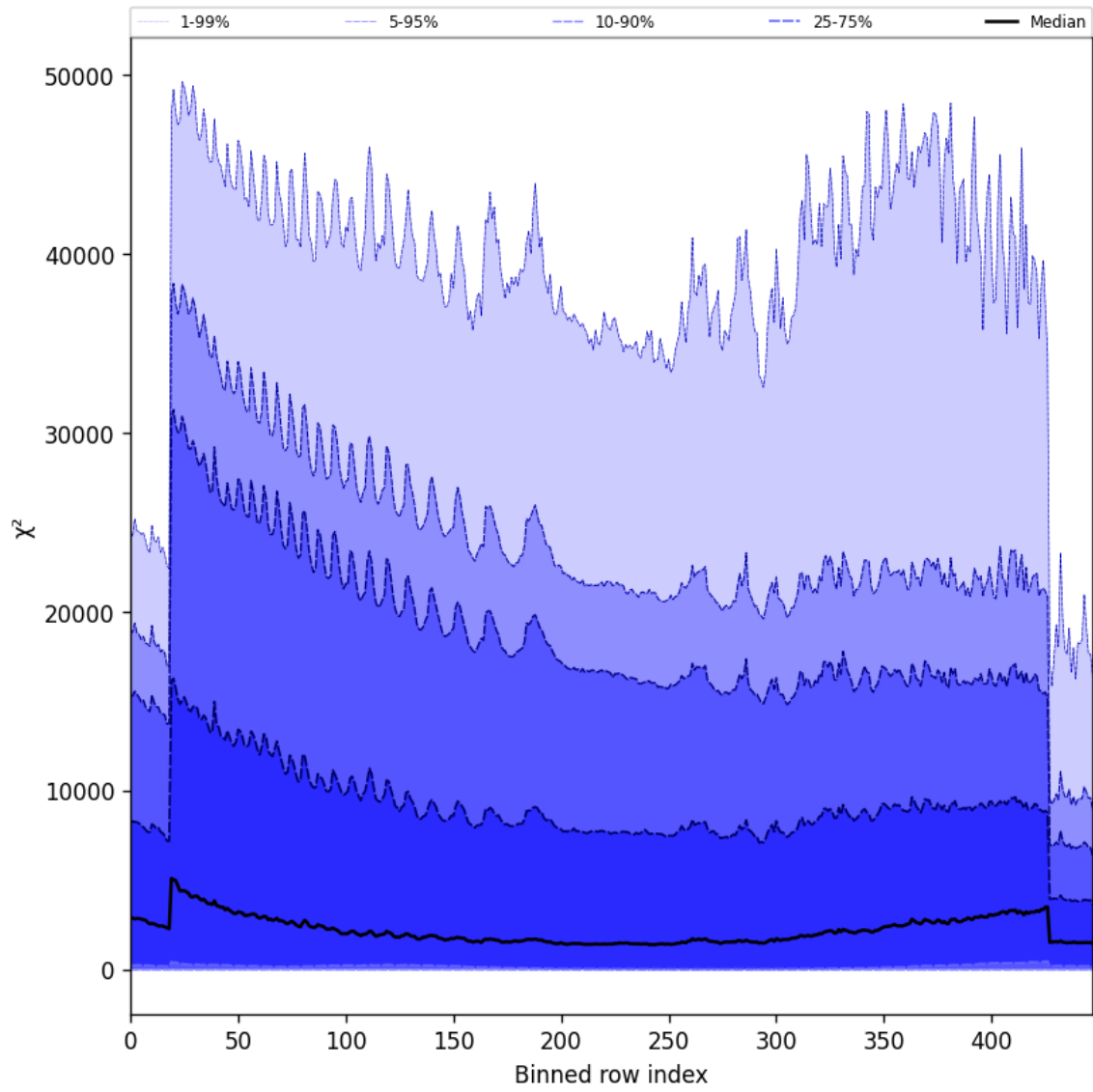
Figure 55: Along track statistics of “ \chi^2 ” for 2024-10-19 to 2024-10-21
