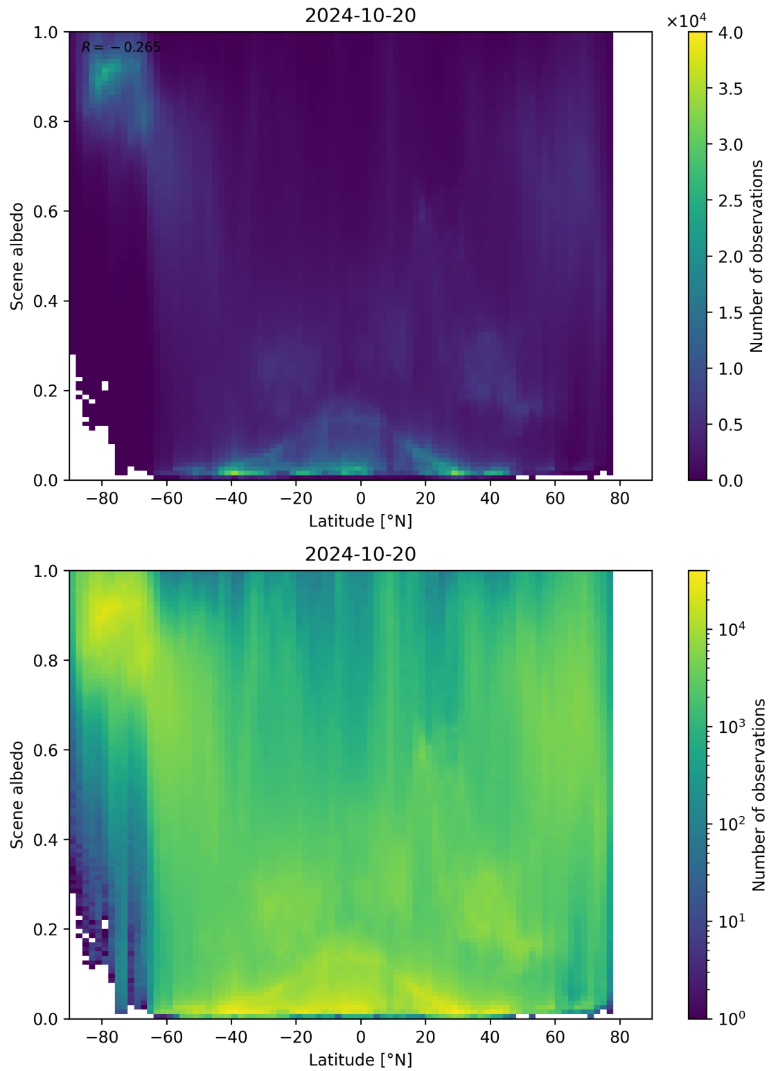
Figure 104: Scatter density plot of “Latitude” against “Scene albedo” for 2024-10-19 to 2024-10-21.
