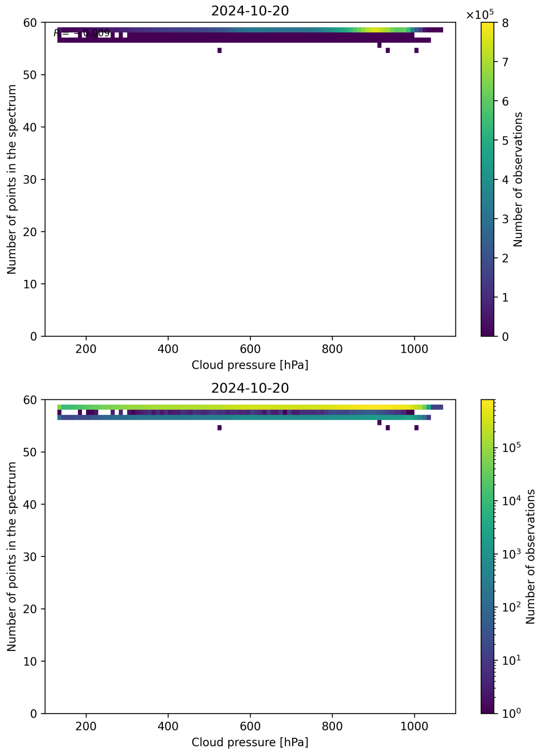
Figure 90: Scatter density plot of “Cloud pressure” against “Number of points in the spectrum” for 2024-10-19 to 2024-10-21.
