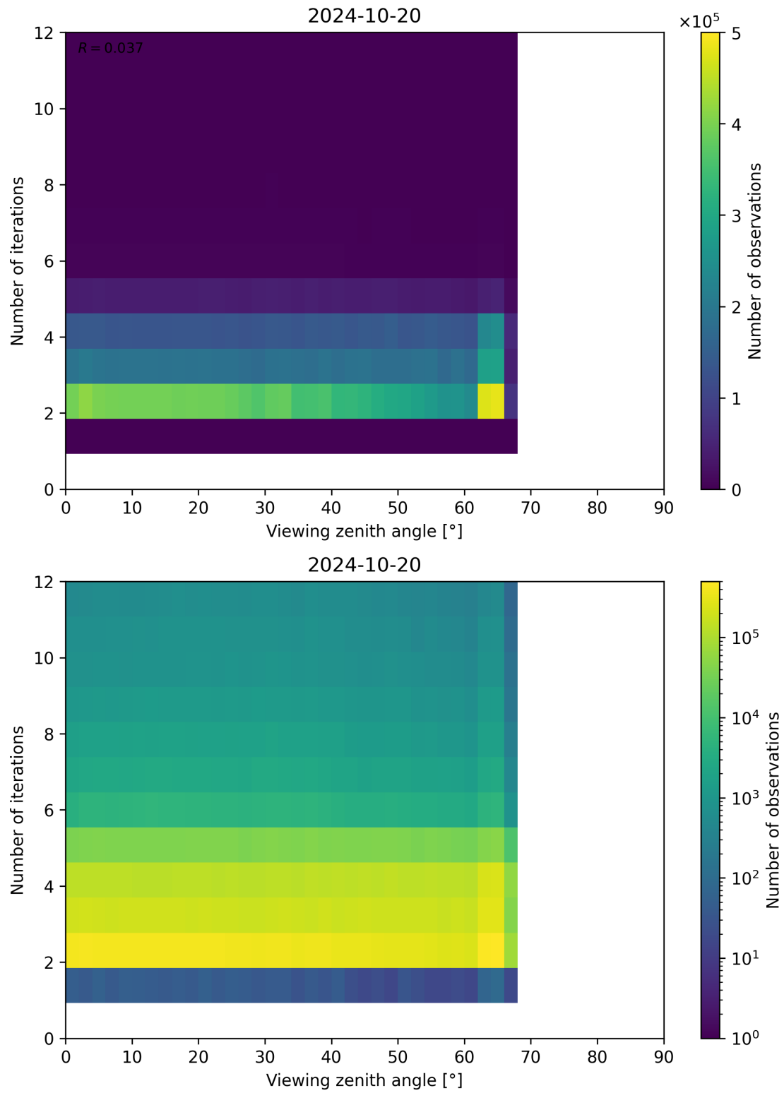
Figure 136: Scatter density plot of “Viewing zenith angle” against “Number of iterations” for 2024-10-19 to 2024-10-21.
