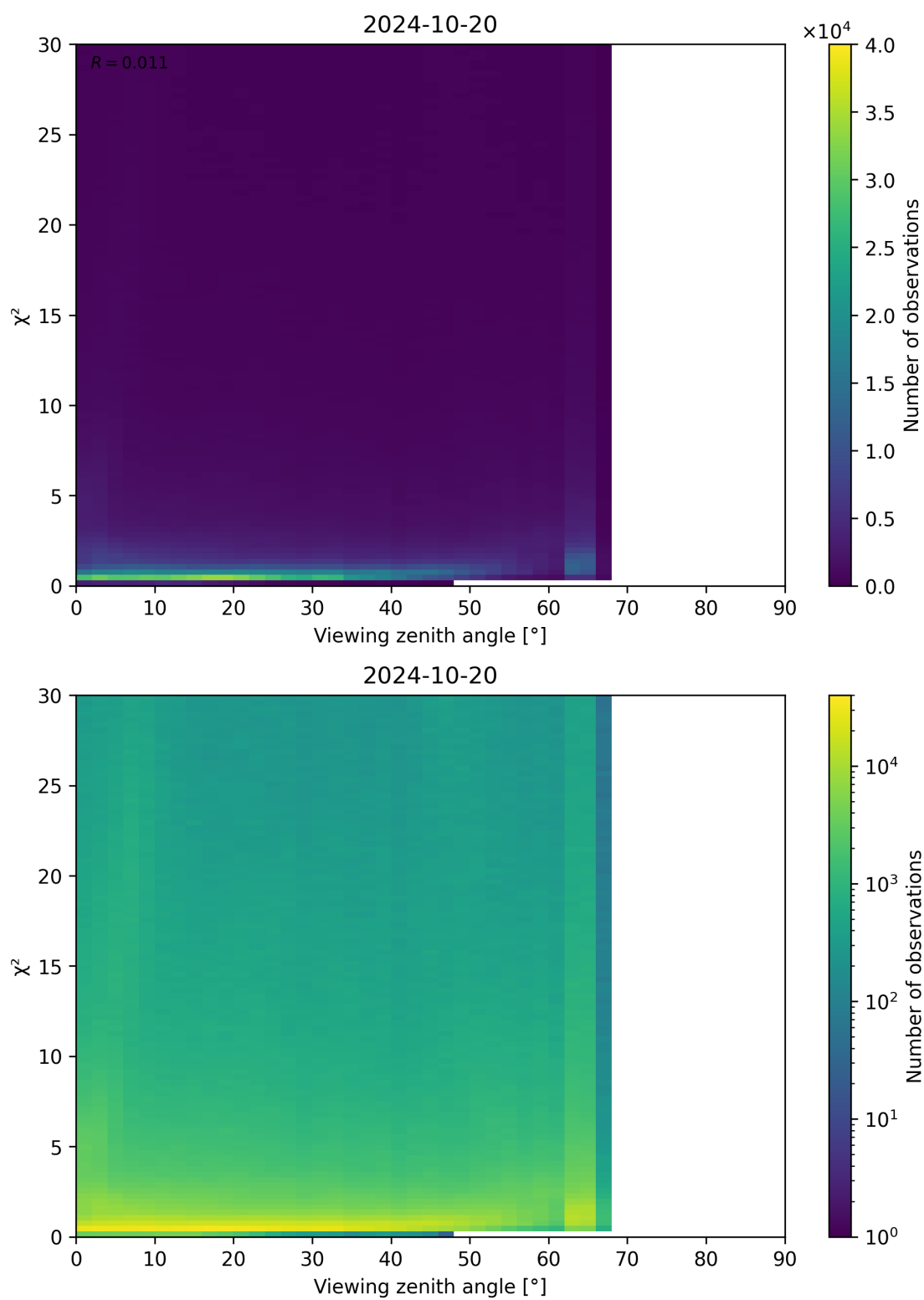
Figure 130: Scatter density plot of “Viewing zenith angle” against “ \chi^2 ” for 2024-10-19 to 2024-10-21.
