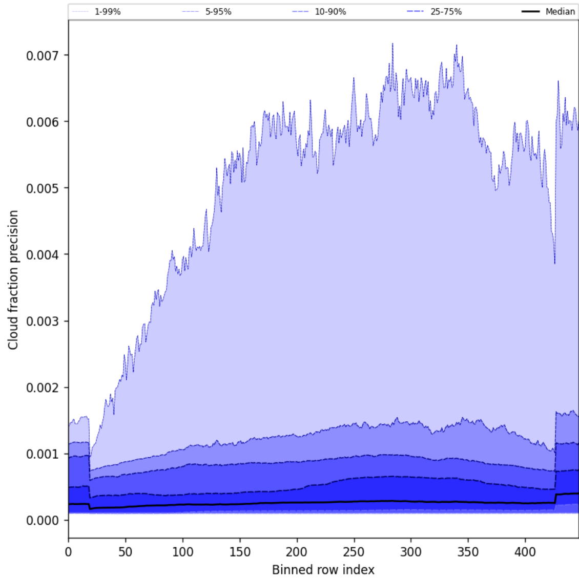
Figure 50: Along track statistics of “Cloud fraction precision” for 2024-10-19 to 2024-10-21
