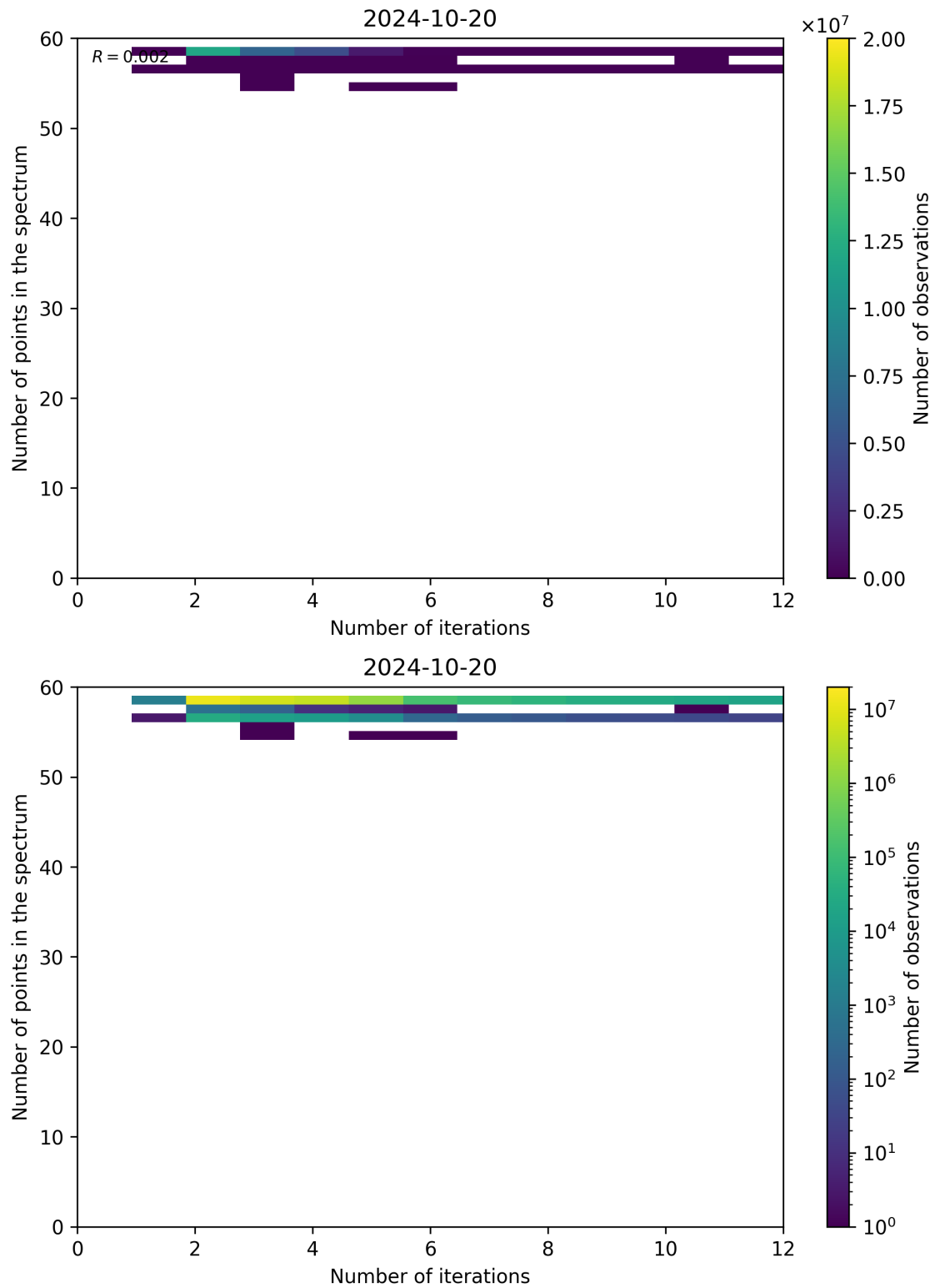
Figure 108: Scatter density plot of “Number of iterations” against “Number of points in the spectrum” for 2024-10-19 to 2024-10-21.
