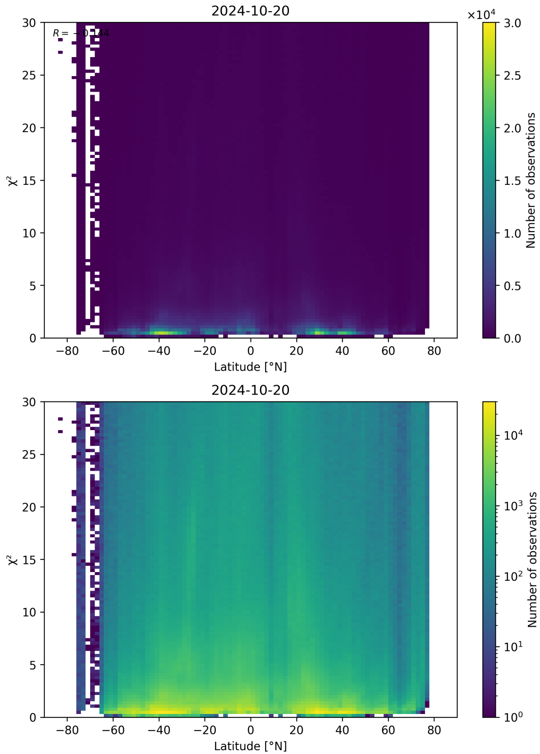
Figure 97: Scatter density plot of “Latitude” against “ \chi^2 ” for 2024-10-19 to 2024-10-21.
