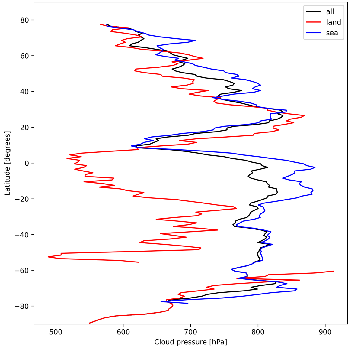
Figure 13: Zonal average of “Cloud pressure” for 2024-10-19 to 2024-10-21.
