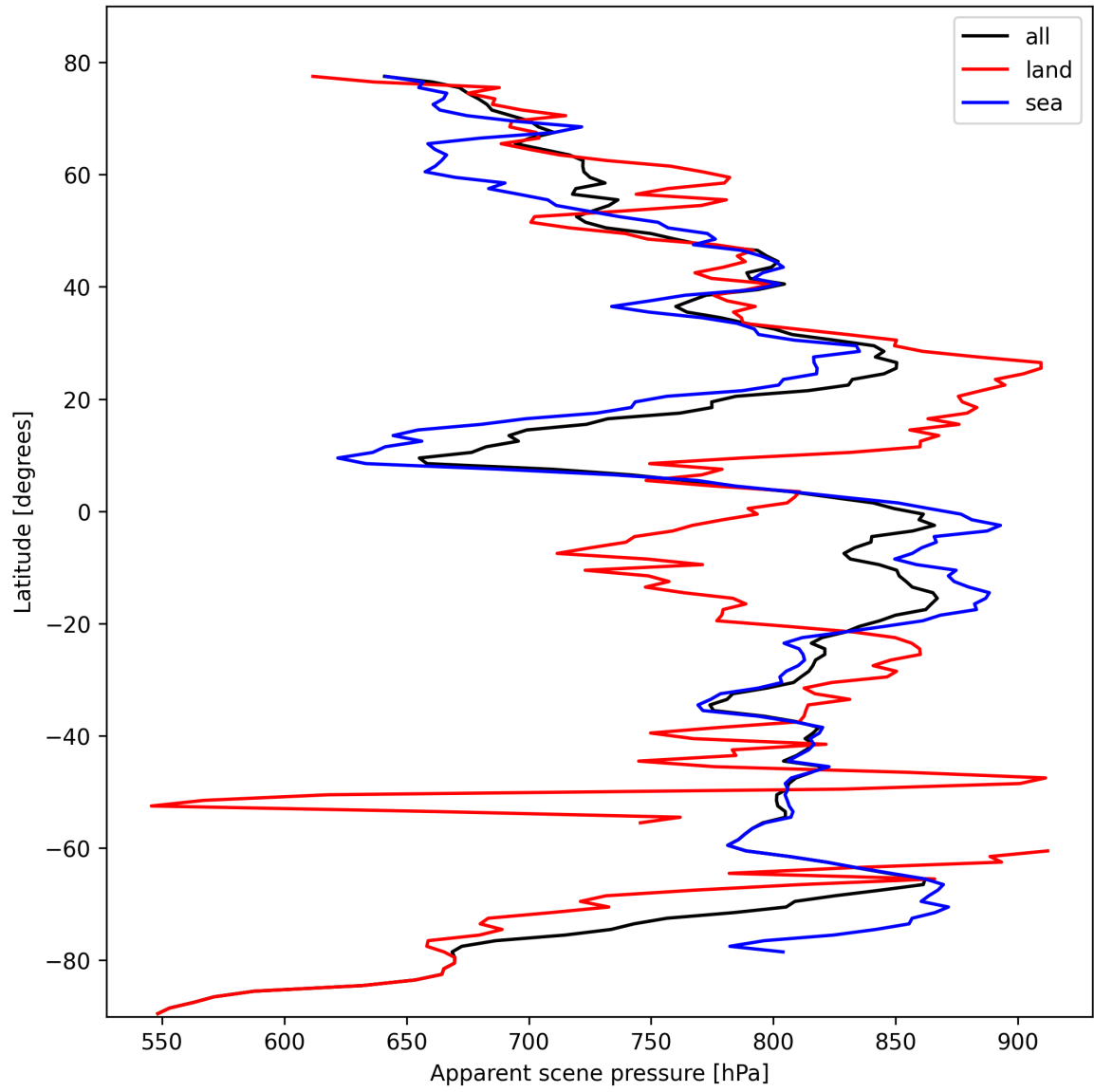
Figure 19: Zonal average of “Apparent scene pressure” for 2024-10-19 to 2024-10-21.
