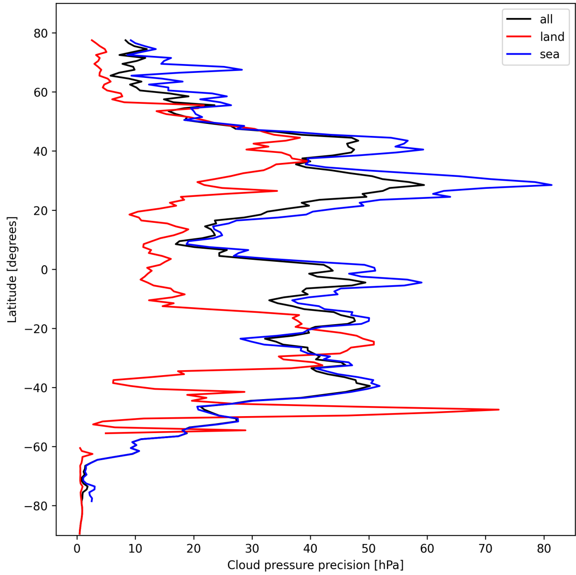
Figure 14: Zonal average of “Cloud pressure precision” for 2024-10-19 to 2024-10-21.
