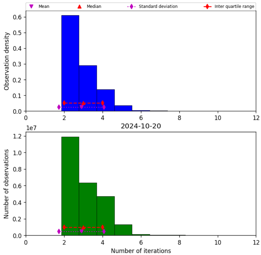
Figure 39: Histogram of “Number of iterations” for 2024-10-19 to 2024-10-21
