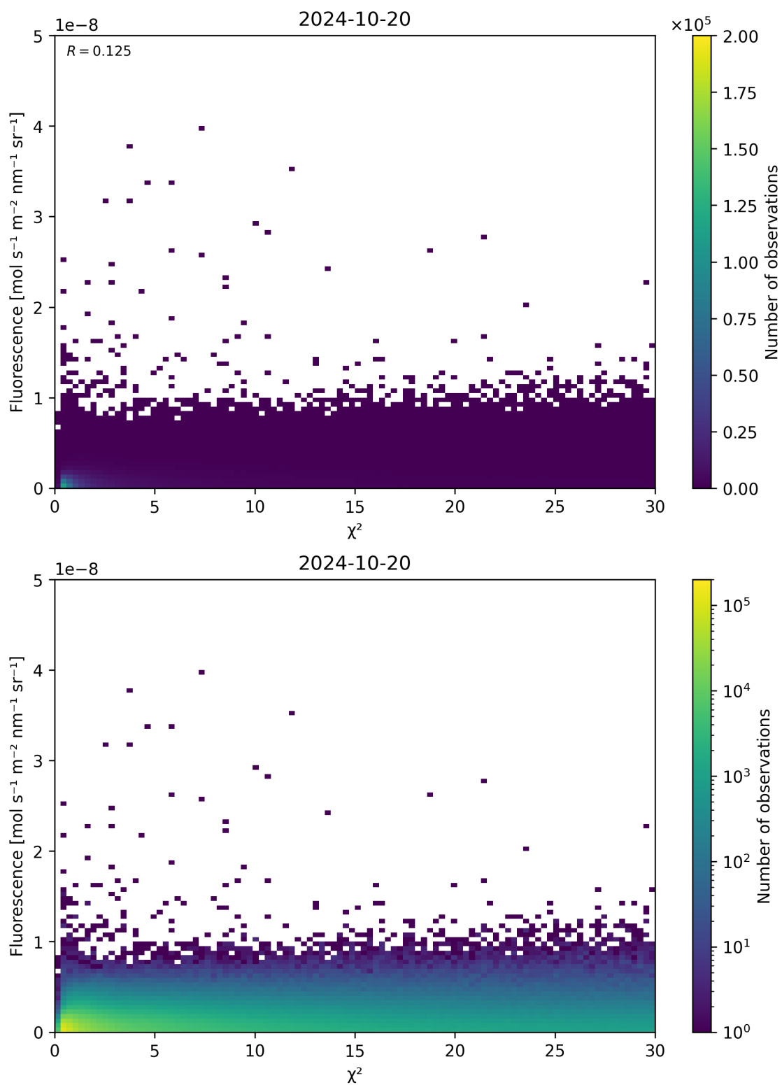
Figure 70: Scatter density plot of “ \chi^2 ” against “Fluorescence” for 2024-10-19 to 2024-10-21.
