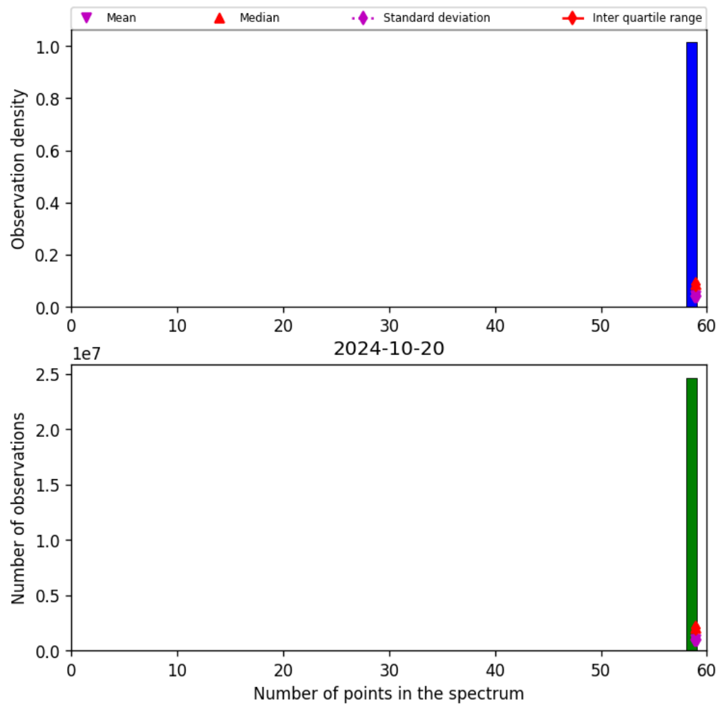
Figure 44: Histogram of “Number of points in the spectrum” for 2024-10-19 to 2024-10-21
