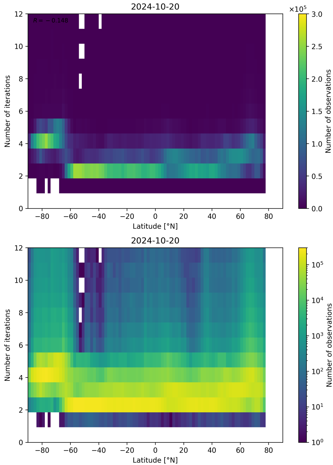
Figure 102: Scatter density plot of “Latitude” against “Number of iterations” for 2024-10-19 to 2024-10-21.
