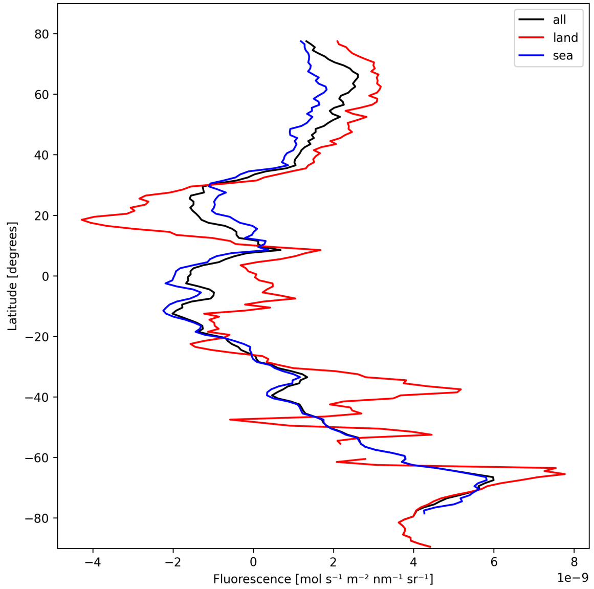
Figure 23: Zonal average of “Fluorescence” for 2024-10-19 to 2024-10-21.
