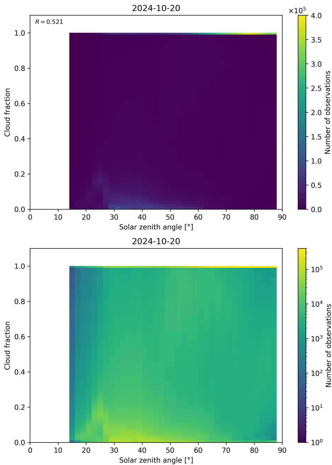
Figure 121: Scatter density plot of “Solar zenith angle” against “Cloud fraction” for 2024-10-19 to 2024-10-21.
