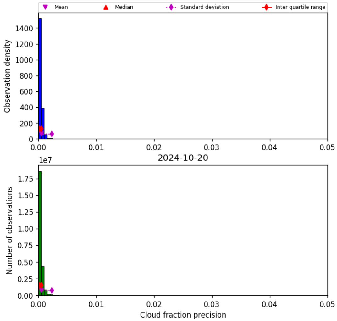
Figure 33: Histogram of “Cloud fraction precision” for 2024-10-19 to 2024-10-21
