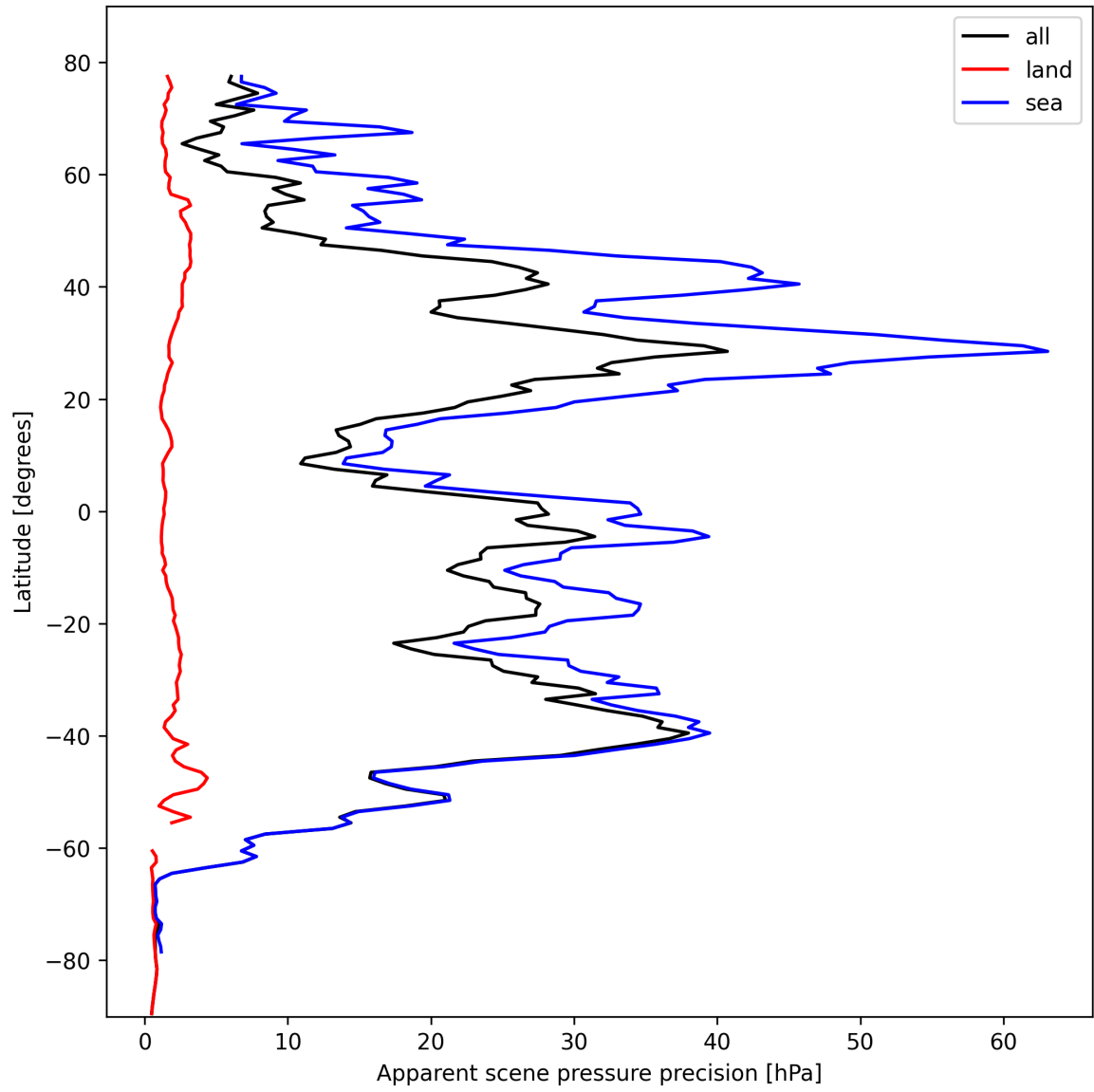
Figure 20: Zonal average of “Apparent scene pressure precision” for 2024-10-19 to 2024-10-21.
