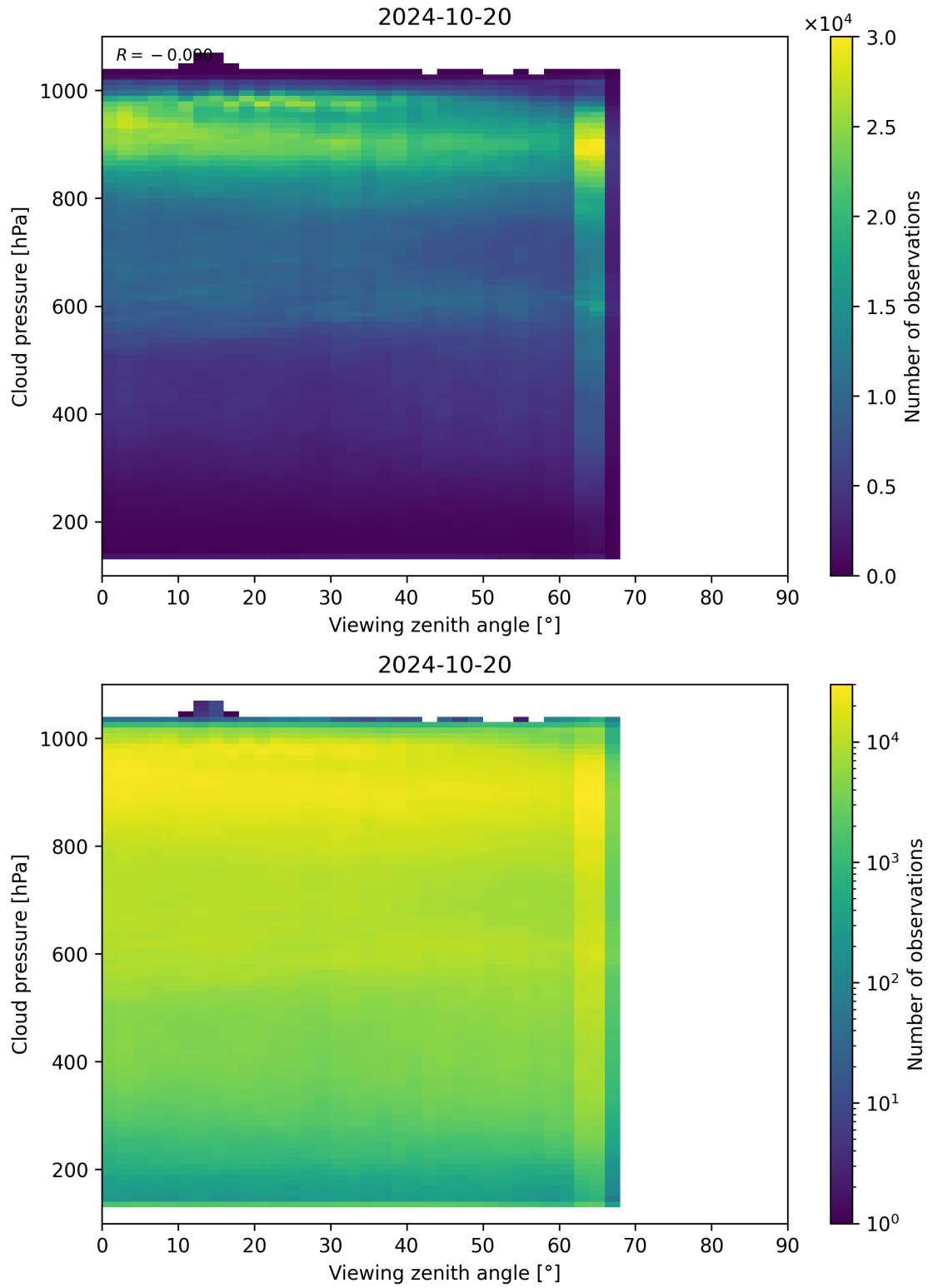
Figure 133: Scatter density plot of “Viewing zenith angle” against “Cloud pressure” for 2024-10-19 to 2024-10-21.
