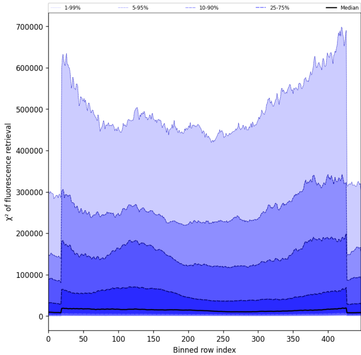
Figure 59: Along track statistics of “ \chi^2 of fluorescence retrieval” for 2024-10-19 to 2024-10-21
