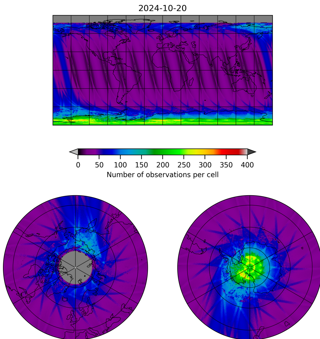
Figure 11: Map of the number of observations for 2024-10-19 to 2024-10-21
