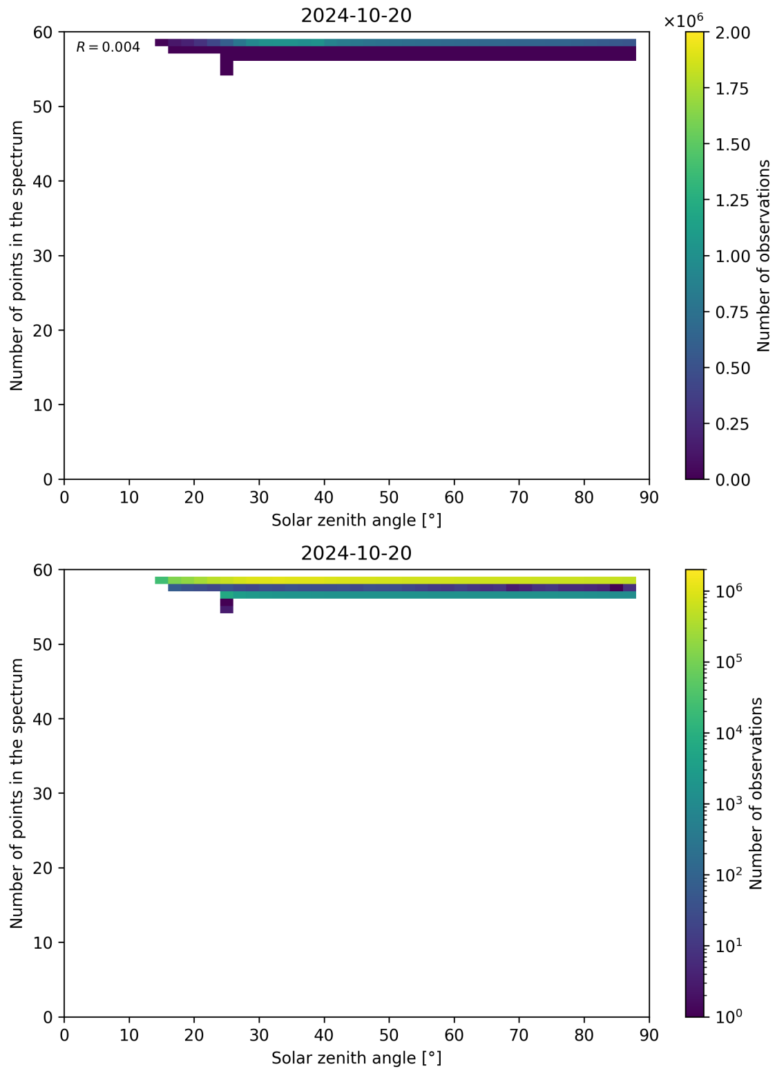
Figure 126: Scatter density plot of “Solar zenith angle” against “Number of points in the spectrum” for 2024-10-19 to 2024-10-21.
