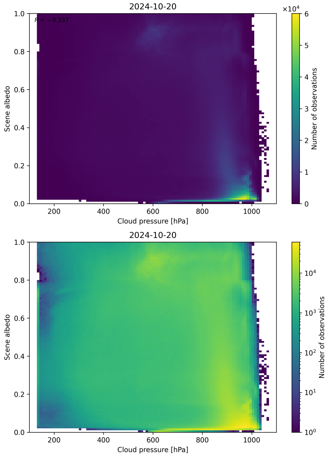
Figure 91: Scatter density plot of “Cloud pressure” against “Scene albedo” for 2024-10-19 to 2024-10-21.
