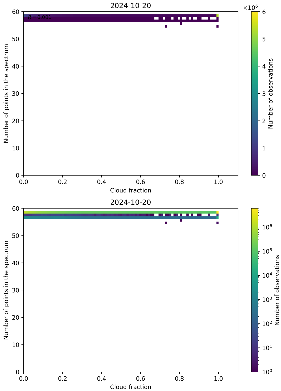
Figure 81: Scatter density plot of “Cloud fraction” against “Number of points in the spectrum” for 2024-10-19 to 2024-10-21.
