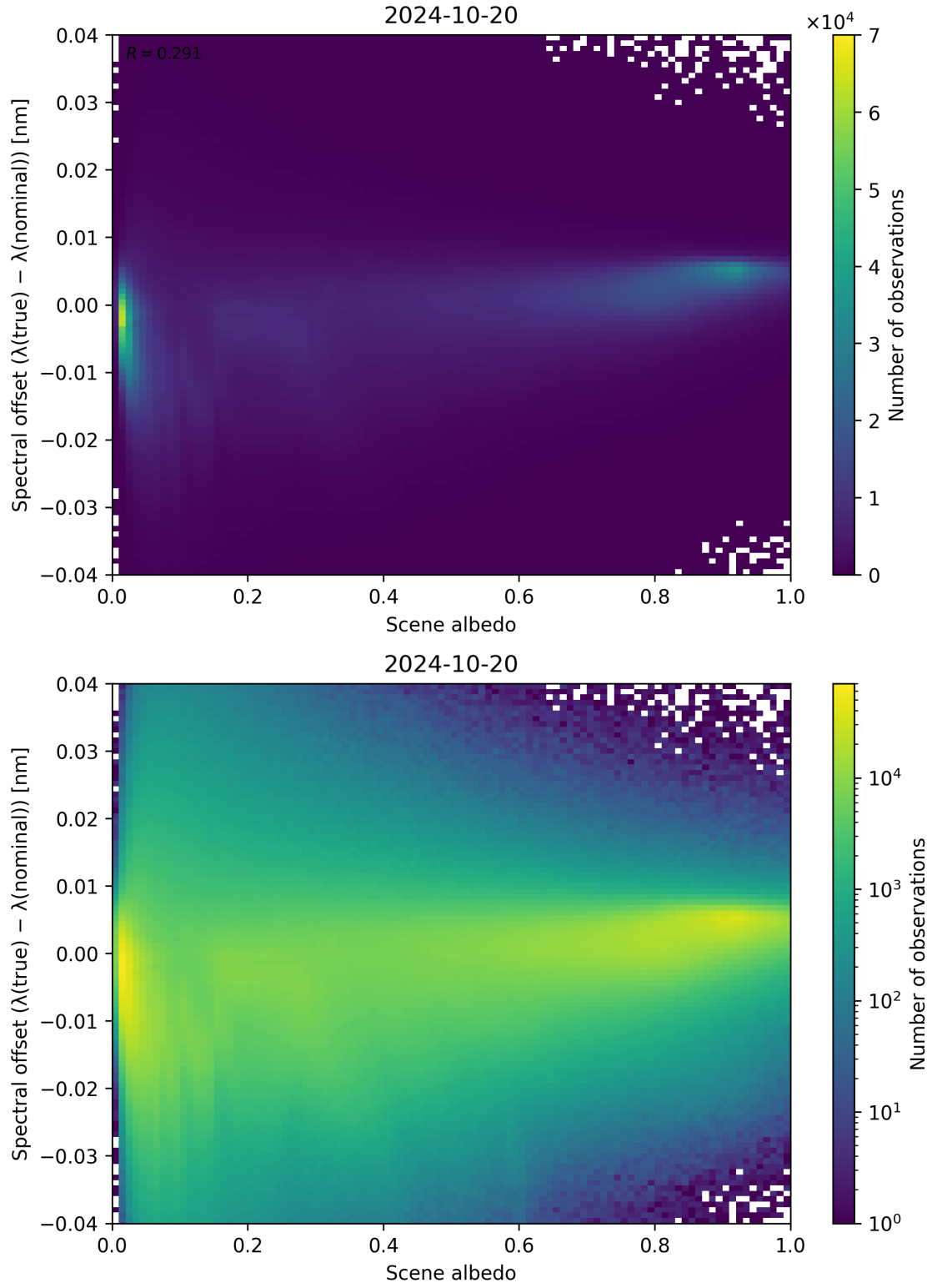
Figure 117: Scatter density plot of “Scene albedo” against “Spectral offset ( \lambda_{\text{true}} - \lambda_{\text{nominal}} )” for 2024-10-19 to 2024-10-21.
