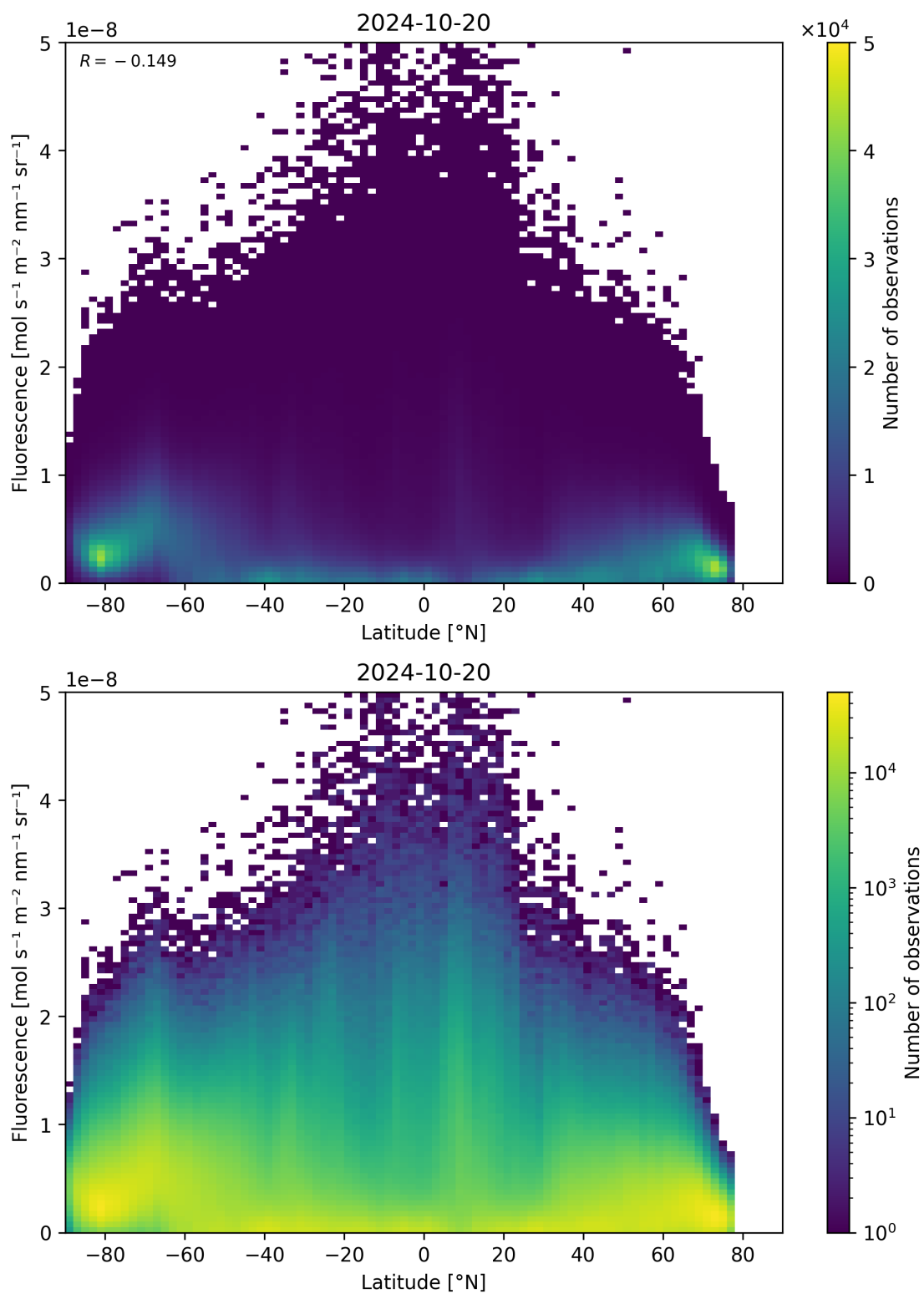
Figure 101: Scatter density plot of “Latitude” against “Fluorescence” for 2024-10-19 to 2024-10-21.
