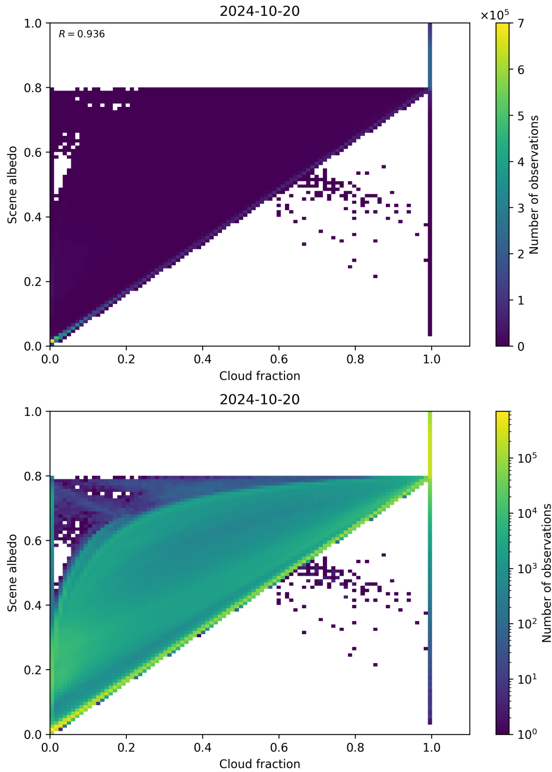
Figure 82: Scatter density plot of “Cloud fraction” against “Scene albedo” for 2024-10-19 to 2024-10-21.
