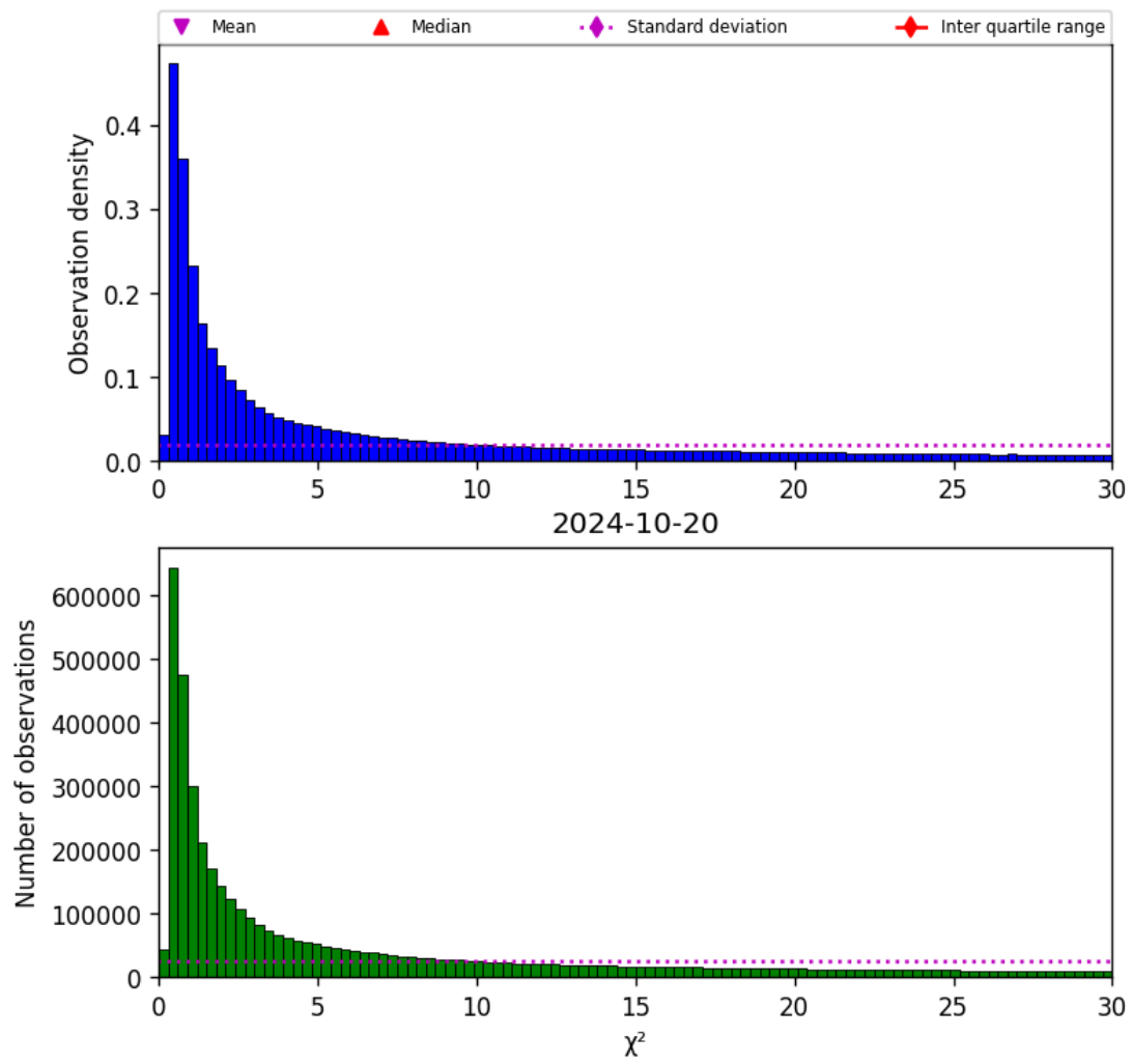
Figure 38: Histogram of " \chi^2 " for 2024-10-19 to 2024-10-21
