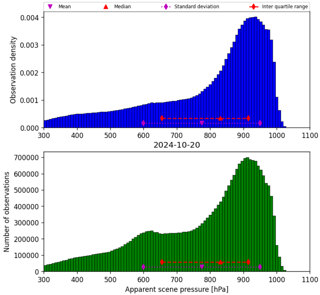
Figure 36: Histogram of “Apparent scene pressure” for 2024-10-19 to 2024-10-21
