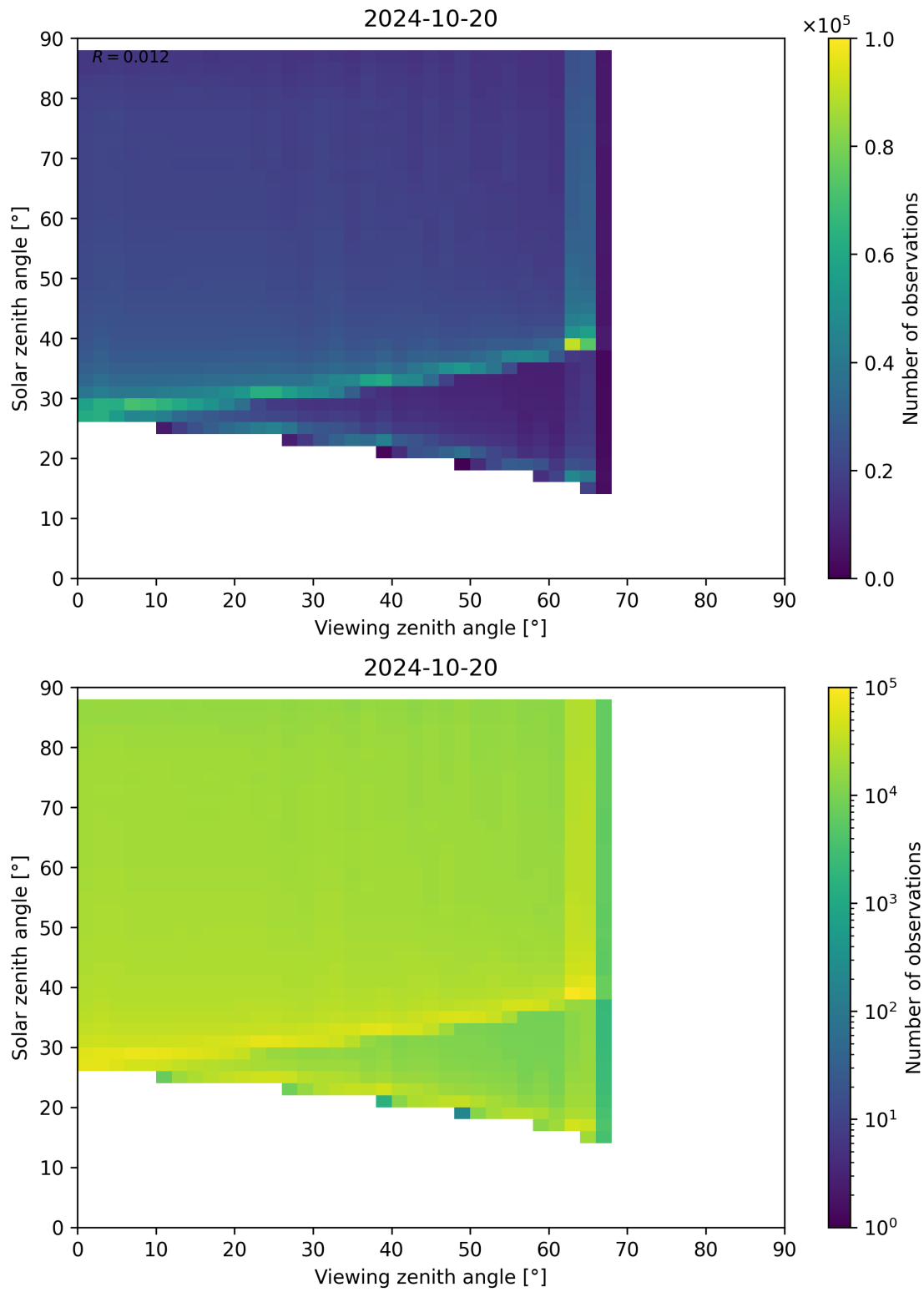
Figure 139: Scatter density plot of “Viewing zenith angle” against “Solar zenith angle” for 2024-10-19 to 2024-10-21.
