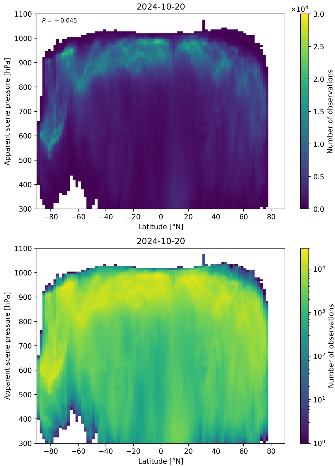
Figure 96: Scatter density plot of “Latitude” against “Apparent scene pressure” for 2024-10-19 to 2024-10-21.
