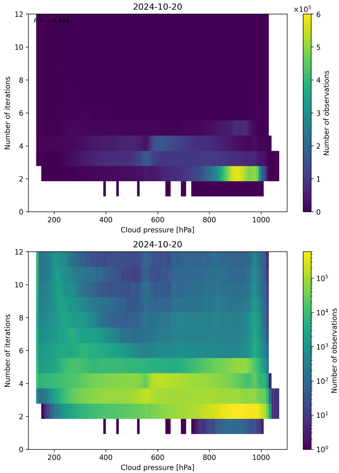
Figure 89: Scatter density plot of “Cloud pressure” against “Number of iterations” for 2024-10-19 to 2024-10-21.
