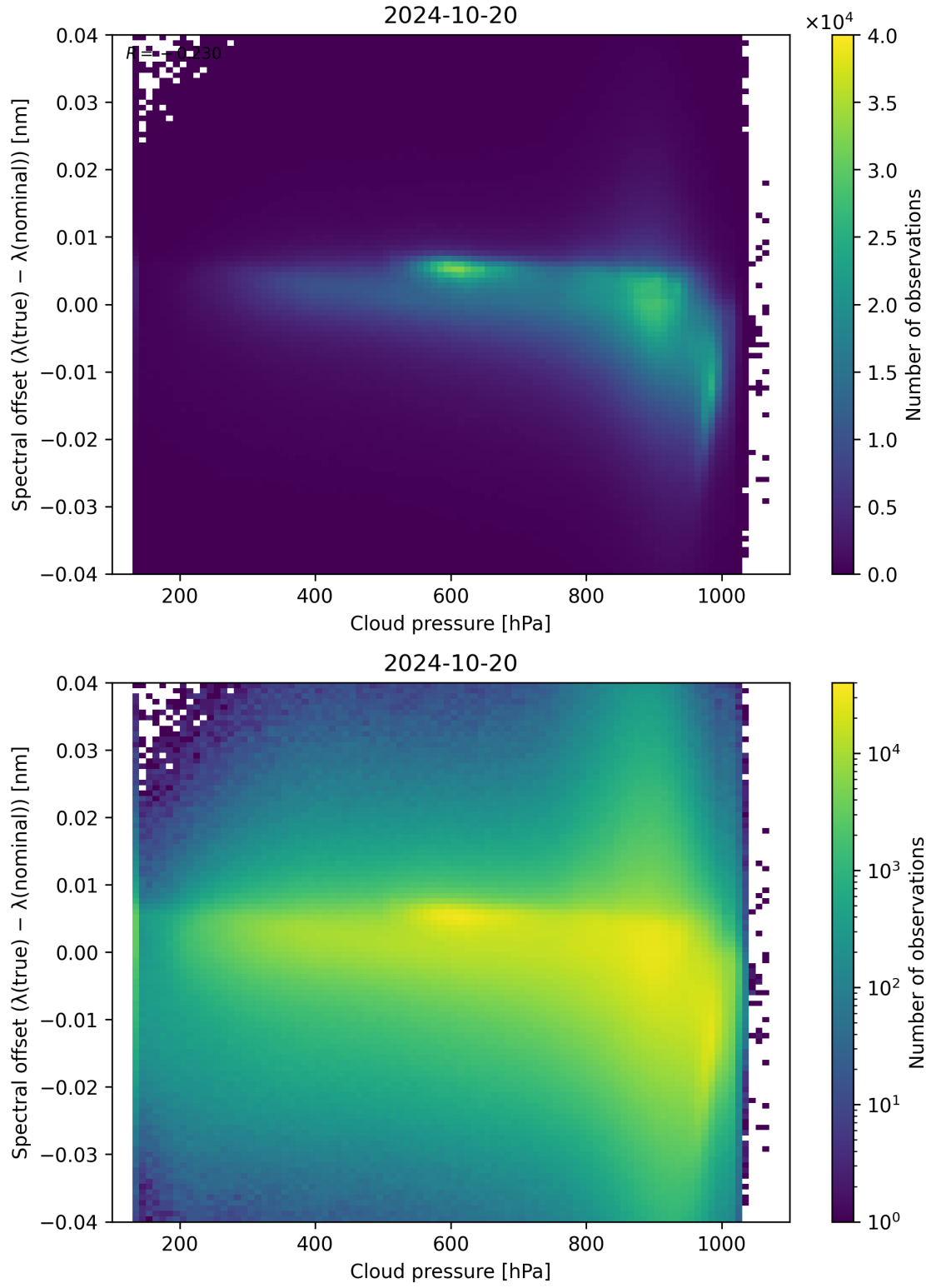
Figure 92: Scatter density plot of “Cloud pressure” against “Spectral offset ( \lambda_{\text{true}} - \lambda_{\text{nominal}} )” for 2024-10-19 to 2024-10-21.
