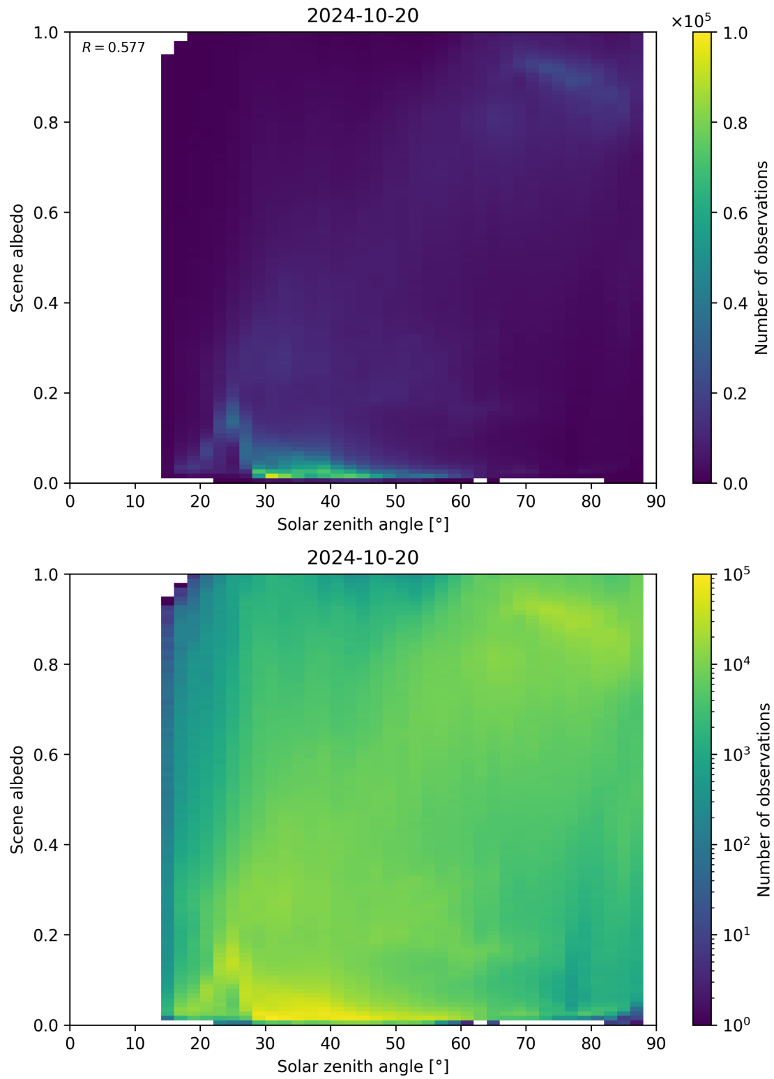
Figure 127: Scatter density plot of “Solar zenith angle” against “Scene albedo” for 2024-10-19 to 2024-10-21.
