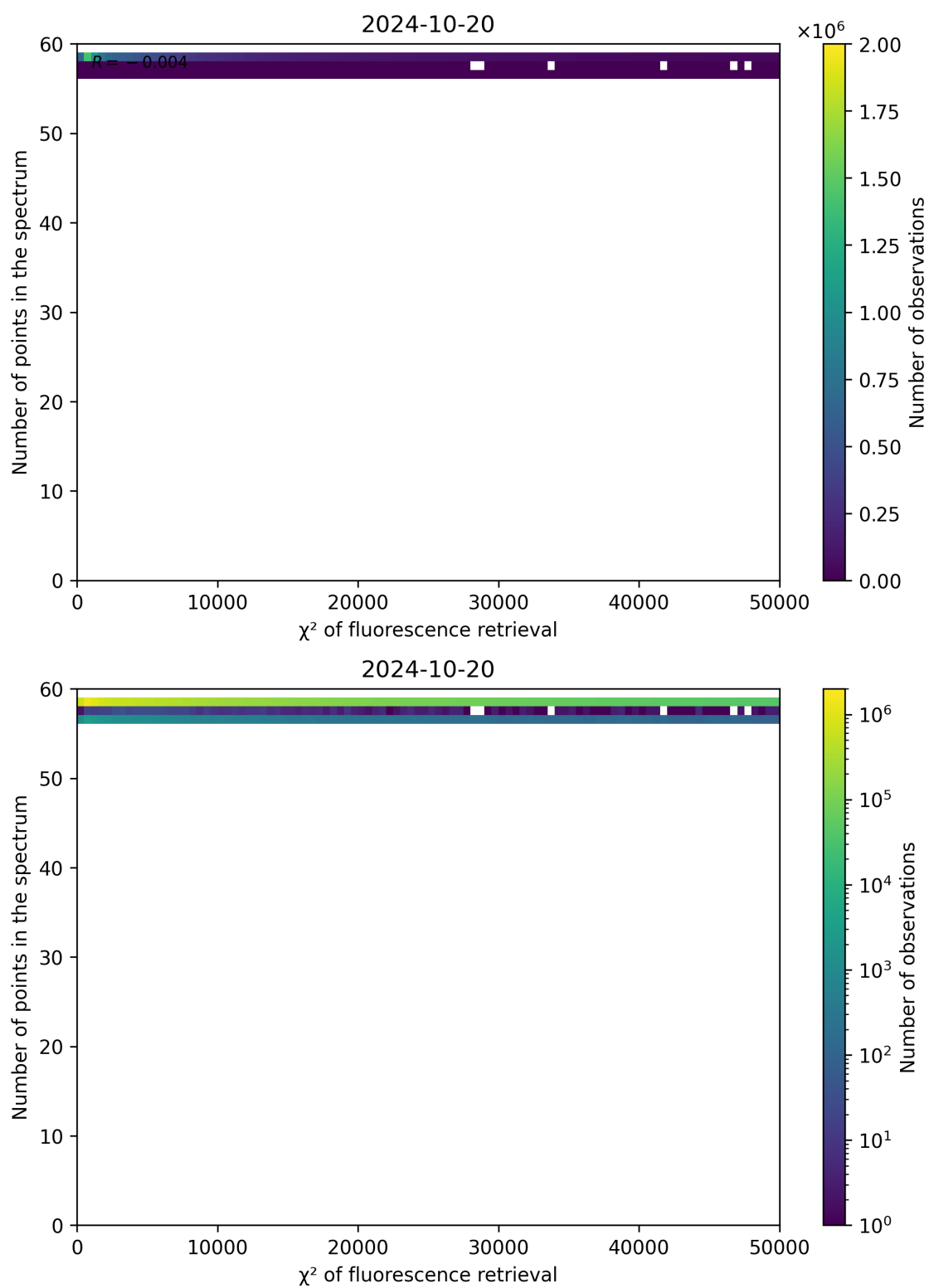
Figure 71: Scatter density plot of “ \chi^2 of fluorescence retrieval” against “Number of points in the spectrum” for 2024-10-19 to 2024-10-21.
