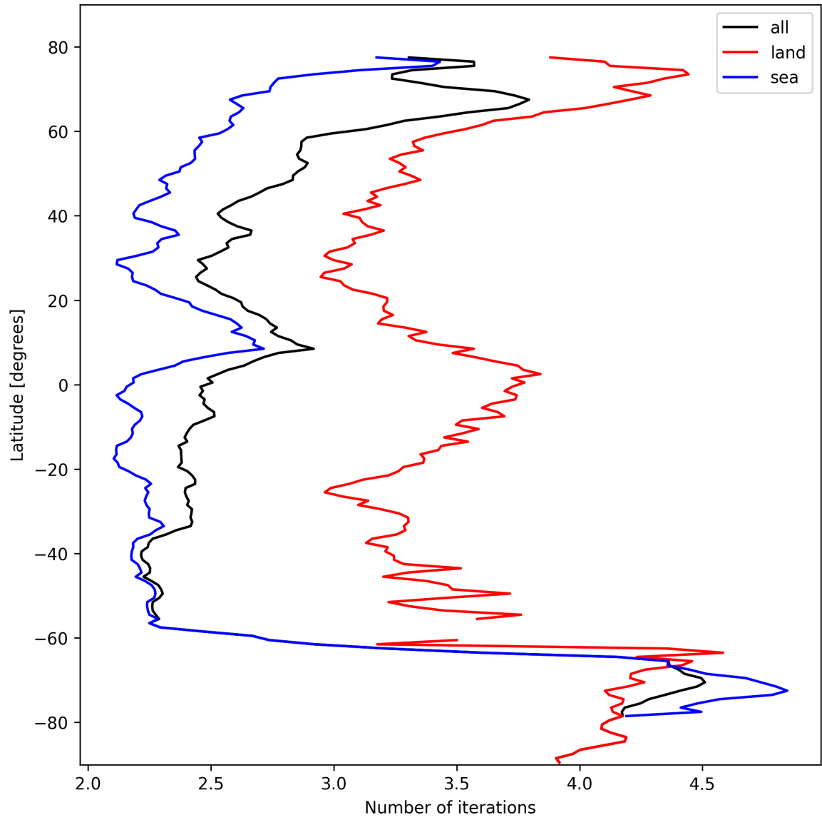
Figure 22: Zonal average of “Number of iterations” for 2024-10-19 to 2024-10-21.
