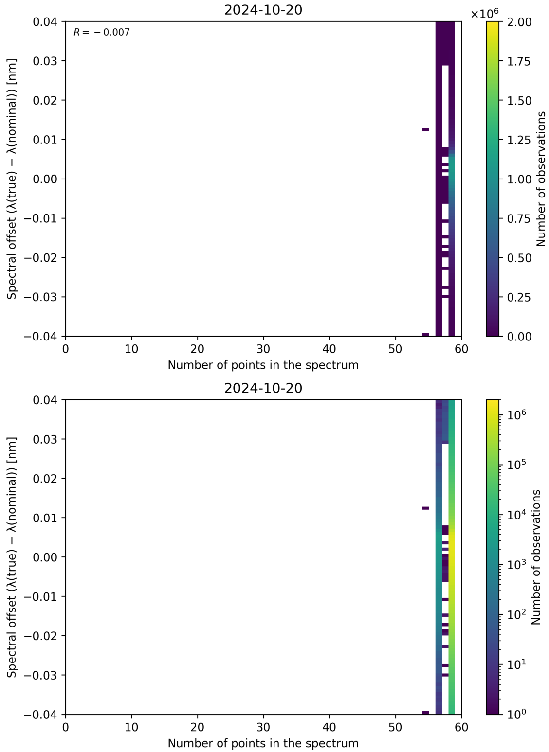
Figure 110: Scatter density plot of “Number of points in the spectrum” against “Spectral offset ( \lambda_{\text{true}} - \lambda_{\text{nominal}} )” for 2024-10-19 to 2024-10-21.
