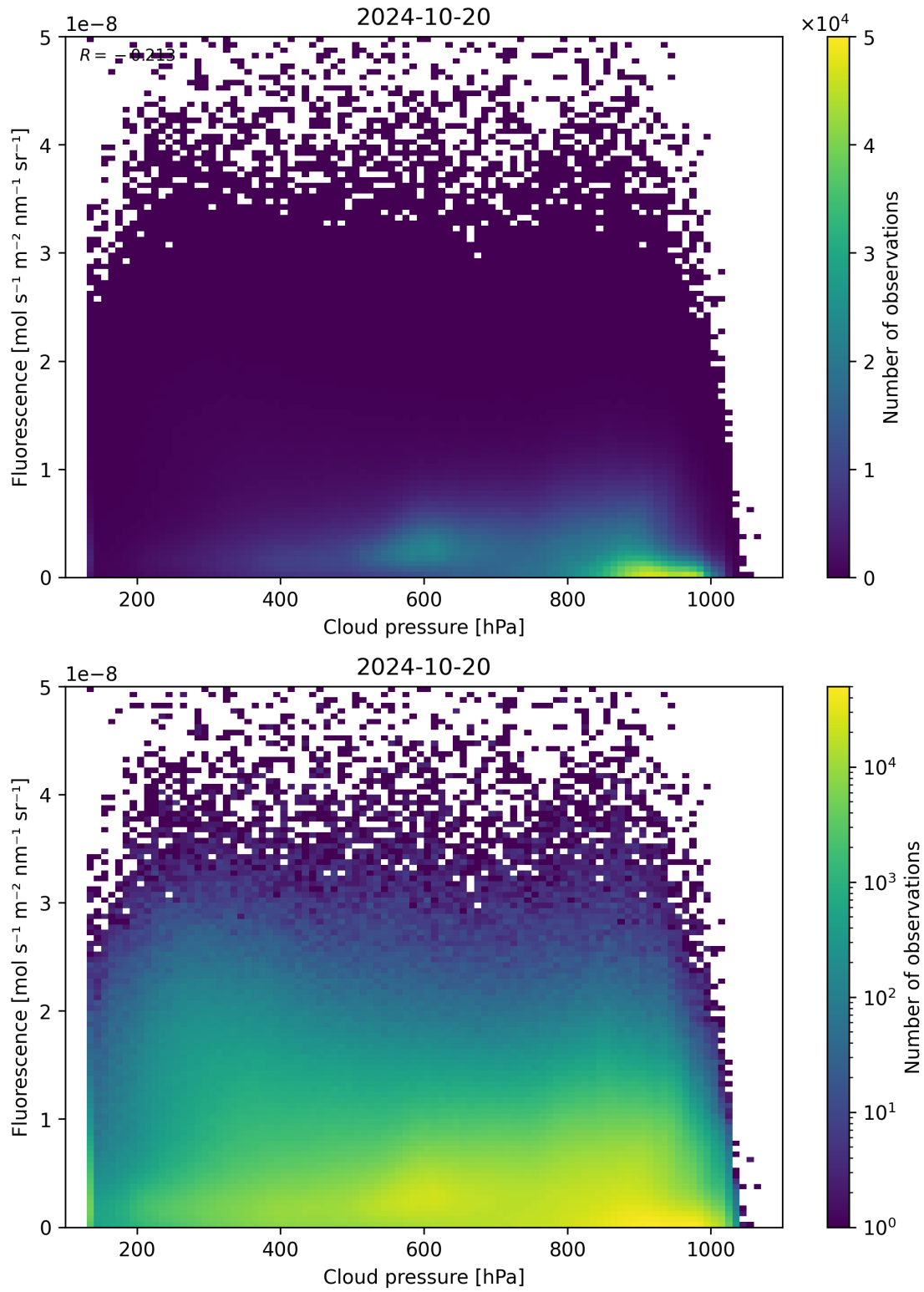
Figure 88: Scatter density plot of “Cloud pressure” against “Fluorescence” for 2024-10-19 to 2024-10-21.
