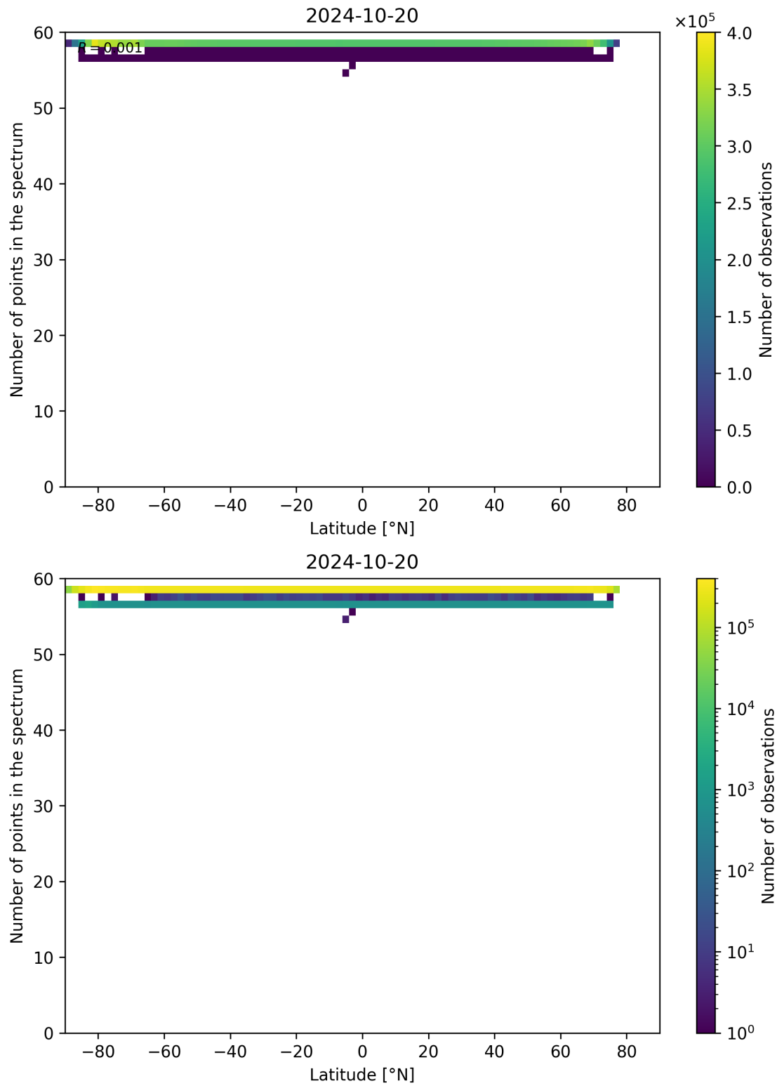
Figure 103: Scatter density plot of “Latitude” against “Number of points in the spectrum” for 2024-10-19 to 2024-10-21.
