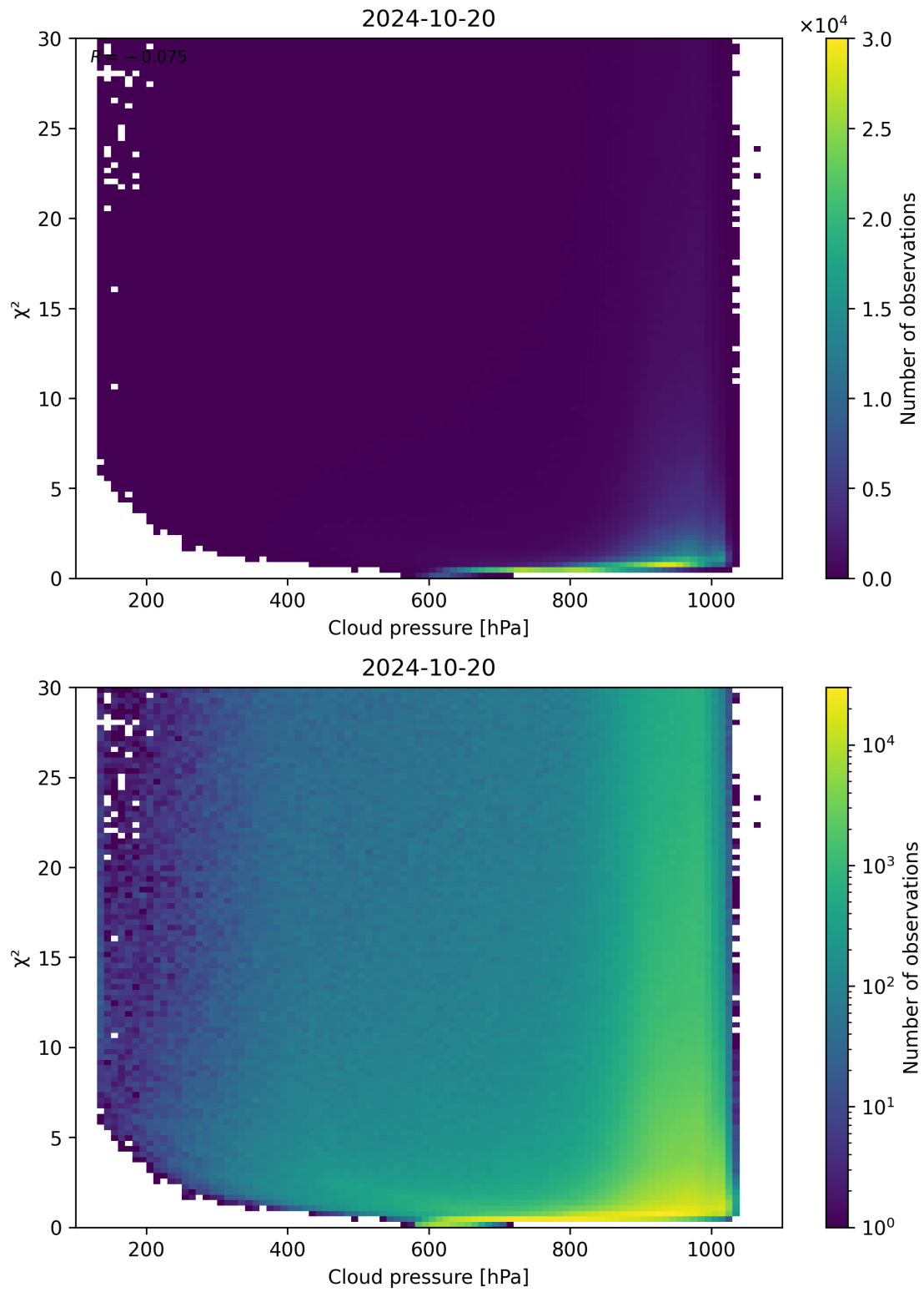
Figure 85: Scatter density plot of “Cloud pressure” against “ \chi^2 ” for 2024-10-19 to 2024-10-21.
