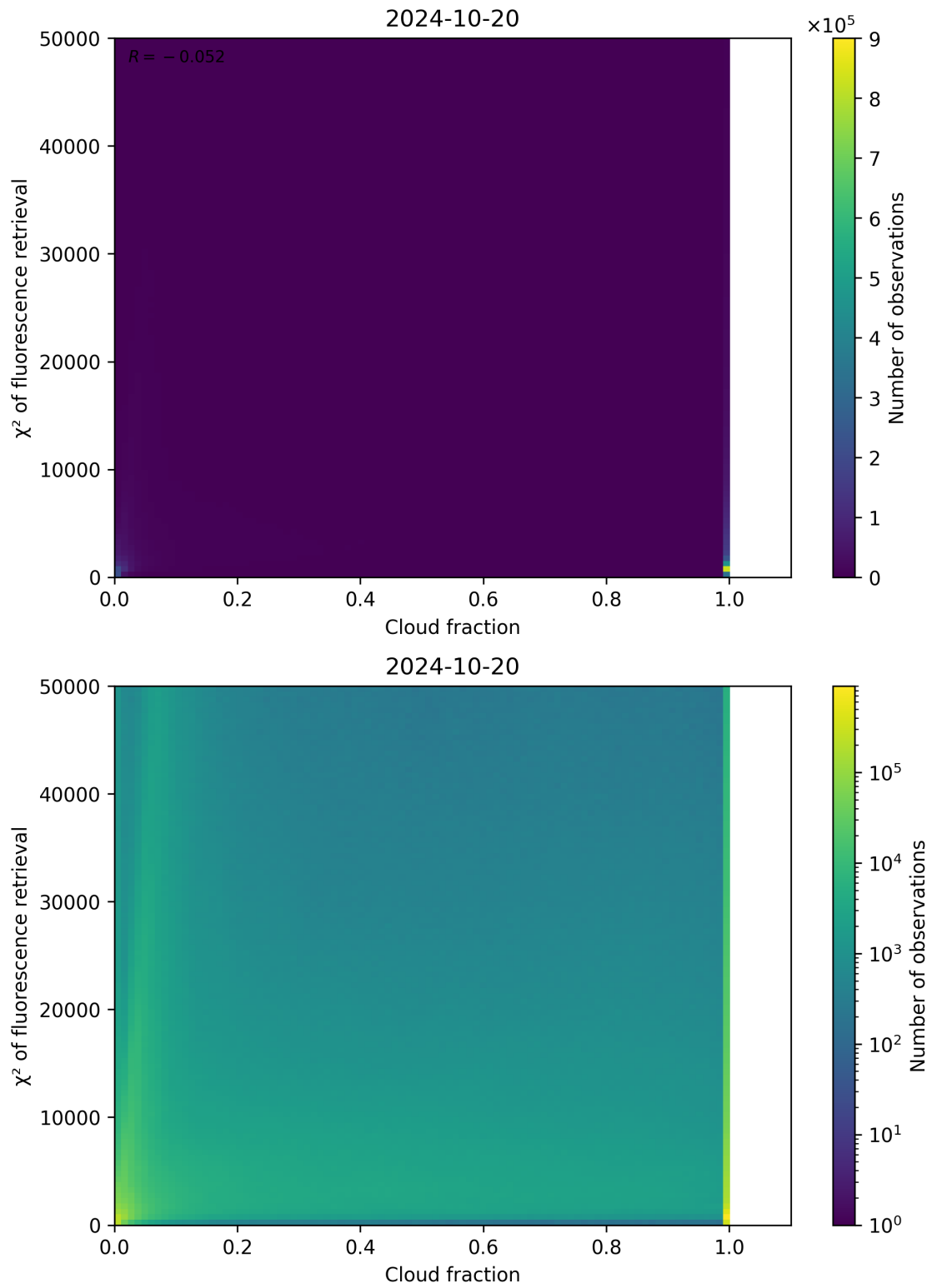
Figure 78: Scatter density plot of “Cloud fraction” against “ \chi^2 of fluorescence retrieval” for 2024-10-19 to 2024-10-21.
