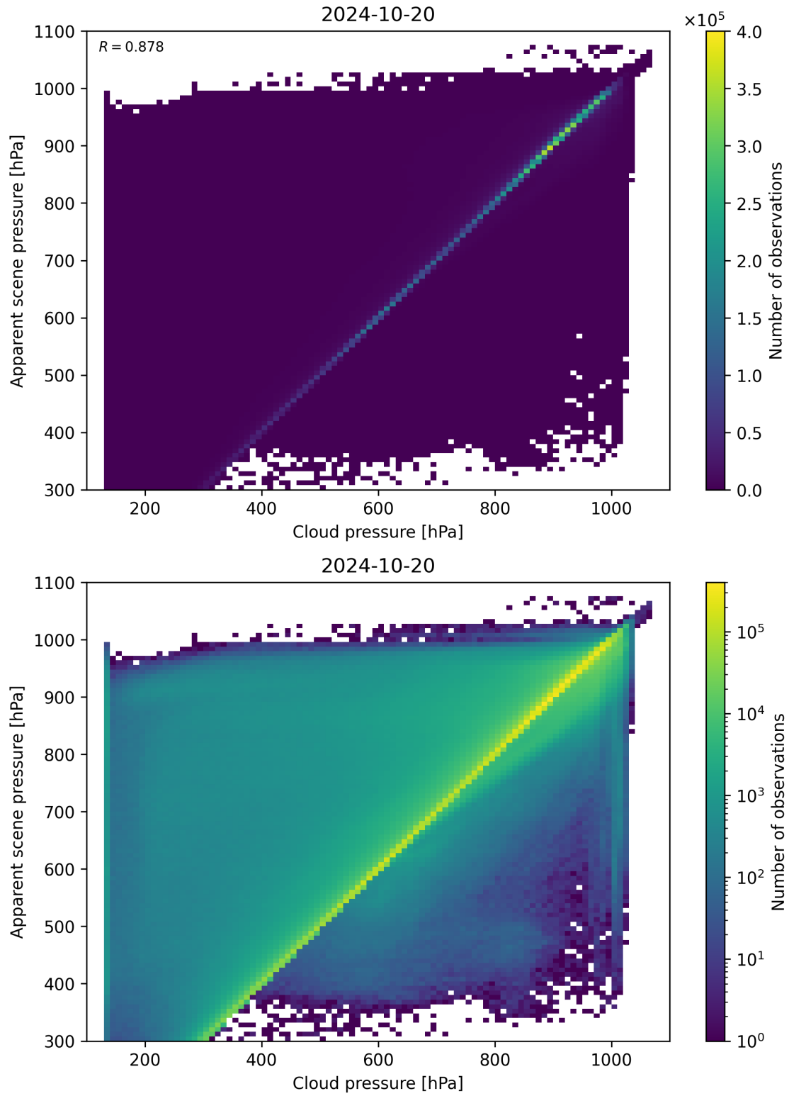
Figure 84: Scatter density plot of “Cloud pressure” against “Apparent scene pressure” for 2024-10-19 to 2024-10-21.
