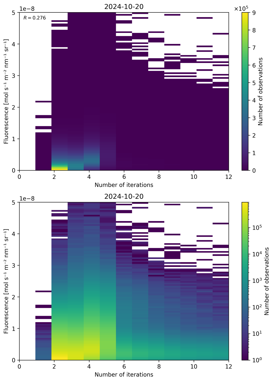
Figure 107: Scatter density plot of “Number of iterations” against “Fluorescence” for 2024-10-19 to 2024-10-21.
