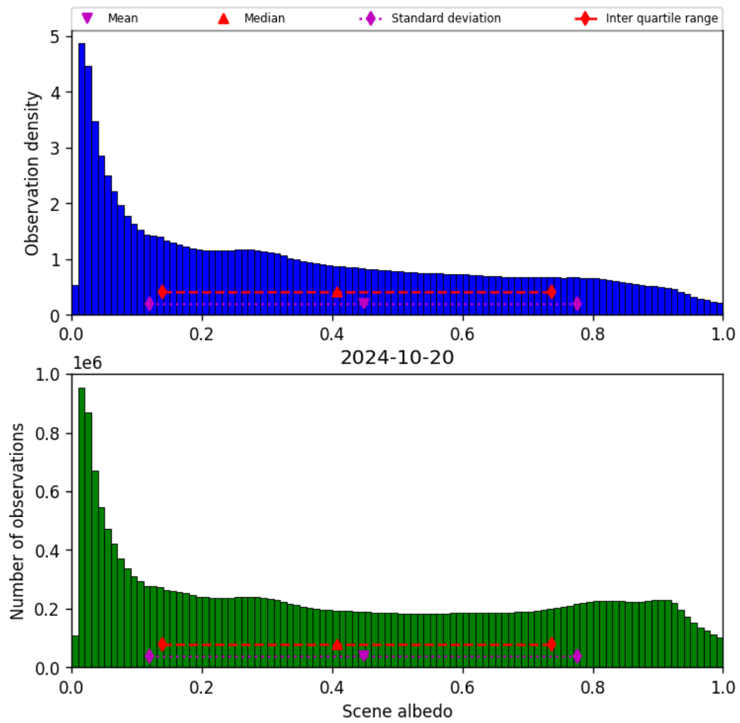
Figure 34: Histogram of “Scene albedo” for 2024-10-19 to 2024-10-21
