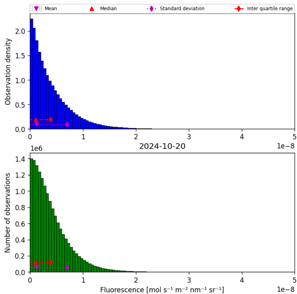
Figure 40: Histogram of “Fluorescence” for 2024-10-19 to 2024-10-21
