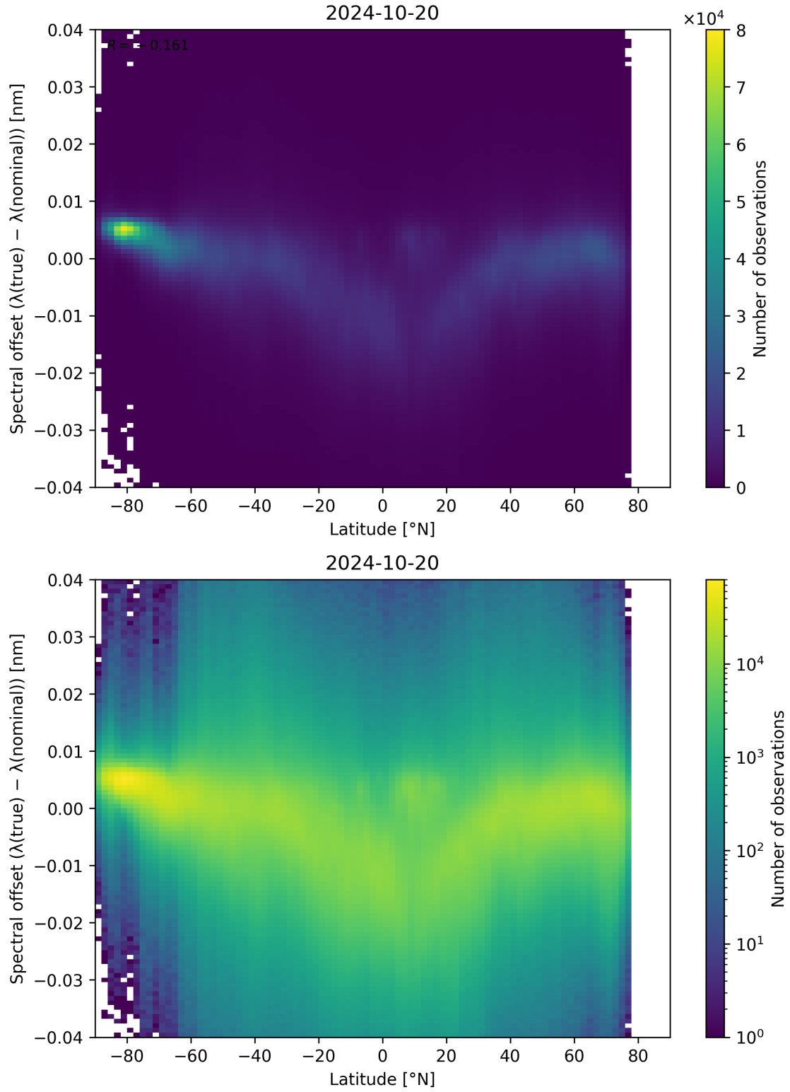
Figure 105: Scatter density plot of “Latitude” against “Spectral offset ( \lambda_{\text{true}} - \lambda_{\text{nominal}} )” for 2024-10-19 to 2024-10-21.
