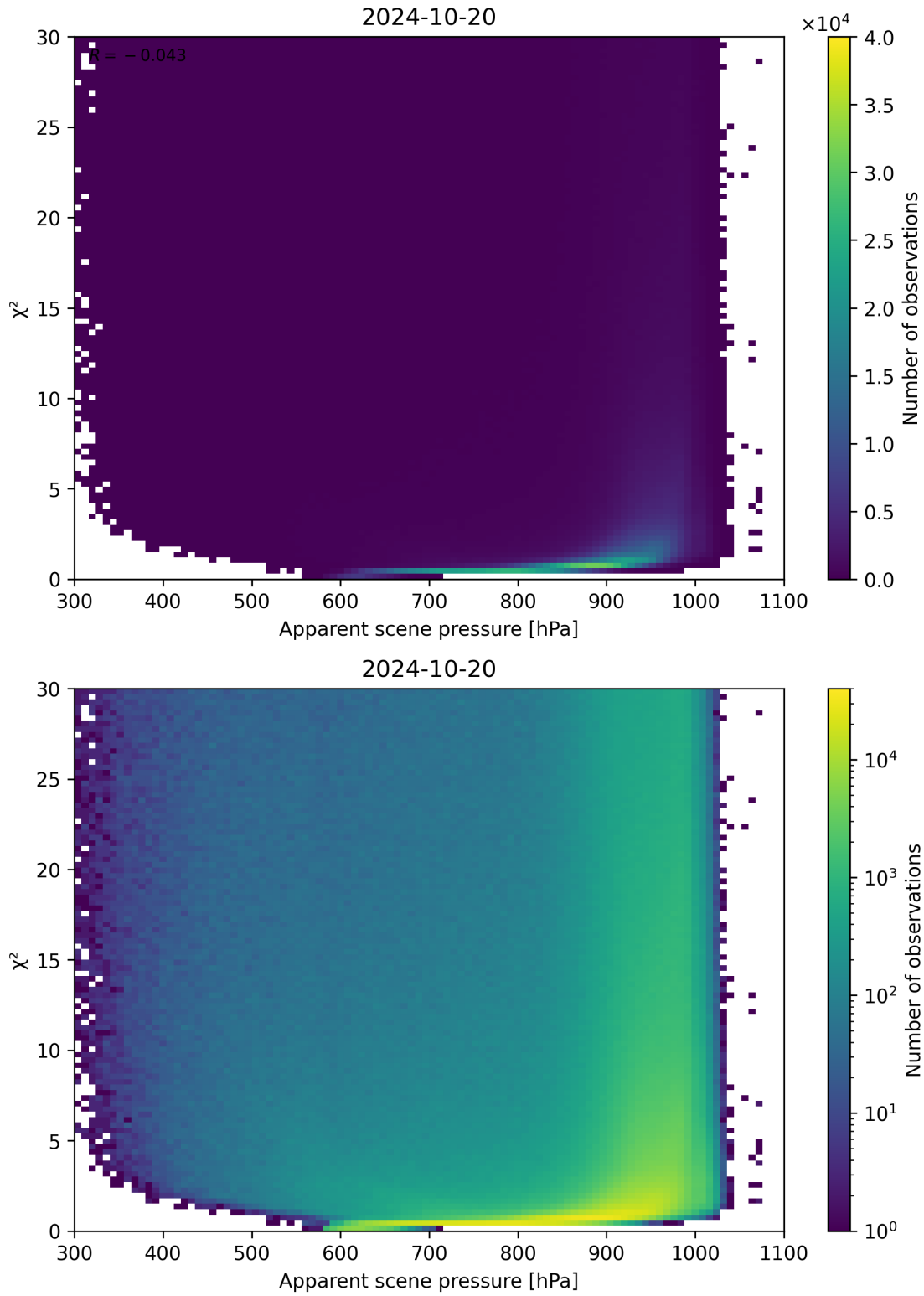
Figure 63: Scatter density plot of “Apparent scene pressure” against “ \chi^2 ” for 2024-10-19 to 2024-10-21.
