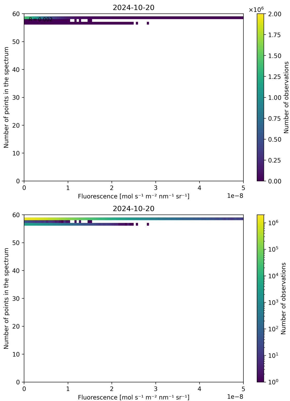
Figure 94: Scatter density plot of “Fluorescence” against “Number of points in the spectrum” for 2024-10-19 to 2024-10-21.
