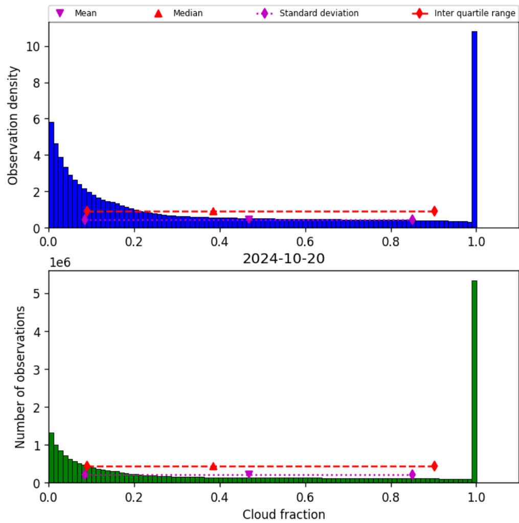
Figure 32: Histogram of “Cloud fraction” for 2024-10-19 to 2024-10-21
