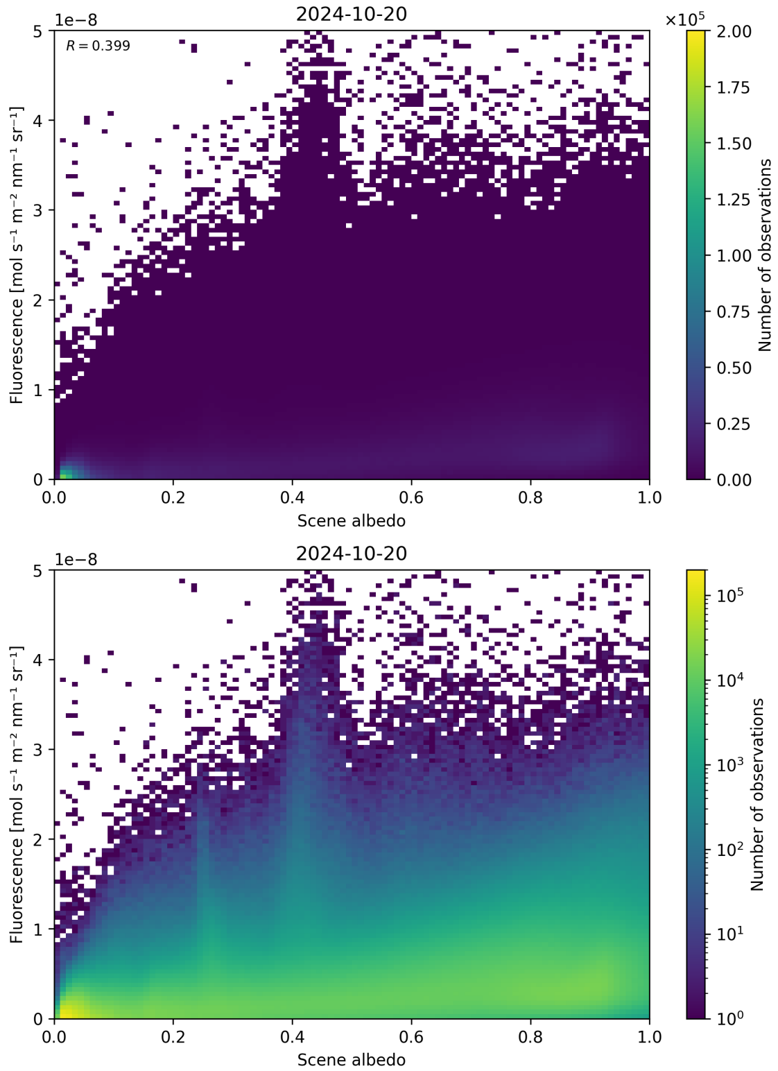
Figure 114: Scatter density plot of “Scene albedo” against “Fluorescence” for 2024-10-19 to 2024-10-21.
