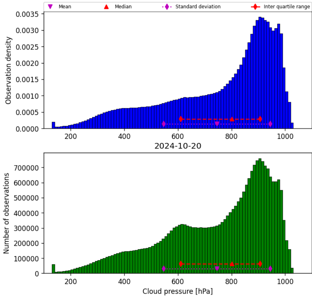
Figure 30: Histogram of “Cloud pressure” for 2024-10-19 to 2024-10-21
