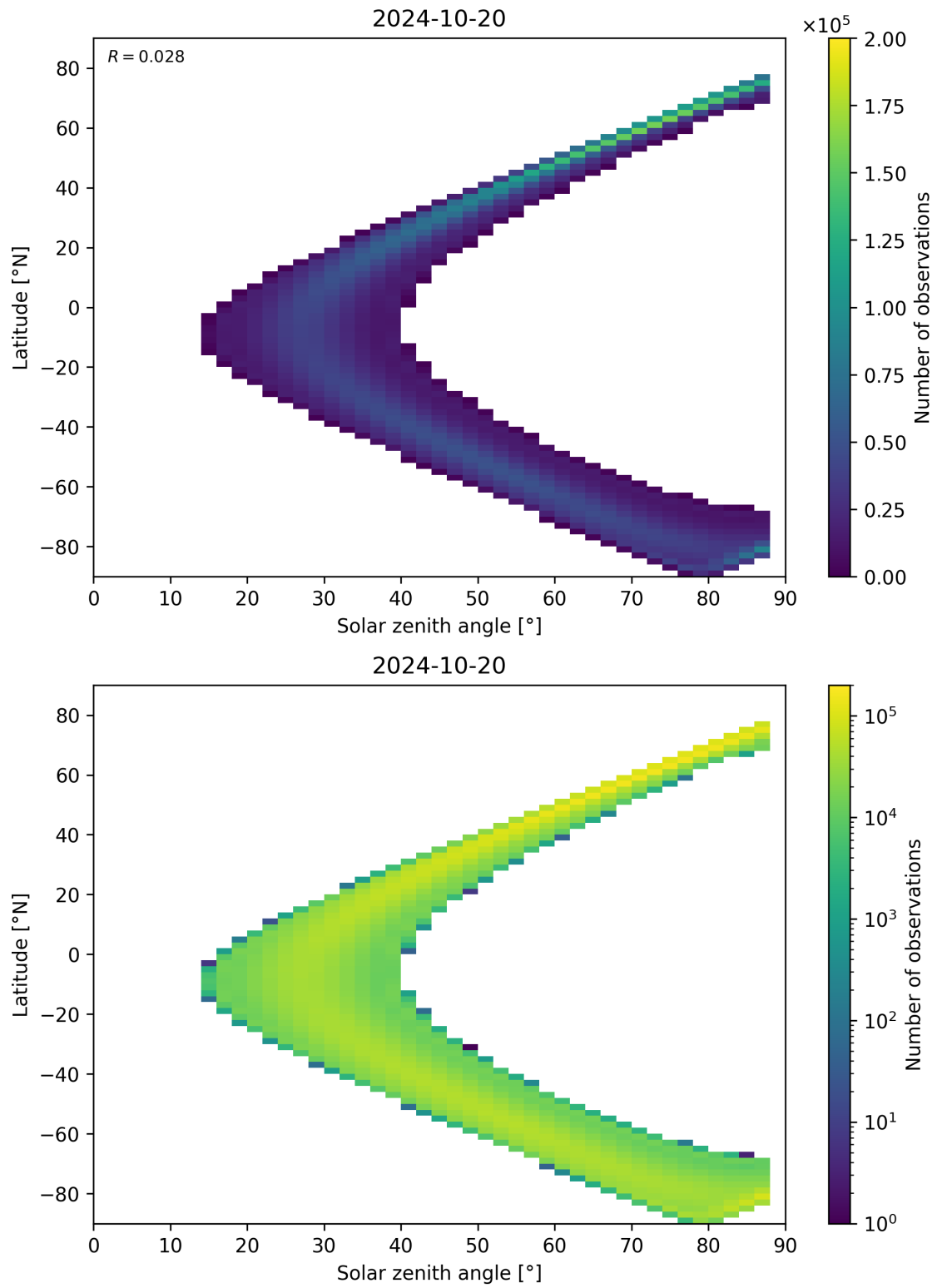
Figure 124: Scatter density plot of “Solar zenith angle” against “Latitude” for 2024-10-19 to 2024-10-21.
