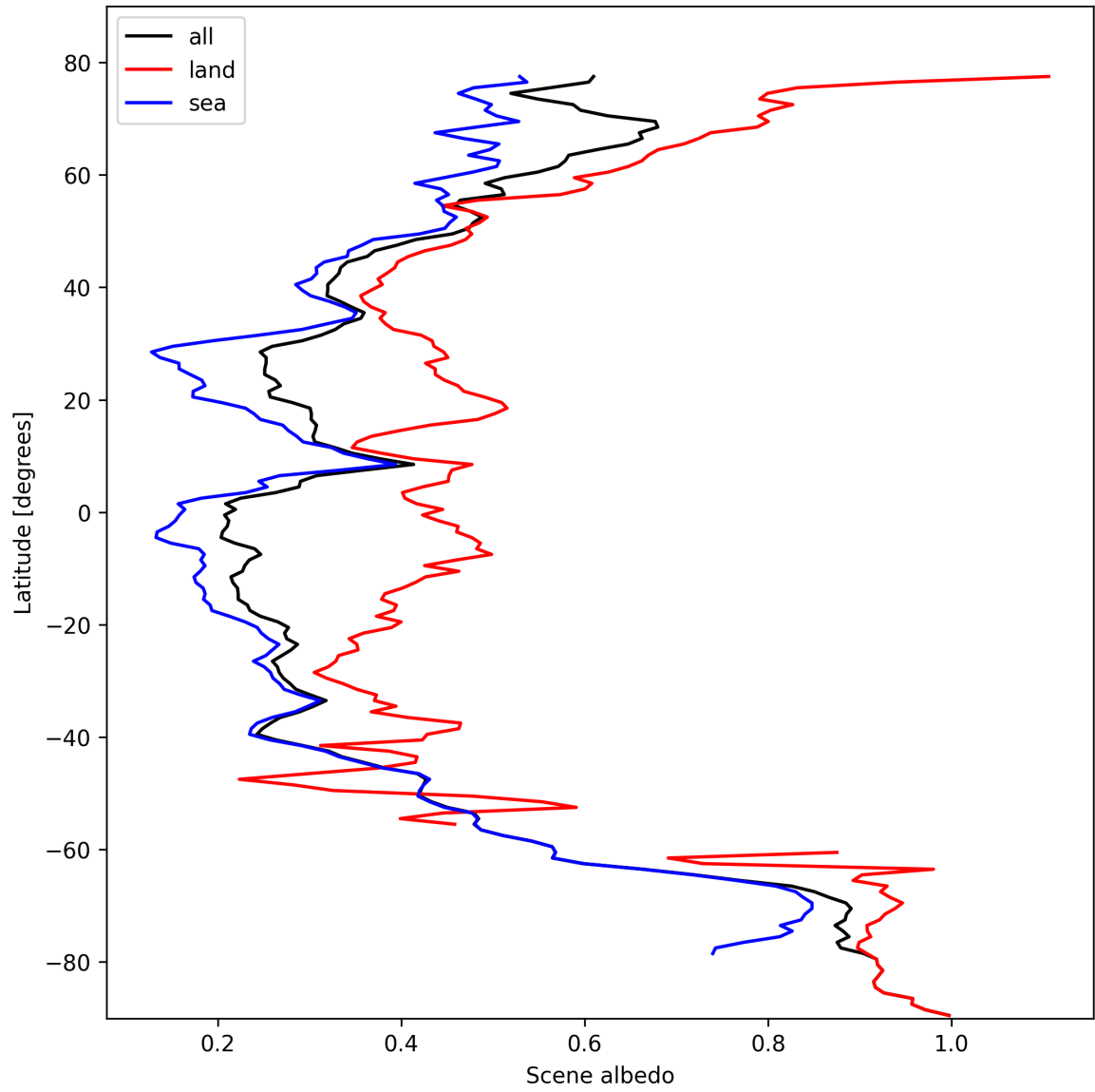
Figure 17: Zonal average of “Scene albedo” for 2024-10-19 to 2024-10-21.
