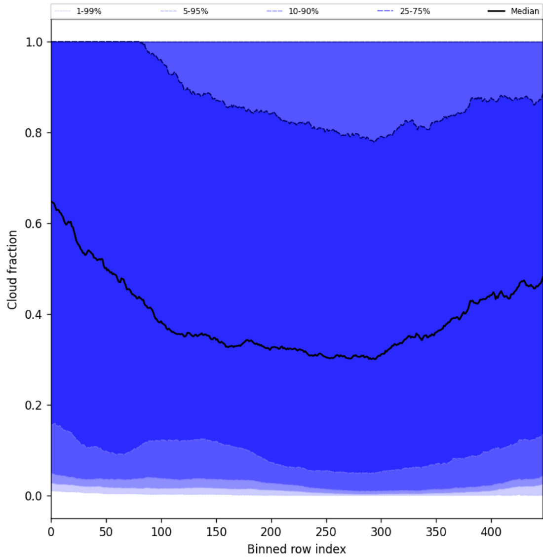
Figure 49: Along track statistics of “Cloud fraction” for 2024-10-19 to 2024-10-21
