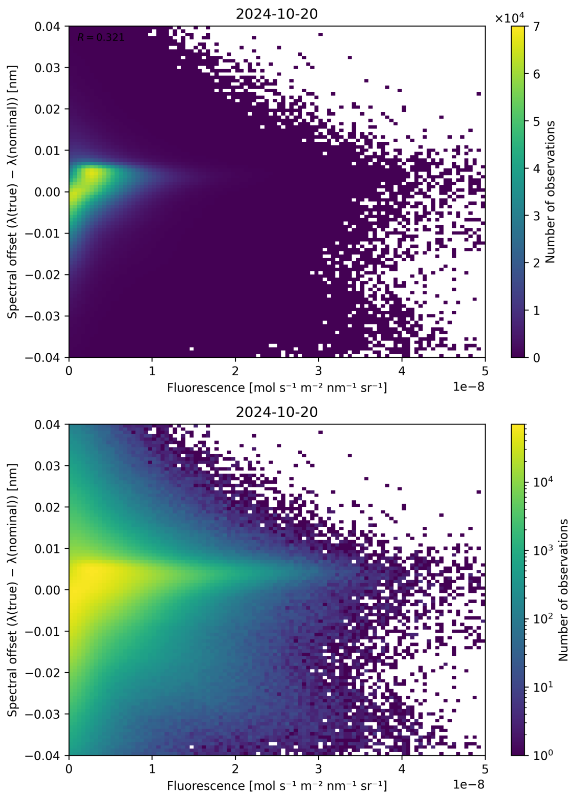
Figure 95: Scatter density plot of “Fluorescence” against “Spectral offset ( \lambda_{\text{true}} - \lambda_{\text{nominal}} )” for 2024-10-19 to 2024-10-21.
