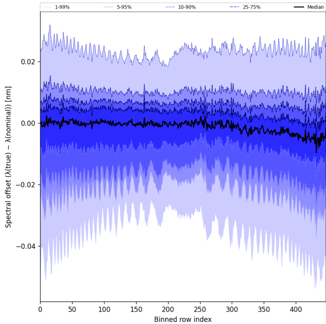
Figure 62: Along track statistics of “Spectral offset ( \lambda_{\text{true}} - \lambda_{\text{nominal}} )” for 2024-10-19 to 2024-10-21
