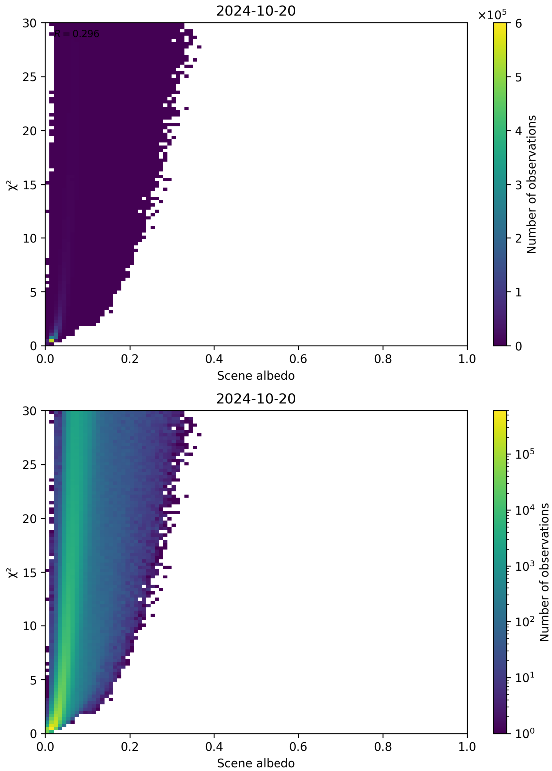
Figure 112: Scatter density plot of “Scene albedo” against “ \chi^2 ” for 2024-10-19 to 2024-10-21.
