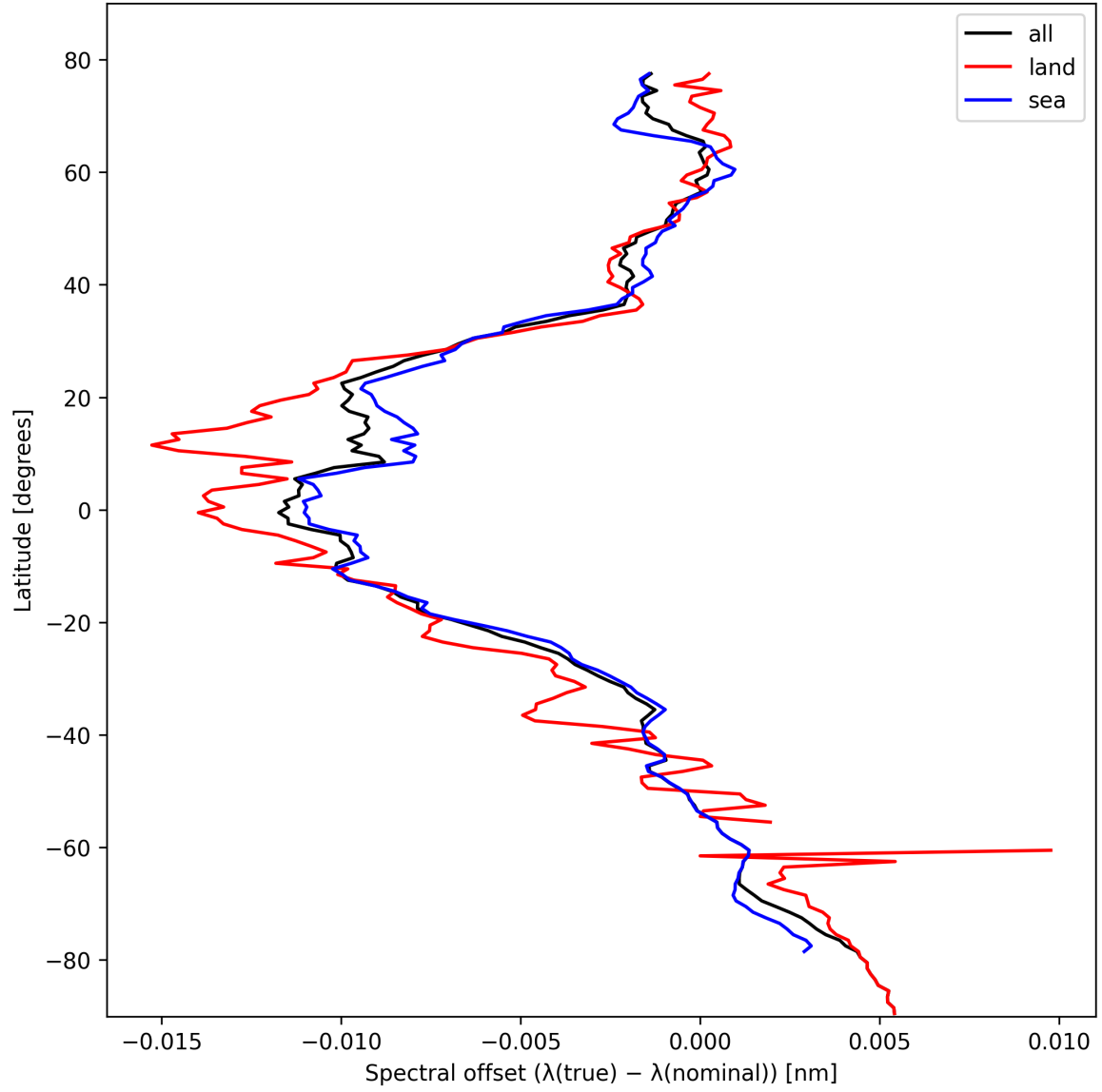
Figure 28: Zonal average of “Spectral offset ( \lambda_{\text{true}} - \lambda_{\text{nominal}} )” for 2024-10-19 to 2024-10-21.
