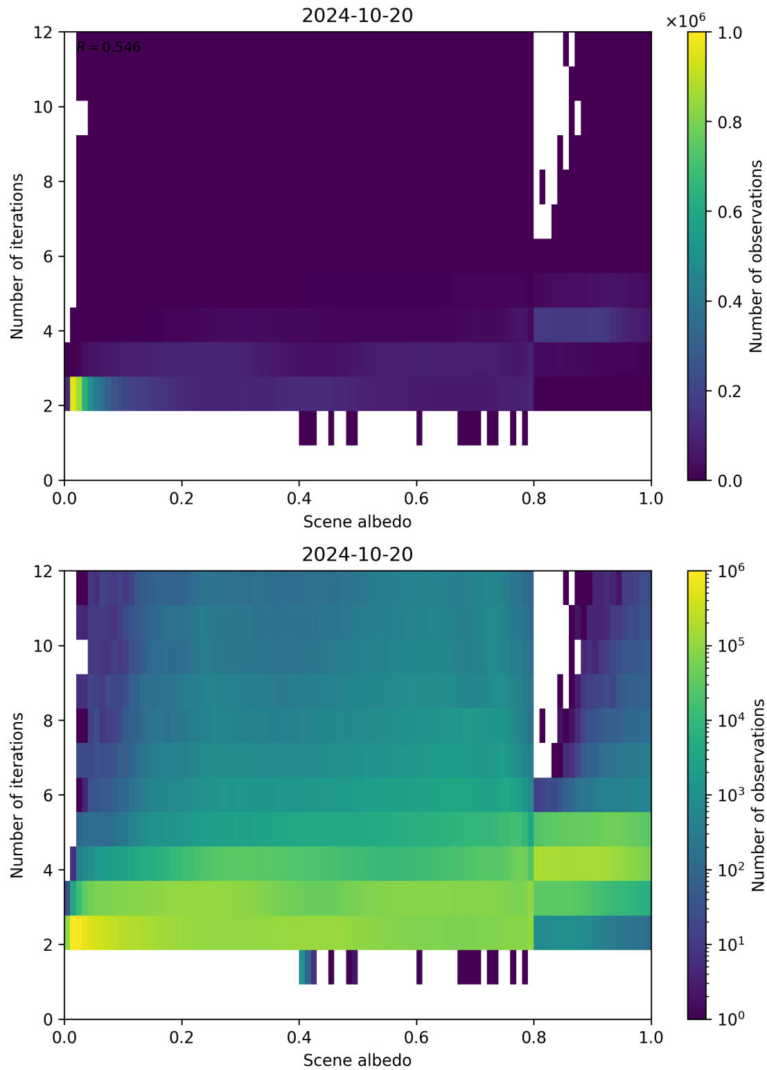
Figure 115: Scatter density plot of “Scene albedo” against “Number of iterations” for 2024-10-19 to 2024-10-21.
