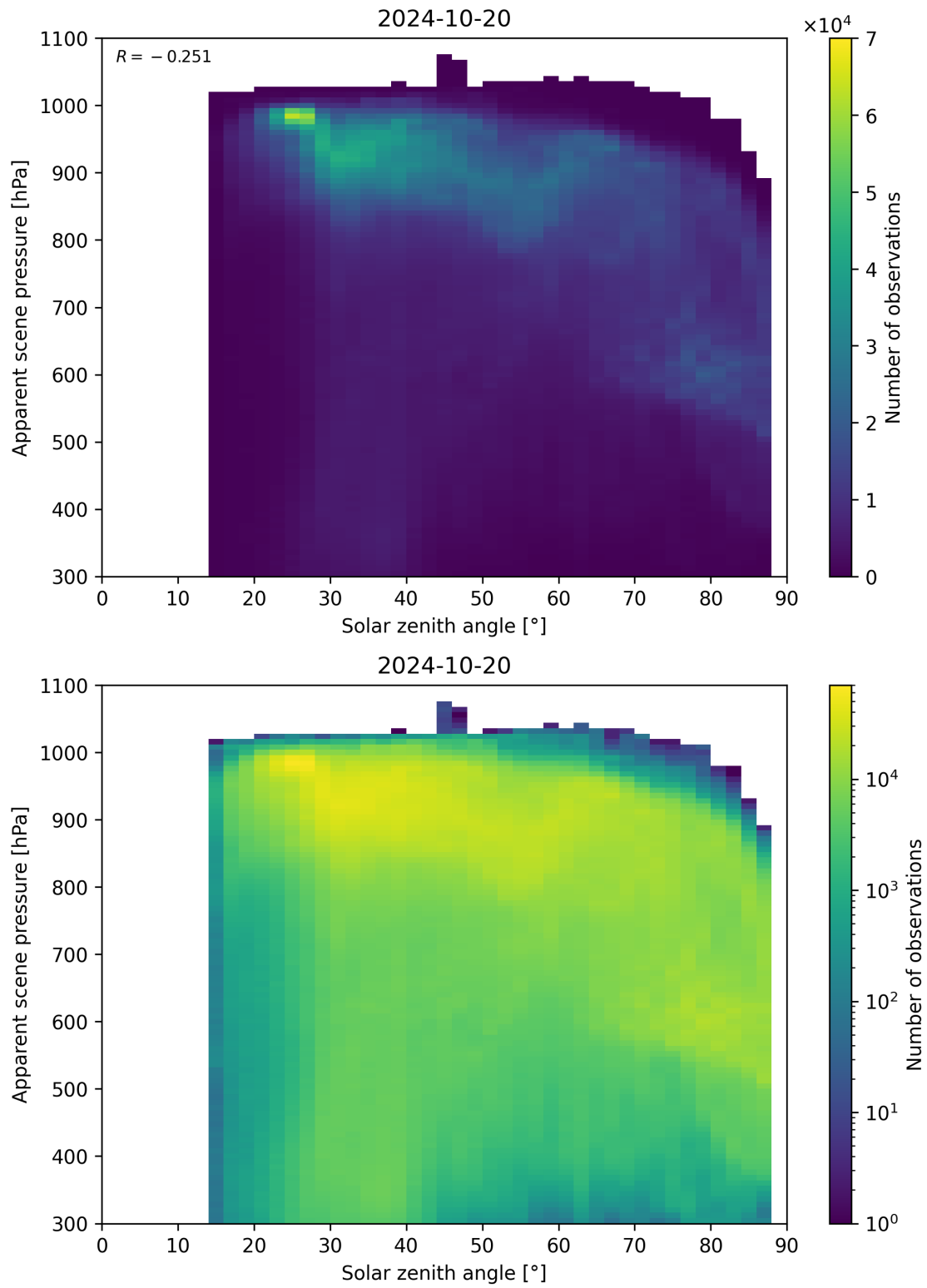
Figure 118: Scatter density plot of “Solar zenith angle” against “Apparent scene pressure” for 2024-10-19 to 2024-10-21.
