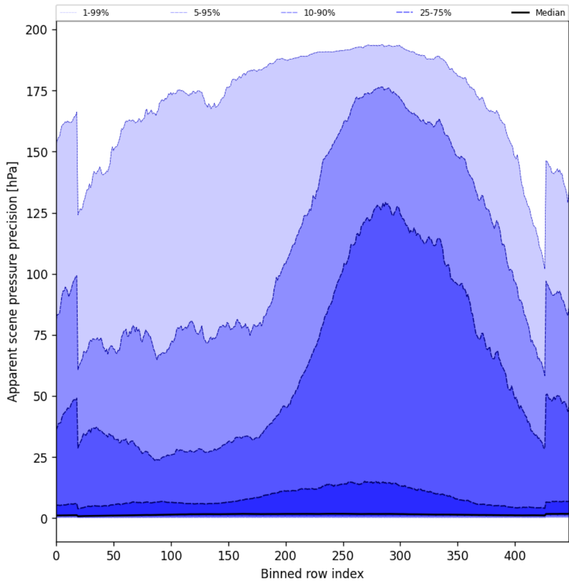
Figure 54: Along track statistics of “Apparent scene pressure precision” for 2024-10-19 to 2024-10-21
