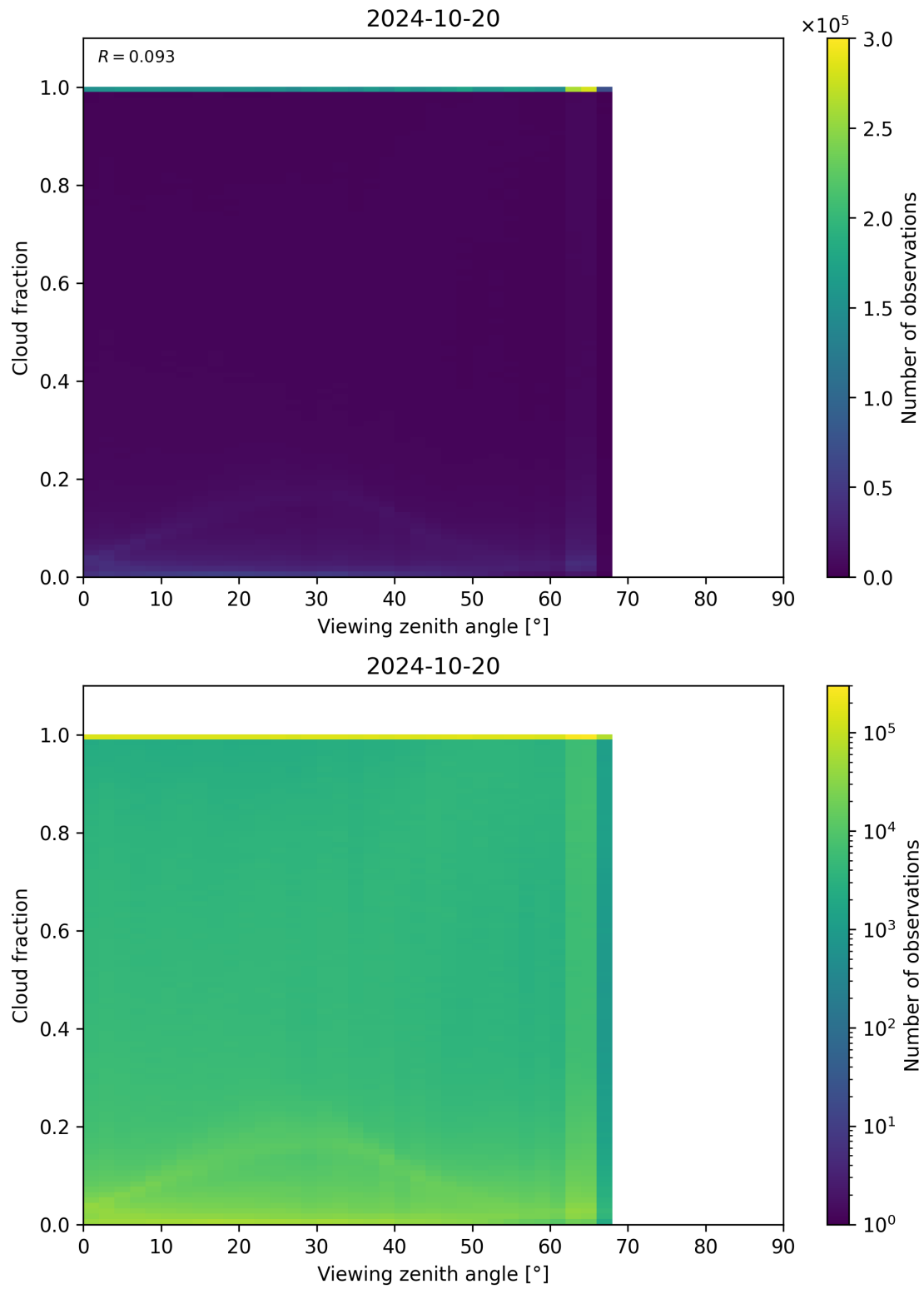
Figure 132: Scatter density plot of “Viewing zenith angle” against “Cloud fraction” for 2024-10-19 to 2024-10-21.
