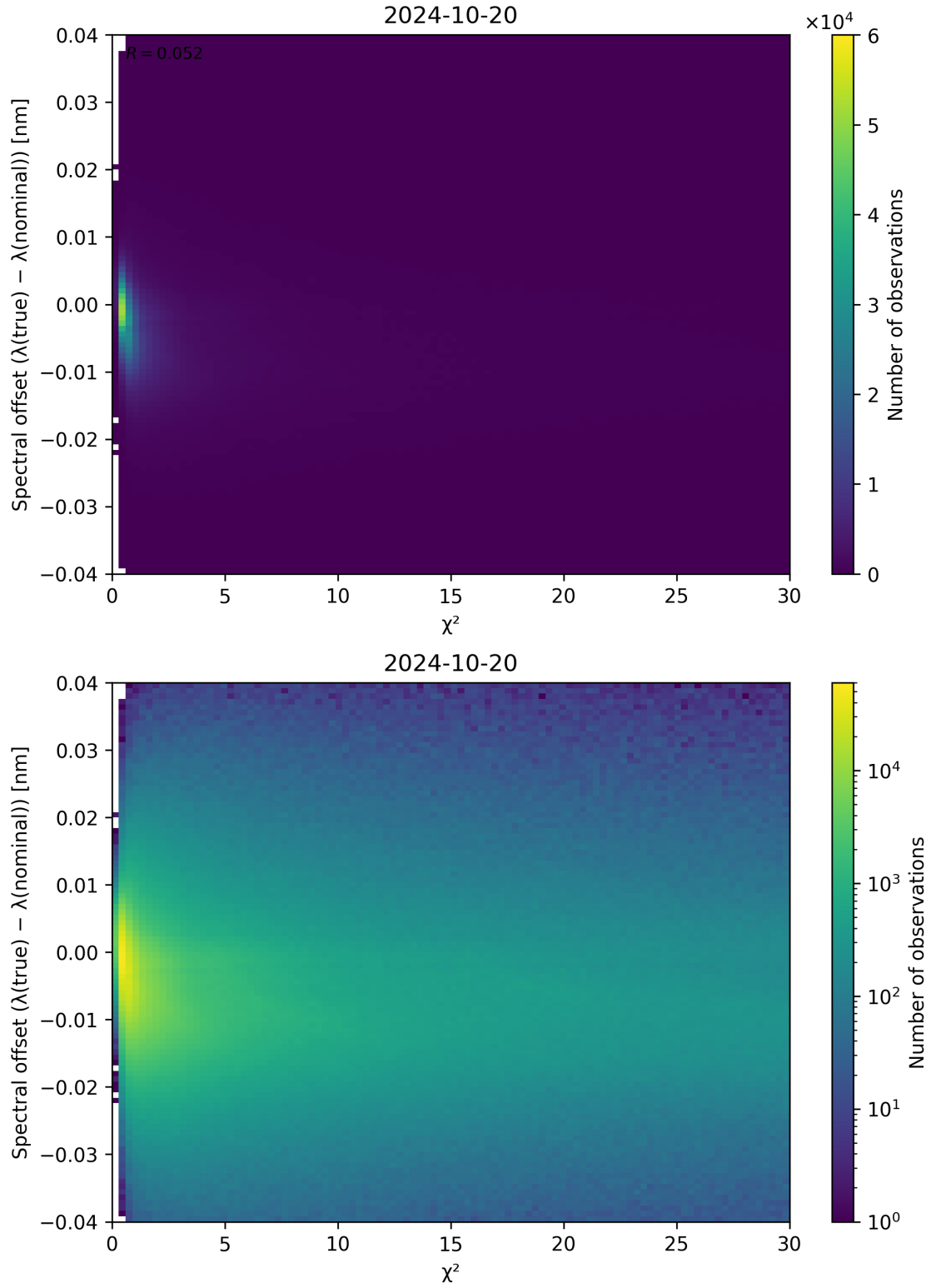
Figure 75: Scatter density plot of “ \chi^2 ” against “Spectral offset ( \lambda_{\text{true}} - \lambda_{\text{nominal}} )” for 2024-10-19 to 2024-10-21.
