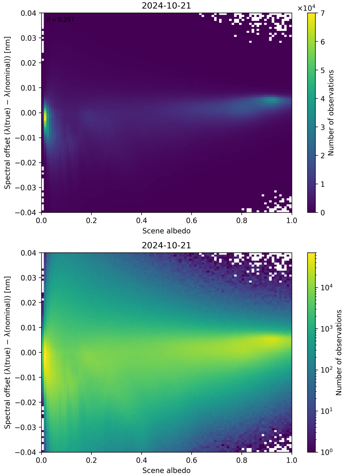
Figure 117: Scatter density plot of “Scene albedo” against “Spectral offset ( \lambda_{\text{true}} - \lambda_{\text{nominal}} )” for 2024-10-20 to 2024-10-22.
