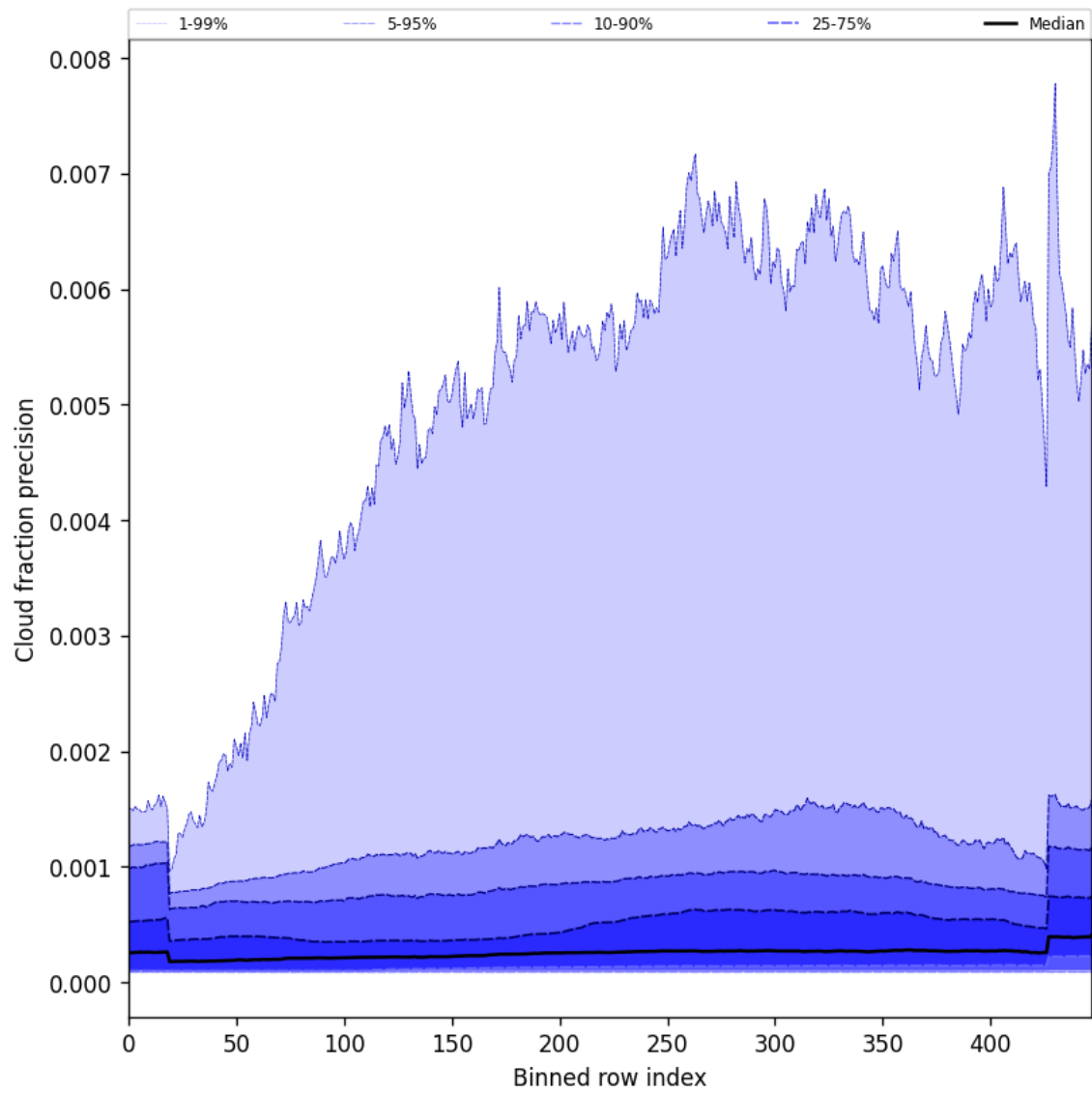
Figure 50: Along track statistics of “Cloud fraction precision” for 2024-10-20 to 2024-10-22
