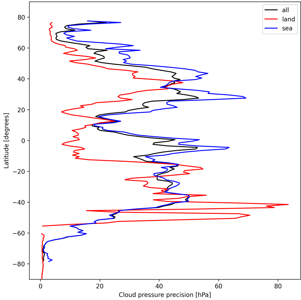
Figure 14: Zonal average of “Cloud pressure precision” for 2024-10-20 to 2024-10-22.
