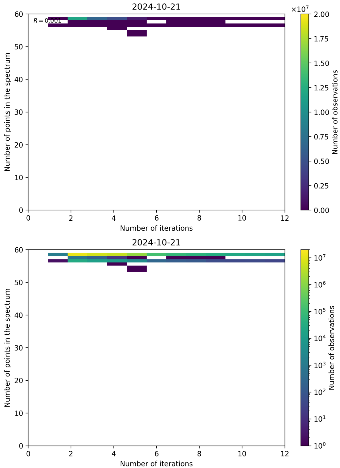
Figure 108: Scatter density plot of “Number of iterations” against “Number of points in the spectrum” for 2024-10-20 to 2024-10-22.
