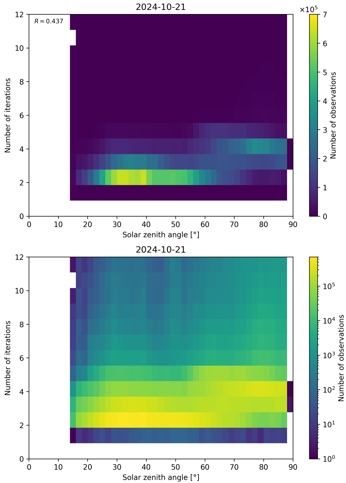
Figure 125: Scatter density plot of “Solar zenith angle” against “Number of iterations” for 2024-10-20 to 2024-10-22.
