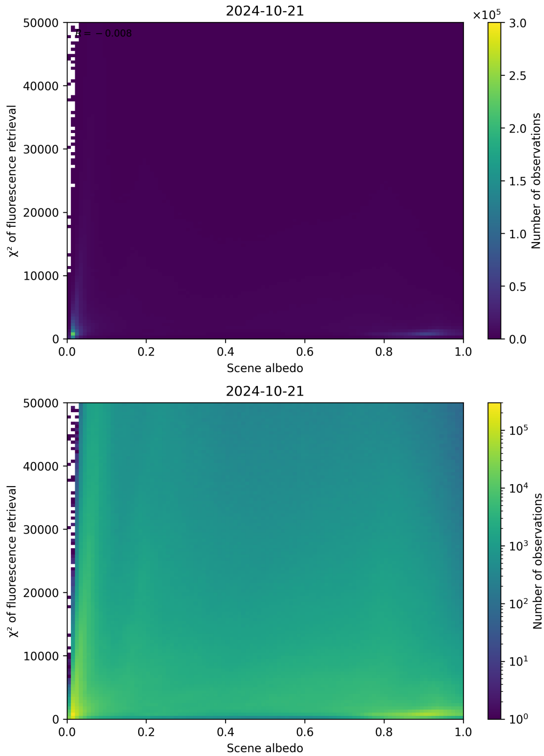
Figure 113: Scatter density plot of “Scene albedo” against “ \chi^2 of fluorescence retrieval” for 2024-10-20 to 2024-10-22.
