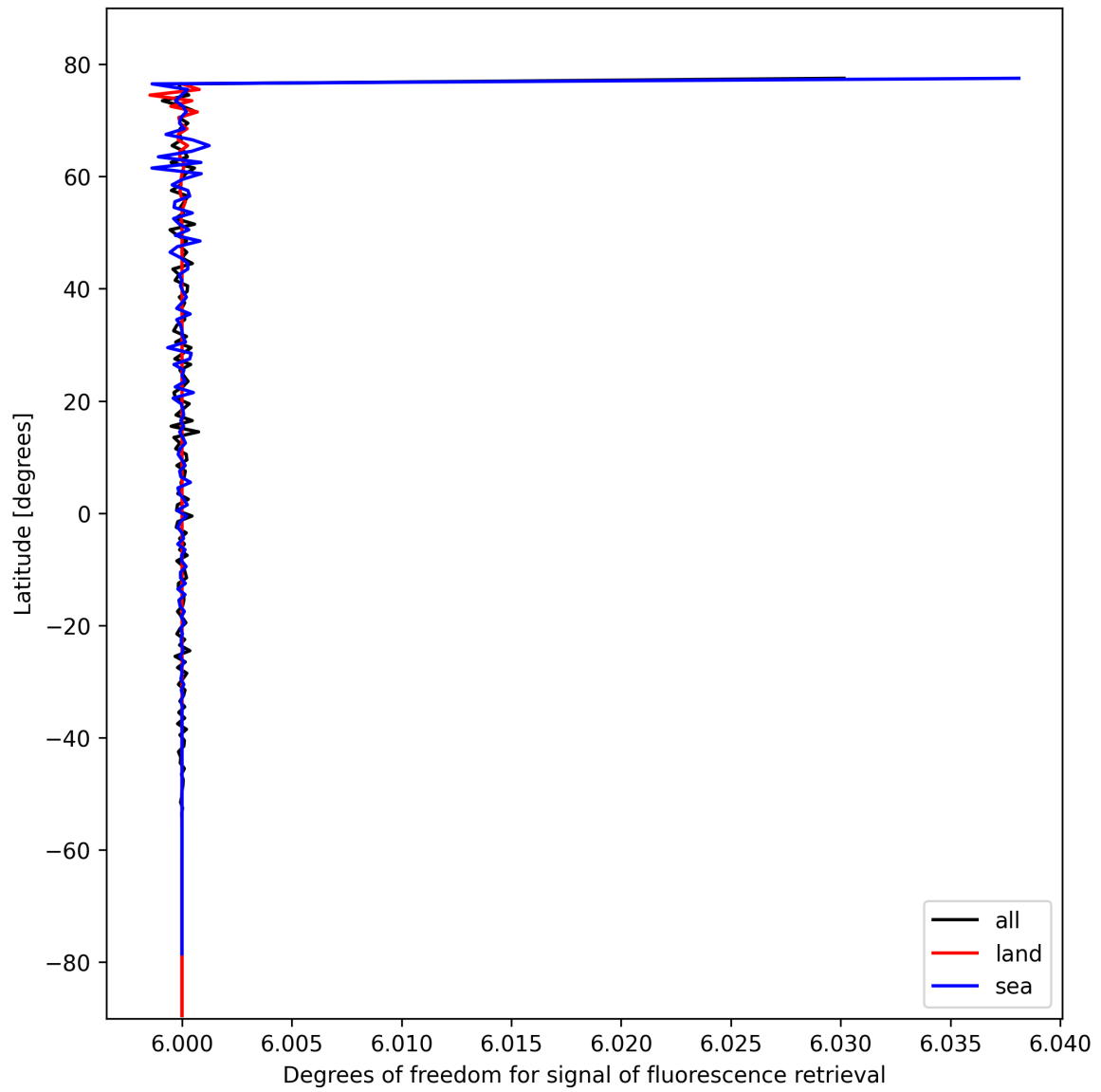
Figure 26: Zonal average of “Degrees of freedom for signal of fluorescence retrieval” for 2024-10-20 to 2024-10-22.
