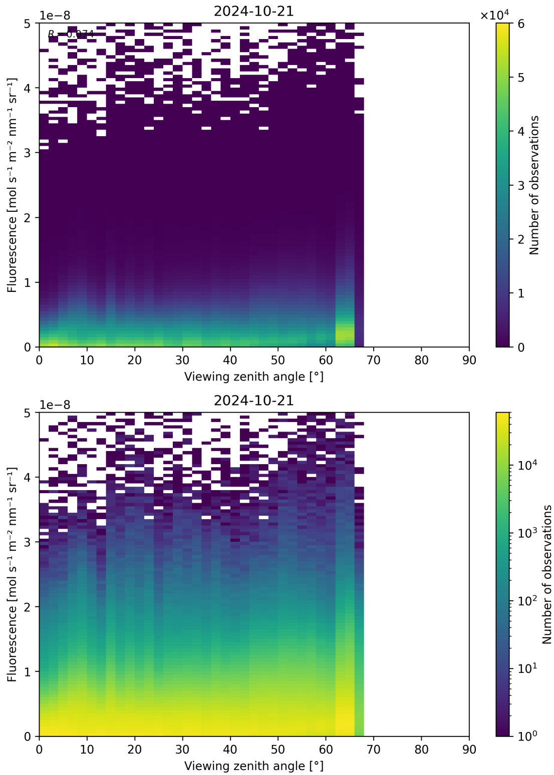
Figure 134: Scatter density plot of “Viewing zenith angle” against “Fluorescence” for 2024-10-20 to 2024-10-22.
