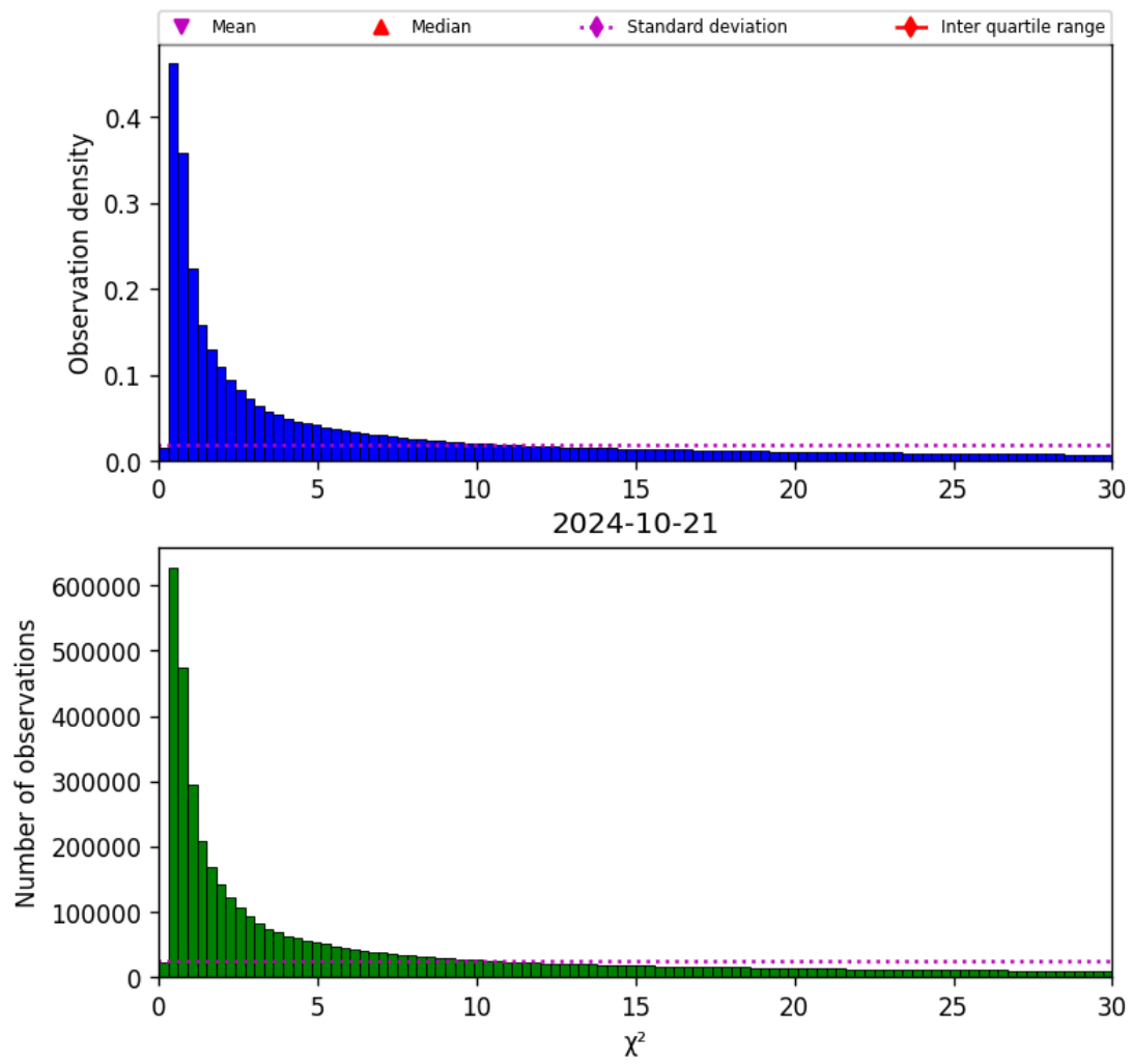
Figure 38: Histogram of " \chi^2 " for 2024-10-20 to 2024-10-22
