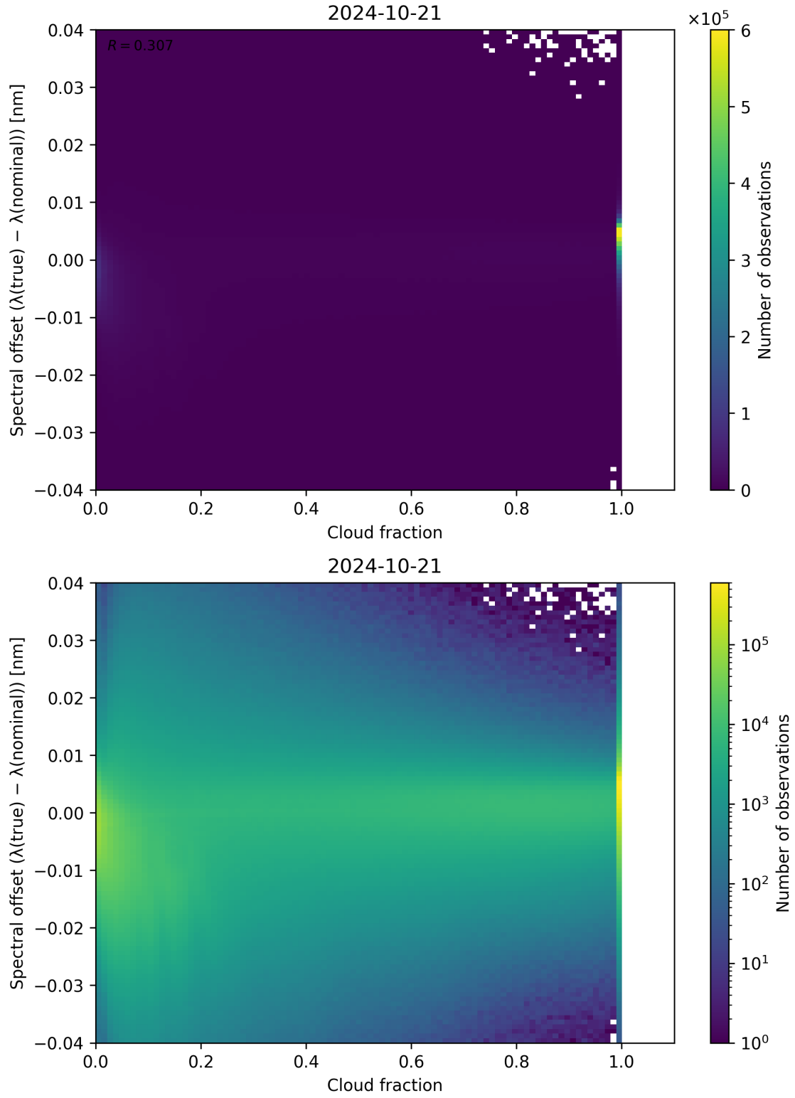
Figure 83: Scatter density plot of “Cloud fraction” against “Spectral offset ( \lambda_{\text{true}} - \lambda_{\text{nominal}} )” for 2024-10-20 to 2024-10-22.
