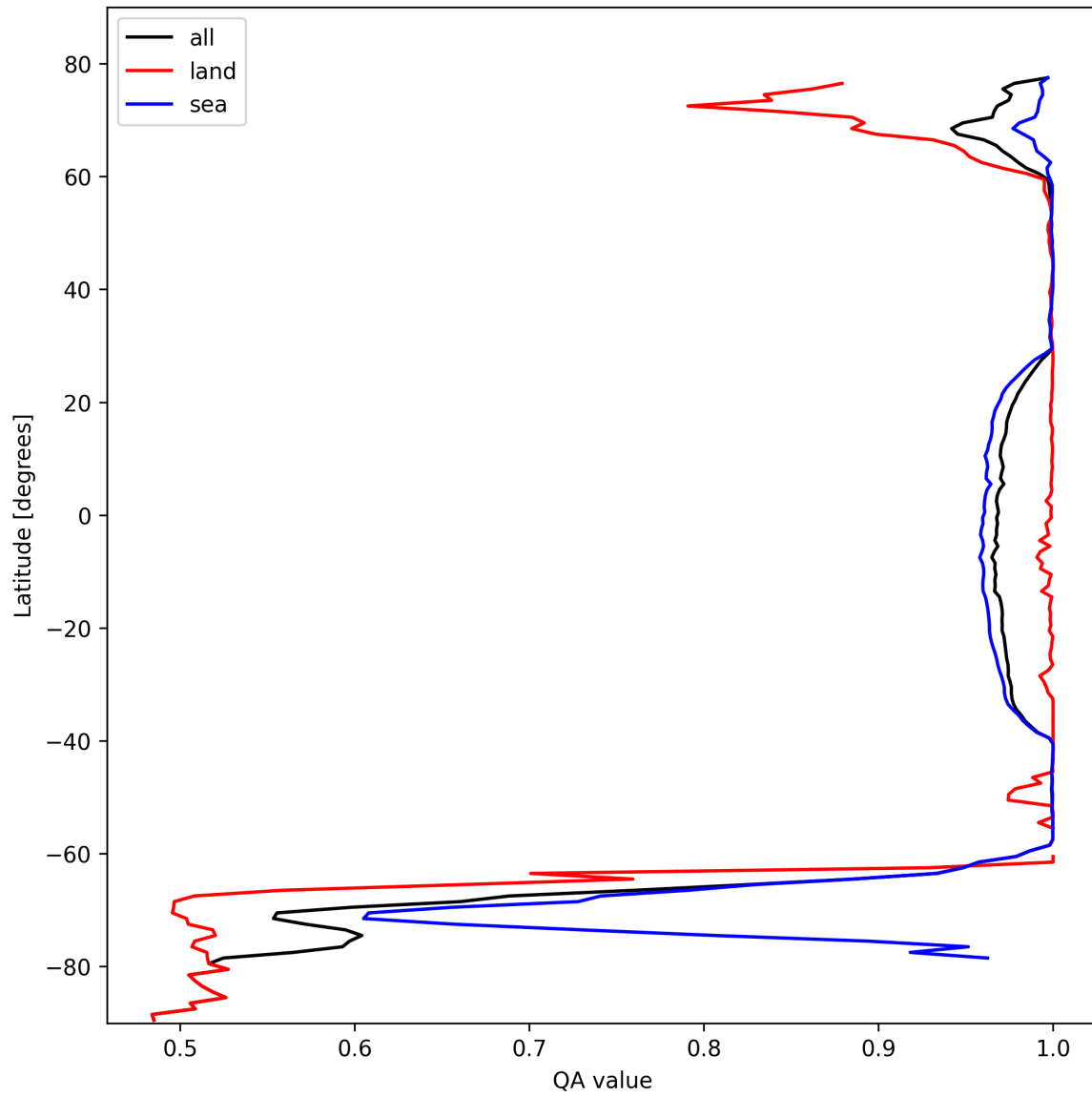
Figure 12: Zonal average of “QA value” for 2024-10-20 to 2024-10-22.
