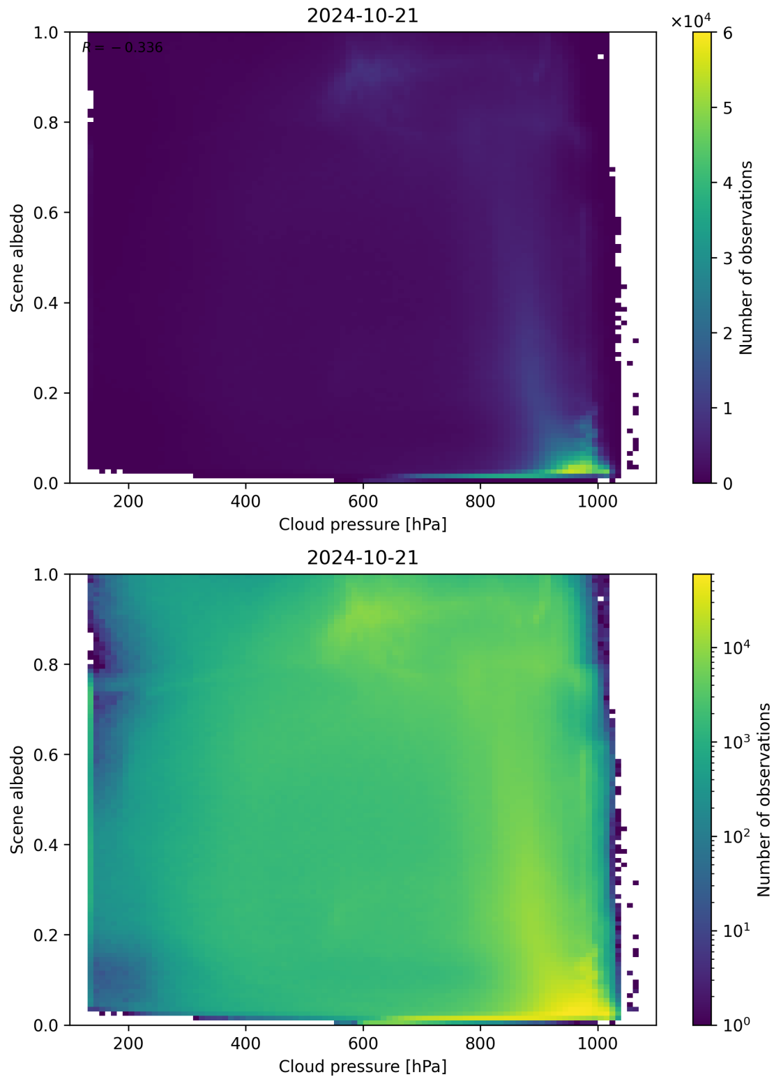
Figure 91: Scatter density plot of “Cloud pressure” against “Scene albedo” for 2024-10-20 to 2024-10-22.
