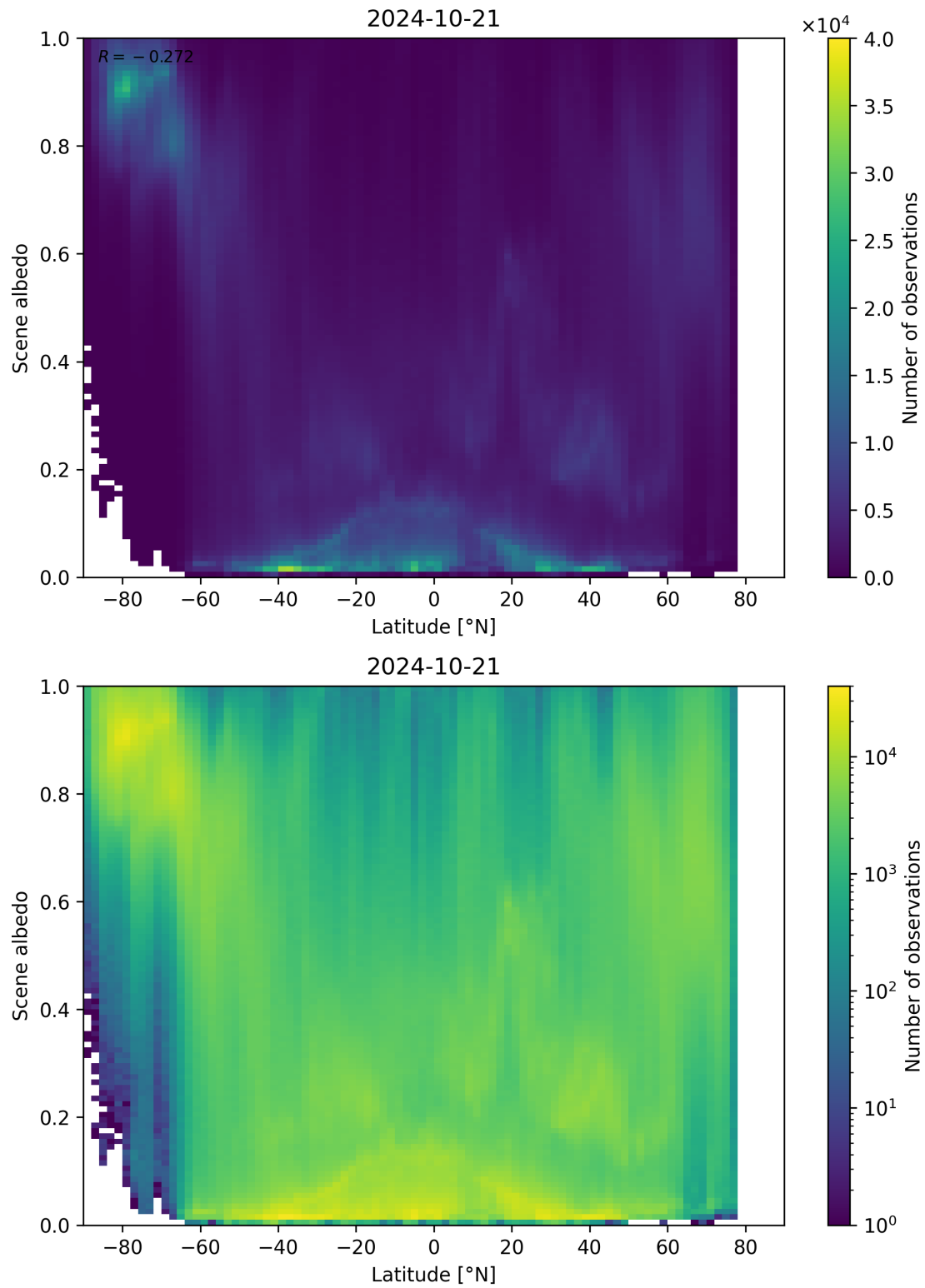
Figure 104: Scatter density plot of “Latitude” against “Scene albedo” for 2024-10-20 to 2024-10-22.
