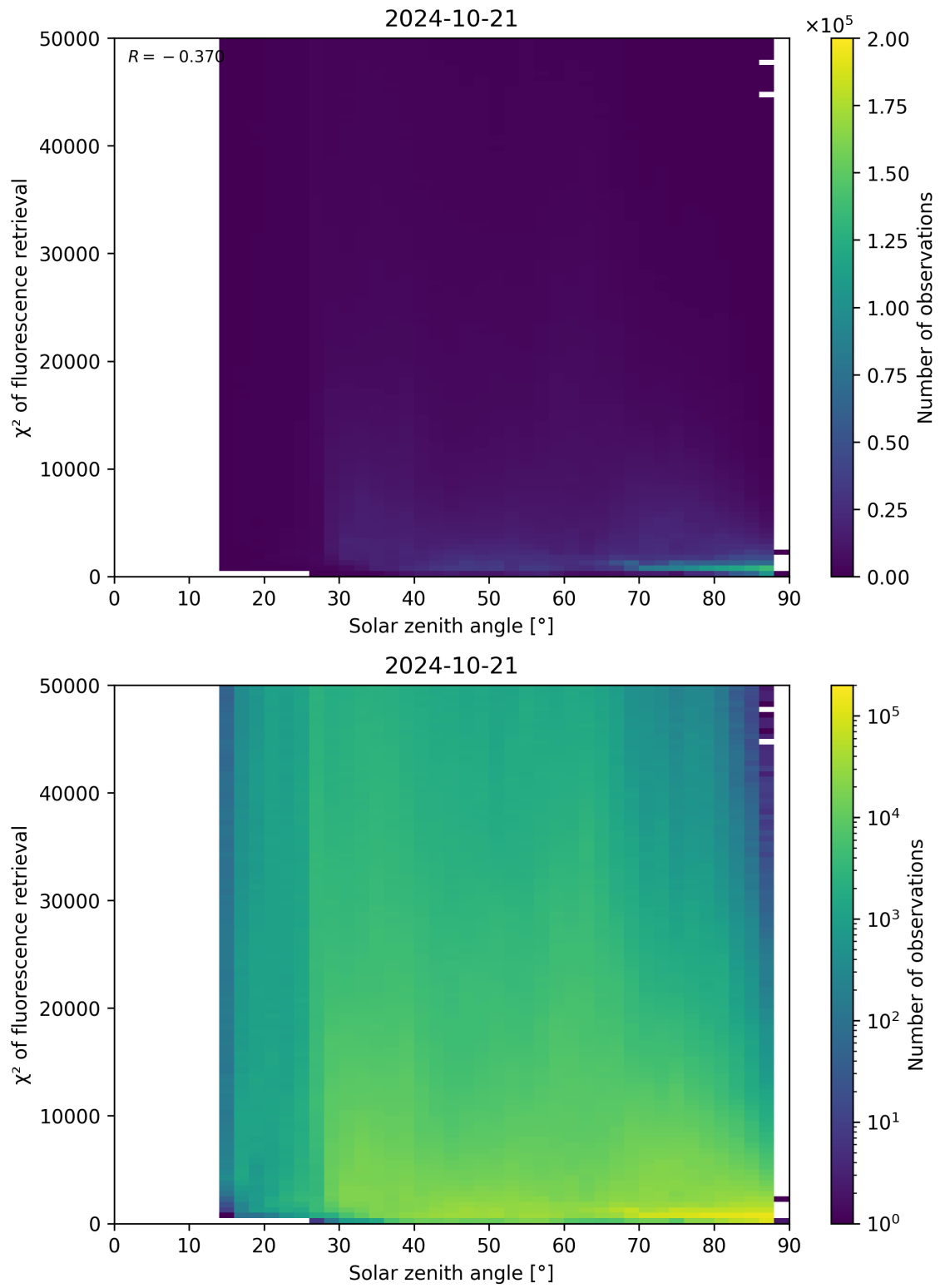
Figure 120: Scatter density plot of “Solar zenith angle” against “ \chi^2 of fluorescence retrieval” for 2024-10-20 to 2024-10-22.
