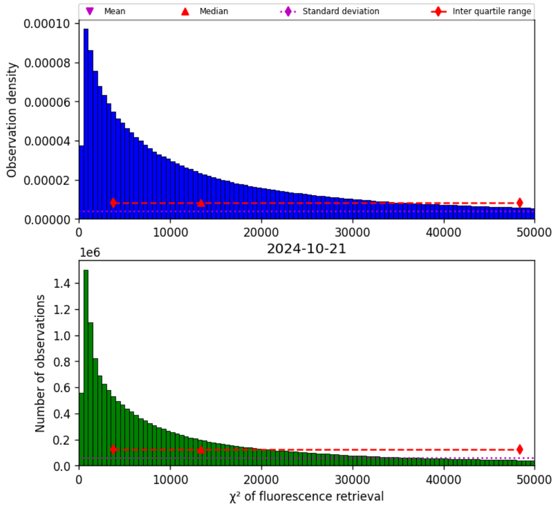
Figure 42: Histogram of “ \chi^2 of fluorescence retrieval” for 2024-10-20 to 2024-10-22
