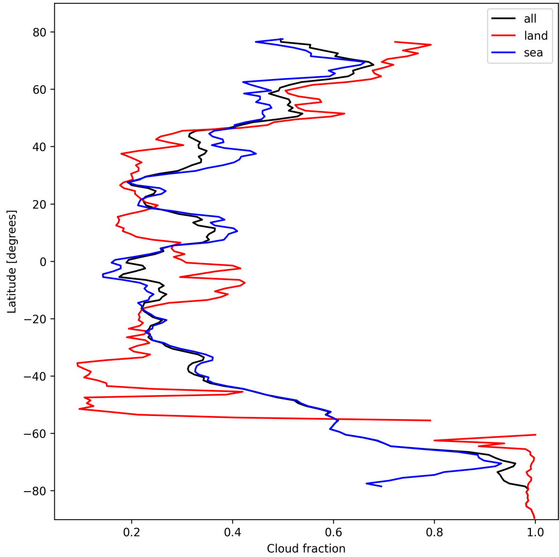
Figure 15: Zonal average of “Cloud fraction” for 2024-10-20 to 2024-10-22.
