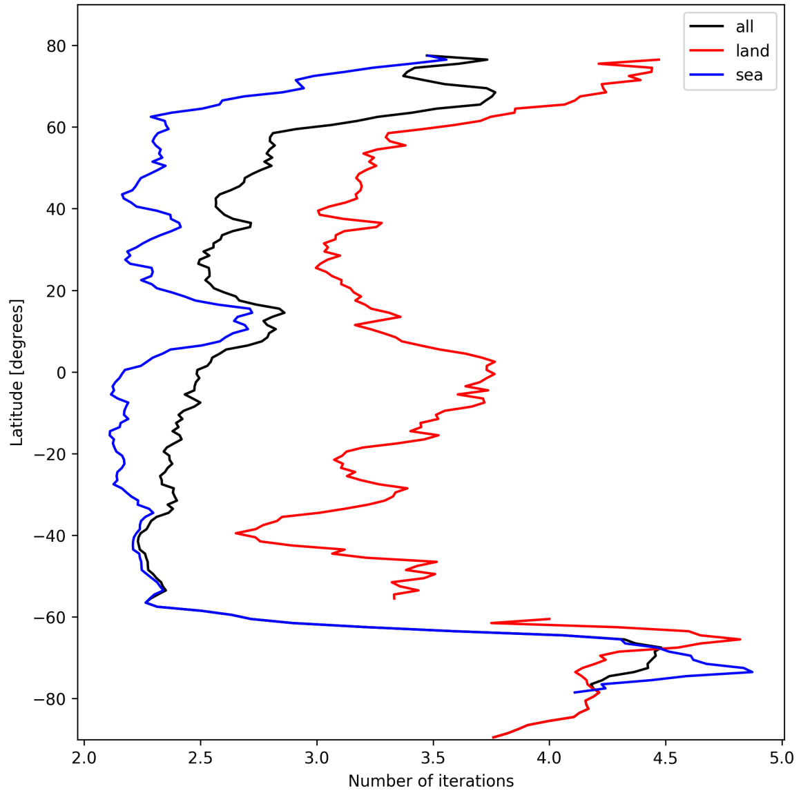
Figure 22: Zonal average of “Number of iterations” for 2024-10-20 to 2024-10-22.
