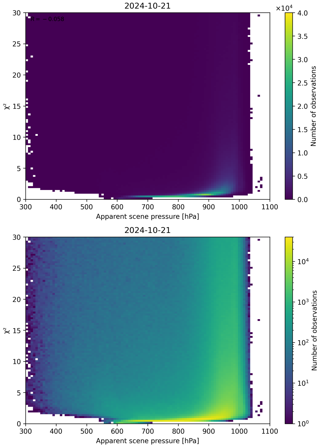
Figure 63: Scatter density plot of “Apparent scene pressure” against “ \chi^2 ” for 2024-10-20 to 2024-10-22.
