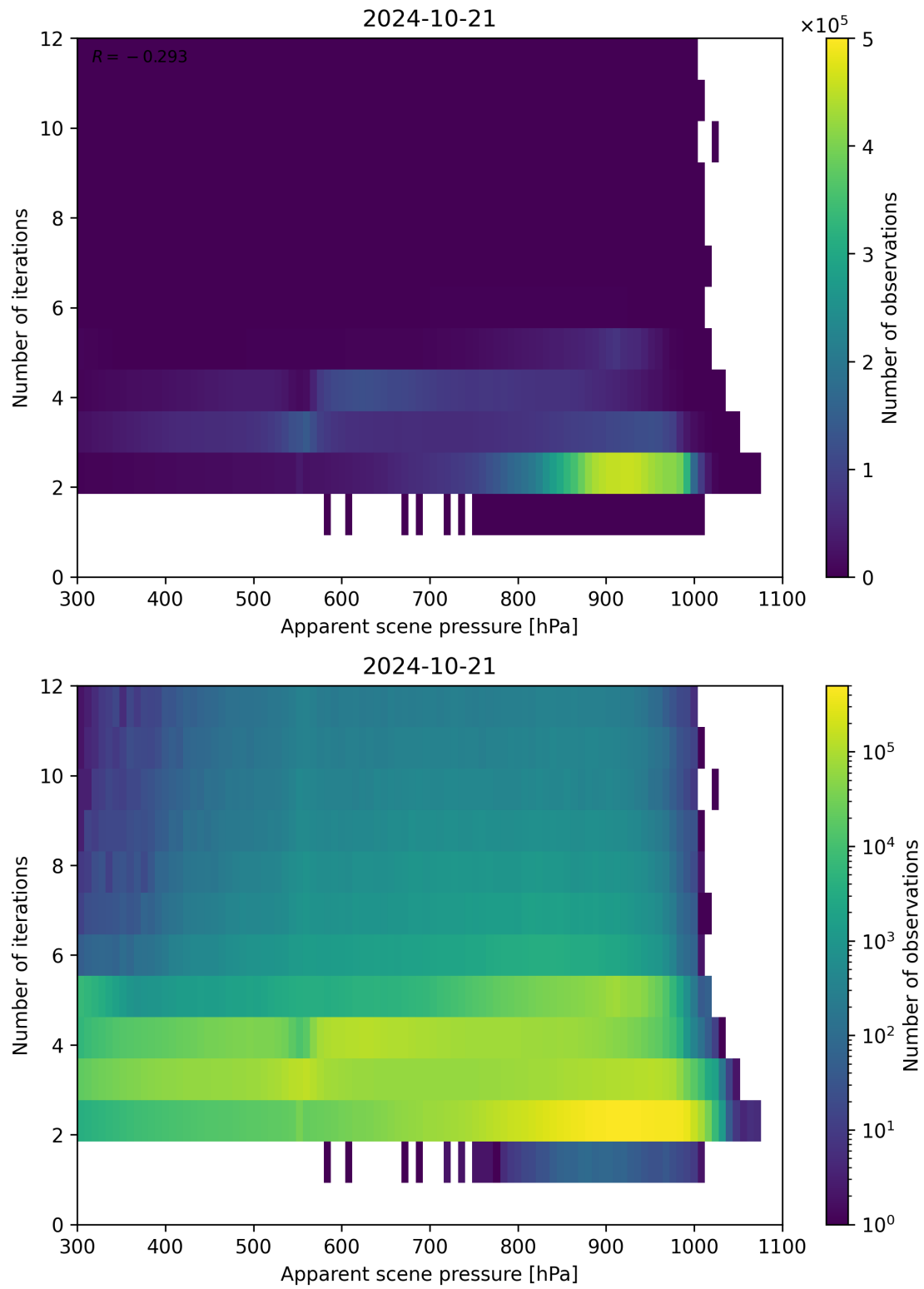
Figure 66: Scatter density plot of “Apparent scene pressure” against “Number of iterations” for 2024-10-20 to 2024-10-22.
