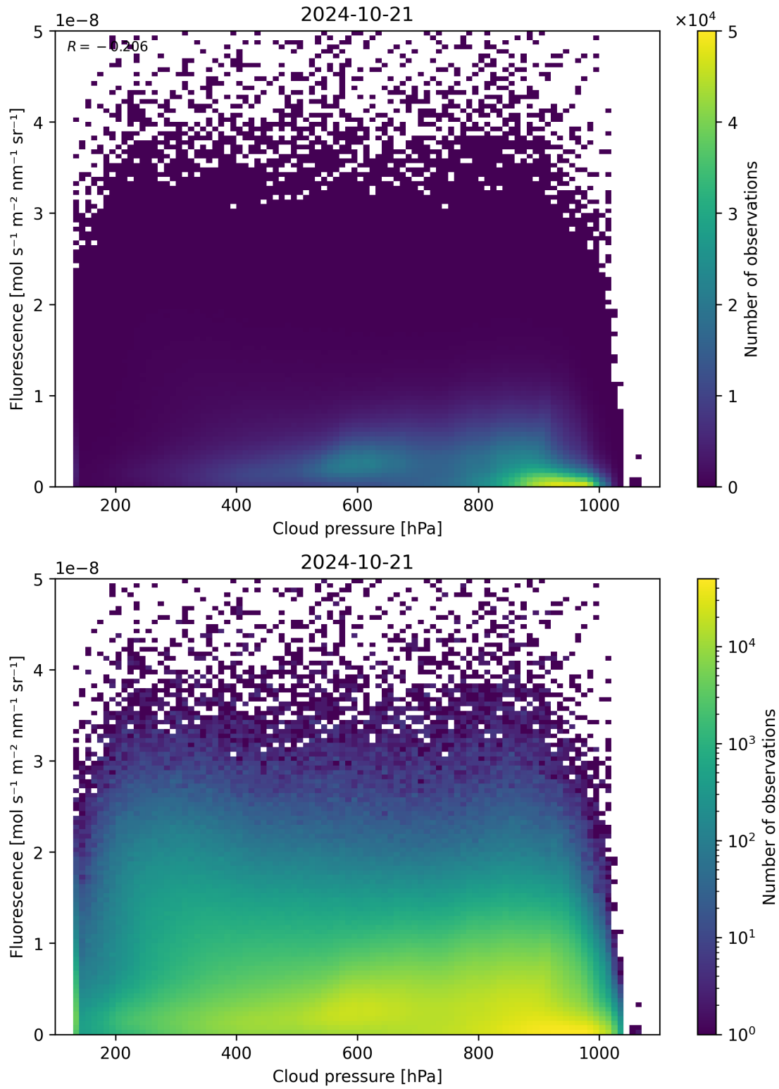
Figure 88: Scatter density plot of “Cloud pressure” against “Fluorescence” for 2024-10-20 to 2024-10-22.
