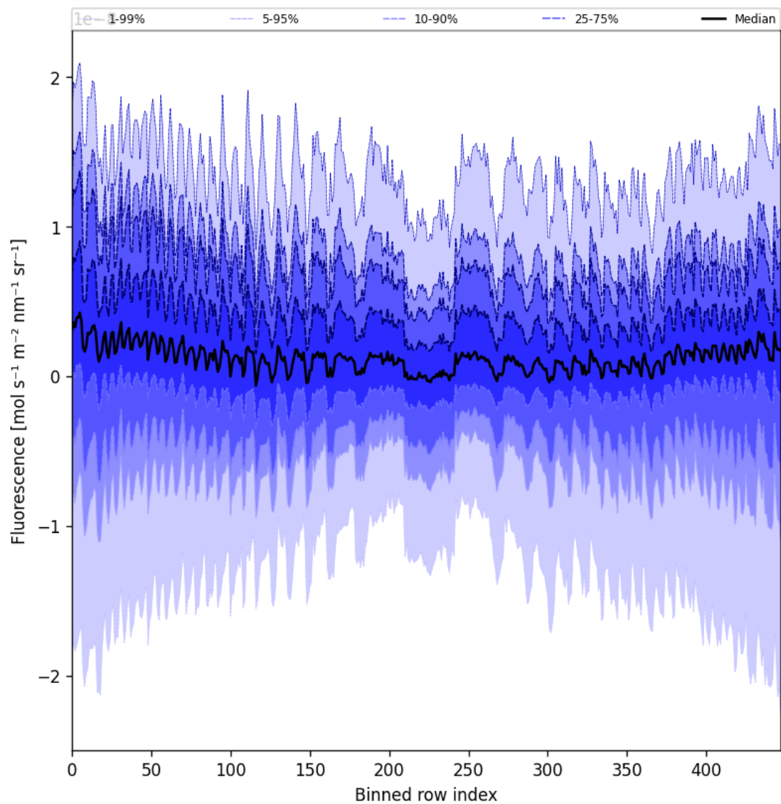
Figure 57: Along track statistics of “Fluorescence” for 2024-10-20 to 2024-10-22
