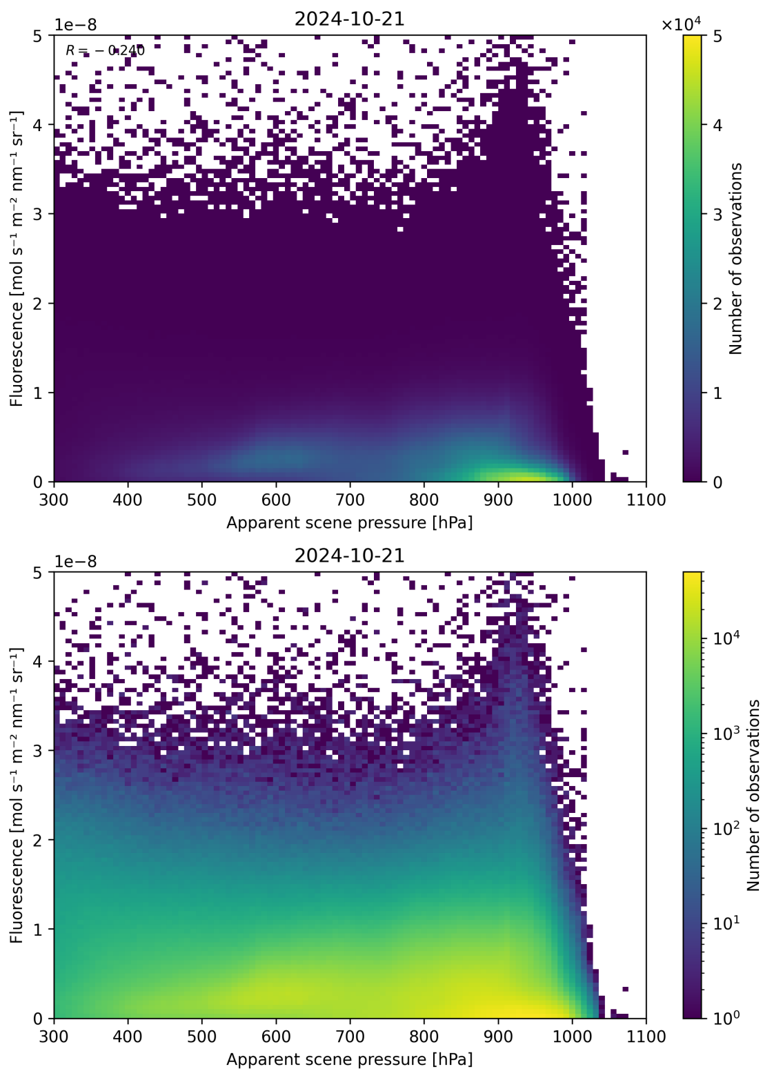
Figure 65: Scatter density plot of “Apparent scene pressure” against “Fluorescence” for 2024-10-20 to 2024-10-22.
