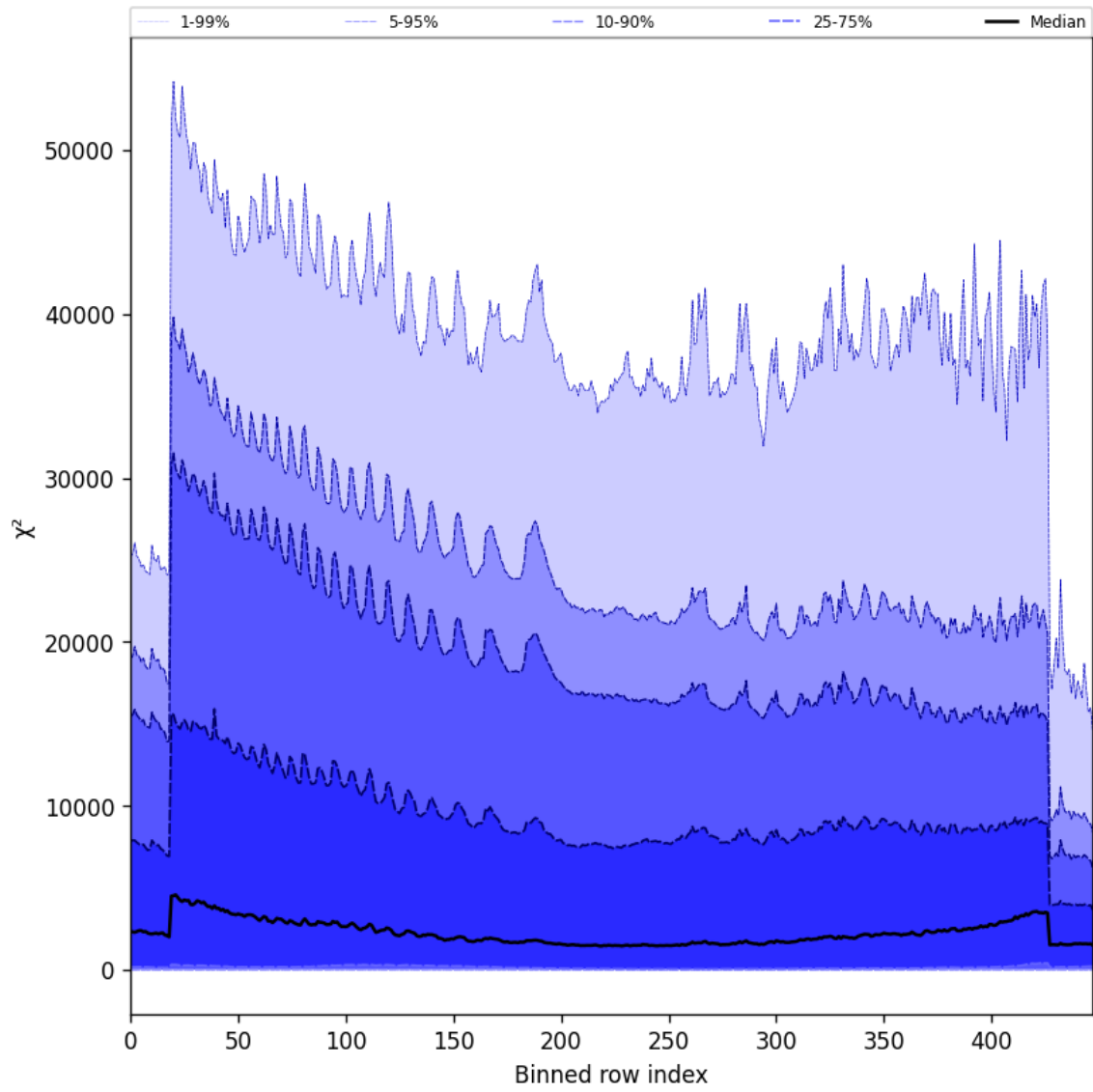
Figure 55: Along track statistics of “ \chi^2 ” for 2024-10-20 to 2024-10-22
