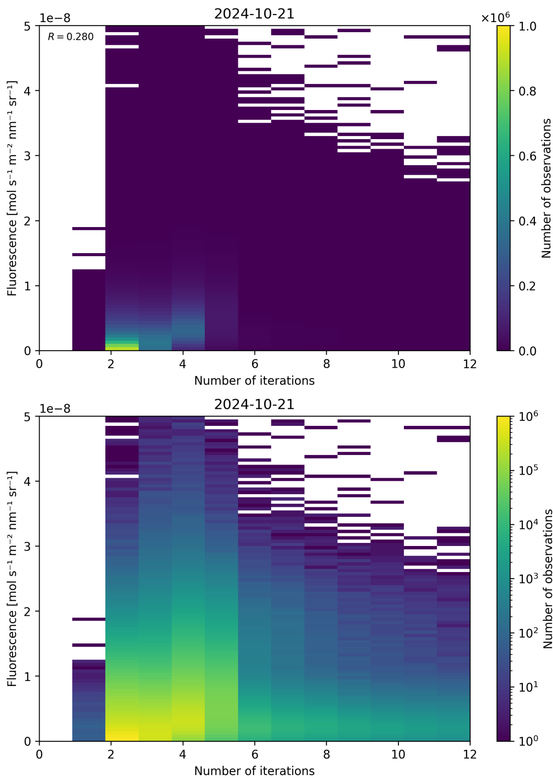
Figure 107: Scatter density plot of “Number of iterations” against “Fluorescence” for 2024-10-20 to 2024-10-22.
