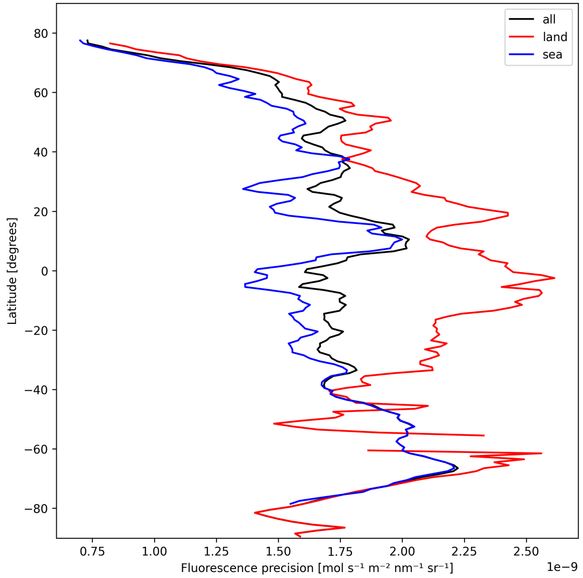
Figure 24: Zonal average of “Fluorescence precision” for 2024-10-20 to 2024-10-22.
