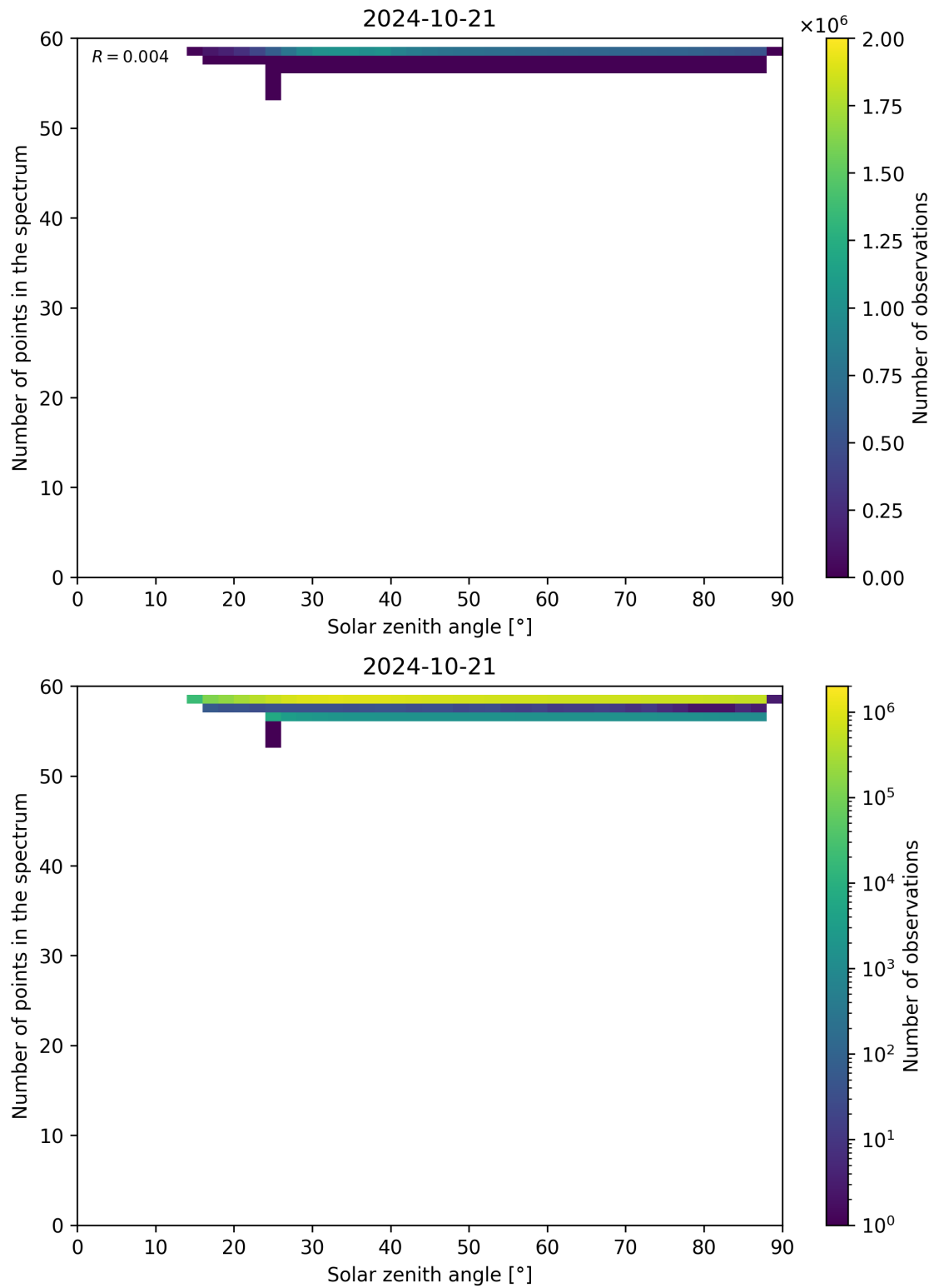
Figure 126: Scatter density plot of “Solar zenith angle” against “Number of points in the spectrum” for 2024-10-20 to 2024-10-22.
