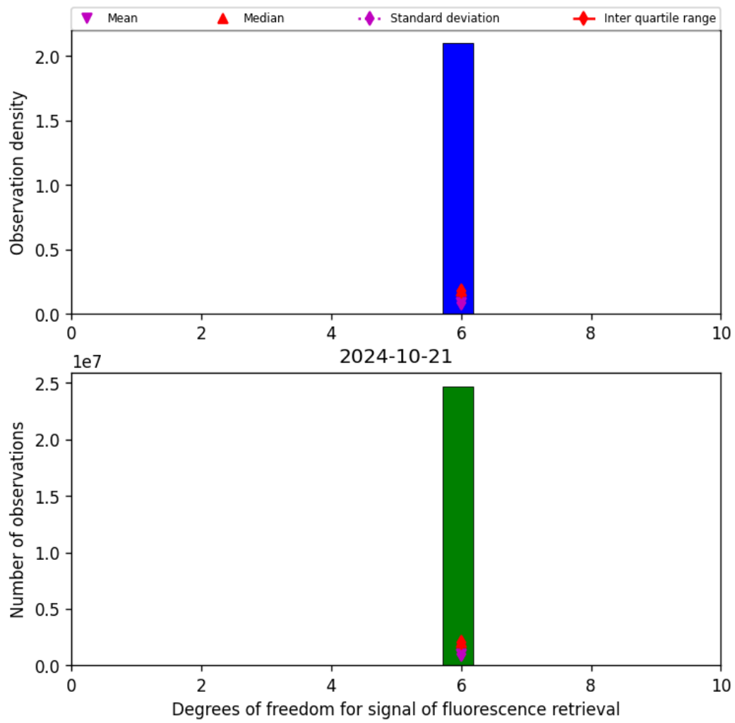
Figure 43: Histogram of “Degrees of freedom for signal of fluorescence retrieval” for 2024-10-20 to 2024-10-22
