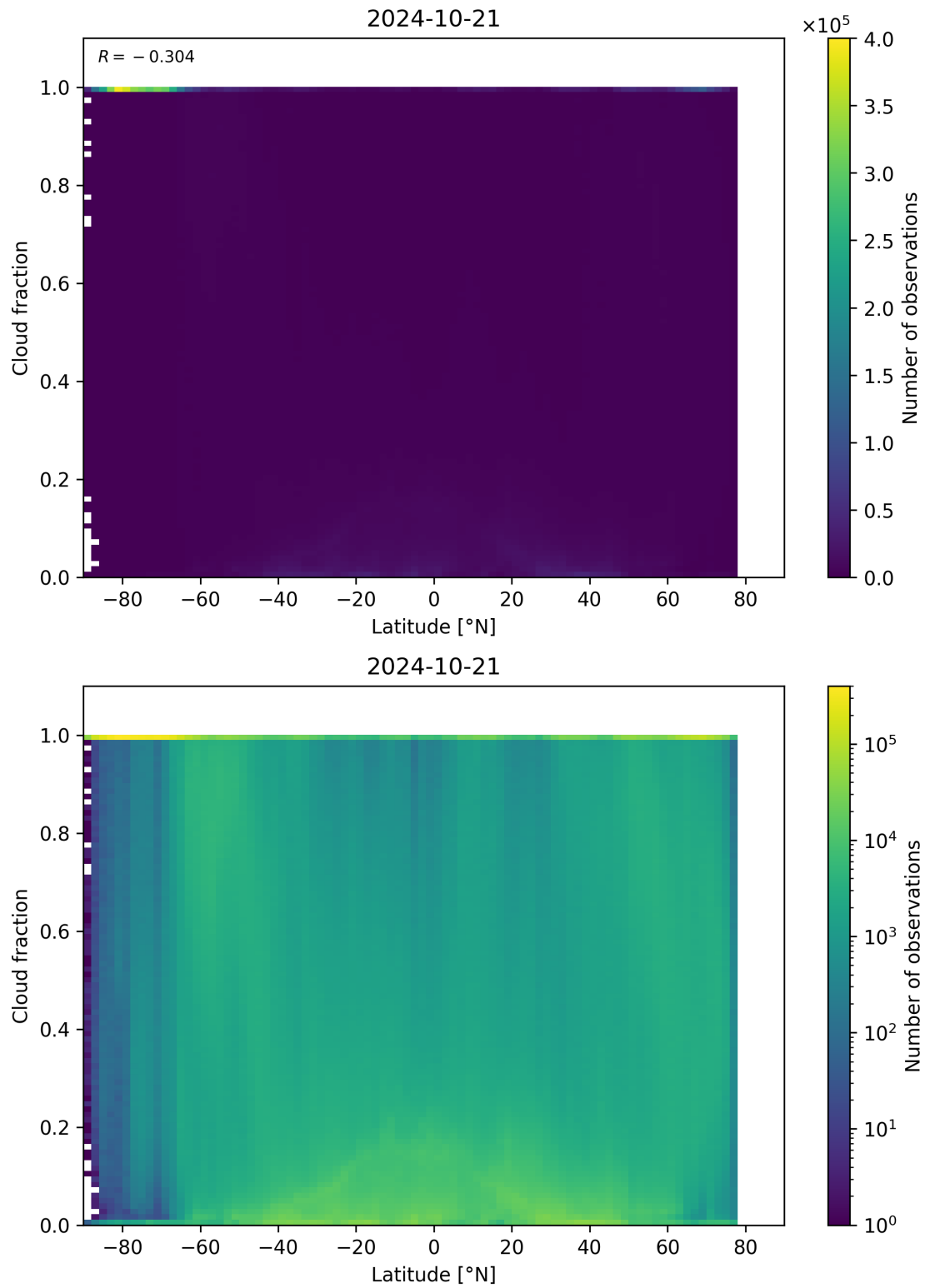
Figure 99: Scatter density plot of “Latitude” against “Cloud fraction” for 2024-10-20 to 2024-10-22.
