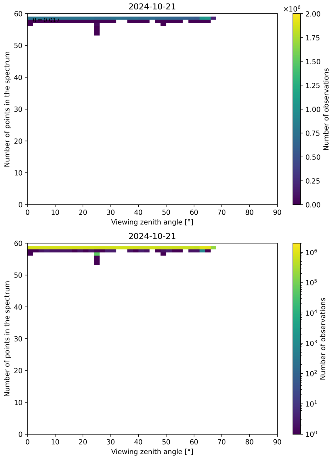
Figure 137: Scatter density plot of “Viewing zenith angle” against “Number of points in the spectrum” for 2024-10-20 to 2024-10-22.
