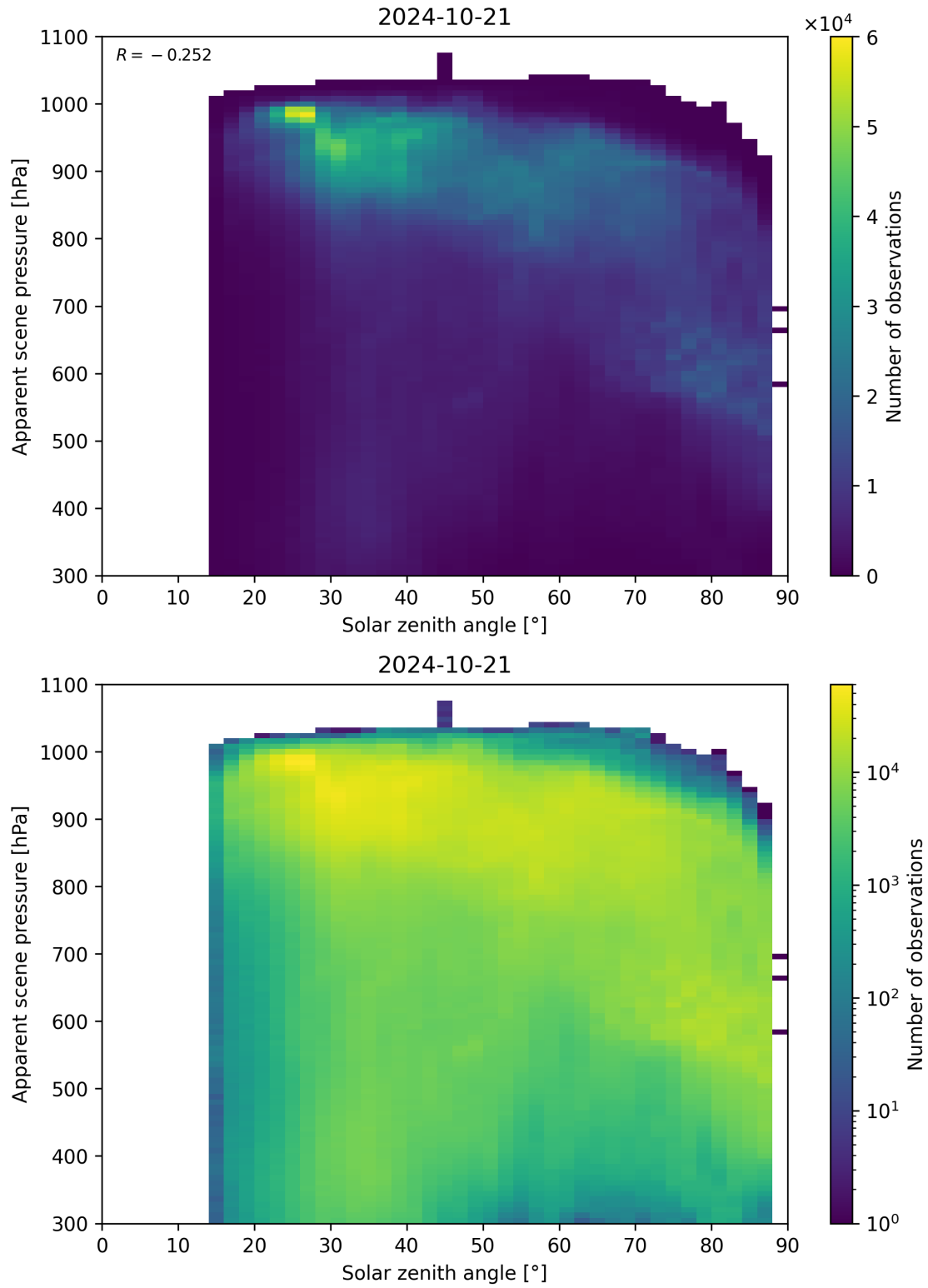
Figure 118: Scatter density plot of “Solar zenith angle” against “Apparent scene pressure” for 2024-10-20 to 2024-10-22.
