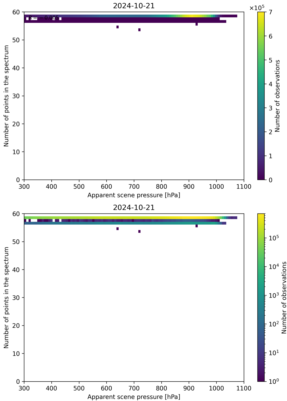
Figure 67: Scatter density plot of “Apparent scene pressure” against “Number of points in the spectrum” for 2024-10-20 to 2024-10-22.
