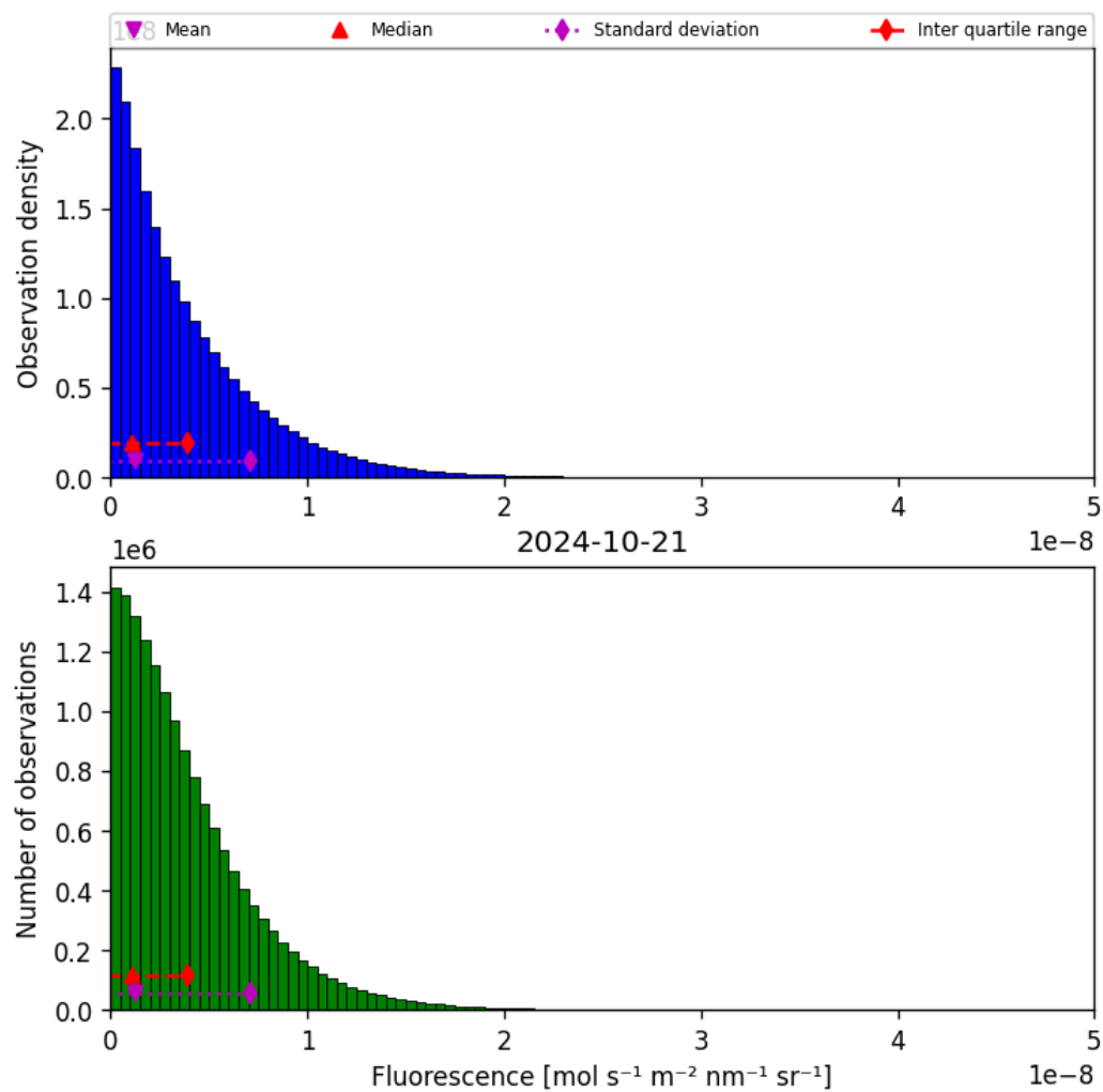
Figure 40: Histogram of “Fluorescence” for 2024-10-20 to 2024-10-22
