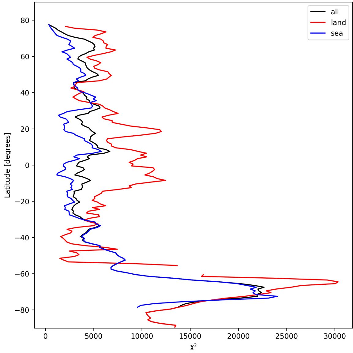
Figure 21: Zonal average of “ \chi^2 ” for 2024-10-20 to 2024-10-22.
