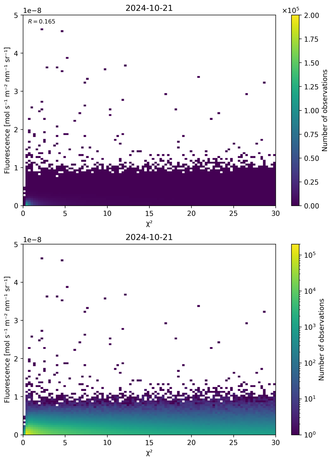
Figure 70: Scatter density plot of “ \chi^2 ” against “Fluorescence” for 2024-10-20 to 2024-10-22.
