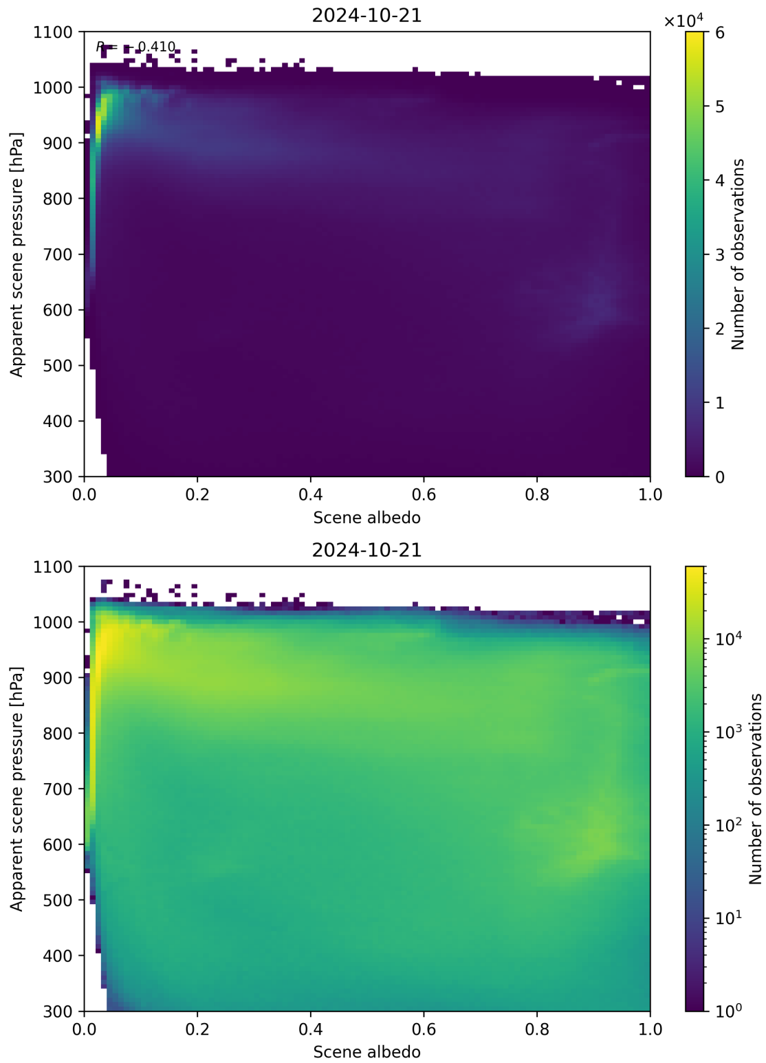
Figure 111: Scatter density plot of “Scene albedo” against “Apparent scene pressure” for 2024-10-20 to 2024-10-22.
