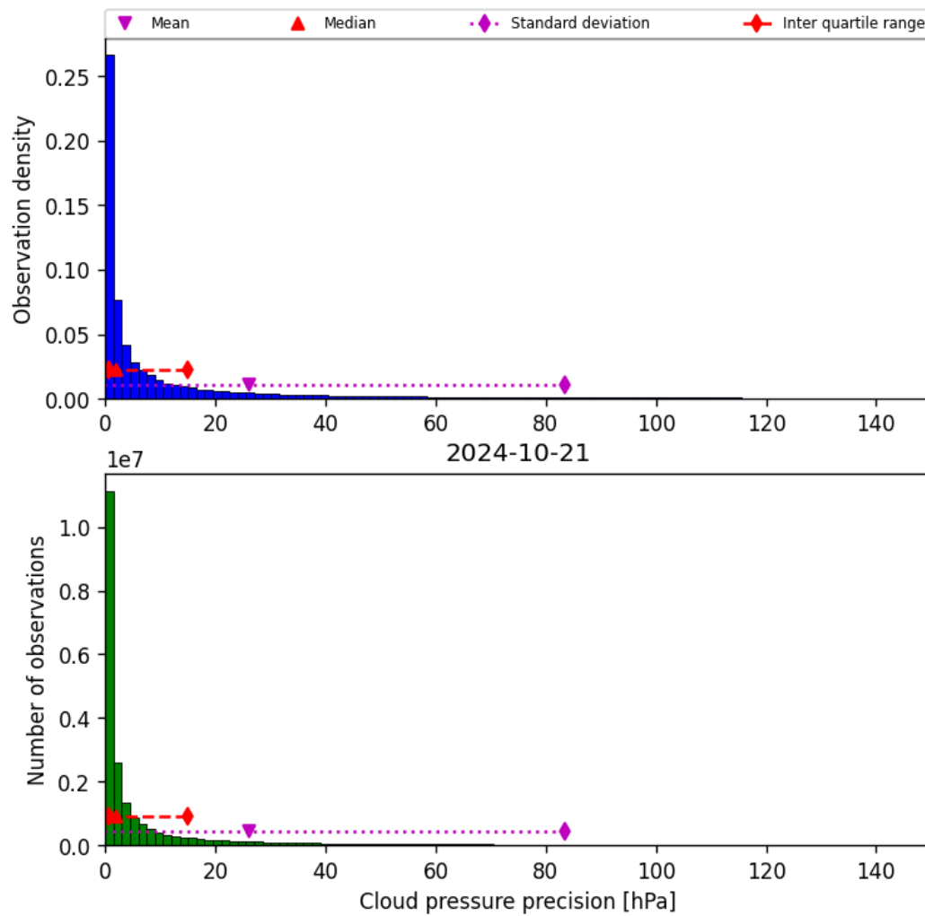
Figure 31: Histogram of “Cloud pressure precision” for 2024-10-20 to 2024-10-22
