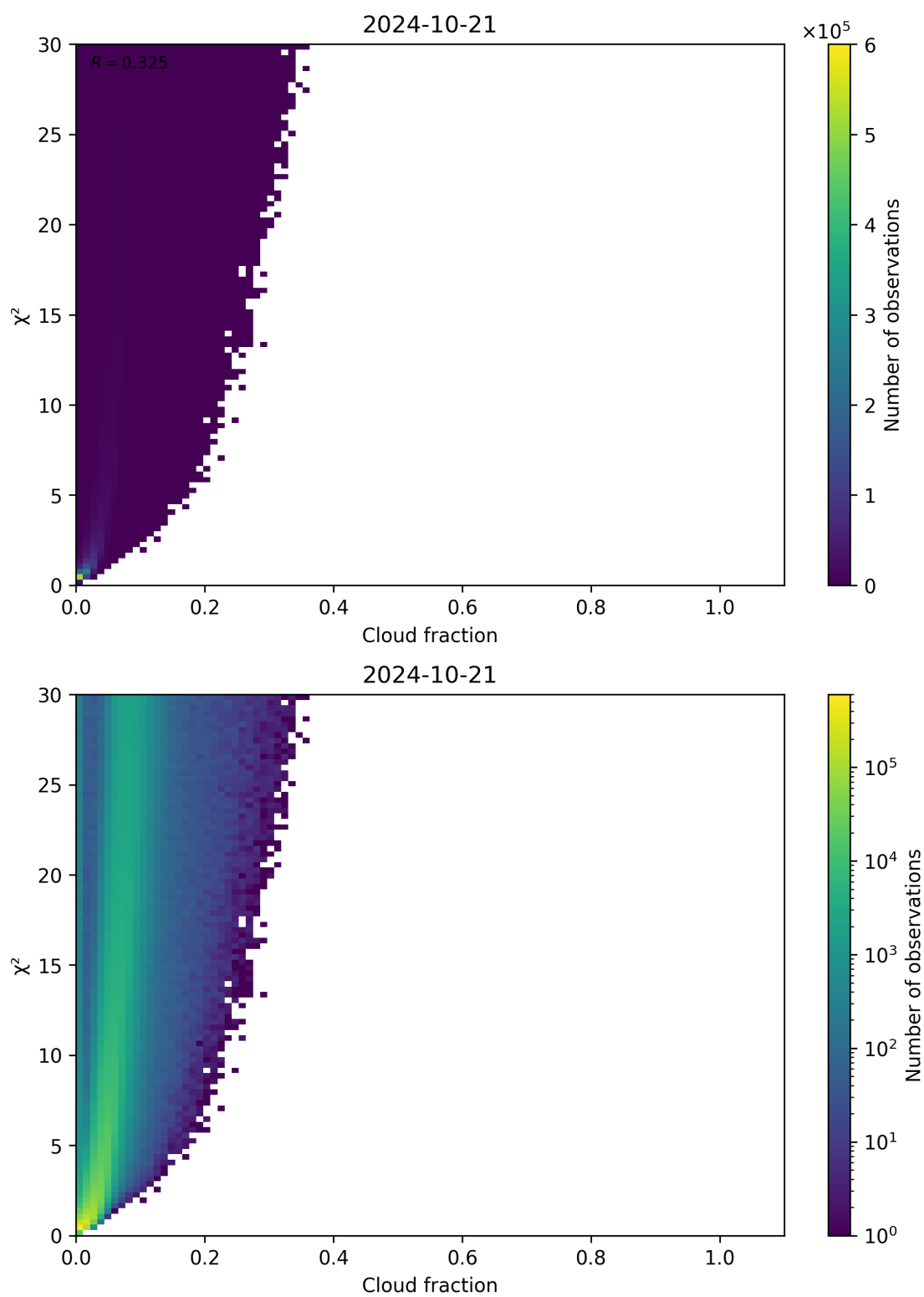
Figure 77: Scatter density plot of “Cloud fraction” against “ \chi^2 ” for 2024-10-20 to 2024-10-22.
