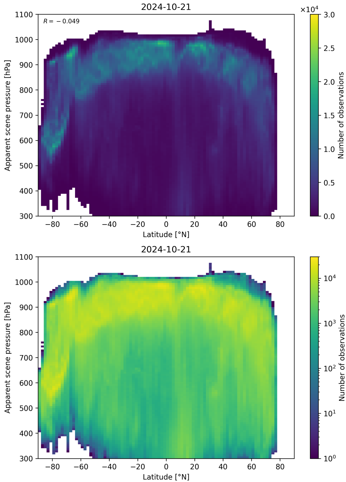
Figure 96: Scatter density plot of “Latitude” against “Apparent scene pressure” for 2024-10-20 to 2024-10-22.
