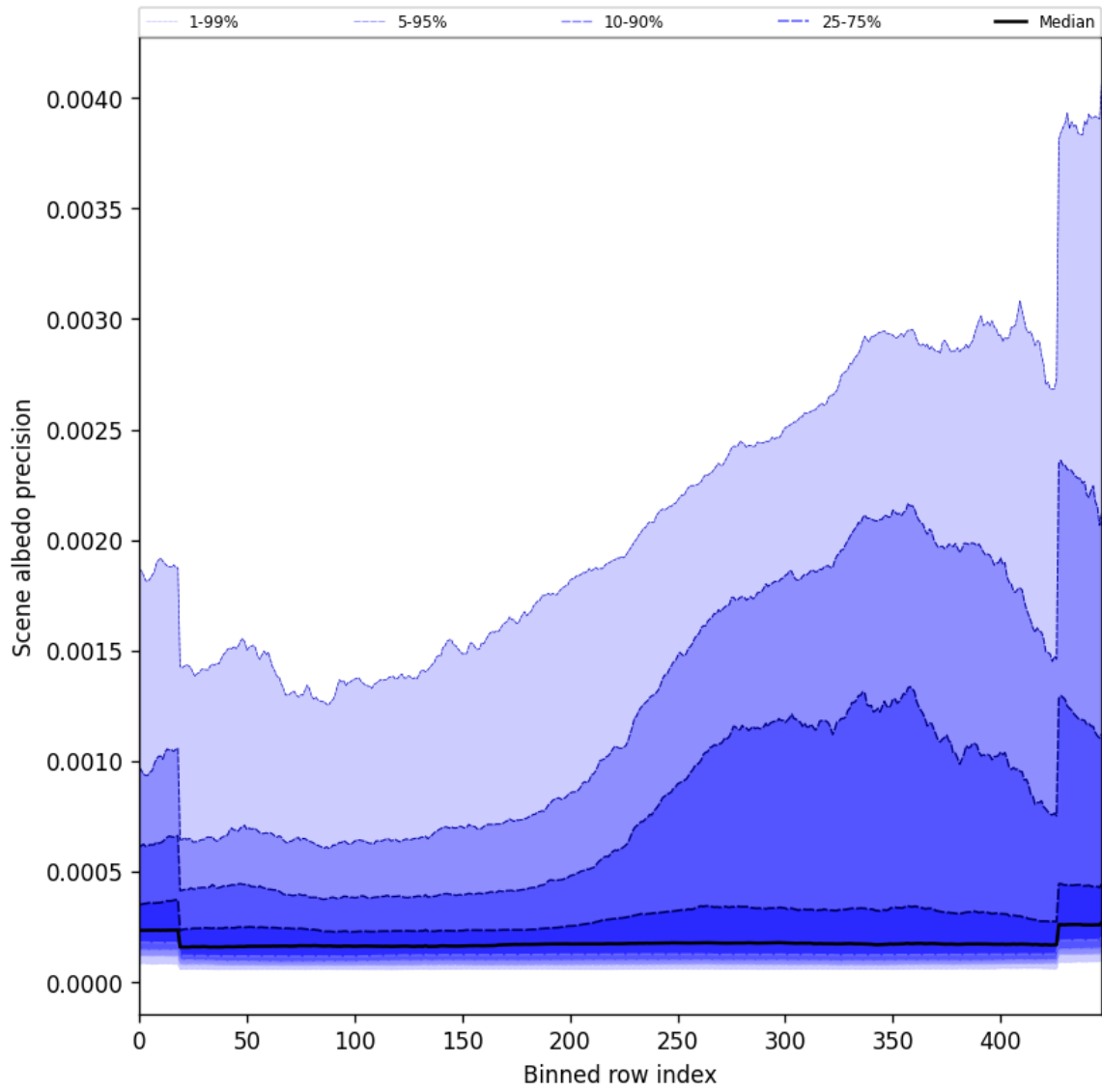
Figure 52: Along track statistics of “Scene albedo precision” for 2024-10-20 to 2024-10-22
