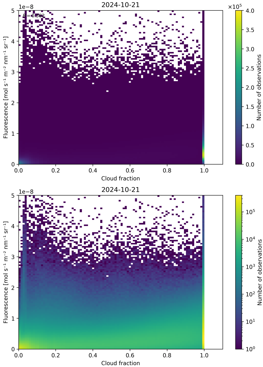
Figure 79: Scatter density plot of “Cloud fraction” against “Fluorescence” for 2024-10-20 to 2024-10-22.
