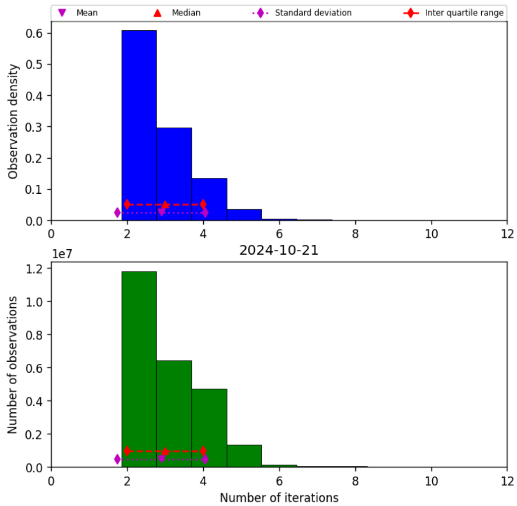
Figure 39: Histogram of “Number of iterations” for 2024-10-20 to 2024-10-22
