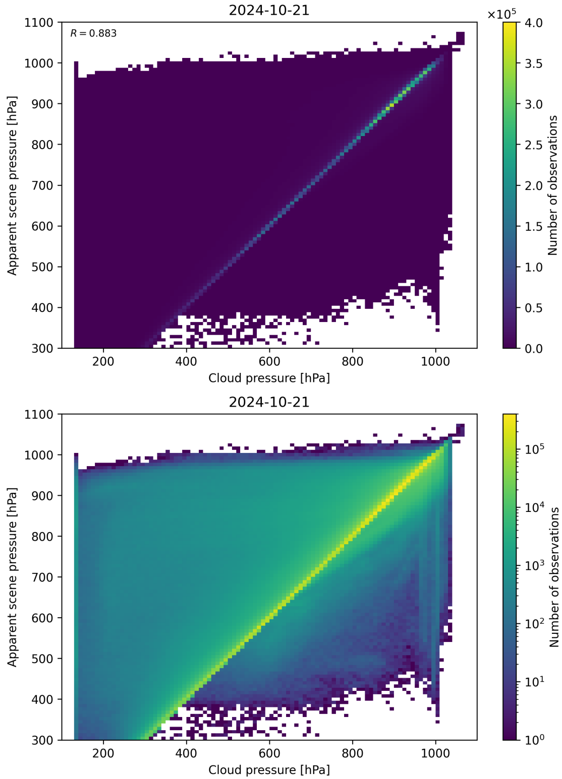
Figure 84: Scatter density plot of “Cloud pressure” against “Apparent scene pressure” for 2024-10-20 to 2024-10-22.
