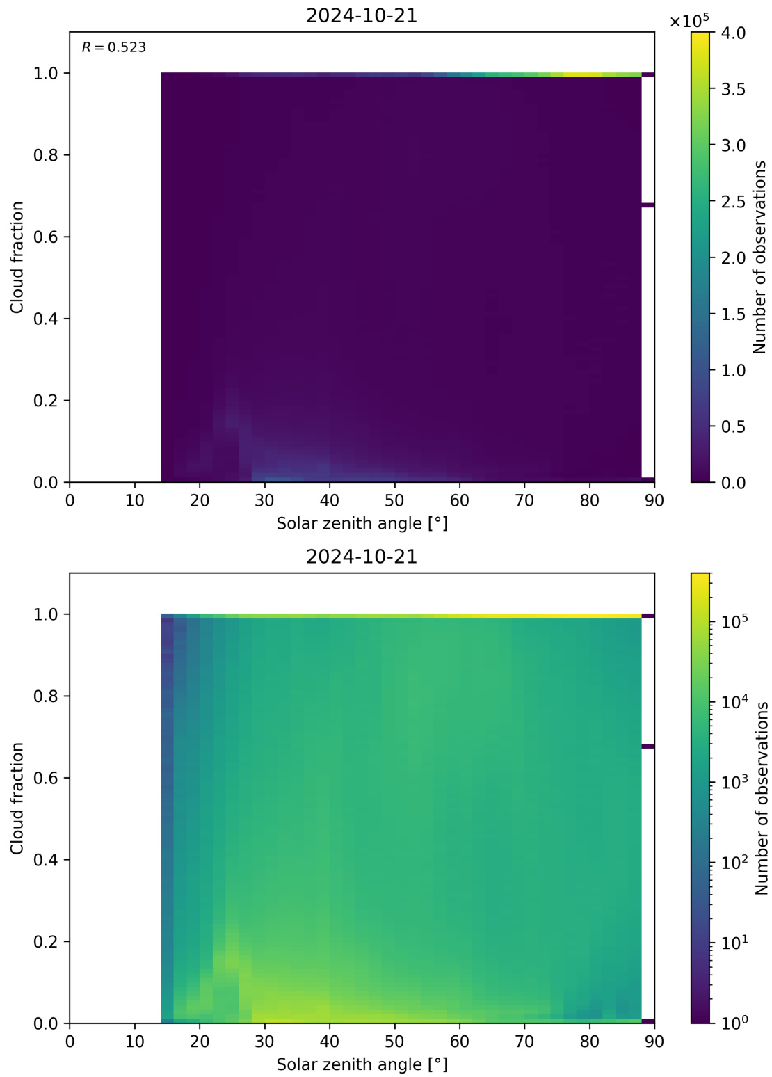
Figure 121: Scatter density plot of “Solar zenith angle” against “Cloud fraction” for 2024-10-20 to 2024-10-22.
