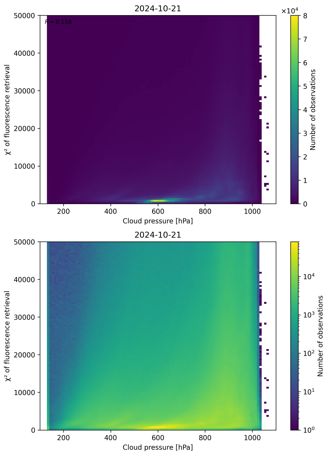
Figure 86: Scatter density plot of “Cloud pressure” against “ \chi^2 of fluorescence retrieval” for 2024-10-20 to 2024-10-22.
