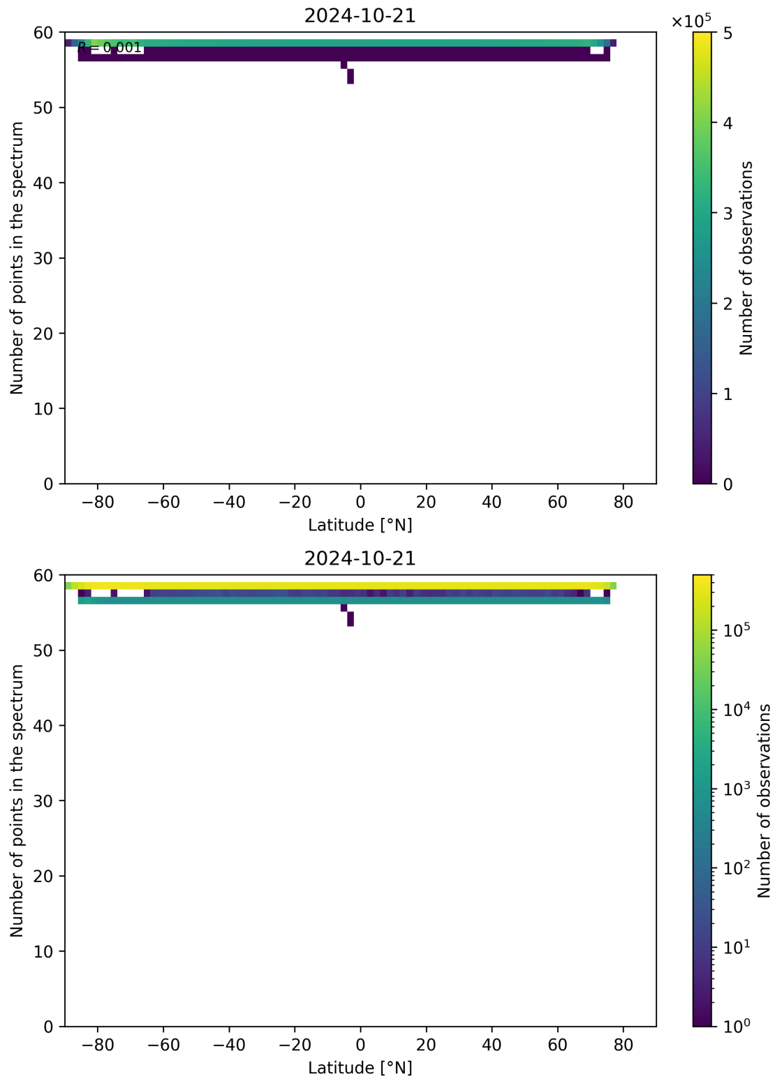
Figure 103: Scatter density plot of “Latitude” against “Number of points in the spectrum” for 2024-10-20 to 2024-10-22.
