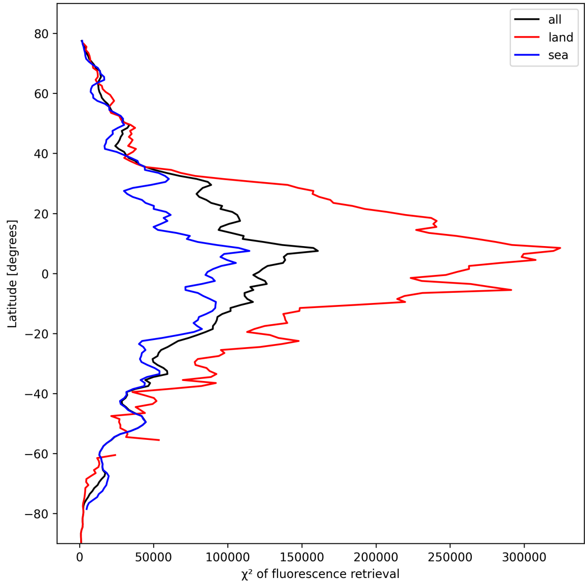
Figure 25: Zonal average of “ \chi^2 of fluorescence retrieval” for 2024-10-20 to 2024-10-22.
