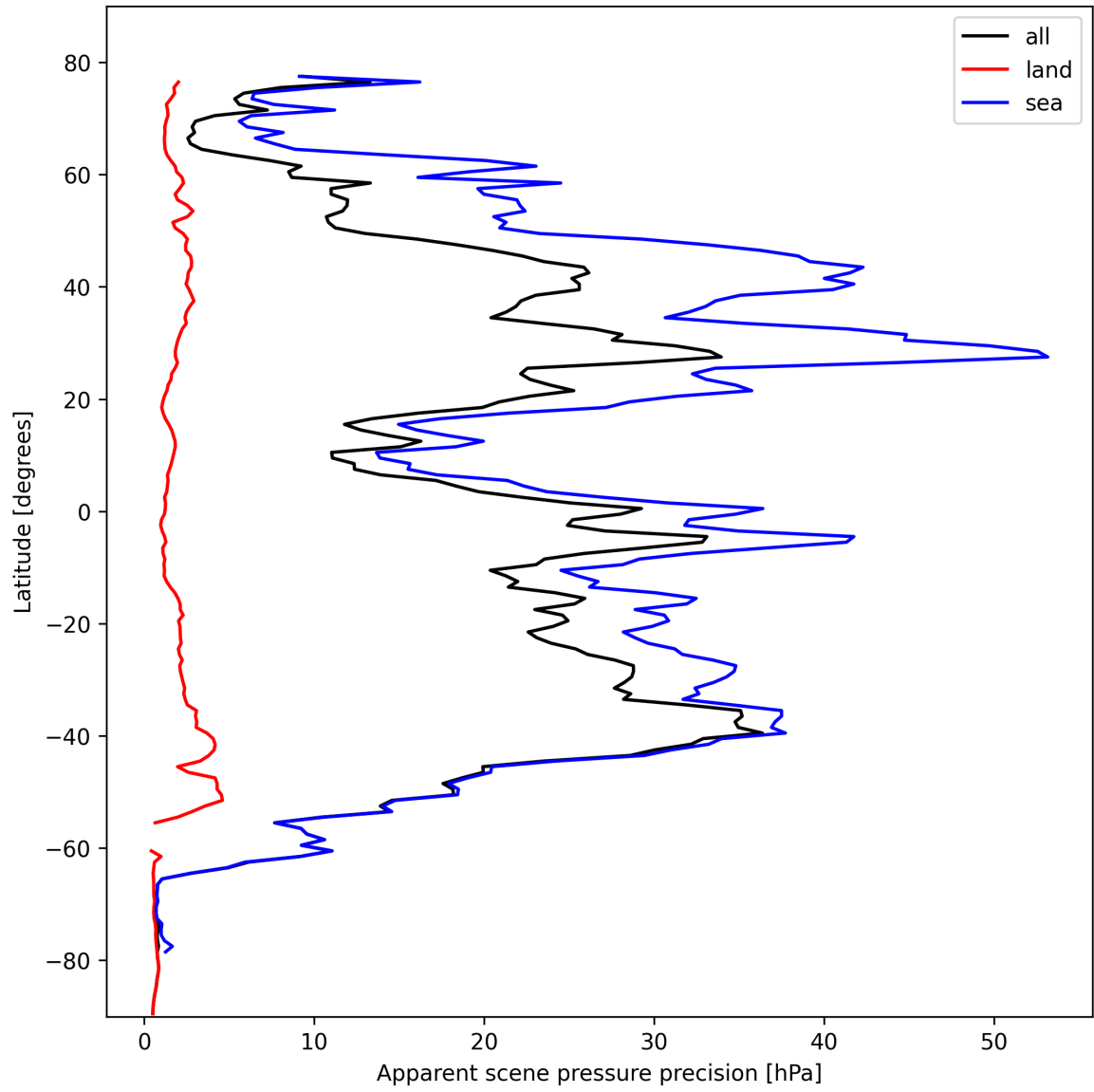
Figure 20: Zonal average of “Apparent scene pressure precision” for 2024-10-20 to 2024-10-22.
