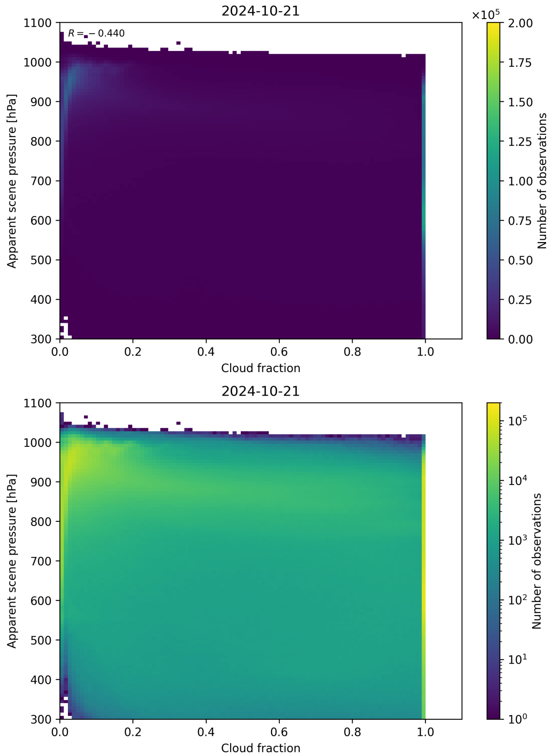
Figure 76: Scatter density plot of “Cloud fraction” against “Apparent scene pressure” for 2024-10-20 to 2024-10-22.
