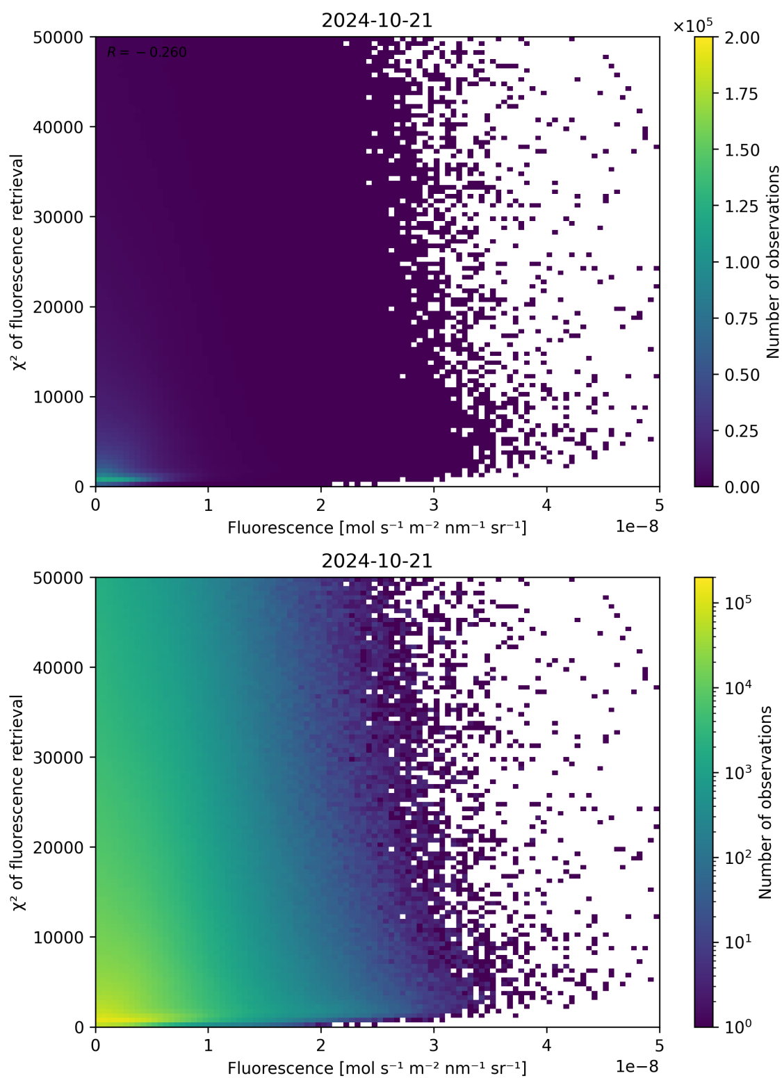
Figure 93: Scatter density plot of “Fluorescence” against “ \chi^2 of fluorescence retrieval” for 2024-10-20 to 2024-10-22.
