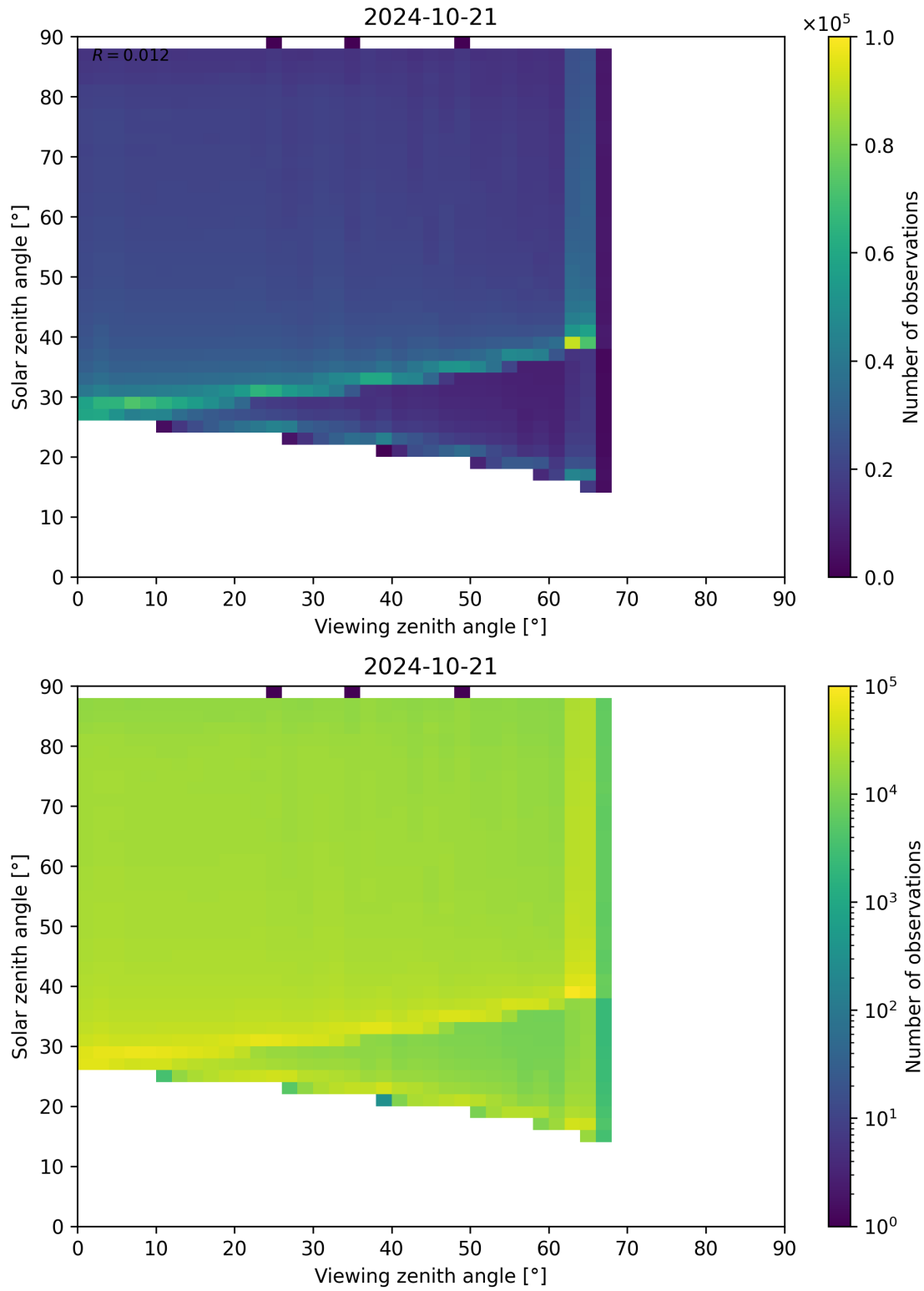
Figure 139: Scatter density plot of “Viewing zenith angle” against “Solar zenith angle” for 2024-10-20 to 2024-10-22.
