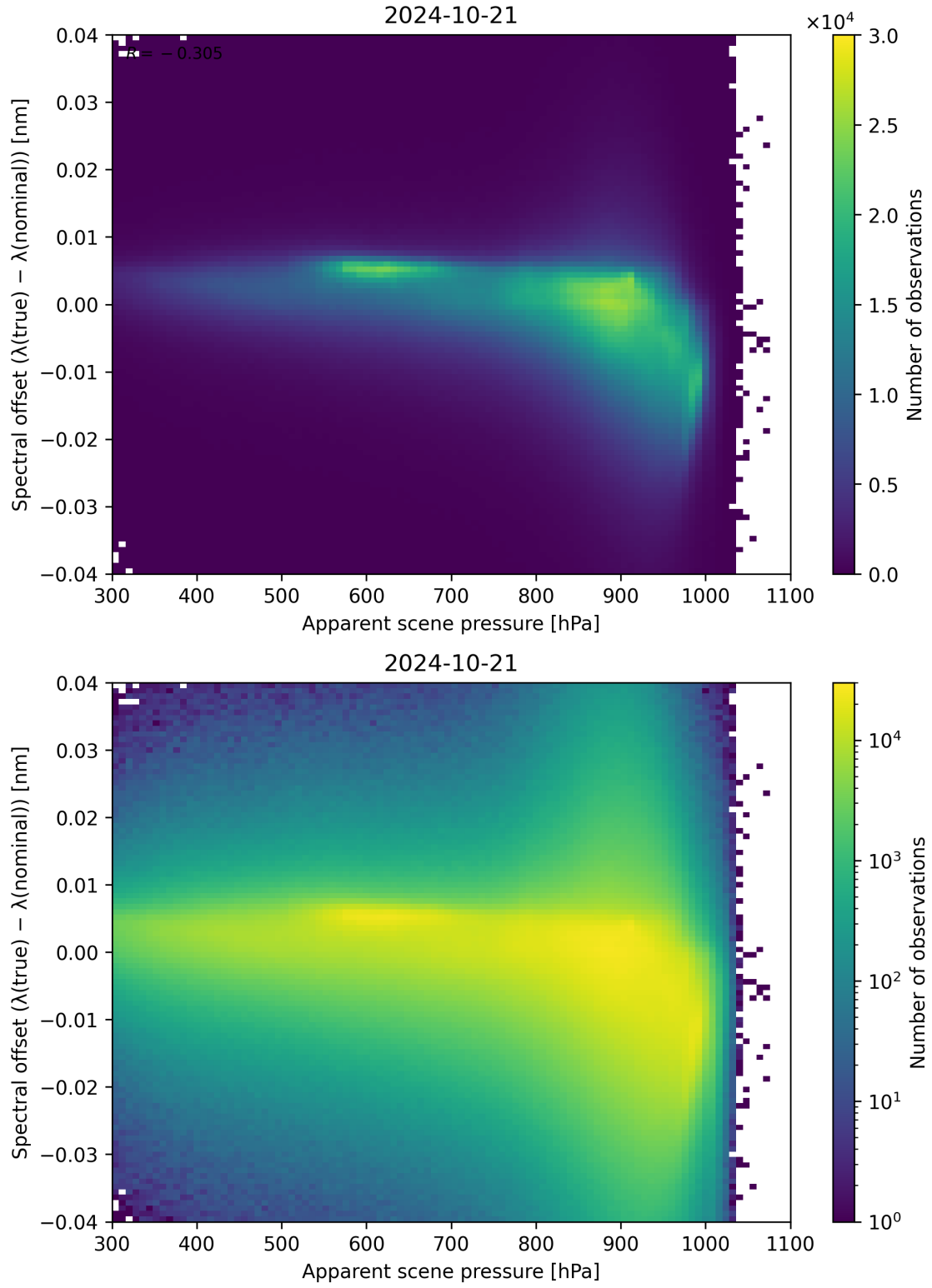
Figure 68: Scatter density plot of “Apparent scene pressure” against “Spectral offset ( \lambda_{\text{true}} - \lambda_{\text{nominal}} )” for 2024-10-20 to 2024-10-22.
