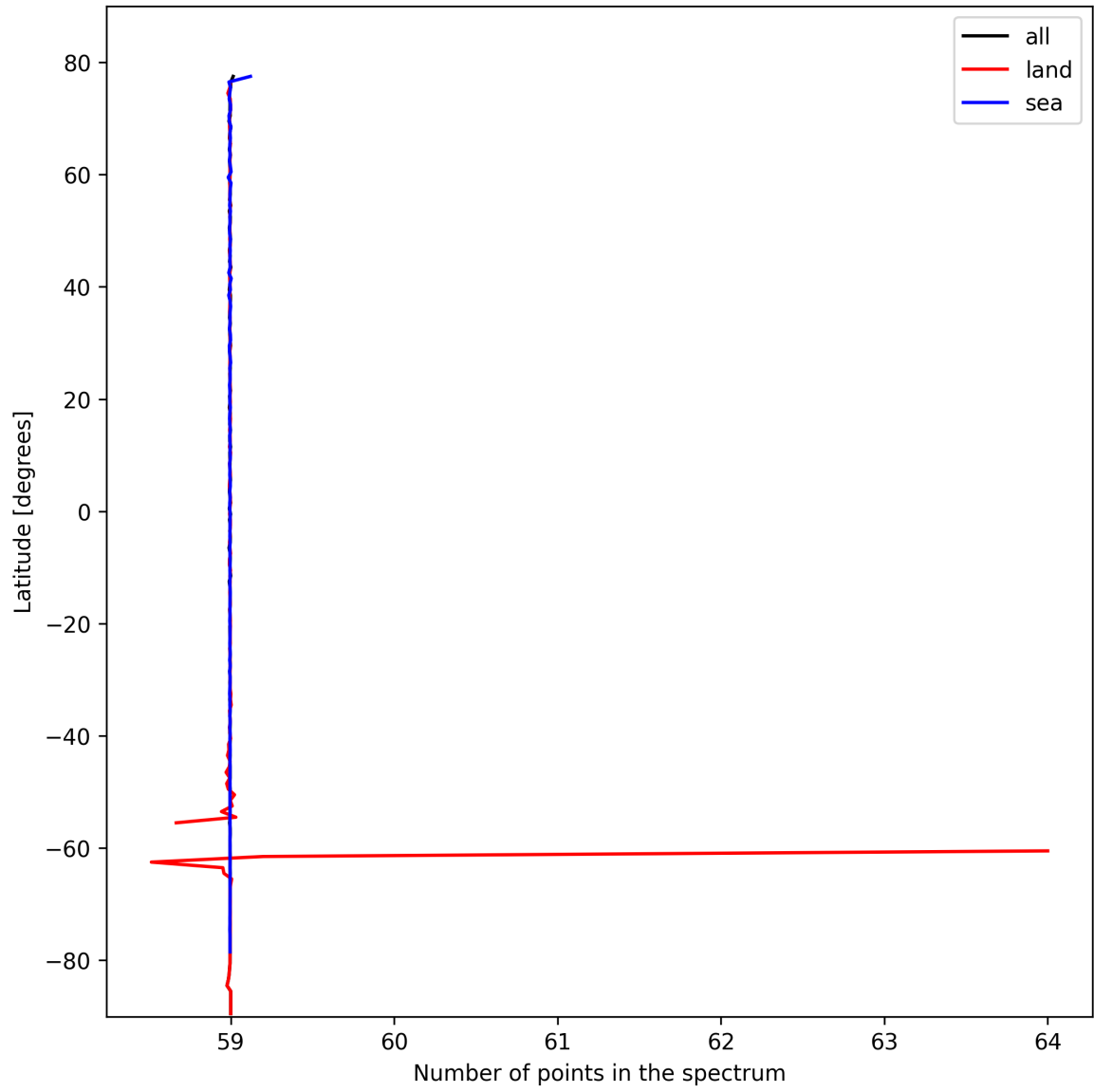
Figure 27: Zonal average of “Number of points in the spectrum” for 2024-10-20 to 2024-10-22.
