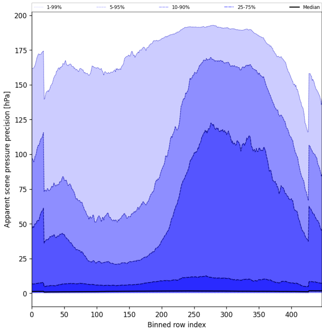
Figure 54: Along track statistics of “Apparent scene pressure precision” for 2024-10-20 to 2024-10-22
