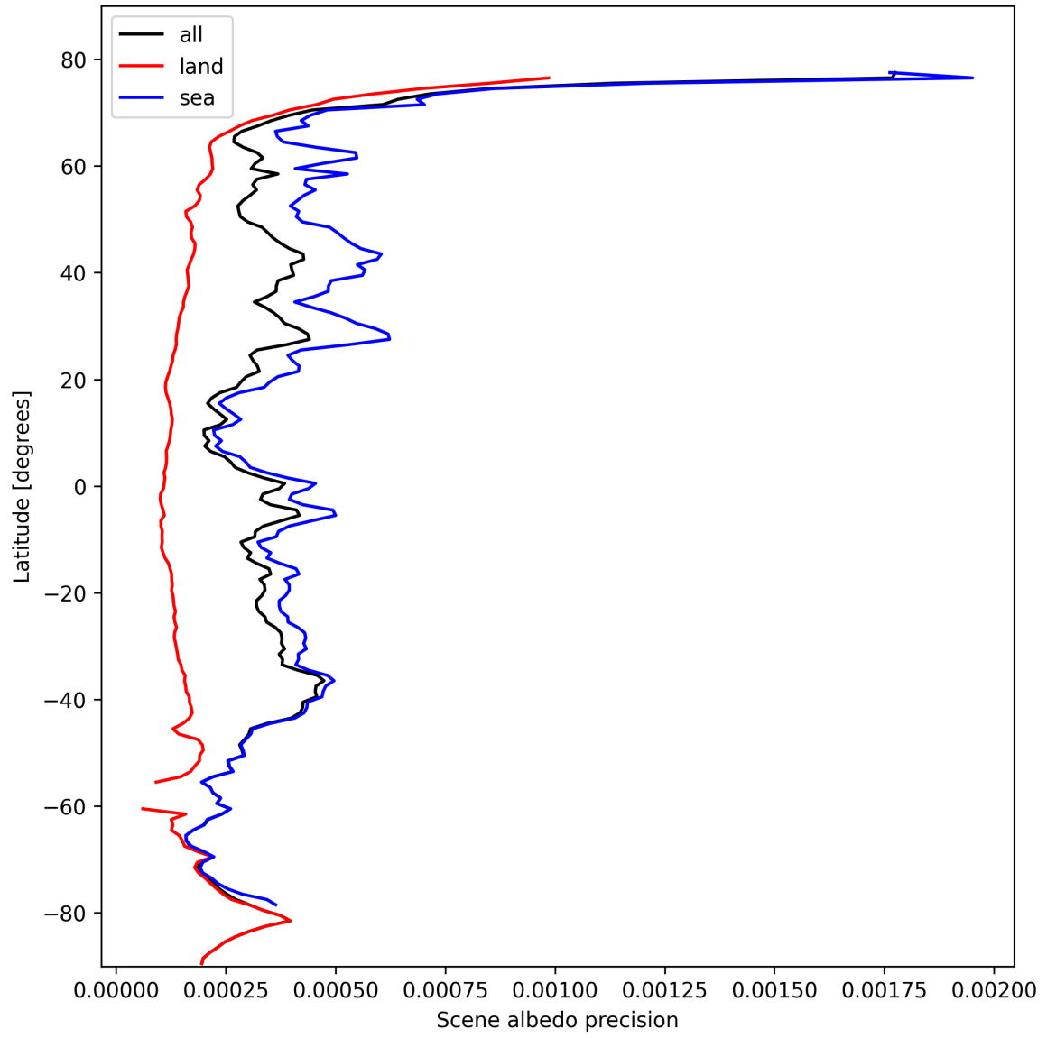
Figure 18: Zonal average of “Scene albedo precision” for 2024-10-20 to 2024-10-22.
