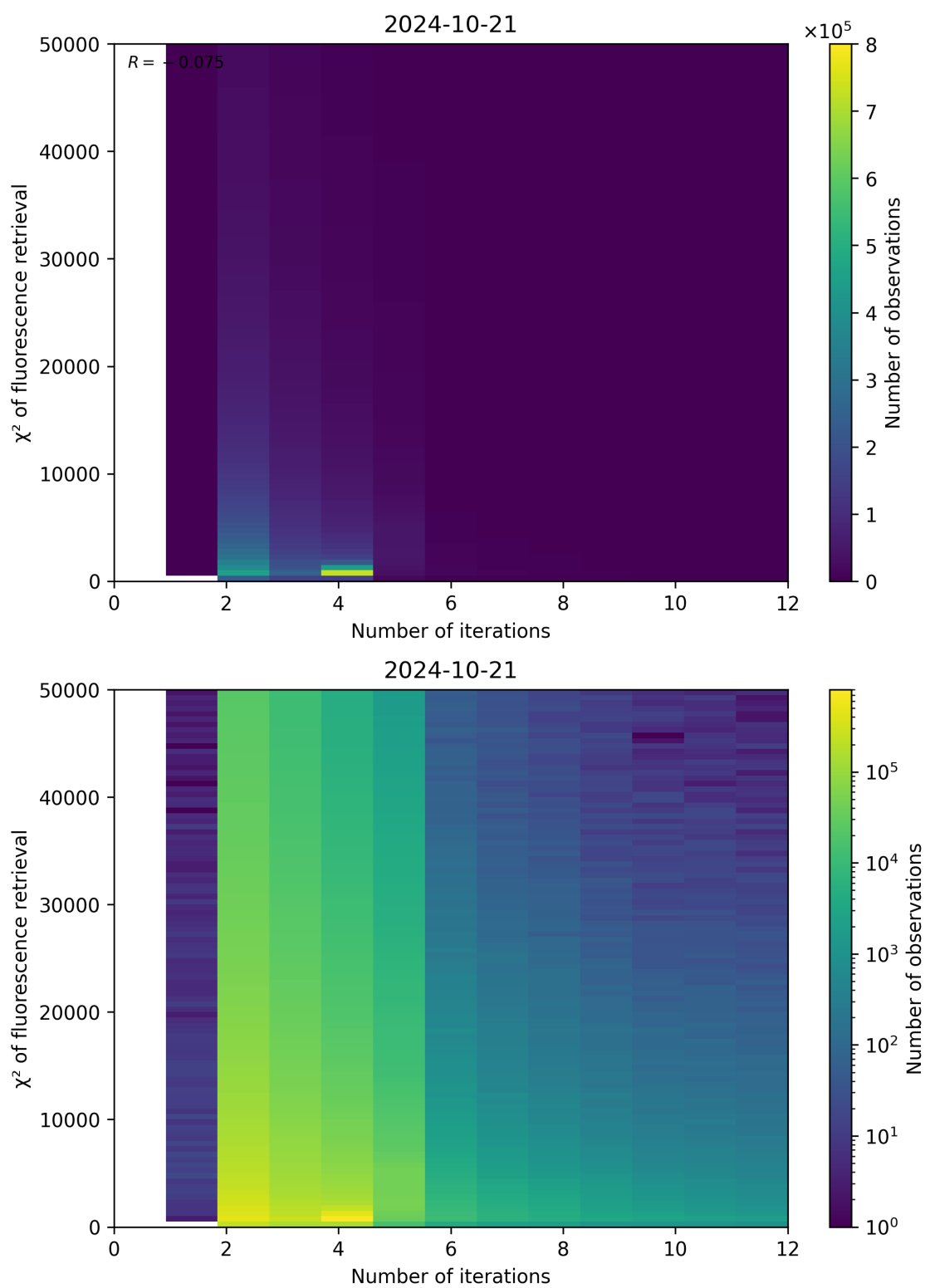
Figure 106: Scatter density plot of “Number of iterations” against “ \chi^2 of fluorescence retrieval” for 2024-10-20 to 2024-10-22.
