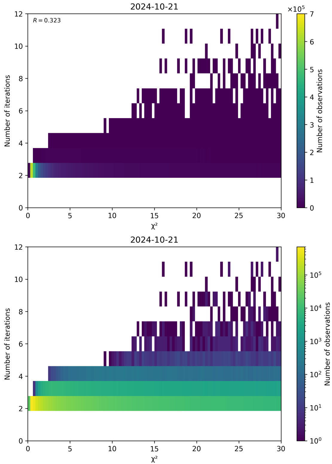
Figure 73: Scatter density plot of “ \chi^2 ” against “Number of iterations” for 2024-10-20 to 2024-10-22.
