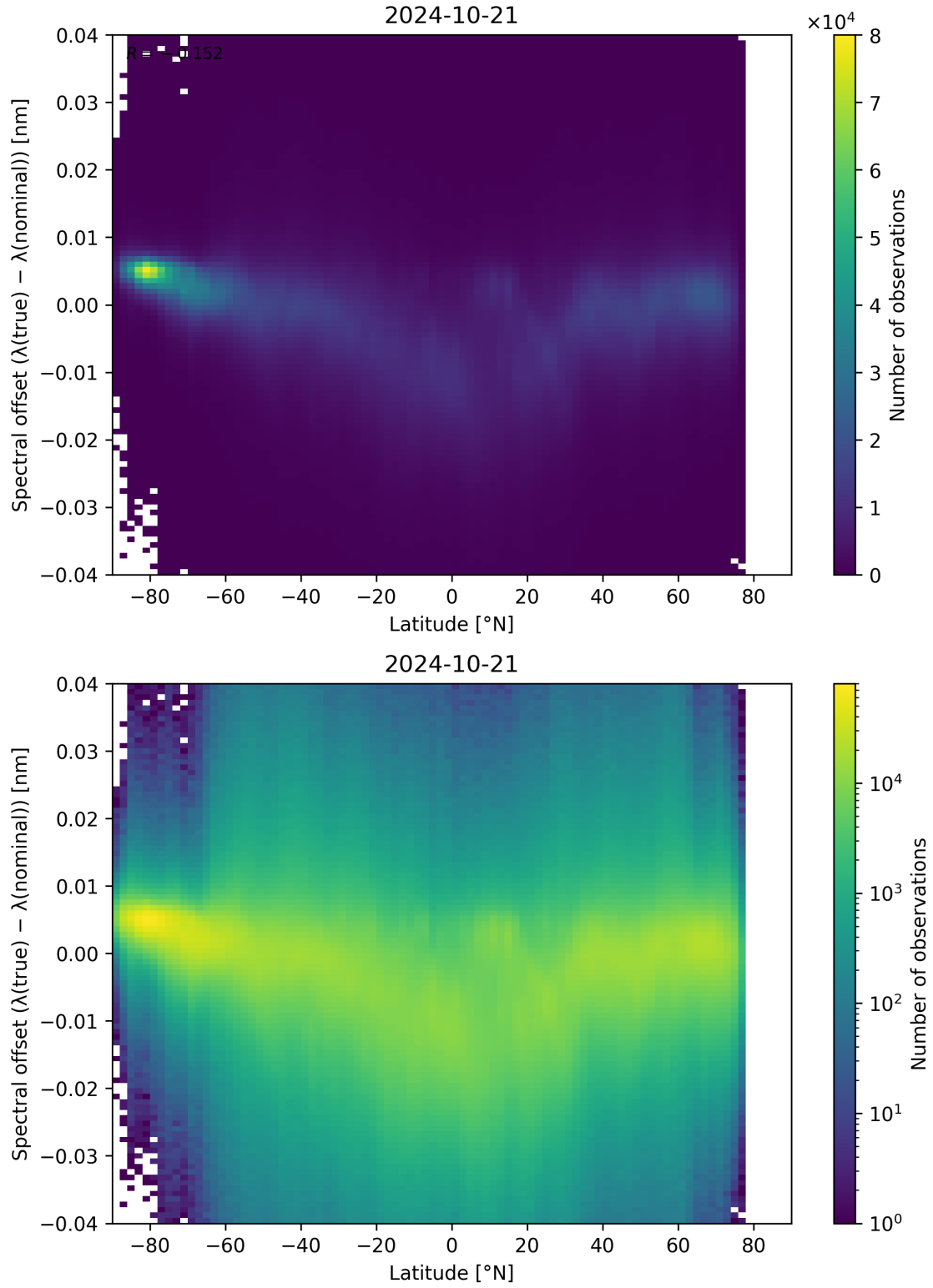
Figure 105: Scatter density plot of “Latitude” against “Spectral offset ( \lambda_{\text{true}} - \lambda_{\text{nominal}} )” for 2024-10-20 to 2024-10-22.
