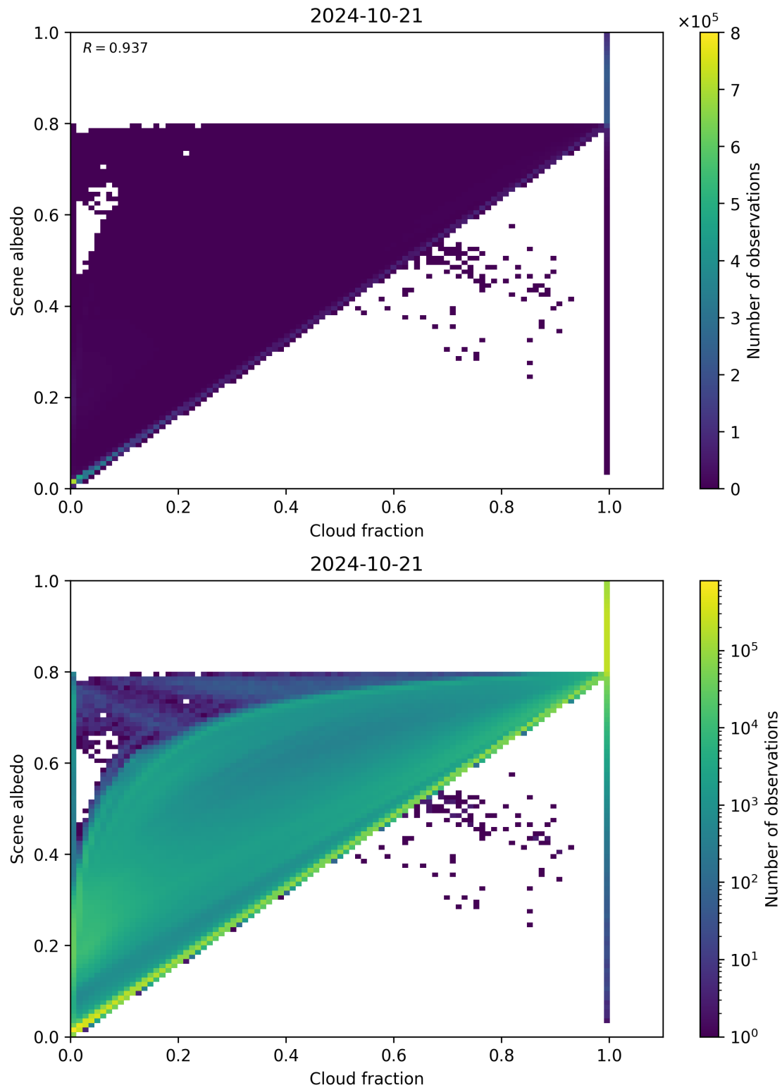
Figure 82: Scatter density plot of “Cloud fraction” against “Scene albedo” for 2024-10-20 to 2024-10-22.
