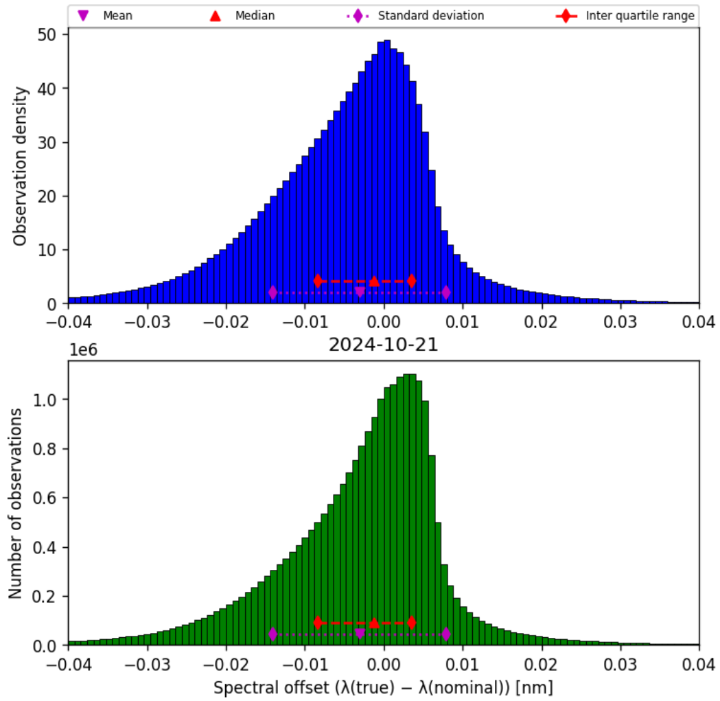
Figure 45: Histogram of “Spectral offset ( \lambda_{\text{true}} - \lambda_{\text{nominal}} )” for 2024-10-20 to 2024-10-22
