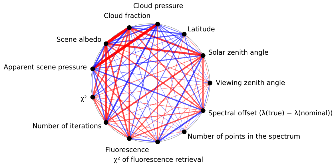
Figure 1: Map of correlation graph for 2024-10-20 to 2024-10-22.
