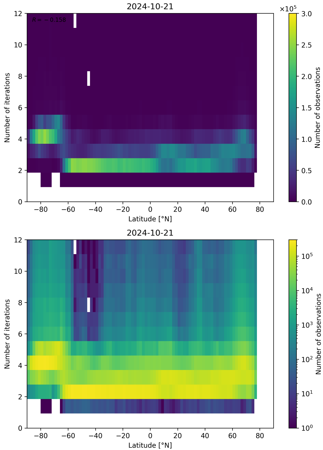
Figure 102: Scatter density plot of “Latitude” against “Number of iterations” for 2024-10-20 to 2024-10-22.
