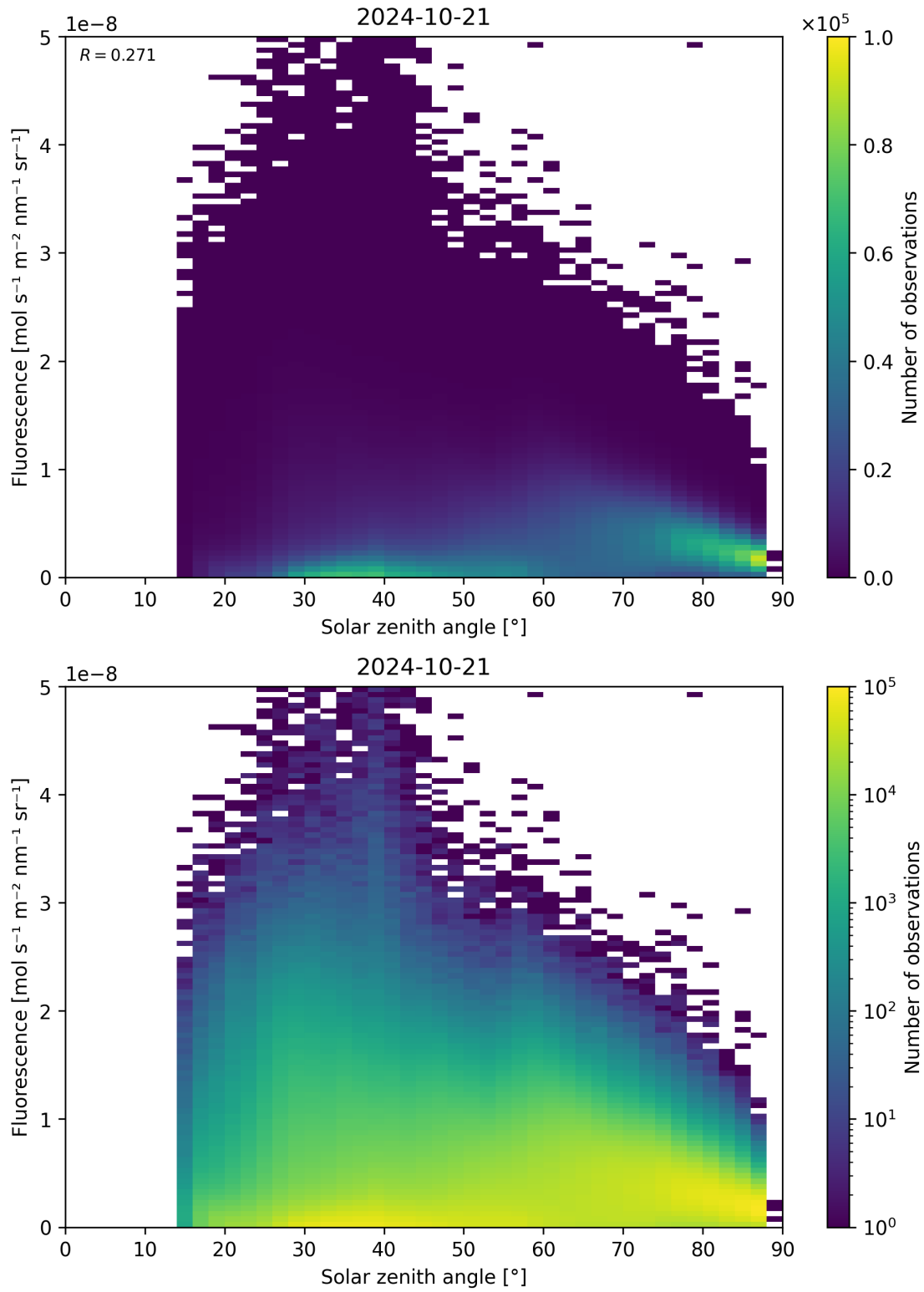
Figure 123: Scatter density plot of “Solar zenith angle” against “Fluorescence” for 2024-10-20 to 2024-10-22.
