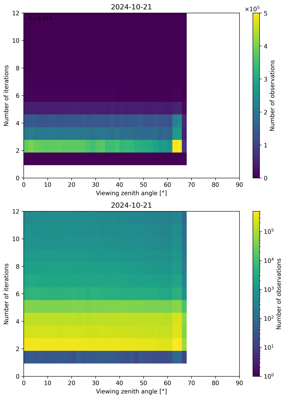
Figure 136: Scatter density plot of “Viewing zenith angle” against “Number of iterations” for 2024-10-20 to 2024-10-22.
