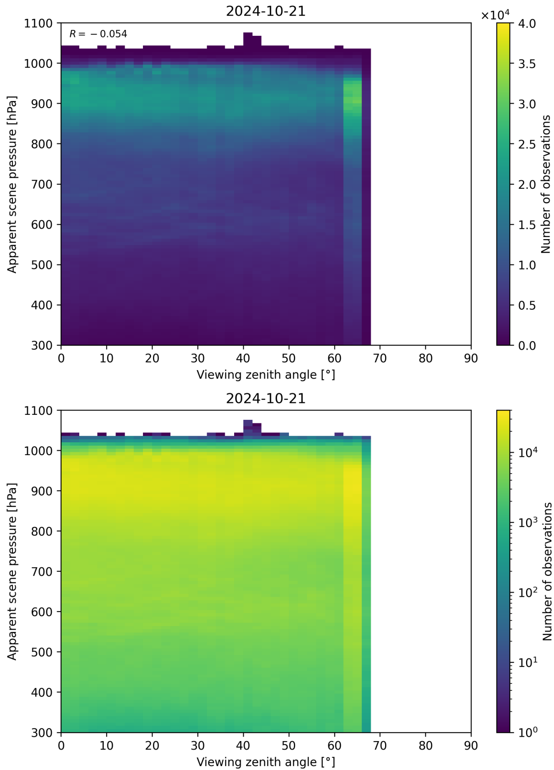
Figure 129: Scatter density plot of “Viewing zenith angle” against “Apparent scene pressure” for 2024-10-20 to 2024-10-22.
