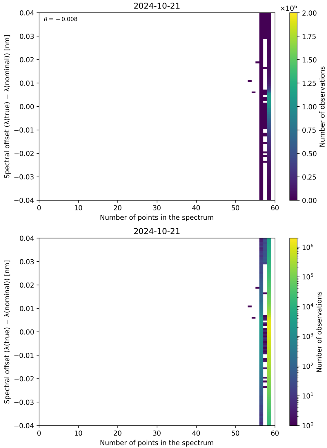
Figure 110: Scatter density plot of “Number of points in the spectrum” against “Spectral offset ( \lambda_{\text{true}} - \lambda_{\text{nominal}} )” for 2024-10-20 to 2024-10-22.
