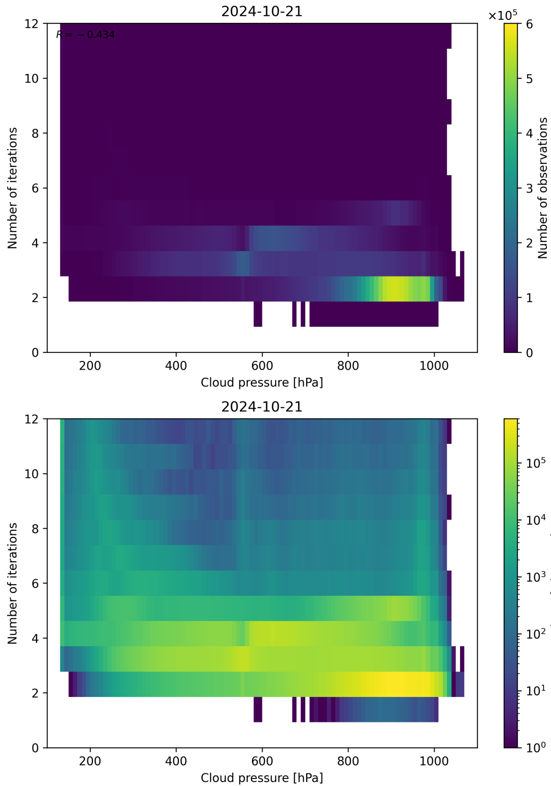
Figure 89: Scatter density plot of “Cloud pressure” against “Number of iterations” for 2024-10-20 to 2024-10-22.
