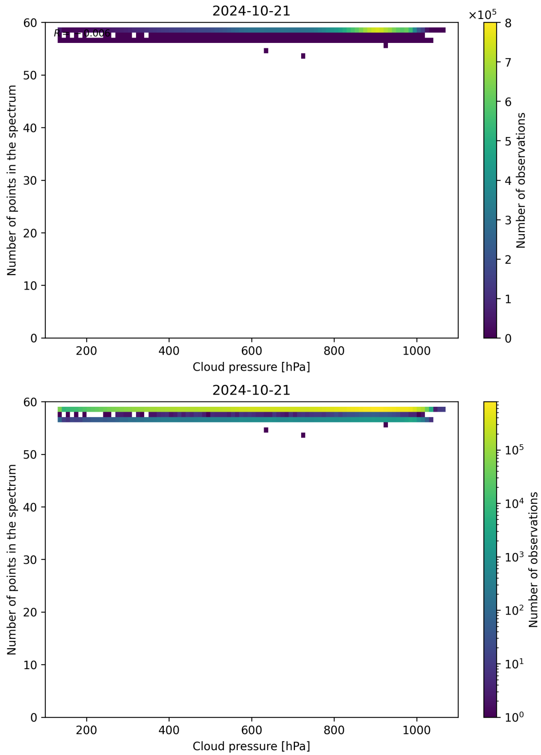
Figure 90: Scatter density plot of “Cloud pressure” against “Number of points in the spectrum” for 2024-10-20 to 2024-10-22.
