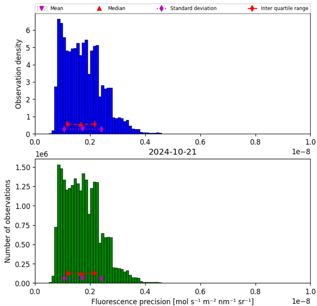
Figure 41: Histogram of “Fluorescence precision” for 2024-10-20 to 2024-10-22
