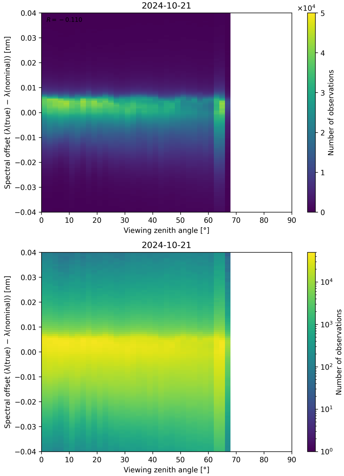
Figure 140: Scatter density plot of “Viewing zenith angle” against “Spectral offset ( \lambda_{\text{true}} - \lambda_{\text{nominal}} )” for 2024-10-20 to 2024-10-22.
