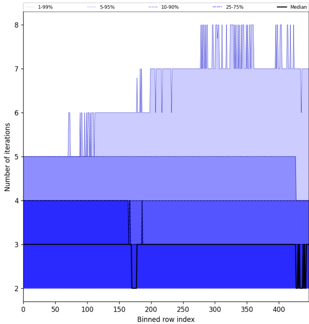
Figure 56: Along track statistics of “Number of iterations” for 2024-10-20 to 2024-10-22
