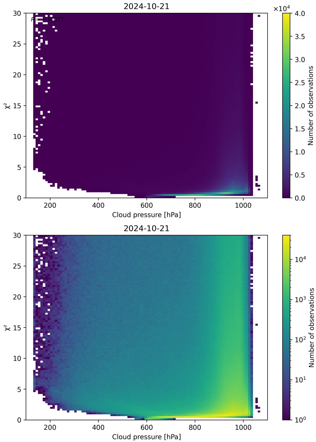
Figure 85: Scatter density plot of “Cloud pressure” against “ \chi^2 ” for 2024-10-20 to 2024-10-22.
