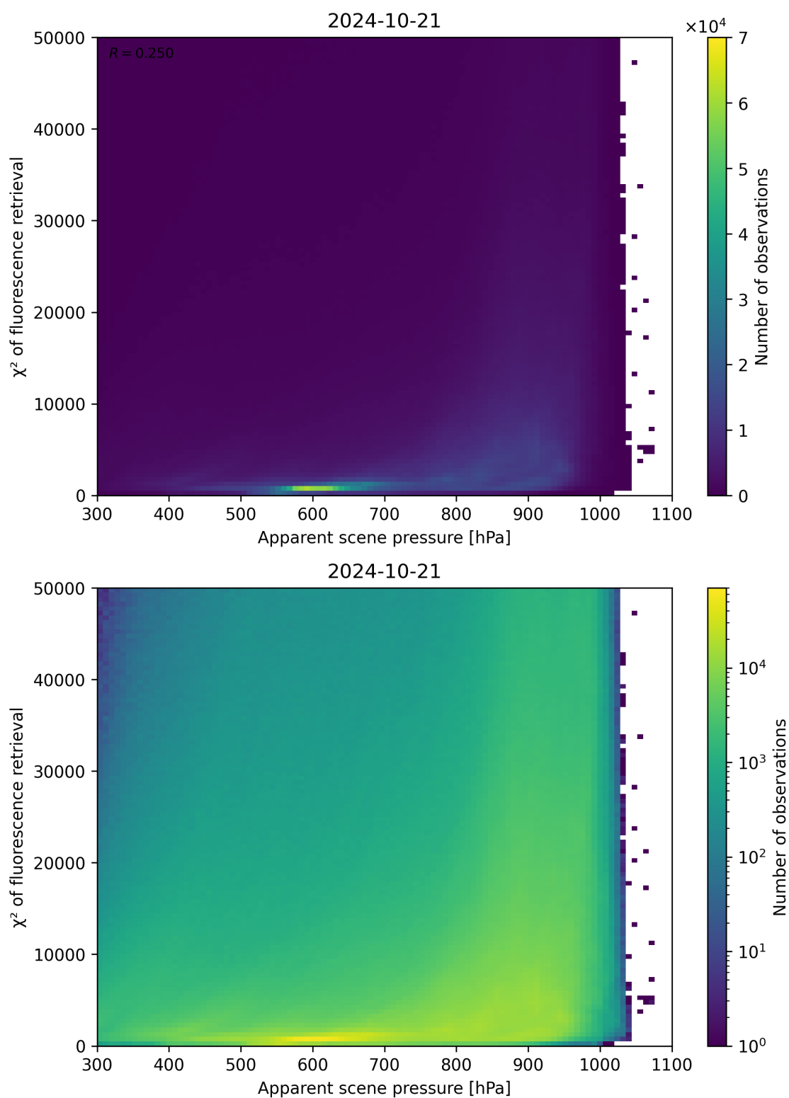
Figure 64: Scatter density plot of “Apparent scene pressure” against “ \chi^2 of fluorescence retrieval” for 2024-10-20 to 2024-10-22.
