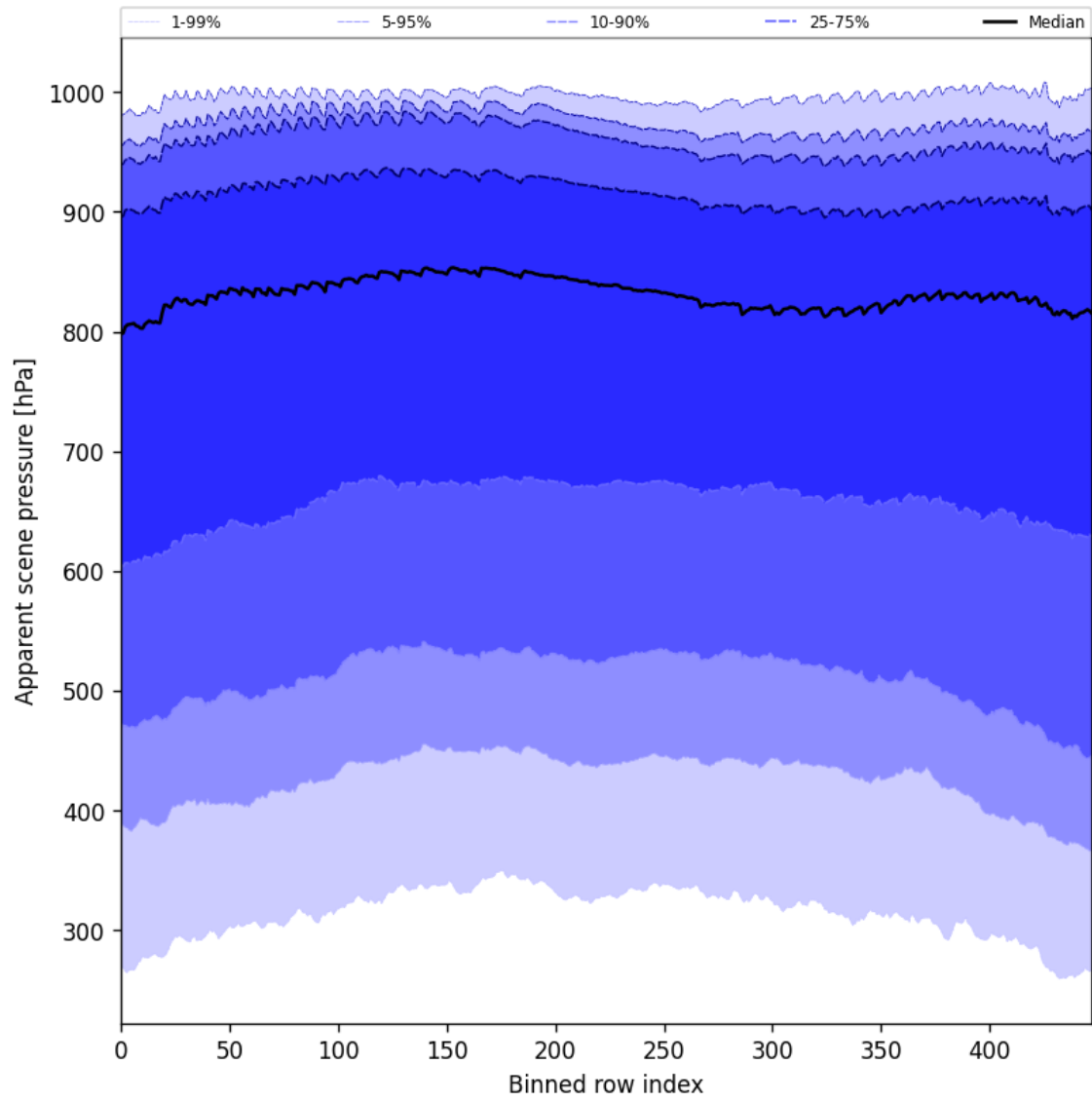
Figure 53: Along track statistics of “Apparent scene pressure” for 2024-10-20 to 2024-10-22
