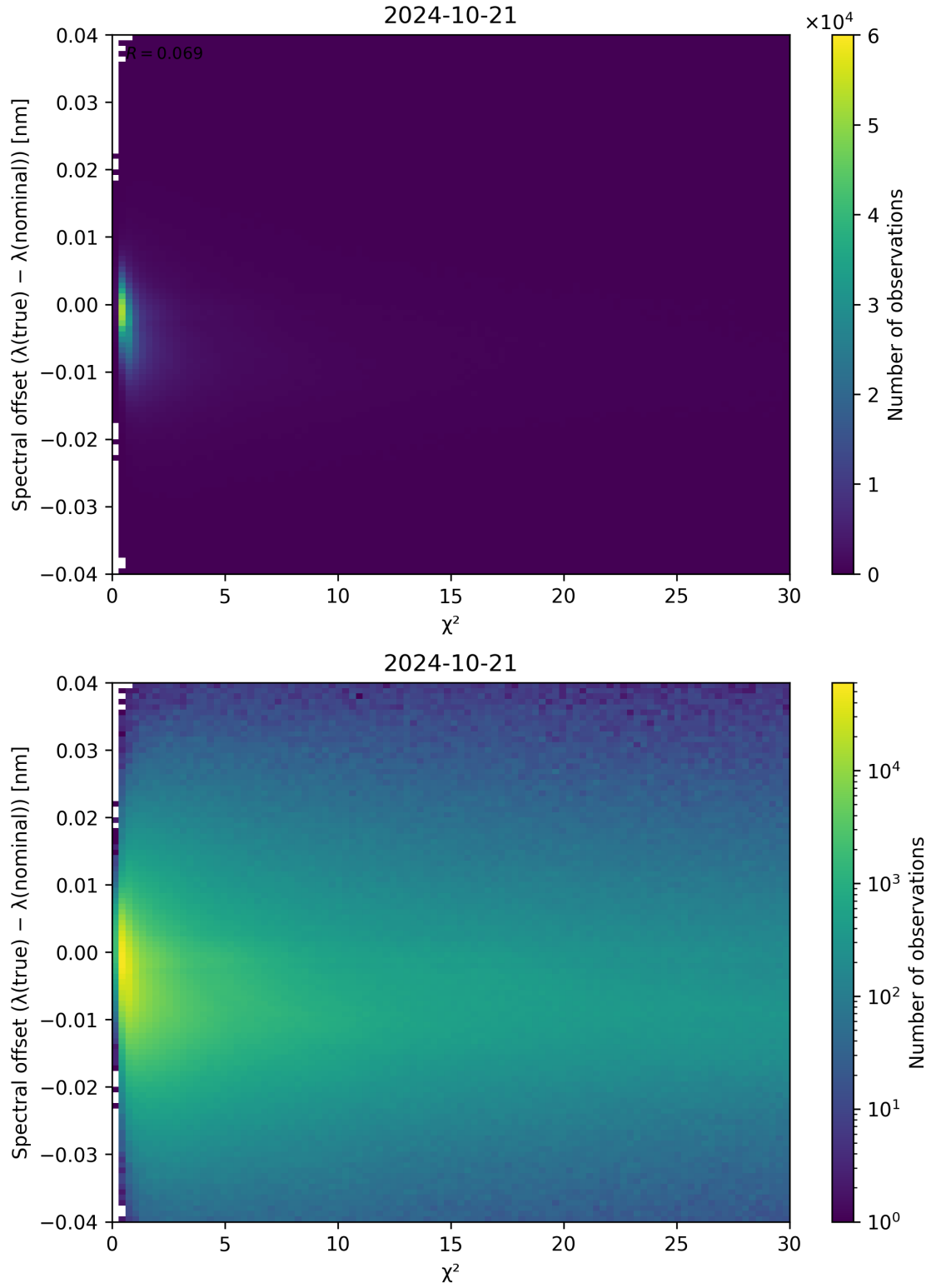
Figure 75: Scatter density plot of “ \chi^2 ” against “Spectral offset ( \lambda_{\text{true}} - \lambda_{\text{nominal}} )” for 2024-10-20 to 2024-10-22.
