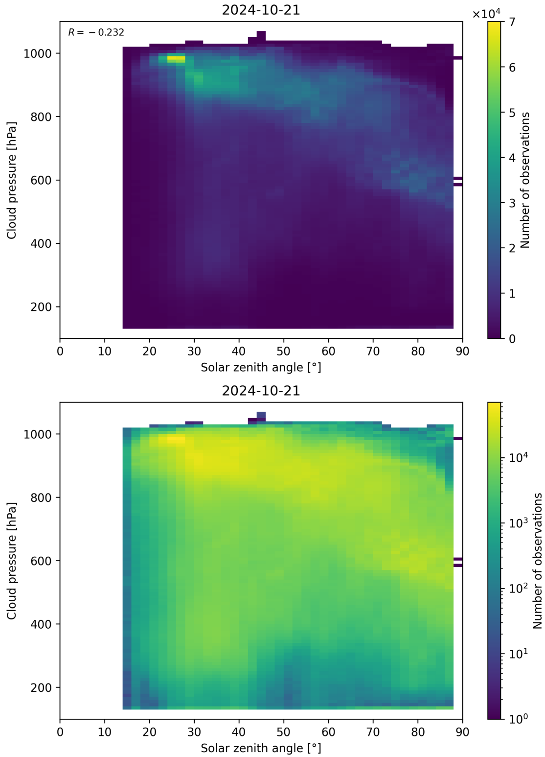
Figure 122: Scatter density plot of “Solar zenith angle” against “Cloud pressure” for 2024-10-20 to 2024-10-22.
