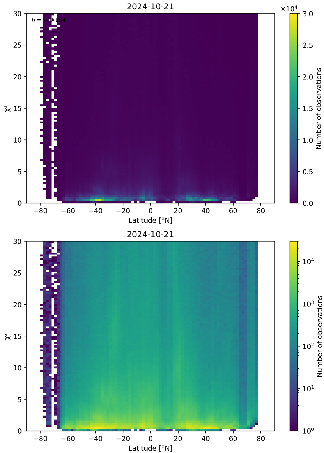
Figure 97: Scatter density plot of “Latitude” against “ \chi^2 ” for 2024-10-20 to 2024-10-22.
