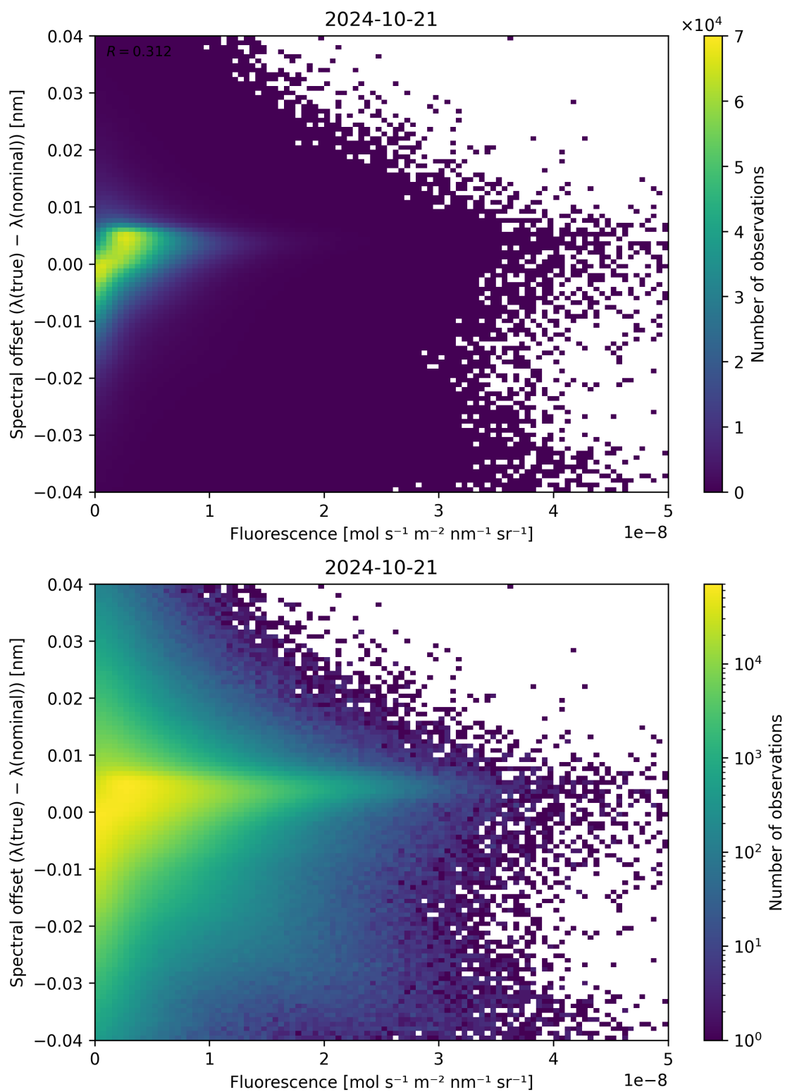
Figure 95: Scatter density plot of “Fluorescence” against “Spectral offset ( \lambda_{\text{true}} - \lambda_{\text{nominal}} )” for 2024-10-20 to 2024-10-22.
