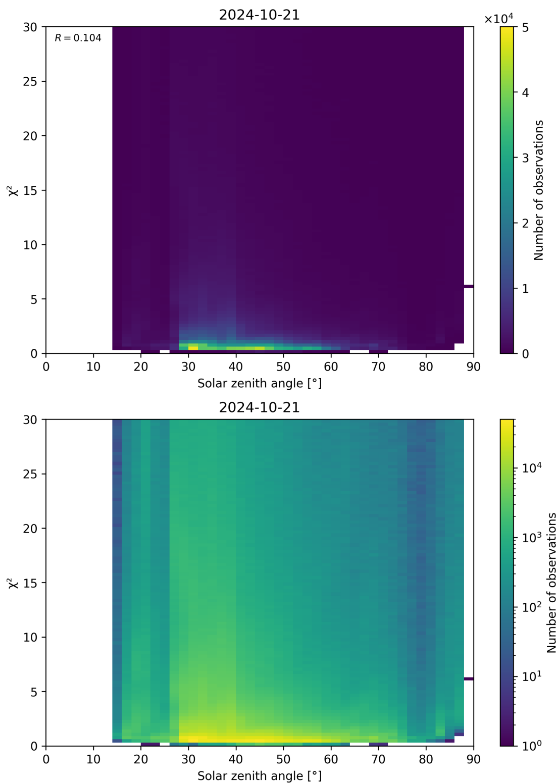
Figure 119: Scatter density plot of “Solar zenith angle” against “ \chi^2 ” for 2024-10-20 to 2024-10-22.
