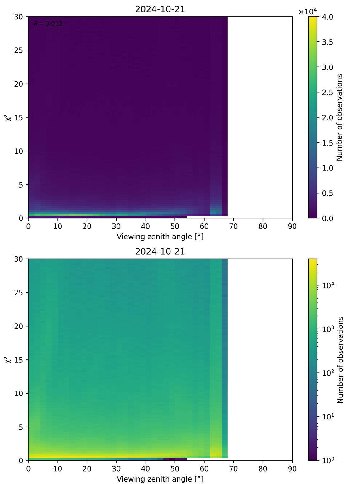
Figure 130: Scatter density plot of “Viewing zenith angle” against “ \chi^2 ” for 2024-10-20 to 2024-10-22.
