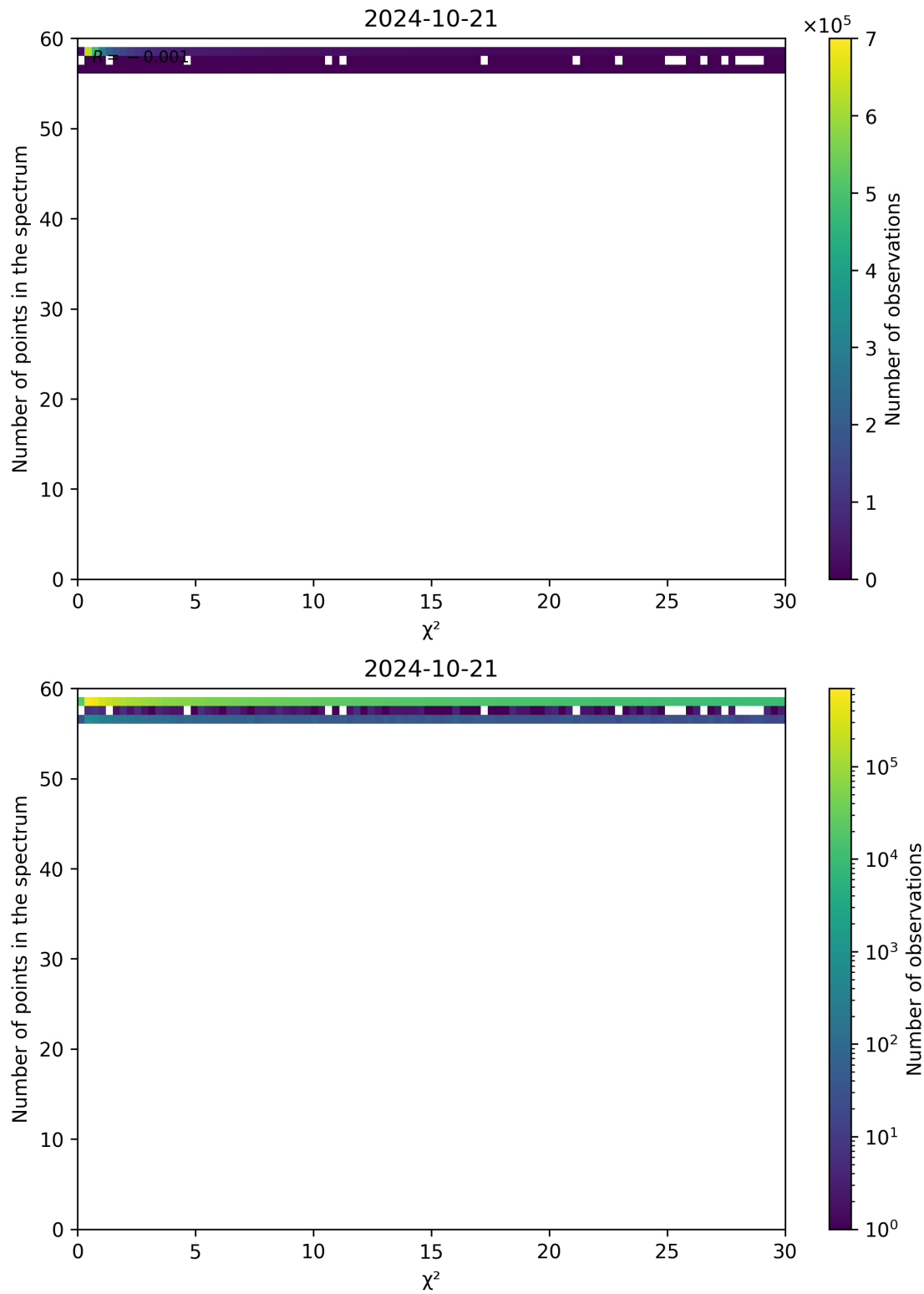
Figure 74: Scatter density plot of " \chi^2 " against "Number of points in the spectrum" for 2024-10-20 to 2024-10-22.
