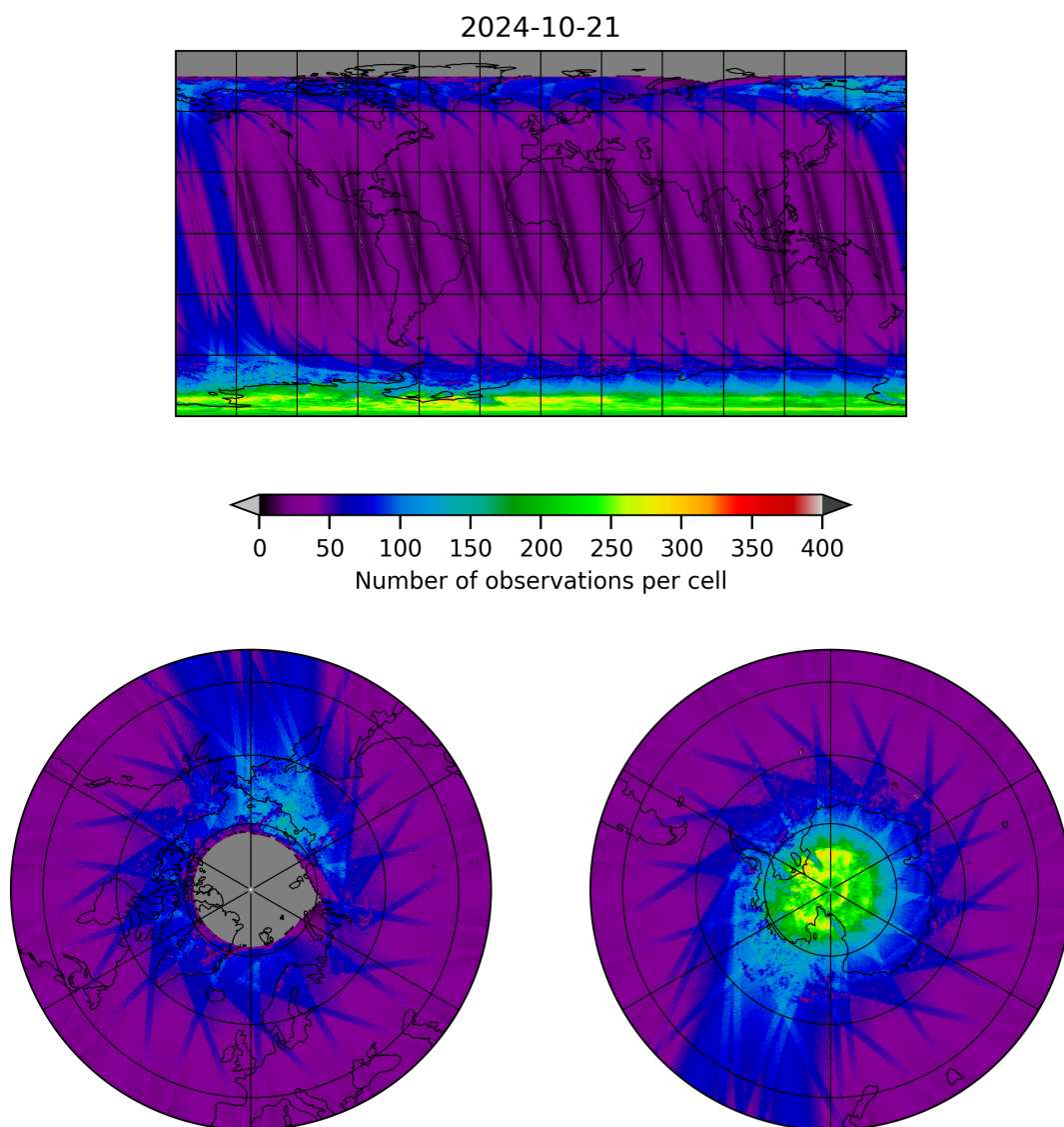
Figure 11: Map of the number of observations for 2024-10-20 to 2024-10-22
