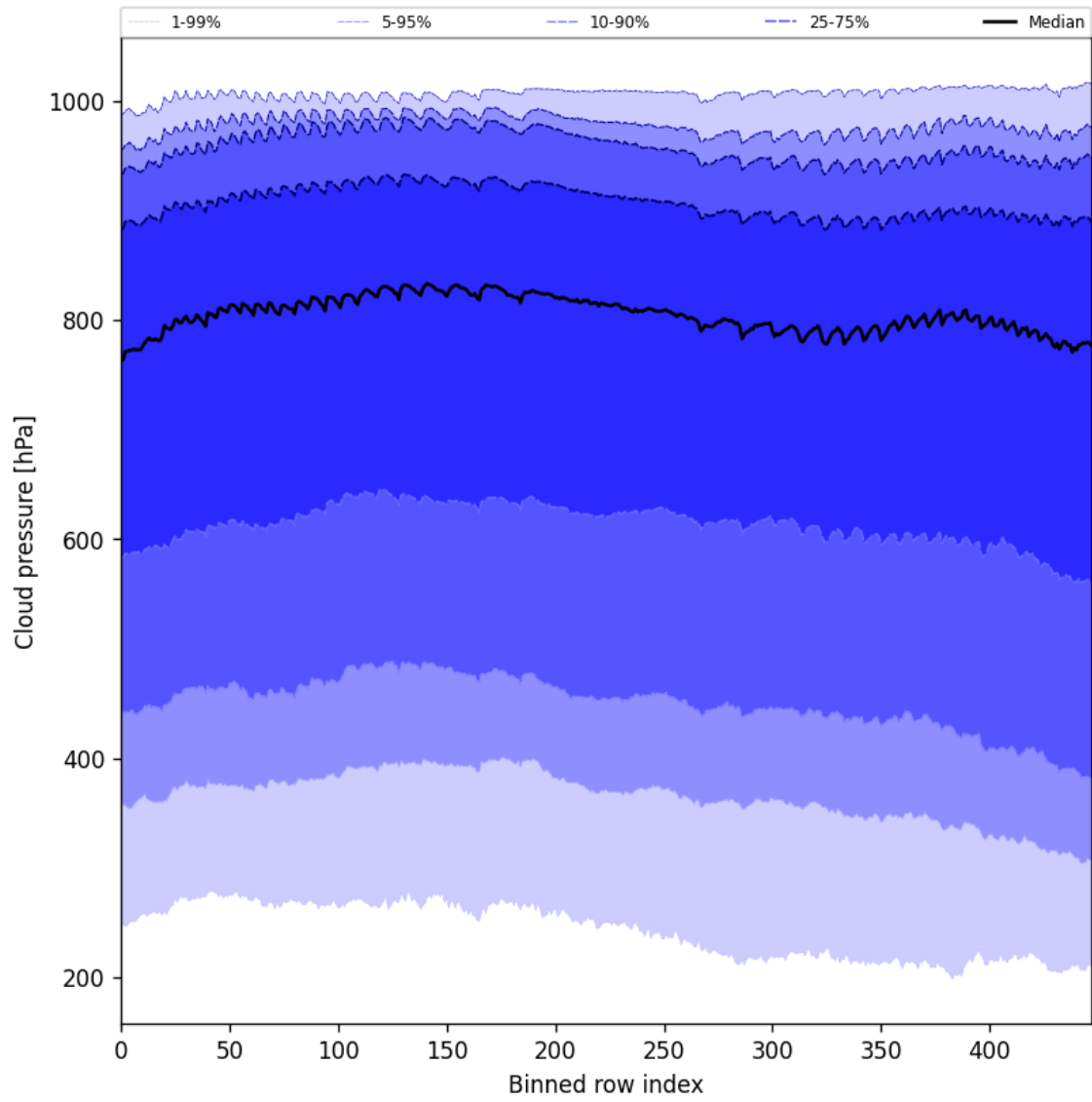
Figure 47: Along track statistics of “Cloud pressure” for 2024-10-20 to 2024-10-22
