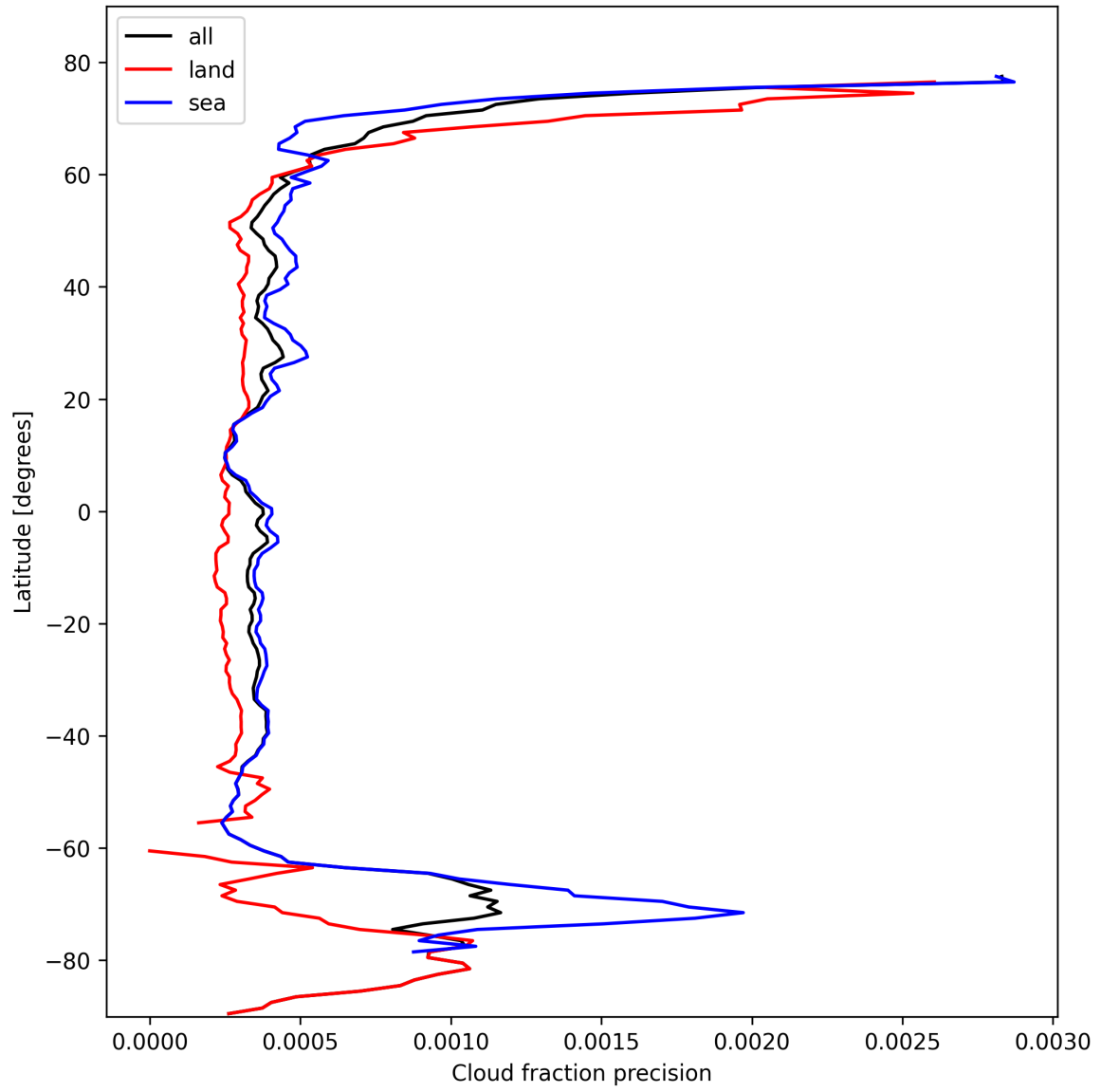
Figure 16: Zonal average of “Cloud fraction precision” for 2024-10-20 to 2024-10-22.
