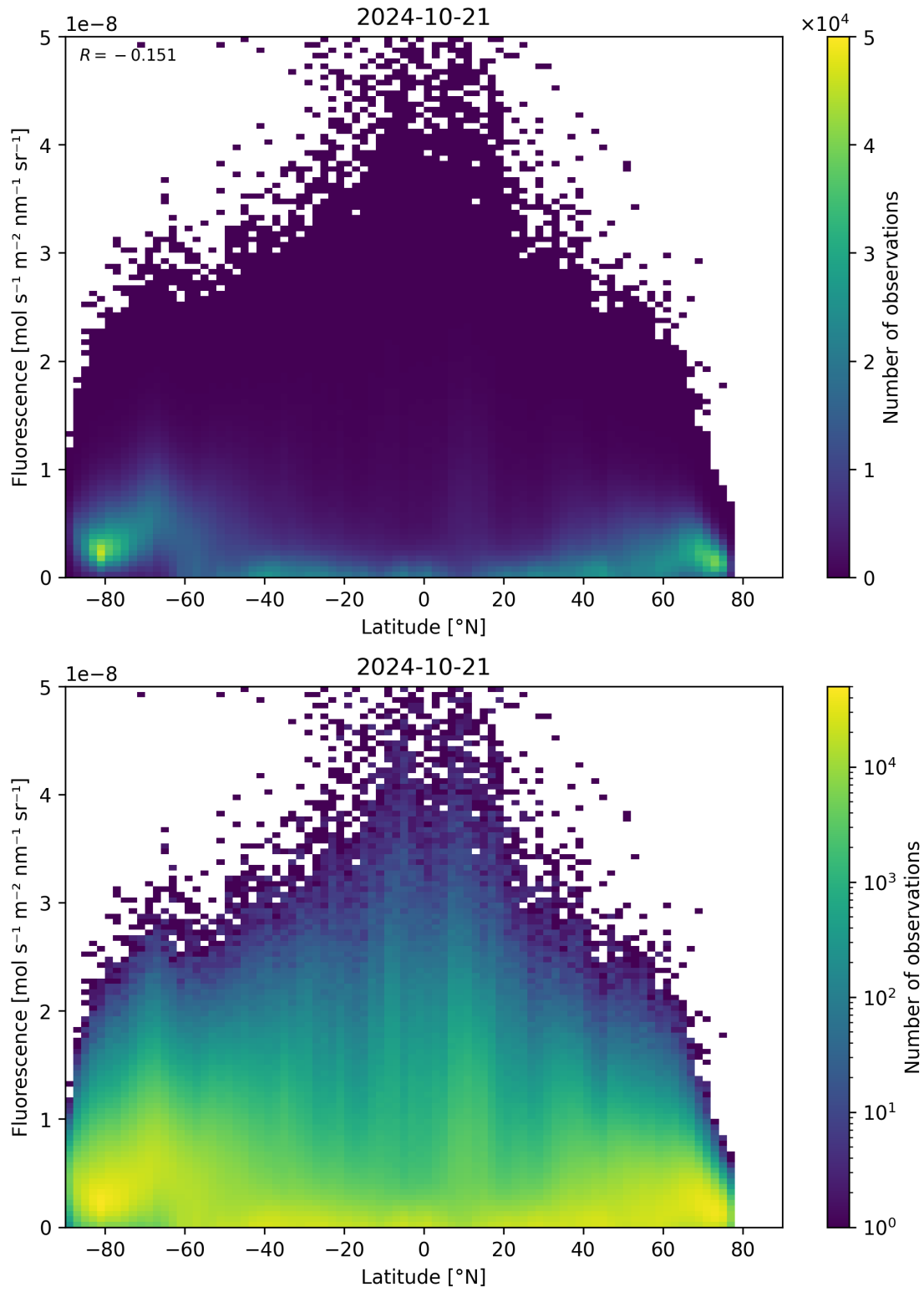
Figure 101: Scatter density plot of “Latitude” against “Fluorescence” for 2024-10-20 to 2024-10-22.
