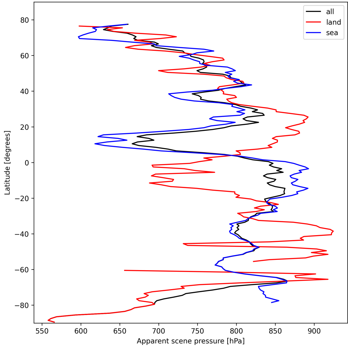
Figure 19: Zonal average of “Apparent scene pressure” for 2024-10-20 to 2024-10-22.
