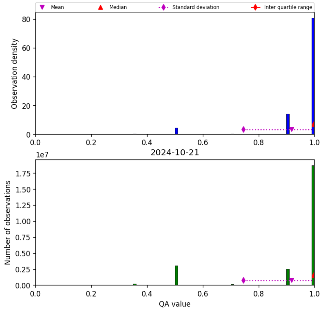
Figure 29: Histogram of “QA value” for 2024-10-20 to 2024-10-22
