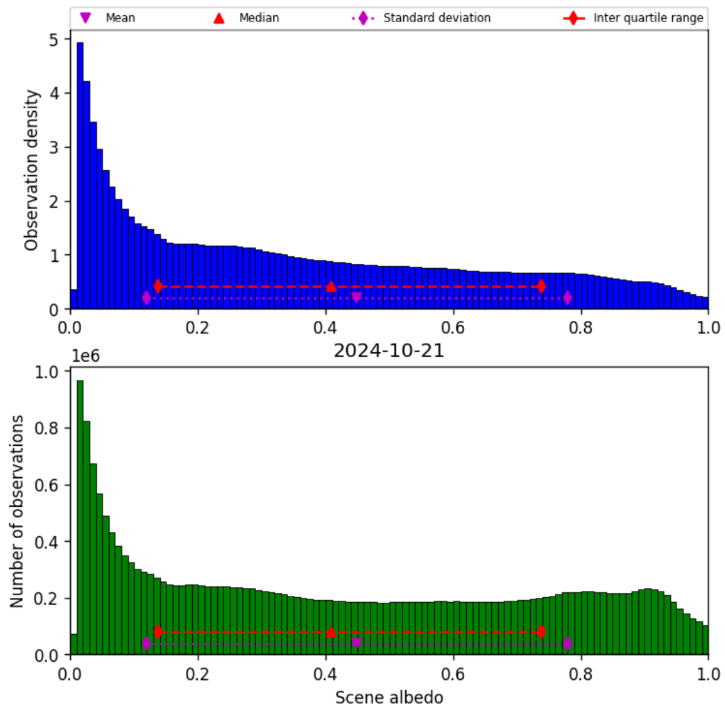
Figure 34: Histogram of “Scene albedo” for 2024-10-20 to 2024-10-22
