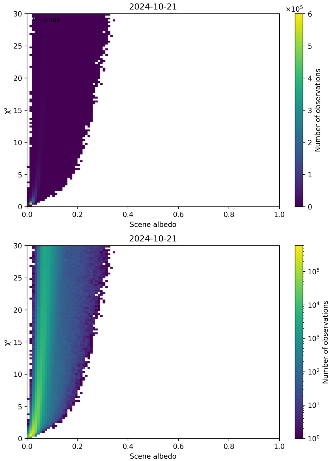
Figure 112: Scatter density plot of “Scene albedo” against “ \chi^2 ” for 2024-10-20 to 2024-10-22.
