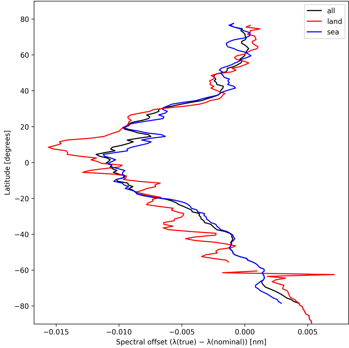
Figure 28: Zonal average of “Spectral offset ( \lambda_{\text{true}} - \lambda_{\text{nominal}} )” for 2024-10-20 to 2024-10-22.
