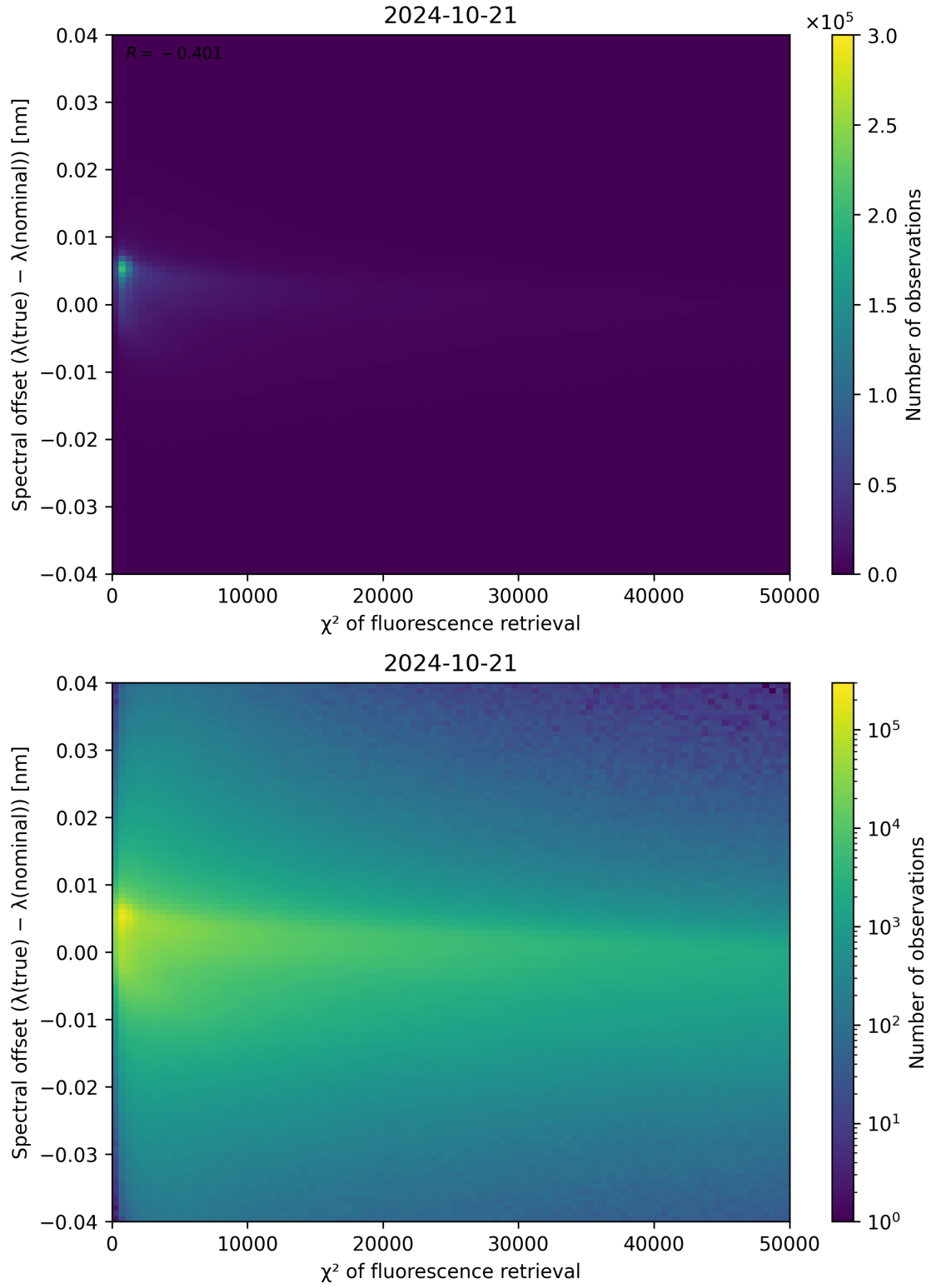
Figure 72: Scatter density plot of “ \chi^2 of fluorescence retrieval” against “Spectral offset ( \lambda_{\text{true}} - \lambda_{\text{nominal}} )” for 2024-10-20 to 2024-10-22.
