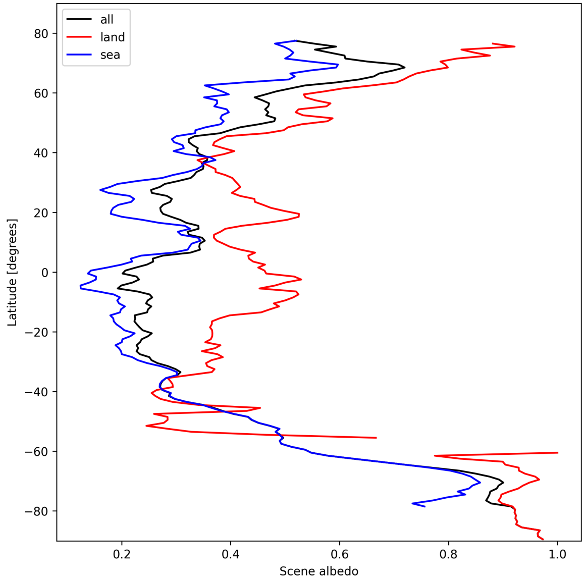
Figure 17: Zonal average of “Scene albedo” for 2024-10-20 to 2024-10-22.
