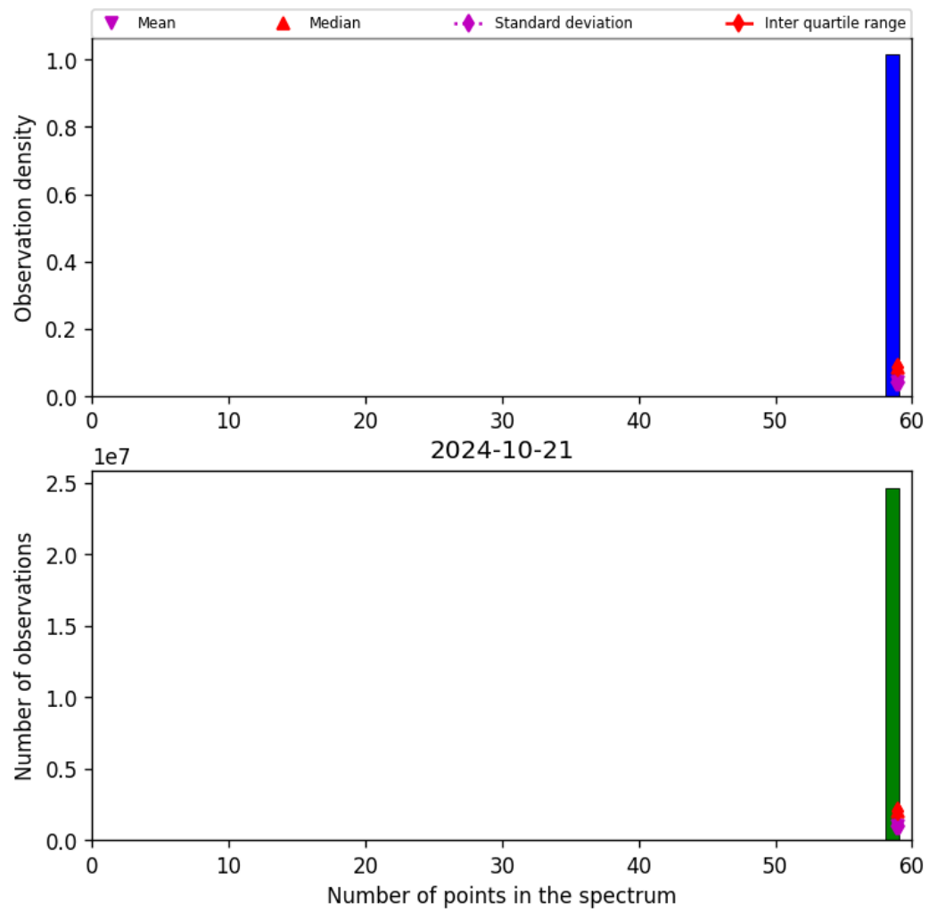
Figure 44: Histogram of “Number of points in the spectrum” for 2024-10-20 to 2024-10-22
