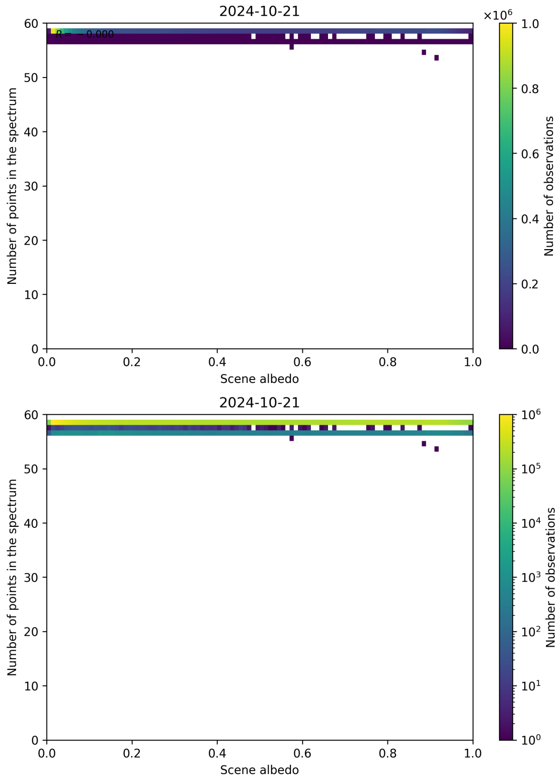
Figure 116: Scatter density plot of “Scene albedo” against “Number of points in the spectrum” for 2024-10-20 to 2024-10-22.
