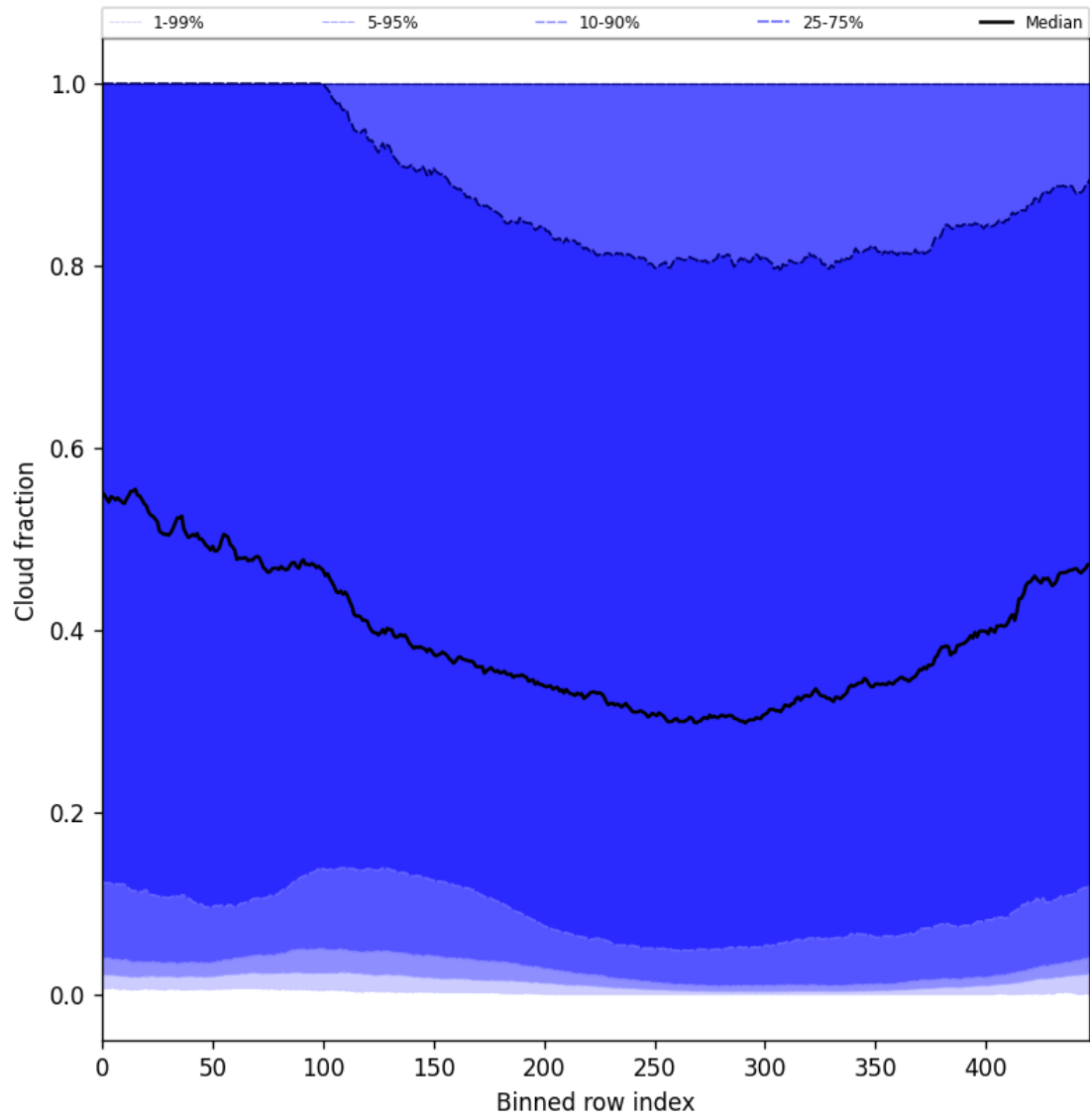
Figure 49: Along track statistics of “Cloud fraction” for 2024-10-20 to 2024-10-22
