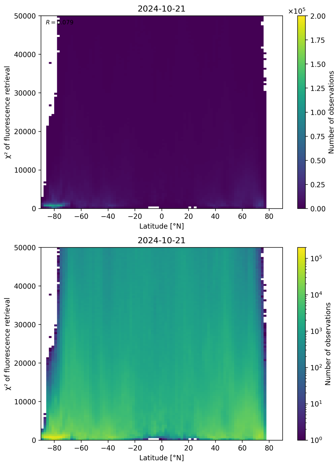
Figure 98: Scatter density plot of “Latitude” against “ \chi^2 of fluorescence retrieval” for 2024-10-20 to 2024-10-22.
