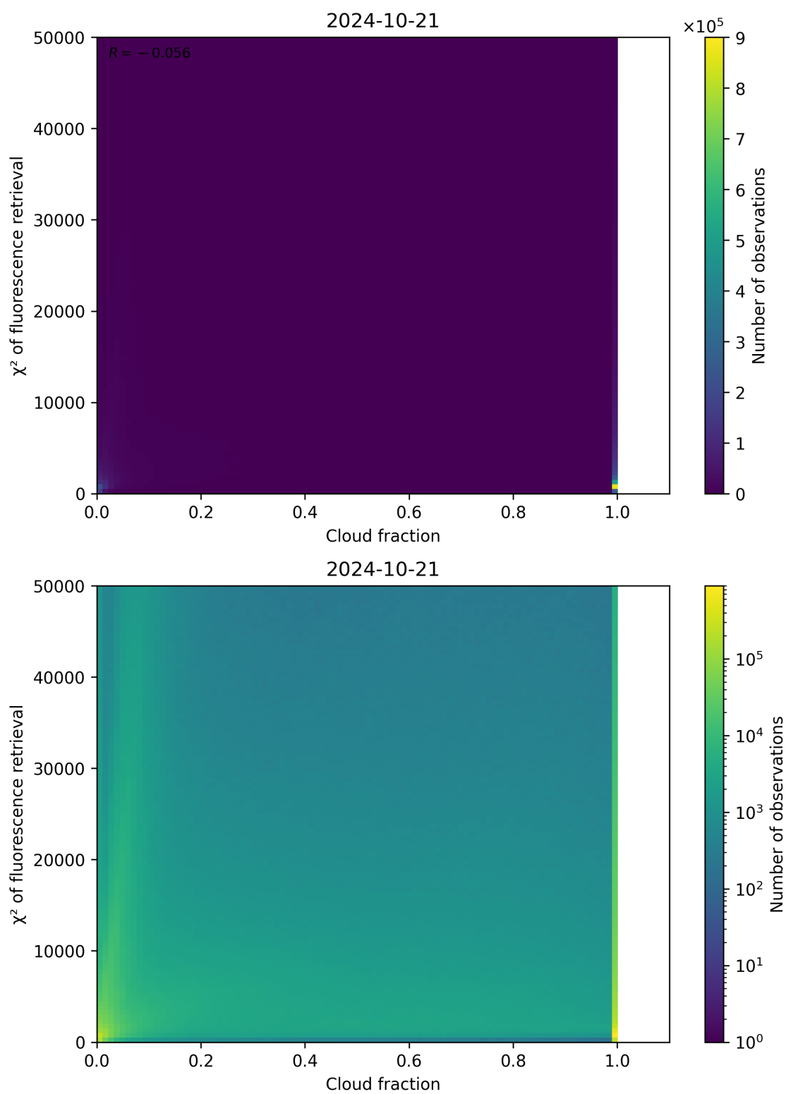
Figure 78: Scatter density plot of “Cloud fraction” against “ \chi^2 of fluorescence retrieval” for 2024-10-20 to 2024-10-22.
