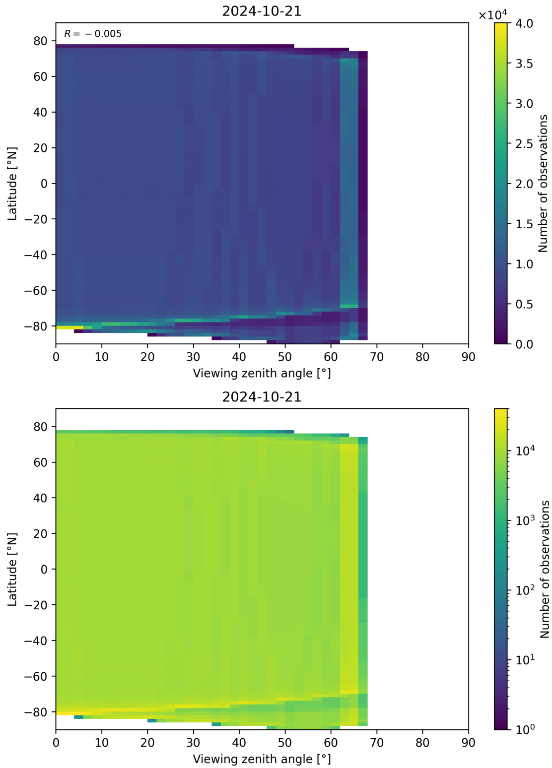
Figure 135: Scatter density plot of “Viewing zenith angle” against “Latitude” for 2024-10-20 to 2024-10-22.
