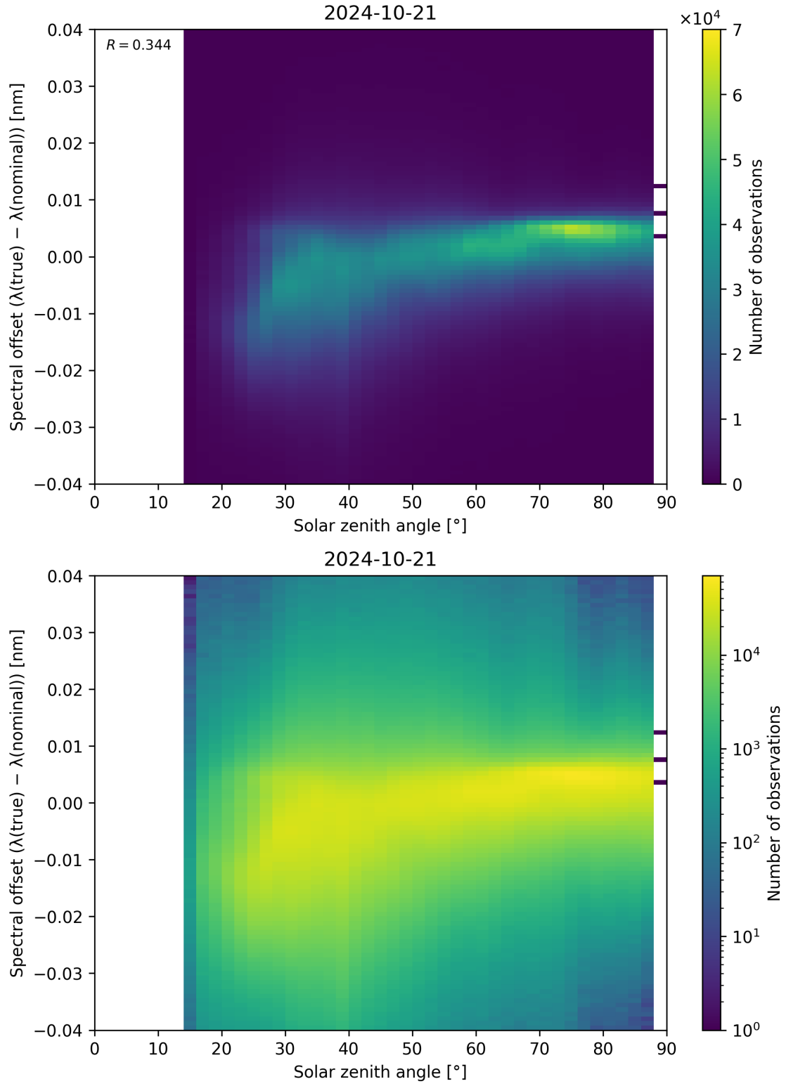
Figure 128: Scatter density plot of “Solar zenith angle” against “Spectral offset ( \lambda_{\text{true}} - \lambda_{\text{nominal}} )” for 2024-10-20 to 2024-10-22.
