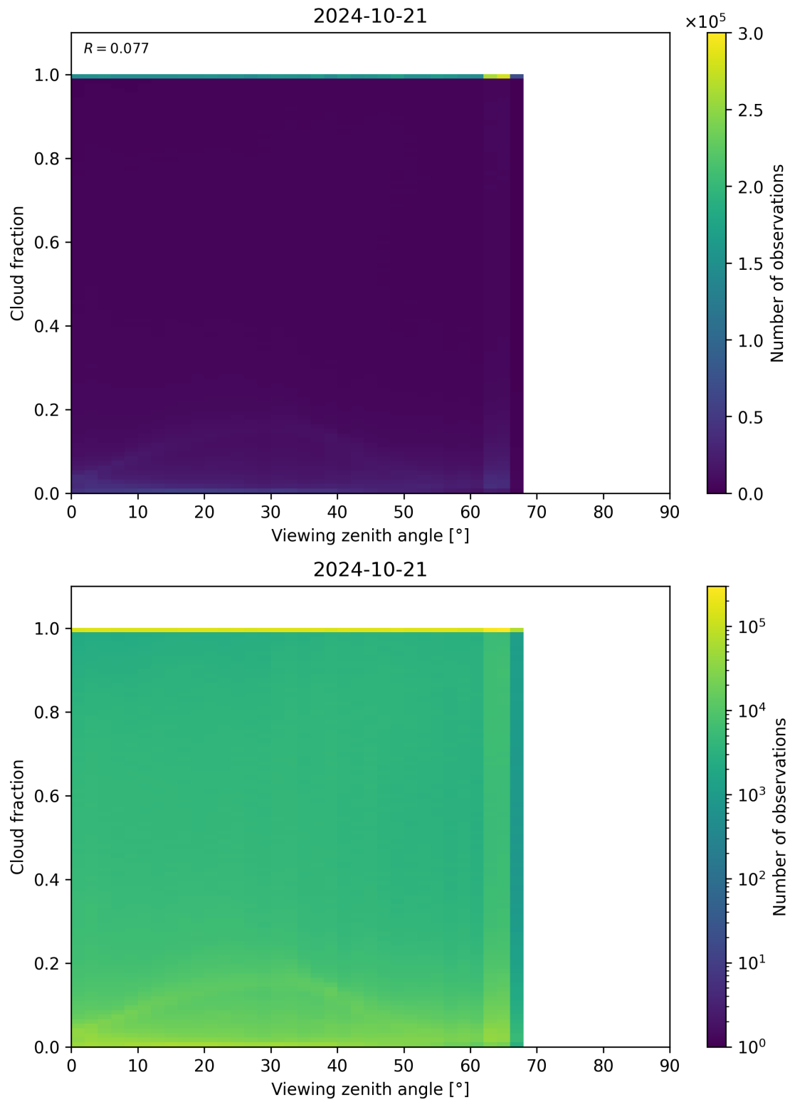
Figure 132: Scatter density plot of “Viewing zenith angle” against “Cloud fraction” for 2024-10-20 to 2024-10-22.
