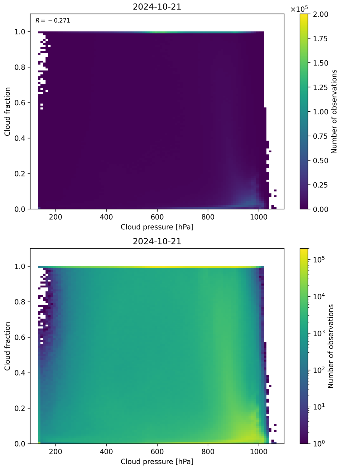
Figure 87: Scatter density plot of “Cloud pressure” against “Cloud fraction” for 2024-10-20 to 2024-10-22.
