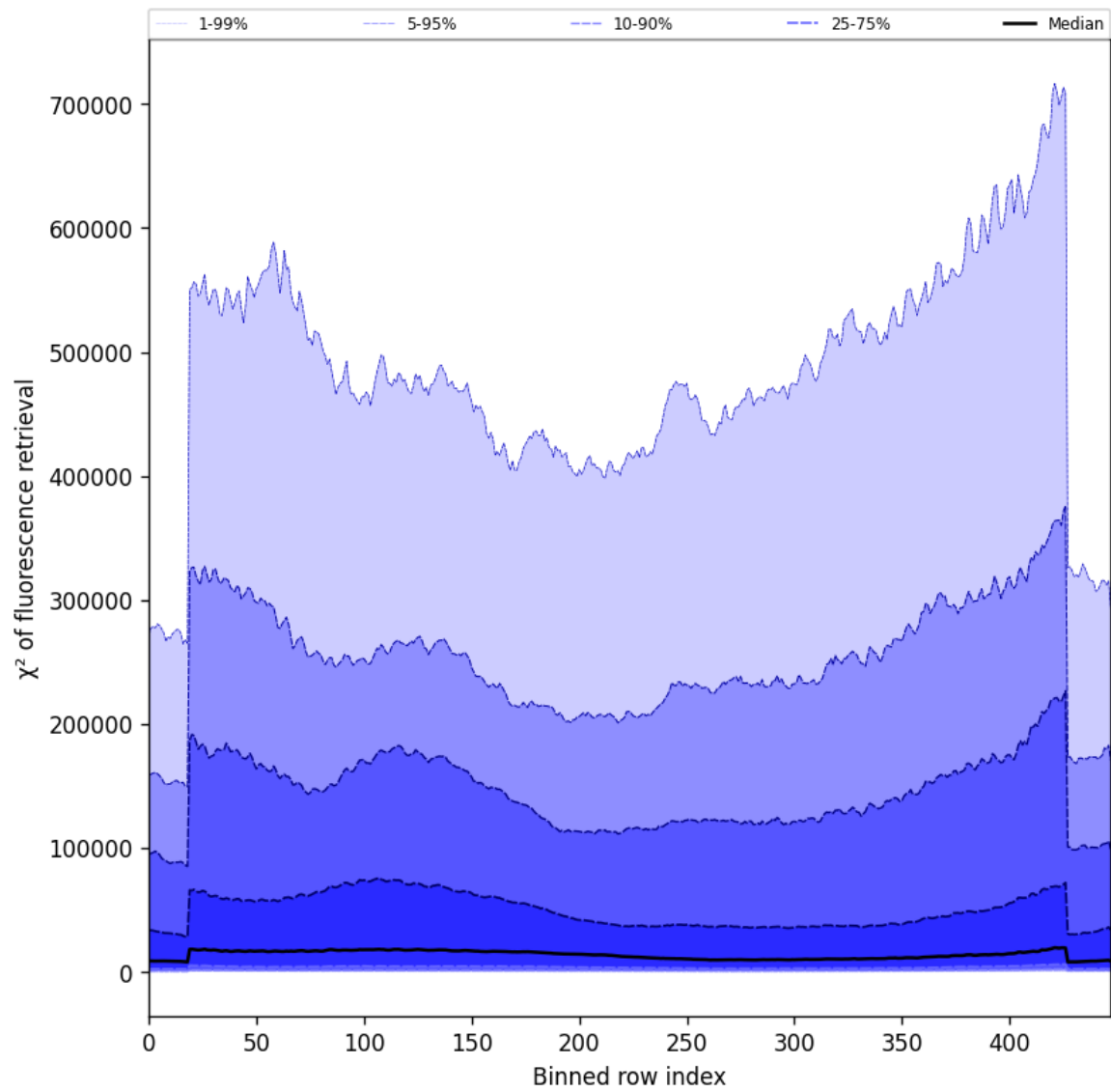
Figure 59: Along track statistics of “ \chi^2 of fluorescence retrieval” for 2024-10-20 to 2024-10-22
