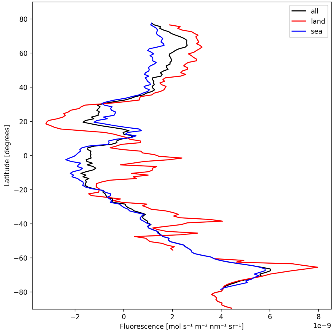
Figure 23: Zonal average of “Fluorescence” for 2024-10-20 to 2024-10-22.
