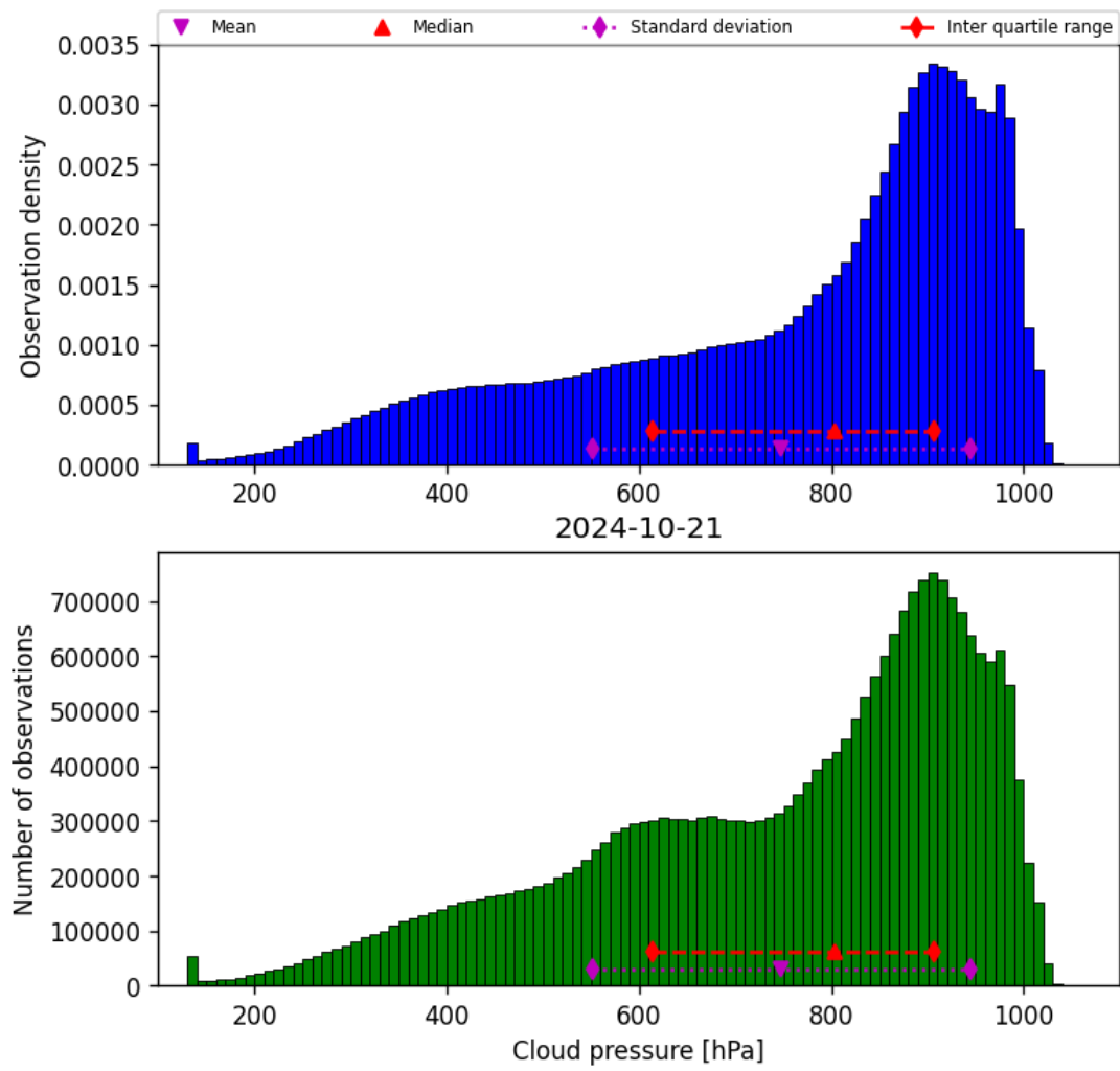
Figure 30: Histogram of “Cloud pressure” for 2024-10-20 to 2024-10-22
