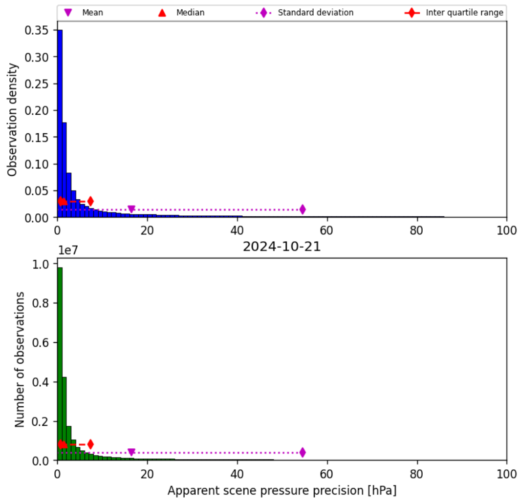
Figure 37: Histogram of “Apparent scene pressure precision” for 2024-10-20 to 2024-10-22
