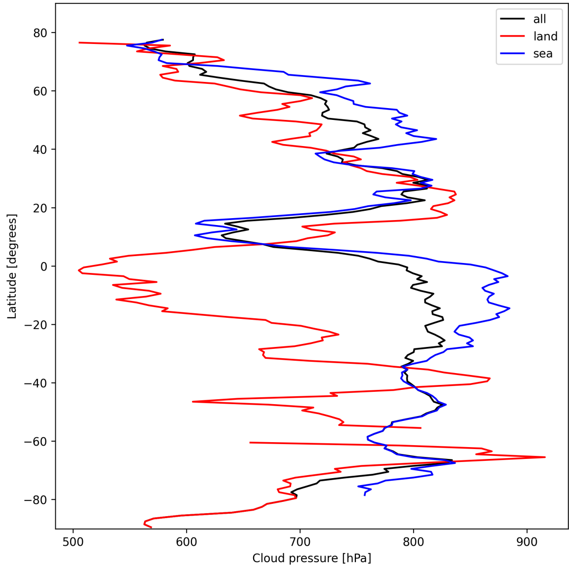
Figure 13: Zonal average of “Cloud pressure” for 2024-10-20 to 2024-10-22.
