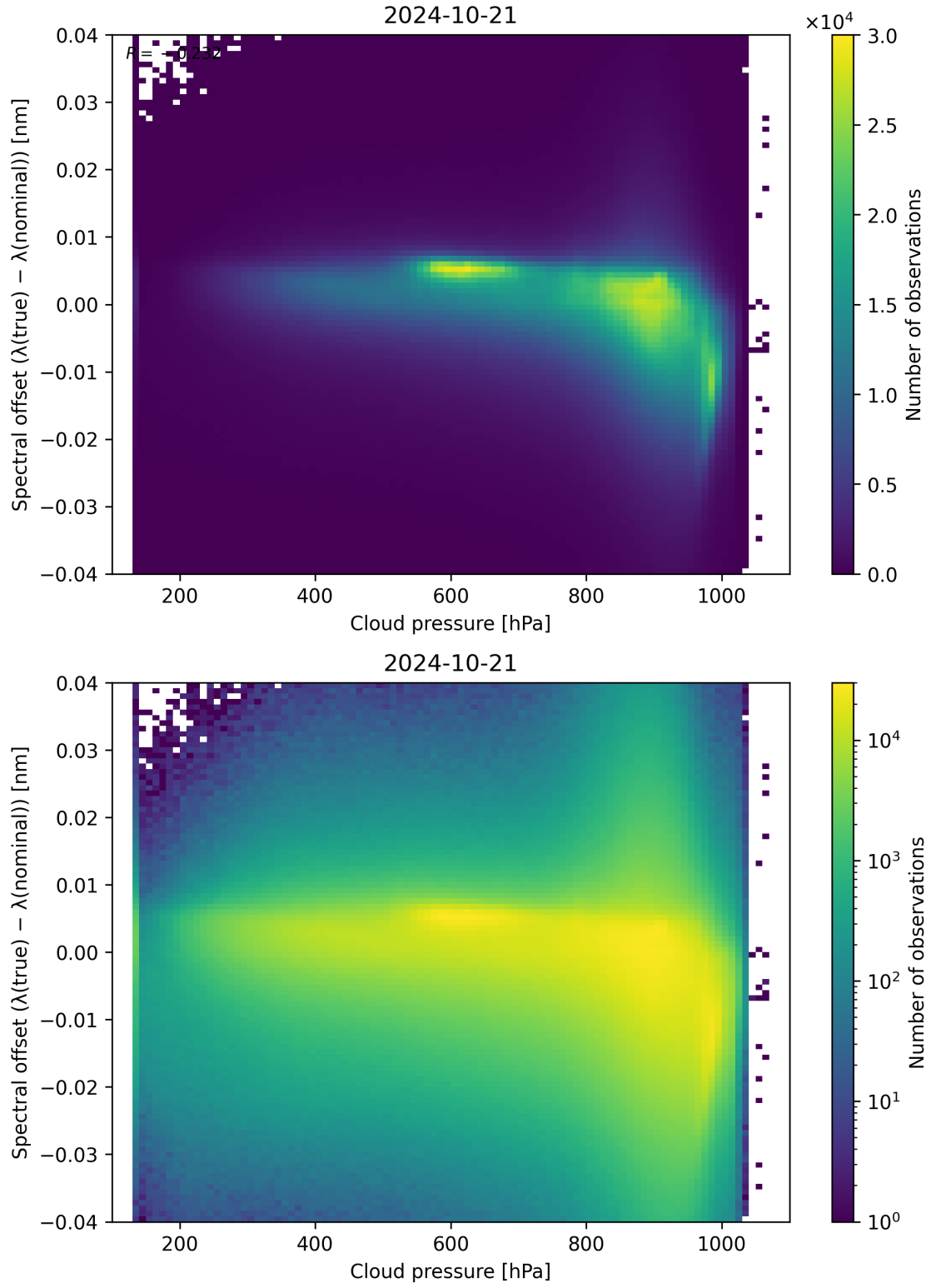
Figure 92: Scatter density plot of “Cloud pressure” against “Spectral offset ( \lambda_{\text{true}} - \lambda_{\text{nominal}} )” for 2024-10-20 to 2024-10-22.
