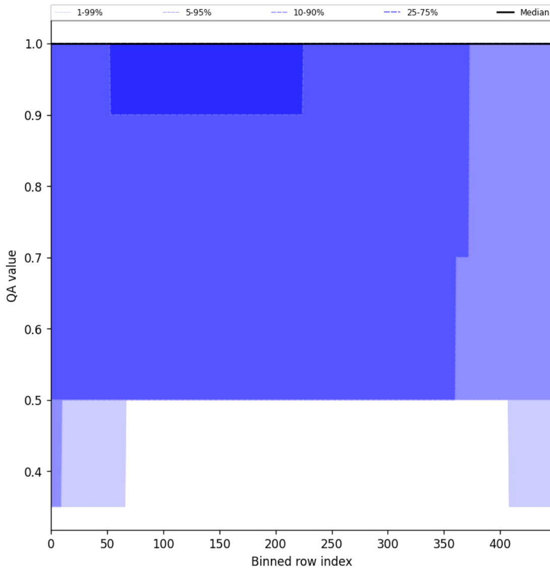
Figure 46: Along track statistics of “QA value” for 2024-10-20 to 2024-10-22
