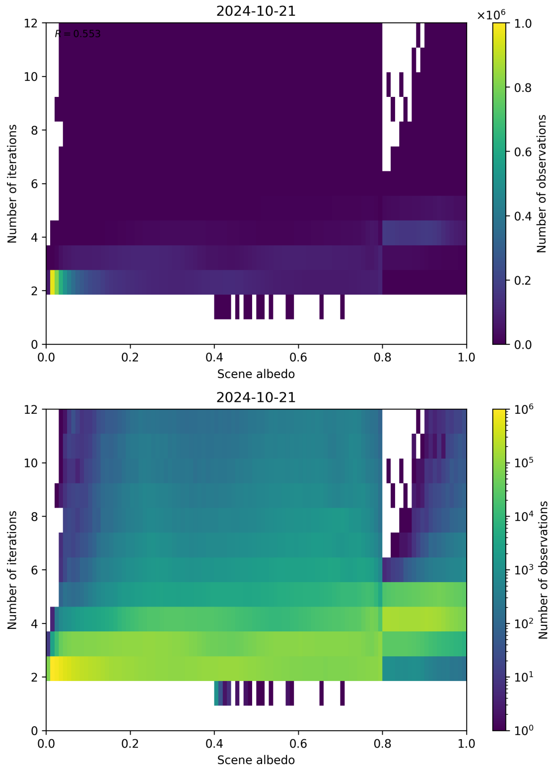
Figure 115: Scatter density plot of “Scene albedo” against “Number of iterations” for 2024-10-20 to 2024-10-22.
