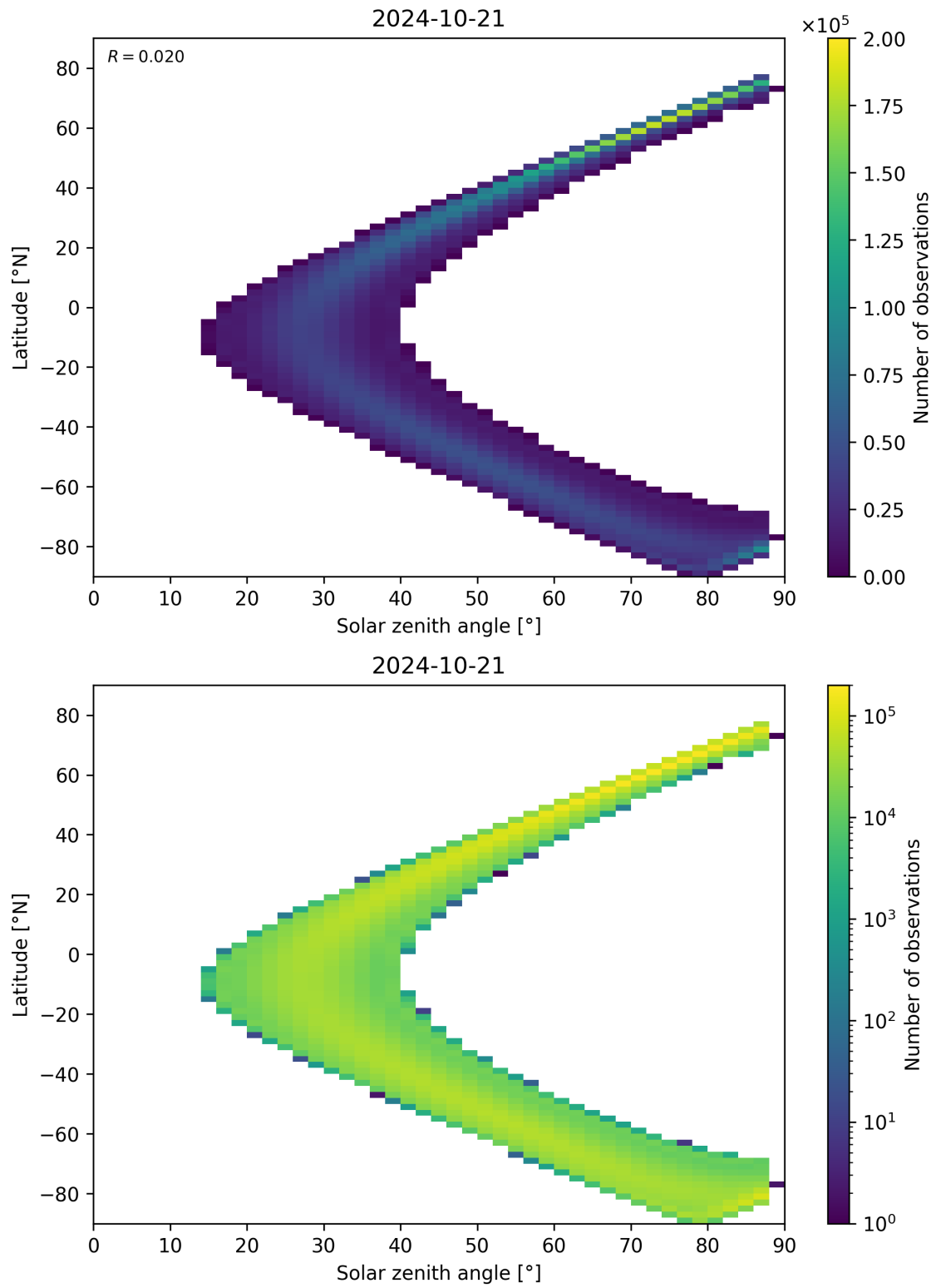
Figure 124: Scatter density plot of “Solar zenith angle” against “Latitude” for 2024-10-20 to 2024-10-22.
