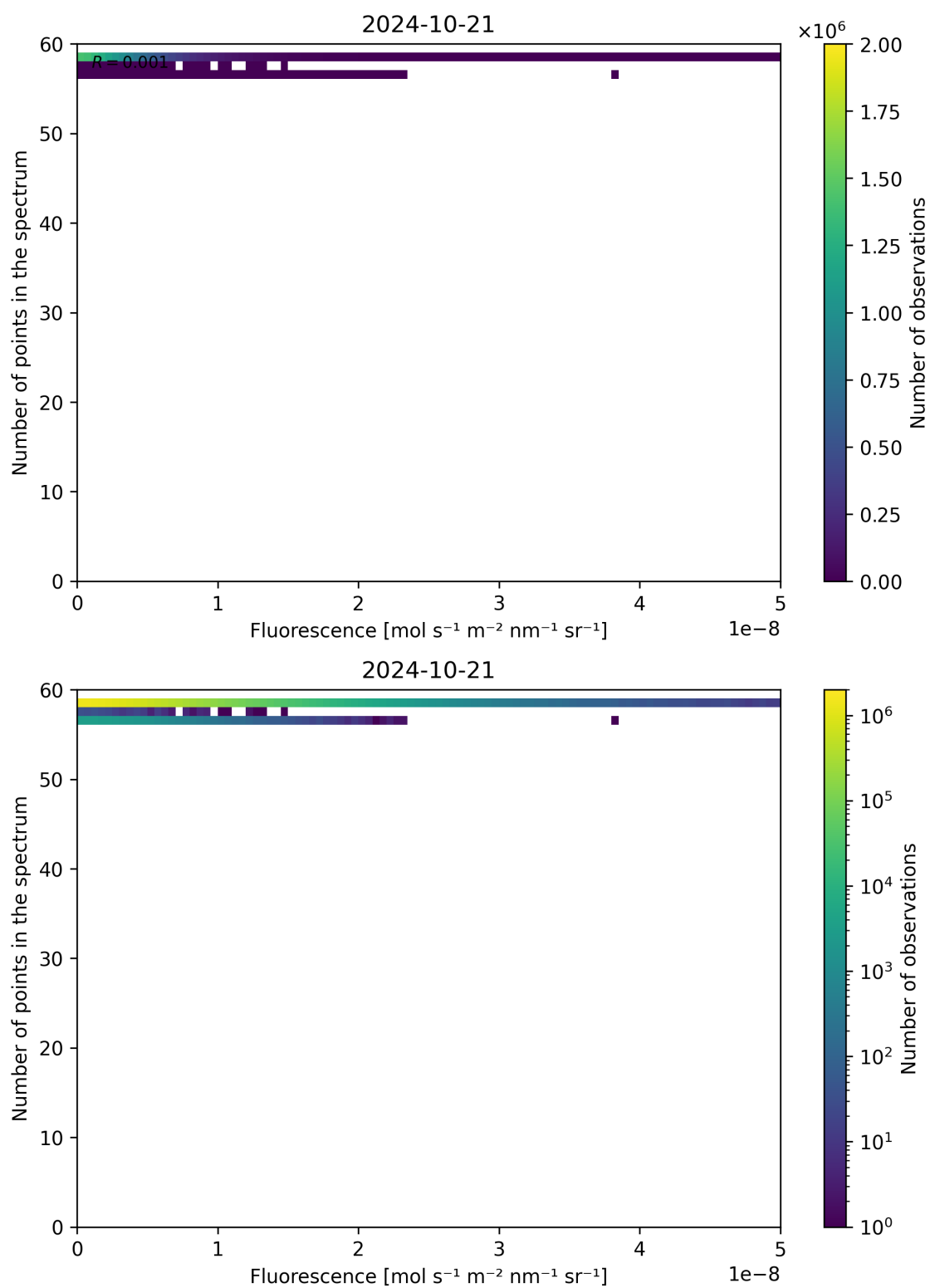
Figure 94: Scatter density plot of “Fluorescence” against “Number of points in the spectrum” for 2024-10-20 to 2024-10-22.
