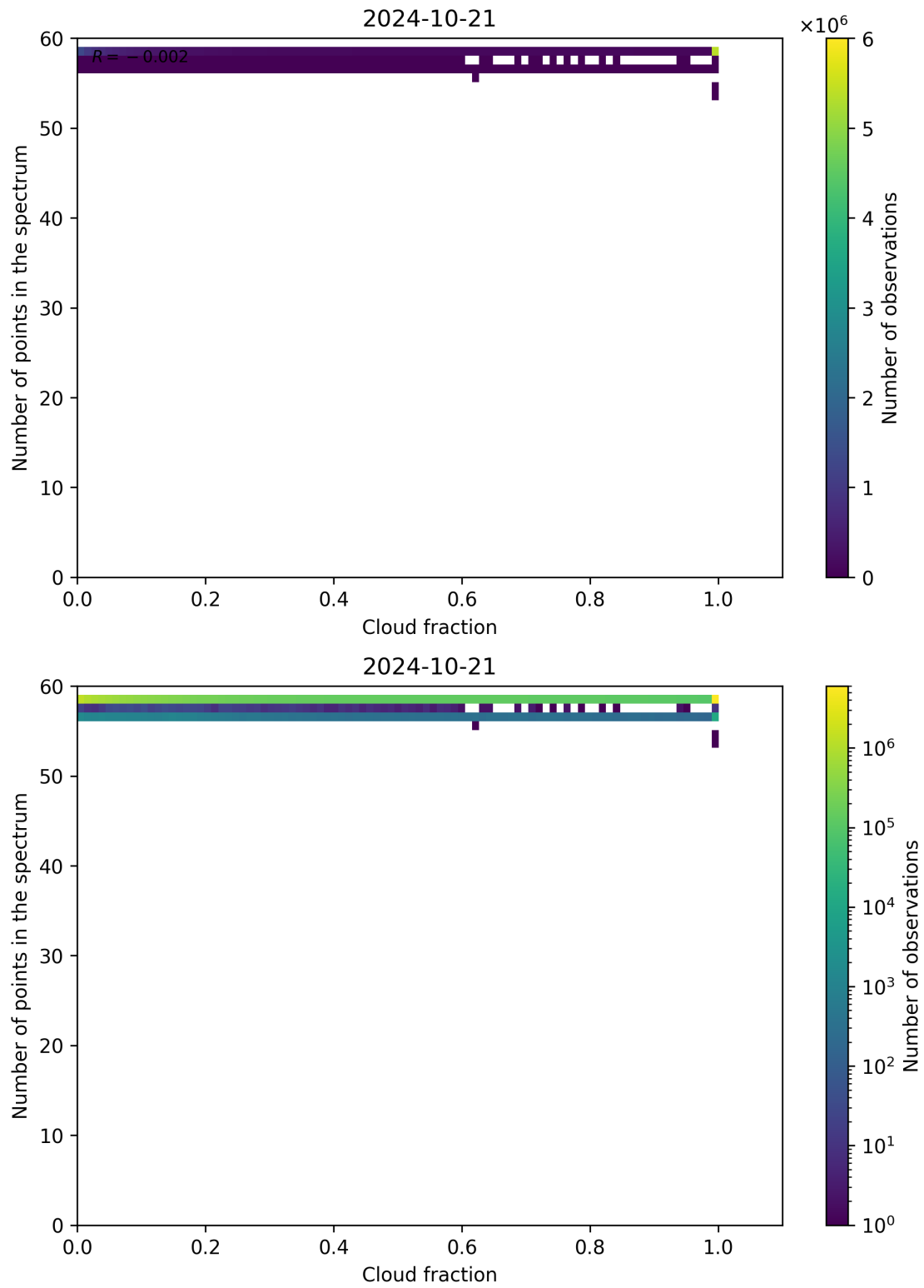
Figure 81: Scatter density plot of “Cloud fraction” against “Number of points in the spectrum” for 2024-10-20 to 2024-10-22.
