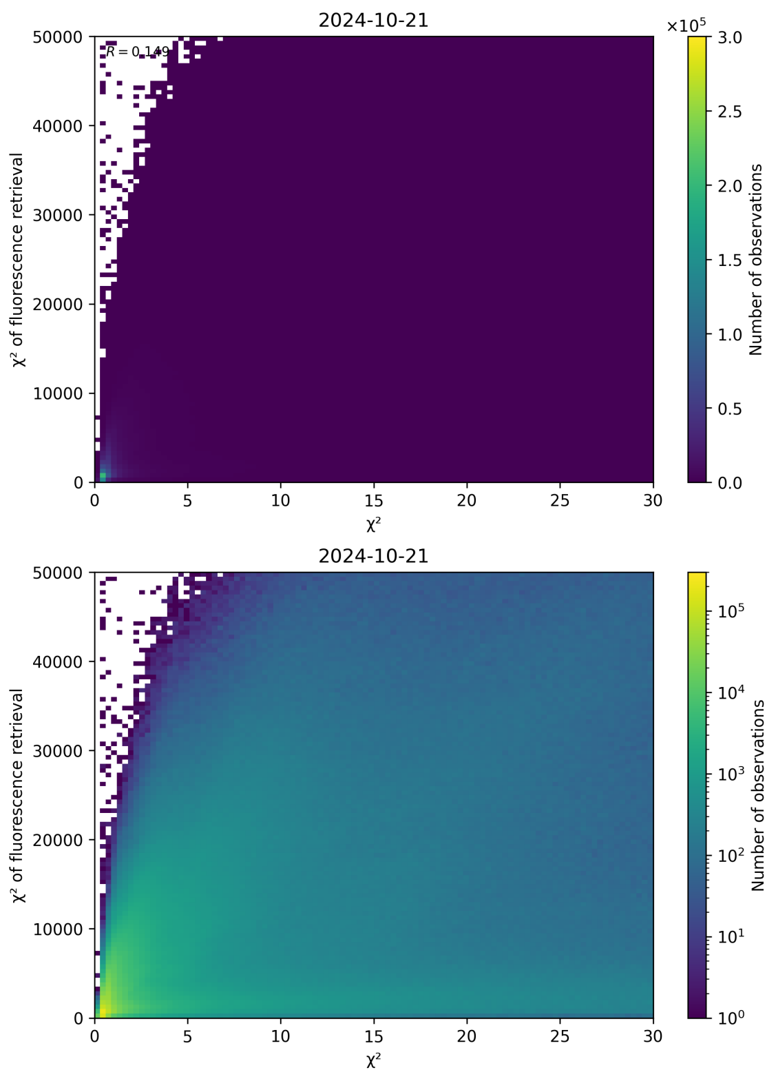
Figure 69: Scatter density plot of “ \chi^2 ” against “ \chi^2 of fluorescence retrieval” for 2024-10-20 to 2024-10-22.
