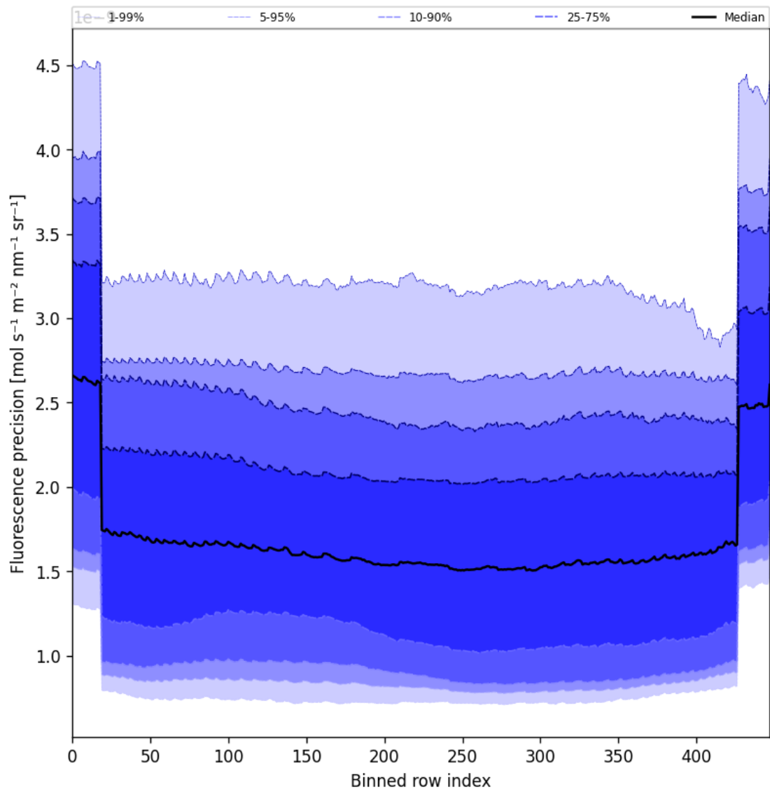
Figure 58: Along track statistics of “Fluorescence precision” for 2024-10-20 to 2024-10-22
