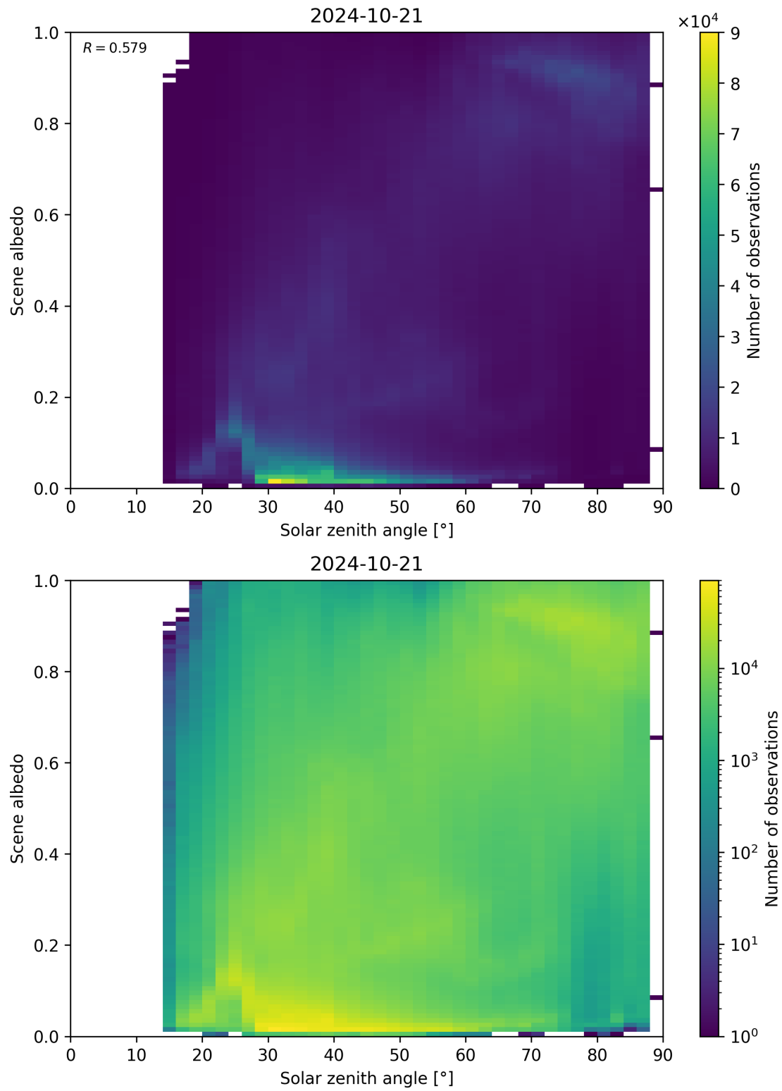
Figure 127: Scatter density plot of “Solar zenith angle” against “Scene albedo” for 2024-10-20 to 2024-10-22.
