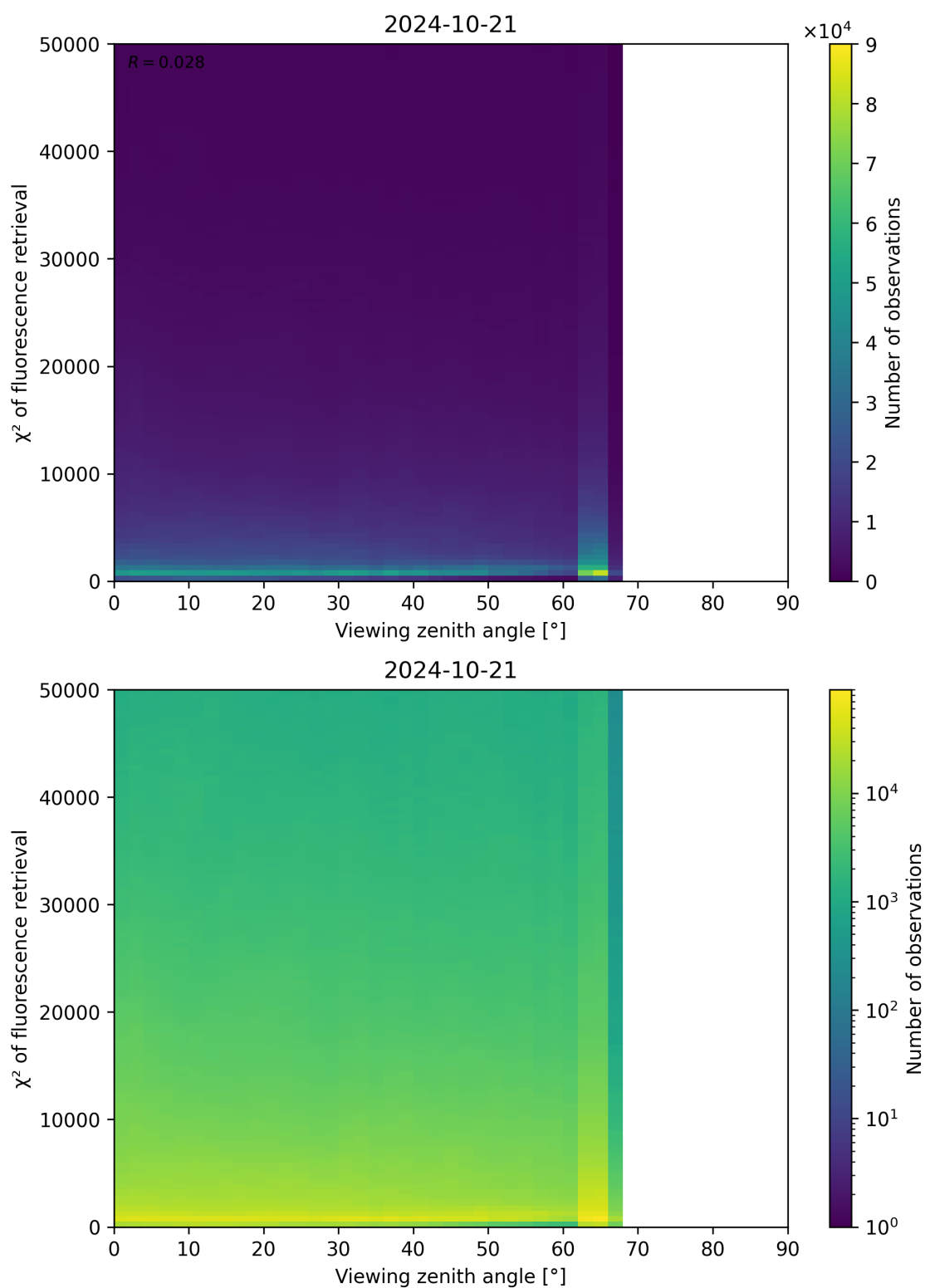
Figure 131: Scatter density plot of “Viewing zenith angle” against “ \chi^2 of fluorescence retrieval” for 2024-10-20 to 2024-10-22.
