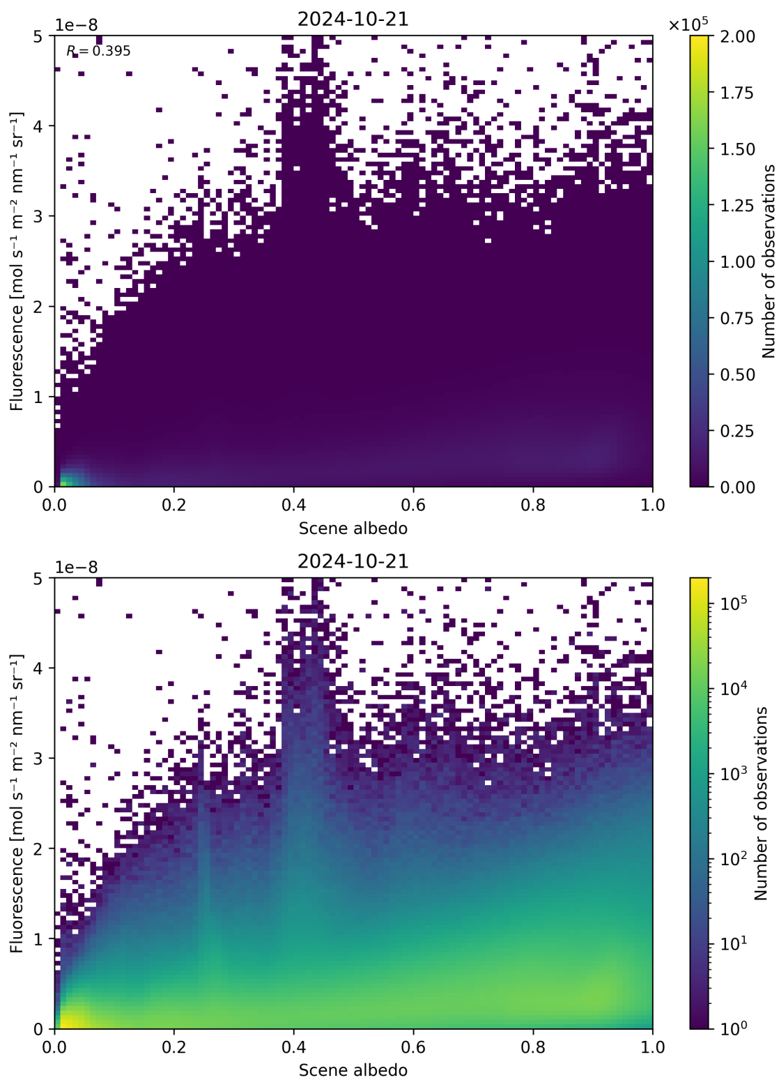
Figure 114: Scatter density plot of “Scene albedo” against “Fluorescence” for 2024-10-20 to 2024-10-22.
