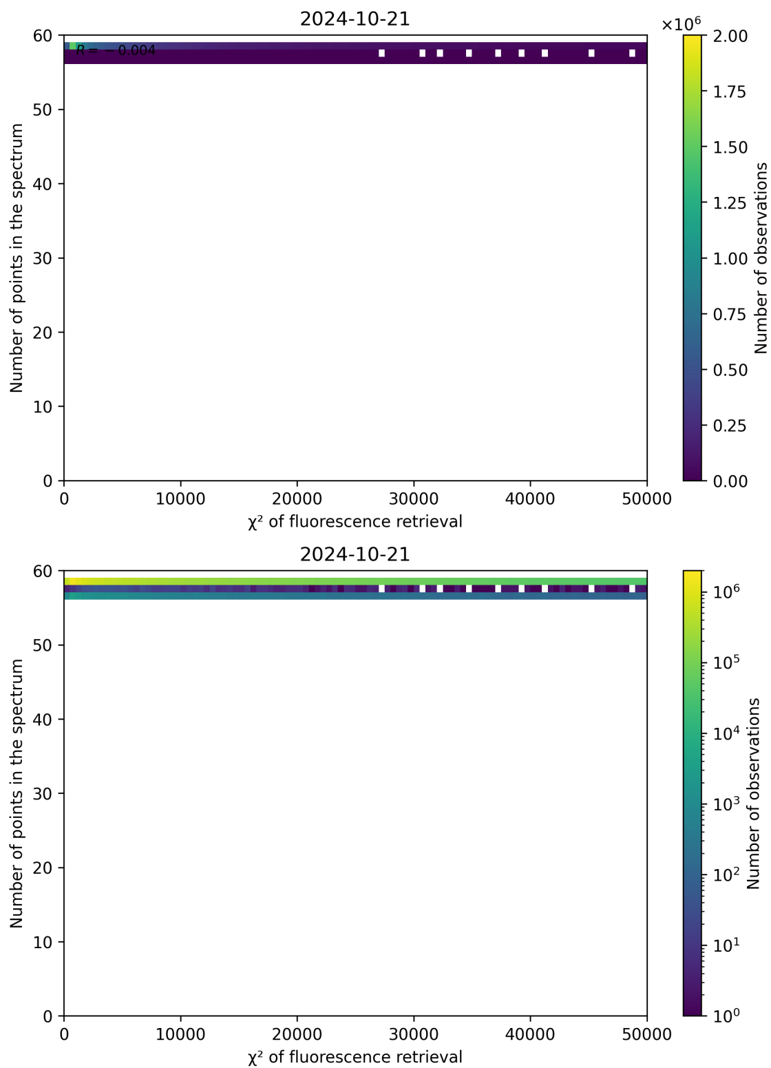
Figure 71: Scatter density plot of " \chi^2 of fluorescence retrieval" against "Number of points in the spectrum" for 2024-10-20 to 2024-10-22.
