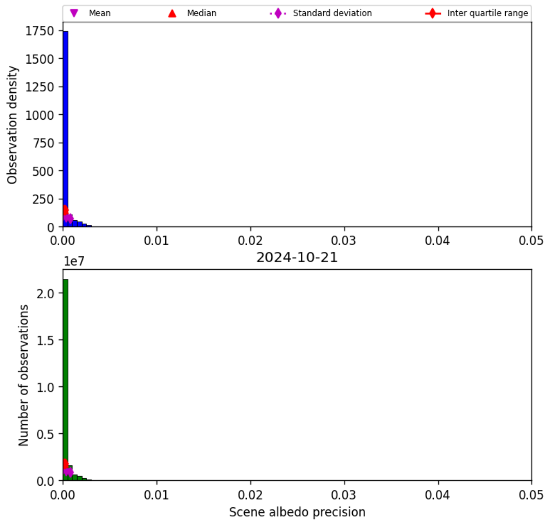
Figure 35: Histogram of “Scene albedo precision” for 2024-10-20 to 2024-10-22
