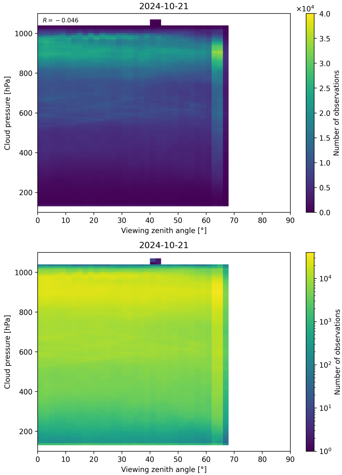
Figure 133: Scatter density plot of “Viewing zenith angle” against “Cloud pressure” for 2024-10-20 to 2024-10-22.
