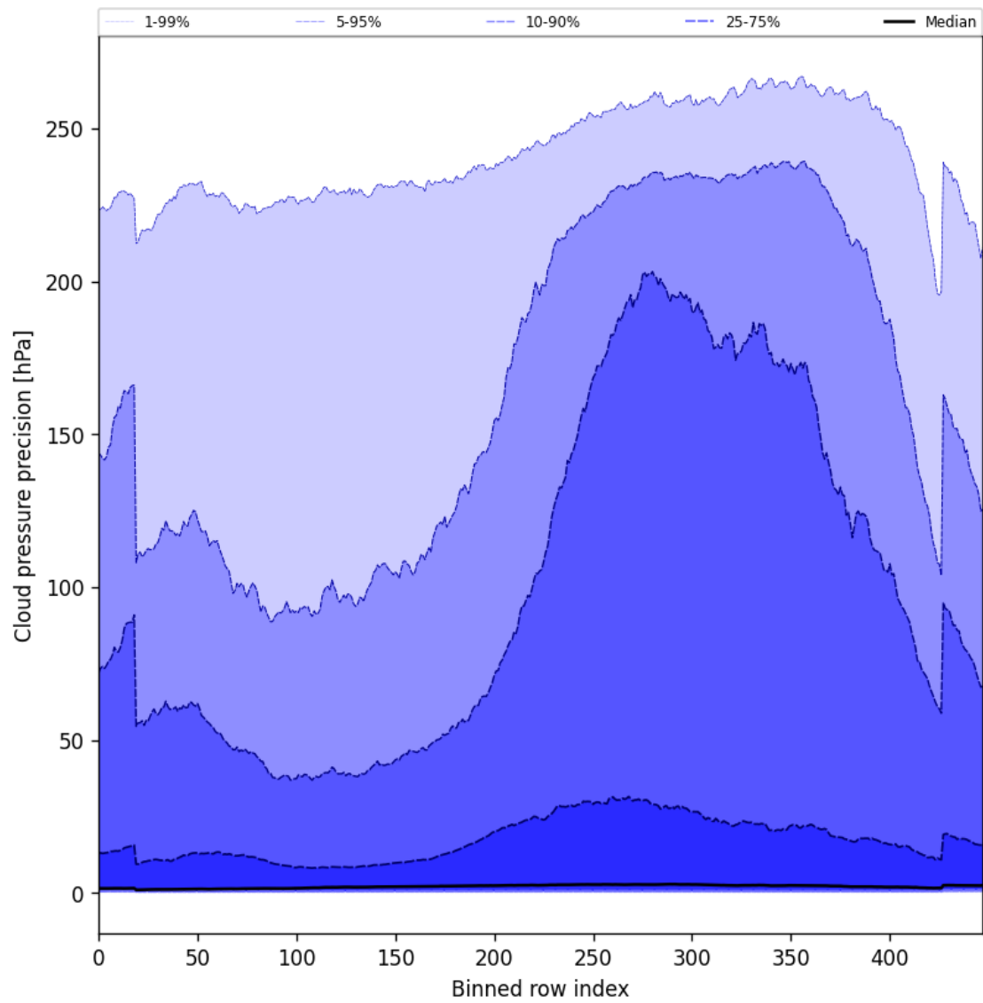
Figure 48: Along track statistics of “Cloud pressure precision” for 2024-10-20 to 2024-10-22
