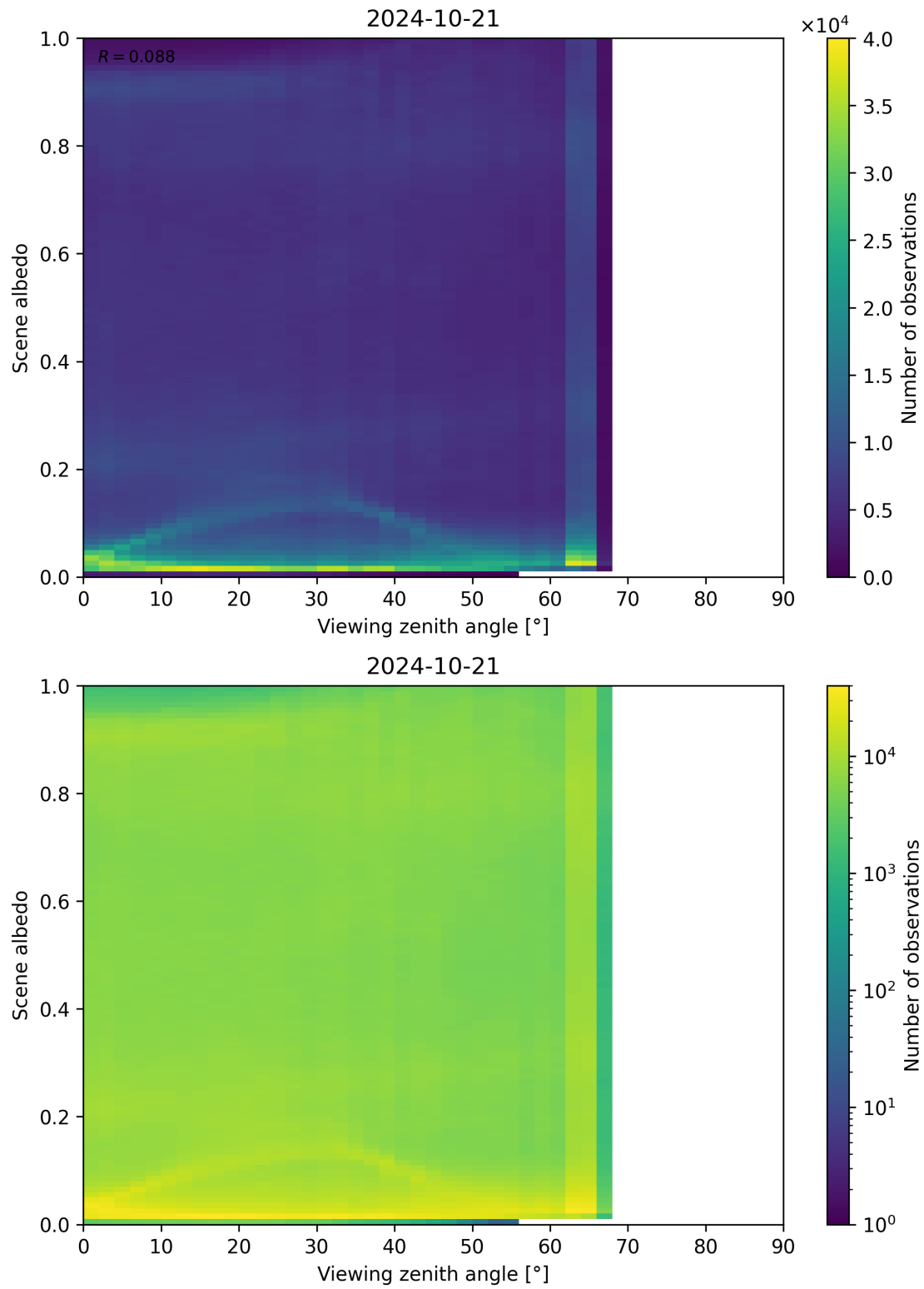
Figure 138: Scatter density plot of “Viewing zenith angle” against “Scene albedo” for 2024-10-20 to 2024-10-22.
