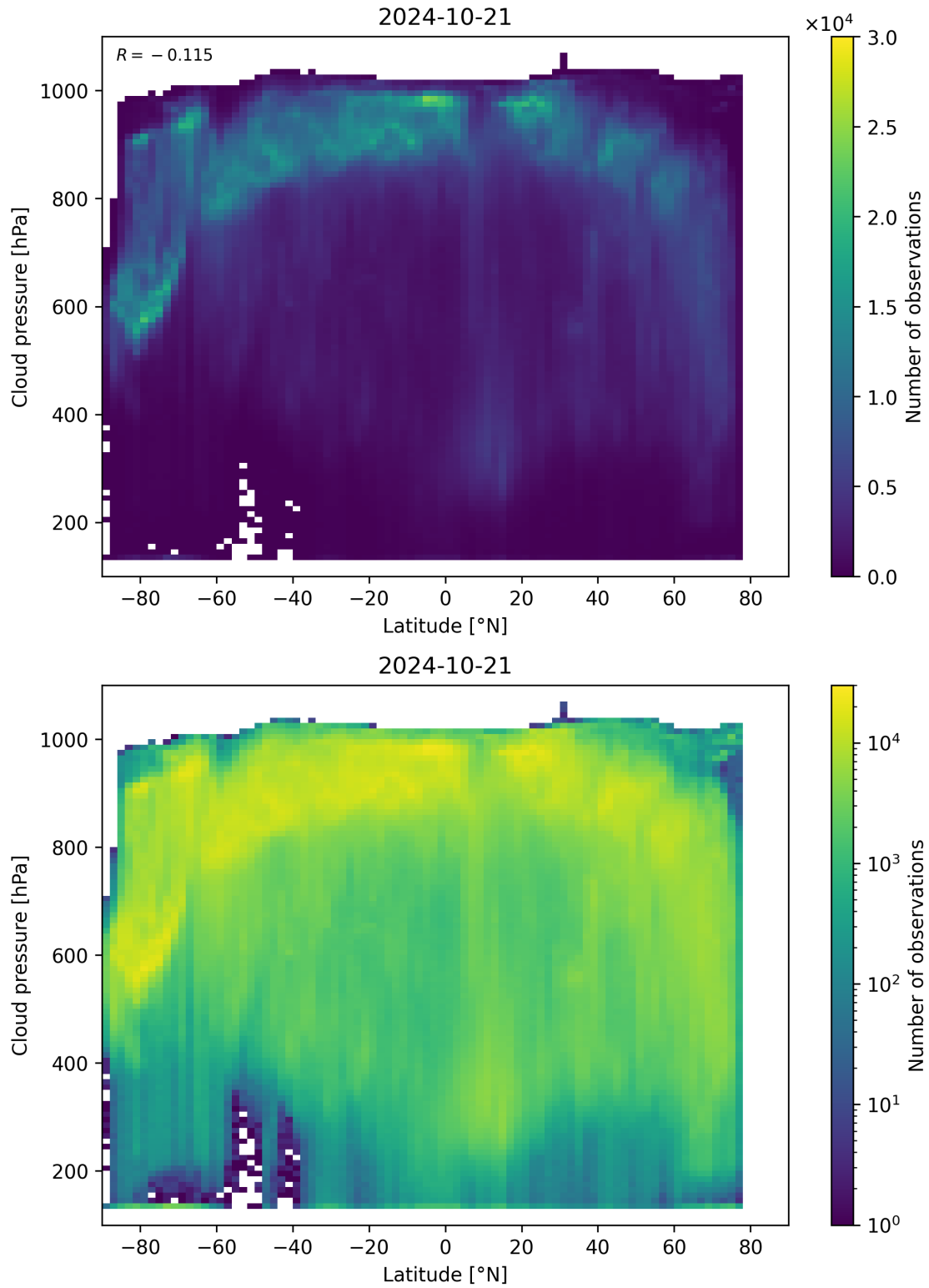
Figure 100: Scatter density plot of “Latitude” against “Cloud pressure” for 2024-10-20 to 2024-10-22.
