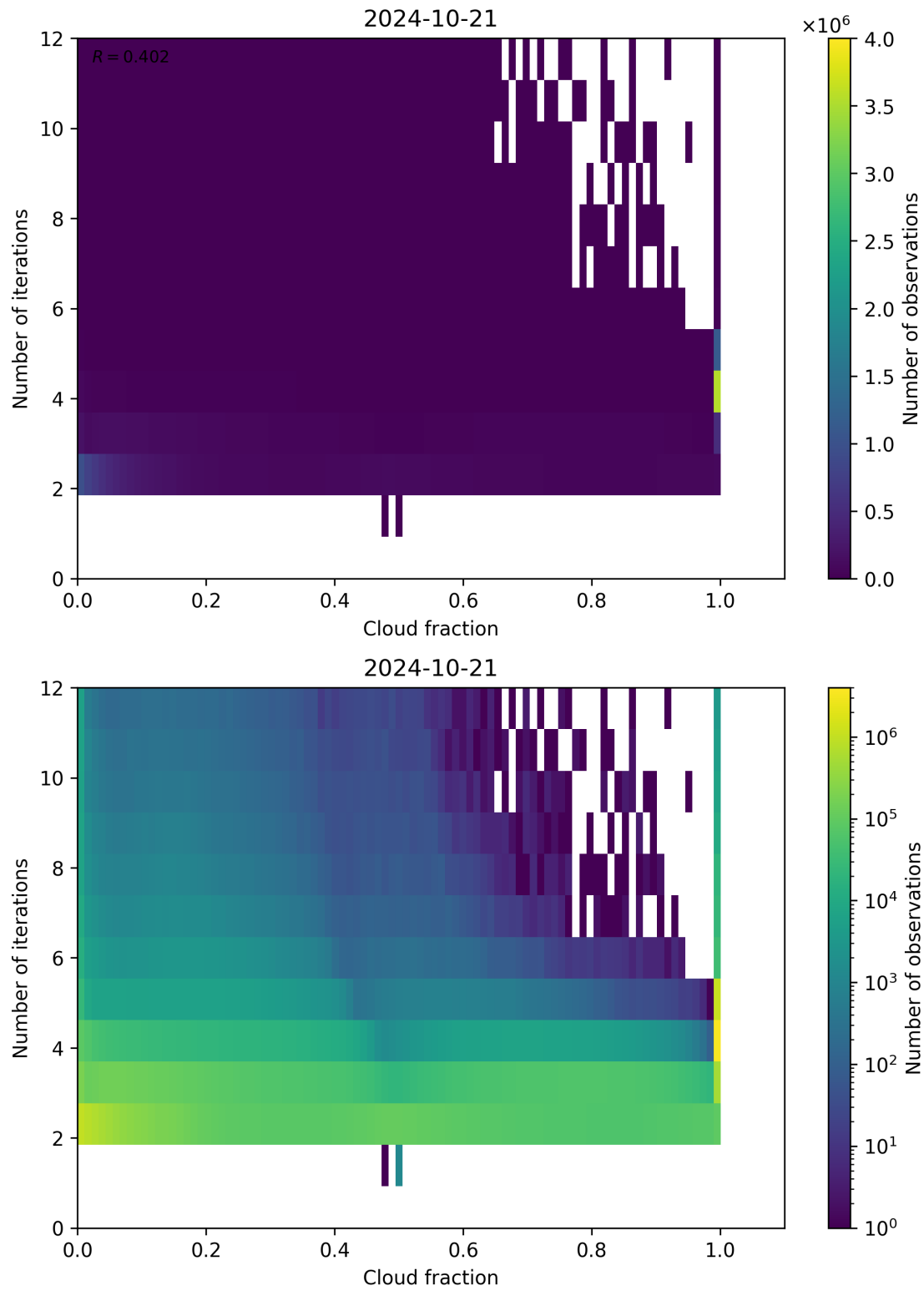
Figure 80: Scatter density plot of “Cloud fraction” against “Number of iterations” for 2024-10-20 to 2024-10-22.
