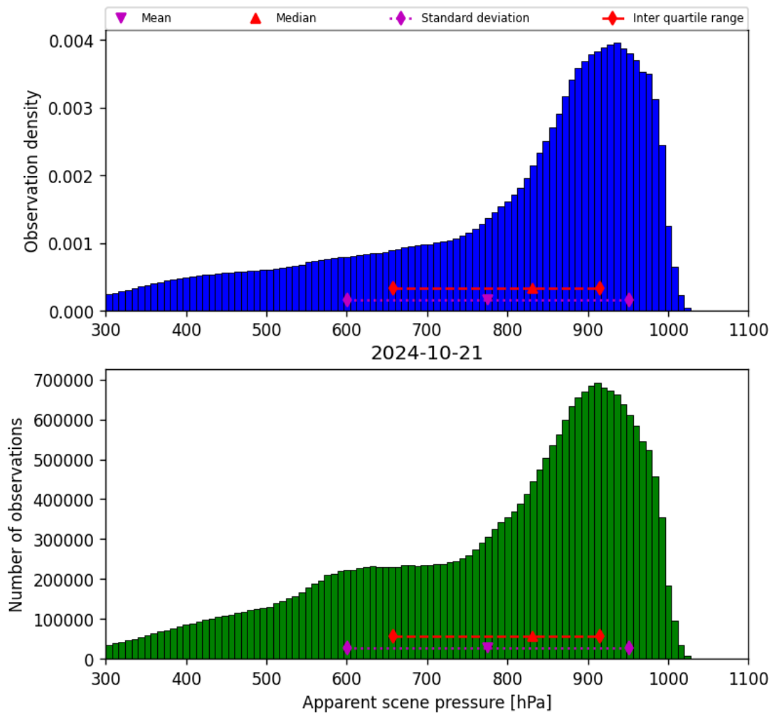
Figure 36: Histogram of “Apparent scene pressure” for 2024-10-20 to 2024-10-22
