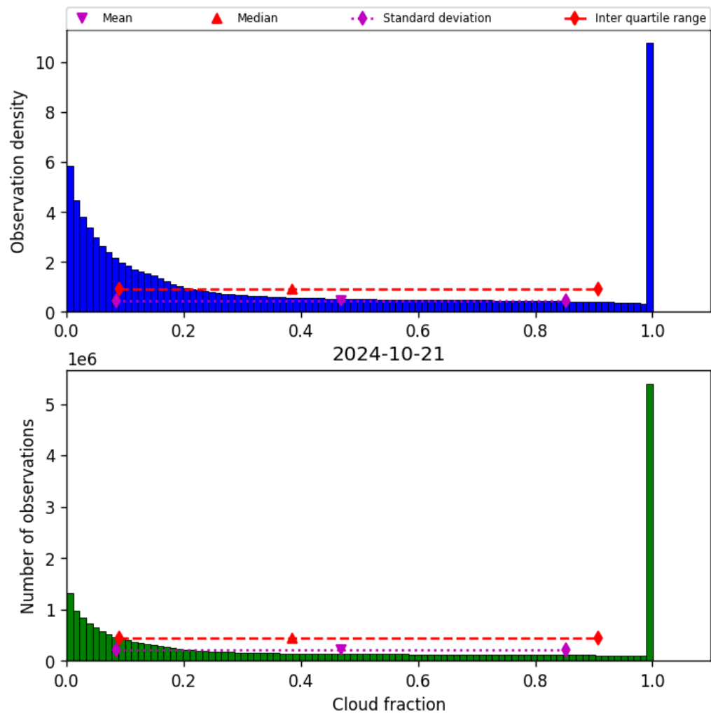
Figure 32: Histogram of “Cloud fraction” for 2024-10-20 to 2024-10-22
