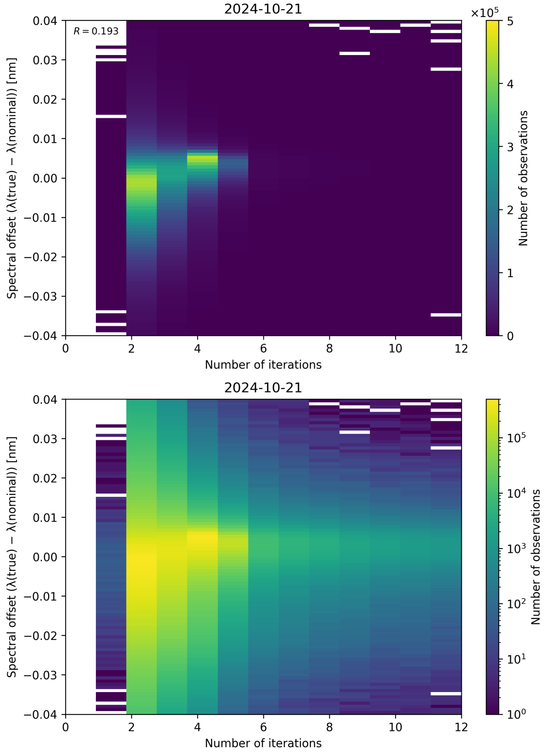
Figure 109: Scatter density plot of “Number of iterations” against “Spectral offset ( \lambda_{\text{true}} - \lambda_{\text{nominal}} )” for 2024-10-20 to 2024-10-22.
