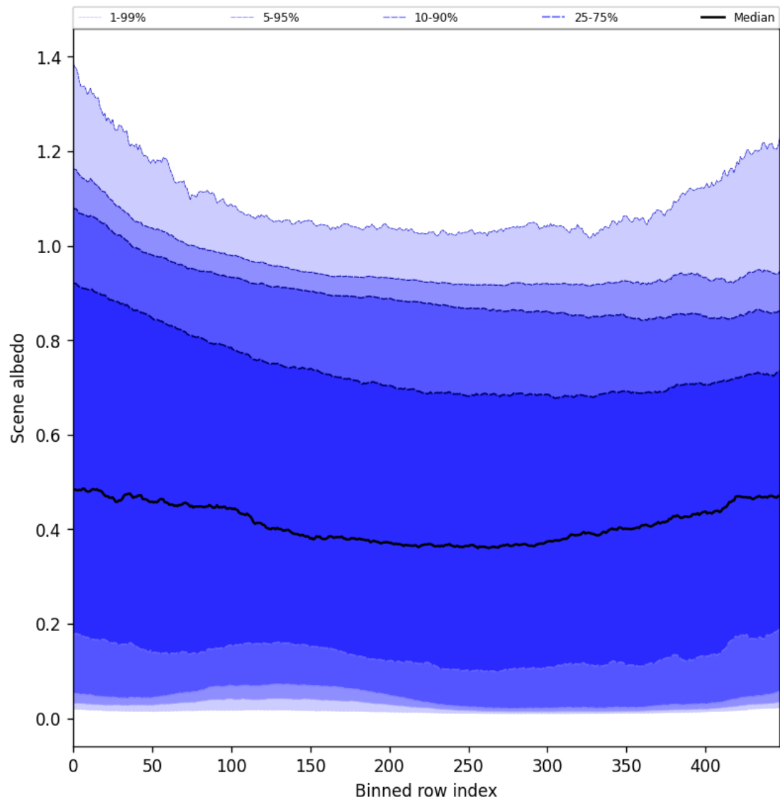
Figure 51: Along track statistics of “Scene albedo” for 2024-10-20 to 2024-10-22
