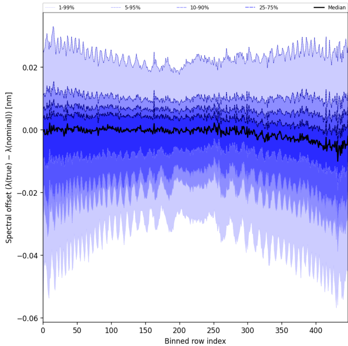
Figure 62: Along track statistics of “Spectral offset ( \lambda_{\text{true}} - \lambda_{\text{nominal}} )” for 2024-10-20 to 2024-10-22
