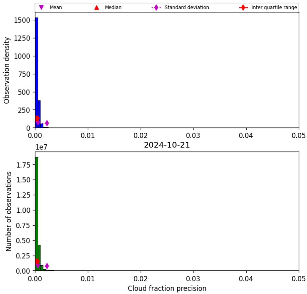
Figure 33: Histogram of “Cloud fraction precision” for 2024-10-20 to 2024-10-22
