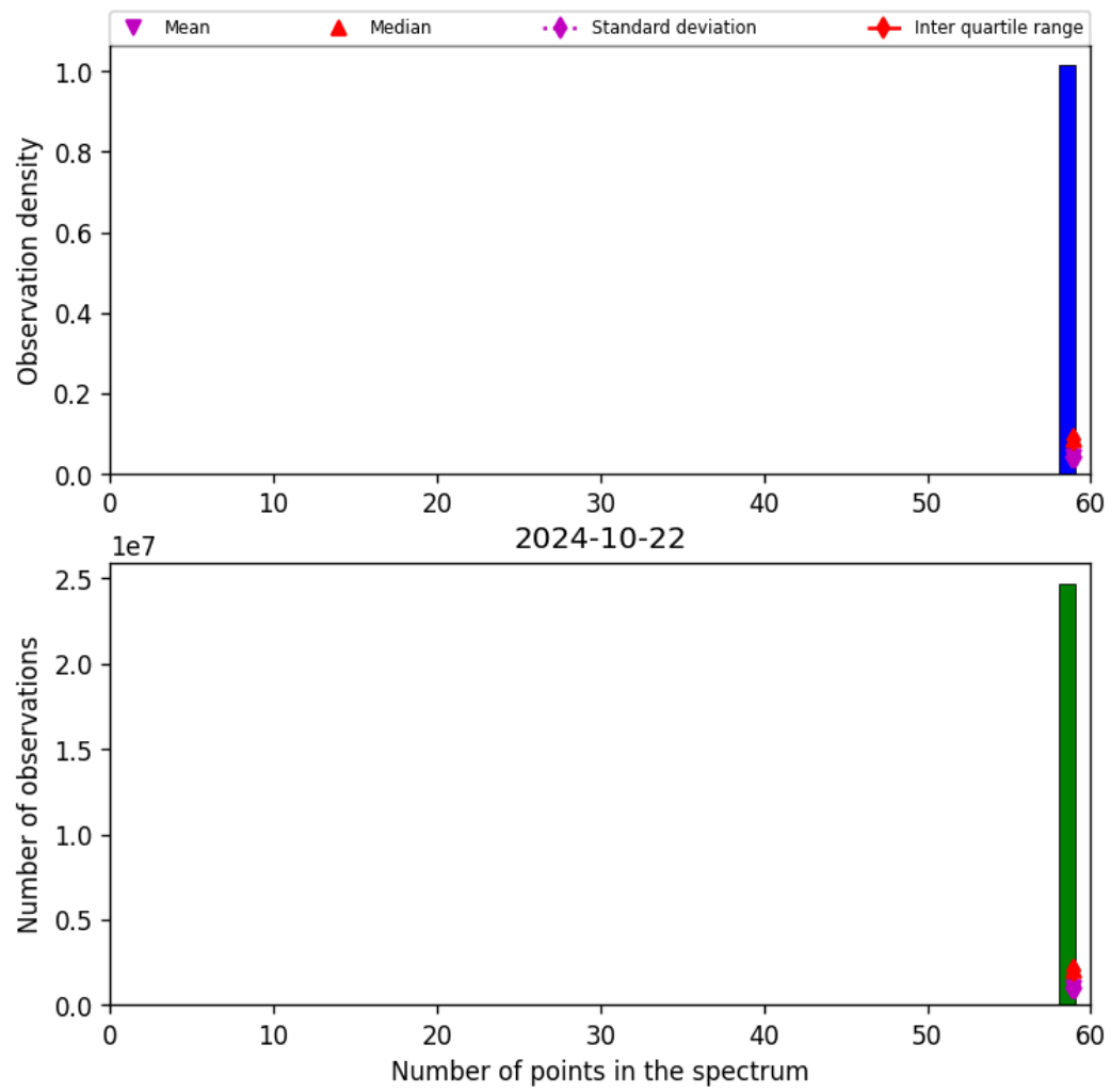
Figure 44: Histogram of “Number of points in the spectrum” for 2024-10-21 to 2024-10-23
