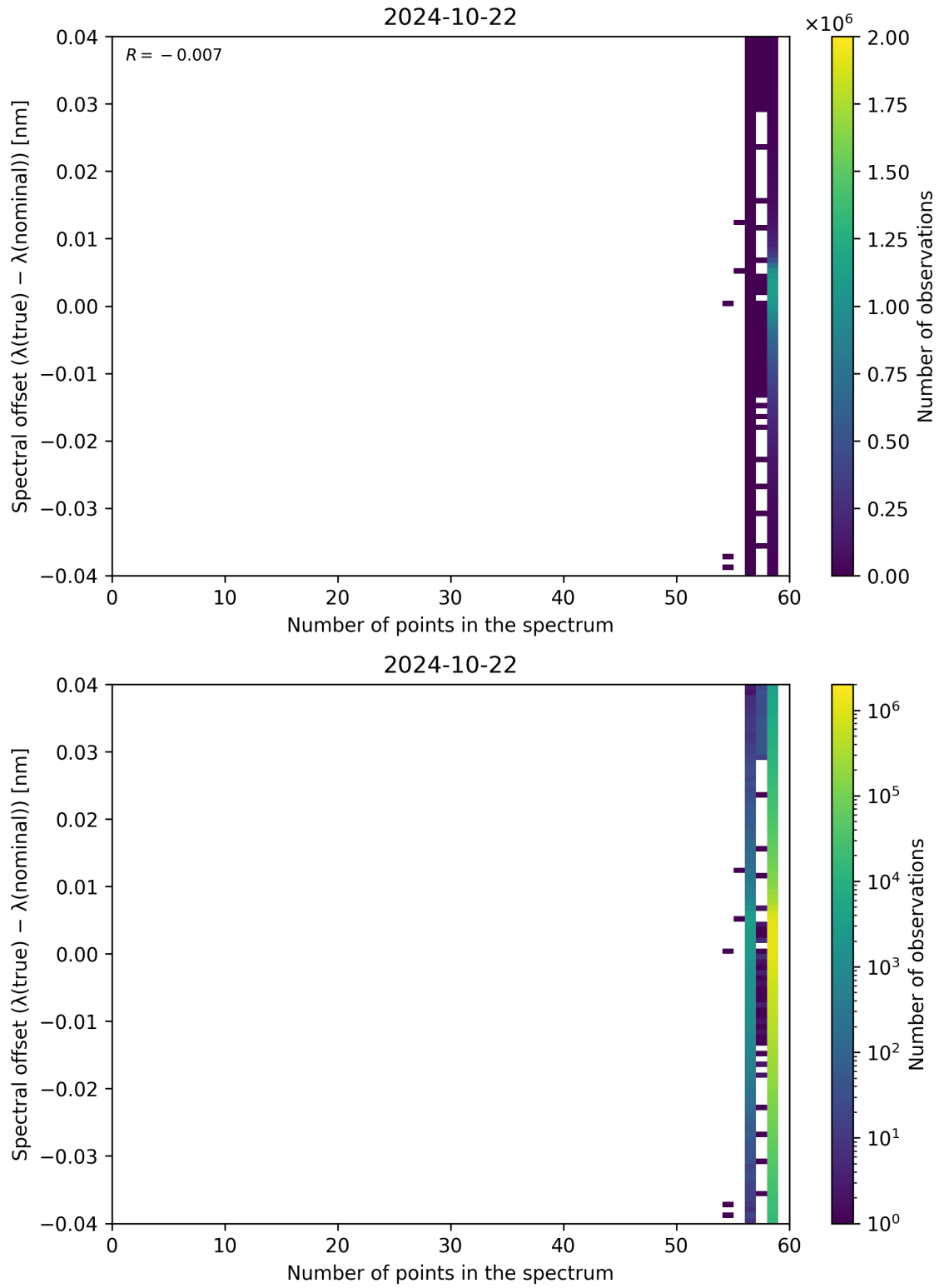
Figure 110: Scatter density plot of “Number of points in the spectrum” against “Spectral offset ( \lambda_{\text{true}} - \lambda_{\text{nominal}} )” for 2024-10-21 to 2024-10-23.
