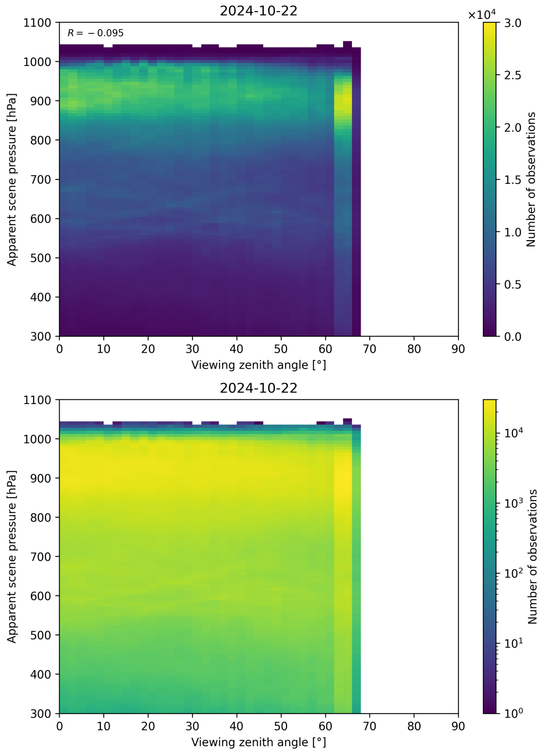
Figure 129: Scatter density plot of “Viewing zenith angle” against “Apparent scene pressure” for 2024-10-21 to 2024-10-23.
