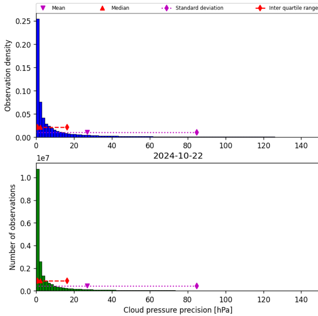
Figure 31: Histogram of “Cloud pressure precision” for 2024-10-21 to 2024-10-23
