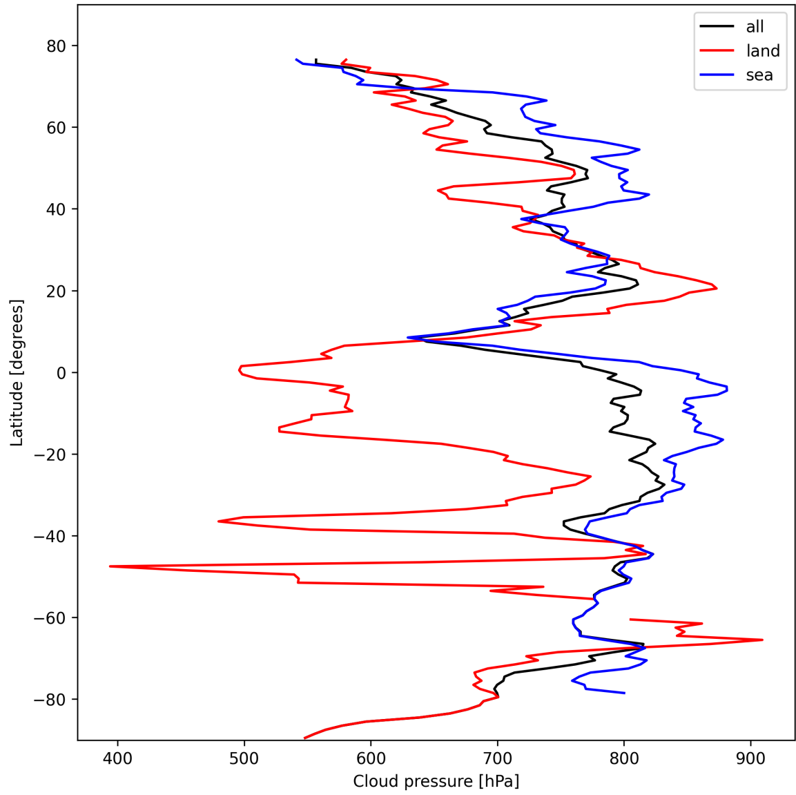
Figure 13: Zonal average of “Cloud pressure” for 2024-10-21 to 2024-10-23.
