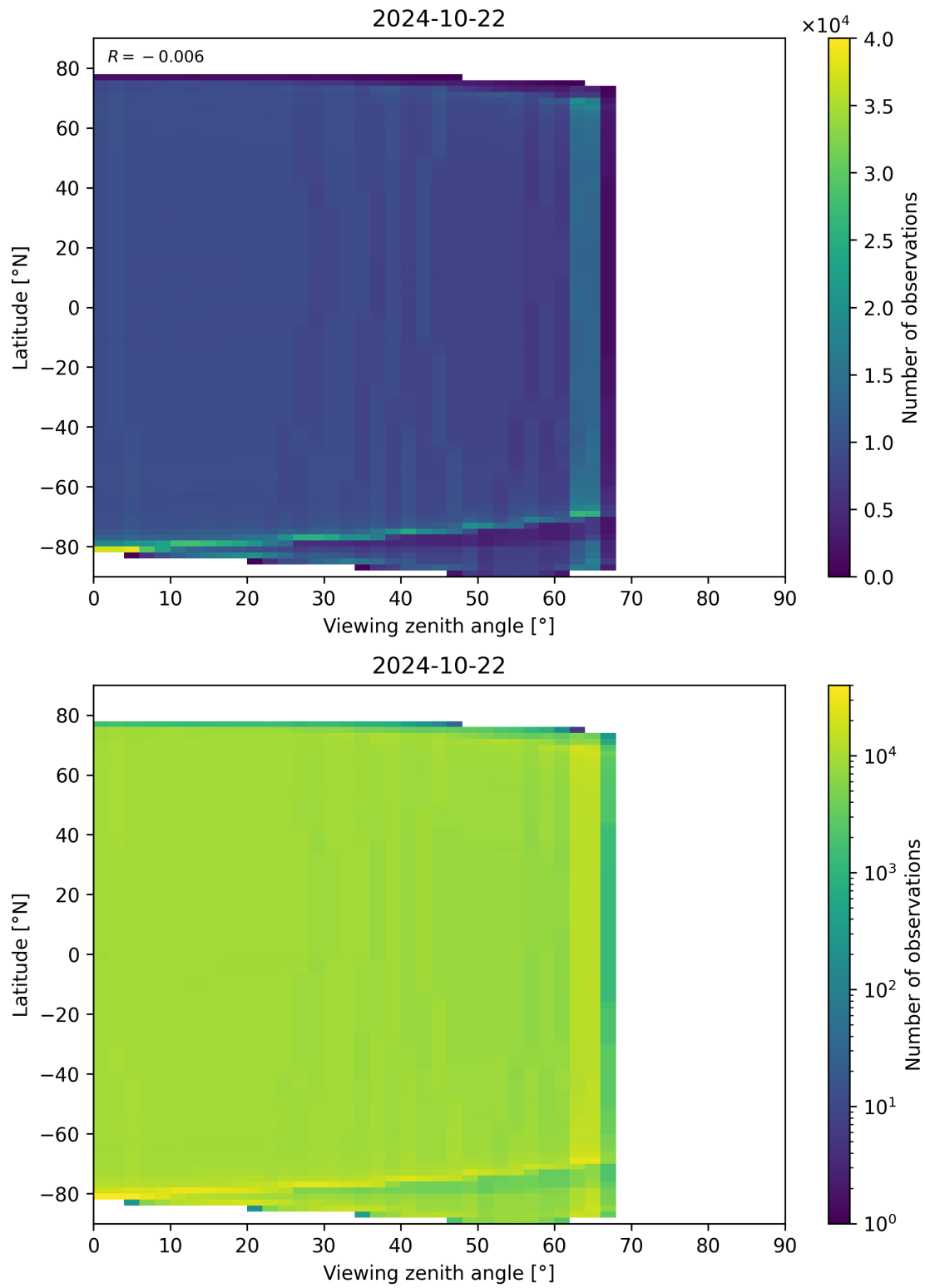
Figure 135: Scatter density plot of “Viewing zenith angle” against “Latitude” for 2024-10-21 to 2024-10-23.
