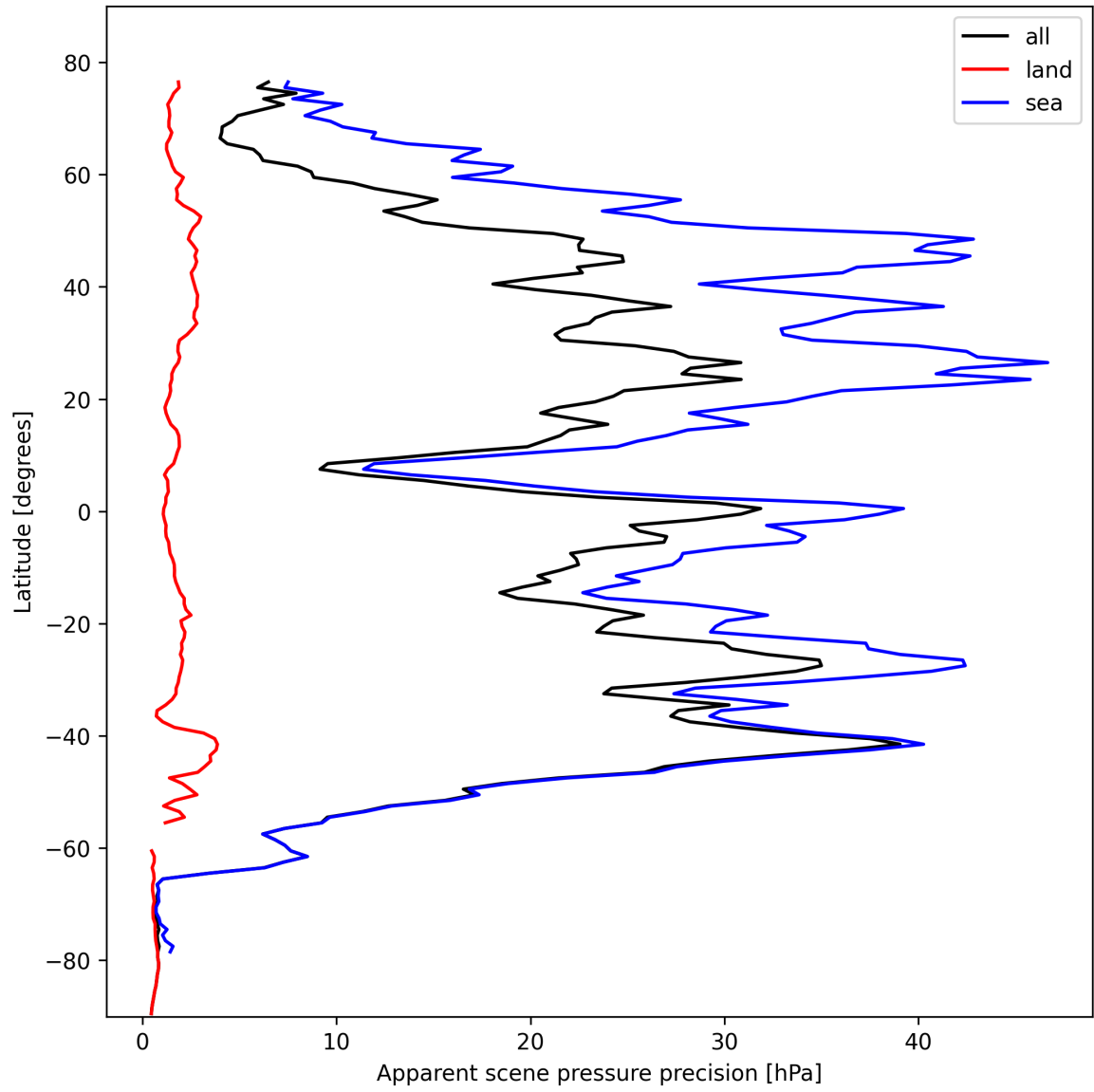
Figure 20: Zonal average of “Apparent scene pressure precision” for 2024-10-21 to 2024-10-23.
