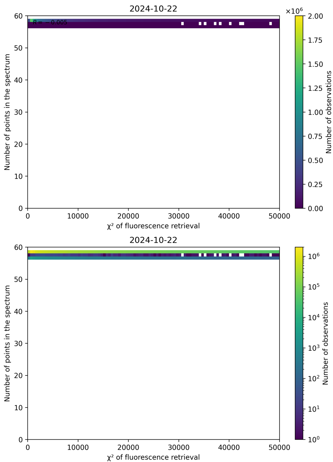
Figure 71: Scatter density plot of " \chi^2 of fluorescence retrieval" against "Number of points in the spectrum" for 2024-10-21 to 2024-10-23.
