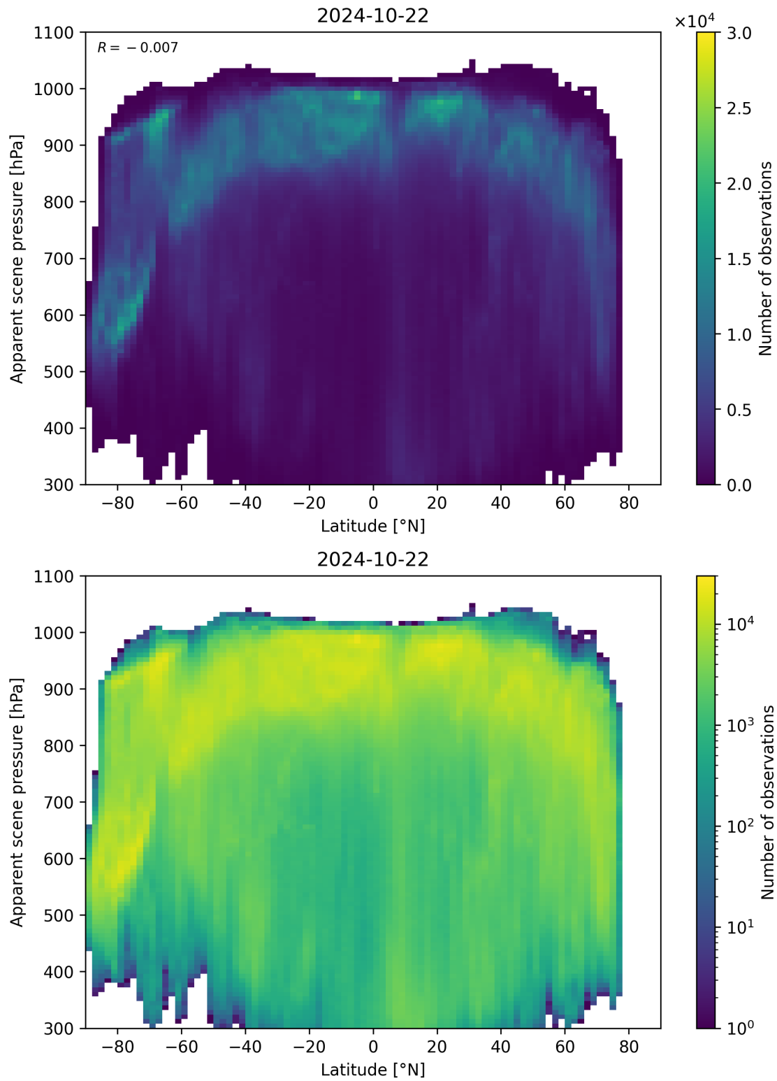
Figure 96: Scatter density plot of “Latitude” against “Apparent scene pressure” for 2024-10-21 to 2024-10-23.
