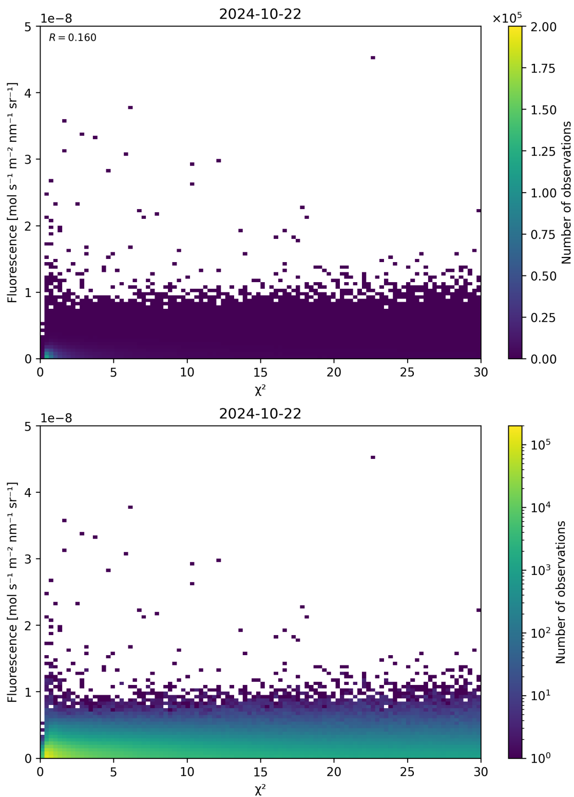
Figure 70: Scatter density plot of “ \chi^2 ” against “Fluorescence” for 2024-10-21 to 2024-10-23.
