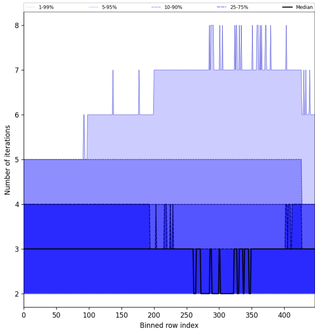
Figure 56: Along track statistics of “Number of iterations” for 2024-10-21 to 2024-10-23
