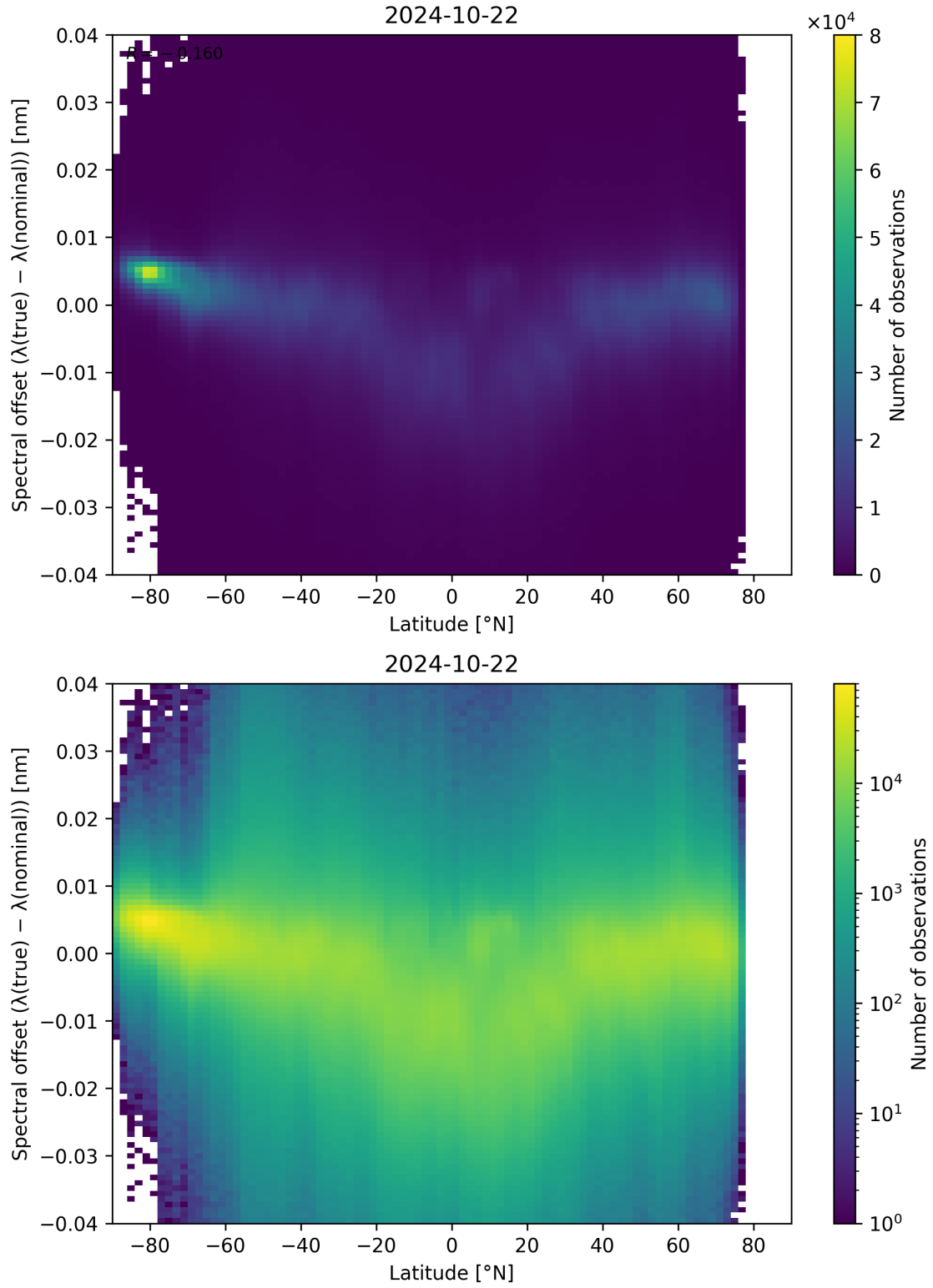
Figure 105: Scatter density plot of “Latitude” against “Spectral offset ( \lambda_{\text{true}} - \lambda_{\text{nominal}} )” for 2024-10-21 to 2024-10-23.
