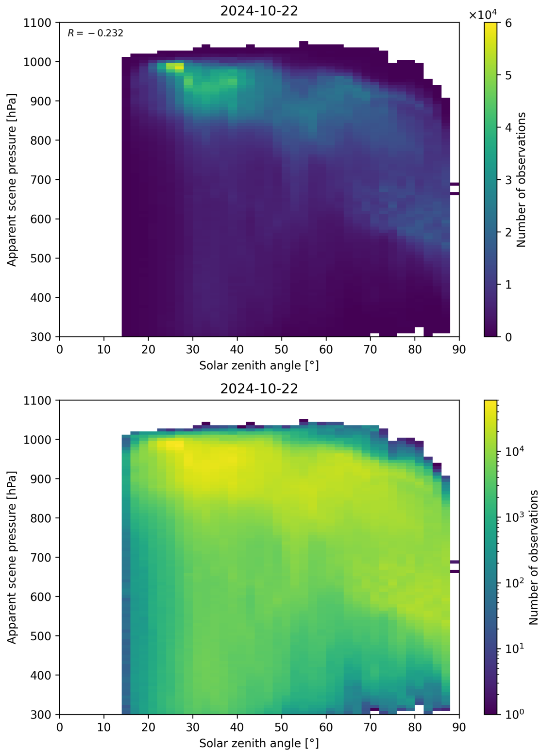
Figure 118: Scatter density plot of “Solar zenith angle” against “Apparent scene pressure” for 2024-10-21 to 2024-10-23.
