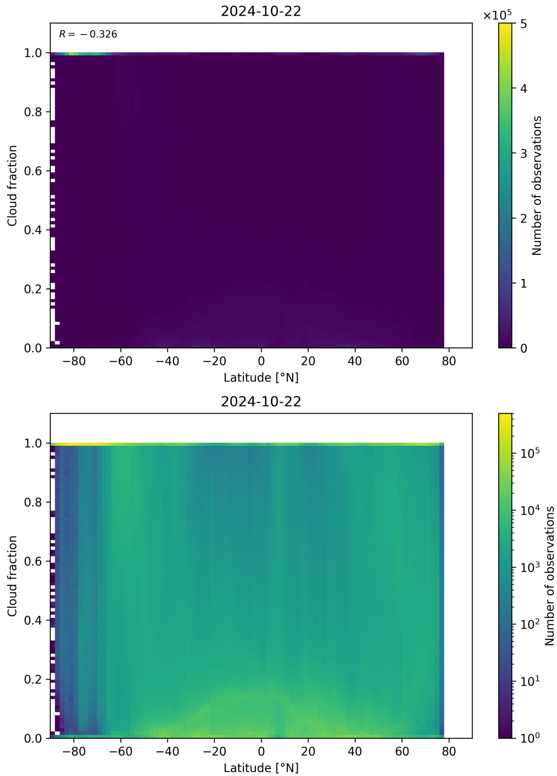
Figure 99: Scatter density plot of “Latitude” against “Cloud fraction” for 2024-10-21 to 2024-10-23.
