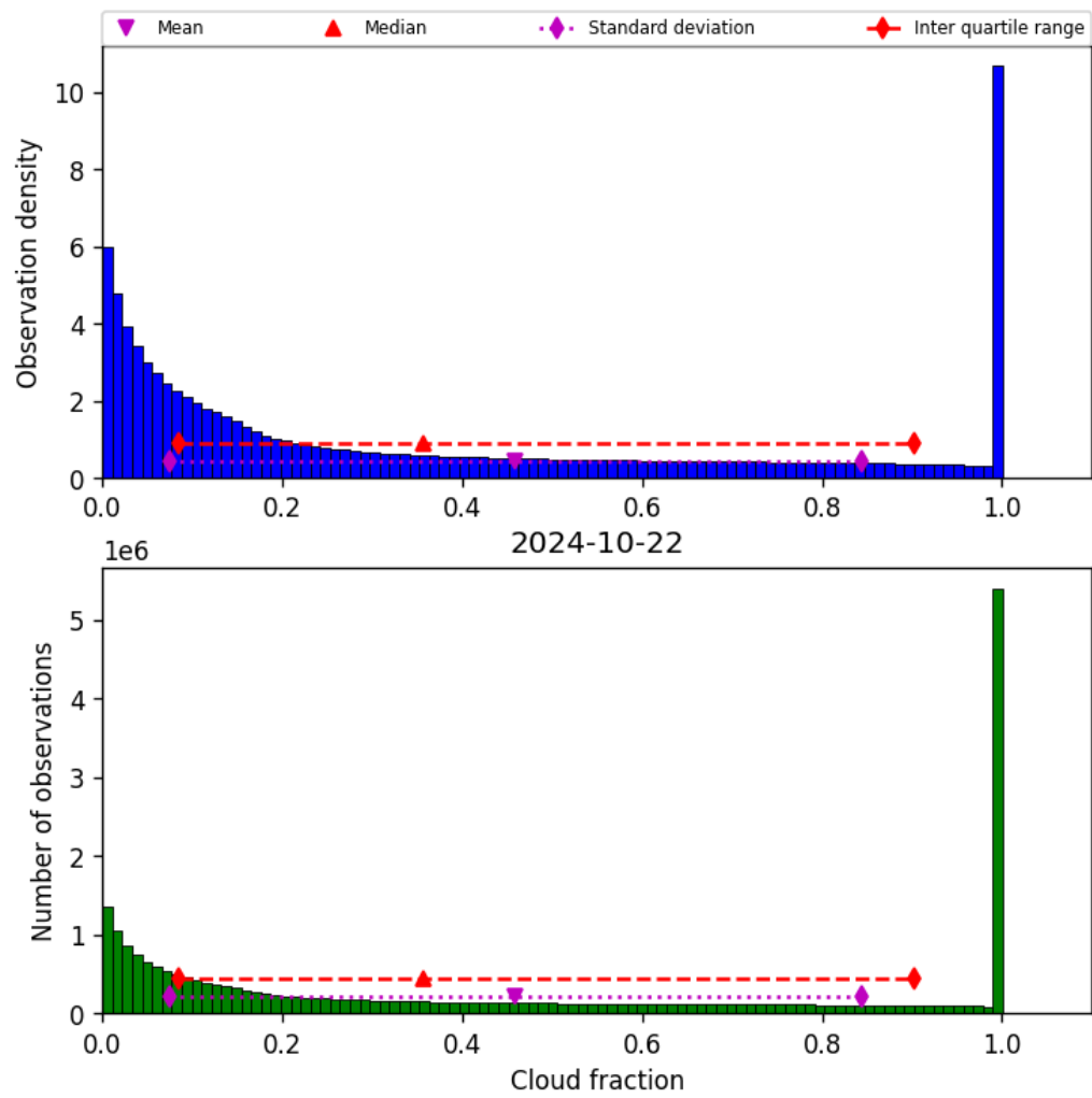
Figure 32: Histogram of “Cloud fraction” for 2024-10-21 to 2024-10-23
