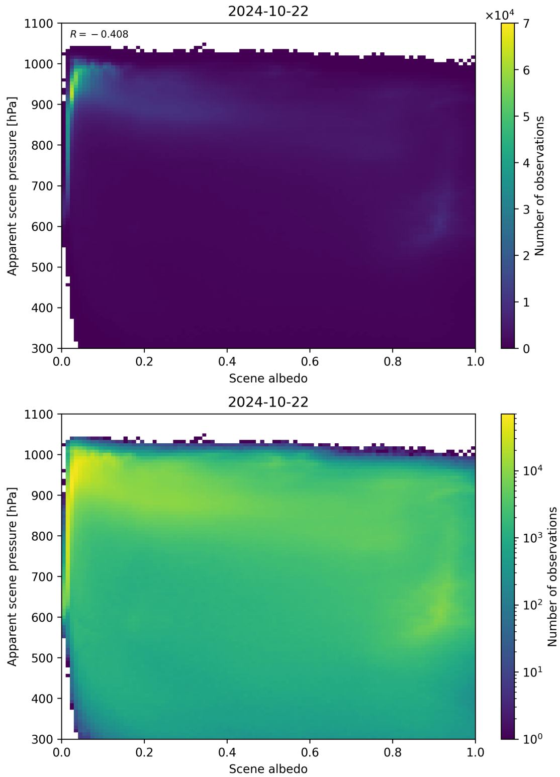
Figure 111: Scatter density plot of “Scene albedo” against “Apparent scene pressure” for 2024-10-21 to 2024-10-23.
