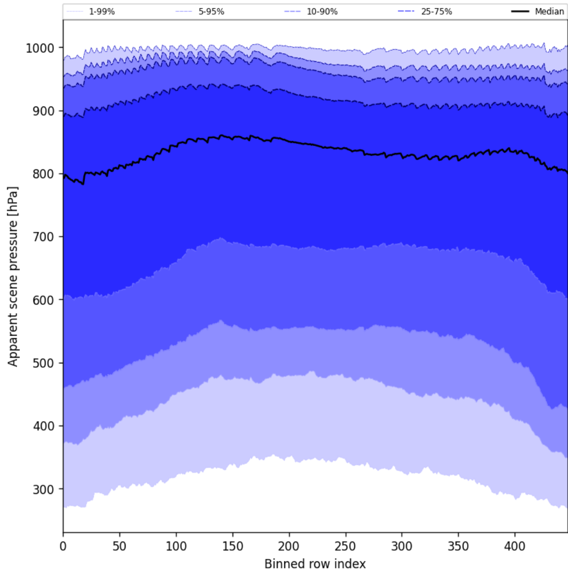
Figure 53: Along track statistics of “Apparent scene pressure” for 2024-10-21 to 2024-10-23
