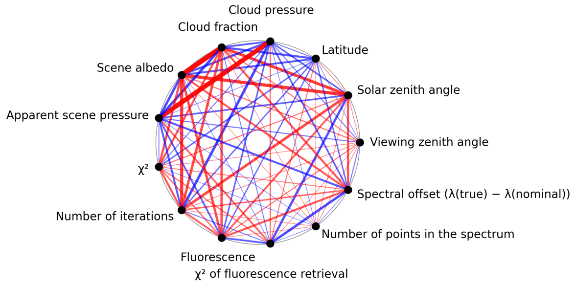
Figure 1: Map of correlation graph for 2024-10-21 to 2024-10-23.
