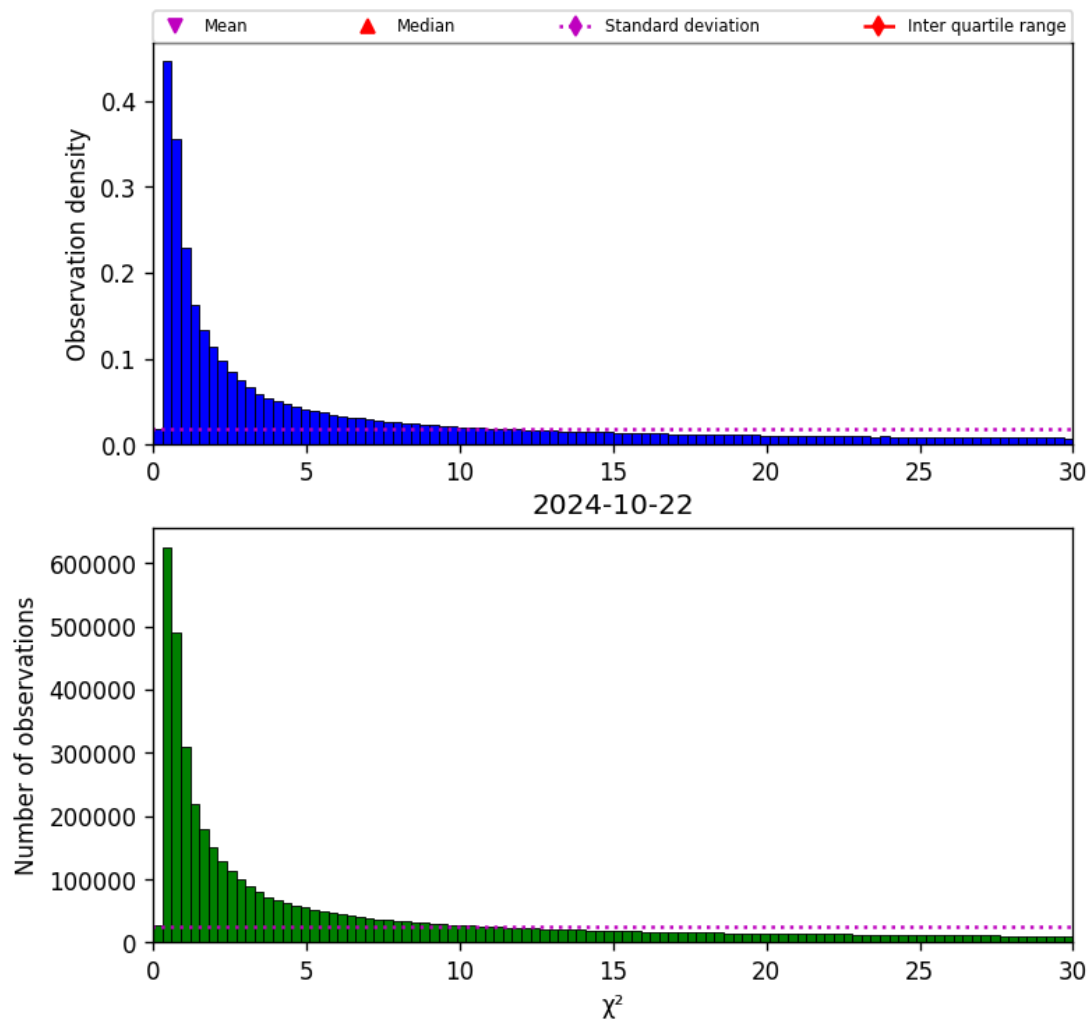
Figure 38: Histogram of “ \chi^2 ” for 2024-10-21 to 2024-10-23
