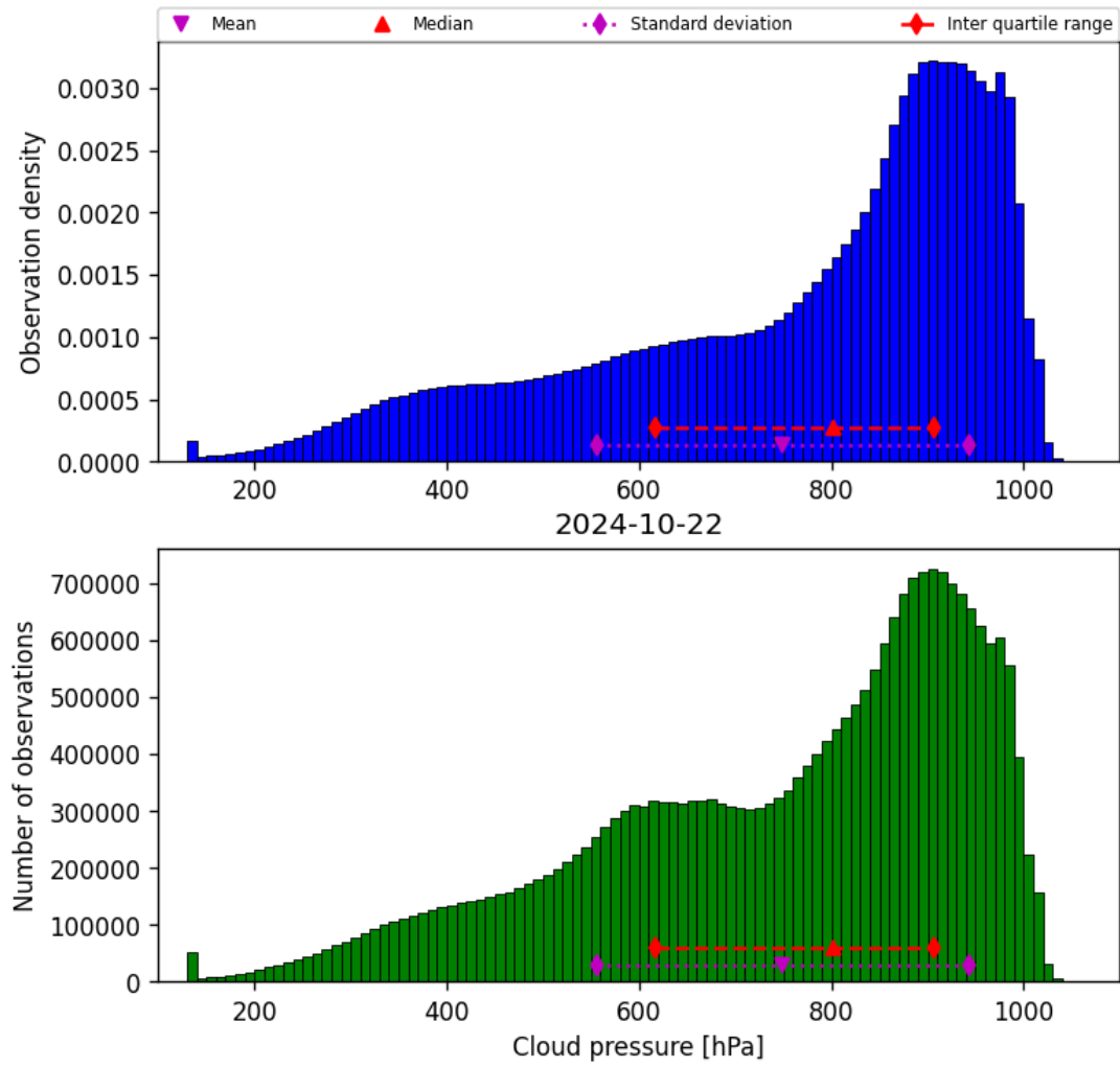
Figure 30: Histogram of “Cloud pressure” for 2024-10-21 to 2024-10-23
