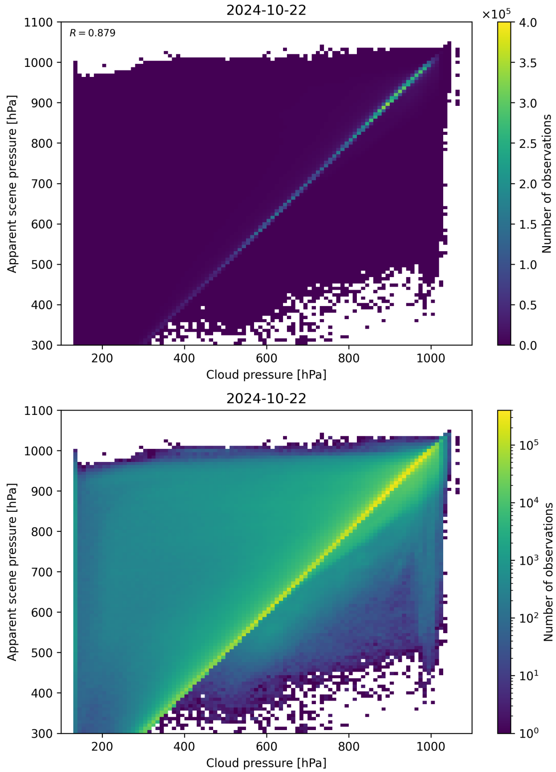
Figure 84: Scatter density plot of “Cloud pressure” against “Apparent scene pressure” for 2024-10-21 to 2024-10-23.
