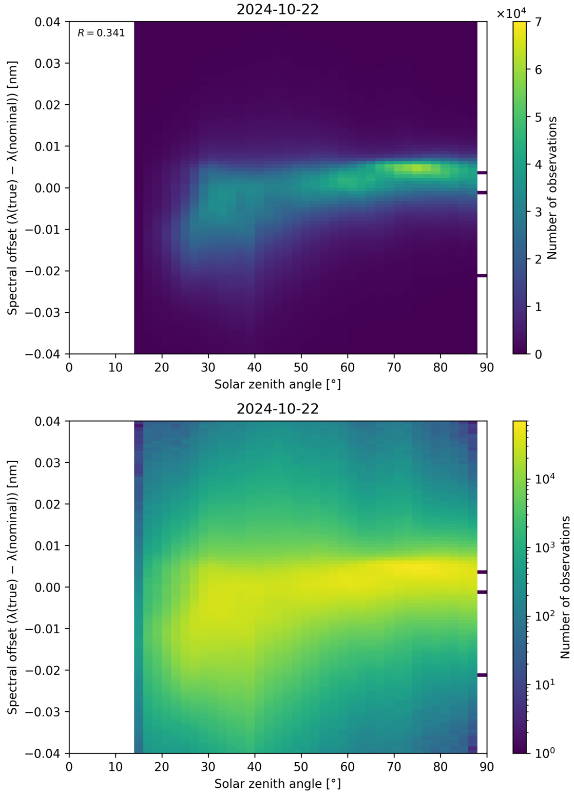
Figure 128: Scatter density plot of “Solar zenith angle” against “Spectral offset ( \lambda_{\text{true}} - \lambda_{\text{nominal}} )” for 2024-10-21 to 2024-10-23.
