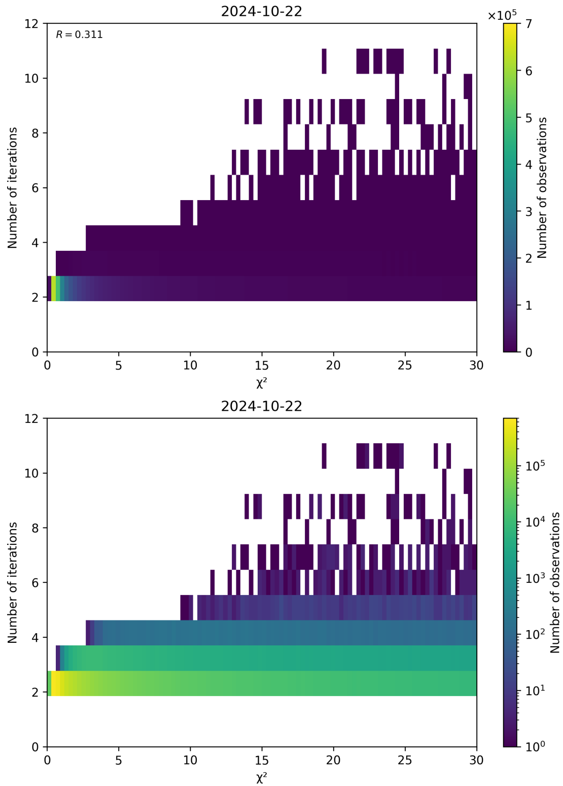
Figure 73: Scatter density plot of “ \chi^2 ” against “Number of iterations” for 2024-10-21 to 2024-10-23.
