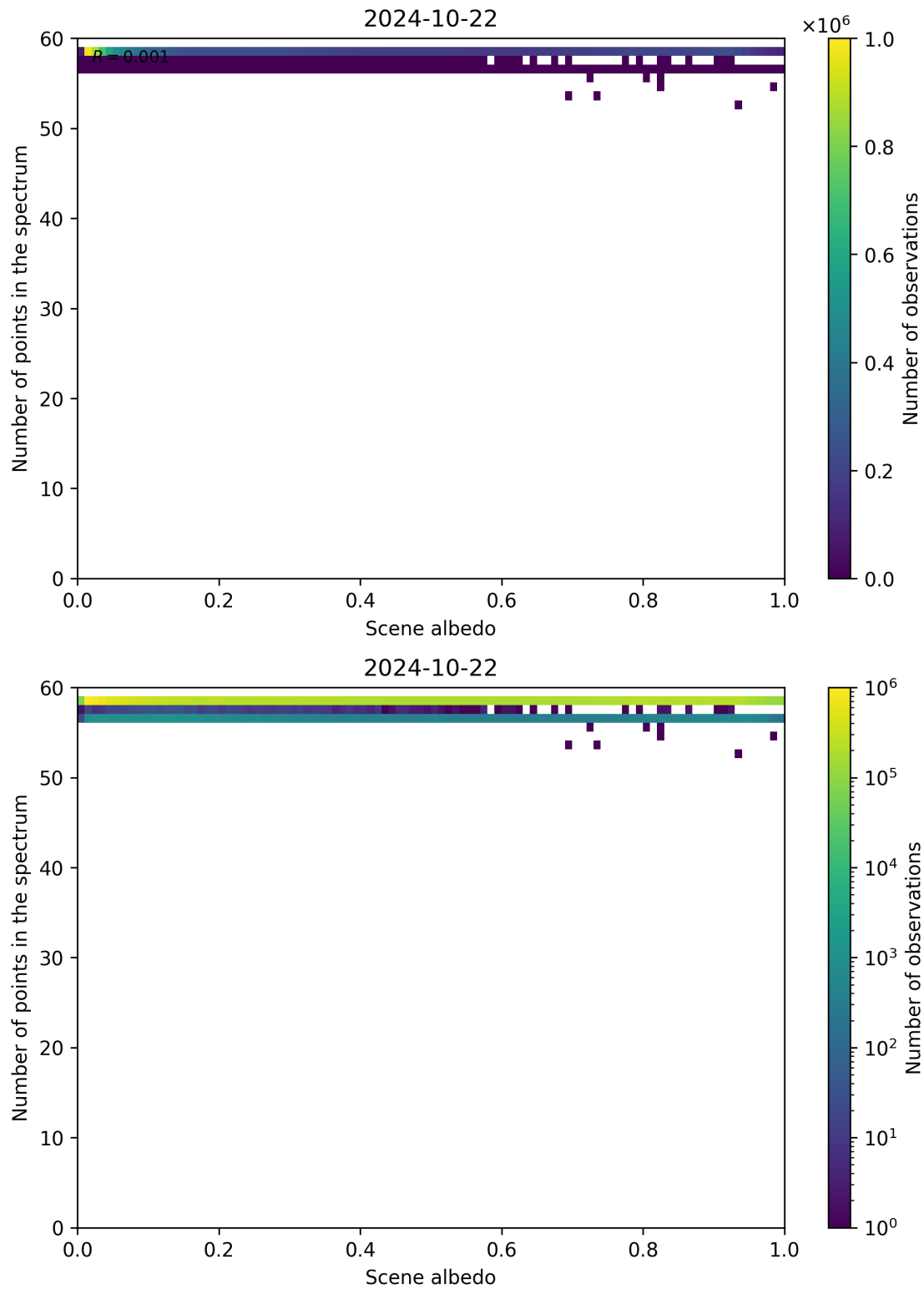
Figure 116: Scatter density plot of “Scene albedo” against “Number of points in the spectrum” for 2024-10-21 to 2024-10-23.
