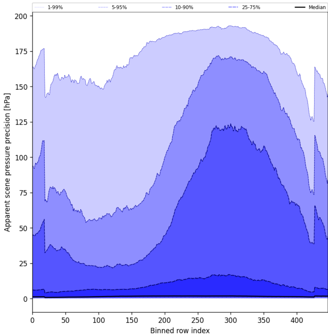
Figure 54: Along track statistics of “Apparent scene pressure precision” for 2024-10-21 to 2024-10-23
