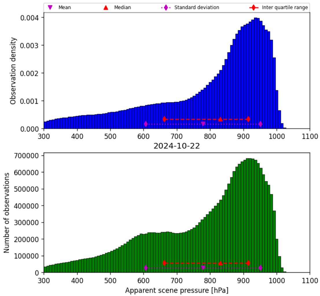
Figure 36: Histogram of “Apparent scene pressure” for 2024-10-21 to 2024-10-23
