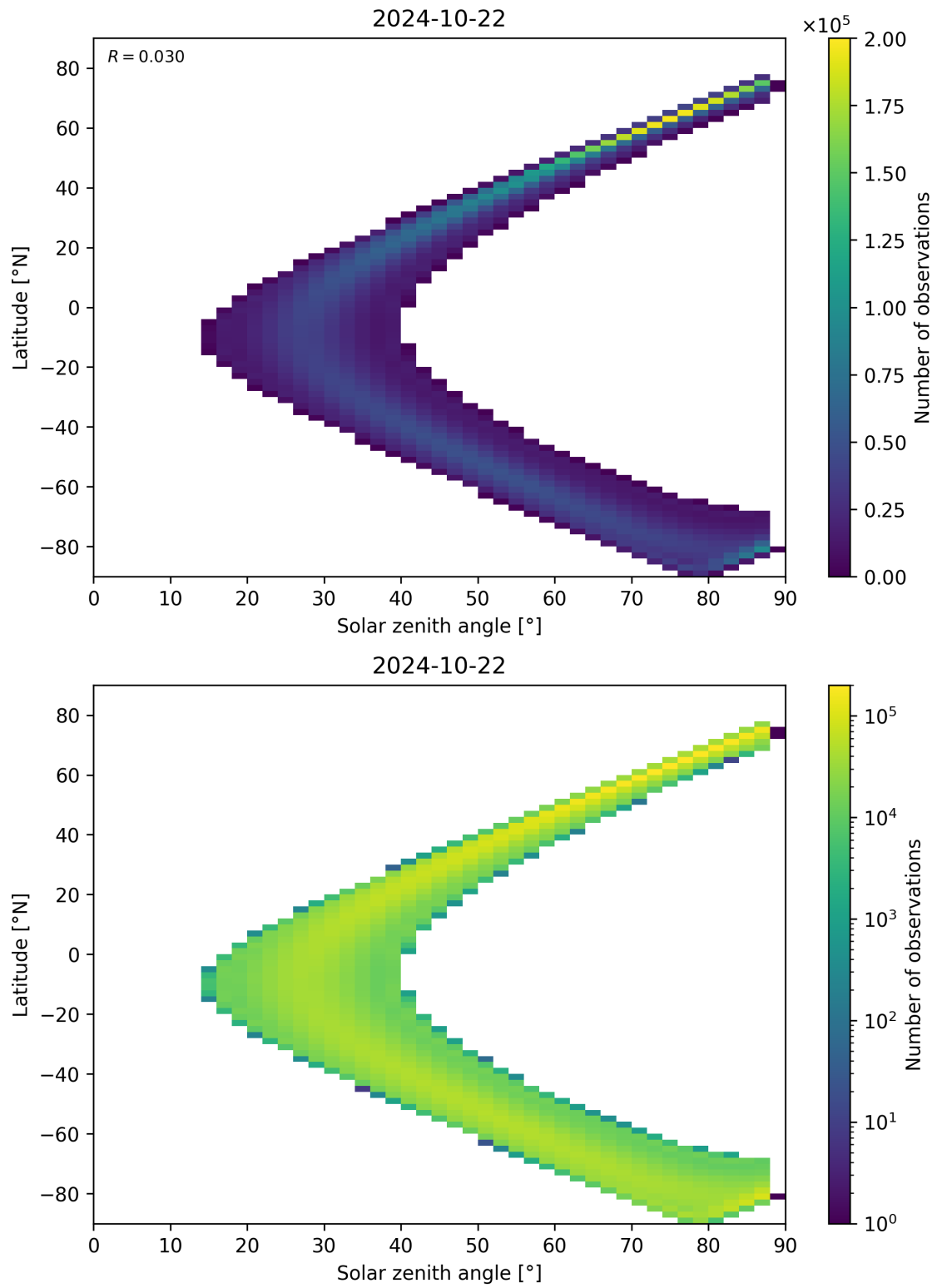
Figure 124: Scatter density plot of “Solar zenith angle” against “Latitude” for 2024-10-21 to 2024-10-23.
