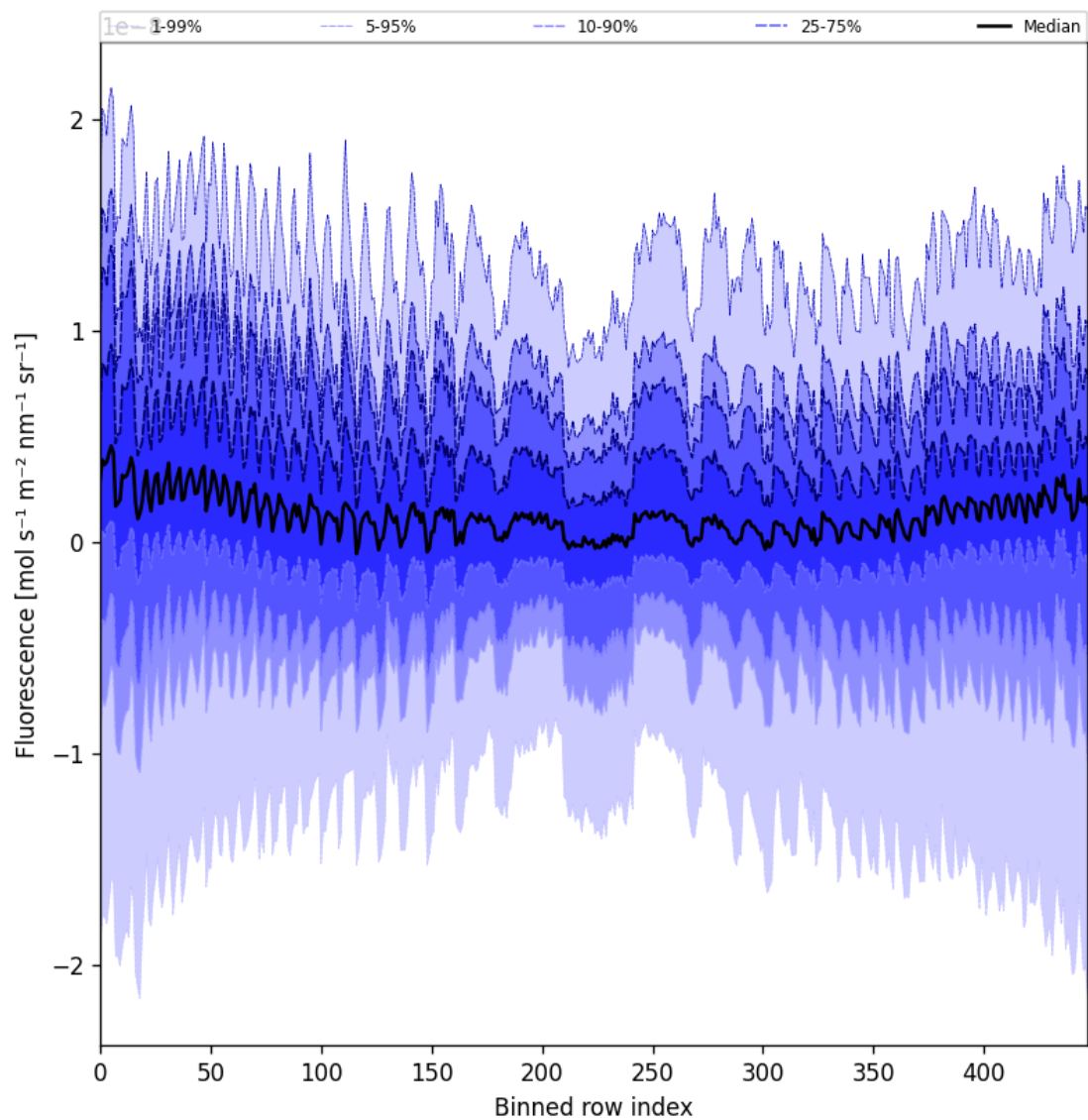
Figure 57: Along track statistics of “Fluorescence” for 2024-10-21 to 2024-10-23
