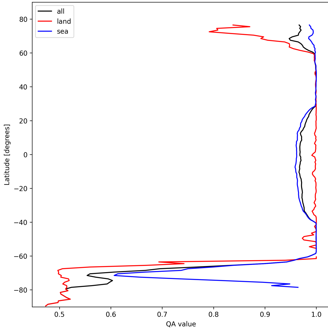
Figure 12: Zonal average of “QA value” for 2024-10-21 to 2024-10-23.
