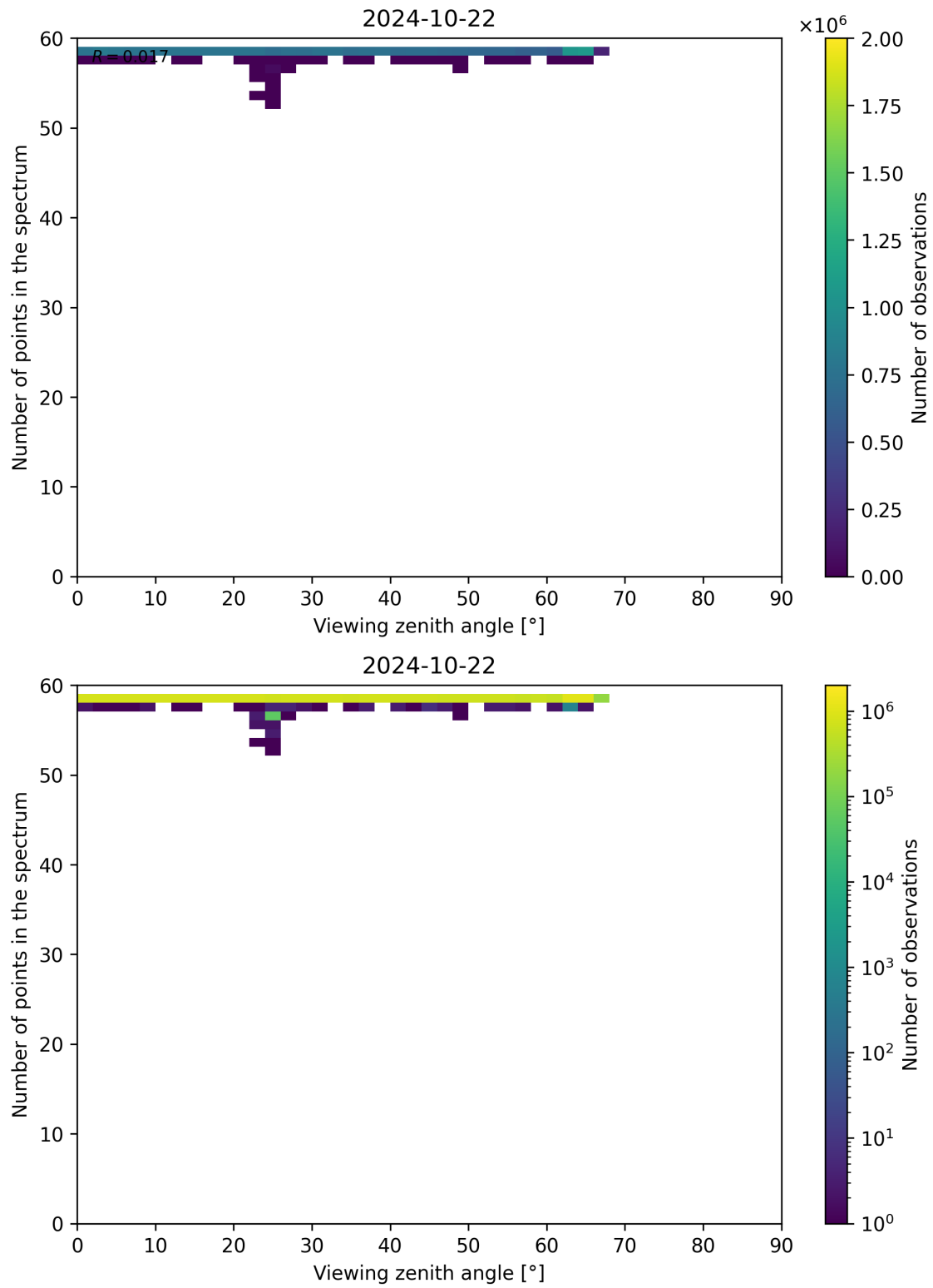
Figure 137: Scatter density plot of “Viewing zenith angle” against “Number of points in the spectrum” for 2024-10-21 to 2024-10-23.
