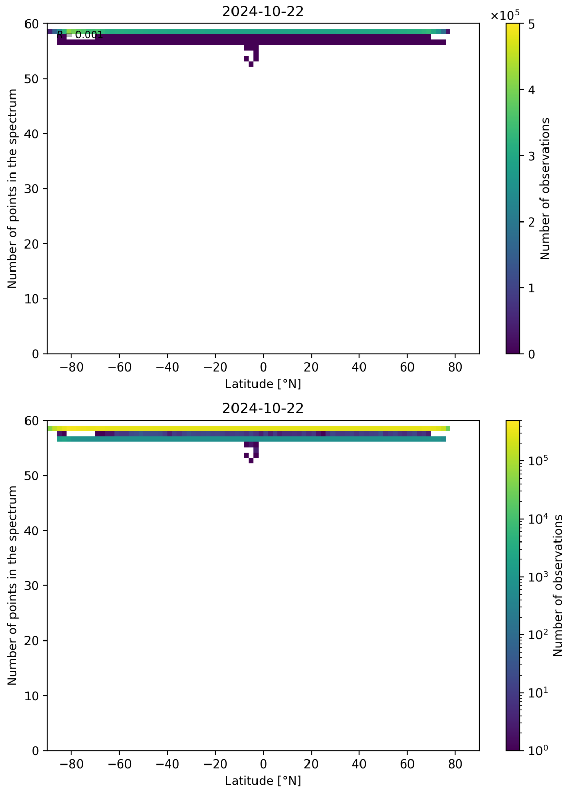
Figure 103: Scatter density plot of “Latitude” against “Number of points in the spectrum” for 2024-10-21 to 2024-10-23.
