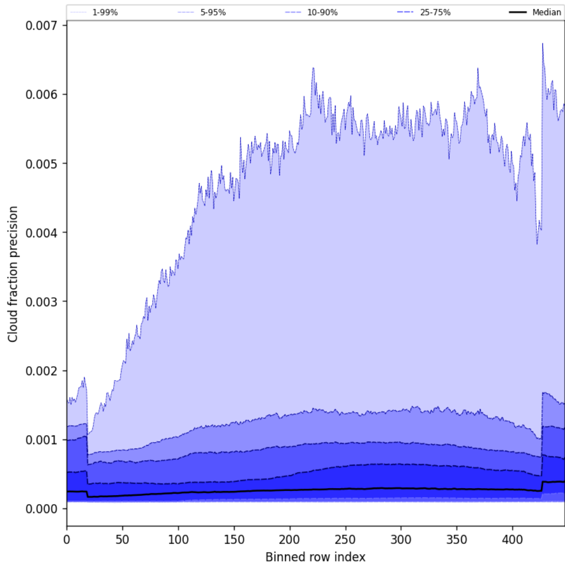
Figure 50: Along track statistics of “Cloud fraction precision” for 2024-10-21 to 2024-10-23
