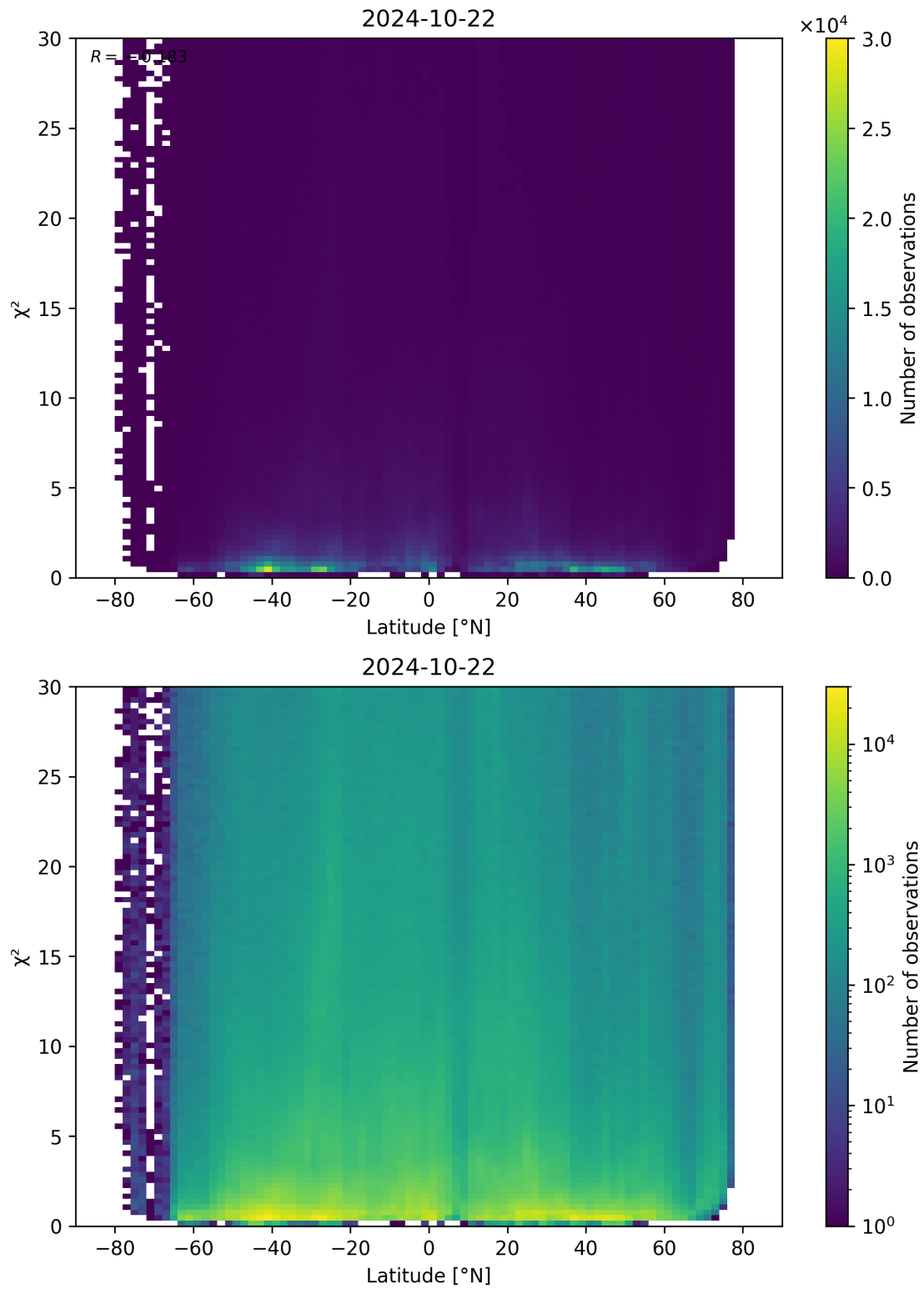
Figure 97: Scatter density plot of “Latitude” against “ \chi^2 ” for 2024-10-21 to 2024-10-23.
