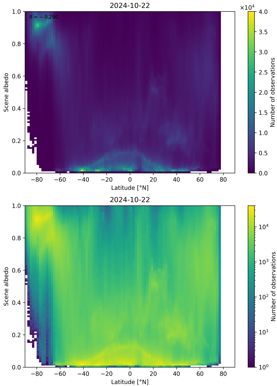
Figure 104: Scatter density plot of “Latitude” against “Scene albedo” for 2024-10-21 to 2024-10-23.
