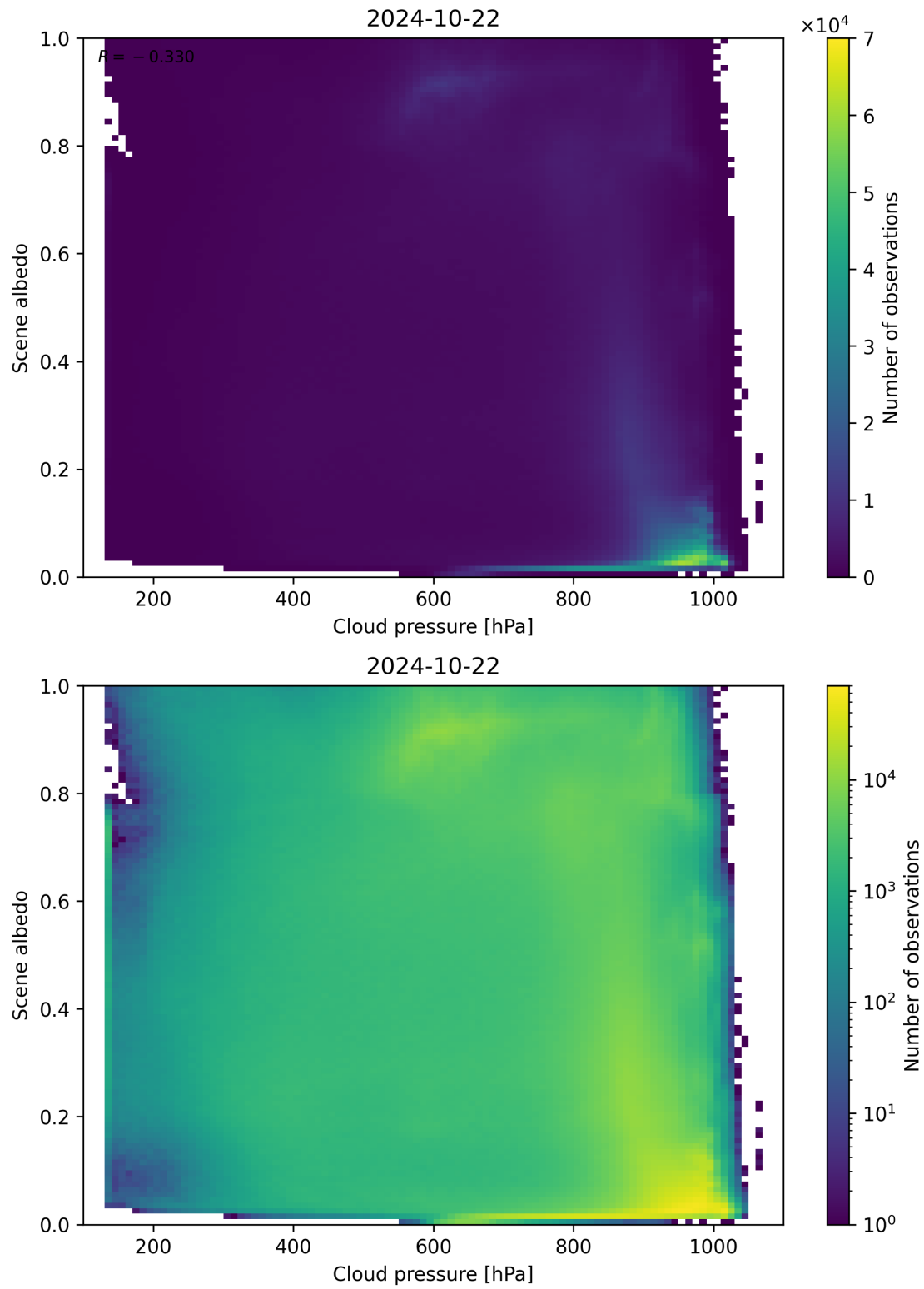
Figure 91: Scatter density plot of “Cloud pressure” against “Scene albedo” for 2024-10-21 to 2024-10-23.
