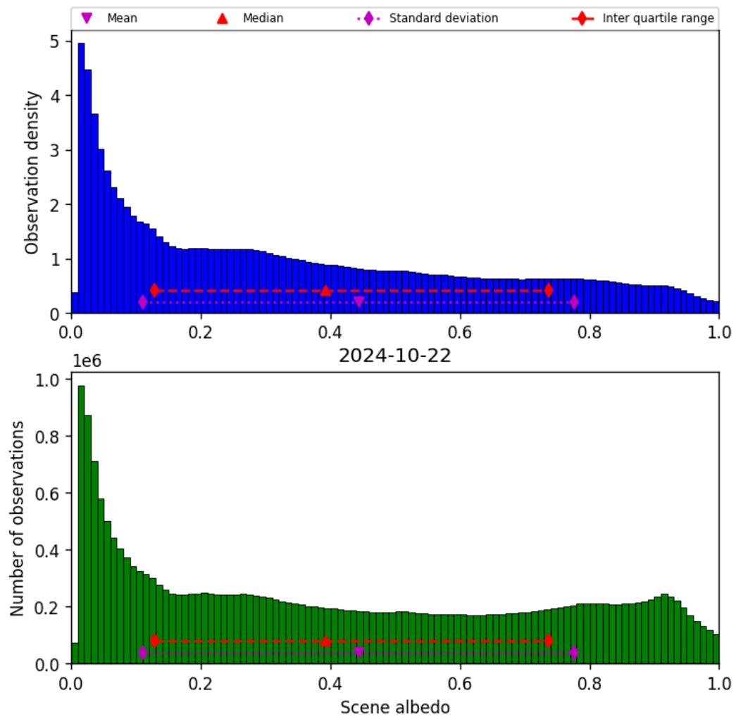
Figure 34: Histogram of “Scene albedo” for 2024-10-21 to 2024-10-23
