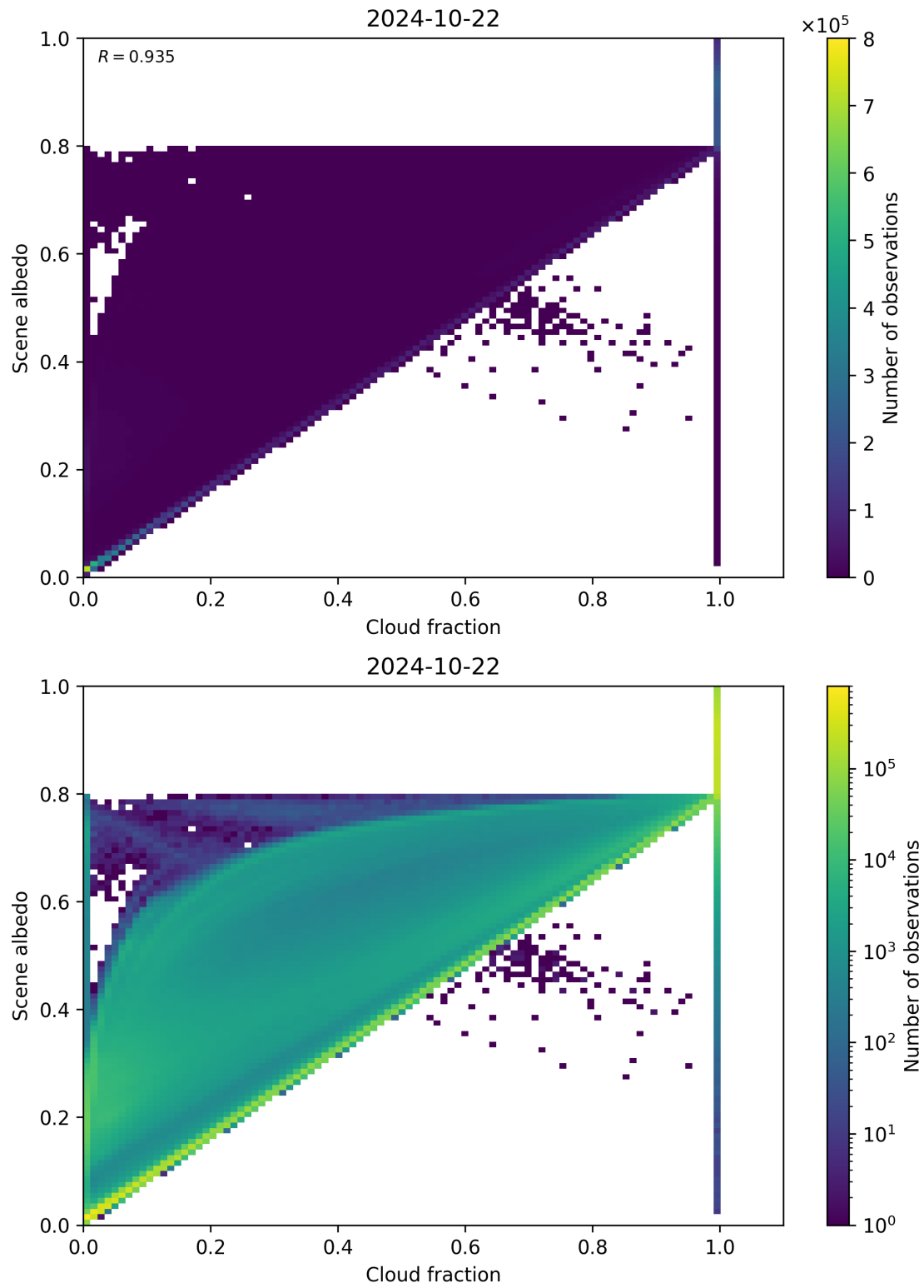
Figure 82: Scatter density plot of “Cloud fraction” against “Scene albedo” for 2024-10-21 to 2024-10-23.
