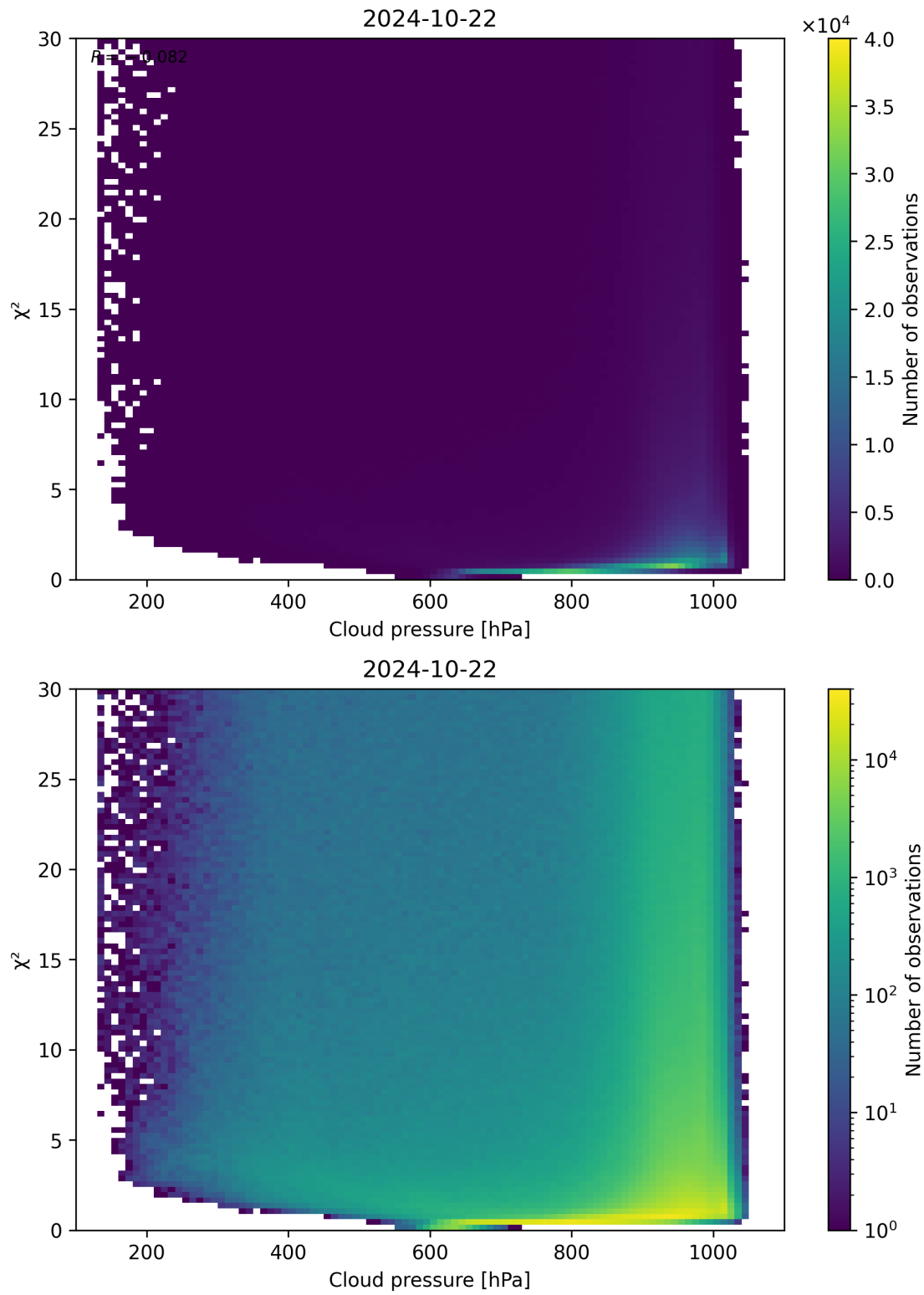
Figure 85: Scatter density plot of “Cloud pressure” against “ \chi^2 ” for 2024-10-21 to 2024-10-23.
