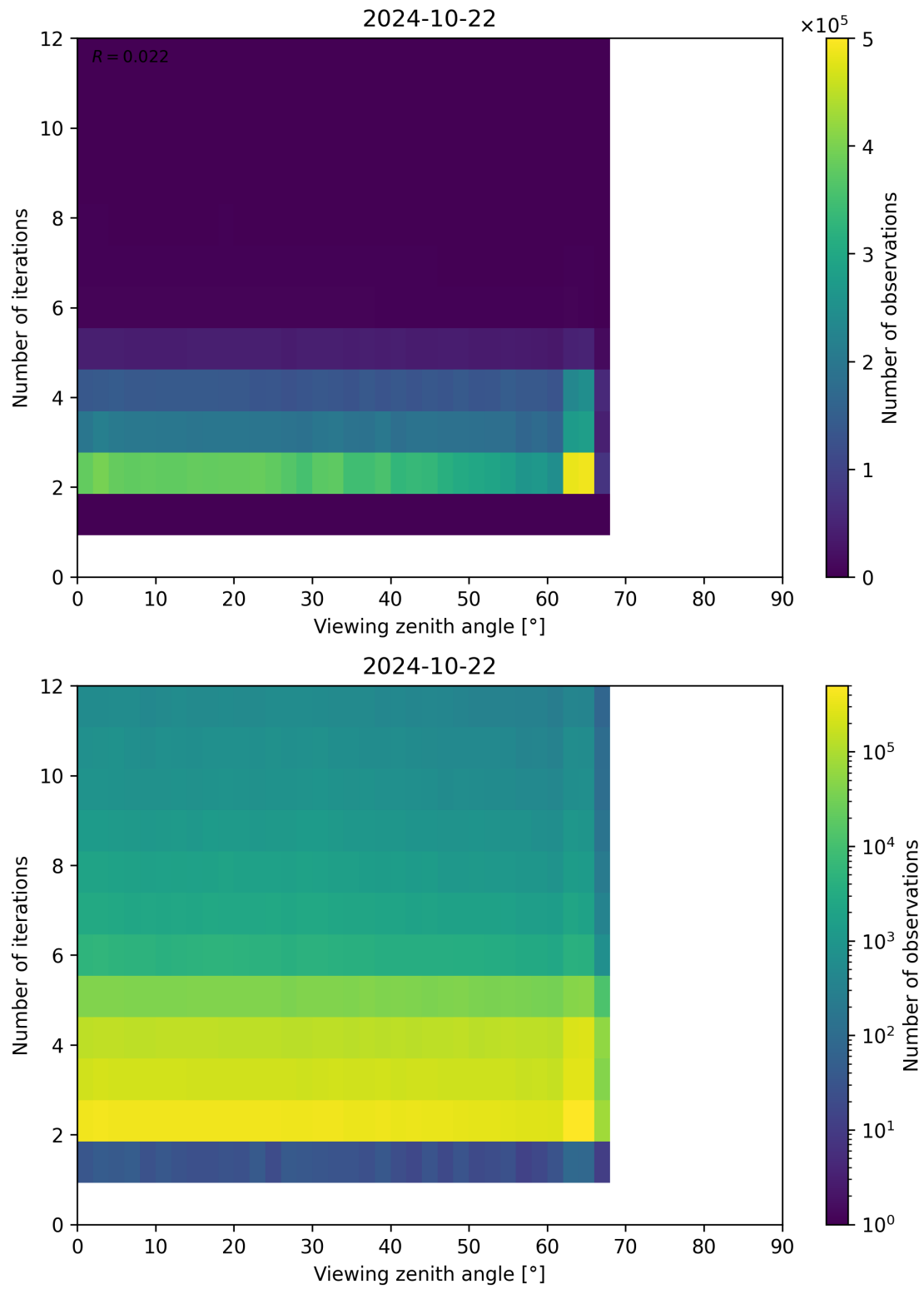
Figure 136: Scatter density plot of “Viewing zenith angle” against “Number of iterations” for 2024-10-21 to 2024-10-23.
