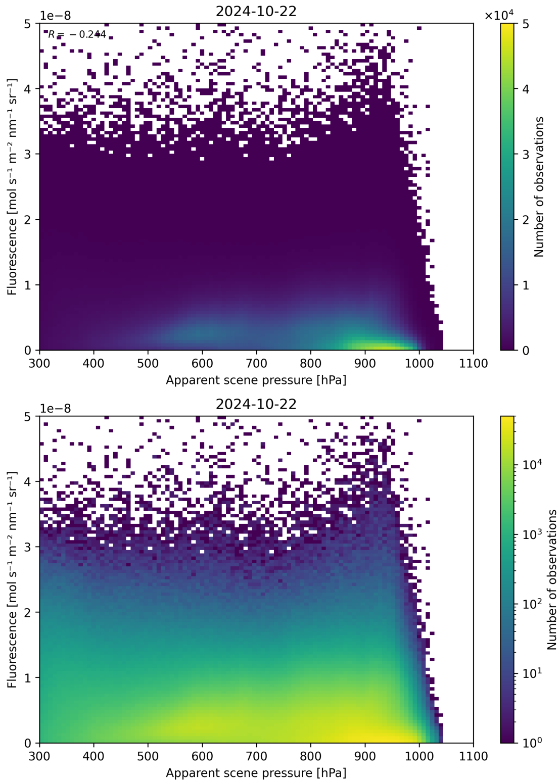
Figure 65: Scatter density plot of “Apparent scene pressure” against “Fluorescence” for 2024-10-21 to 2024-10-23.
