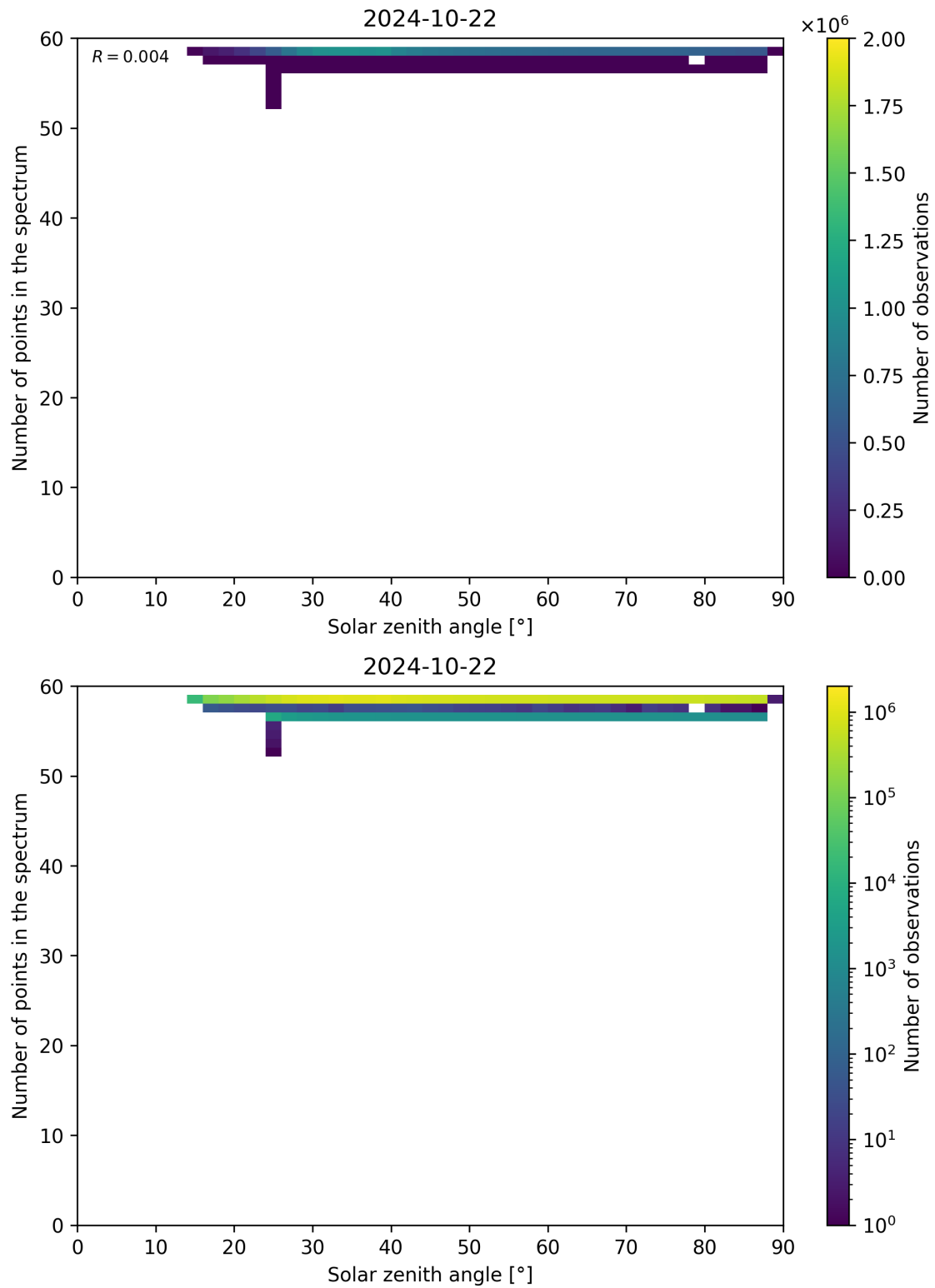
Figure 126: Scatter density plot of “Solar zenith angle” against “Number of points in the spectrum” for 2024-10-21 to 2024-10-23.
