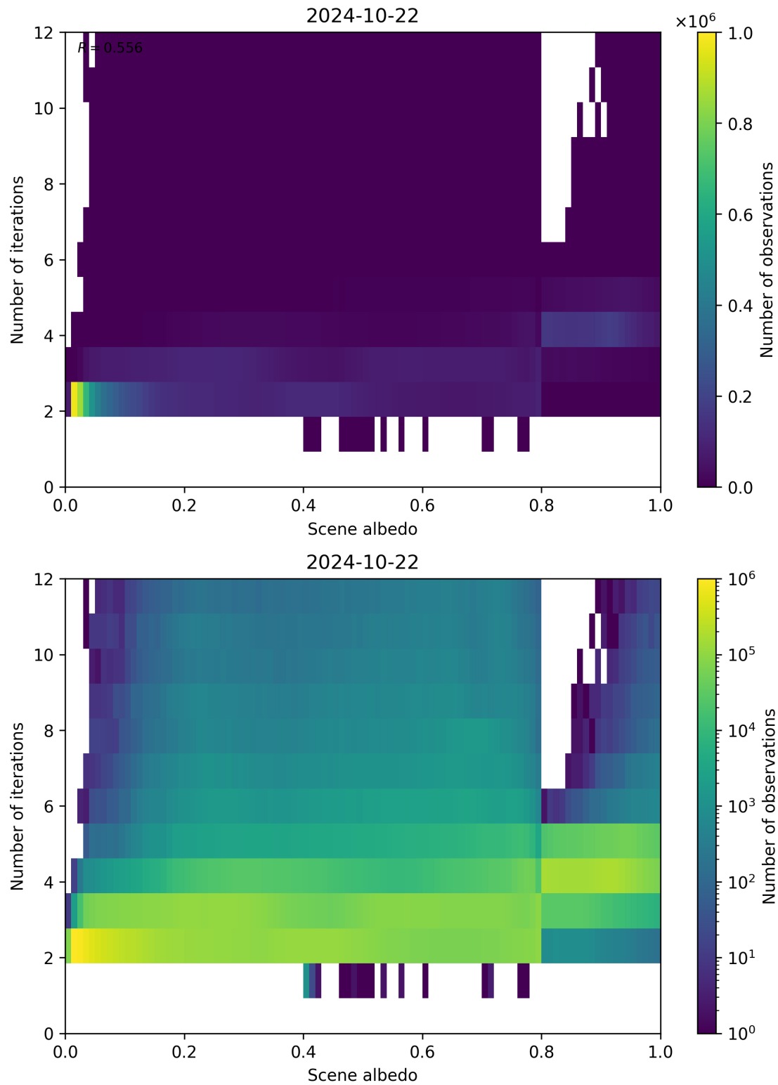
Figure 115: Scatter density plot of “Scene albedo” against “Number of iterations” for 2024-10-21 to 2024-10-23.
