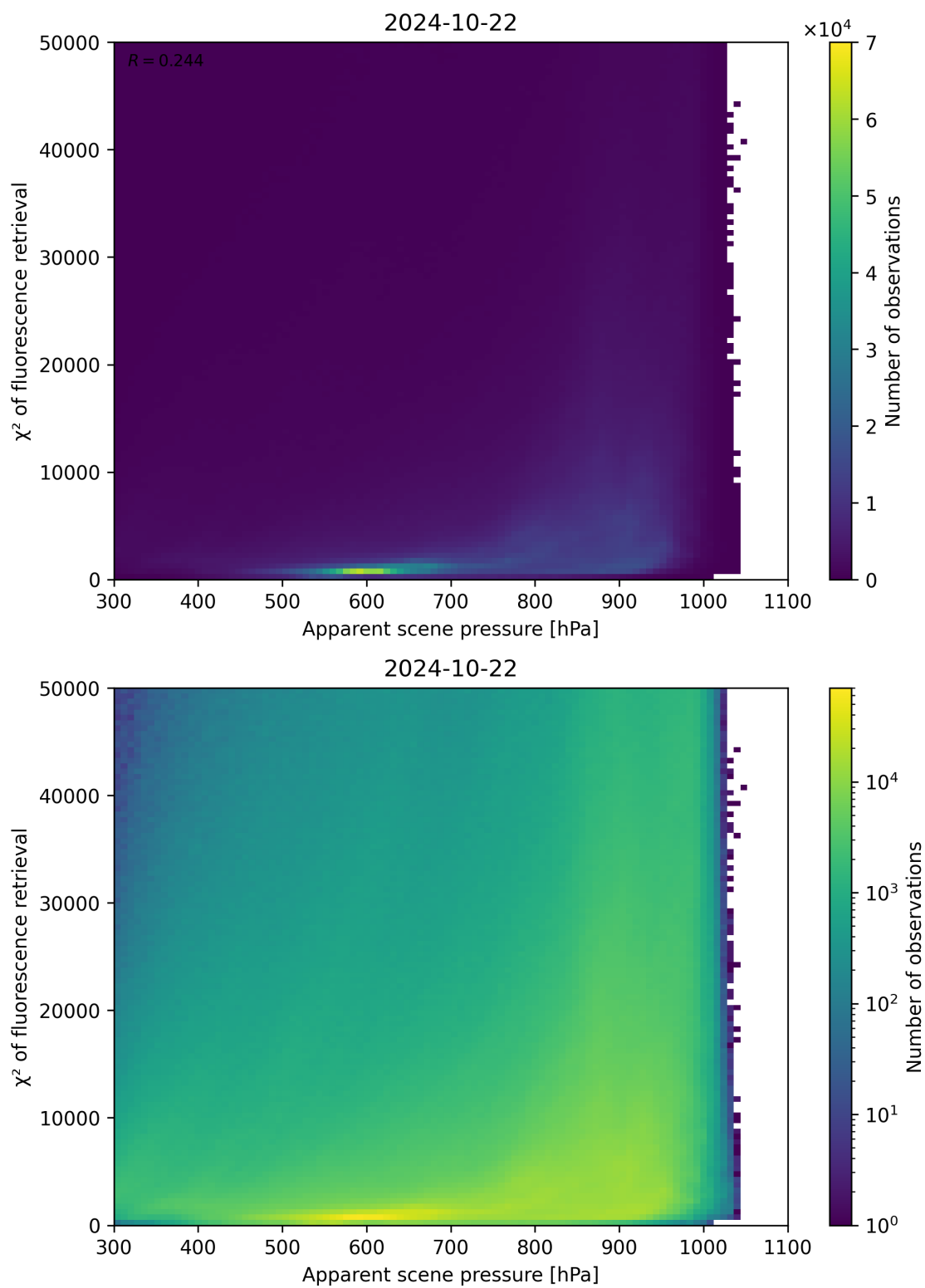
Figure 64: Scatter density plot of “Apparent scene pressure” against “ \chi^2 of fluorescence retrieval” for 2024-10-21 to 2024-10-23.
