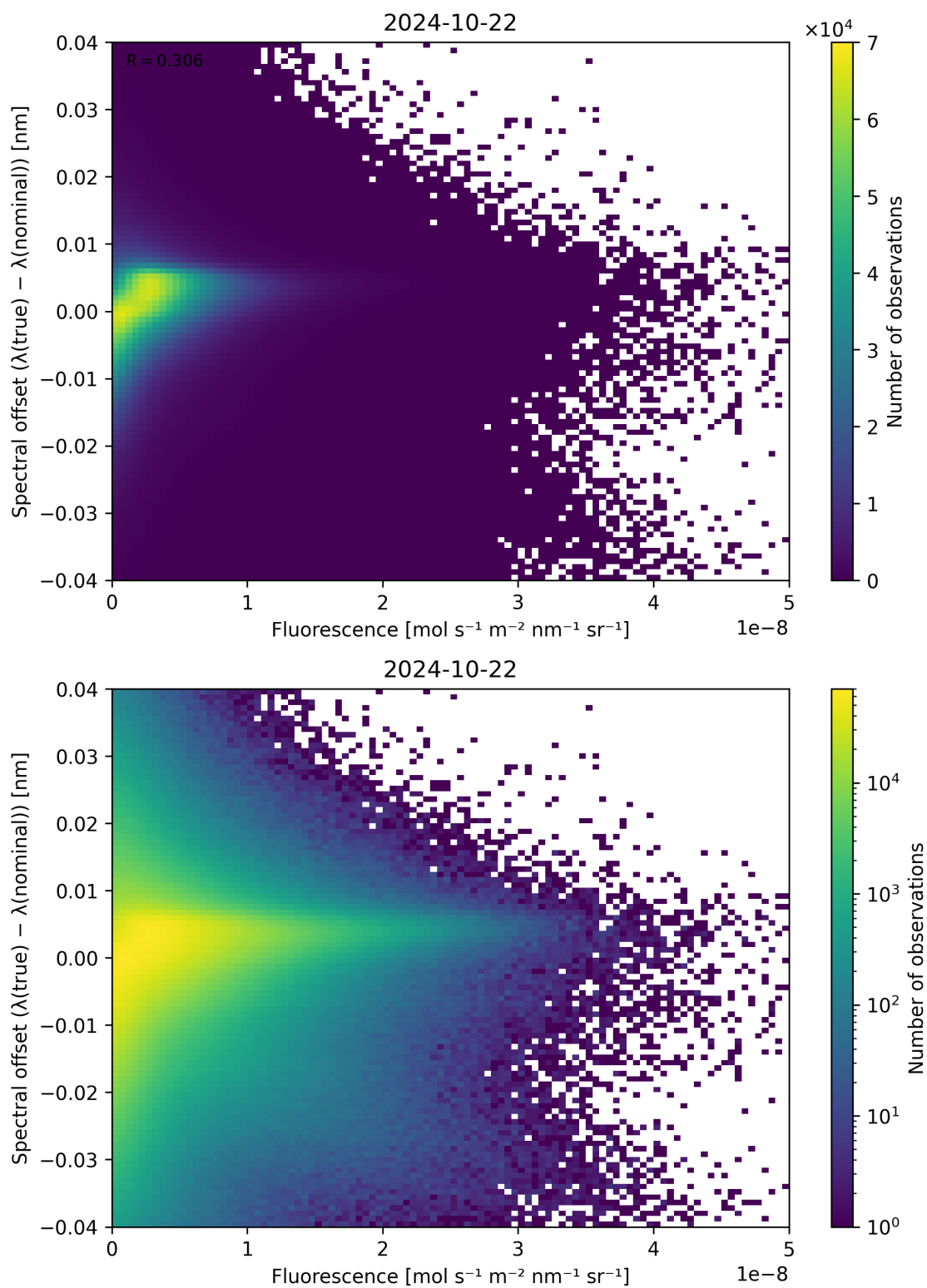
Figure 95: Scatter density plot of “Fluorescence” against “Spectral offset ( \lambda_{\text{true}} - \lambda_{\text{nominal}} )” for 2024-10-21 to 2024-10-23.
