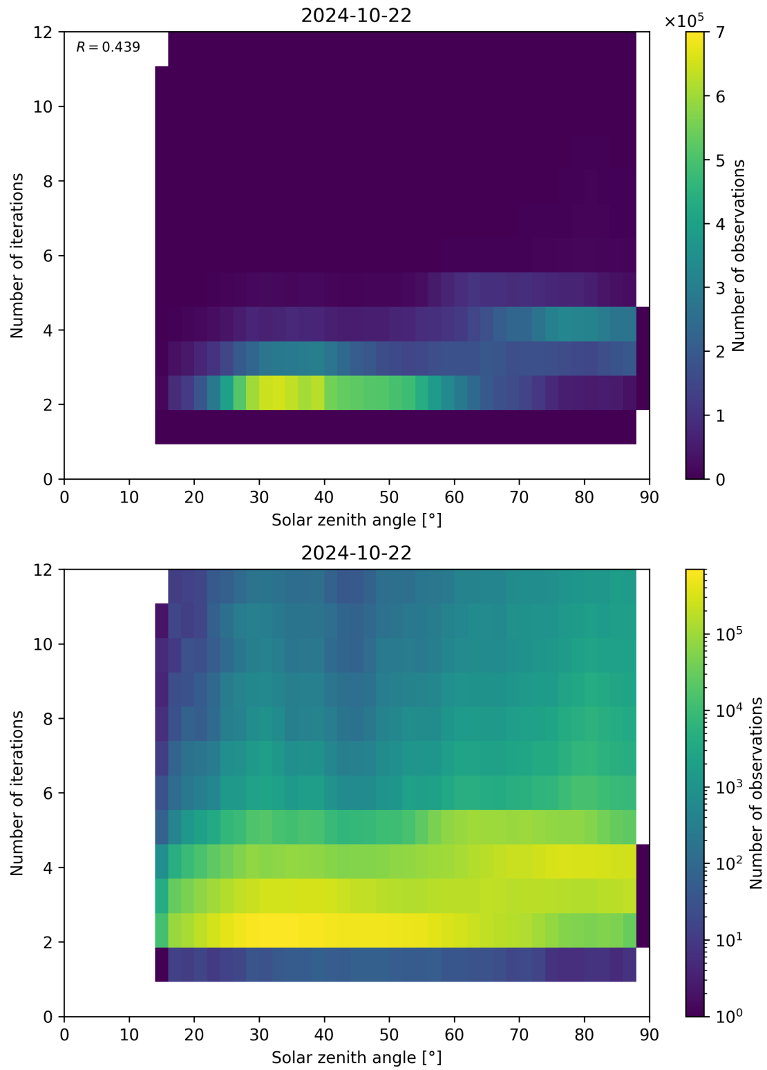
Figure 125: Scatter density plot of “Solar zenith angle” against “Number of iterations” for 2024-10-21 to 2024-10-23.
