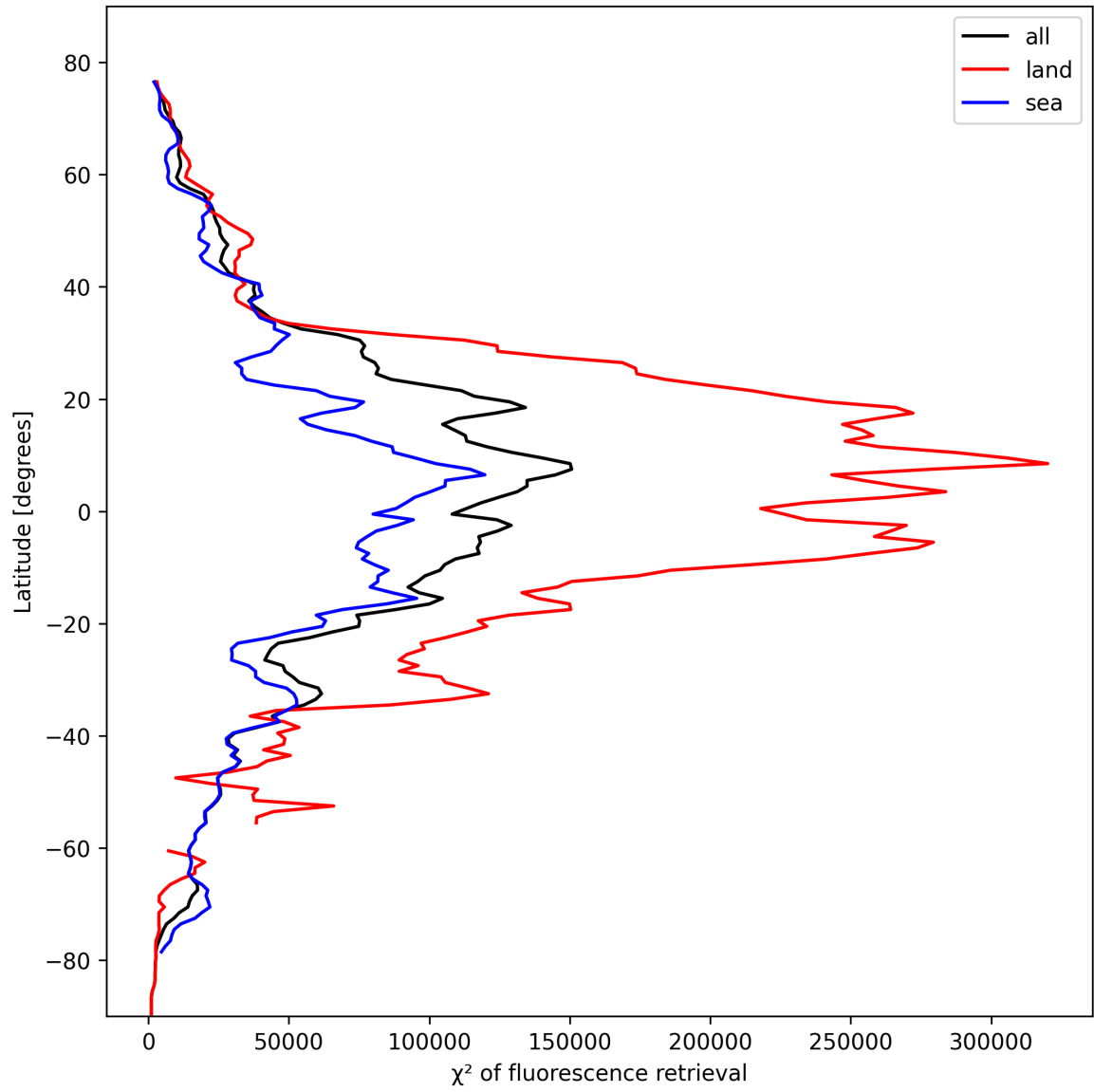
Figure 25: Zonal average of “ \chi^2 of fluorescence retrieval” for 2024-10-21 to 2024-10-23.
