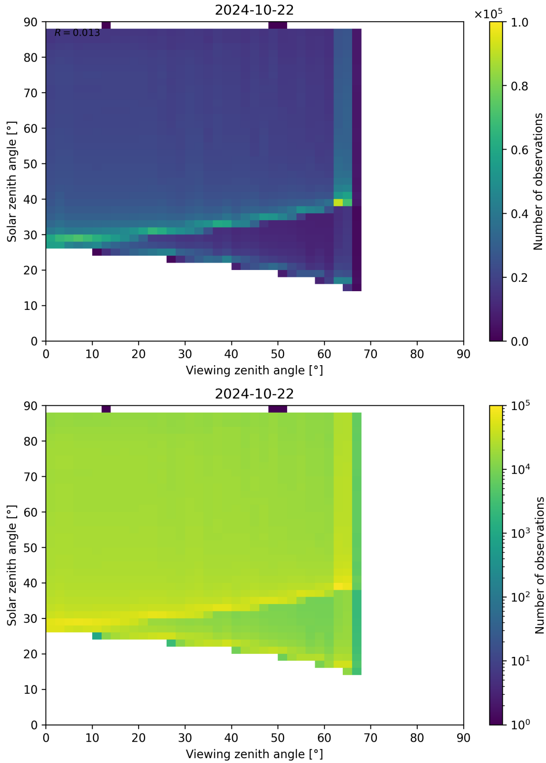
Figure 139: Scatter density plot of “Viewing zenith angle” against “Solar zenith angle” for 2024-10-21 to 2024-10-23.
