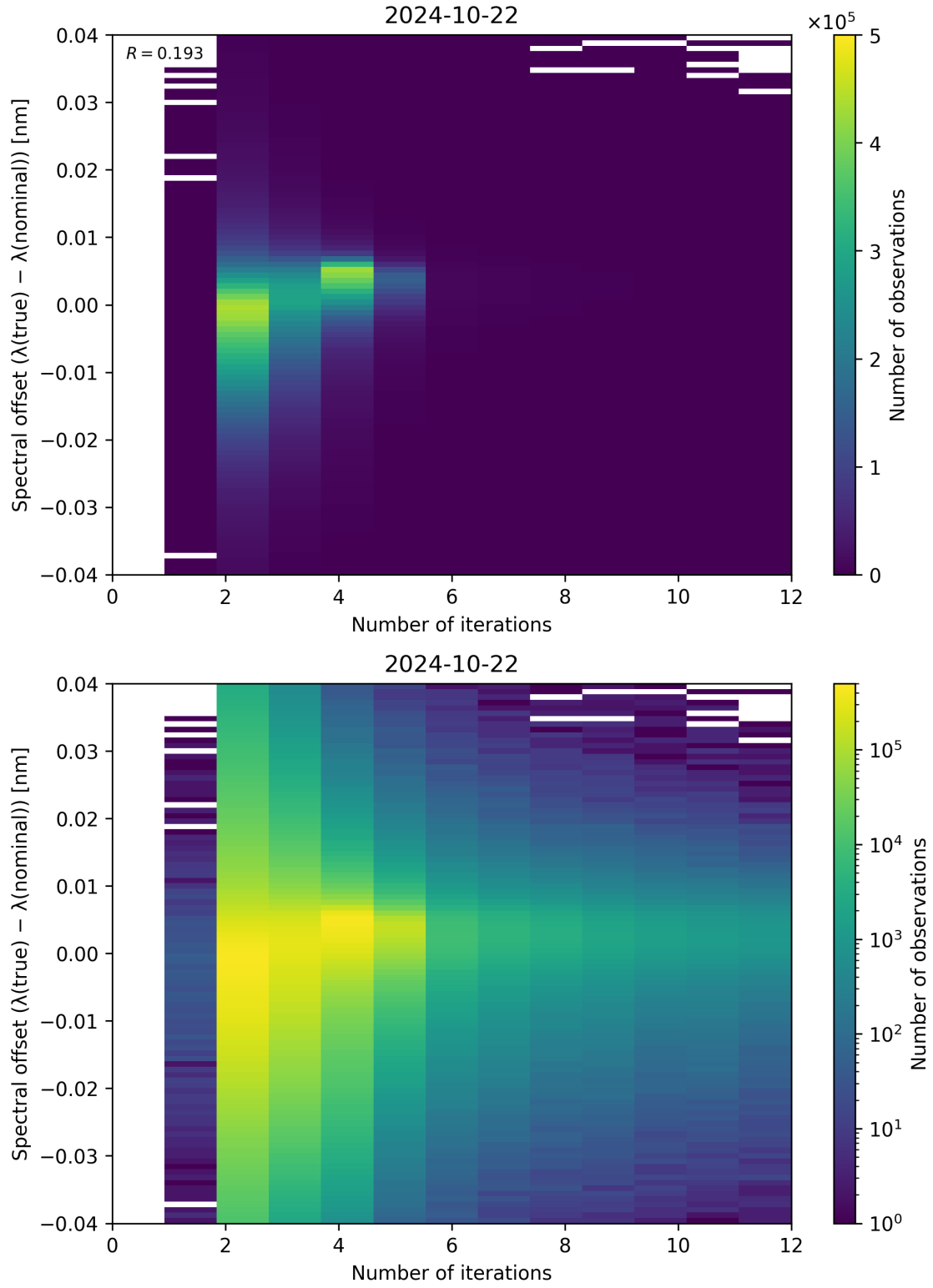
Figure 109: Scatter density plot of “Number of iterations” against “Spectral offset ( \lambda_{\text{true}} - \lambda_{\text{nominal}} )” for 2024-10-21 to 2024-10-23.
