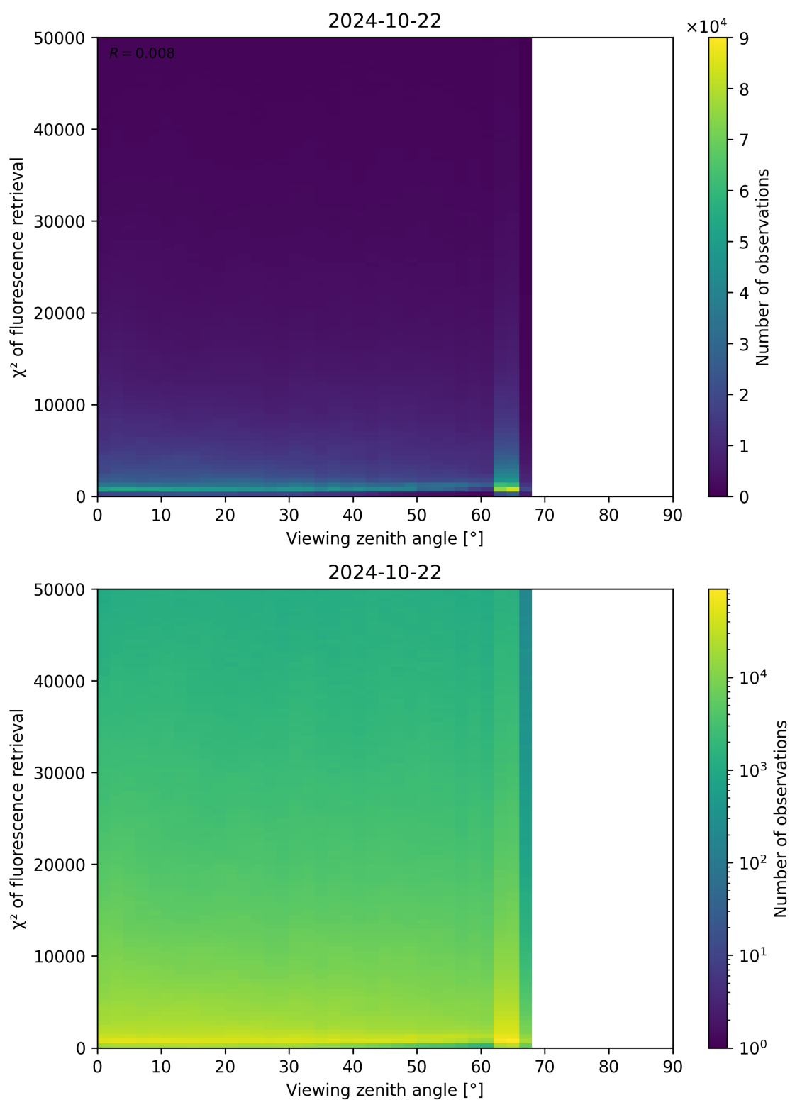
Figure 131: Scatter density plot of “Viewing zenith angle” against “ \chi^2 of fluorescence retrieval” for 2024-10-21 to 2024-10-23.
