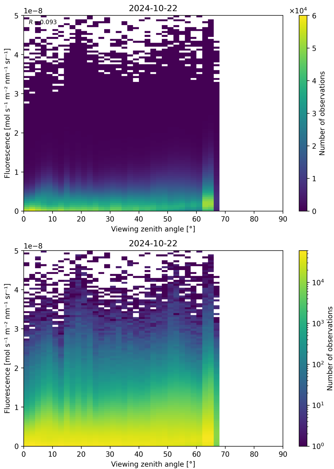
Figure 134: Scatter density plot of “Viewing zenith angle” against “Fluorescence” for 2024-10-21 to 2024-10-23.
