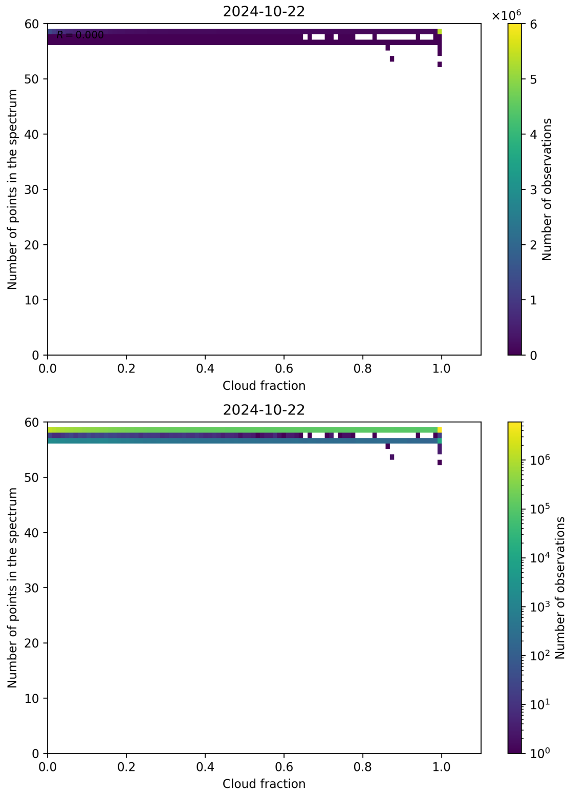
Figure 81: Scatter density plot of “Cloud fraction” against “Number of points in the spectrum” for 2024-10-21 to 2024-10-23.
