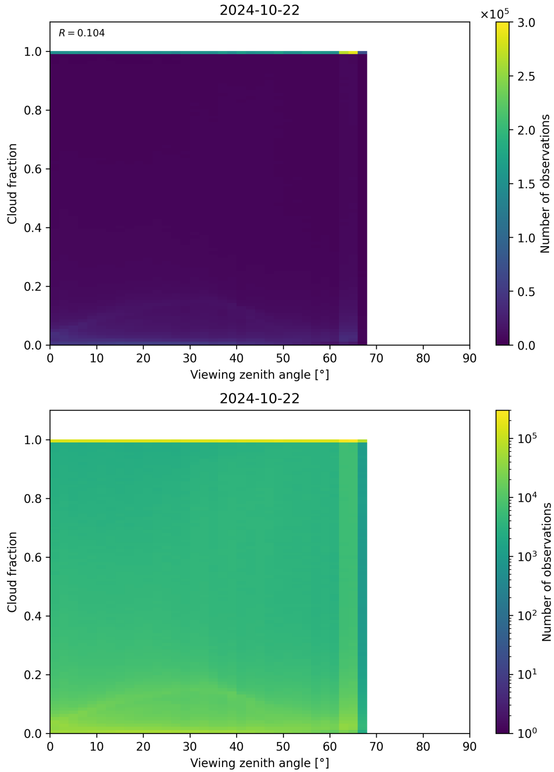
Figure 132: Scatter density plot of “Viewing zenith angle” against “Cloud fraction” for 2024-10-21 to 2024-10-23.
