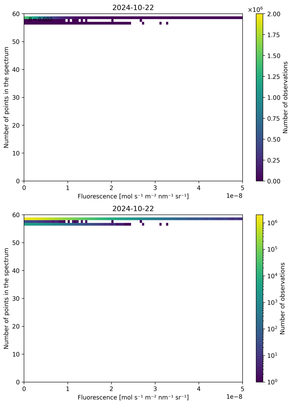
Figure 94: Scatter density plot of “Fluorescence” against “Number of points in the spectrum” for 2024-10-21 to 2024-10-23.
