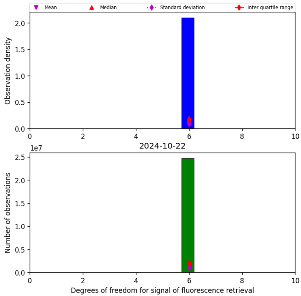
Figure 43: Histogram of “Degrees of freedom for signal of fluorescence retrieval” for 2024-10-21 to 2024-10-23
