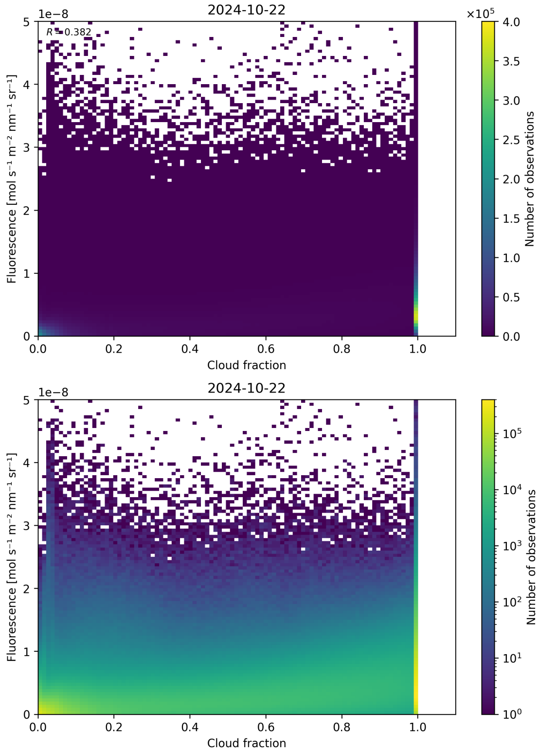
Figure 79: Scatter density plot of “Cloud fraction” against “Fluorescence” for 2024-10-21 to 2024-10-23.
