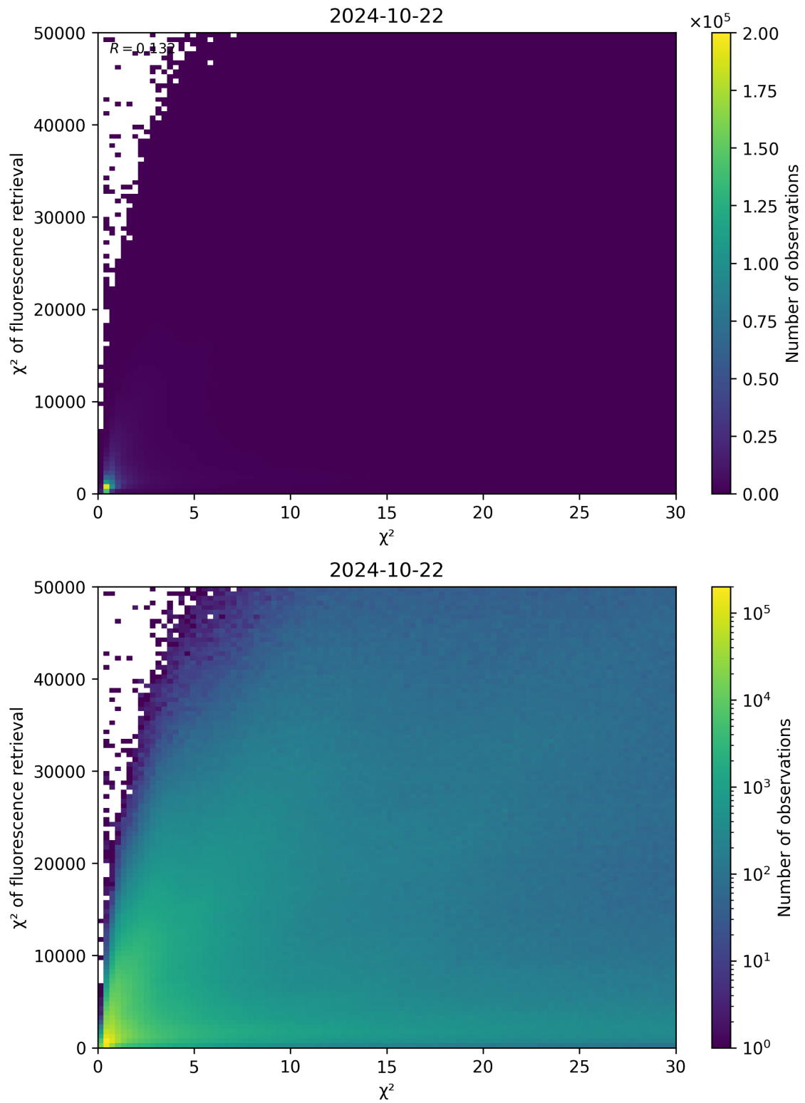
Figure 69: Scatter density plot of “ \chi^2 ” against “ \chi^2 of fluorescence retrieval” for 2024-10-21 to 2024-10-23.
