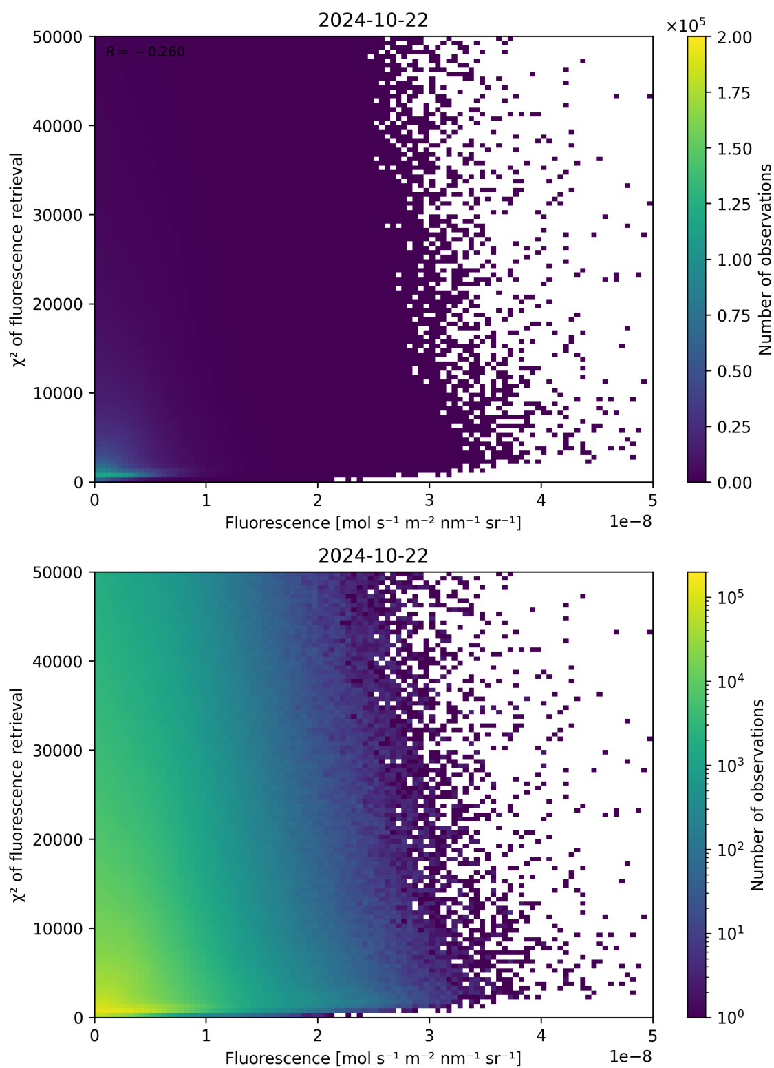
Figure 93: Scatter density plot of “Fluorescence” against “ \chi^2 of fluorescence retrieval” for 2024-10-21 to 2024-10-23.
