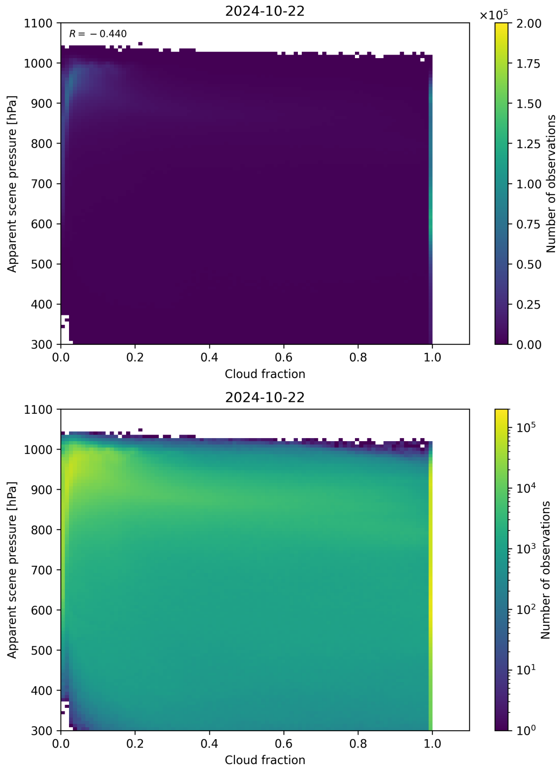
Figure 76: Scatter density plot of “Cloud fraction” against “Apparent scene pressure” for 2024-10-21 to 2024-10-23.
