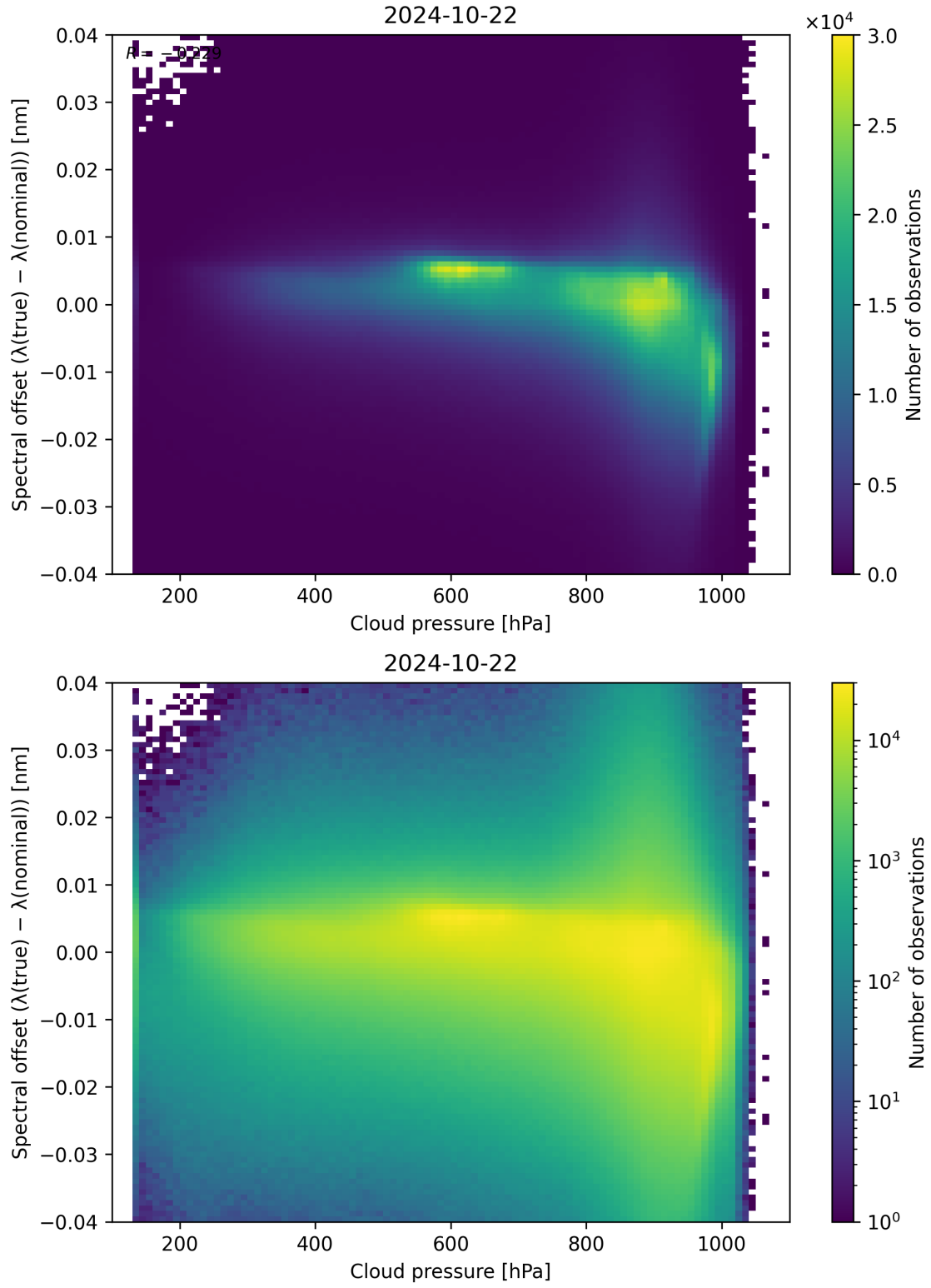
Figure 92: Scatter density plot of “Cloud pressure” against “Spectral offset ( \lambda_{\text{true}} - \lambda_{\text{nominal}} )” for 2024-10-21 to 2024-10-23.
