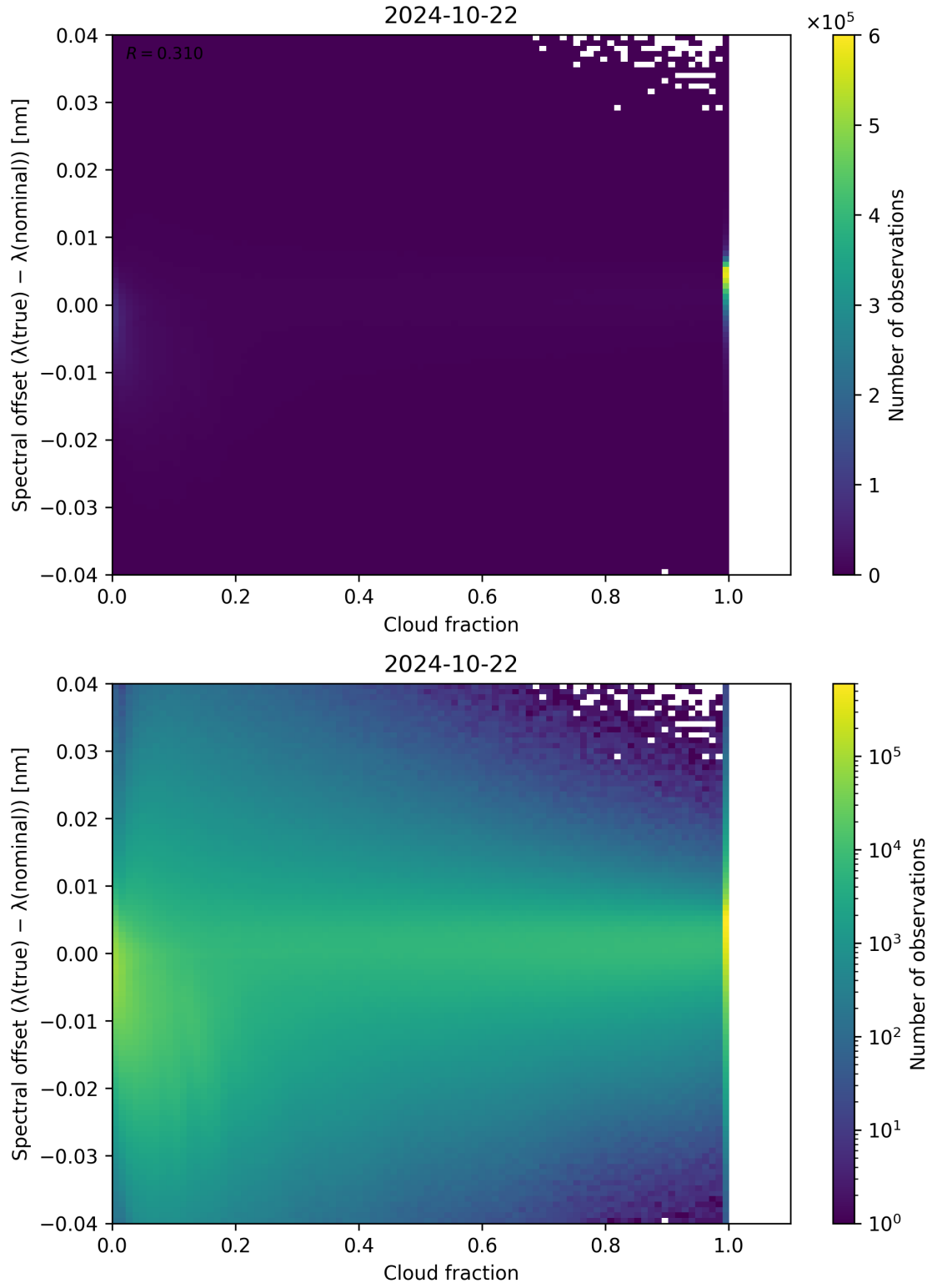
Figure 83: Scatter density plot of “Cloud fraction” against “Spectral offset ( \lambda_{\text{true}} - \lambda_{\text{nominal}} )” for 2024-10-21 to 2024-10-23.
