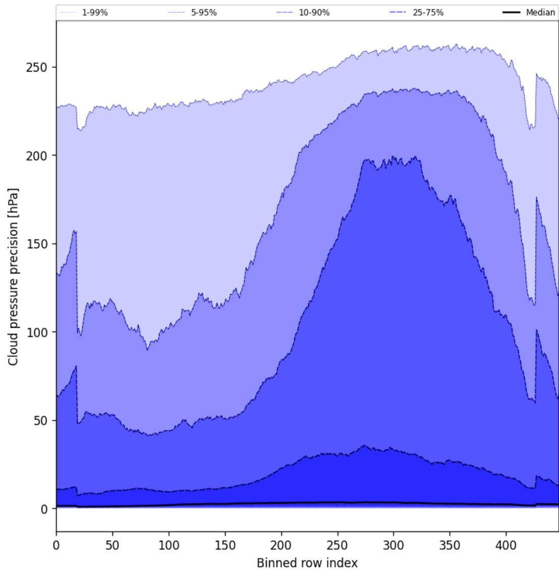
Figure 48: Along track statistics of “Cloud pressure precision” for 2024-10-21 to 2024-10-23
