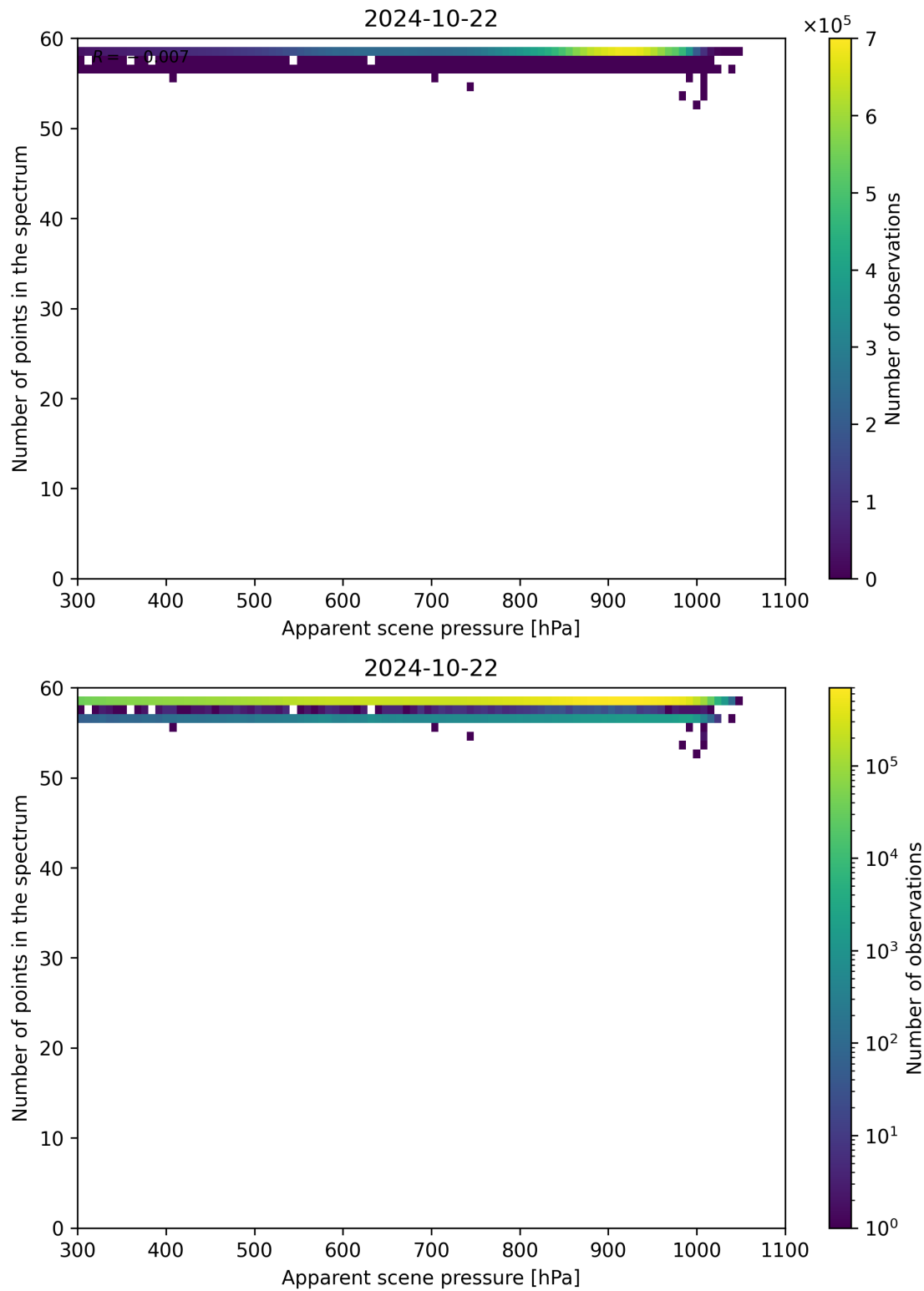
Figure 67: Scatter density plot of “Apparent scene pressure” against “Number of points in the spectrum” for 2024-10-21 to 2024-10-23.
