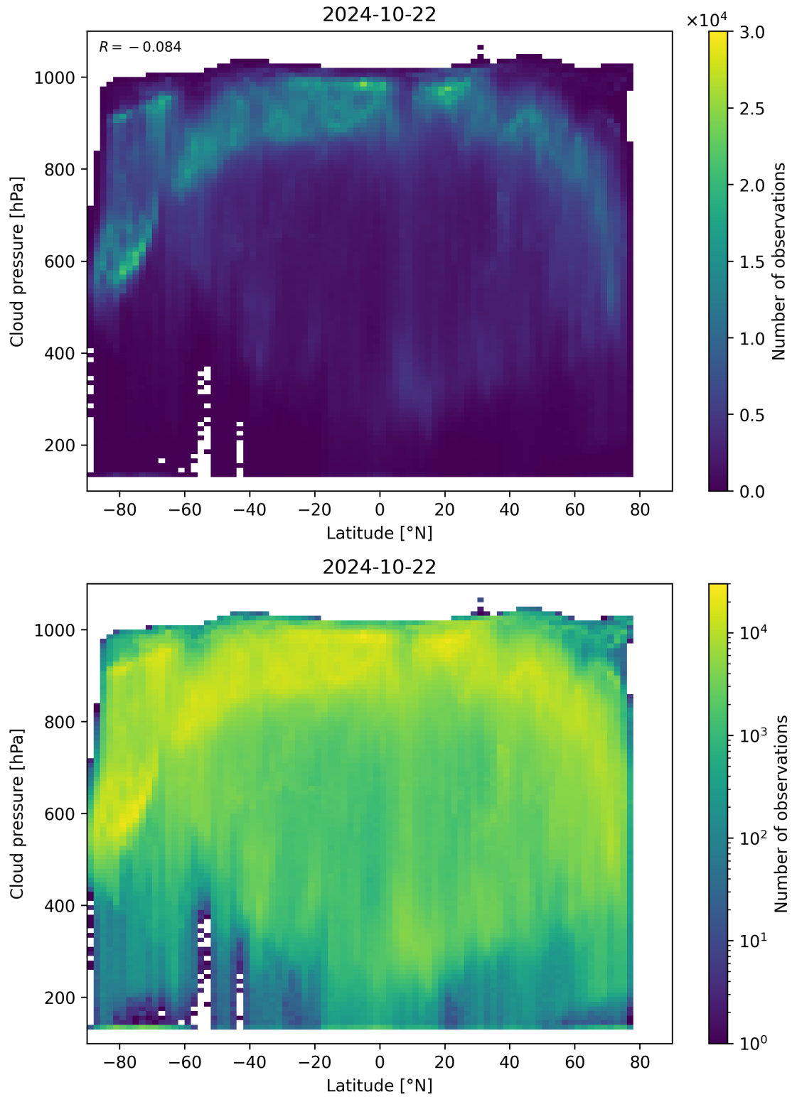
Figure 100: Scatter density plot of “Latitude” against “Cloud pressure” for 2024-10-21 to 2024-10-23.
