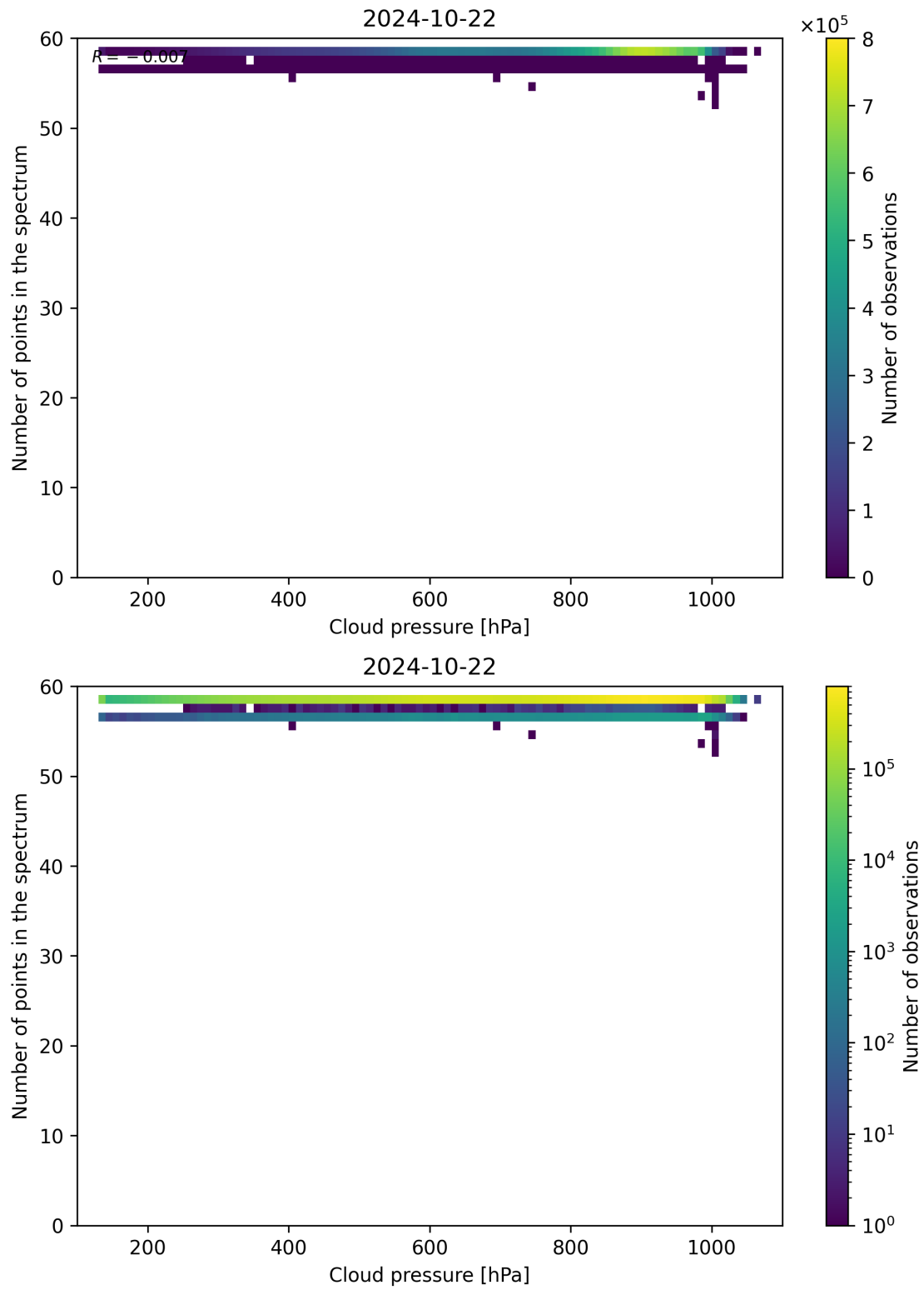
Figure 90: Scatter density plot of “Cloud pressure” against “Number of points in the spectrum” for 2024-10-21 to 2024-10-23.
