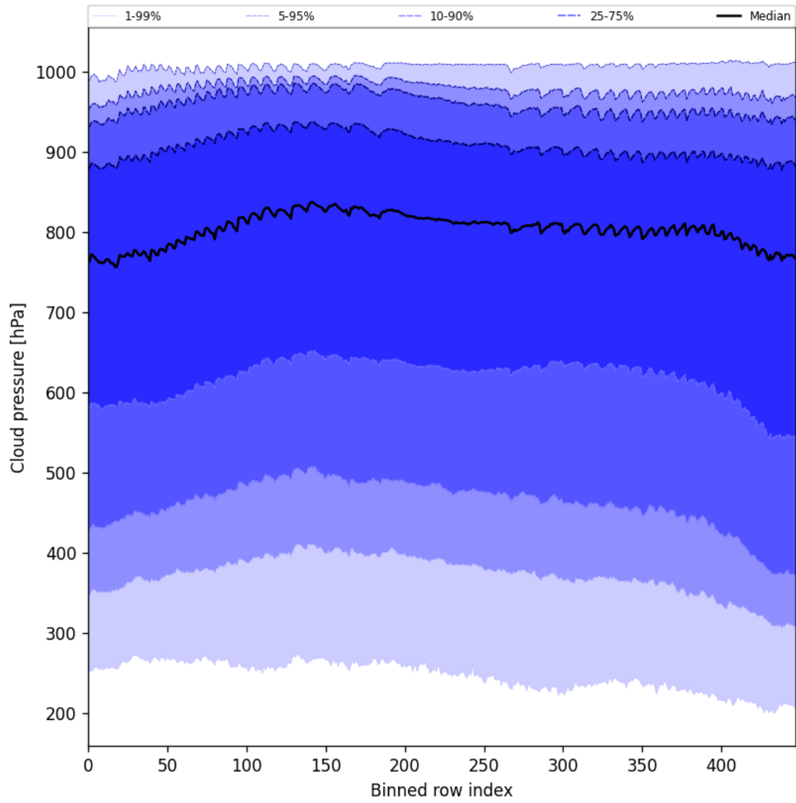
Figure 47: Along track statistics of “Cloud pressure” for 2024-10-21 to 2024-10-23
