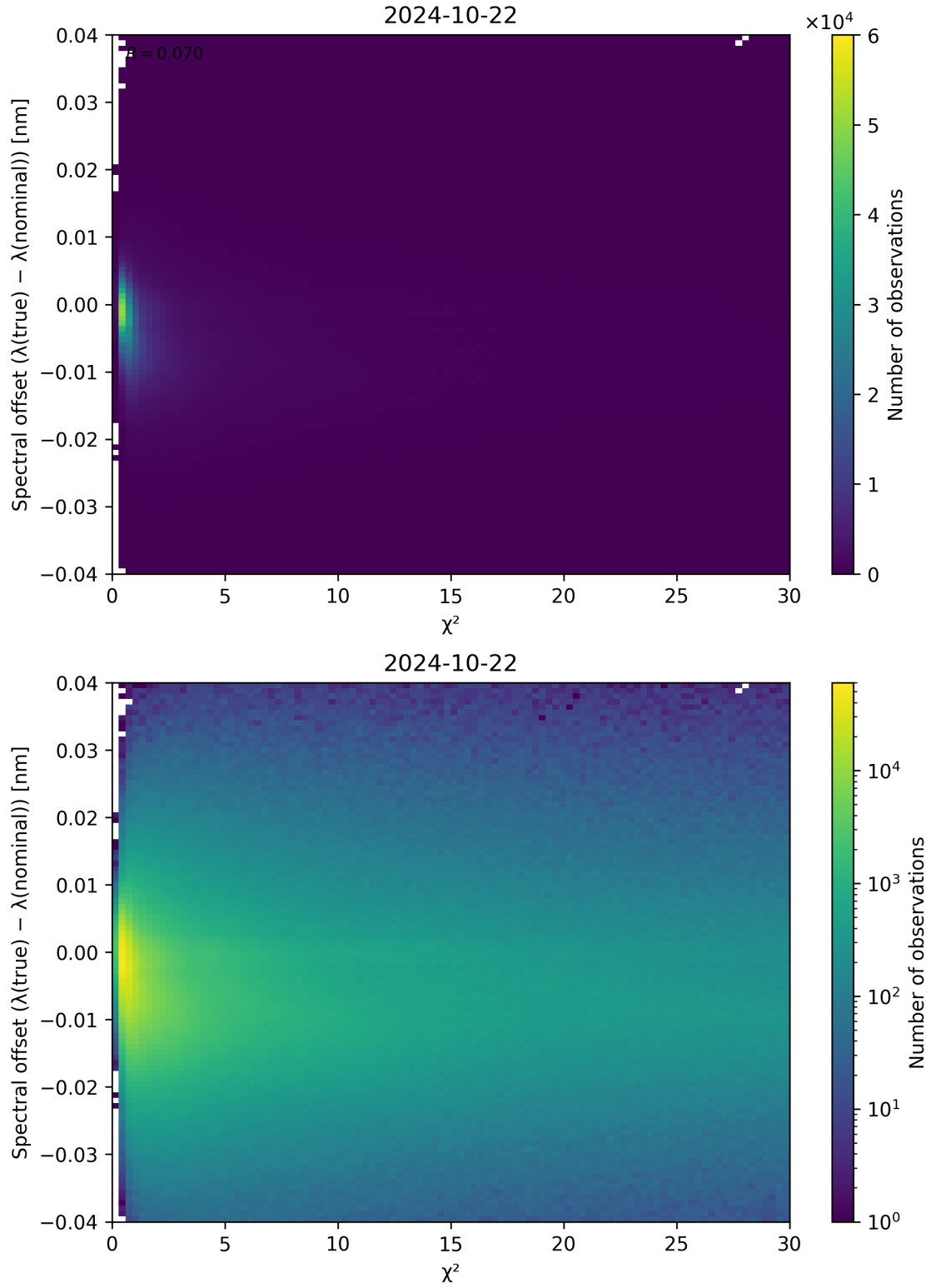
Figure 75: Scatter density plot of “ \chi^2 ” against “Spectral offset ( \lambda_{\text{true}} - \lambda_{\text{nominal}} )” for 2024-10-21 to 2024-10-23.
