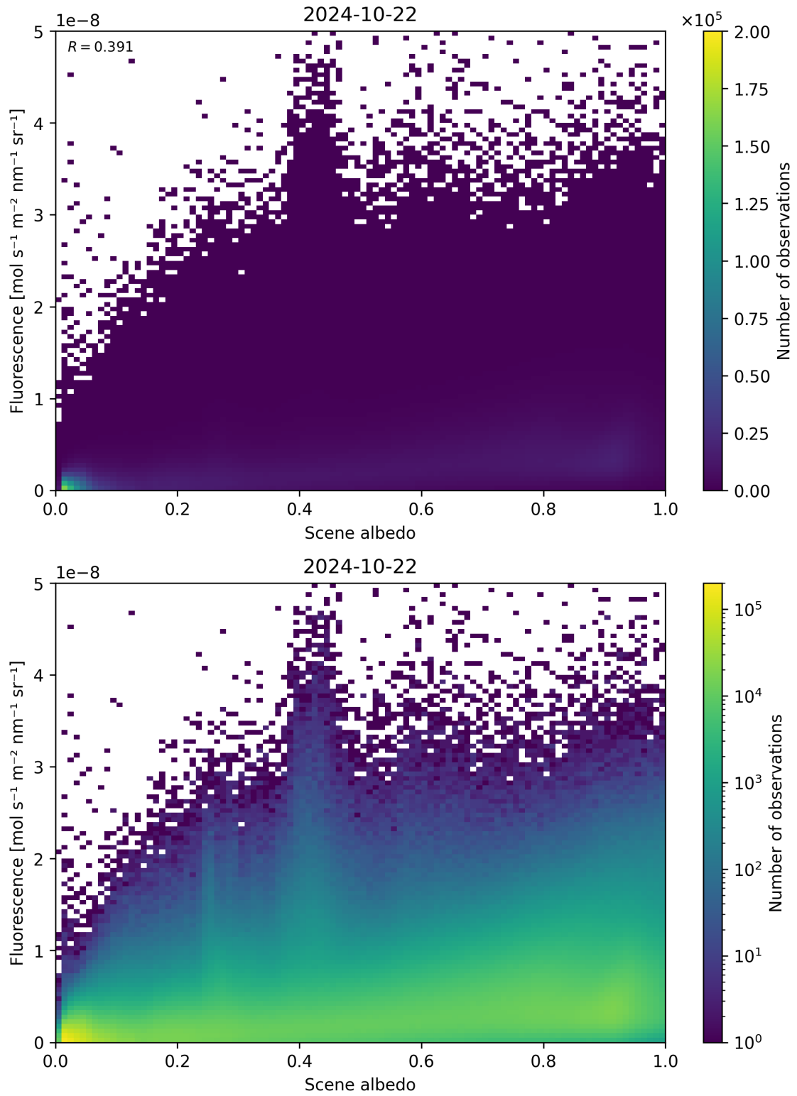
Figure 114: Scatter density plot of “Scene albedo” against “Fluorescence” for 2024-10-21 to 2024-10-23.
