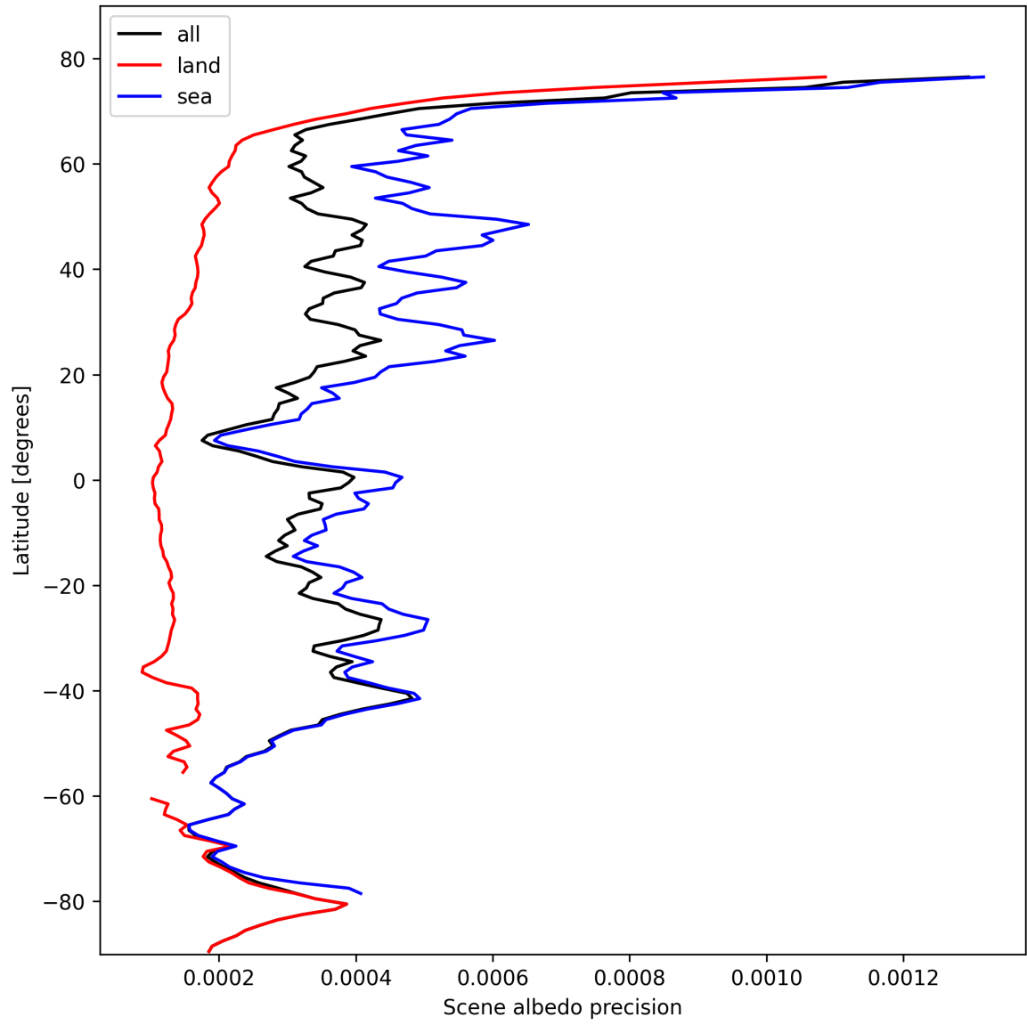
Figure 18: Zonal average of “Scene albedo precision” for 2024-10-21 to 2024-10-23.
