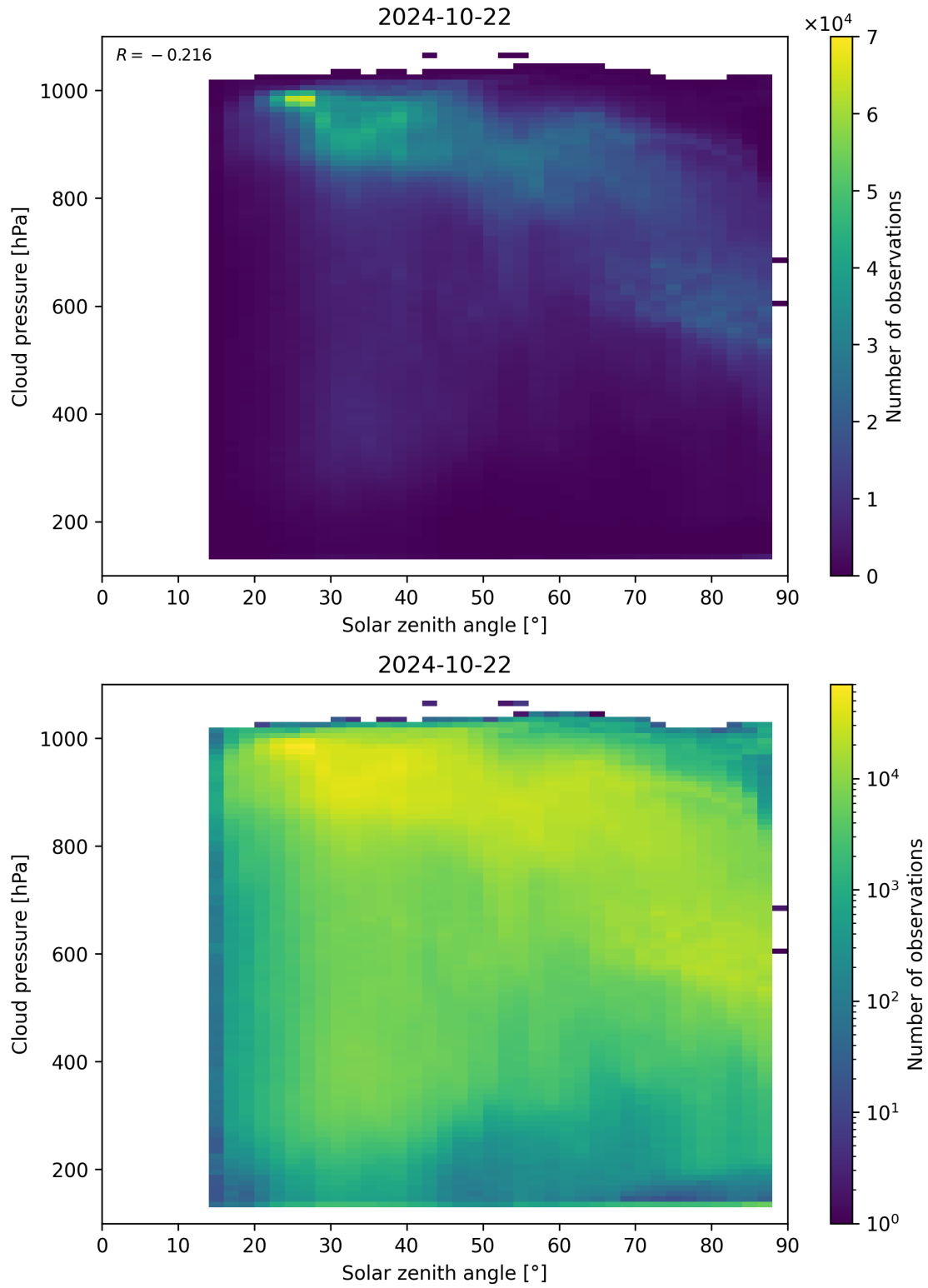
Figure 122: Scatter density plot of “Solar zenith angle” against “Cloud pressure” for 2024-10-21 to 2024-10-23.
