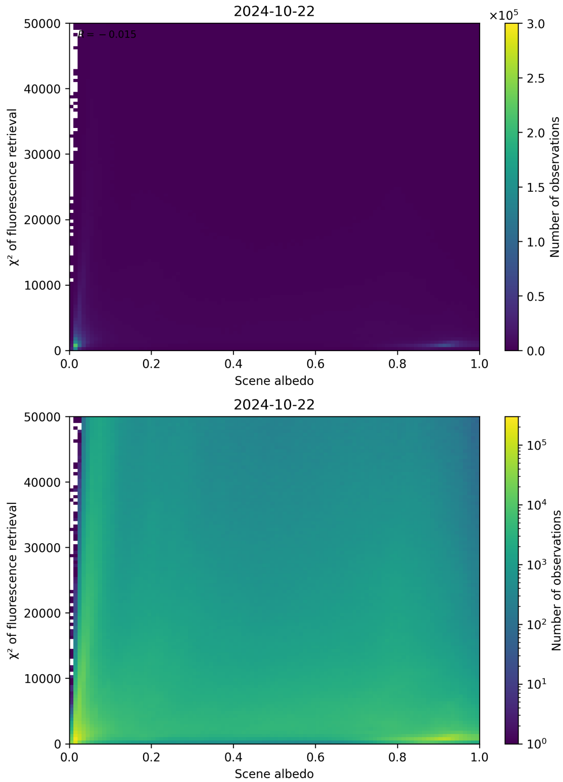
Figure 113: Scatter density plot of “Scene albedo” against “ \chi^2 of fluorescence retrieval” for 2024-10-21 to 2024-10-23.
