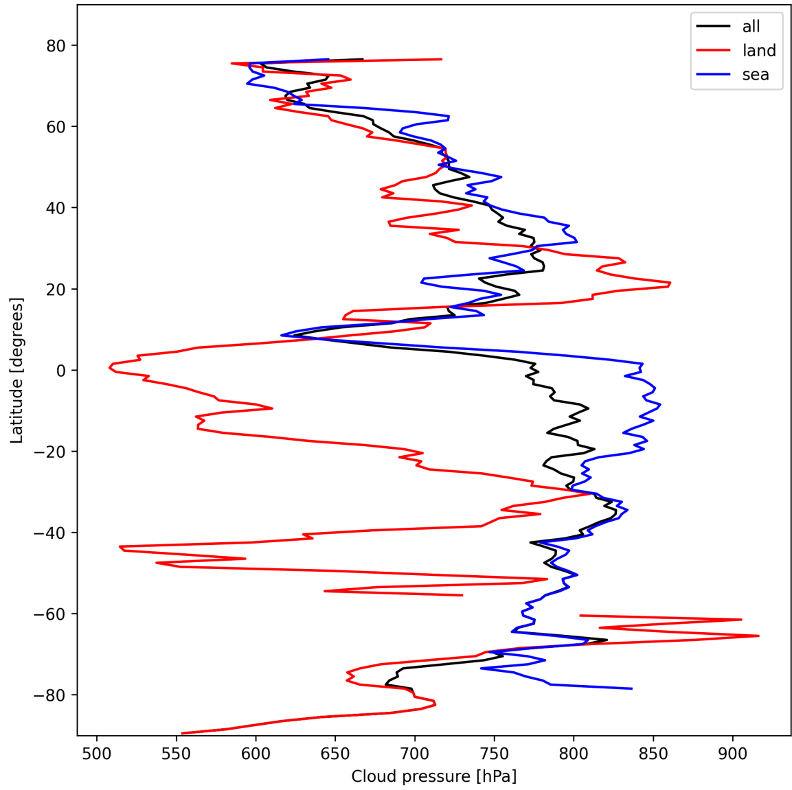
Figure 13: Zonal average of “Cloud pressure” for 2024-10-24 to 2024-10-25.
