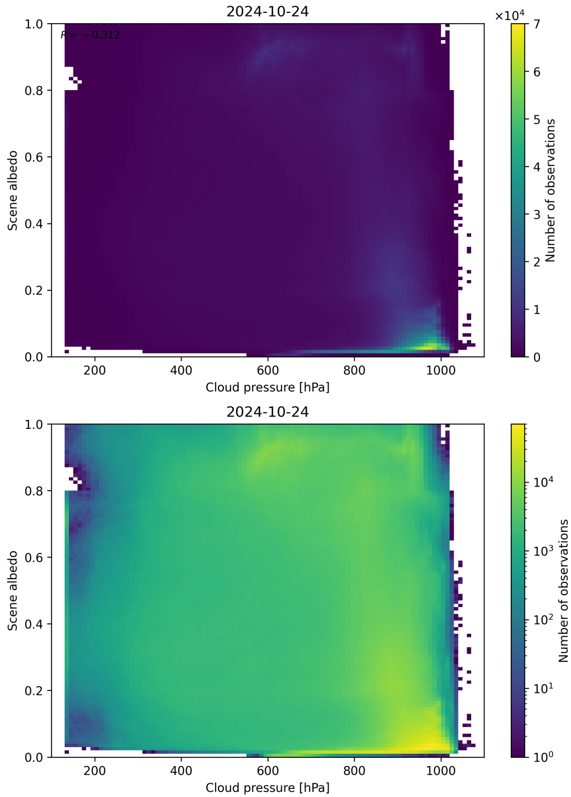
Figure 91: Scatter density plot of “Cloud pressure” against “Scene albedo” for 2024-10-24 to 2024-10-25.
