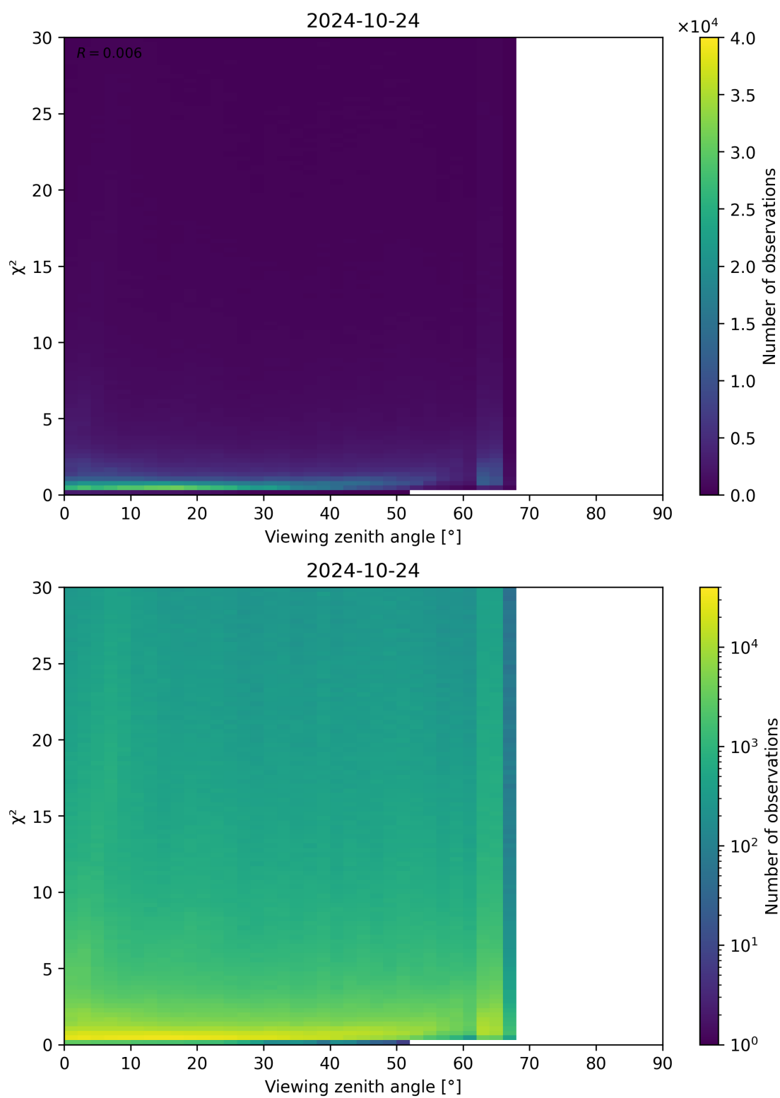
Figure 130: Scatter density plot of “Viewing zenith angle” against “ \chi^2 ” for 2024-10-24 to 2024-10-25.
