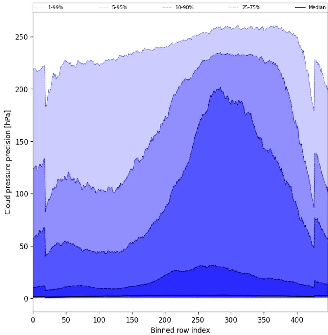
Figure 48: Along track statistics of “Cloud pressure precision” for 2024-10-24 to 2024-10-25
