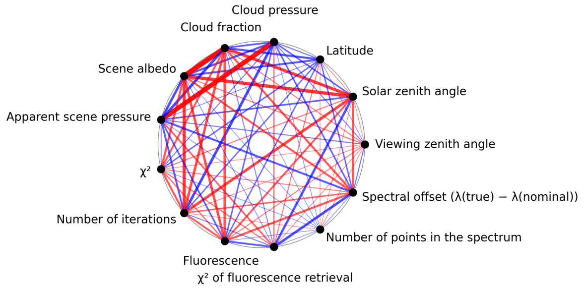
Figure 1: Map of correlation graph for 2024-10-24 to 2024-10-25.
