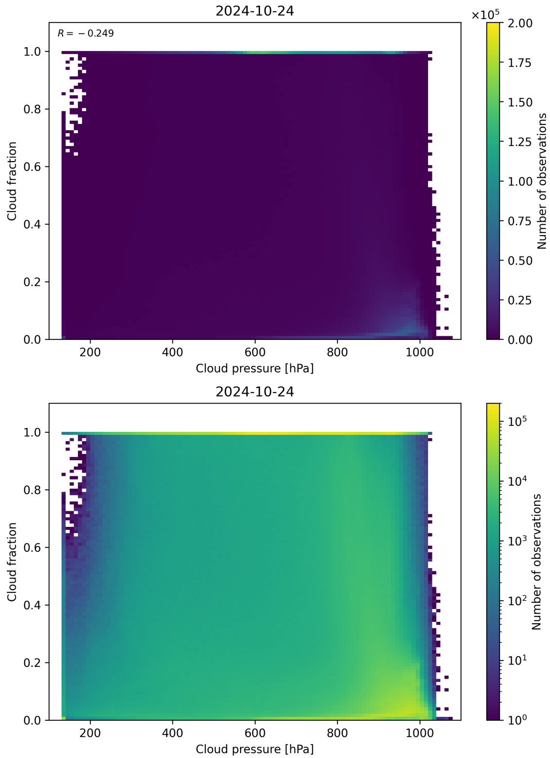
Figure 87: Scatter density plot of “Cloud pressure” against “Cloud fraction” for 2024-10-24 to 2024-10-25.
