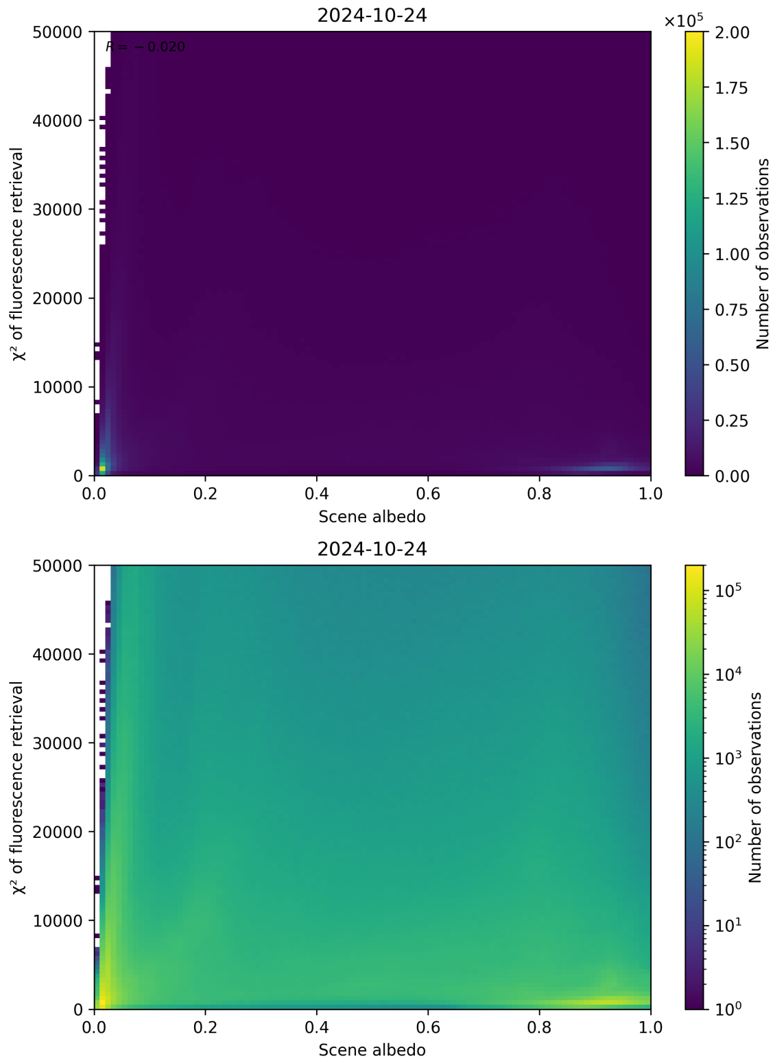
Figure 113: Scatter density plot of “Scene albedo” against “ \chi^2 of fluorescence retrieval” for 2024-10-24 to 2024-10-25.
