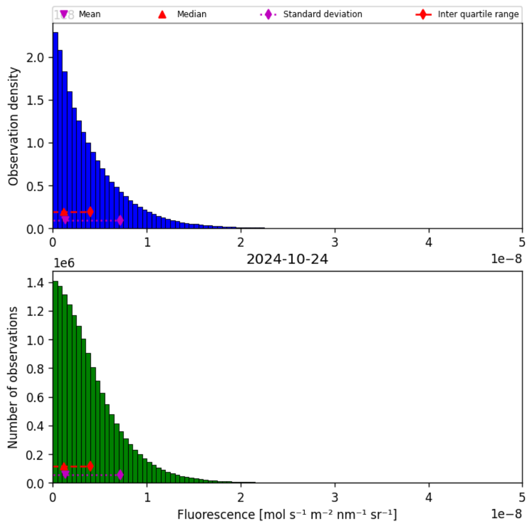
Figure 40: Histogram of “Fluorescence” for 2024-10-24 to 2024-10-25
