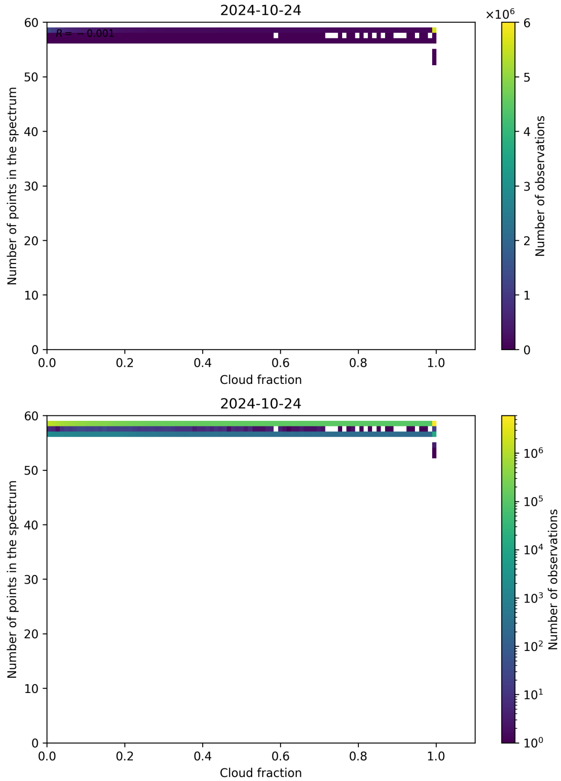
Figure 81: Scatter density plot of “Cloud fraction” against “Number of points in the spectrum” for 2024-10-24 to 2024-10-25.
