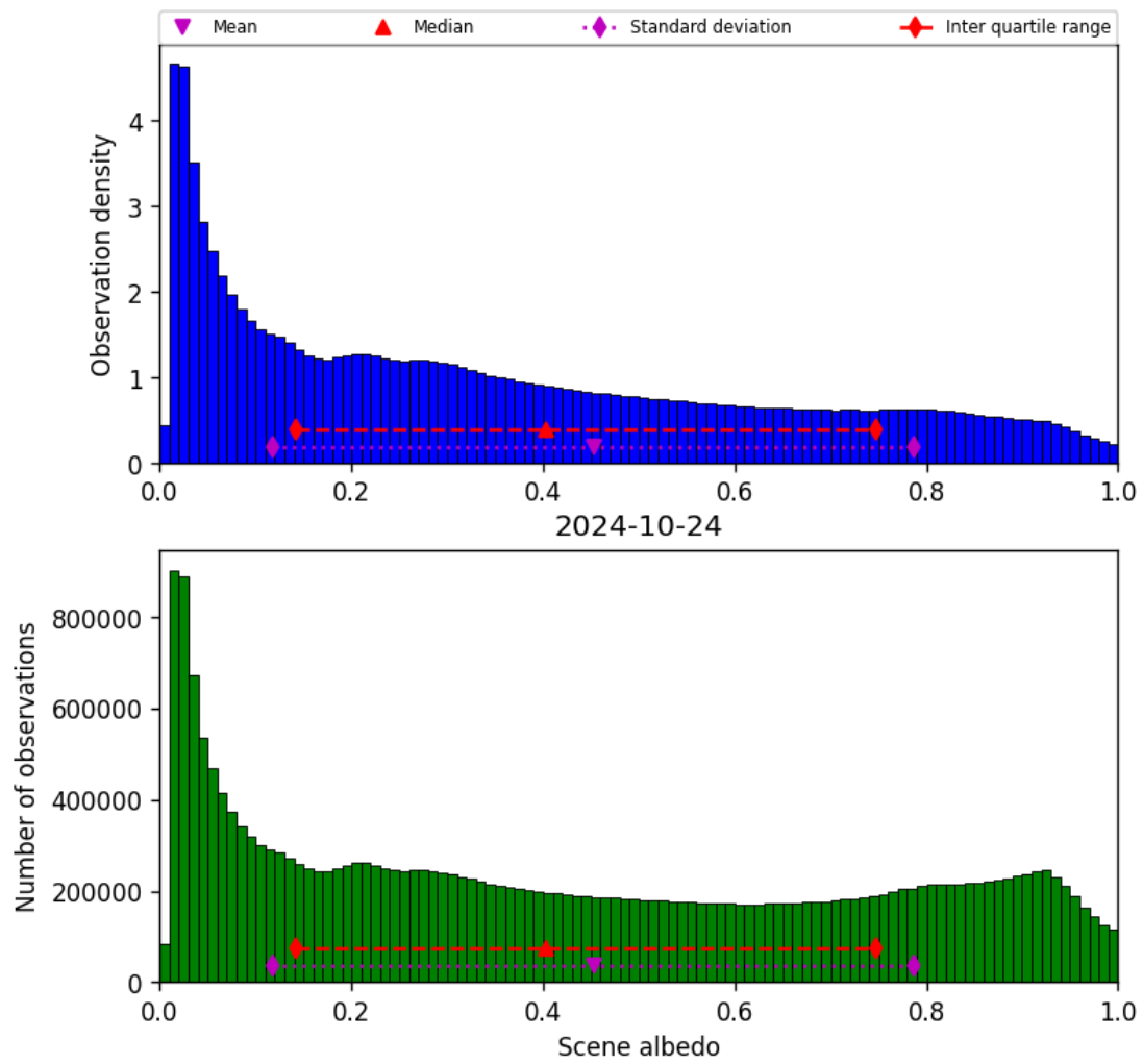
Figure 34: Histogram of “Scene albedo” for 2024-10-24 to 2024-10-25
