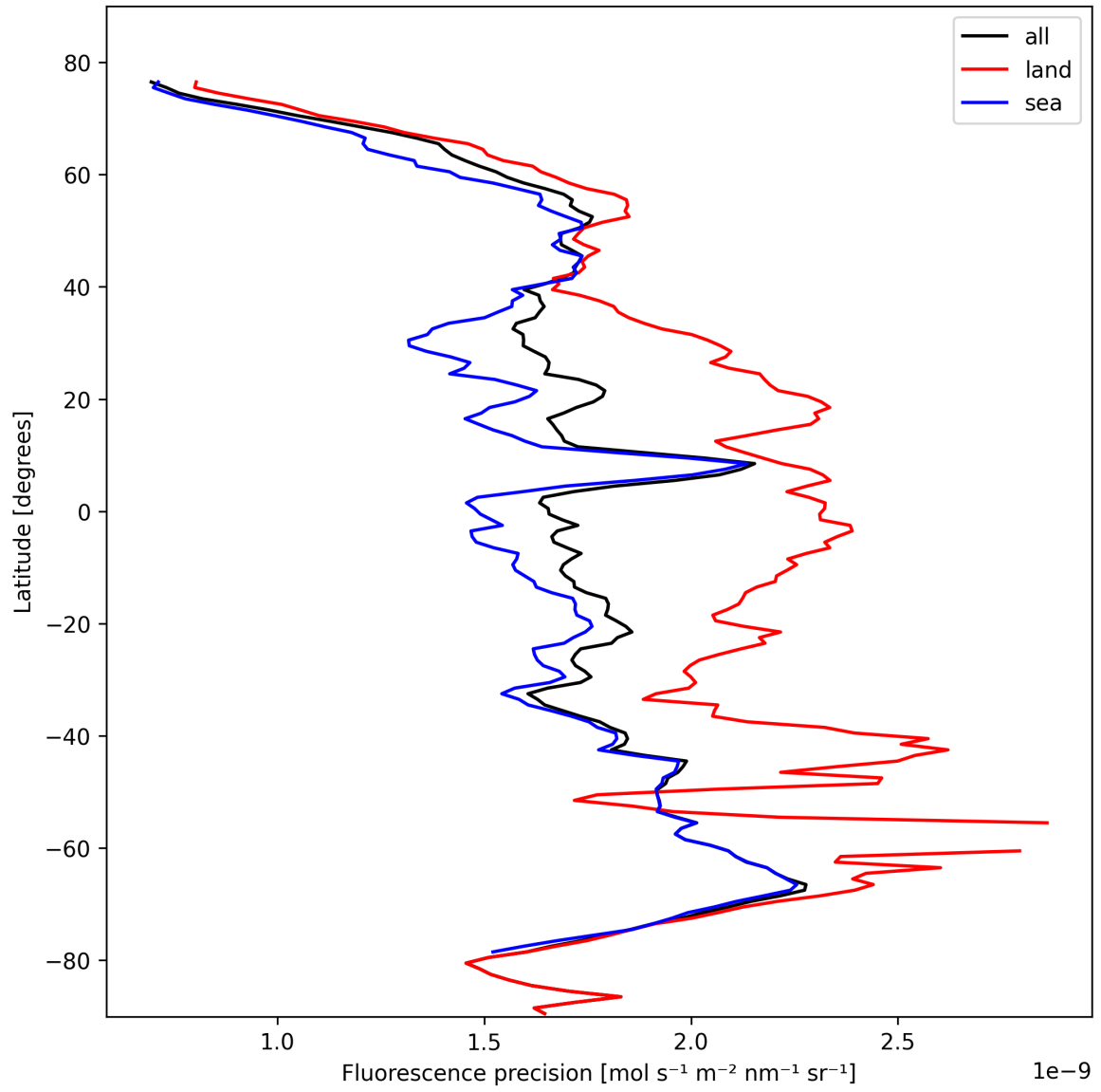
Figure 24: Zonal average of “Fluorescence precision” for 2024-10-24 to 2024-10-25.
