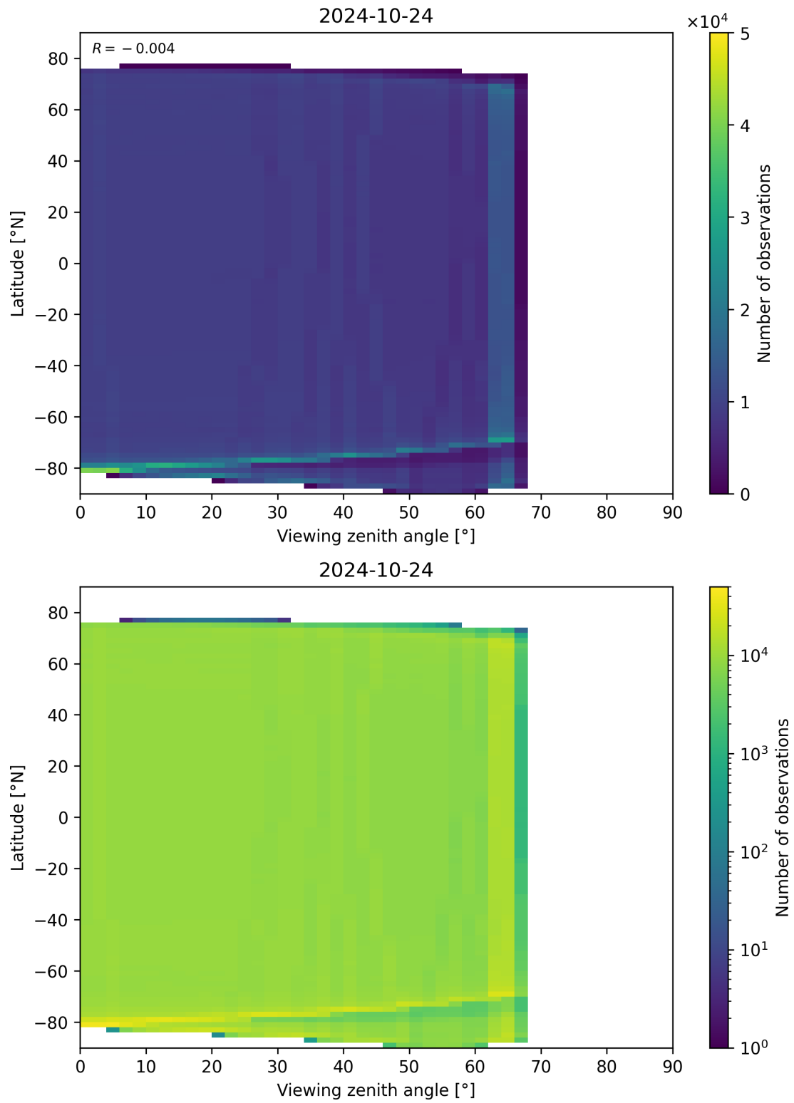
Figure 135: Scatter density plot of “Viewing zenith angle” against “Latitude” for 2024-10-24 to 2024-10-25.
