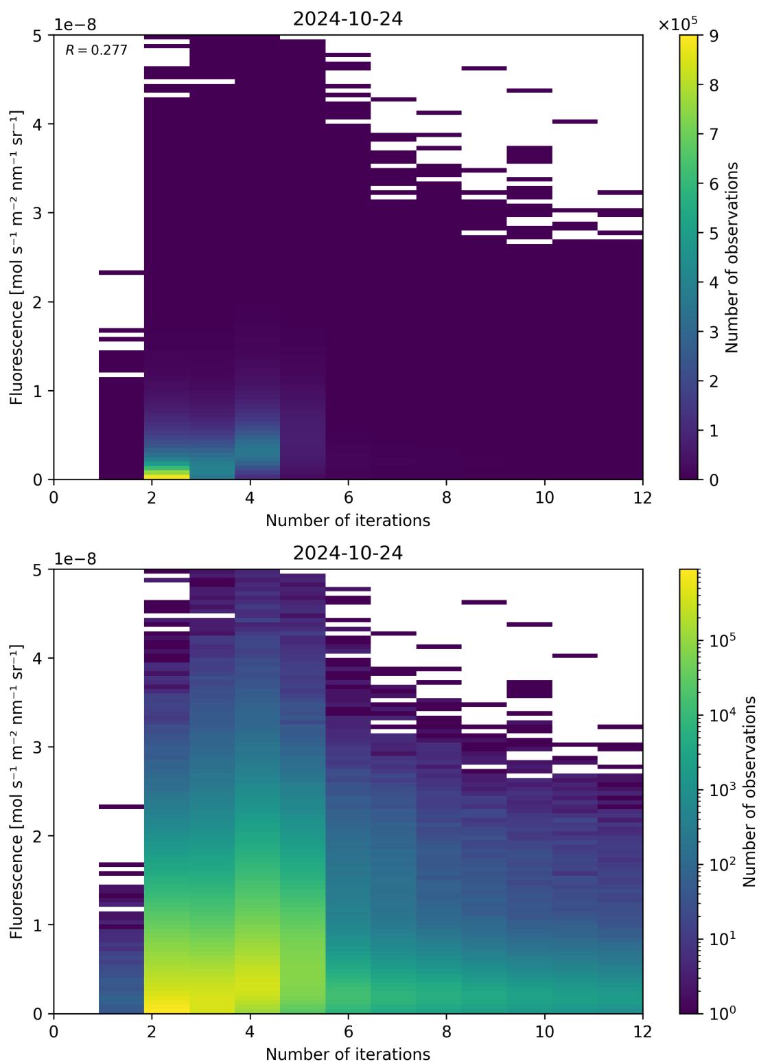
Figure 107: Scatter density plot of “Number of iterations” against “Fluorescence” for 2024-10-24 to 2024-10-25.
