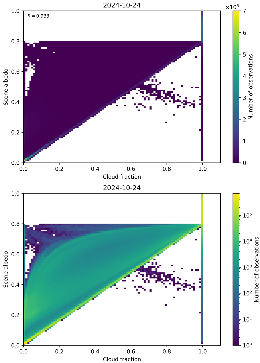
Figure 82: Scatter density plot of “Cloud fraction” against “Scene albedo” for 2024-10-24 to 2024-10-25.
