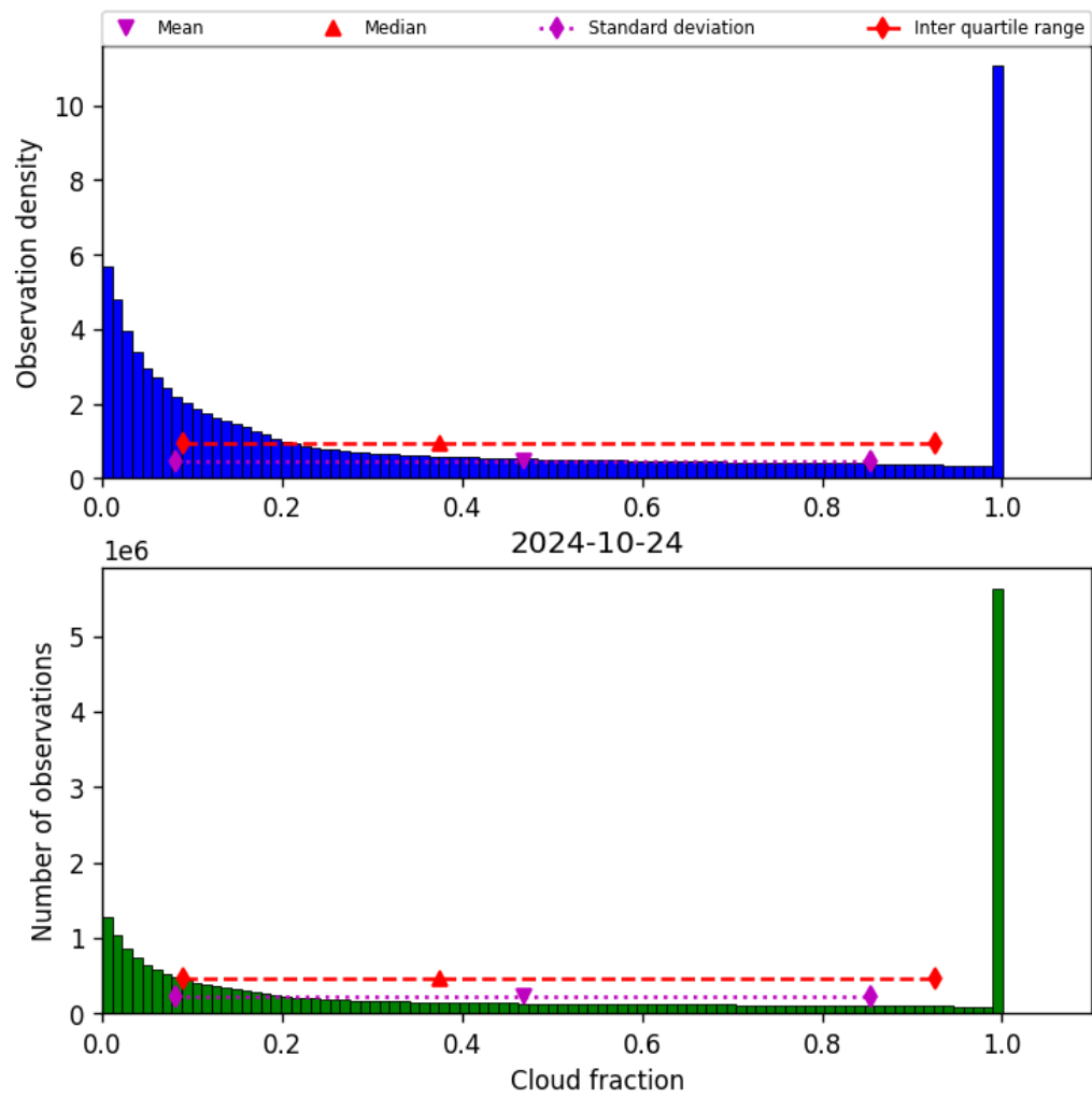
Figure 32: Histogram of “Cloud fraction” for 2024-10-24 to 2024-10-25
