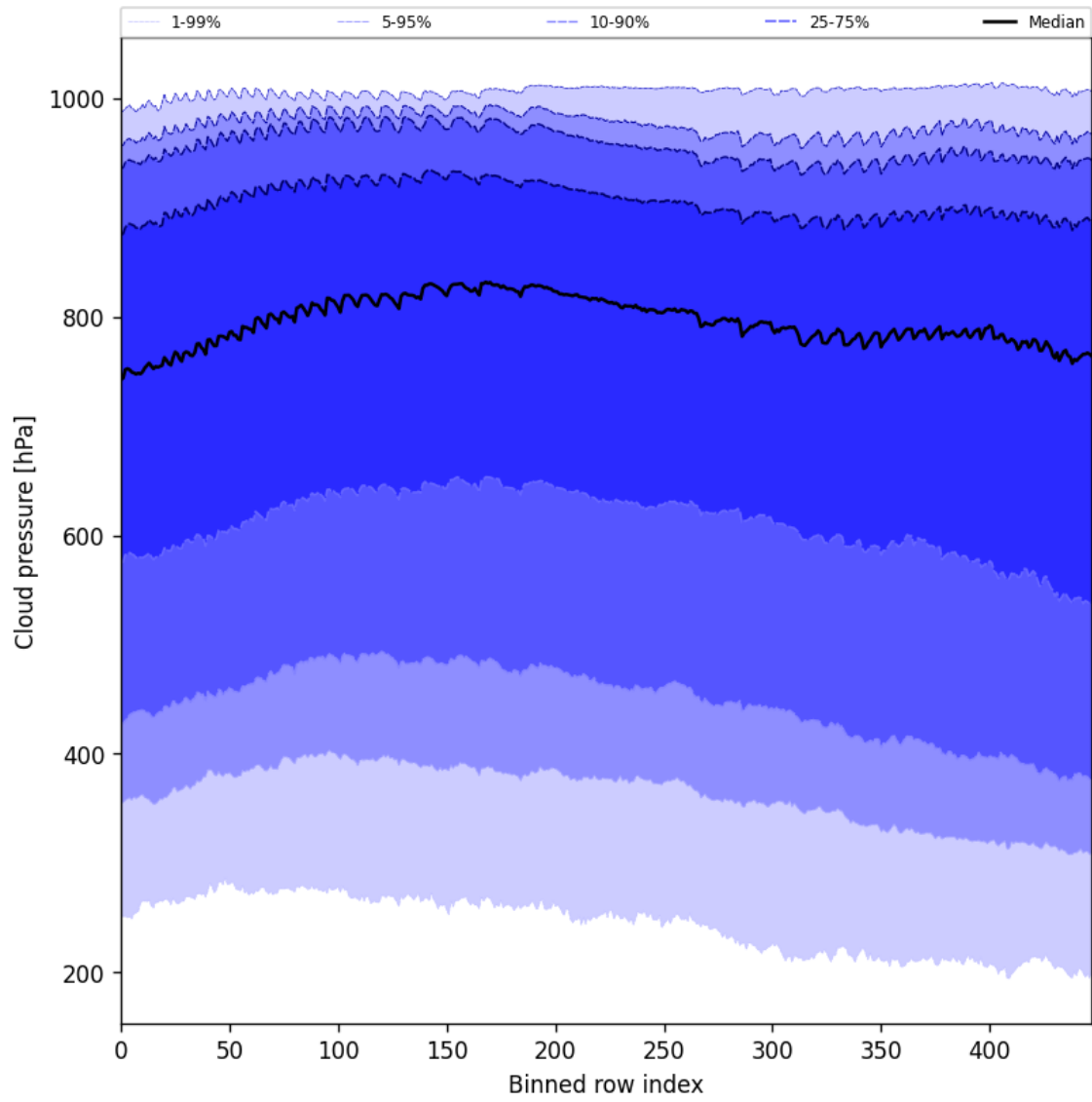
Figure 47: Along track statistics of "Cloud pressure" for 2024-10-24 to 2024-10-25
