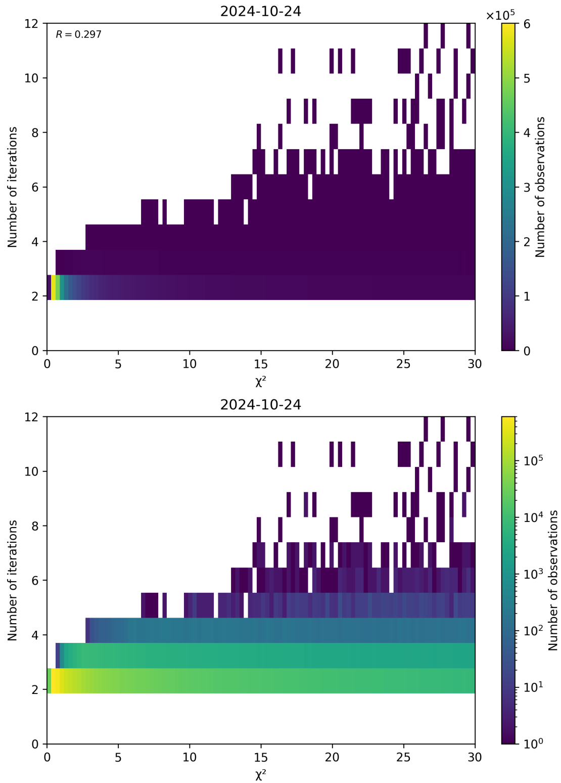
Figure 73: Scatter density plot of “ \chi^2 ” against “Number of iterations” for 2024-10-24 to 2024-10-25.
