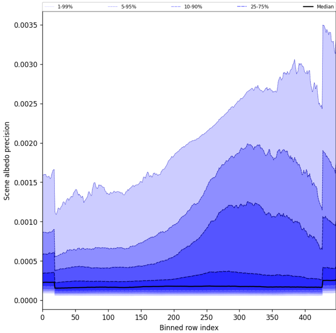
Figure 52: Along track statistics of “Scene albedo precision” for 2024-10-24 to 2024-10-25
