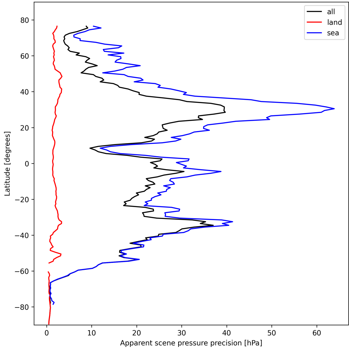
Figure 20: Zonal average of “Apparent scene pressure precision” for 2024-10-24 to 2024-10-25.
