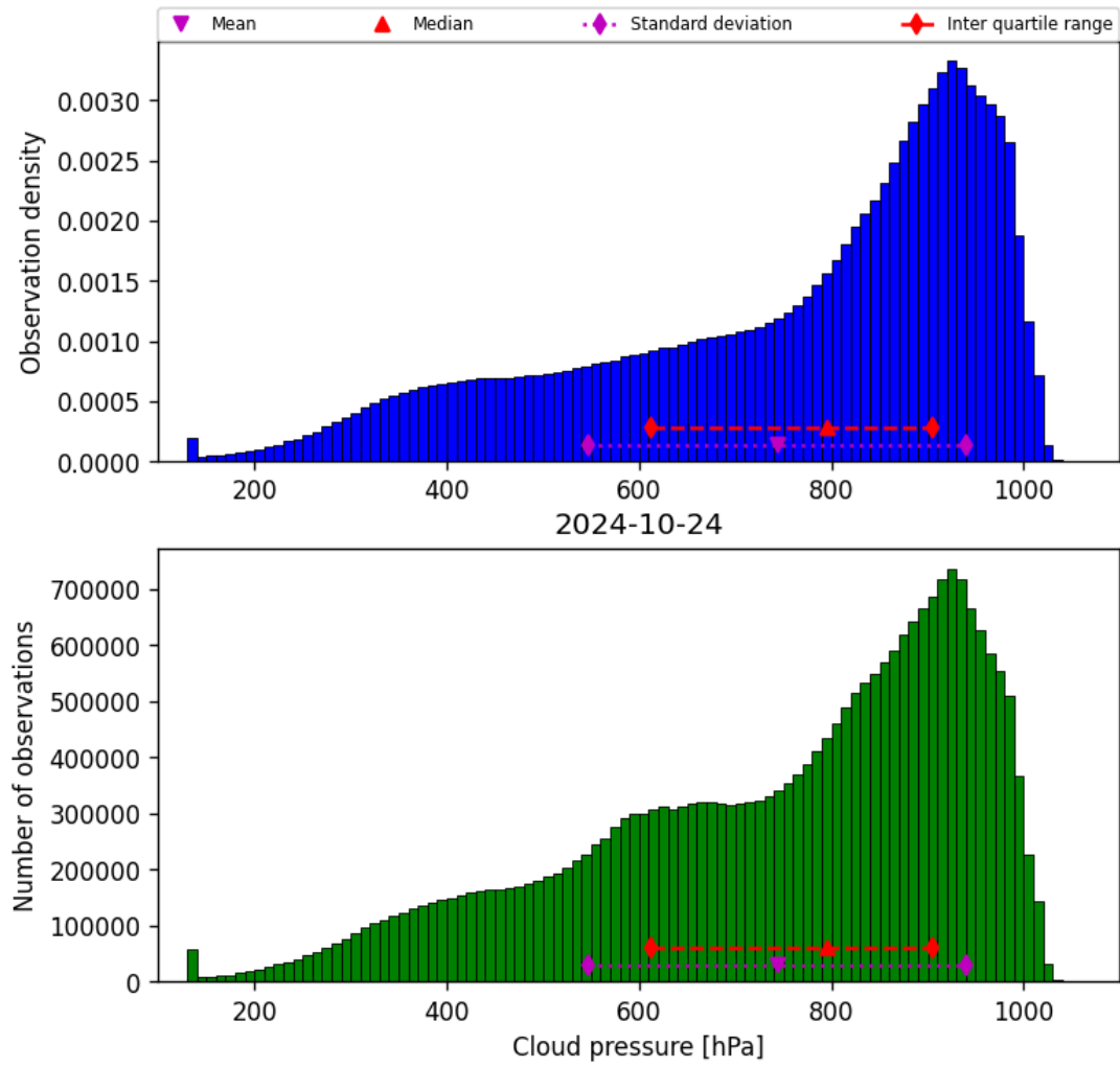
Figure 30: Histogram of “Cloud pressure” for 2024-10-24 to 2024-10-25
