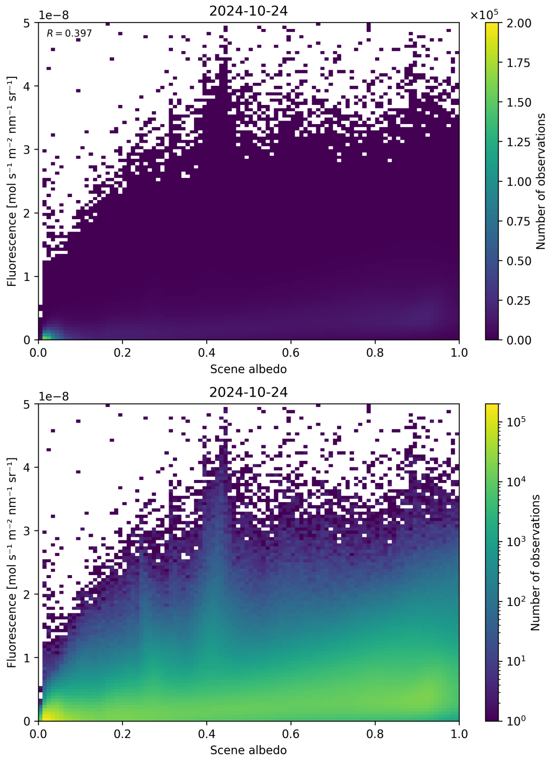
Figure 114: Scatter density plot of “Scene albedo” against “Fluorescence” for 2024-10-24 to 2024-10-25.
