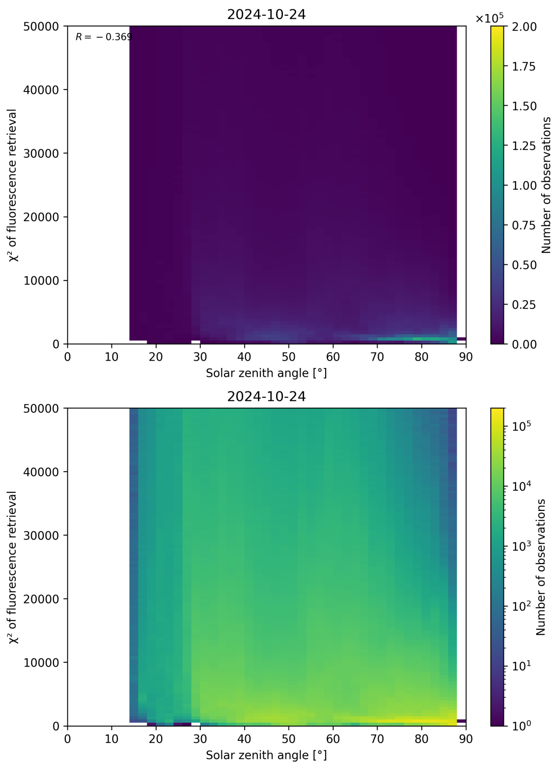
Figure 120: Scatter density plot of “Solar zenith angle” against “ \chi^2 of fluorescence retrieval” for 2024-10-24 to 2024-10-25.
