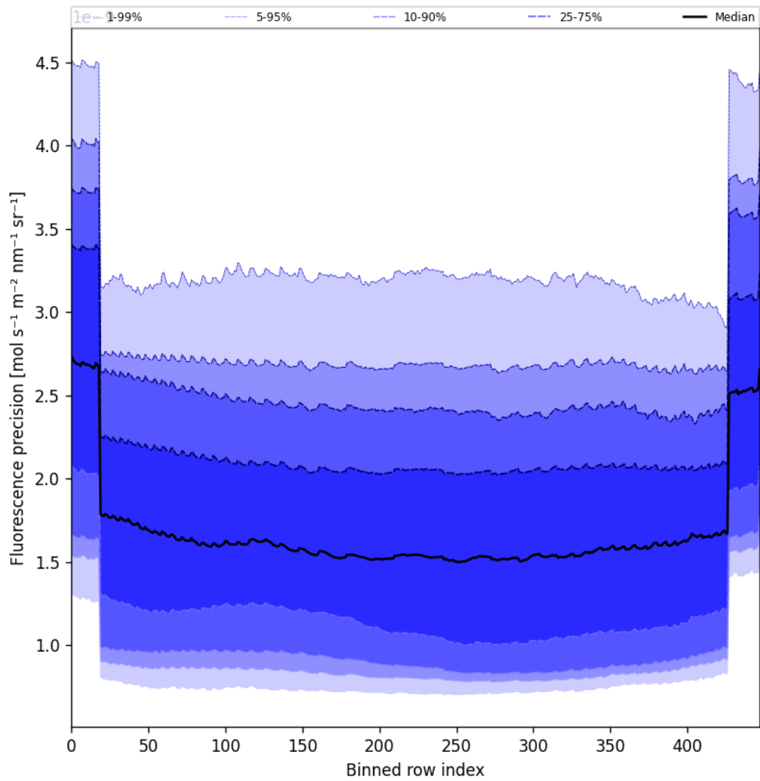
Figure 58: Along track statistics of “Fluorescence precision” for 2024-10-24 to 2024-10-25
