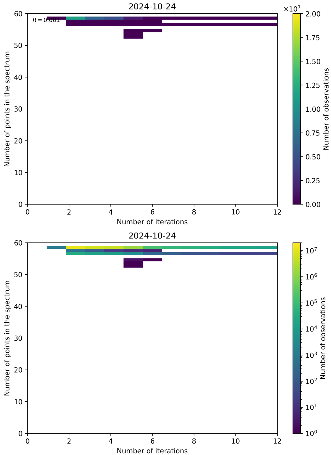
Figure 108: Scatter density plot of “Number of iterations” against “Number of points in the spectrum” for 2024-10-24 to 2024-10-25.
