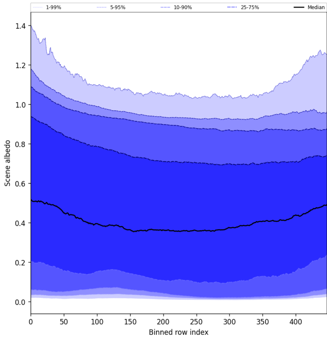
Figure 51: Along track statistics of “Scene albedo” for 2024-10-24 to 2024-10-25
