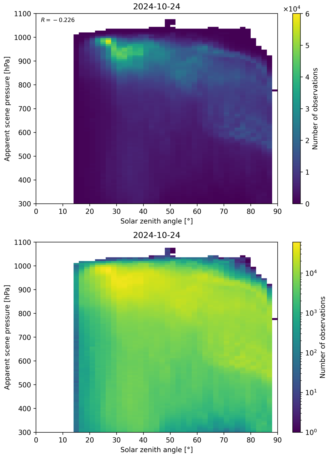
Figure 118: Scatter density plot of “Solar zenith angle” against “Apparent scene pressure” for 2024-10-24 to 2024-10-25.
