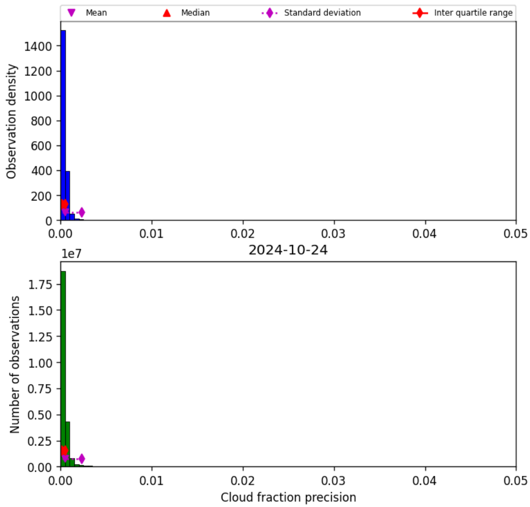
Figure 33: Histogram of “Cloud fraction precision” for 2024-10-24 to 2024-10-25
