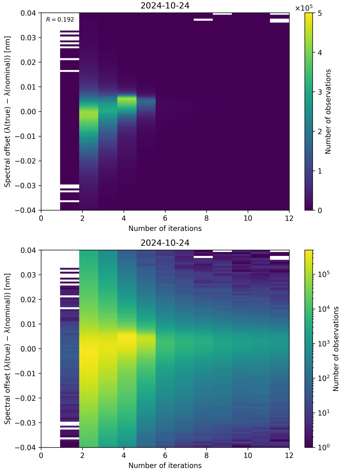
Figure 109: Scatter density plot of “Number of iterations” against “Spectral offset ( \lambda_{\text{true}} - \lambda_{\text{nominal}} )” for 2024-10-24 to 2024-10-25.
