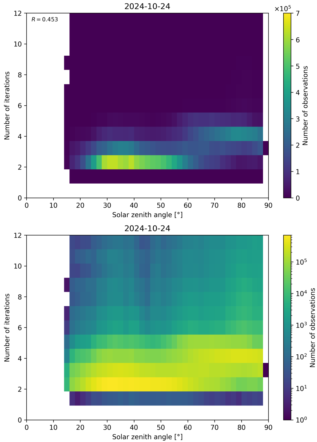
Figure 125: Scatter density plot of “Solar zenith angle” against “Number of iterations” for 2024-10-24 to 2024-10-25.
