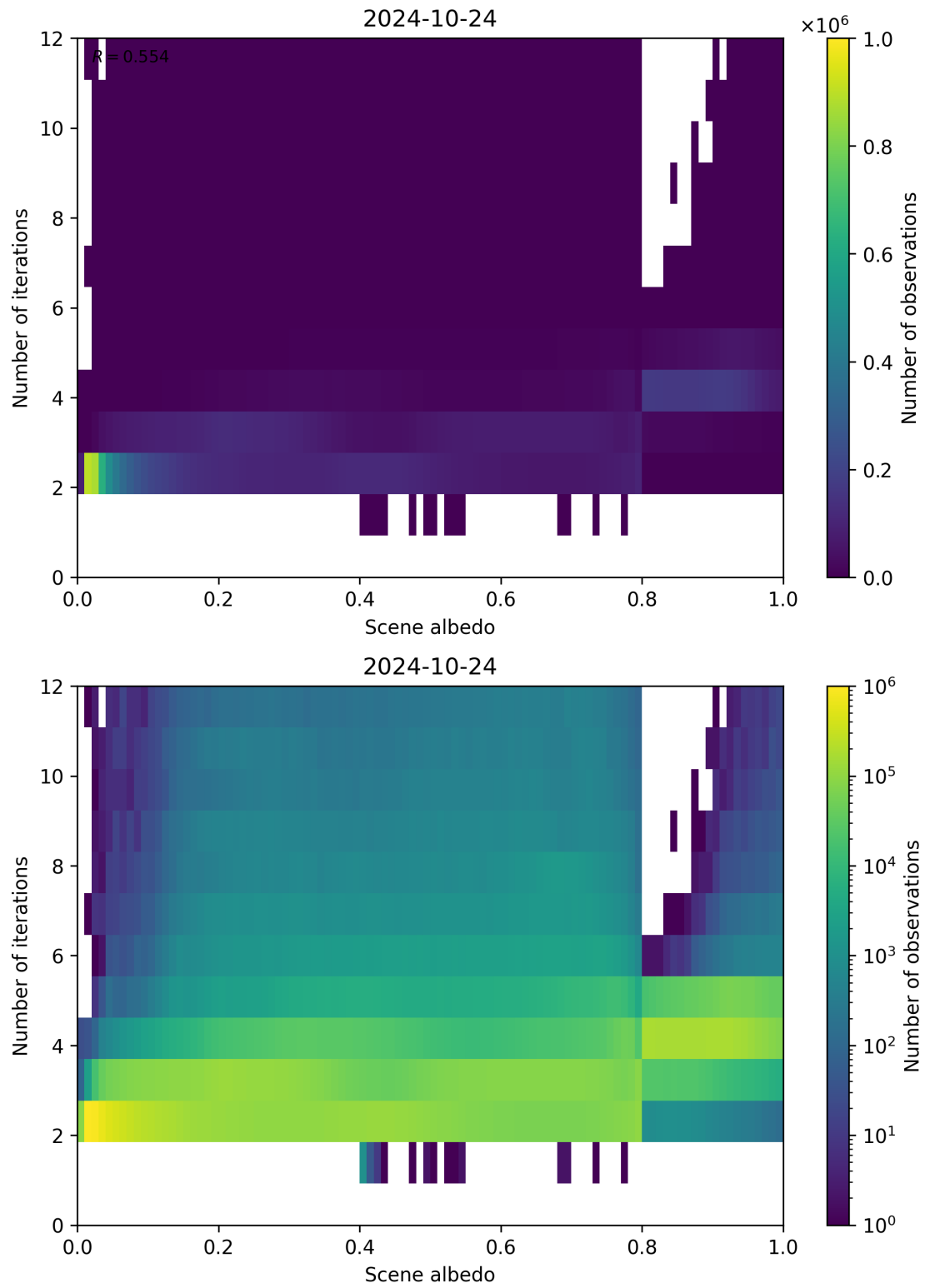
Figure 115: Scatter density plot of “Scene albedo” against “Number of iterations” for 2024-10-24 to 2024-10-25.
