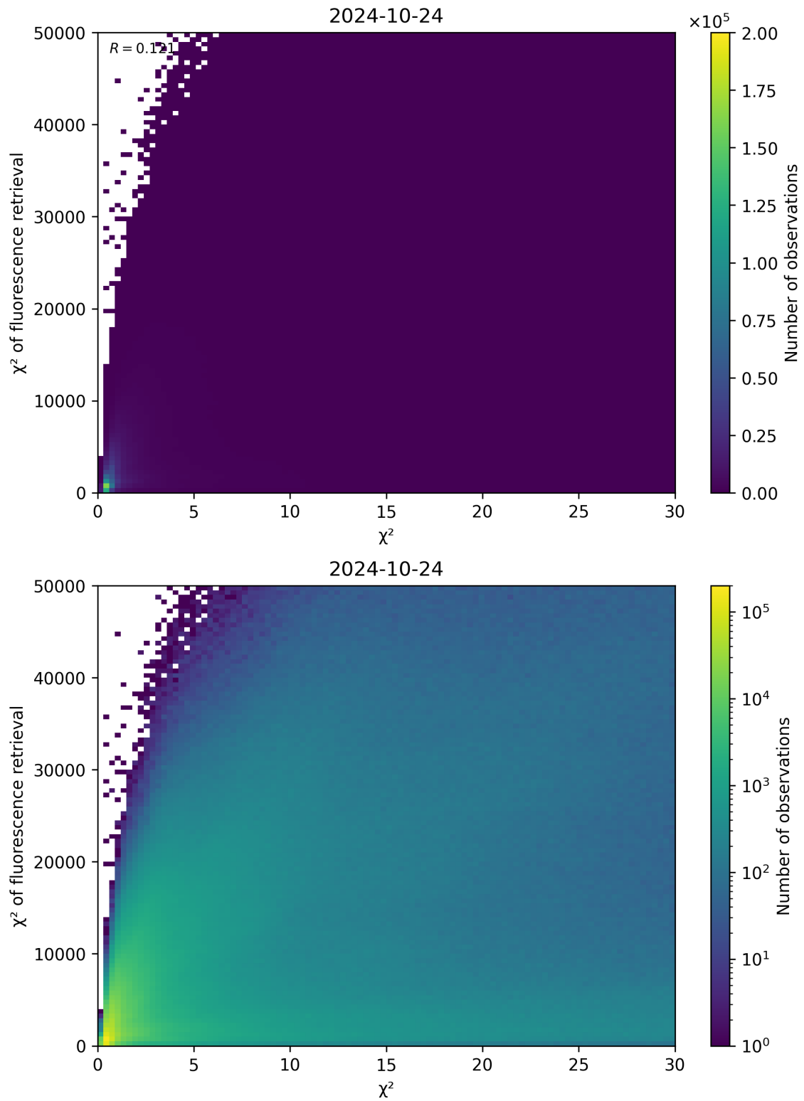
Figure 69: Scatter density plot of “ \chi^2 ” against “ \chi^2 of fluorescence retrieval” for 2024-10-24 to 2024-10-25.
