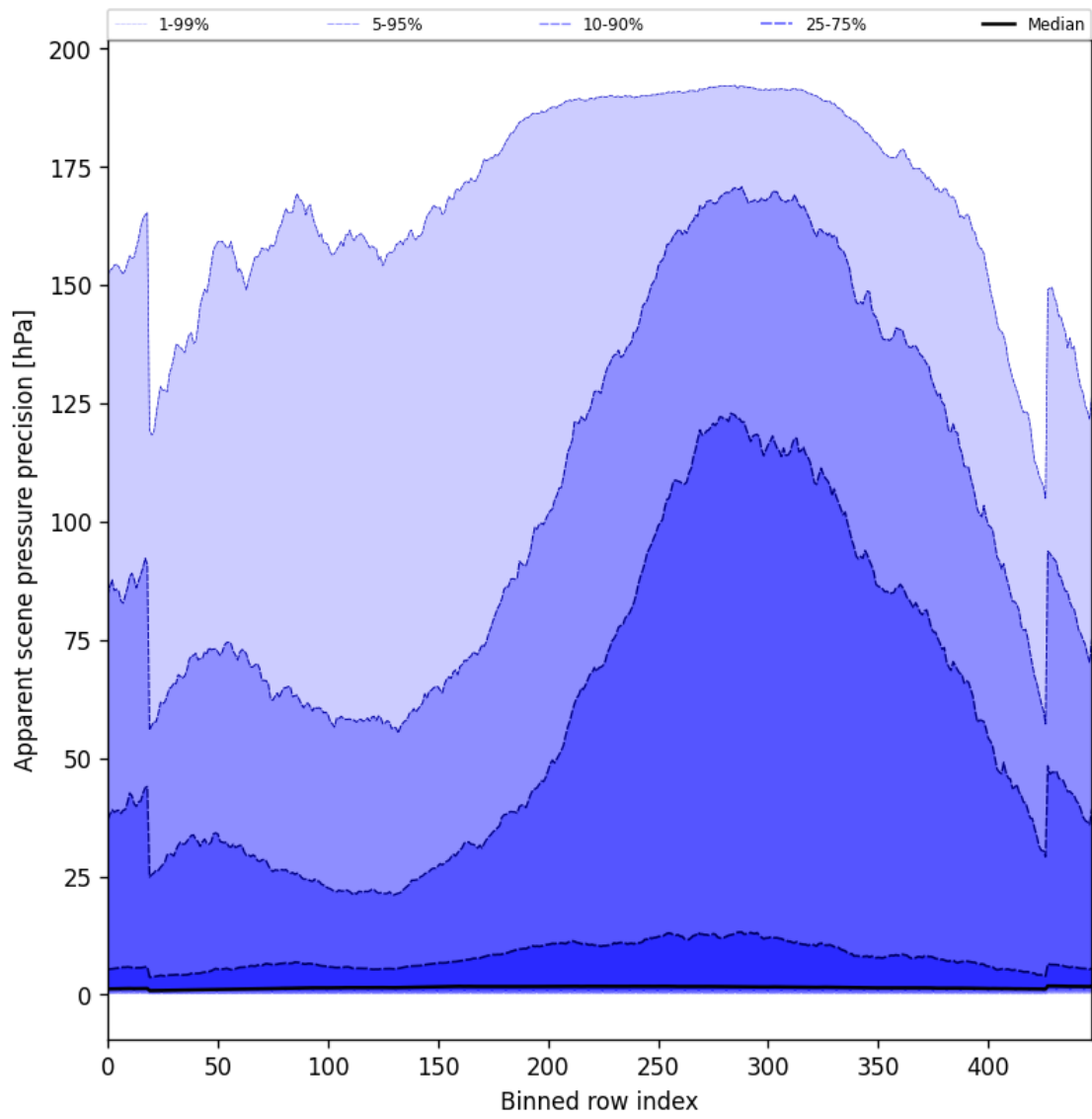
Figure 54: Along track statistics of “Apparent scene pressure precision” for 2024-10-24 to 2024-10-25
