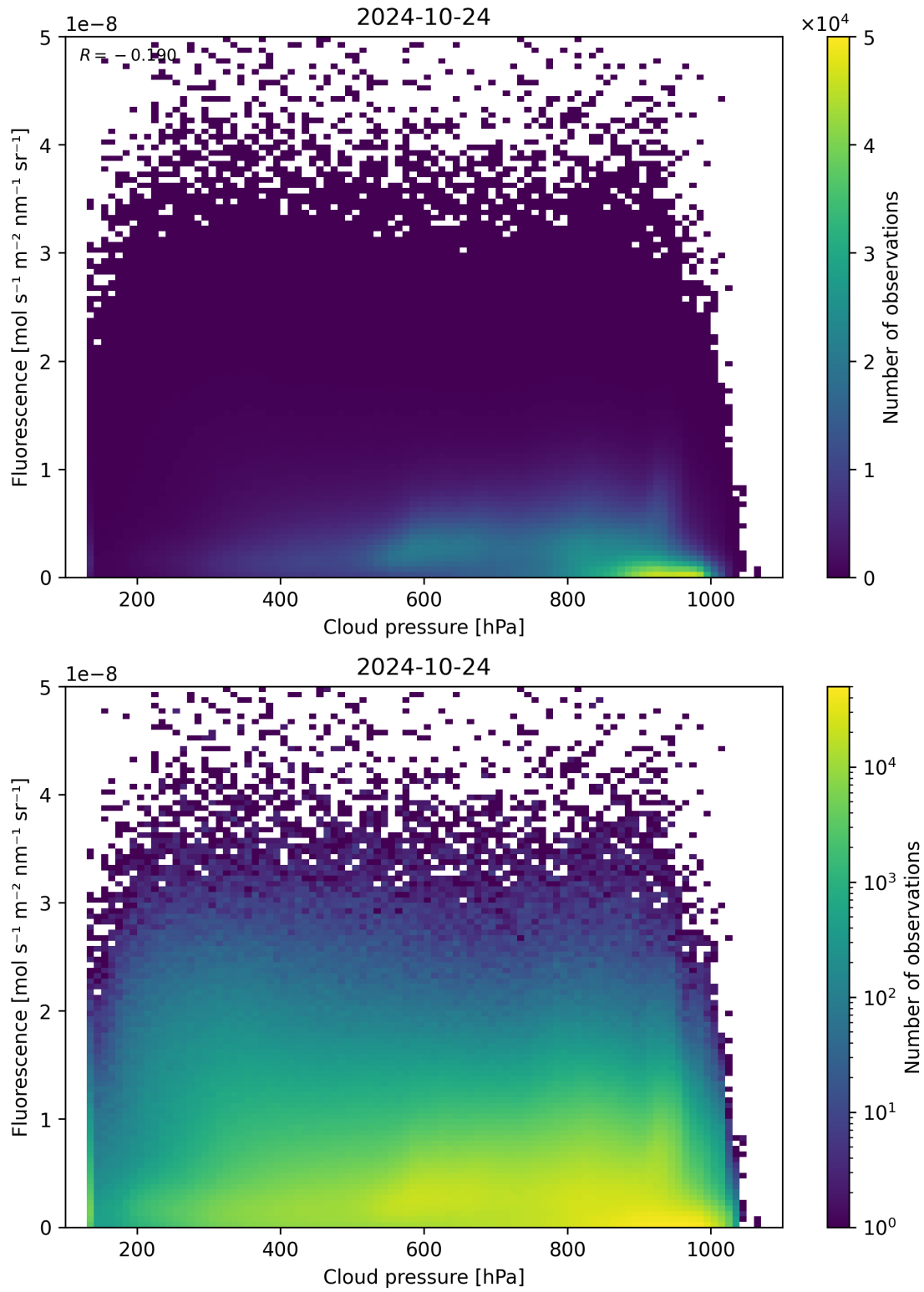
Figure 88: Scatter density plot of “Cloud pressure” against “Fluorescence” for 2024-10-24 to 2024-10-25.
