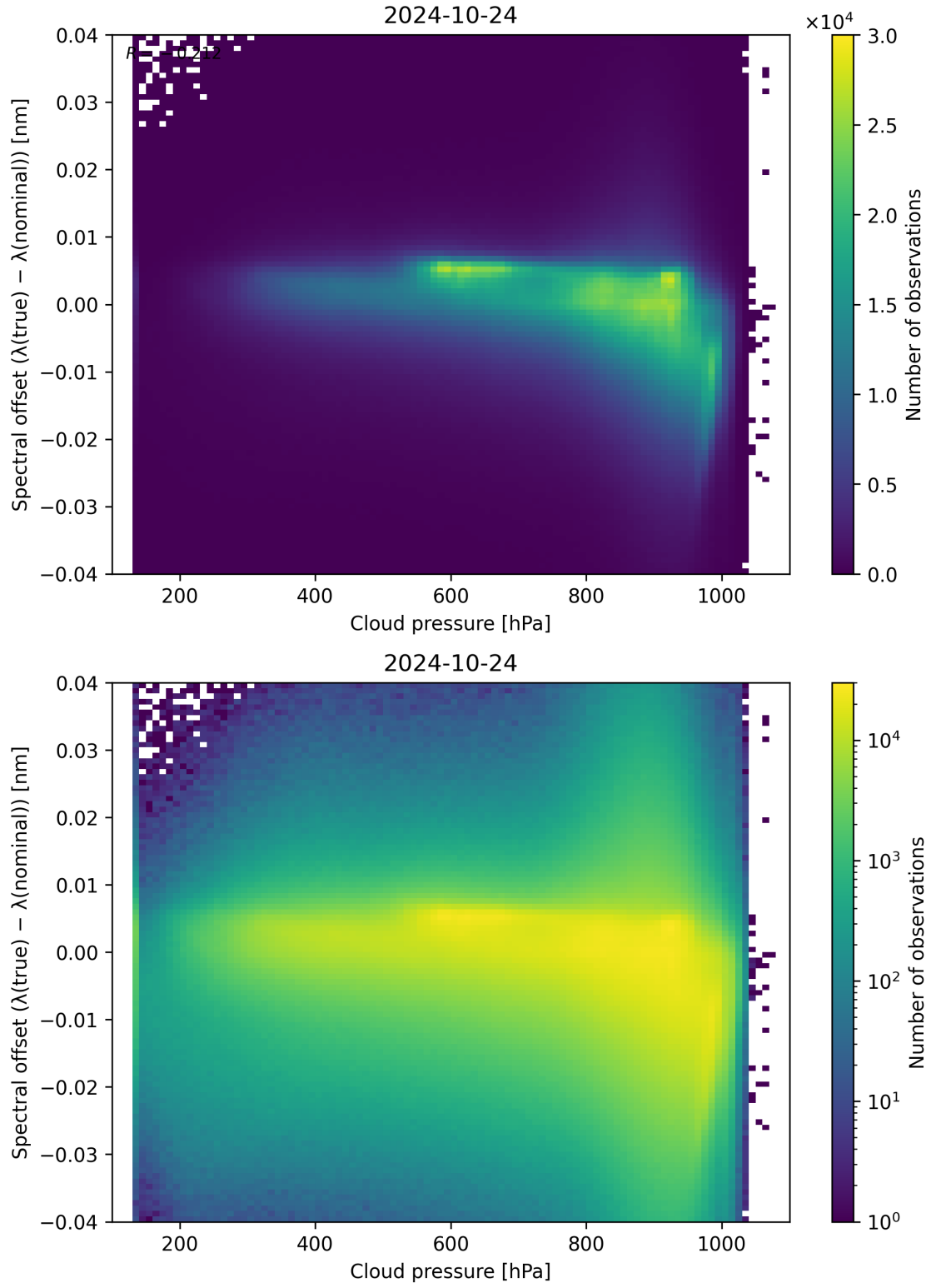
Figure 92: Scatter density plot of “Cloud pressure” against “Spectral offset ( \lambda_{\text{true}} - \lambda_{\text{nominal}} )” for 2024-10-24 to 2024-10-25.
