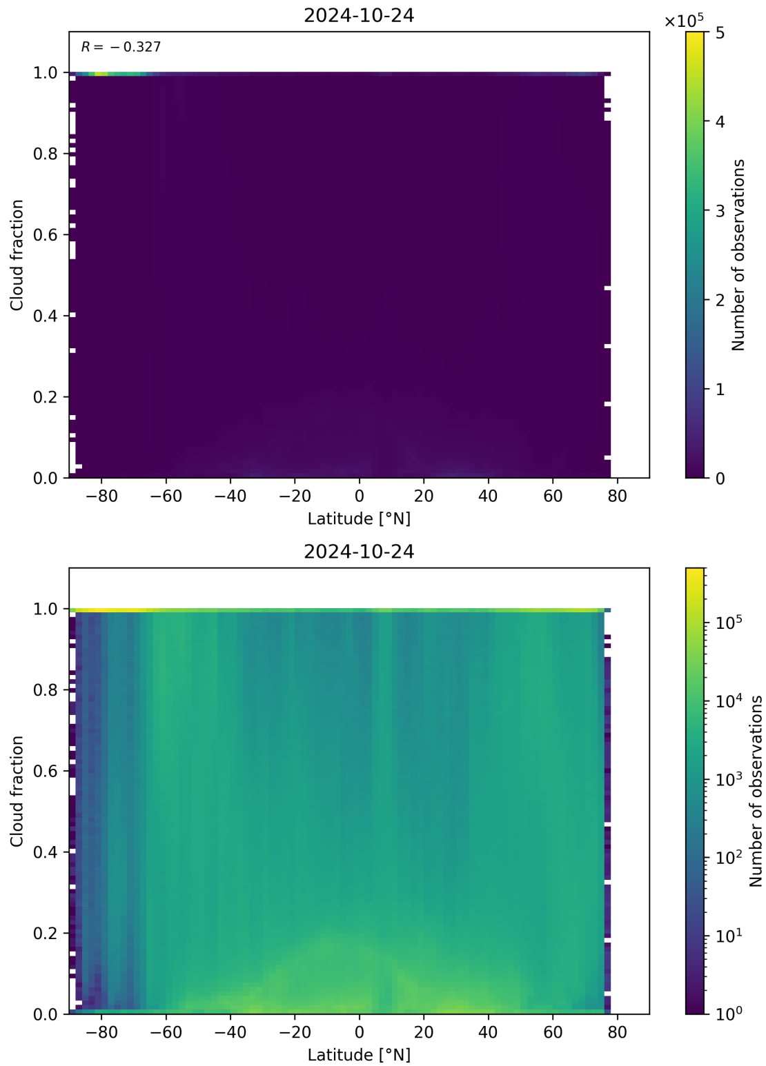
Figure 99: Scatter density plot of “Latitude” against “Cloud fraction” for 2024-10-24 to 2024-10-25.
