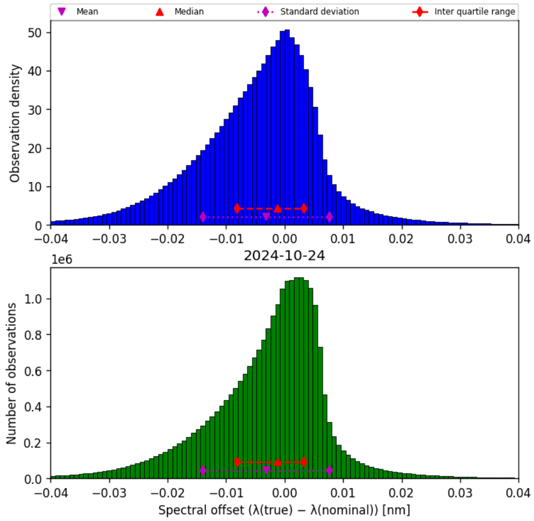
Figure 45: Histogram of “Spectral offset ( \lambda_{\text{true}} - \lambda_{\text{nominal}} )” for 2024-10-24 to 2024-10-25
