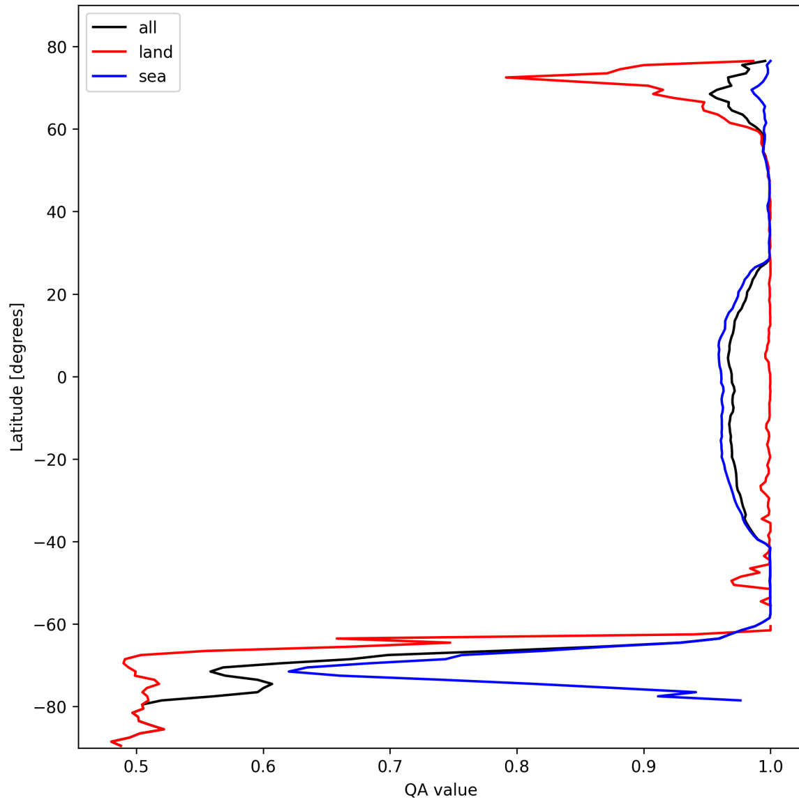
Figure 12: Zonal average of “QA value” for 2024-10-24 to 2024-10-25.
