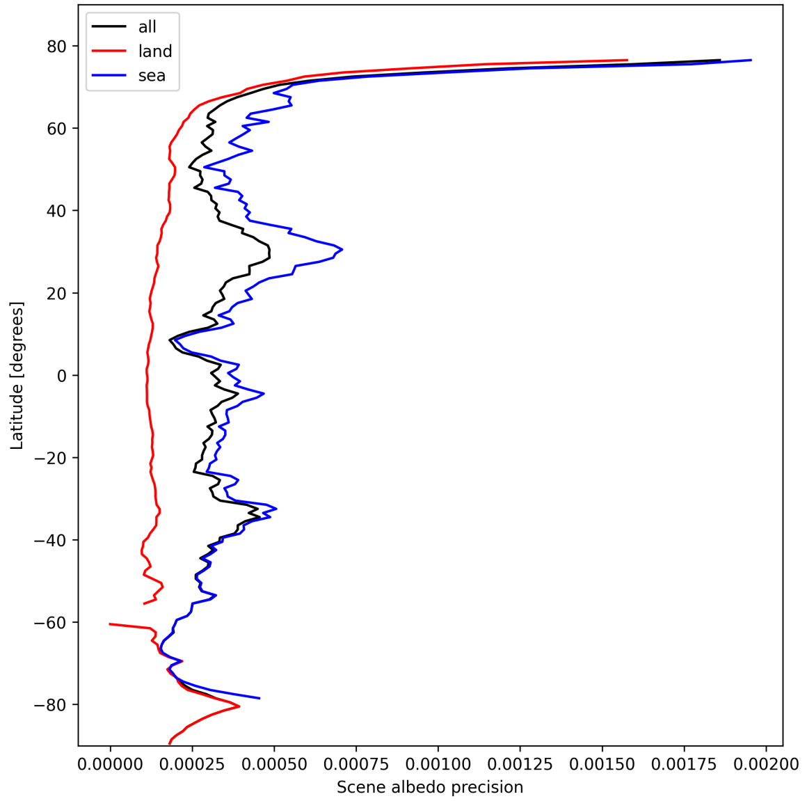
Figure 18: Zonal average of "Scene albedo precision" for 2024-10-24 to 2024-10-25.
