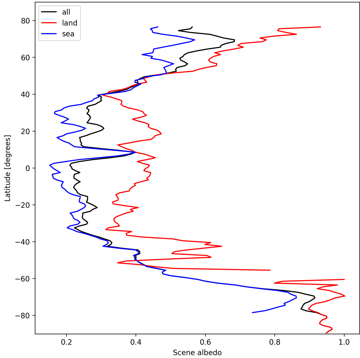
Figure 17: Zonal average of “Scene albedo” for 2024-10-24 to 2024-10-25.
