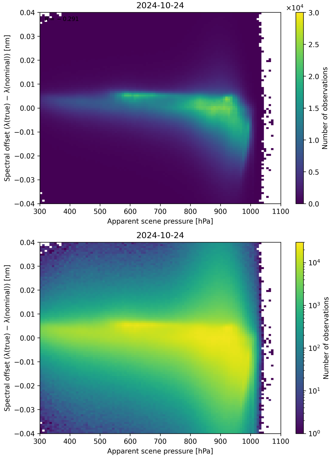
Figure 68: Scatter density plot of “Apparent scene pressure” against “Spectral offset ( \lambda_{\text{true}} - \lambda_{\text{nominal}} )” for 2024-10-24 to 2024-10-25.
