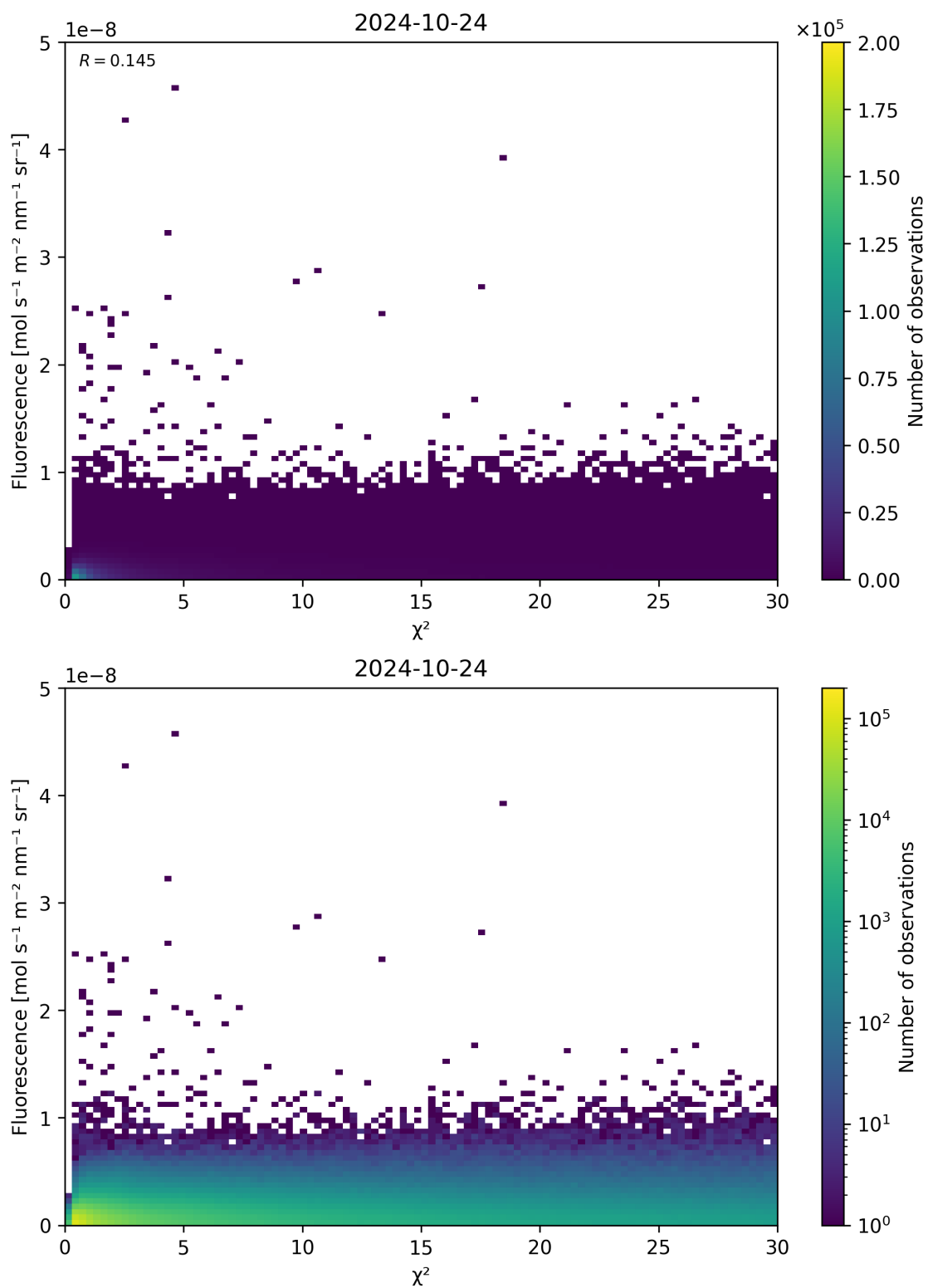
Figure 70: Scatter density plot of “ \chi^2 ” against “Fluorescence” for 2024-10-24 to 2024-10-25.
