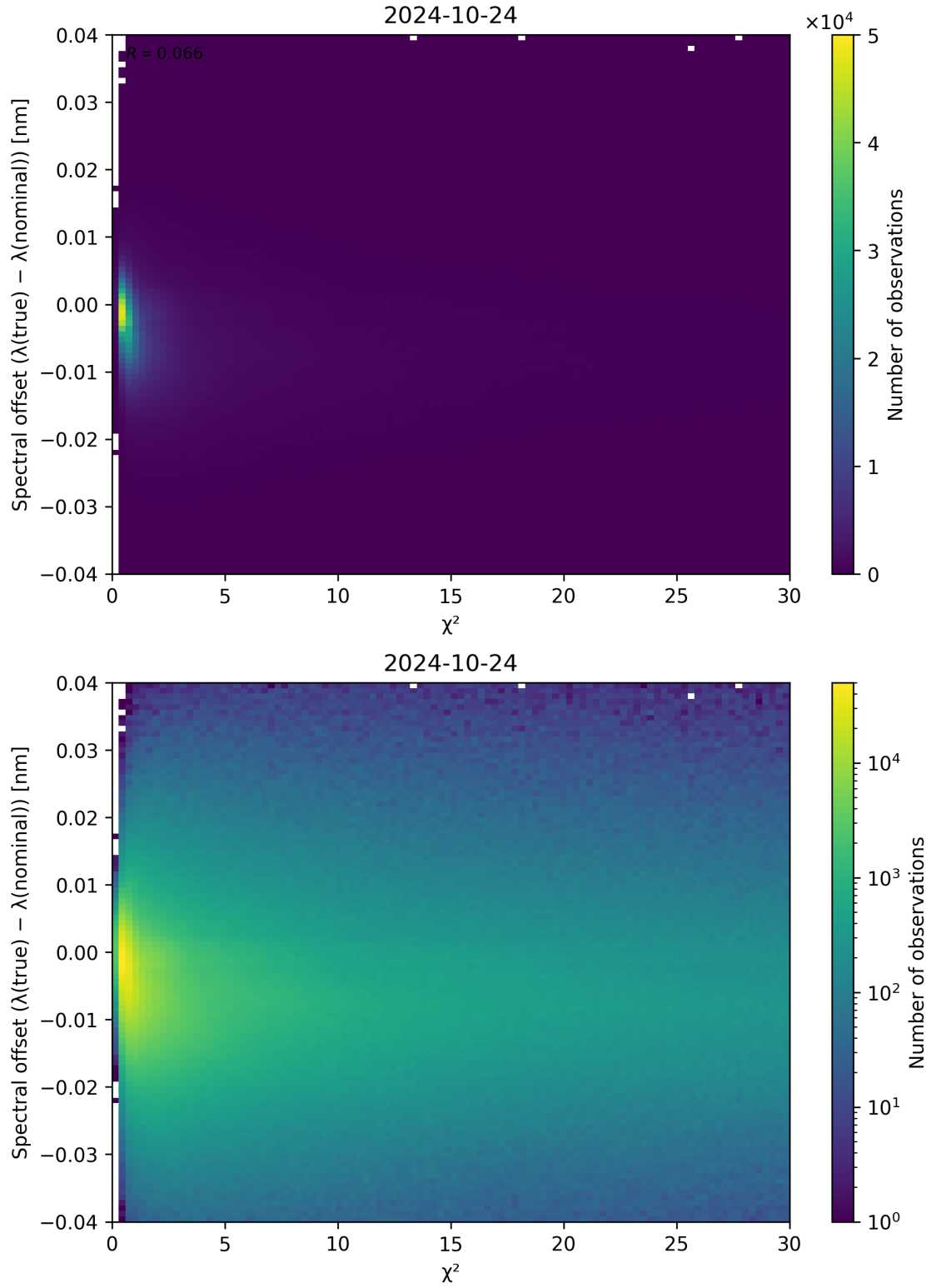
Figure 75: Scatter density plot of “ \chi^2 ” against “Spectral offset ( \lambda_{\text{true}} - \lambda_{\text{nominal}} )” for 2024-10-24 to 2024-10-25.
