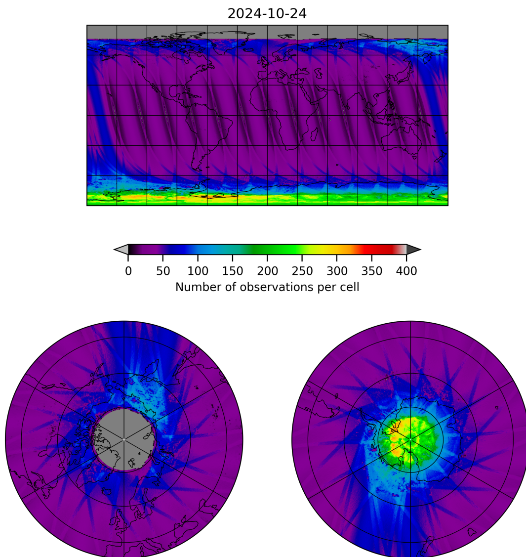
Figure 11: Map of the number of observations for 2024-10-24 to 2024-10-25
