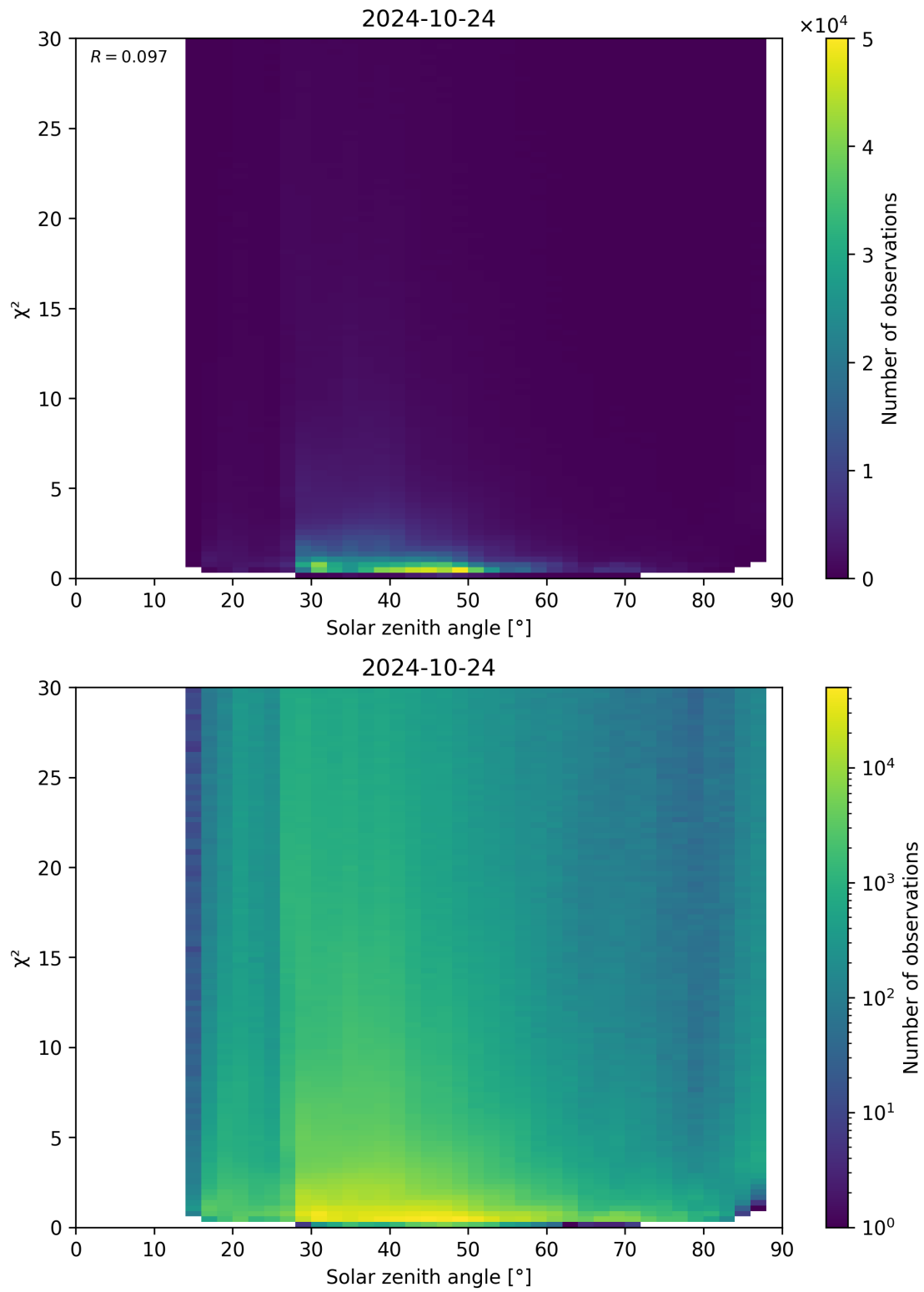
Figure 119: Scatter density plot of “Solar zenith angle” against “ \chi^2 ” for 2024-10-24 to 2024-10-25.
