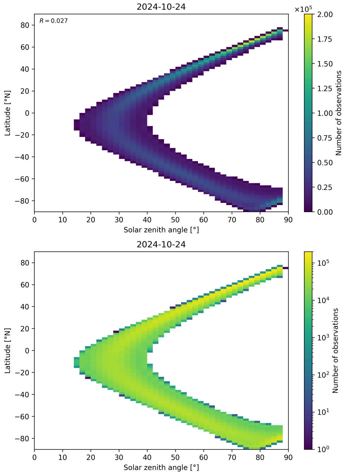
Figure 124: Scatter density plot of “Solar zenith angle” against “Latitude” for 2024-10-24 to 2024-10-25.
