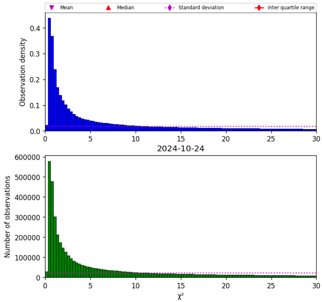
Figure 38: Histogram of “ \chi^2 ” for 2024-10-24 to 2024-10-25
