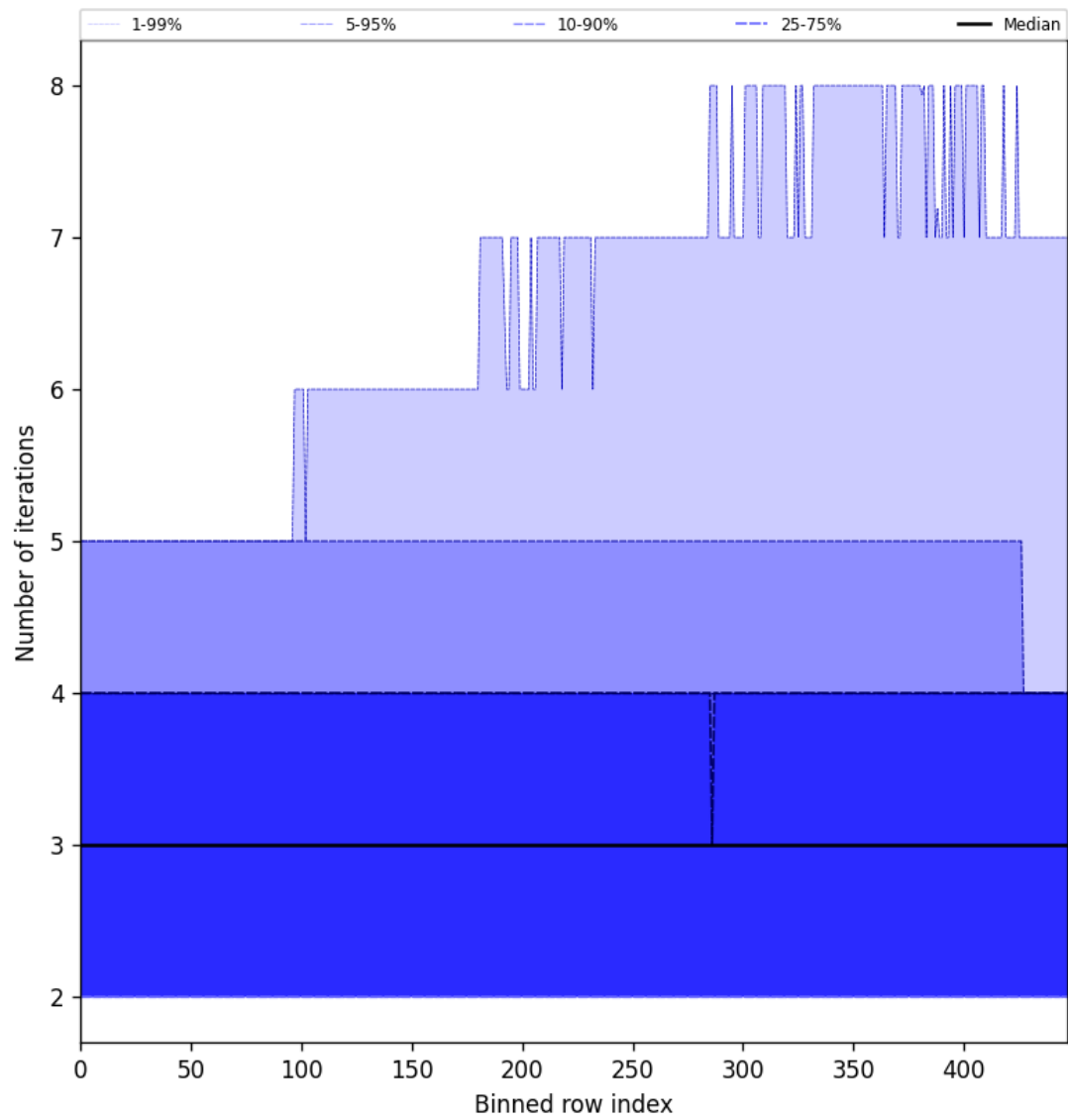
Figure 56: Along track statistics of “Number of iterations” for 2024-10-24 to 2024-10-25
