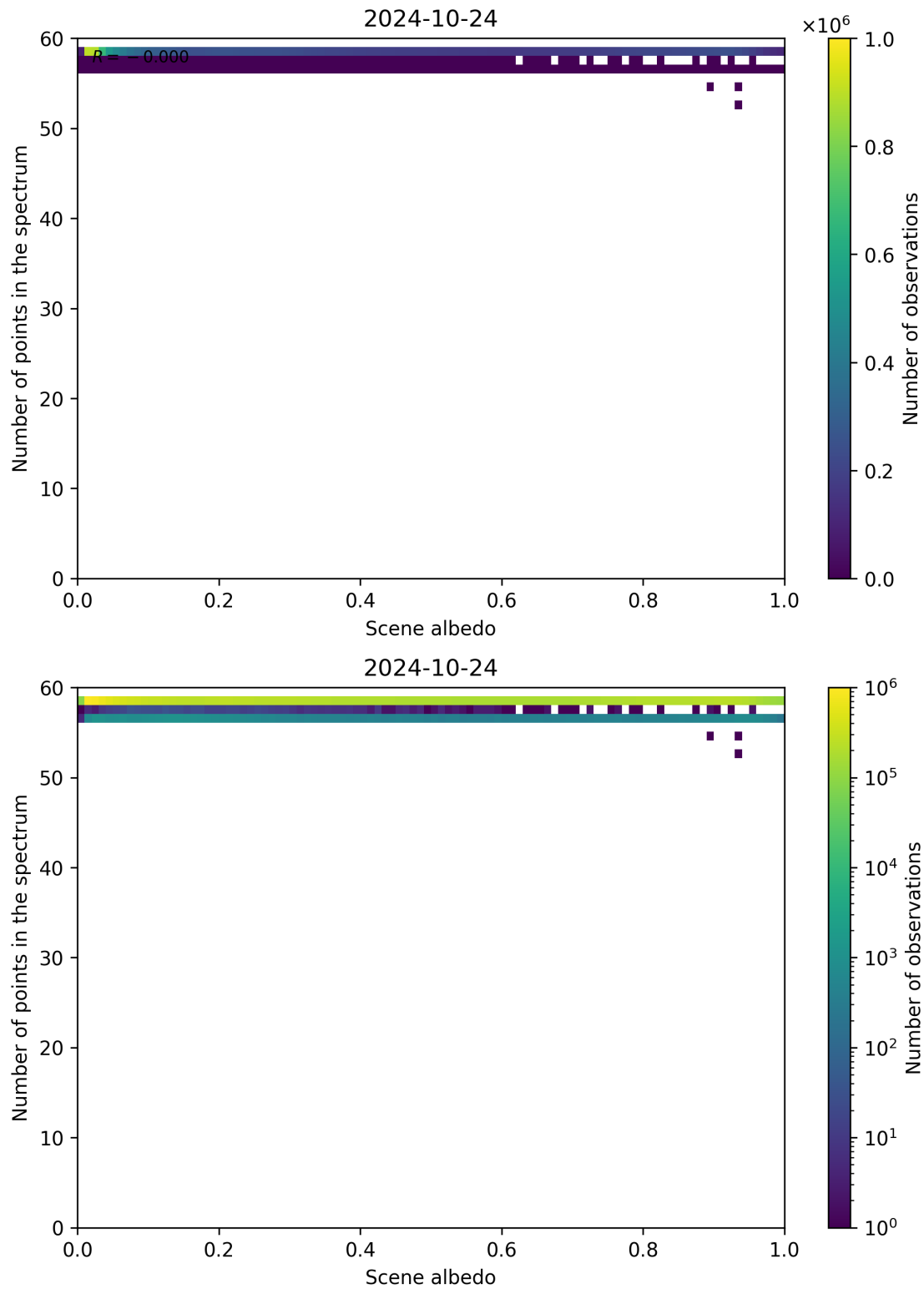
Figure 116: Scatter density plot of “Scene albedo” against “Number of points in the spectrum” for 2024-10-24 to 2024-10-25.
