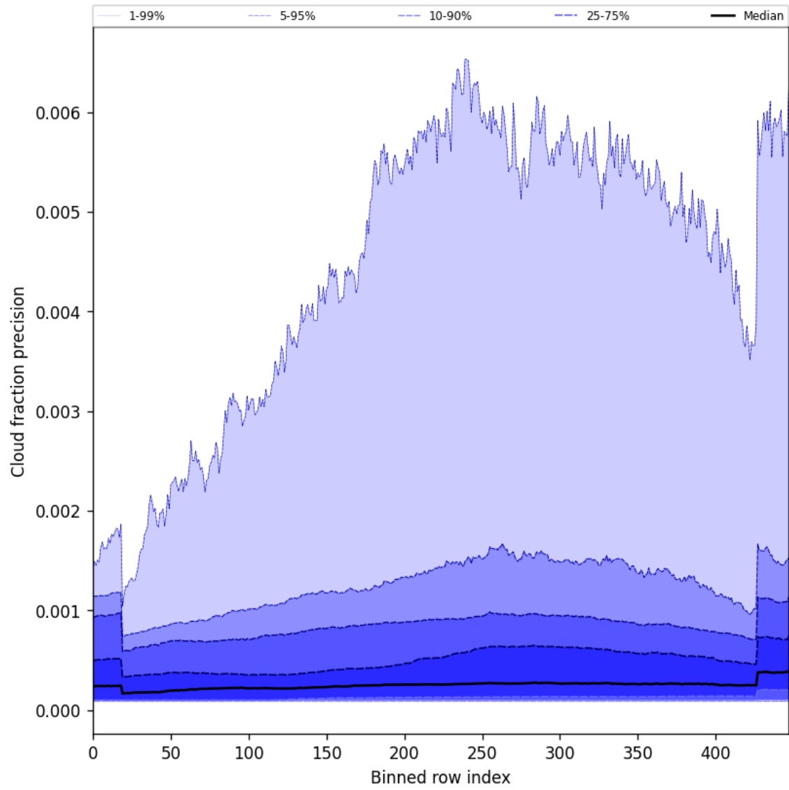
Figure 50: Along track statistics of “Cloud fraction precision” for 2024-10-24 to 2024-10-25
