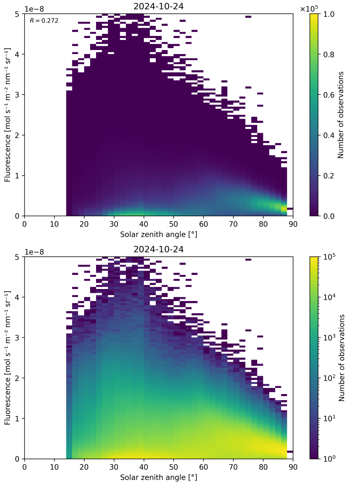
Figure 123: Scatter density plot of “Solar zenith angle” against “Fluorescence” for 2024-10-24 to 2024-10-25.
