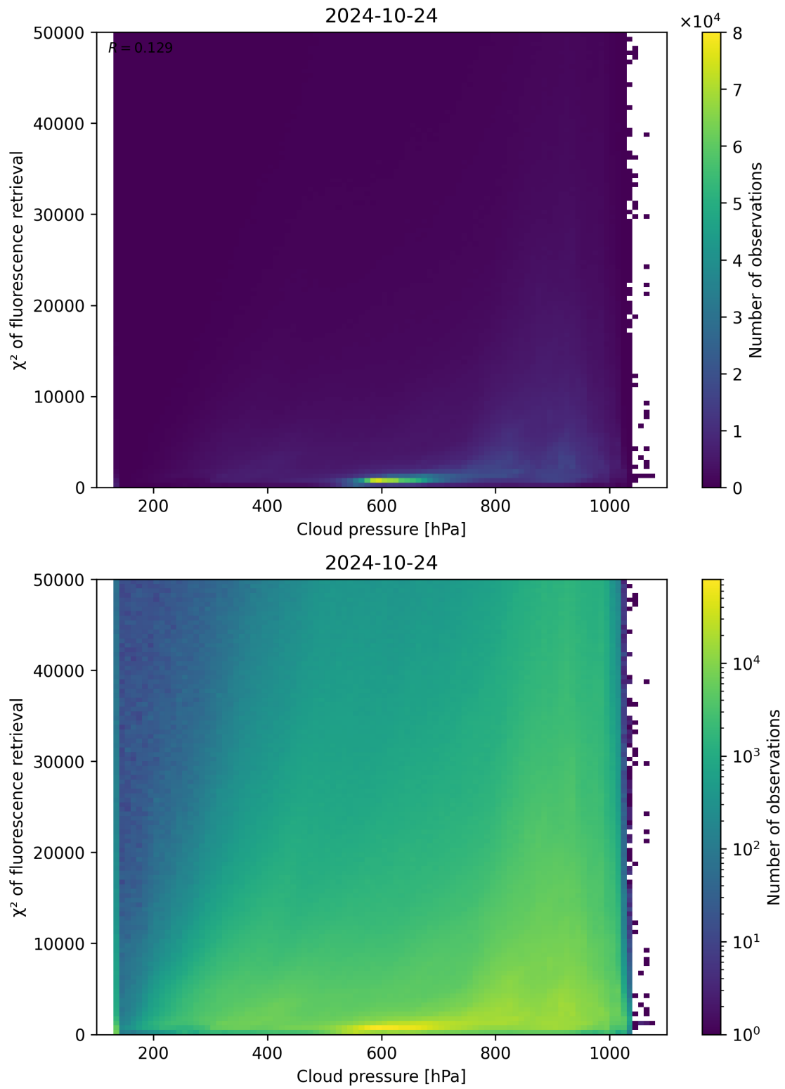
Figure 86: Scatter density plot of “Cloud pressure” against “ \chi^2 of fluorescence retrieval” for 2024-10-24 to 2024-10-25.
