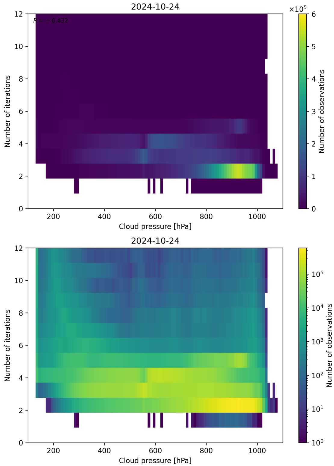
Figure 89: Scatter density plot of “Cloud pressure” against “Number of iterations” for 2024-10-24 to 2024-10-25.
