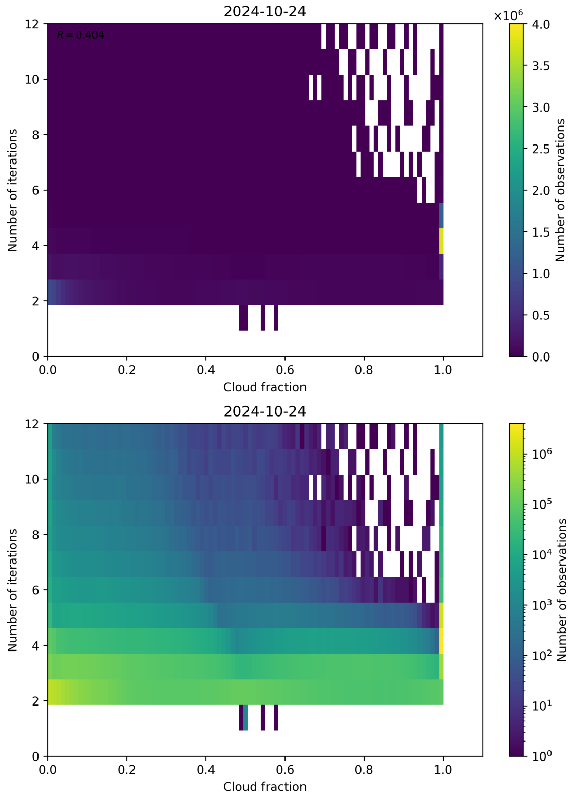
Figure 80: Scatter density plot of “Cloud fraction” against “Number of iterations” for 2024-10-24 to 2024-10-25.
