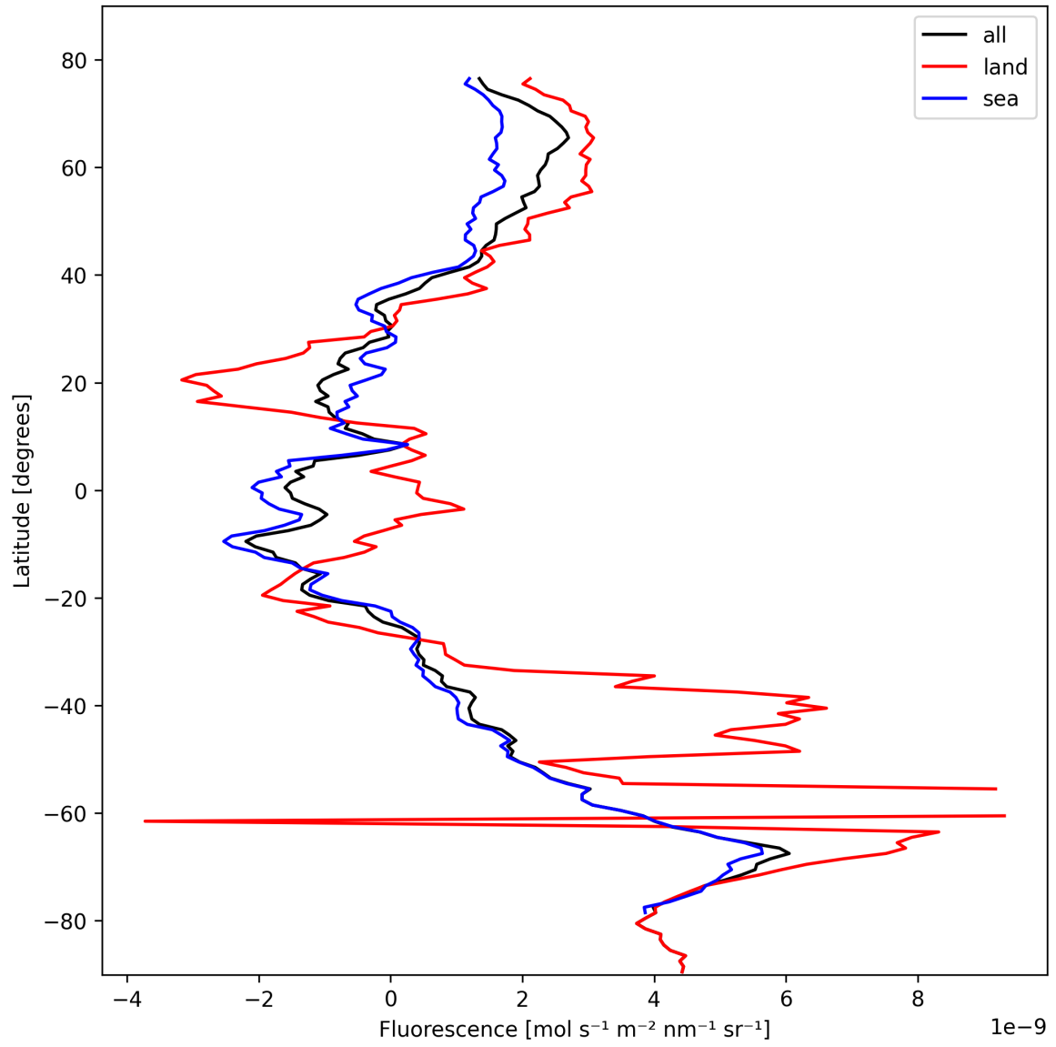
Figure 23: Zonal average of “Fluorescence” for 2024-10-24 to 2024-10-25.
