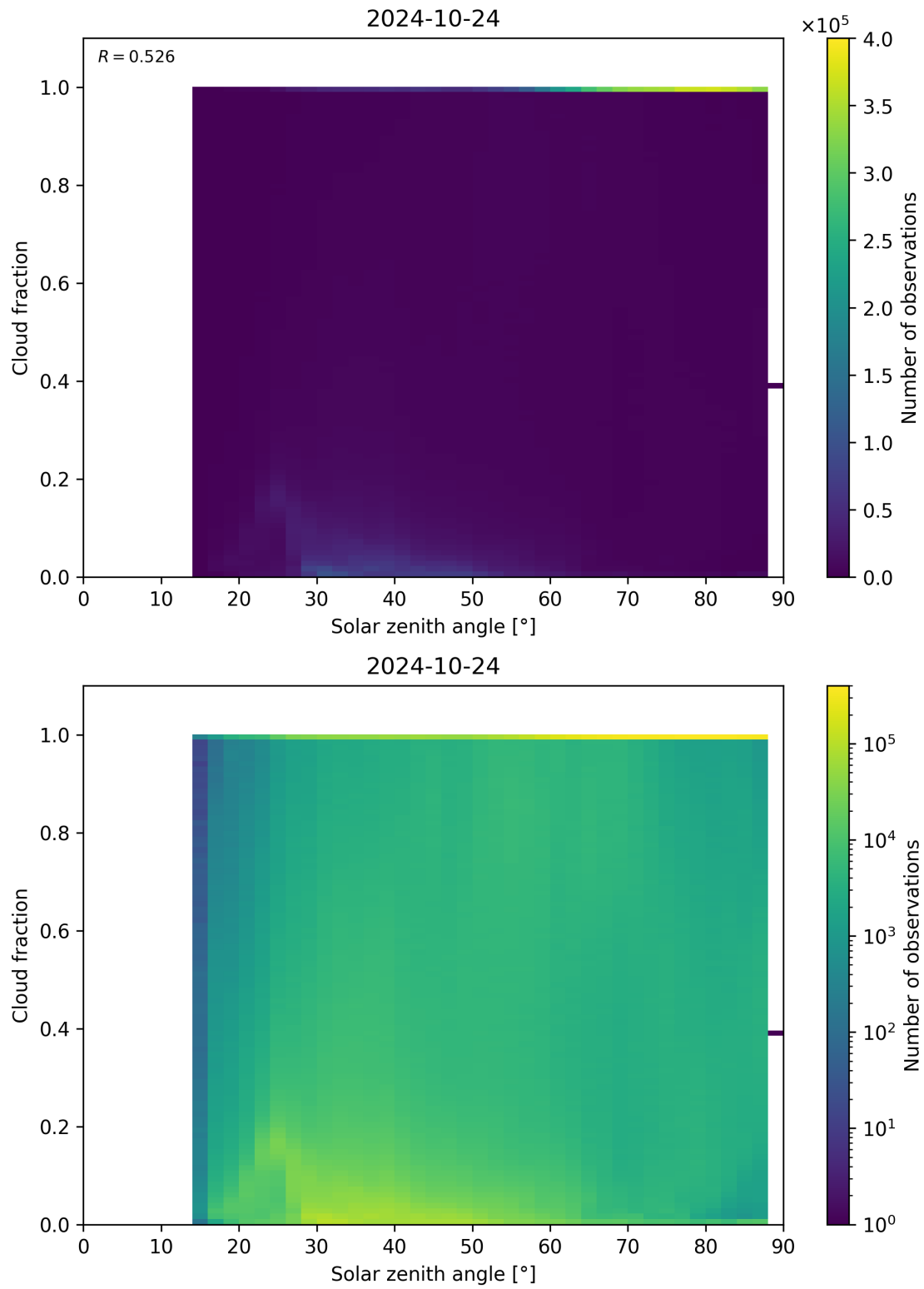
Figure 121: Scatter density plot of “Solar zenith angle” against “Cloud fraction” for 2024-10-24 to 2024-10-25.
