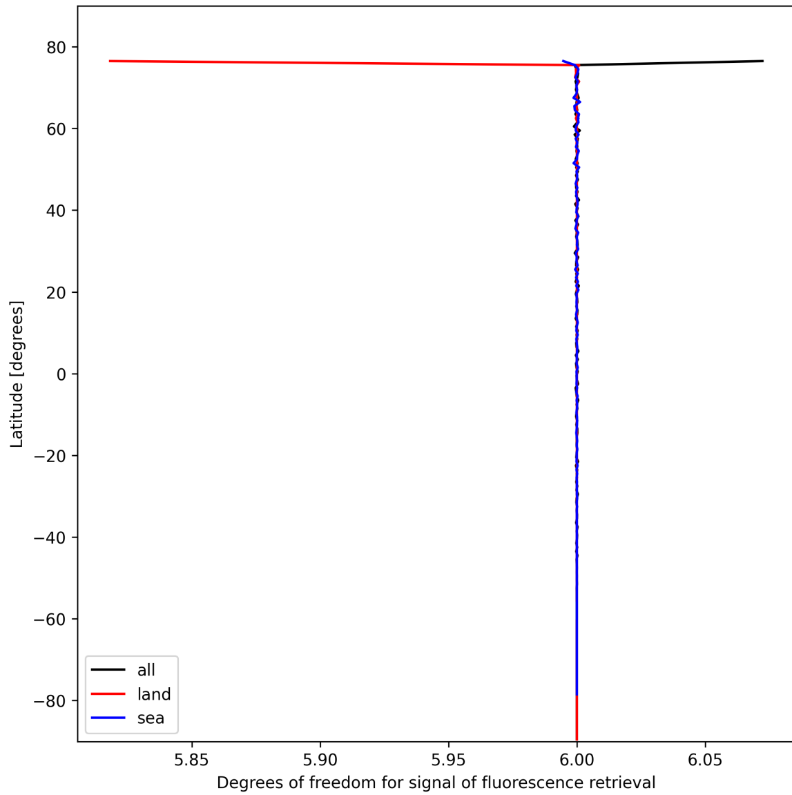
Figure 26: Zonal average of “Degrees of freedom for signal of fluorescence retrieval” for 2024-10-24 to 2024-10-25.
