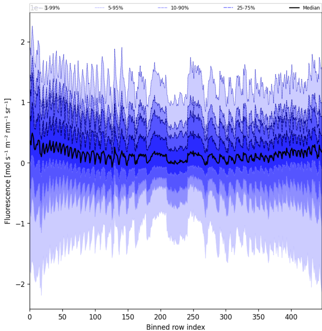
Figure 57: Along track statistics of “Fluorescence” for 2024-10-24 to 2024-10-25
