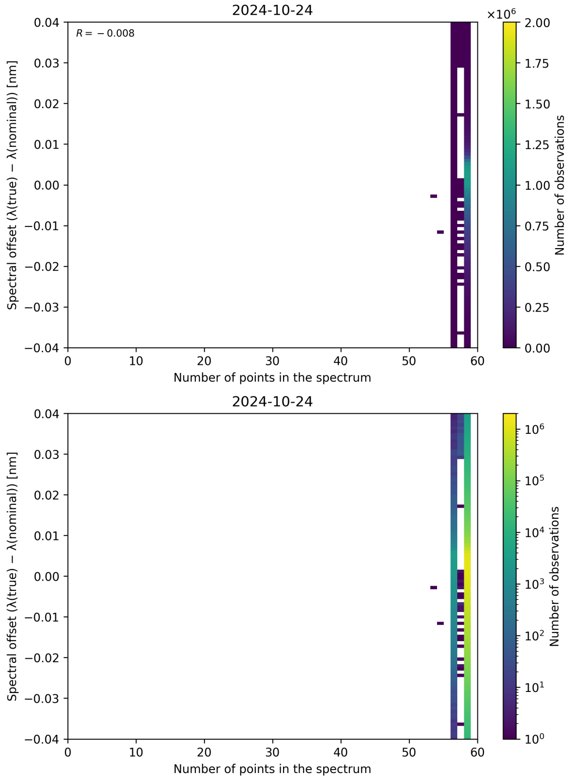
Figure 110: Scatter density plot of “Number of points in the spectrum” against “Spectral offset ( \lambda_{\text{true}} - \lambda_{\text{nominal}} )” for 2024-10-24 to 2024-10-25.
