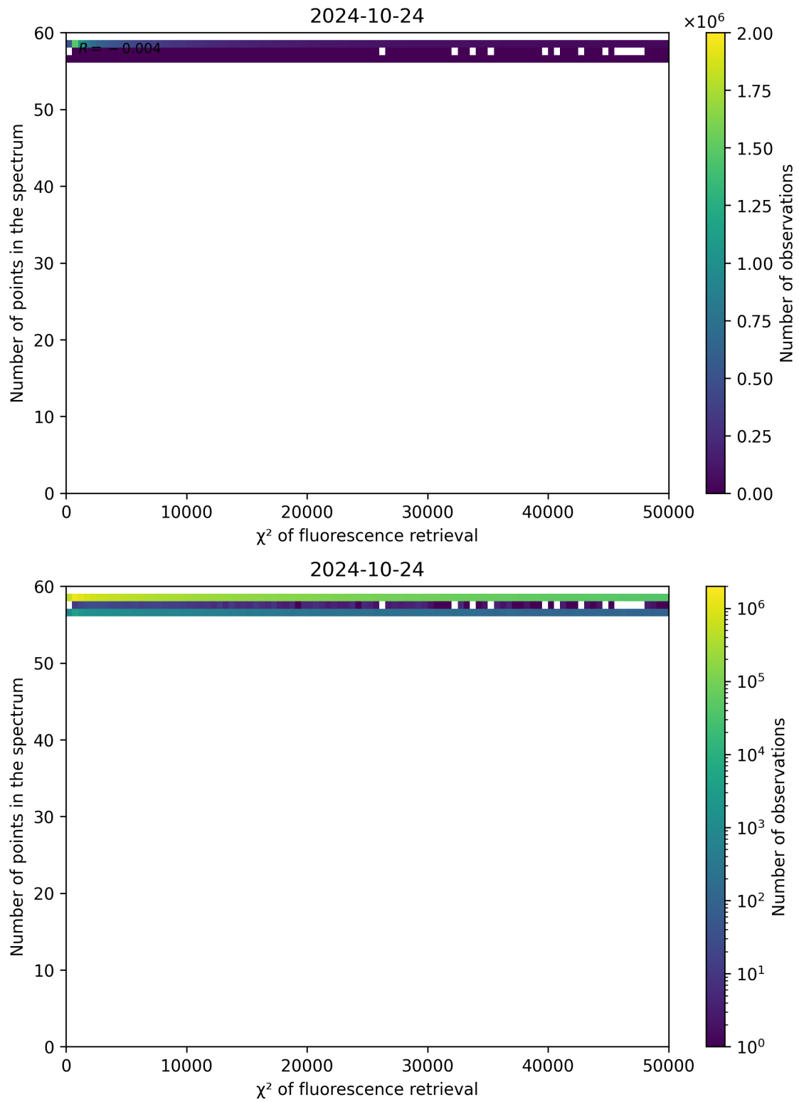
Figure 71: Scatter density plot of " \chi^2 of fluorescence retrieval" against "Number of points in the spectrum" for 2024-10-24 to 2024-10-25.
