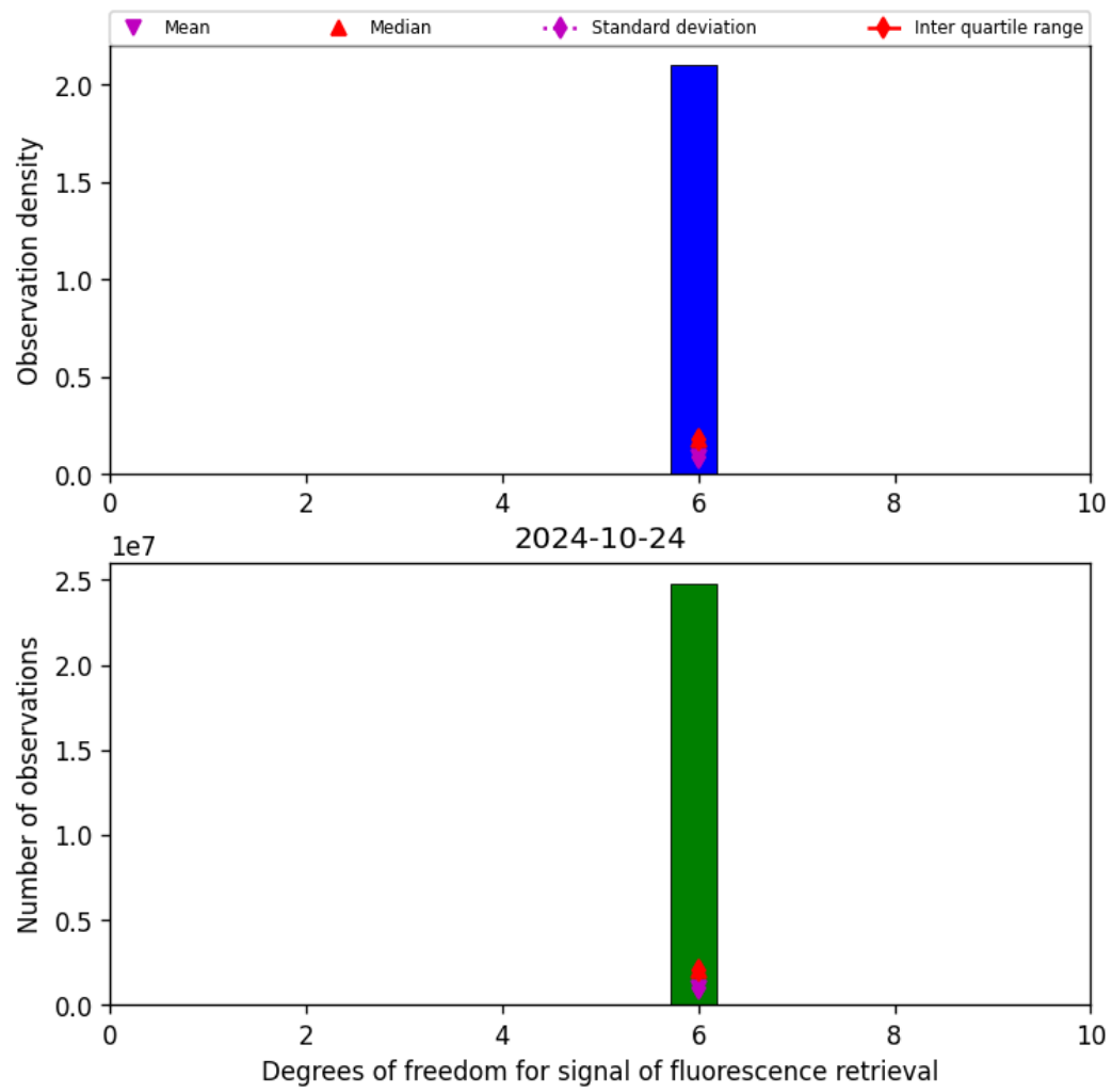
Figure 43: Histogram of “Degrees of freedom for signal of fluorescence retrieval” for 2024-10-24 to 2024-10-25
