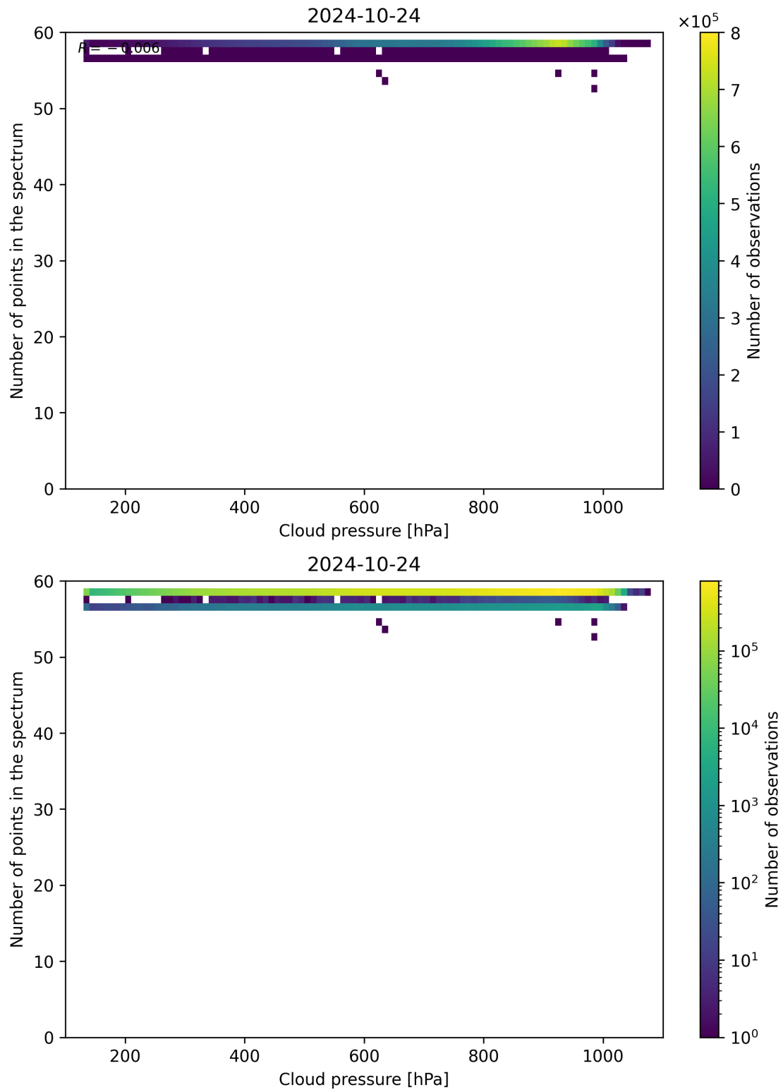
Figure 90: Scatter density plot of “Cloud pressure” against “Number of points in the spectrum” for 2024-10-24 to 2024-10-25.
