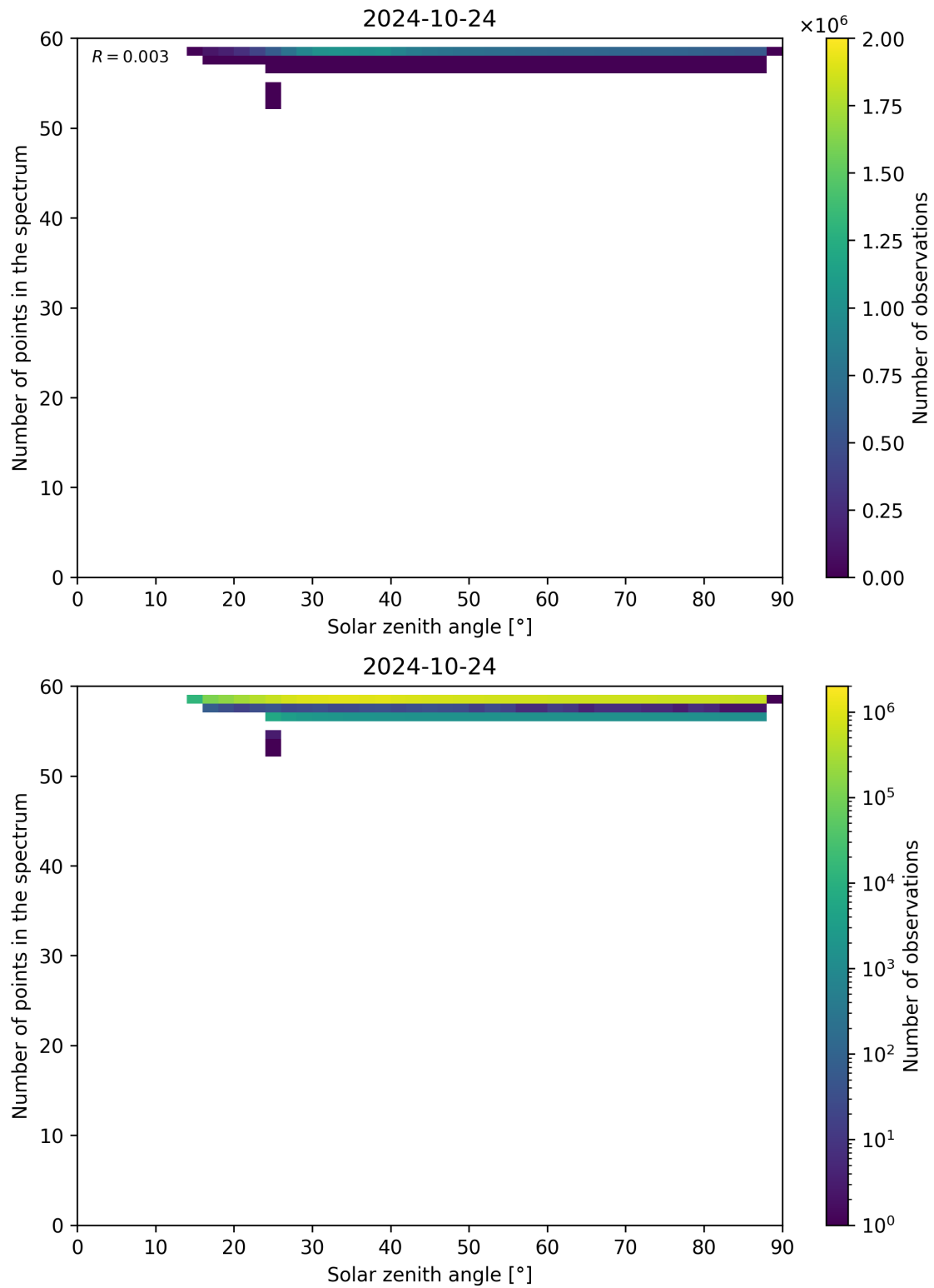
Figure 126: Scatter density plot of “Solar zenith angle” against “Number of points in the spectrum” for 2024-10-24 to 2024-10-25.
