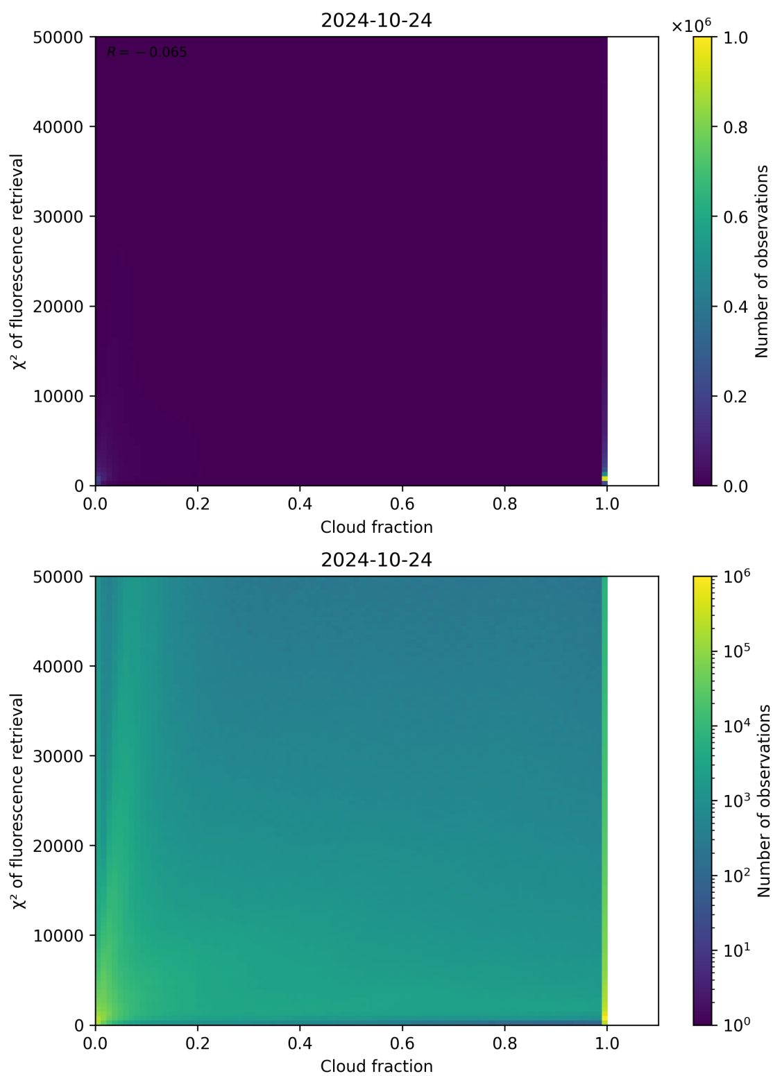
Figure 78: Scatter density plot of “Cloud fraction” against “ \chi^2 of fluorescence retrieval” for 2024-10-24 to 2024-10-25.
