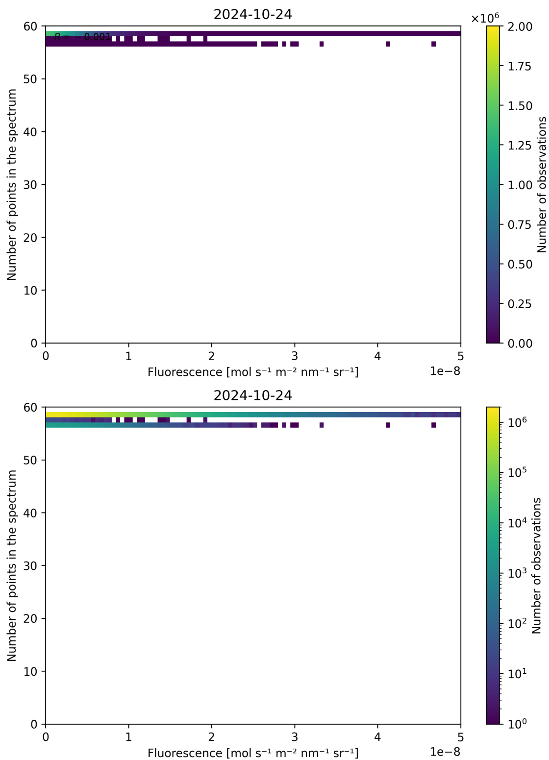
Figure 94: Scatter density plot of “Fluorescence” against “Number of points in the spectrum” for 2024-10-24 to 2024-10-25.
