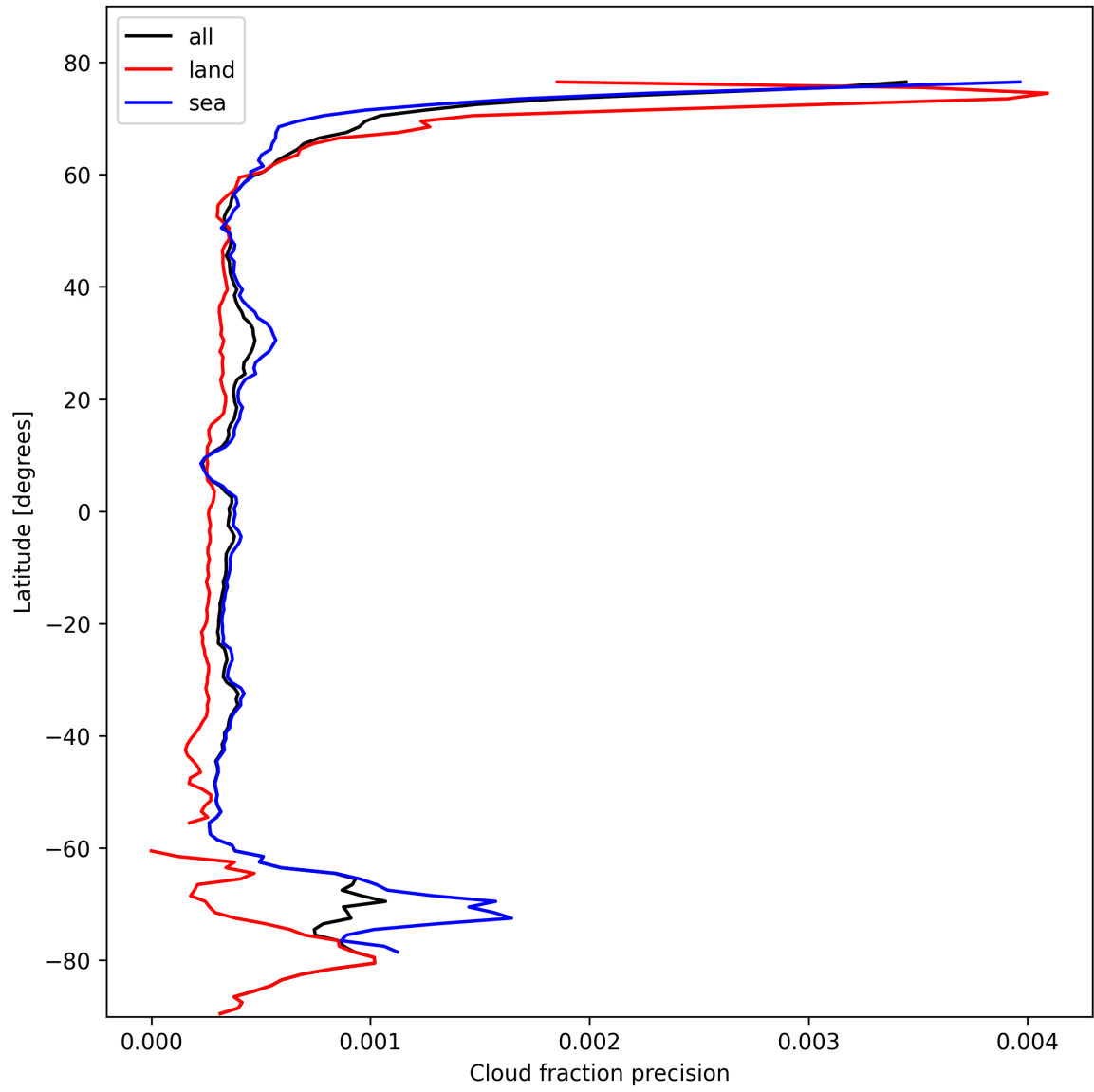
Figure 16: Zonal average of “Cloud fraction precision” for 2024-10-24 to 2024-10-25.
