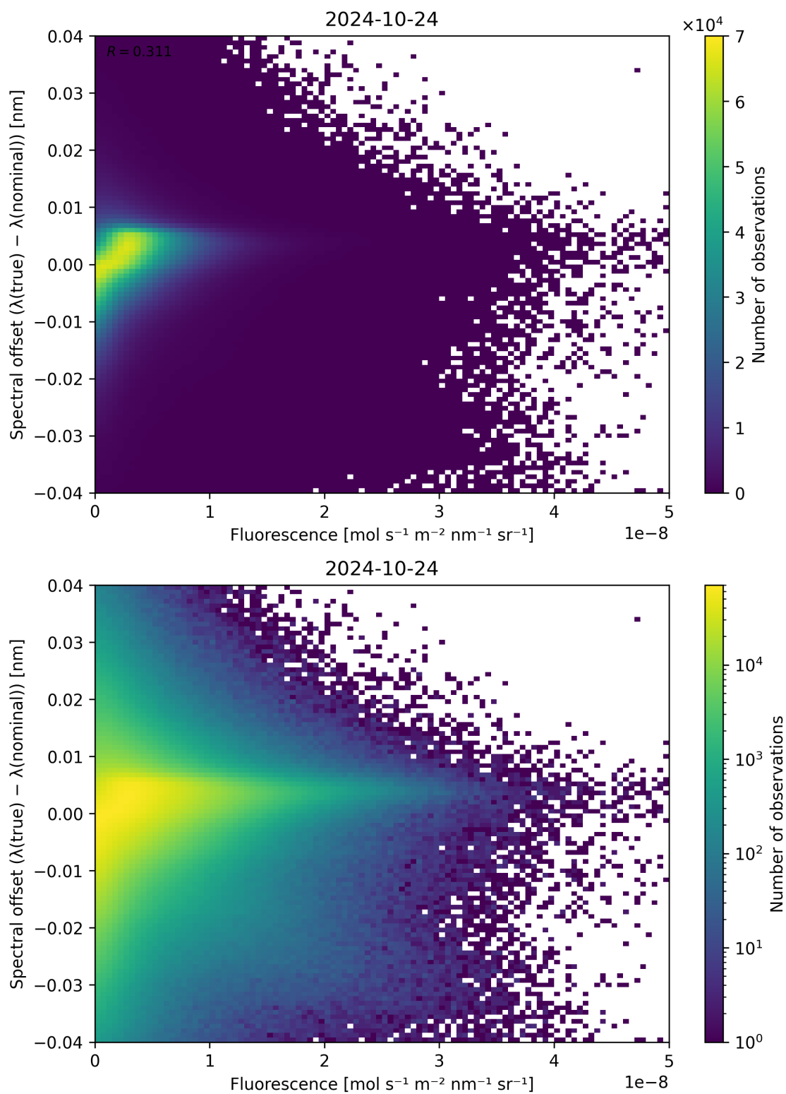
Figure 95: Scatter density plot of “Fluorescence” against “Spectral offset ( \lambda_{\text{true}} - \lambda_{\text{nominal}} )” for 2024-10-24 to 2024-10-25.
