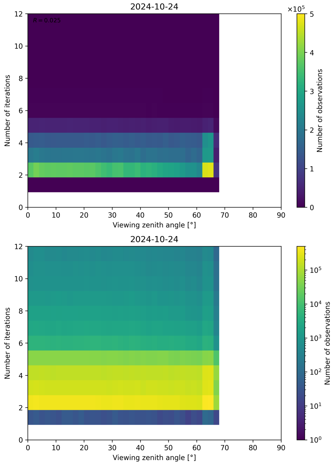
Figure 136: Scatter density plot of “Viewing zenith angle” against “Number of iterations” for 2024-10-24 to 2024-10-25.
