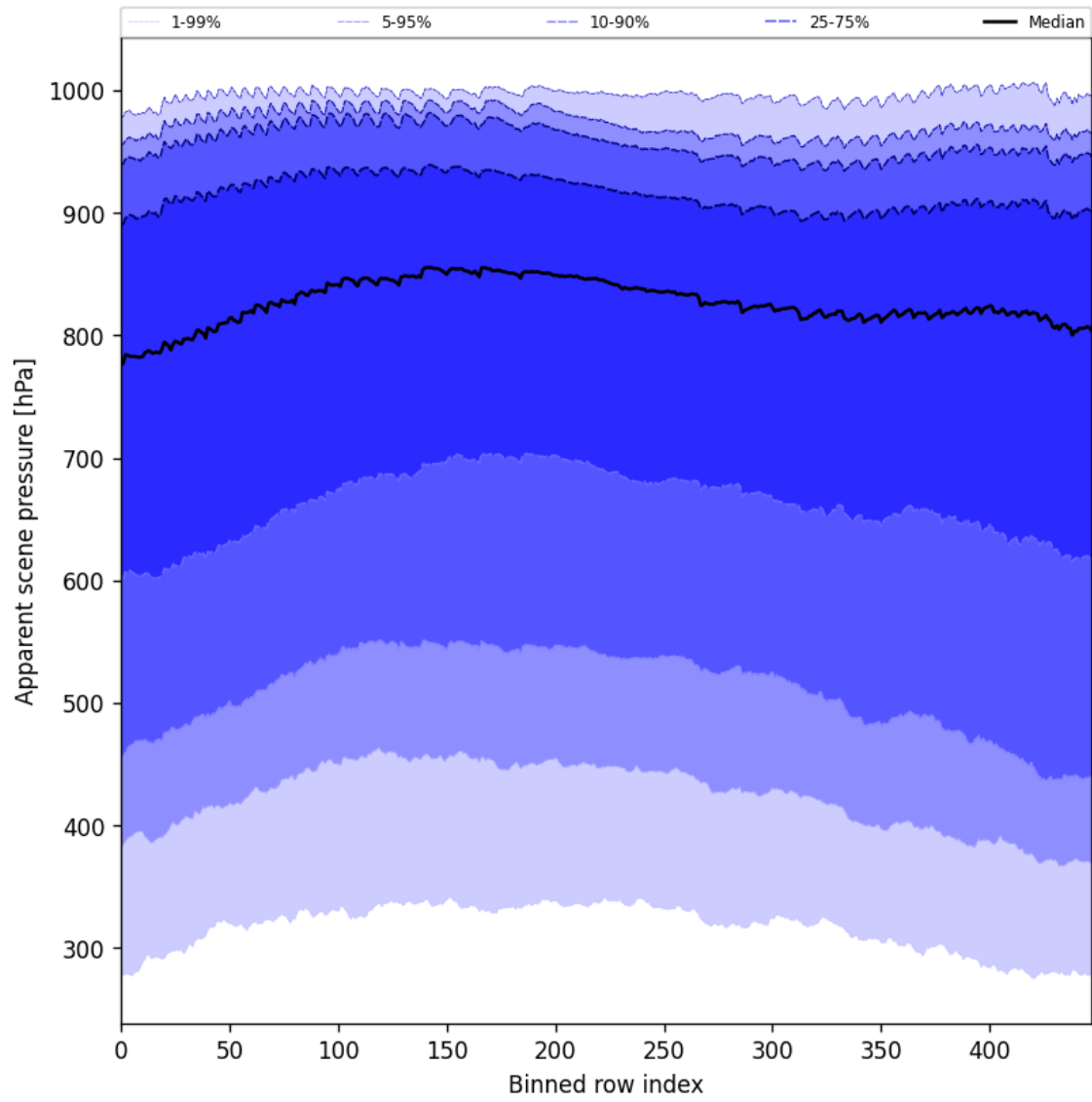
Figure 53: Along track statistics of “Apparent scene pressure” for 2024-10-24 to 2024-10-25
