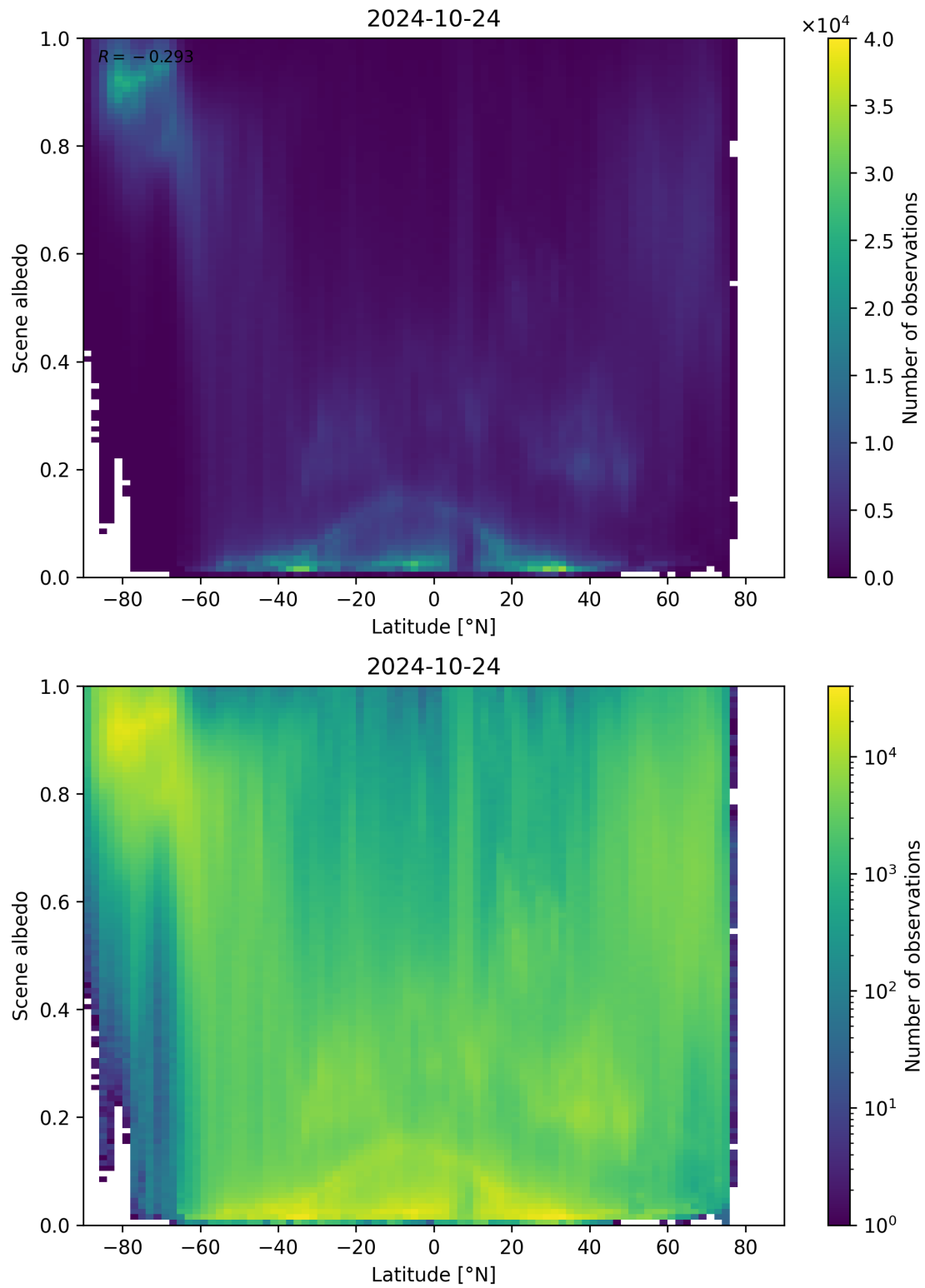
Figure 104: Scatter density plot of “Latitude” against “Scene albedo” for 2024-10-24 to 2024-10-25.
