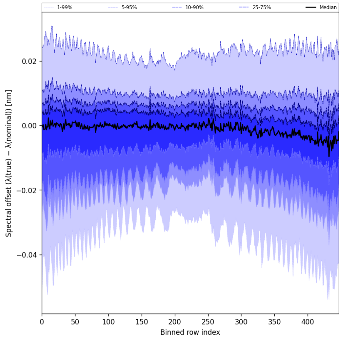
Figure 62: Along track statistics of “Spectral offset ( \lambda_{\text{true}} - \lambda_{\text{nominal}} )” for 2024-10-24 to 2024-10-25
