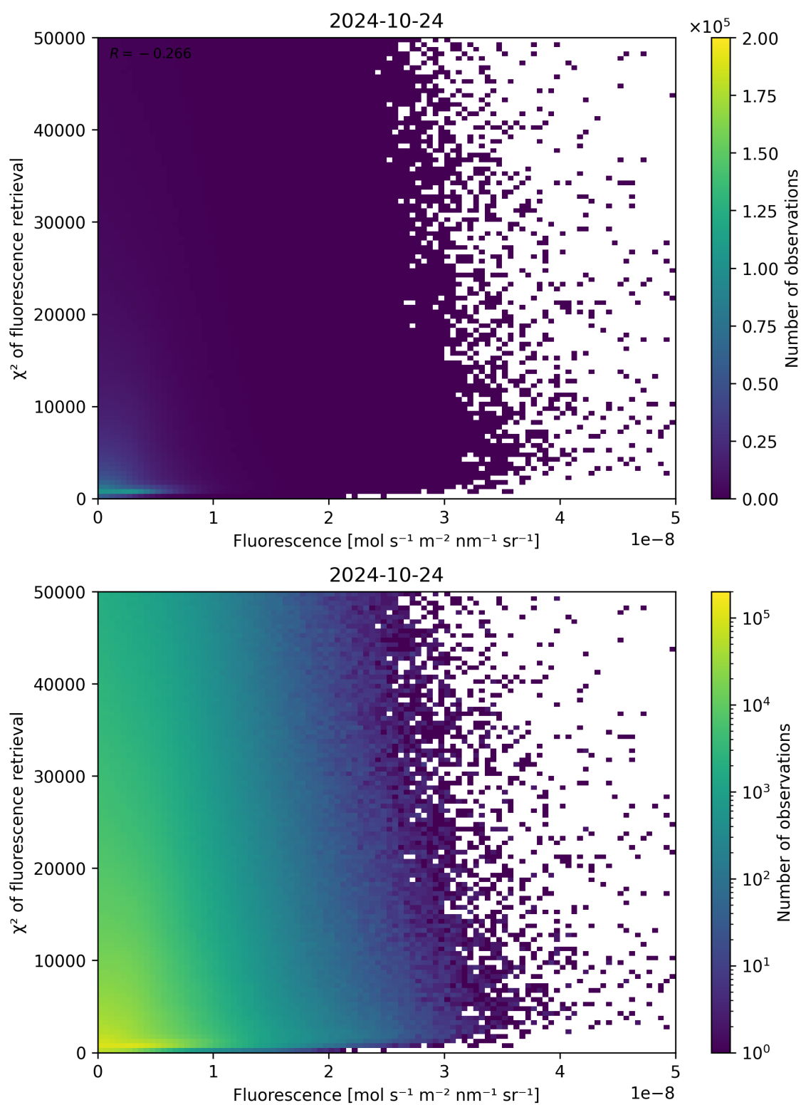
Figure 93: Scatter density plot of “Fluorescence” against “ \chi^2 of fluorescence retrieval” for 2024-10-24 to 2024-10-25.
