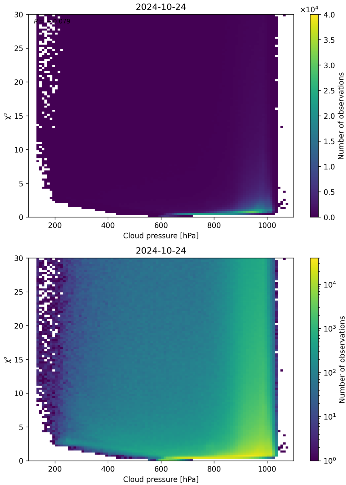
Figure 85: Scatter density plot of “Cloud pressure” against “ \chi^2 ” for 2024-10-24 to 2024-10-25.
