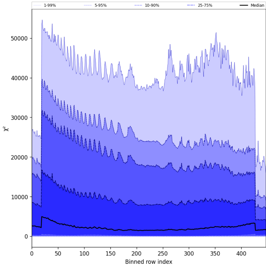
Figure 55: Along track statistics of “ \chi^2 ” for 2024-10-24 to 2024-10-25
