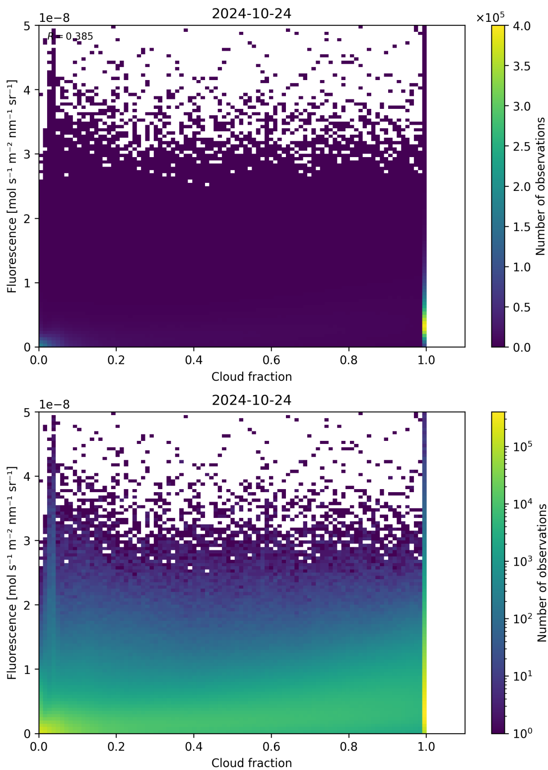
Figure 79: Scatter density plot of “Cloud fraction” against “Fluorescence” for 2024-10-24 to 2024-10-25.
