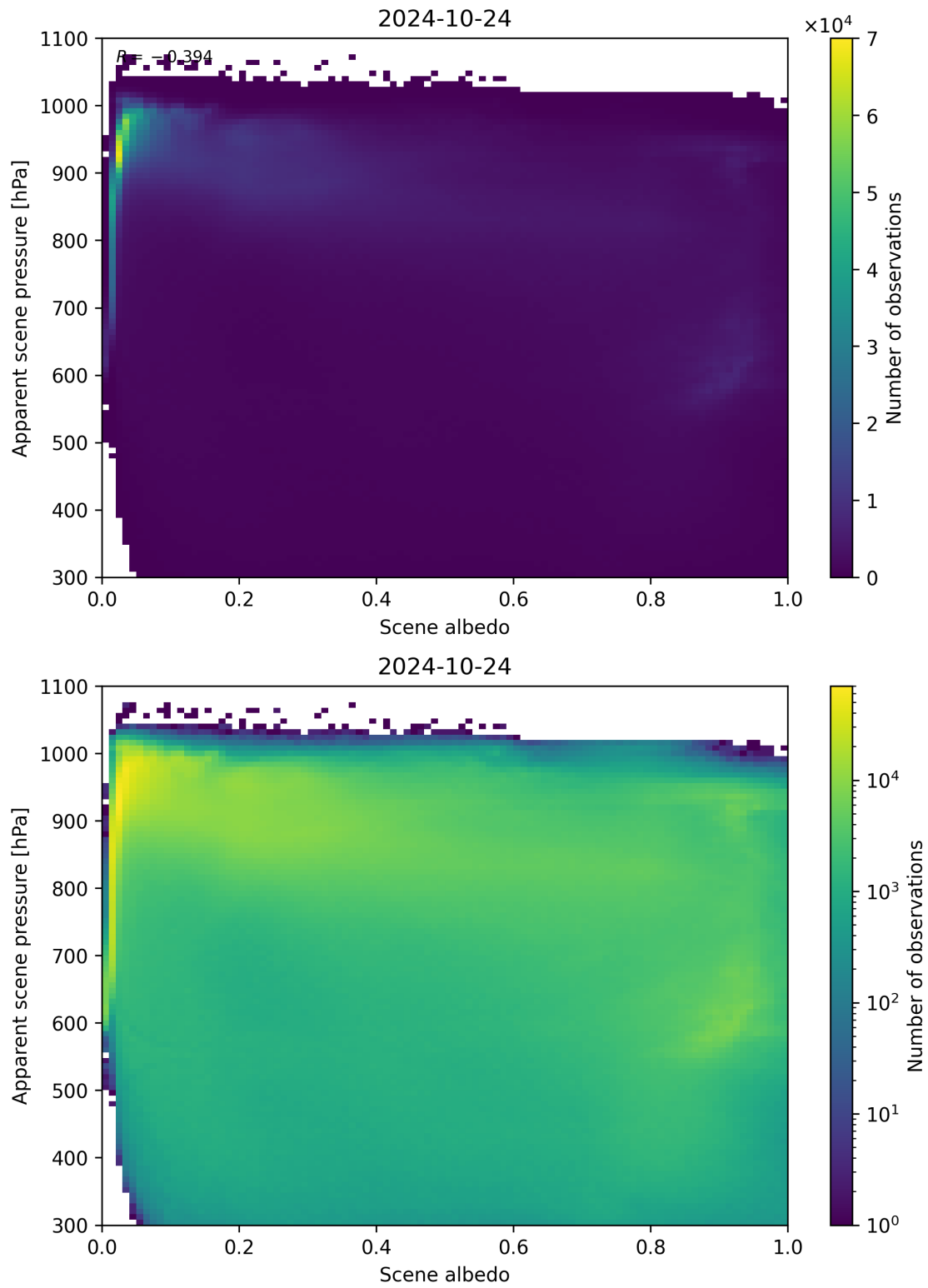
Figure 111: Scatter density plot of “Scene albedo” against “Apparent scene pressure” for 2024-10-24 to 2024-10-25.
