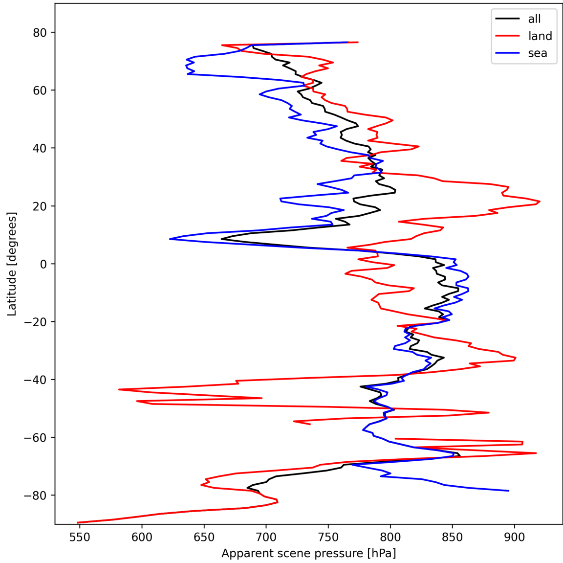
Figure 19: Zonal average of “Apparent scene pressure” for 2024-10-24 to 2024-10-25.
