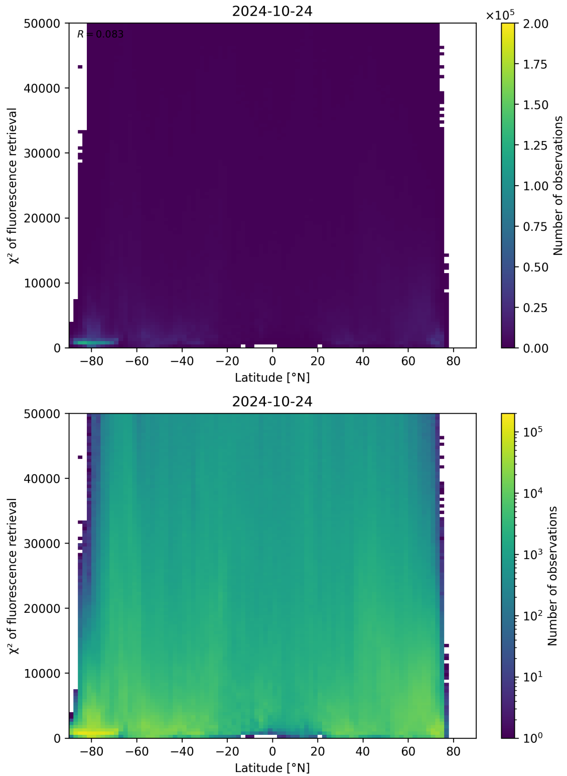
Figure 98: Scatter density plot of “Latitude” against “ \chi^2 of fluorescence retrieval” for 2024-10-24 to 2024-10-25.
