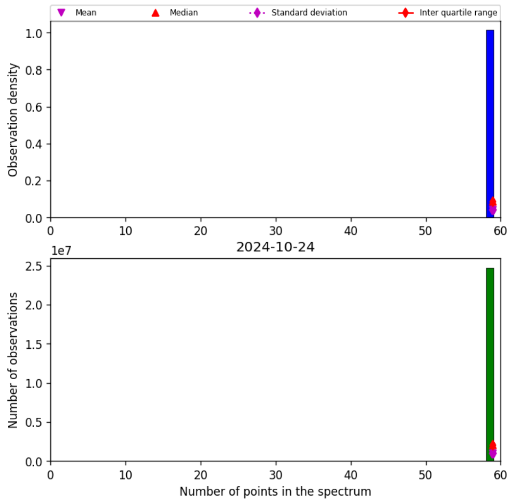
Figure 44: Histogram of “Number of points in the spectrum” for 2024-10-24 to 2024-10-25
