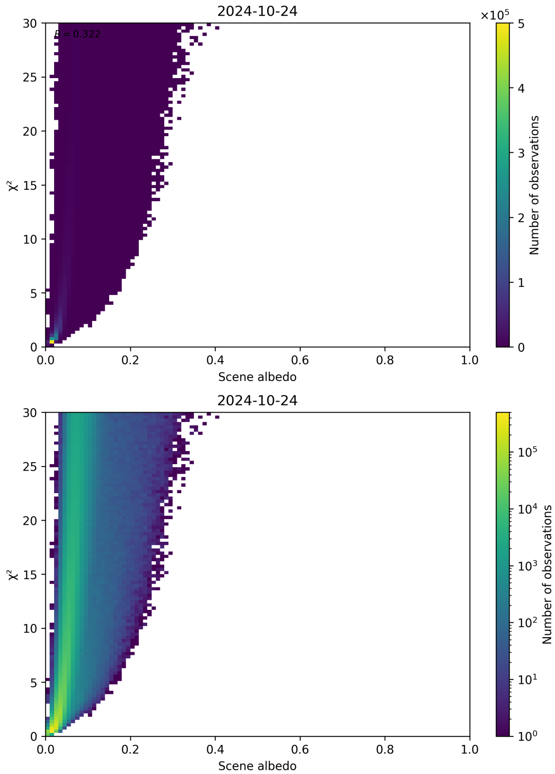
Figure 112: Scatter density plot of “Scene albedo” against “ \chi^2 ” for 2024-10-24 to 2024-10-25.
