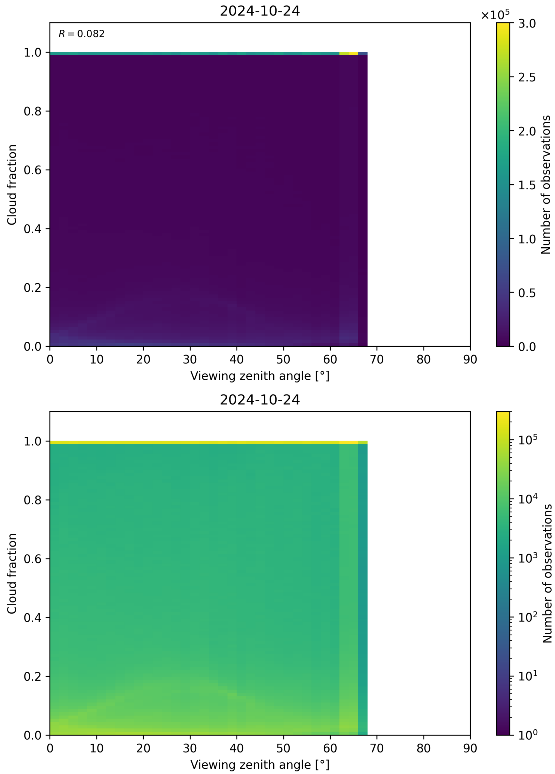
Figure 132: Scatter density plot of “Viewing zenith angle” against “Cloud fraction” for 2024-10-24 to 2024-10-25.
