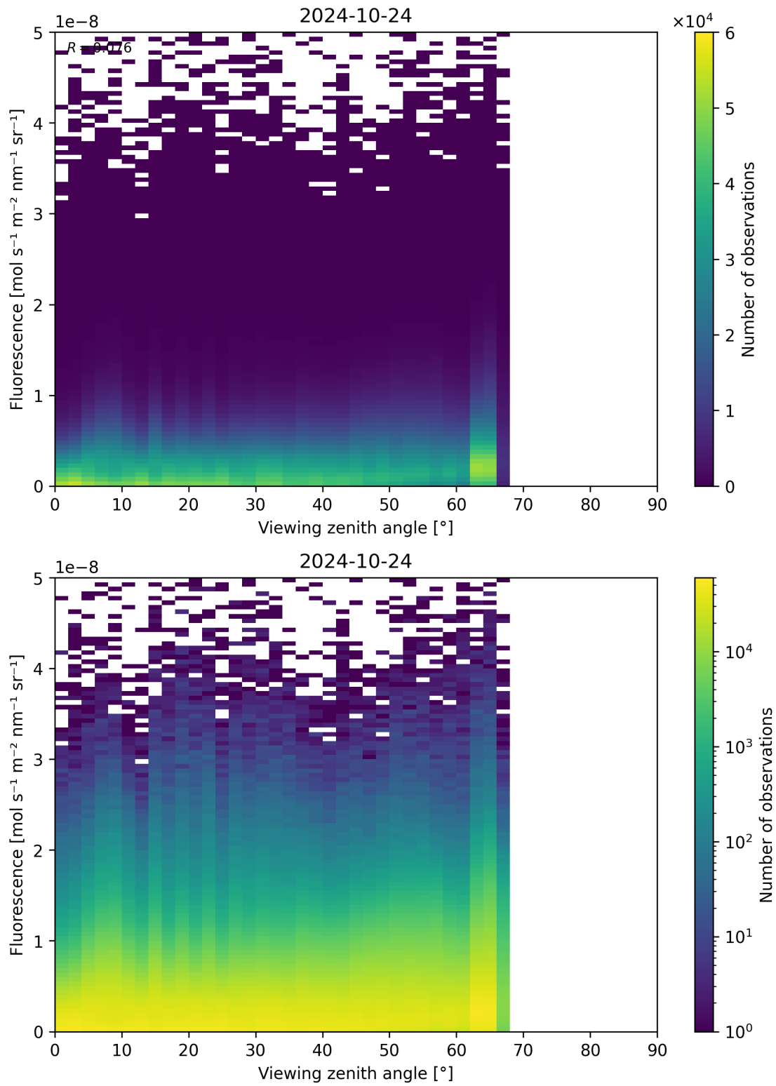
Figure 134: Scatter density plot of “Viewing zenith angle” against “Fluorescence” for 2024-10-24 to 2024-10-25.
