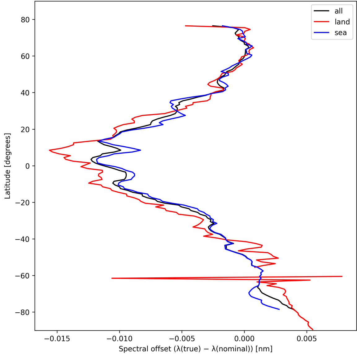
Figure 28: Zonal average of “Spectral offset ( \lambda_{\text{true}} - \lambda_{\text{nominal}} )” for 2024-10-24 to 2024-10-25.
