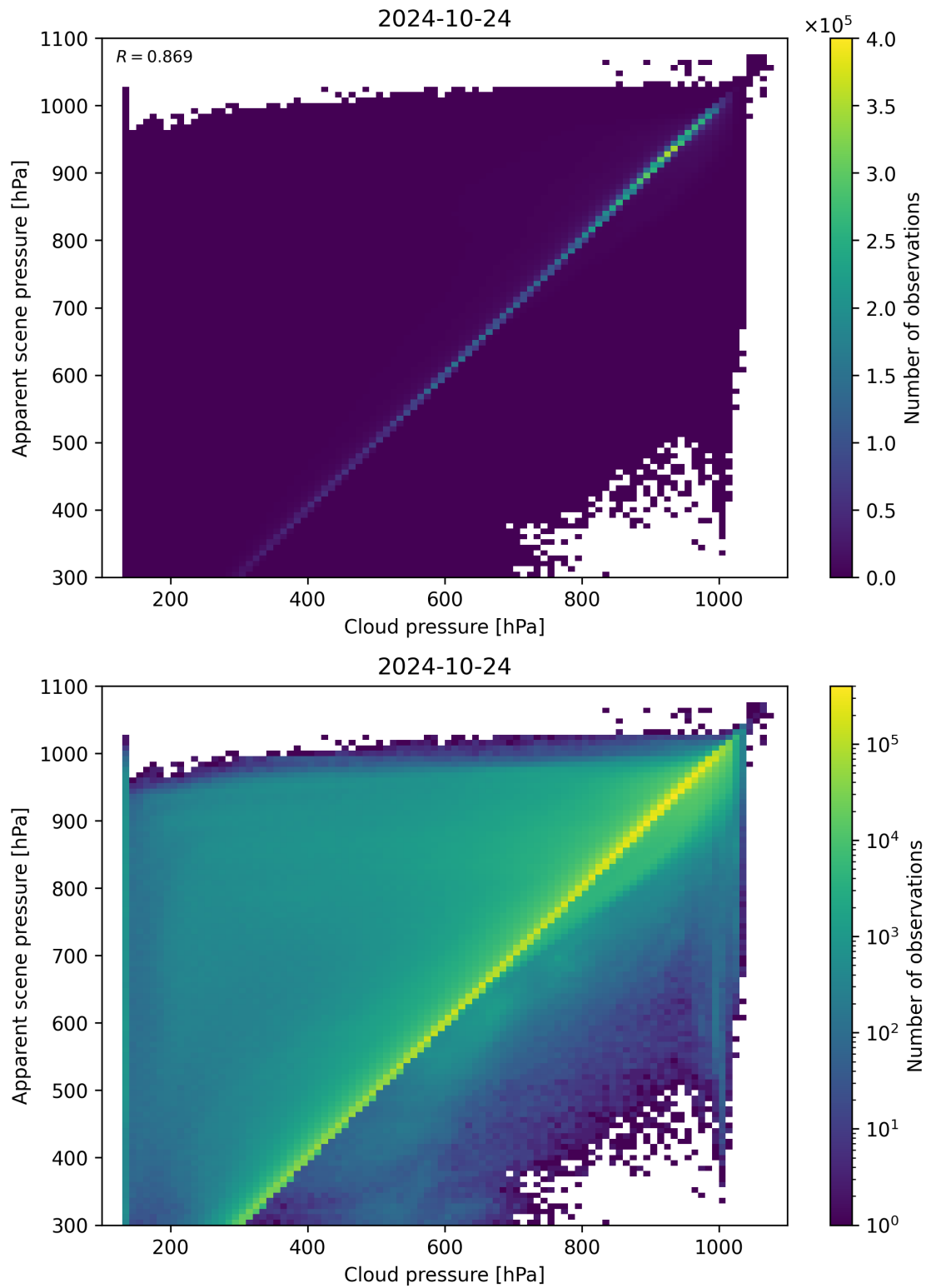
Figure 84: Scatter density plot of “Cloud pressure” against “Apparent scene pressure” for 2024-10-24 to 2024-10-25.
