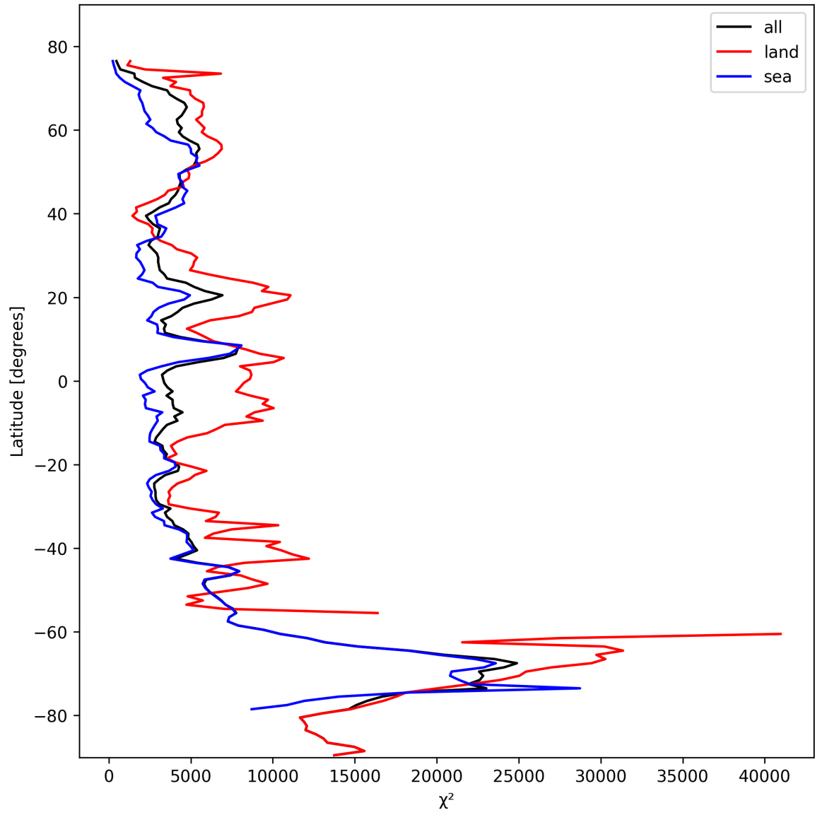
Figure 21: Zonal average of “ \chi^2 ” for 2024-10-24 to 2024-10-25.
