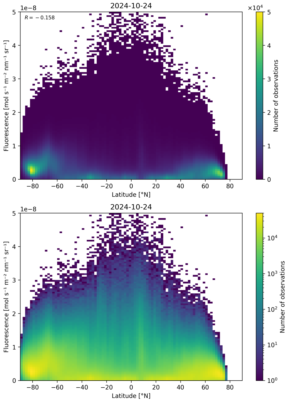
Figure 101: Scatter density plot of “Latitude” against “Fluorescence” for 2024-10-24 to 2024-10-25.
