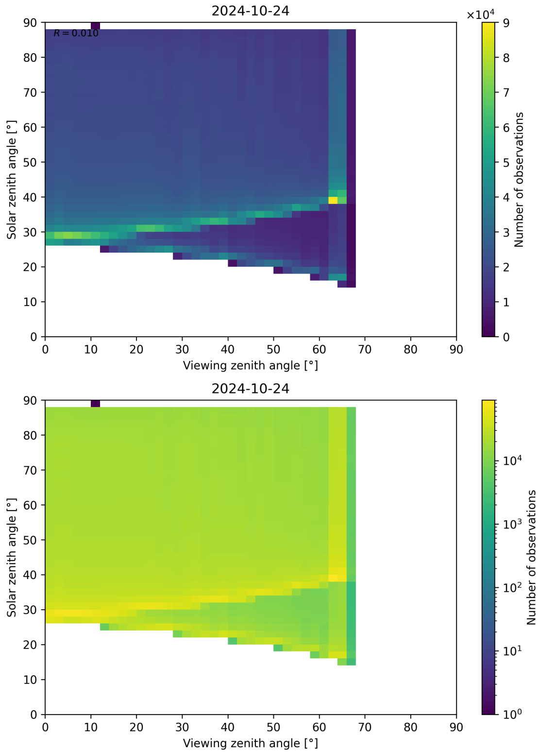
Figure 139: Scatter density plot of “Viewing zenith angle” against “Solar zenith angle” for 2024-10-24 to 2024-10-25.
