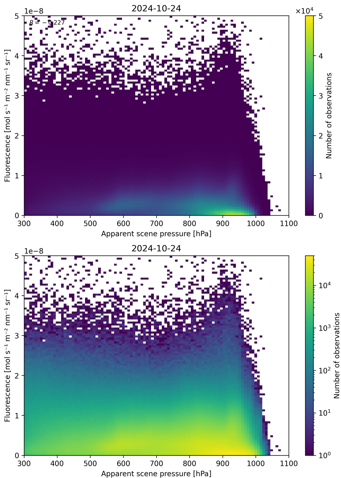
Figure 65: Scatter density plot of “Apparent scene pressure” against “Fluorescence” for 2024-10-24 to 2024-10-25.
