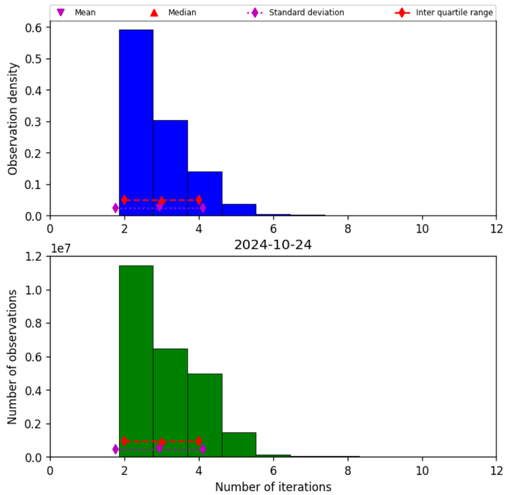
Figure 39: Histogram of “Number of iterations” for 2024-10-24 to 2024-10-25
