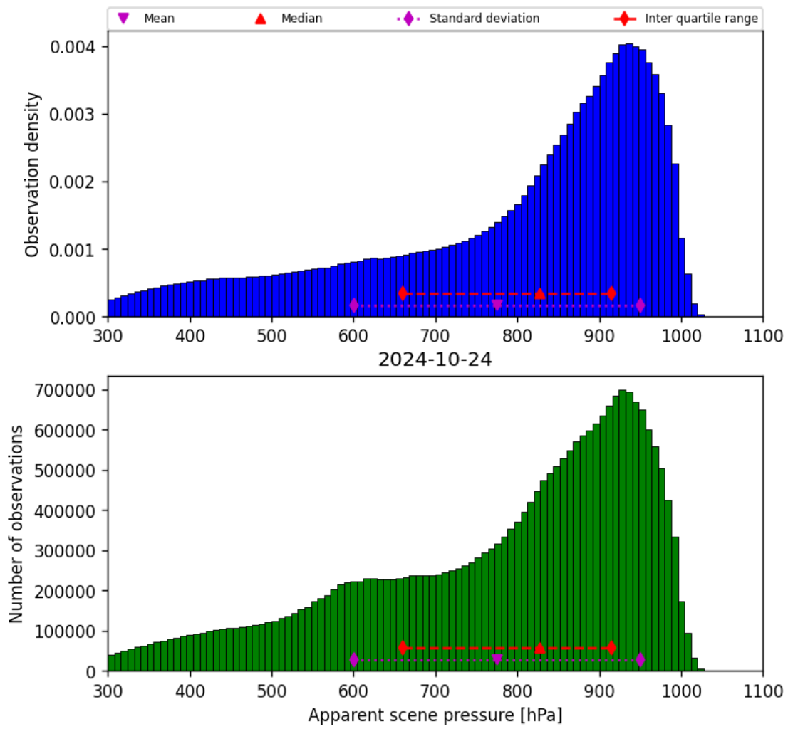
Figure 36: Histogram of “Apparent scene pressure” for 2024-10-24 to 2024-10-25
