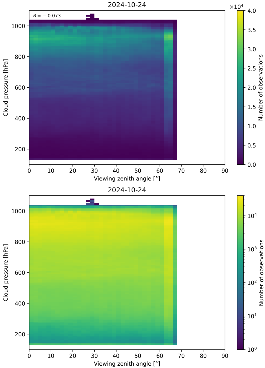
Figure 133: Scatter density plot of “Viewing zenith angle” against “Cloud pressure” for 2024-10-24 to 2024-10-25.
