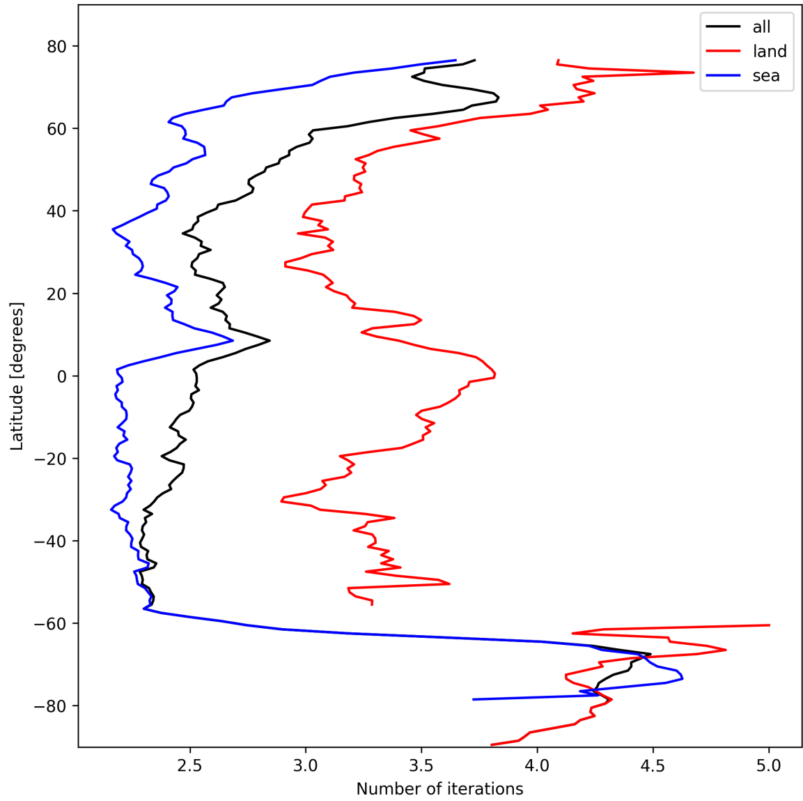
Figure 22: Zonal average of “Number of iterations” for 2024-10-24 to 2024-10-25.
