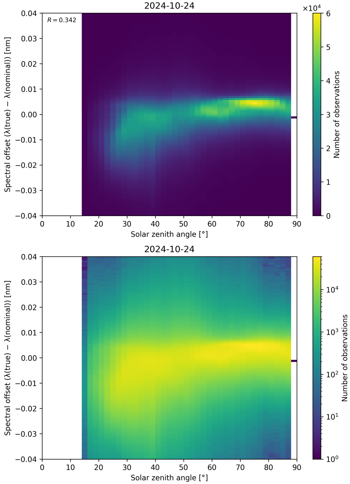
Figure 128: Scatter density plot of “Solar zenith angle” against “Spectral offset ( \lambda_{\text{true}} - \lambda_{\text{nominal}} )” for 2024-10-24 to 2024-10-25.
