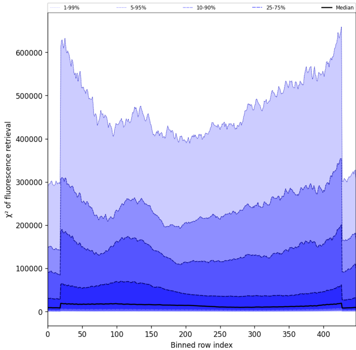
Figure 59: Along track statistics of “ \chi^2 of fluorescence retrieval” for 2024-10-24 to 2024-10-25
