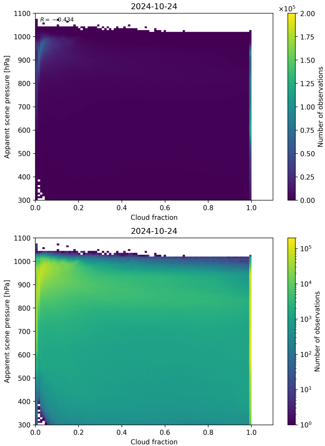
Figure 76: Scatter density plot of “Cloud fraction” against “Apparent scene pressure” for 2024-10-24 to 2024-10-25.
