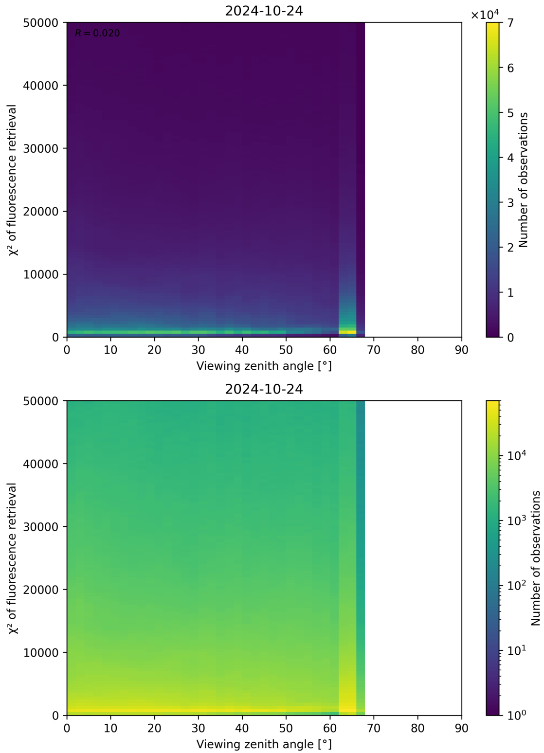
Figure 131: Scatter density plot of “Viewing zenith angle” against “ \chi^2 of fluorescence retrieval” for 2024-10-24 to 2024-10-25.
