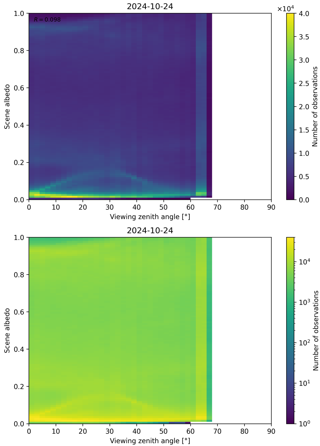
Figure 138: Scatter density plot of “Viewing zenith angle” against “Scene albedo” for 2024-10-24 to 2024-10-25.
