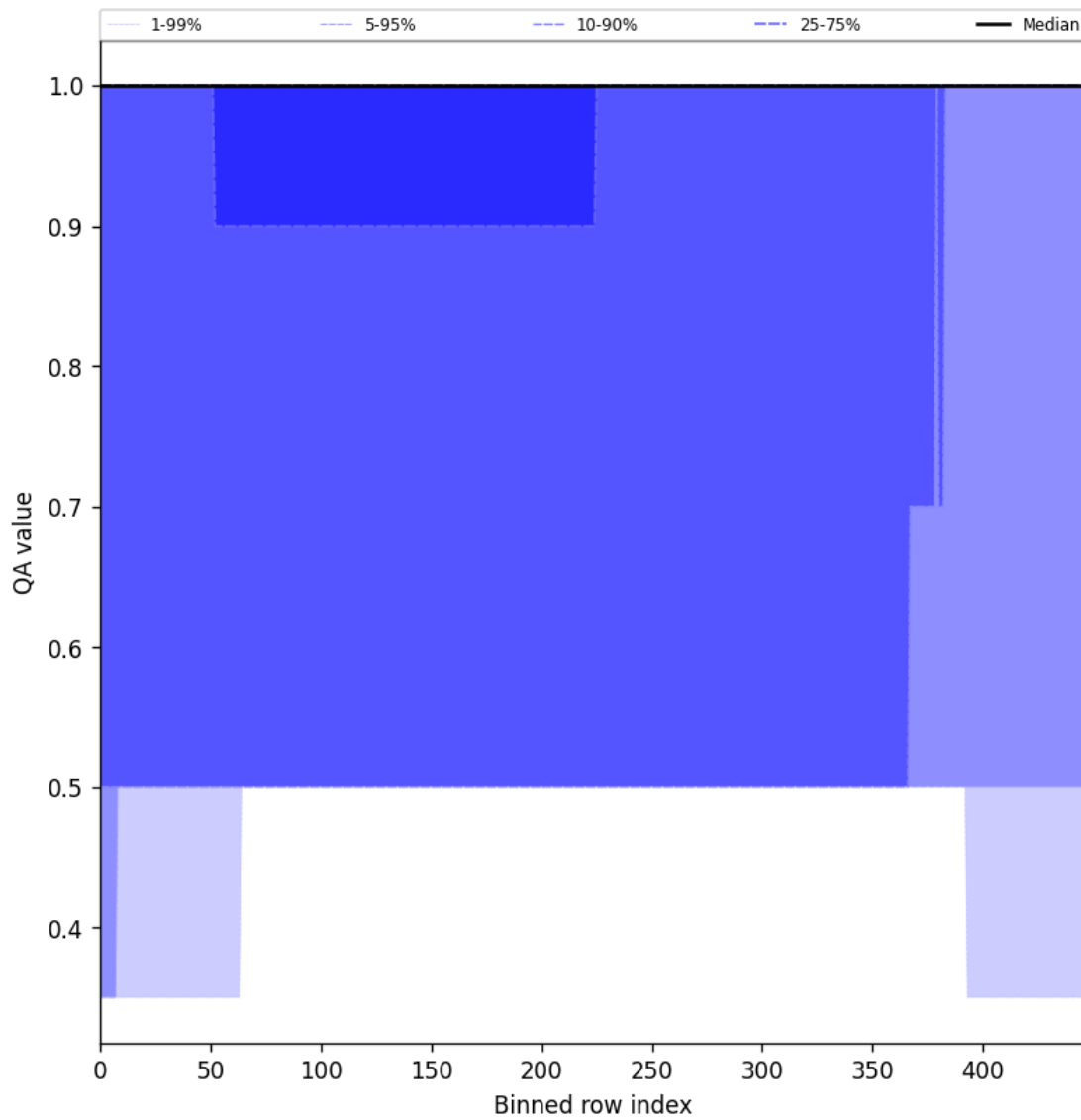
Figure 46: Along track statistics of “QA value” for 2024-10-24 to 2024-10-25
