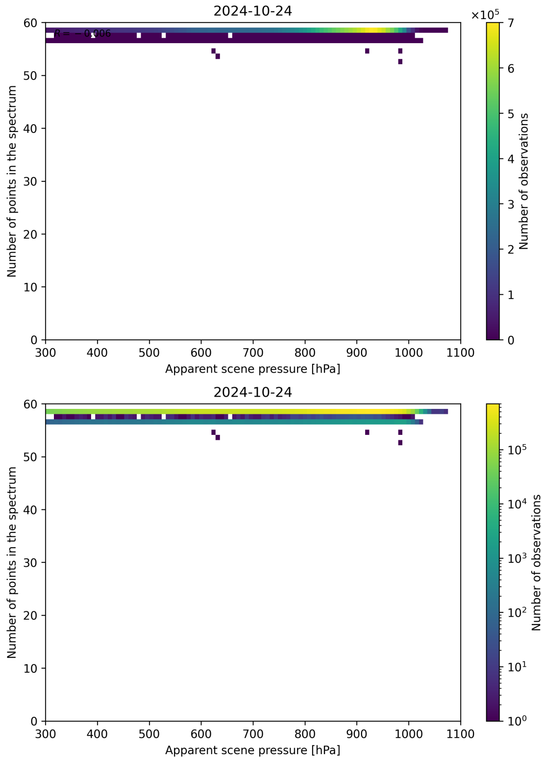
Figure 67: Scatter density plot of “Apparent scene pressure” against “Number of points in the spectrum” for 2024-10-24 to 2024-10-25.
