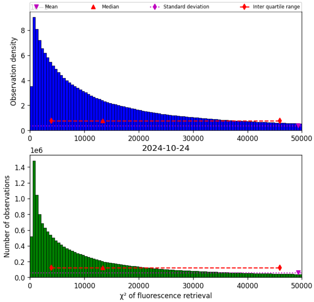
Figure 42: Histogram of “ \chi^2 of fluorescence retrieval” for 2024-10-24 to 2024-10-25
