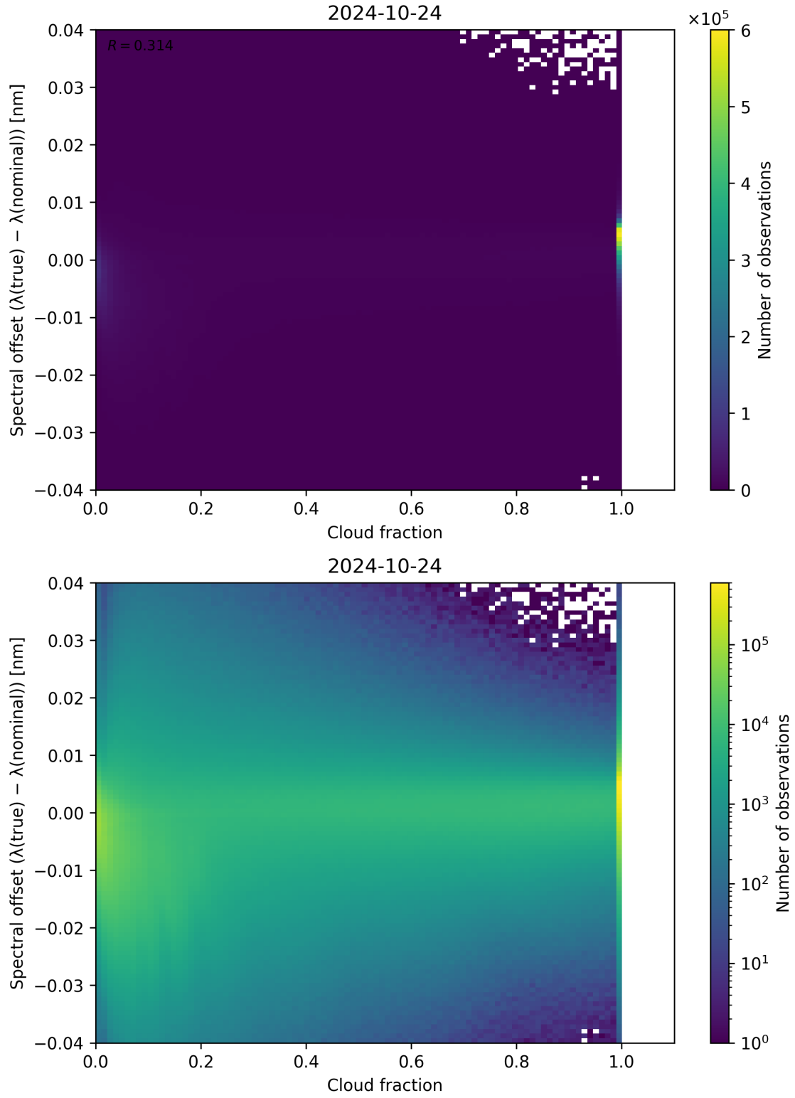
Figure 83: Scatter density plot of “Cloud fraction” against “Spectral offset ( \lambda_{\text{true}} - \lambda_{\text{nominal}} )” for 2024-10-24 to 2024-10-25.
