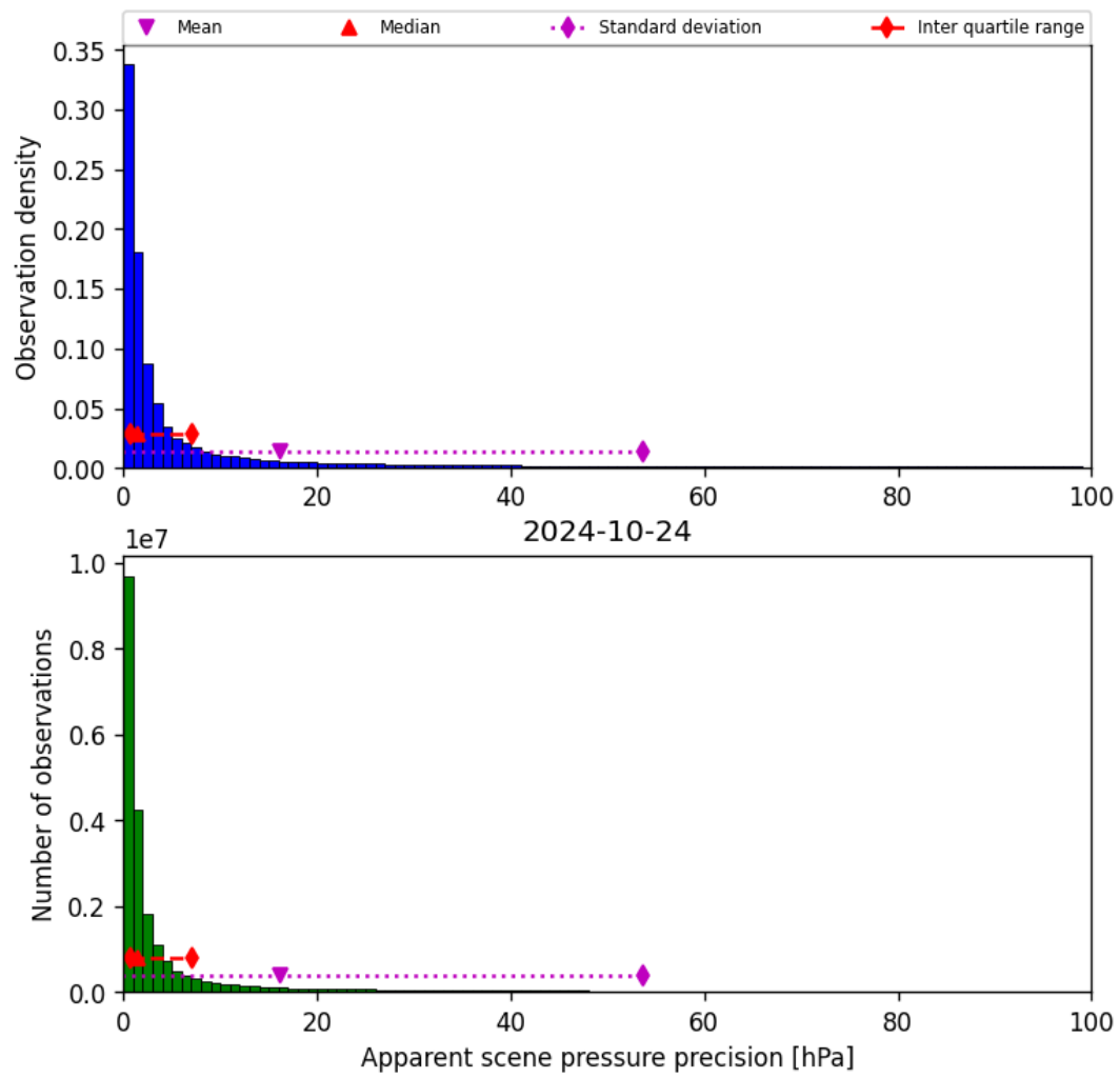
Figure 37: Histogram of “Apparent scene pressure precision” for 2024-10-24 to 2024-10-25
