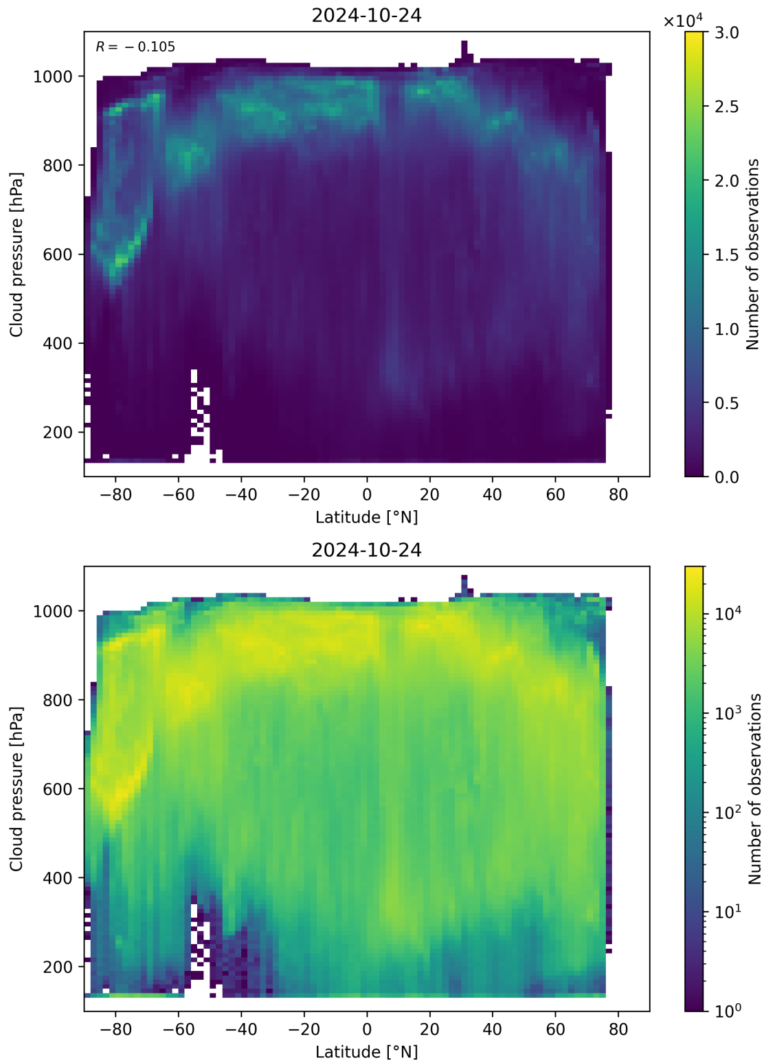
Figure 100: Scatter density plot of “Latitude” against “Cloud pressure” for 2024-10-24 to 2024-10-25.
