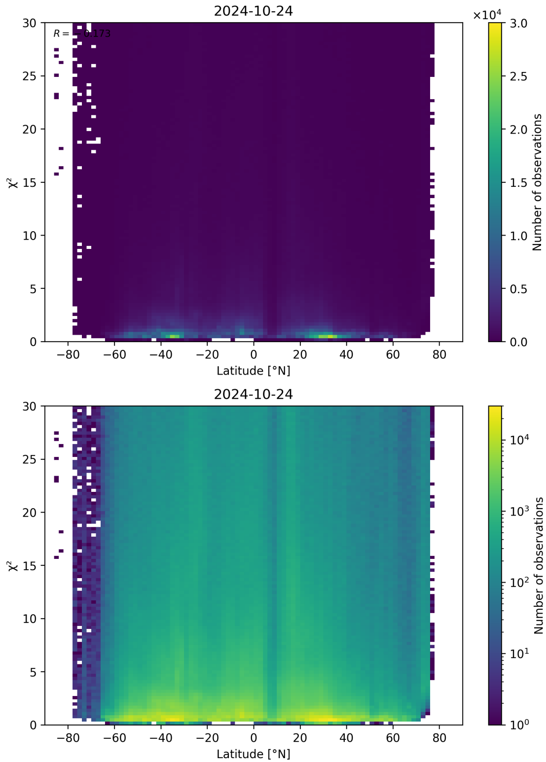
Figure 97: Scatter density plot of “Latitude” against “ \chi^2 ” for 2024-10-24 to 2024-10-25.
