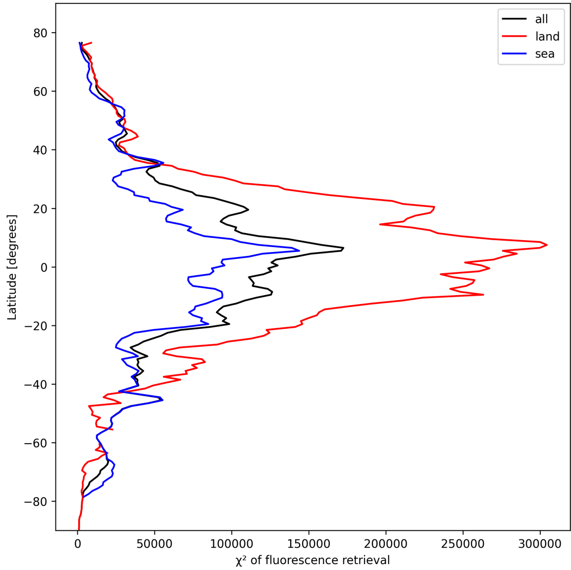
Figure 25: Zonal average of “ \chi^2 of fluorescence retrieval” for 2024-10-24 to 2024-10-25.
