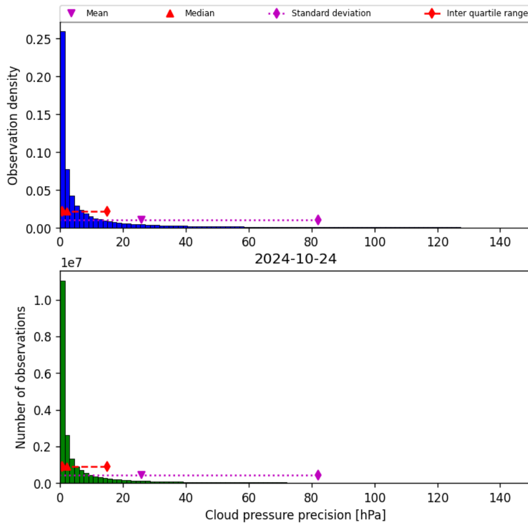
Figure 31: Histogram of “Cloud pressure precision” for 2024-10-24 to 2024-10-25
