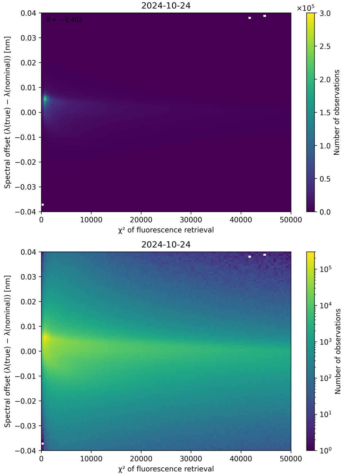
Figure 72: Scatter density plot of “ \chi^2 of fluorescence retrieval” against “Spectral offset ( \lambda_{\text{true}} - \lambda_{\text{nominal}} )” for 2024-10-24 to 2024-10-25.
