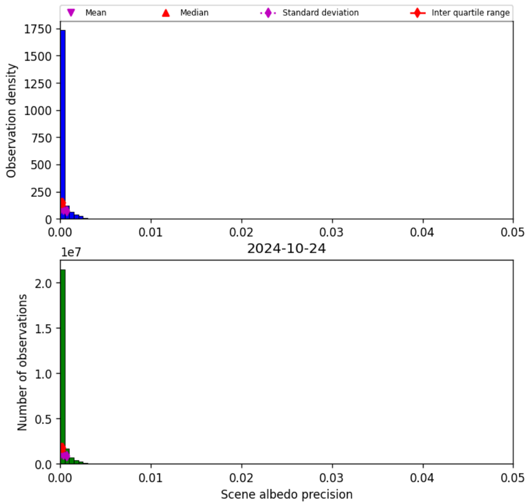
Figure 35: Histogram of “Scene albedo precision” for 2024-10-24 to 2024-10-25
