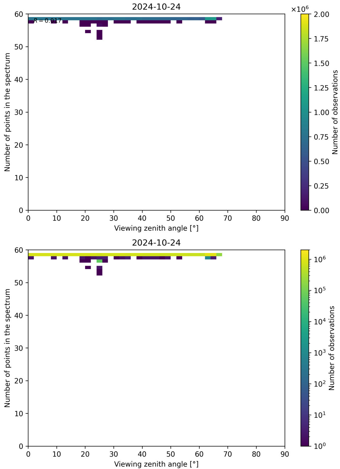
Figure 137: Scatter density plot of “Viewing zenith angle” against “Number of points in the spectrum” for 2024-10-24 to 2024-10-25.
