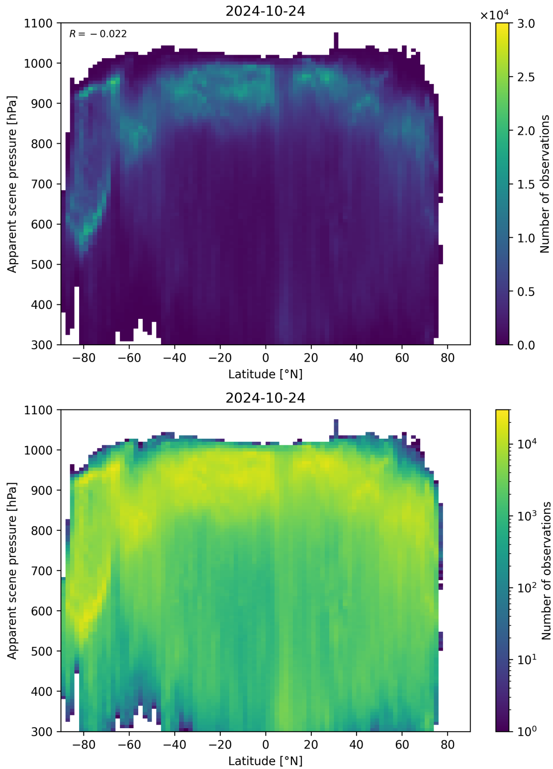
Figure 96: Scatter density plot of “Latitude” against “Apparent scene pressure” for 2024-10-24 to 2024-10-25.
