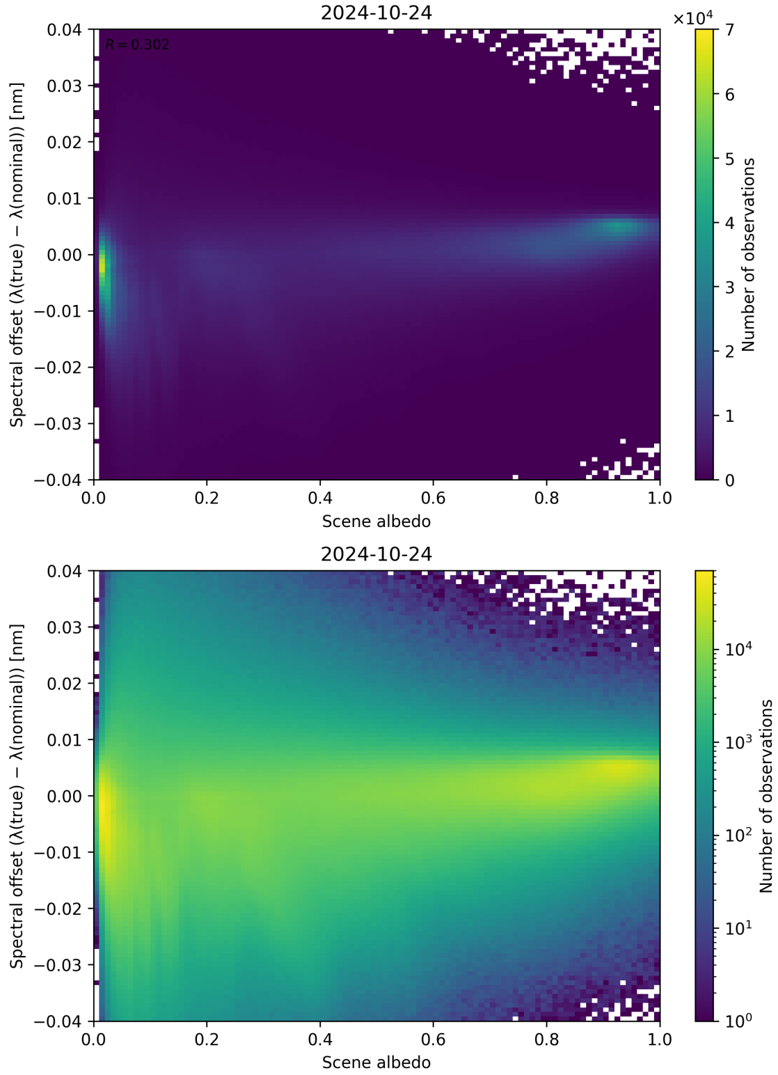
Figure 117: Scatter density plot of “Scene albedo” against “Spectral offset ( \lambda_{\text{true}} - \lambda_{\text{nominal}} )” for 2024-10-24 to 2024-10-25.
