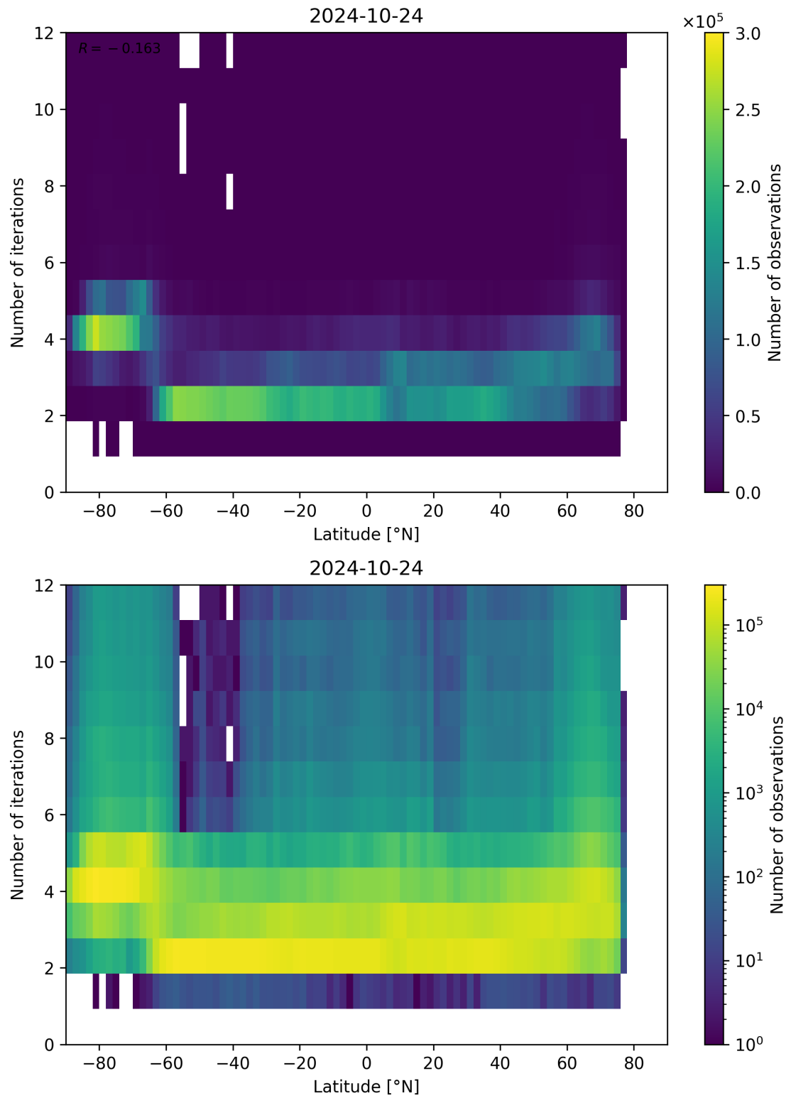
Figure 102: Scatter density plot of “Latitude” against “Number of iterations” for 2024-10-24 to 2024-10-25.
