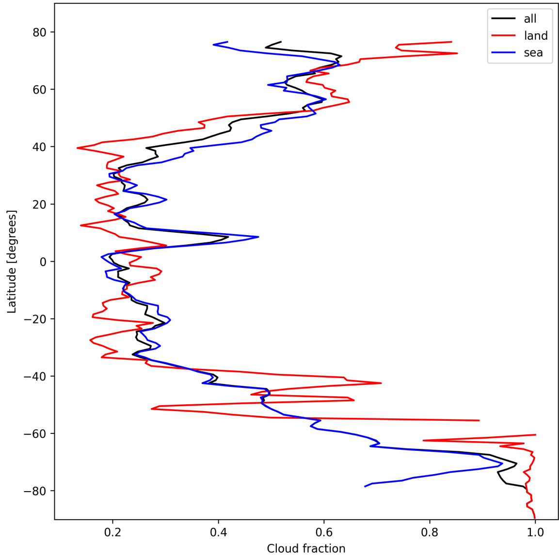
Figure 15: Zonal average of “Cloud fraction” for 2024-10-24 to 2024-10-25.
