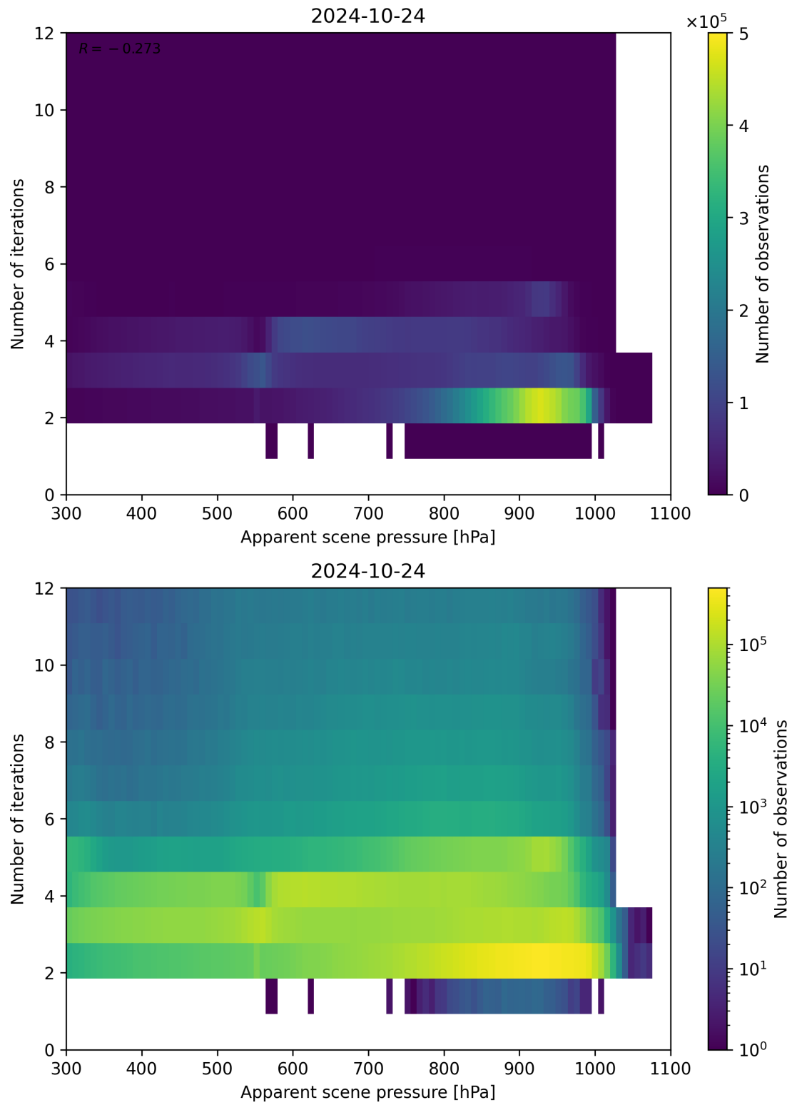
Figure 66: Scatter density plot of “Apparent scene pressure” against “Number of iterations” for 2024-10-24 to 2024-10-25.
