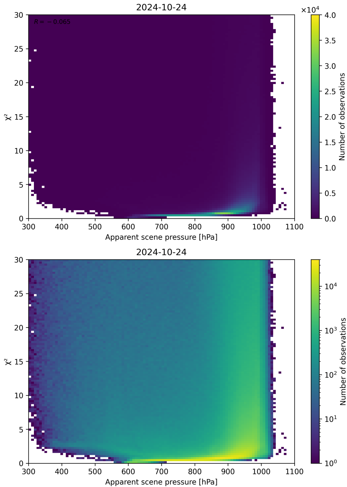
Figure 63: Scatter density plot of “Apparent scene pressure” against “ \chi^2 ” for 2024-10-24 to 2024-10-25.
