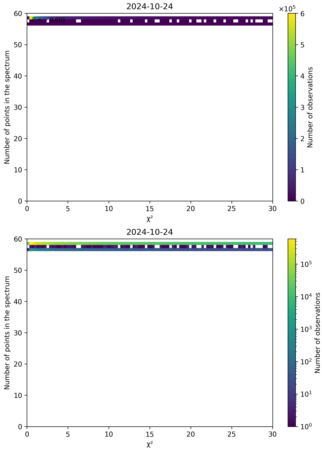
Figure 74: Scatter density plot of " \chi^2 " against "Number of points in the spectrum" for 2024-10-24 to 2024-10-25.
