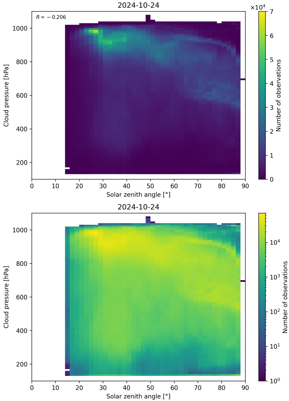
Figure 122: Scatter density plot of “Solar zenith angle” against “Cloud pressure” for 2024-10-24 to 2024-10-25.
