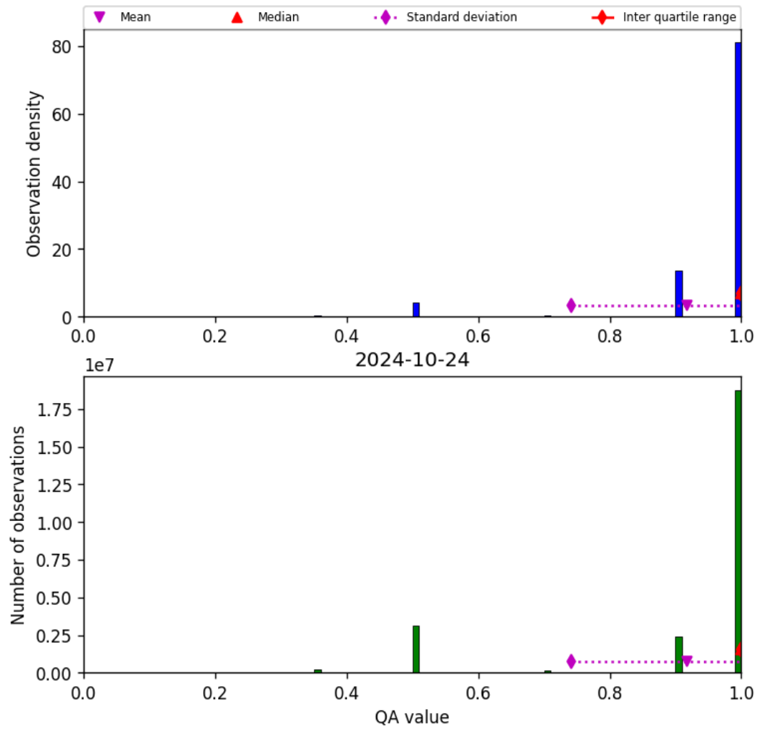
Figure 29: Histogram of “QA value” for 2024-10-24 to 2024-10-25
