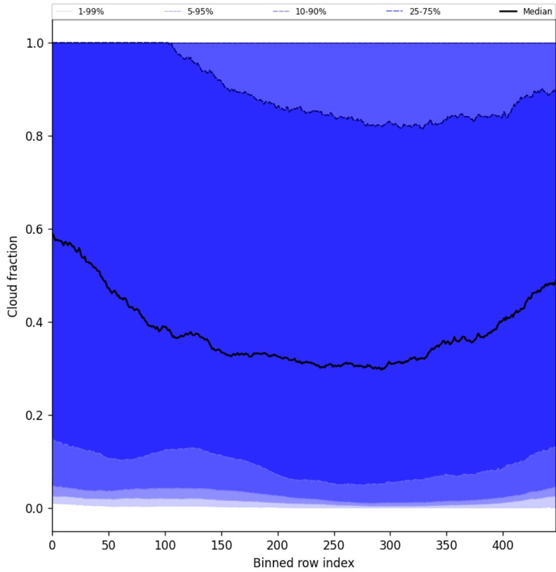
Figure 49: Along track statistics of “Cloud fraction” for 2024-10-24 to 2024-10-25
