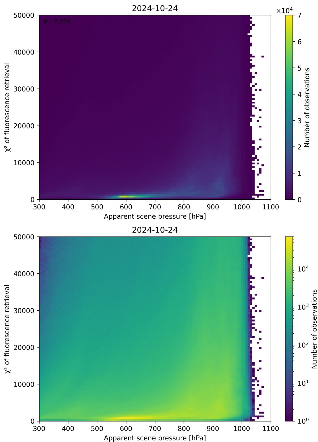
Figure 64: Scatter density plot of “Apparent scene pressure” against “ \chi^2 of fluorescence retrieval” for 2024-10-24 to 2024-10-25.
