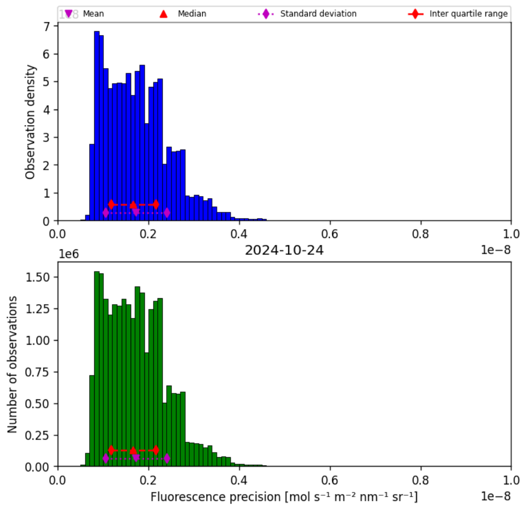
Figure 41: Histogram of “Fluorescence precision” for 2024-10-24 to 2024-10-25
