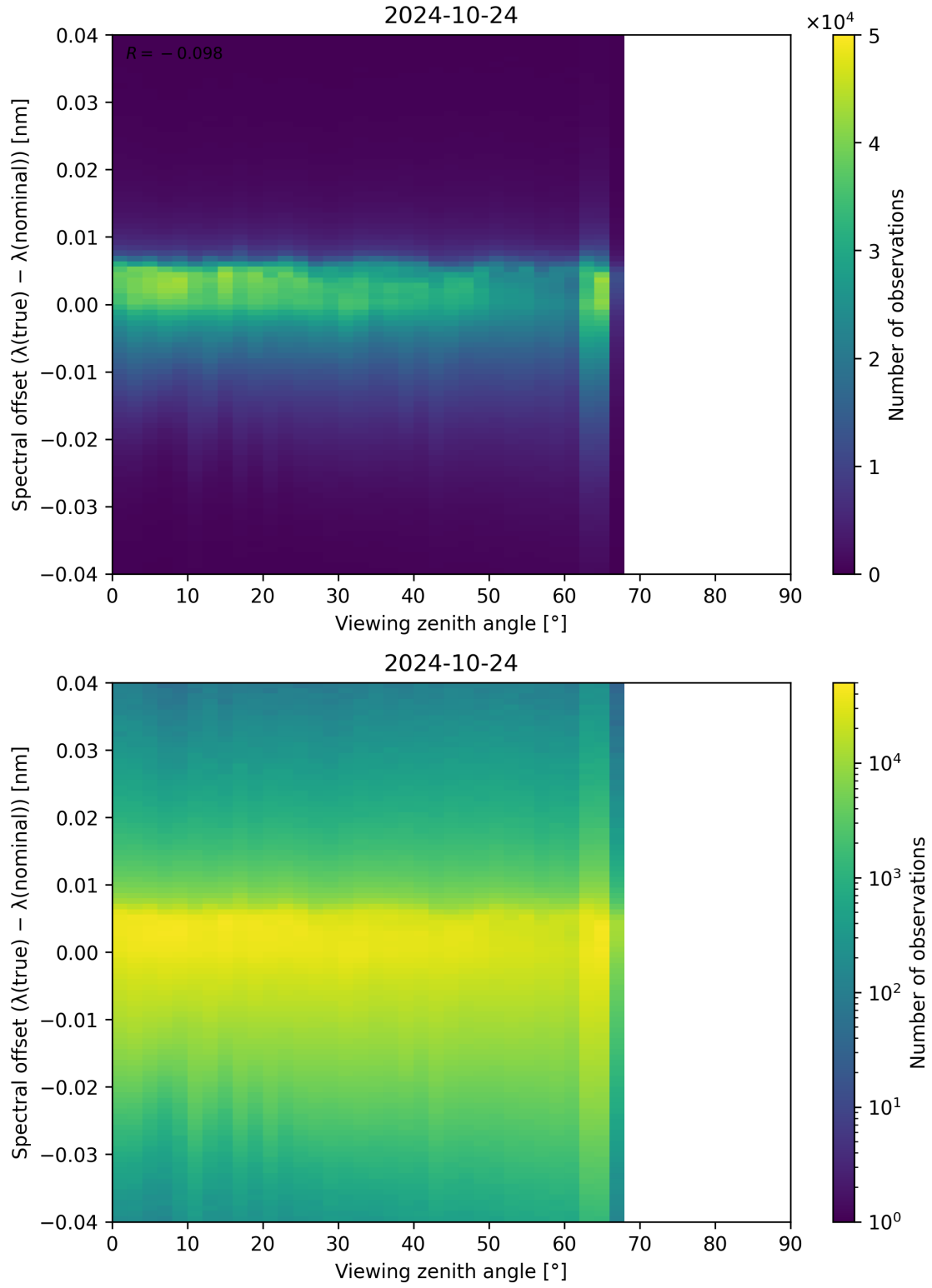
Figure 140: Scatter density plot of “Viewing zenith angle” against “Spectral offset ( \lambda_{\text{true}} - \lambda_{\text{nominal}} )” for 2024-10-24 to 2024-10-25.
