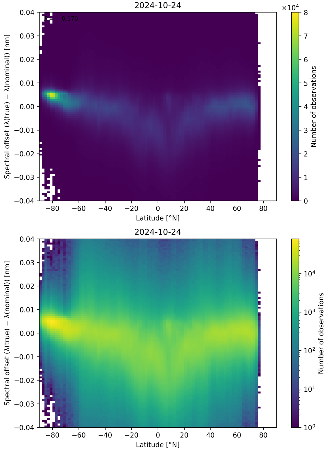
Figure 105: Scatter density plot of “Latitude” against “Spectral offset ( \lambda_{\text{true}} - \lambda_{\text{nominal}} )” for 2024-10-24 to 2024-10-25.
