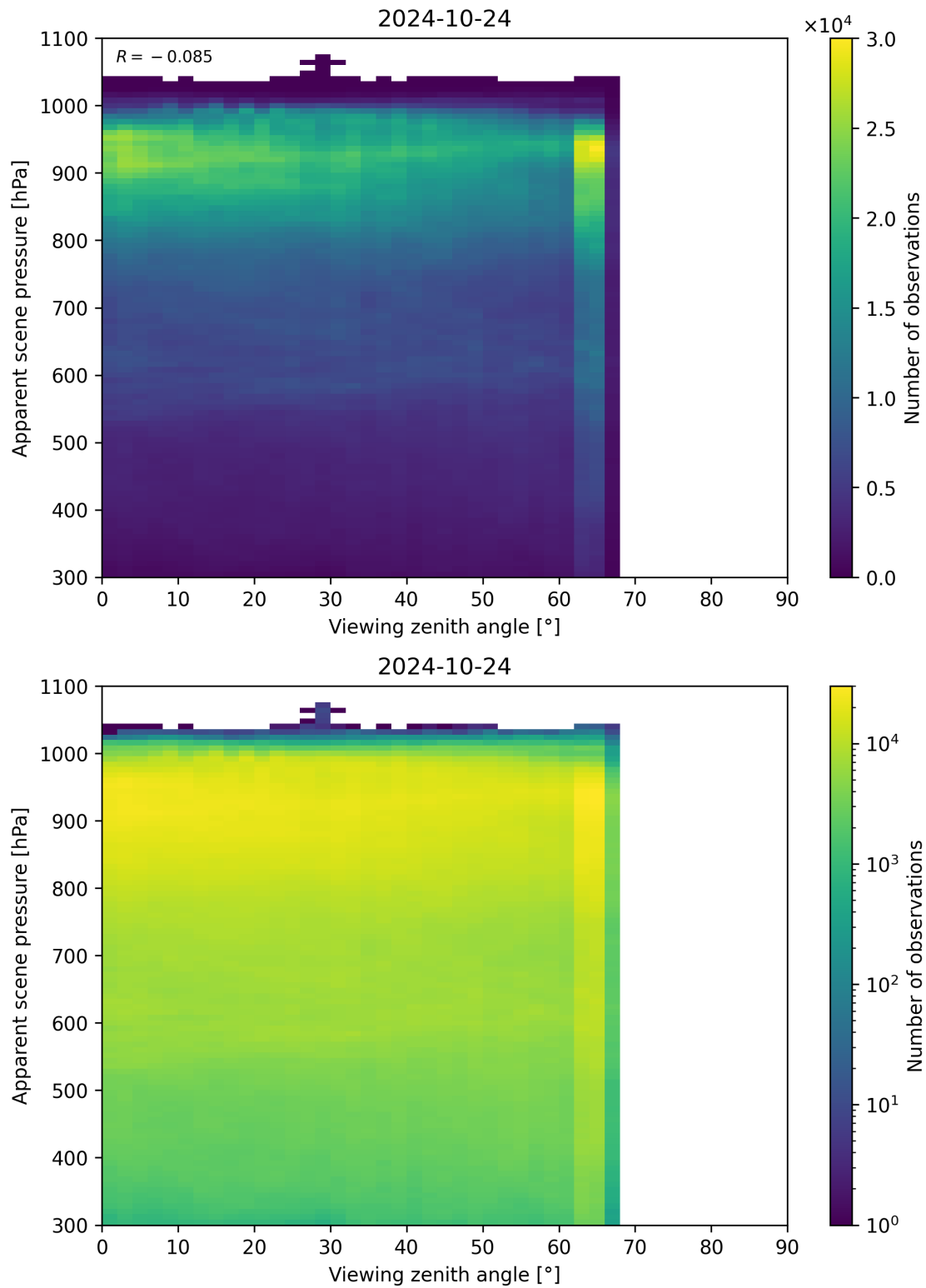
Figure 129: Scatter density plot of “Viewing zenith angle” against “Apparent scene pressure” for 2024-10-24 to 2024-10-25.
