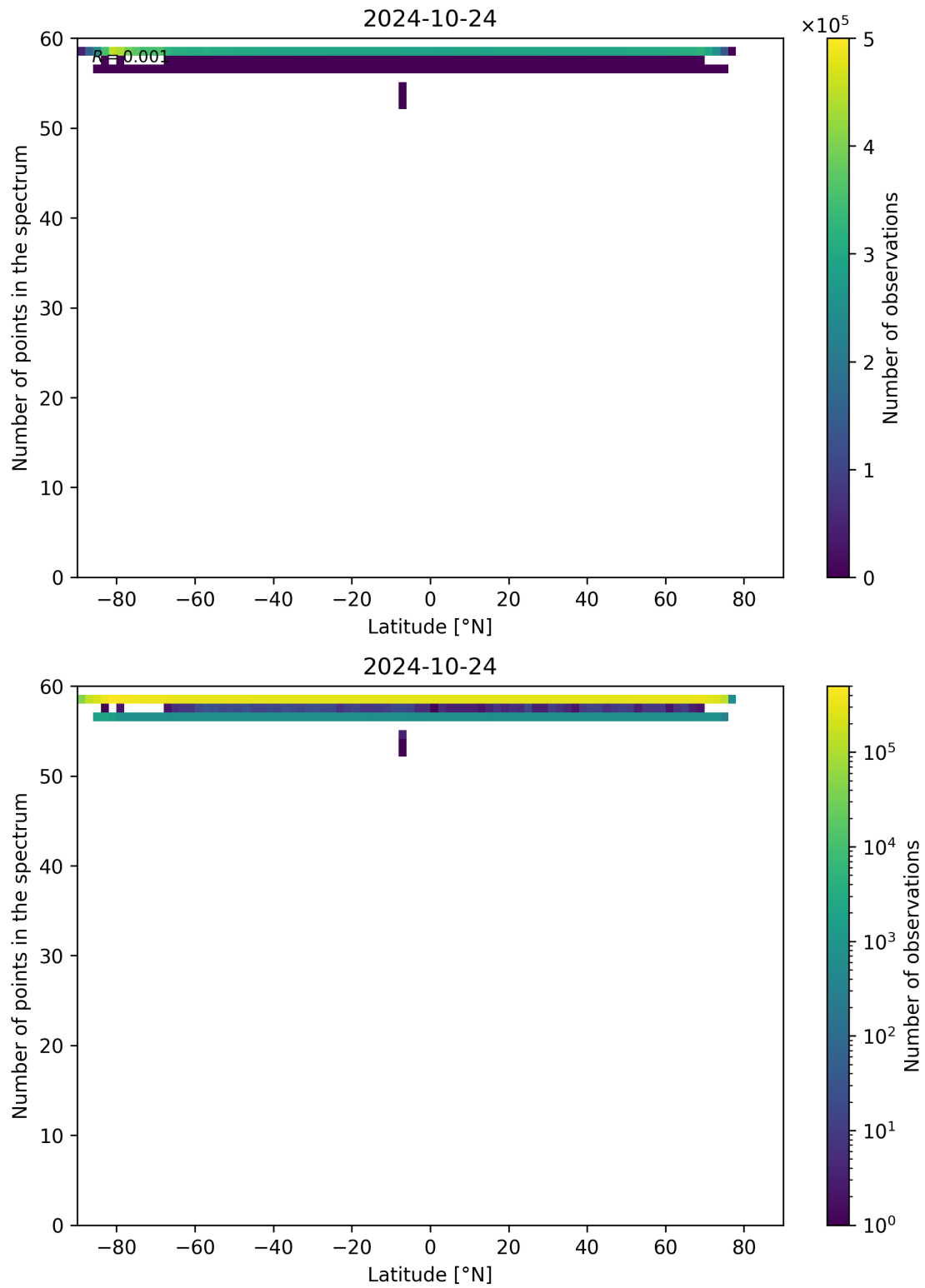
Figure 103: Scatter density plot of “Latitude” against “Number of points in the spectrum” for 2024-10-24 to 2024-10-25.
