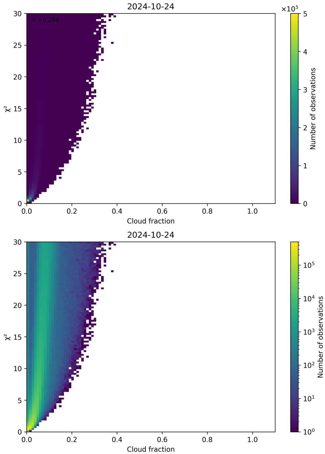
Figure 77: Scatter density plot of “Cloud fraction” against “ \chi^2 ” for 2024-10-24 to 2024-10-25.
