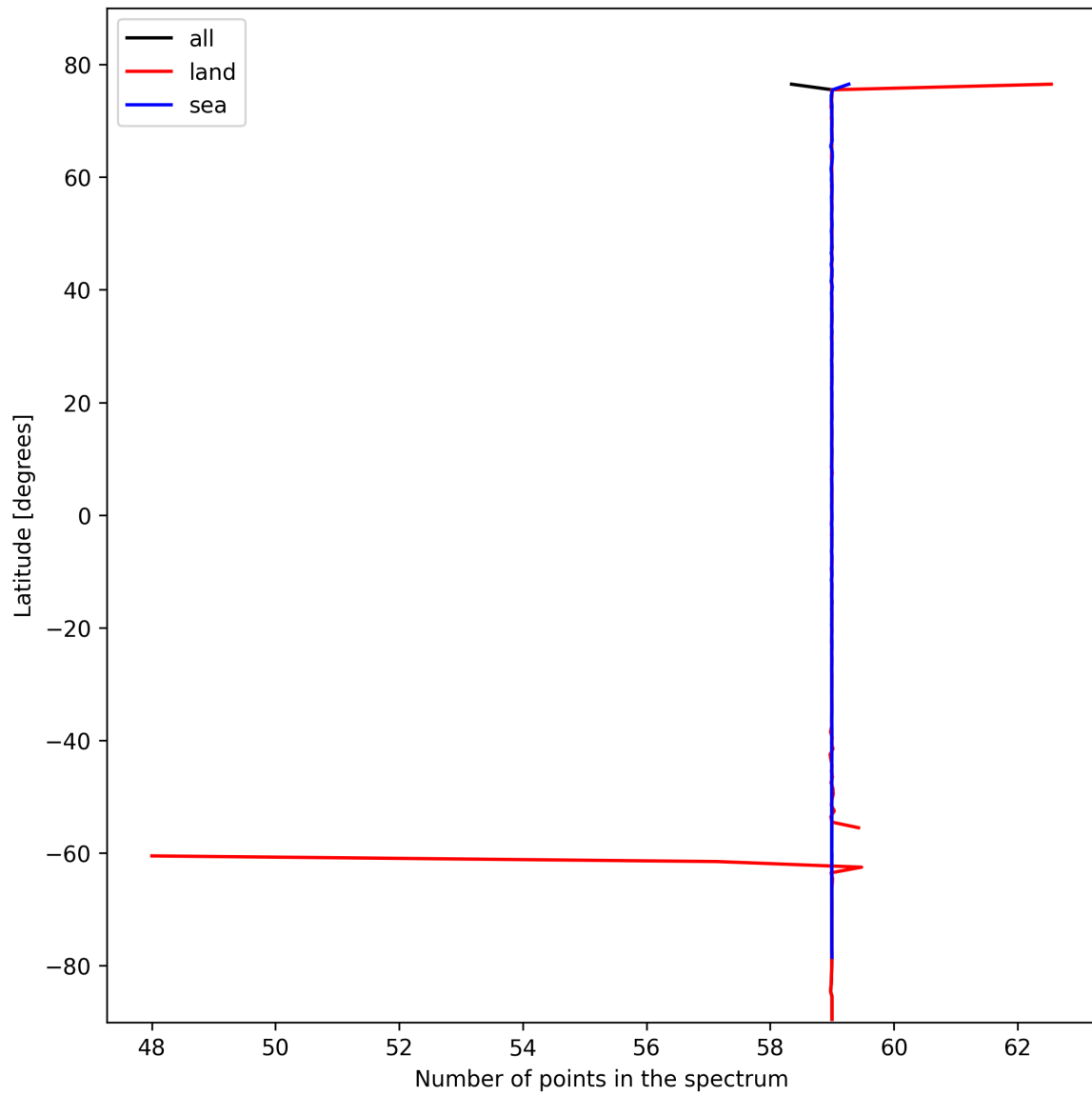
Figure 27: Zonal average of “Number of points in the spectrum” for 2024-10-24 to 2024-10-25.
