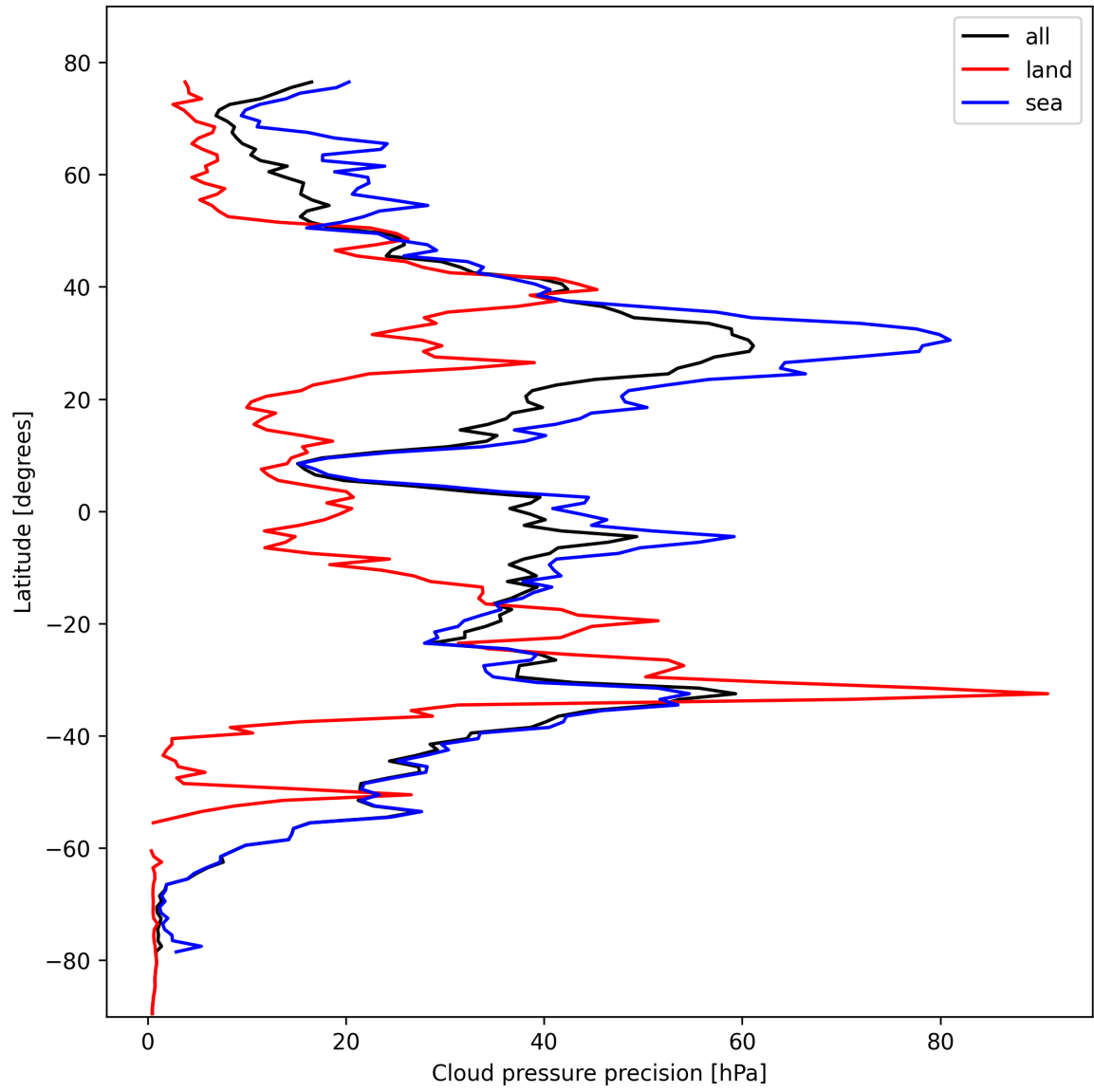
Figure 14: Zonal average of “Cloud pressure precision” for 2024-10-24 to 2024-10-25.
