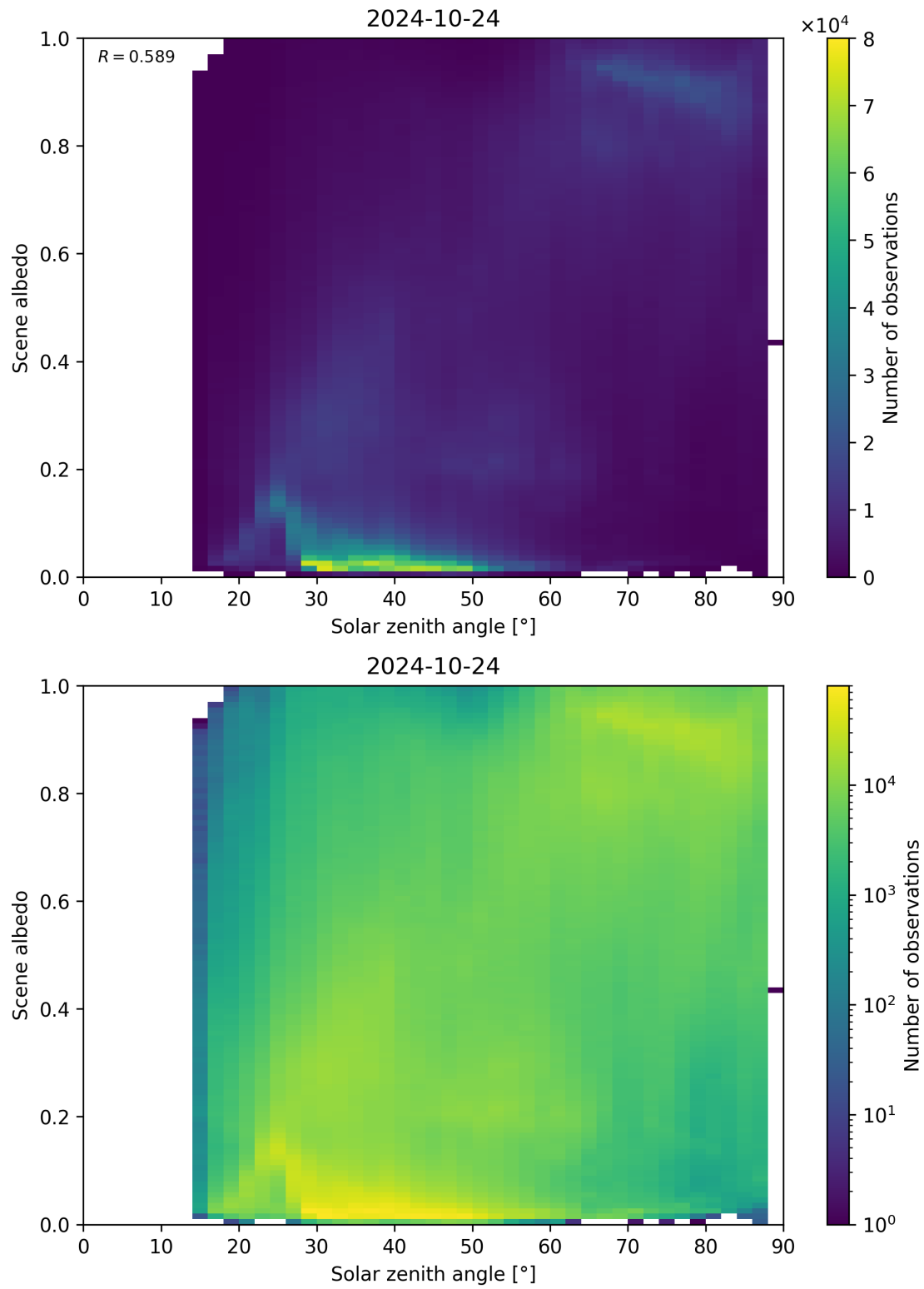
Figure 127: Scatter density plot of “Solar zenith angle” against “Scene albedo” for 2024-10-24 to 2024-10-25.
