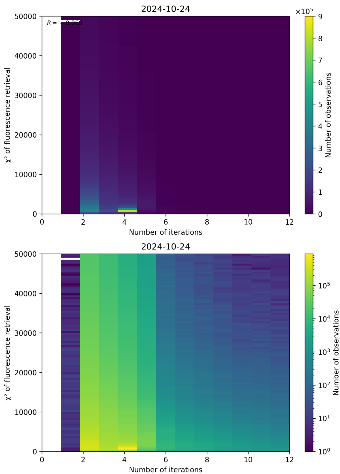
Figure 106: Scatter density plot of “Number of iterations” against “ \chi^2 of fluorescence retrieval” for 2024-10-24 to 2024-10-25.
