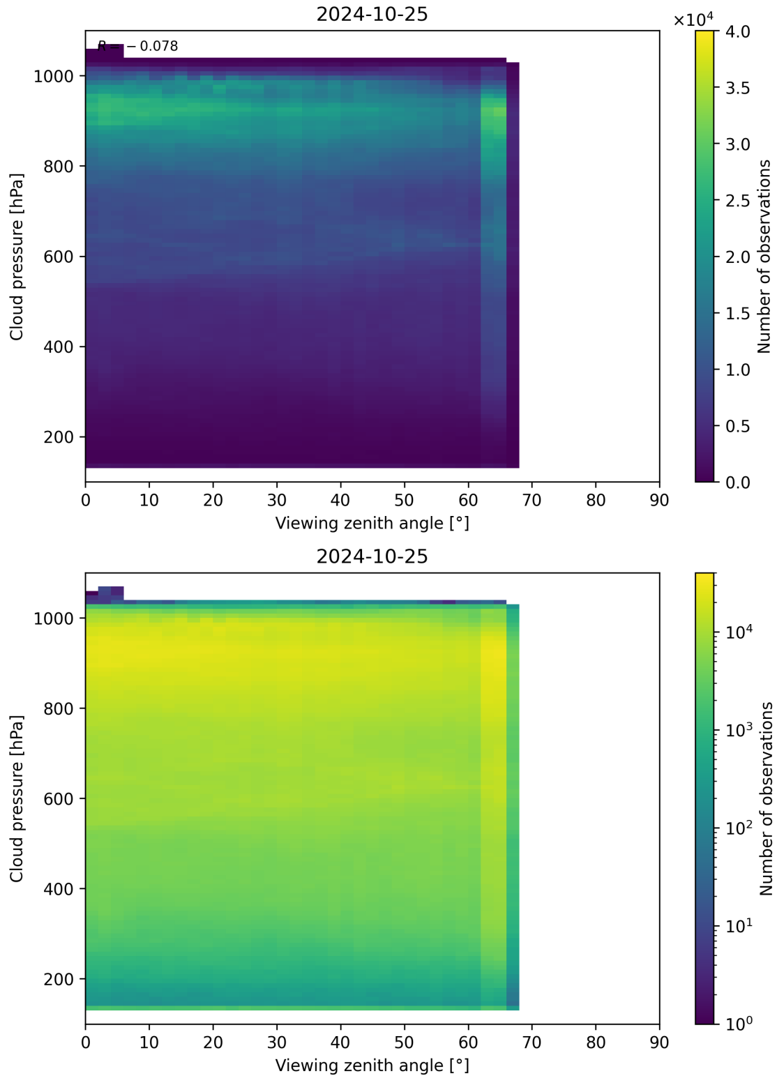
Figure 133: Scatter density plot of “Viewing zenith angle” against “Cloud pressure” for 2024-10-24 to 2024-10-26.
