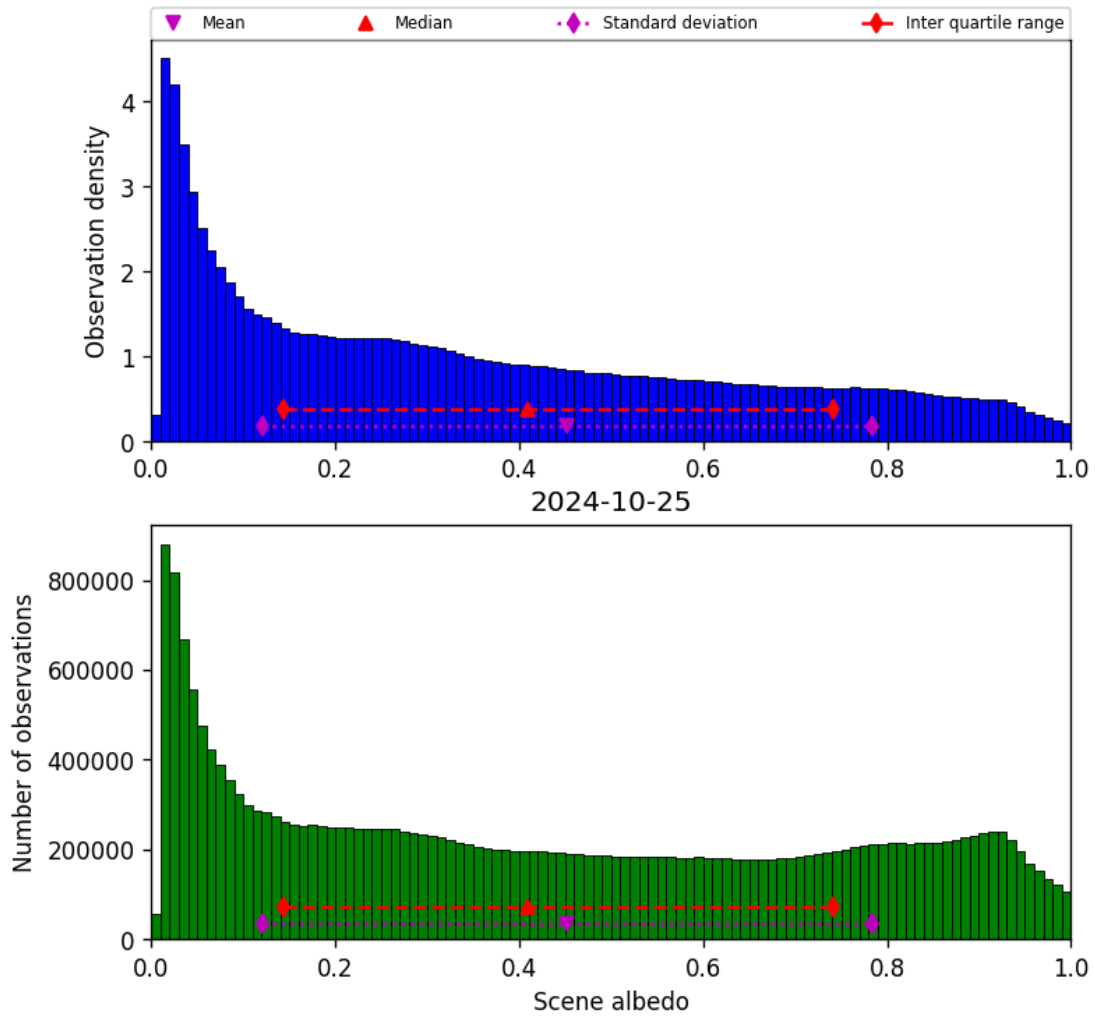
Figure 34: Histogram of “Scene albedo” for 2024-10-24 to 2024-10-26
