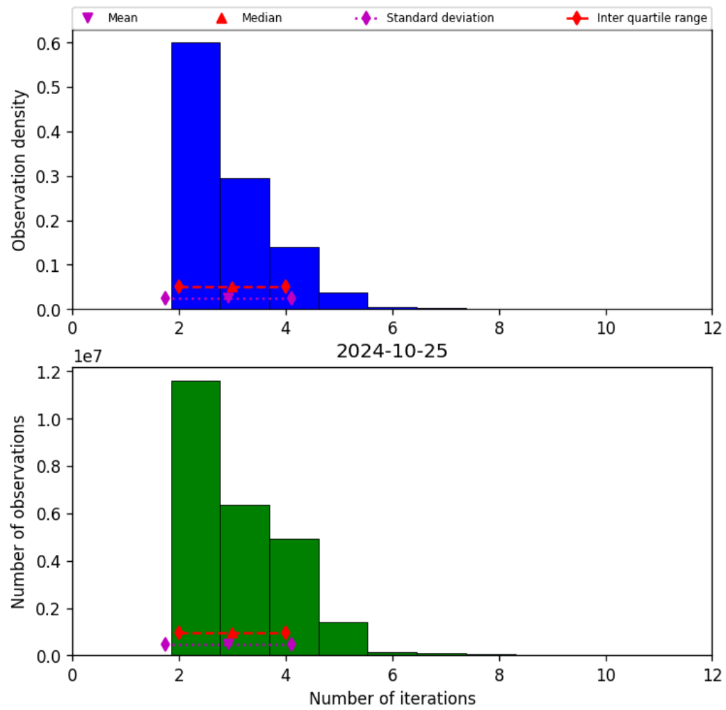
Figure 39: Histogram of “Number of iterations” for 2024-10-24 to 2024-10-26
