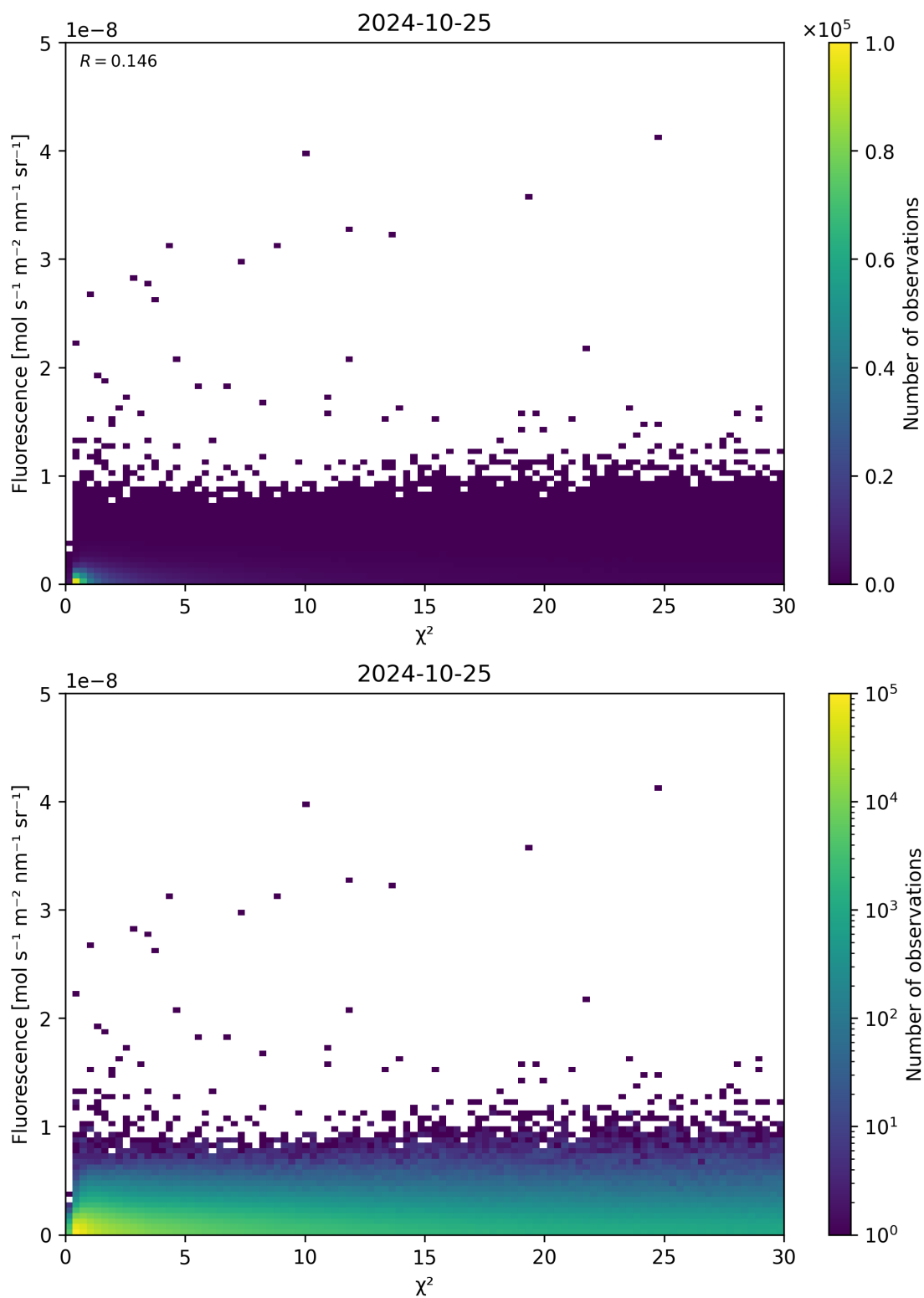
Figure 70: Scatter density plot of “ \chi^2 ” against “Fluorescence” for 2024-10-24 to 2024-10-26.
