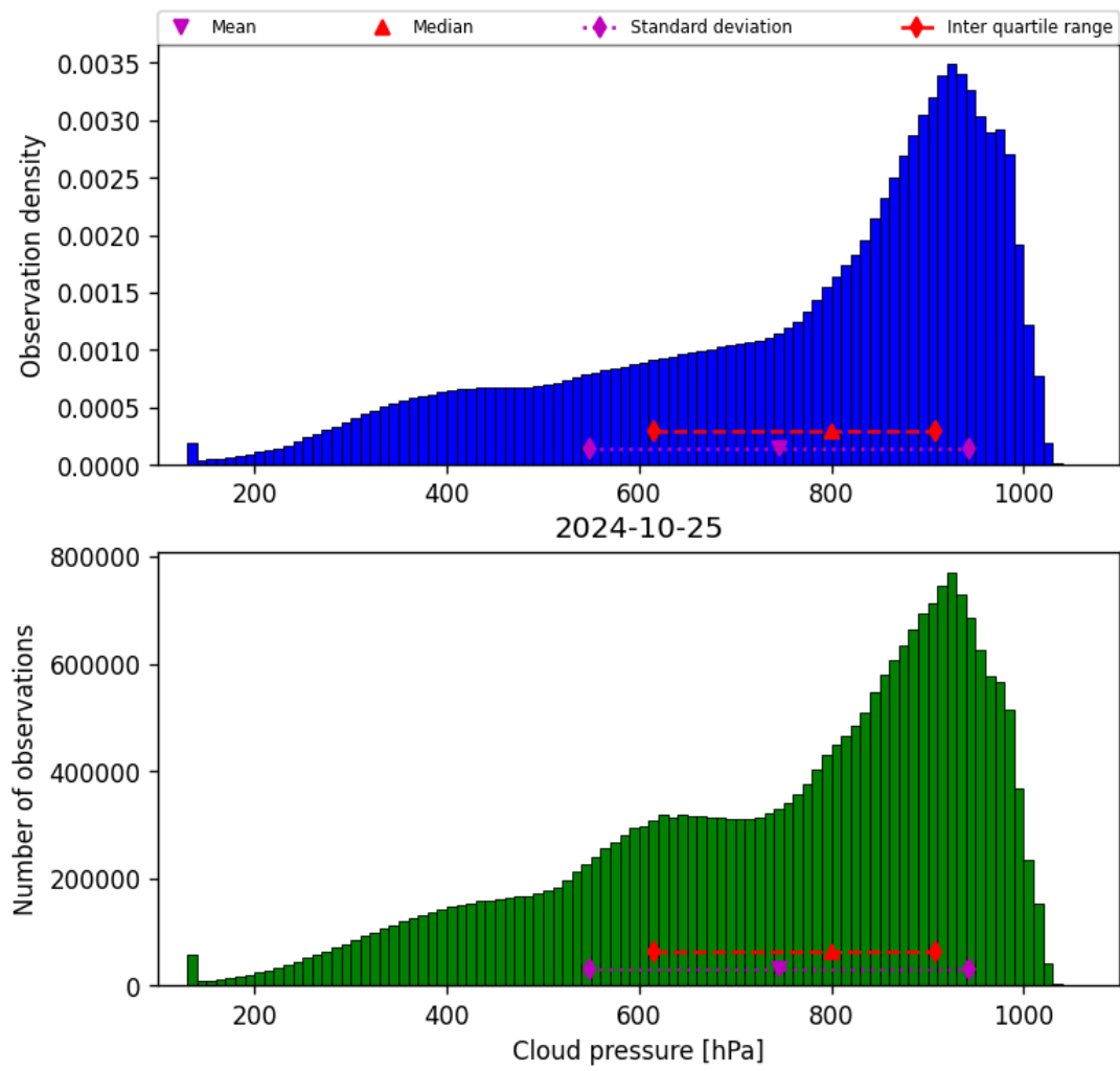
Figure 30: Histogram of “Cloud pressure” for 2024-10-24 to 2024-10-26
