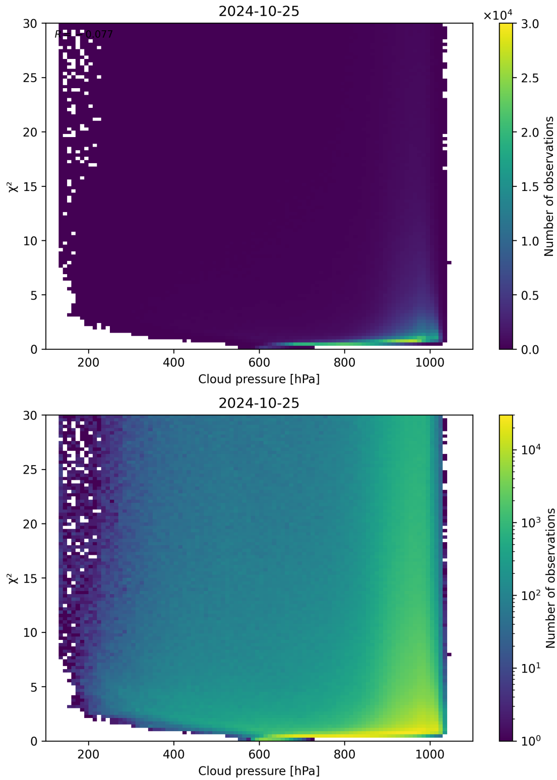
Figure 85: Scatter density plot of “Cloud pressure” against “ \chi^2 ” for 2024-10-24 to 2024-10-26.
