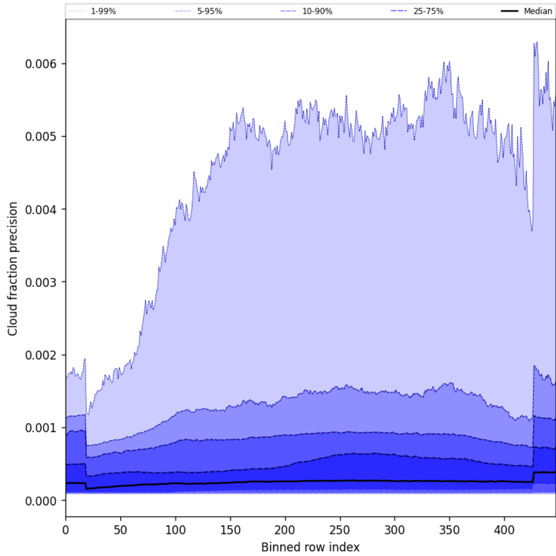
Figure 50: Along track statistics of “Cloud fraction precision” for 2024-10-24 to 2024-10-26
