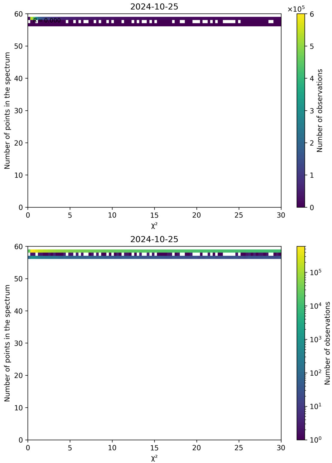
Figure 74: Scatter density plot of “ \chi^2 ” against “Number of points in the spectrum” for 2024-10-24 to 2024-10-26.
