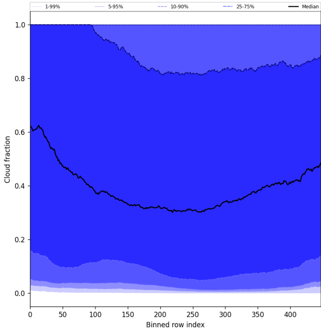
Figure 49: Along track statistics of “Cloud fraction” for 2024-10-24 to 2024-10-26
