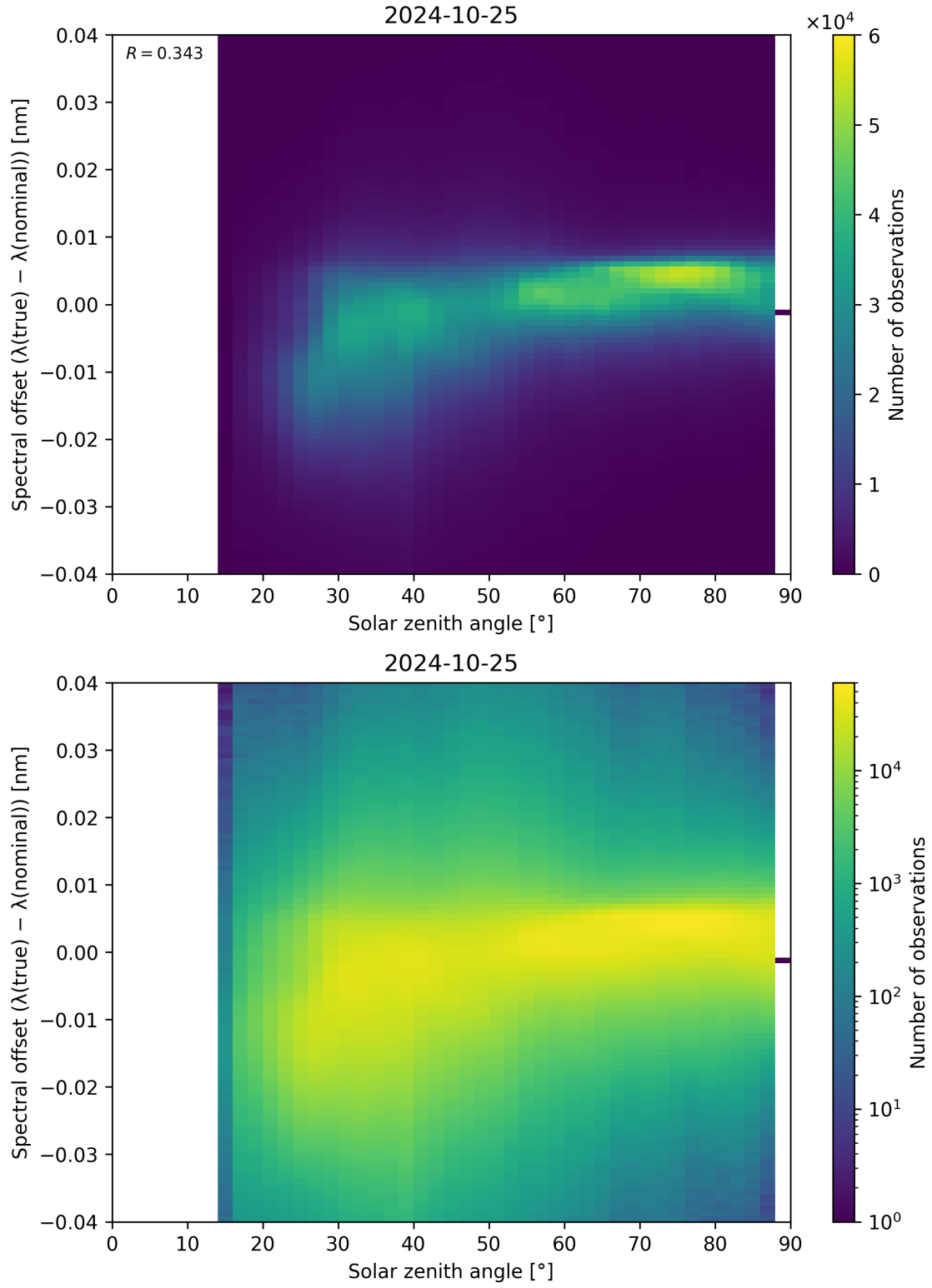
Figure 128: Scatter density plot of “Solar zenith angle” against “Spectral offset ( \lambda_{\text{true}} - \lambda_{\text{nominal}} )” for 2024-10-24 to 2024-10-26.
