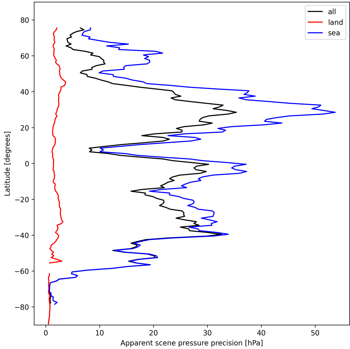
Figure 20: Zonal average of “Apparent scene pressure precision” for 2024-10-24 to 2024-10-26.
