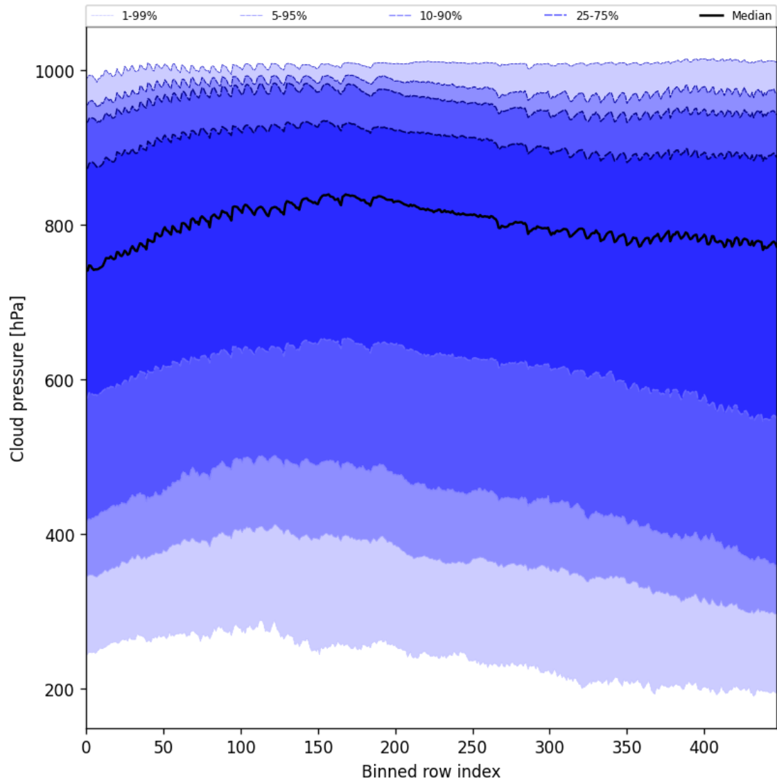
Figure 47: Along track statistics of “Cloud pressure” for 2024-10-24 to 2024-10-26
