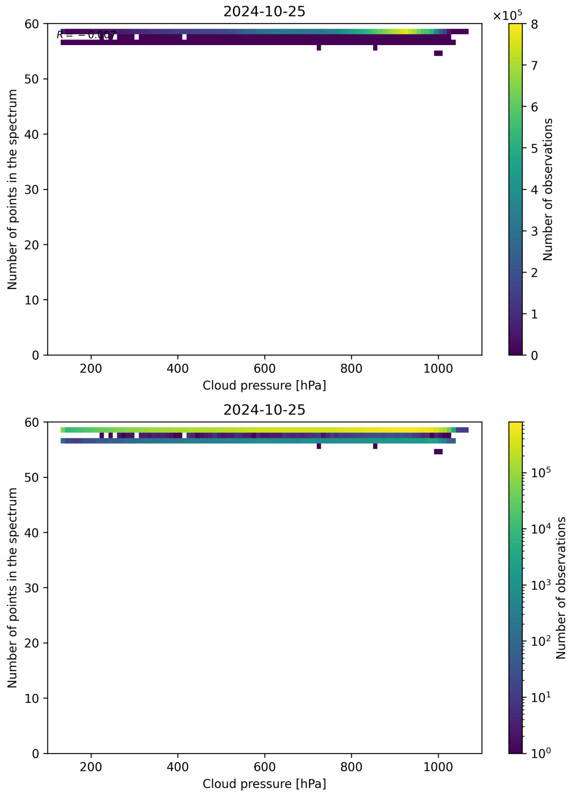
Figure 90: Scatter density plot of “Cloud pressure” against “Number of points in the spectrum” for 2024-10-24 to 2024-10-26.
