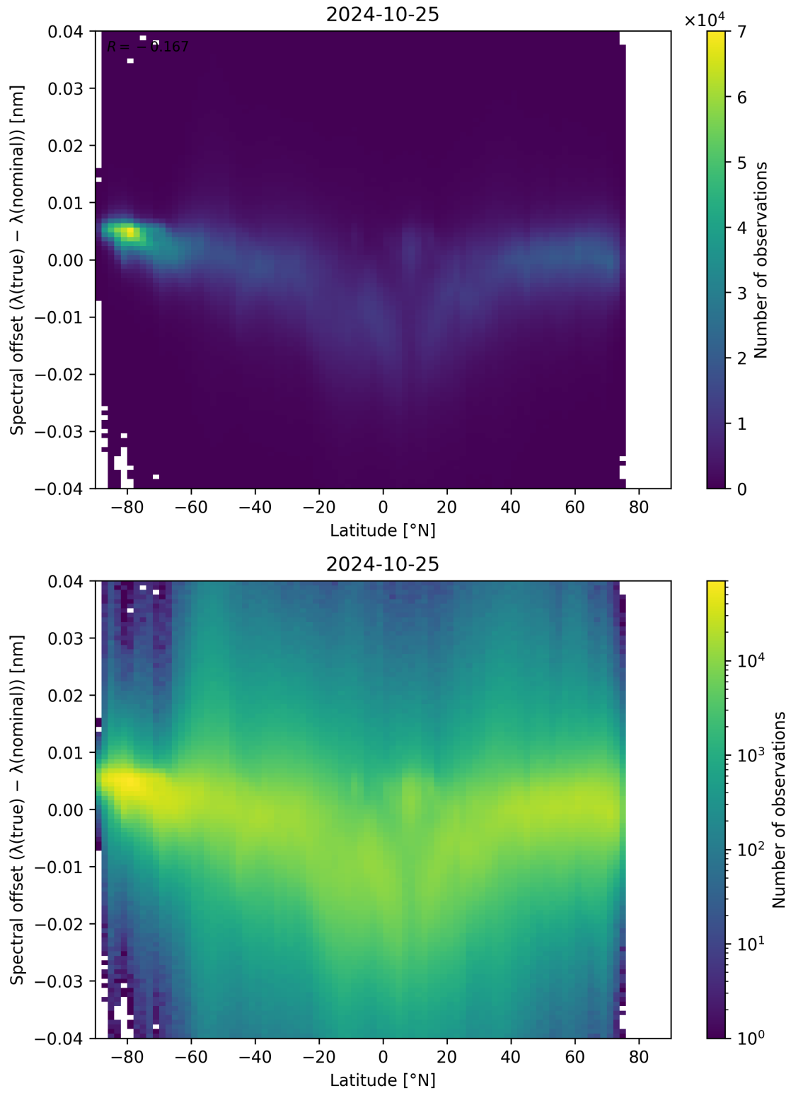
Figure 105: Scatter density plot of “Latitude” against “Spectral offset ( \lambda_{\text{true}} - \lambda_{\text{nominal}} )” for 2024-10-24 to 2024-10-26.
