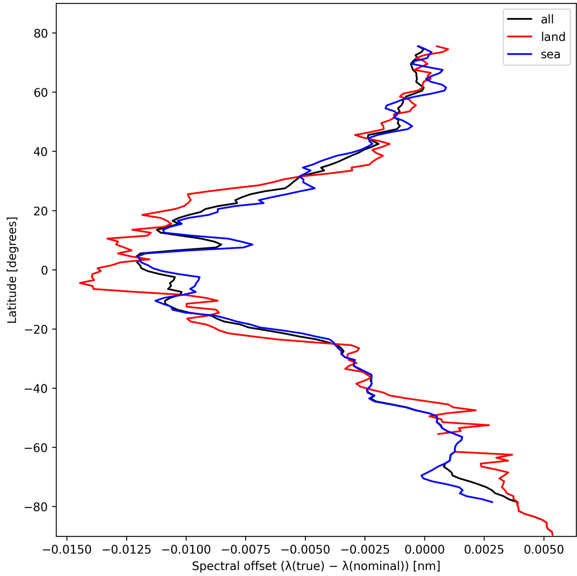
Figure 28: Zonal average of “Spectral offset ( \lambda_{\text{true}} - \lambda_{\text{nominal}} )” for 2024-10-24 to 2024-10-26.
