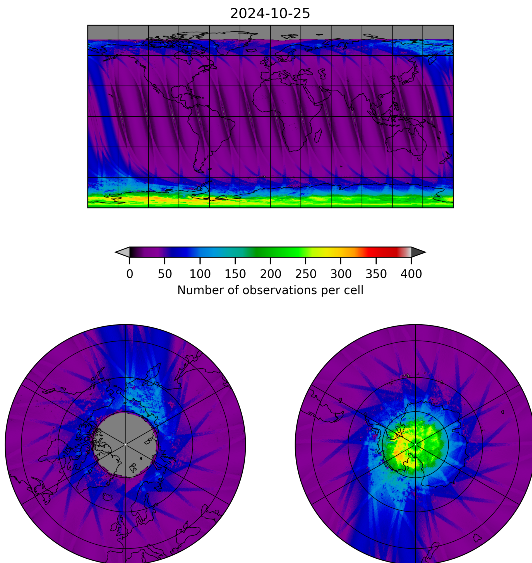
Figure 11: Map of the number of observations for 2024-10-24 to 2024-10-26
