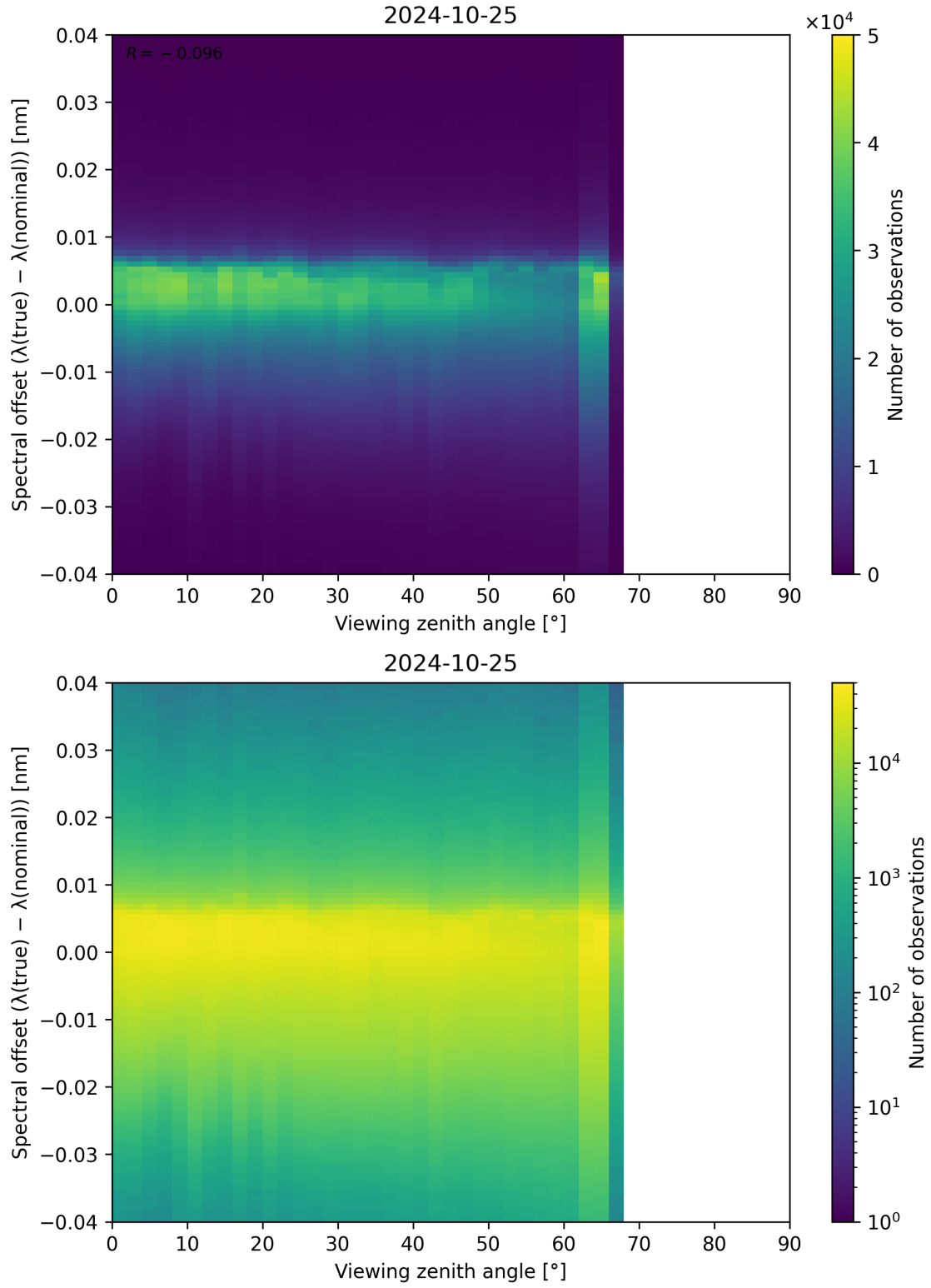
Figure 140: Scatter density plot of “Viewing zenith angle” against “Spectral offset ( \lambda_{\text{true}} - \lambda_{\text{nominal}} )” for 2024-10-24 to 2024-10-26.
