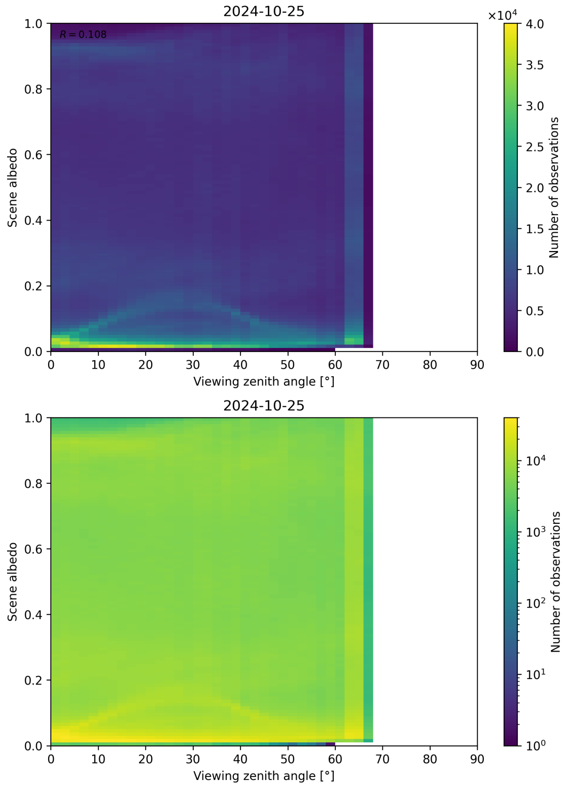
Figure 138: Scatter density plot of “Viewing zenith angle” against “Scene albedo” for 2024-10-24 to 2024-10-26.
