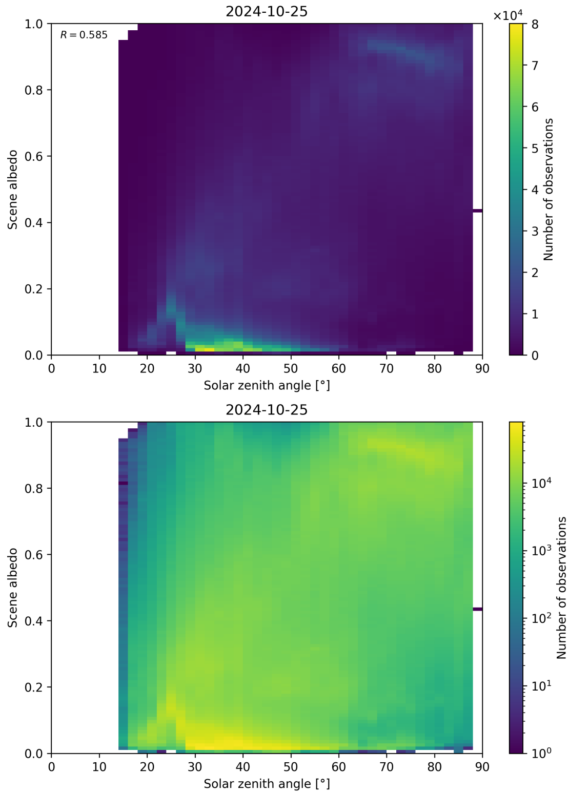
Figure 127: Scatter density plot of “Solar zenith angle” against “Scene albedo” for 2024-10-24 to 2024-10-26.
