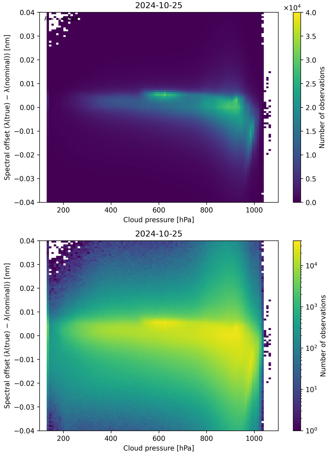
Figure 92: Scatter density plot of “Cloud pressure” against “Spectral offset ( \lambda_{\text{true}} - \lambda_{\text{nominal}} )” for 2024-10-24 to 2024-10-26.
