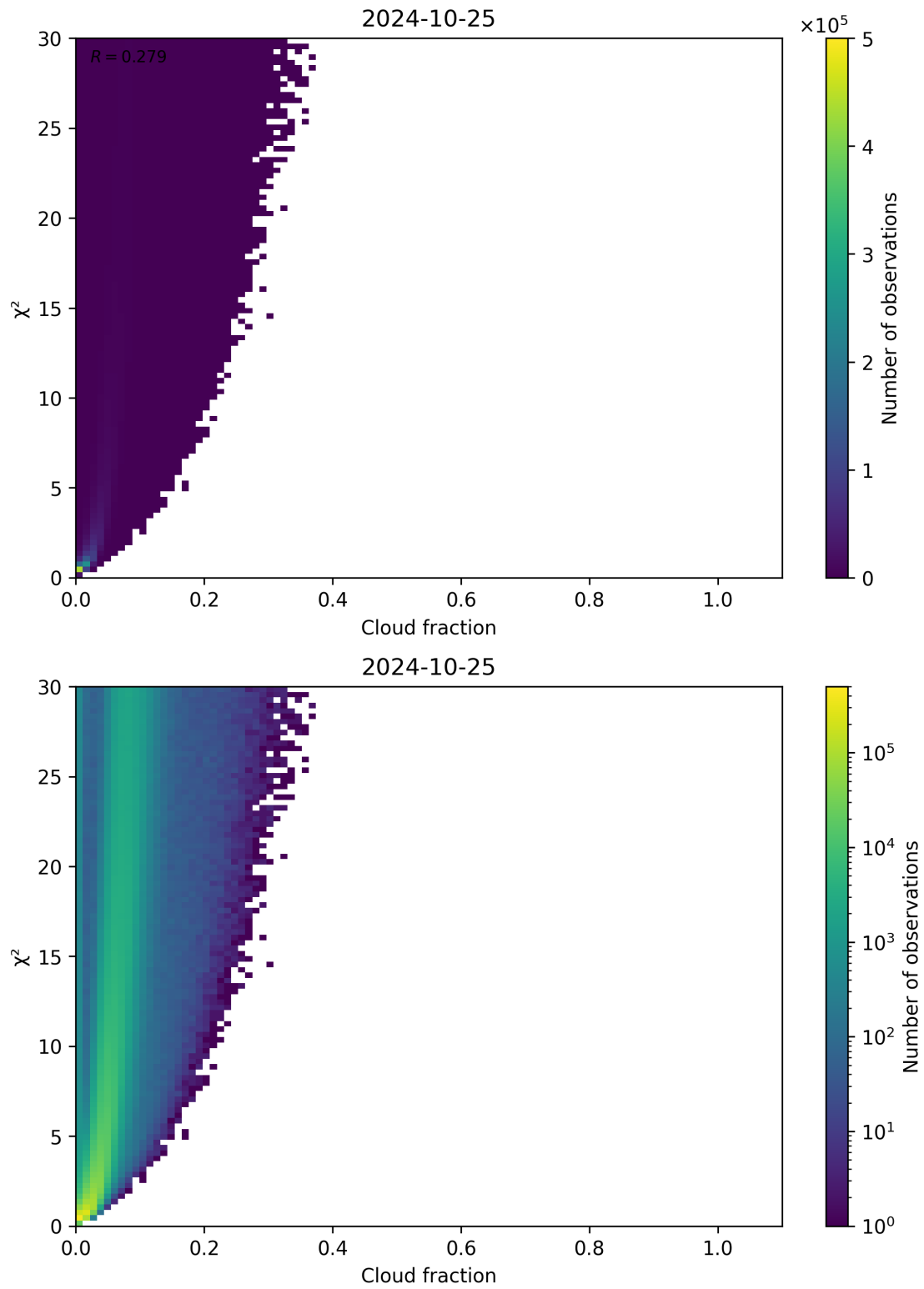
Figure 77: Scatter density plot of “Cloud fraction” against “ \chi^2 ” for 2024-10-24 to 2024-10-26.
