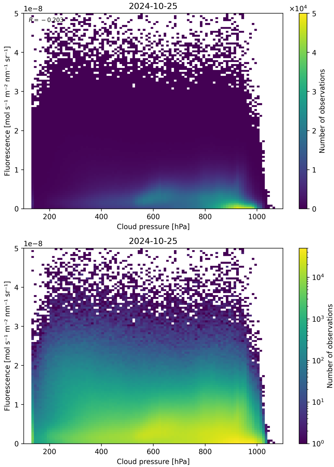
Figure 88: Scatter density plot of “Cloud pressure” against “Fluorescence” for 2024-10-24 to 2024-10-26.
