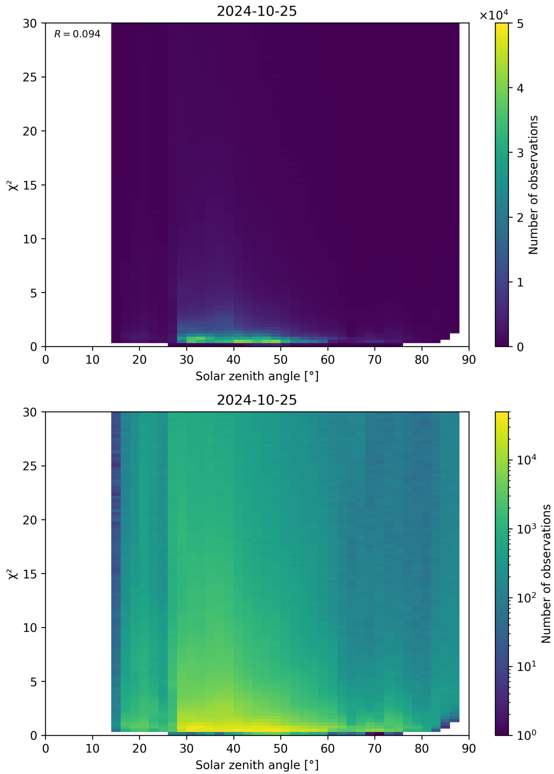
Figure 119: Scatter density plot of “Solar zenith angle” against “ \chi^2 ” for 2024-10-24 to 2024-10-26.
