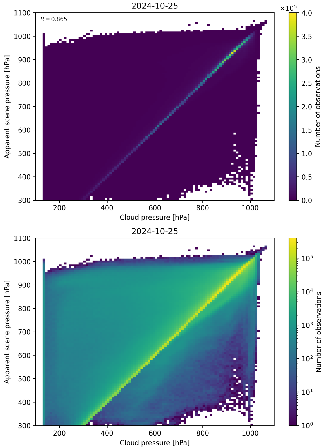
Figure 84: Scatter density plot of “Cloud pressure” against “Apparent scene pressure” for 2024-10-24 to 2024-10-26.
