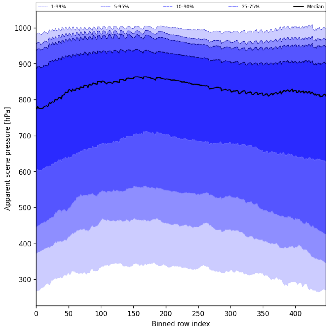
Figure 53: Along track statistics of “Apparent scene pressure” for 2024-10-24 to 2024-10-26
