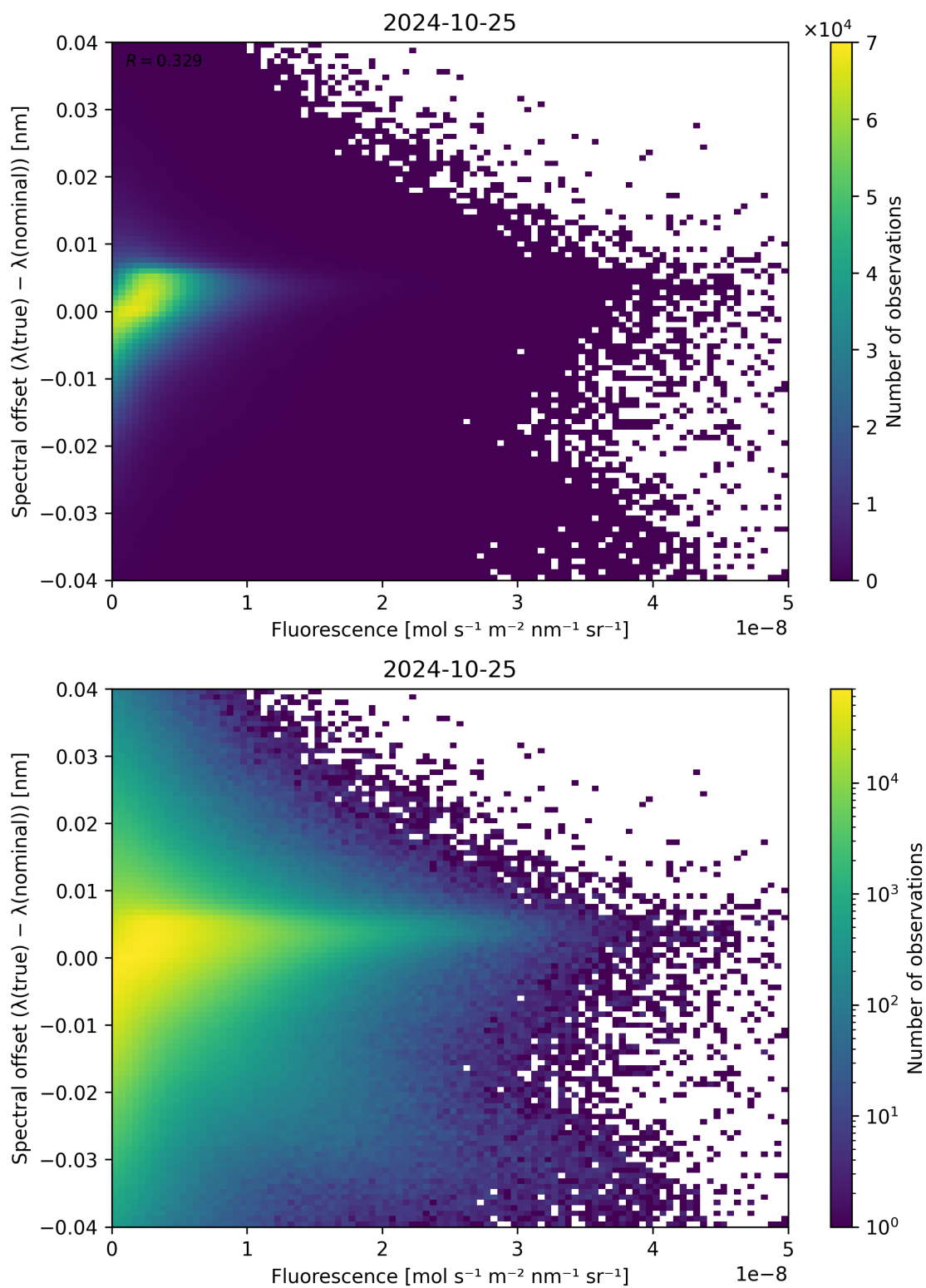
Figure 95: Scatter density plot of “Fluorescence” against “Spectral offset ( \lambda_{\text{true}} - \lambda_{\text{nominal}} )” for 2024-10-24 to 2024-10-26.
