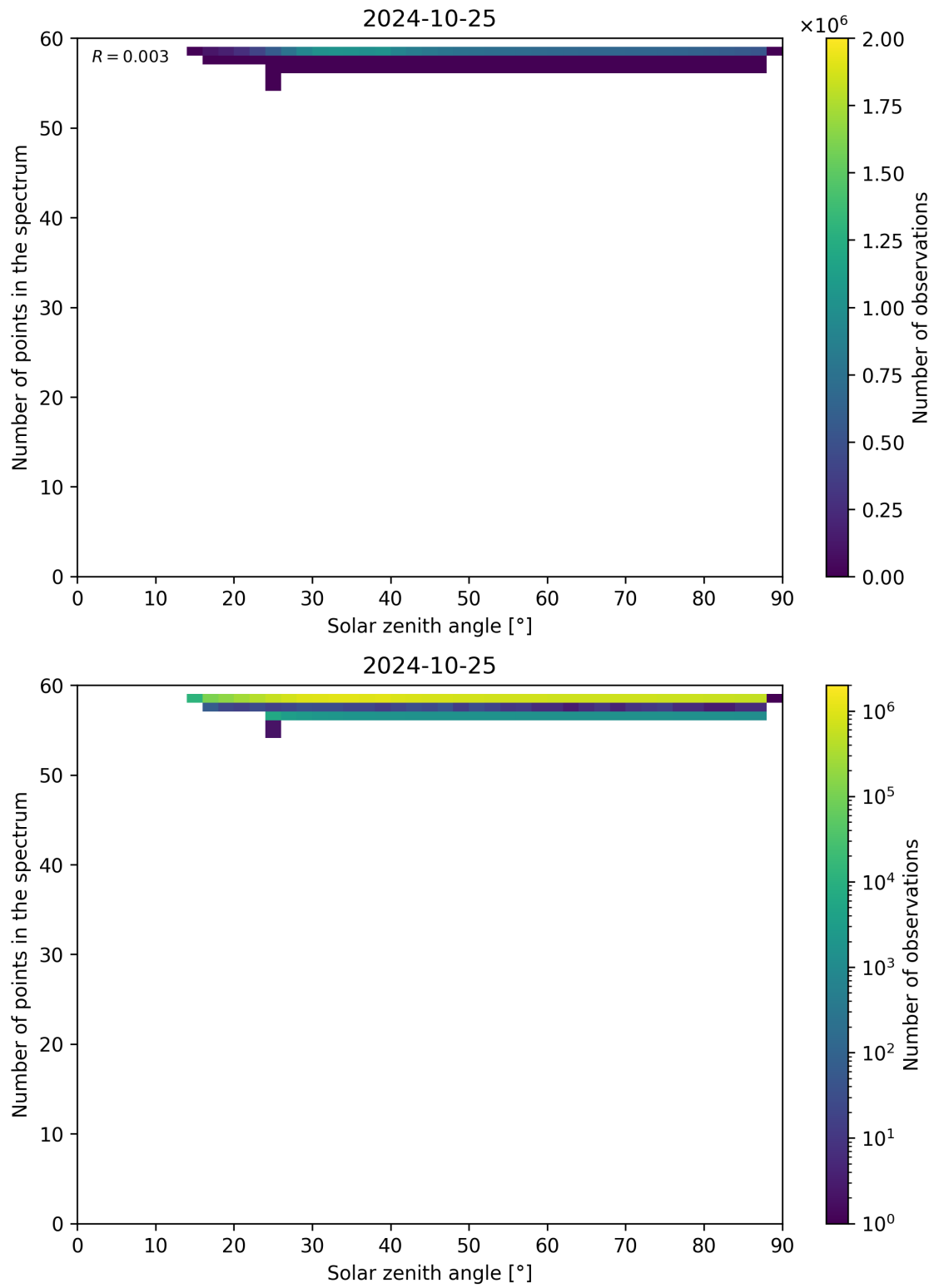
Figure 126: Scatter density plot of “Solar zenith angle” against “Number of points in the spectrum” for 2024-10-24 to 2024-10-26.
