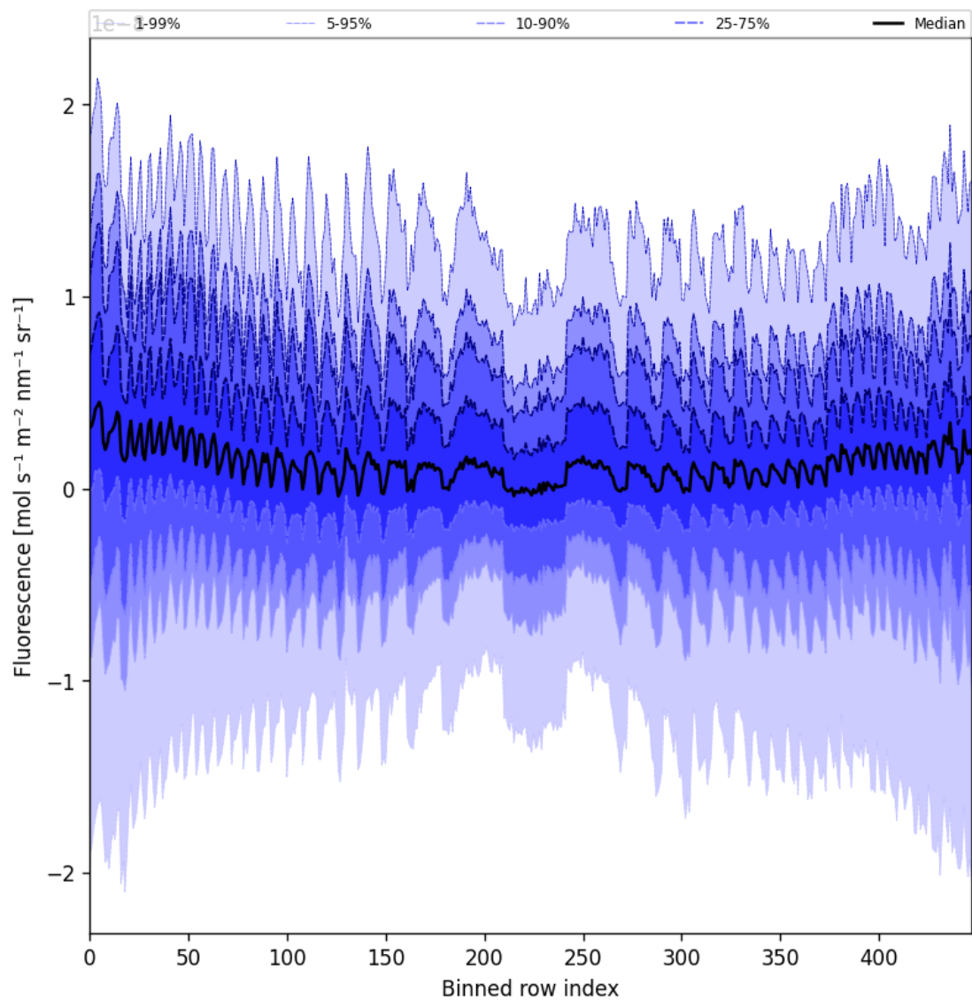
Figure 57: Along track statistics of “Fluorescence” for 2024-10-24 to 2024-10-26
