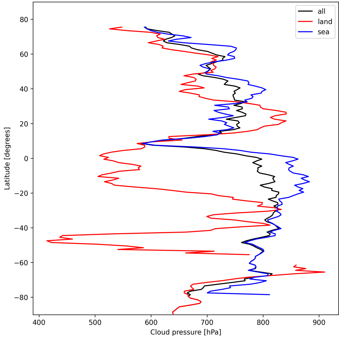
Figure 13: Zonal average of “Cloud pressure” for 2024-10-24 to 2024-10-26.
