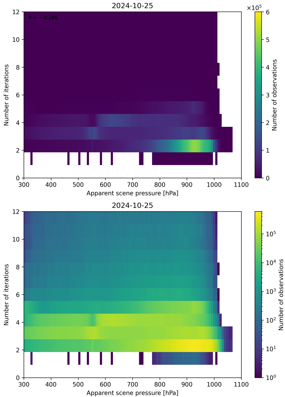
Figure 66: Scatter density plot of “Apparent scene pressure” against “Number of iterations” for 2024-10-24 to 2024-10-26.
