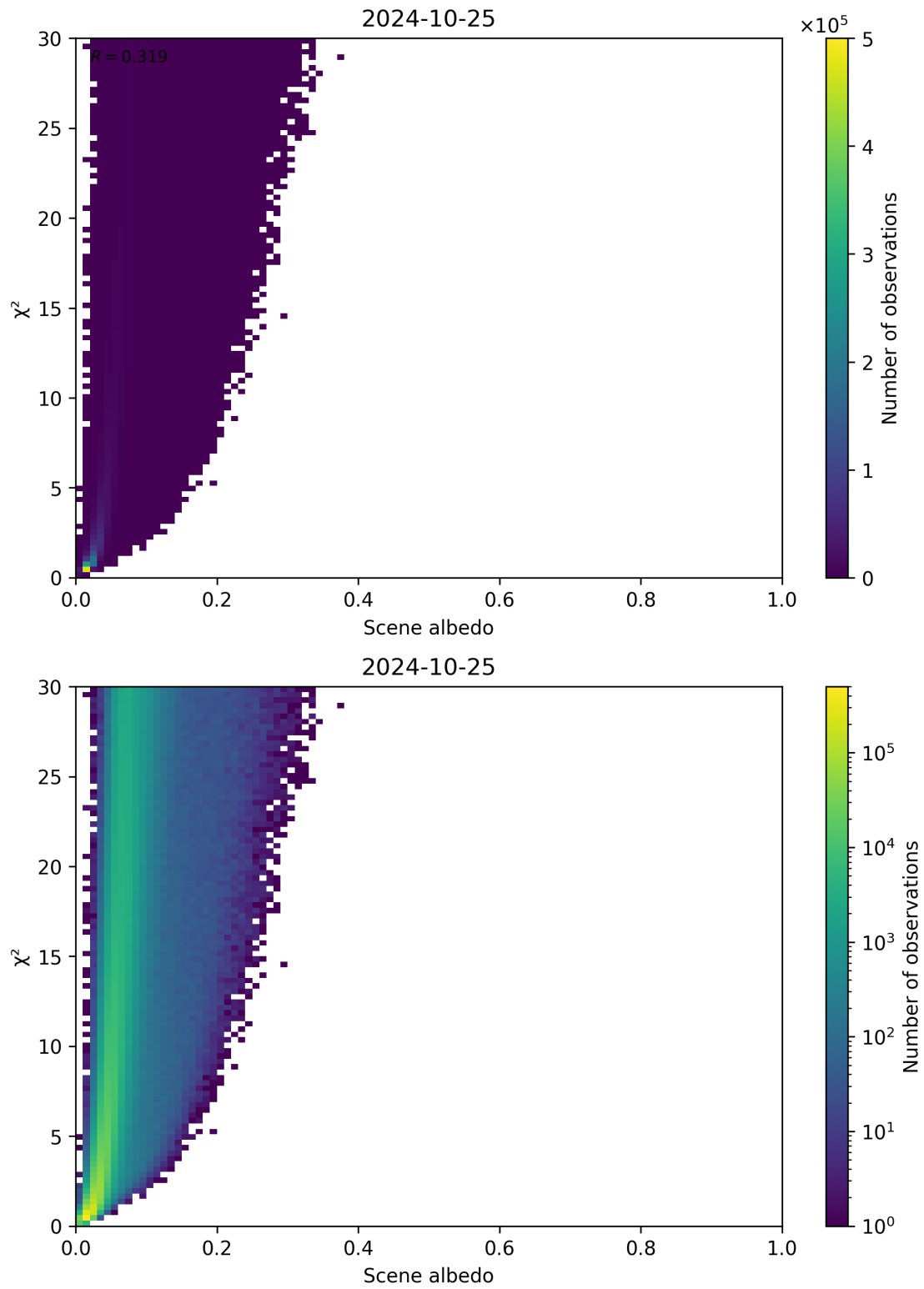
Figure 112: Scatter density plot of “Scene albedo” against “ \chi^2 ” for 2024-10-24 to 2024-10-26.
