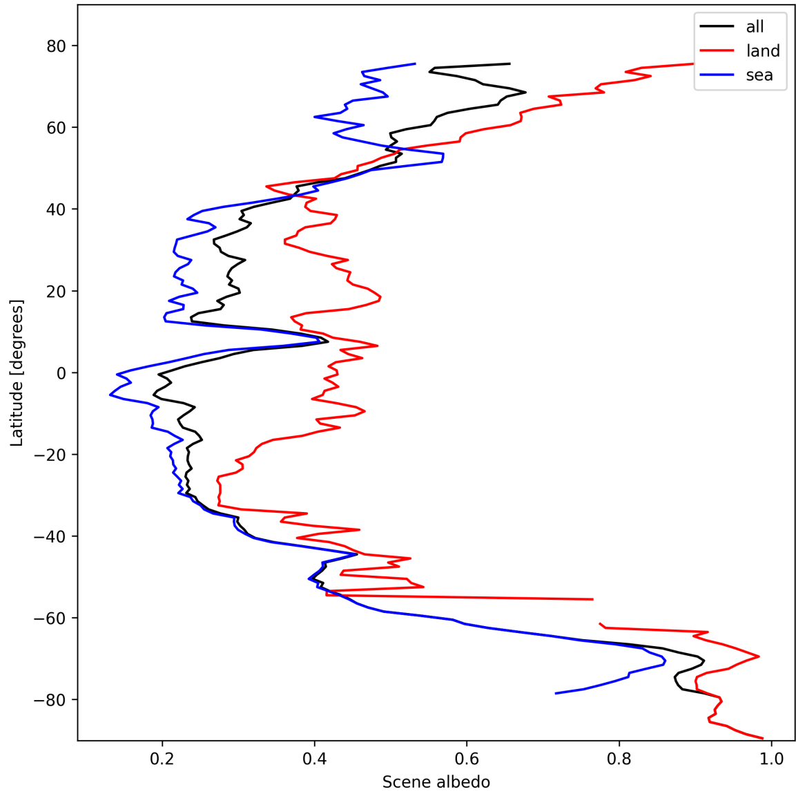
Figure 17: Zonal average of “Scene albedo” for 2024-10-24 to 2024-10-26.
