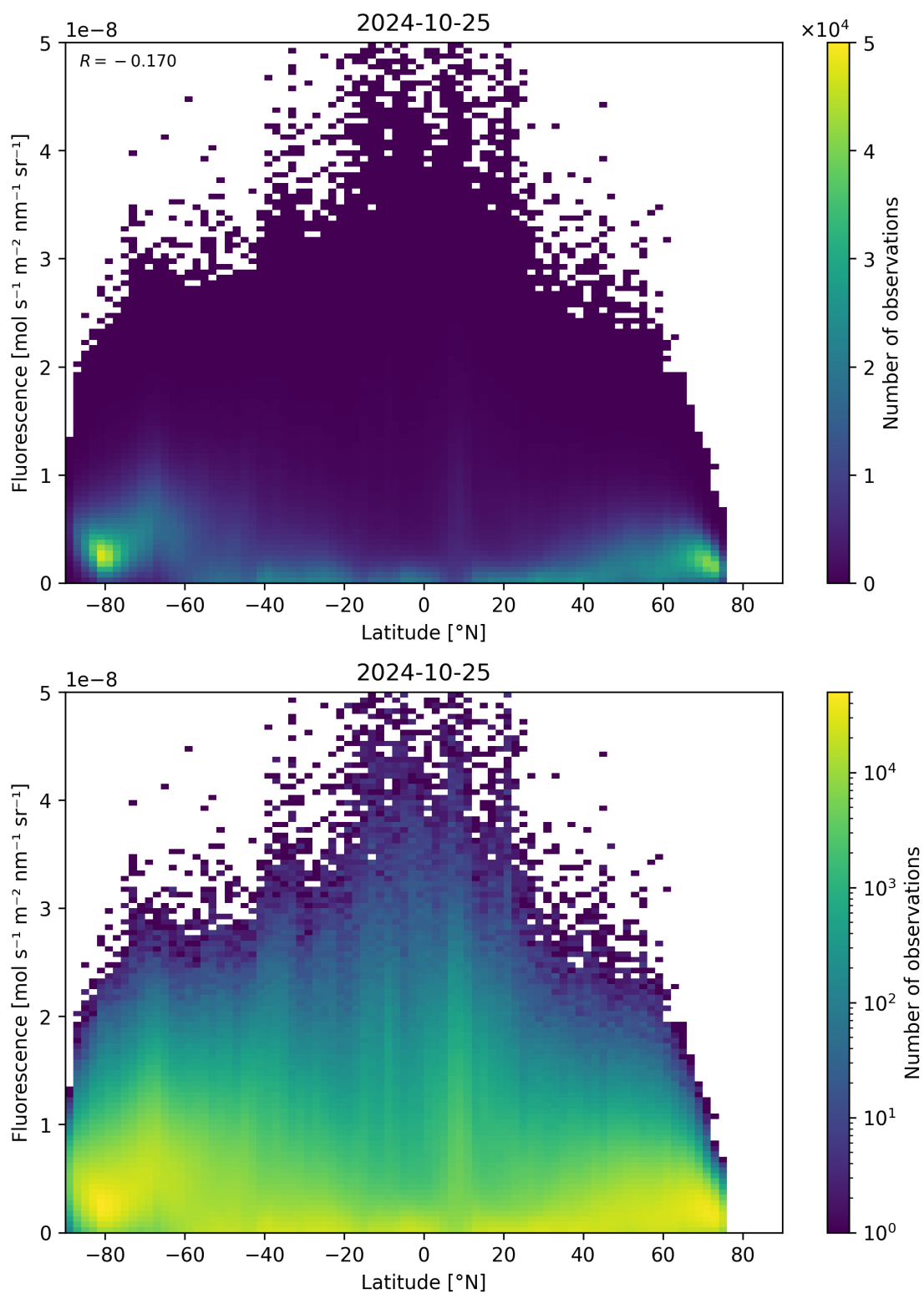
Figure 101: Scatter density plot of “Latitude” against “Fluorescence” for 2024-10-24 to 2024-10-26.
