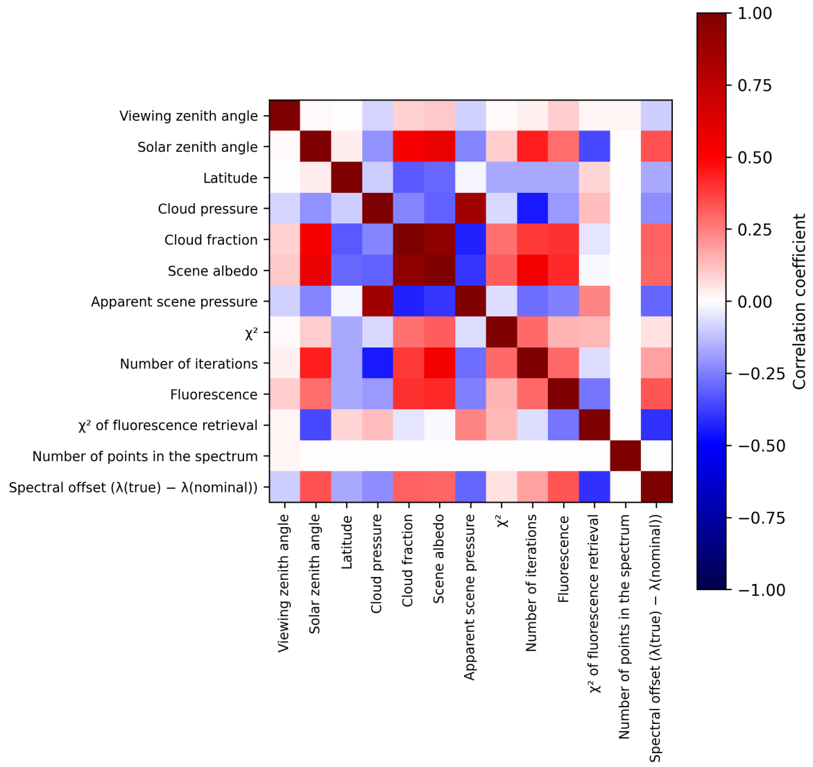
Figure 2: Map of correlation matrix for 2024-10-24 to 2024-10-26.
