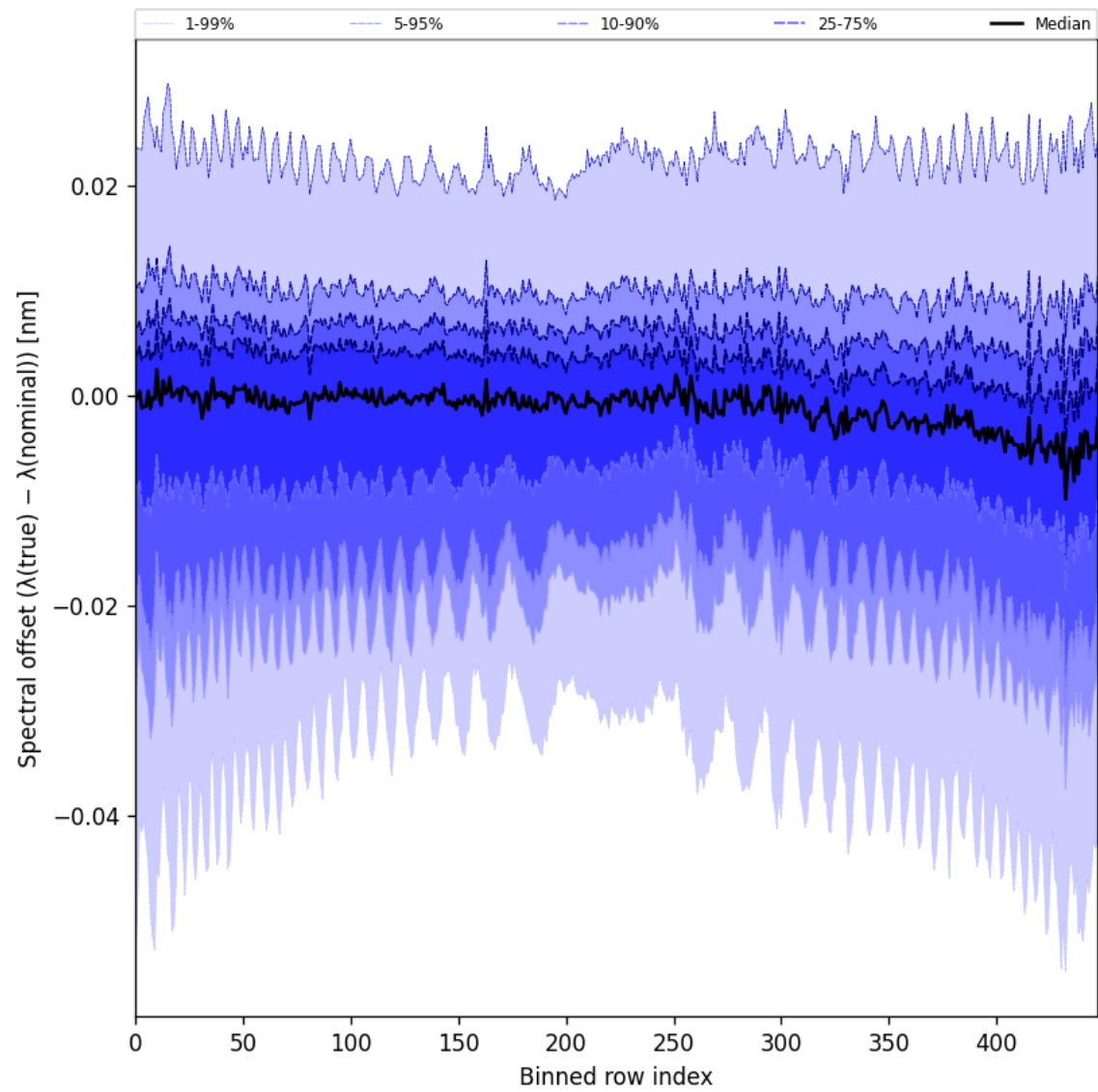
Figure 62: Along track statistics of “Spectral offset ( \lambda_{\text{true}} - \lambda_{\text{nominal}} )” for 2024-10-24 to 2024-10-26
