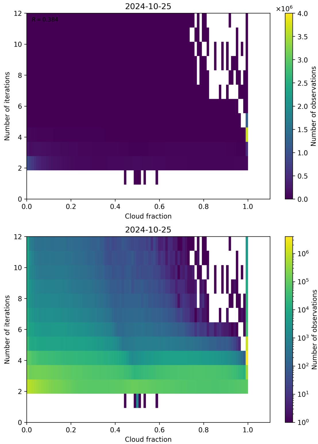
Figure 80: Scatter density plot of “Cloud fraction” against “Number of iterations” for 2024-10-24 to 2024-10-26.
