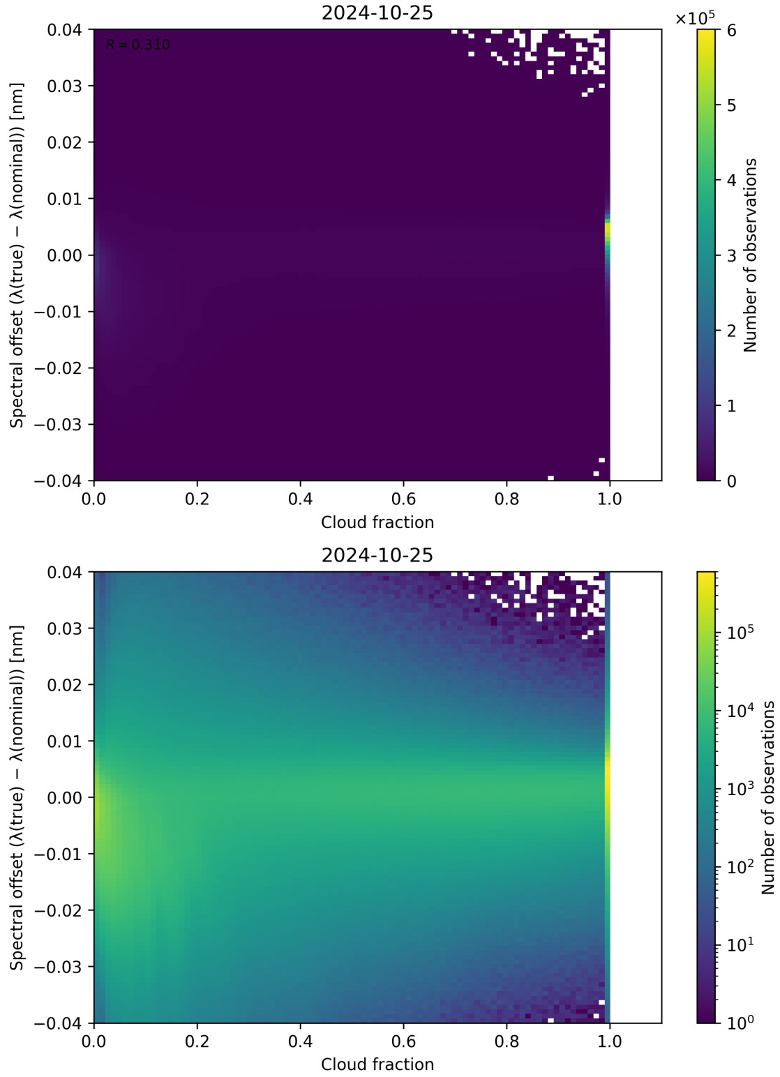
Figure 83: Scatter density plot of “Cloud fraction” against “Spectral offset ( \lambda_{\text{true}} - \lambda_{\text{nominal}} )” for 2024-10-24 to 2024-10-26.
