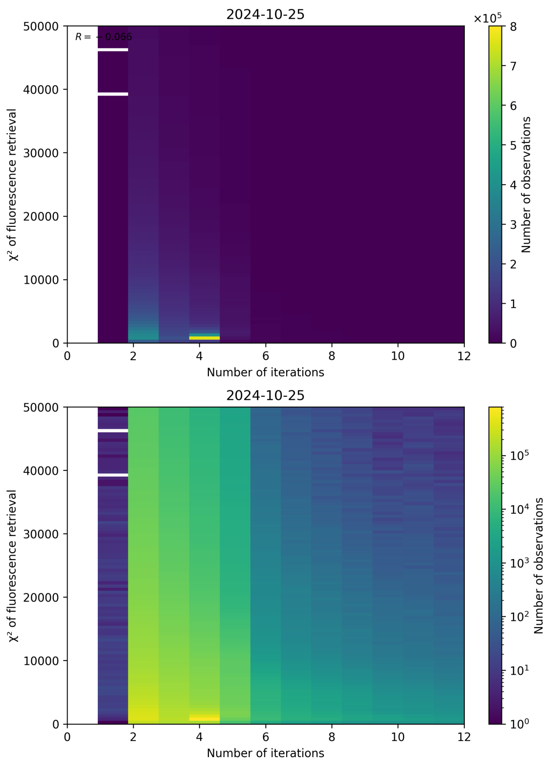
Figure 106: Scatter density plot of “Number of iterations” against “ \chi^2 of fluorescence retrieval” for 2024-10-24 to 2024-10-26.
