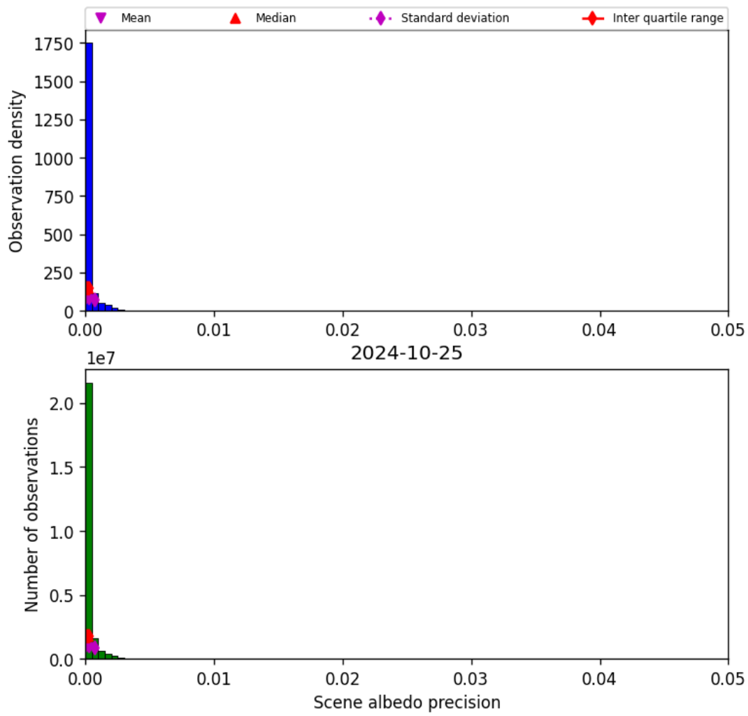
Figure 35: Histogram of “Scene albedo precision” for 2024-10-24 to 2024-10-26
