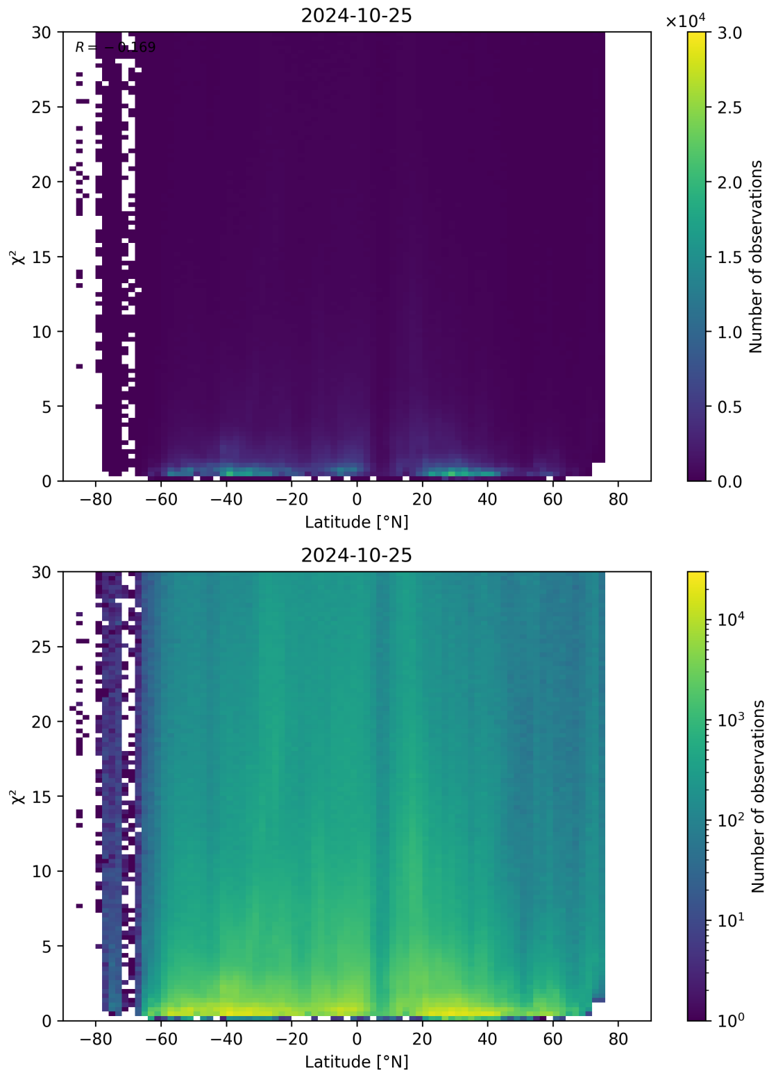
Figure 97: Scatter density plot of “Latitude” against “ \chi^2 ” for 2024-10-24 to 2024-10-26.
