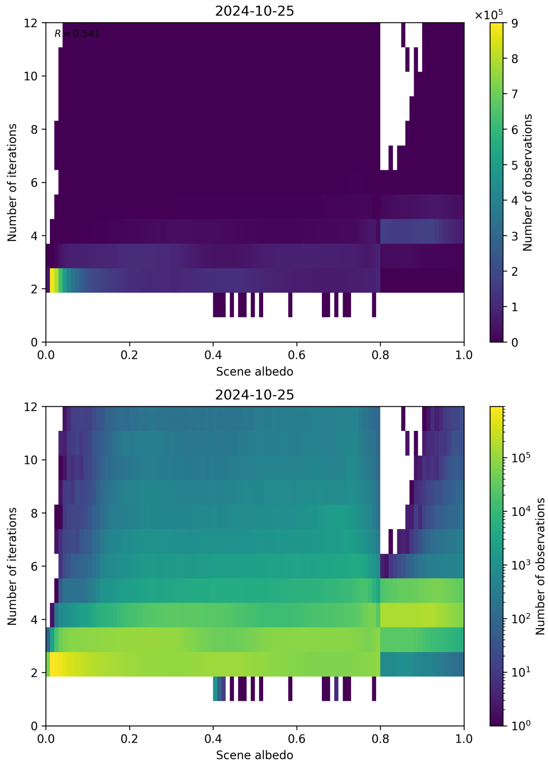
Figure 115: Scatter density plot of “Scene albedo” against “Number of iterations” for 2024-10-24 to 2024-10-26.
