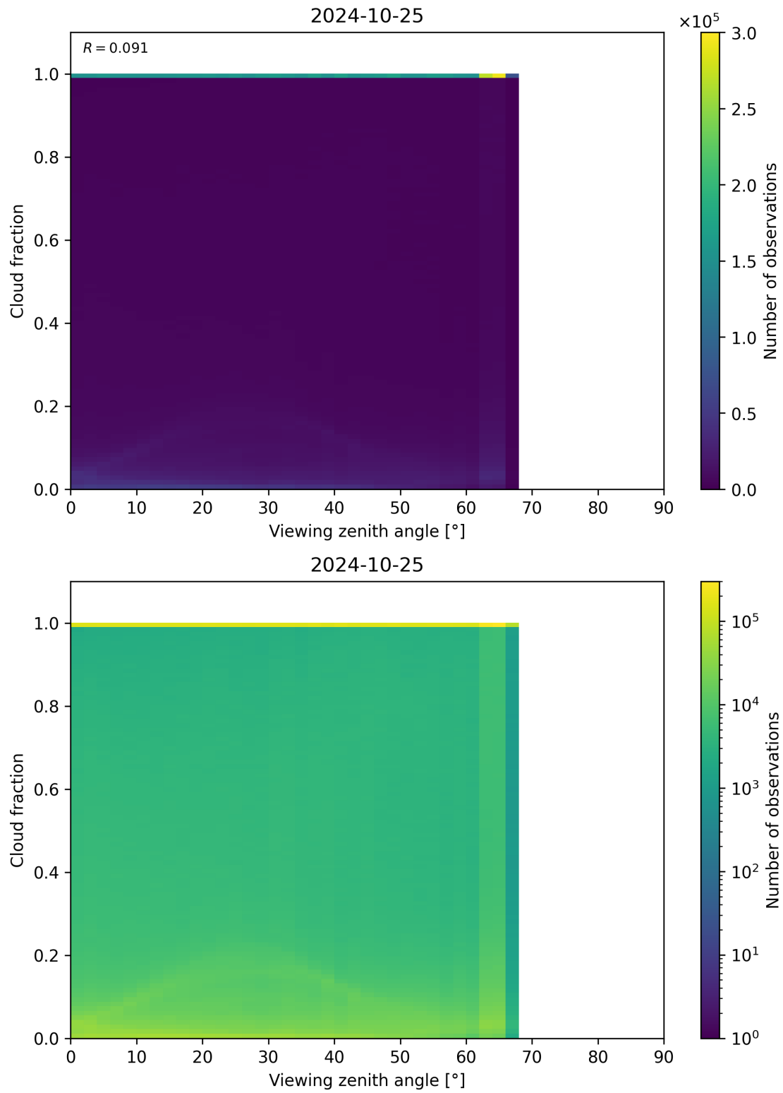
Figure 132: Scatter density plot of “Viewing zenith angle” against “Cloud fraction” for 2024-10-24 to 2024-10-26.
