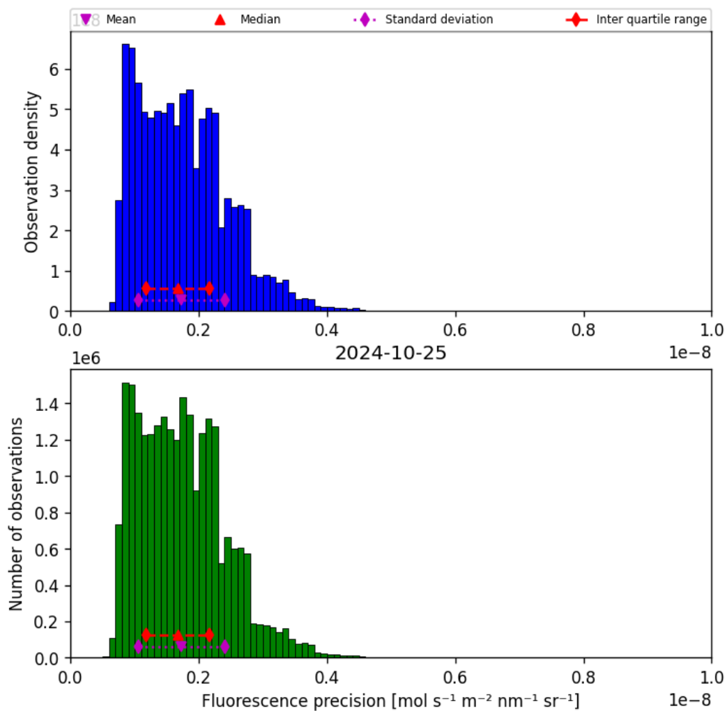
Figure 41: Histogram of “Fluorescence precision” for 2024-10-24 to 2024-10-26
