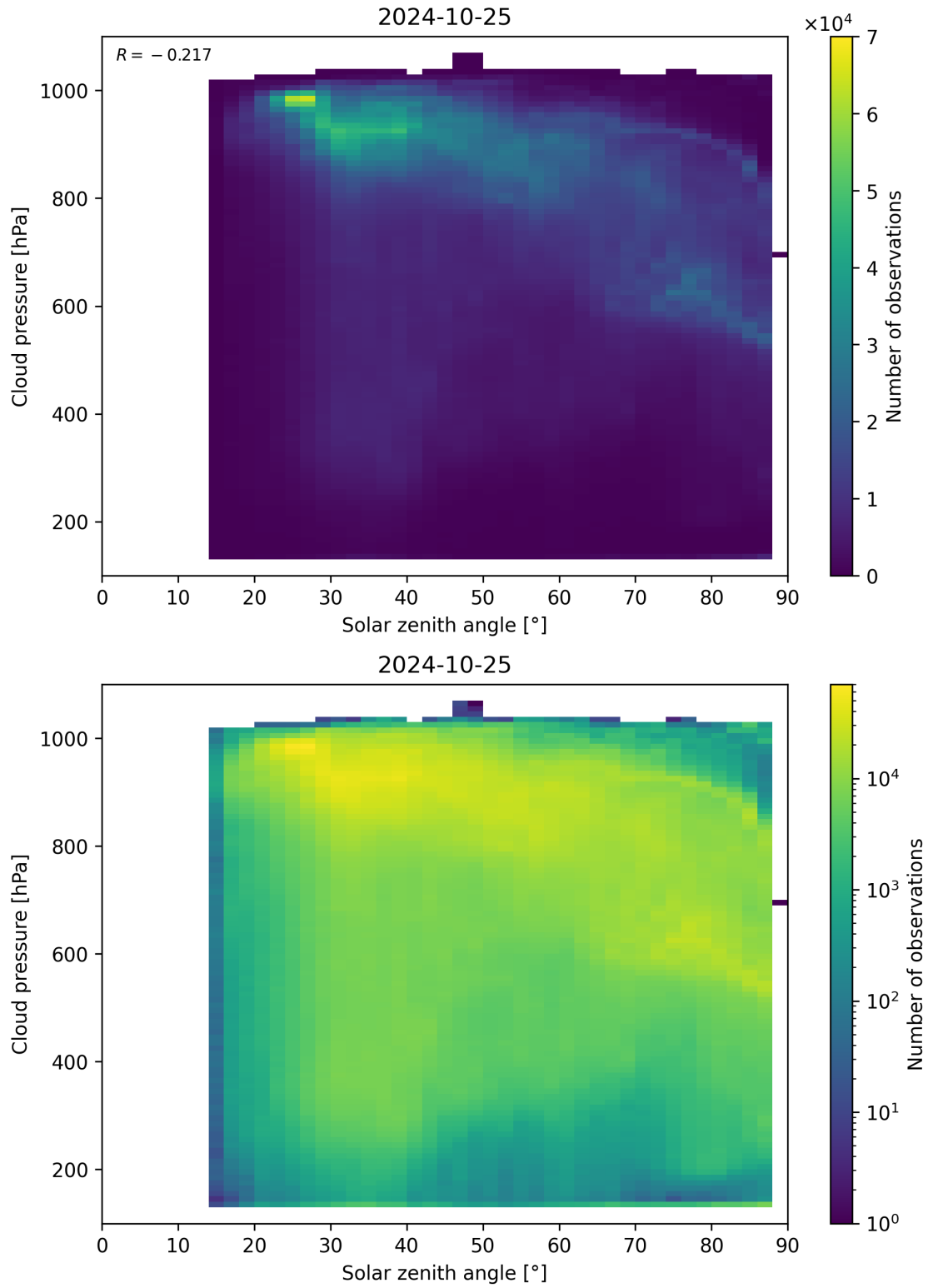
Figure 122: Scatter density plot of “Solar zenith angle” against “Cloud pressure” for 2024-10-24 to 2024-10-26.
