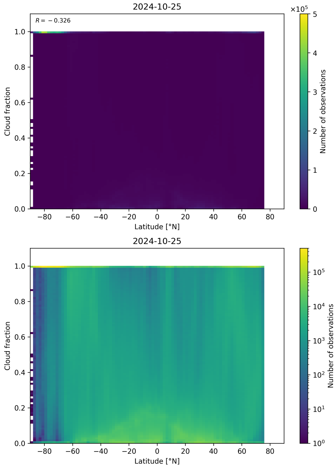
Figure 99: Scatter density plot of “Latitude” against “Cloud fraction” for 2024-10-24 to 2024-10-26.
