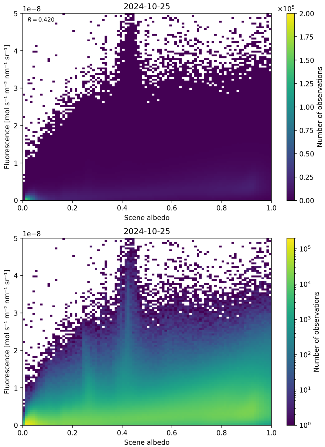
Figure 114: Scatter density plot of “Scene albedo” against “Fluorescence” for 2024-10-24 to 2024-10-26.
