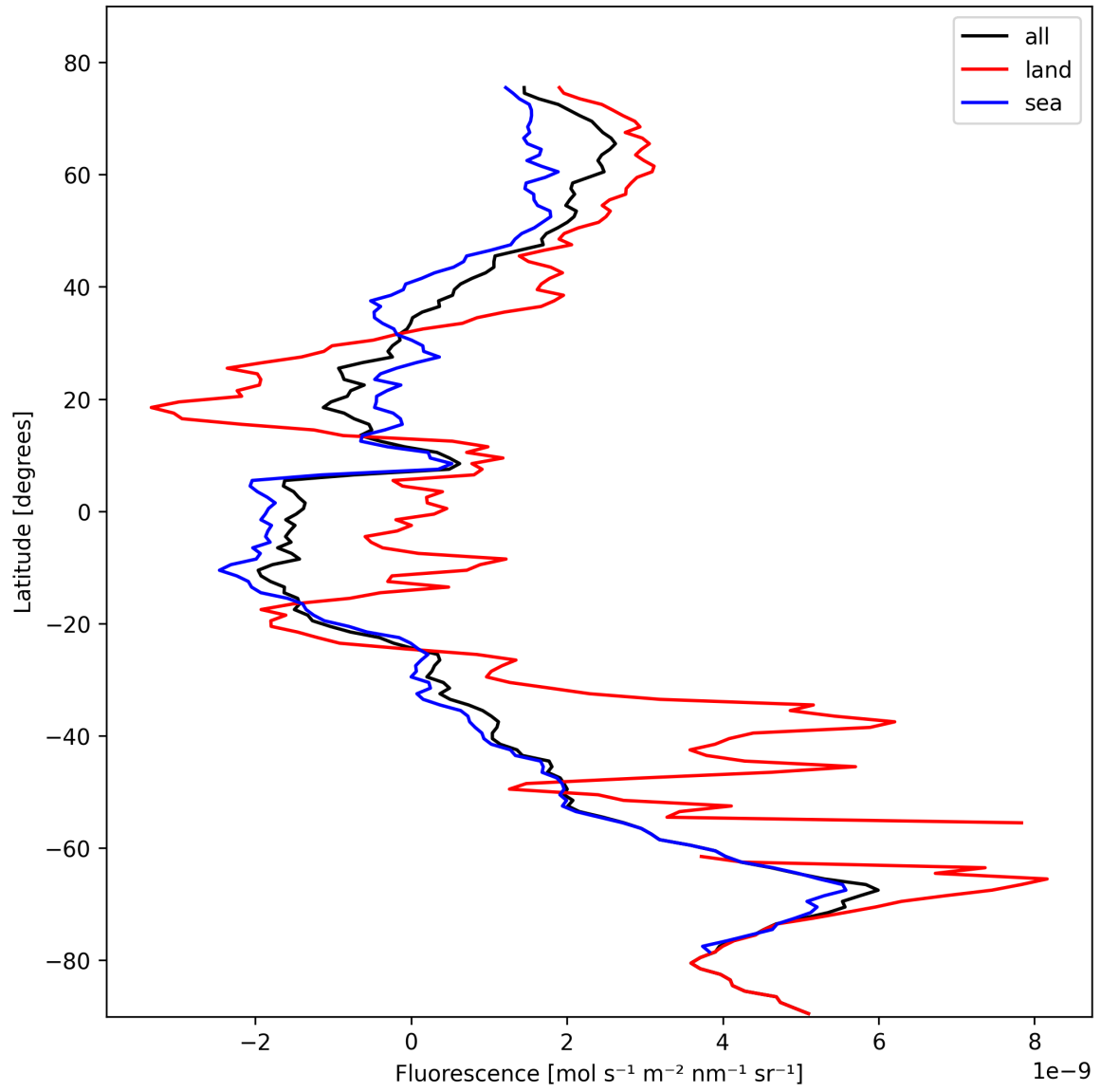
Figure 23: Zonal average of “Fluorescence” for 2024-10-24 to 2024-10-26.
