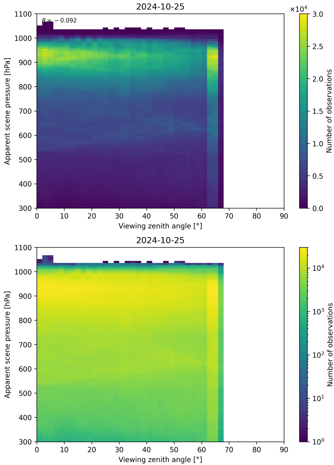
Figure 129: Scatter density plot of “Viewing zenith angle” against “Apparent scene pressure” for 2024-10-24 to 2024-10-26.
