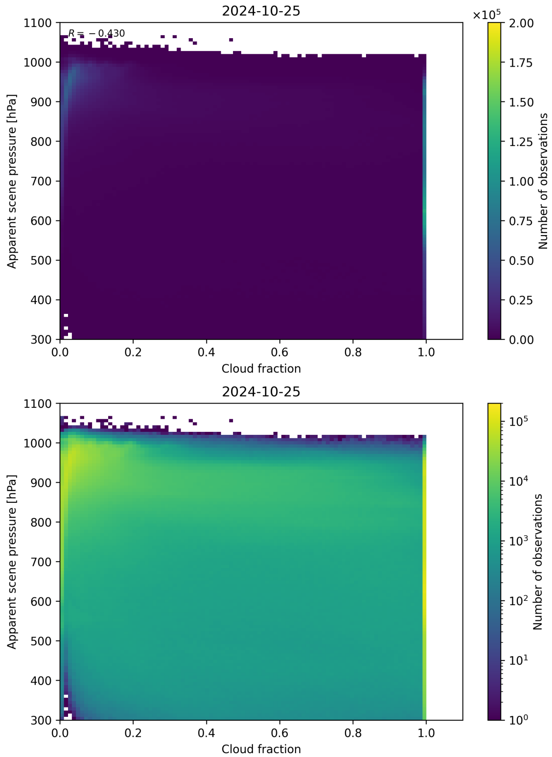
Figure 76: Scatter density plot of “Cloud fraction” against “Apparent scene pressure” for 2024-10-24 to 2024-10-26.
