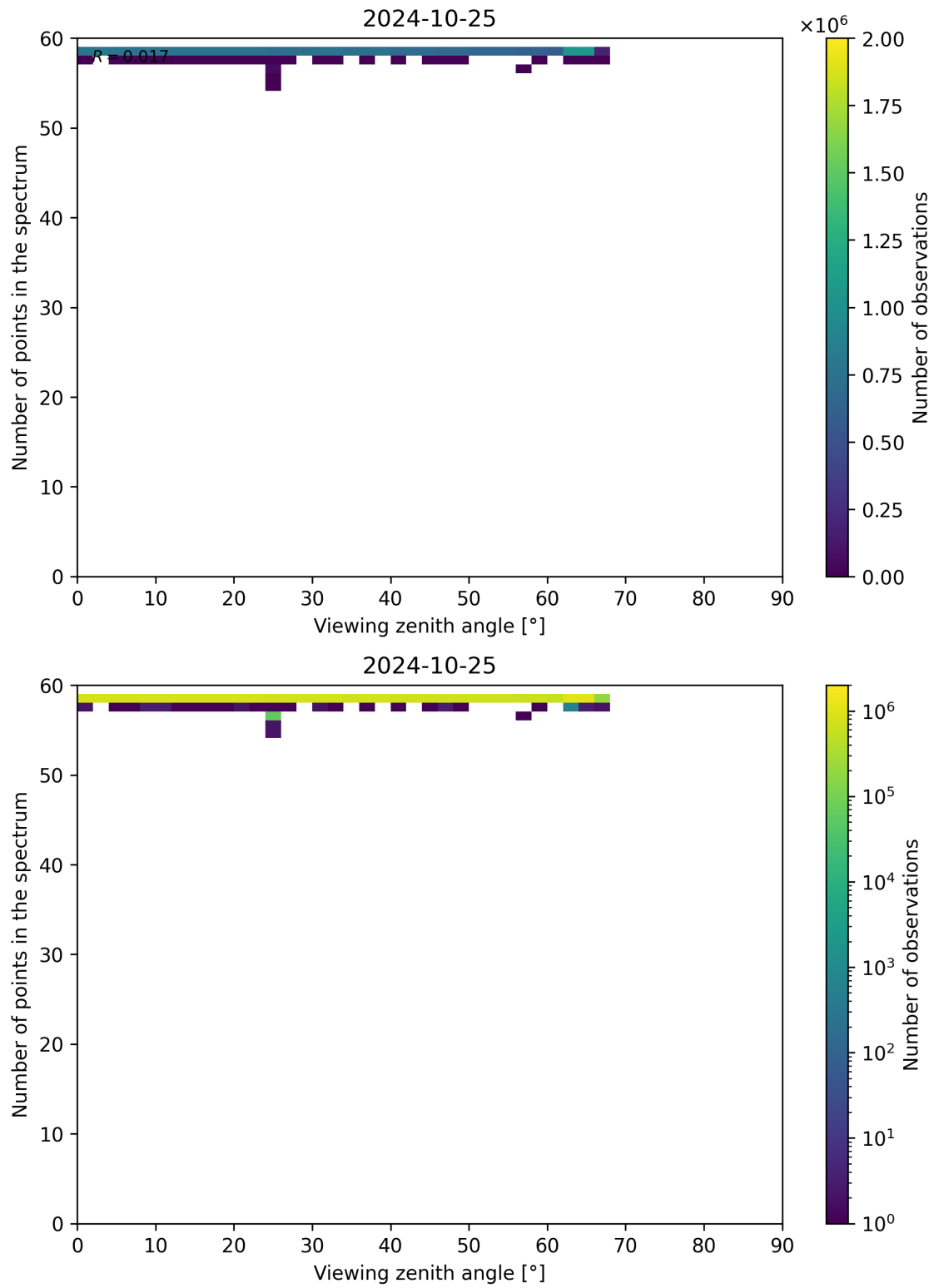
Figure 137: Scatter density plot of “Viewing zenith angle” against “Number of points in the spectrum” for 2024-10-24 to 2024-10-26.
