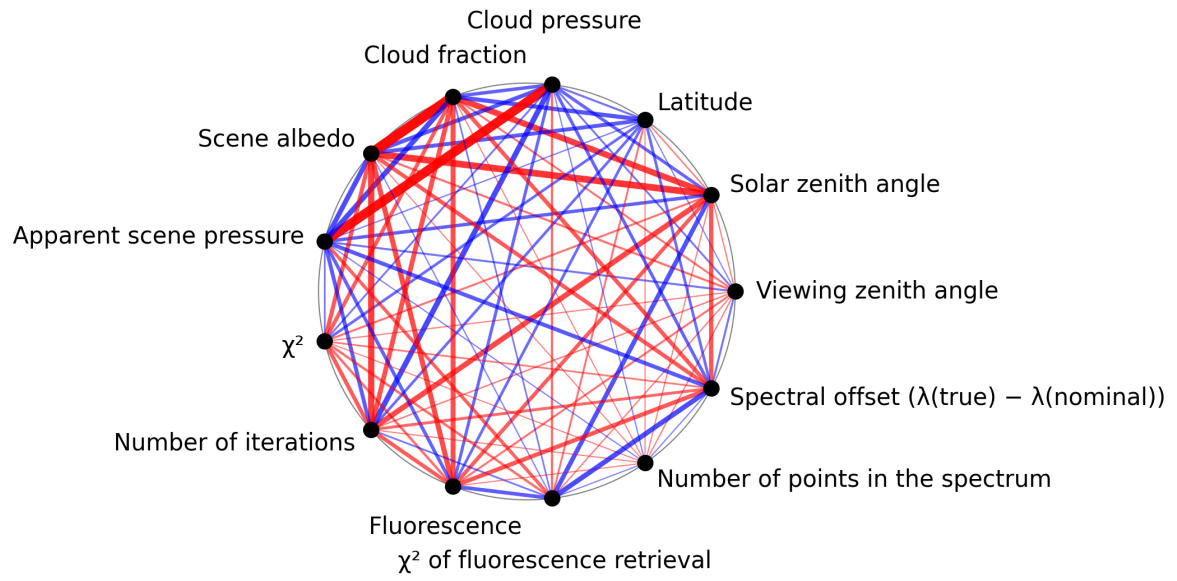
Figure 1: Map of correlation graph for 2024-10-24 to 2024-10-26.
