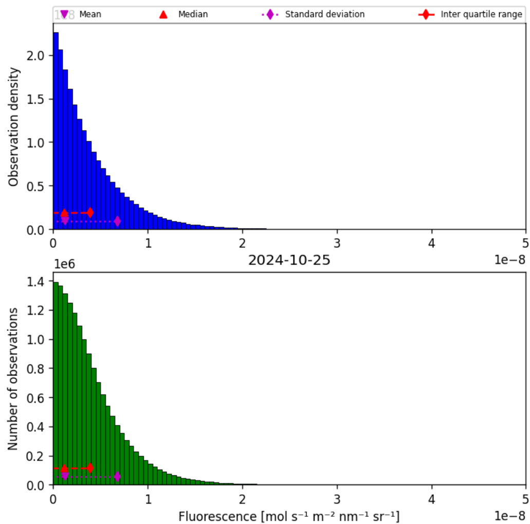
Figure 40: Histogram of “Fluorescence” for 2024-10-24 to 2024-10-26
