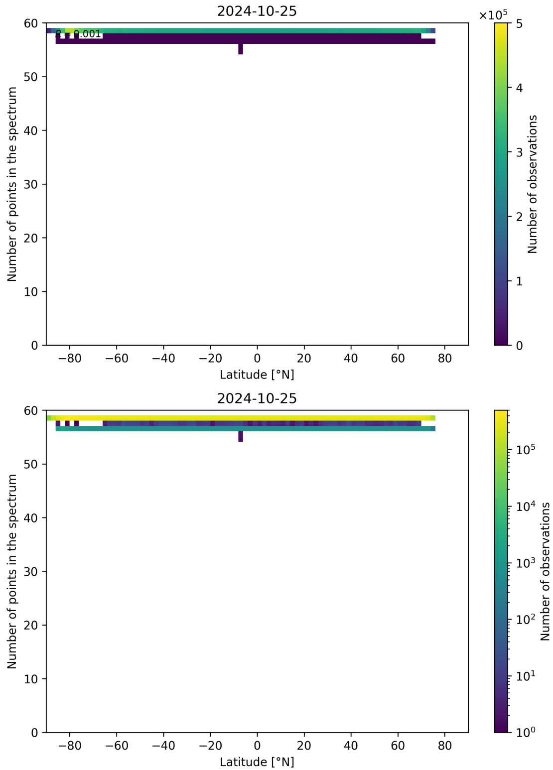
Figure 103: Scatter density plot of “Latitude” against “Number of points in the spectrum” for 2024-10-24 to 2024-10-26.
