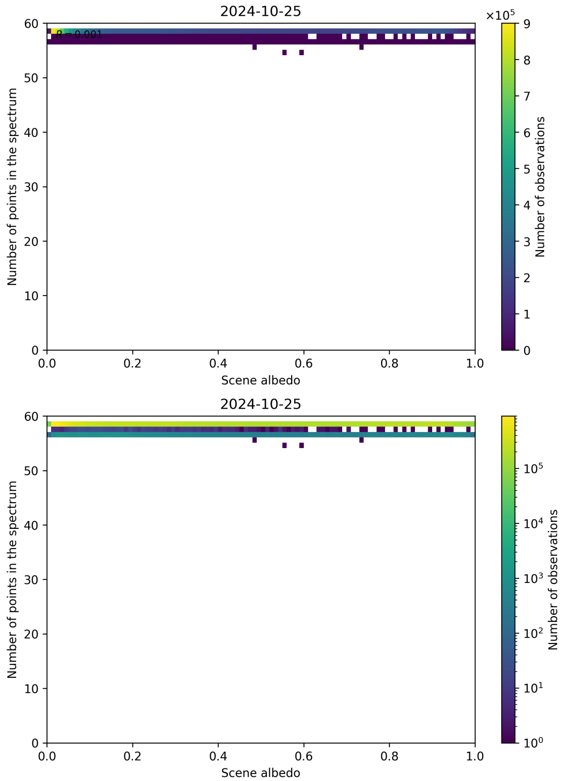
Figure 116: Scatter density plot of “Scene albedo” against “Number of points in the spectrum” for 2024-10-24 to 2024-10-26.
