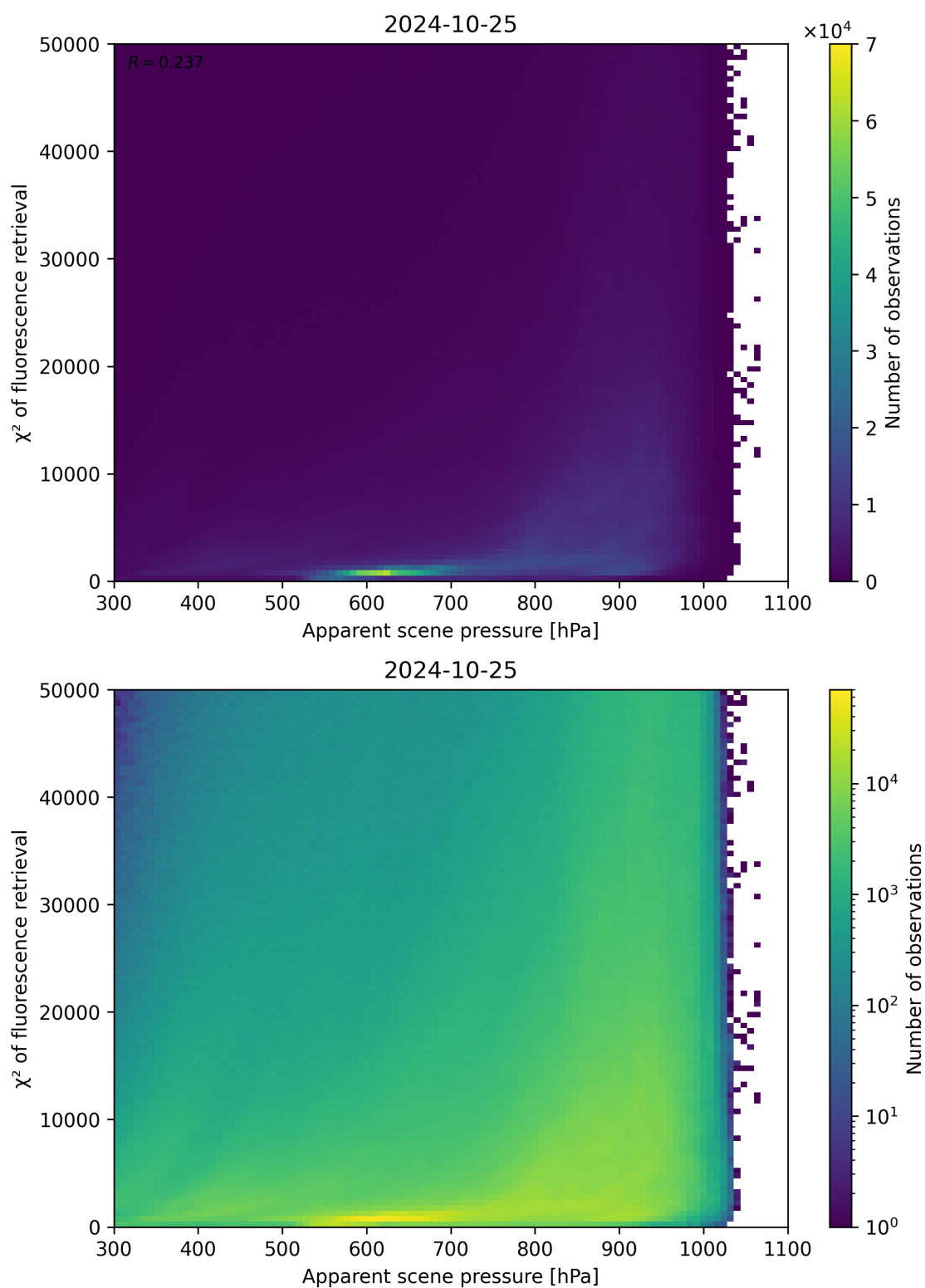
Figure 64: Scatter density plot of “Apparent scene pressure” against “ \chi^2 of fluorescence retrieval” for 2024-10-24 to 2024-10-26.
