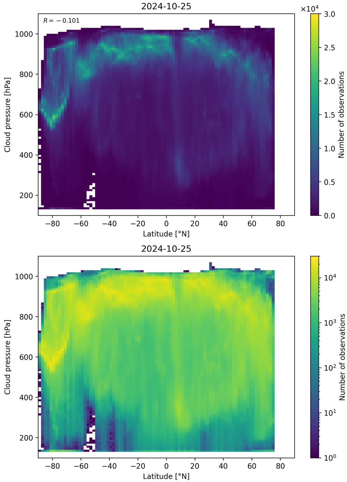
Figure 100: Scatter density plot of “Latitude” against “Cloud pressure” for 2024-10-24 to 2024-10-26.
