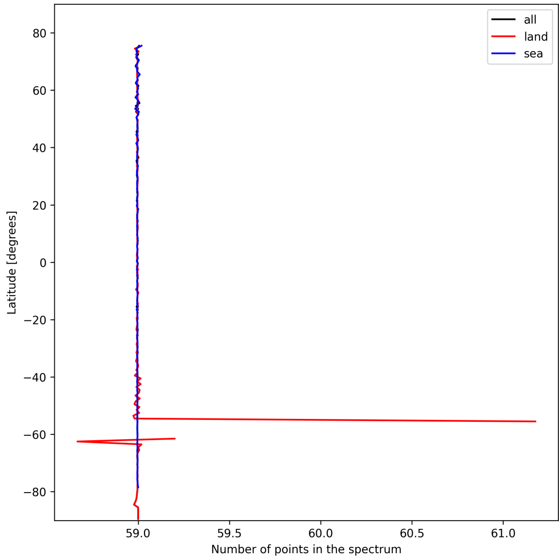
Figure 27: Zonal average of “Number of points in the spectrum” for 2024-10-24 to 2024-10-26.
