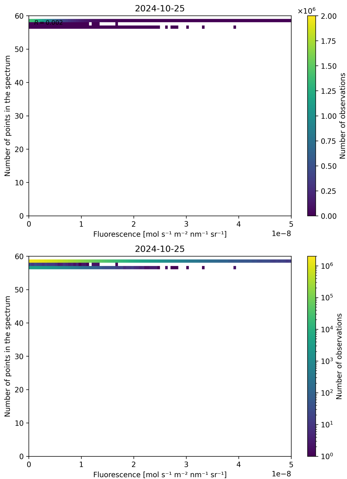
Figure 94: Scatter density plot of “Fluorescence” against “Number of points in the spectrum” for 2024-10-24 to 2024-10-26.
