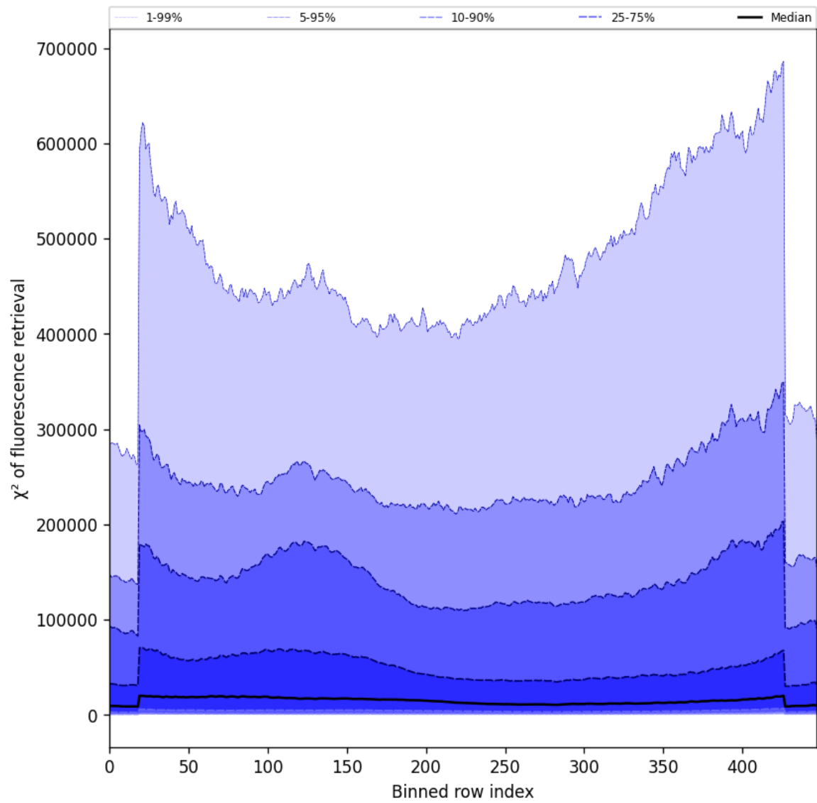
Figure 59: Along track statistics of “ \chi^2 of fluorescence retrieval” for 2024-10-24 to 2024-10-26
