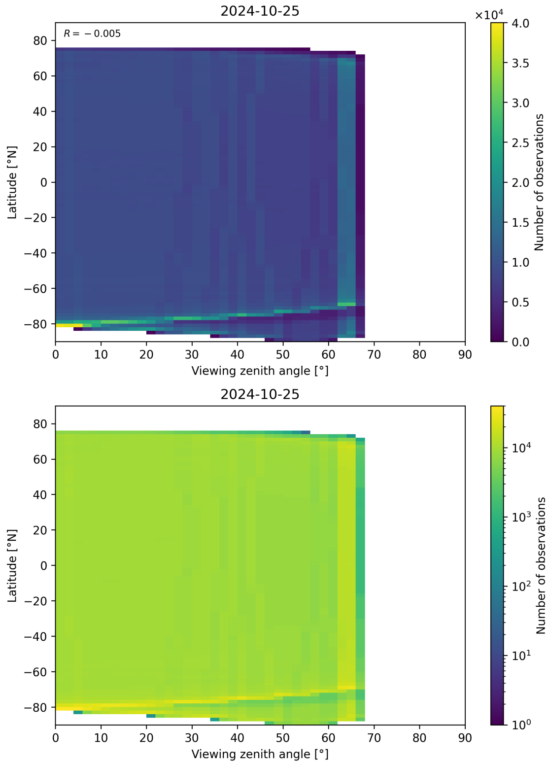
Figure 135: Scatter density plot of “Viewing zenith angle” against “Latitude” for 2024-10-24 to 2024-10-26.
