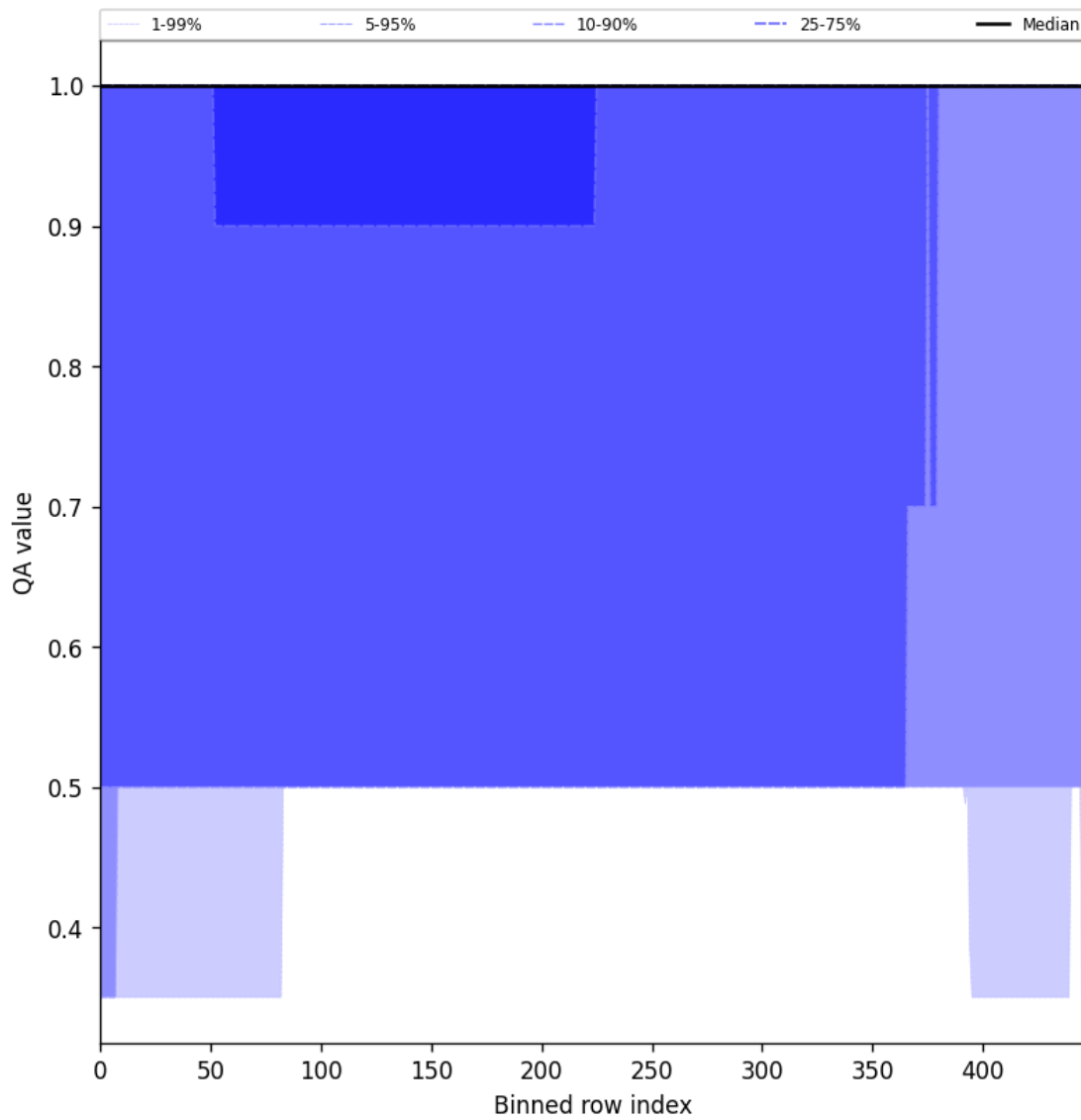
Figure 46: Along track statistics of “QA value” for 2024-10-24 to 2024-10-26
