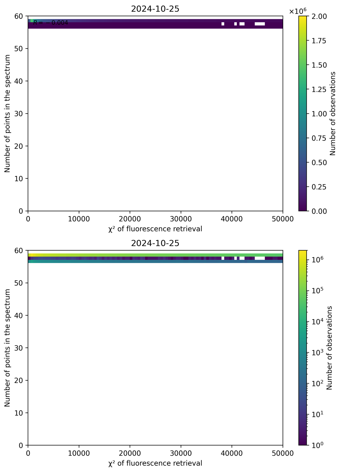
Figure 71: Scatter density plot of " \chi^2 of fluorescence retrieval" against "Number of points in the spectrum" for 2024-10-24 to 2024-10-26.
