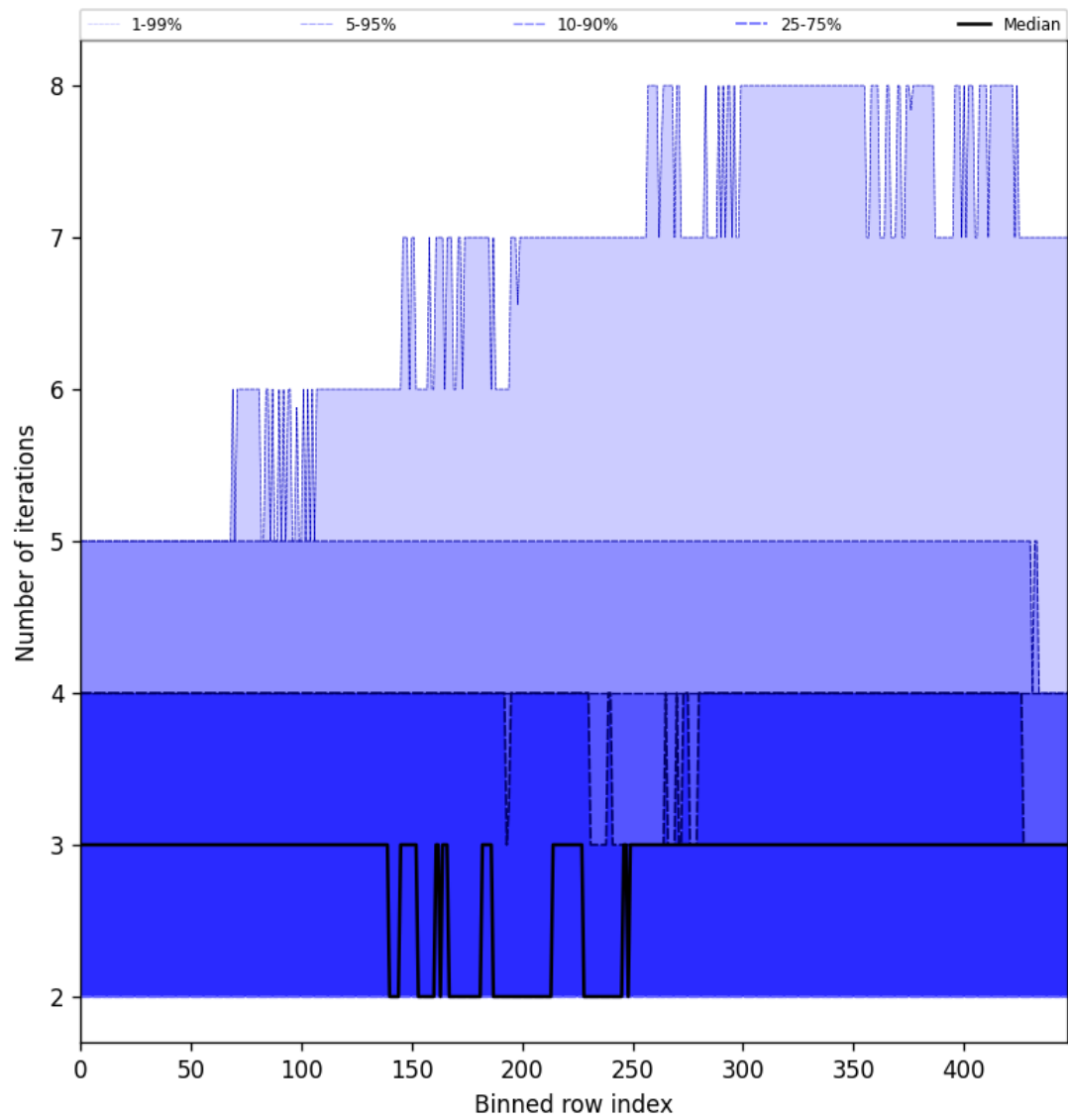
Figure 56: Along track statistics of “Number of iterations” for 2024-10-24 to 2024-10-26
