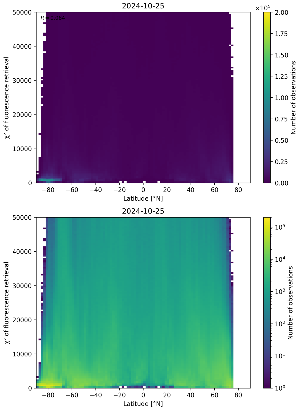
Figure 98: Scatter density plot of “Latitude” against “ \chi^2 of fluorescence retrieval” for 2024-10-24 to 2024-10-26.
