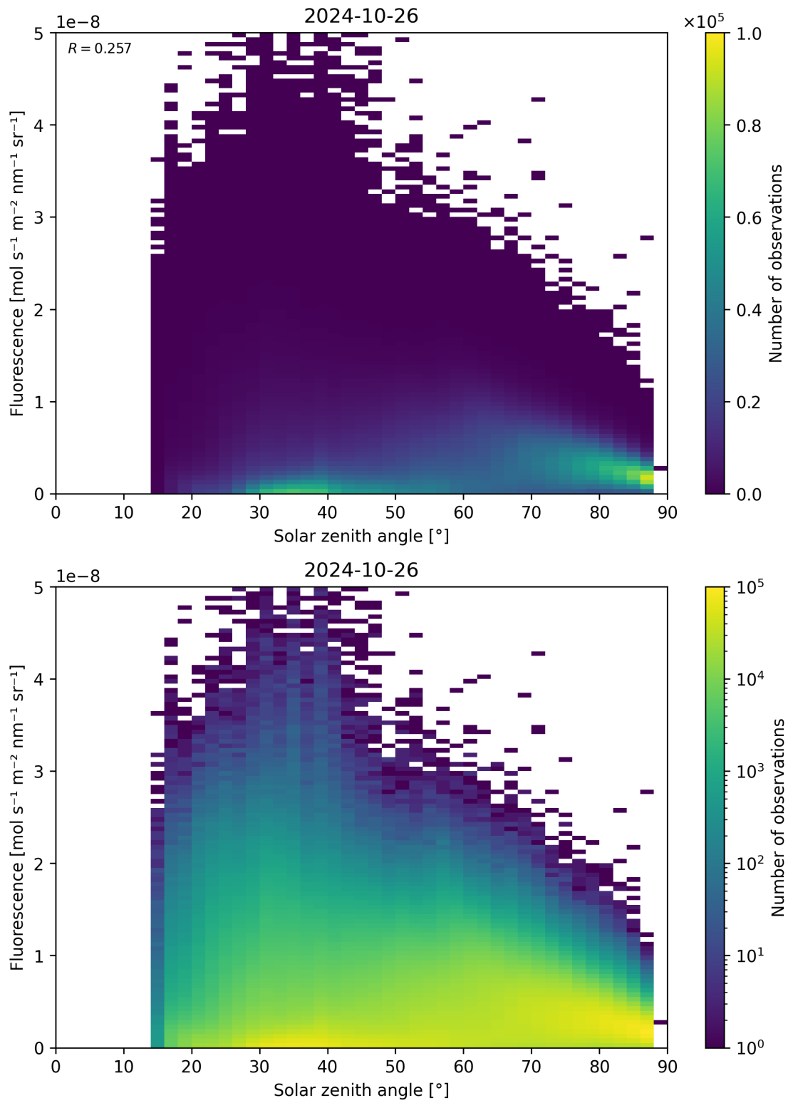
Figure 123: Scatter density plot of “Solar zenith angle” against “Fluorescence” for 2024-10-25 to 2024-10-27.
