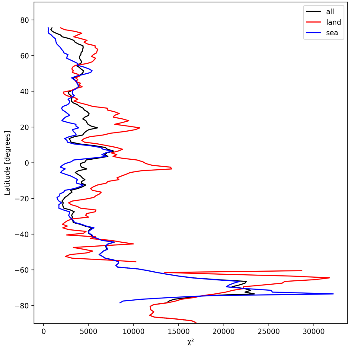
Figure 21: Zonal average of “ \chi^2 ” for 2024-10-25 to 2024-10-27.
