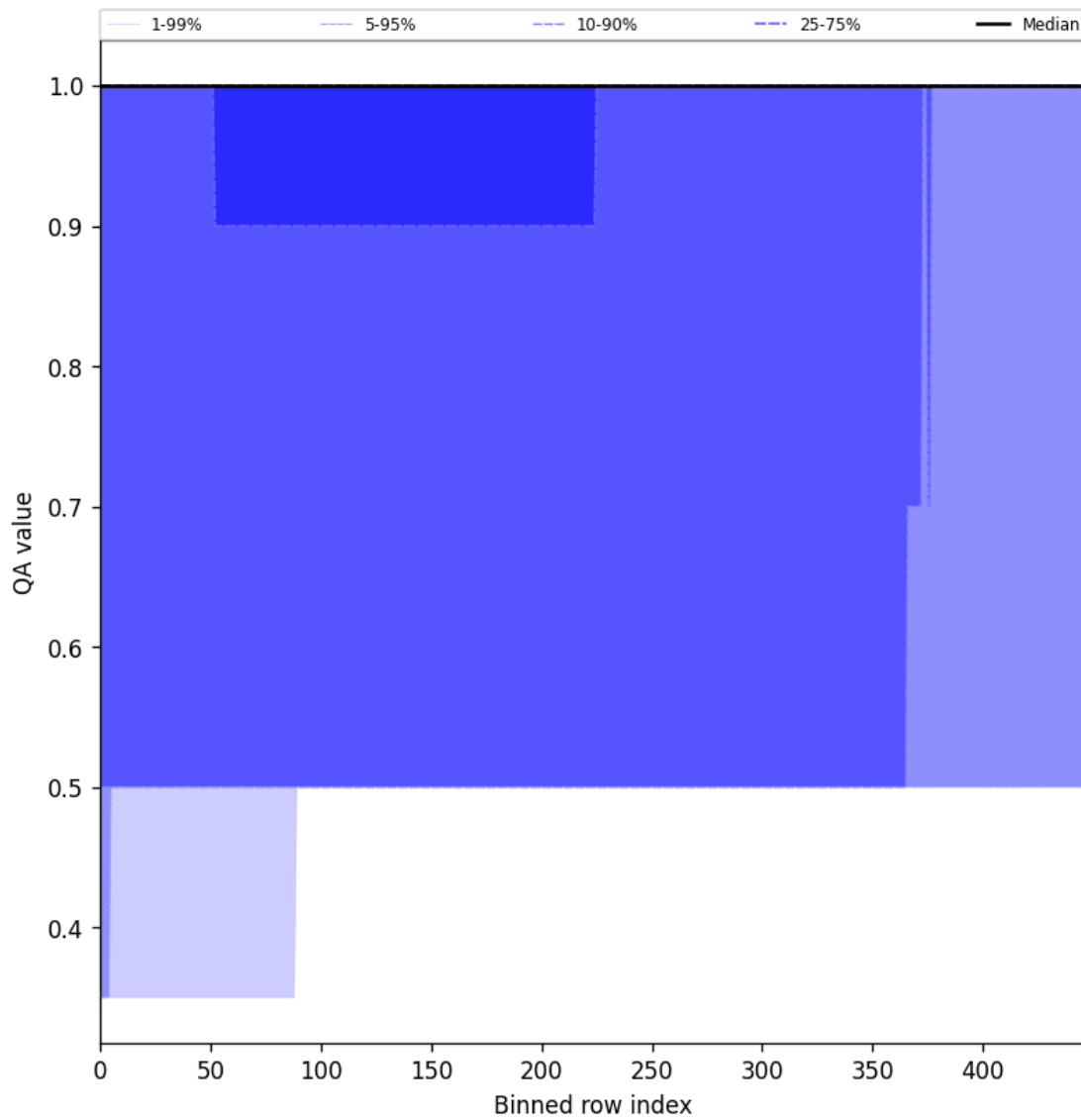
Figure 46: Along track statistics of “QA value” for 2024-10-25 to 2024-10-27
