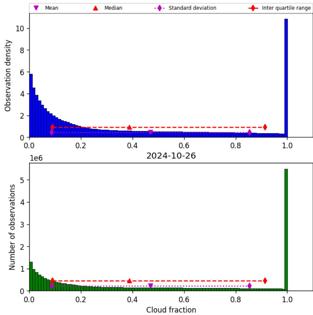
Figure 32: Histogram of “Cloud fraction” for 2024-10-25 to 2024-10-27
