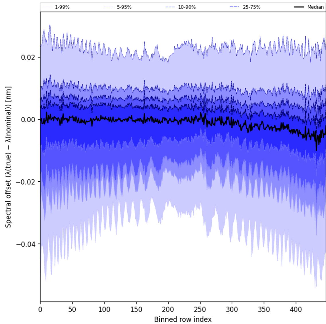
Figure 62: Along track statistics of “Spectral offset ( \lambda_{\text{true}} - \lambda_{\text{nominal}} )” for 2024-10-25 to 2024-10-27
