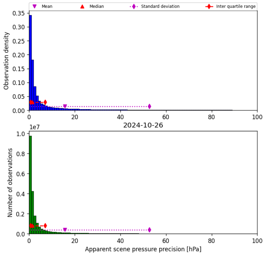
Figure 37: Histogram of “Apparent scene pressure precision” for 2024-10-25 to 2024-10-27
