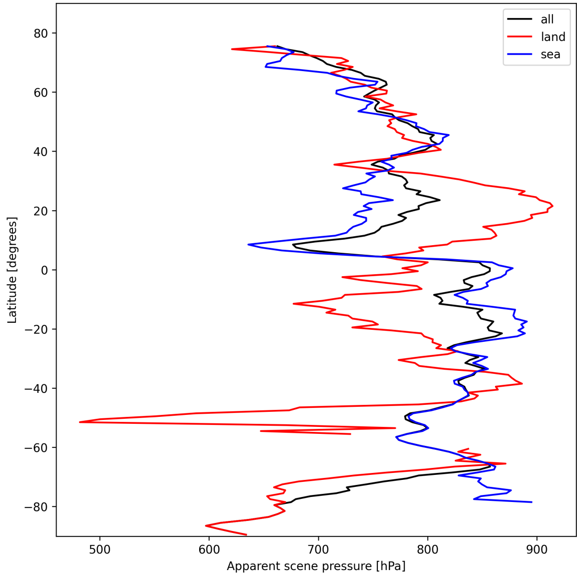
Figure 19: Zonal average of “Apparent scene pressure” for 2024-10-25 to 2024-10-27.
