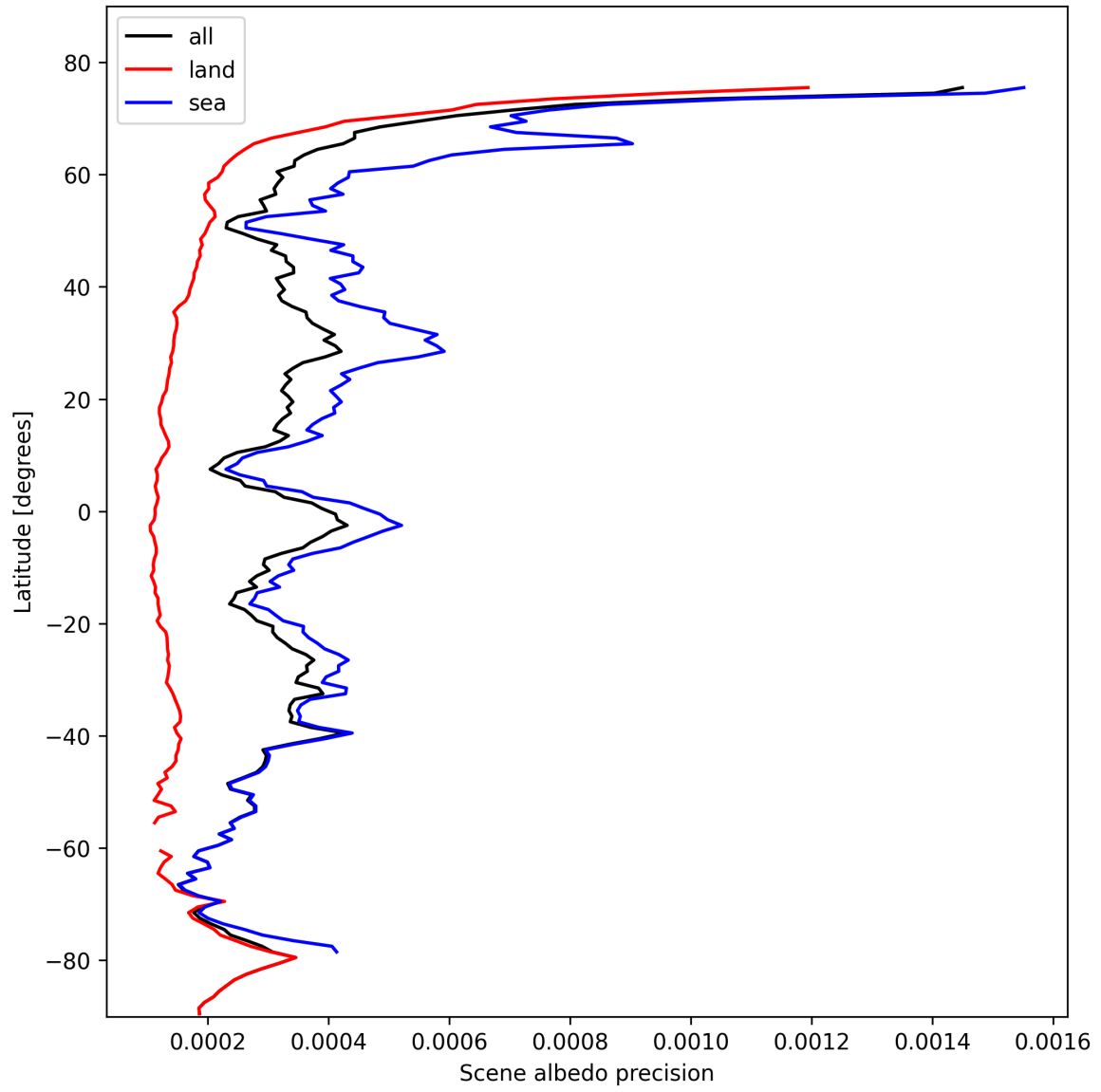
Figure 18: Zonal average of "Scene albedo precision" for 2024-10-25 to 2024-10-27.
