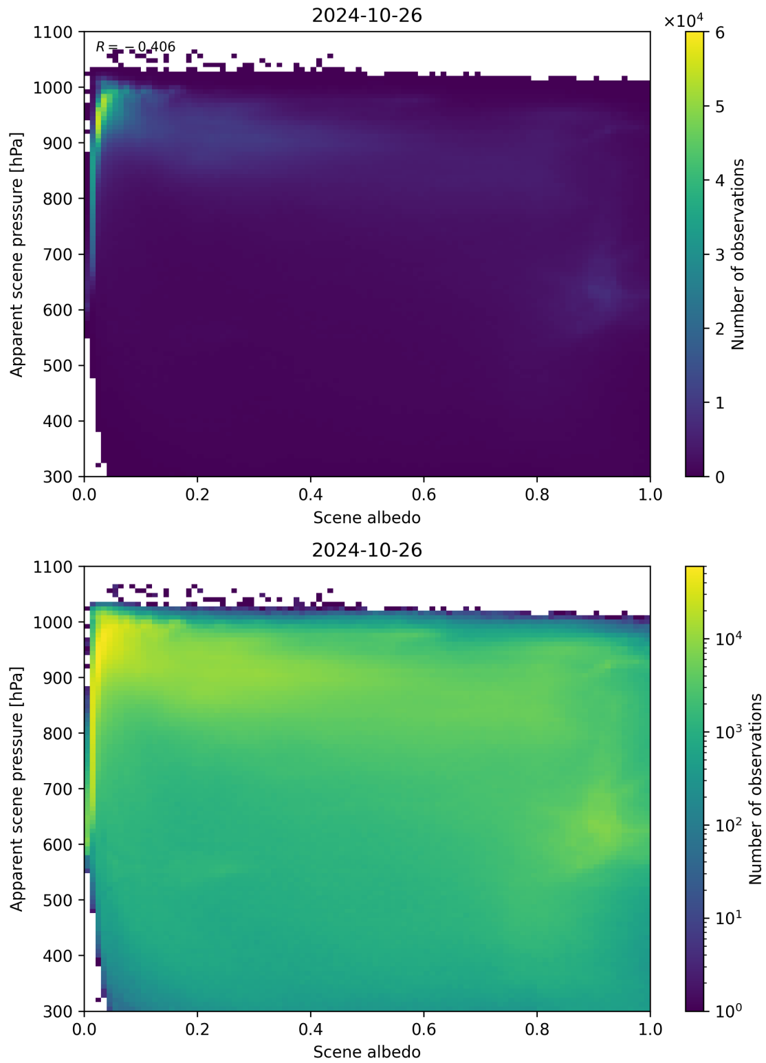
Figure 111: Scatter density plot of “Scene albedo” against “Apparent scene pressure” for 2024-10-25 to 2024-10-27.
