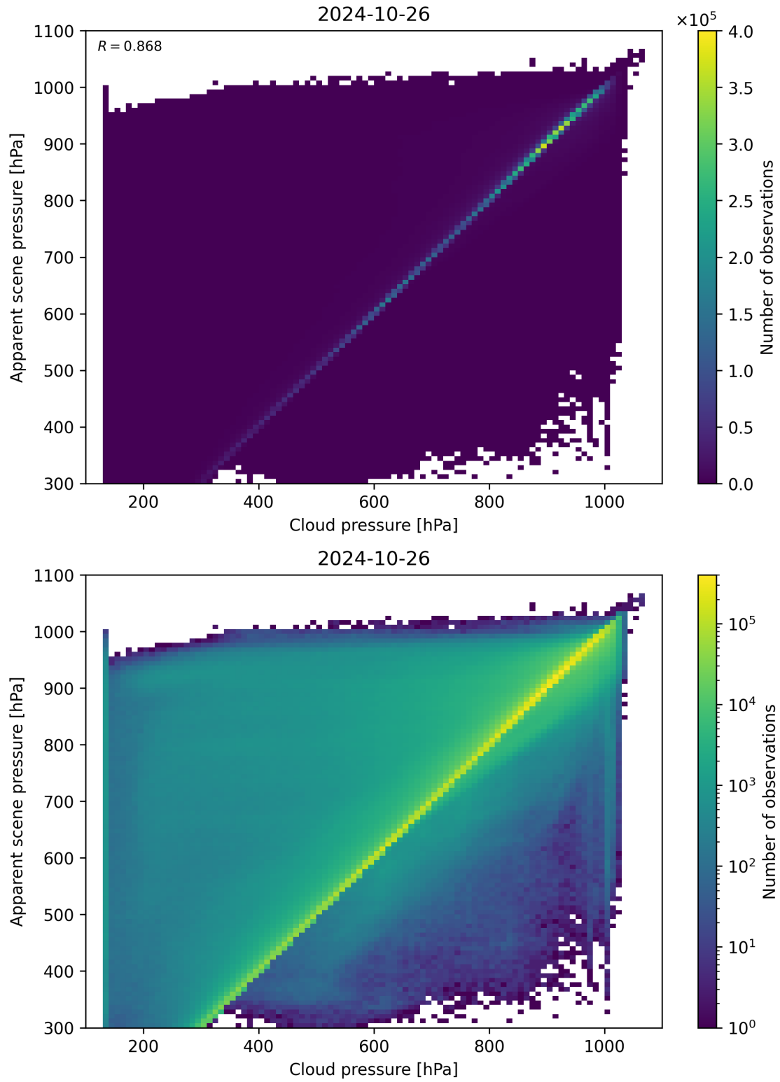
Figure 84: Scatter density plot of “Cloud pressure” against “Apparent scene pressure” for 2024-10-25 to 2024-10-27.
