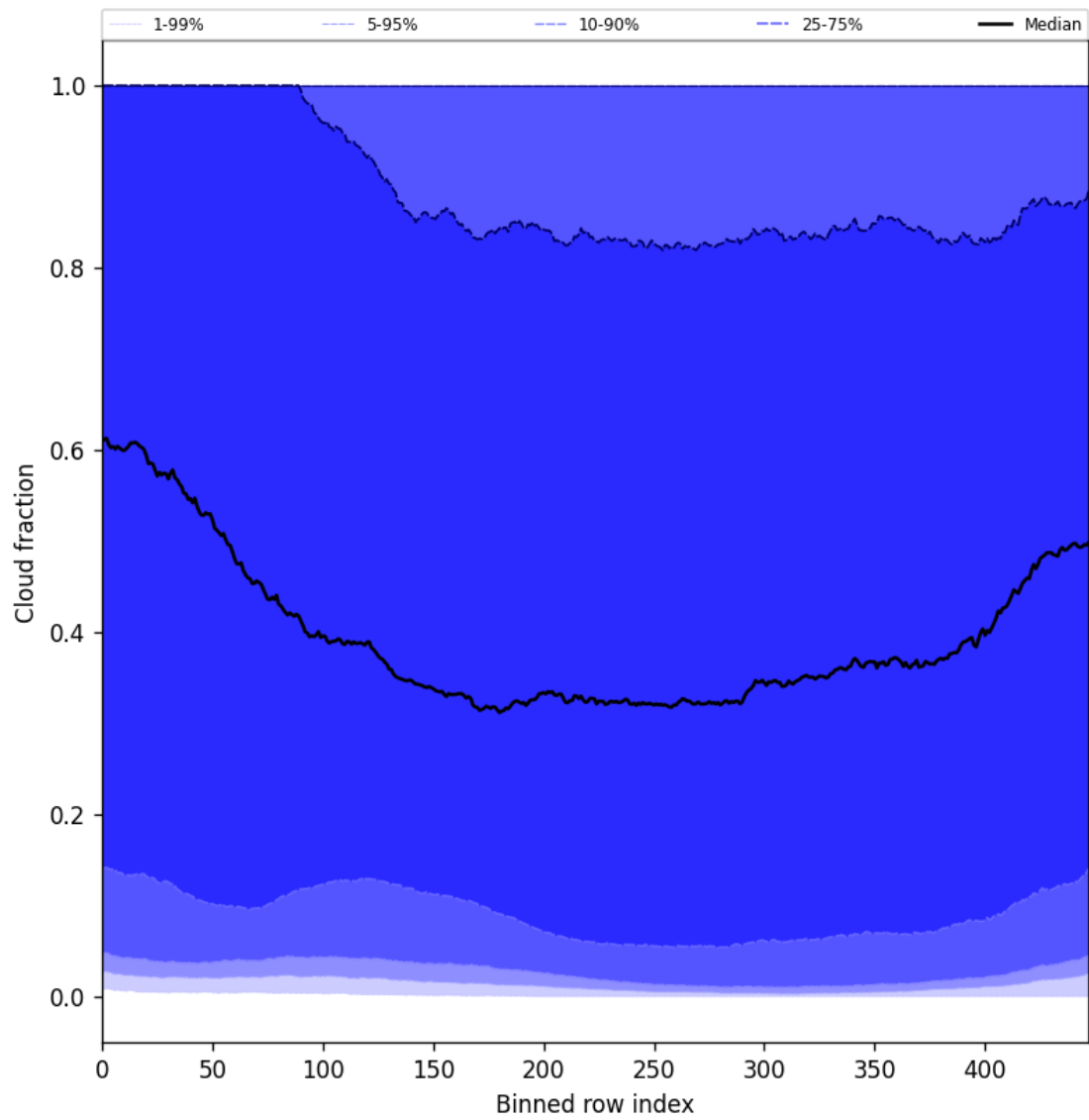
Figure 49: Along track statistics of “Cloud fraction” for 2024-10-25 to 2024-10-27
