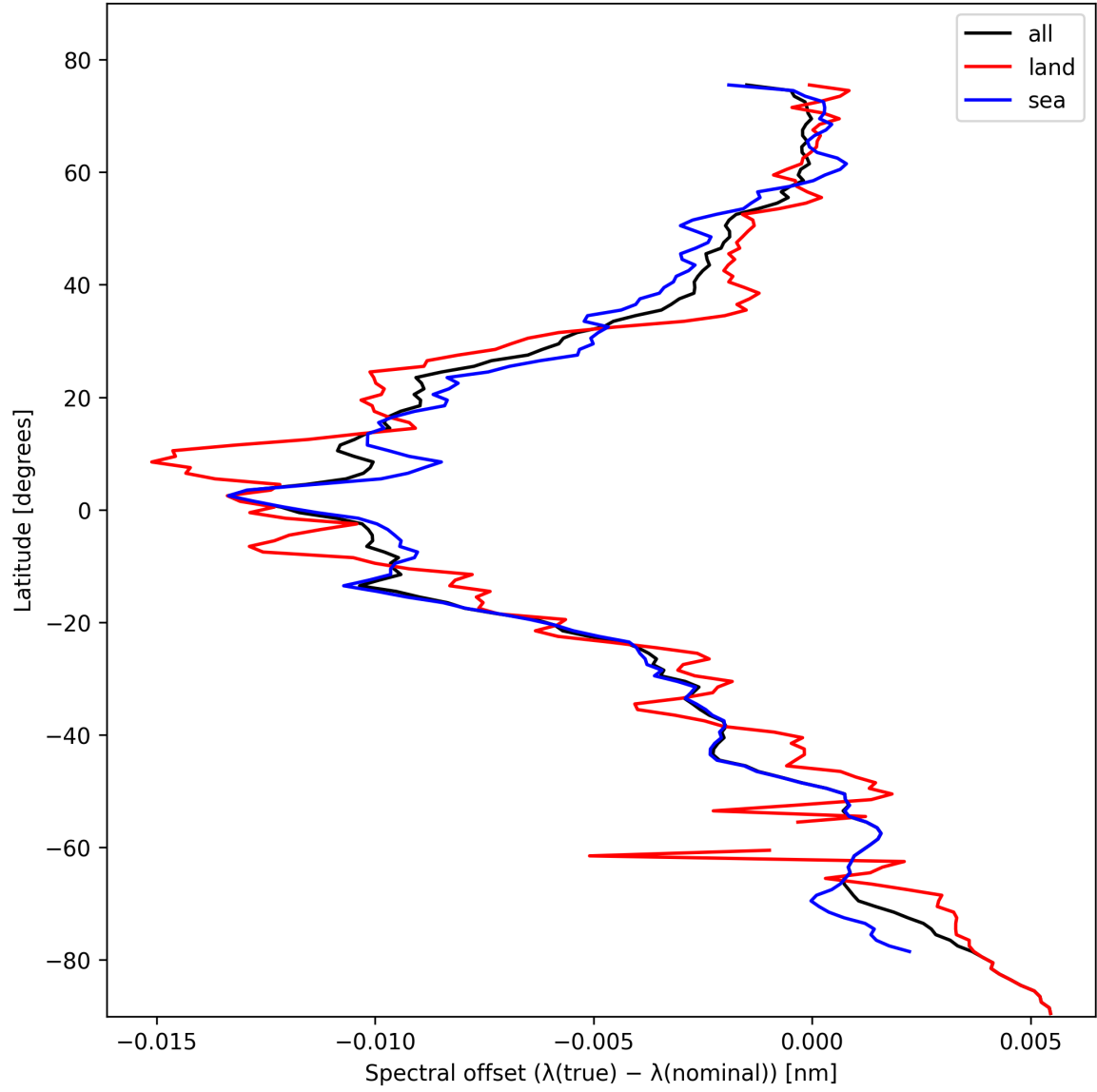
Figure 28: Zonal average of “Spectral offset ( \lambda_{\text{true}} - \lambda_{\text{nominal}} )” for 2024-10-25 to 2024-10-27.
