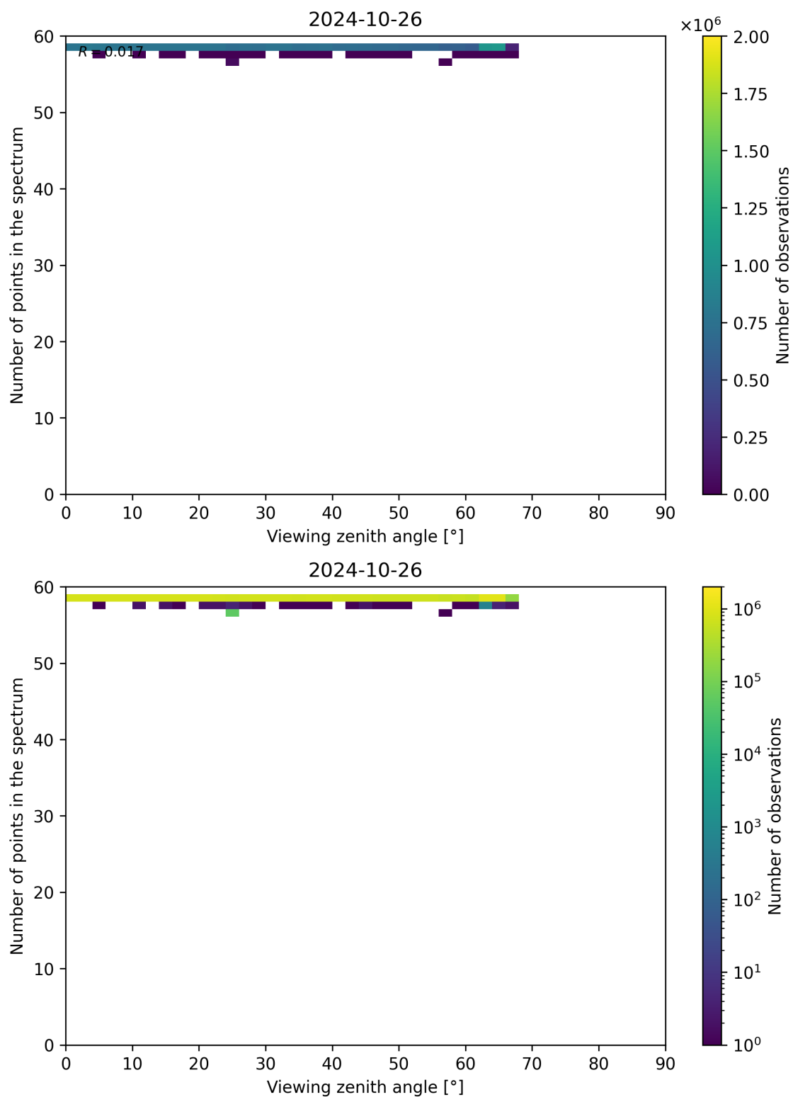
Figure 137: Scatter density plot of “Viewing zenith angle” against “Number of points in the spectrum” for 2024-10-25 to 2024-10-27.
