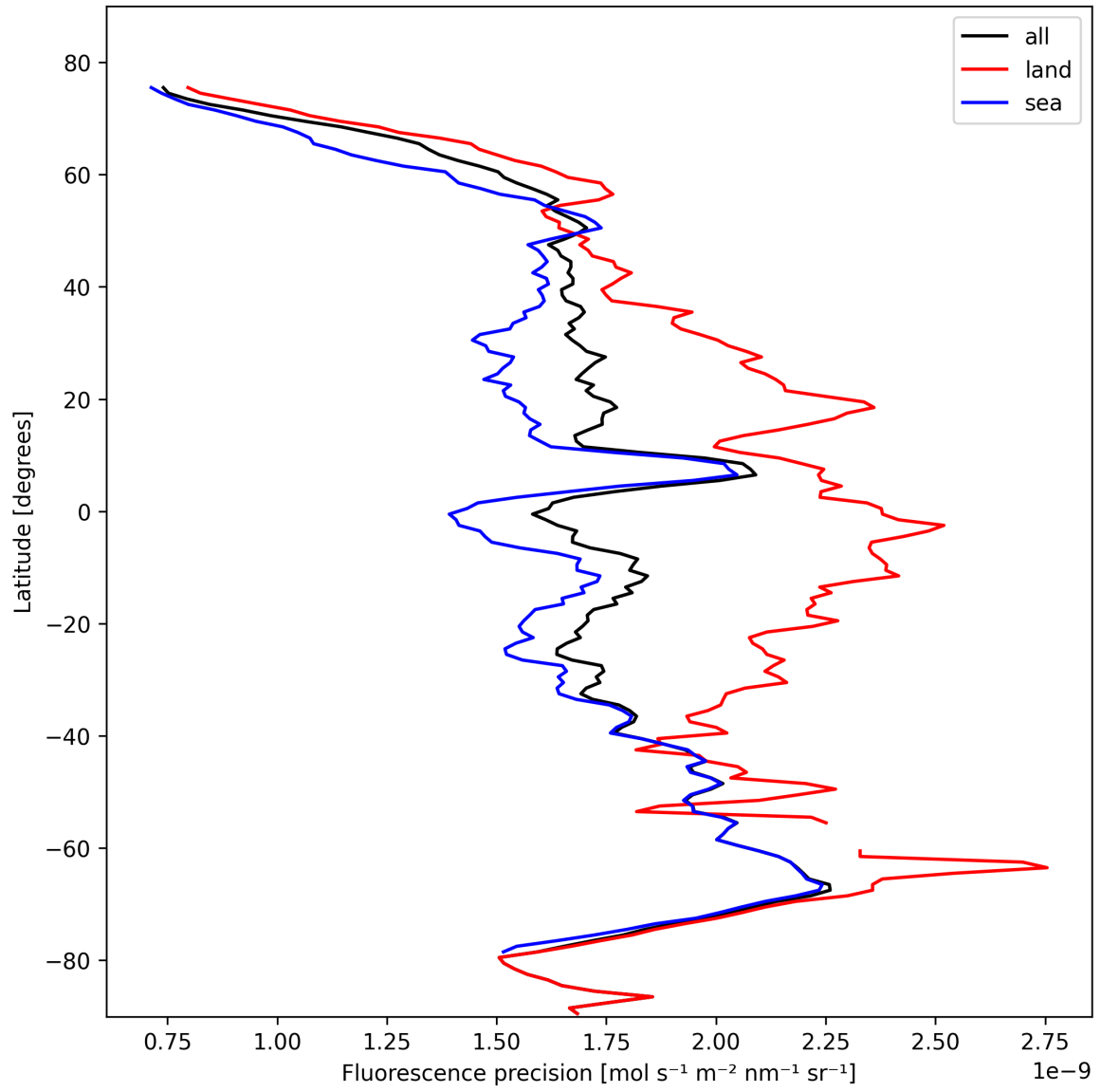
Figure 24: Zonal average of “Fluorescence precision” for 2024-10-25 to 2024-10-27.
