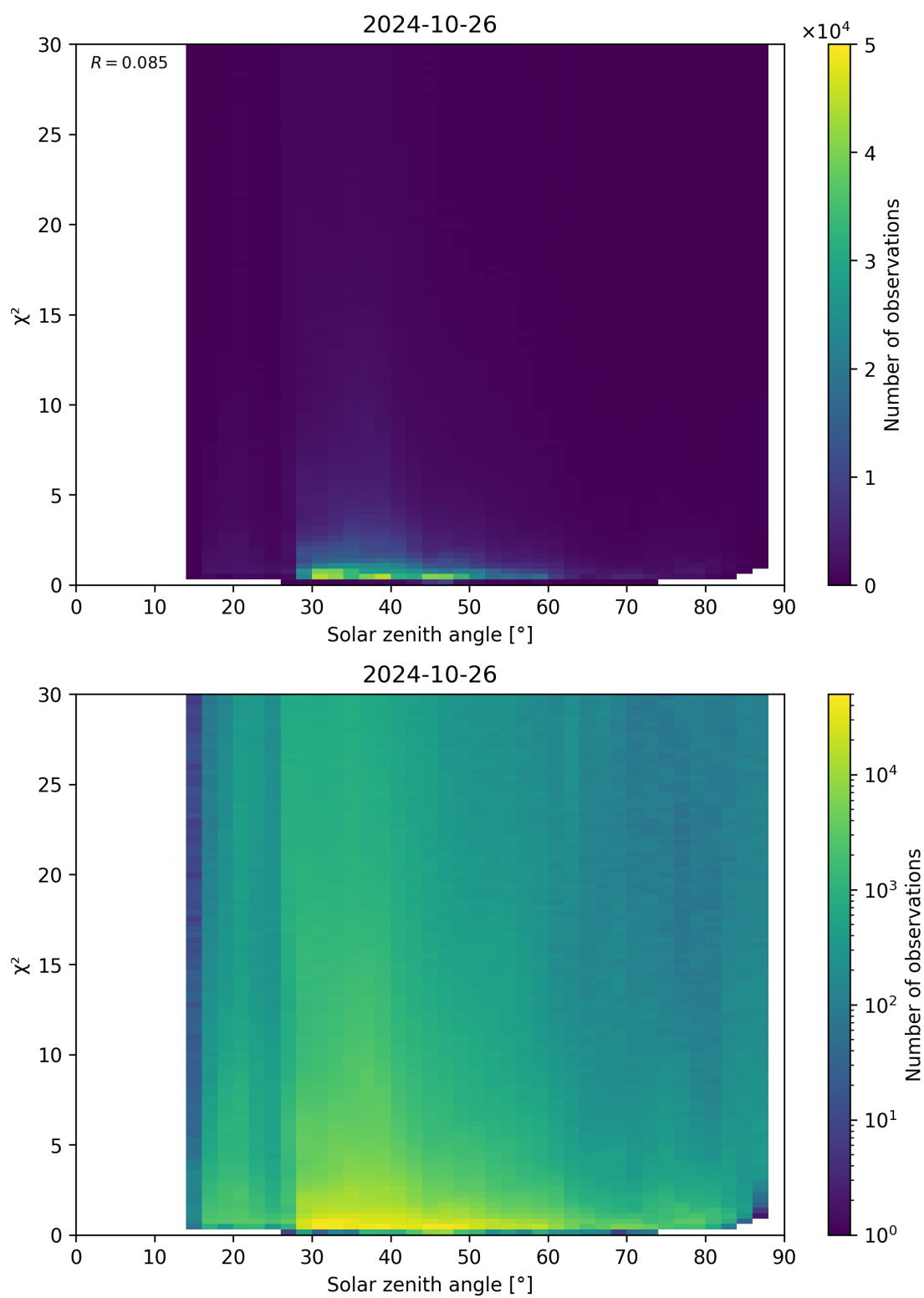
Figure 119: Scatter density plot of “Solar zenith angle” against “ \chi^2 ” for 2024-10-25 to 2024-10-27.
