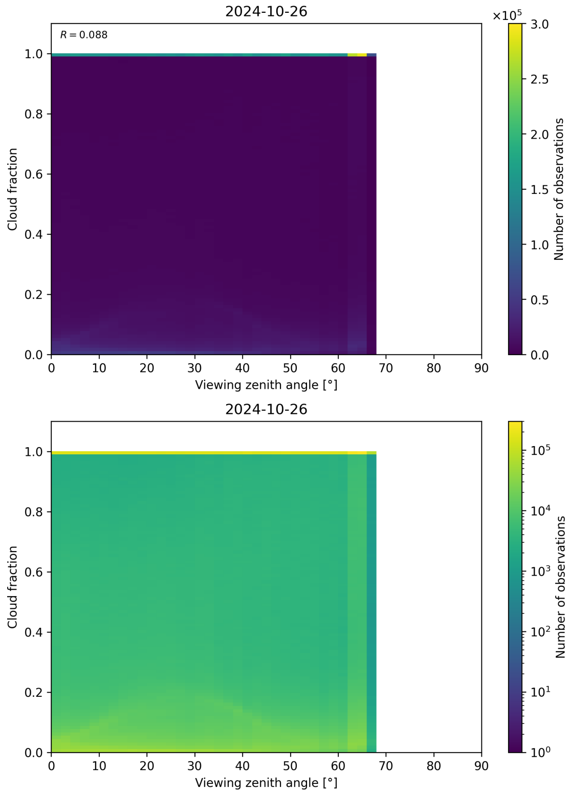
Figure 132: Scatter density plot of “Viewing zenith angle” against “Cloud fraction” for 2024-10-25 to 2024-10-27.
