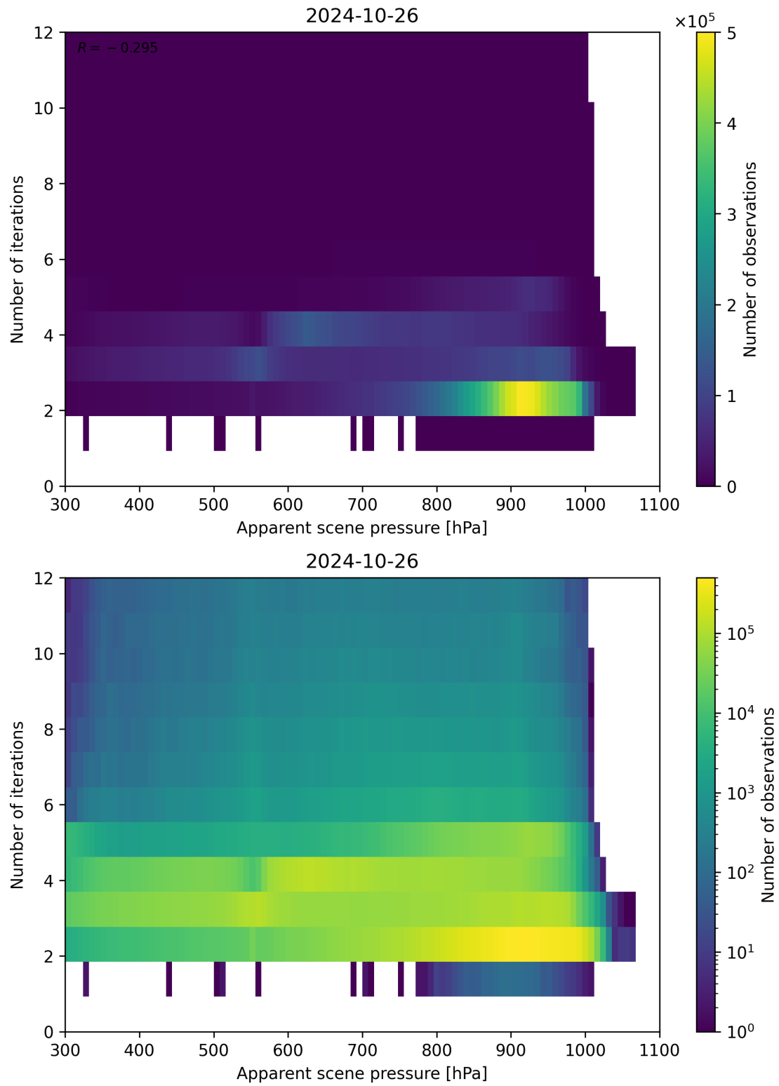
Figure 66: Scatter density plot of “Apparent scene pressure” against “Number of iterations” for 2024-10-25 to 2024-10-27.
