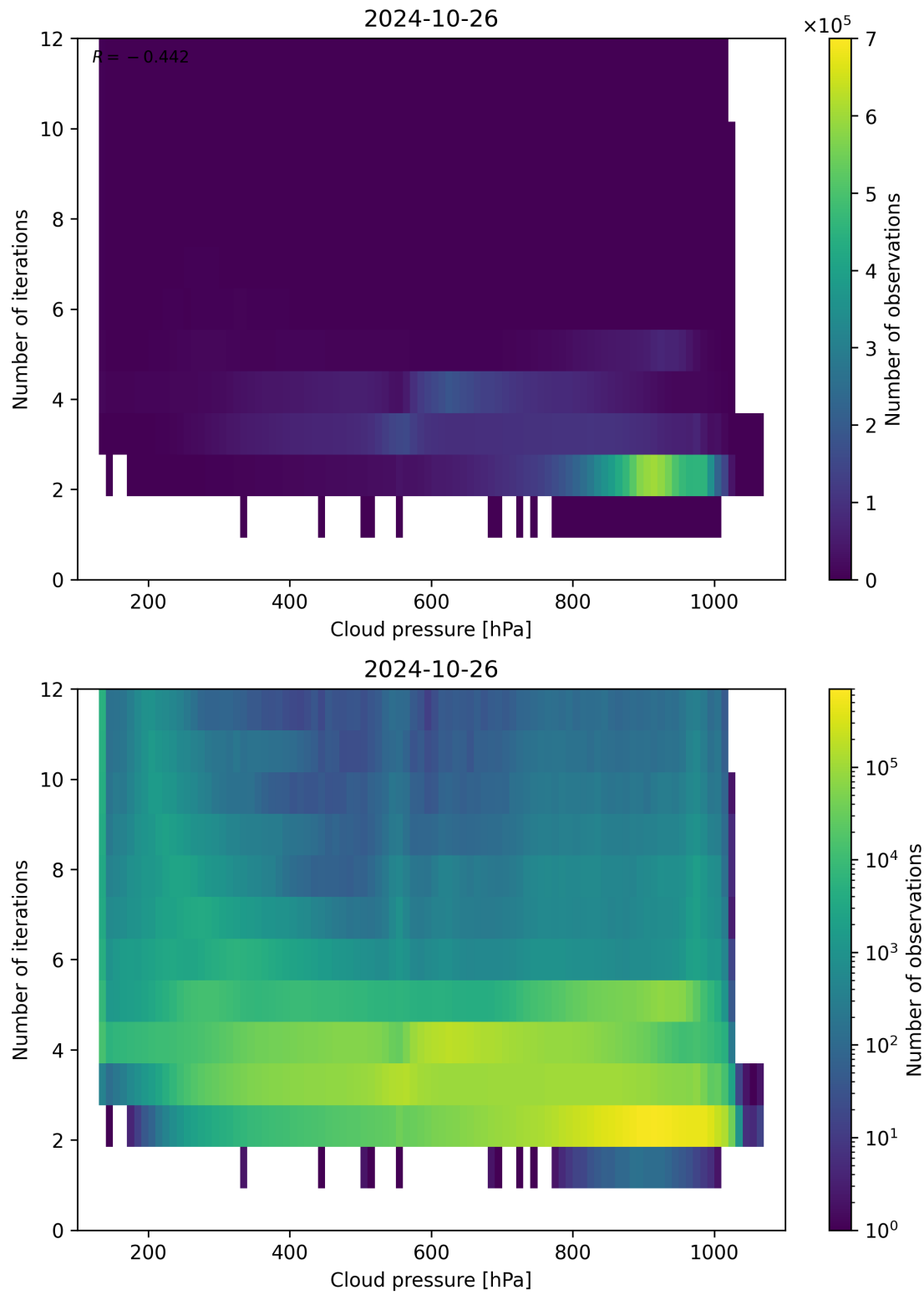
Figure 89: Scatter density plot of “Cloud pressure” against “Number of iterations” for 2024-10-25 to 2024-10-27.
