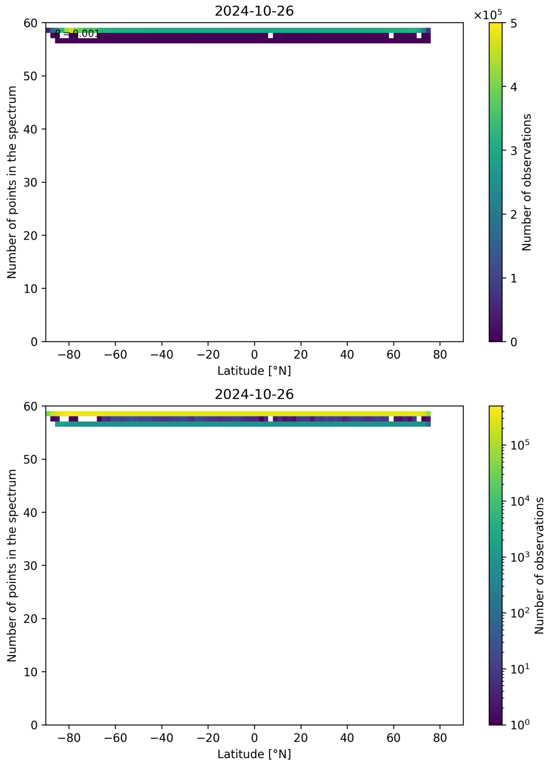
Figure 103: Scatter density plot of “Latitude” against “Number of points in the spectrum” for 2024-10-25 to 2024-10-27.
