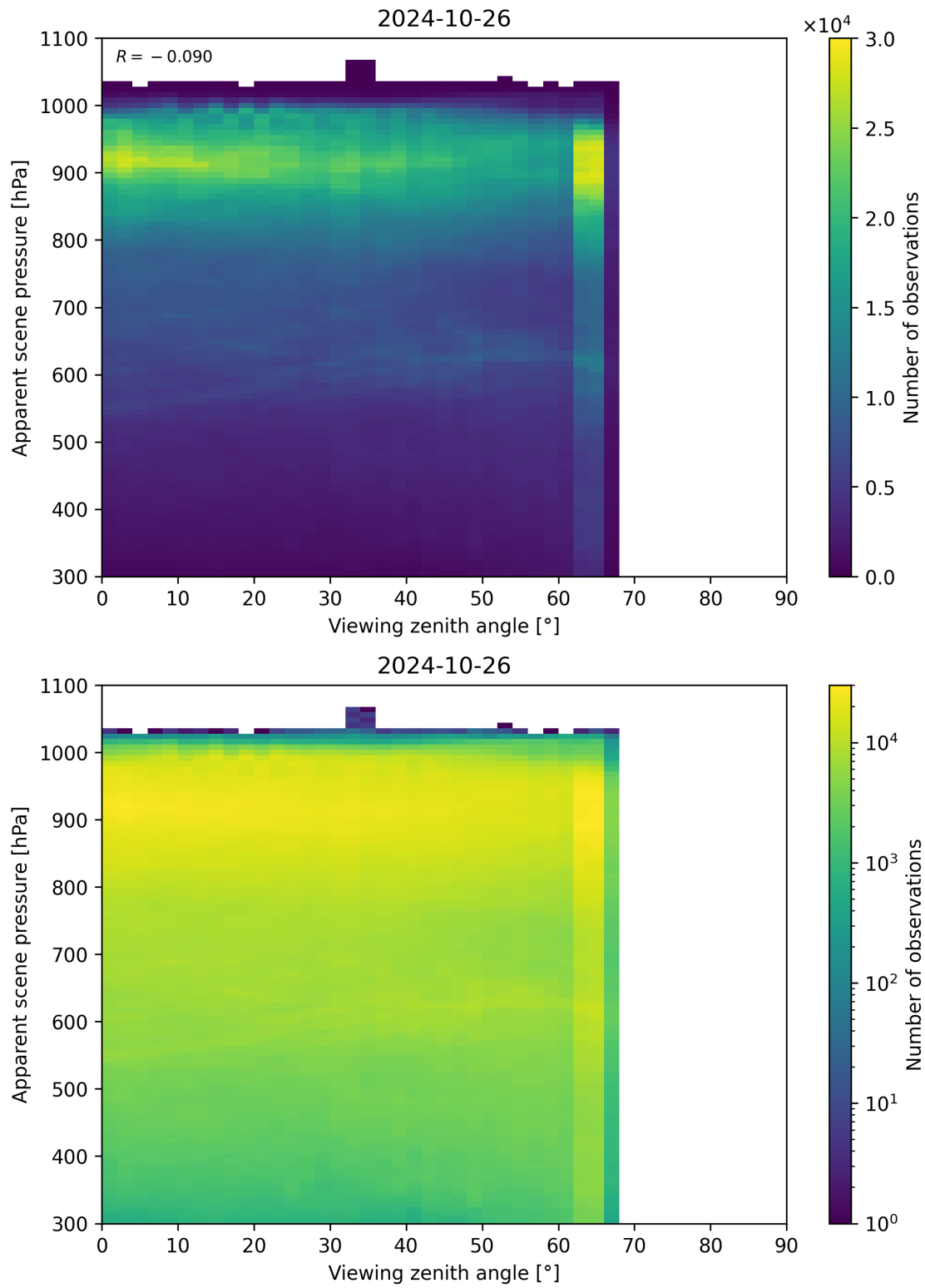
Figure 129: Scatter density plot of “Viewing zenith angle” against “Apparent scene pressure” for 2024-10-25 to 2024-10-27.
