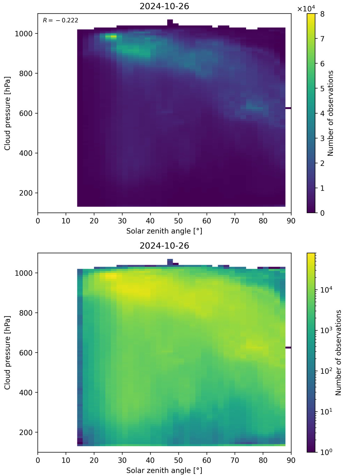
Figure 122: Scatter density plot of “Solar zenith angle” against “Cloud pressure” for 2024-10-25 to 2024-10-27.
