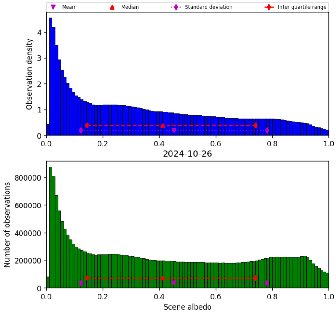
Figure 34: Histogram of “Scene albedo” for 2024-10-25 to 2024-10-27
