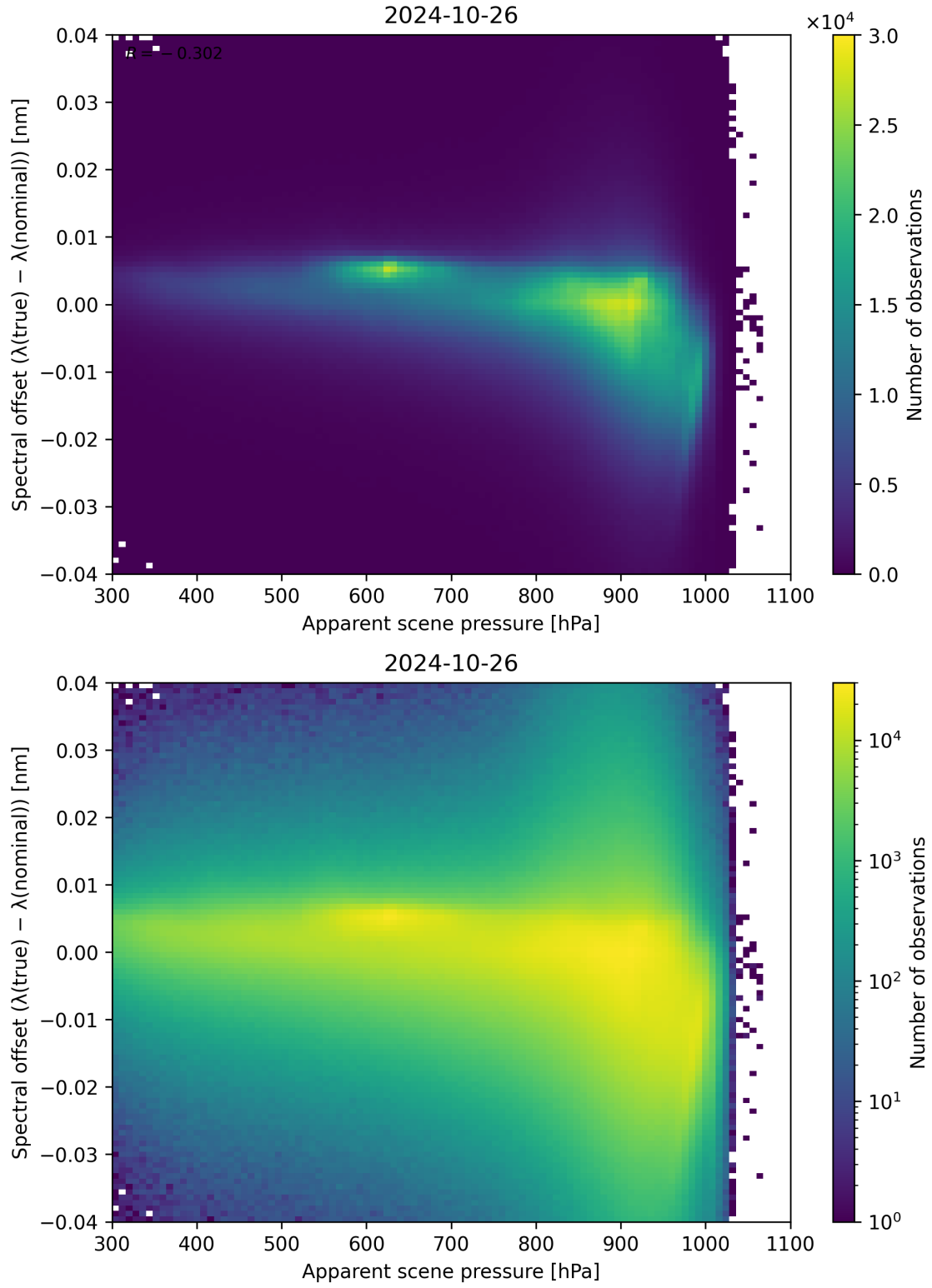
Figure 68: Scatter density plot of “Apparent scene pressure” against “Spectral offset ( \lambda_{\text{true}} - \lambda_{\text{nominal}} )” for 2024-10-25 to 2024-10-27.
