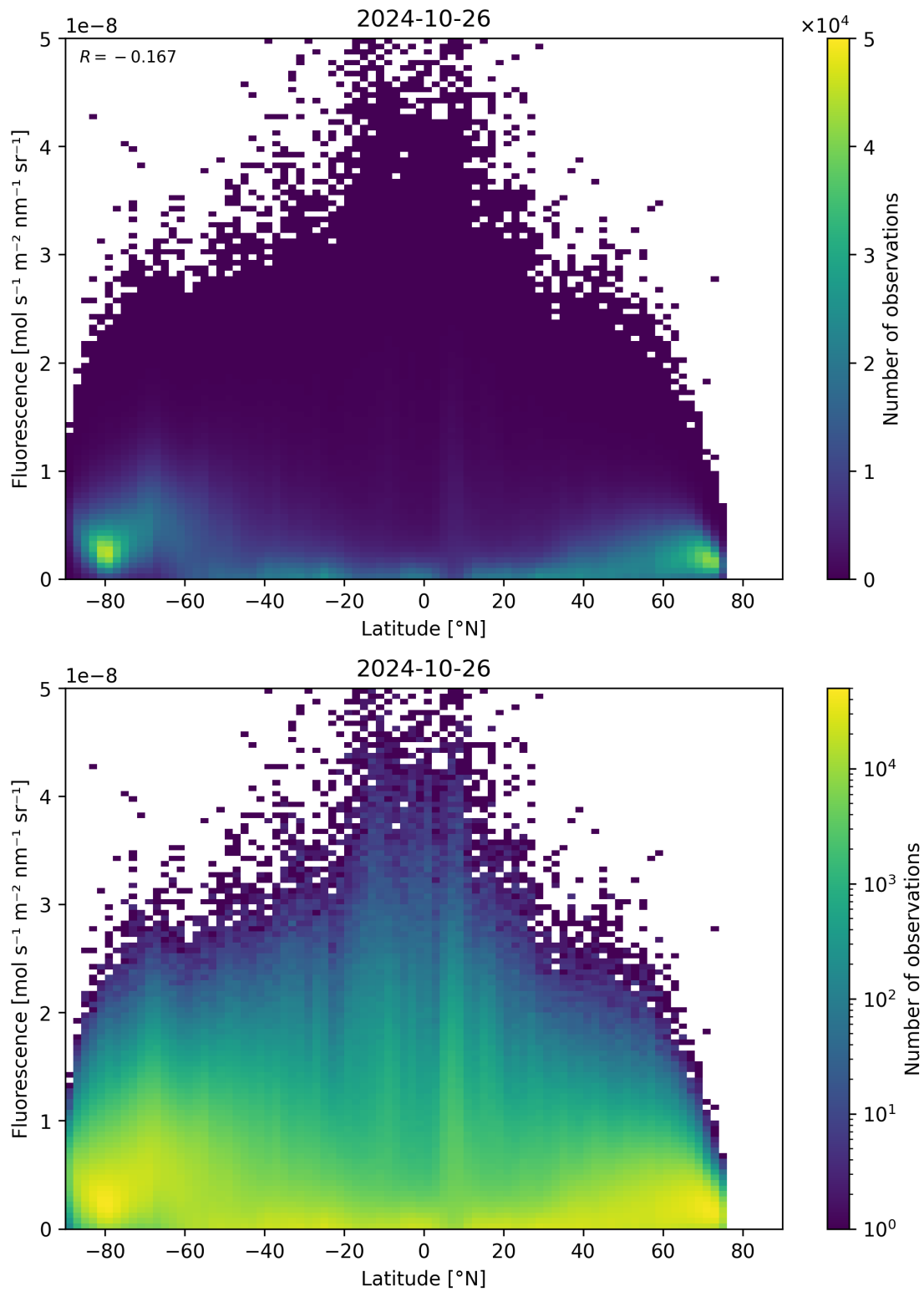
Figure 101: Scatter density plot of “Latitude” against “Fluorescence” for 2024-10-25 to 2024-10-27.
