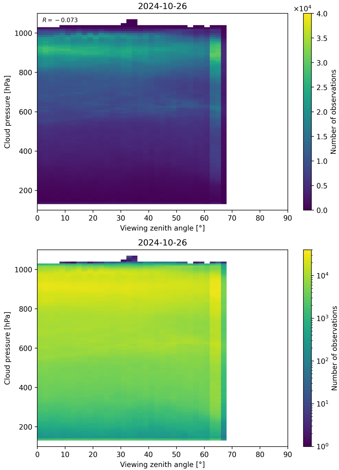
Figure 133: Scatter density plot of “Viewing zenith angle” against “Cloud pressure” for 2024-10-25 to 2024-10-27.
