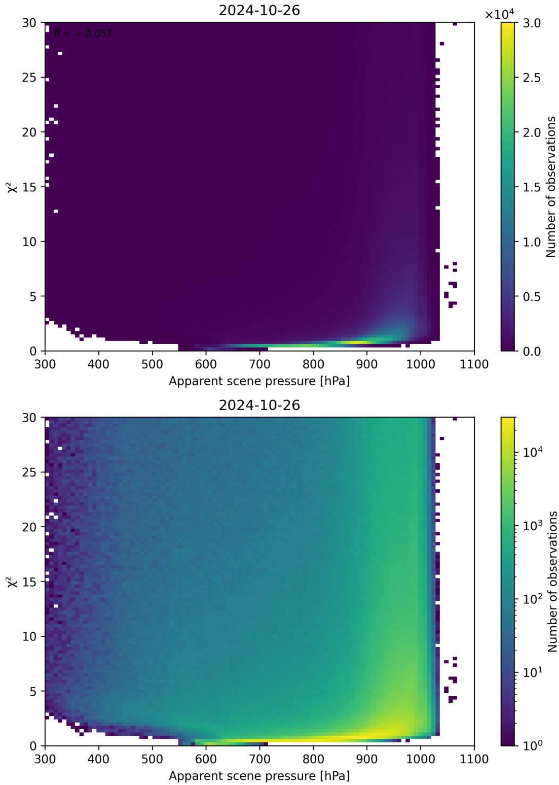
Figure 63: Scatter density plot of “Apparent scene pressure” against “ \chi^2 ” for 2024-10-25 to 2024-10-27.
