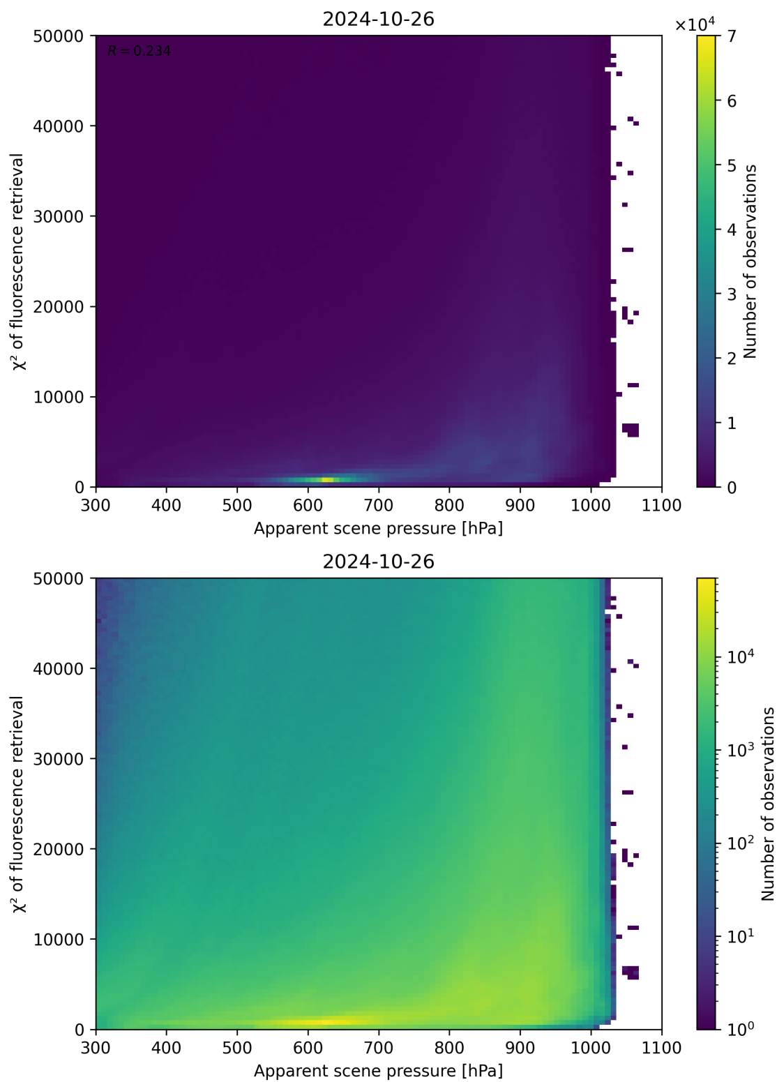
Figure 64: Scatter density plot of “Apparent scene pressure” against “ \chi^2 of fluorescence retrieval” for 2024-10-25 to 2024-10-27.
