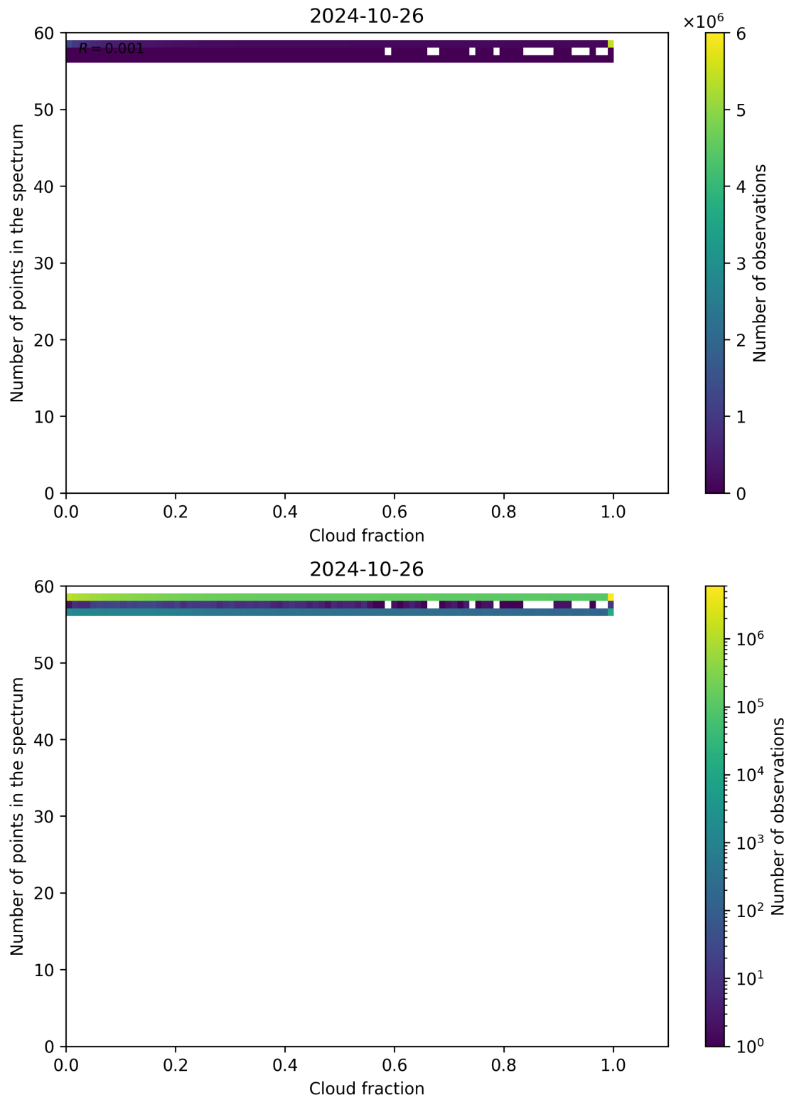
Figure 81: Scatter density plot of “Cloud fraction” against “Number of points in the spectrum” for 2024-10-25 to 2024-10-27.
