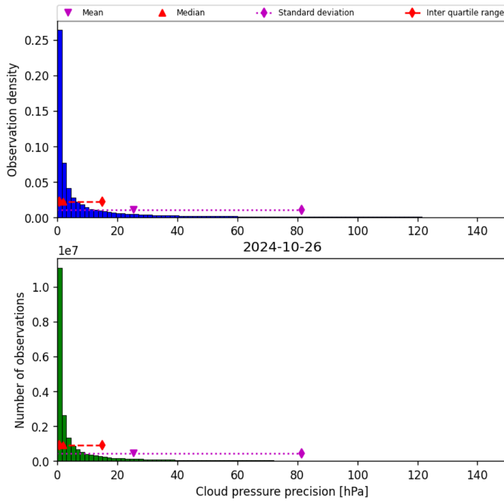
Figure 31: Histogram of “Cloud pressure precision” for 2024-10-25 to 2024-10-27
