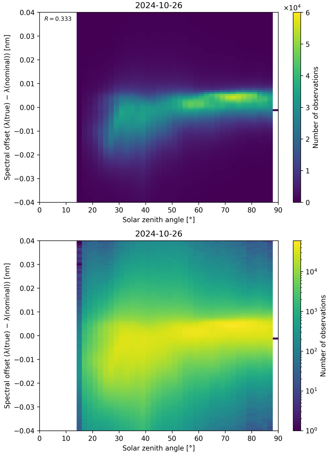
Figure 128: Scatter density plot of “Solar zenith angle” against “Spectral offset ( \lambda_{\text{true}} - \lambda_{\text{nominal}} )” for 2024-10-25 to 2024-10-27.
