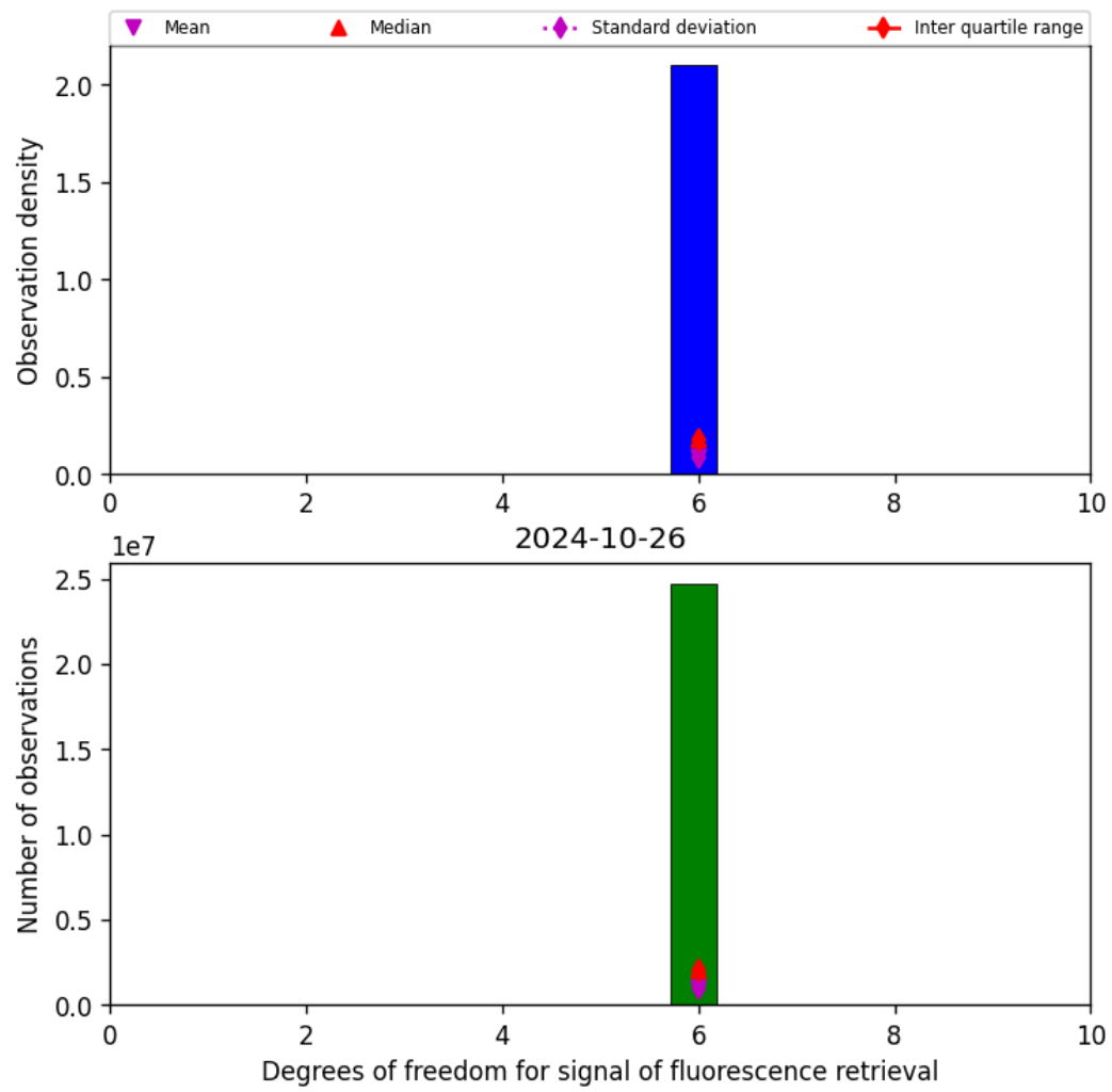
Figure 43: Histogram of “Degrees of freedom for signal of fluorescence retrieval” for 2024-10-25 to 2024-10-27
