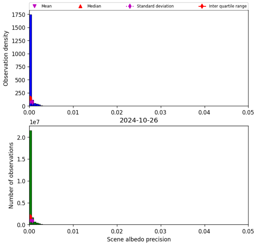
Figure 35: Histogram of “Scene albedo precision” for 2024-10-25 to 2024-10-27
