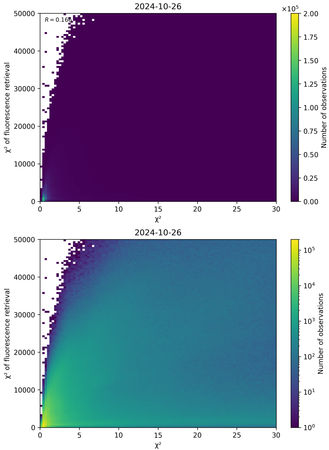
Figure 69: Scatter density plot of “ \chi^2 ” against “ \chi^2 of fluorescence retrieval” for 2024-10-25 to 2024-10-27.
