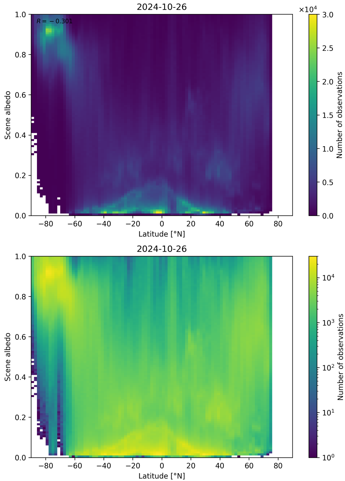
Figure 104: Scatter density plot of “Latitude” against “Scene albedo” for 2024-10-25 to 2024-10-27.
