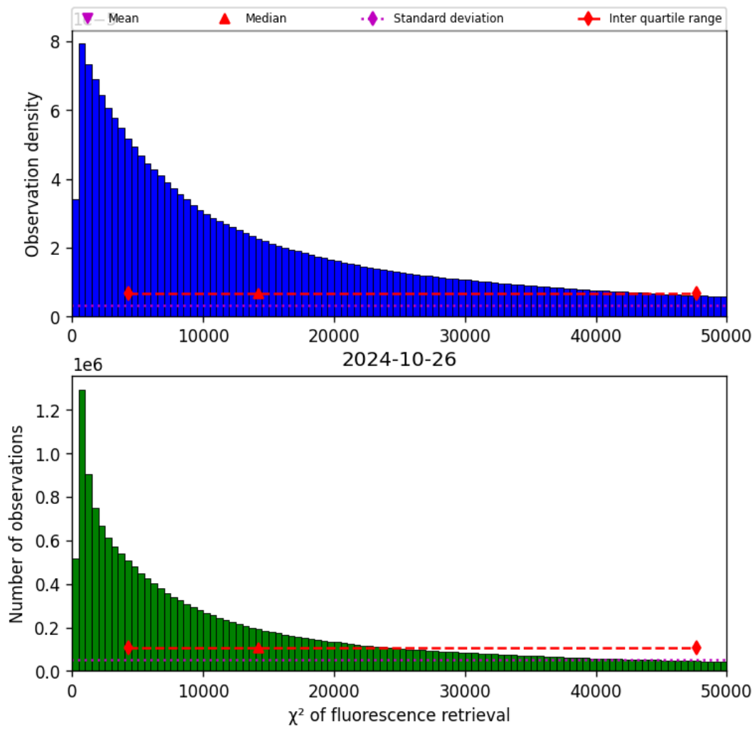
Figure 42: Histogram of “ \chi^2 of fluorescence retrieval” for 2024-10-25 to 2024-10-27
