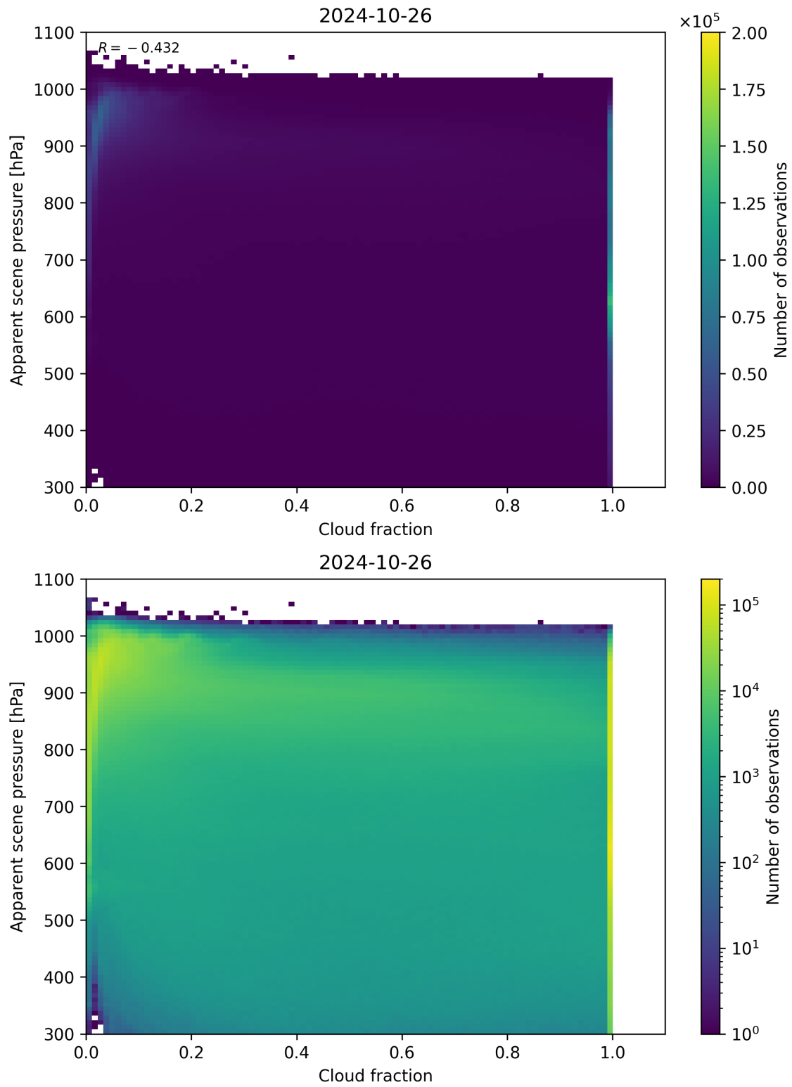
Figure 76: Scatter density plot of “Cloud fraction” against “Apparent scene pressure” for 2024-10-25 to 2024-10-27.
