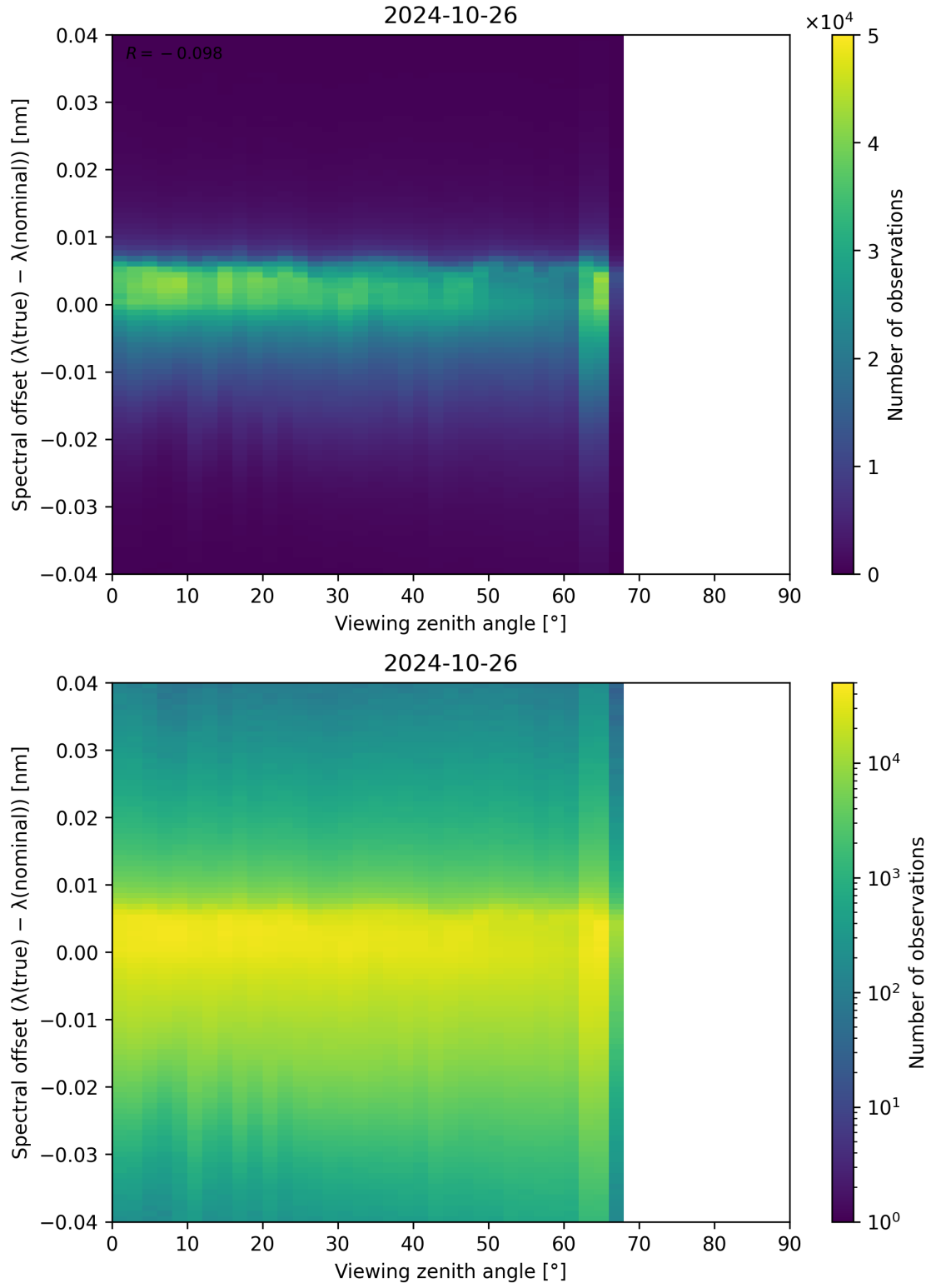
Figure 140: Scatter density plot of “Viewing zenith angle” against “Spectral offset ( \lambda_{\text{true}} - \lambda_{\text{nominal}} )” for 2024-10-25 to 2024-10-27.
