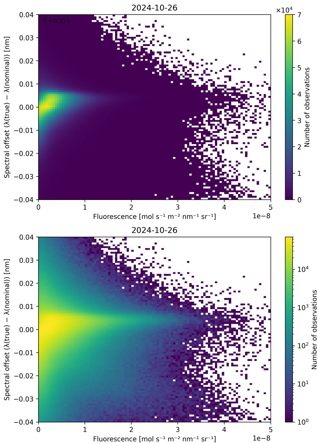
Figure 95: Scatter density plot of “Fluorescence” against “Spectral offset ( \lambda_{\text{true}} - \lambda_{\text{nominal}} )” for 2024-10-25 to 2024-10-27.
