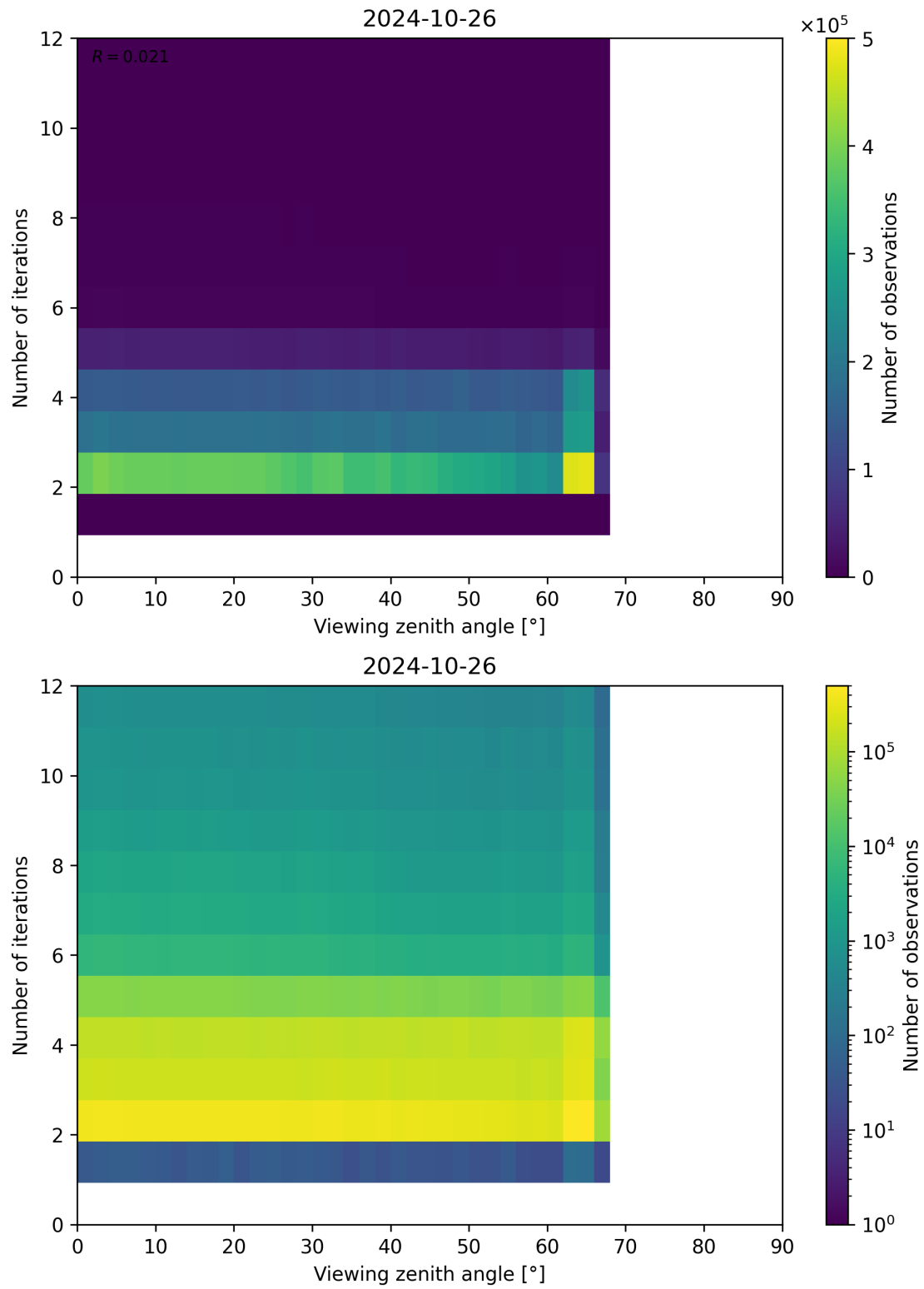
Figure 136: Scatter density plot of “Viewing zenith angle” against “Number of iterations” for 2024-10-25 to 2024-10-27.
