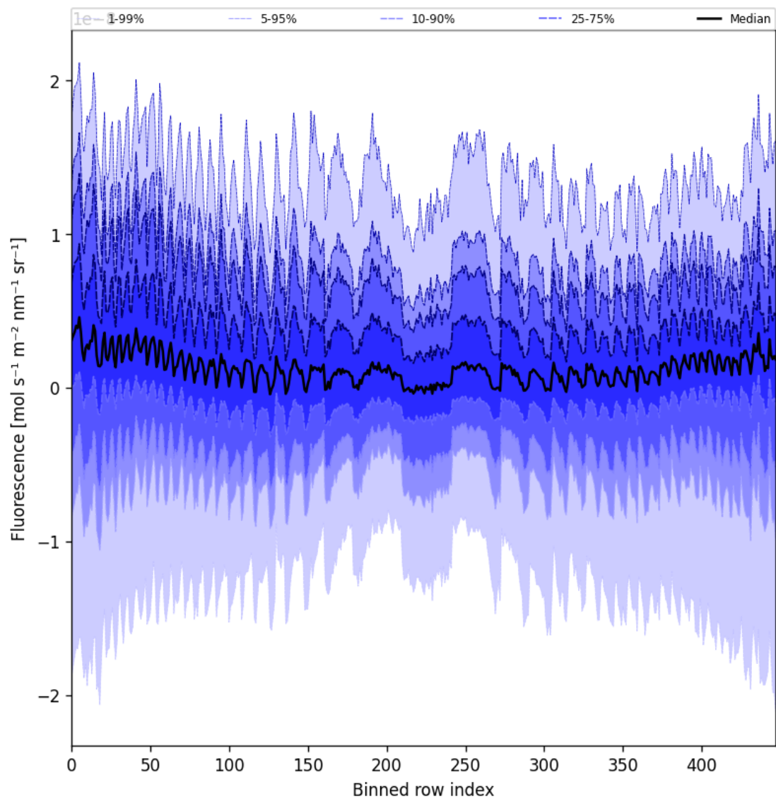
Figure 57: Along track statistics of “Fluorescence” for 2024-10-25 to 2024-10-27
