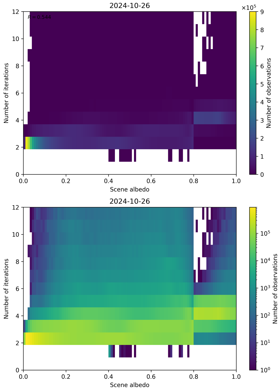
Figure 115: Scatter density plot of “Scene albedo” against “Number of iterations” for 2024-10-25 to 2024-10-27.
