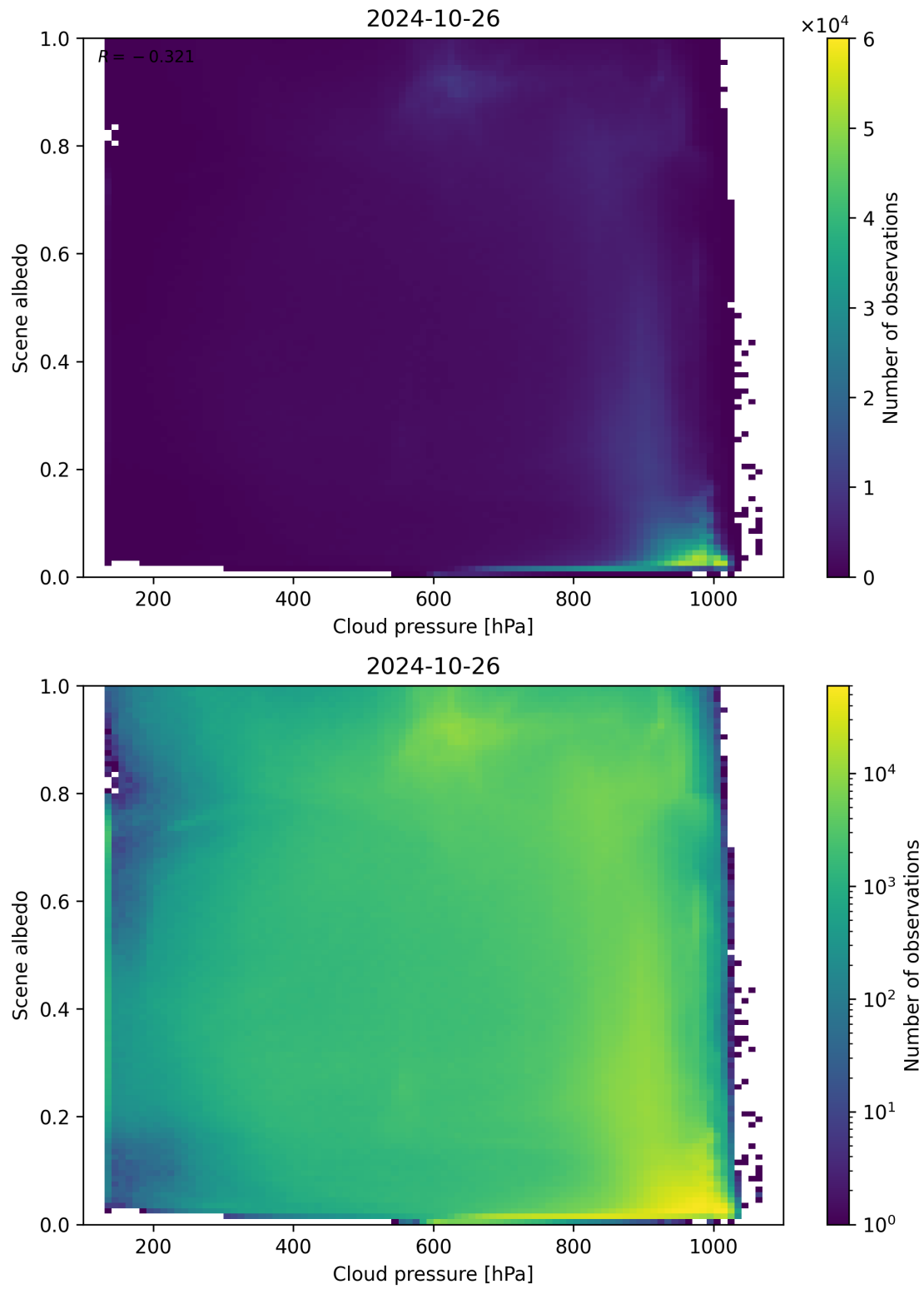
Figure 91: Scatter density plot of “Cloud pressure” against “Scene albedo” for 2024-10-25 to 2024-10-27.
