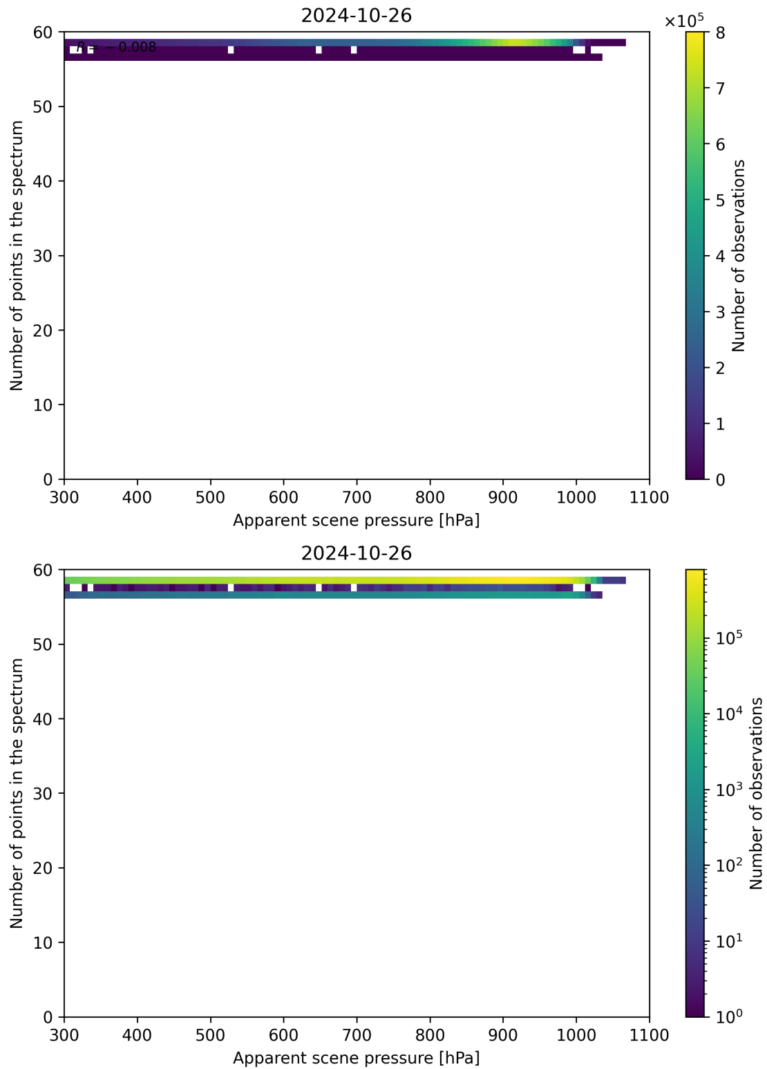
Figure 67: Scatter density plot of “Apparent scene pressure” against “Number of points in the spectrum” for 2024-10-25 to 2024-10-27.
