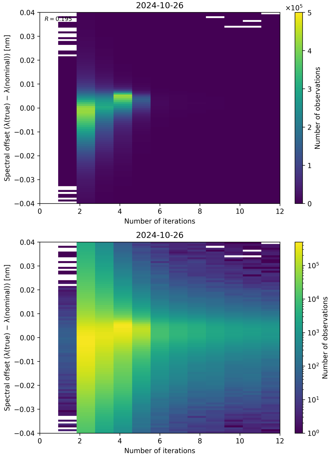
Figure 109: Scatter density plot of “Number of iterations” against “Spectral offset ( \lambda_{\text{true}} - \lambda_{\text{nominal}} )” for 2024-10-25 to 2024-10-27.
