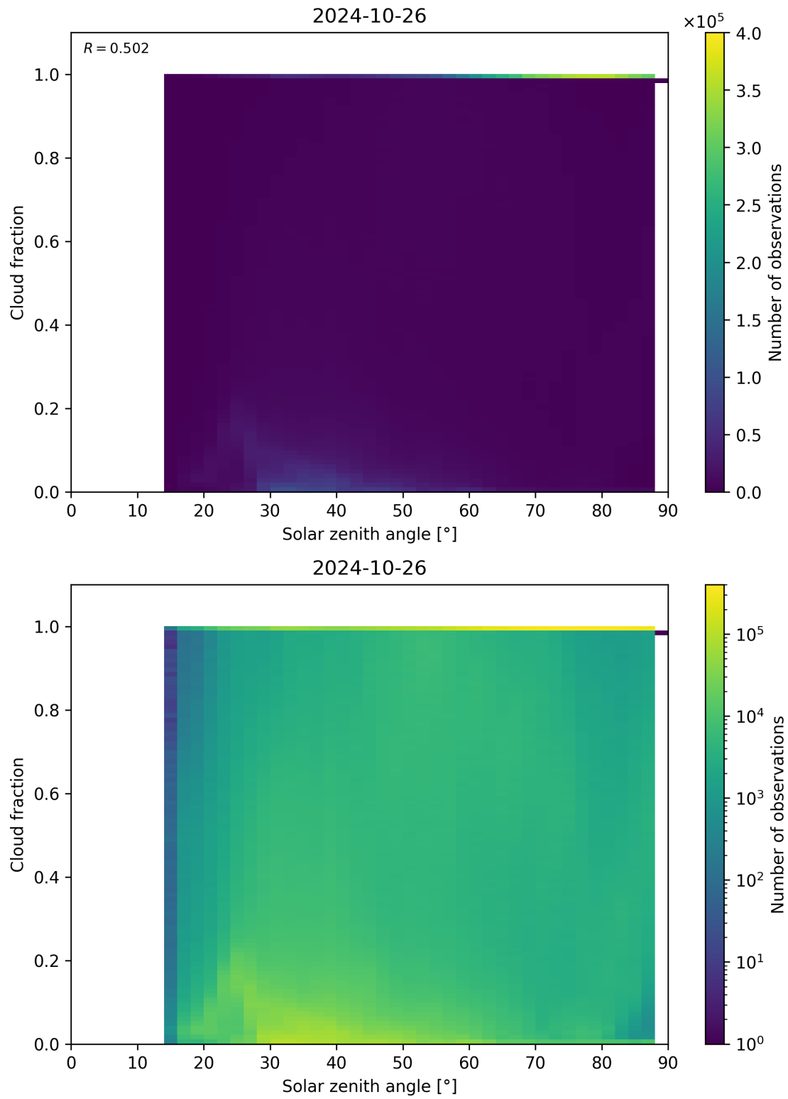
Figure 121: Scatter density plot of “Solar zenith angle” against “Cloud fraction” for 2024-10-25 to 2024-10-27.
