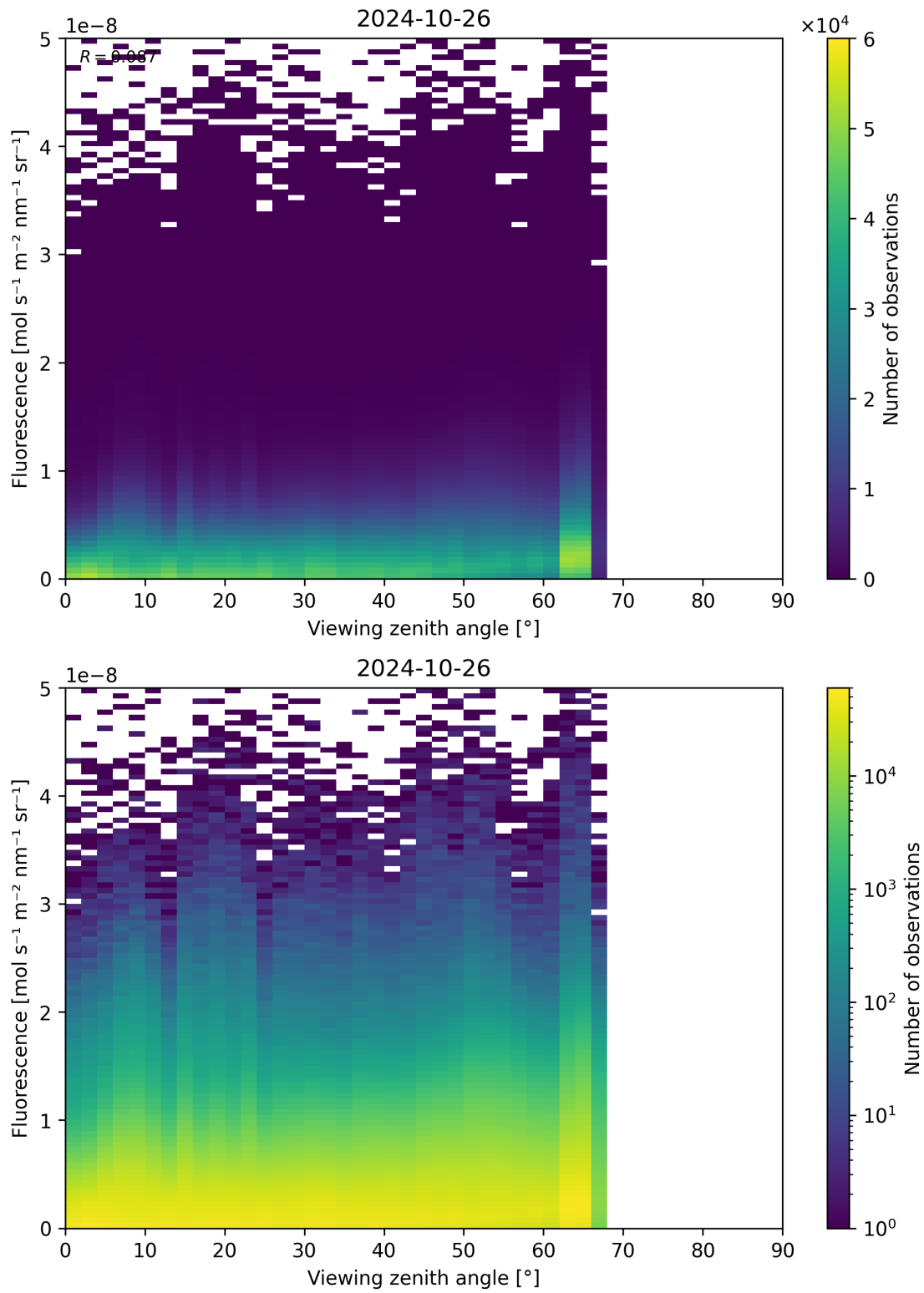
Figure 134: Scatter density plot of “Viewing zenith angle” against “Fluorescence” for 2024-10-25 to 2024-10-27.
