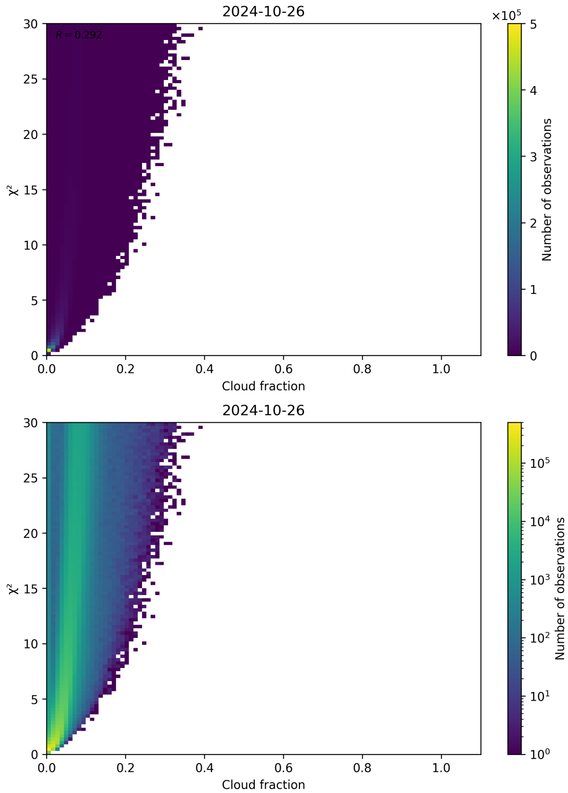
Figure 77: Scatter density plot of “Cloud fraction” against “ \chi^2 ” for 2024-10-25 to 2024-10-27.
