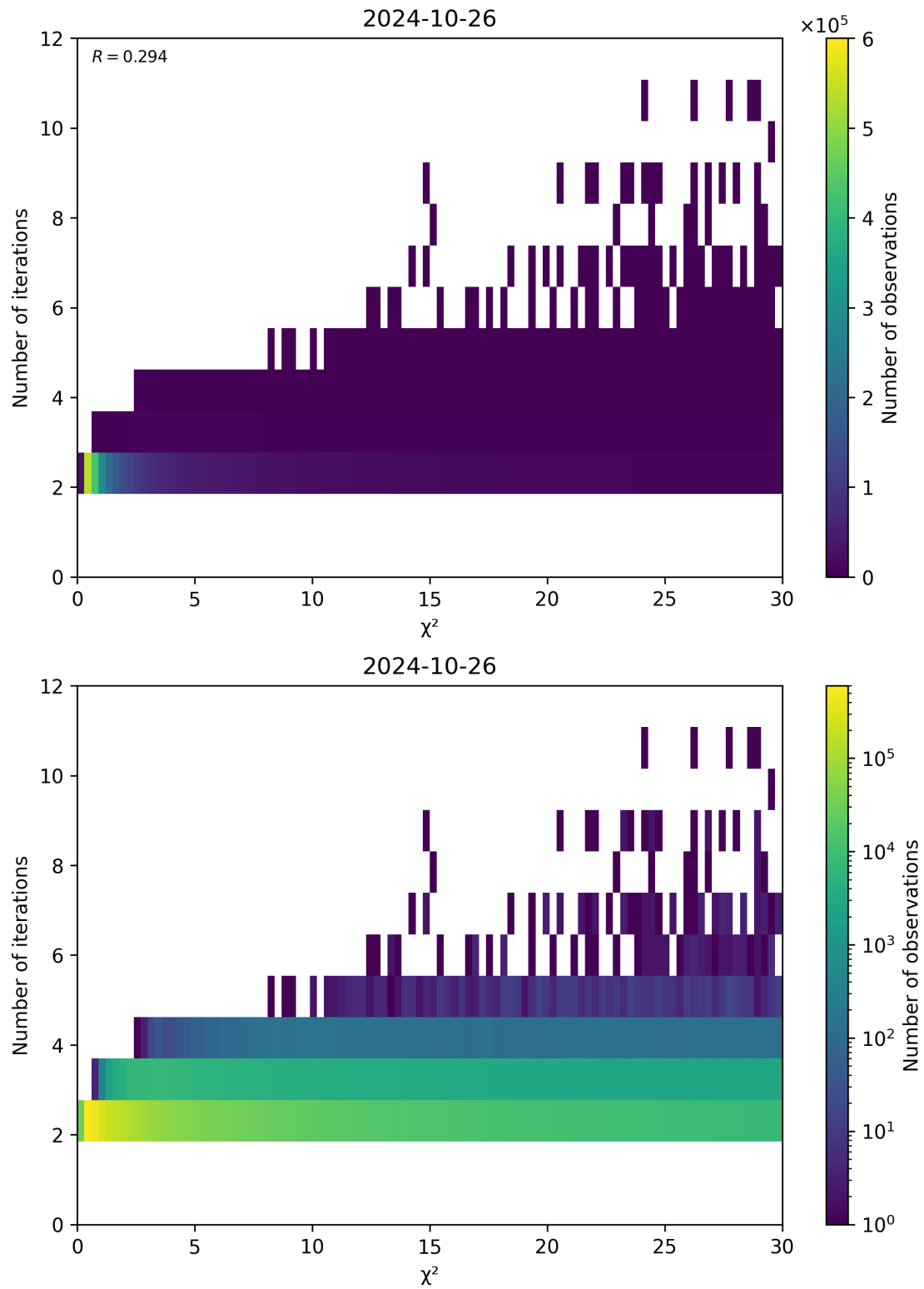
Figure 73: Scatter density plot of “ \chi^2 ” against “Number of iterations” for 2024-10-25 to 2024-10-27.
