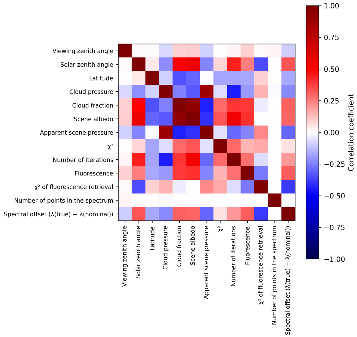
Figure 2: Map of correlation matrix for 2024-10-25 to 2024-10-27.
