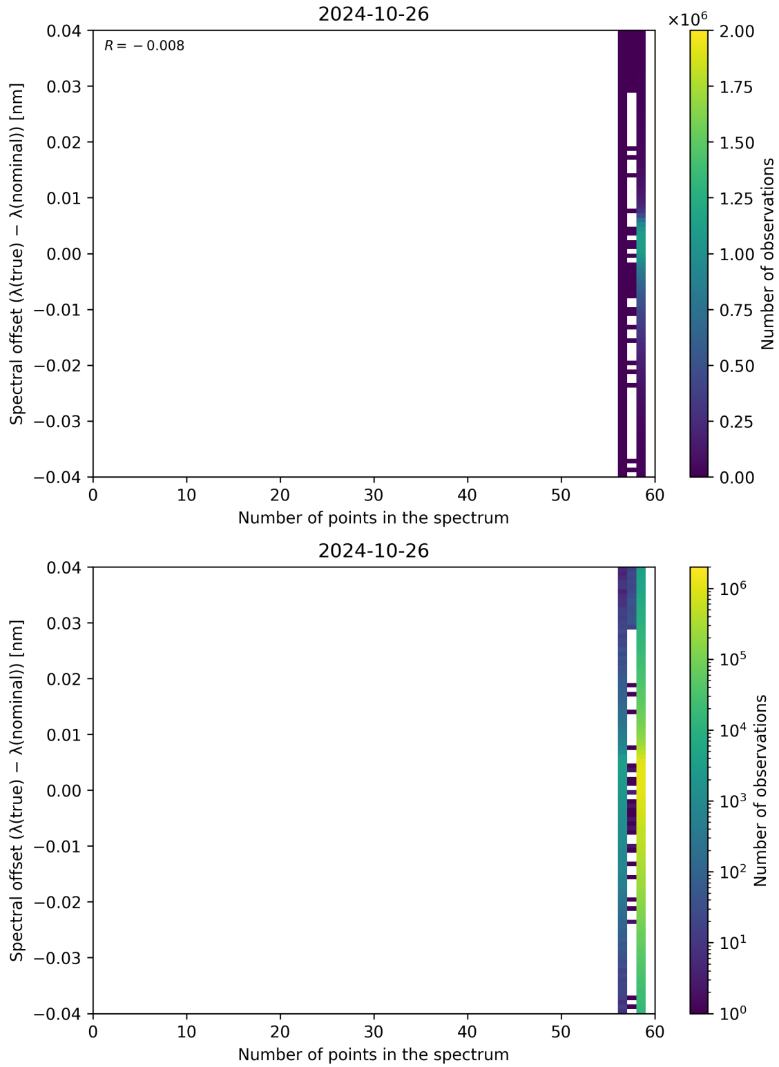
Figure 110: Scatter density plot of “Number of points in the spectrum” against “Spectral offset ( \lambda_{\text{true}} - \lambda_{\text{nominal}} )” for 2024-10-25 to 2024-10-27.
