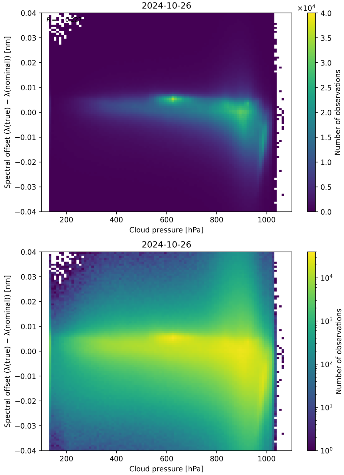
Figure 92: Scatter density plot of “Cloud pressure” against “Spectral offset ( \lambda_{\text{true}} - \lambda_{\text{nominal}} )” for 2024-10-25 to 2024-10-27.
