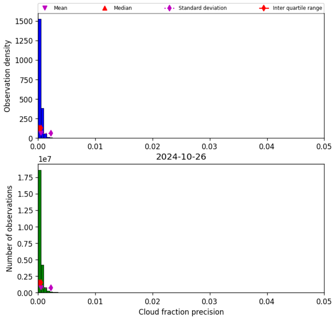
Figure 33: Histogram of “Cloud fraction precision” for 2024-10-25 to 2024-10-27
