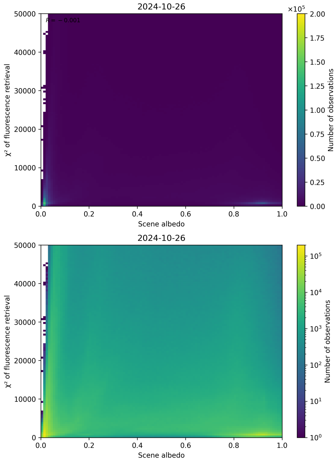
Figure 113: Scatter density plot of “Scene albedo” against “ \chi^2 of fluorescence retrieval” for 2024-10-25 to 2024-10-27.
