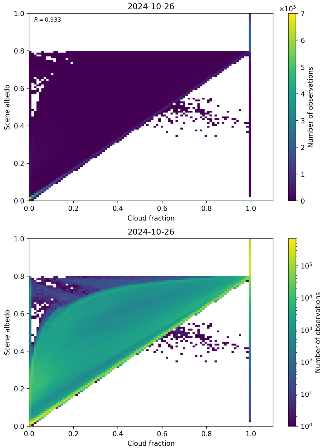
Figure 82: Scatter density plot of “Cloud fraction” against “Scene albedo” for 2024-10-25 to 2024-10-27.
