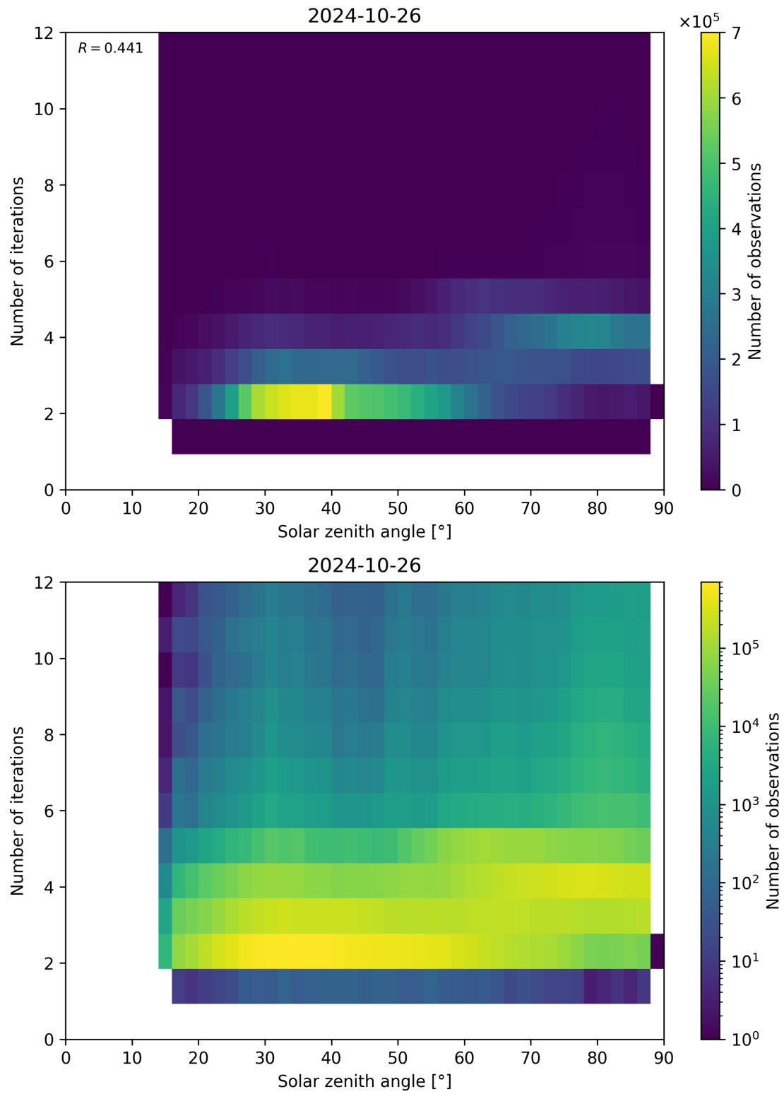
Figure 125: Scatter density plot of “Solar zenith angle” against “Number of iterations” for 2024-10-25 to 2024-10-27.
