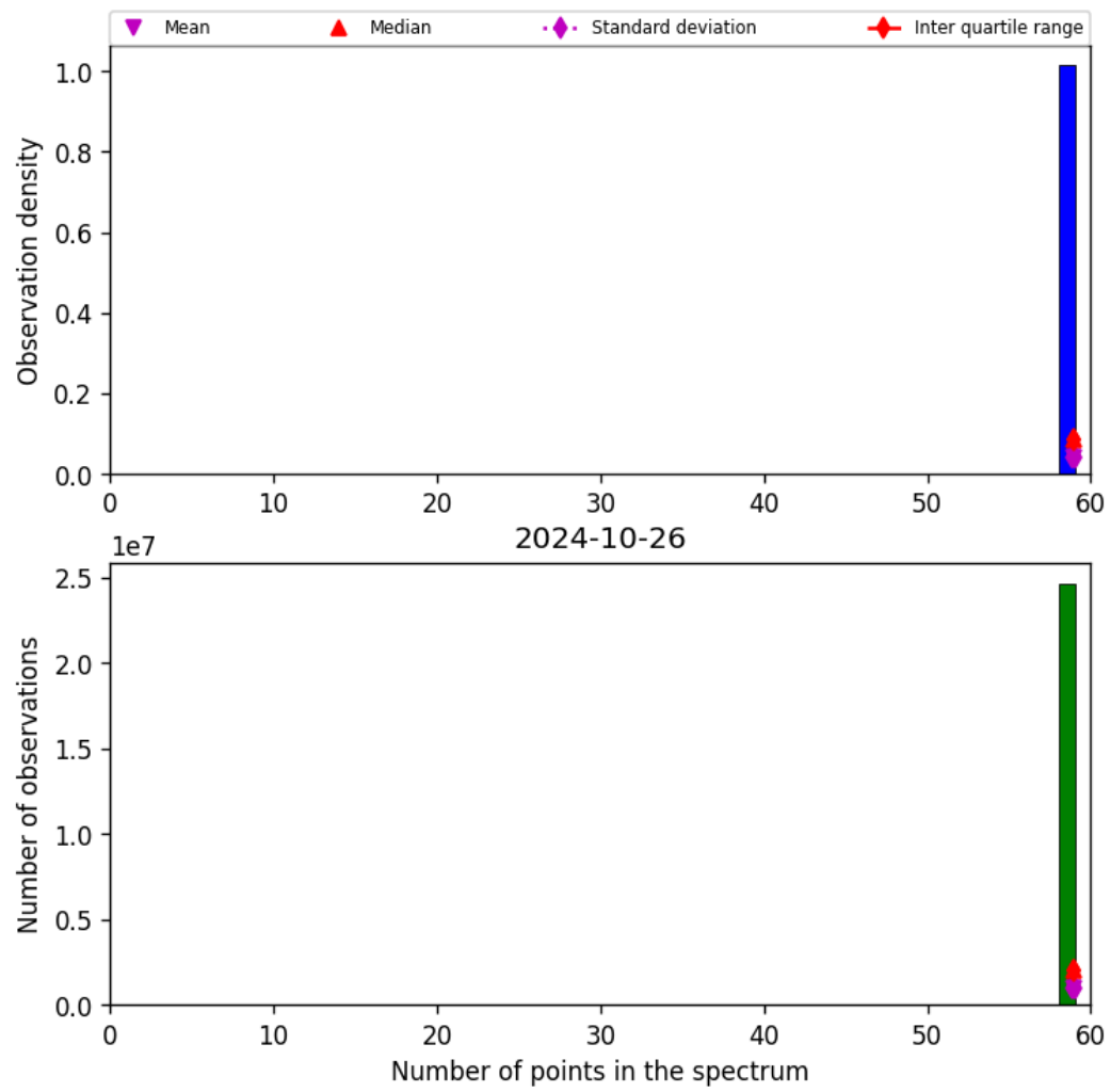
Figure 44: Histogram of “Number of points in the spectrum” for 2024-10-25 to 2024-10-27
