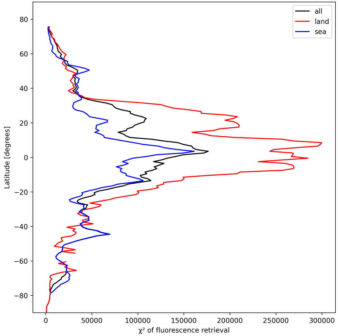
Figure 25: Zonal average of “ \chi^2 of fluorescence retrieval” for 2024-10-25 to 2024-10-27.
