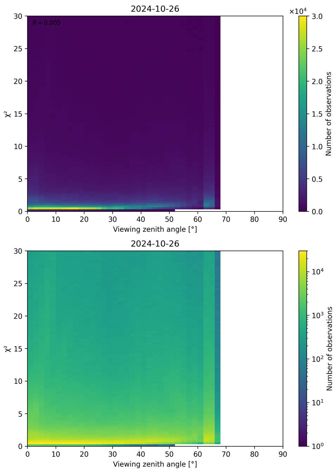
Figure 130: Scatter density plot of “Viewing zenith angle” against “ \chi^2 ” for 2024-10-25 to 2024-10-27.
