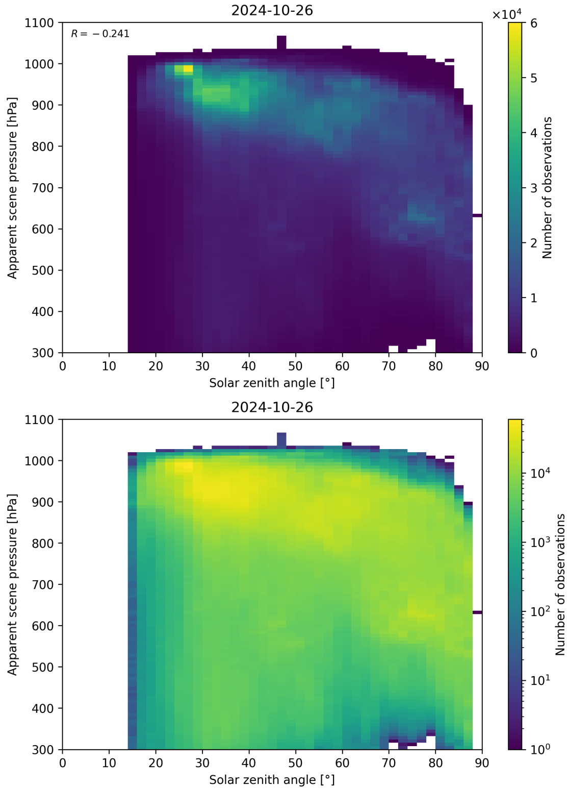
Figure 118: Scatter density plot of “Solar zenith angle” against “Apparent scene pressure” for 2024-10-25 to 2024-10-27.
