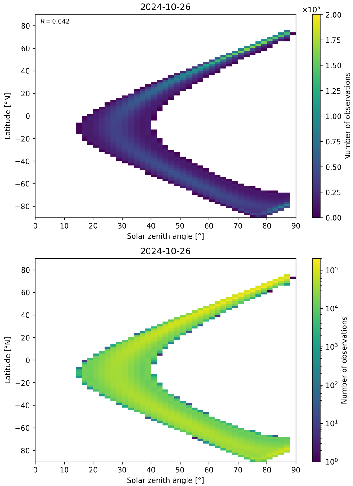
Figure 124: Scatter density plot of “Solar zenith angle” against “Latitude” for 2024-10-25 to 2024-10-27.
