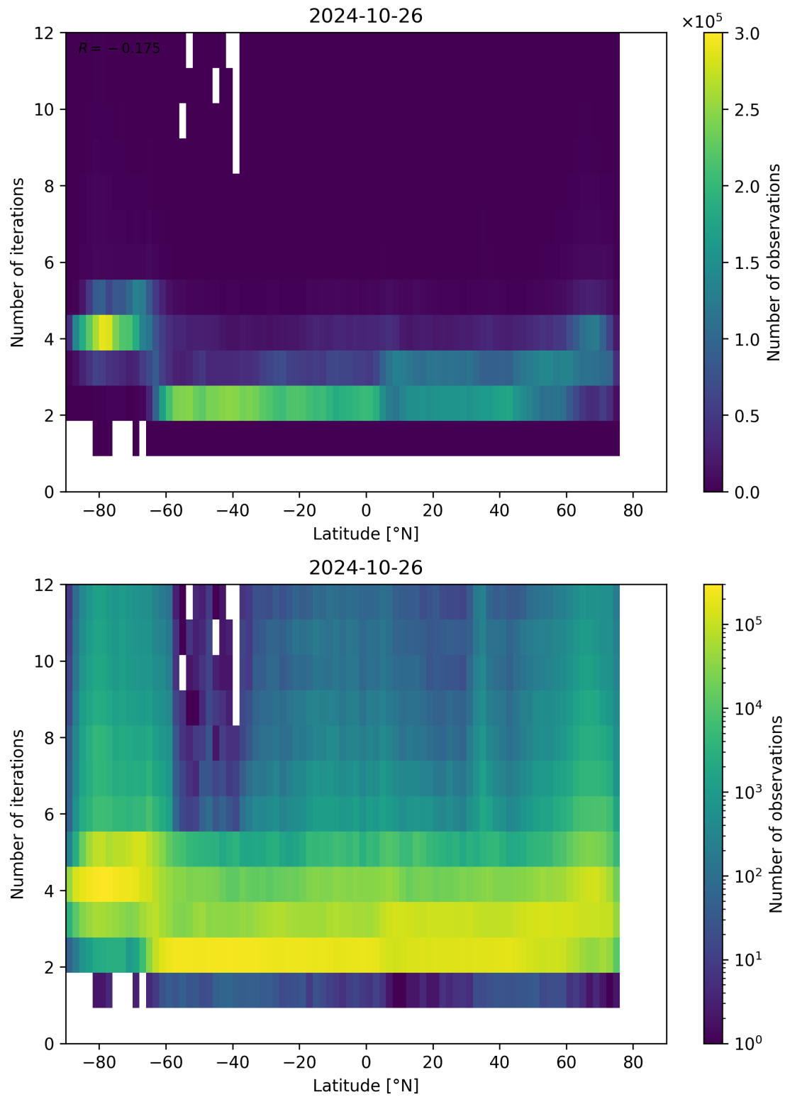
Figure 102: Scatter density plot of “Latitude” against “Number of iterations” for 2024-10-25 to 2024-10-27.
