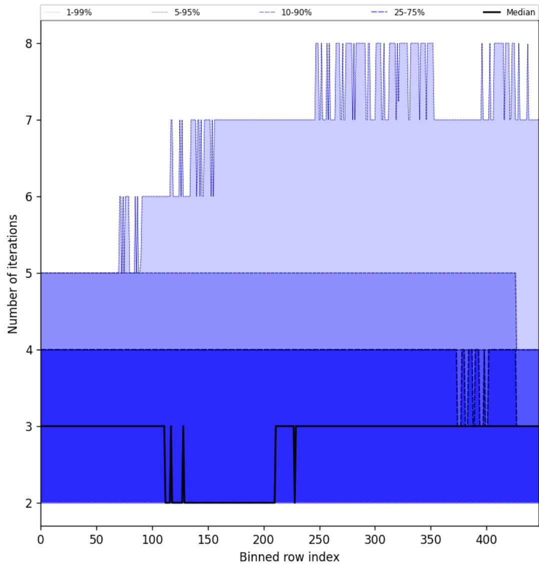
Figure 56: Along track statistics of “Number of iterations” for 2024-10-25 to 2024-10-27
