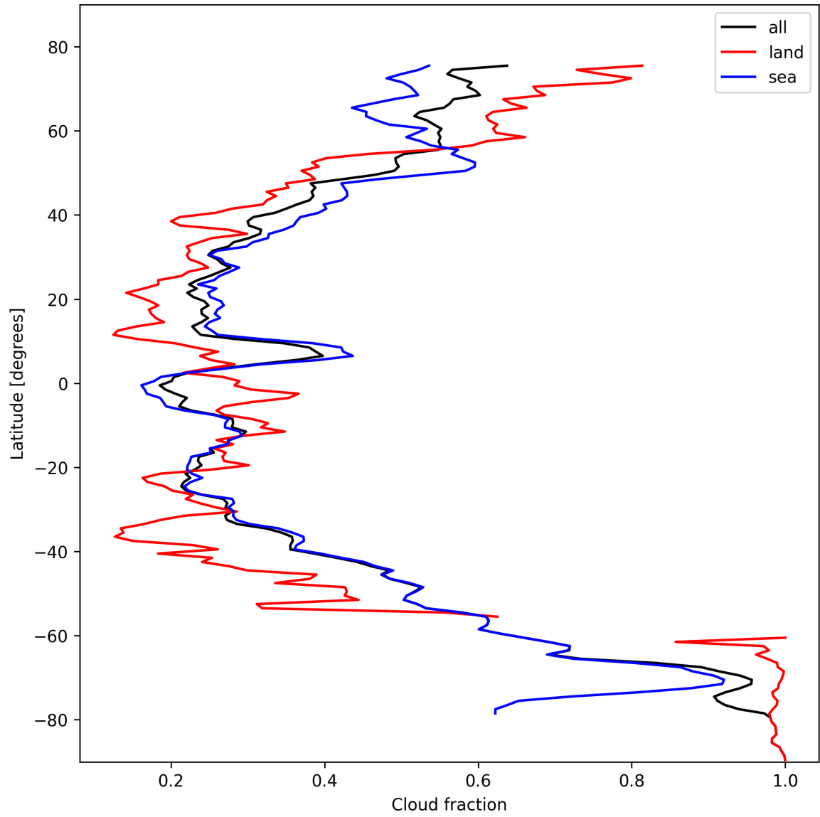
Figure 15: Zonal average of “Cloud fraction” for 2024-10-25 to 2024-10-27.
