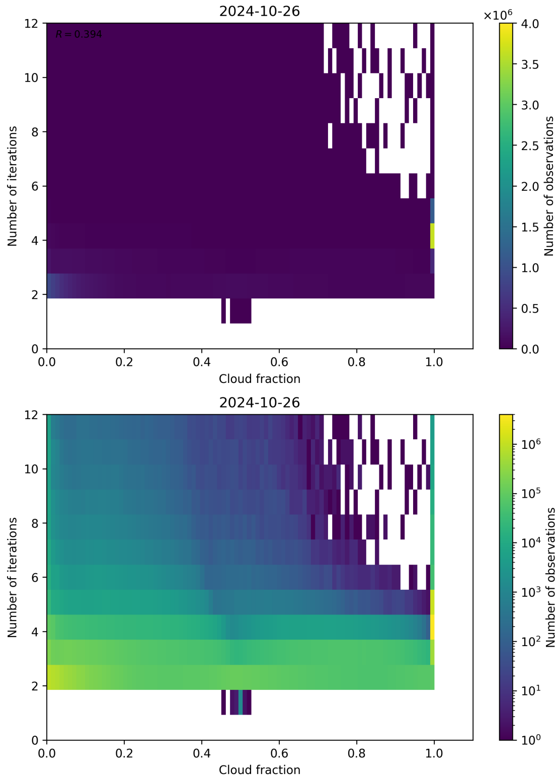
Figure 80: Scatter density plot of “Cloud fraction” against “Number of iterations” for 2024-10-25 to 2024-10-27.
