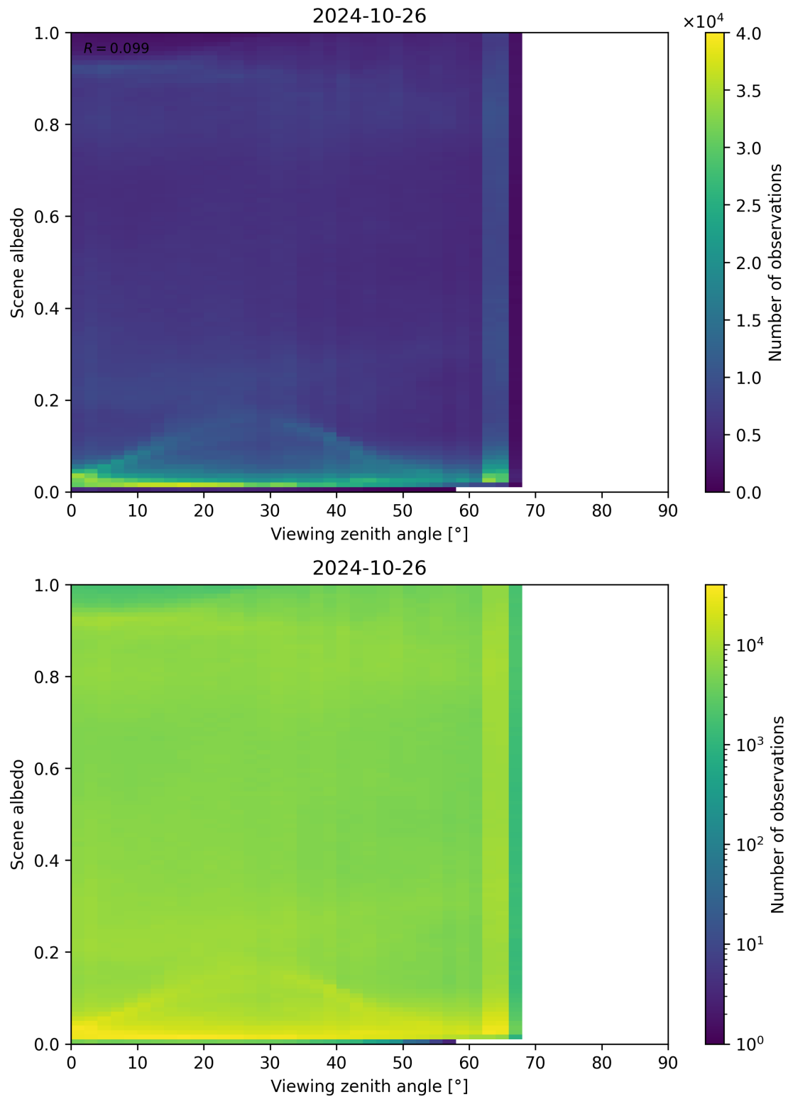
Figure 138: Scatter density plot of “Viewing zenith angle” against “Scene albedo” for 2024-10-25 to 2024-10-27.
