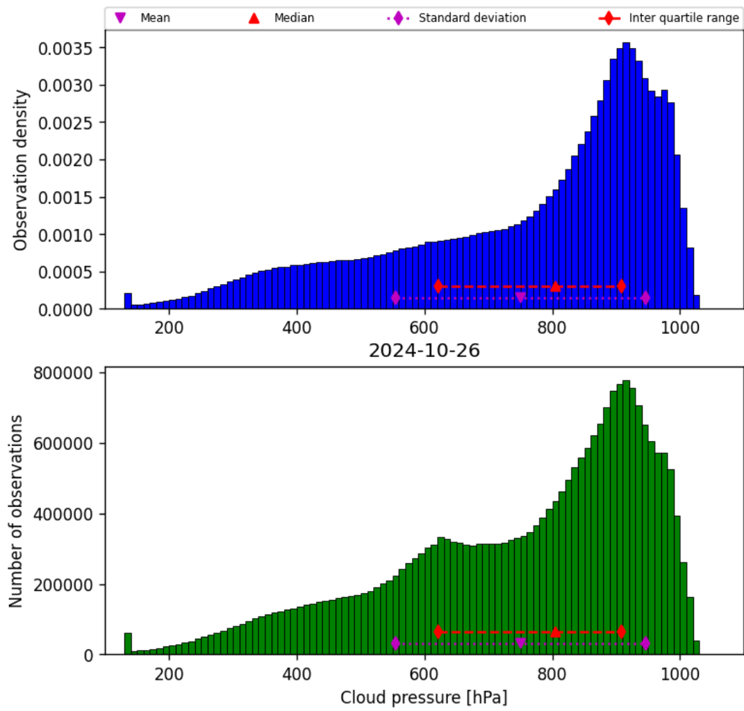
Figure 30: Histogram of “Cloud pressure” for 2024-10-25 to 2024-10-27
