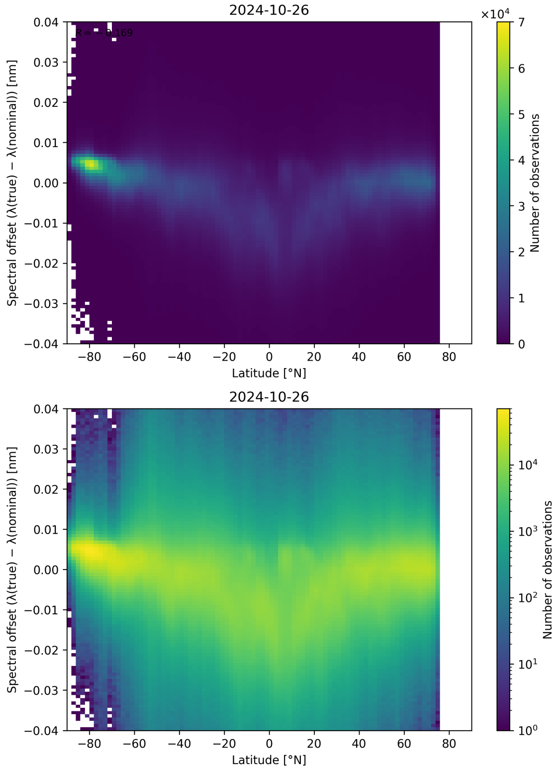
Figure 105: Scatter density plot of “Latitude” against “Spectral offset ( \lambda_{\text{true}} - \lambda_{\text{nominal}} )” for 2024-10-25 to 2024-10-27.
