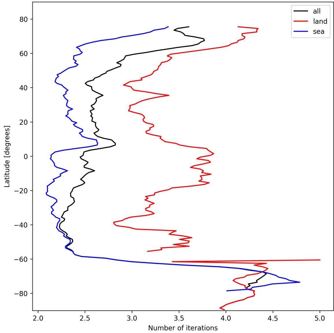
Figure 22: Zonal average of “Number of iterations” for 2024-10-25 to 2024-10-27.
