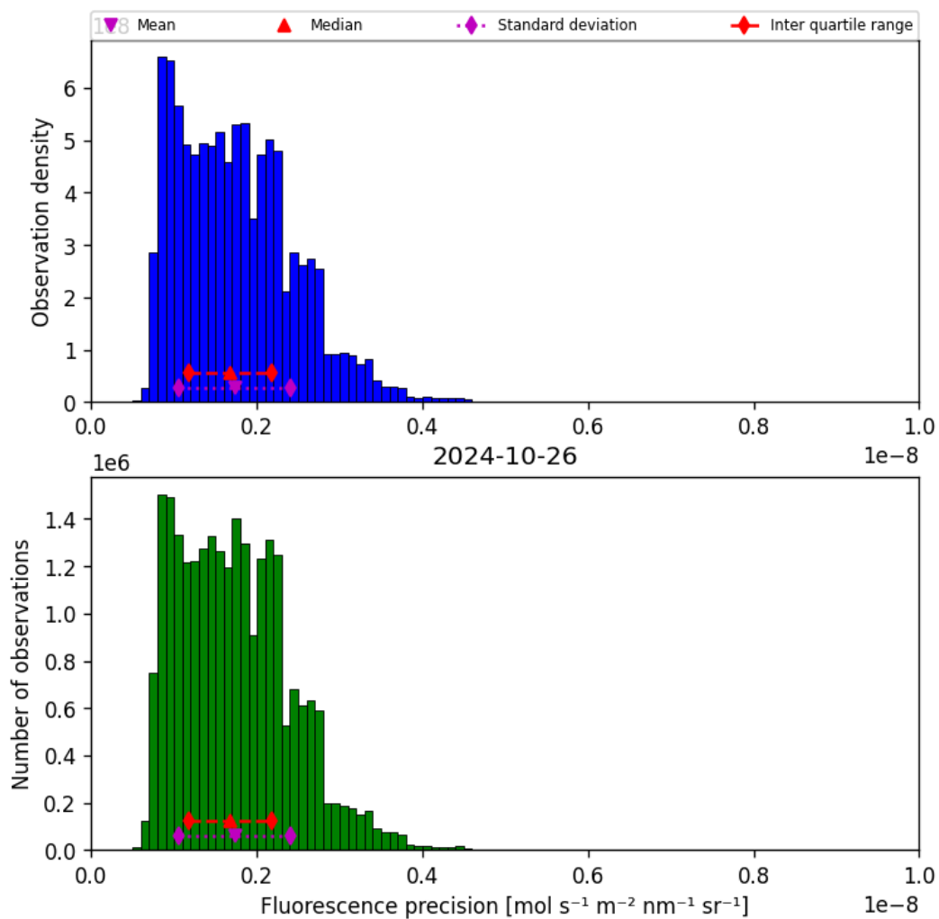
Figure 41: Histogram of “Fluorescence precision” for 2024-10-25 to 2024-10-27
