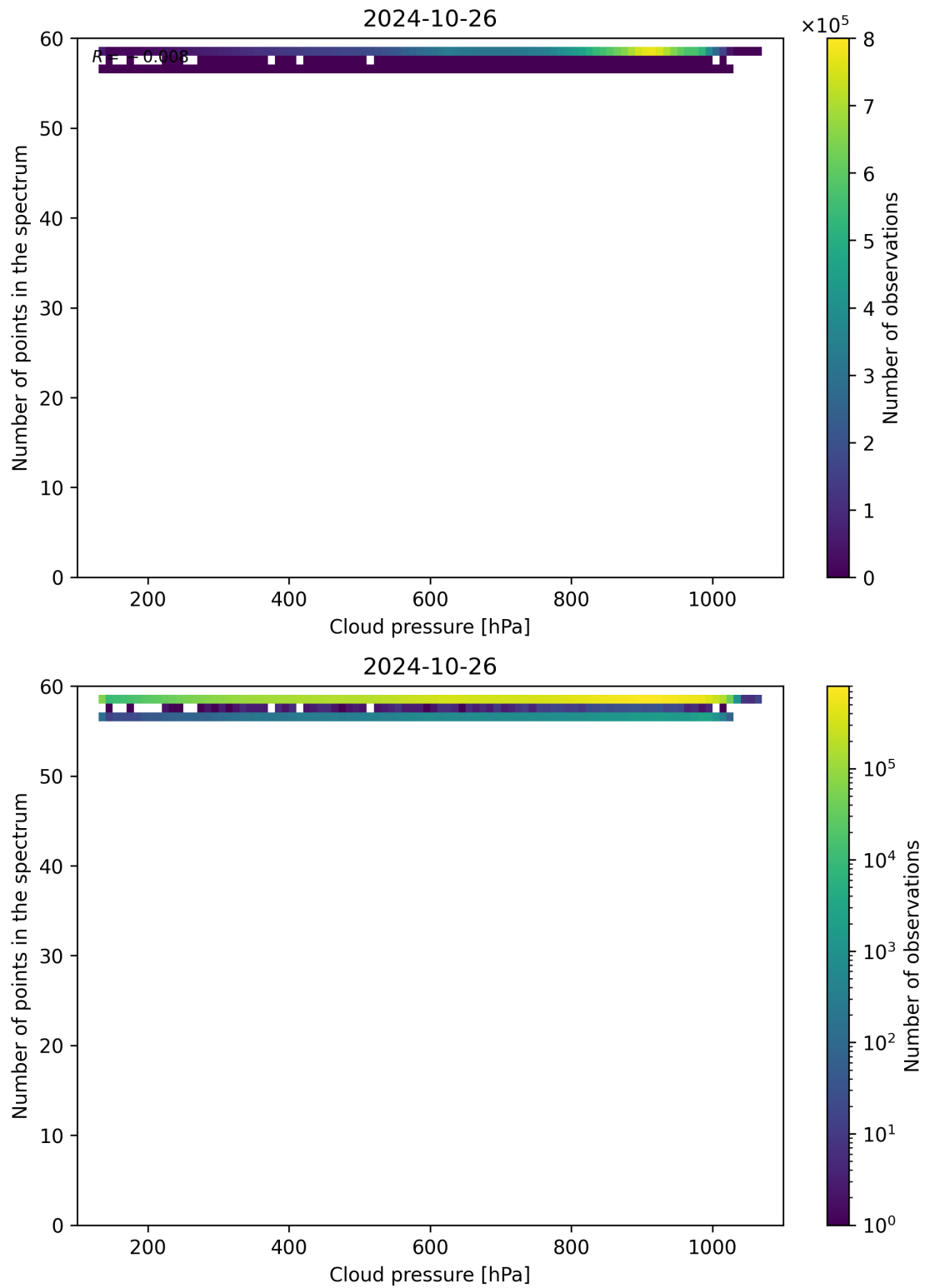
Figure 90: Scatter density plot of “Cloud pressure” against “Number of points in the spectrum” for 2024-10-25 to 2024-10-27.
