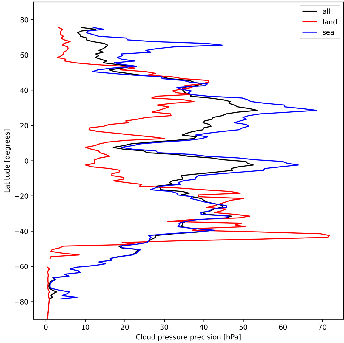
Figure 14: Zonal average of “Cloud pressure precision” for 2024-10-25 to 2024-10-27.
