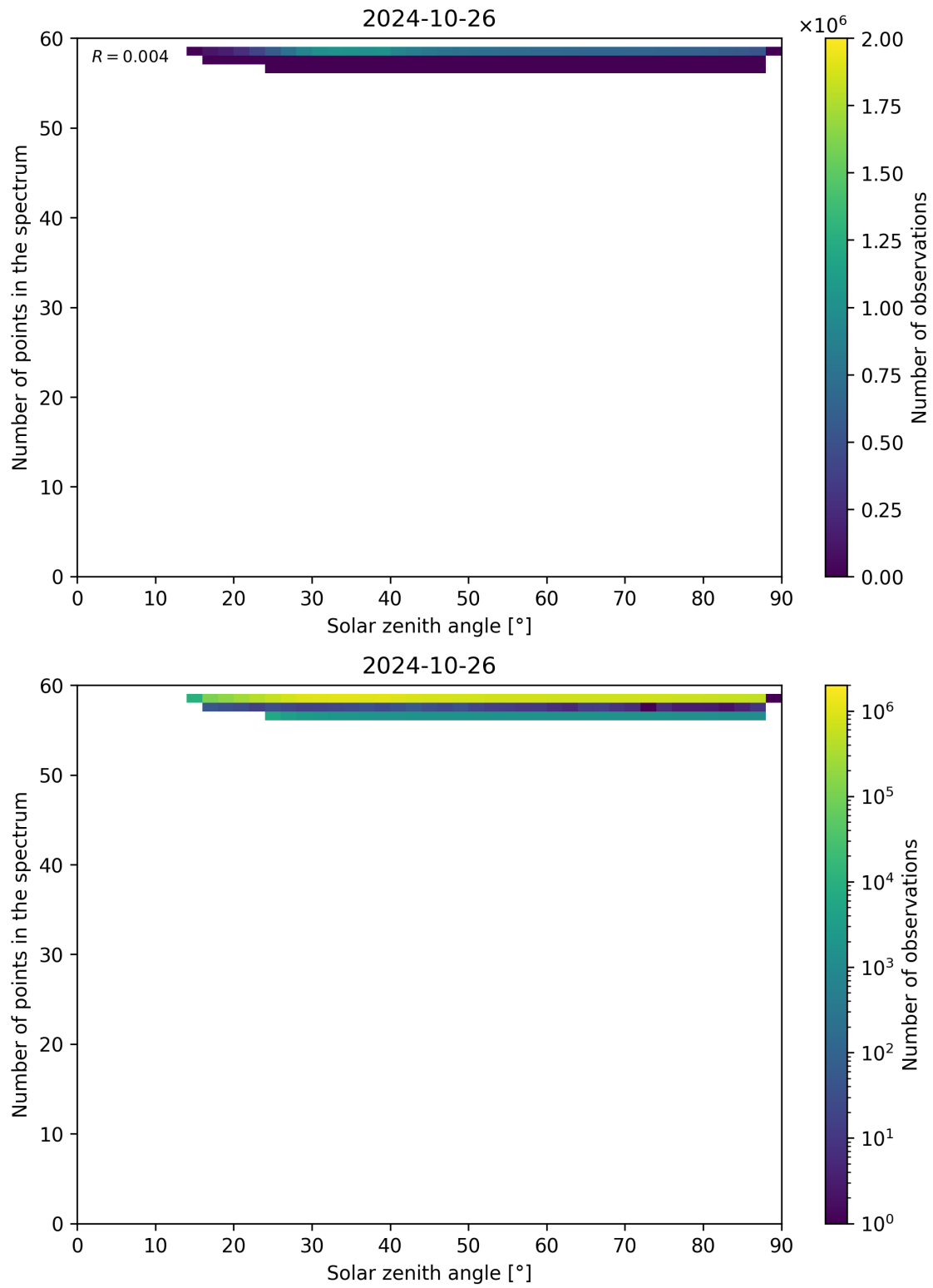
Figure 126: Scatter density plot of “Solar zenith angle” against “Number of points in the spectrum” for 2024-10-25 to 2024-10-27.
