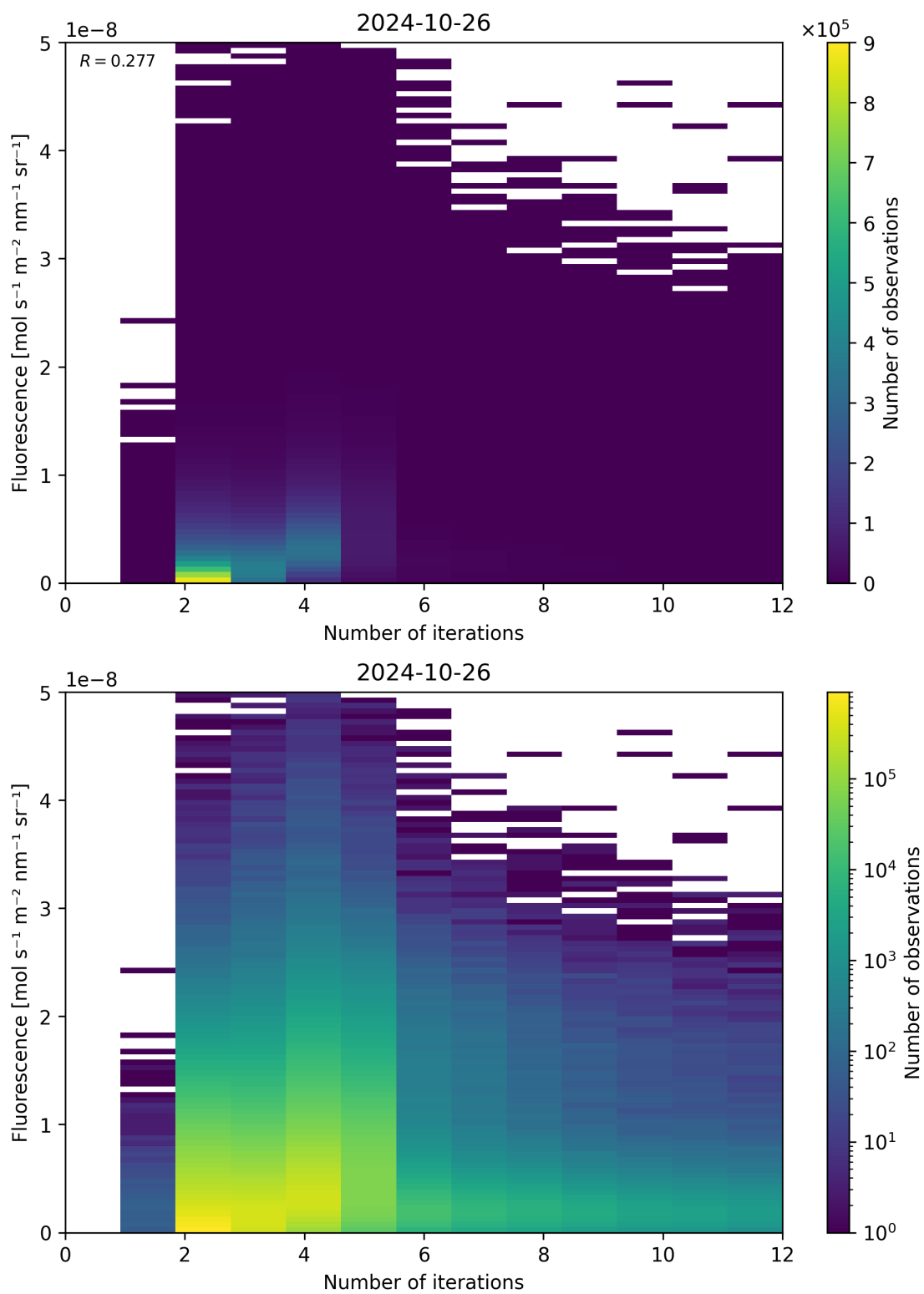
Figure 107: Scatter density plot of “Number of iterations” against “Fluorescence” for 2024-10-25 to 2024-10-27.
