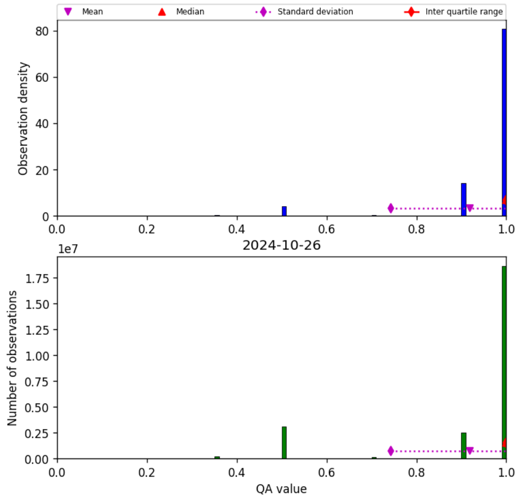
Figure 29: Histogram of “QA value” for 2024-10-25 to 2024-10-27
