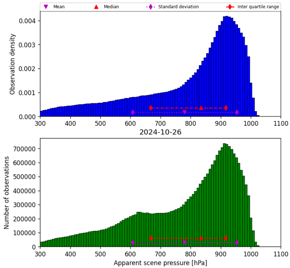
Figure 36: Histogram of “Apparent scene pressure” for 2024-10-25 to 2024-10-27
