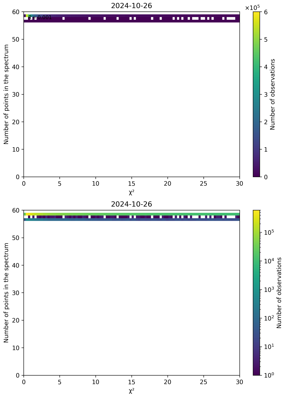
Figure 74: Scatter density plot of " \chi^2 " against "Number of points in the spectrum" for 2024-10-25 to 2024-10-27.
