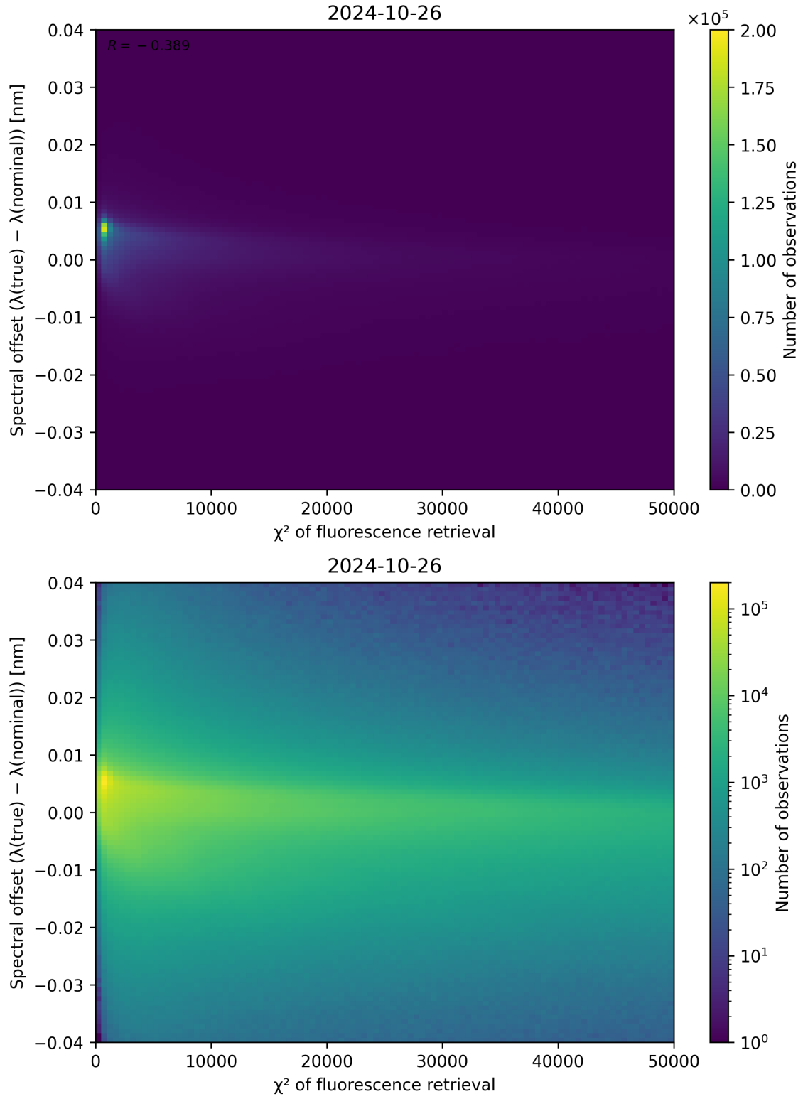
Figure 72: Scatter density plot of “ \chi^2 of fluorescence retrieval” against “Spectral offset ( \lambda_{\text{true}} - \lambda_{\text{nominal}} )” for 2024-10-25 to 2024-10-27.
