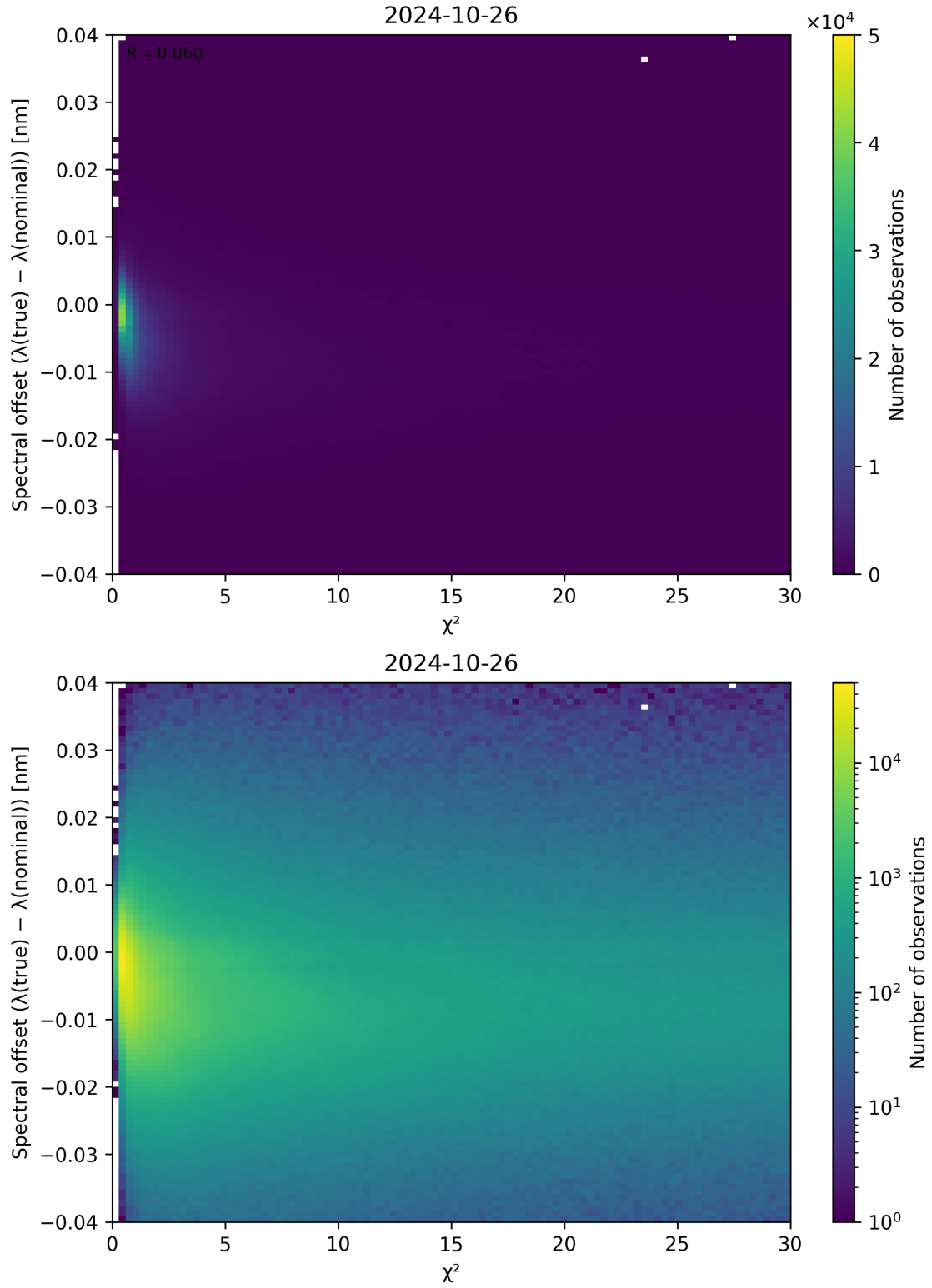
Figure 75: Scatter density plot of “ \chi^2 ” against “Spectral offset ( \lambda_{\text{true}} - \lambda_{\text{nominal}} )” for 2024-10-25 to 2024-10-27.
