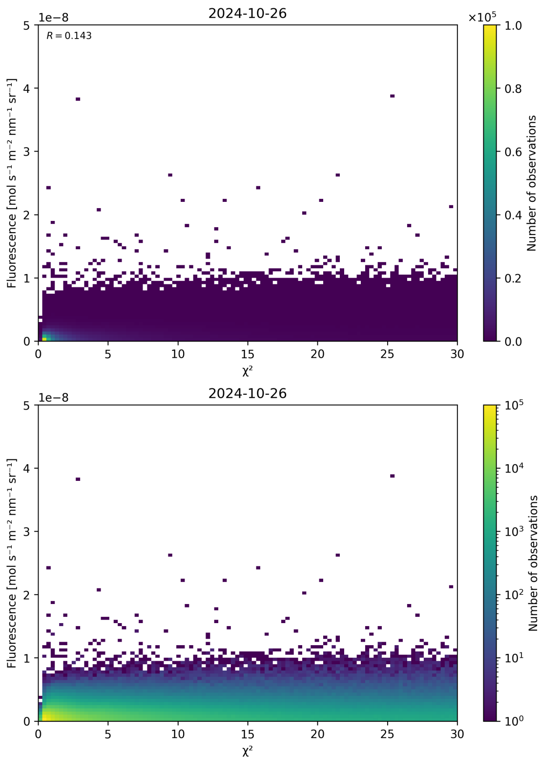
Figure 70: Scatter density plot of “ \chi^2 ” against “Fluorescence” for 2024-10-25 to 2024-10-27.
