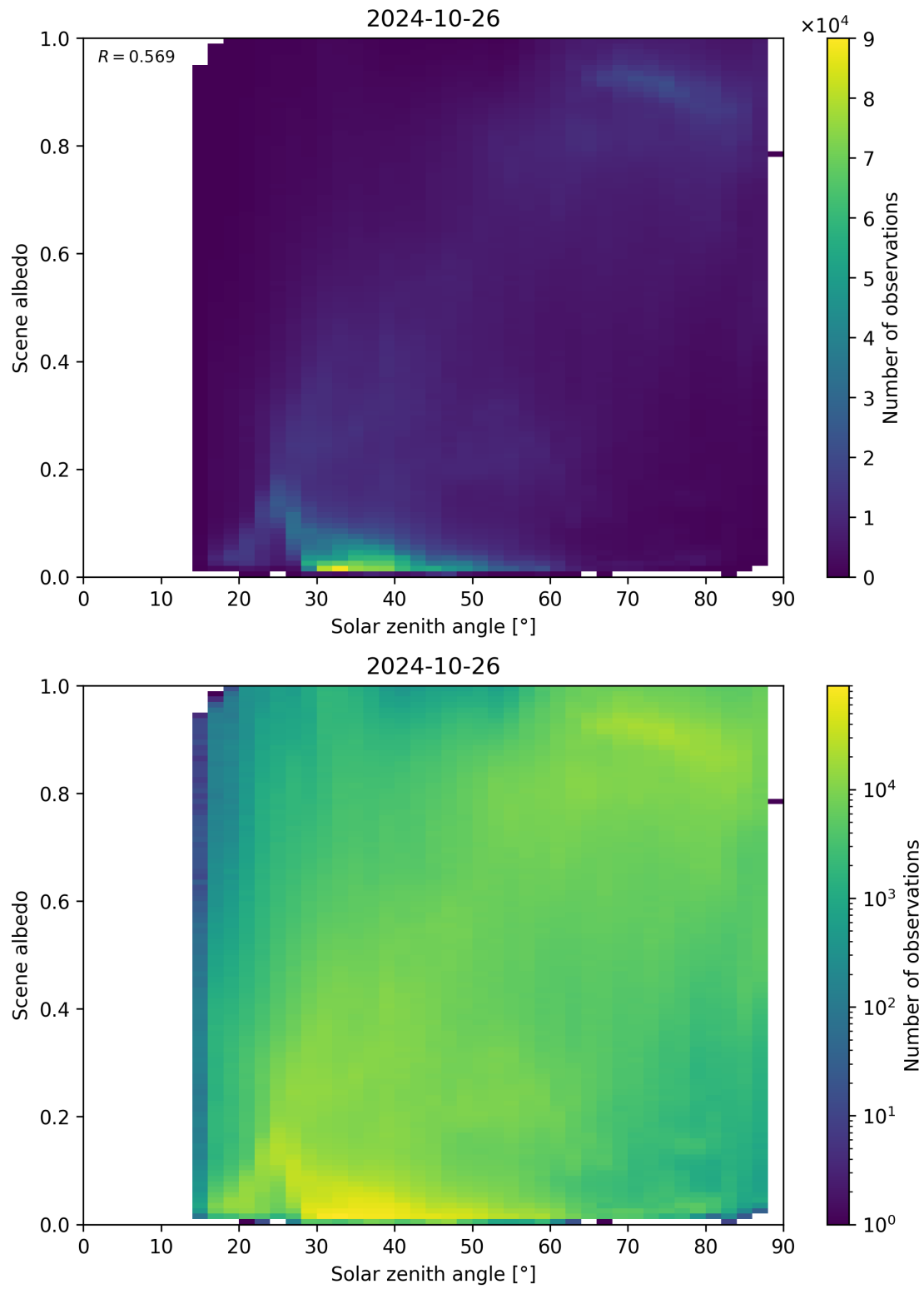
Figure 127: Scatter density plot of “Solar zenith angle” against “Scene albedo” for 2024-10-25 to 2024-10-27.
