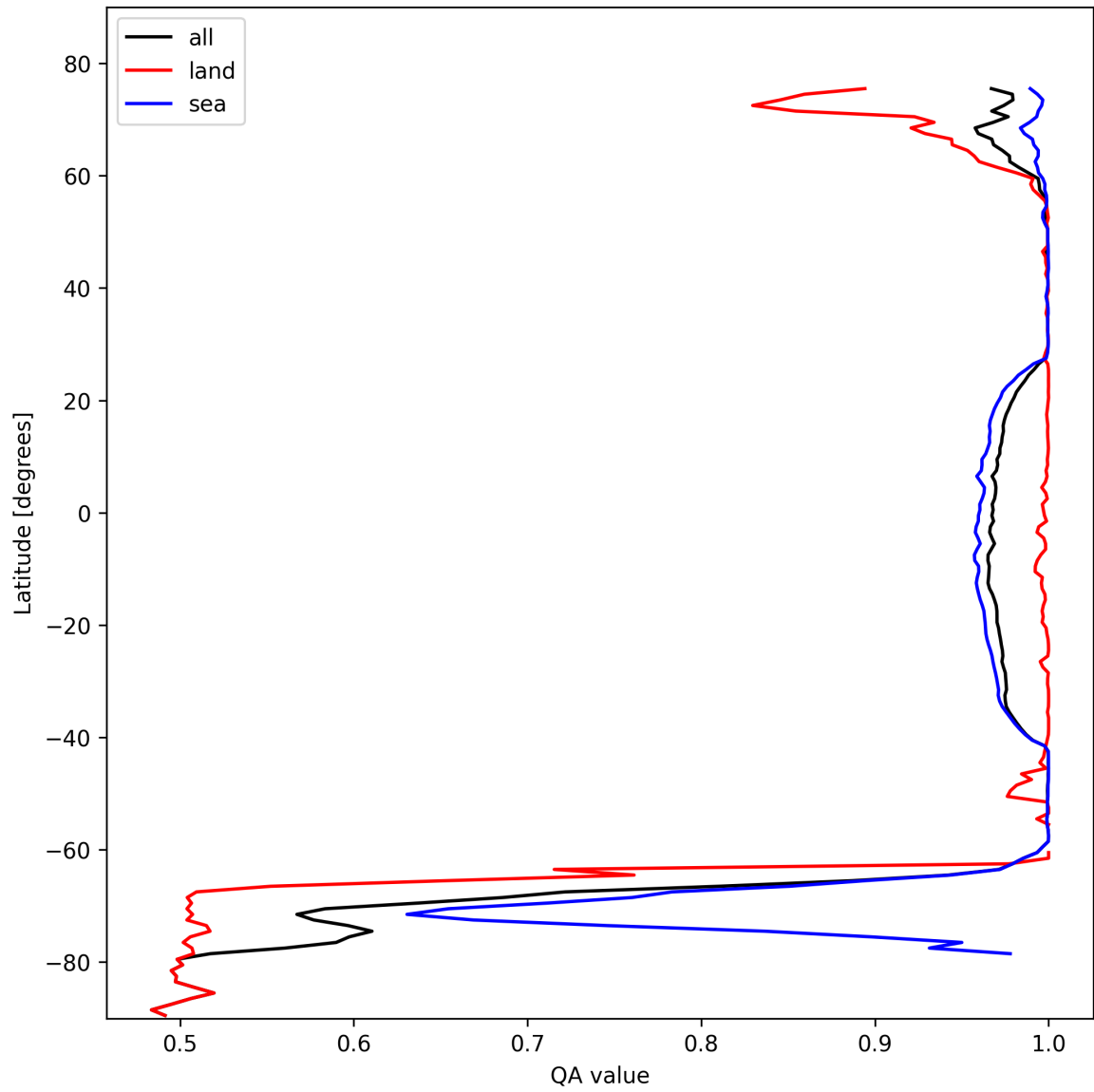
Figure 12: Zonal average of “QA value” for 2024-10-25 to 2024-10-27.
