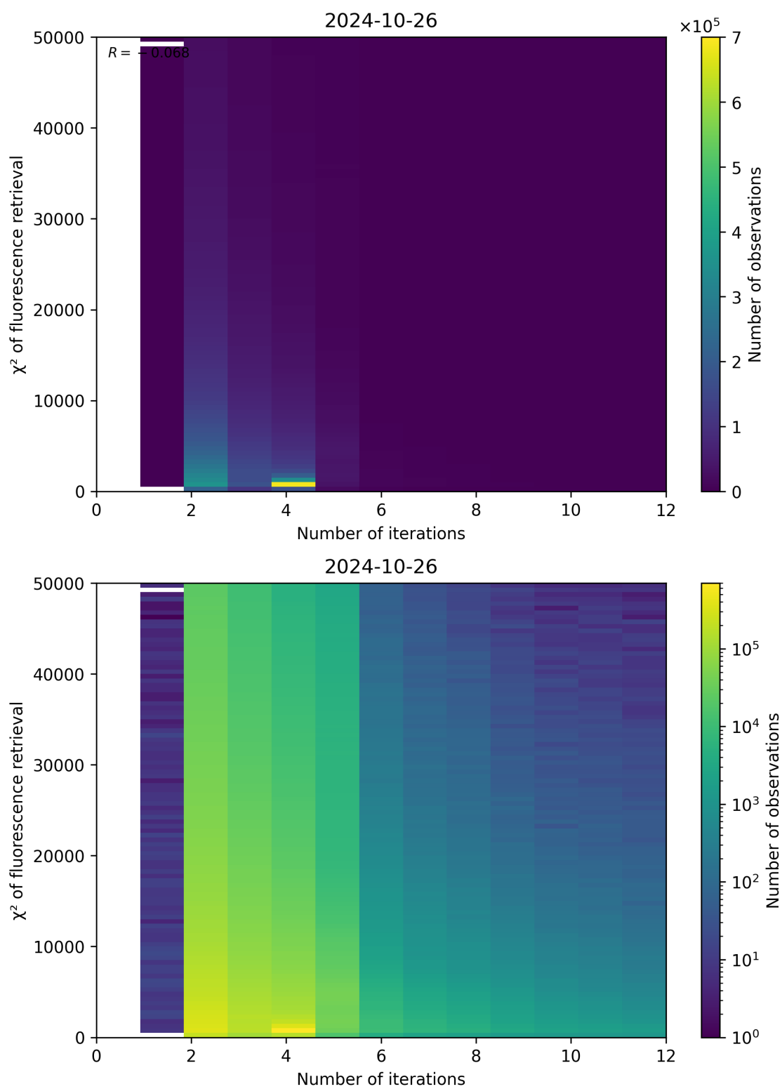
Figure 106: Scatter density plot of “Number of iterations” against “ \chi^2 of fluorescence retrieval” for 2024-10-25 to 2024-10-27.
