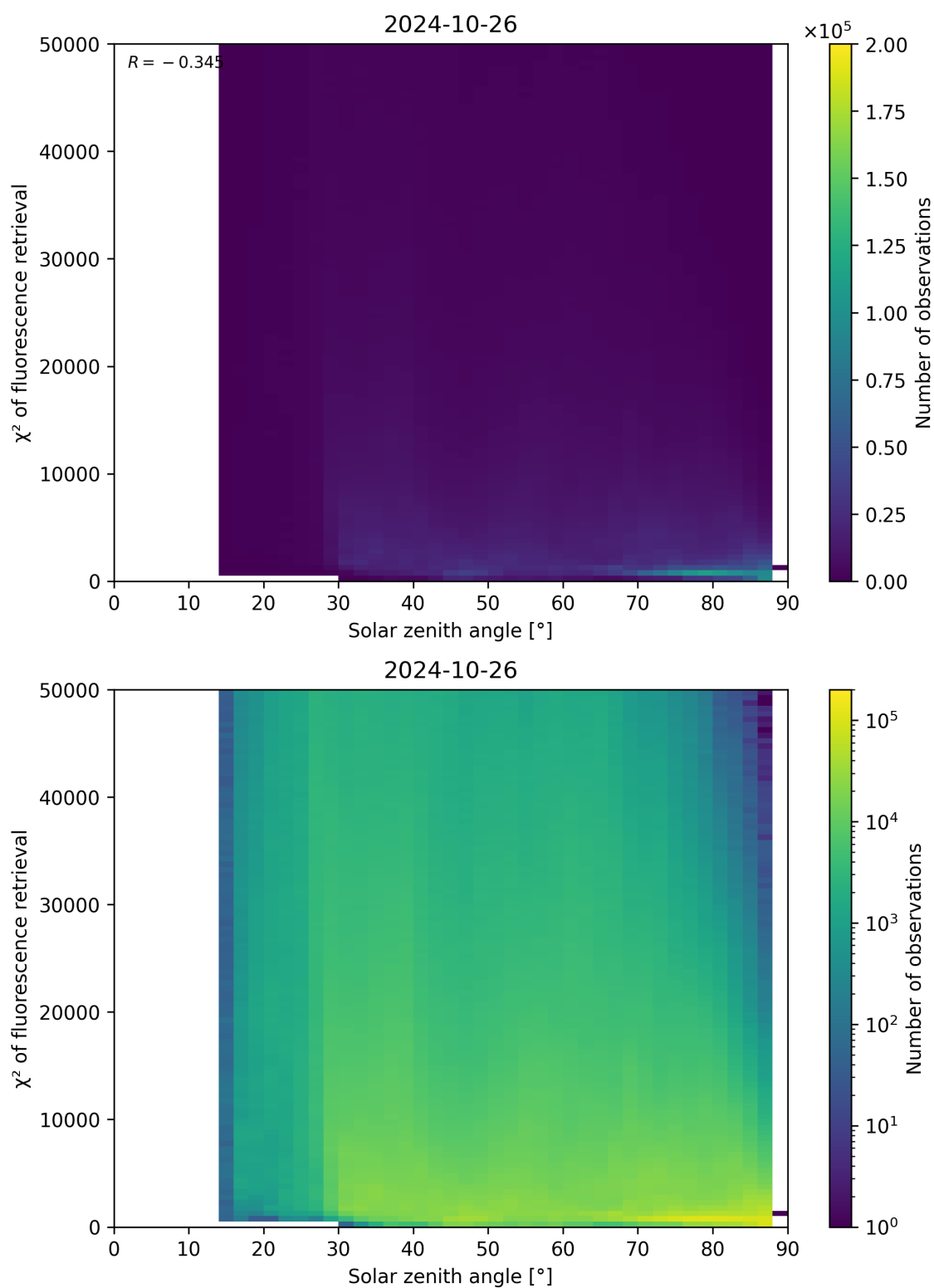
Figure 120: Scatter density plot of “Solar zenith angle” against “ \chi^2 of fluorescence retrieval” for 2024-10-25 to 2024-10-27.
