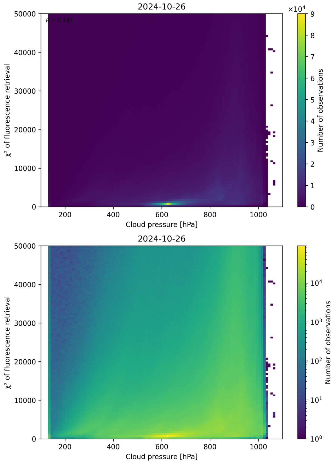
Figure 86: Scatter density plot of “Cloud pressure” against “ \chi^2 of fluorescence retrieval” for 2024-10-25 to 2024-10-27.
