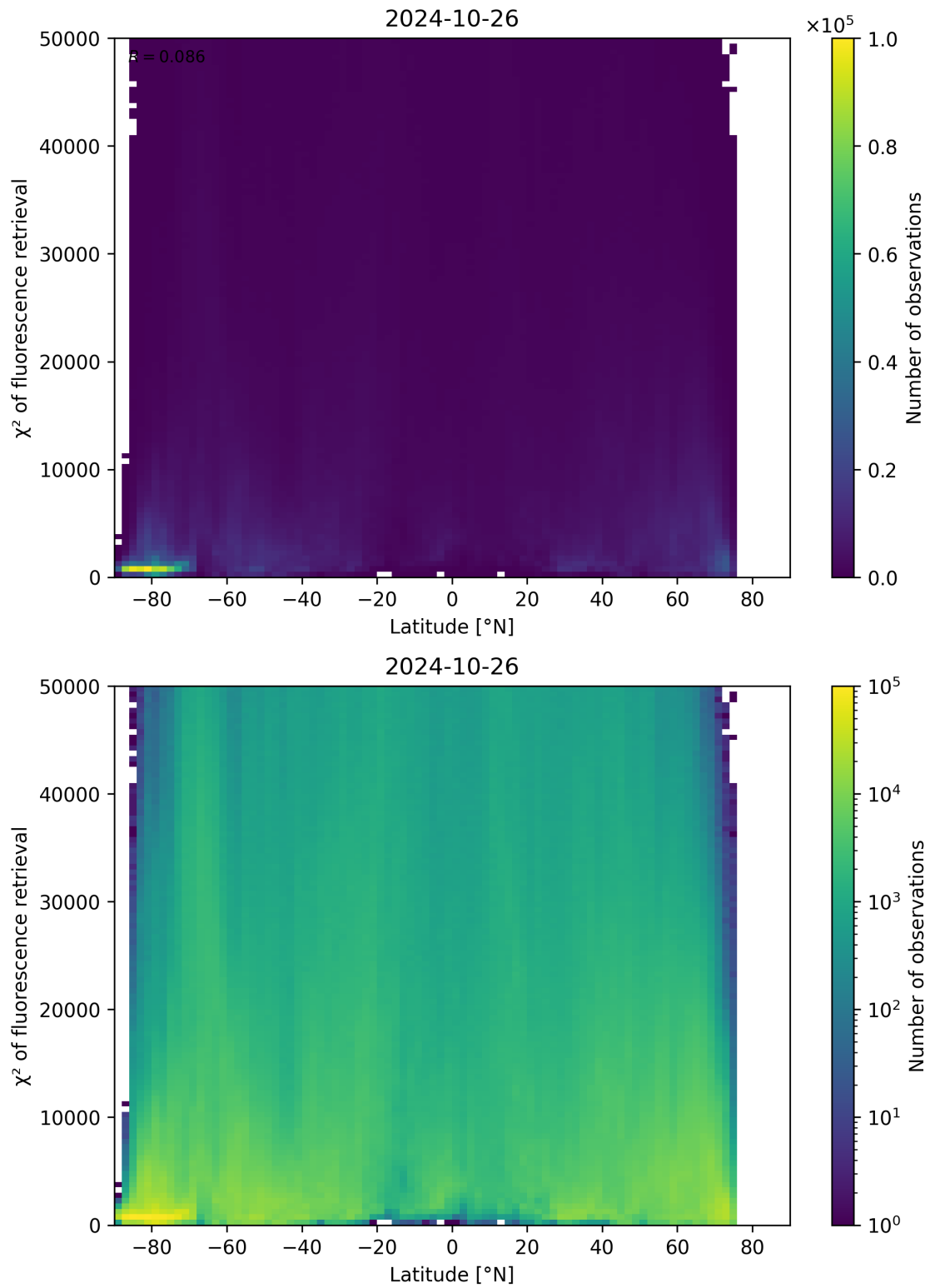
Figure 98: Scatter density plot of “Latitude” against “ \chi^2 of fluorescence retrieval” for 2024-10-25 to 2024-10-27.
