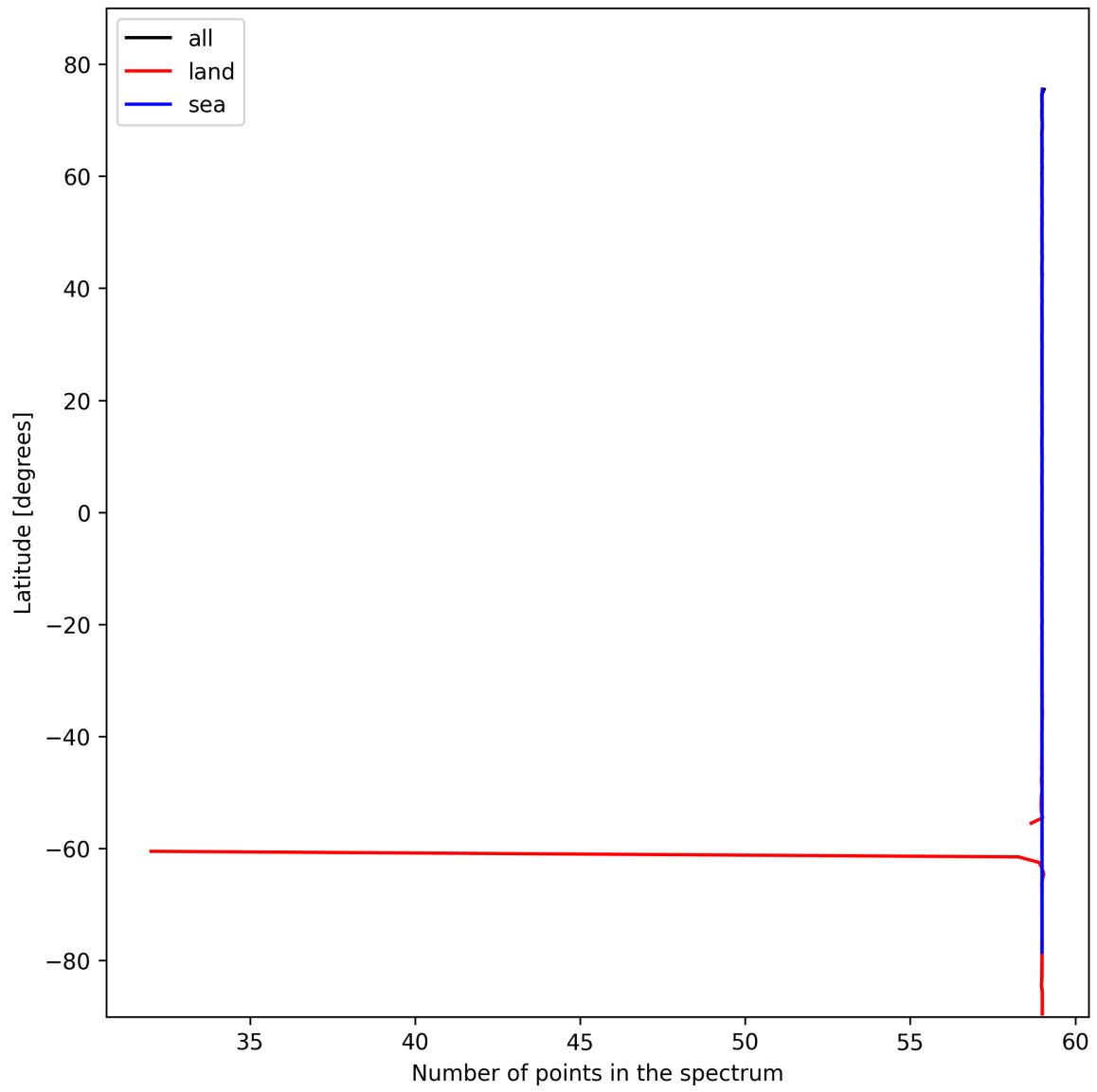
Figure 27: Zonal average of “Number of points in the spectrum” for 2024-10-25 to 2024-10-27.
