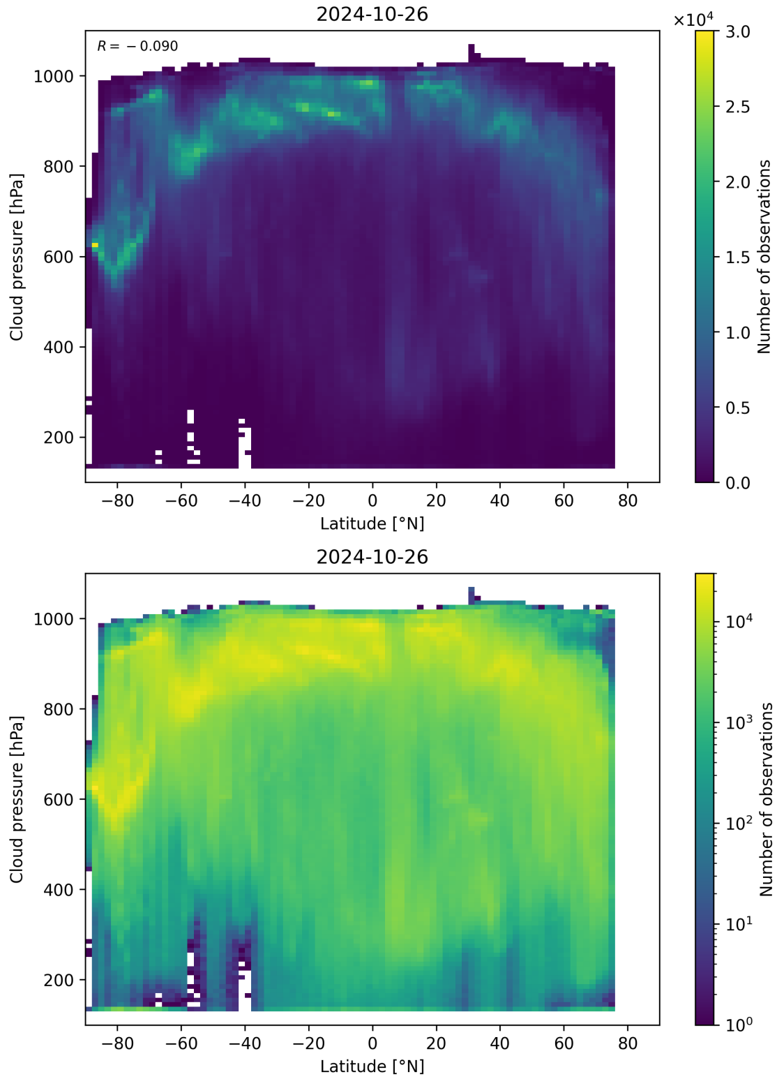
Figure 100: Scatter density plot of “Latitude” against “Cloud pressure” for 2024-10-25 to 2024-10-27.
