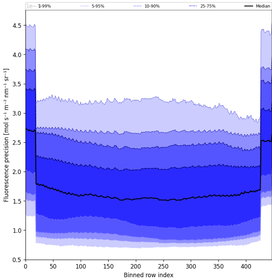
Figure 58: Along track statistics of “Fluorescence precision” for 2024-10-25 to 2024-10-27
