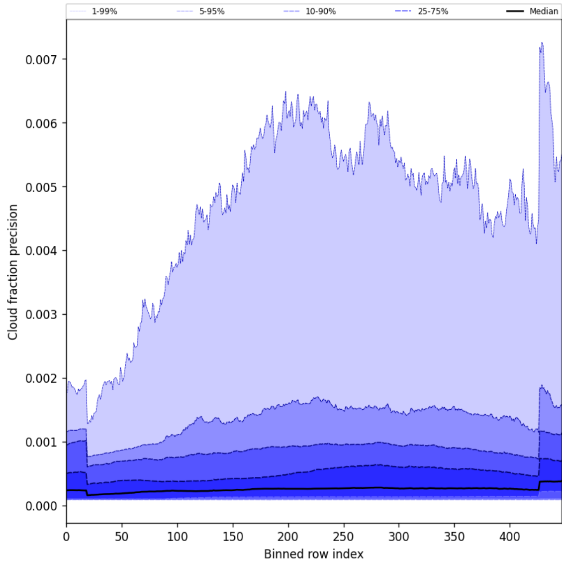
Figure 50: Along track statistics of “Cloud fraction precision” for 2024-10-25 to 2024-10-27
