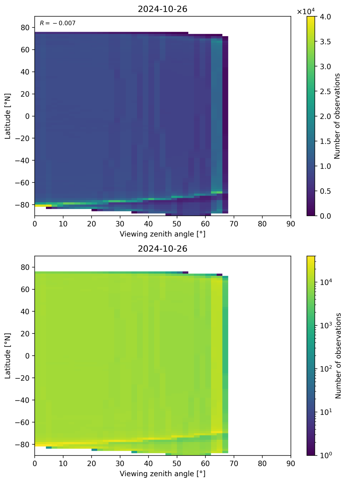
Figure 135: Scatter density plot of “Viewing zenith angle” against “Latitude” for 2024-10-25 to 2024-10-27.
