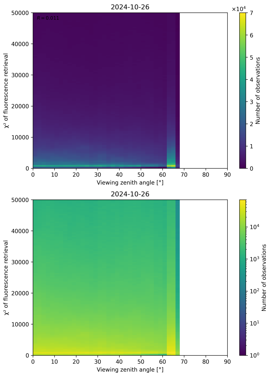
Figure 131: Scatter density plot of “Viewing zenith angle” against “ \chi^2 of fluorescence retrieval” for 2024-10-25 to 2024-10-27.
