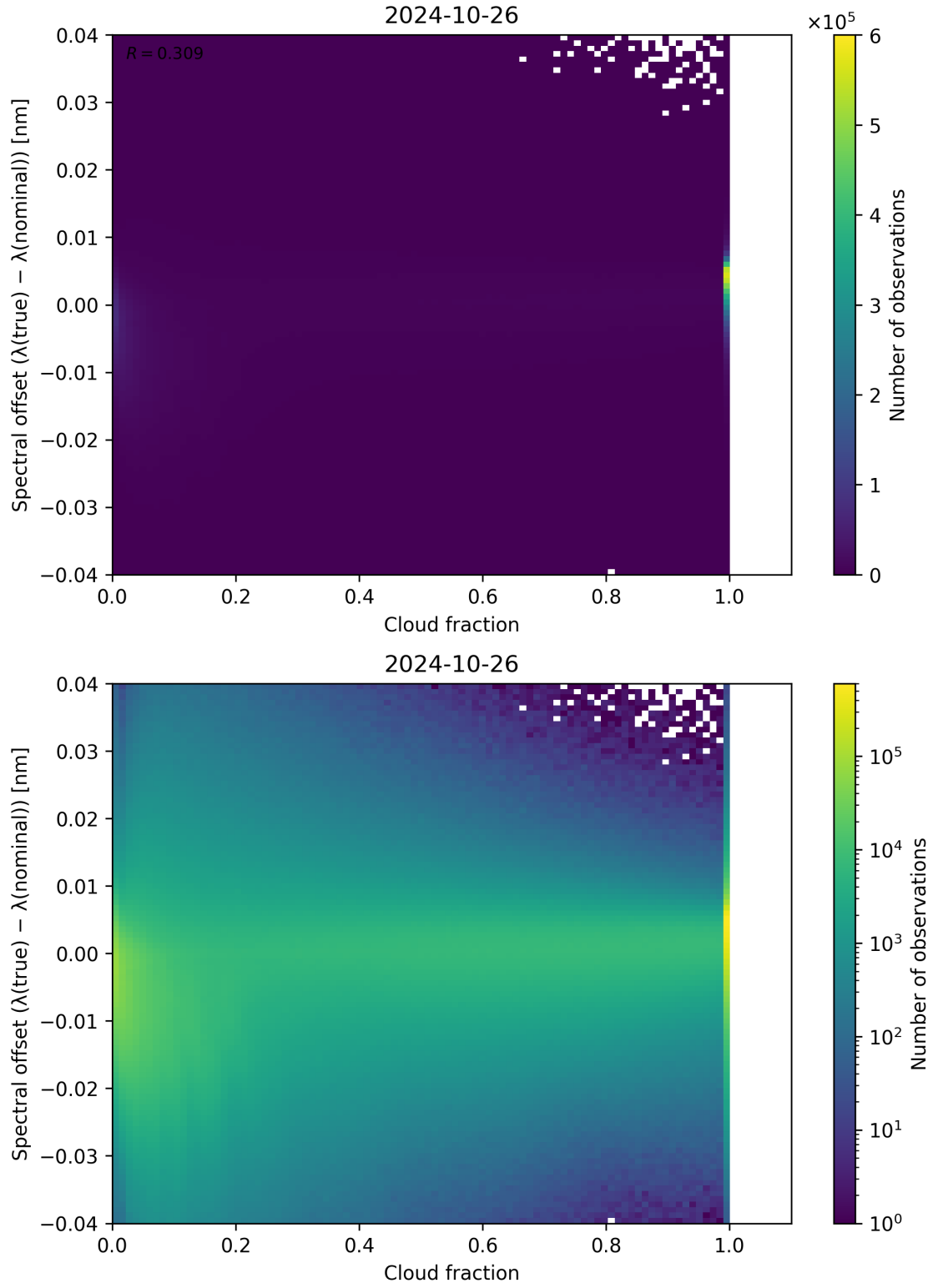
Figure 83: Scatter density plot of “Cloud fraction” against “Spectral offset ( \lambda_{\text{true}} - \lambda_{\text{nominal}} )” for 2024-10-25 to 2024-10-27.
