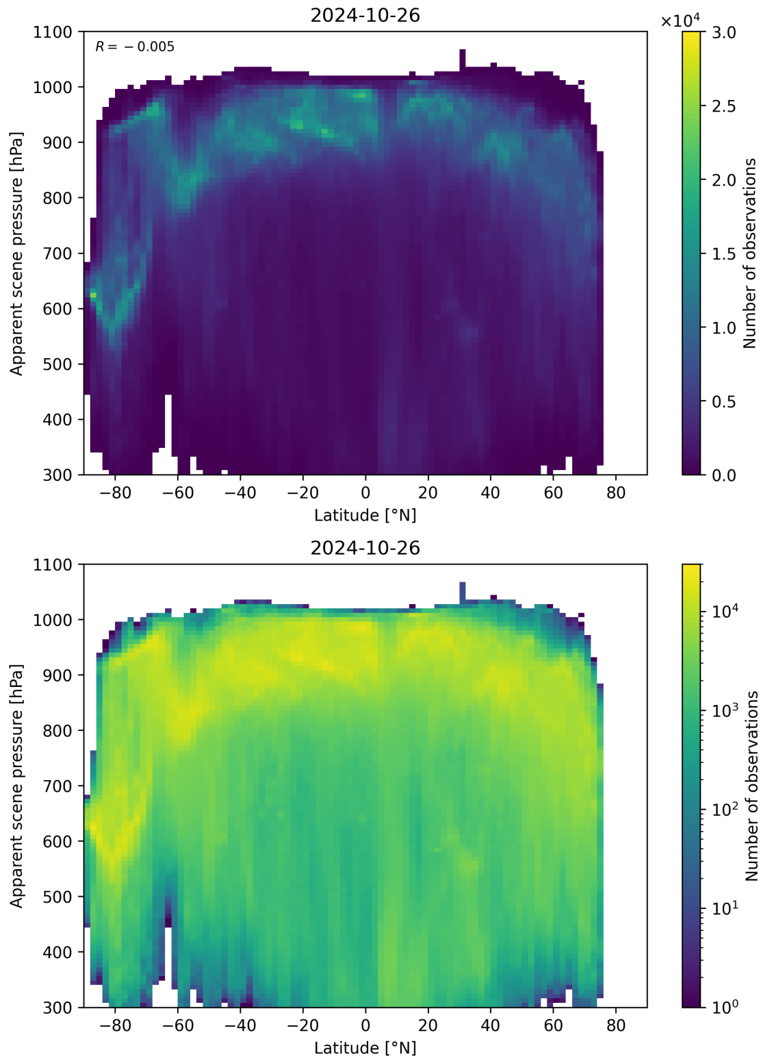
Figure 96: Scatter density plot of “Latitude” against “Apparent scene pressure” for 2024-10-25 to 2024-10-27.
