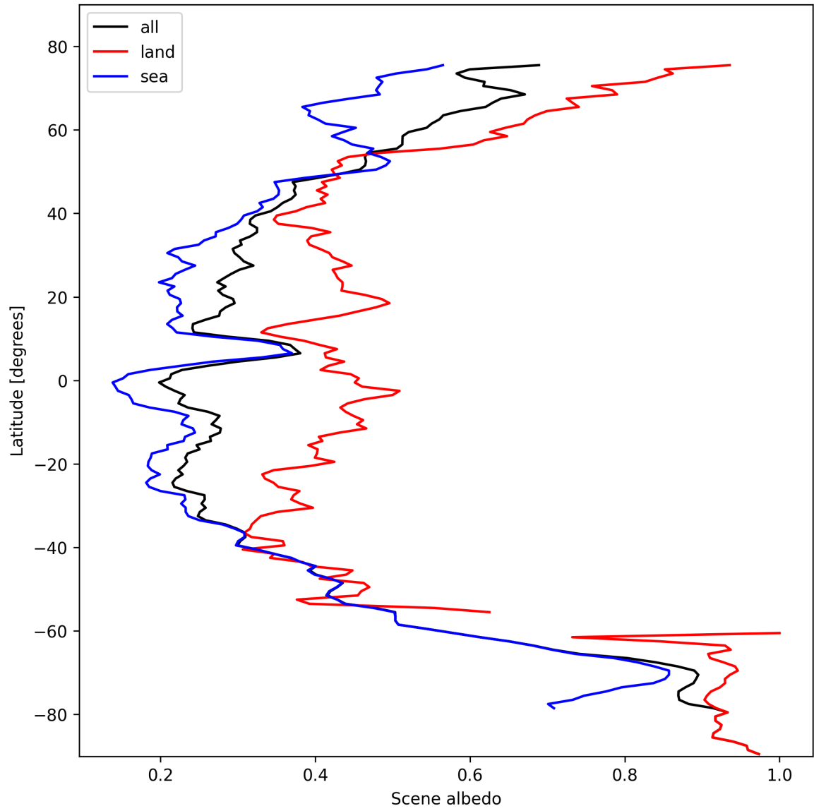
Figure 17: Zonal average of “Scene albedo” for 2024-10-25 to 2024-10-27.
