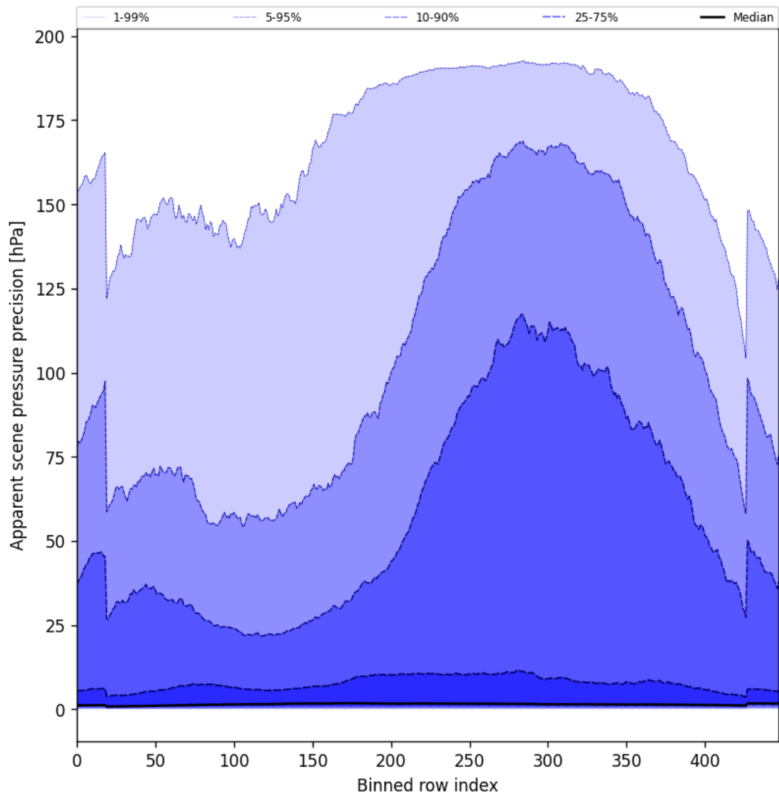
Figure 54: Along track statistics of “Apparent scene pressure precision” for 2024-10-25 to 2024-10-27
