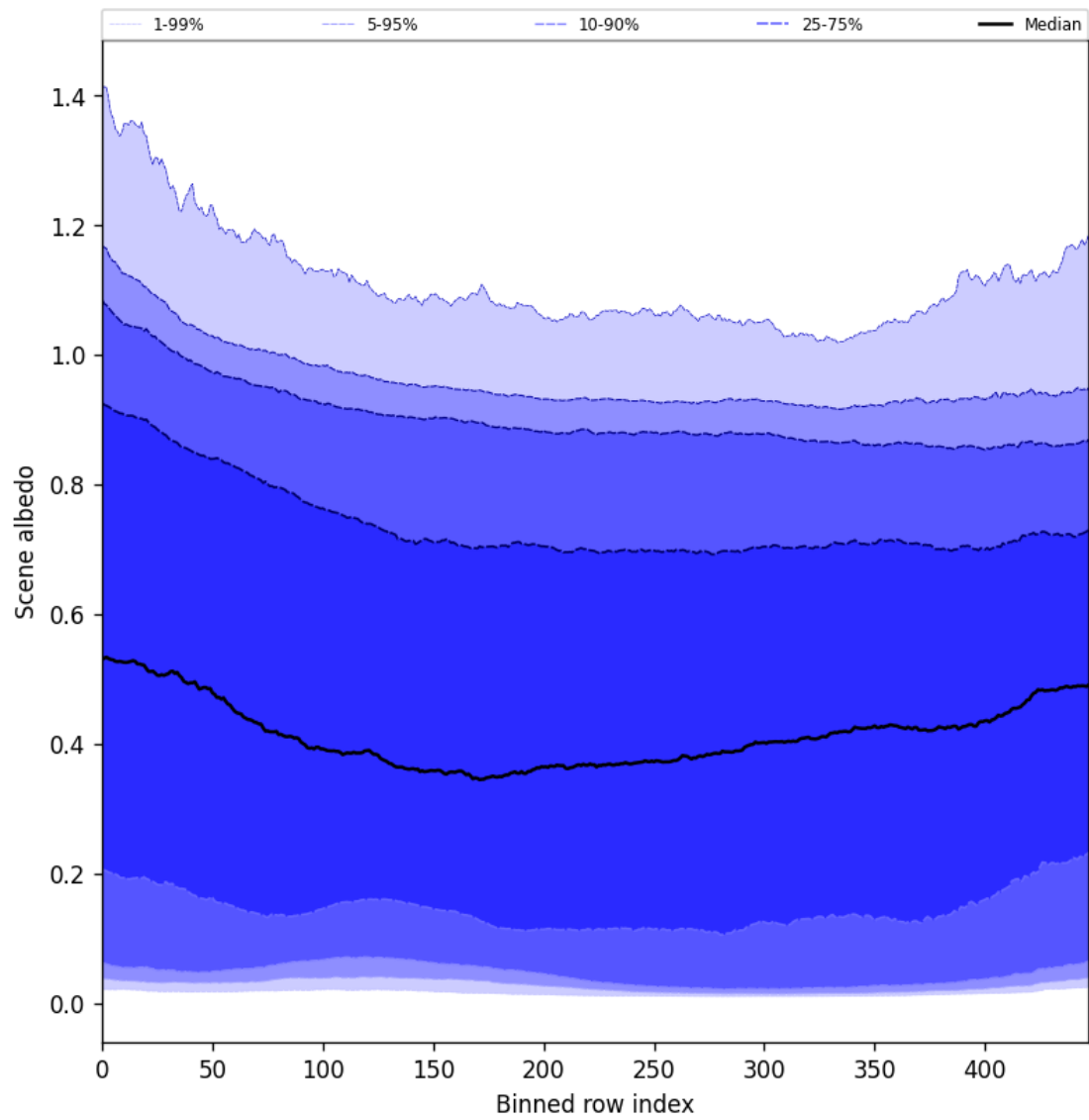
Figure 51: Along track statistics of “Scene albedo” for 2024-10-25 to 2024-10-27
