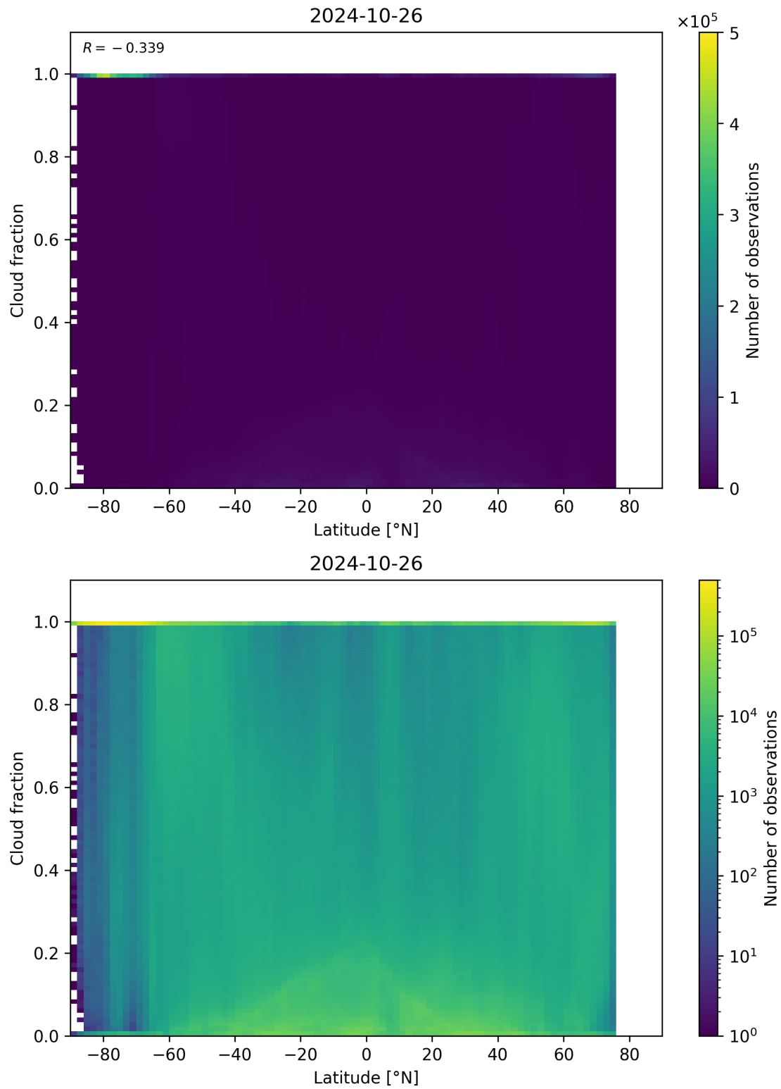
Figure 99: Scatter density plot of “Latitude” against “Cloud fraction” for 2024-10-25 to 2024-10-27.
