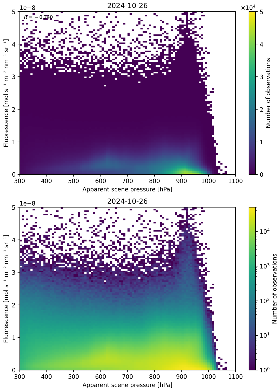
Figure 65: Scatter density plot of “Apparent scene pressure” against “Fluorescence” for 2024-10-25 to 2024-10-27.
