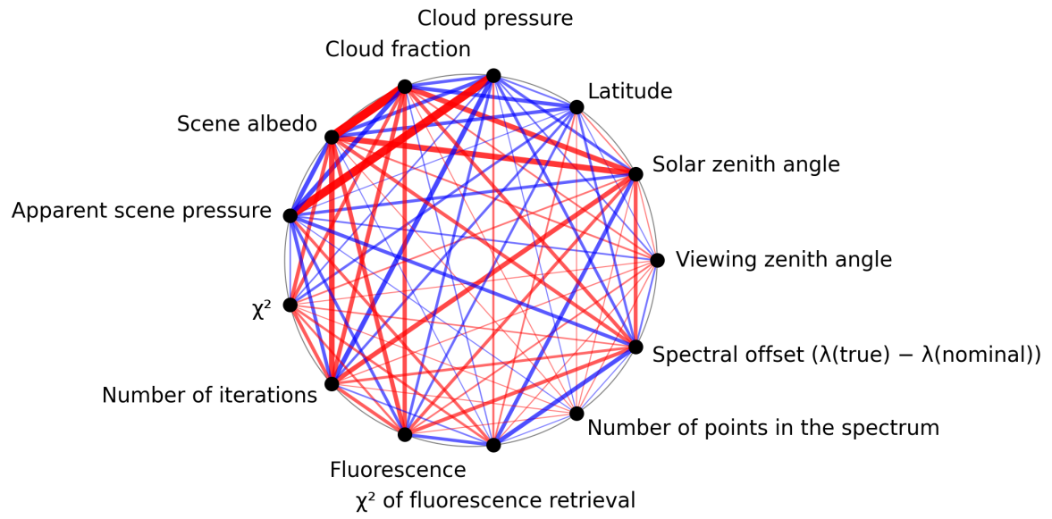
Figure 1: Map of correlation graph for 2024-10-25 to 2024-10-27.
