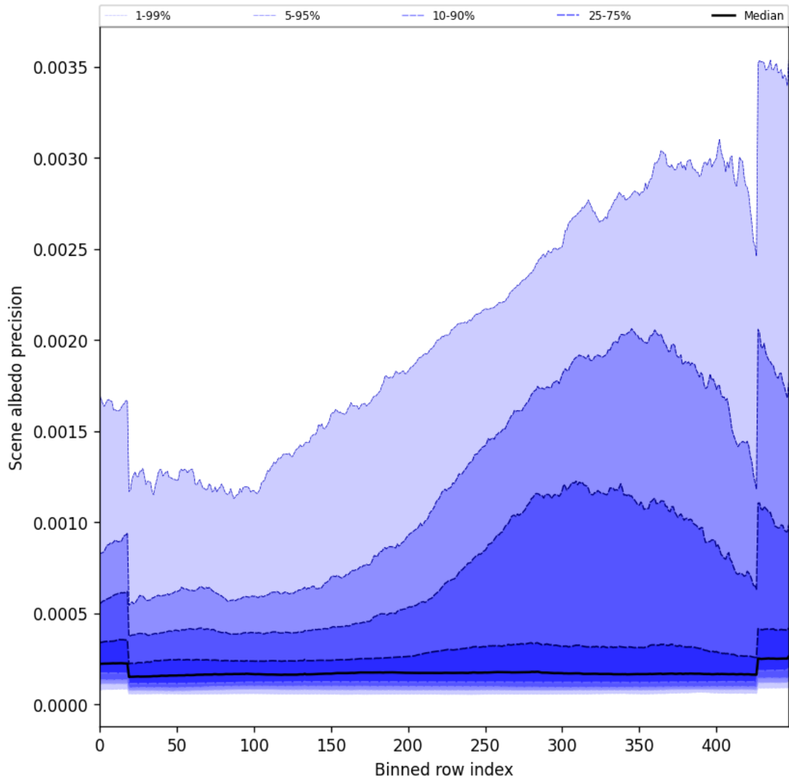
Figure 52: Along track statistics of “Scene albedo precision” for 2024-10-25 to 2024-10-27
