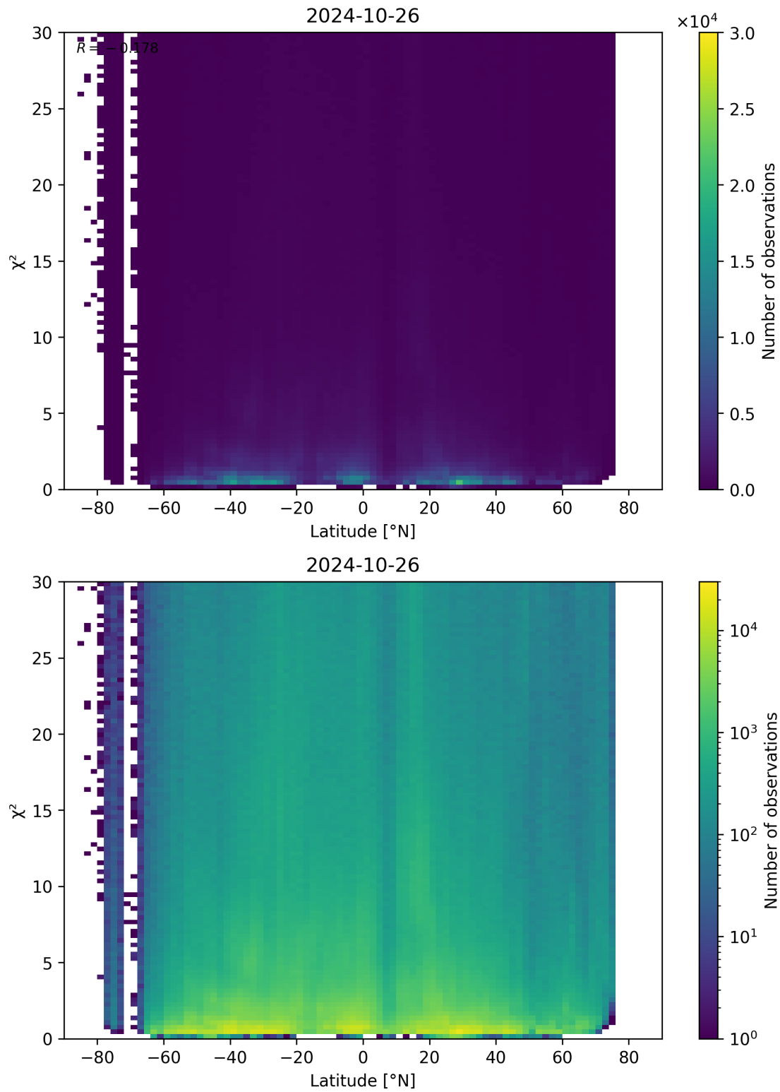
Figure 97: Scatter density plot of “Latitude” against “ \chi^2 ” for 2024-10-25 to 2024-10-27.
