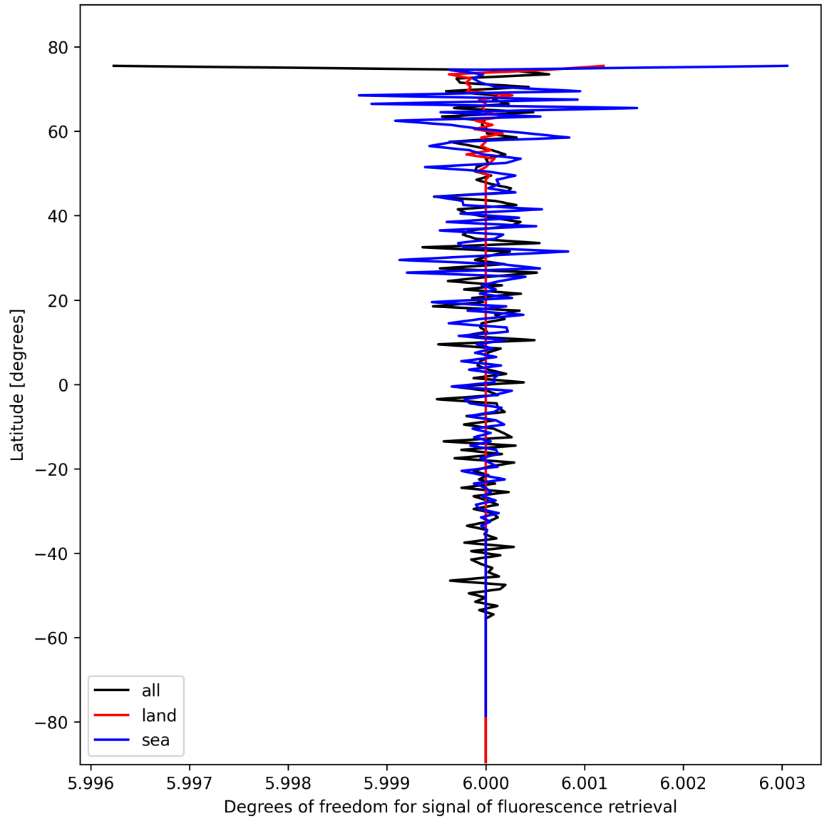
Figure 26: Zonal average of “Degrees of freedom for signal of fluorescence retrieval” for 2024-10-25 to 2024-10-27.
