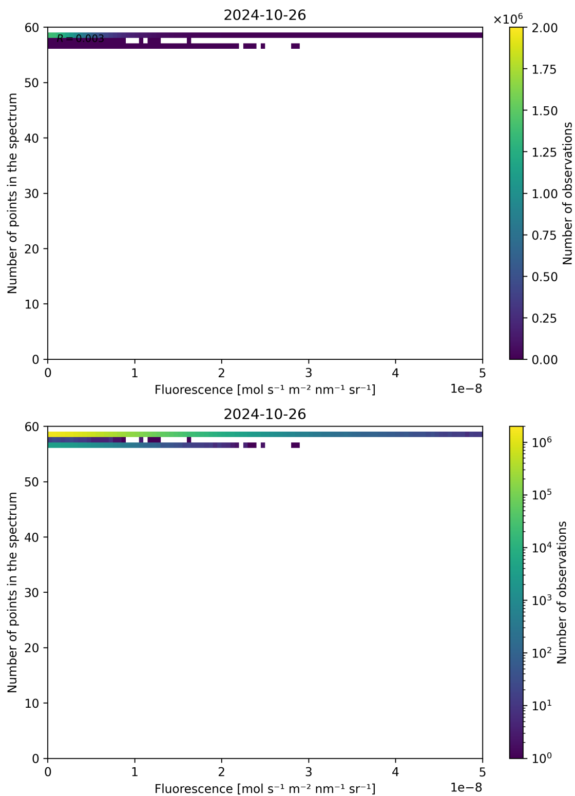
Figure 94: Scatter density plot of “Fluorescence” against “Number of points in the spectrum” for 2024-10-25 to 2024-10-27.
