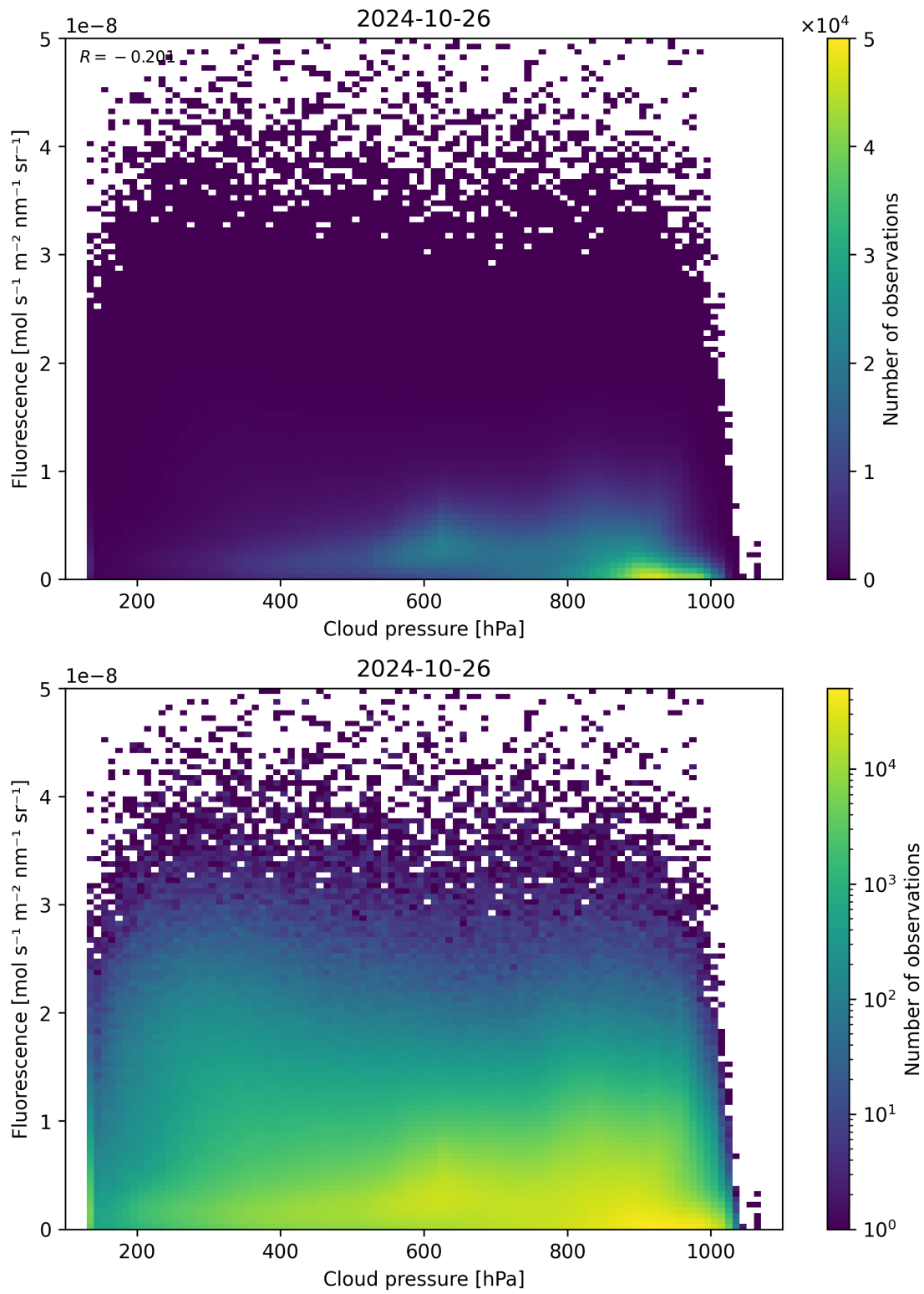
Figure 88: Scatter density plot of “Cloud pressure” against “Fluorescence” for 2024-10-25 to 2024-10-27.
