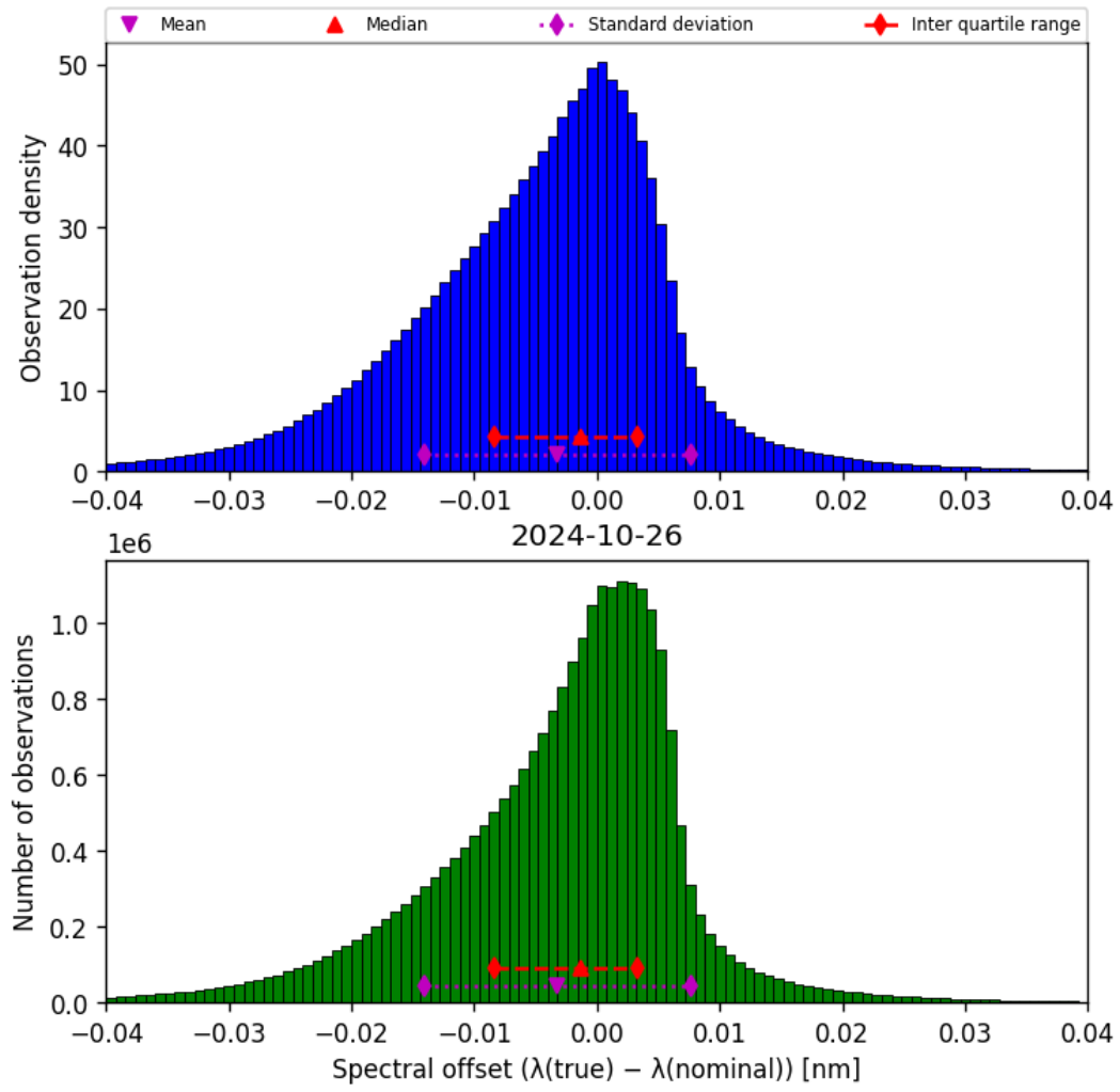
Figure 45: Histogram of “Spectral offset ( \lambda_{\text{true}} - \lambda_{\text{nominal}} )” for 2024-10-25 to 2024-10-27
