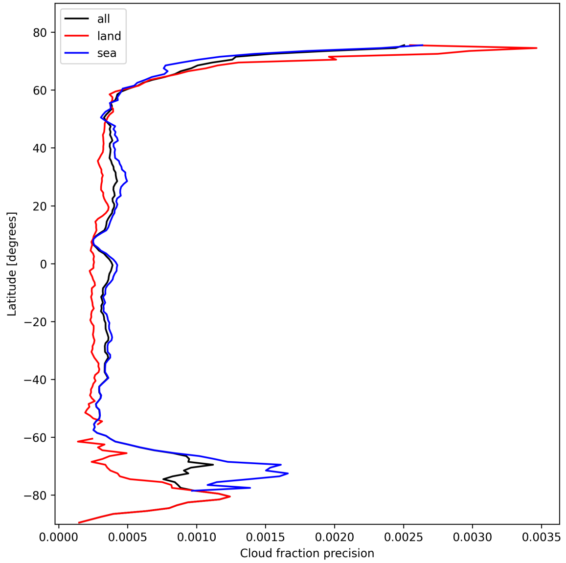
Figure 16: Zonal average of “Cloud fraction precision” for 2024-10-25 to 2024-10-27.
