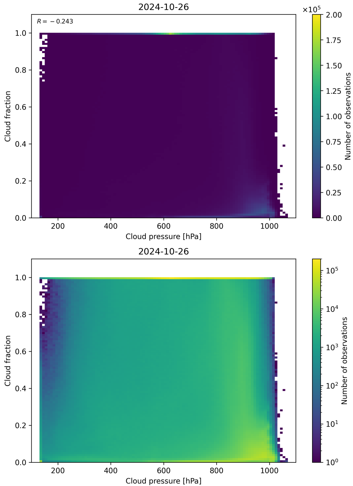
Figure 87: Scatter density plot of “Cloud pressure” against “Cloud fraction” for 2024-10-25 to 2024-10-27.
