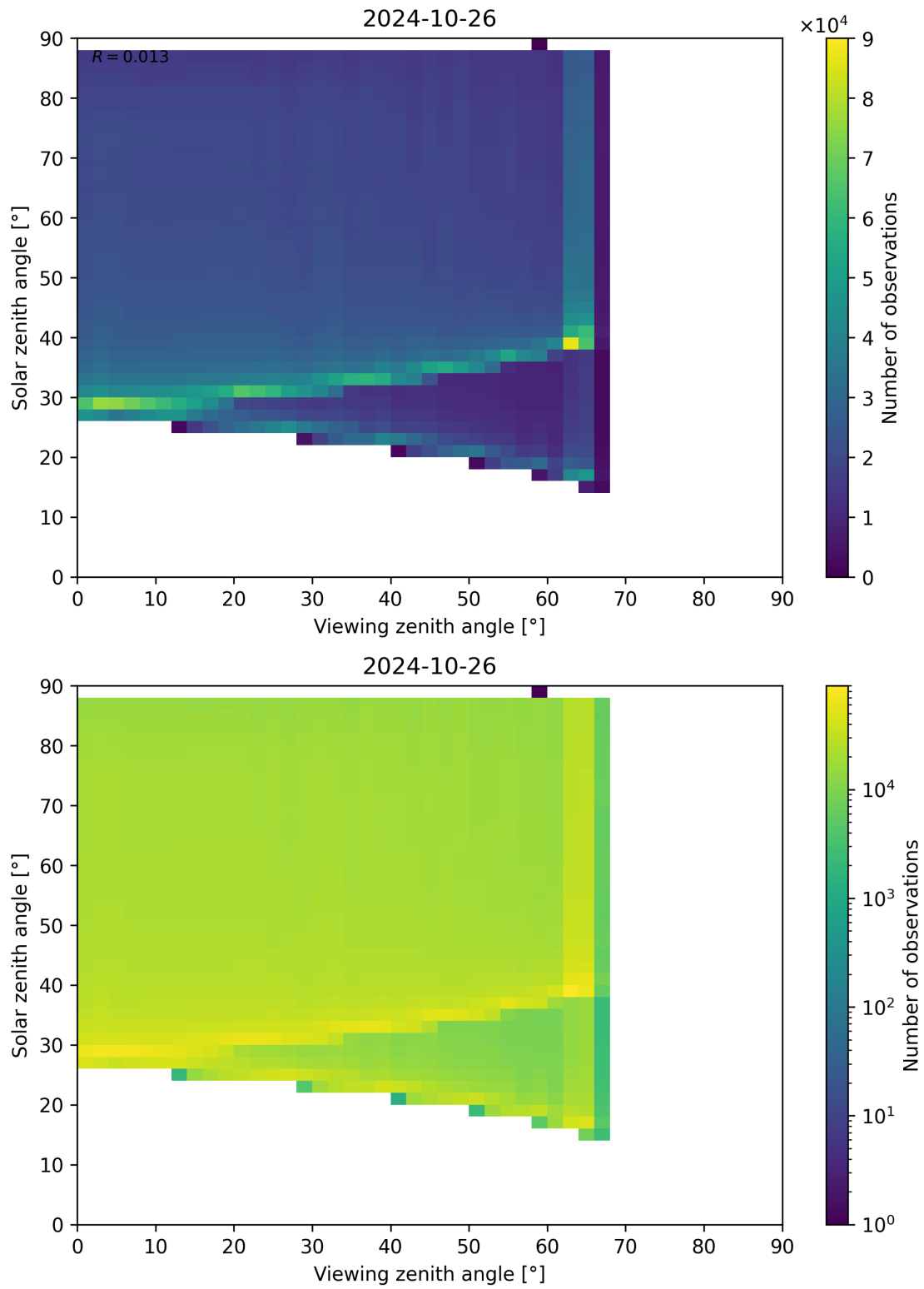
Figure 139: Scatter density plot of “Viewing zenith angle” against “Solar zenith angle” for 2024-10-25 to 2024-10-27.
