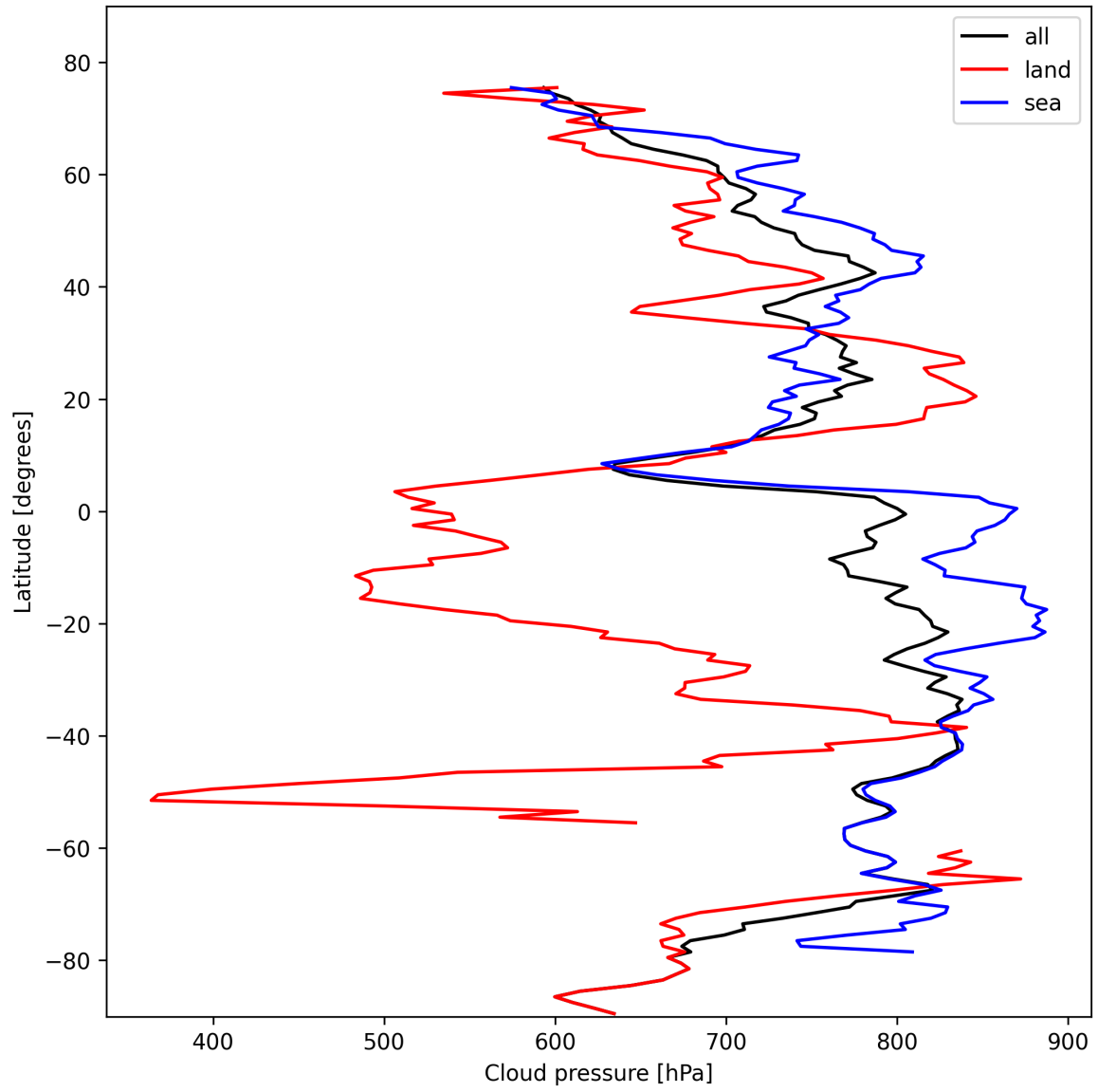
Figure 13: Zonal average of “Cloud pressure” for 2024-10-25 to 2024-10-27.
