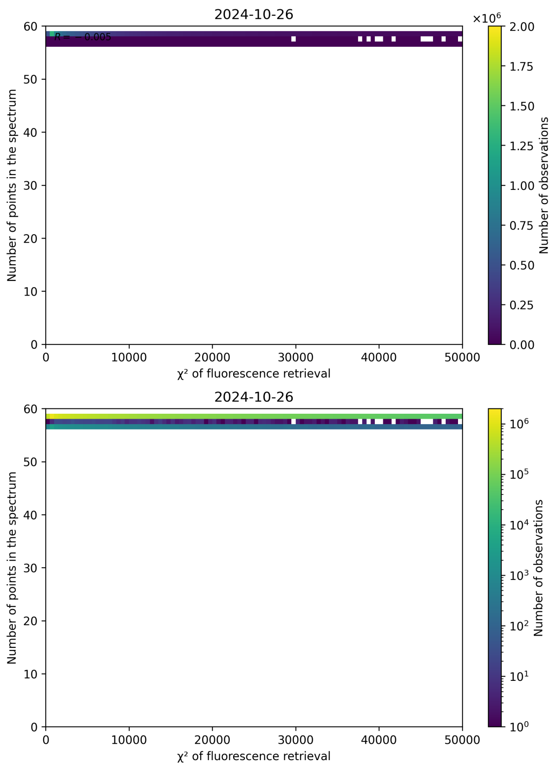
Figure 71: Scatter density plot of “ \chi^2 of fluorescence retrieval” against “Number of points in the spectrum” for 2024-10-25 to 2024-10-27.
