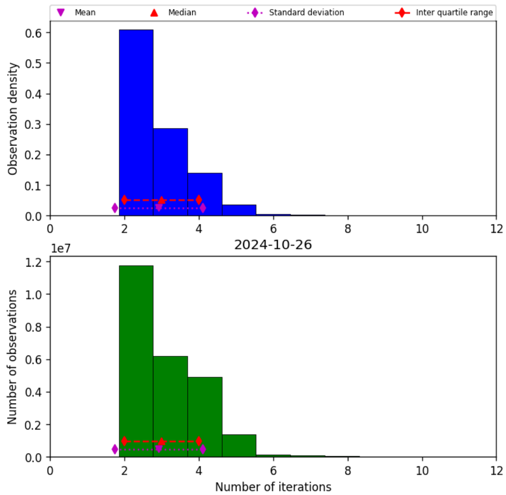
Figure 39: Histogram of “Number of iterations” for 2024-10-25 to 2024-10-27
