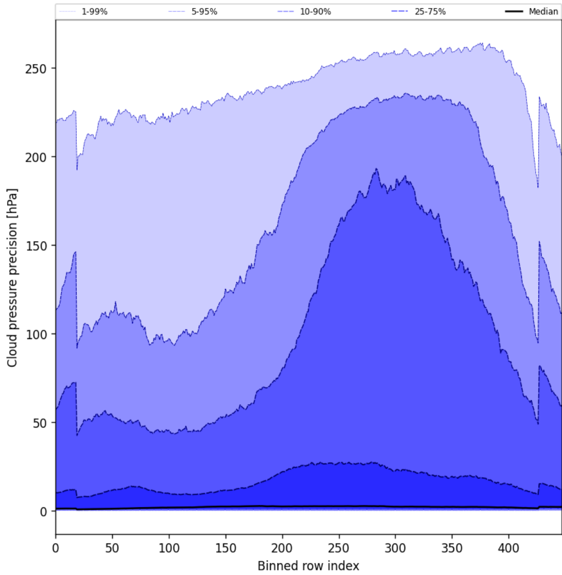
Figure 48: Along track statistics of “Cloud pressure precision” for 2024-10-25 to 2024-10-27
