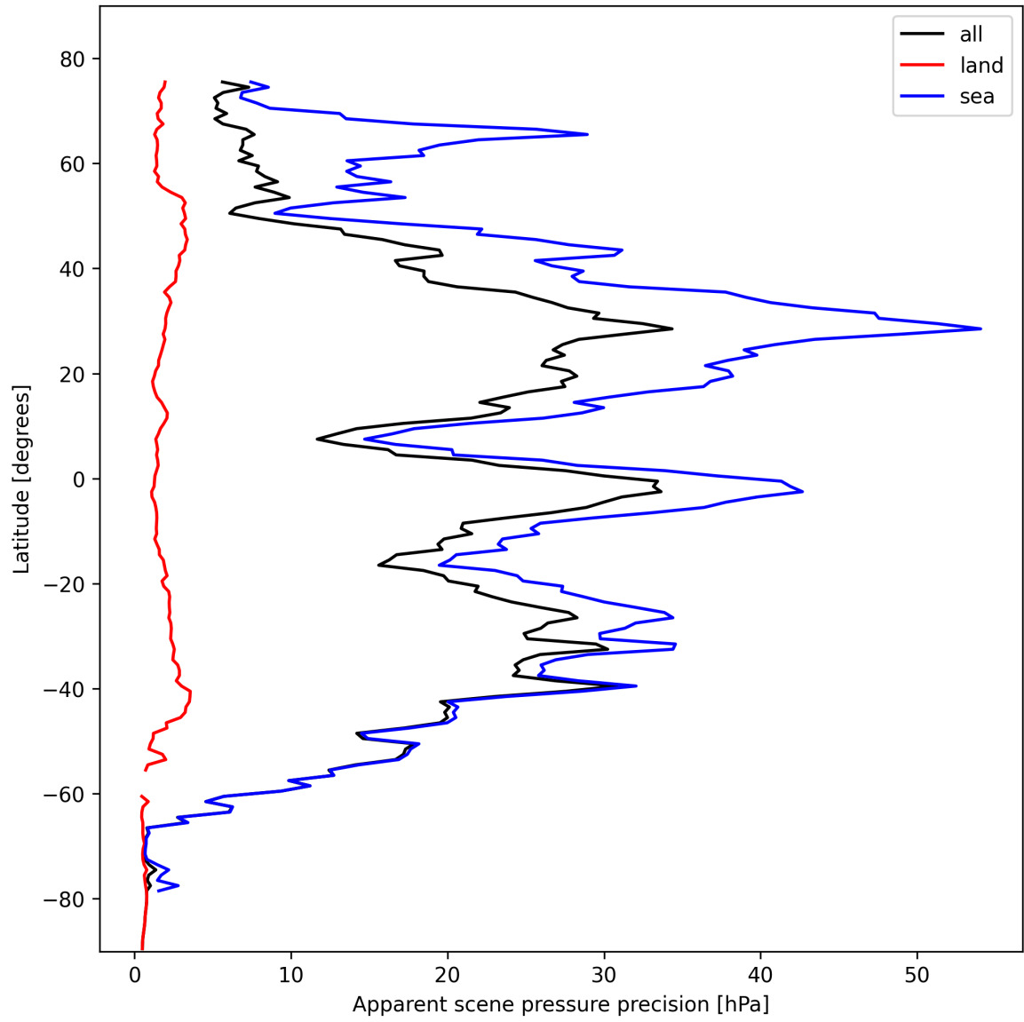
Figure 20: Zonal average of “Apparent scene pressure precision” for 2024-10-25 to 2024-10-27.
