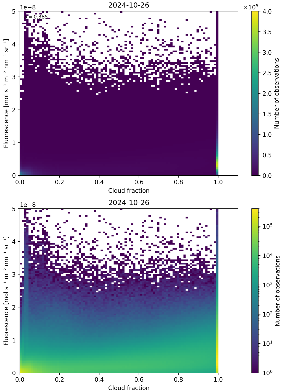
Figure 79: Scatter density plot of “Cloud fraction” against “Fluorescence” for 2024-10-25 to 2024-10-27.
