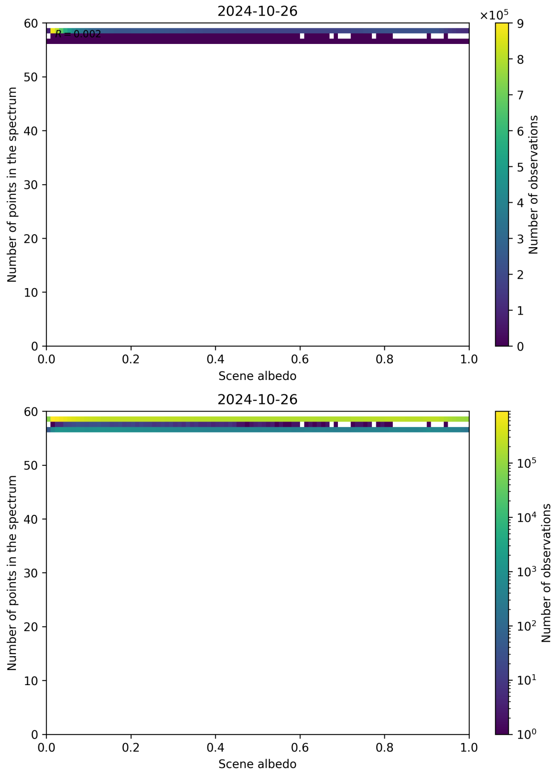
Figure 116: Scatter density plot of “Scene albedo” against “Number of points in the spectrum” for 2024-10-25 to 2024-10-27.
