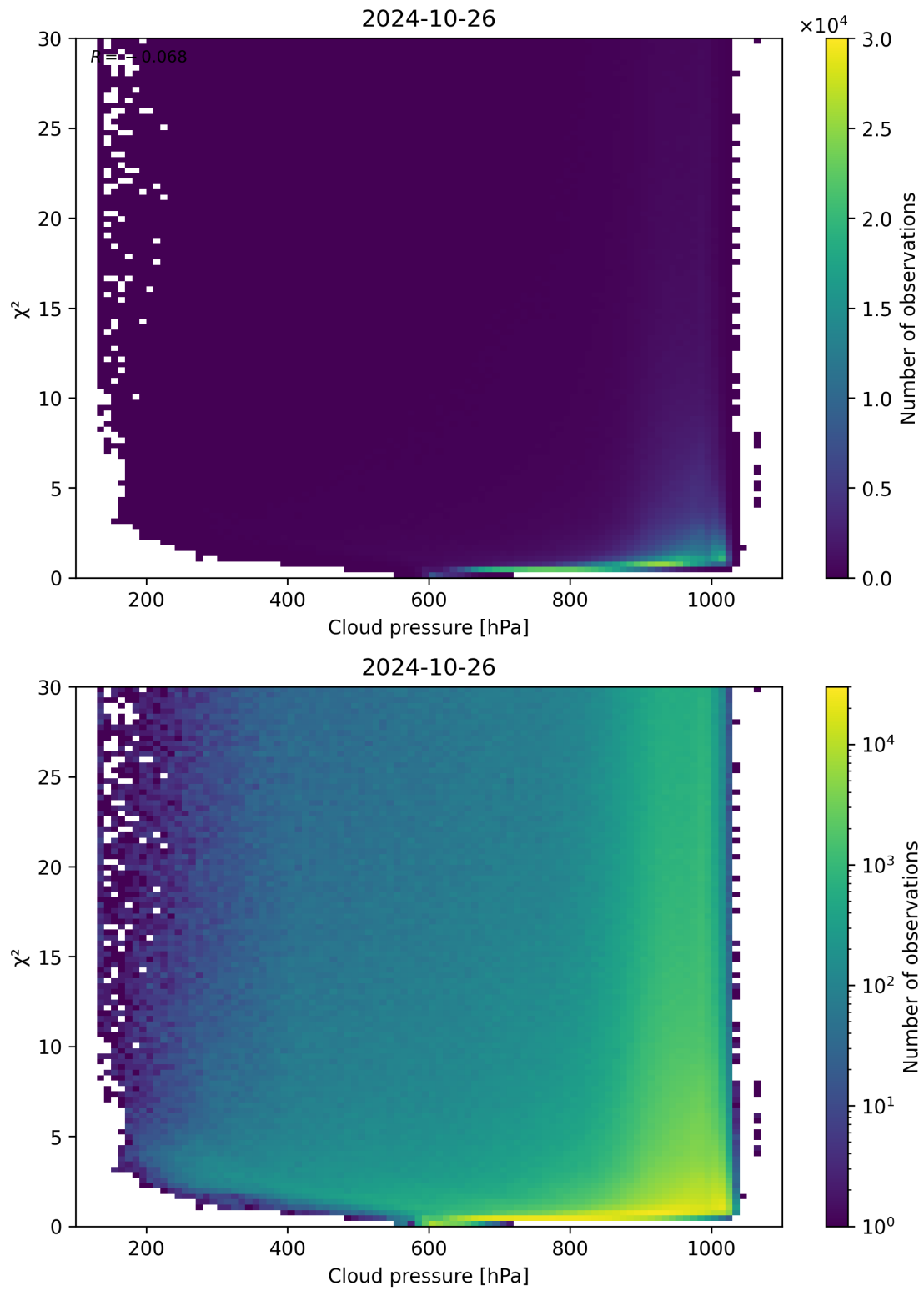
Figure 85: Scatter density plot of “Cloud pressure” against “ \chi^2 ” for 2024-10-25 to 2024-10-27.
