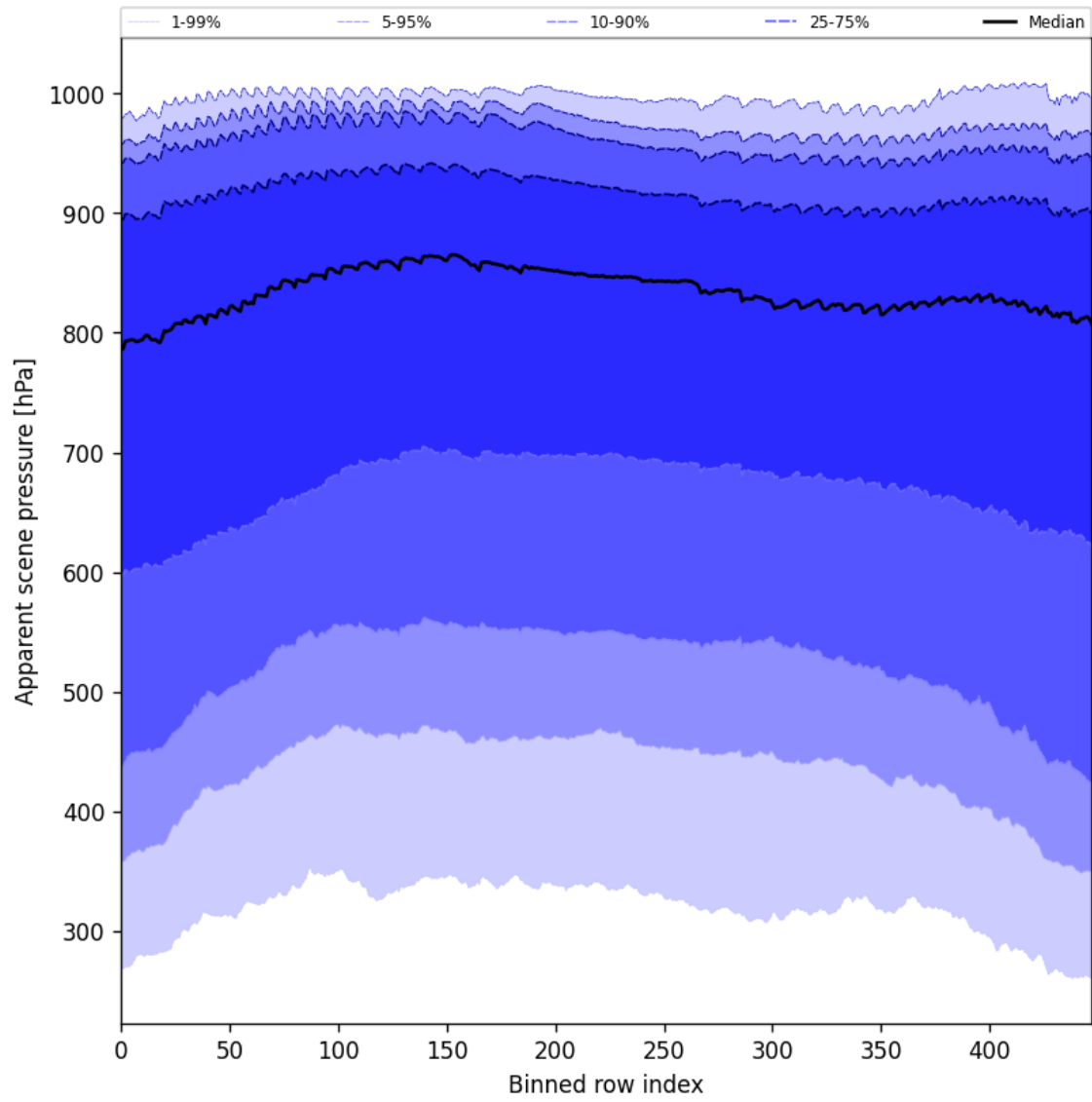
Figure 53: Along track statistics of “Apparent scene pressure” for 2024-10-25 to 2024-10-27
