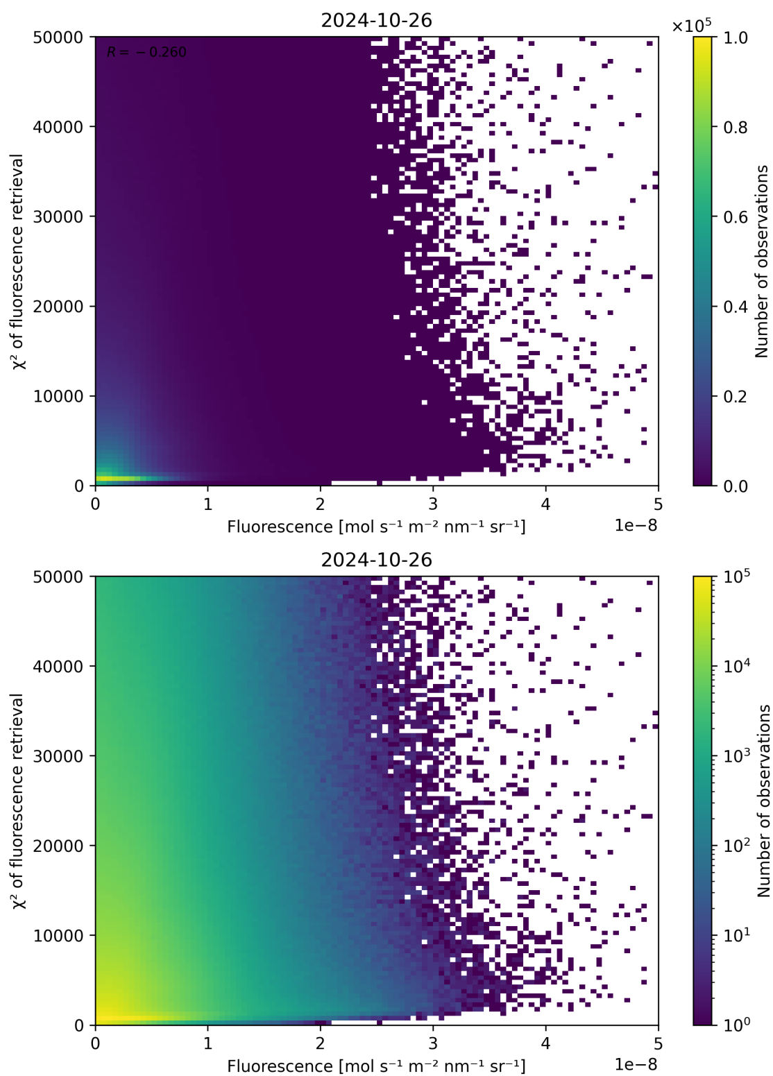
Figure 93: Scatter density plot of “Fluorescence” against “ \chi^2 of fluorescence retrieval” for 2024-10-25 to 2024-10-27.
