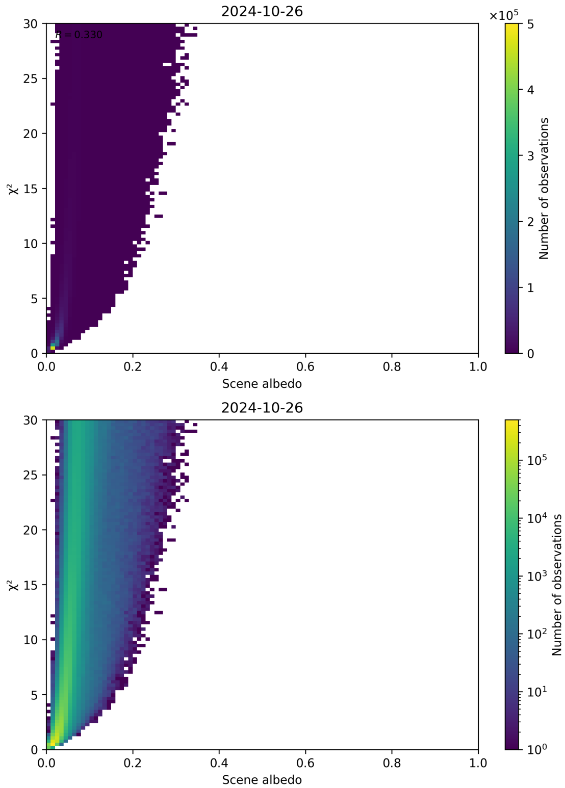
Figure 112: Scatter density plot of “Scene albedo” against “ \chi^2 ” for 2024-10-25 to 2024-10-27.
