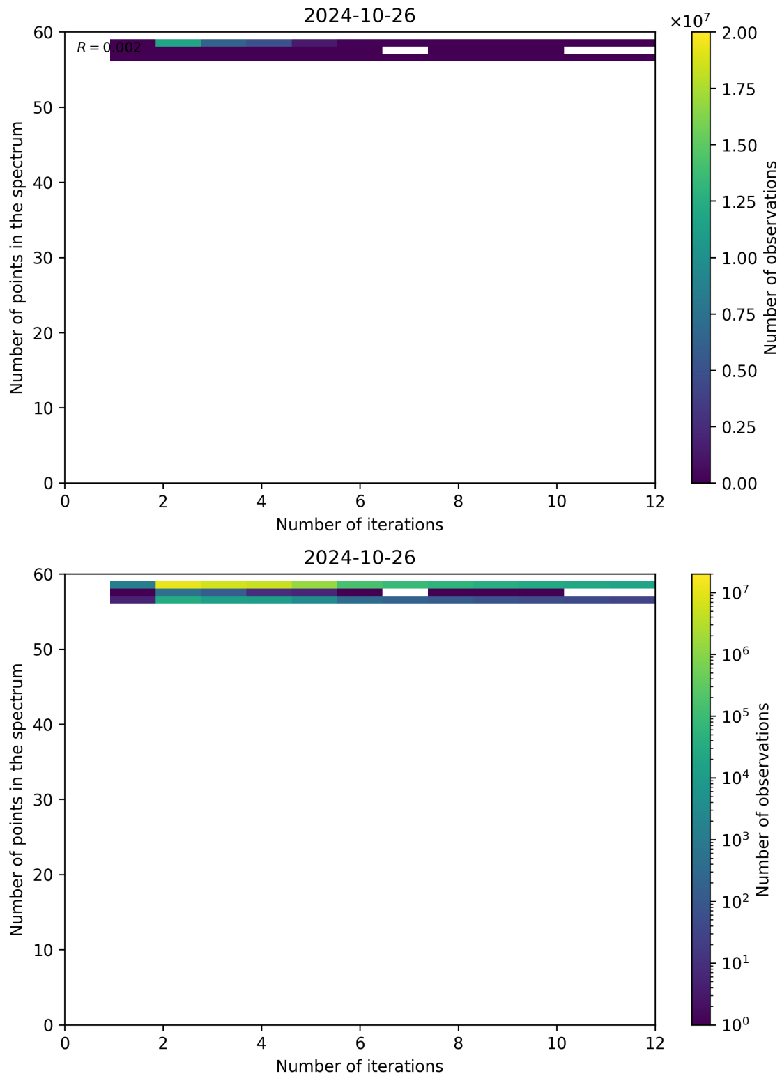
Figure 108: Scatter density plot of “Number of iterations” against “Number of points in the spectrum” for 2024-10-25 to 2024-10-27.
