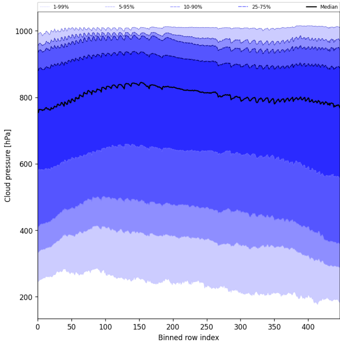
Figure 47: Along track statistics of “Cloud pressure” for 2024-10-25 to 2024-10-27
