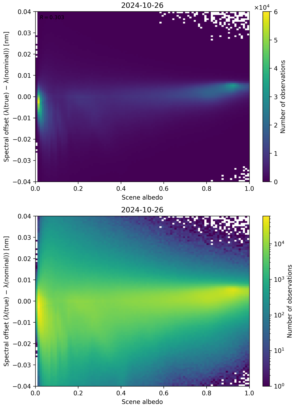
Figure 117: Scatter density plot of “Scene albedo” against “Spectral offset ( \lambda_{\text{true}} - \lambda_{\text{nominal}} )” for 2024-10-25 to 2024-10-27.
