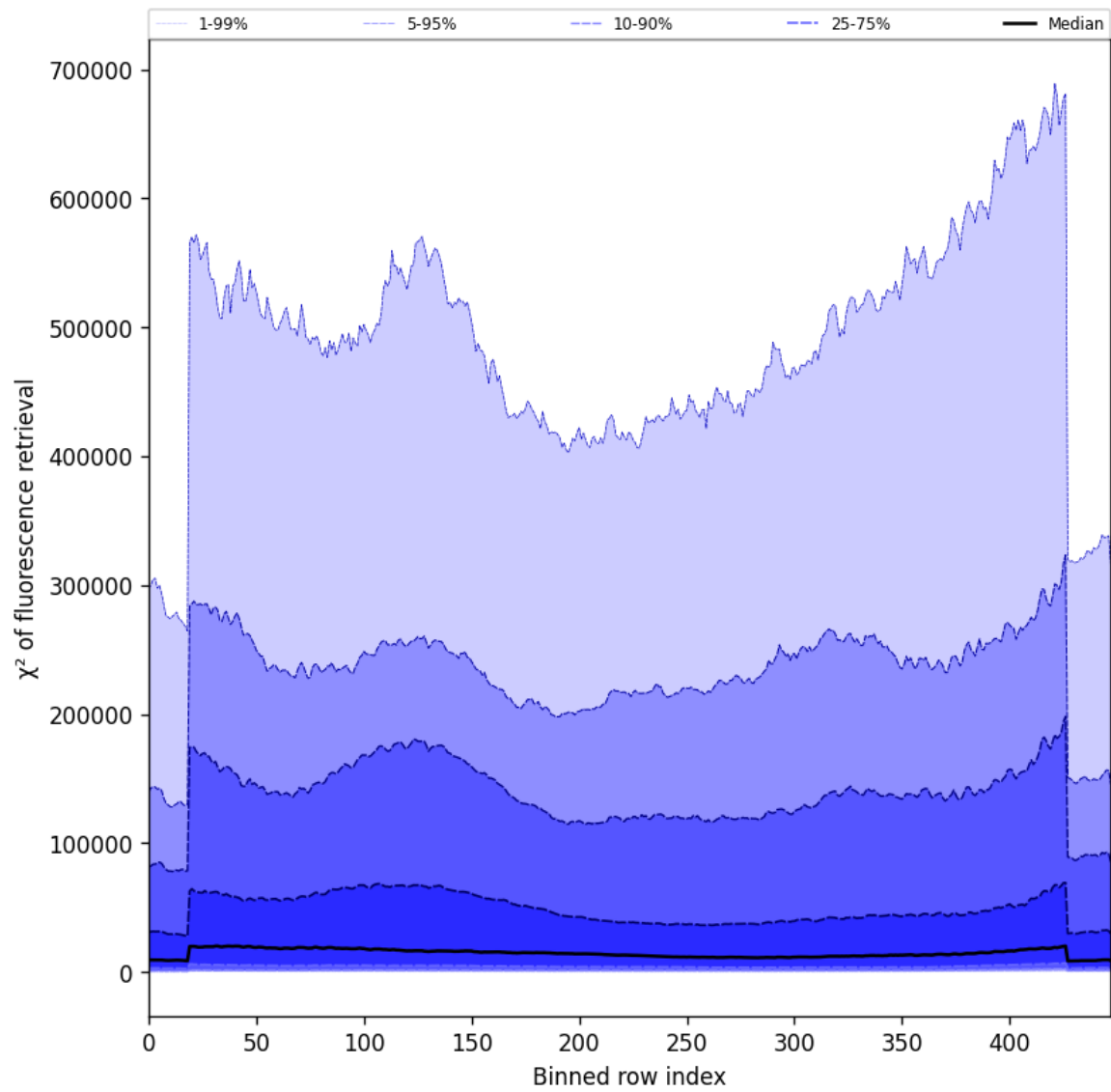
Figure 59: Along track statistics of “ \chi^2 of fluorescence retrieval” for 2024-10-25 to 2024-10-27
