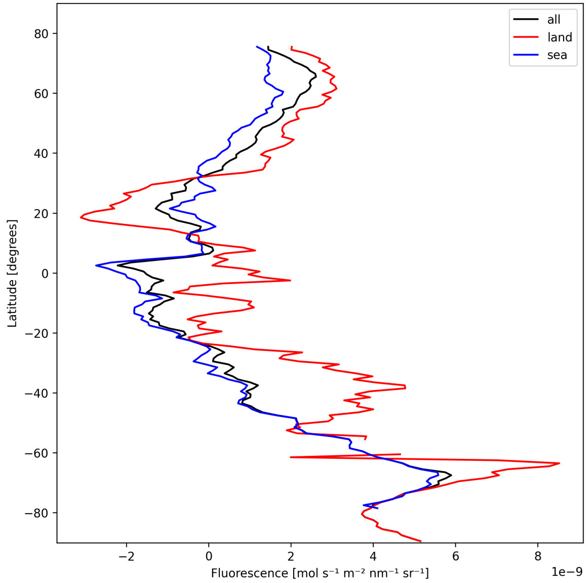
Figure 23: Zonal average of “Fluorescence” for 2024-10-25 to 2024-10-27.
