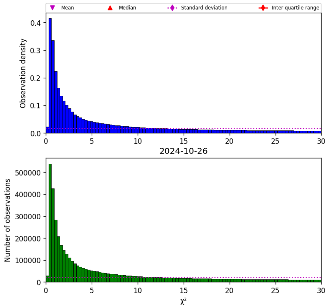
Figure 38: Histogram of “ \chi^2 ” for 2024-10-25 to 2024-10-27
