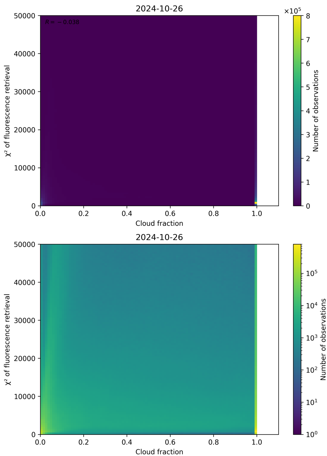
Figure 78: Scatter density plot of “Cloud fraction” against “ \chi^2 of fluorescence retrieval” for 2024-10-25 to 2024-10-27.
