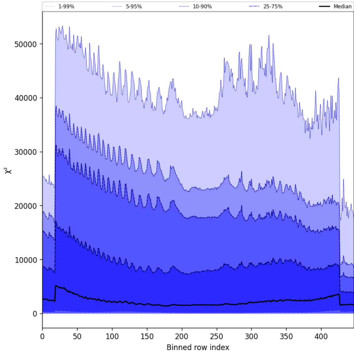
Figure 55: Along track statistics of “ \chi^2 ” for 2024-10-25 to 2024-10-27
