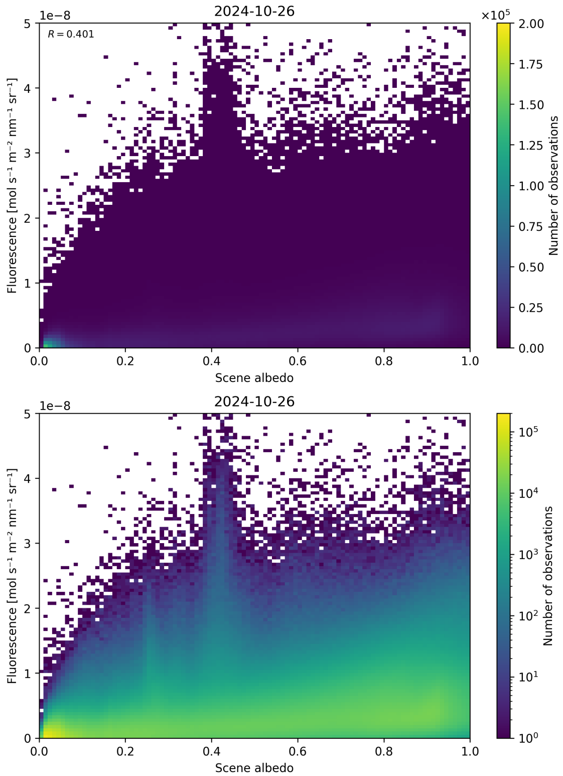
Figure 114: Scatter density plot of “Scene albedo” against “Fluorescence” for 2024-10-25 to 2024-10-27.
