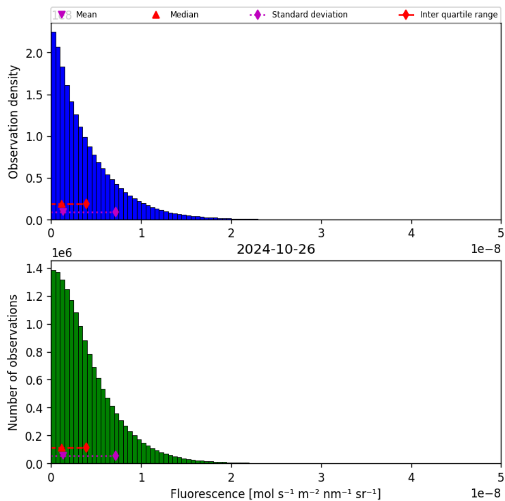
Figure 40: Histogram of “Fluorescence” for 2024-10-25 to 2024-10-27
