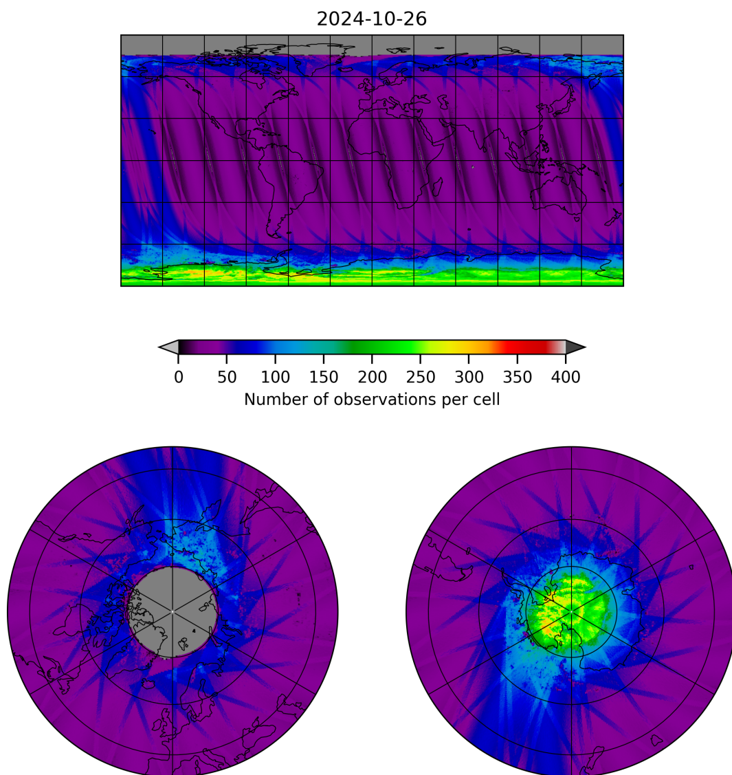
Figure 11: Map of the number of observations for 2024-10-25 to 2024-10-27
