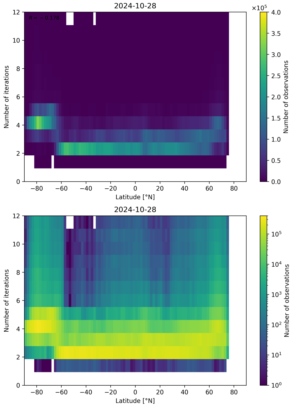
Figure 102: Scatter density plot of “Latitude” against “Number of iterations” for 2024-10-27 to 2024-10-29.
