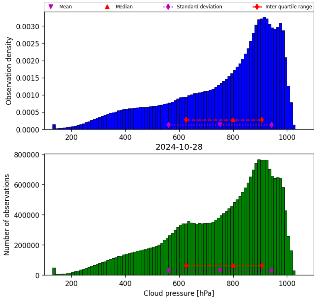
Figure 30: Histogram of “Cloud pressure” for 2024-10-27 to 2024-10-29
