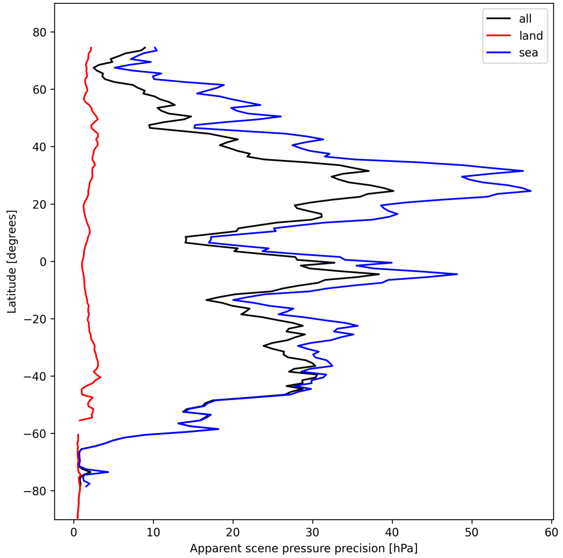
Figure 20: Zonal average of “Apparent scene pressure precision” for 2024-10-27 to 2024-10-29.
