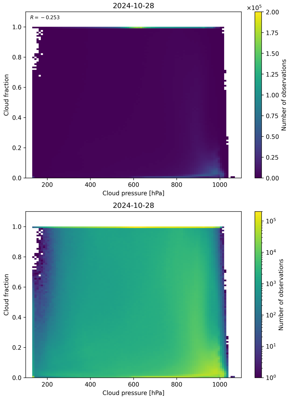
Figure 87: Scatter density plot of “Cloud pressure” against “Cloud fraction” for 2024-10-27 to 2024-10-29.
