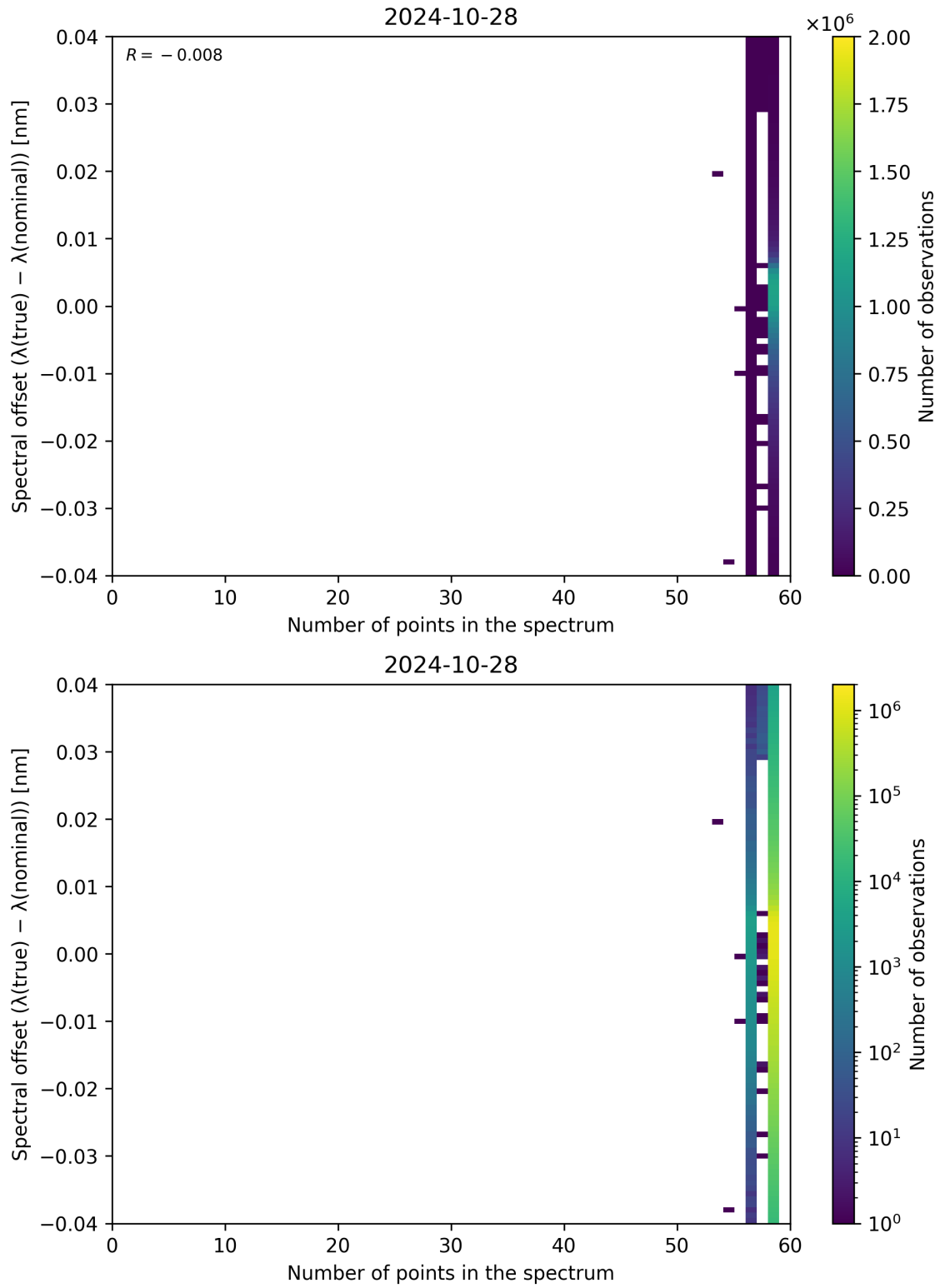
Figure 110: Scatter density plot of “Number of points in the spectrum” against “Spectral offset ( \lambda_{\text{true}} - \lambda_{\text{nominal}} )” for 2024-10-27 to 2024-10-29.
