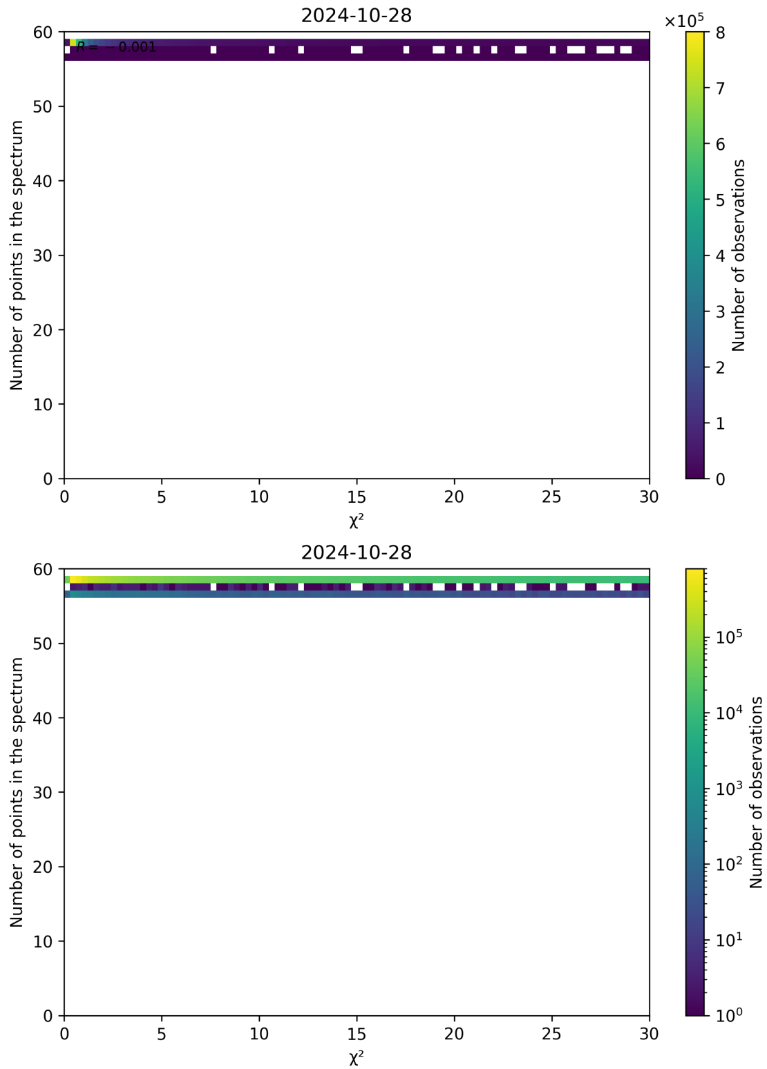
Figure 74: Scatter density plot of “ \chi^2 ” against “Number of points in the spectrum” for 2024-10-27 to 2024-10-29.
