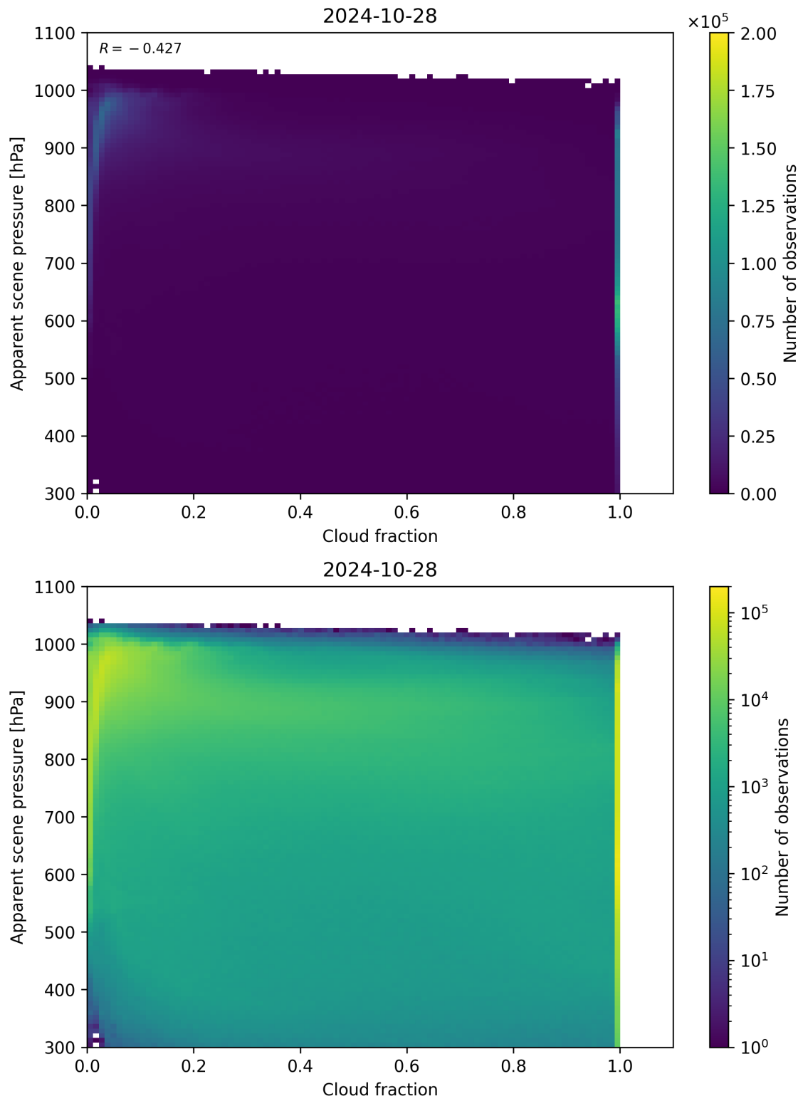
Figure 76: Scatter density plot of “Cloud fraction” against “Apparent scene pressure” for 2024-10-27 to 2024-10-29.
