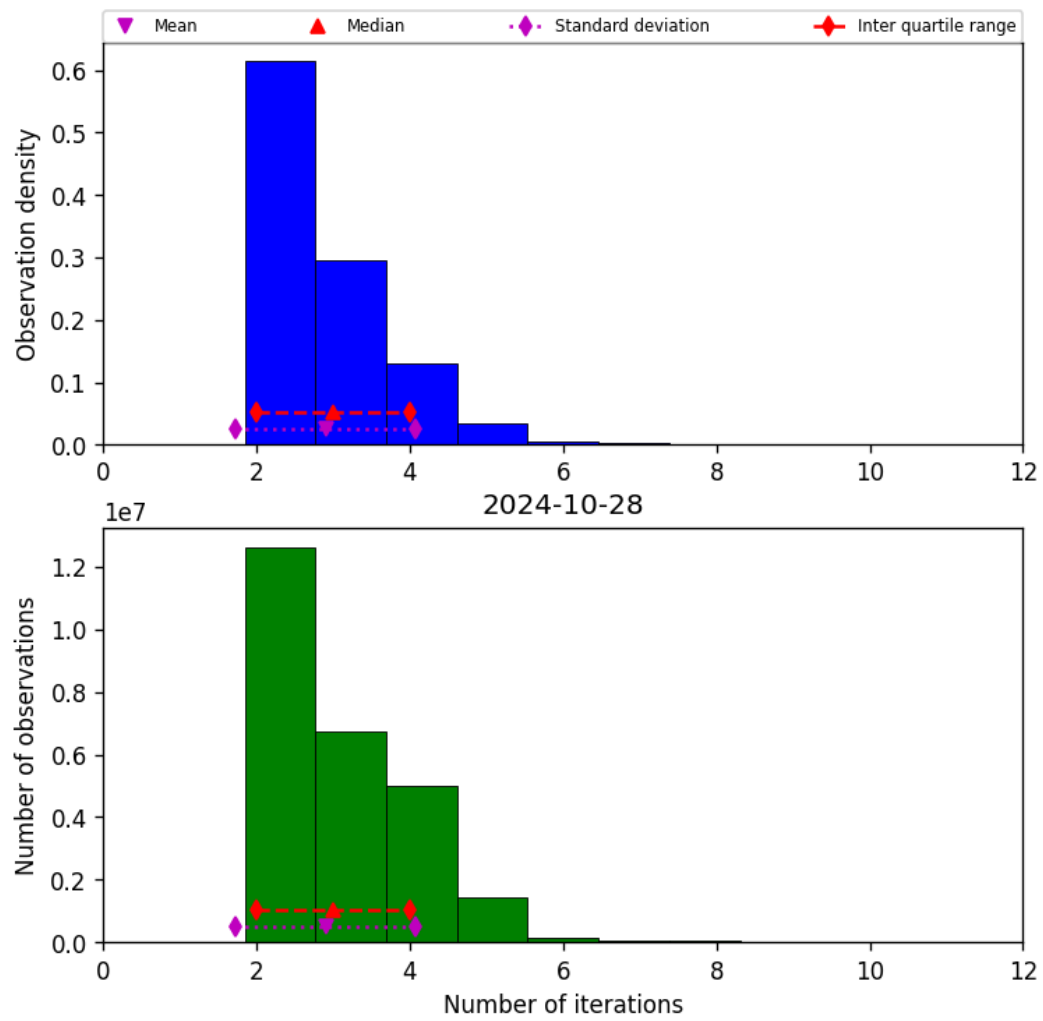
Figure 39: Histogram of “Number of iterations” for 2024-10-27 to 2024-10-29
