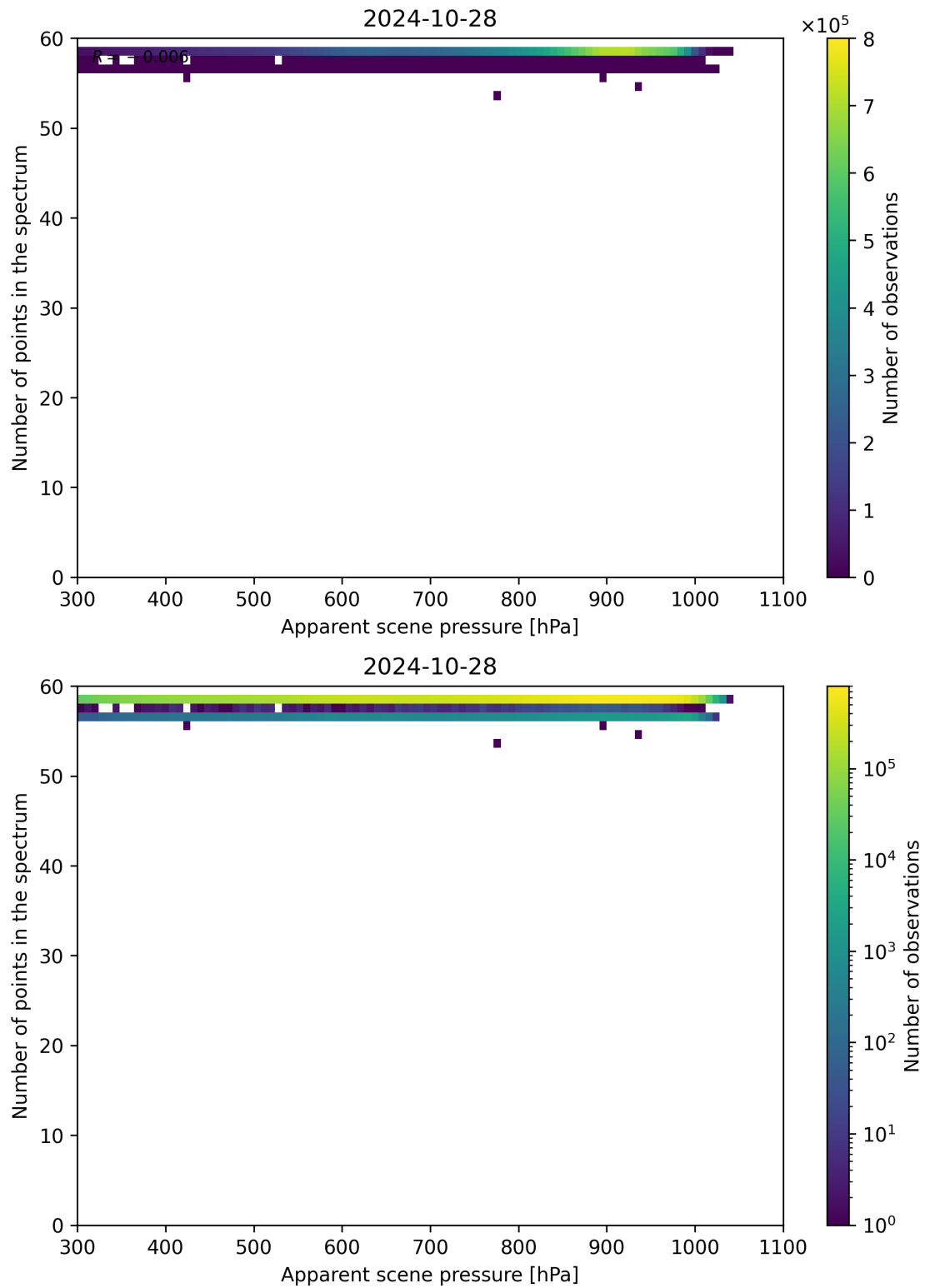
Figure 67: Scatter density plot of “Apparent scene pressure” against “Number of points in the spectrum” for 2024-10-27 to 2024-10-29.
