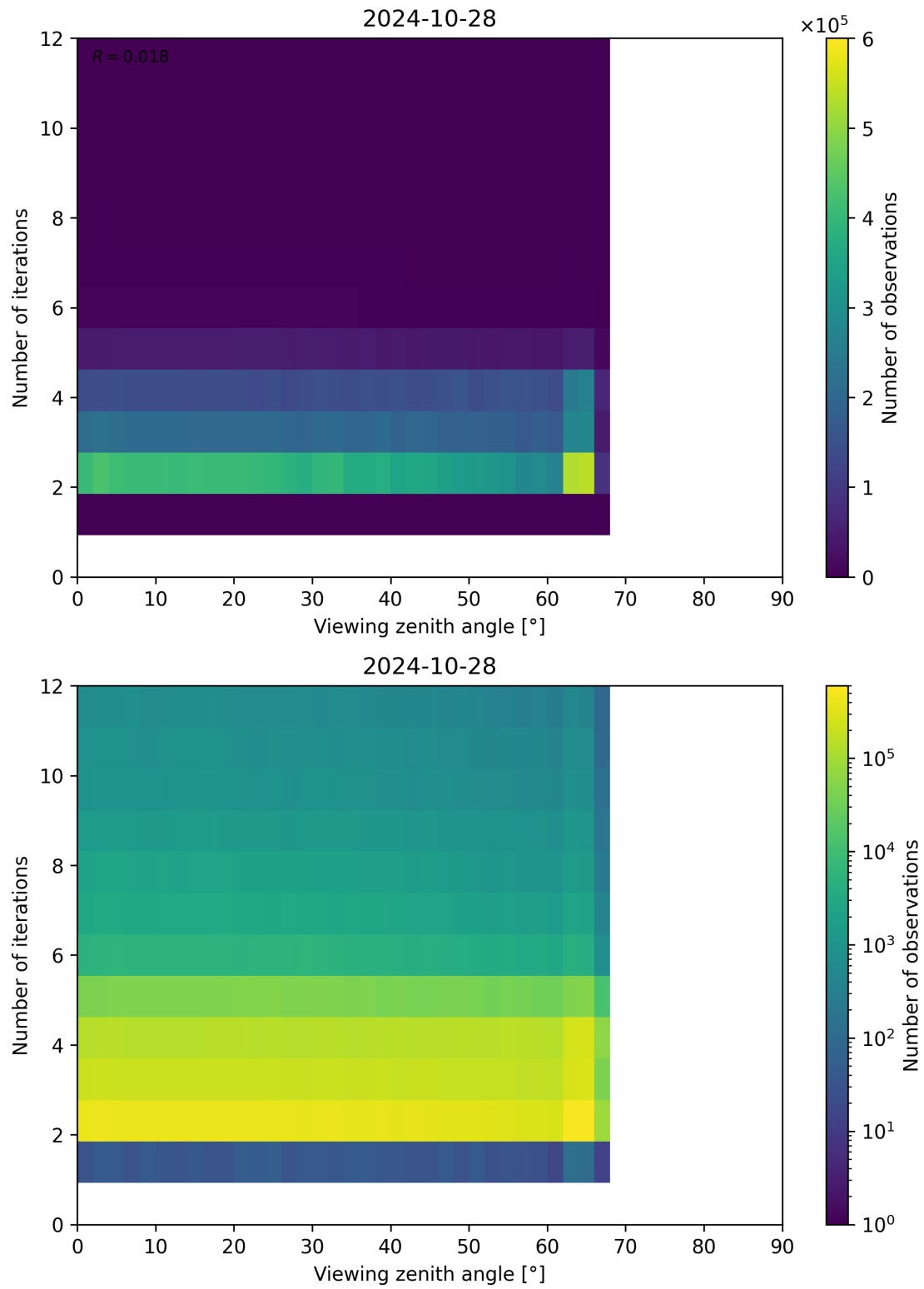
Figure 136: Scatter density plot of “Viewing zenith angle” against “Number of iterations” for 2024-10-27 to 2024-10-29.
