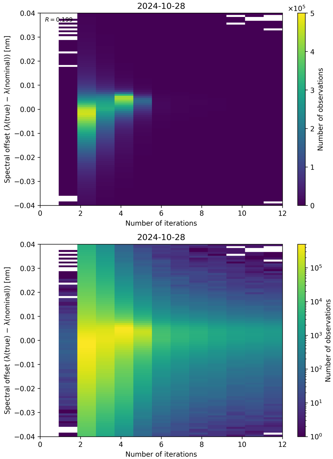
Figure 109: Scatter density plot of “Number of iterations” against “Spectral offset ( \lambda_{\text{true}} - \lambda_{\text{nominal}} )” for 2024-10-27 to 2024-10-29.
