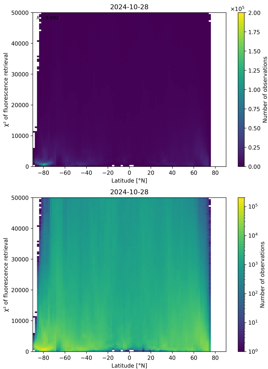
Figure 98: Scatter density plot of “Latitude” against “ \chi^2 of fluorescence retrieval” for 2024-10-27 to 2024-10-29.
