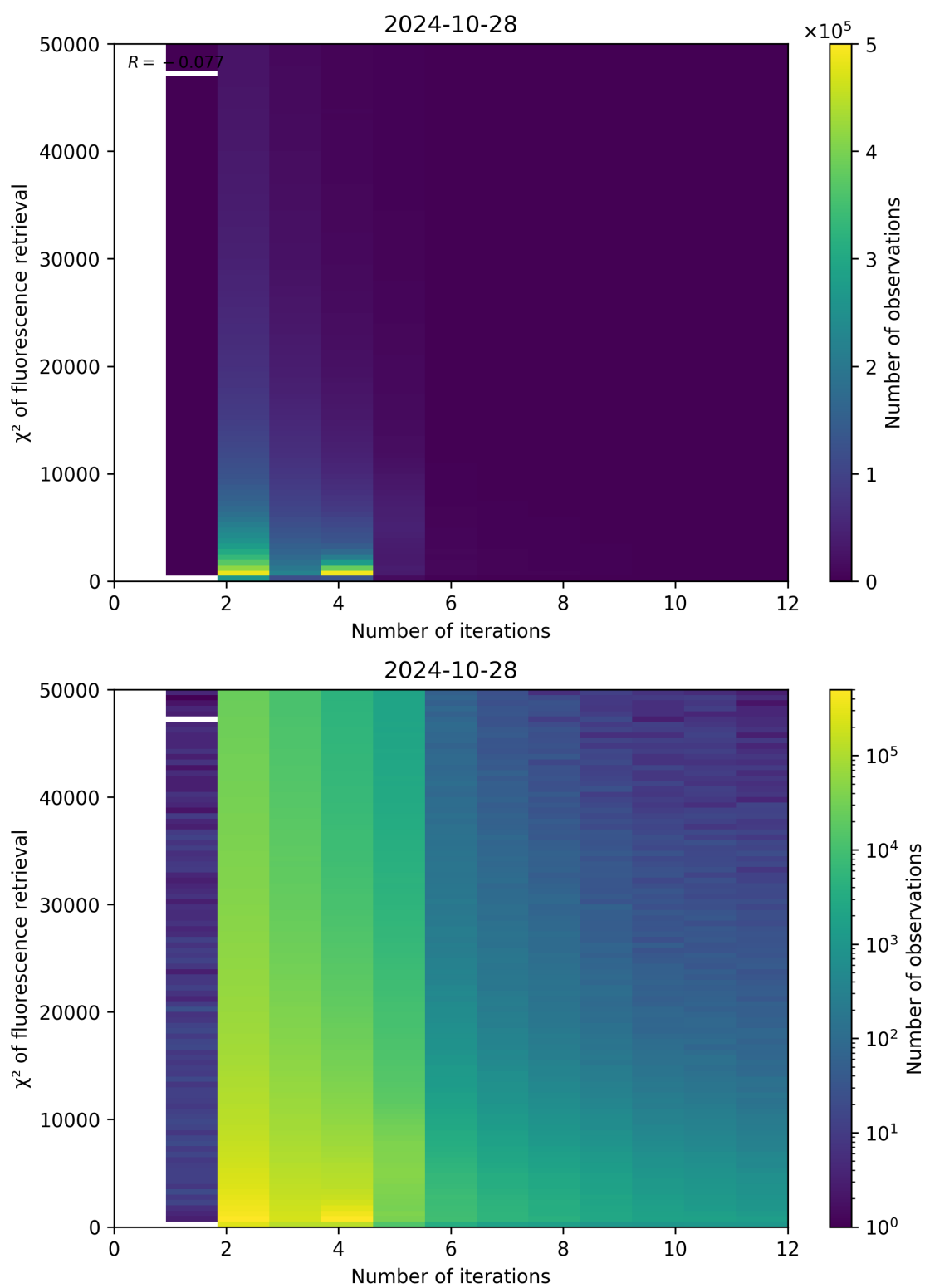
Figure 106: Scatter density plot of “Number of iterations” against “ \chi^2 of fluorescence retrieval” for 2024-10-27 to 2024-10-29.
