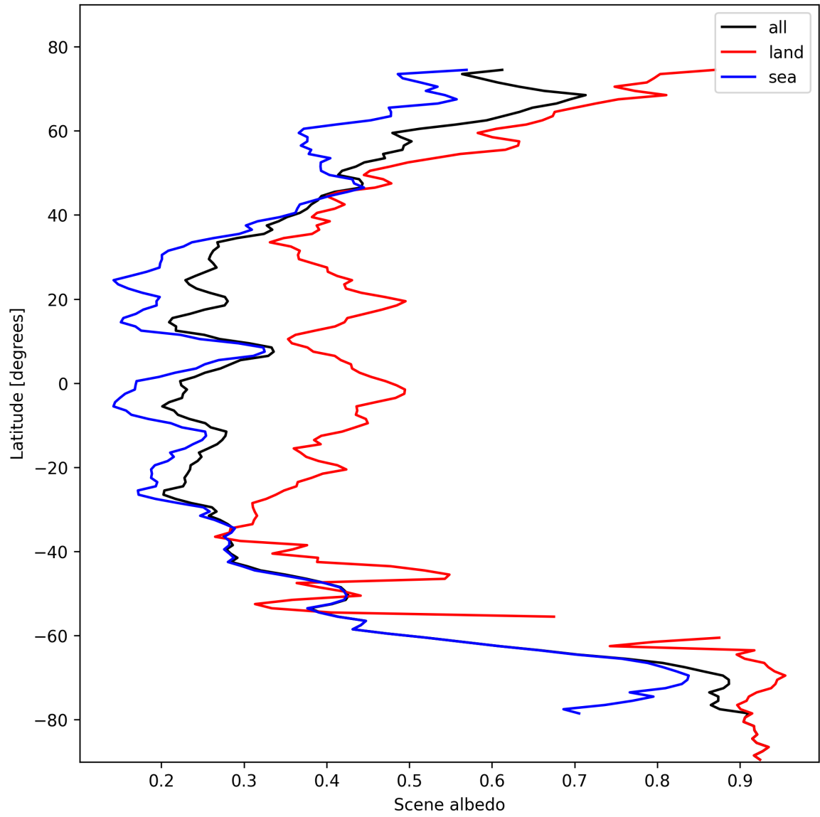
Figure 17: Zonal average of “Scene albedo” for 2024-10-27 to 2024-10-29.
