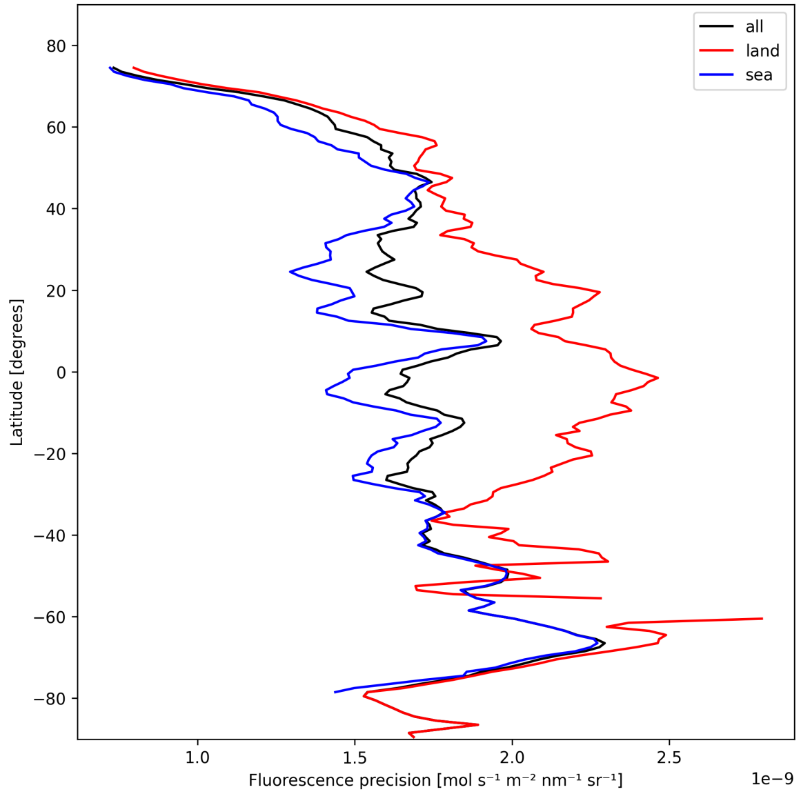
Figure 24: Zonal average of “Fluorescence precision” for 2024-10-27 to 2024-10-29.
