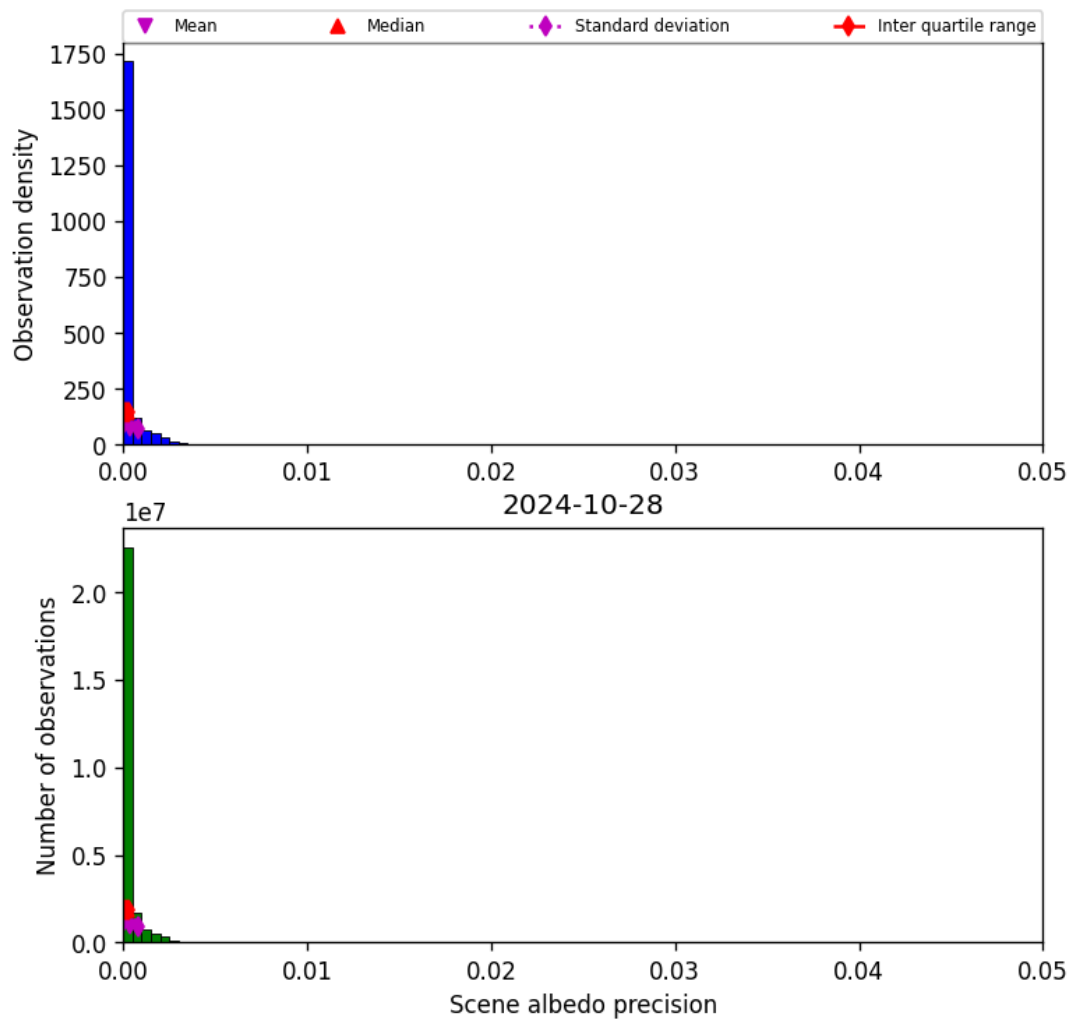
Figure 35: Histogram of “Scene albedo precision” for 2024-10-27 to 2024-10-29
