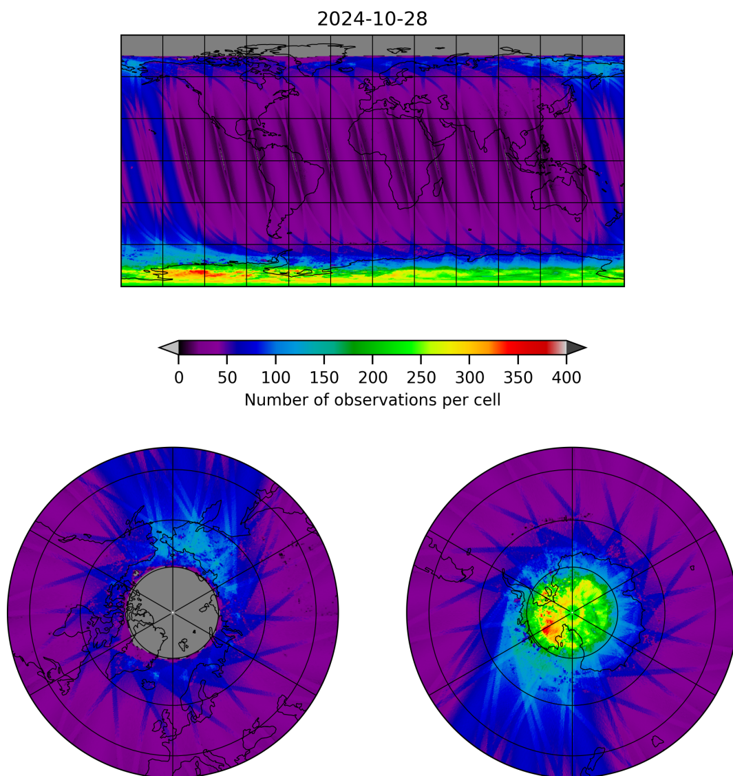
Figure 11: Map of the number of observations for 2024-10-27 to 2024-10-29
