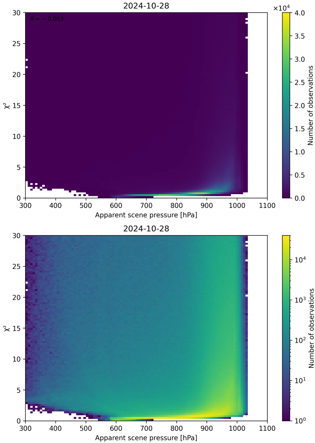
Figure 63: Scatter density plot of “Apparent scene pressure” against “ \chi^2 ” for 2024-10-27 to 2024-10-29.
