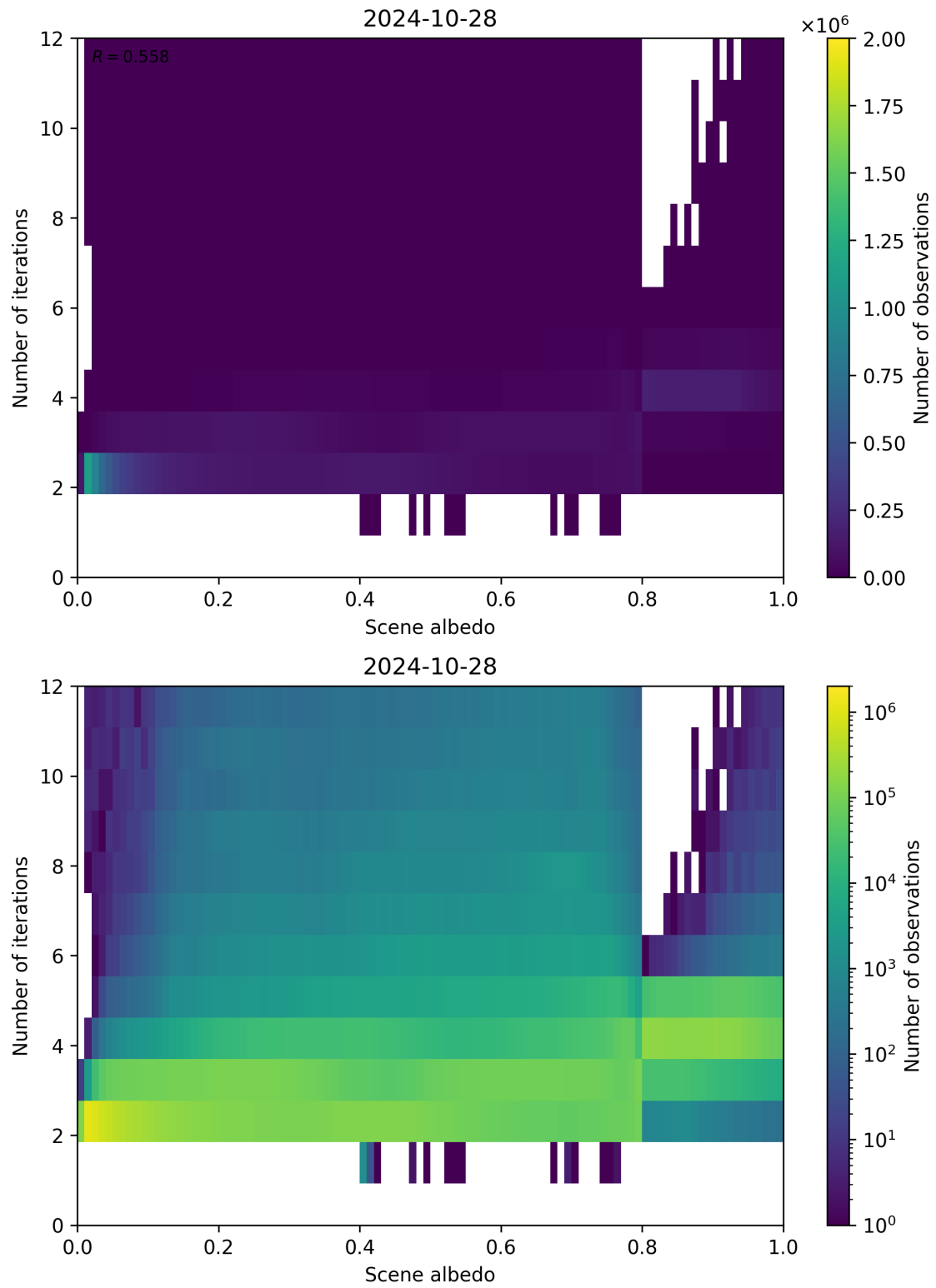
Figure 115: Scatter density plot of “Scene albedo” against “Number of iterations” for 2024-10-27 to 2024-10-29.
