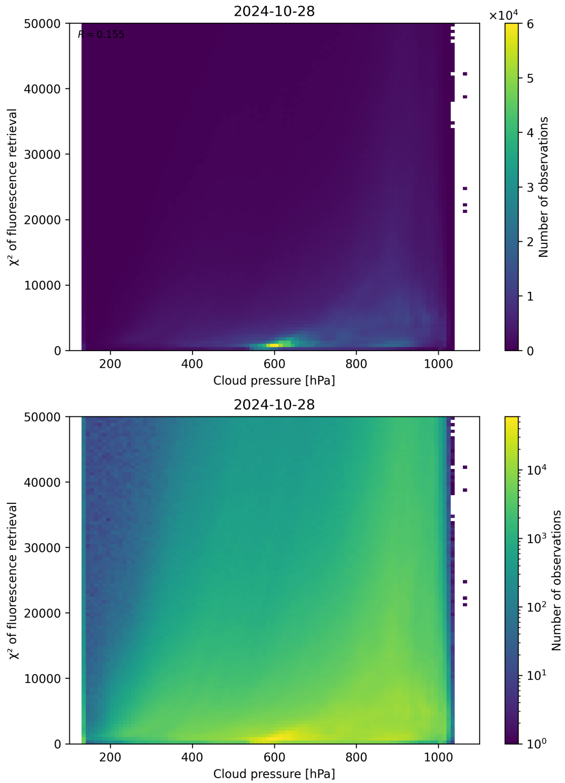
Figure 86: Scatter density plot of “Cloud pressure” against “ \chi^2 of fluorescence retrieval” for 2024-10-27 to 2024-10-29.
