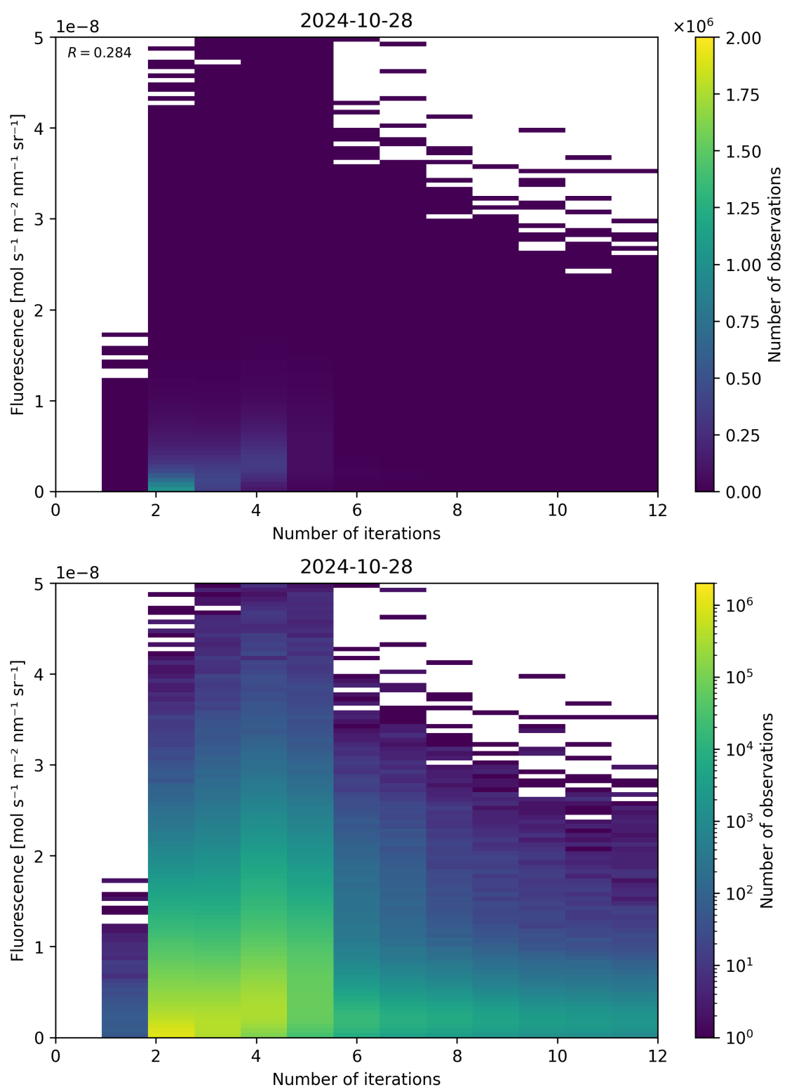
Figure 107: Scatter density plot of “Number of iterations” against “Fluorescence” for 2024-10-27 to 2024-10-29.
