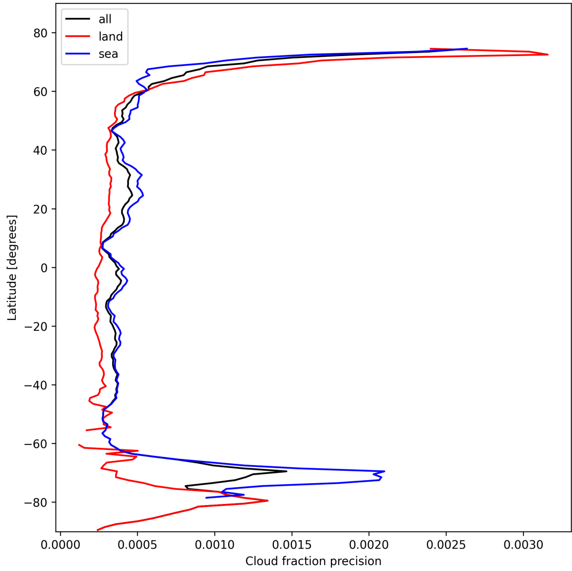
Figure 16: Zonal average of “Cloud fraction precision” for 2024-10-27 to 2024-10-29.
