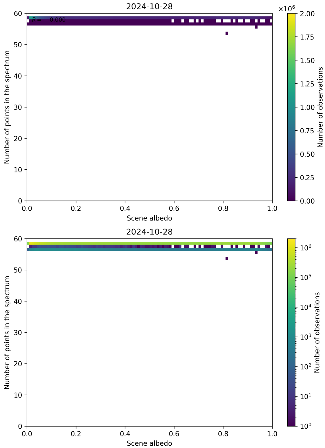
Figure 116: Scatter density plot of “Scene albedo” against “Number of points in the spectrum” for 2024-10-27 to 2024-10-29.
