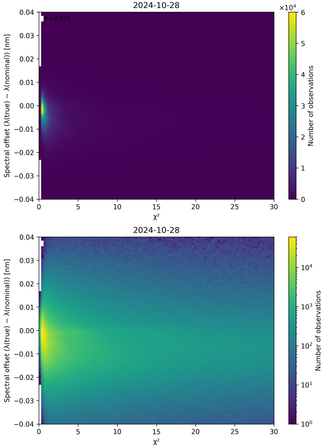
Figure 75: Scatter density plot of “ \chi^2 ” against “Spectral offset ( \lambda_{\text{true}} - \lambda_{\text{nominal}} )” for 2024-10-27 to 2024-10-29.
