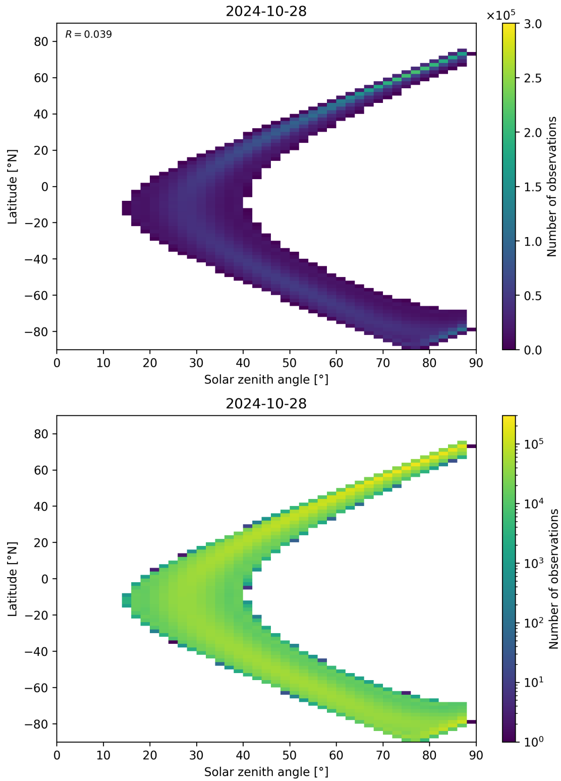
Figure 124: Scatter density plot of “Solar zenith angle” against “Latitude” for 2024-10-27 to 2024-10-29.
