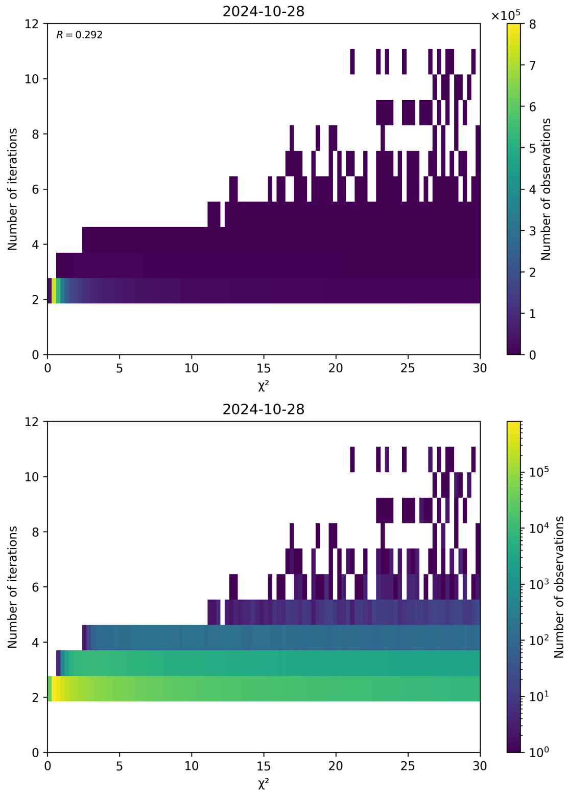
Figure 73: Scatter density plot of “ \chi^2 ” against “Number of iterations” for 2024-10-27 to 2024-10-29.
