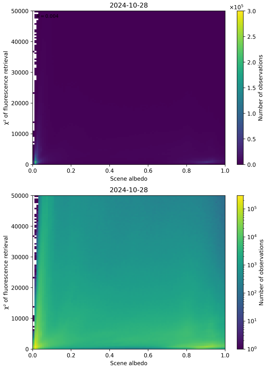
Figure 113: Scatter density plot of “Scene albedo” against “ \chi^2 of fluorescence retrieval” for 2024-10-27 to 2024-10-29.
