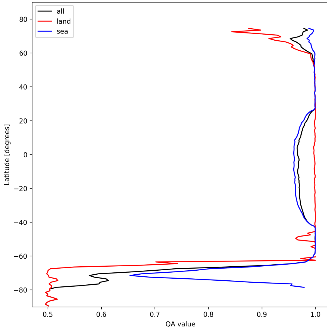
Figure 12: Zonal average of “QA value” for 2024-10-27 to 2024-10-29.
