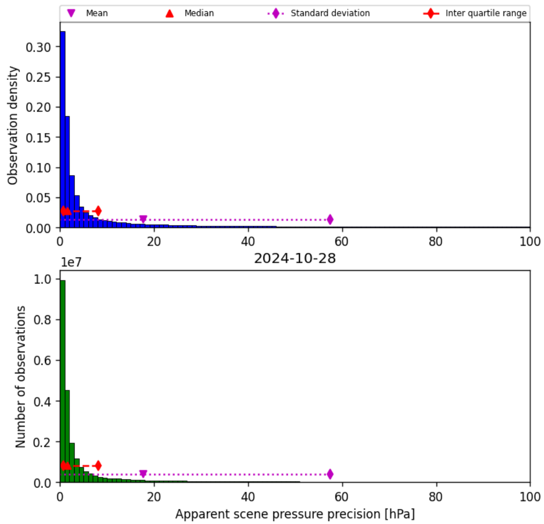
Figure 37: Histogram of “Apparent scene pressure precision” for 2024-10-27 to 2024-10-29
