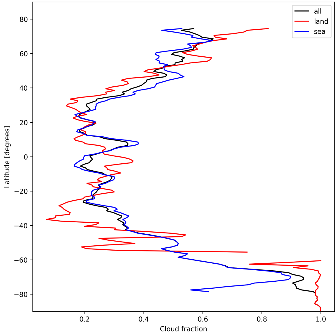
Figure 15: Zonal average of “Cloud fraction” for 2024-10-27 to 2024-10-29.
