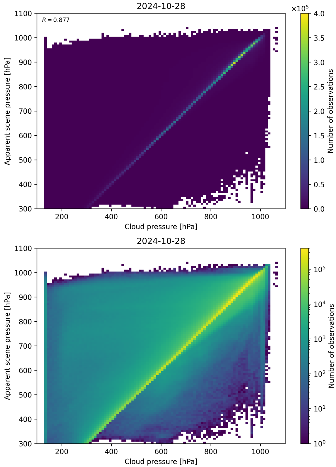
Figure 84: Scatter density plot of “Cloud pressure” against “Apparent scene pressure” for 2024-10-27 to 2024-10-29.
