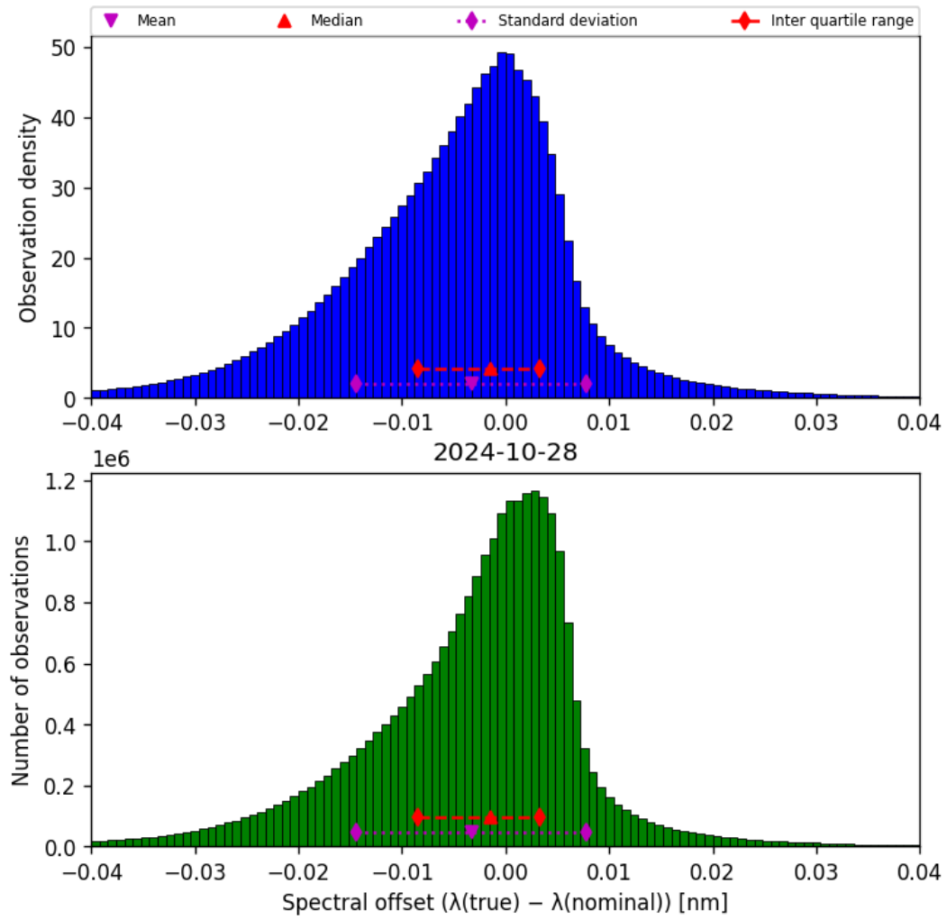
Figure 45: Histogram of “Spectral offset ( \lambda_{\text{true}} - \lambda_{\text{nominal}} )” for 2024-10-27 to 2024-10-29
