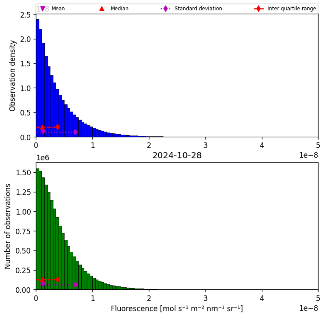
Figure 40: Histogram of “Fluorescence” for 2024-10-27 to 2024-10-29
