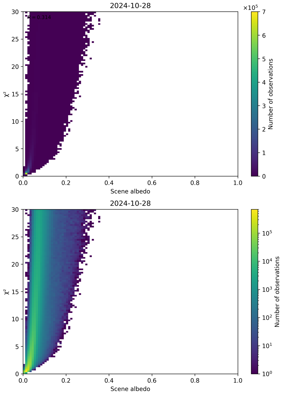
Figure 112: Scatter density plot of “Scene albedo” against “ \chi^2 ” for 2024-10-27 to 2024-10-29.
