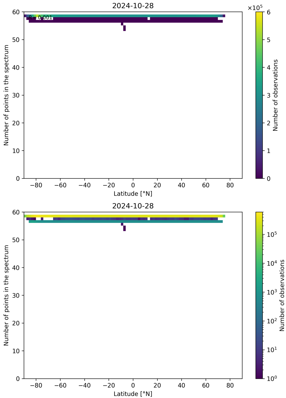
Figure 103: Scatter density plot of “Latitude” against “Number of points in the spectrum” for 2024-10-27 to 2024-10-29.
