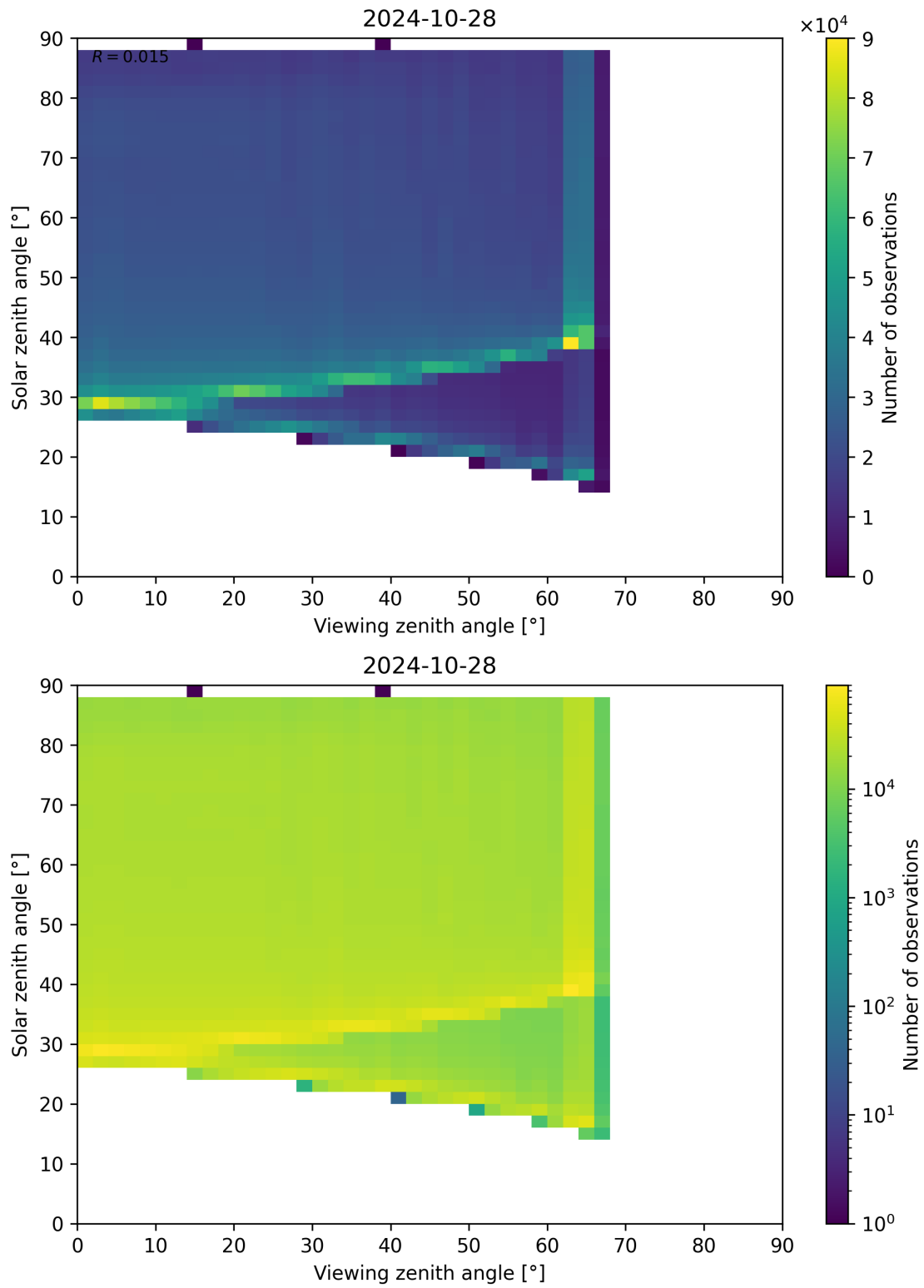
Figure 139: Scatter density plot of “Viewing zenith angle” against “Solar zenith angle” for 2024-10-27 to 2024-10-29.
