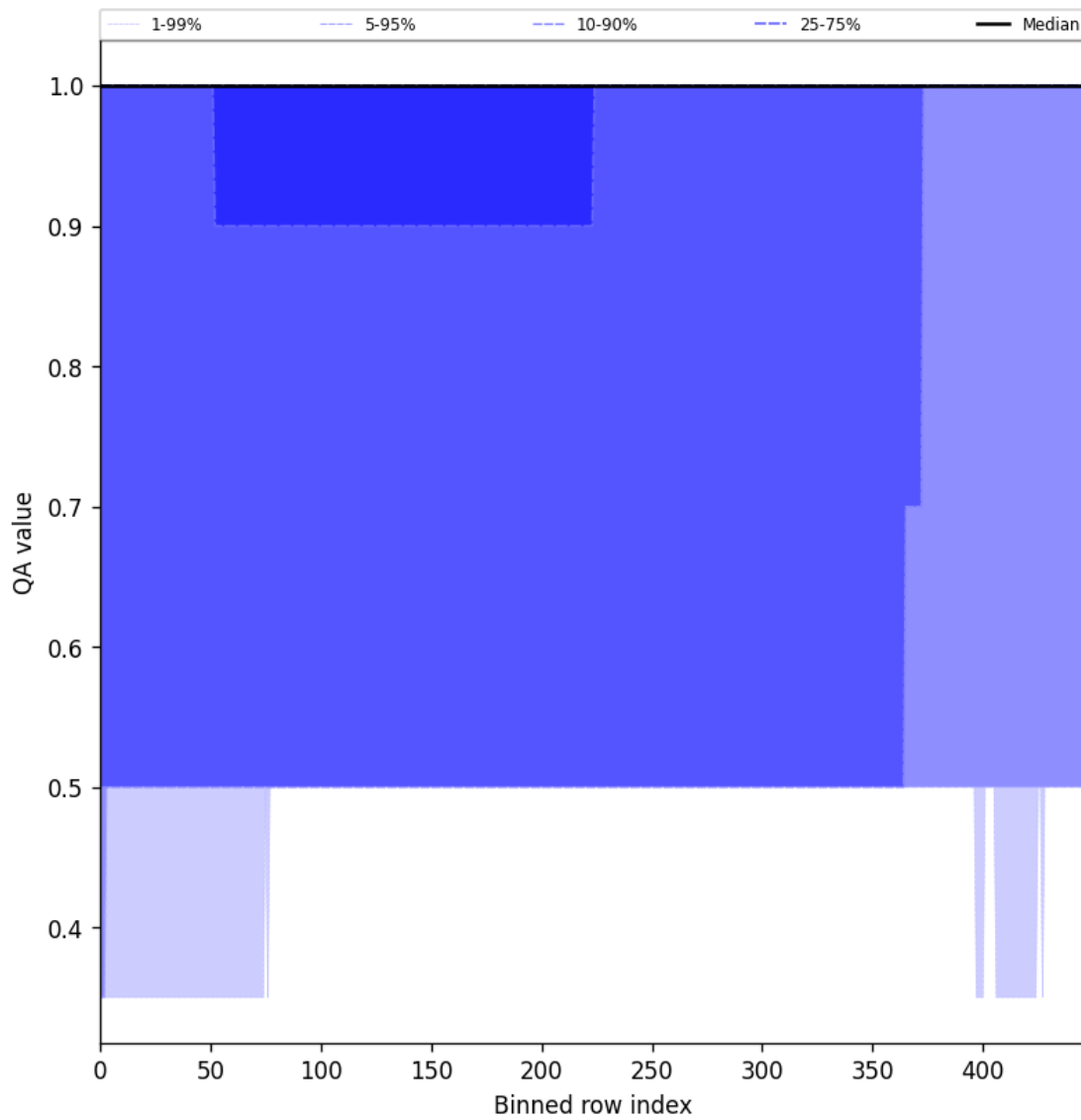
Figure 46: Along track statistics of “QA value” for 2024-10-27 to 2024-10-29
