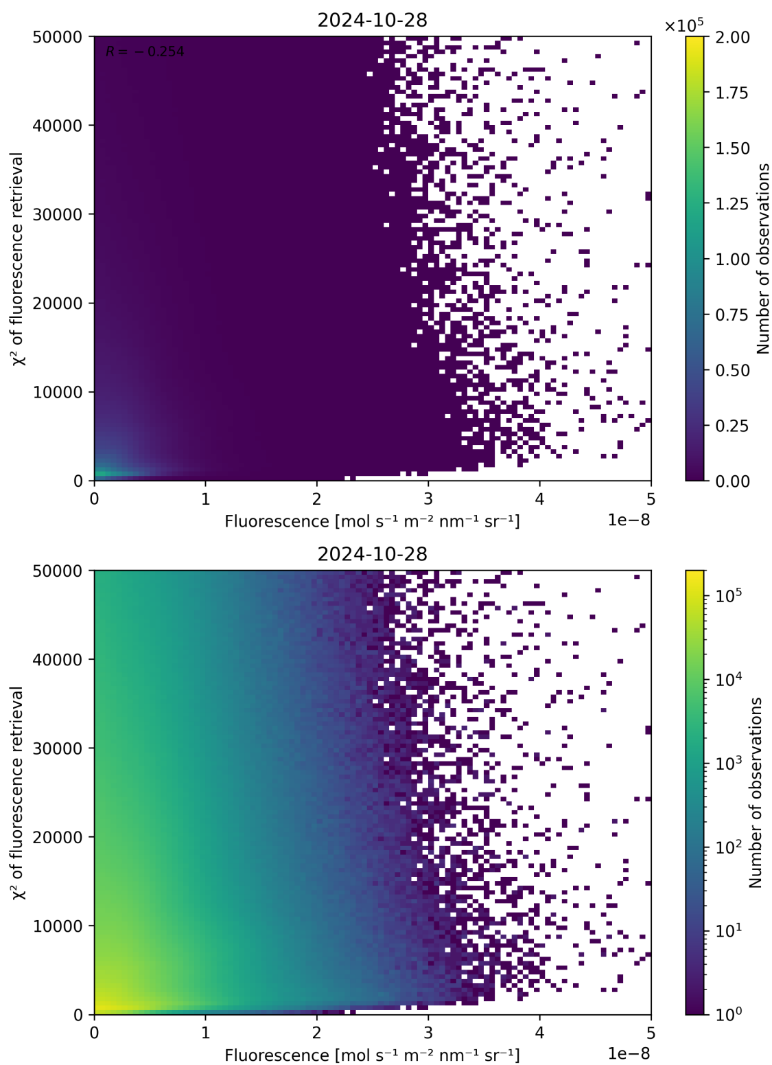
Figure 93: Scatter density plot of “Fluorescence” against “ \chi^2 of fluorescence retrieval” for 2024-10-27 to 2024-10-29.
