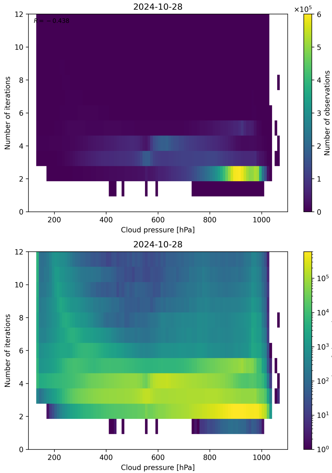
Figure 89: Scatter density plot of “Cloud pressure” against “Number of iterations” for 2024-10-27 to 2024-10-29.
