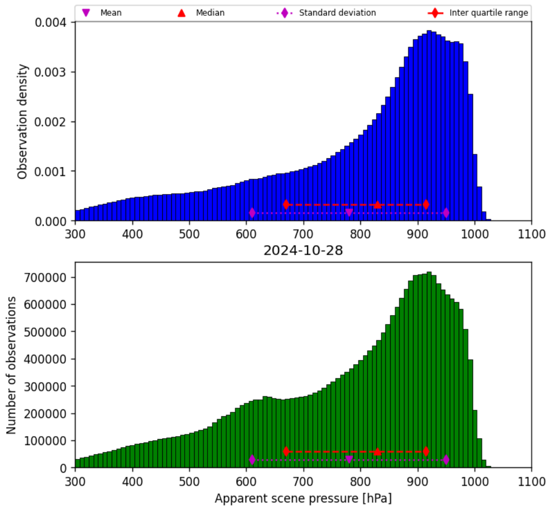
Figure 36: Histogram of “Apparent scene pressure” for 2024-10-27 to 2024-10-29
