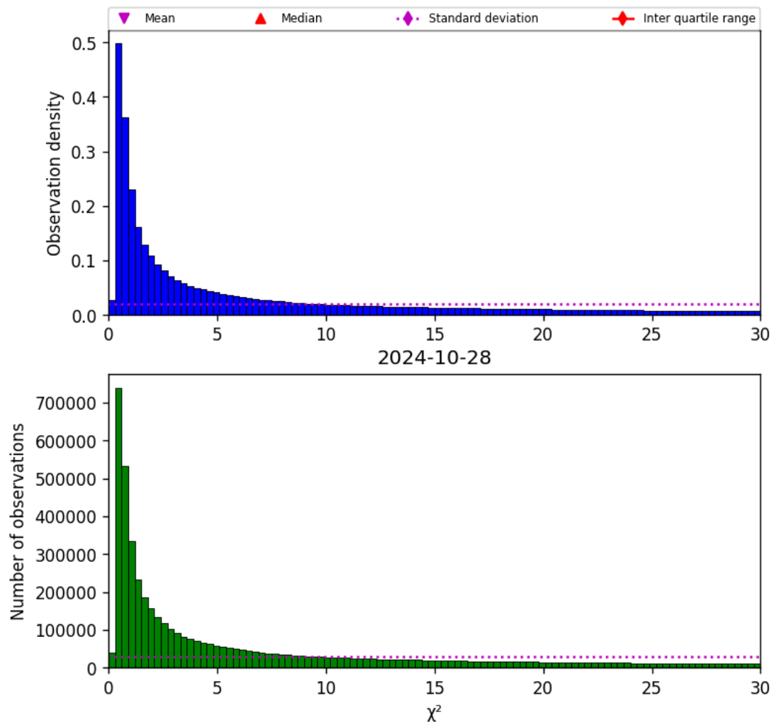
Figure 38: Histogram of “ \chi^2 ” for 2024-10-27 to 2024-10-29
