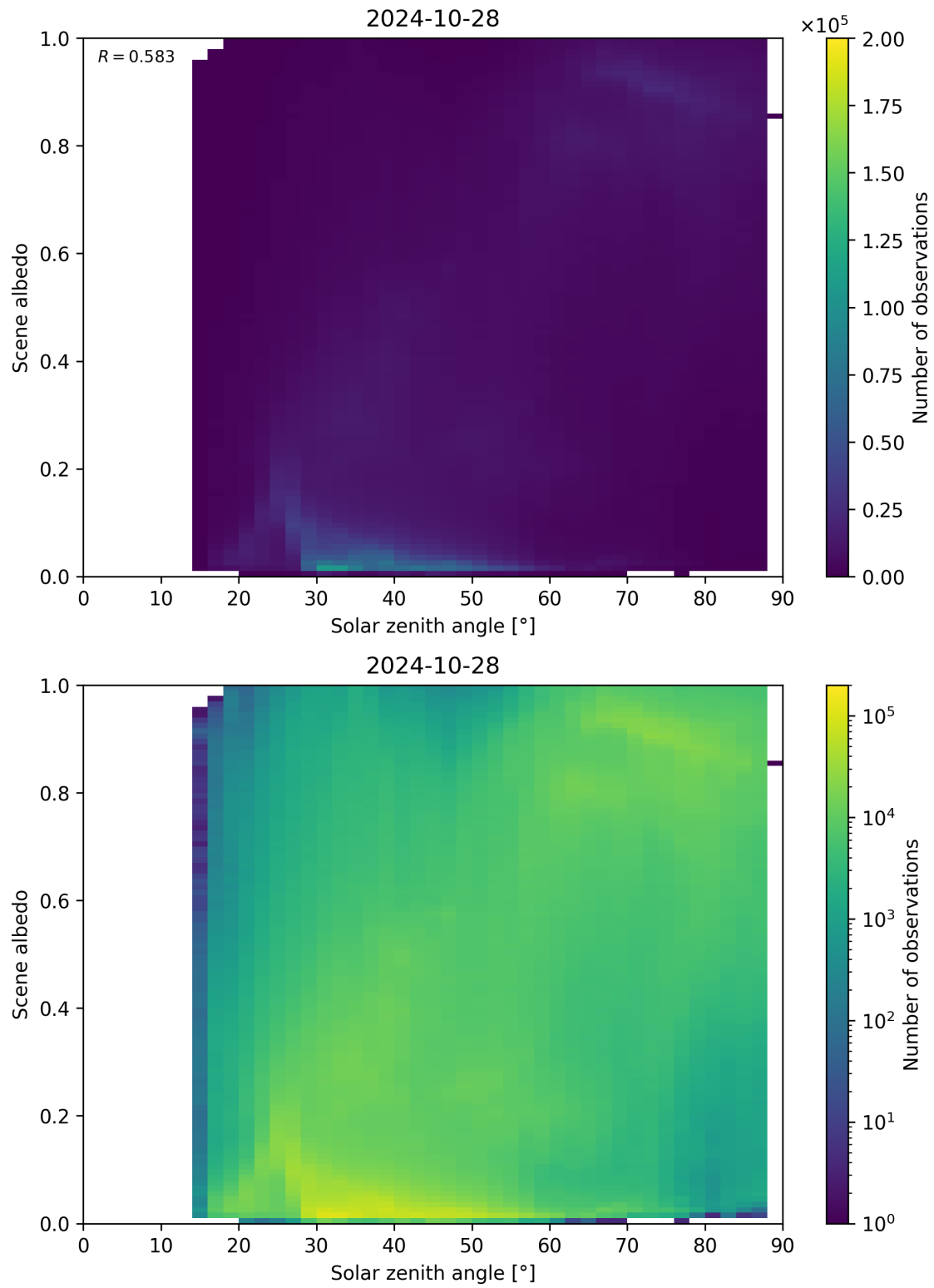
Figure 127: Scatter density plot of “Solar zenith angle” against “Scene albedo” for 2024-10-27 to 2024-10-29.
