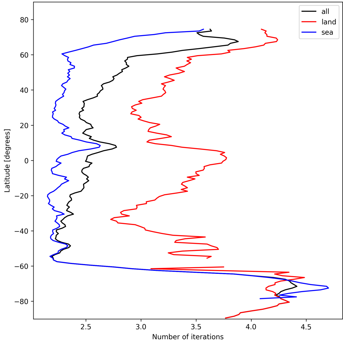
Figure 22: Zonal average of “Number of iterations” for 2024-10-27 to 2024-10-29.
