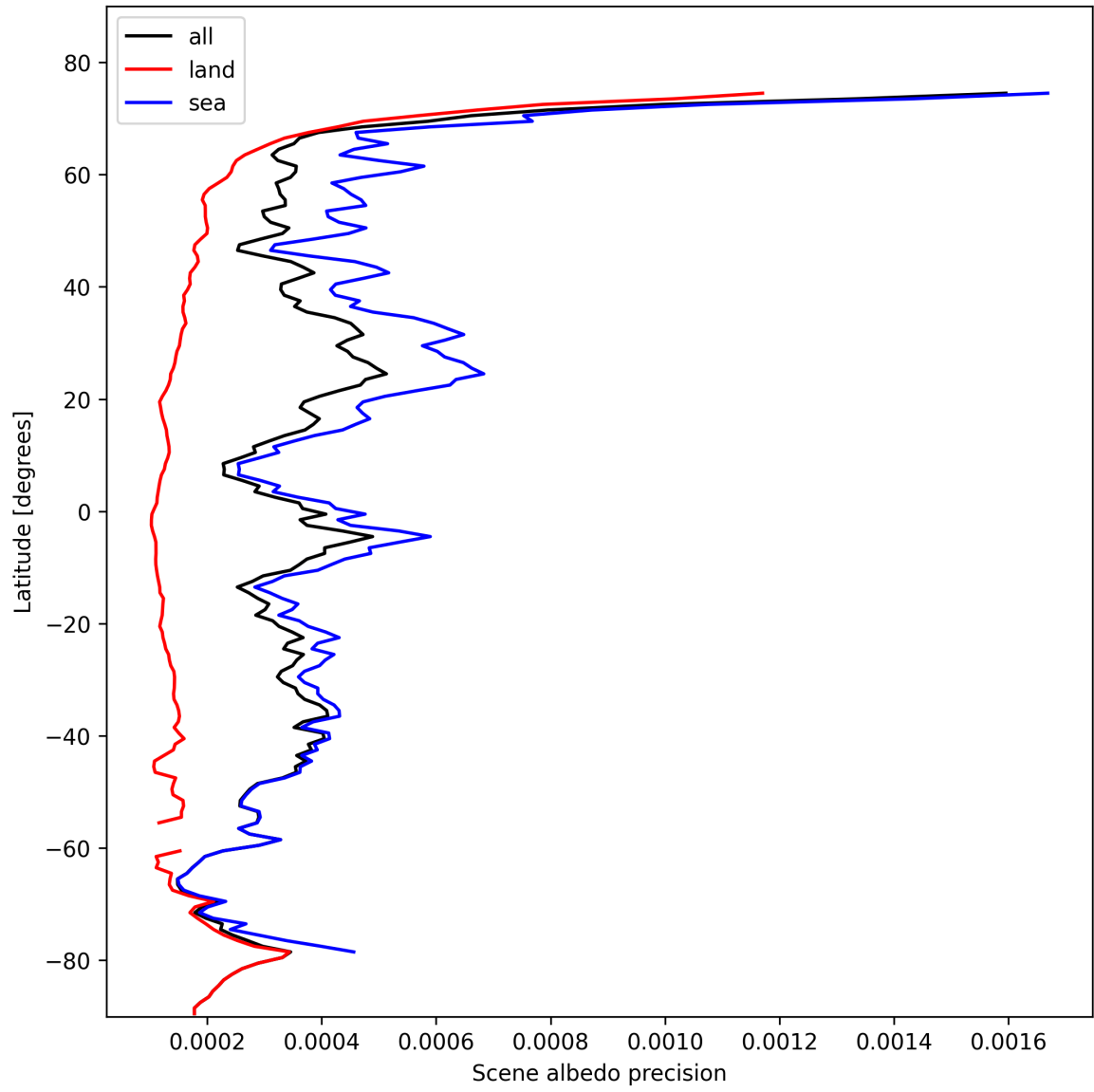
Figure 18: Zonal average of “Scene albedo precision” for 2024-10-27 to 2024-10-29.
