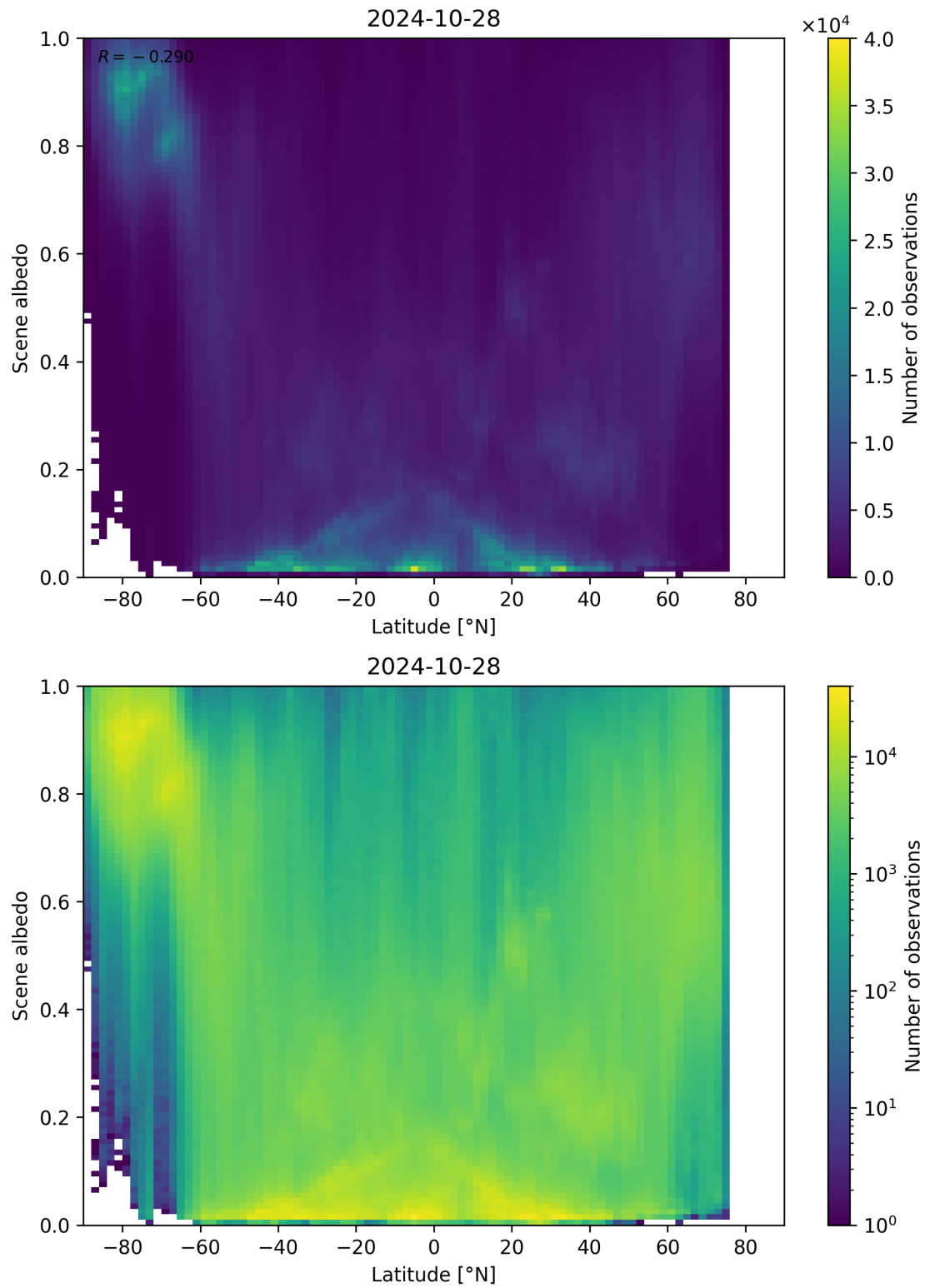
Figure 104: Scatter density plot of “Latitude” against “Scene albedo” for 2024-10-27 to 2024-10-29.
