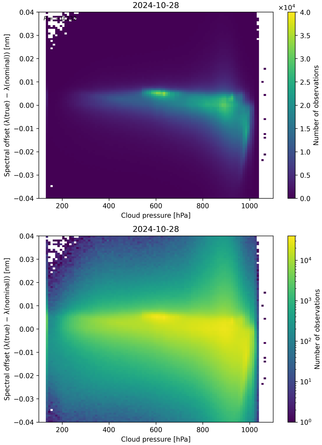
Figure 92: Scatter density plot of “Cloud pressure” against “Spectral offset ( \lambda_{\text{true}} - \lambda_{\text{nominal}} )” for 2024-10-27 to 2024-10-29.
