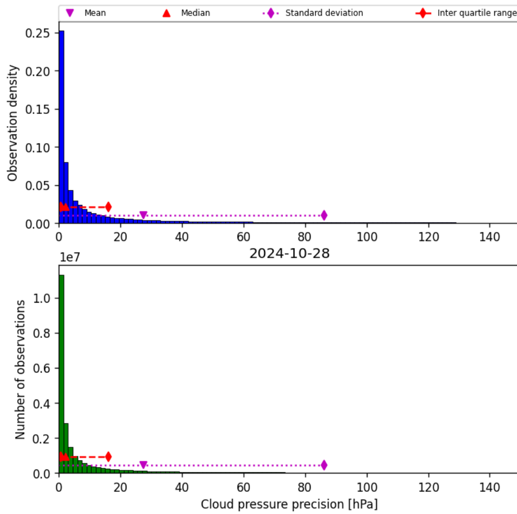
Figure 31: Histogram of “Cloud pressure precision” for 2024-10-27 to 2024-10-29
