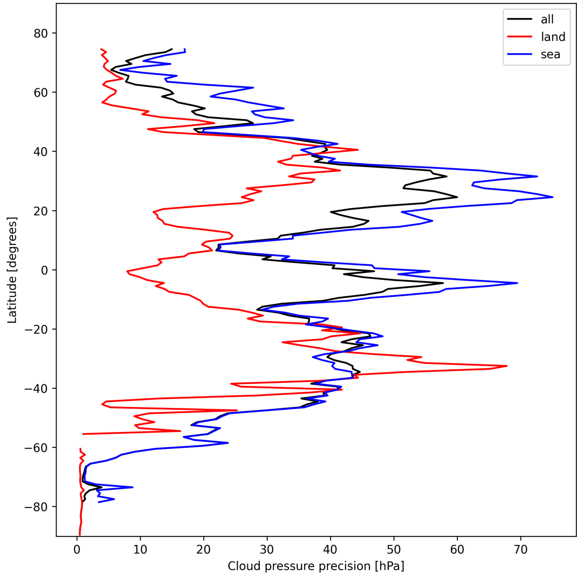
Figure 14: Zonal average of “Cloud pressure precision” for 2024-10-27 to 2024-10-29.
