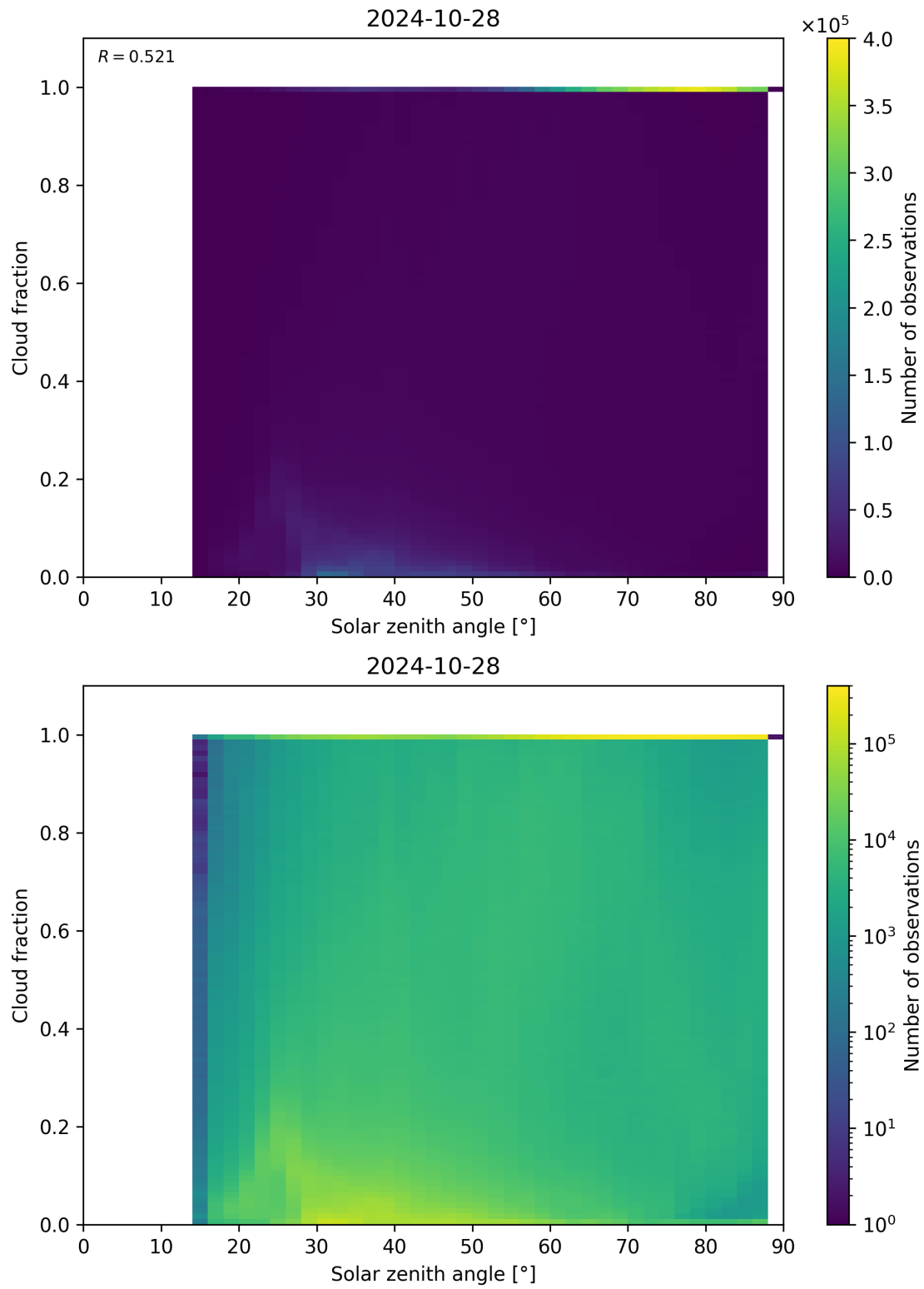
Figure 121: Scatter density plot of “Solar zenith angle” against “Cloud fraction” for 2024-10-27 to 2024-10-29.
