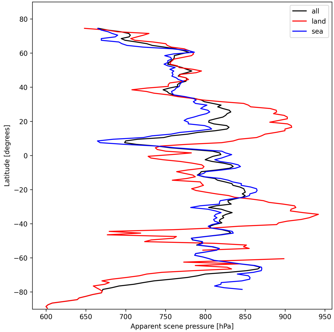
Figure 19: Zonal average of “Apparent scene pressure” for 2024-10-27 to 2024-10-29.
