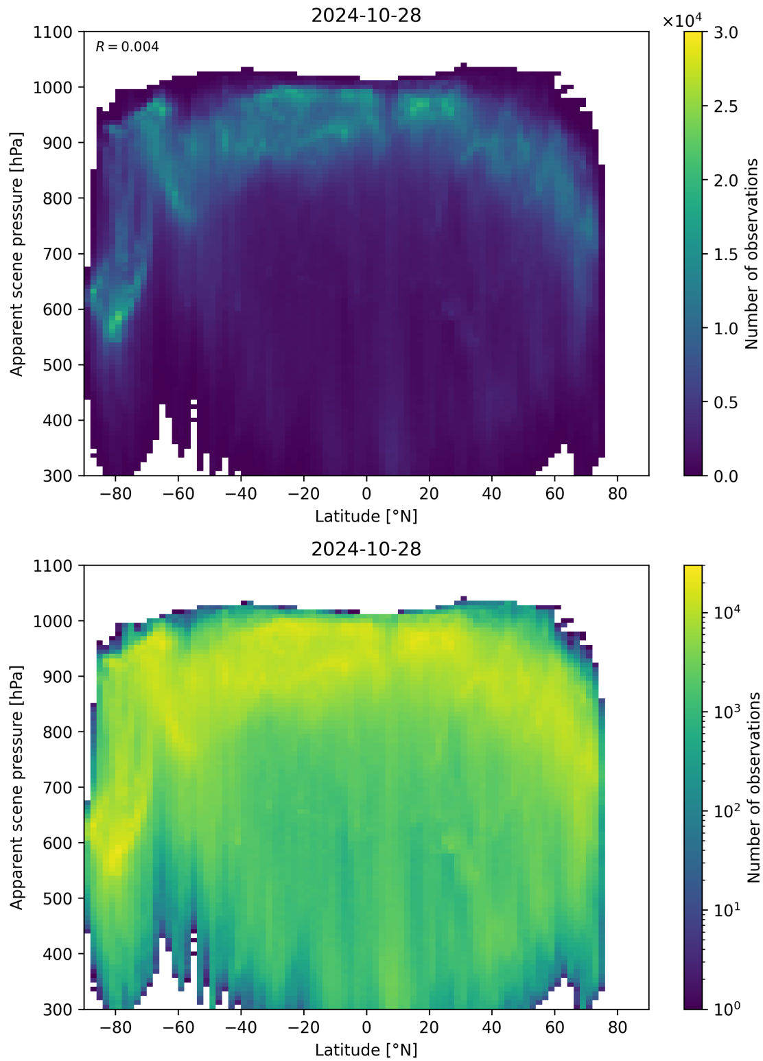
Figure 96: Scatter density plot of “Latitude” against “Apparent scene pressure” for 2024-10-27 to 2024-10-29.
