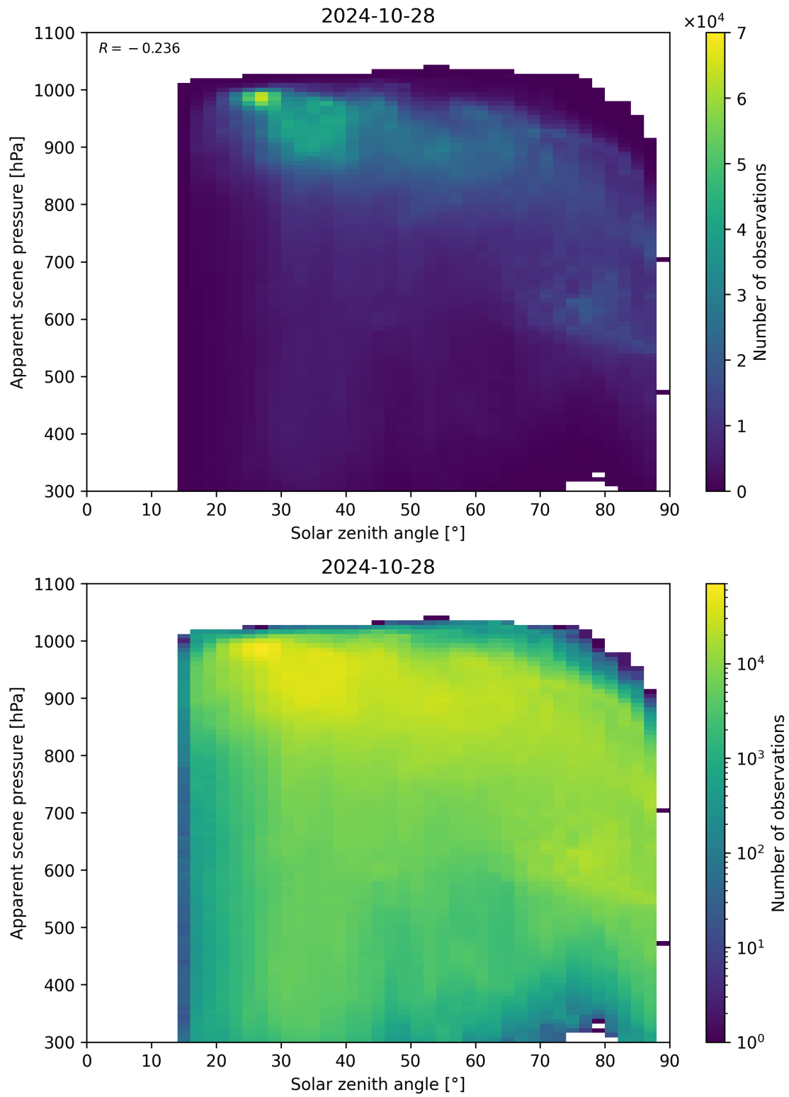
Figure 118: Scatter density plot of “Solar zenith angle” against “Apparent scene pressure” for 2024-10-27 to 2024-10-29.
