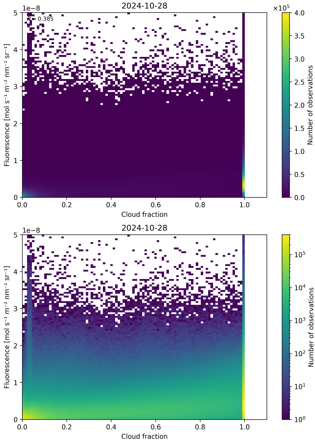
Figure 79: Scatter density plot of “Cloud fraction” against “Fluorescence” for 2024-10-27 to 2024-10-29.
