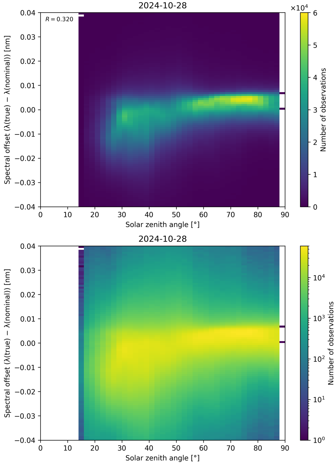
Figure 128: Scatter density plot of “Solar zenith angle” against “Spectral offset ( \lambda_{\text{true}} - \lambda_{\text{nominal}} )” for 2024-10-27 to 2024-10-29.
