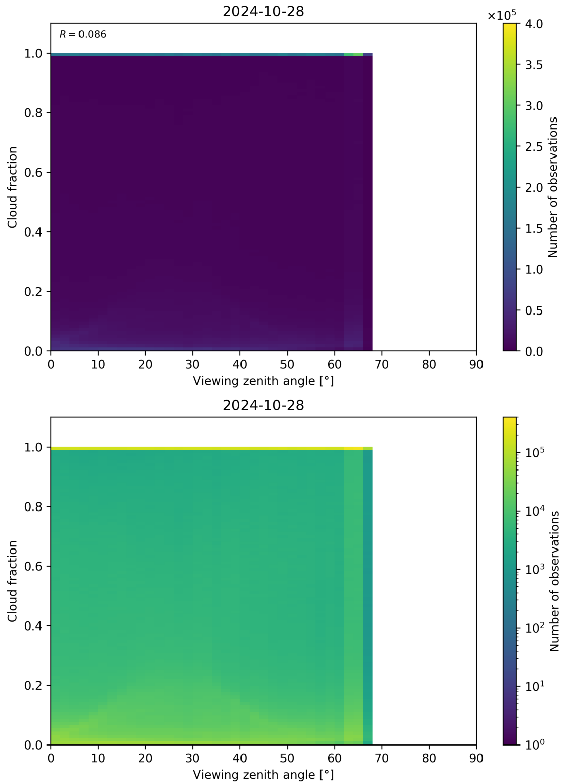
Figure 132: Scatter density plot of “Viewing zenith angle” against “Cloud fraction” for 2024-10-27 to 2024-10-29.
