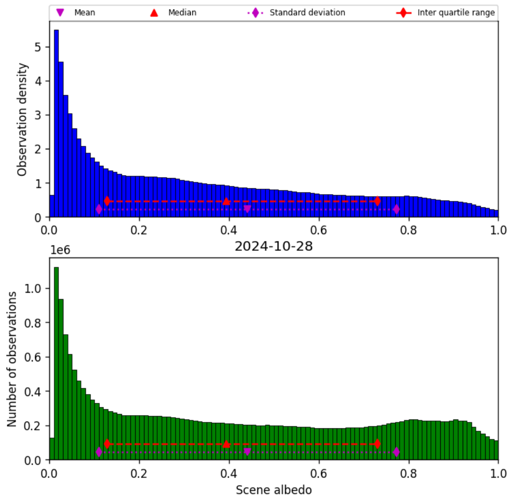
Figure 34: Histogram of “Scene albedo” for 2024-10-27 to 2024-10-29
