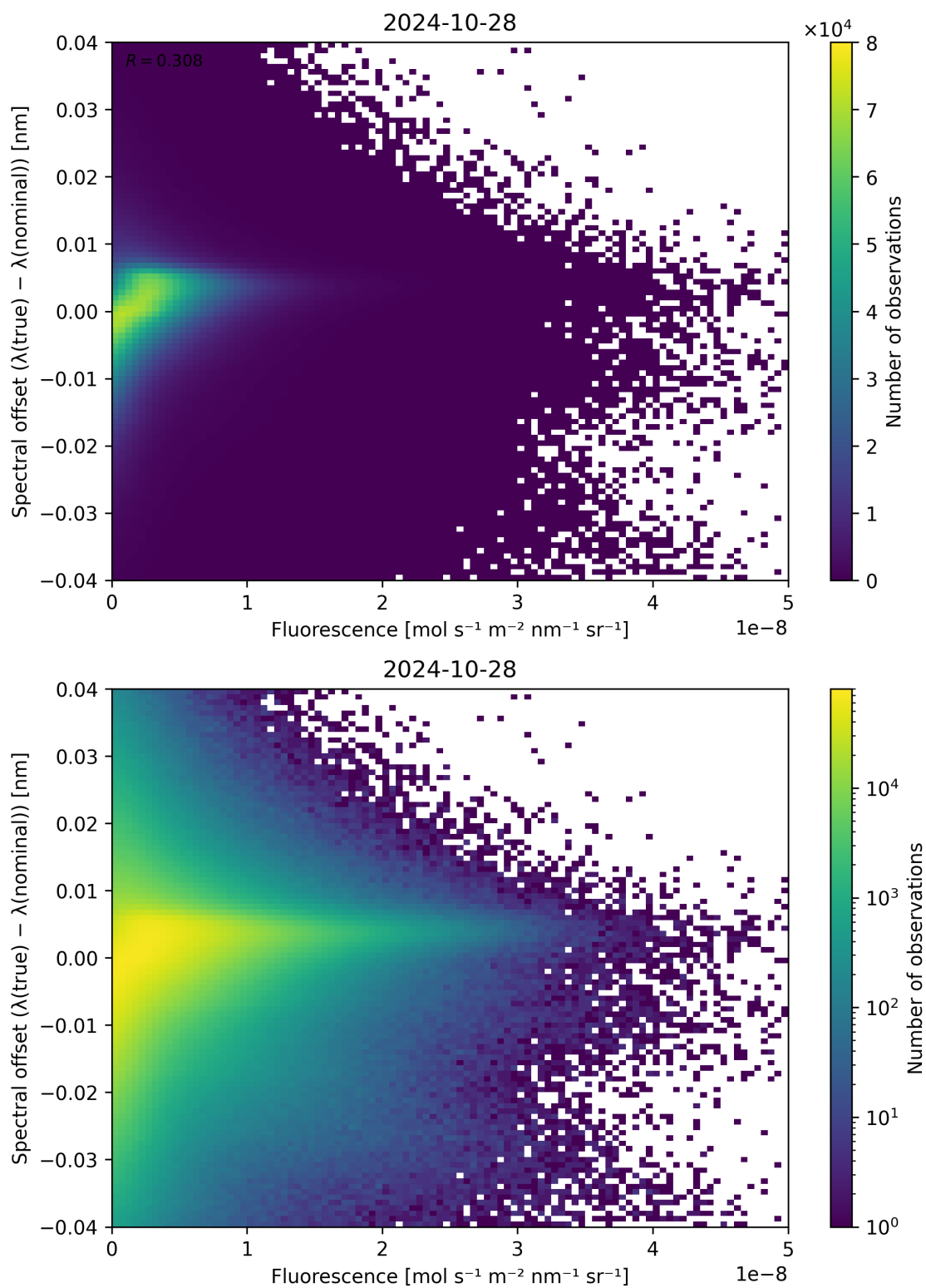
Figure 95: Scatter density plot of “Fluorescence” against “Spectral offset ( \lambda_{\text{true}} - \lambda_{\text{nominal}} )” for 2024-10-27 to 2024-10-29.
