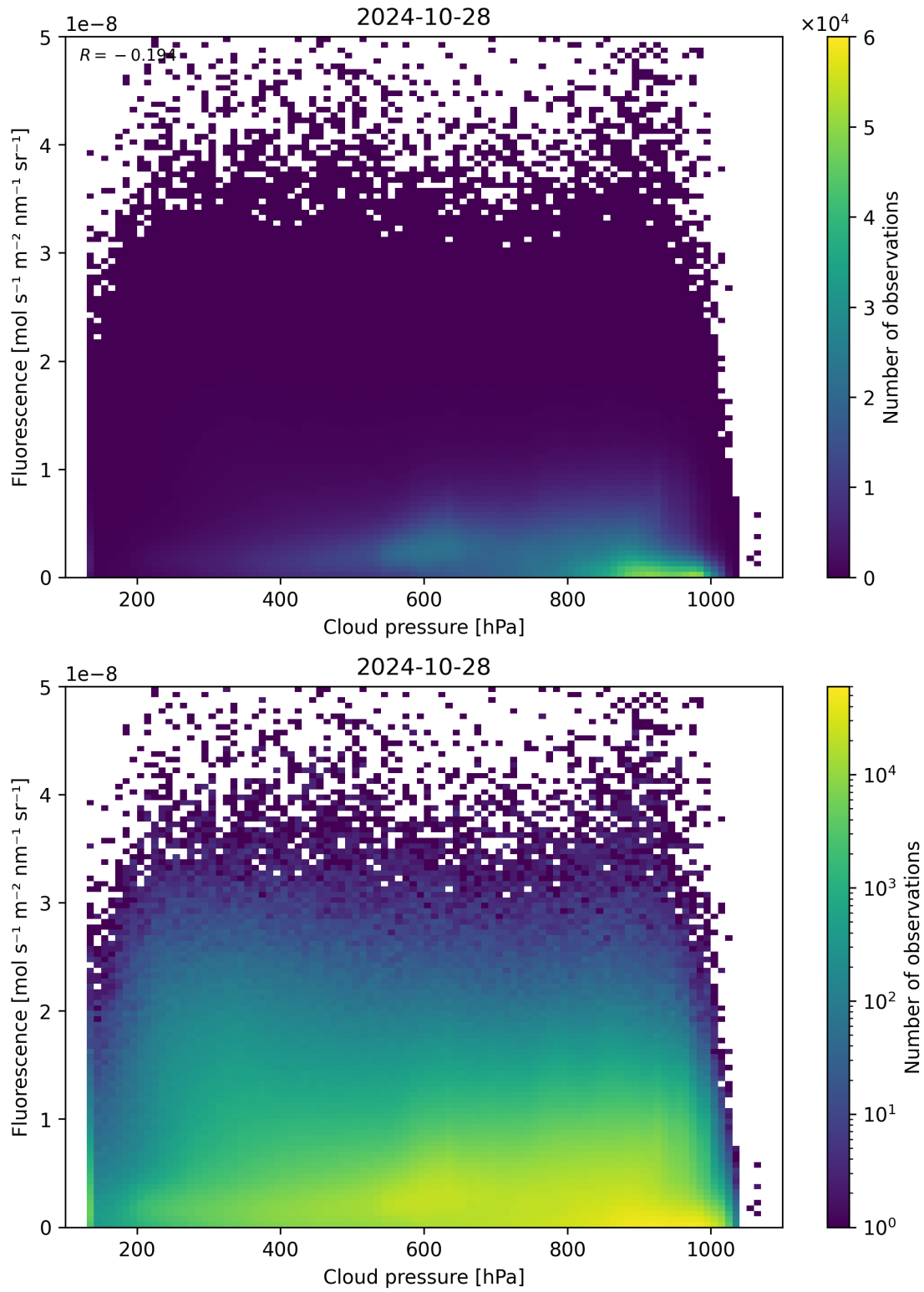
Figure 88: Scatter density plot of “Cloud pressure” against “Fluorescence” for 2024-10-27 to 2024-10-29.
