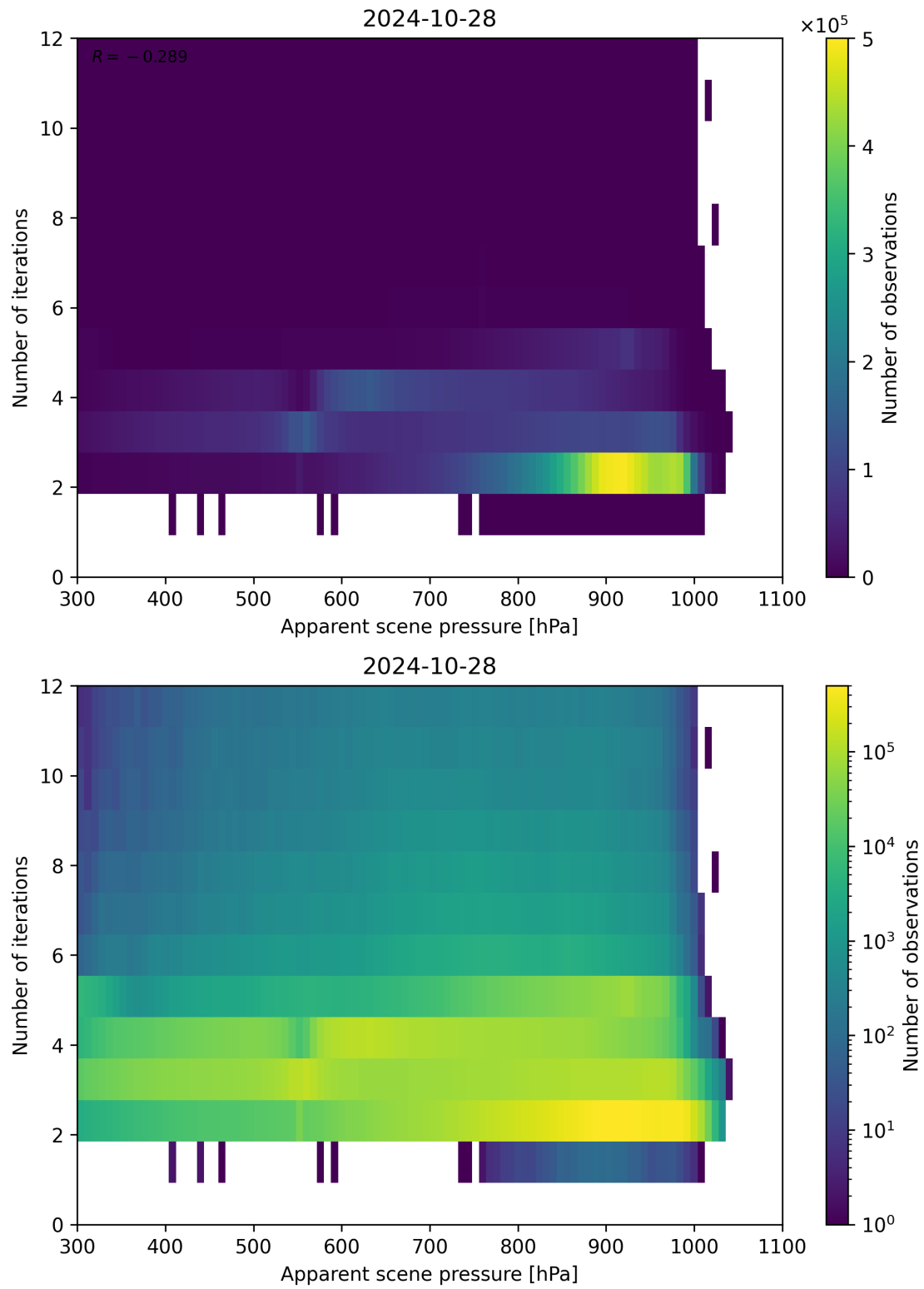
Figure 66: Scatter density plot of “Apparent scene pressure” against “Number of iterations” for 2024-10-27 to 2024-10-29.
