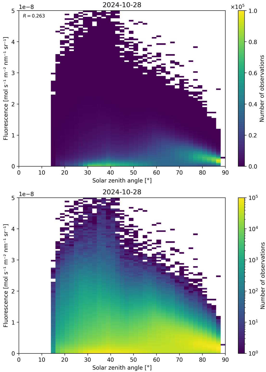
Figure 123: Scatter density plot of “Solar zenith angle” against “Fluorescence” for 2024-10-27 to 2024-10-29.
