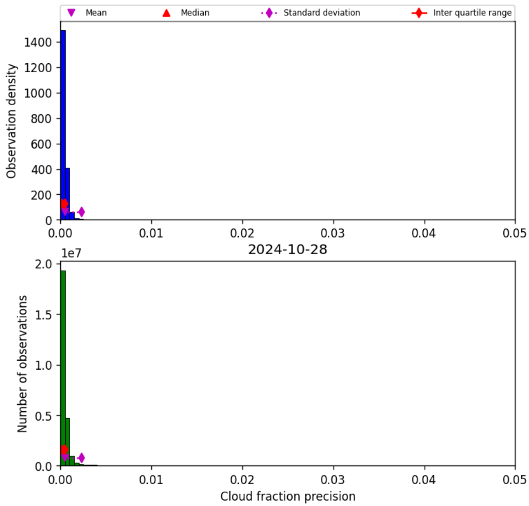
Figure 33: Histogram of “Cloud fraction precision” for 2024-10-27 to 2024-10-29
