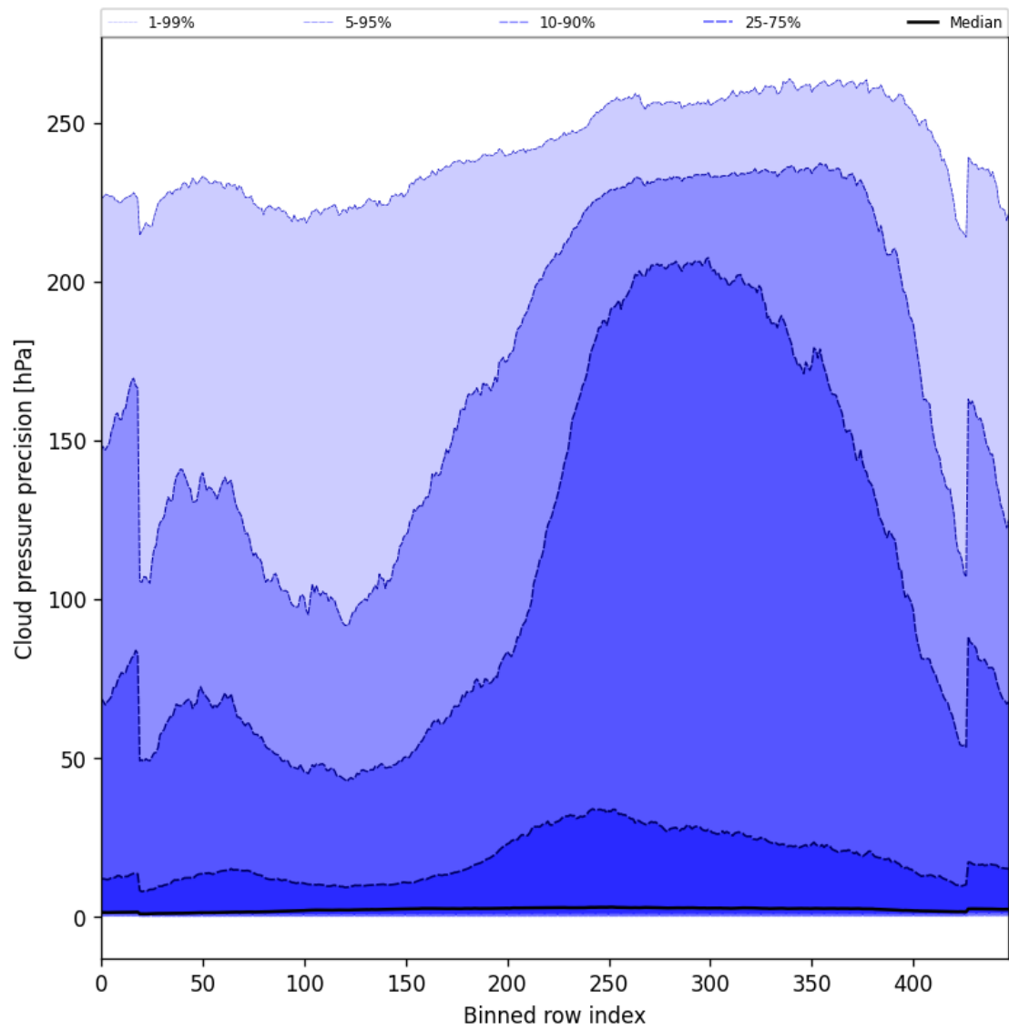
Figure 48: Along track statistics of “Cloud pressure precision” for 2024-10-27 to 2024-10-29
