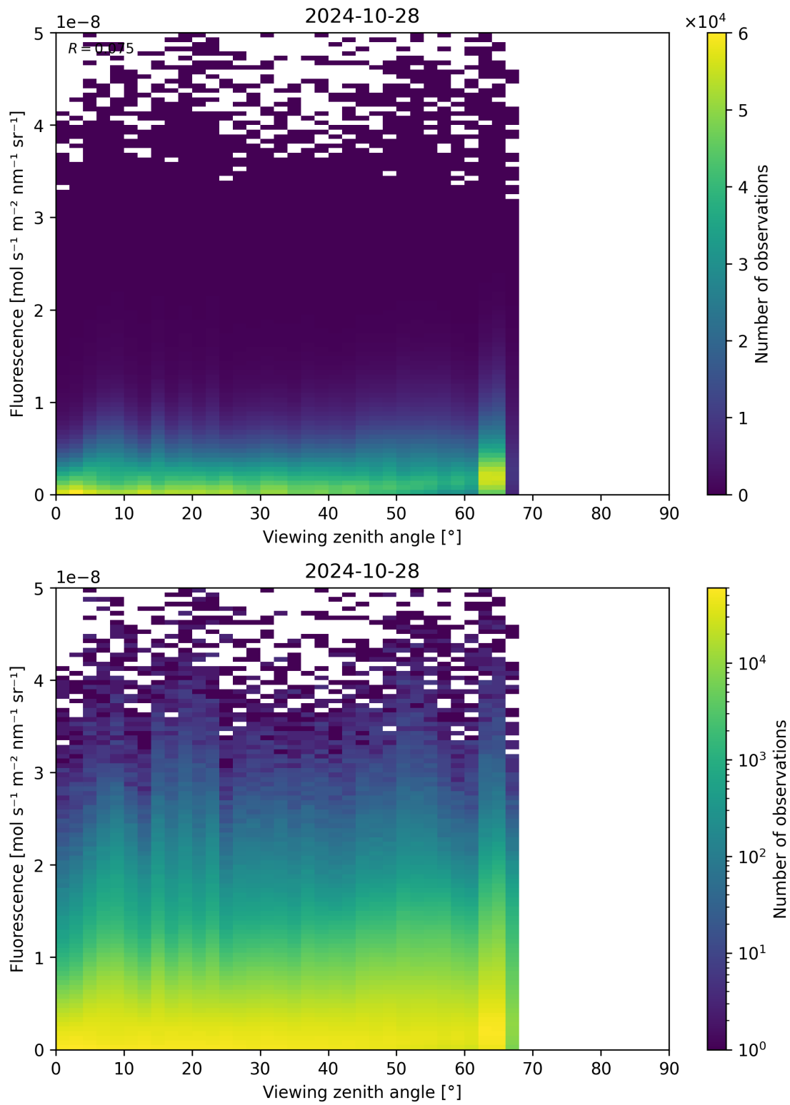
Figure 134: Scatter density plot of “Viewing zenith angle” against “Fluorescence” for 2024-10-27 to 2024-10-29.
