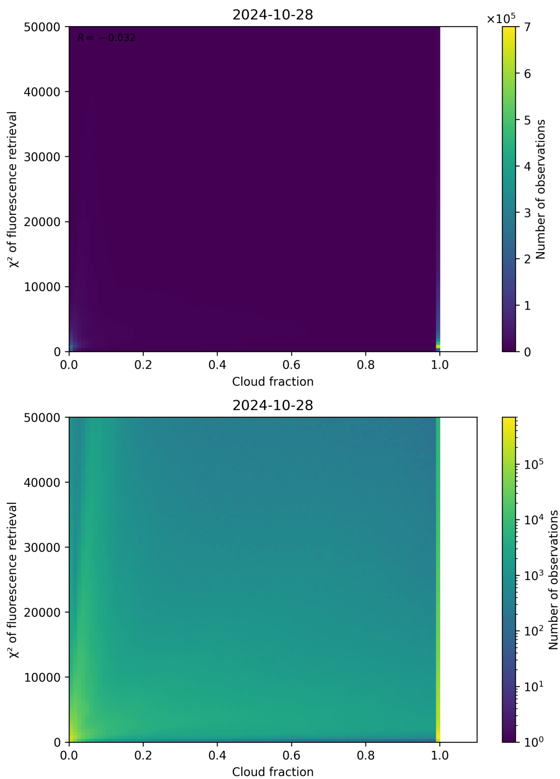
Figure 78: Scatter density plot of “Cloud fraction” against “ \chi^2 of fluorescence retrieval” for 2024-10-27 to 2024-10-29.
