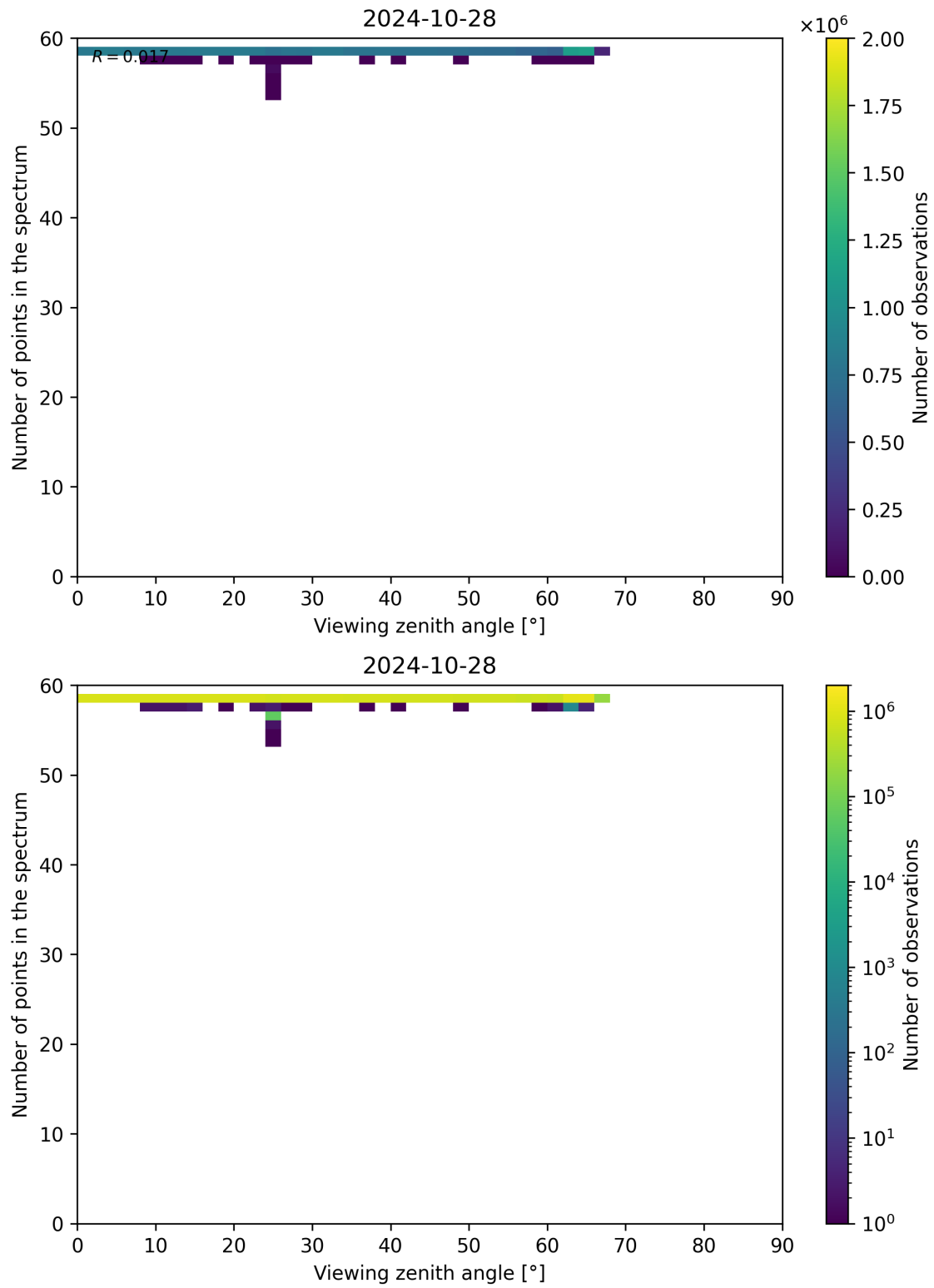
Figure 137: Scatter density plot of “Viewing zenith angle” against “Number of points in the spectrum” for 2024-10-27 to 2024-10-29.
