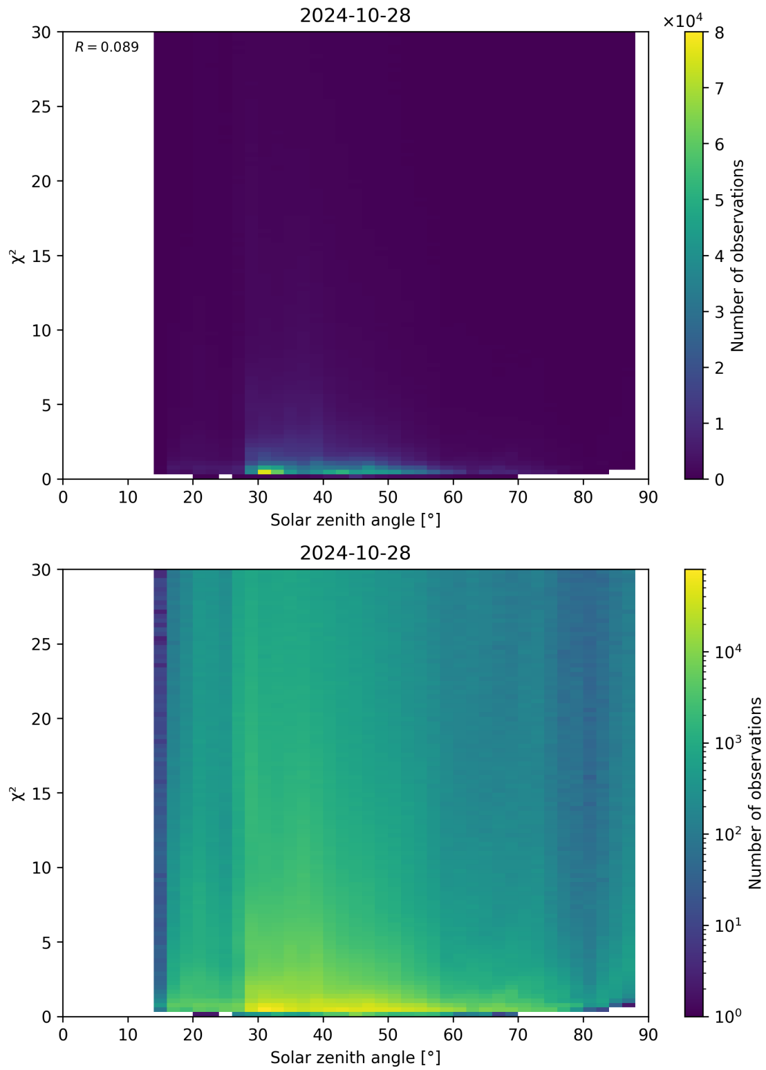
Figure 119: Scatter density plot of “Solar zenith angle” against “ \chi^2 ” for 2024-10-27 to 2024-10-29.
