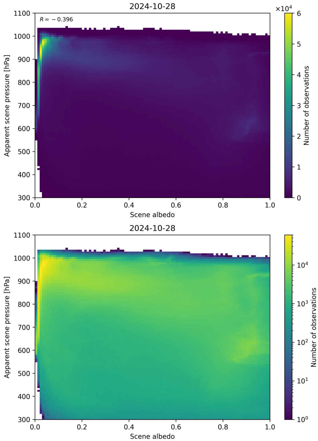
Figure 111: Scatter density plot of “Scene albedo” against “Apparent scene pressure” for 2024-10-27 to 2024-10-29.
