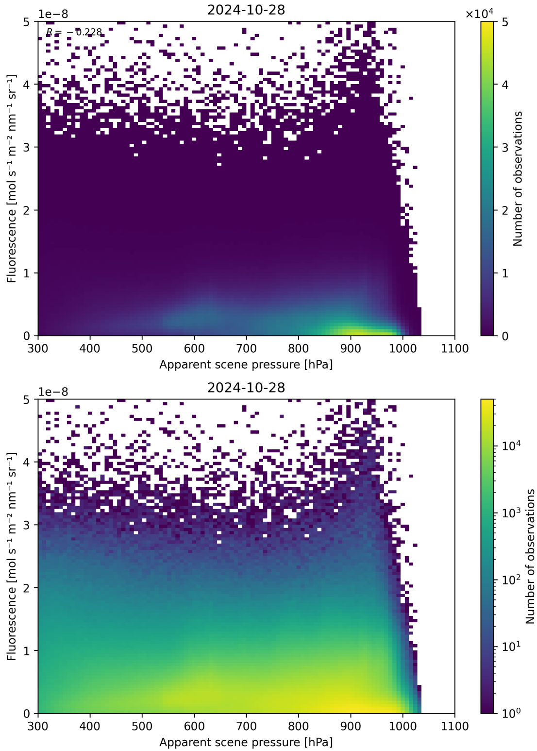
Figure 65: Scatter density plot of “Apparent scene pressure” against “Fluorescence” for 2024-10-27 to 2024-10-29.
