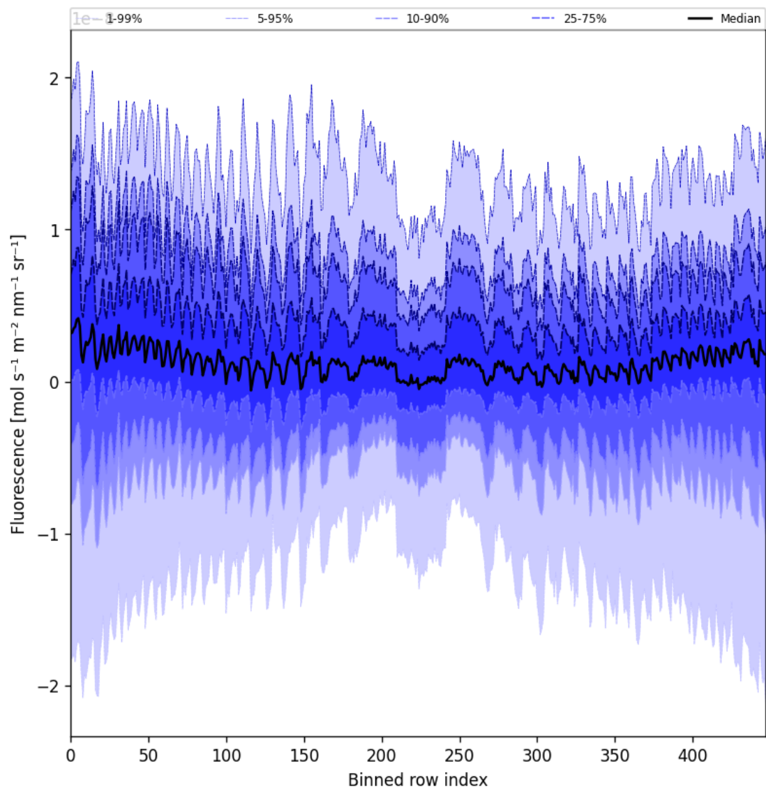
Figure 57: Along track statistics of “Fluorescence” for 2024-10-27 to 2024-10-29
