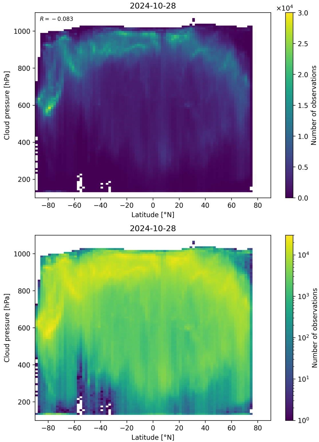
Figure 100: Scatter density plot of “Latitude” against “Cloud pressure” for 2024-10-27 to 2024-10-29.
