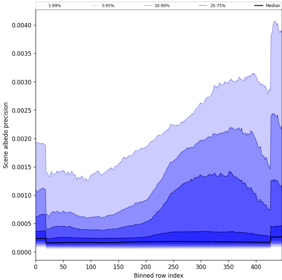
Figure 52: Along track statistics of “Scene albedo precision” for 2024-10-27 to 2024-10-29
