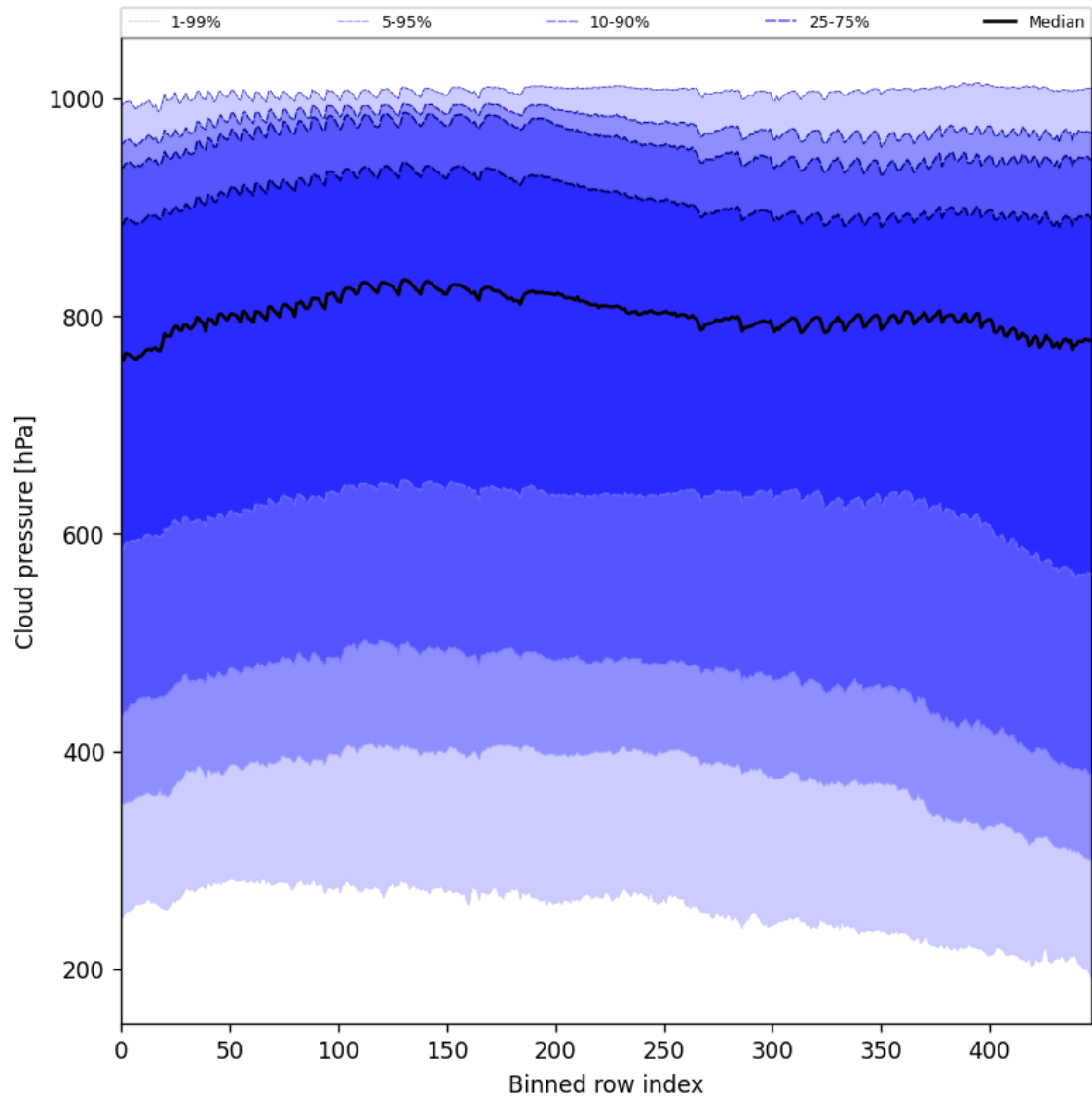
Figure 47: Along track statistics of “Cloud pressure” for 2024-10-27 to 2024-10-29
