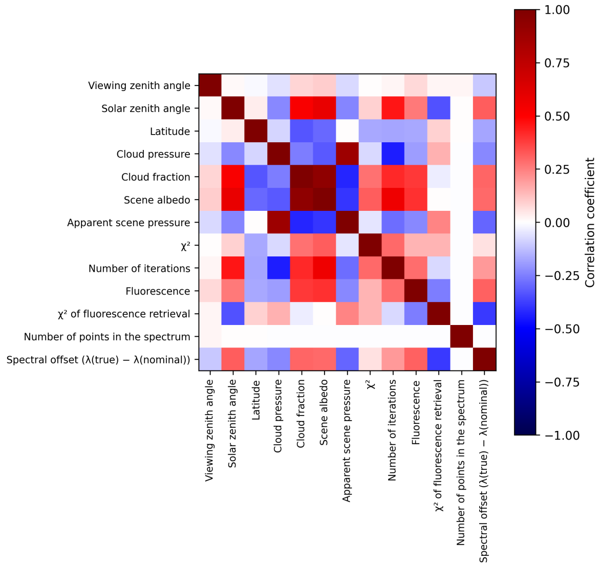
Figure 2: Map of correlation matrix for 2024-10-27 to 2024-10-29.
