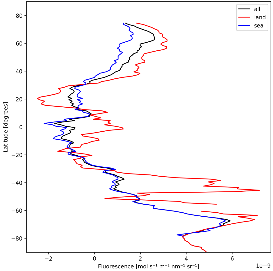
Figure 23: Zonal average of “Fluorescence” for 2024-10-27 to 2024-10-29.
