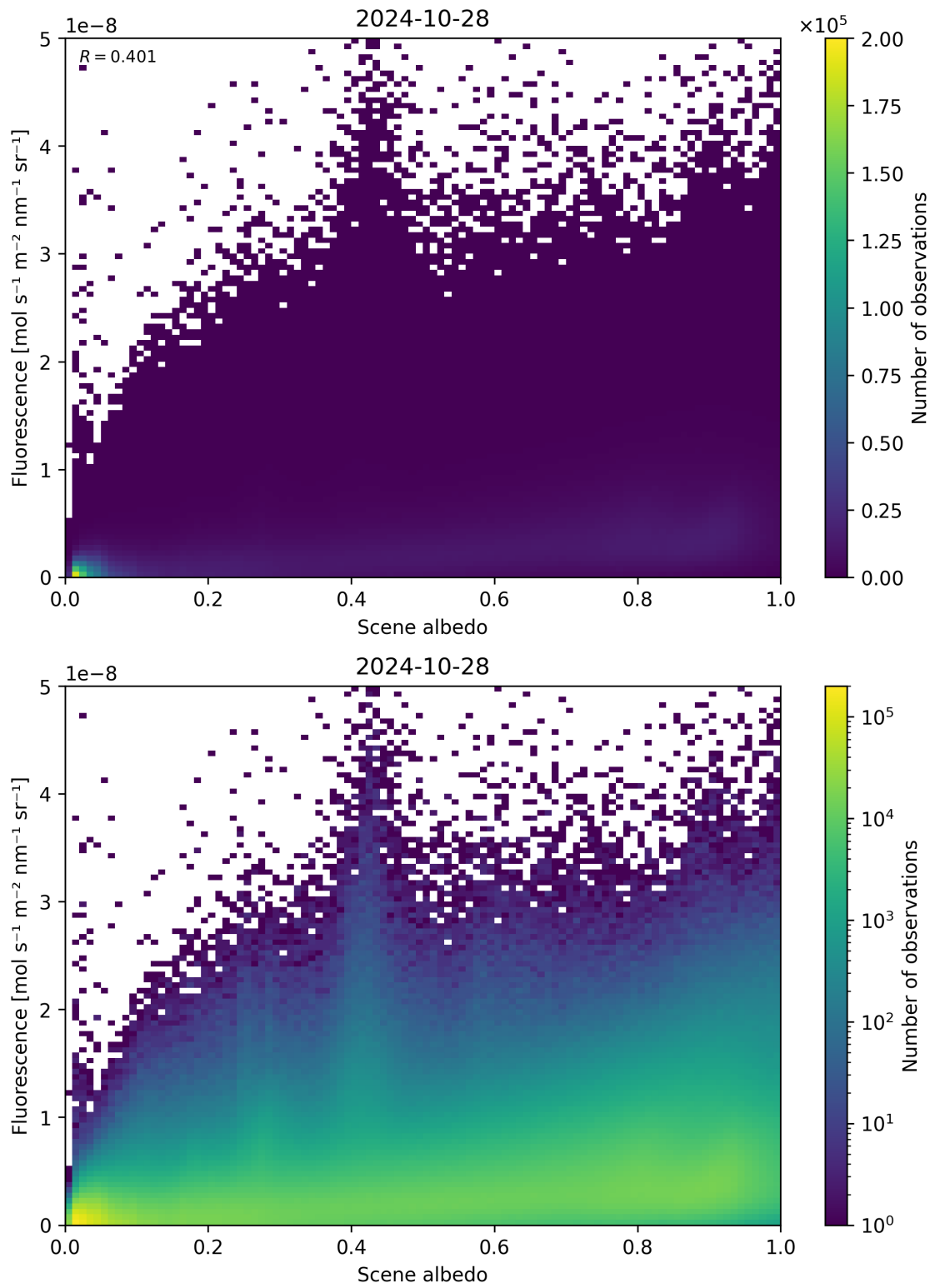
Figure 114: Scatter density plot of “Scene albedo” against “Fluorescence” for 2024-10-27 to 2024-10-29.
