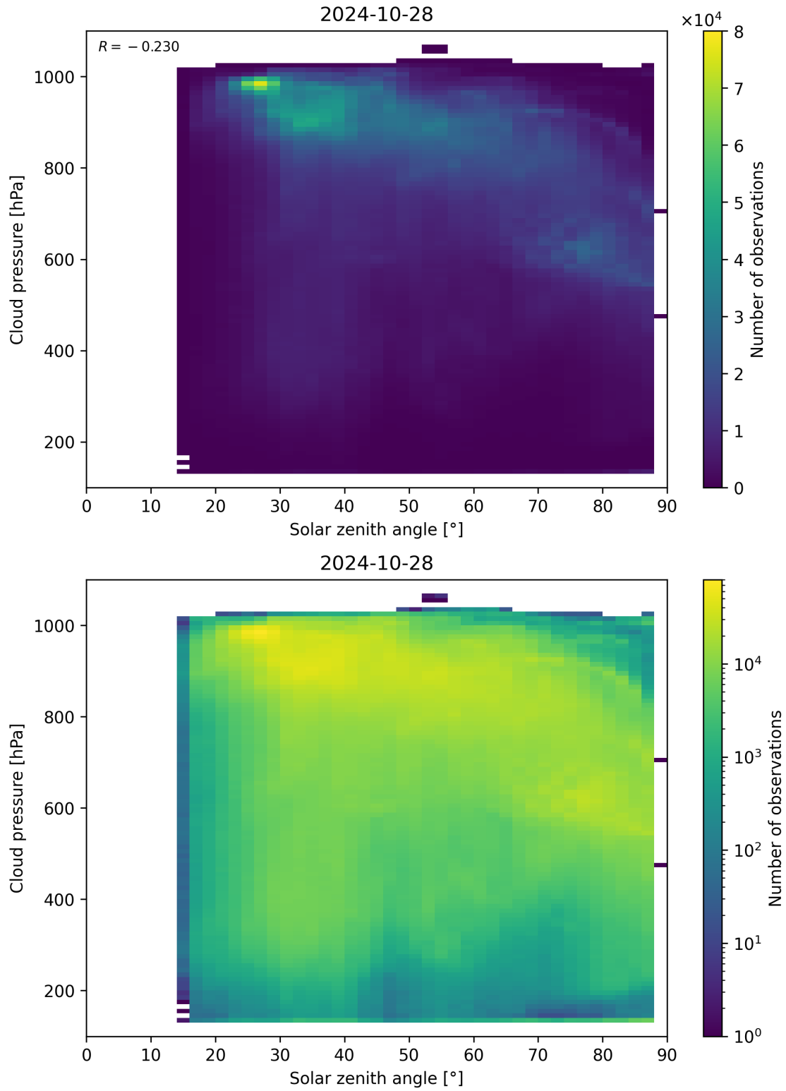
Figure 122: Scatter density plot of “Solar zenith angle” against “Cloud pressure” for 2024-10-27 to 2024-10-29.
