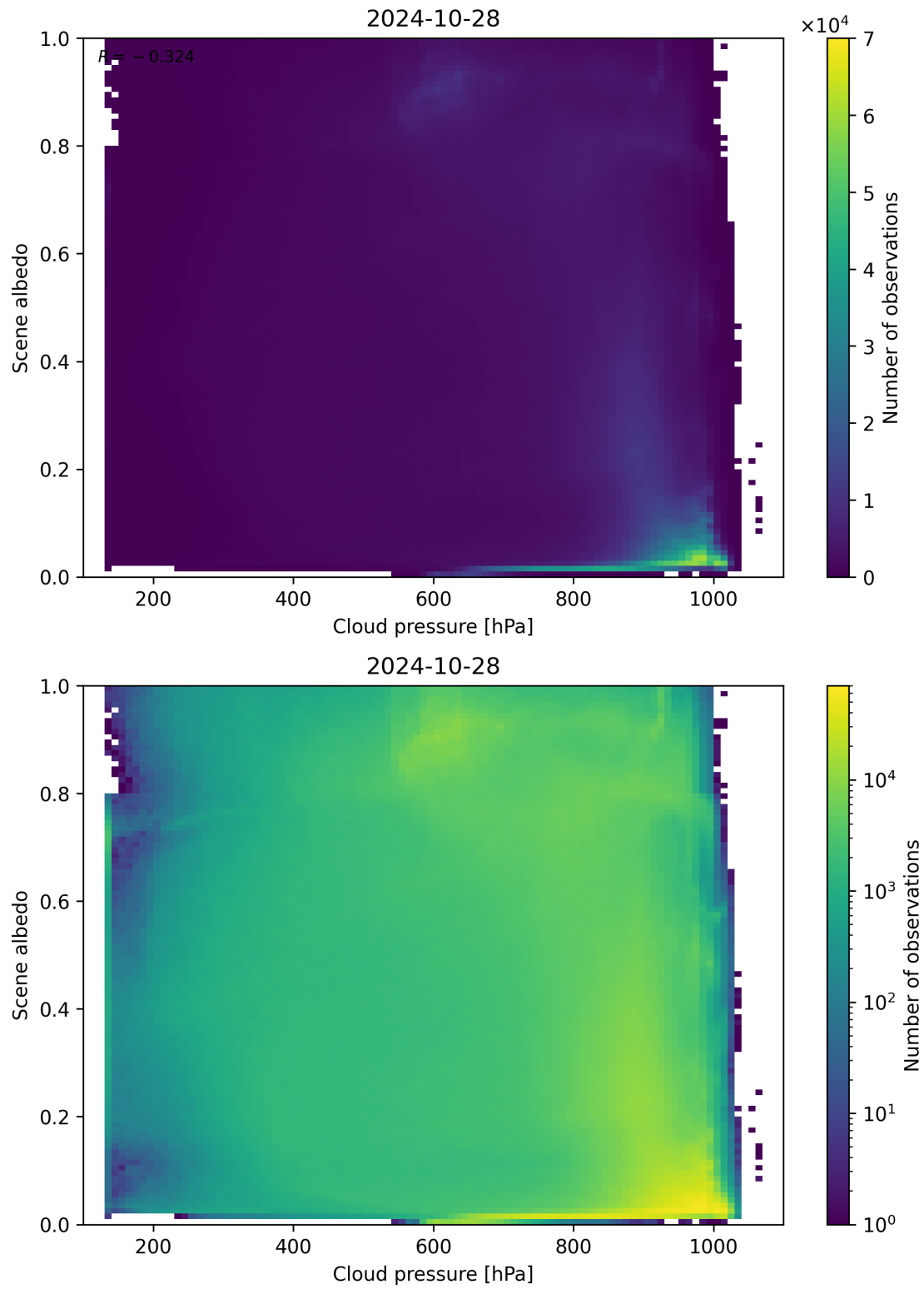
Figure 91: Scatter density plot of “Cloud pressure” against “Scene albedo” for 2024-10-27 to 2024-10-29.
