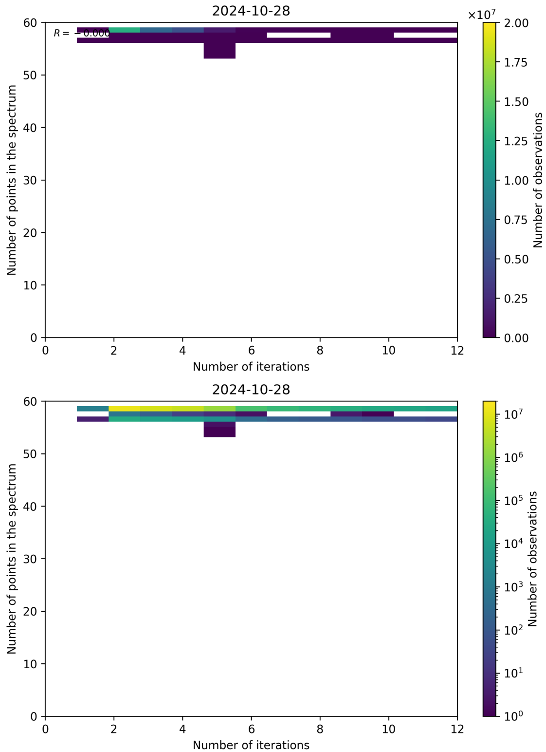
Figure 108: Scatter density plot of “Number of iterations” against “Number of points in the spectrum” for 2024-10-27 to 2024-10-29.
