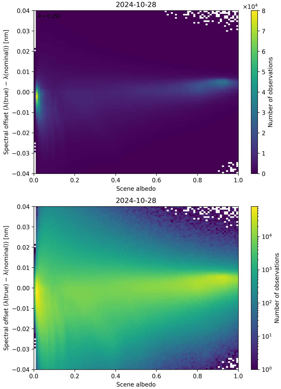
Figure 117: Scatter density plot of “Scene albedo” against “Spectral offset ( \lambda_{\text{true}} - \lambda_{\text{nominal}} )” for 2024-10-27 to 2024-10-29.
