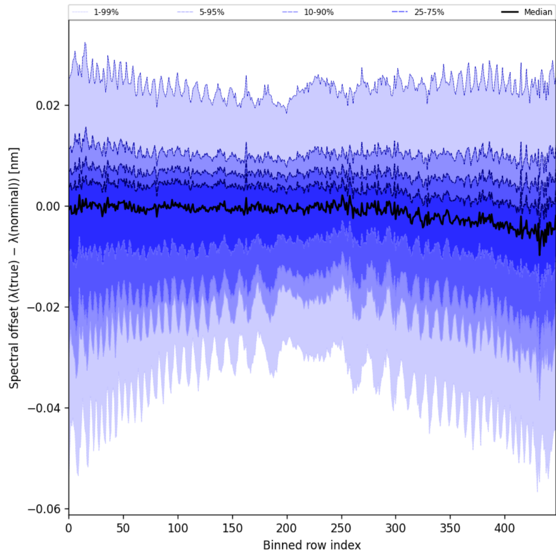
Figure 62: Along track statistics of “Spectral offset ( \lambda_{\text{true}} - \lambda_{\text{nominal}} )” for 2024-10-27 to 2024-10-29
