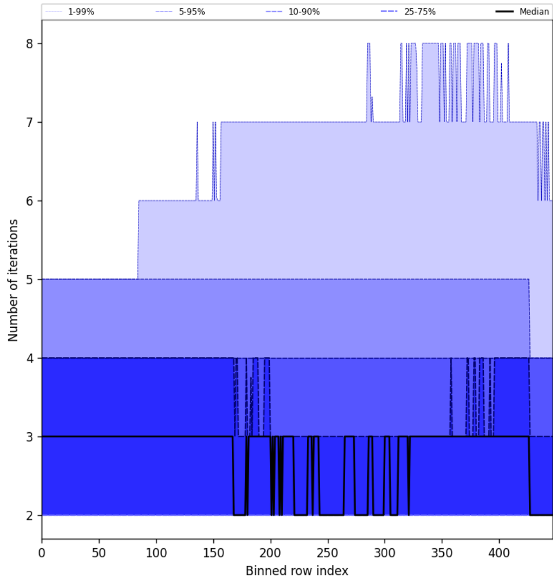
Figure 56: Along track statistics of “Number of iterations” for 2024-10-27 to 2024-10-29
