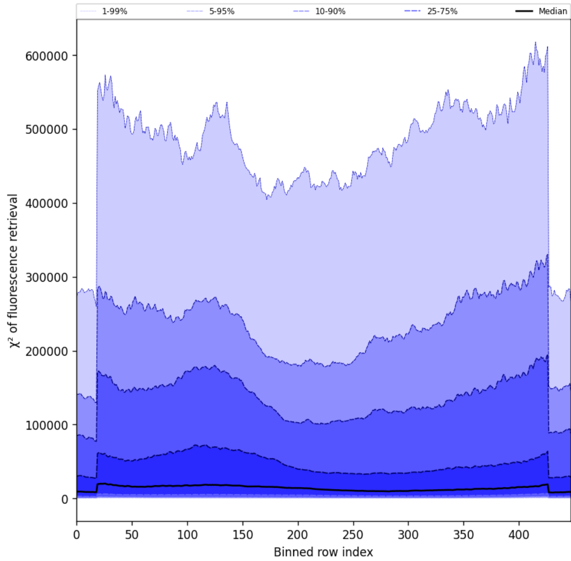
Figure 59: Along track statistics of “ \chi^2 of fluorescence retrieval” for 2024-10-27 to 2024-10-29
