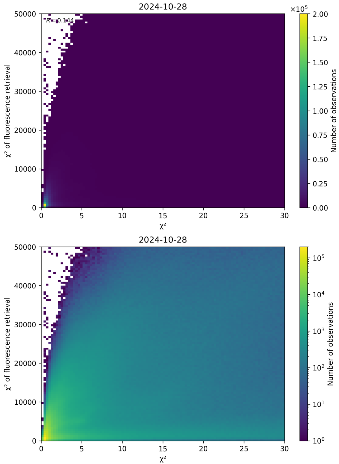
Figure 69: Scatter density plot of “ \chi^2 ” against “ \chi^2 of fluorescence retrieval” for 2024-10-27 to 2024-10-29.
