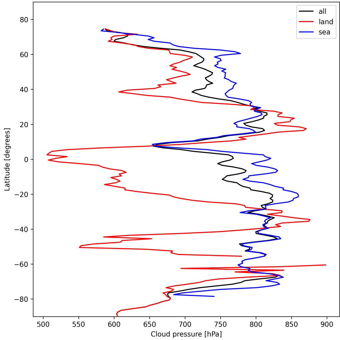
Figure 13: Zonal average of “Cloud pressure” for 2024-10-27 to 2024-10-29.
