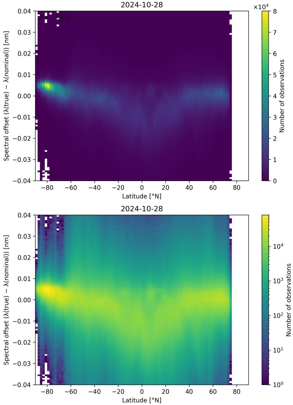
Figure 105: Scatter density plot of “Latitude” against “Spectral offset ( \lambda_{\text{true}} - \lambda_{\text{nominal}} )” for 2024-10-27 to 2024-10-29.
