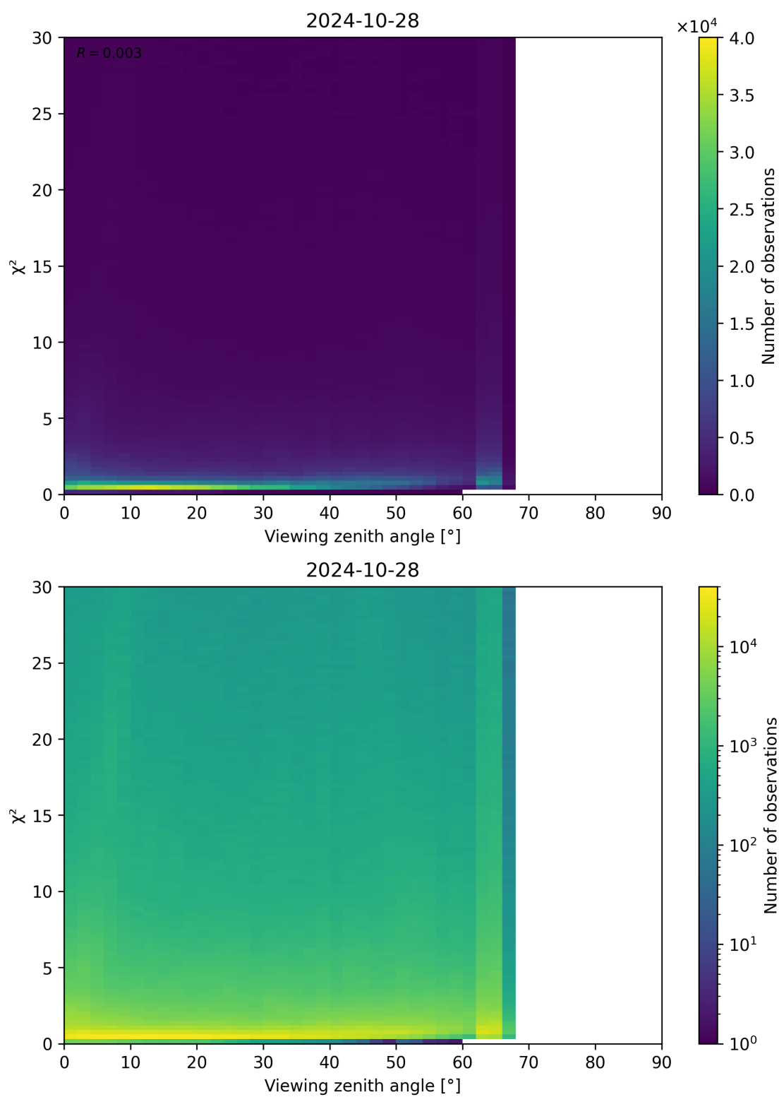
Figure 130: Scatter density plot of “Viewing zenith angle” against “ \chi^2 ” for 2024-10-27 to 2024-10-29.
