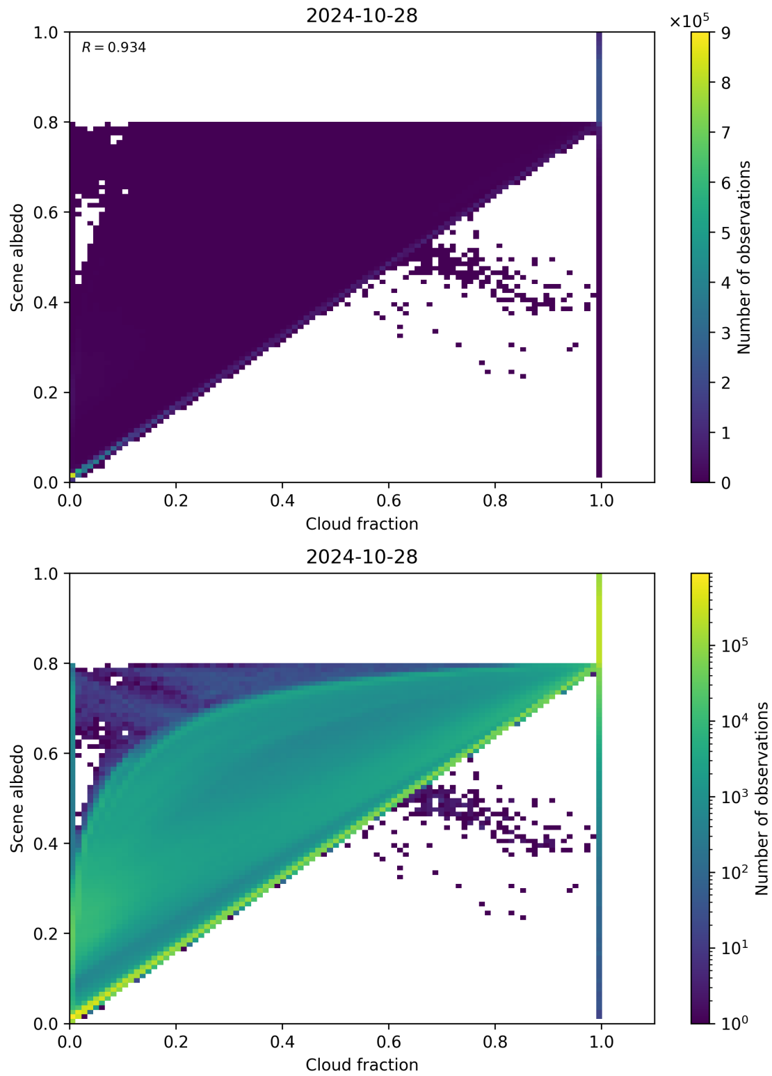
Figure 82: Scatter density plot of “Cloud fraction” against “Scene albedo” for 2024-10-27 to 2024-10-29.
