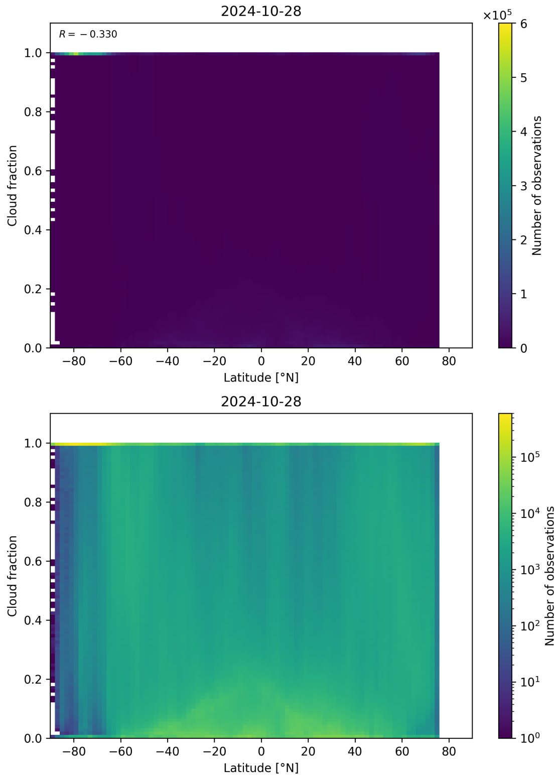
Figure 99: Scatter density plot of “Latitude” against “Cloud fraction” for 2024-10-27 to 2024-10-29.
