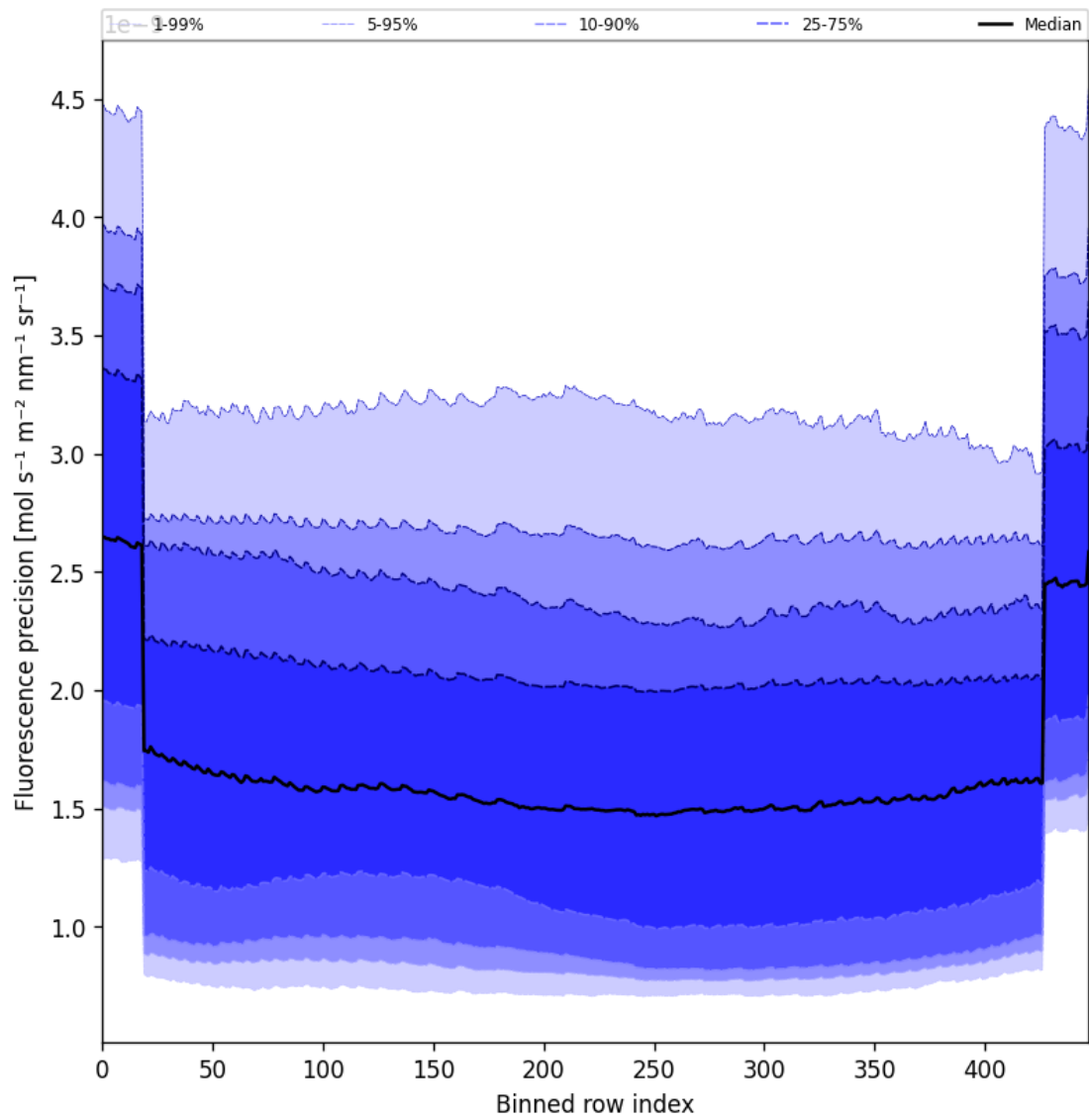
Figure 58: Along track statistics of “Fluorescence precision” for 2024-10-27 to 2024-10-29
