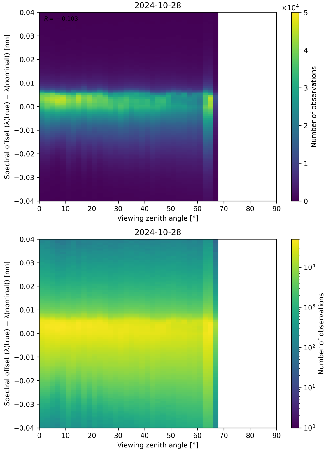
Figure 140: Scatter density plot of “Viewing zenith angle” against “Spectral offset ( \lambda_{\text{true}} - \lambda_{\text{nominal}} )” for 2024-10-27 to 2024-10-29.
