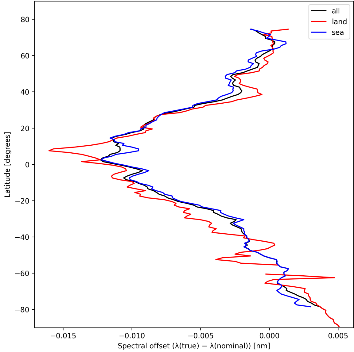
Figure 28: Zonal average of “Spectral offset ( \lambda_{\text{true}} - \lambda_{\text{nominal}} )” for 2024-10-27 to 2024-10-29.
