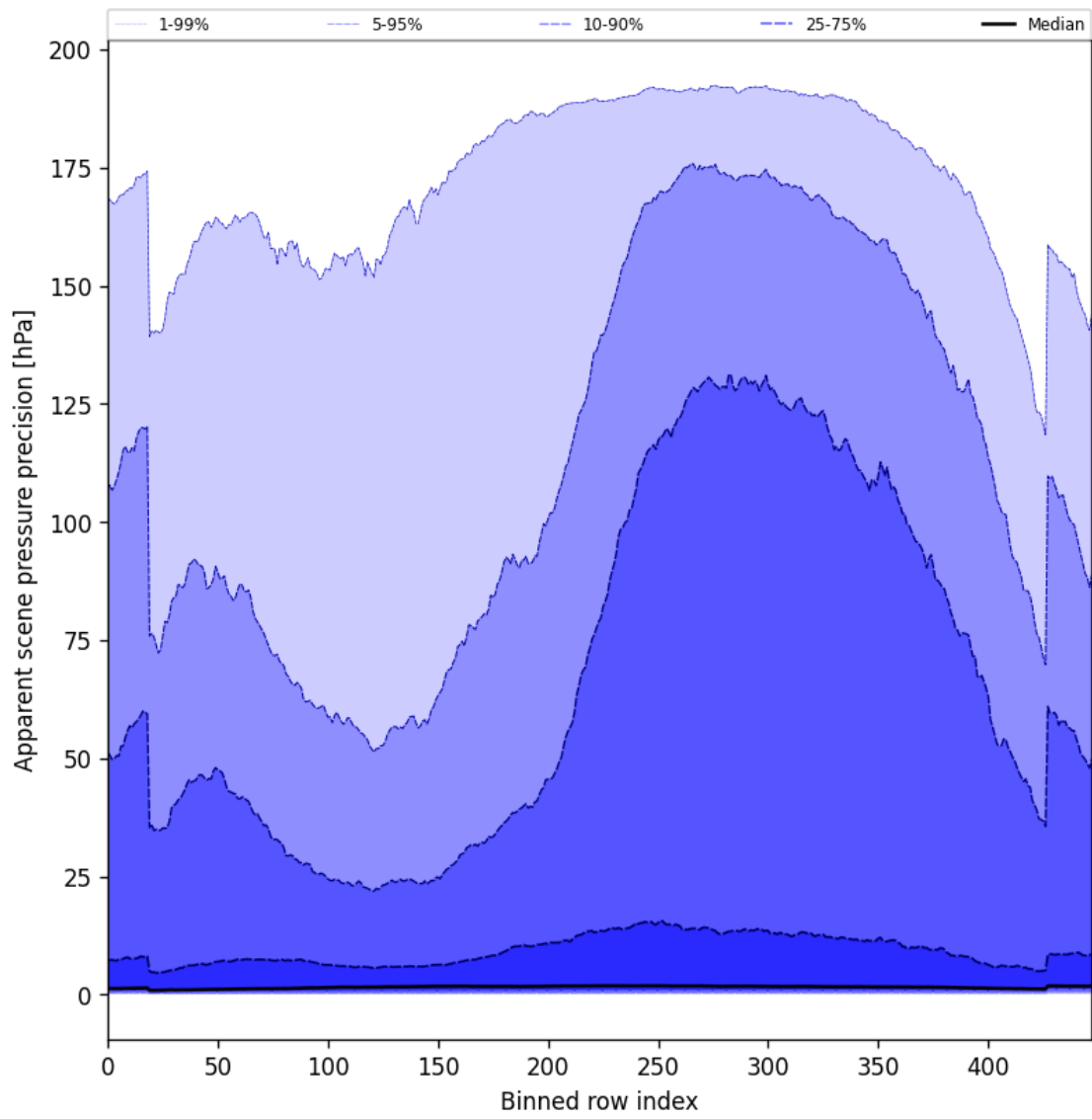
Figure 54: Along track statistics of “Apparent scene pressure precision” for 2024-10-27 to 2024-10-29
