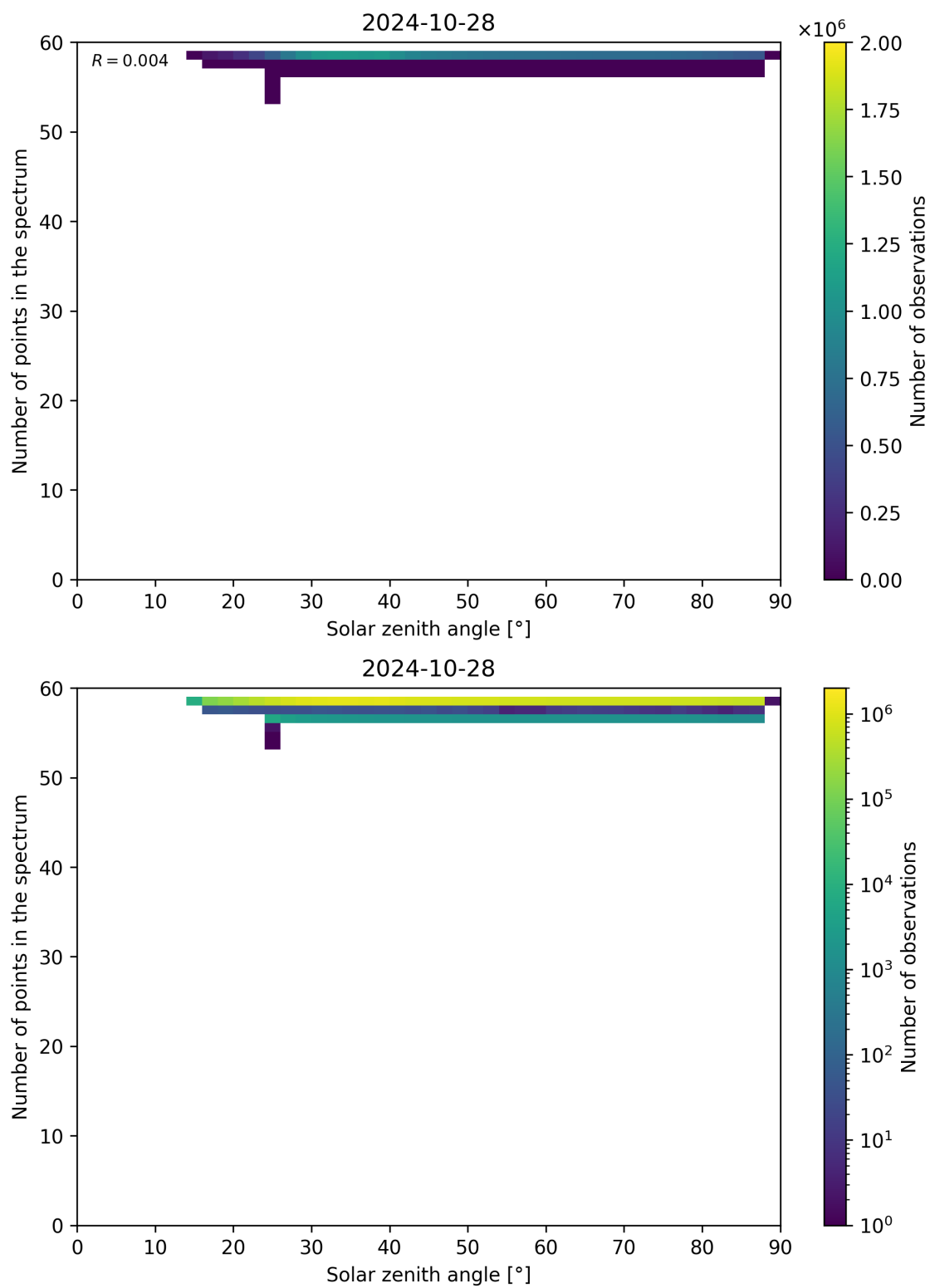
Figure 126: Scatter density plot of “Solar zenith angle” against “Number of points in the spectrum” for 2024-10-27 to 2024-10-29.
