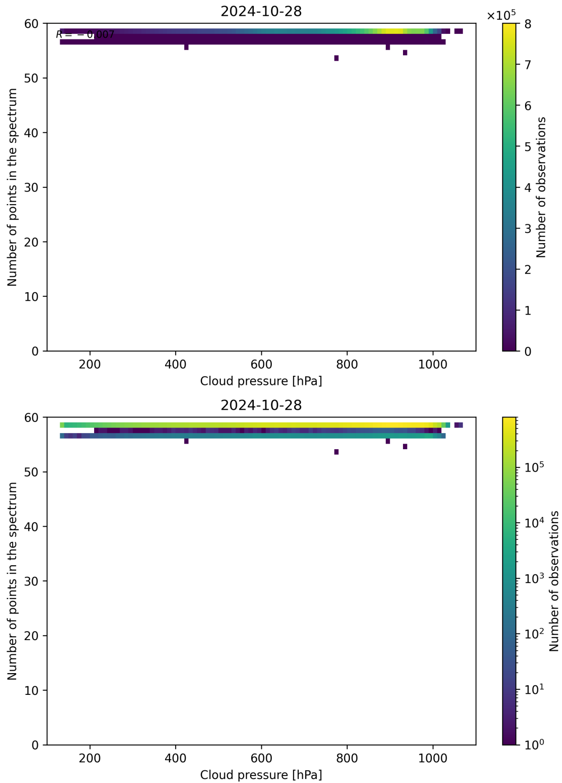
Figure 90: Scatter density plot of “Cloud pressure” against “Number of points in the spectrum” for 2024-10-27 to 2024-10-29.
