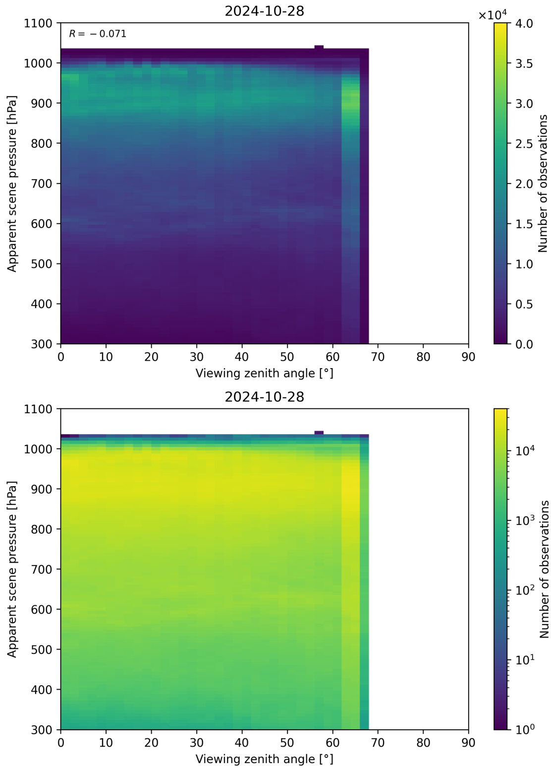
Figure 129: Scatter density plot of “Viewing zenith angle” against “Apparent scene pressure” for 2024-10-27 to 2024-10-29.
