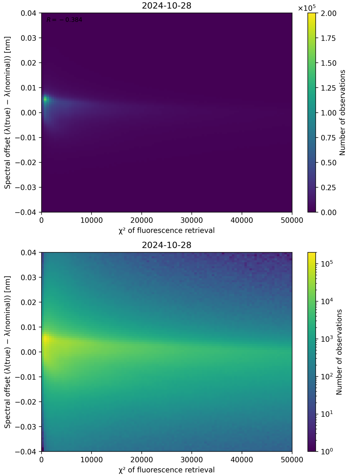
Figure 72: Scatter density plot of “ \chi^2 of fluorescence retrieval” against “Spectral offset ( \lambda_{\text{true}} - \lambda_{\text{nominal}} )” for 2024-10-27 to 2024-10-29.
