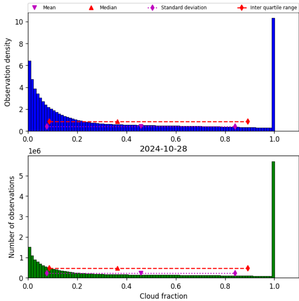
Figure 32: Histogram of “Cloud fraction” for 2024-10-27 to 2024-10-29
