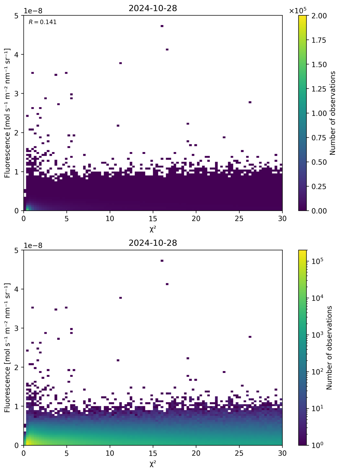
Figure 70: Scatter density plot of “ \chi^2 ” against “Fluorescence” for 2024-10-27 to 2024-10-29.
