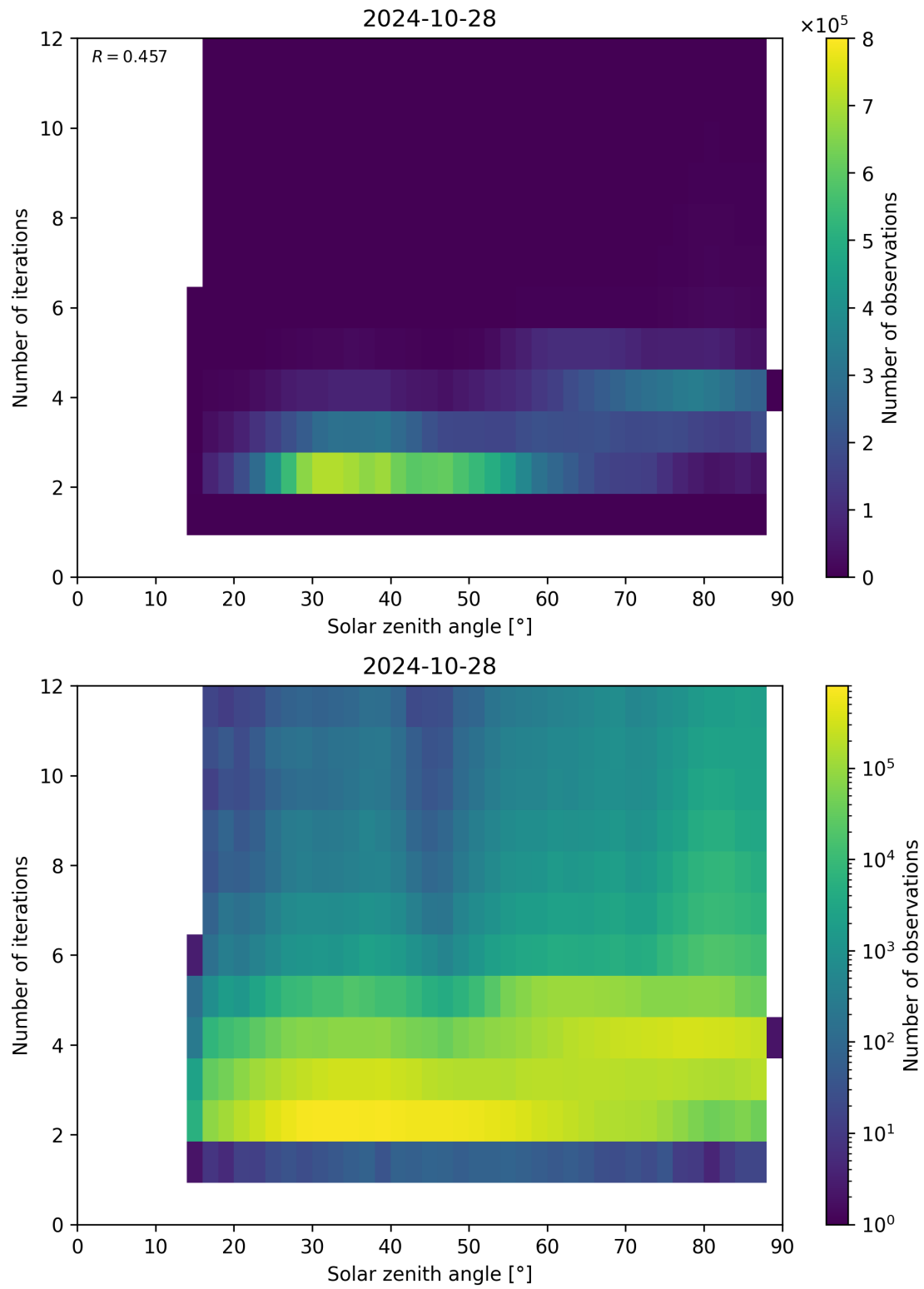
Figure 125: Scatter density plot of “Solar zenith angle” against “Number of iterations” for 2024-10-27 to 2024-10-29.
