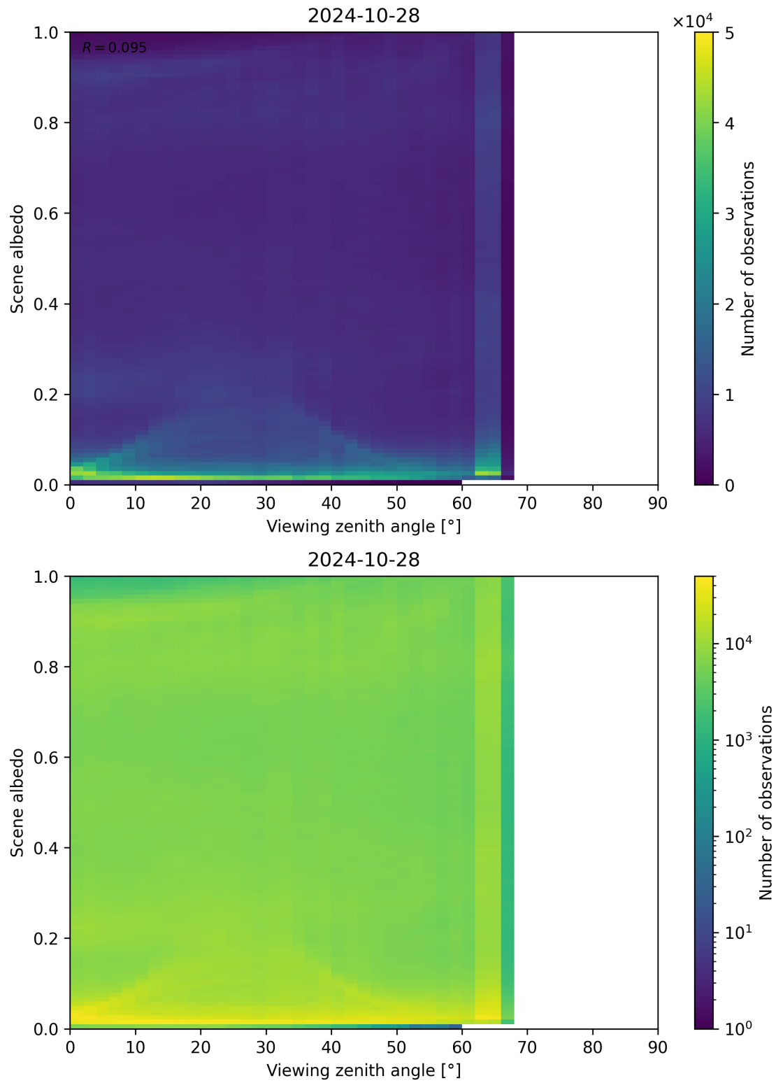
Figure 138: Scatter density plot of “Viewing zenith angle” against “Scene albedo” for 2024-10-27 to 2024-10-29.
