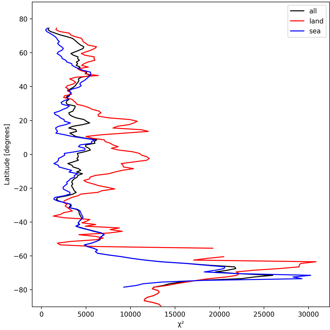
Figure 21: Zonal average of “ \chi^2 ” for 2024-10-27 to 2024-10-29.
