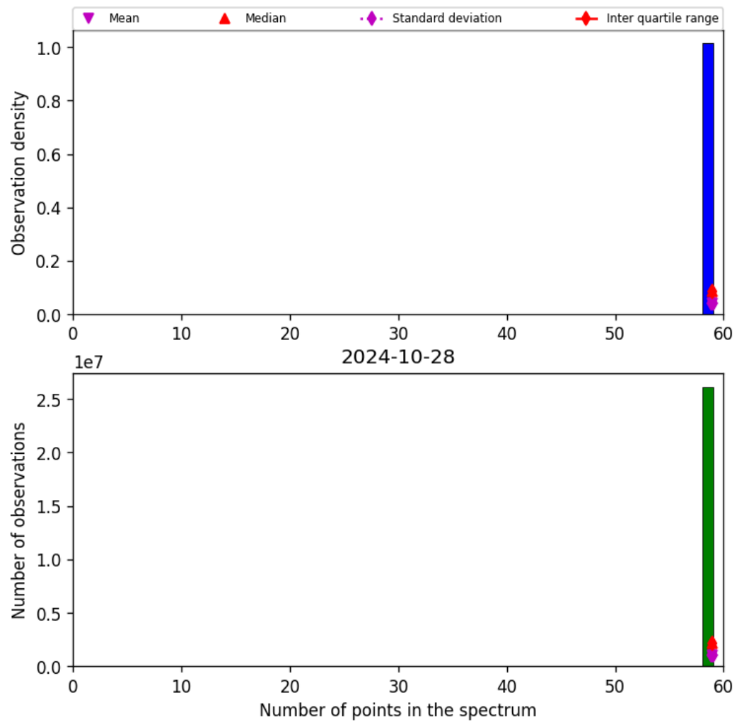
Figure 44: Histogram of “Number of points in the spectrum” for 2024-10-27 to 2024-10-29
