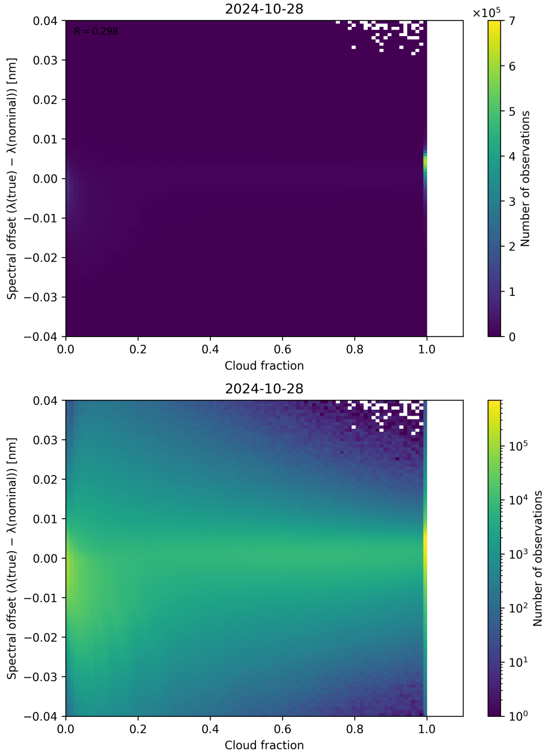
Figure 83: Scatter density plot of “Cloud fraction” against “Spectral offset ( \lambda_{\text{true}} - \lambda_{\text{nominal}} )” for 2024-10-27 to 2024-10-29.
