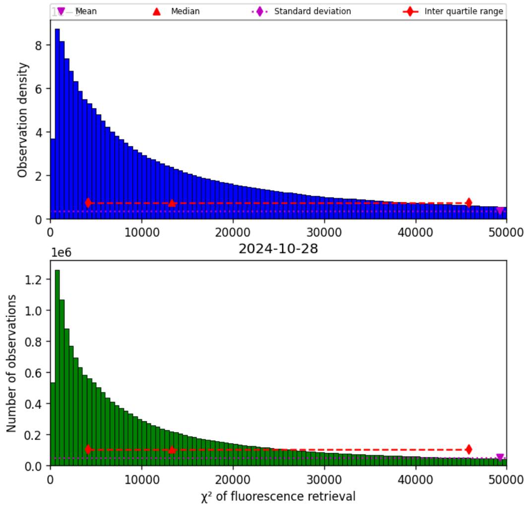
Figure 42: Histogram of “ \chi^2 of fluorescence retrieval” for 2024-10-27 to 2024-10-29
