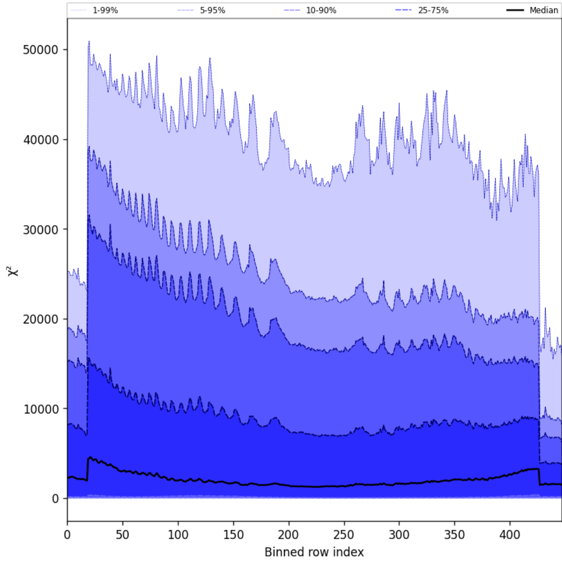
Figure 55: Along track statistics of “ \chi^2 ” for 2024-10-27 to 2024-10-29
