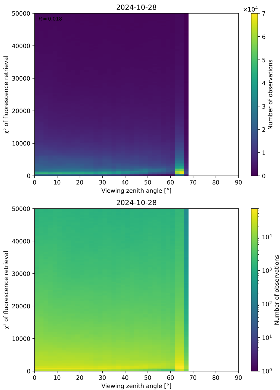
Figure 131: Scatter density plot of “Viewing zenith angle” against “ \chi^2 of fluorescence retrieval” for 2024-10-27 to 2024-10-29.
