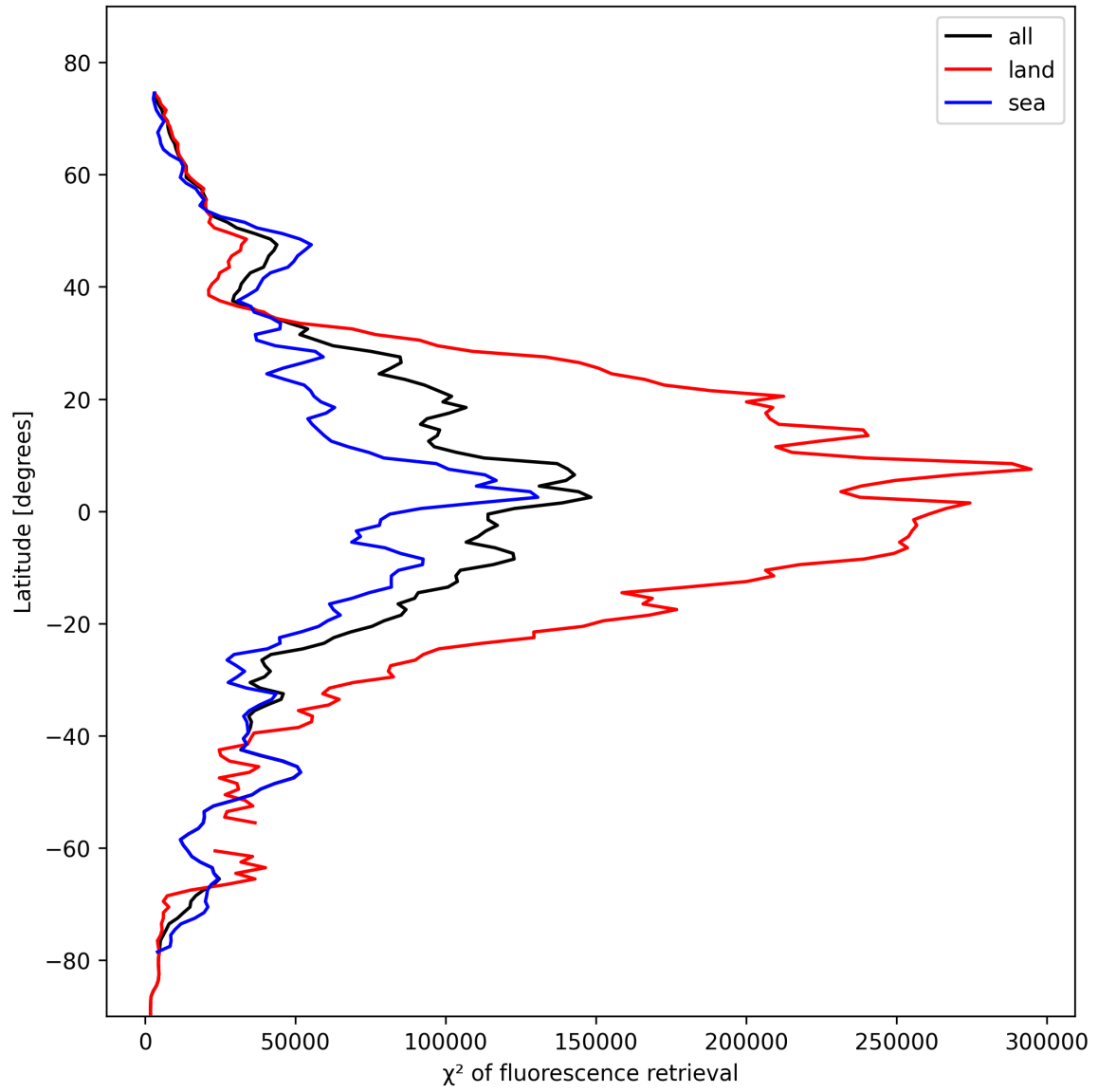
Figure 25: Zonal average of “ \chi^2 of fluorescence retrieval” for 2024-10-27 to 2024-10-29.
