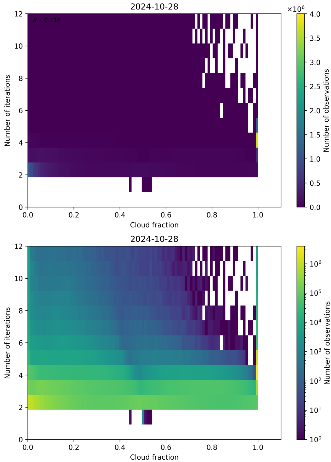
Figure 80: Scatter density plot of “Cloud fraction” against “Number of iterations” for 2024-10-27 to 2024-10-29.
