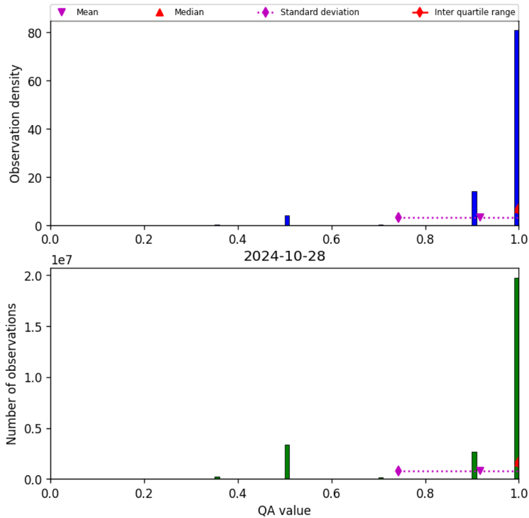
Figure 29: Histogram of “QA value” for 2024-10-27 to 2024-10-29
