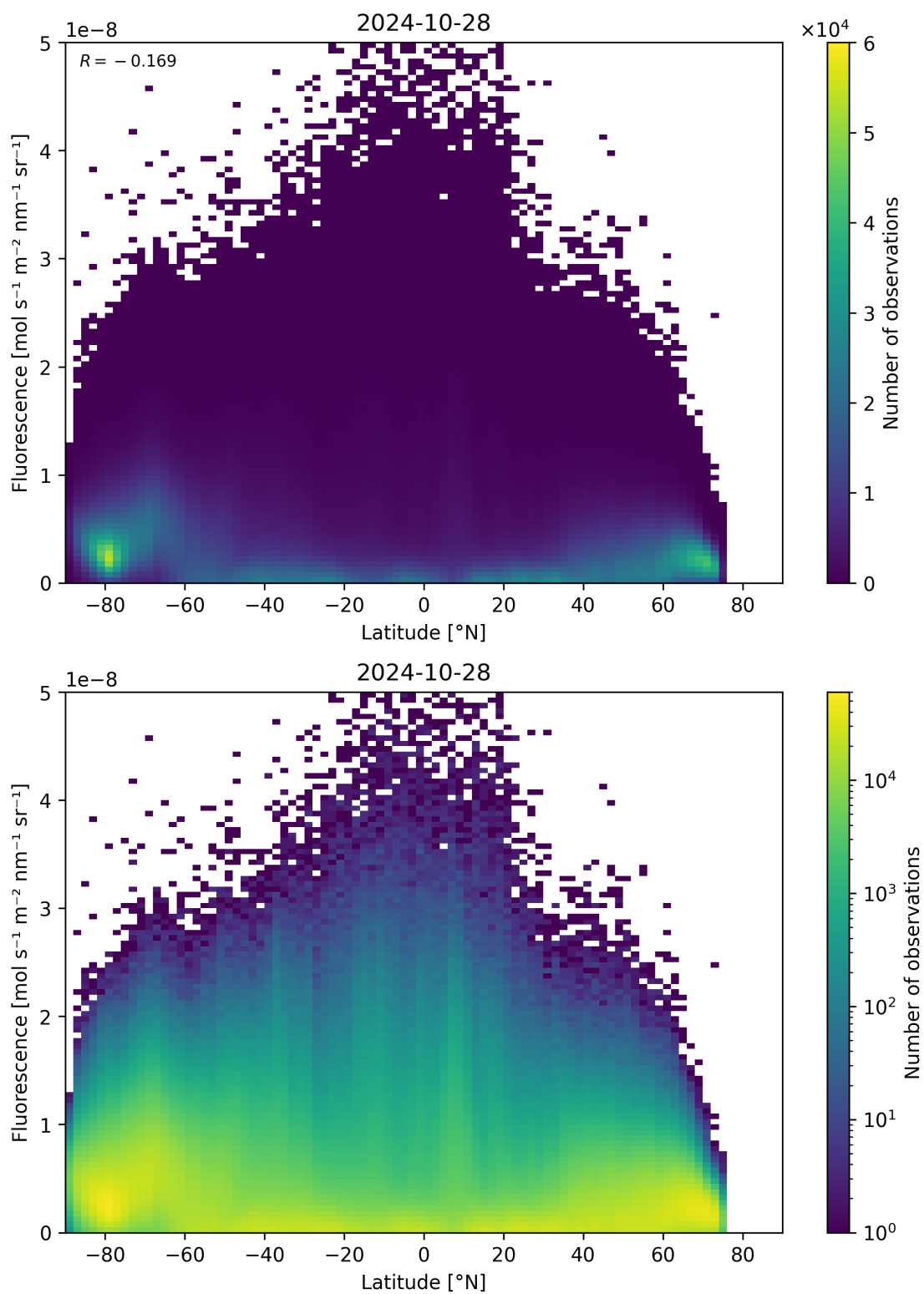
Figure 101: Scatter density plot of “Latitude” against “Fluorescence” for 2024-10-27 to 2024-10-29.
