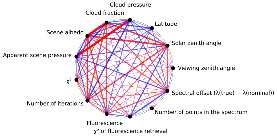
Figure 1: Map of correlation graph for 2024-10-27 to 2024-10-29.
