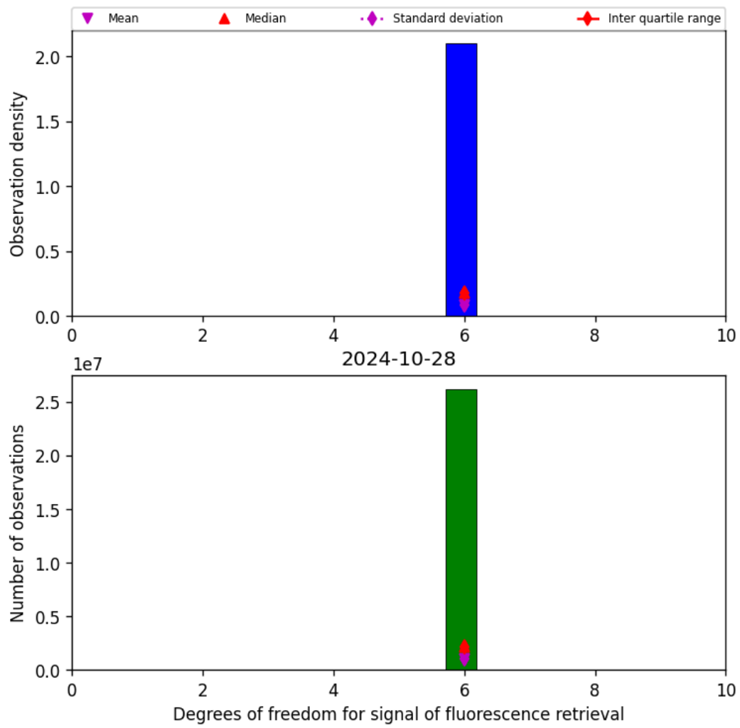
Figure 43: Histogram of "Degrees of freedom for signal of fluorescence retrieval" for 2024-10-27 to 2024-10-29
