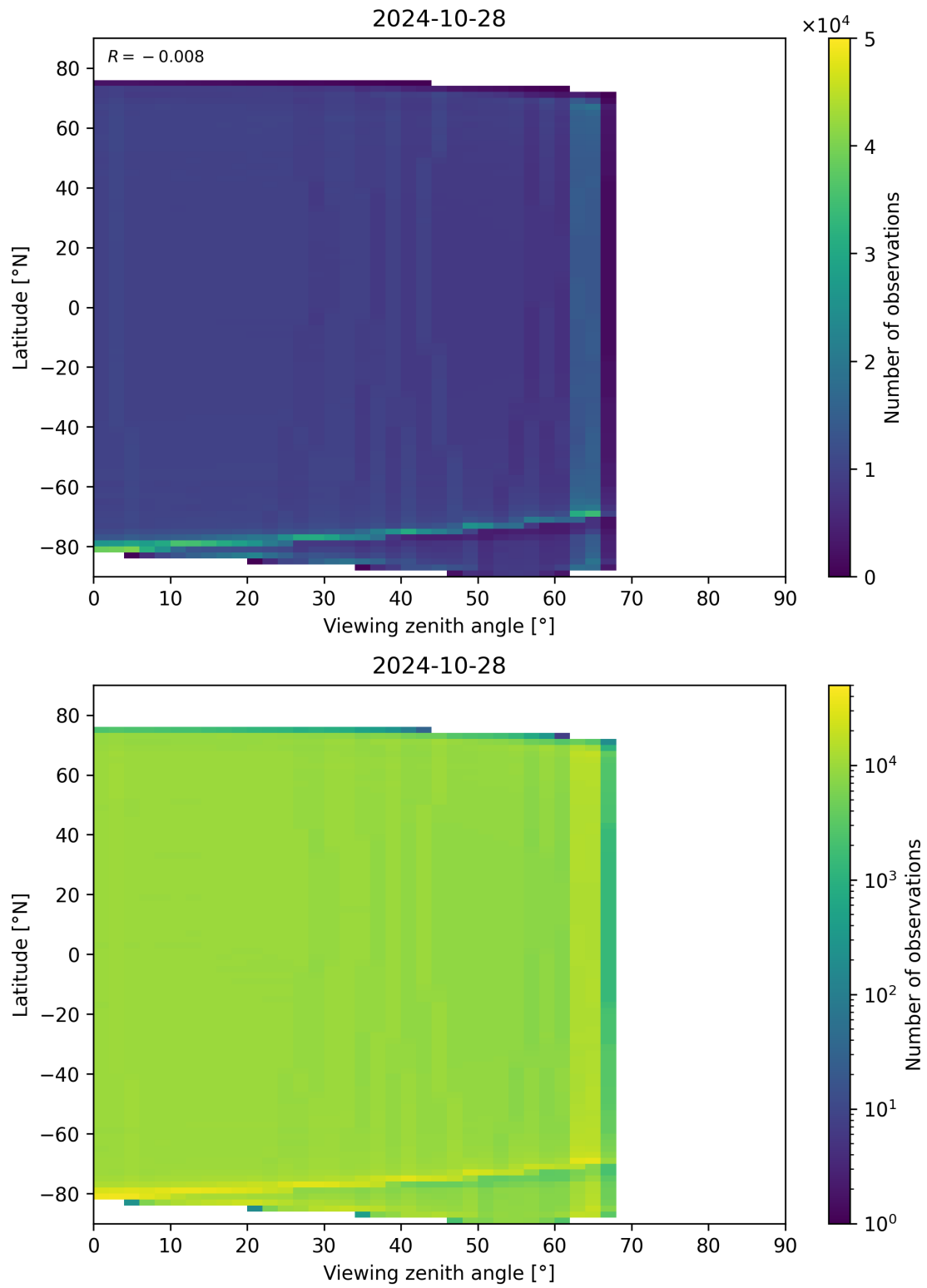
Figure 135: Scatter density plot of “Viewing zenith angle” against “Latitude” for 2024-10-27 to 2024-10-29.
