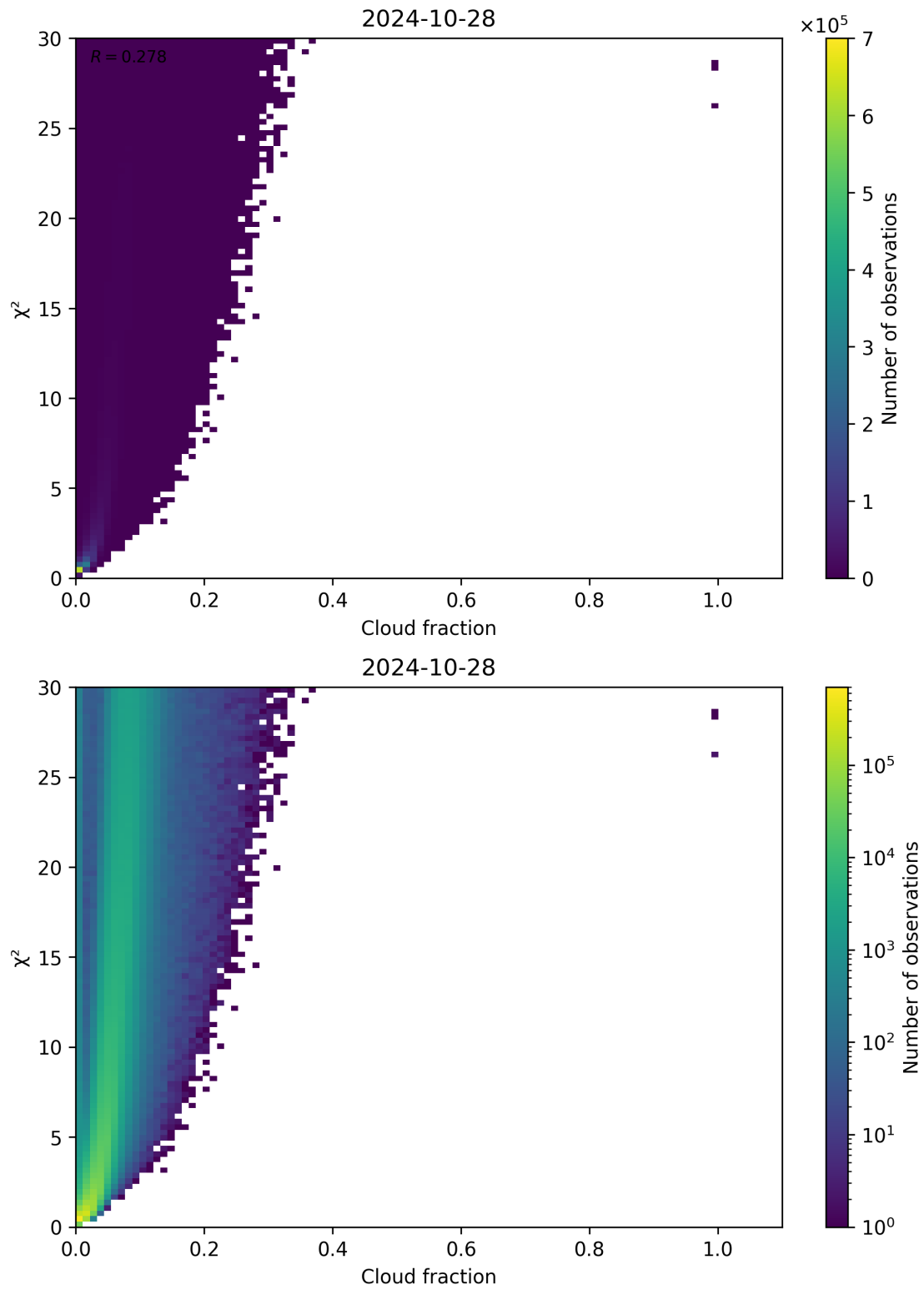
Figure 77: Scatter density plot of “Cloud fraction” against “ \chi^2 ” for 2024-10-27 to 2024-10-29.
