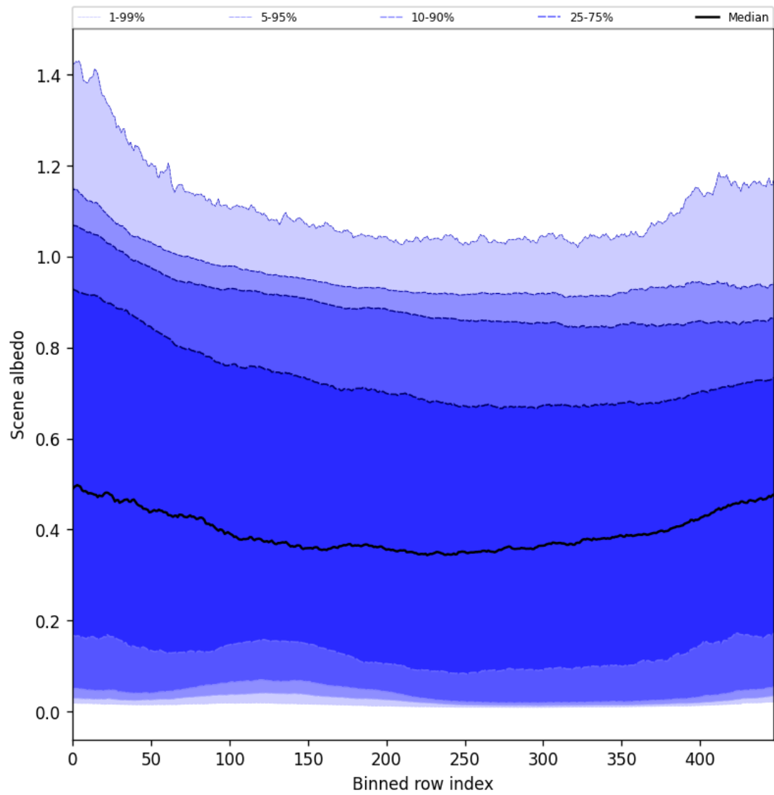
Figure 51: Along track statistics of “Scene albedo” for 2024-10-27 to 2024-10-29
