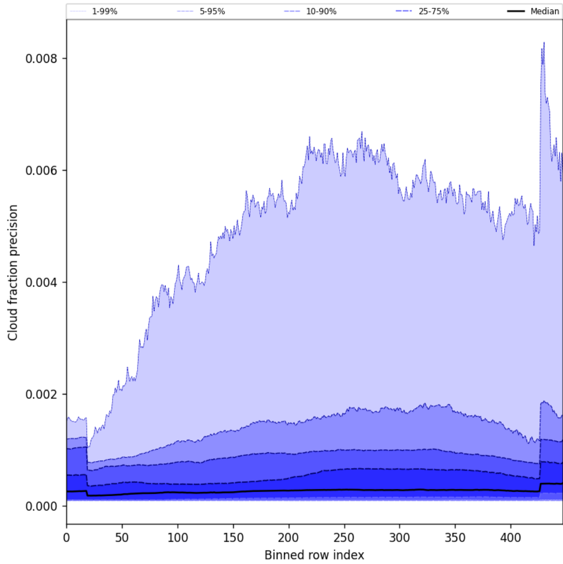
Figure 50: Along track statistics of “Cloud fraction precision” for 2024-10-27 to 2024-10-29
