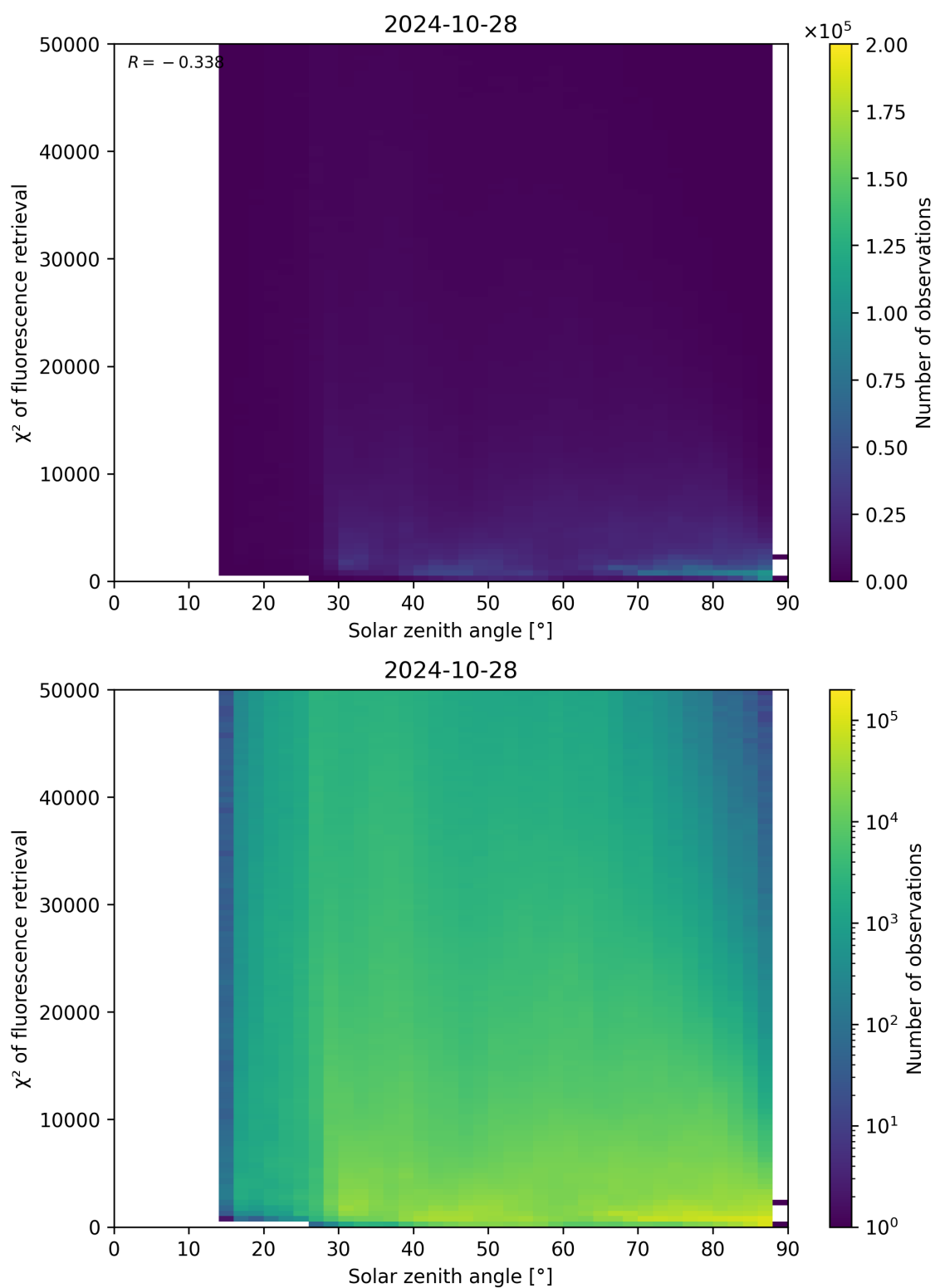
Figure 120: Scatter density plot of “Solar zenith angle” against “ \chi^2 of fluorescence retrieval” for 2024-10-27 to 2024-10-29.
