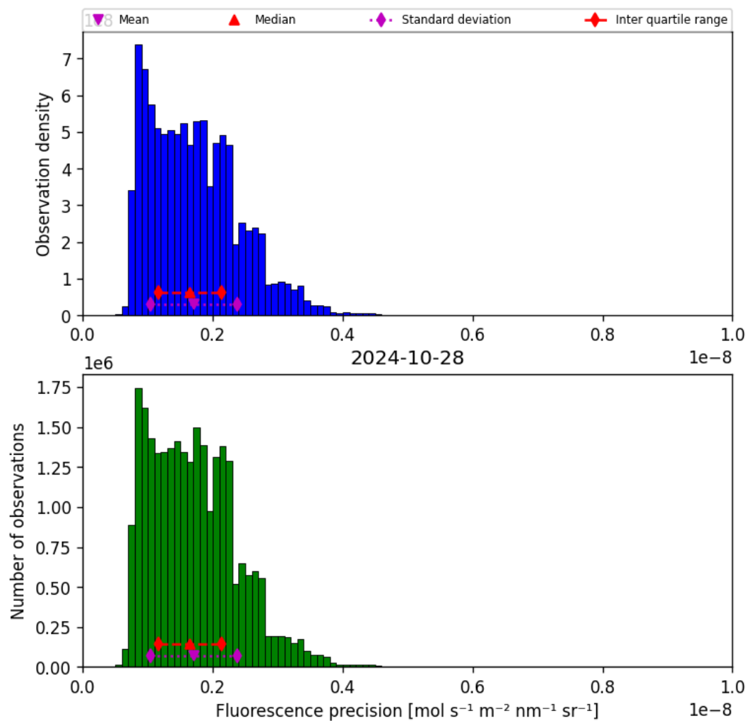
Figure 41: Histogram of “Fluorescence precision” for 2024-10-27 to 2024-10-29
