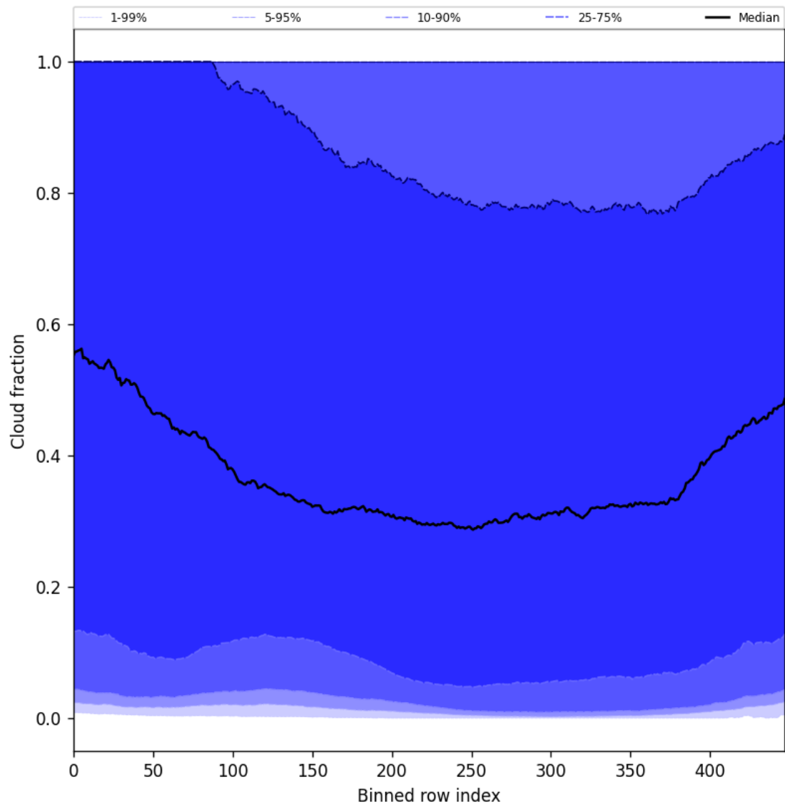
Figure 49: Along track statistics of “Cloud fraction” for 2024-10-27 to 2024-10-29
