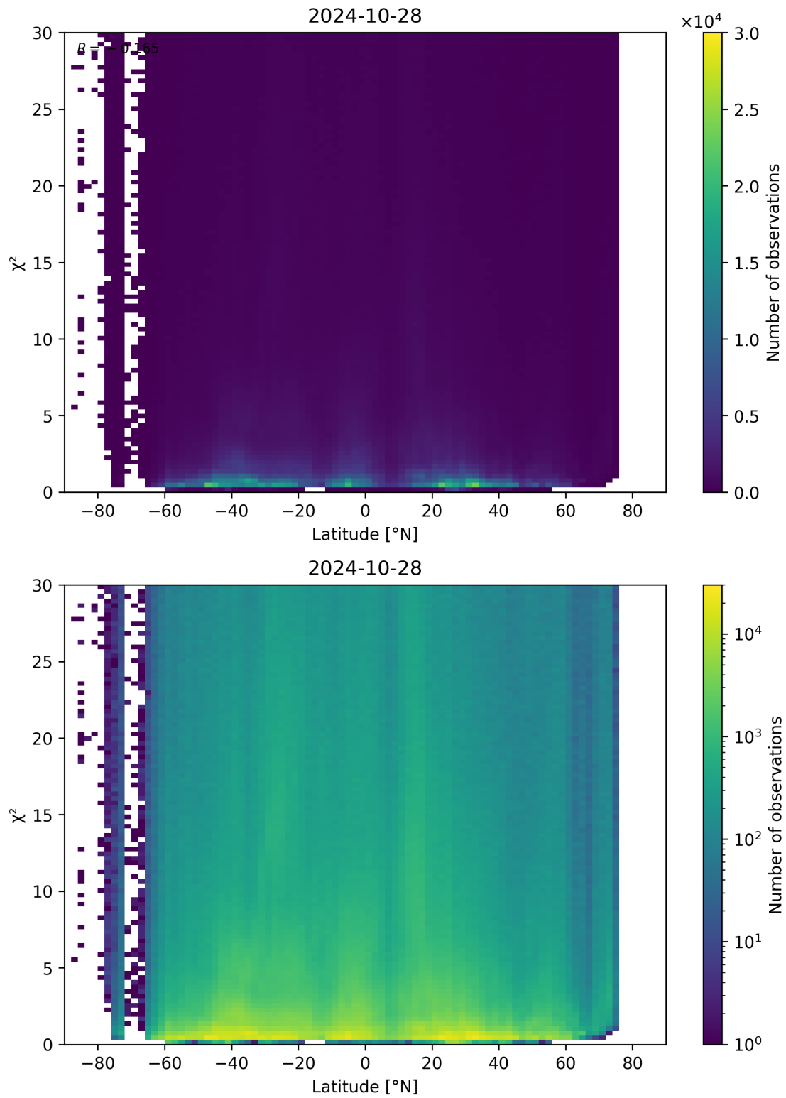
Figure 97: Scatter density plot of “Latitude” against “ \chi^2 ” for 2024-10-27 to 2024-10-29.
