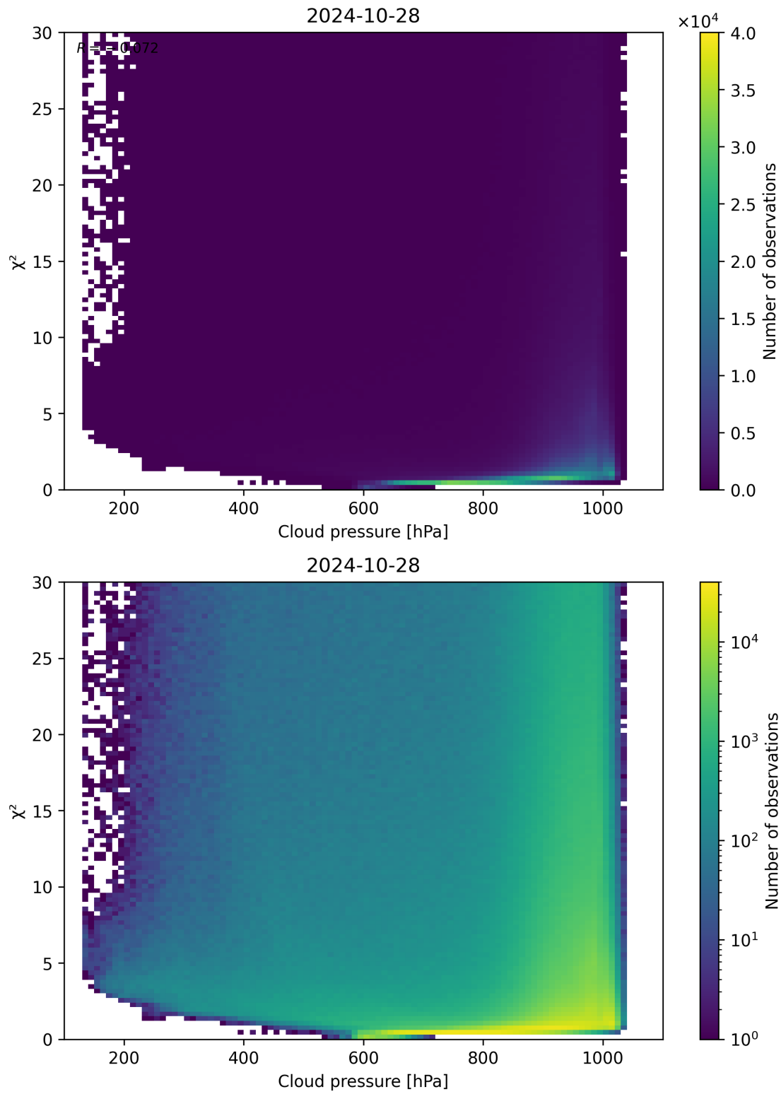
Figure 85: Scatter density plot of “Cloud pressure” against “ \chi^2 ” for 2024-10-27 to 2024-10-29.
