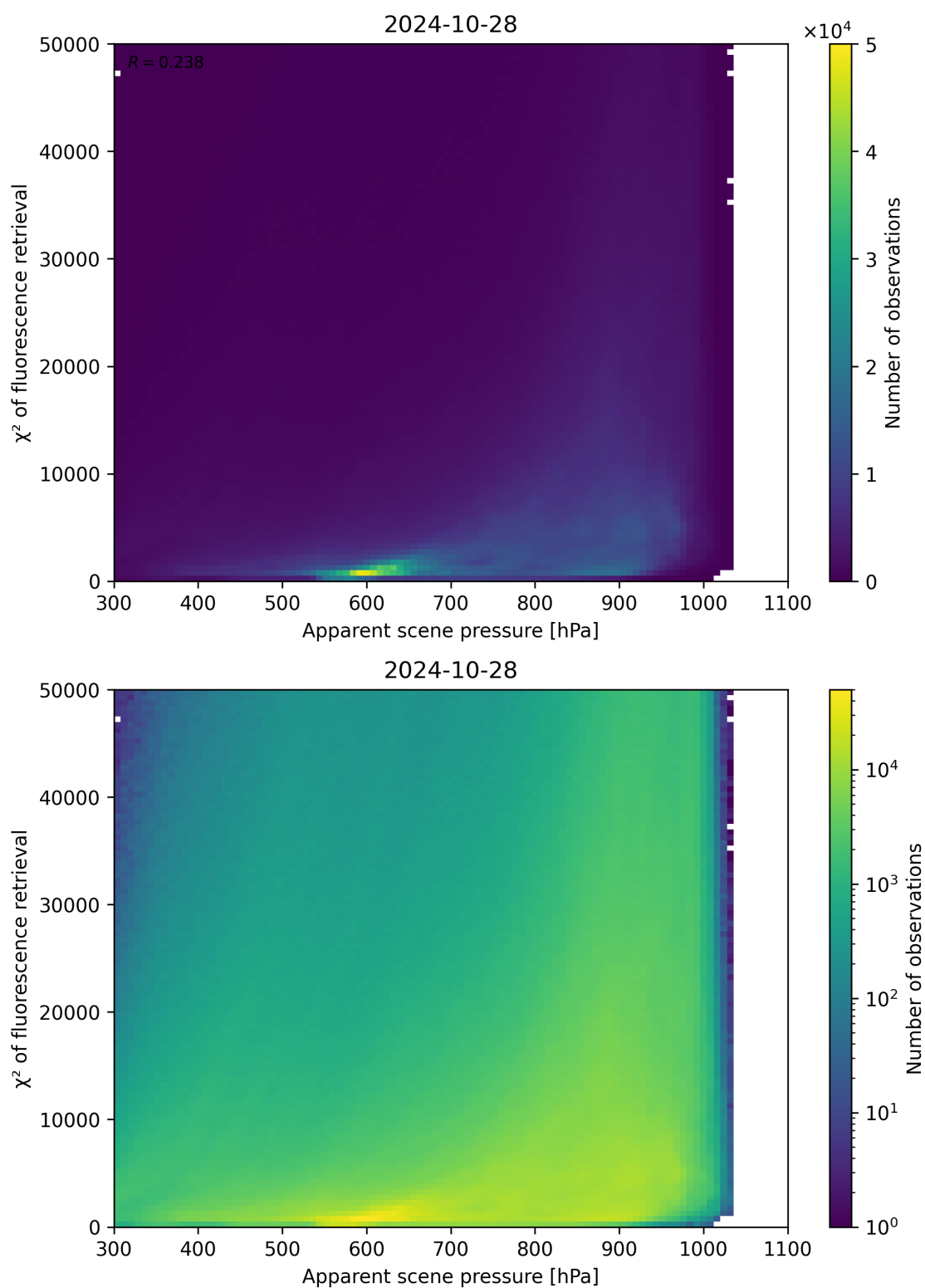
Figure 64: Scatter density plot of “Apparent scene pressure” against “ \chi^2 of fluorescence retrieval” for 2024-10-27 to 2024-10-29.
