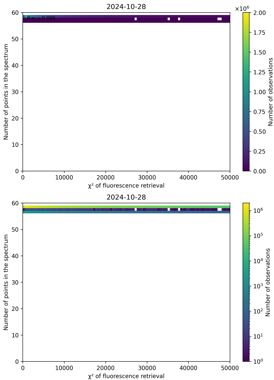
Figure 71: Scatter density plot of “ \chi^2 of fluorescence retrieval” against “Number of points in the spectrum” for 2024-10-27 to 2024-10-29.
