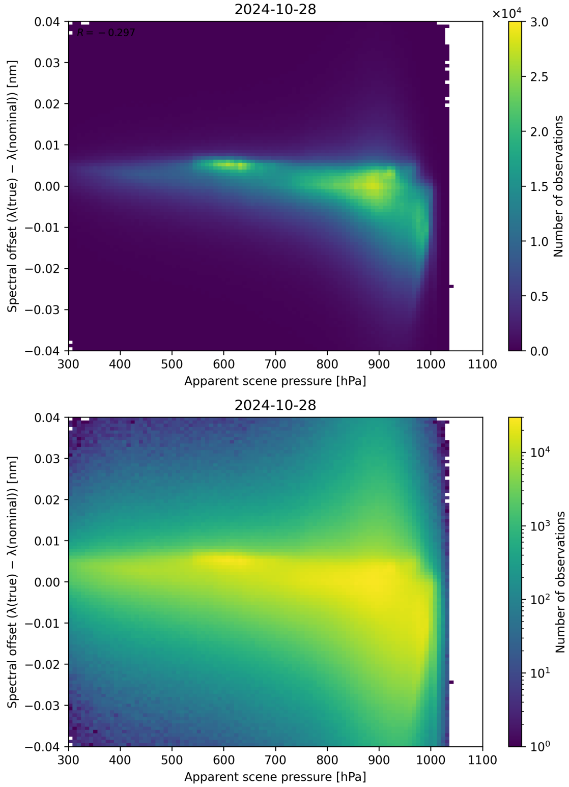
Figure 68: Scatter density plot of “Apparent scene pressure” against “Spectral offset ( \lambda_{\text{true}} - \lambda_{\text{nominal}} )” for 2024-10-27 to 2024-10-29.
