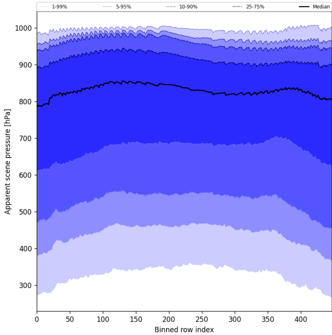
Figure 53: Along track statistics of “Apparent scene pressure” for 2024-10-27 to 2024-10-29
