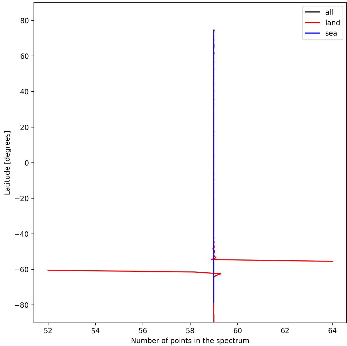
Figure 27: Zonal average of “Number of points in the spectrum” for 2024-10-27 to 2024-10-29.
