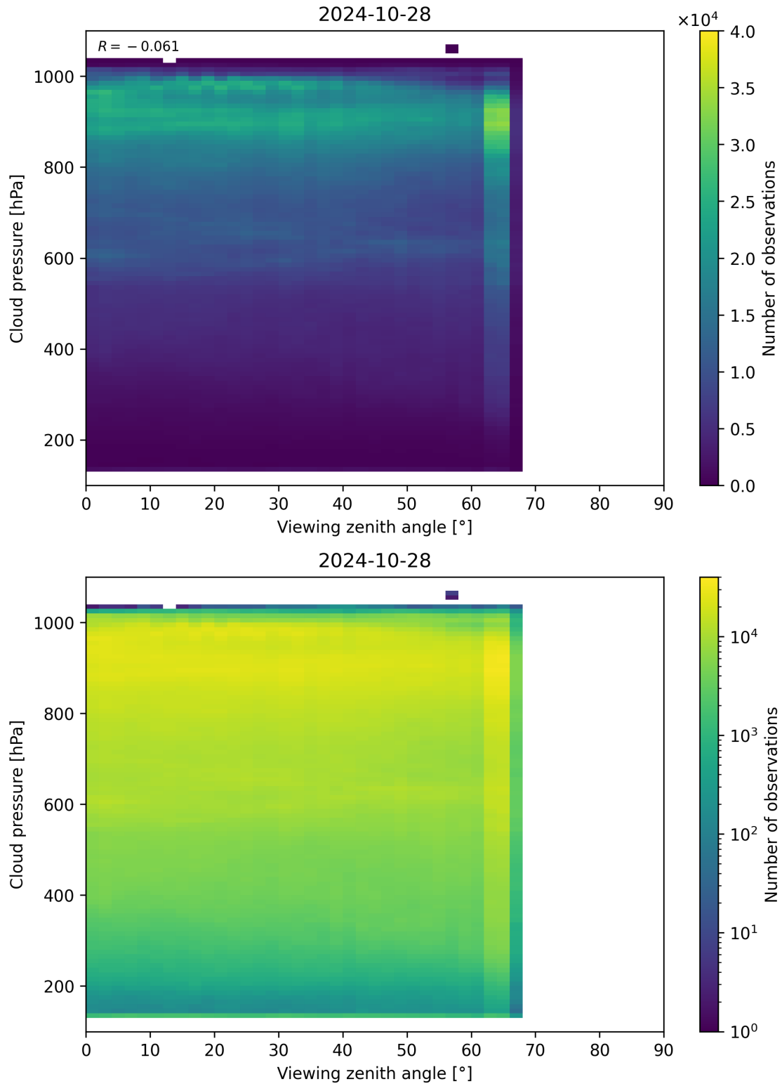
Figure 133: Scatter density plot of “Viewing zenith angle” against “Cloud pressure” for 2024-10-27 to 2024-10-29.
