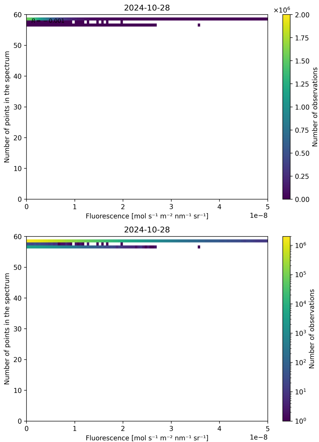
Figure 94: Scatter density plot of “Fluorescence” against “Number of points in the spectrum” for 2024-10-27 to 2024-10-29.
