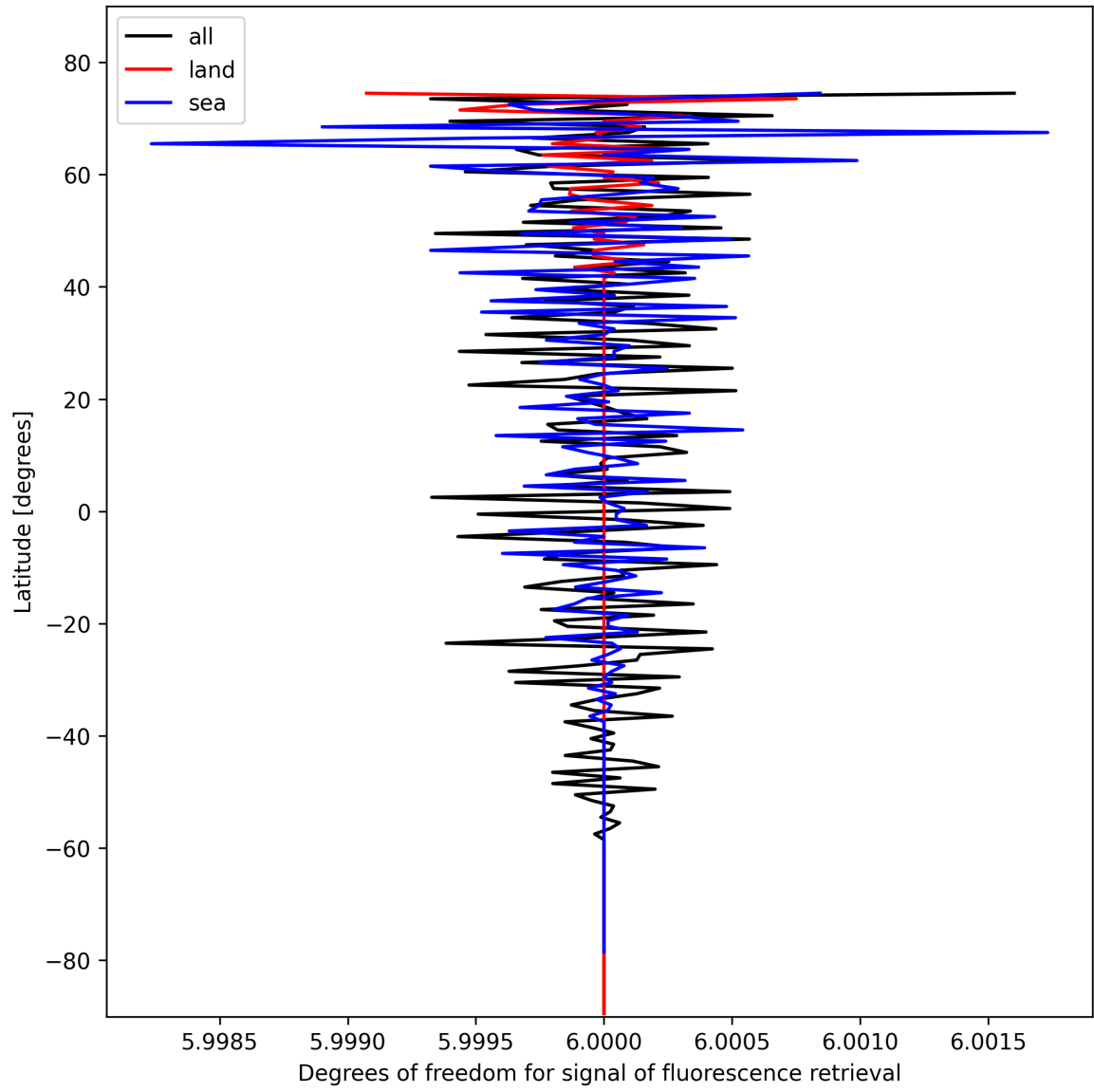
Figure 26: Zonal average of “Degrees of freedom for signal of fluorescence retrieval” for 2024-10-27 to 2024-10-29.
