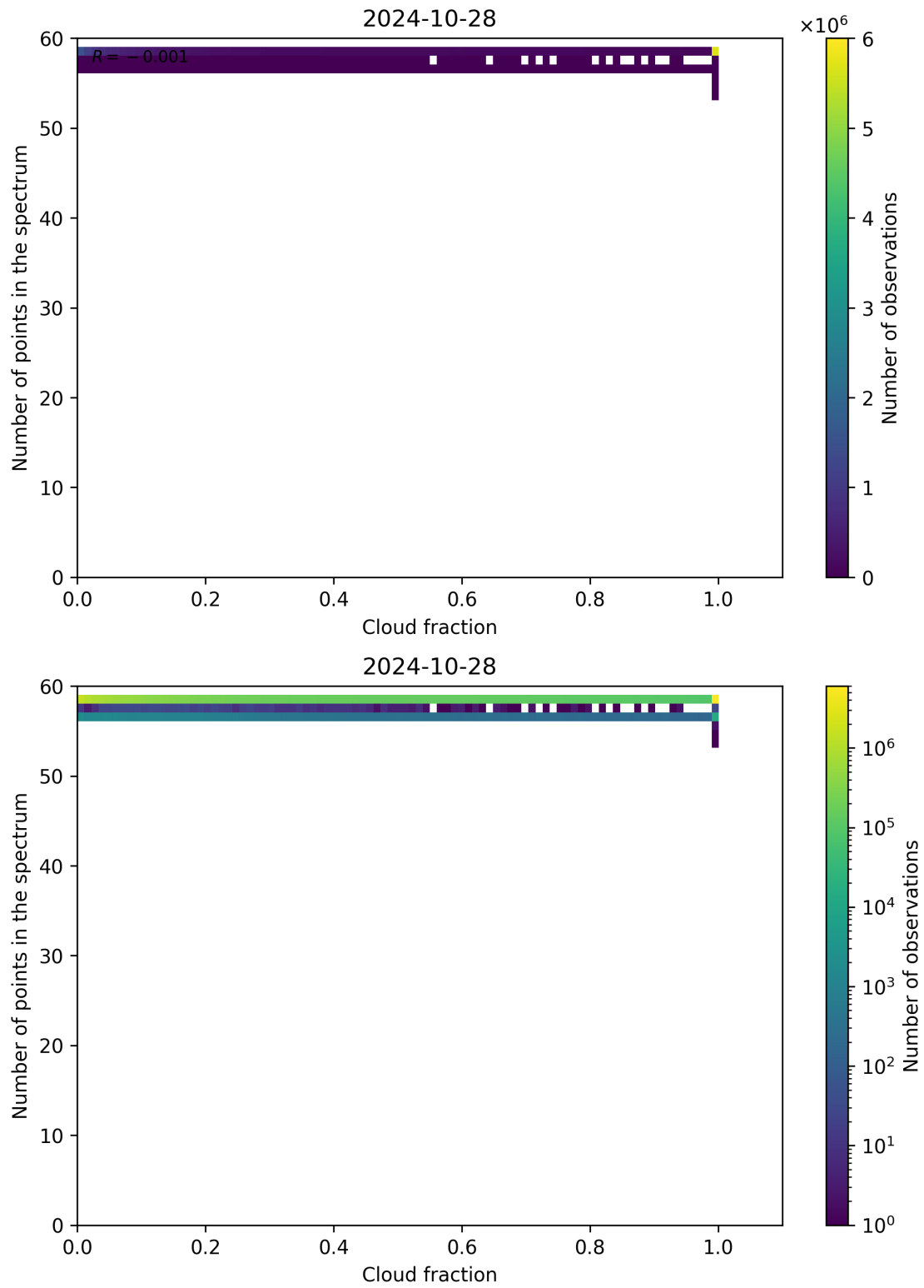
Figure 81: Scatter density plot of “Cloud fraction” against “Number of points in the spectrum” for 2024-10-27 to 2024-10-29.
