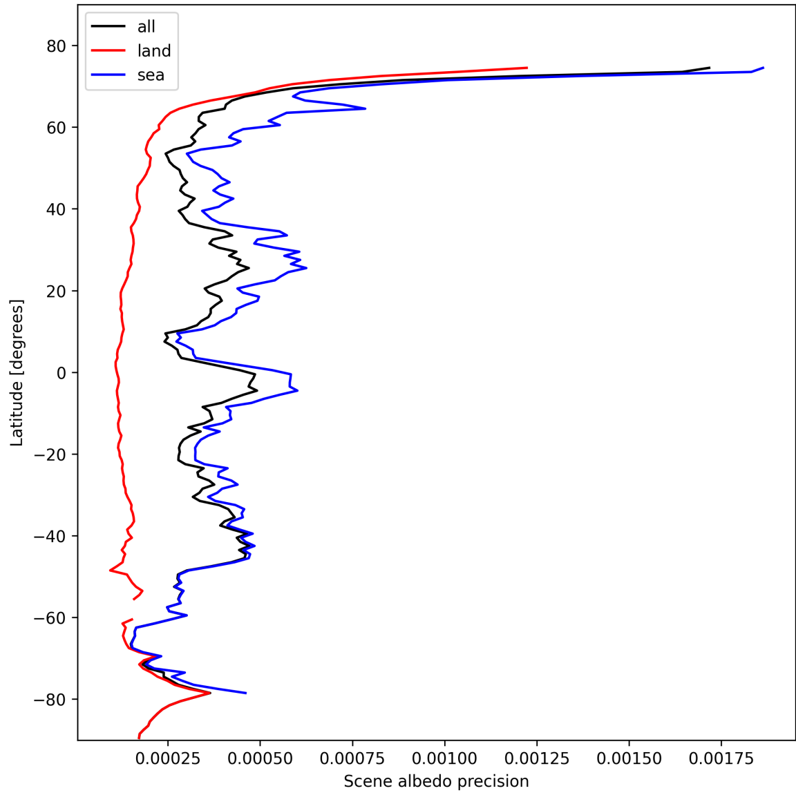
Figure 18: Zonal average of “Scene albedo precision” for 2024-10-29 to 2024-10-30.
