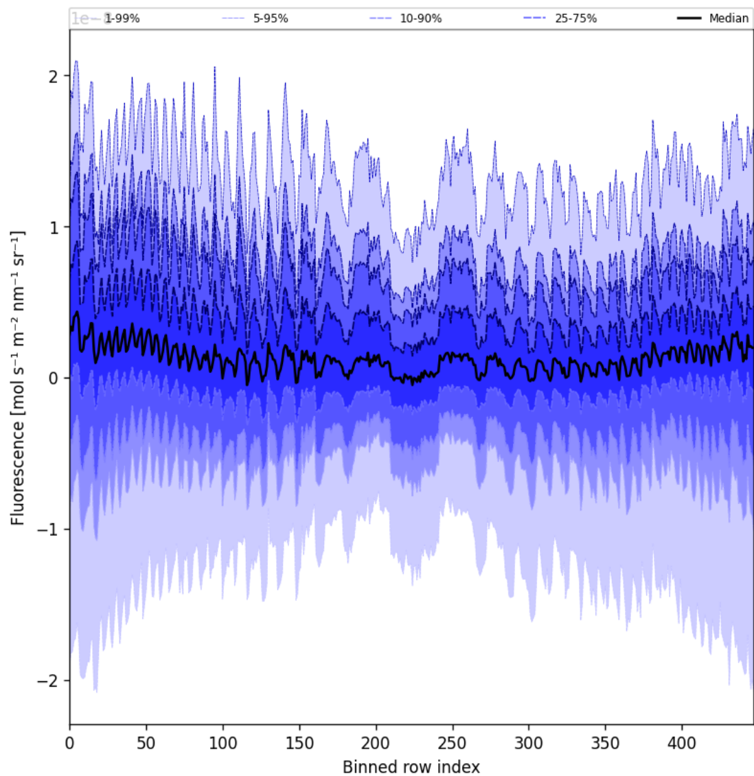
Figure 57: Along track statistics of “Fluorescence” for 2024-10-29 to 2024-10-30
