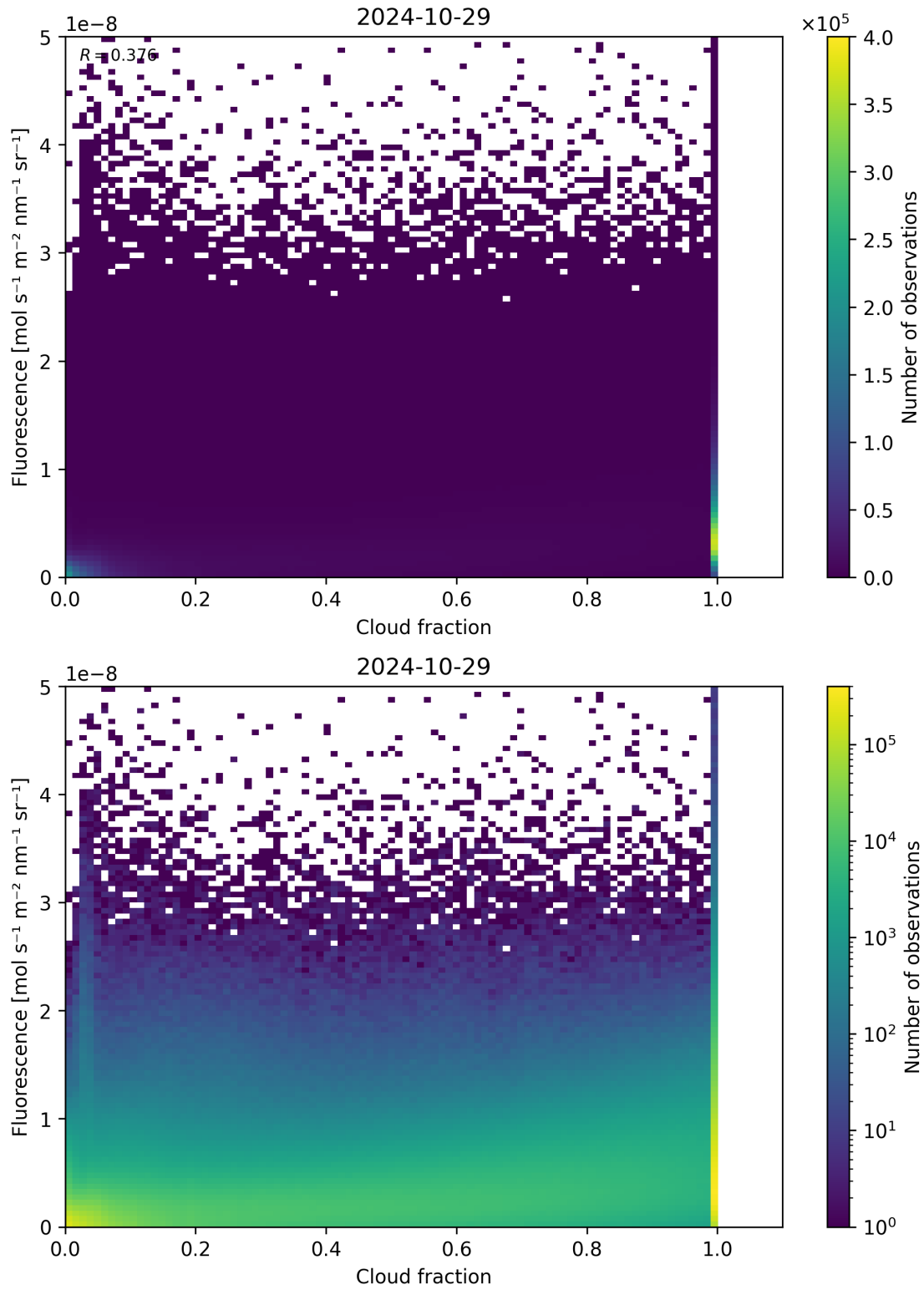
Figure 79: Scatter density plot of “Cloud fraction” against “Fluorescence” for 2024-10-29 to 2024-10-30.
