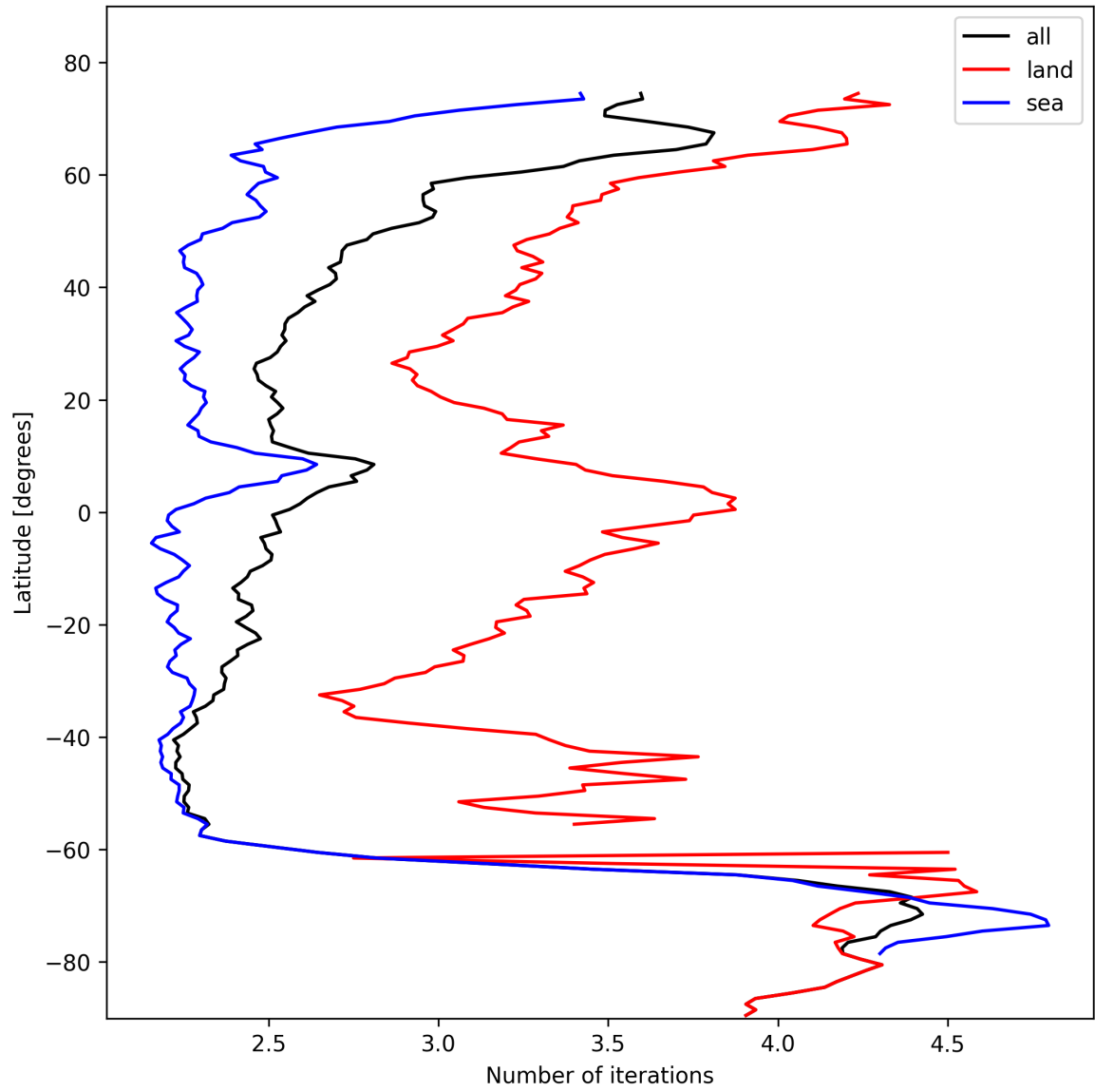
Figure 22: Zonal average of “Number of iterations” for 2024-10-29 to 2024-10-30.
