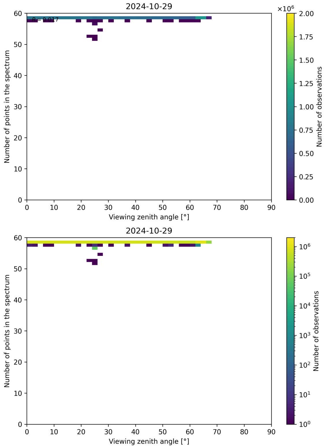
Figure 137: Scatter density plot of “Viewing zenith angle” against “Number of points in the spectrum” for 2024-10-29 to 2024-10-30.
