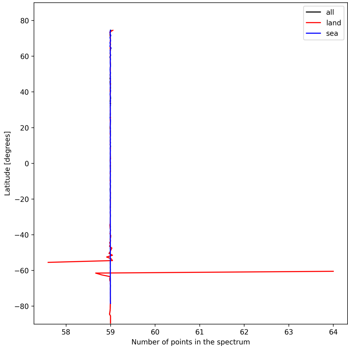
Figure 27: Zonal average of “Number of points in the spectrum” for 2024-10-29 to 2024-10-30.
