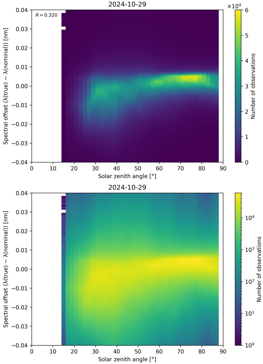
Figure 128: Scatter density plot of “Solar zenith angle” against “Spectral offset ( \lambda_{\text{true}} - \lambda_{\text{nominal}} )” for 2024-10-29 to 2024-10-30.
