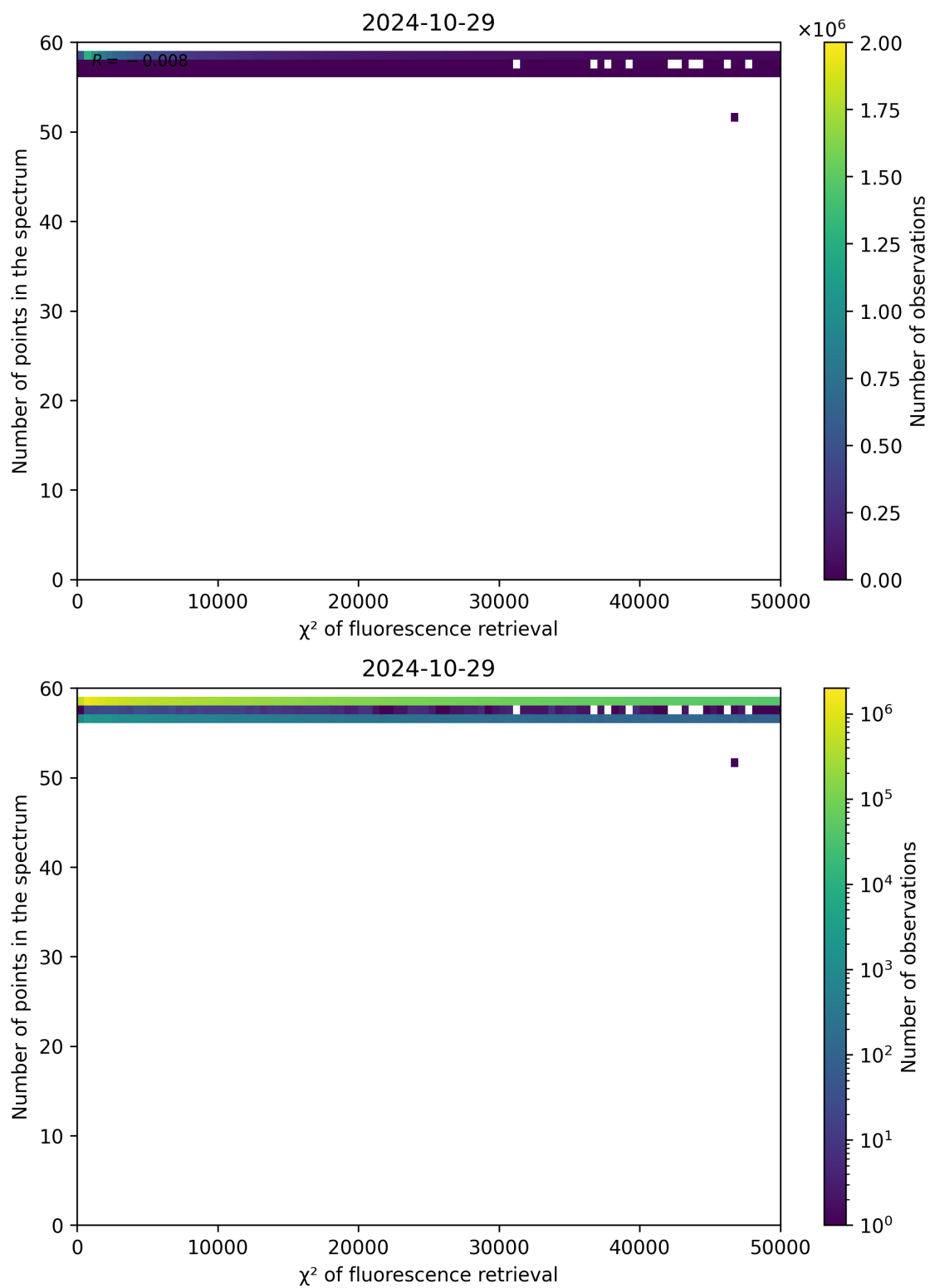
Figure 71: Scatter density plot of “ \chi^2 of fluorescence retrieval” against “Number of points in the spectrum” for 2024-10-29 to 2024-10-30.
