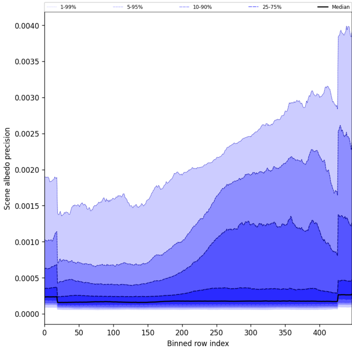
Figure 52: Along track statistics of “Scene albedo precision” for 2024-10-29 to 2024-10-30
