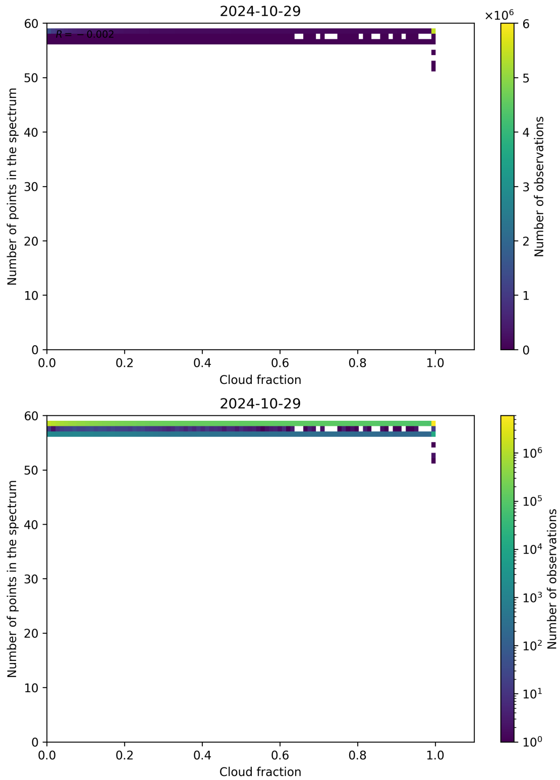
Figure 81: Scatter density plot of “Cloud fraction” against “Number of points in the spectrum” for 2024-10-29 to 2024-10-30.
