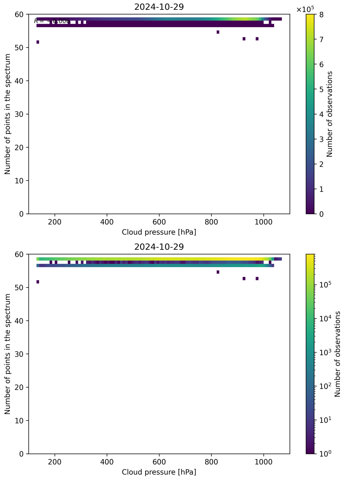
Figure 90: Scatter density plot of “Cloud pressure” against “Number of points in the spectrum” for 2024-10-29 to 2024-10-30.
