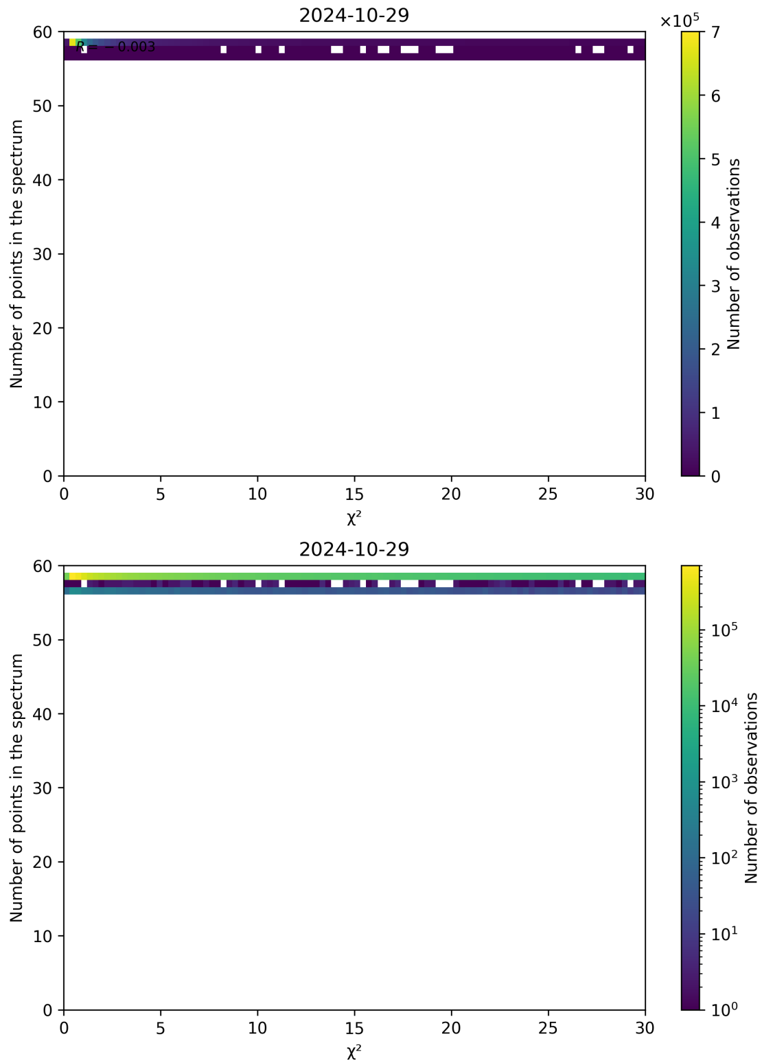
Figure 74: Scatter density plot of " \chi^2 " against "Number of points in the spectrum" for 2024-10-29 to 2024-10-30.
