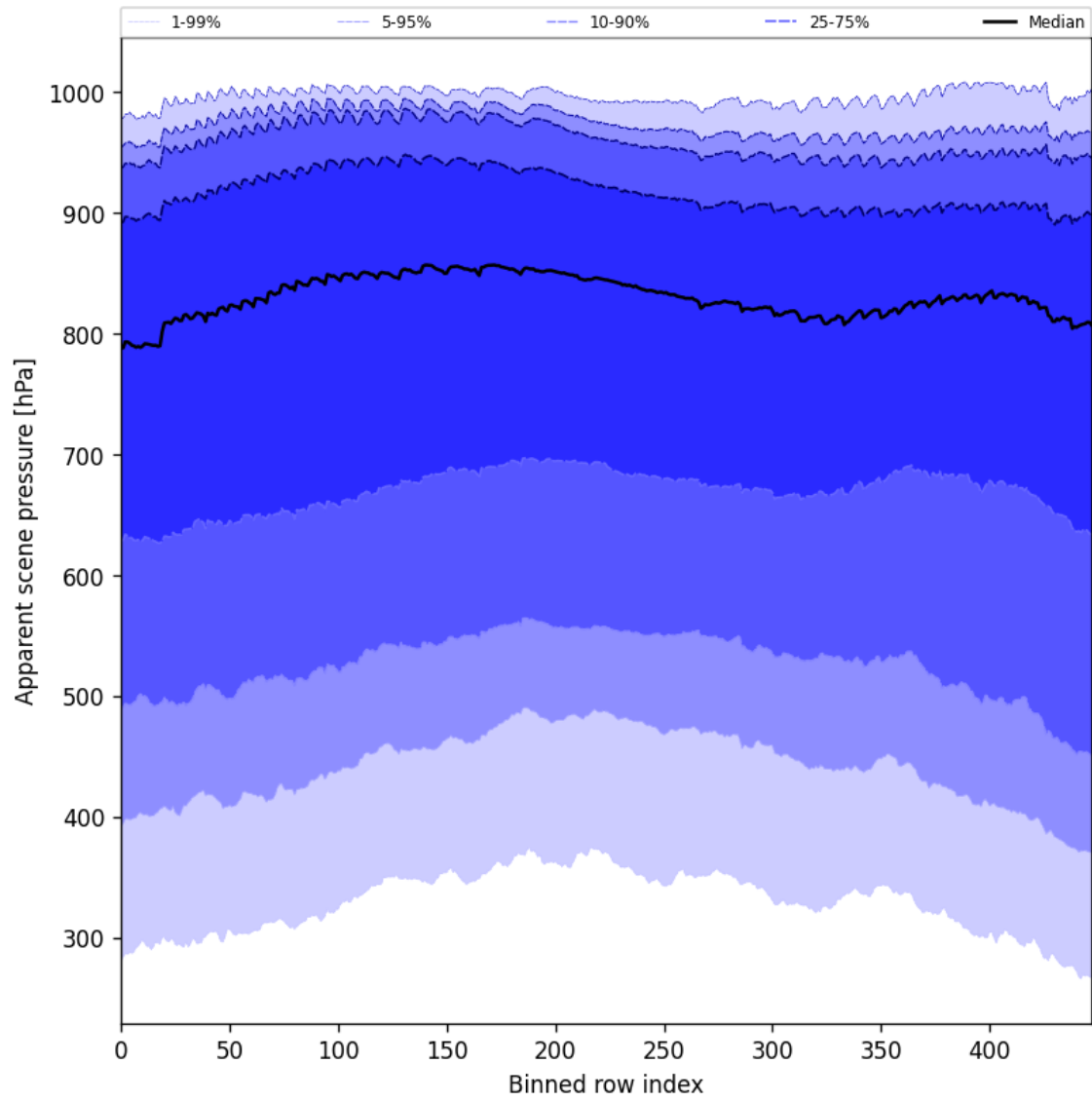
Figure 53: Along track statistics of “Apparent scene pressure” for 2024-10-29 to 2024-10-30
