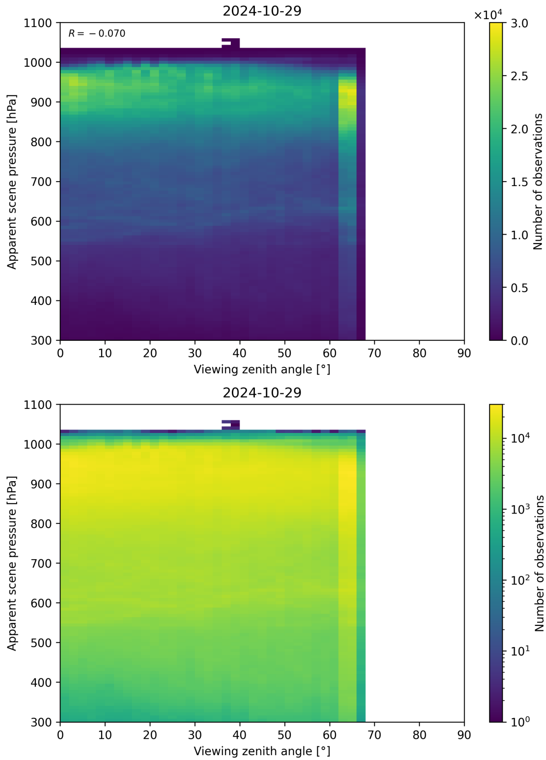
Figure 129: Scatter density plot of “Viewing zenith angle” against “Apparent scene pressure” for 2024-10-29 to 2024-10-30.
