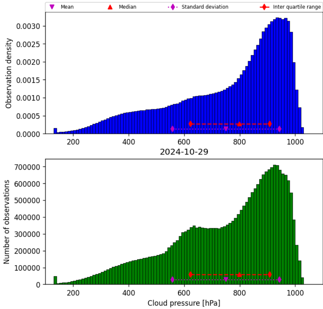
Figure 30: Histogram of “Cloud pressure” for 2024-10-29 to 2024-10-30
