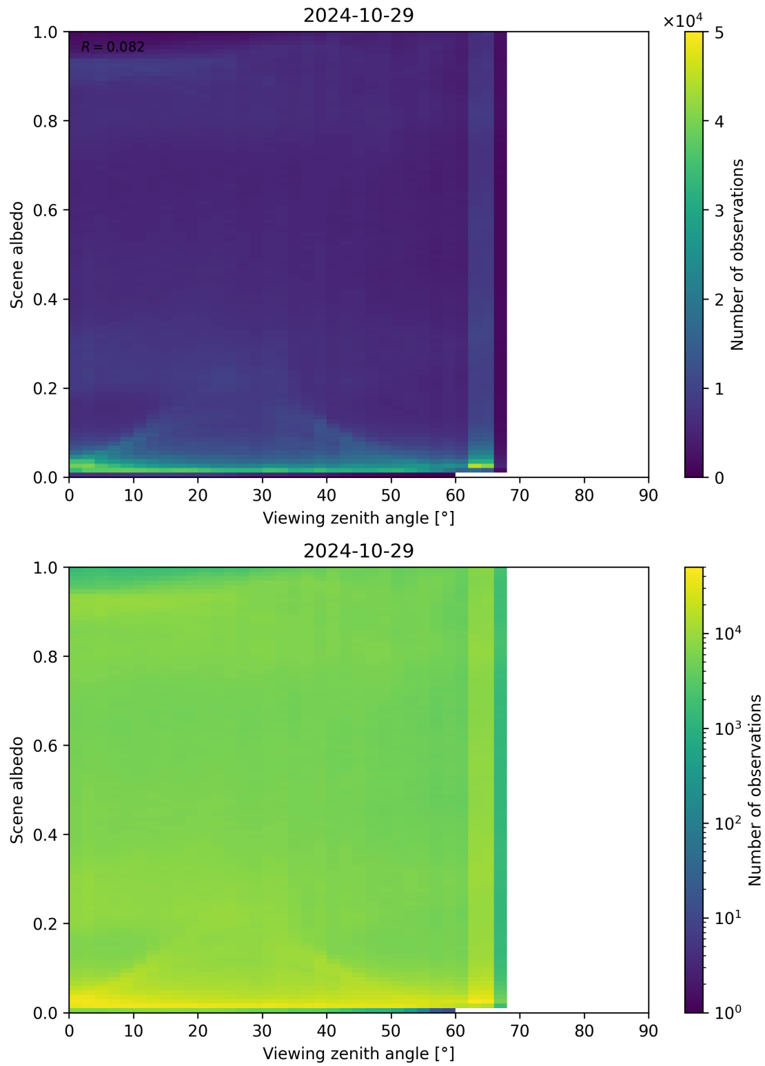
Figure 138: Scatter density plot of “Viewing zenith angle” against “Scene albedo” for 2024-10-29 to 2024-10-30.
