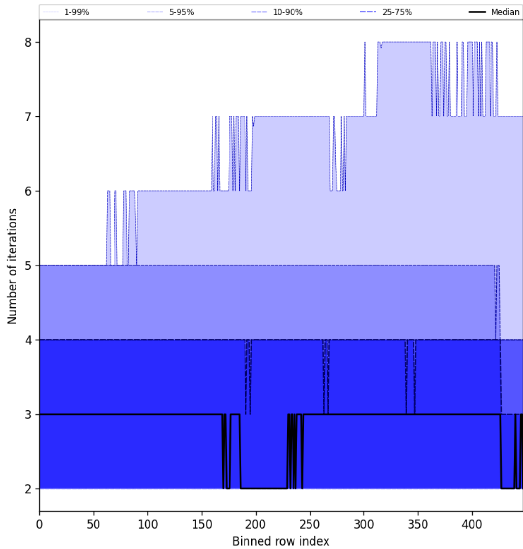
Figure 56: Along track statistics of “Number of iterations” for 2024-10-29 to 2024-10-30
