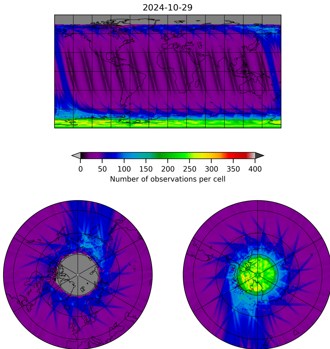
Figure 11: Map of the number of observations for 2024-10-29 to 2024-10-30
