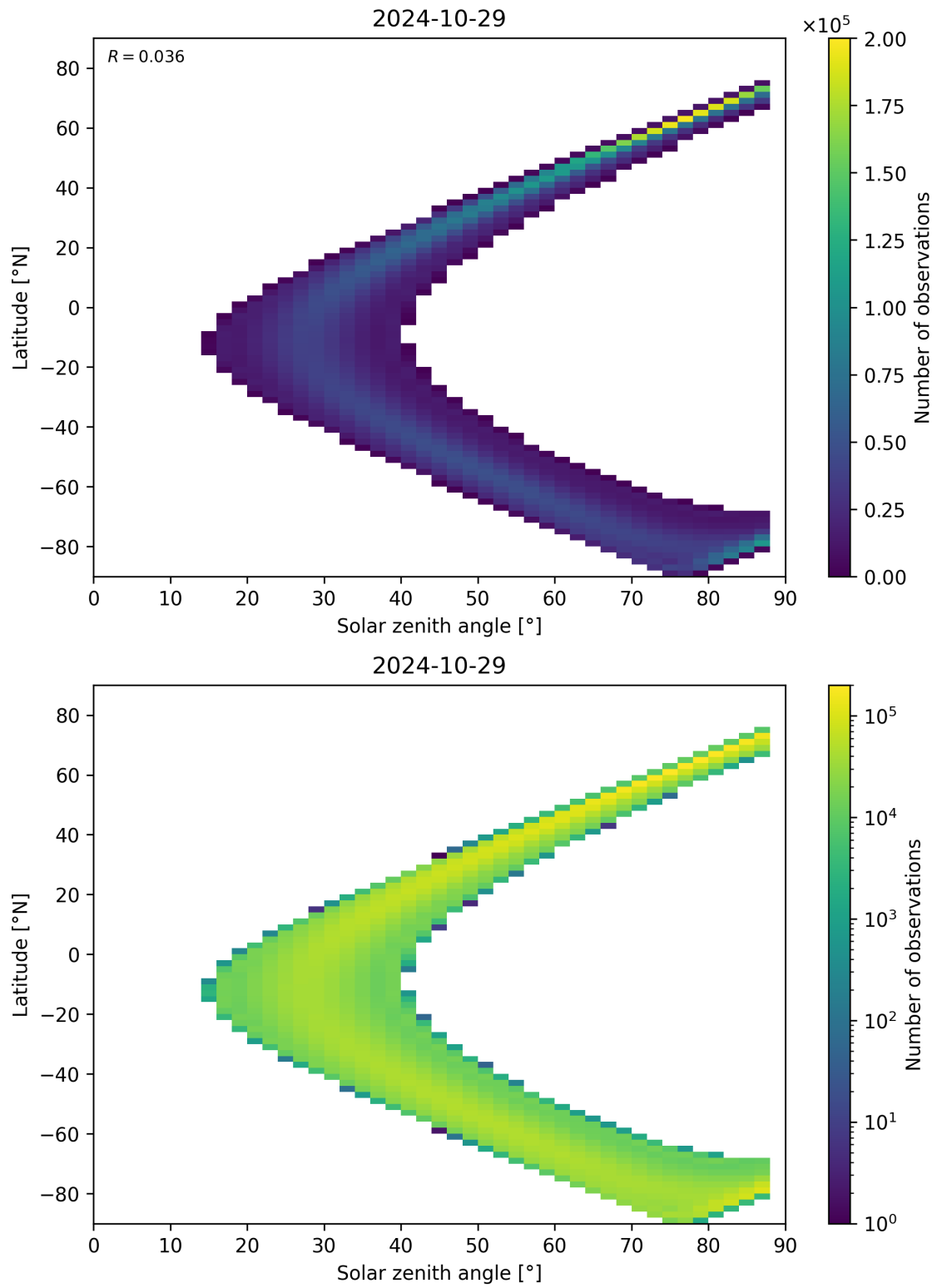
Figure 124: Scatter density plot of “Solar zenith angle” against “Latitude” for 2024-10-29 to 2024-10-30.
