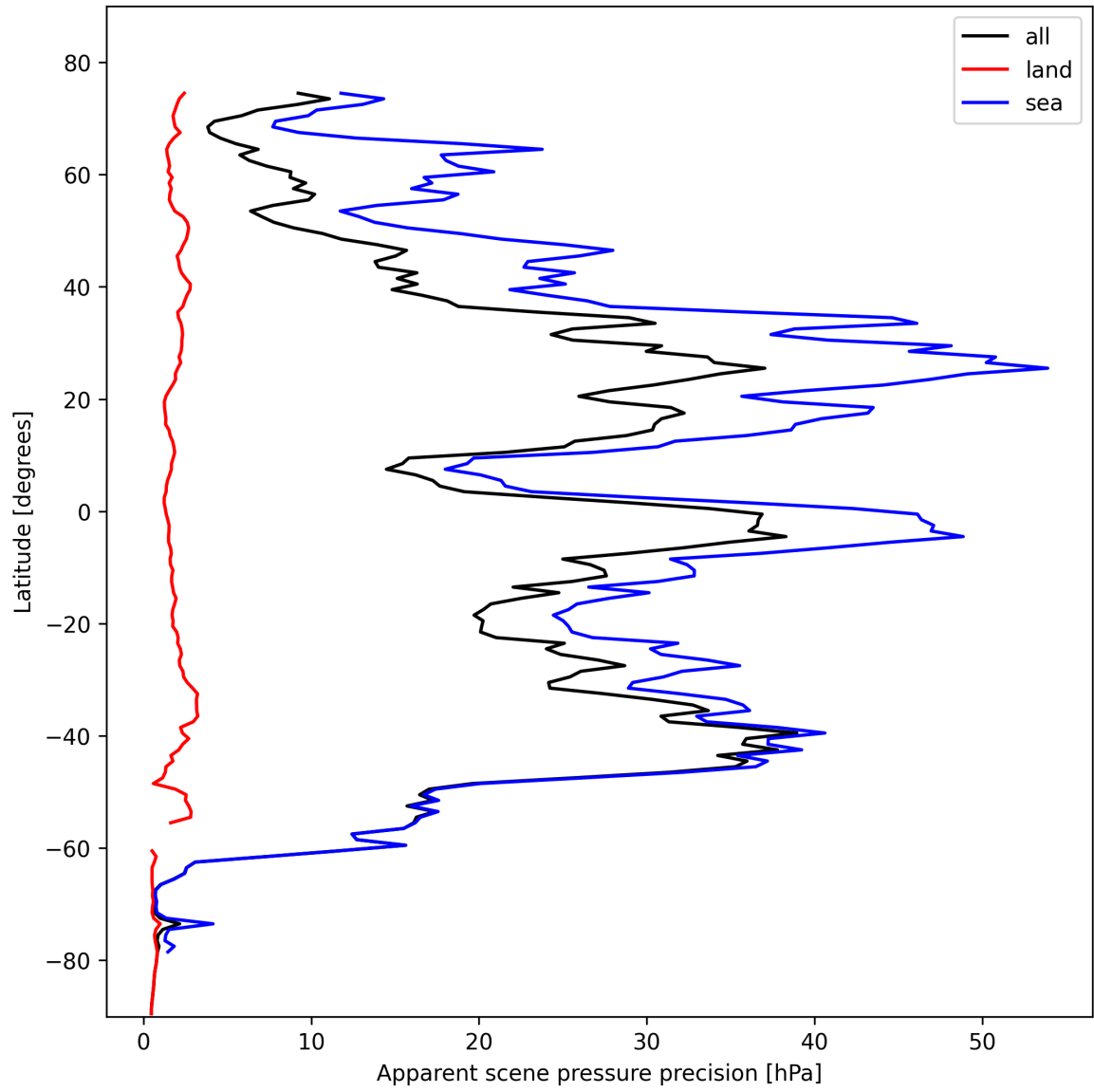
Figure 20: Zonal average of “Apparent scene pressure precision” for 2024-10-29 to 2024-10-30.
