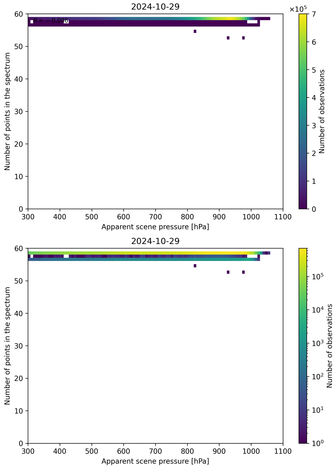
Figure 67: Scatter density plot of “Apparent scene pressure” against “Number of points in the spectrum” for 2024-10-29 to 2024-10-30.
