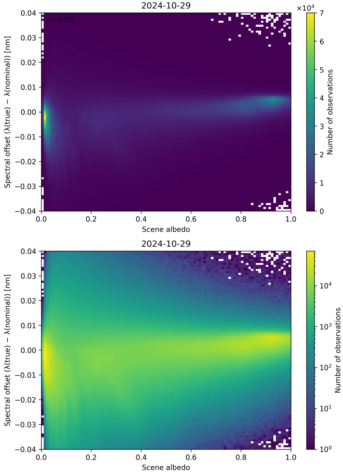
Figure 117: Scatter density plot of “Scene albedo” against “Spectral offset ( \lambda_{\text{true}} - \lambda_{\text{nominal}} )” for 2024-10-29 to 2024-10-30.
