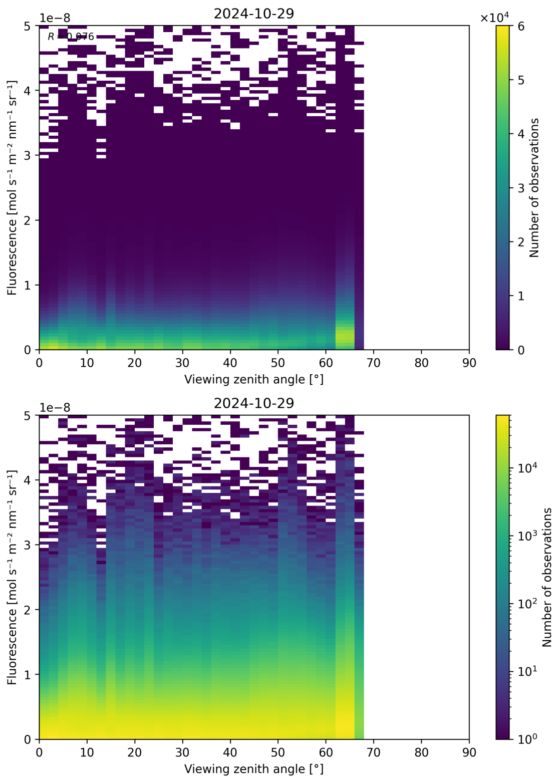
Figure 134: Scatter density plot of “Viewing zenith angle” against “Fluorescence” for 2024-10-29 to 2024-10-30.
