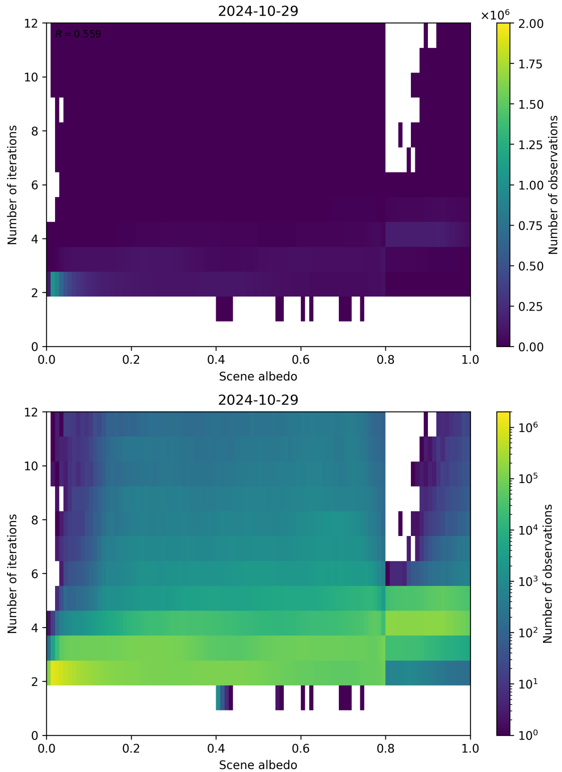
Figure 115: Scatter density plot of “Scene albedo” against “Number of iterations” for 2024-10-29 to 2024-10-30.
