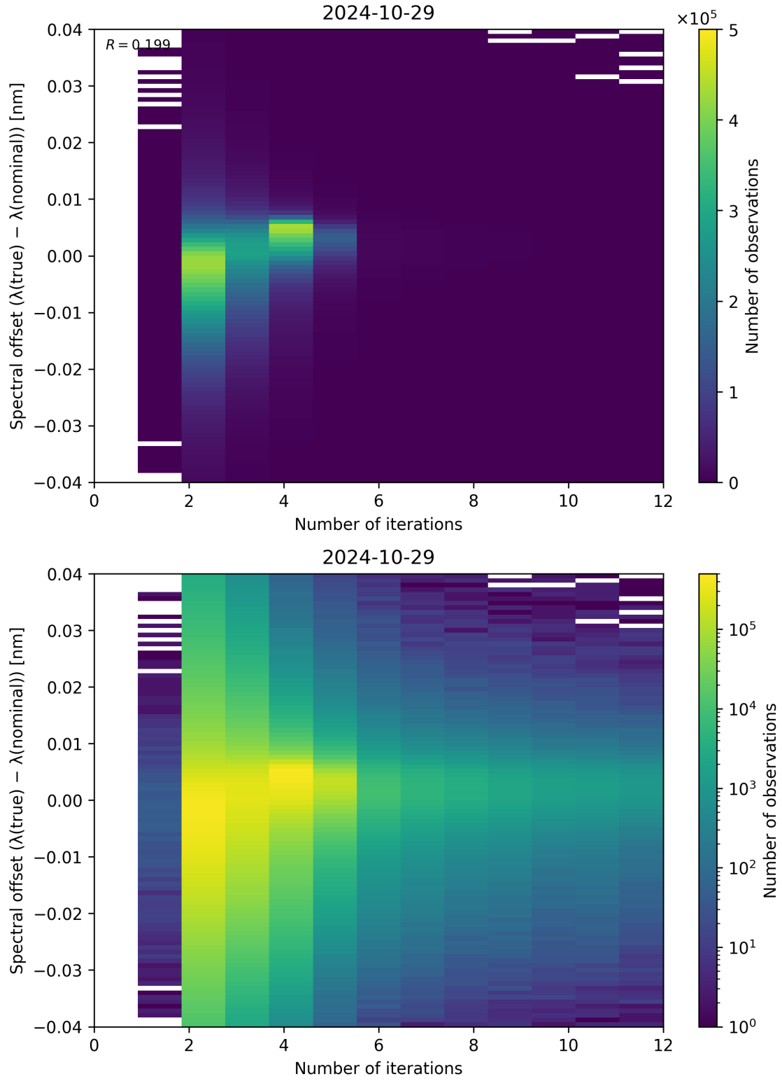
Figure 109: Scatter density plot of “Number of iterations” against “Spectral offset ( \lambda_{\text{true}} - \lambda_{\text{nominal}} )” for 2024-10-29 to 2024-10-30.
