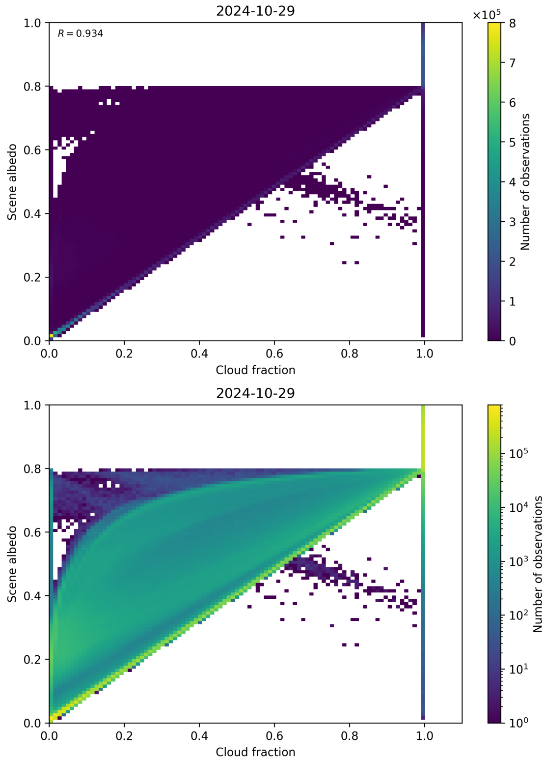
Figure 82: Scatter density plot of “Cloud fraction” against “Scene albedo” for 2024-10-29 to 2024-10-30.
