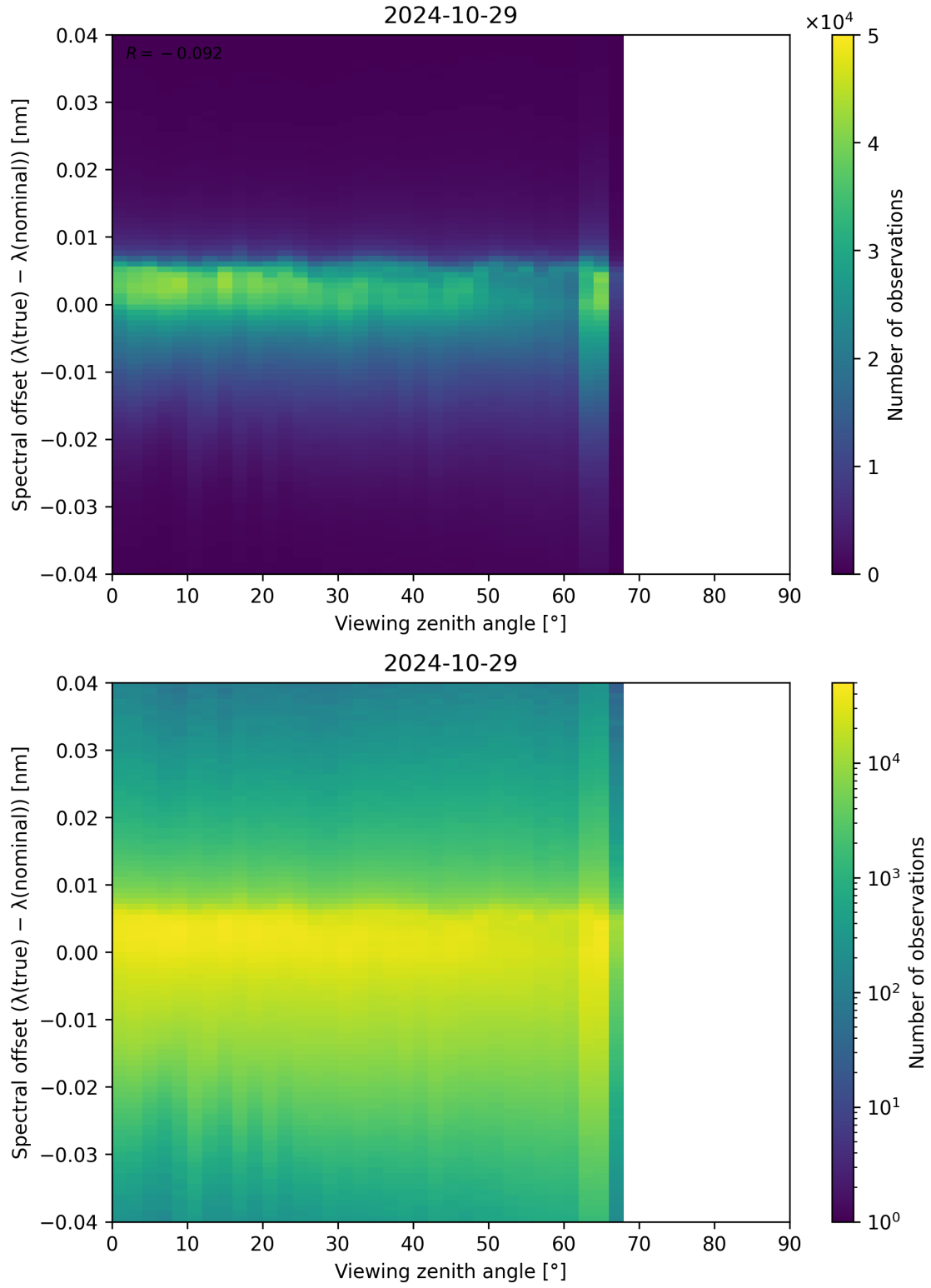
Figure 140: Scatter density plot of “Viewing zenith angle” against “Spectral offset ( \lambda_{\text{true}} - \lambda_{\text{nominal}} )” for 2024-10-29 to 2024-10-30.
