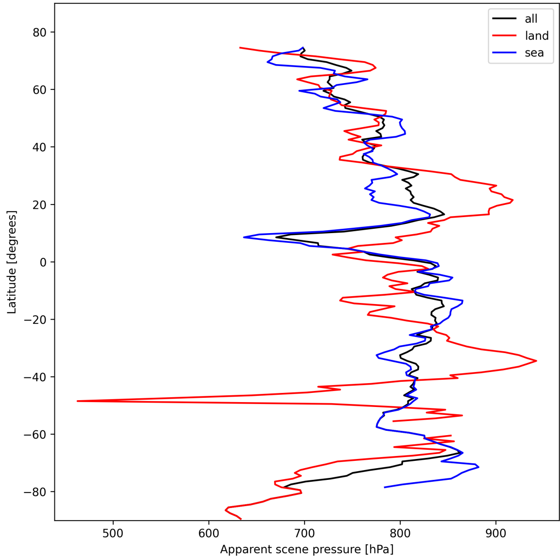
Figure 19: Zonal average of “Apparent scene pressure” for 2024-10-29 to 2024-10-30.
