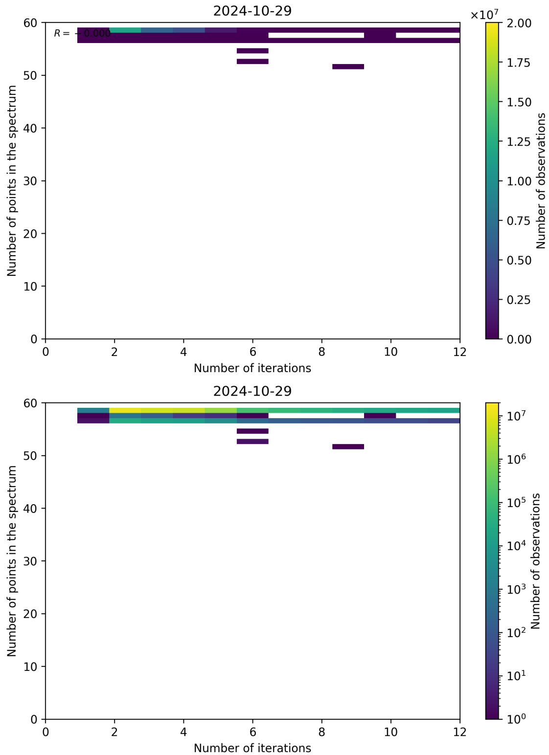
Figure 108: Scatter density plot of “Number of iterations” against “Number of points in the spectrum” for 2024-10-29 to 2024-10-30.
