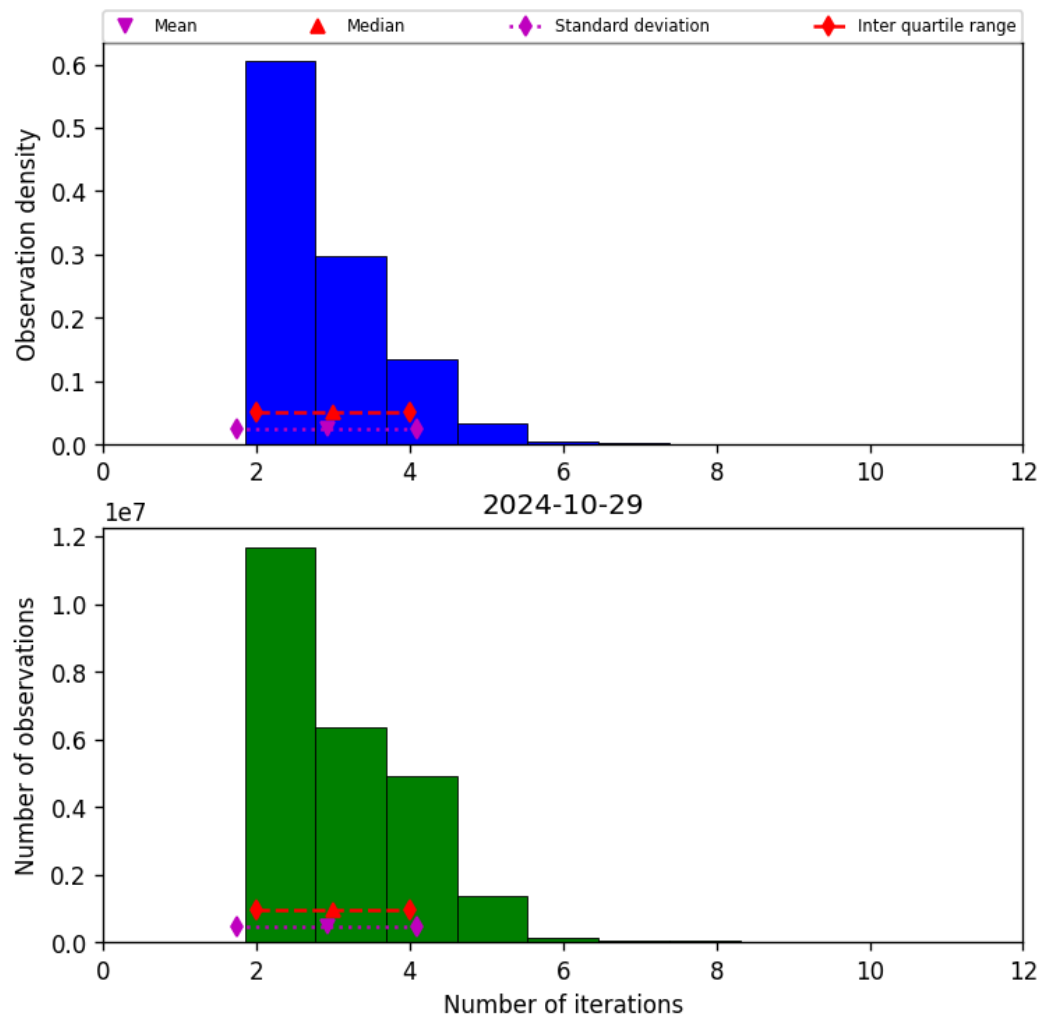
Figure 39: Histogram of “Number of iterations” for 2024-10-29 to 2024-10-30
