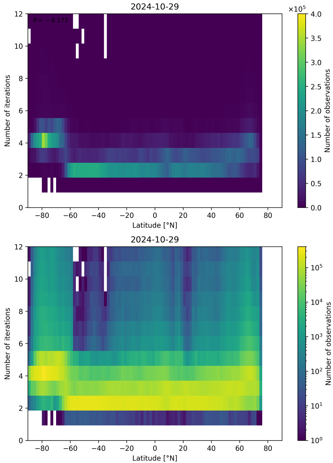
Figure 102: Scatter density plot of “Latitude” against “Number of iterations” for 2024-10-29 to 2024-10-30.
