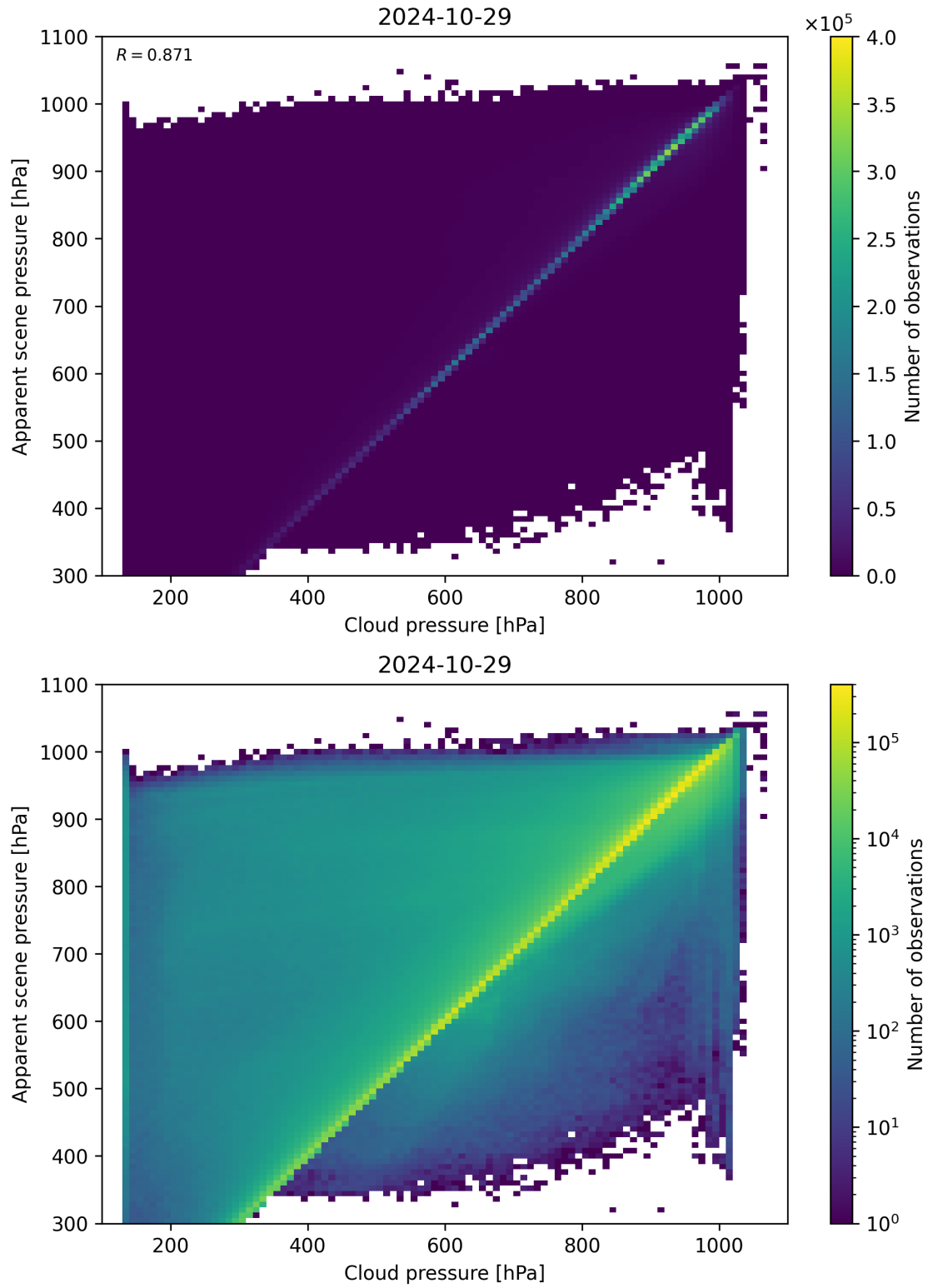
Figure 84: Scatter density plot of “Cloud pressure” against “Apparent scene pressure” for 2024-10-29 to 2024-10-30.
