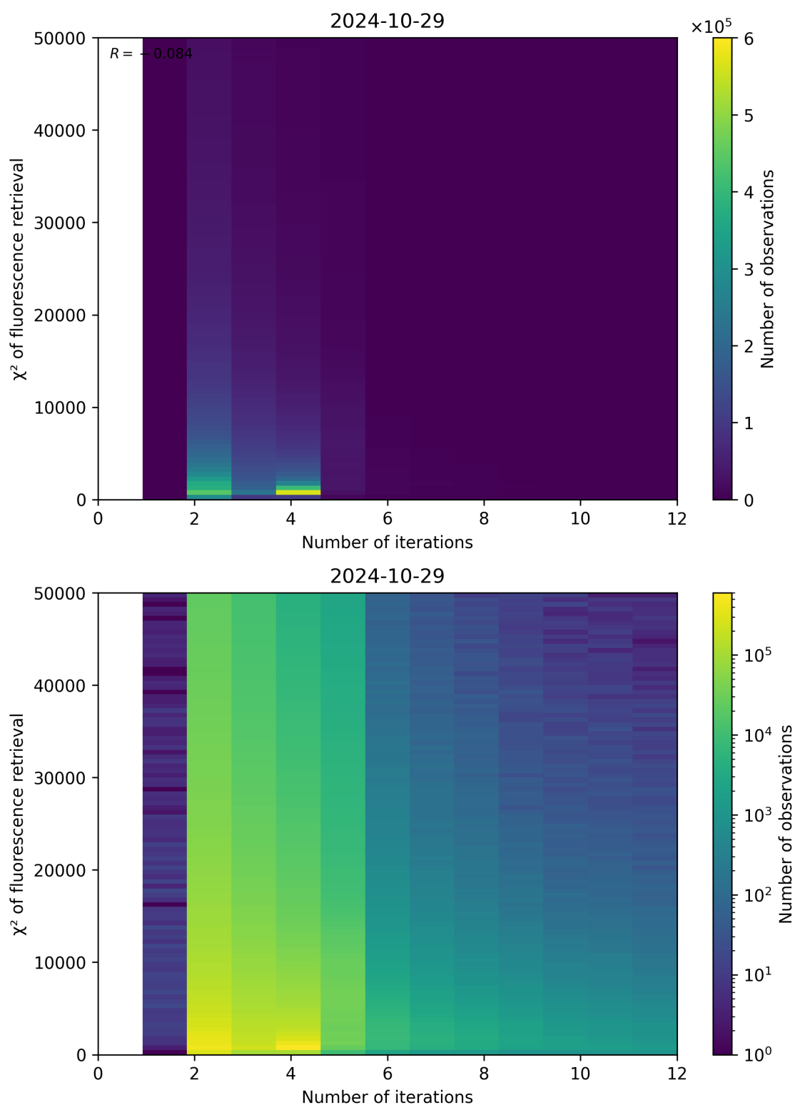
Figure 106: Scatter density plot of “Number of iterations” against “ \chi^2 of fluorescence retrieval” for 2024-10-29 to 2024-10-30.
