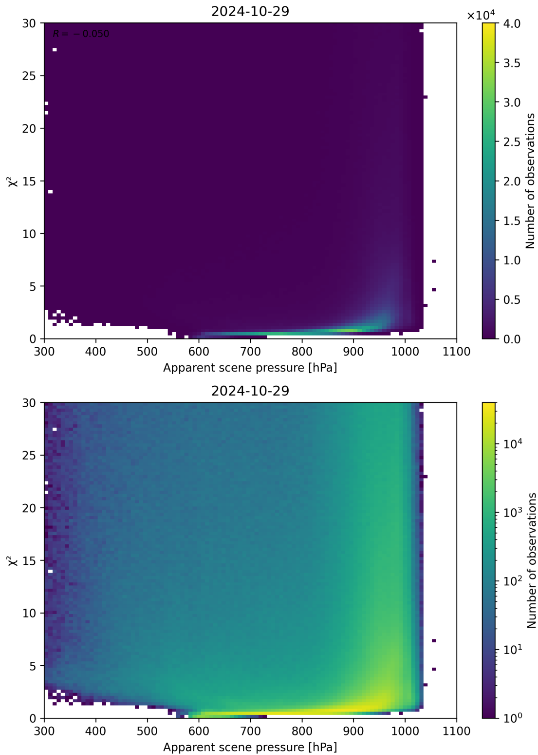
Figure 63: Scatter density plot of “Apparent scene pressure” against “ \chi^2 ” for 2024-10-29 to 2024-10-30.
