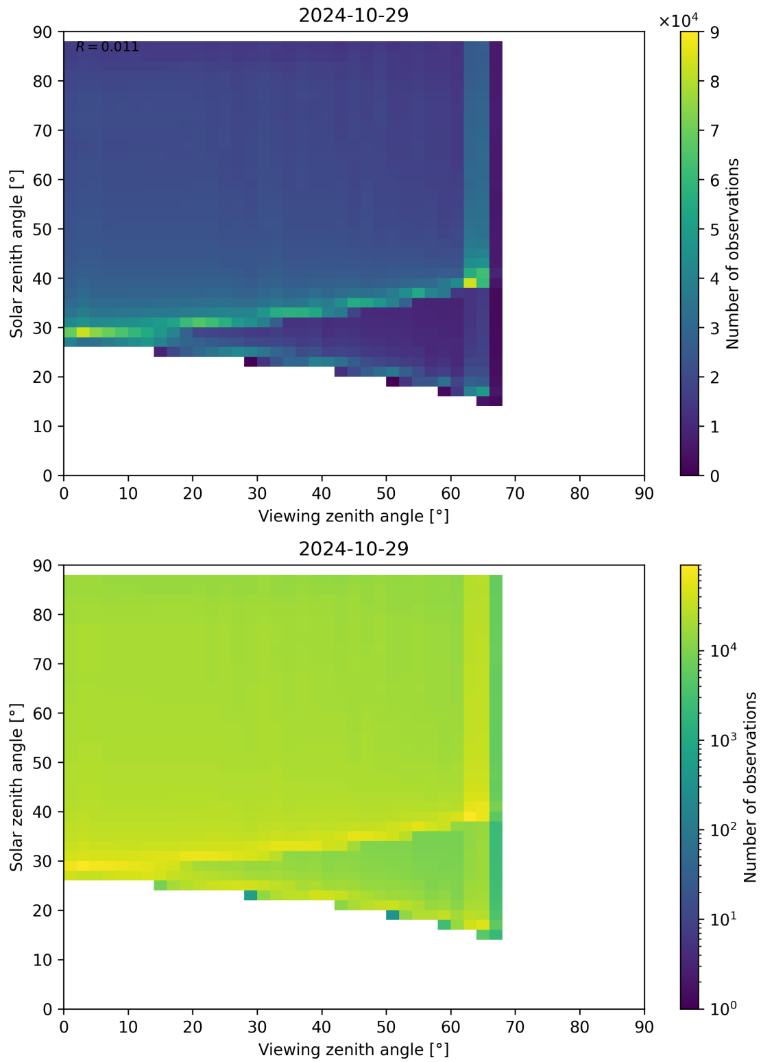
Figure 139: Scatter density plot of “Viewing zenith angle” against “Solar zenith angle” for 2024-10-29 to 2024-10-30.
