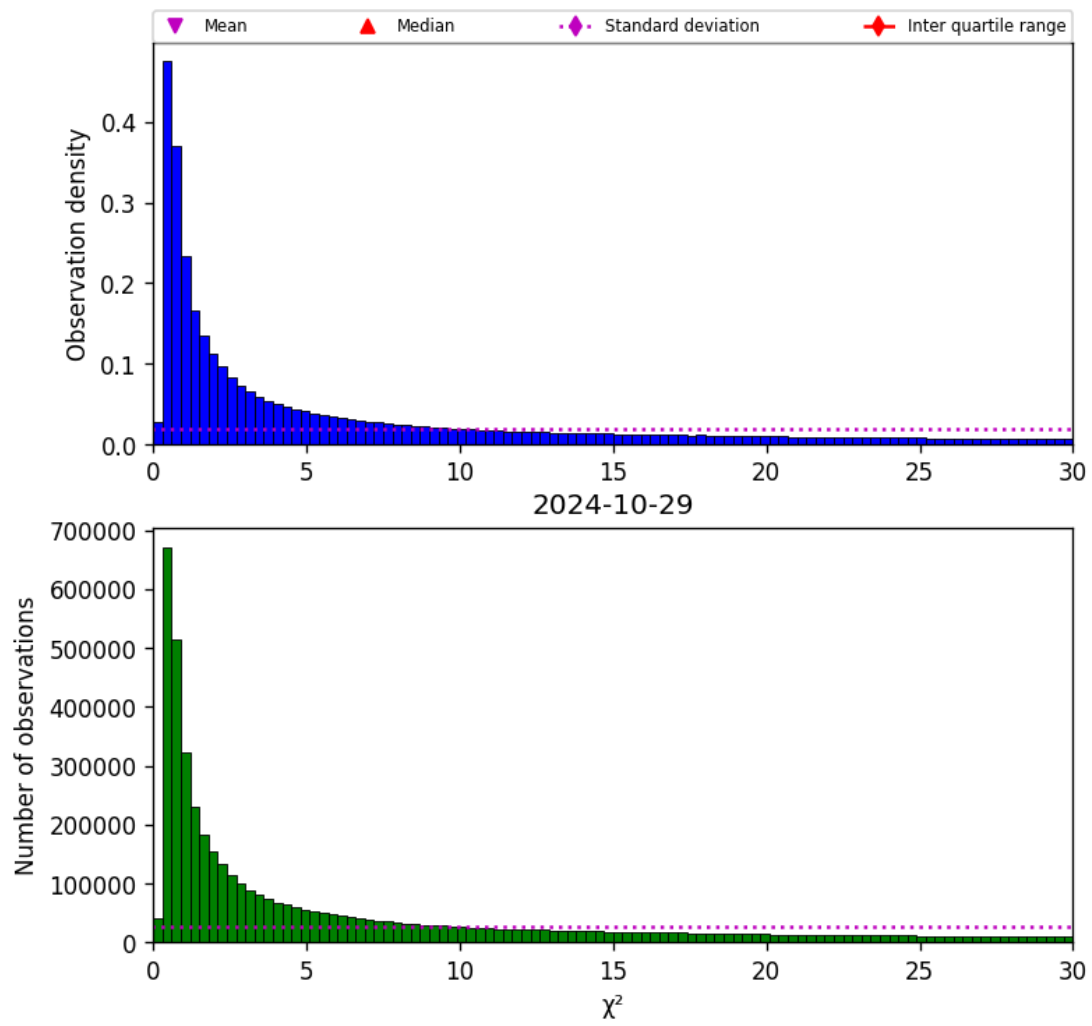
Figure 38: Histogram of “ \chi^2 ” for 2024-10-29 to 2024-10-30
