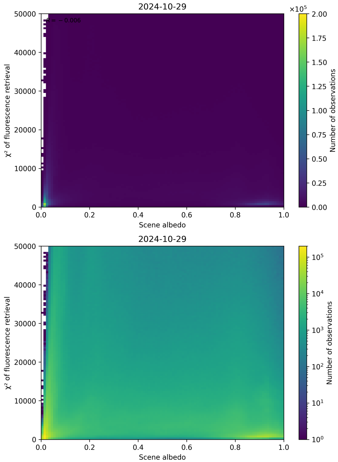
Figure 113: Scatter density plot of “Scene albedo” against “ \chi^2 of fluorescence retrieval” for 2024-10-29 to 2024-10-30.
