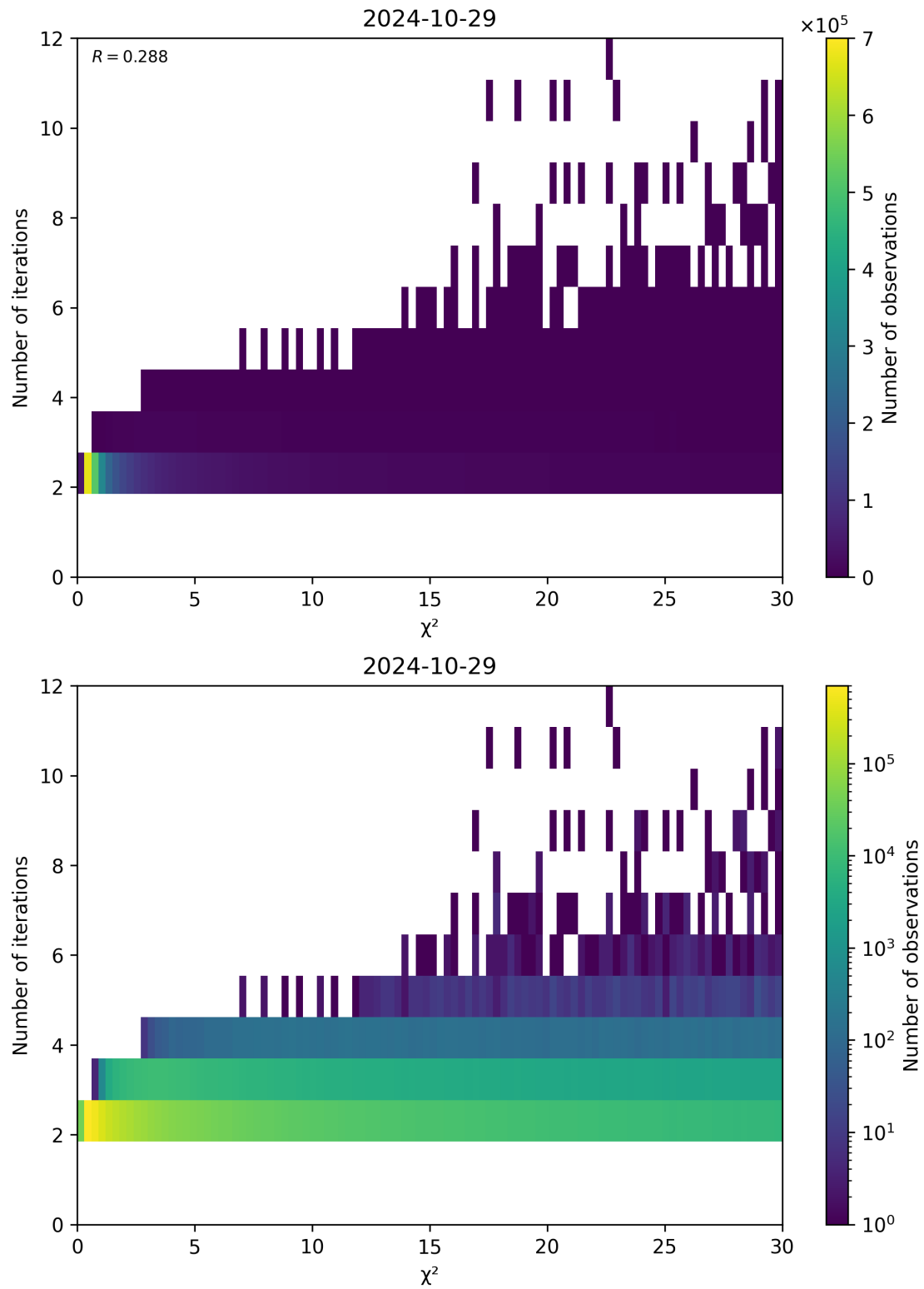
Figure 73: Scatter density plot of “ \chi^2 ” against “Number of iterations” for 2024-10-29 to 2024-10-30.
