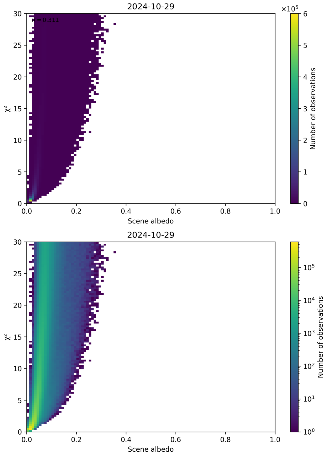
Figure 112: Scatter density plot of “Scene albedo” against “ \chi^2 ” for 2024-10-29 to 2024-10-30.
