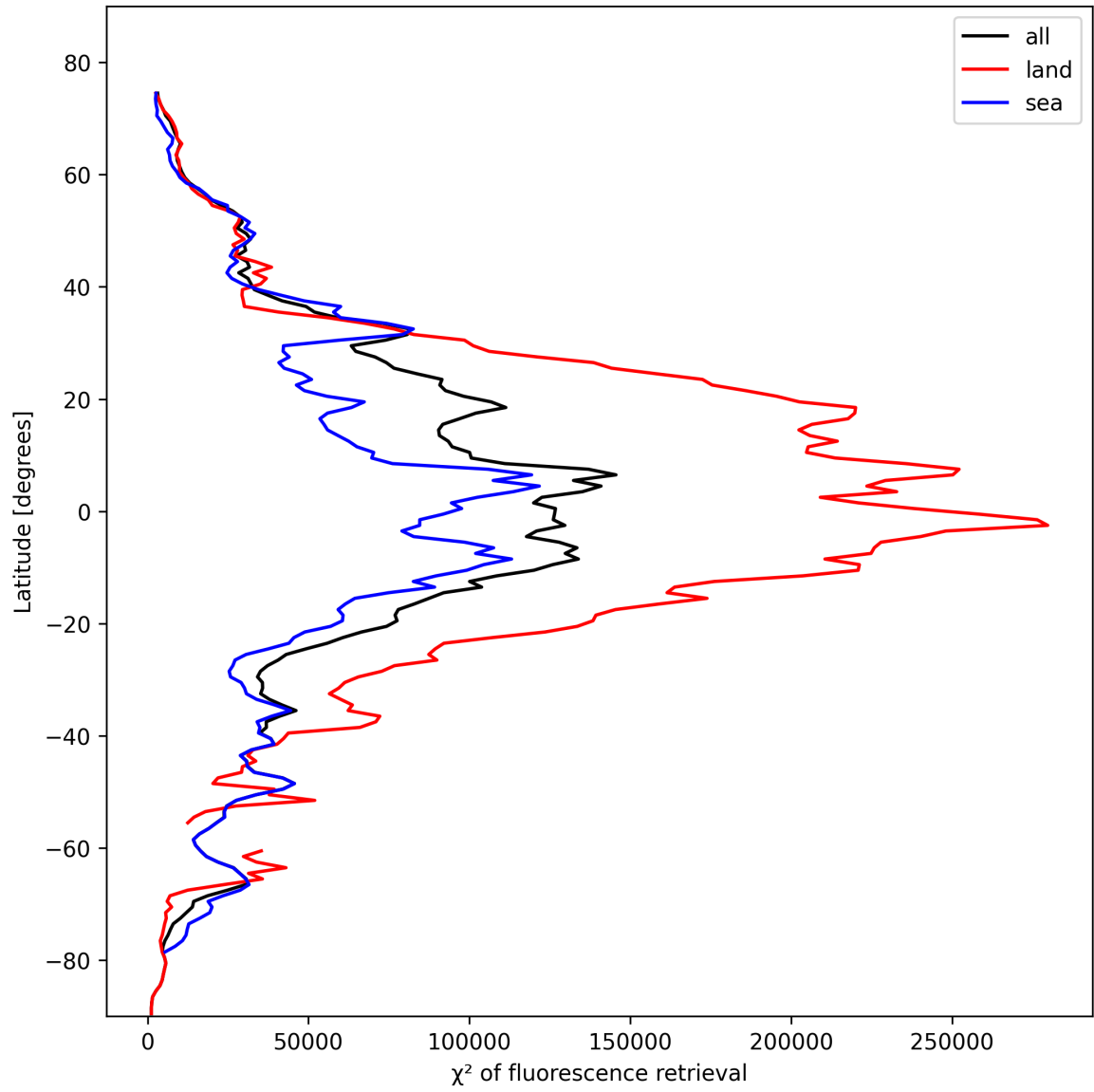
Figure 25: Zonal average of “ \chi^2 of fluorescence retrieval” for 2024-10-29 to 2024-10-30.
