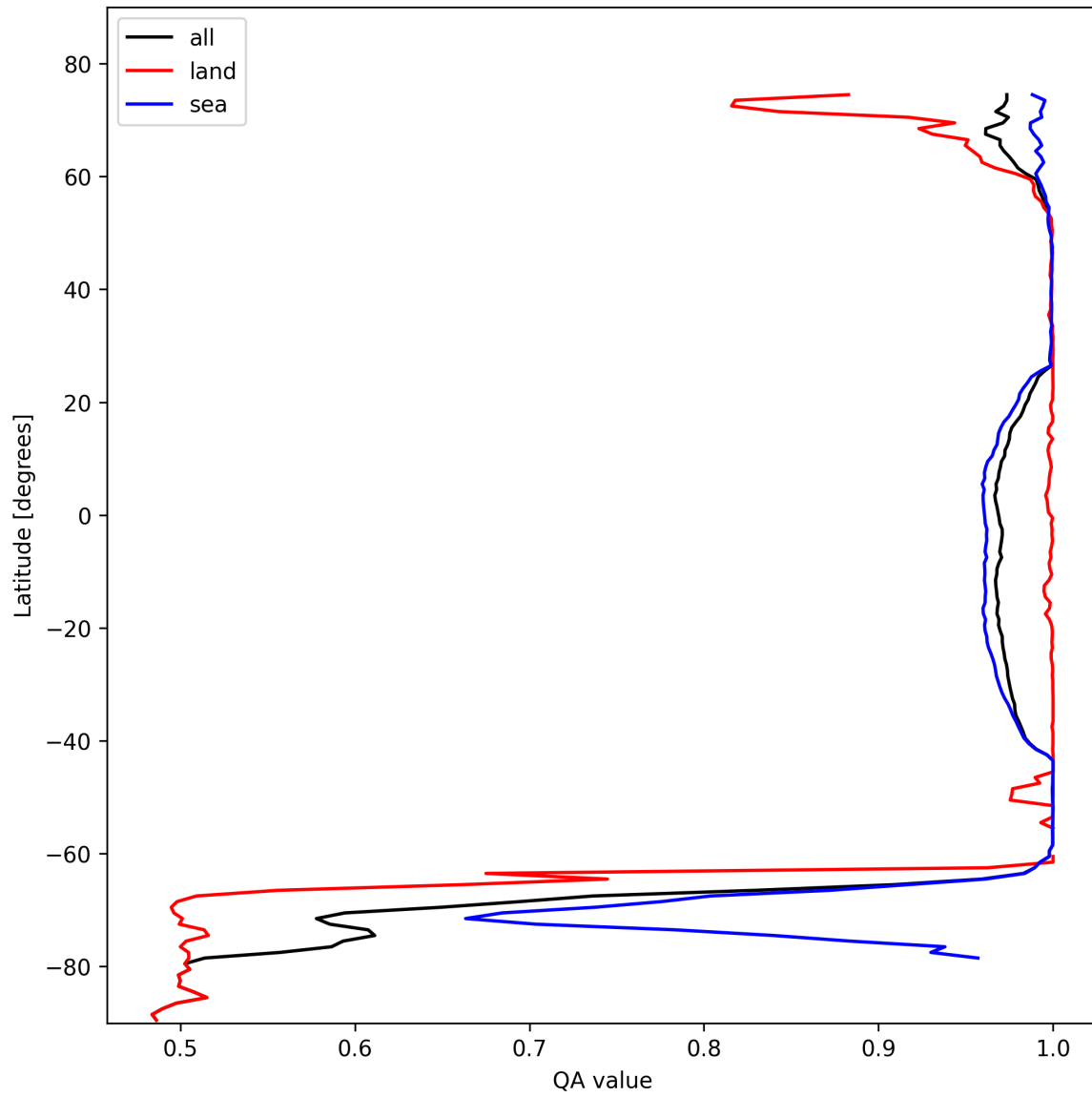
Figure 12: Zonal average of “QA value” for 2024-10-29 to 2024-10-30.
