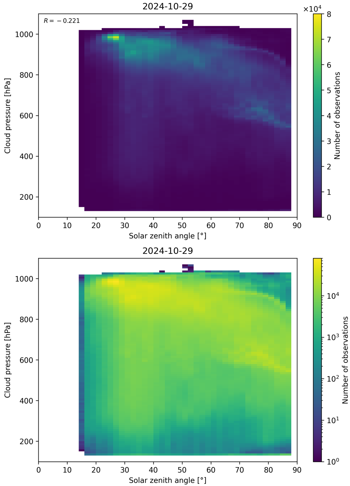
Figure 122: Scatter density plot of “Solar zenith angle” against “Cloud pressure” for 2024-10-29 to 2024-10-30.
