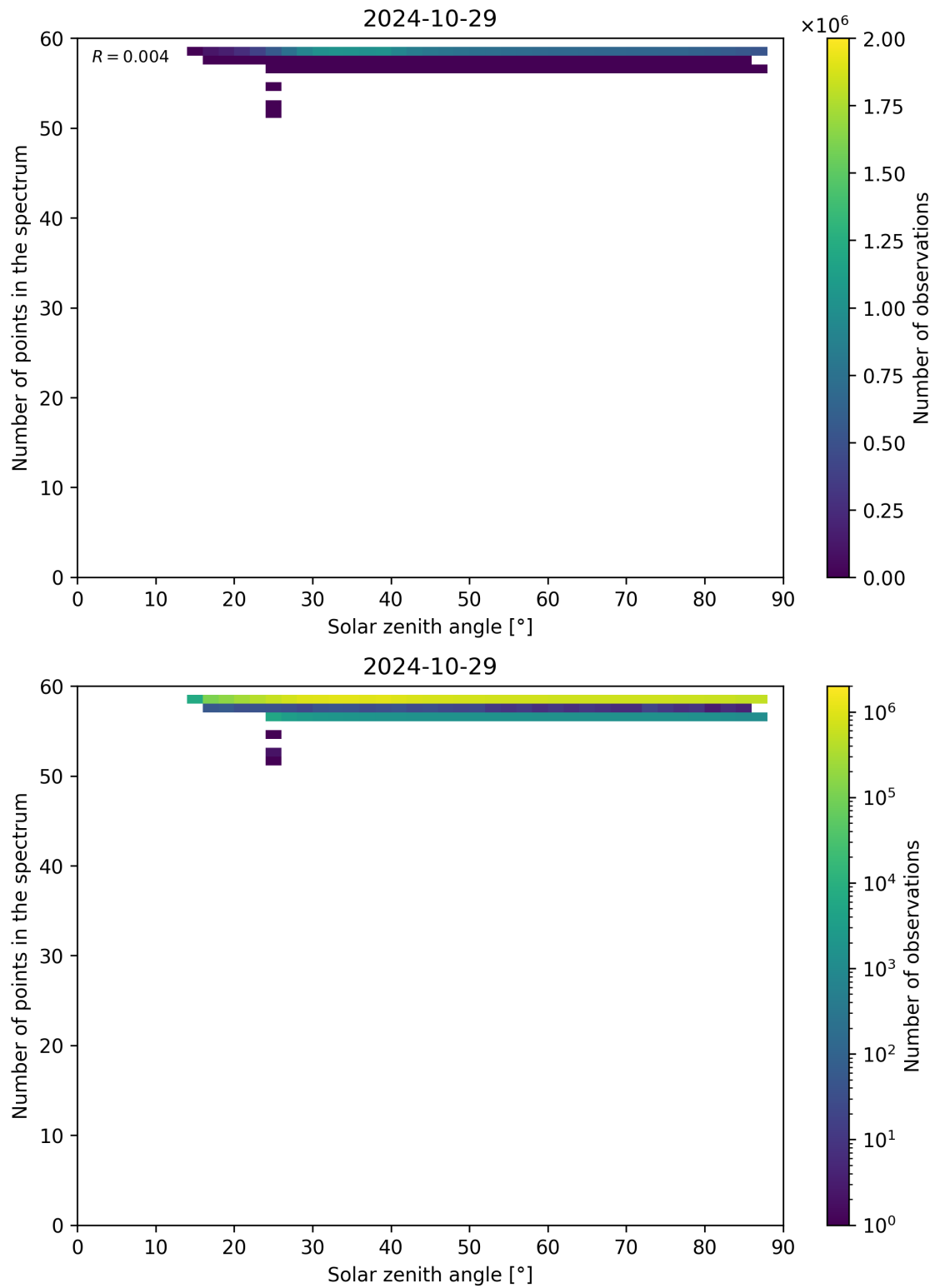
Figure 126: Scatter density plot of “Solar zenith angle” against “Number of points in the spectrum” for 2024-10-29 to 2024-10-30.
