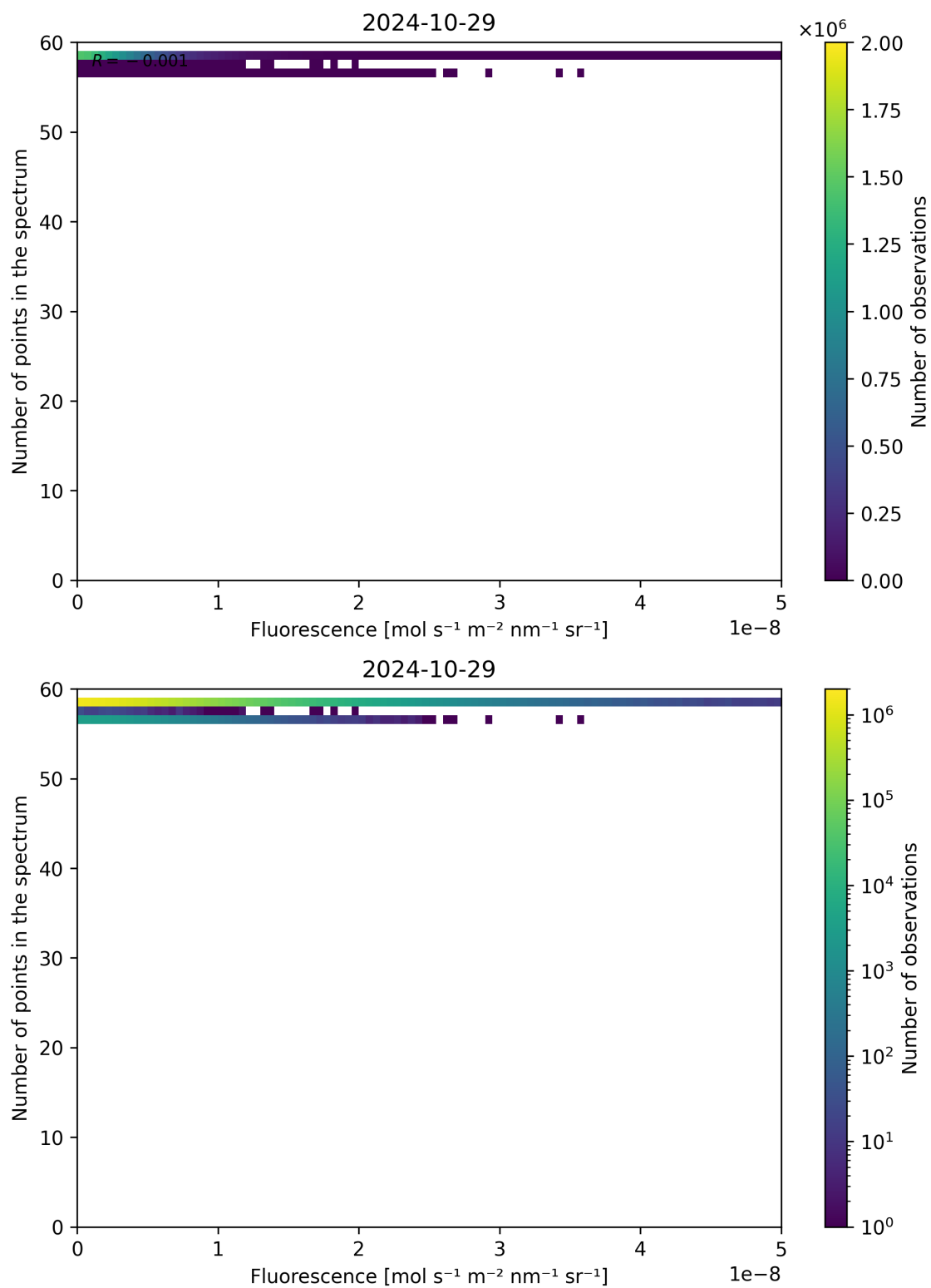
Figure 94: Scatter density plot of “Fluorescence” against “Number of points in the spectrum” for 2024-10-29 to 2024-10-30.
