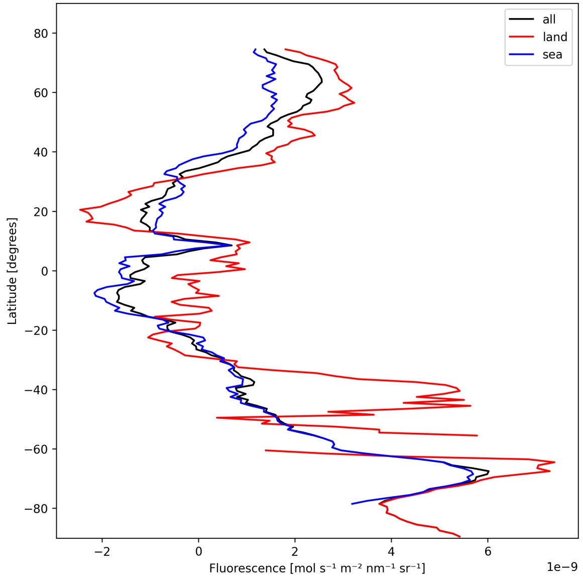
Figure 23: Zonal average of “Fluorescence” for 2024-10-29 to 2024-10-30.
