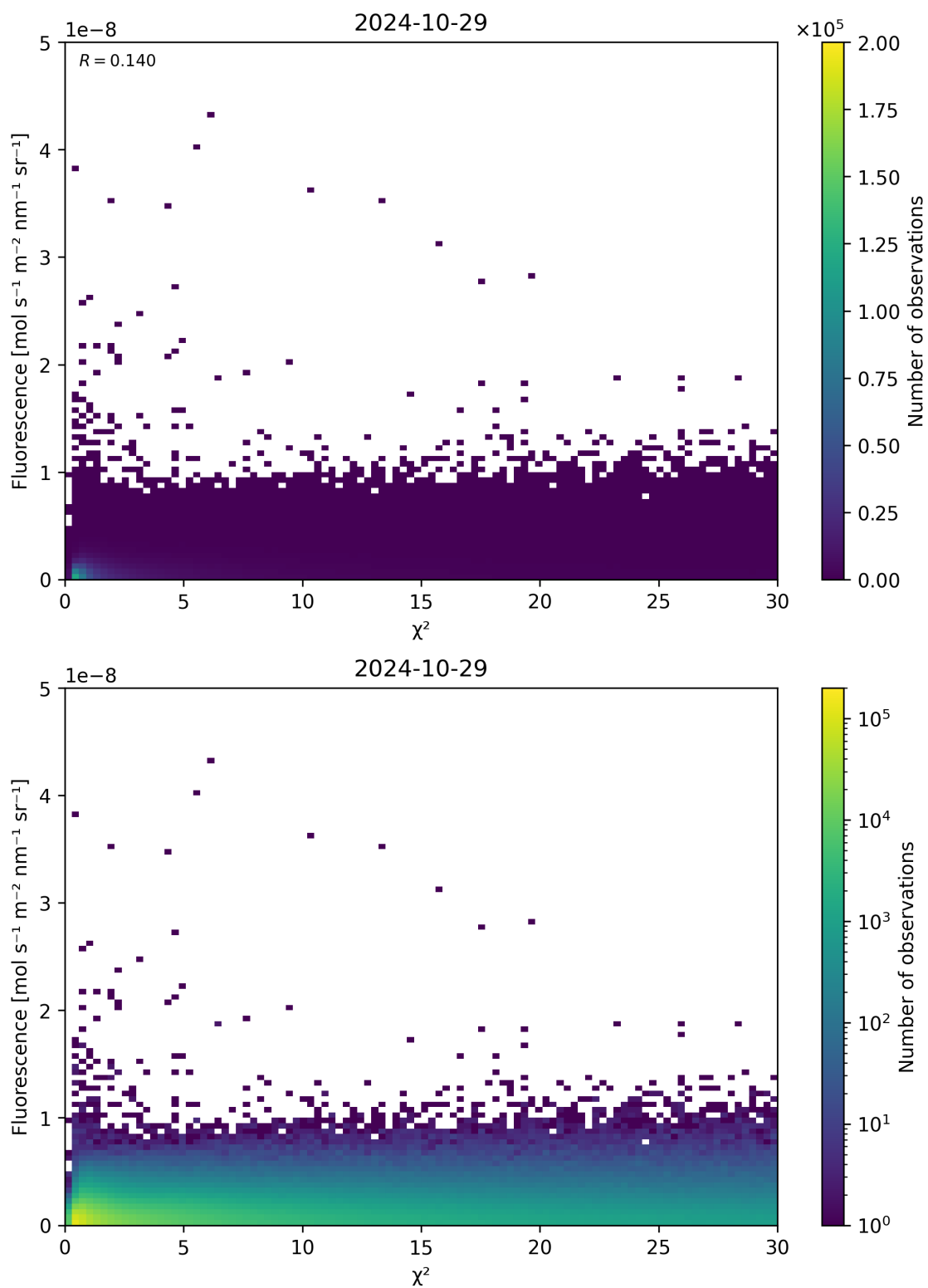
Figure 70: Scatter density plot of “ \chi^2 ” against “Fluorescence” for 2024-10-29 to 2024-10-30.
