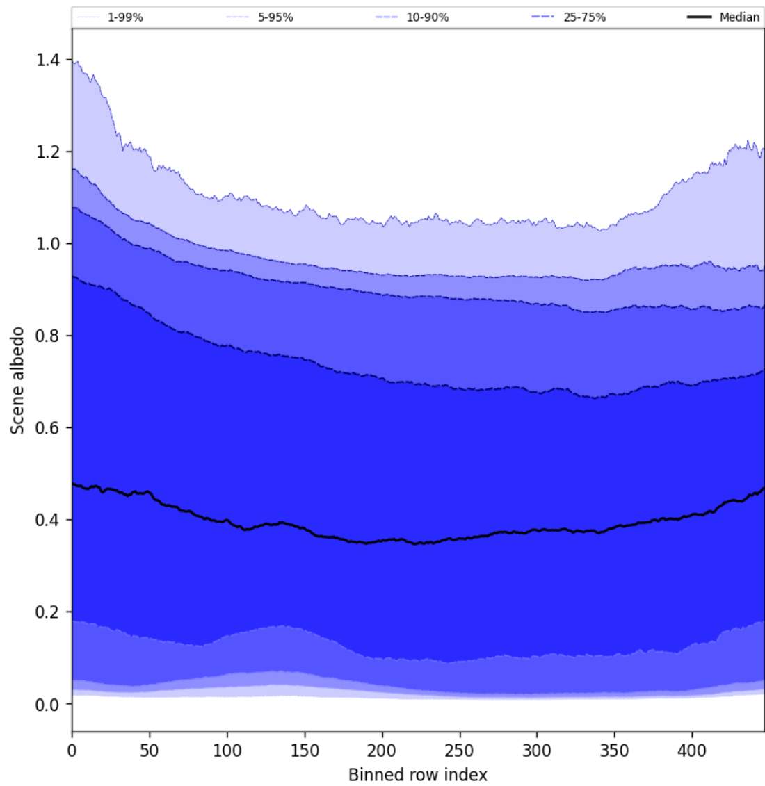
Figure 51: Along track statistics of “Scene albedo” for 2024-10-29 to 2024-10-30
