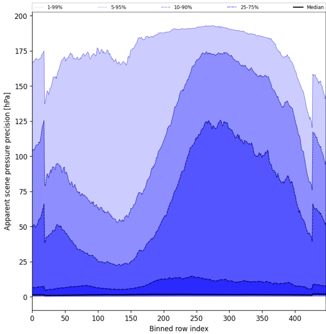
Figure 54: Along track statistics of “Apparent scene pressure precision” for 2024-10-29 to 2024-10-30
