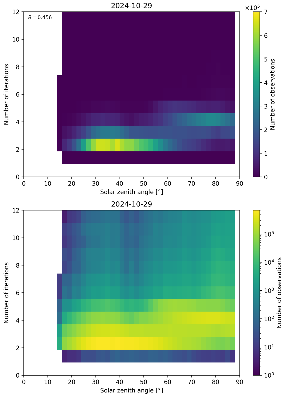
Figure 125: Scatter density plot of “Solar zenith angle” against “Number of iterations” for 2024-10-29 to 2024-10-30.
