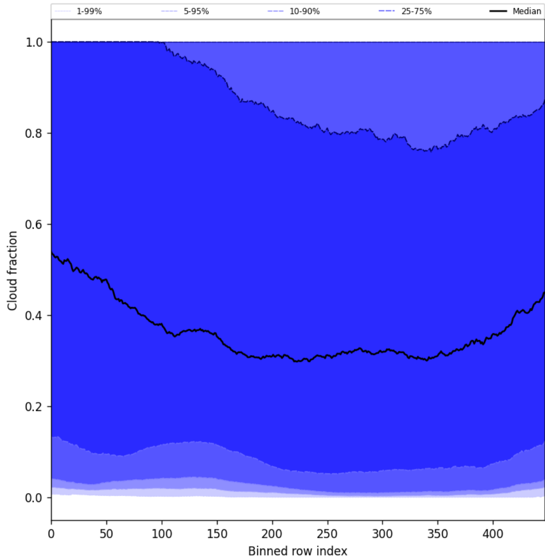
Figure 49: Along track statistics of “Cloud fraction” for 2024-10-29 to 2024-10-30
