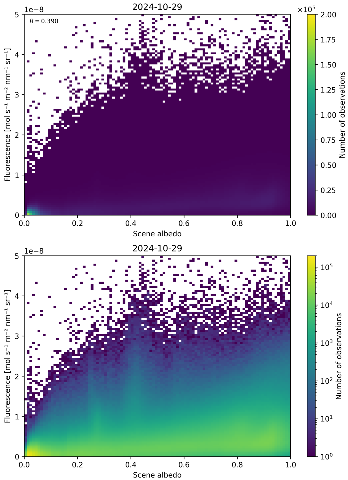
Figure 114: Scatter density plot of “Scene albedo” against “Fluorescence” for 2024-10-29 to 2024-10-30.
