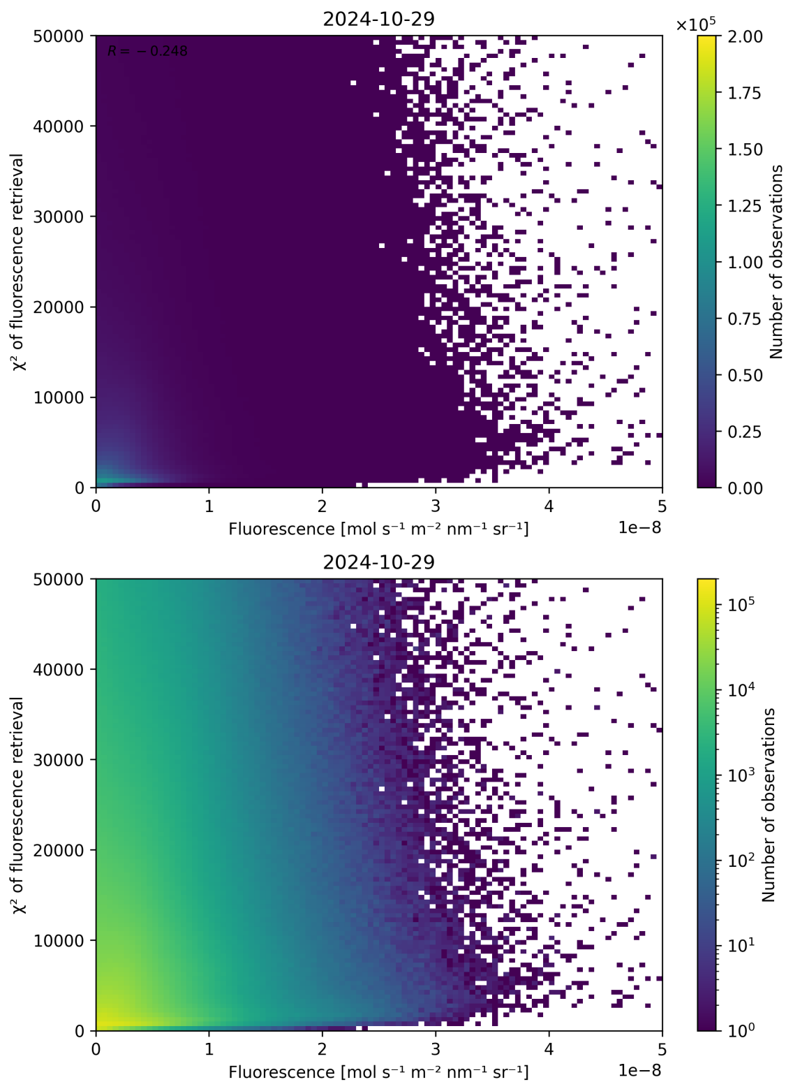
Figure 93: Scatter density plot of “Fluorescence” against “ \chi^2 of fluorescence retrieval” for 2024-10-29 to 2024-10-30.
