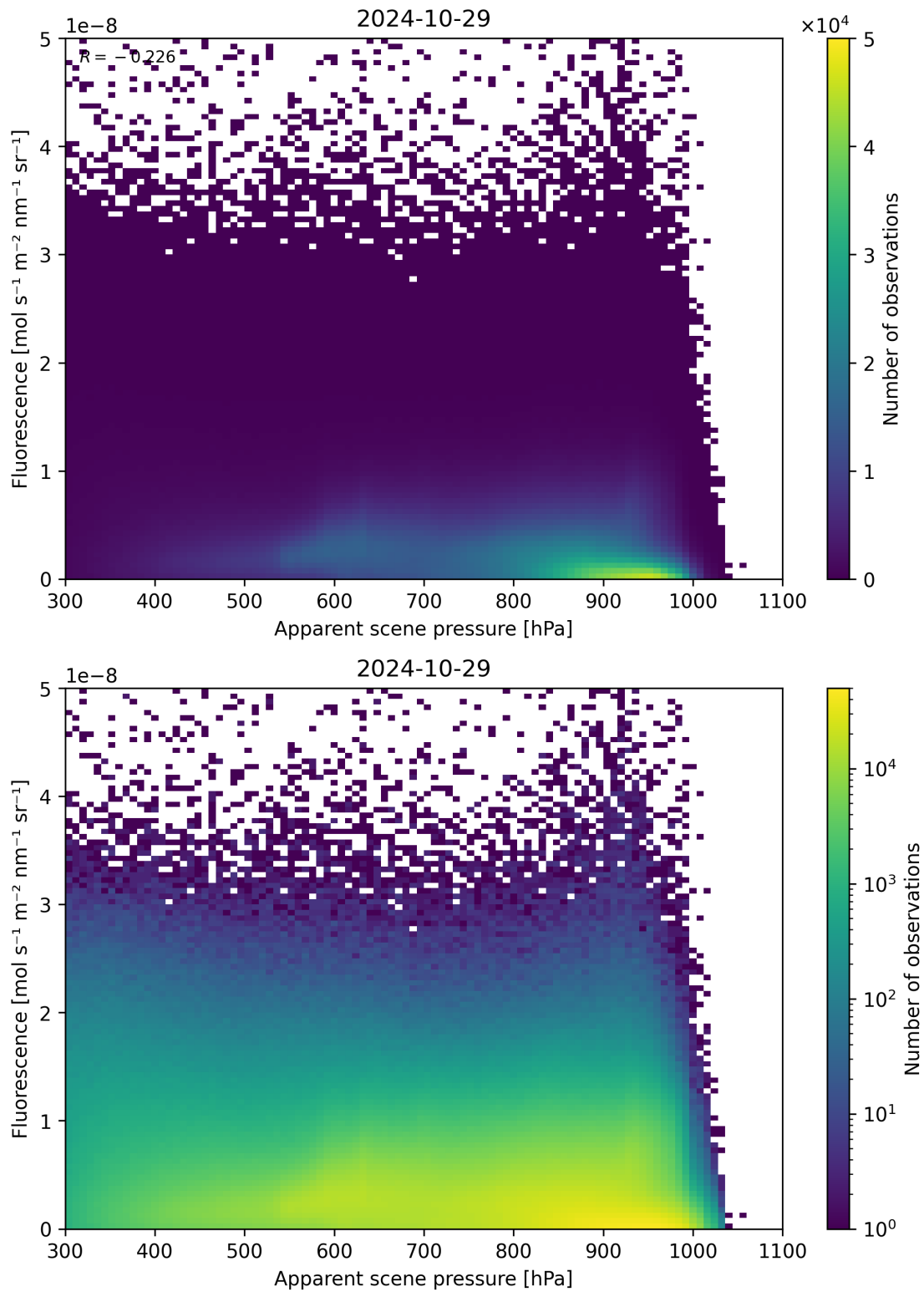
Figure 65: Scatter density plot of “Apparent scene pressure” against “Fluorescence” for 2024-10-29 to 2024-10-30.
