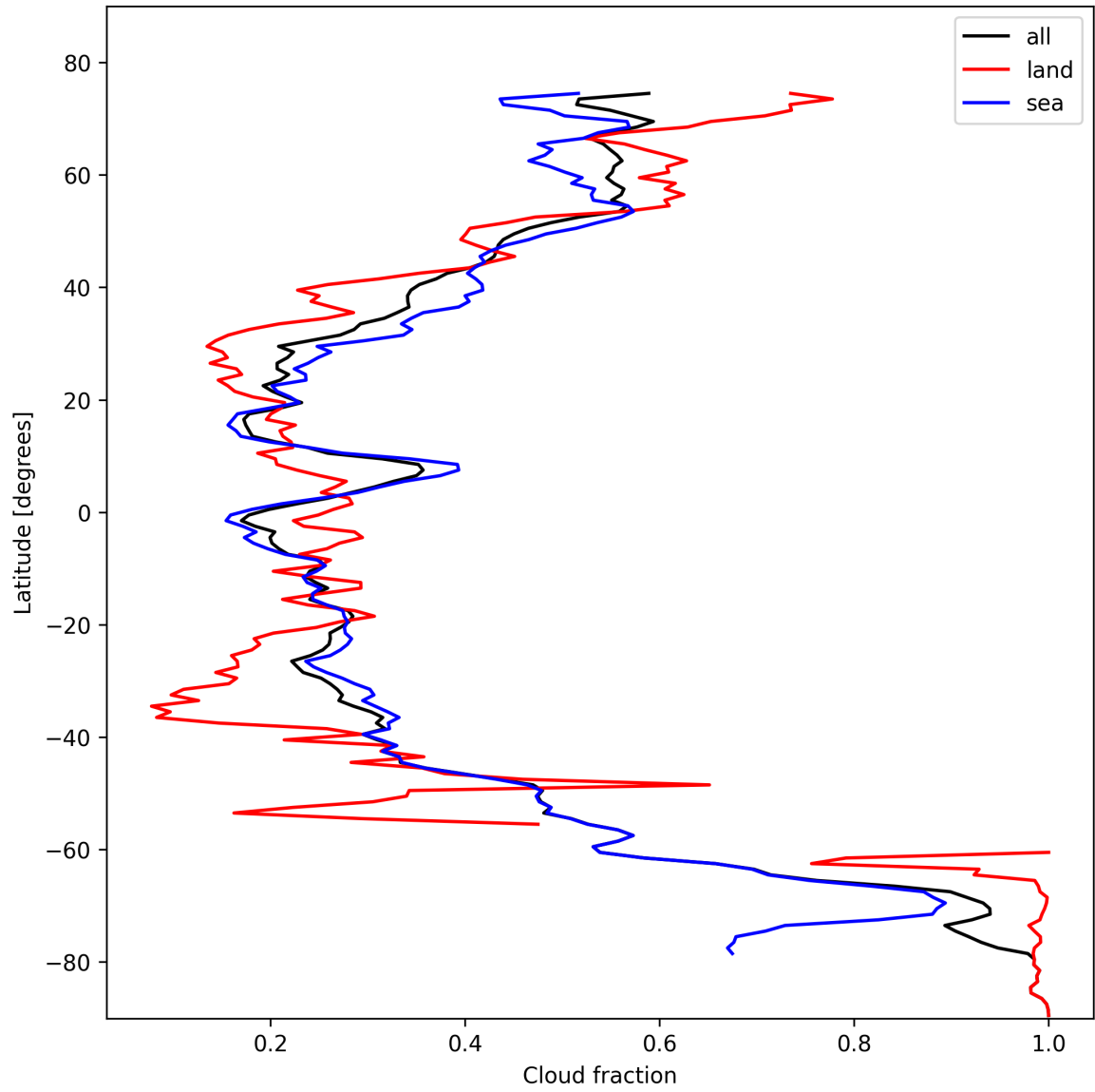
Figure 15: Zonal average of “Cloud fraction” for 2024-10-29 to 2024-10-30.
