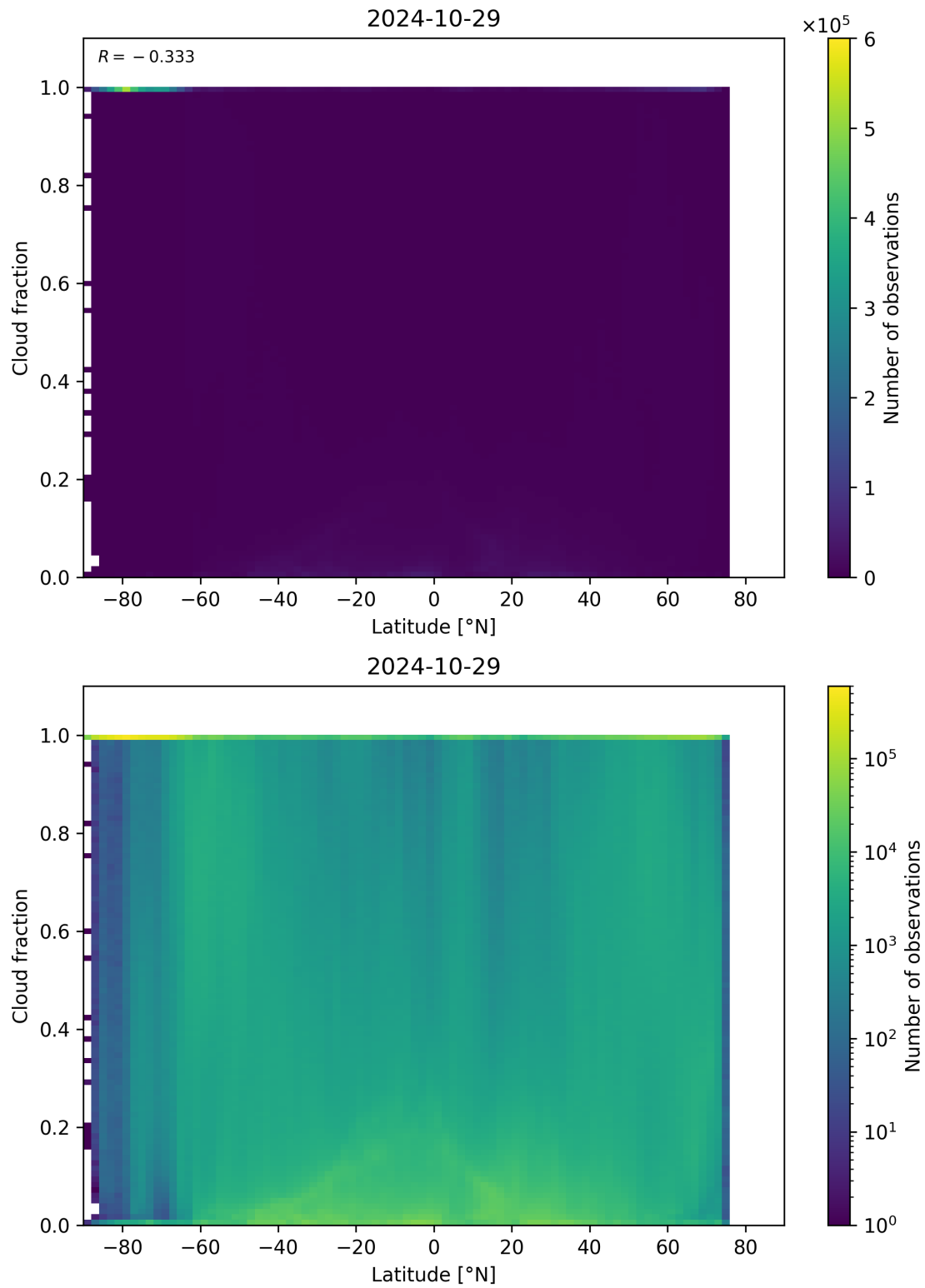
Figure 99: Scatter density plot of “Latitude” against “Cloud fraction” for 2024-10-29 to 2024-10-30.
