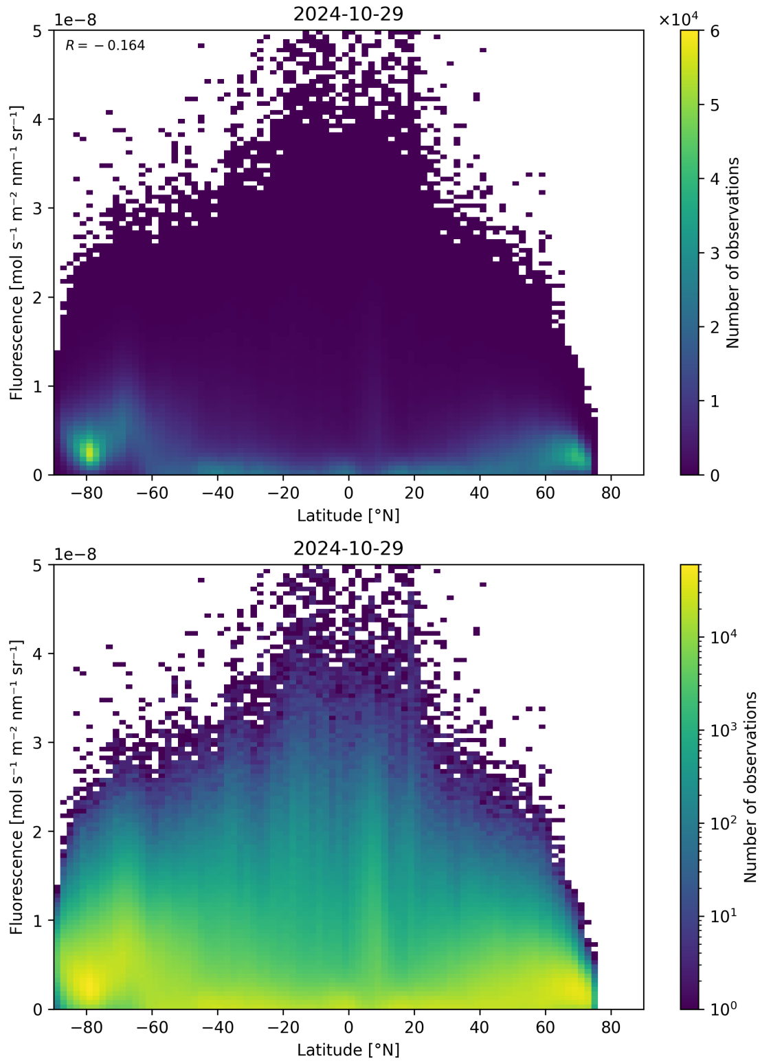
Figure 101: Scatter density plot of “Latitude” against “Fluorescence” for 2024-10-29 to 2024-10-30.
