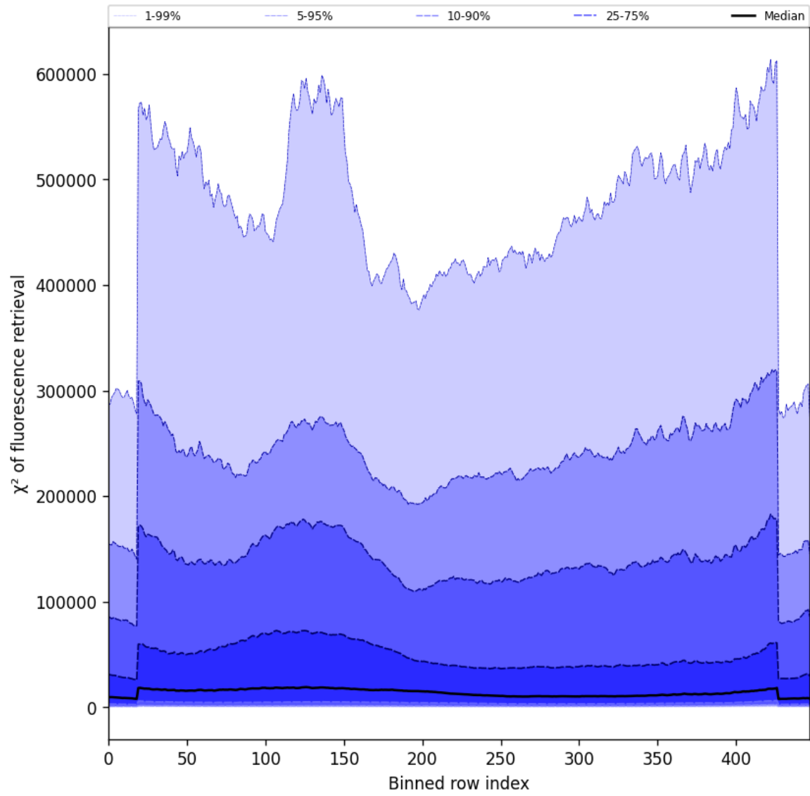
Figure 59: Along track statistics of “ \chi^2 of fluorescence retrieval” for 2024-10-29 to 2024-10-30
