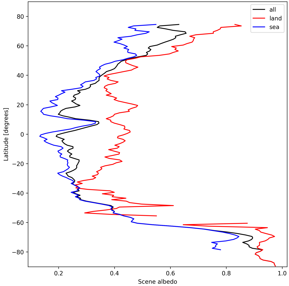
Figure 17: Zonal average of “Scene albedo” for 2024-10-29 to 2024-10-30.
