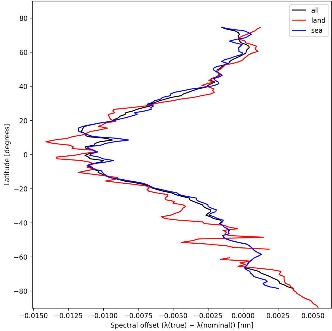
Figure 28: Zonal average of “Spectral offset ( \lambda_{\text{true}} - \lambda_{\text{nominal}} )” for 2024-10-29 to 2024-10-30.
