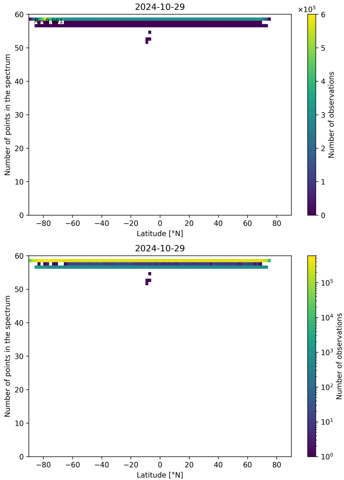
Figure 103: Scatter density plot of “Latitude” against “Number of points in the spectrum” for 2024-10-29 to 2024-10-30.
