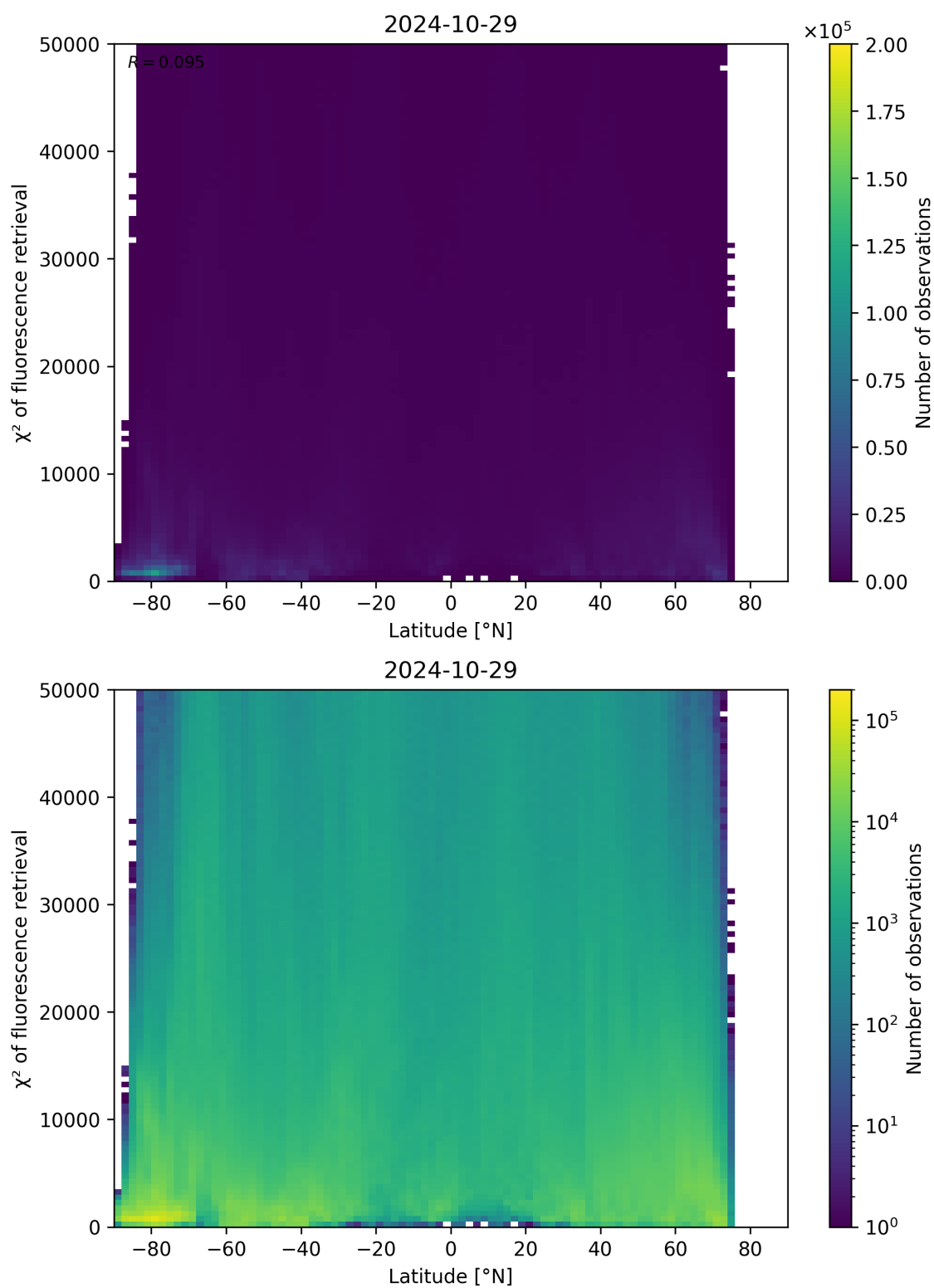
Figure 98: Scatter density plot of “Latitude” against “ \chi^2 of fluorescence retrieval” for 2024-10-29 to 2024-10-30.
