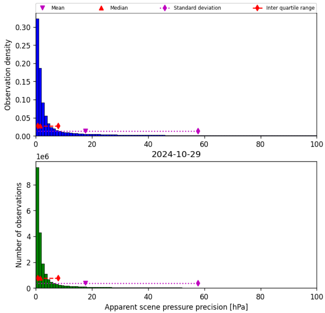
Figure 37: Histogram of “Apparent scene pressure precision” for 2024-10-29 to 2024-10-30
