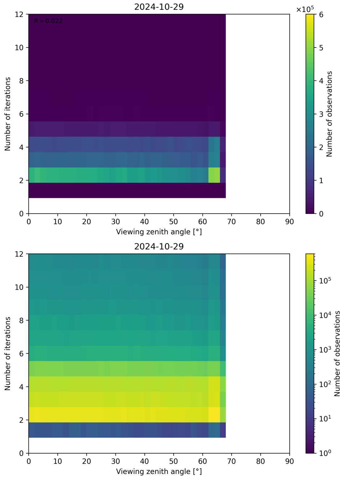
Figure 136: Scatter density plot of “Viewing zenith angle” against “Number of iterations” for 2024-10-29 to 2024-10-30.
