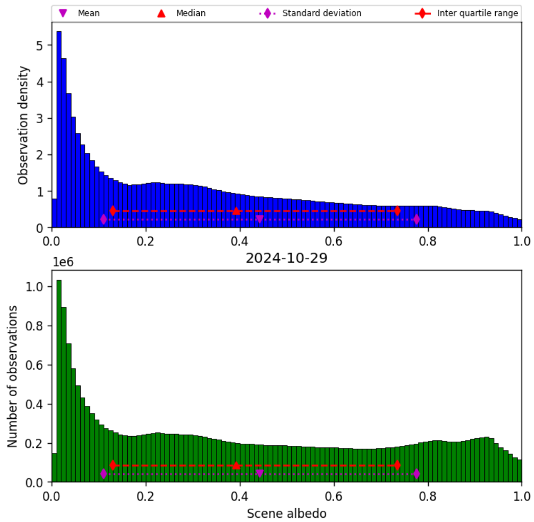
Figure 34: Histogram of “Scene albedo” for 2024-10-29 to 2024-10-30
