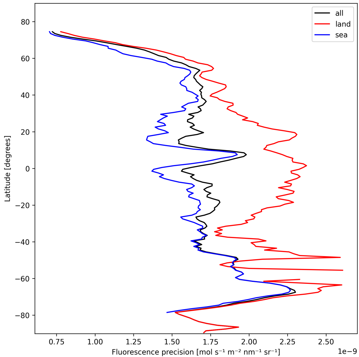
Figure 24: Zonal average of “Fluorescence precision” for 2024-10-29 to 2024-10-30.
