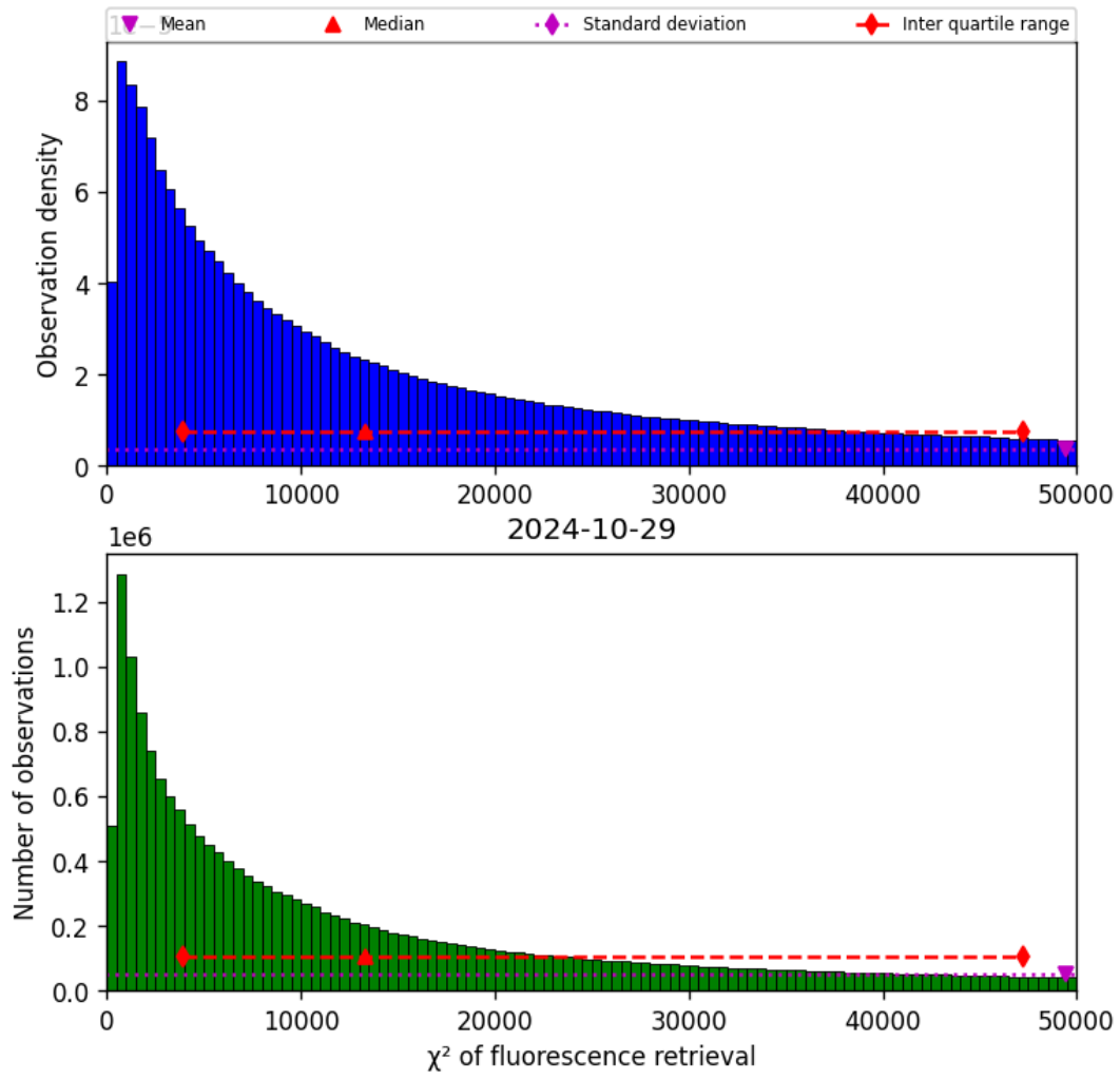
Figure 42: Histogram of “ \chi^2 of fluorescence retrieval” for 2024-10-29 to 2024-10-30
