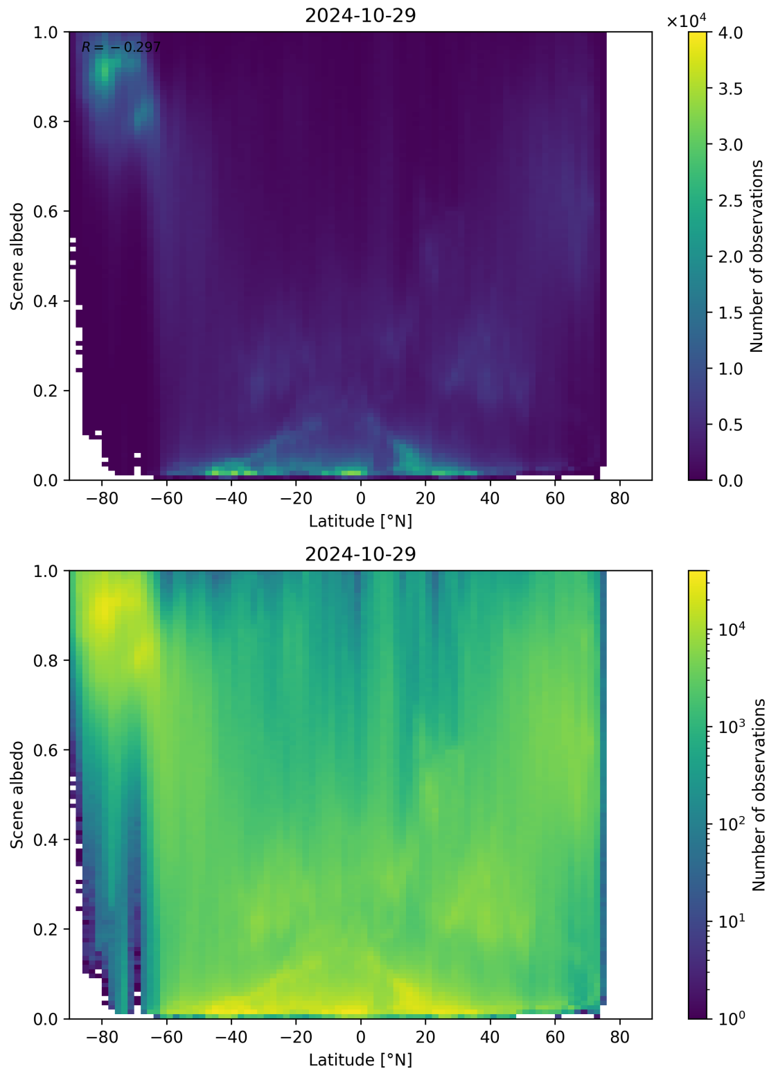
Figure 104: Scatter density plot of “Latitude” against “Scene albedo” for 2024-10-29 to 2024-10-30.
