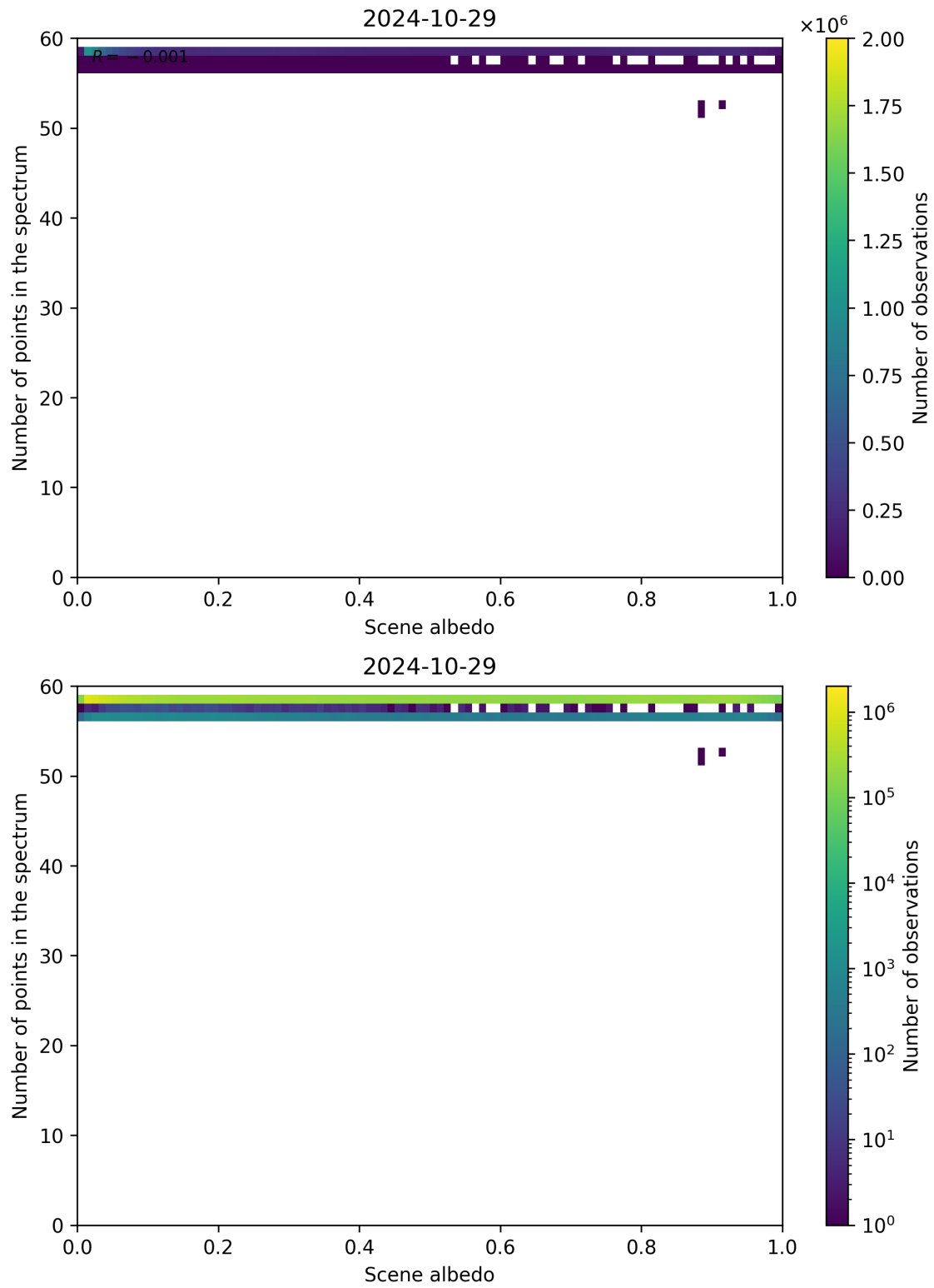
Figure 116: Scatter density plot of “Scene albedo” against “Number of points in the spectrum” for 2024-10-29 to 2024-10-30.
