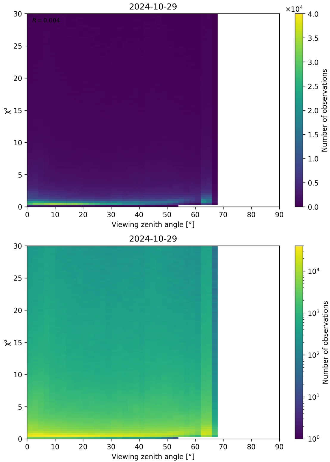
Figure 130: Scatter density plot of “Viewing zenith angle” against “ \chi^2 ” for 2024-10-29 to 2024-10-30.
