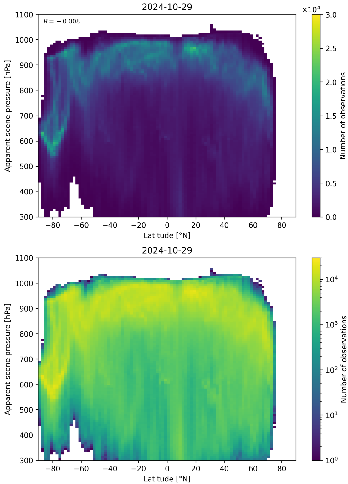
Figure 96: Scatter density plot of “Latitude” against “Apparent scene pressure” for 2024-10-29 to 2024-10-30.
