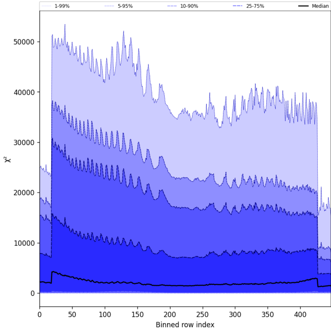
Figure 55: Along track statistics of “ \chi^2 ” for 2024-10-29 to 2024-10-30
