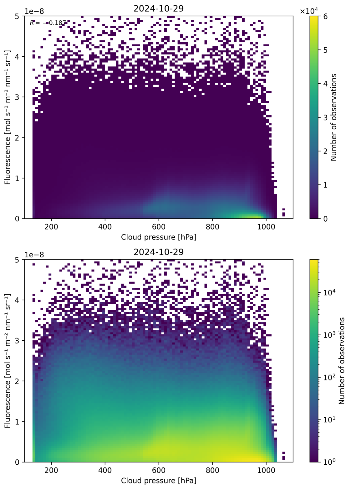
Figure 88: Scatter density plot of “Cloud pressure” against “Fluorescence” for 2024-10-29 to 2024-10-30.
