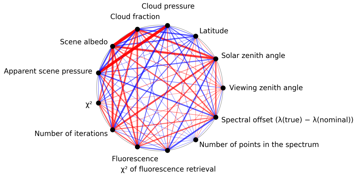
Figure 1: Map of correlation graph for 2024-10-29 to 2024-10-30.
