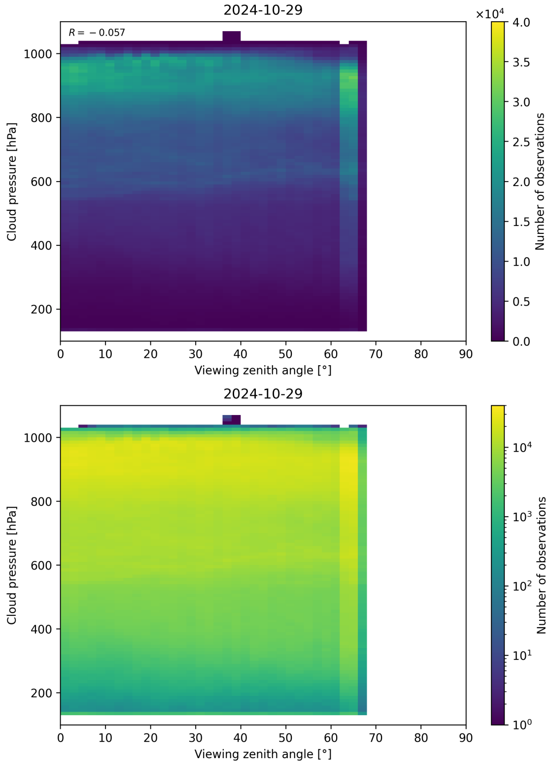
Figure 133: Scatter density plot of “Viewing zenith angle” against “Cloud pressure” for 2024-10-29 to 2024-10-30.
