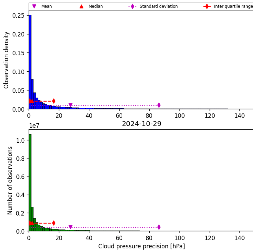
Figure 31: Histogram of “Cloud pressure precision” for 2024-10-29 to 2024-10-30
