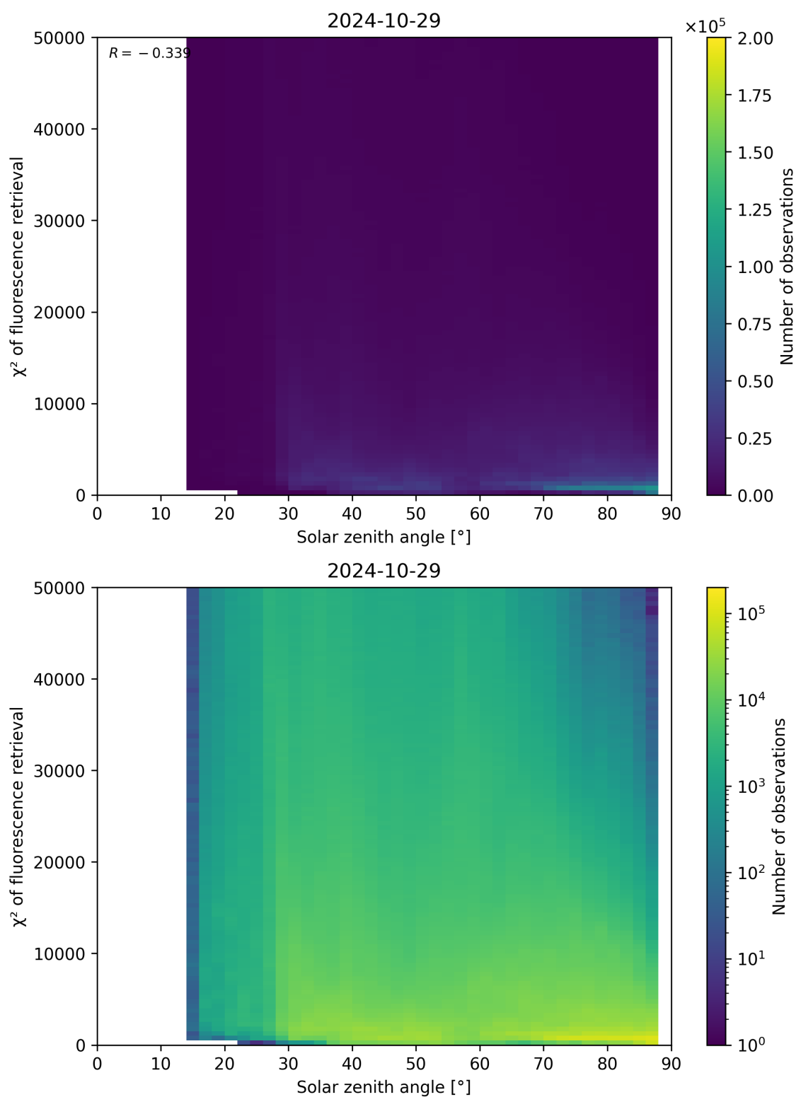
Figure 120: Scatter density plot of “Solar zenith angle” against “ \chi^2 of fluorescence retrieval” for 2024-10-29 to 2024-10-30.
