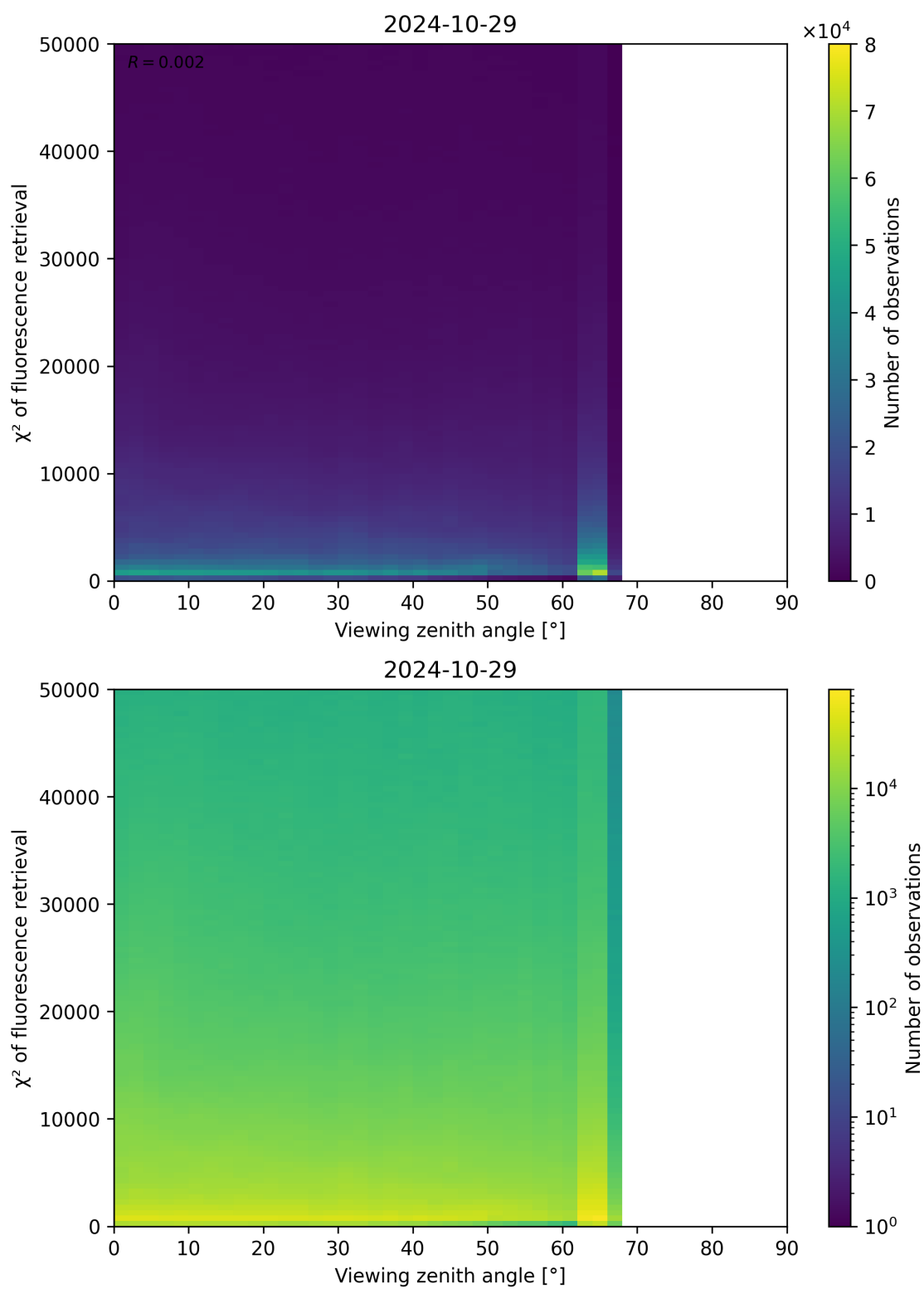
Figure 131: Scatter density plot of “Viewing zenith angle” against “ \chi^2 of fluorescence retrieval” for 2024-10-29 to 2024-10-30.
