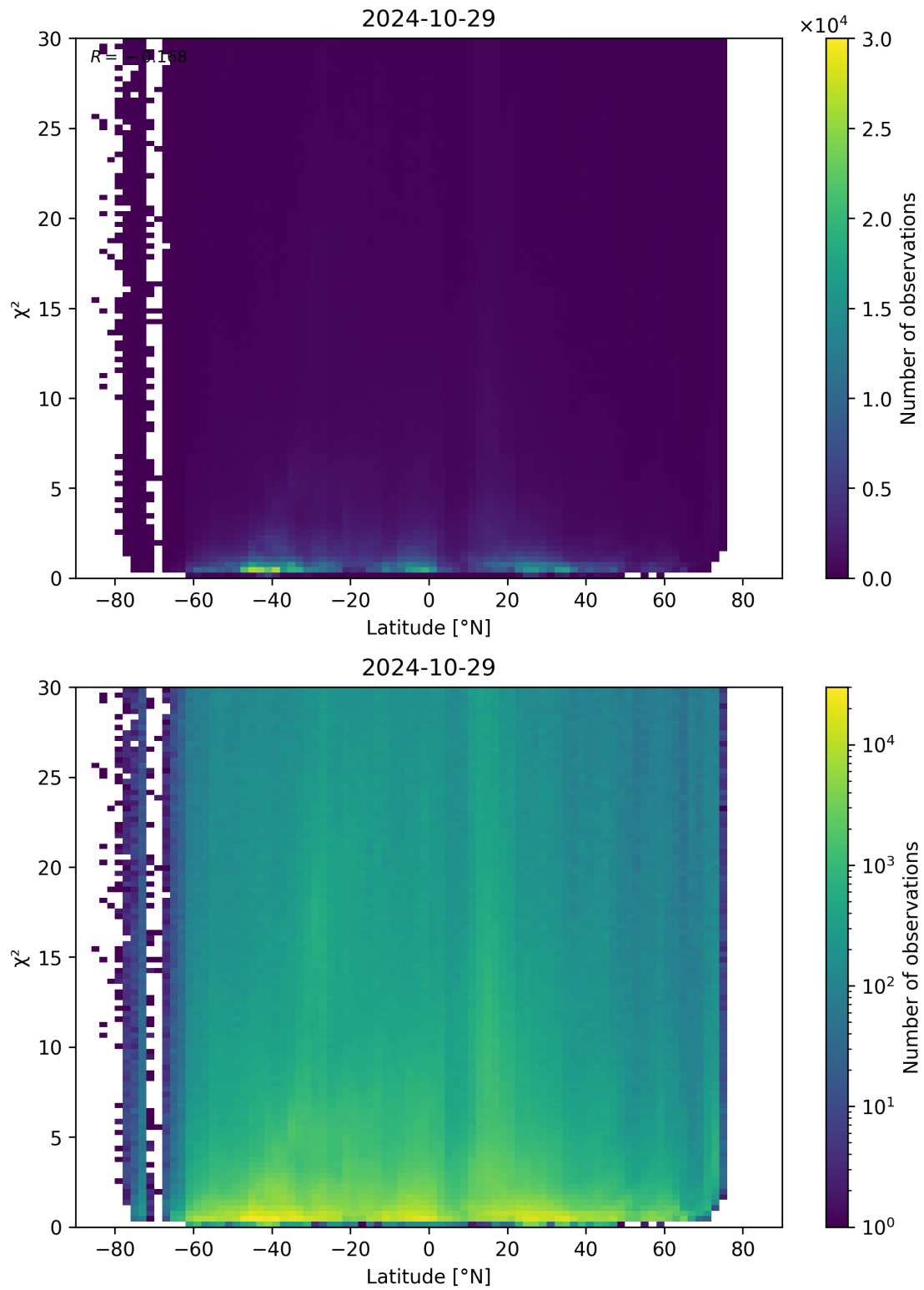
Figure 97: Scatter density plot of “Latitude” against “ \chi^2 ” for 2024-10-29 to 2024-10-30.
