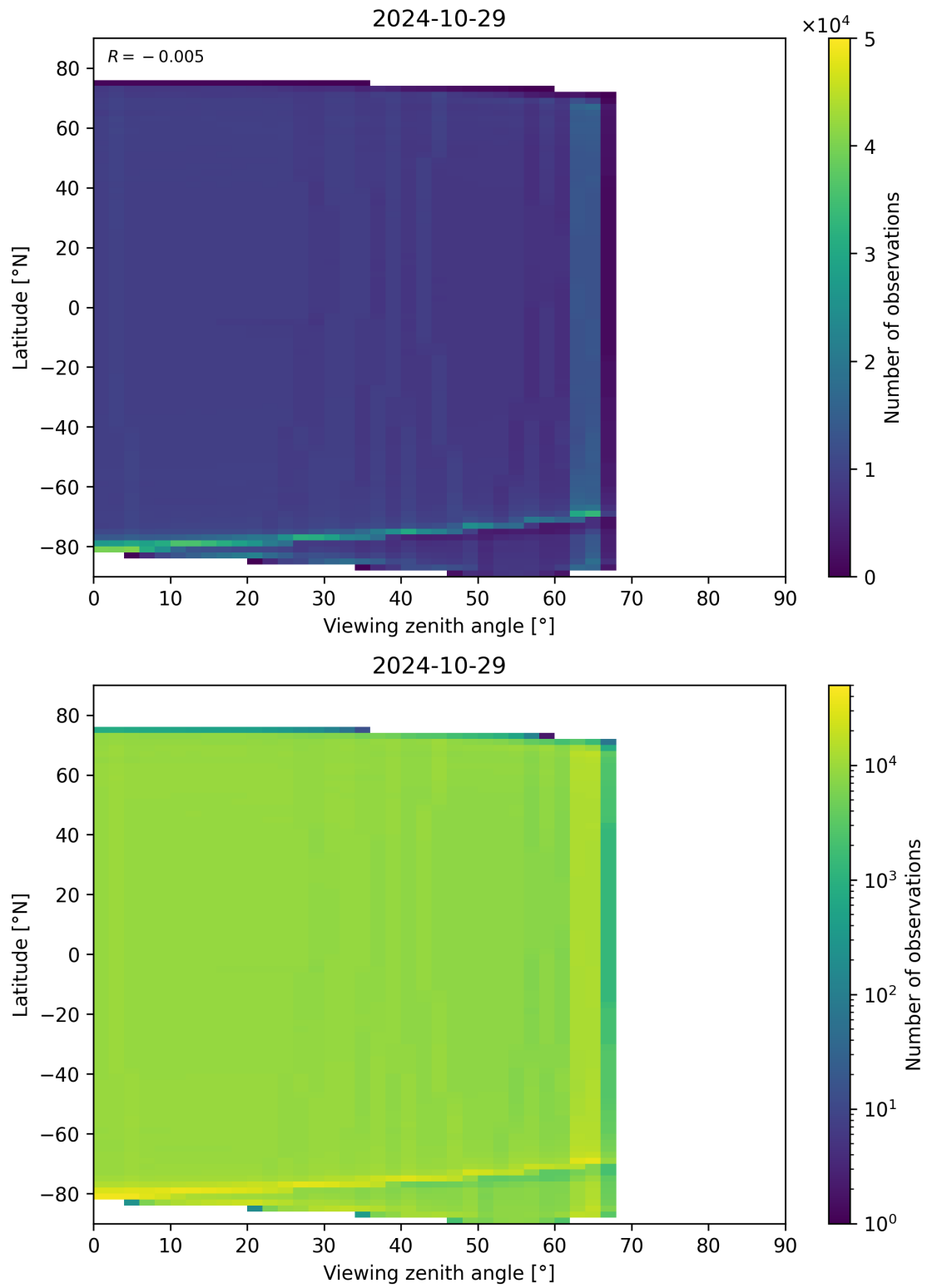
Figure 135: Scatter density plot of “Viewing zenith angle” against “Latitude” for 2024-10-29 to 2024-10-30.
