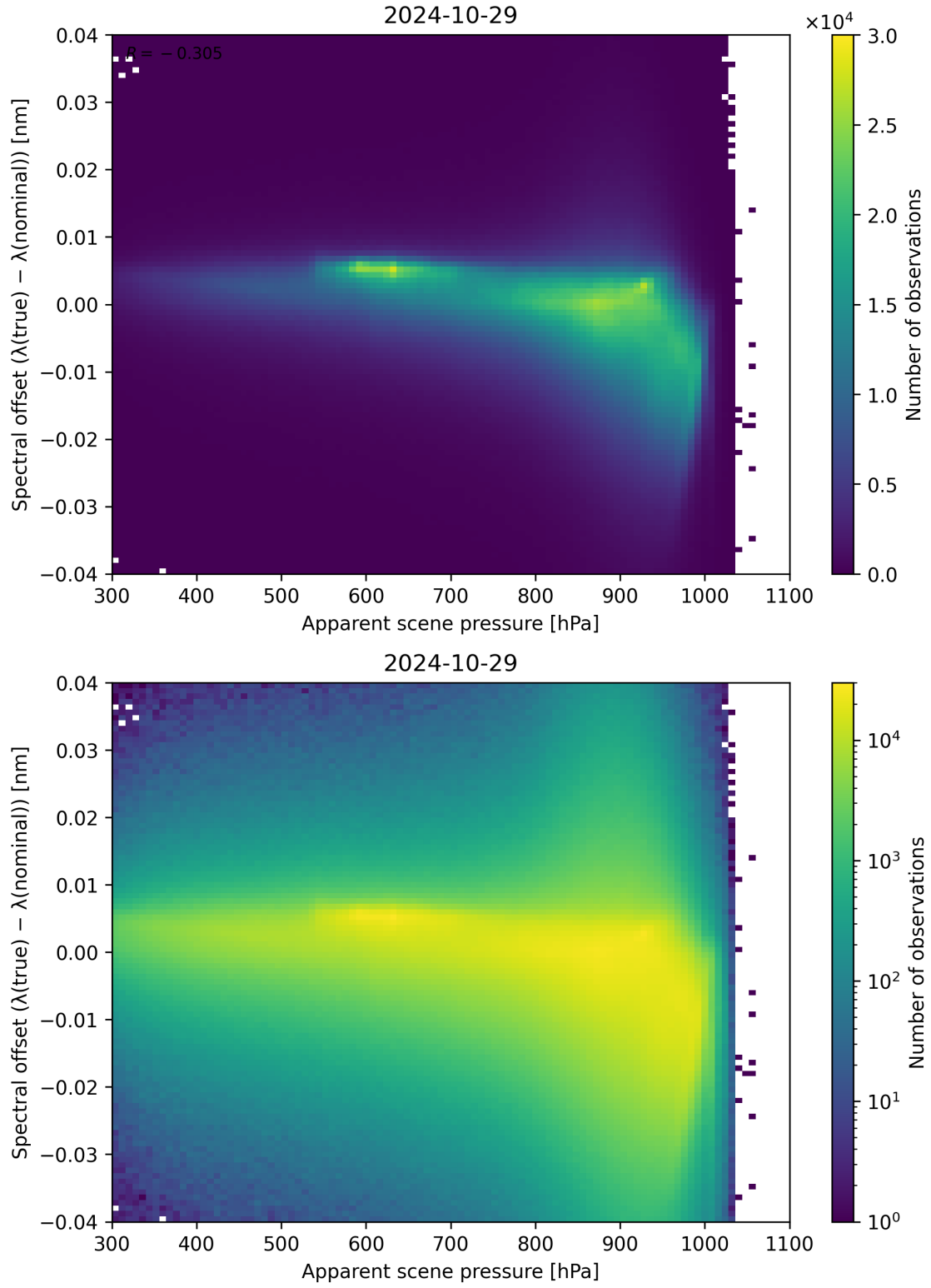
Figure 68: Scatter density plot of “Apparent scene pressure” against “Spectral offset ( \lambda_{\text{true}} - \lambda_{\text{nominal}} )” for 2024-10-29 to 2024-10-30.
