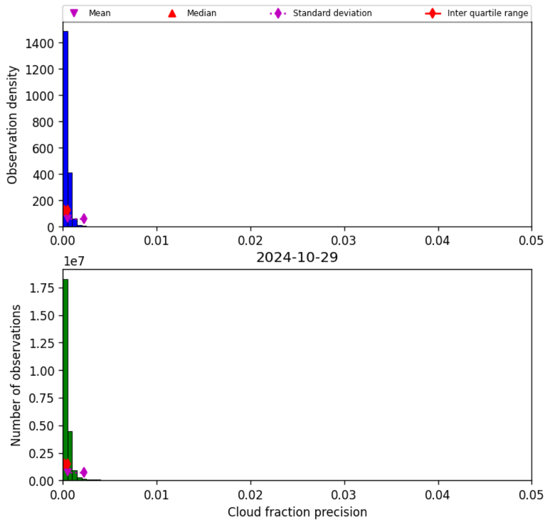
Figure 33: Histogram of “Cloud fraction precision” for 2024-10-29 to 2024-10-30
