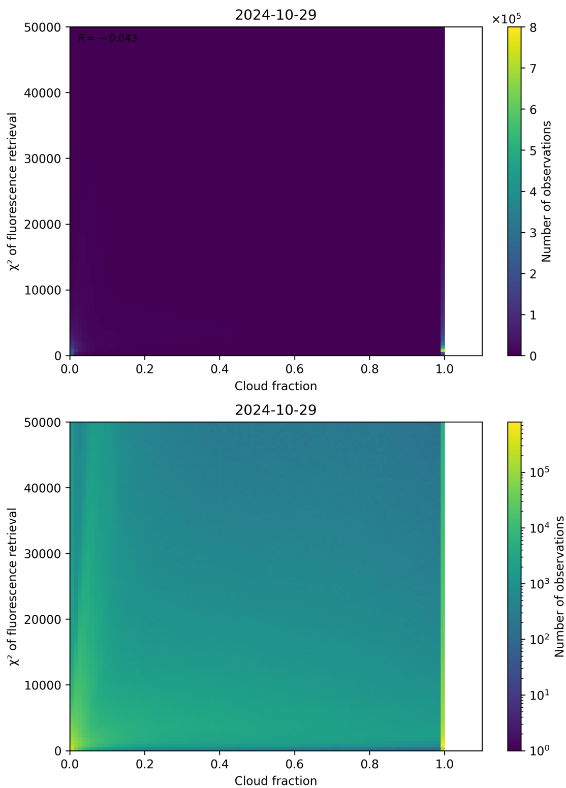
Figure 78: Scatter density plot of “Cloud fraction” against “ \chi^2 of fluorescence retrieval” for 2024-10-29 to 2024-10-30.
