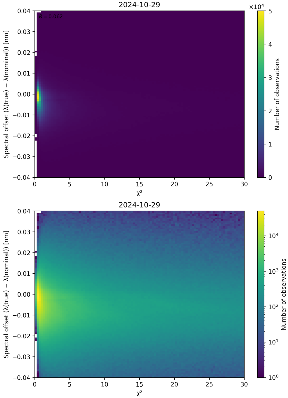
Figure 75: Scatter density plot of “ \chi^2 ” against “Spectral offset ( \lambda_{\text{true}} - \lambda_{\text{nominal}} )” for 2024-10-29 to 2024-10-30.
