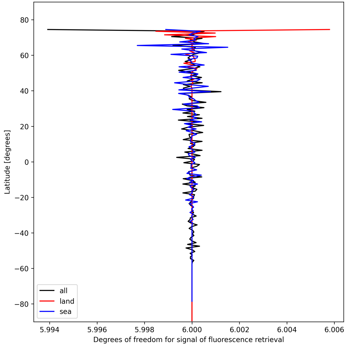
Figure 26: Zonal average of “Degrees of freedom for signal of fluorescence retrieval” for 2024-10-29 to 2024-10-30.
