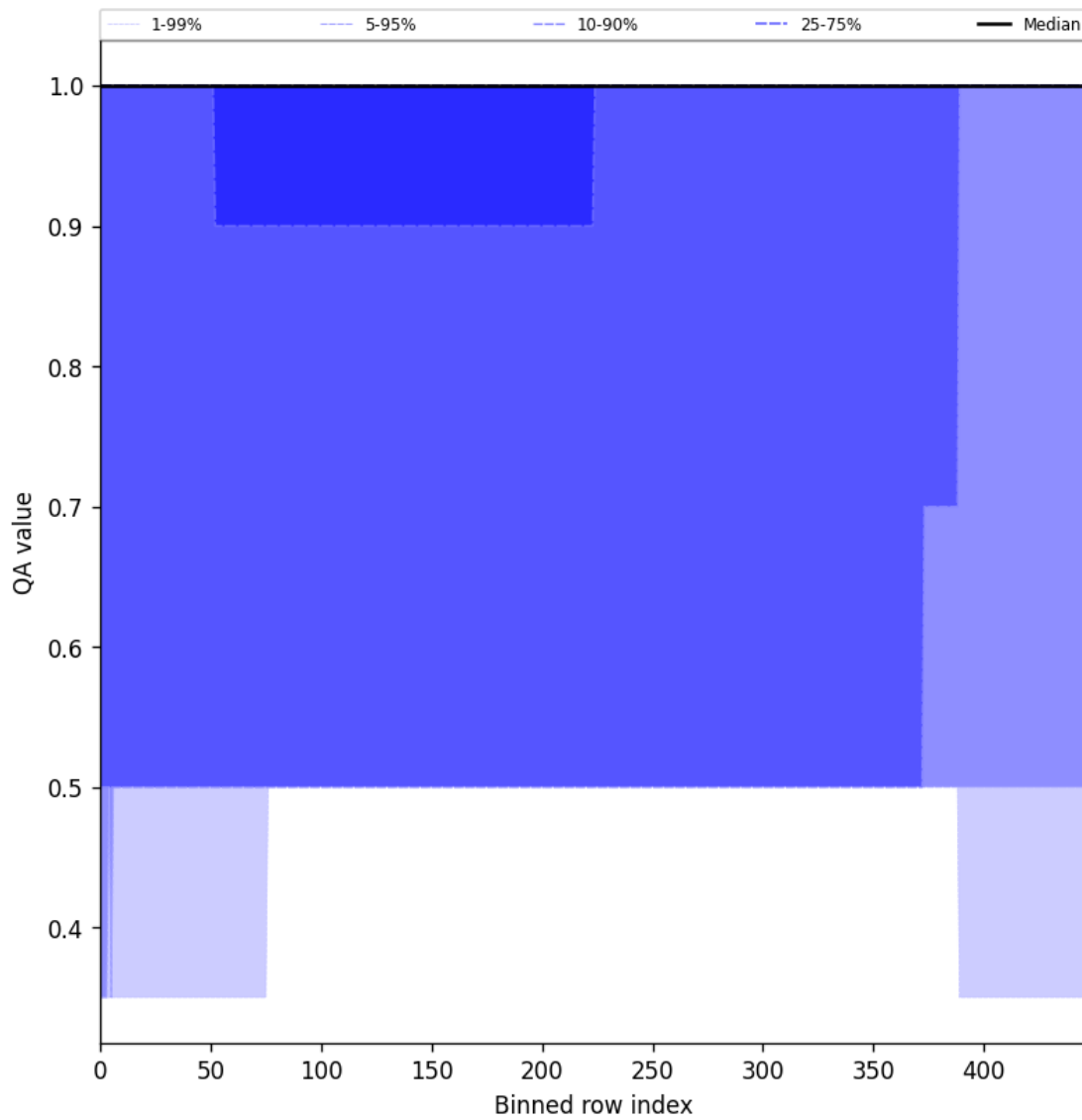
Figure 46: Along track statistics of “QA value” for 2024-10-29 to 2024-10-30
