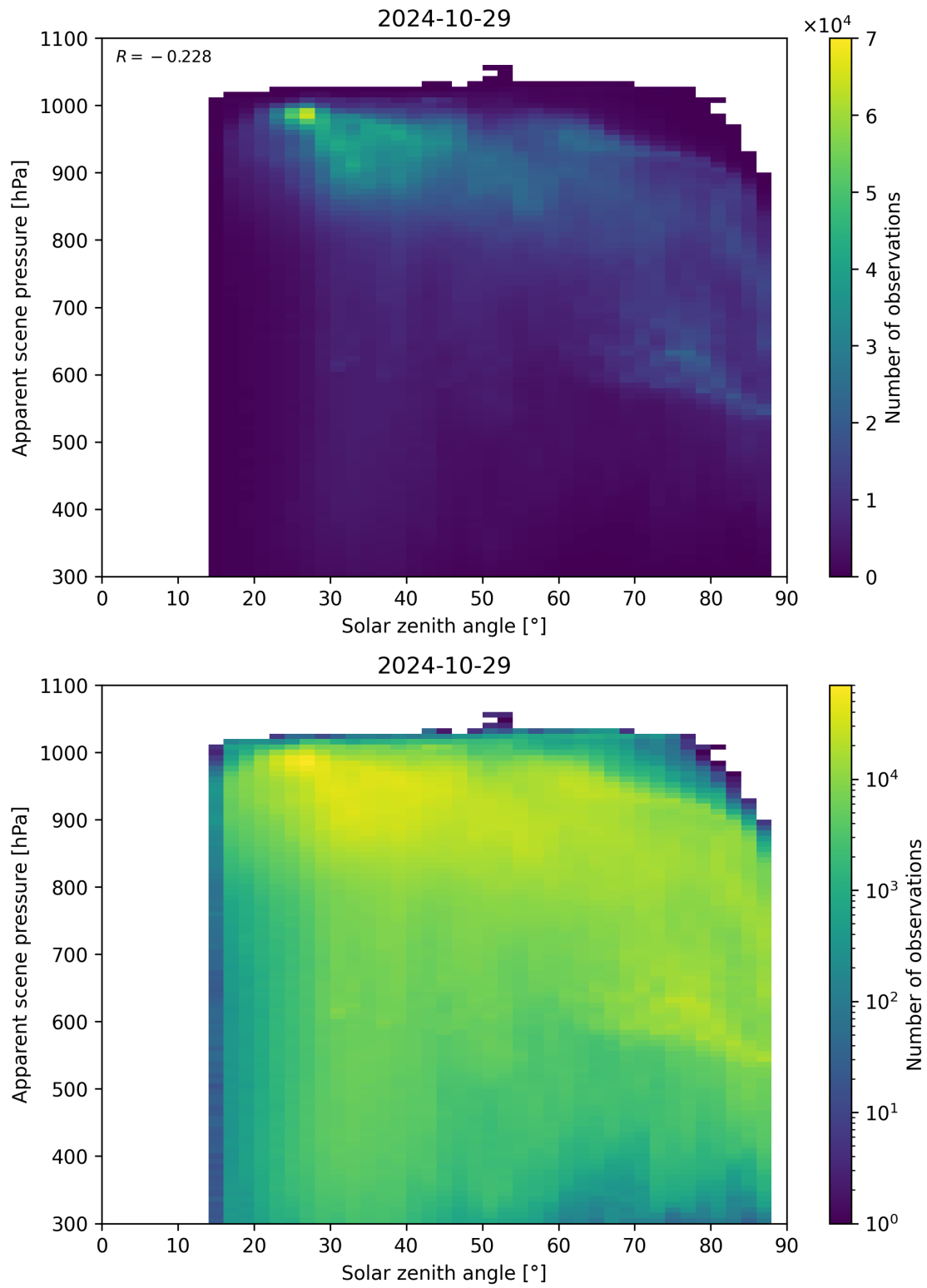
Figure 118: Scatter density plot of “Solar zenith angle” against “Apparent scene pressure” for 2024-10-29 to 2024-10-30.
