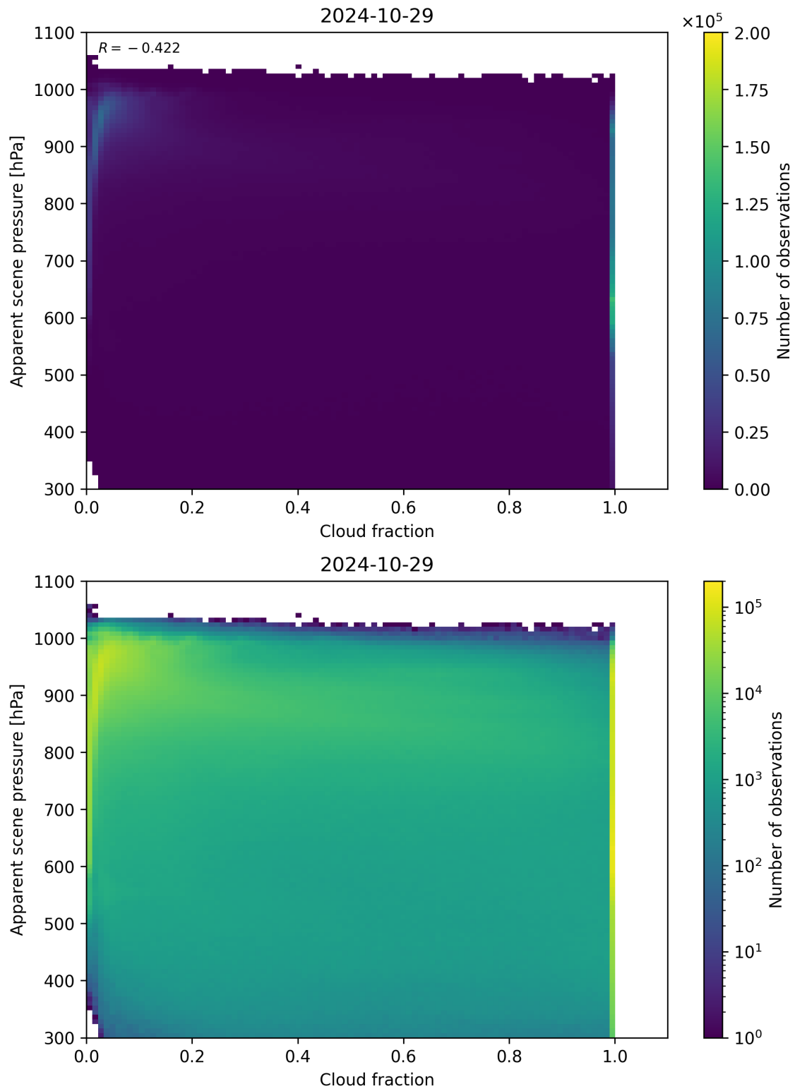
Figure 76: Scatter density plot of “Cloud fraction” against “Apparent scene pressure” for 2024-10-29 to 2024-10-30.
