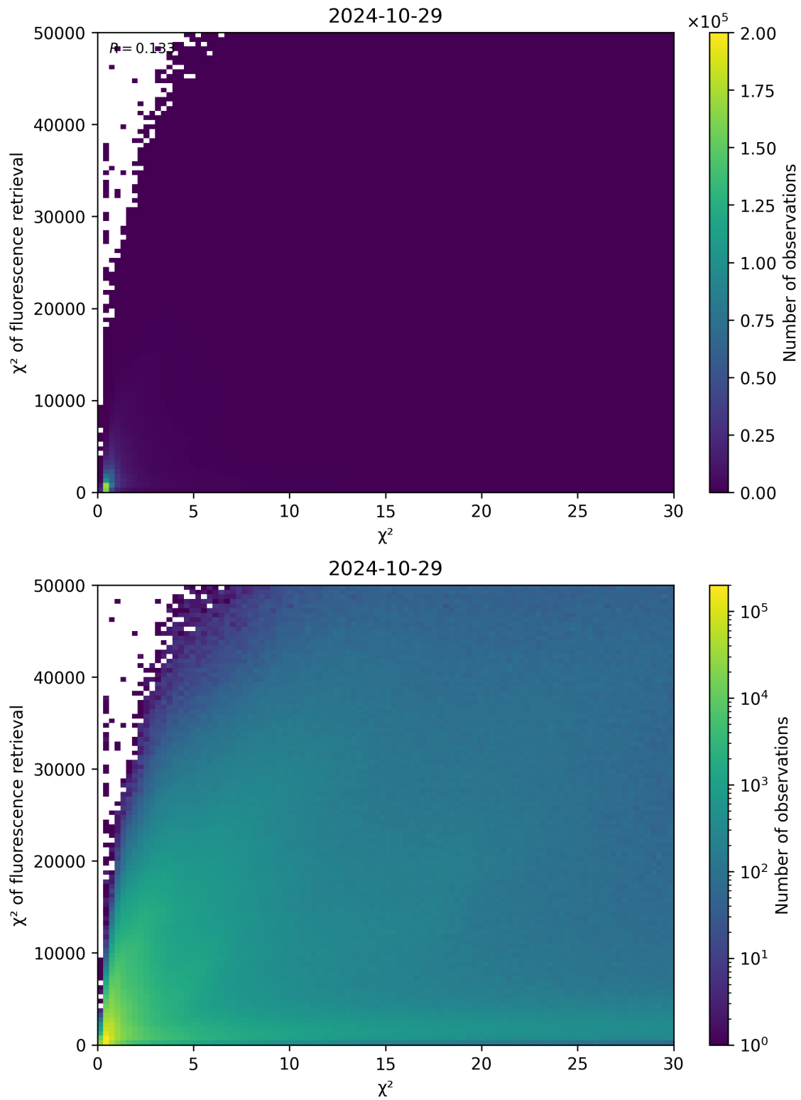
Figure 69: Scatter density plot of “ \chi^2 ” against “ \chi^2 of fluorescence retrieval” for 2024-10-29 to 2024-10-30.
