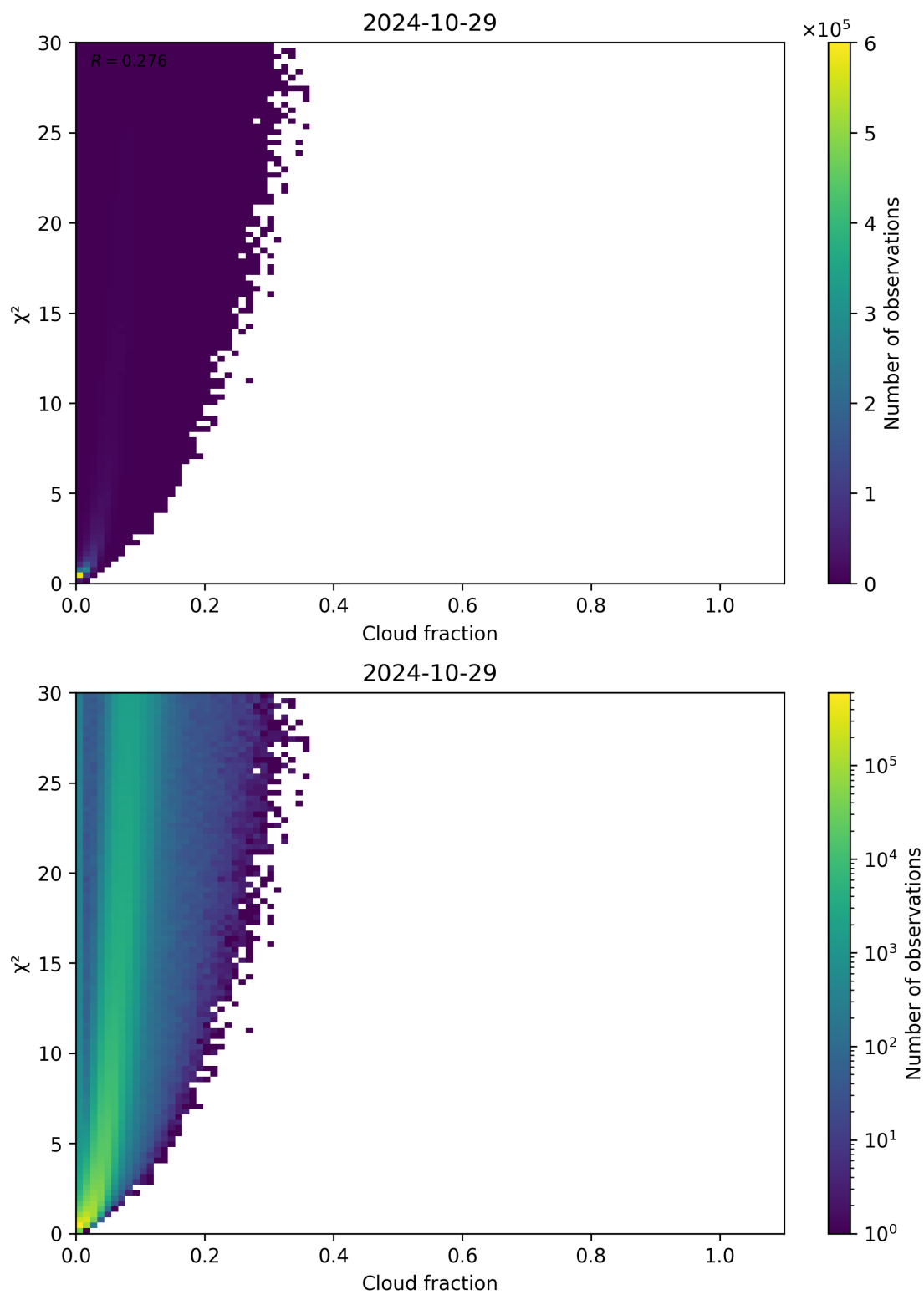
Figure 77: Scatter density plot of “Cloud fraction” against “ \chi^2 ” for 2024-10-29 to 2024-10-30.
