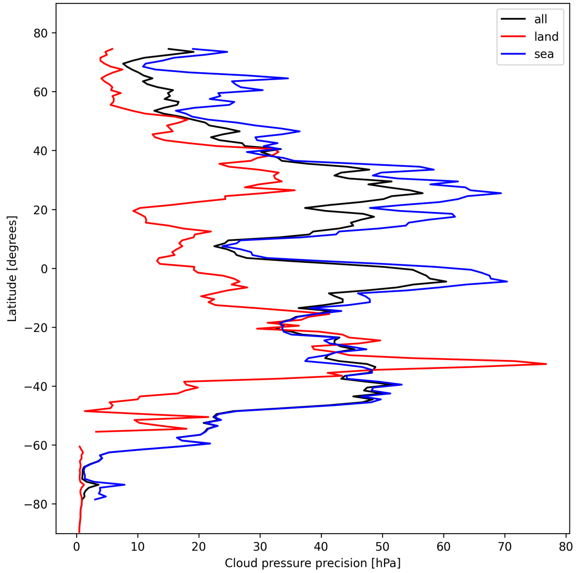
Figure 14: Zonal average of “Cloud pressure precision” for 2024-10-29 to 2024-10-30.
