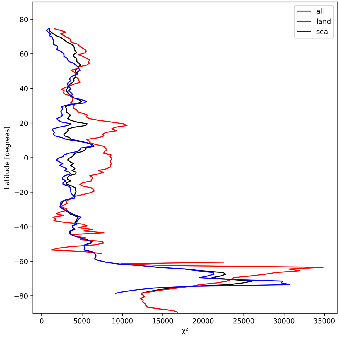
Figure 21: Zonal average of “ \chi^2 ” for 2024-10-29 to 2024-10-30.
