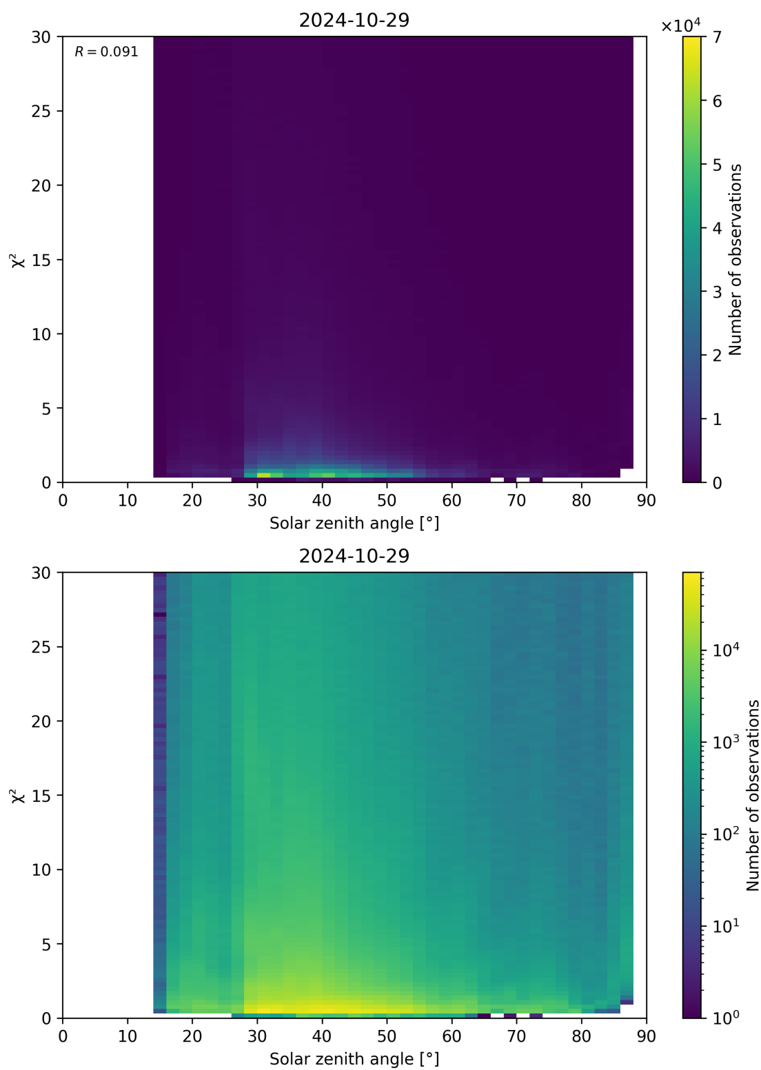
Figure 119: Scatter density plot of “Solar zenith angle” against “ \chi^2 ” for 2024-10-29 to 2024-10-30.
