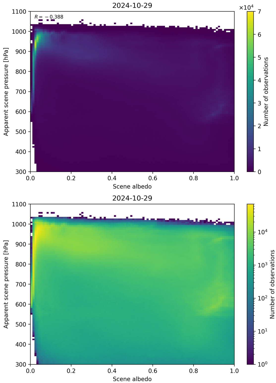
Figure 111: Scatter density plot of “Scene albedo” against “Apparent scene pressure” for 2024-10-29 to 2024-10-30.
