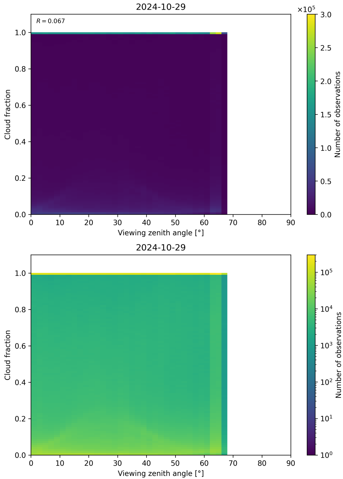
Figure 132: Scatter density plot of “Viewing zenith angle” against “Cloud fraction” for 2024-10-29 to 2024-10-30.
