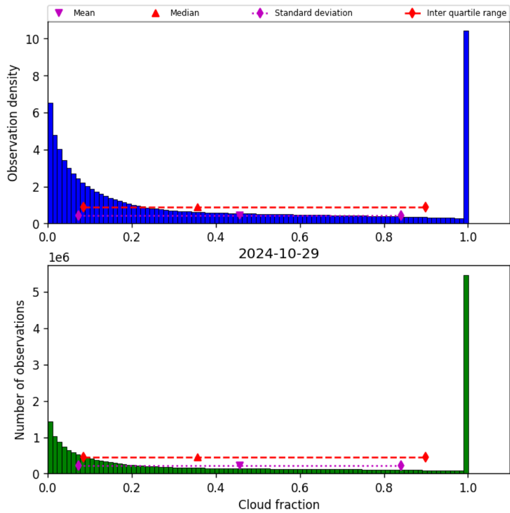
Figure 32: Histogram of “Cloud fraction” for 2024-10-29 to 2024-10-30
