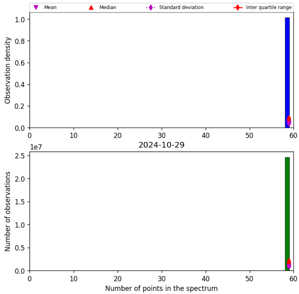
Figure 44: Histogram of “Number of points in the spectrum” for 2024-10-29 to 2024-10-30
