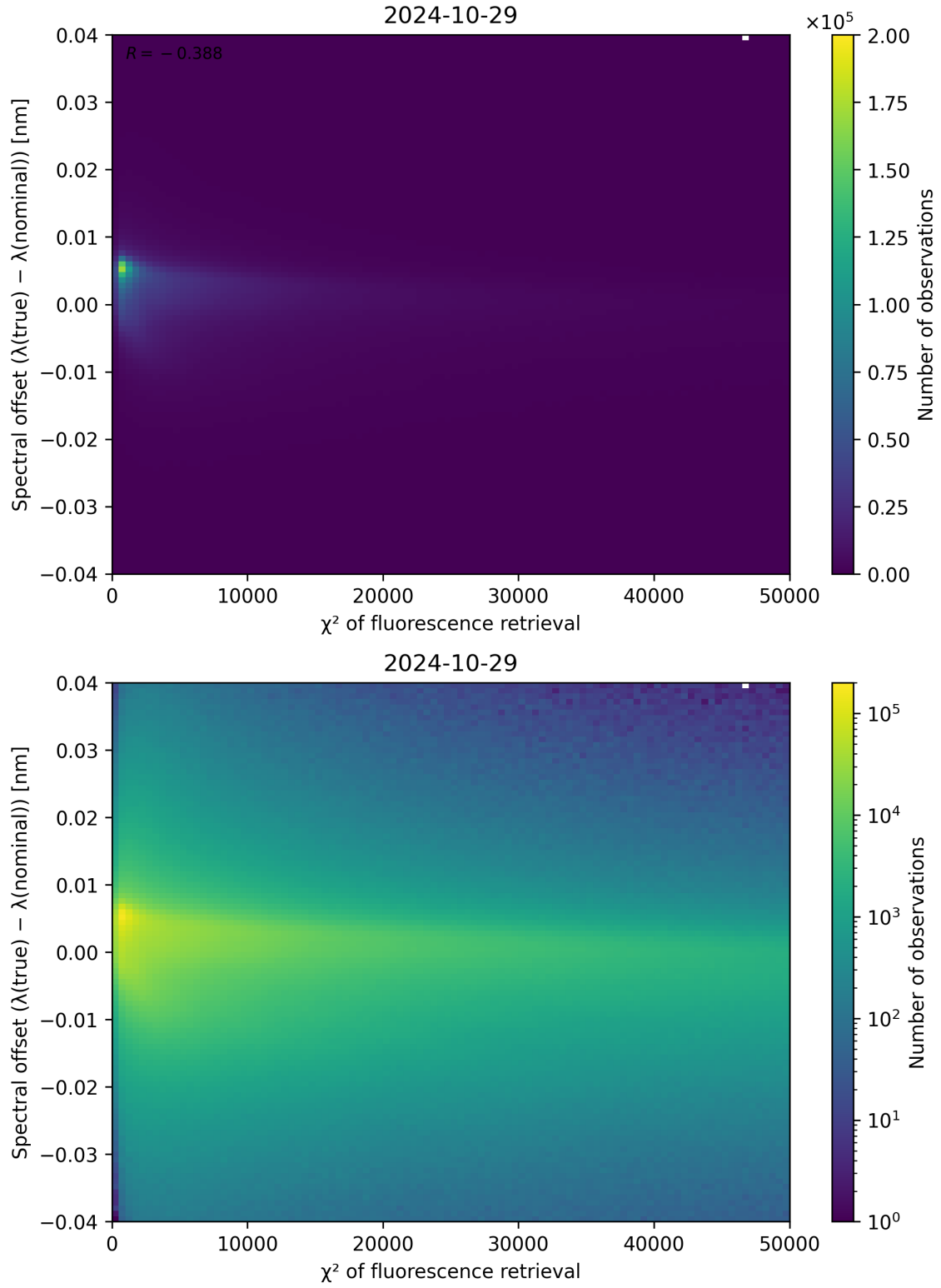
Figure 72: Scatter density plot of “ \chi^2 of fluorescence retrieval” against “Spectral offset ( \lambda_{\text{true}} - \lambda_{\text{nominal}} )” for 2024-10-29 to 2024-10-30.
