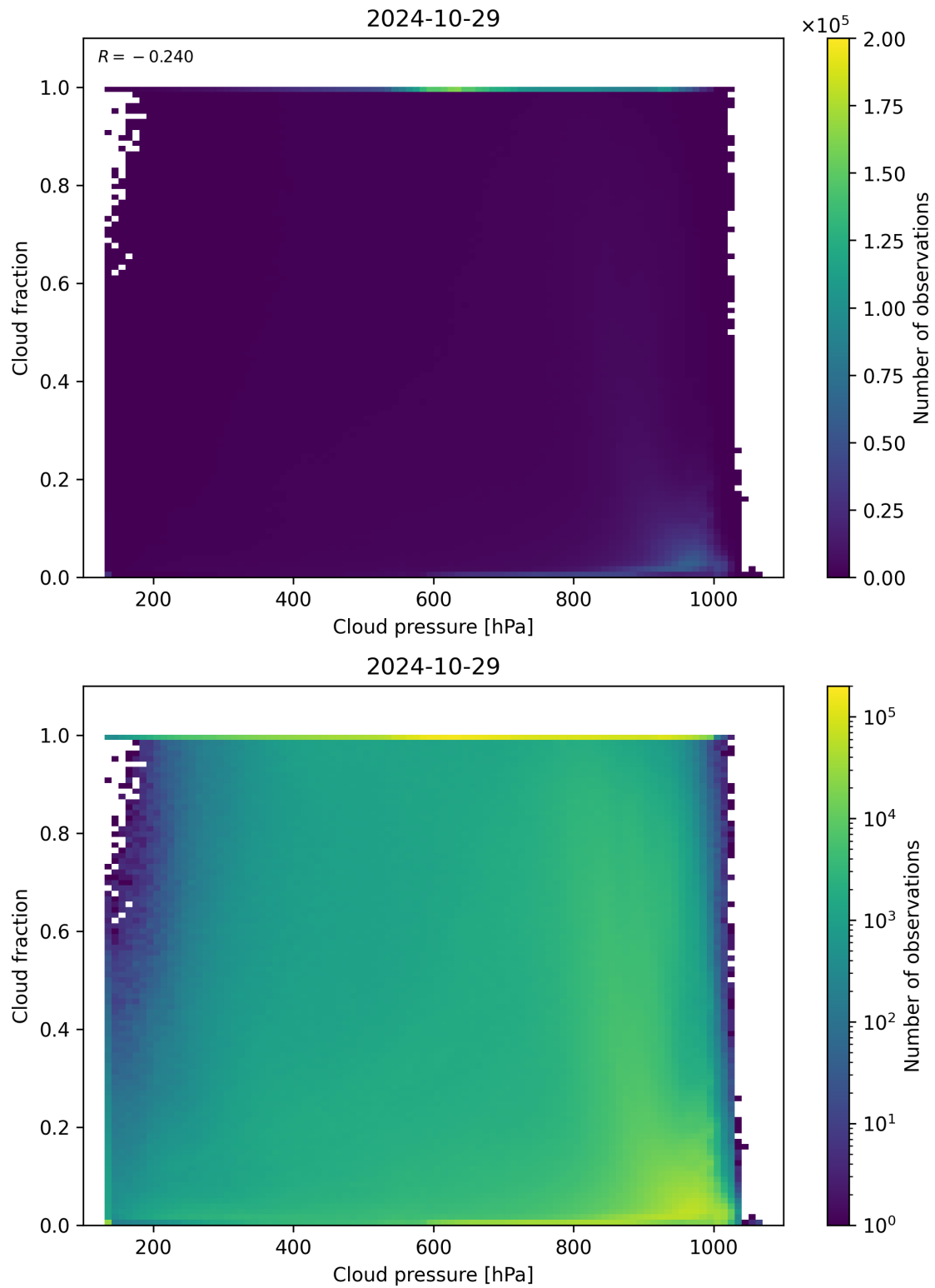
Figure 87: Scatter density plot of “Cloud pressure” against “Cloud fraction” for 2024-10-29 to 2024-10-30.
