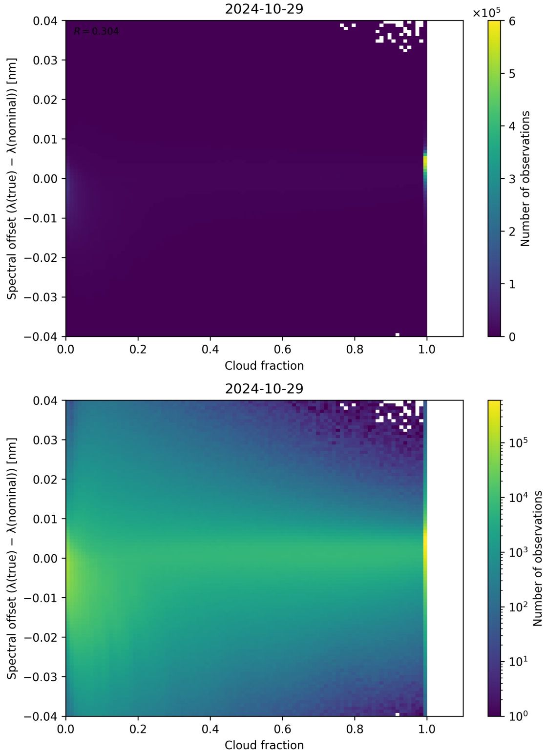
Figure 83: Scatter density plot of “Cloud fraction” against “Spectral offset ( \lambda_{\text{true}} - \lambda_{\text{nominal}} )” for 2024-10-29 to 2024-10-30.
