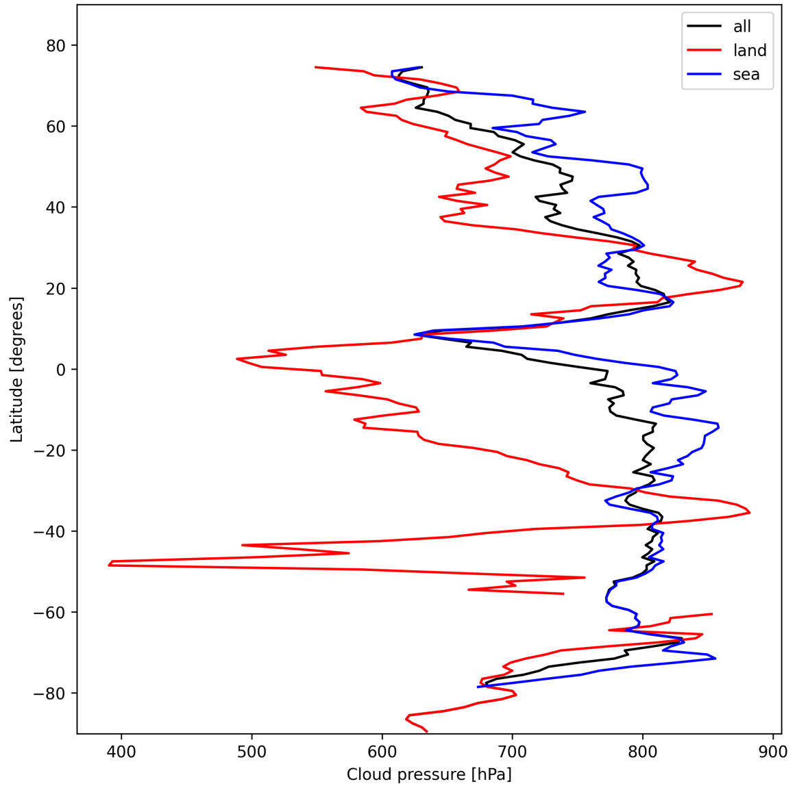
Figure 13: Zonal average of “Cloud pressure” for 2024-10-29 to 2024-10-30.
