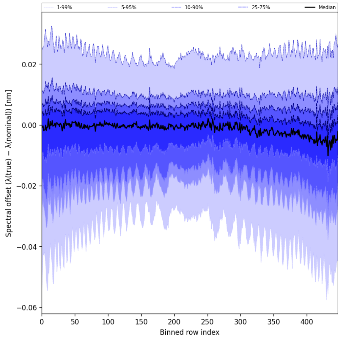
Figure 62: Along track statistics of “Spectral offset ( \lambda_{\text{true}} - \lambda_{\text{nominal}} )” for 2024-10-29 to 2024-10-30
