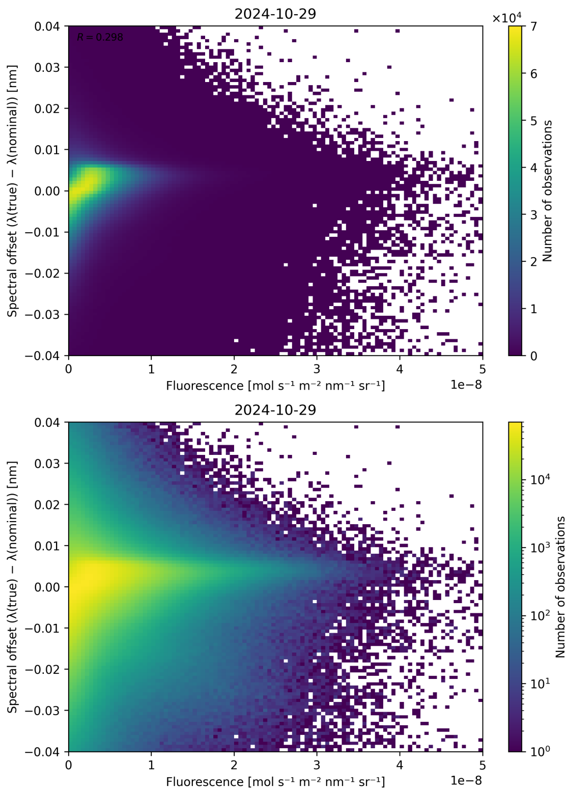
Figure 95: Scatter density plot of “Fluorescence” against “Spectral offset ( \lambda_{\text{true}} - \lambda_{\text{nominal}} )” for 2024-10-29 to 2024-10-30.
