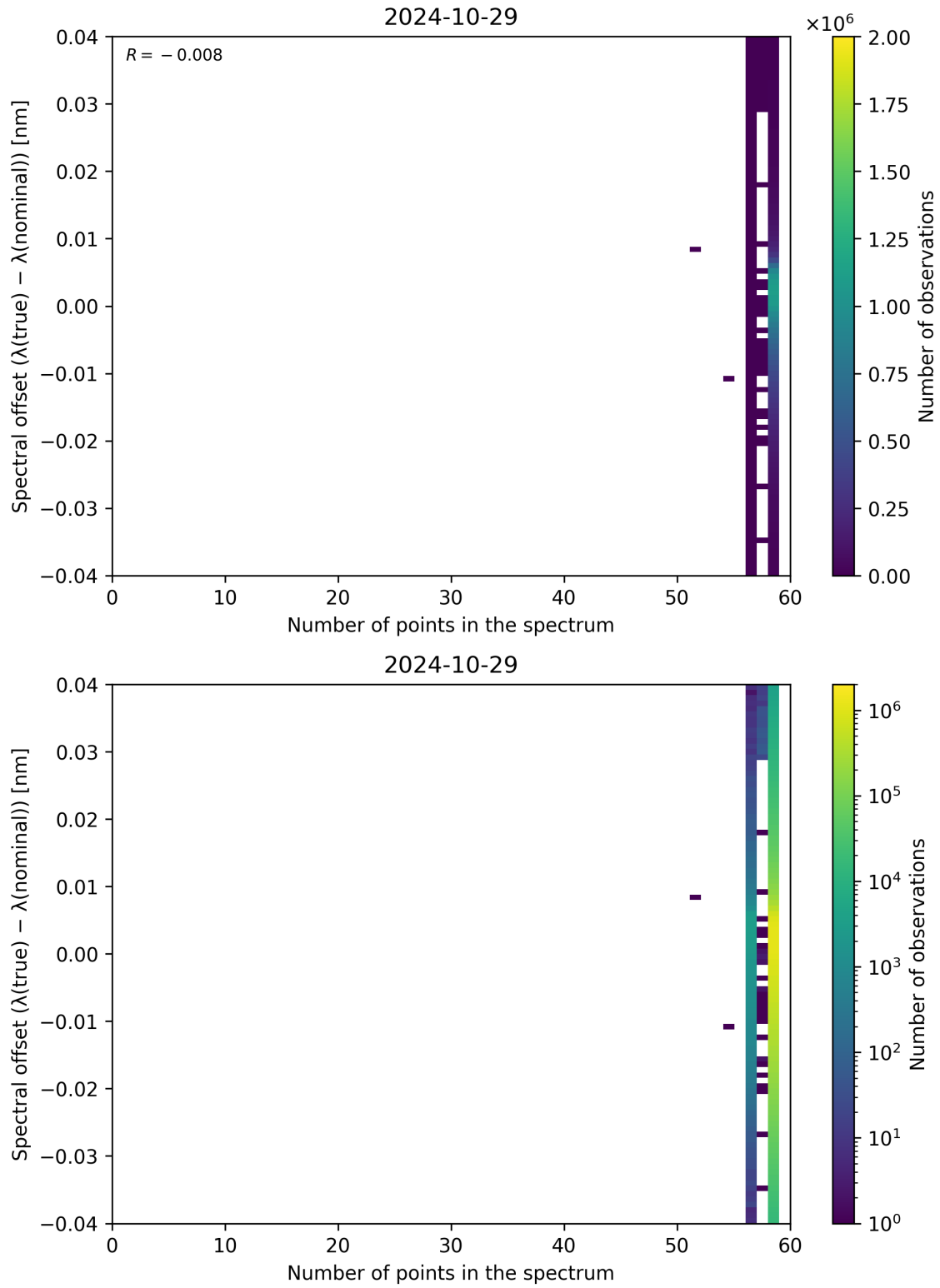
Figure 110: Scatter density plot of “Number of points in the spectrum” against “Spectral offset ( \lambda_{\text{true}} - \lambda_{\text{nominal}} )” for 2024-10-29 to 2024-10-30.
