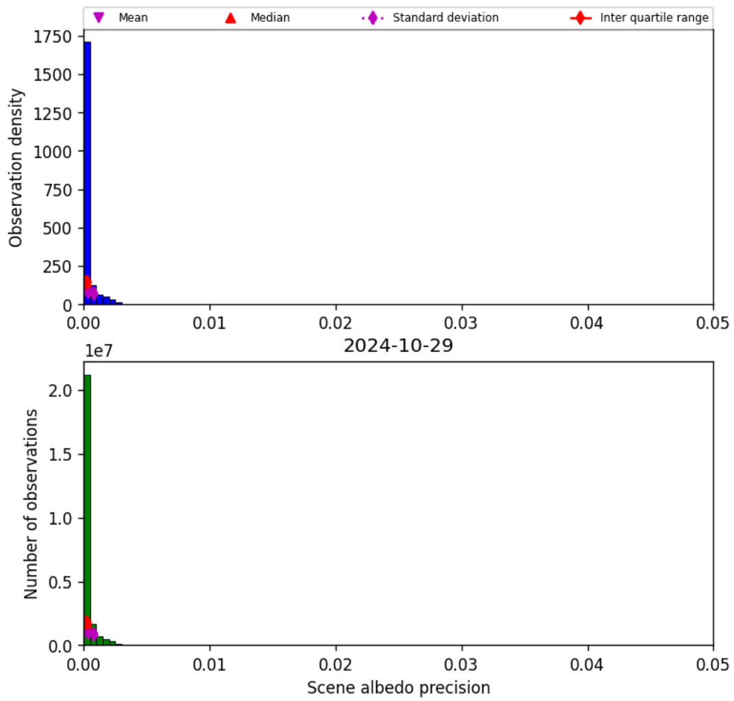
Figure 35: Histogram of “Scene albedo precision” for 2024-10-29 to 2024-10-30
