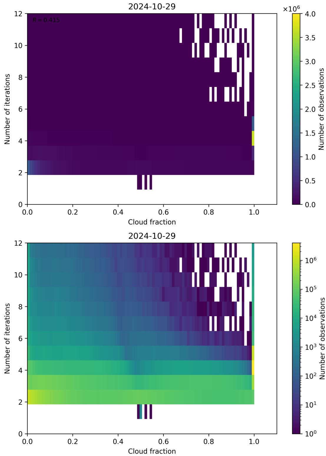
Figure 80: Scatter density plot of “Cloud fraction” against “Number of iterations” for 2024-10-29 to 2024-10-30.
