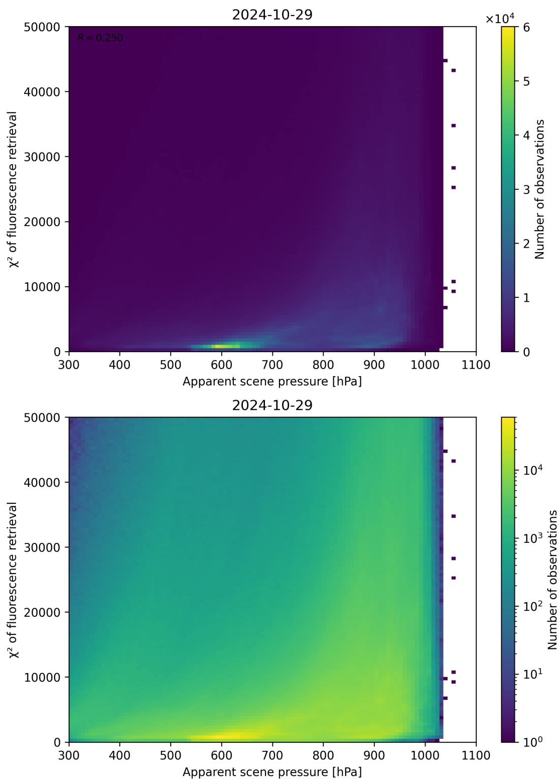
Figure 64: Scatter density plot of “Apparent scene pressure” against “ \chi^2 of fluorescence retrieval” for 2024-10-29 to 2024-10-30.
