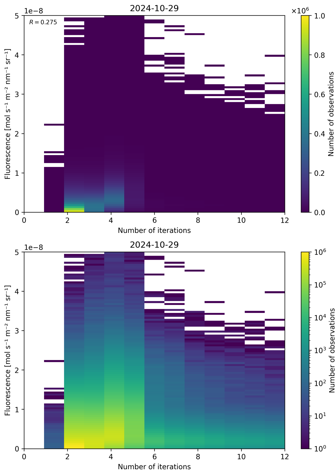
Figure 107: Scatter density plot of “Number of iterations” against “Fluorescence” for 2024-10-29 to 2024-10-30.
