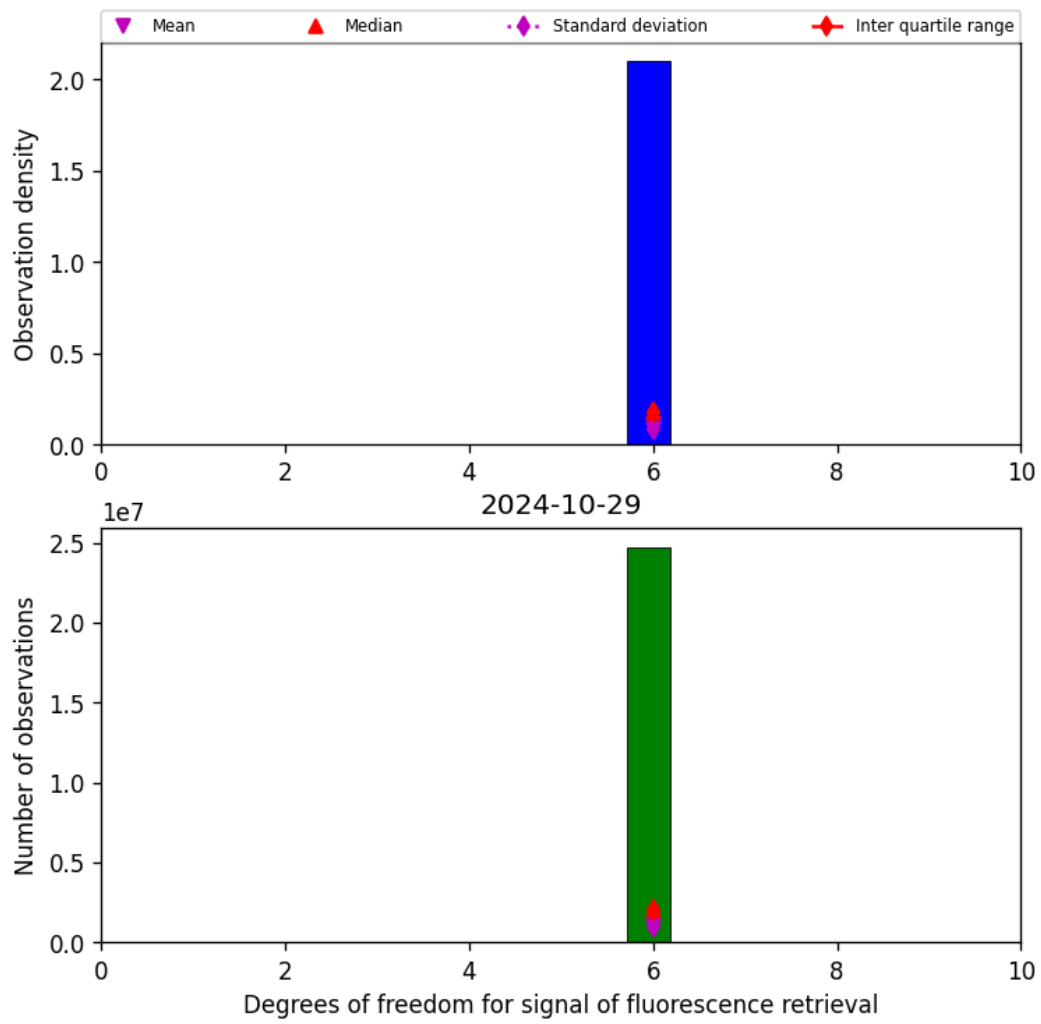
Figure 43: Histogram of “Degrees of freedom for signal of fluorescence retrieval” for 2024-10-29 to 2024-10-30
