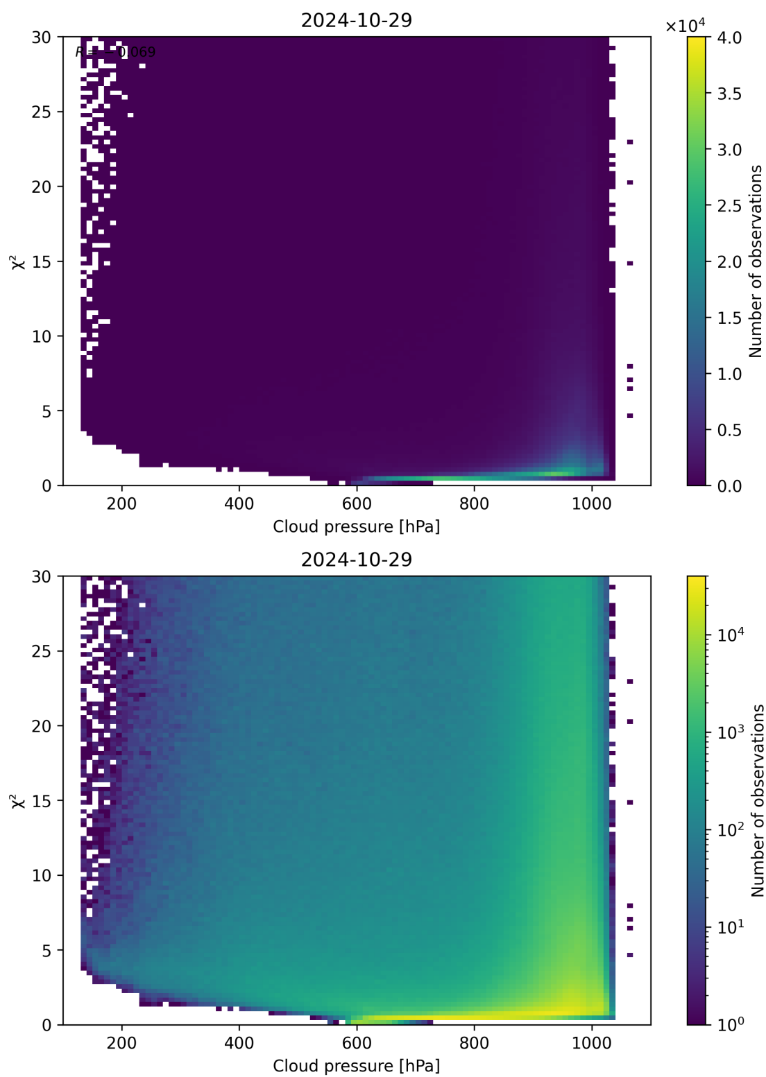
Figure 85: Scatter density plot of “Cloud pressure” against “ \chi^2 ” for 2024-10-29 to 2024-10-30.
