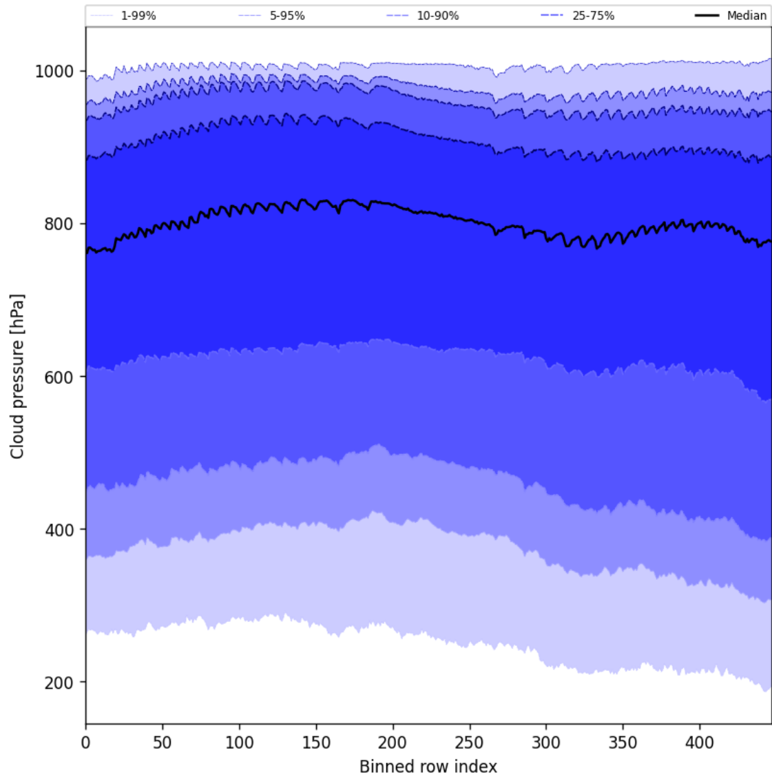
Figure 47: Along track statistics of “Cloud pressure” for 2024-10-29 to 2024-10-30
