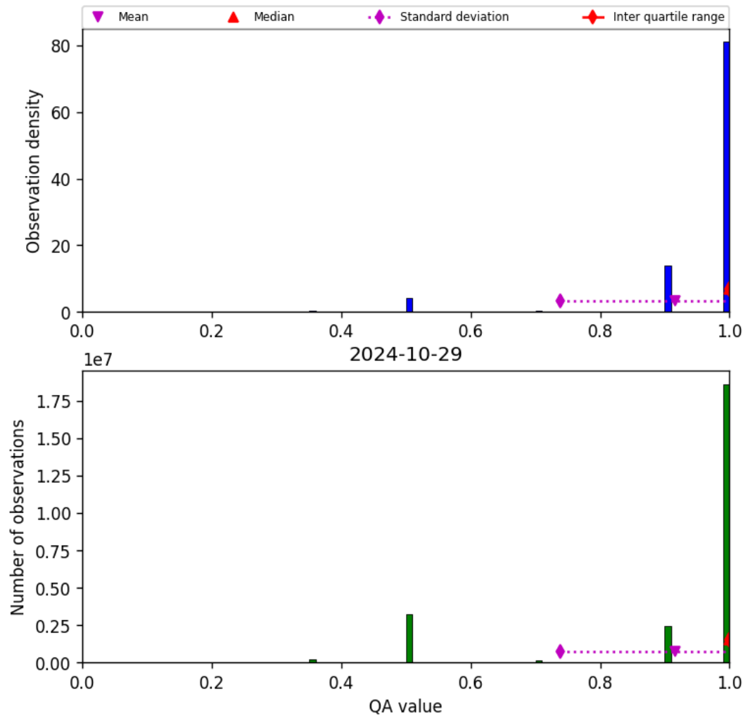
Figure 29: Histogram of “QA value” for 2024-10-29 to 2024-10-30
