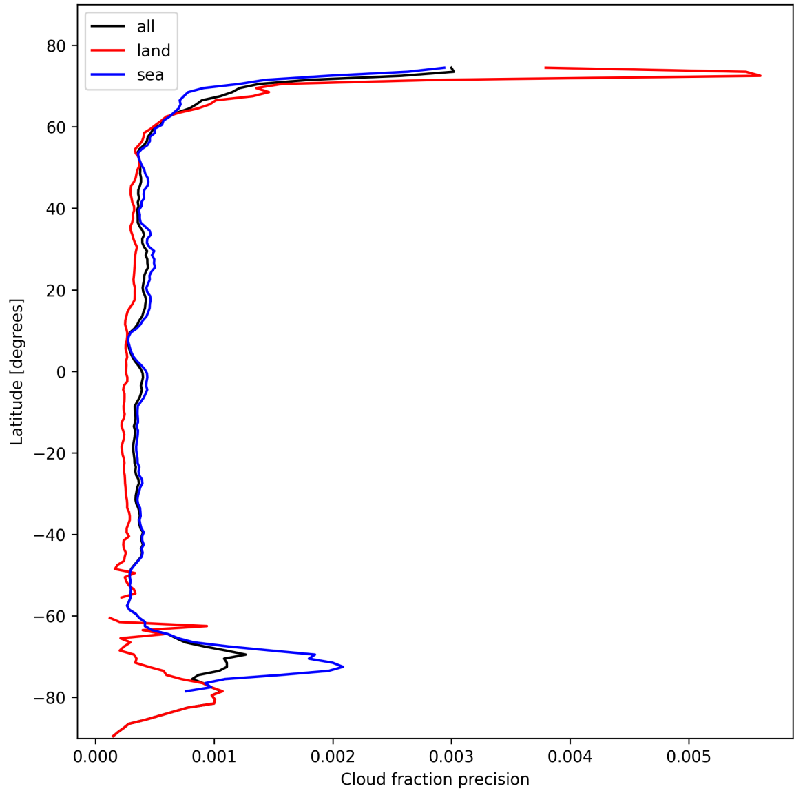
Figure 16: Zonal average of “Cloud fraction precision” for 2024-10-29 to 2024-10-30.
