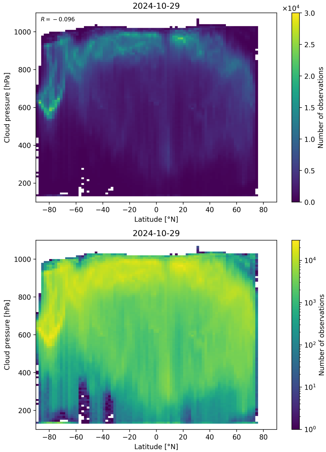
Figure 100: Scatter density plot of “Latitude” against “Cloud pressure” for 2024-10-29 to 2024-10-30.
