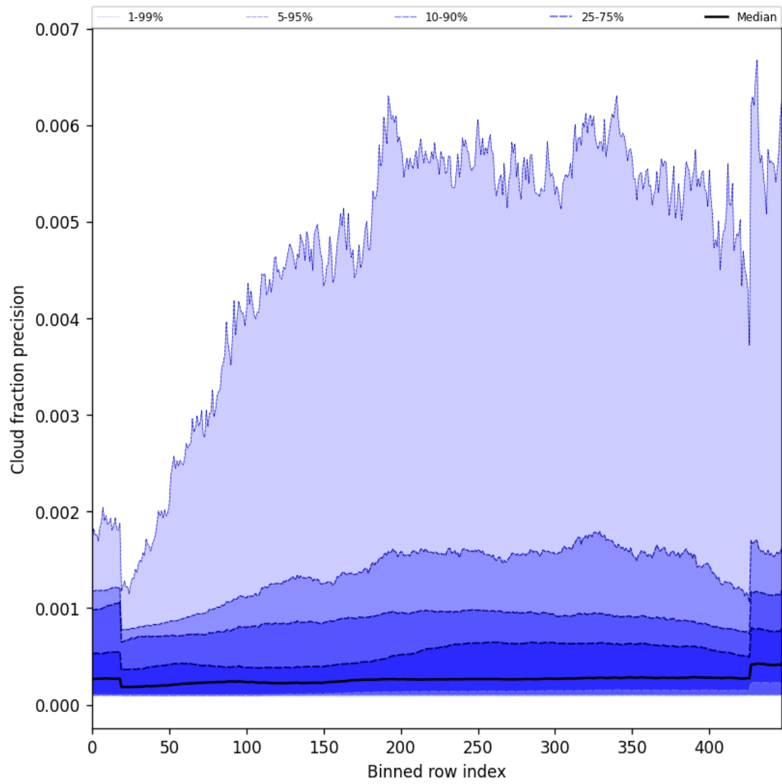
Figure 50: Along track statistics of “Cloud fraction precision” for 2024-10-29 to 2024-10-30
