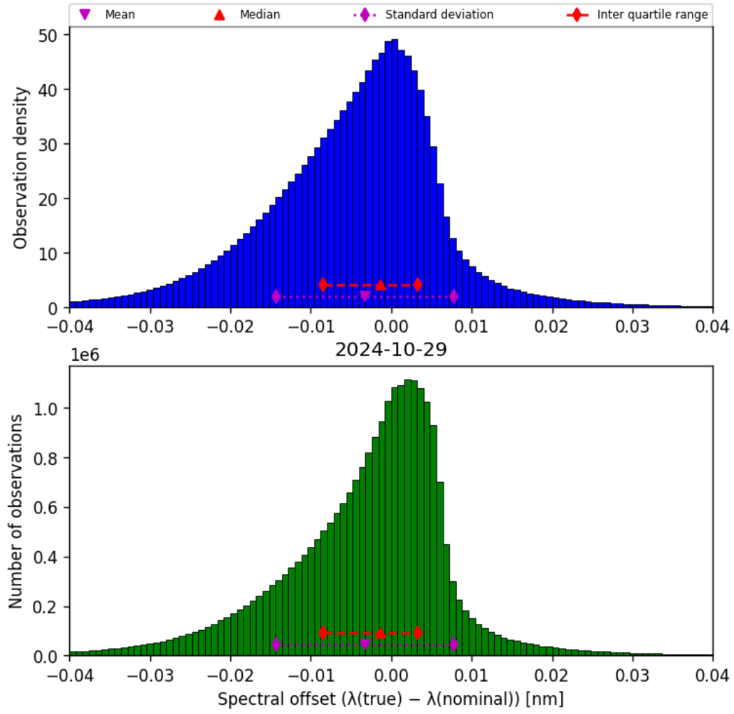
Figure 45: Histogram of “Spectral offset ( \lambda_{\text{true}} - \lambda_{\text{nominal}} )” for 2024-10-29 to 2024-10-30
