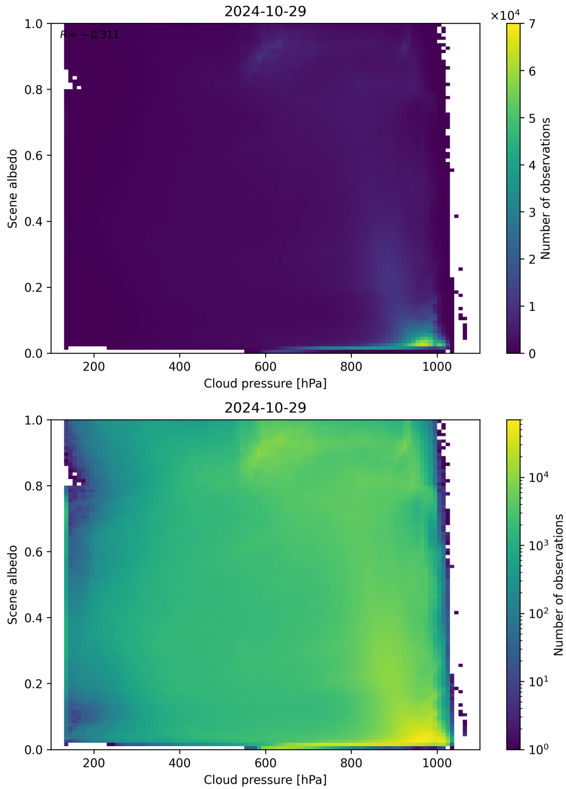
Figure 91: Scatter density plot of “Cloud pressure” against “Scene albedo” for 2024-10-29 to 2024-10-30.
