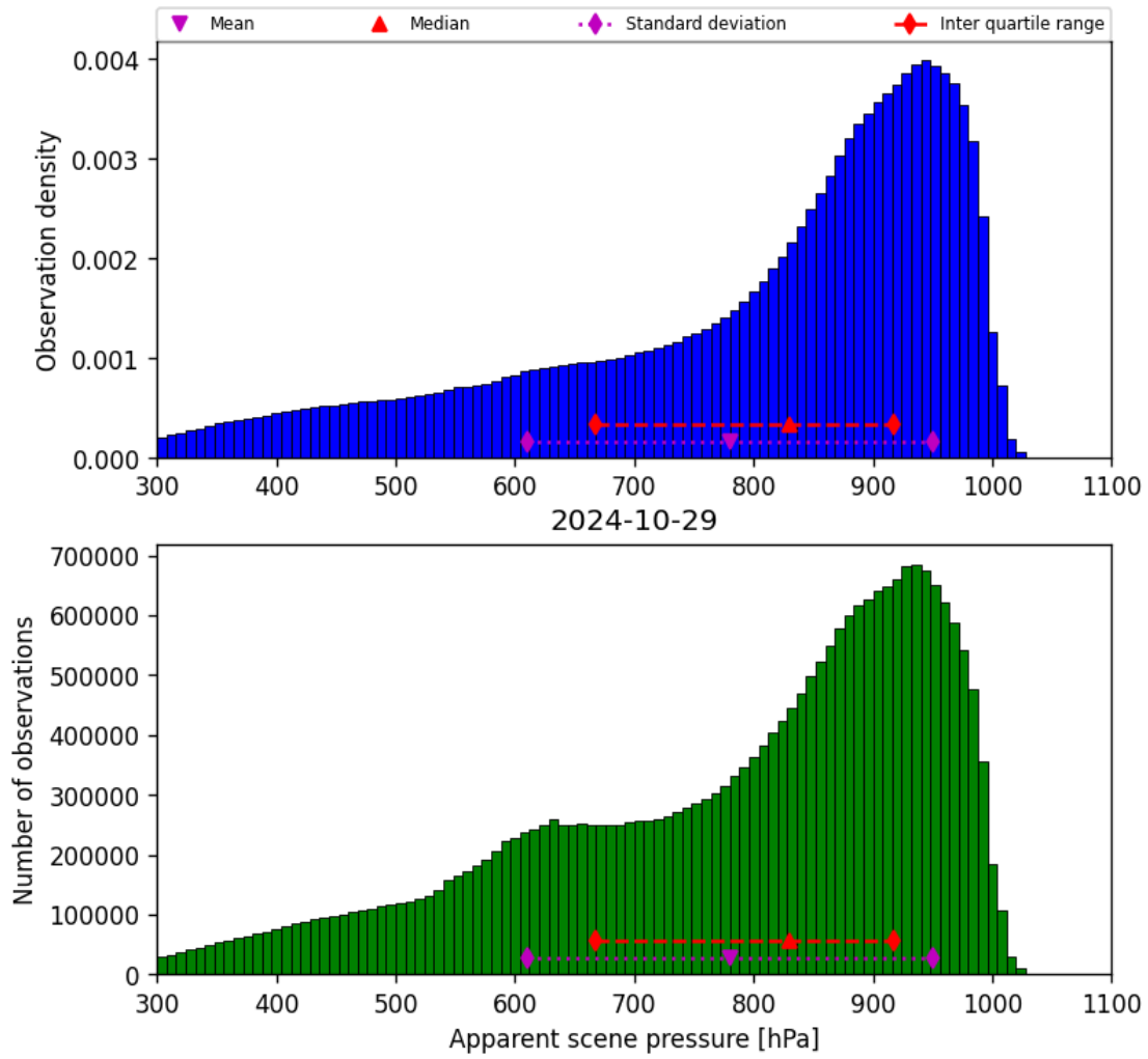
Figure 36: Histogram of “Apparent scene pressure” for 2024-10-29 to 2024-10-30
