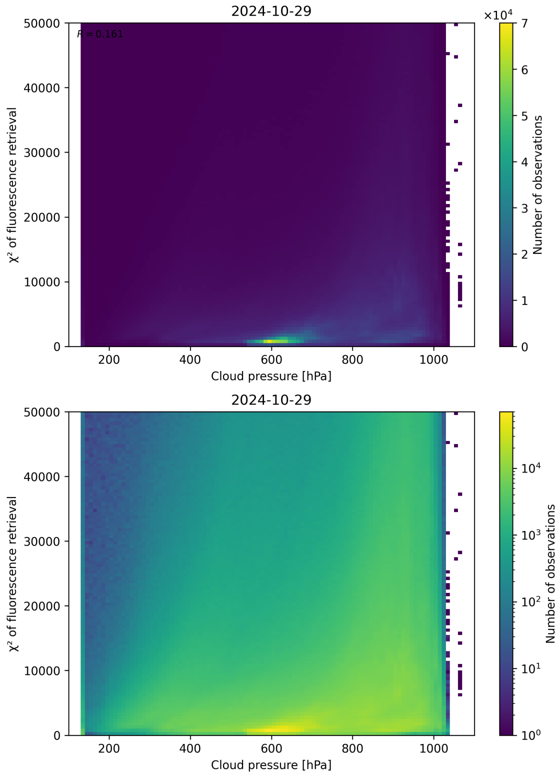
Figure 86: Scatter density plot of “Cloud pressure” against “ \chi^2 of fluorescence retrieval” for 2024-10-29 to 2024-10-30.
