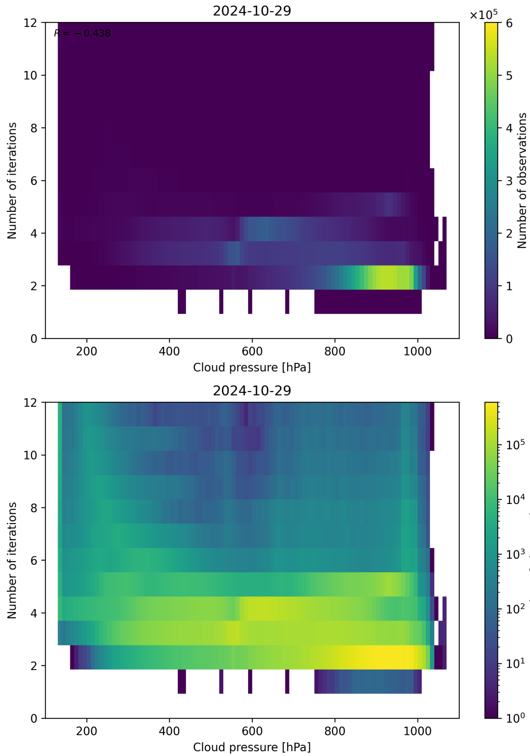
Figure 89: Scatter density plot of “Cloud pressure” against “Number of iterations” for 2024-10-29 to 2024-10-30.
