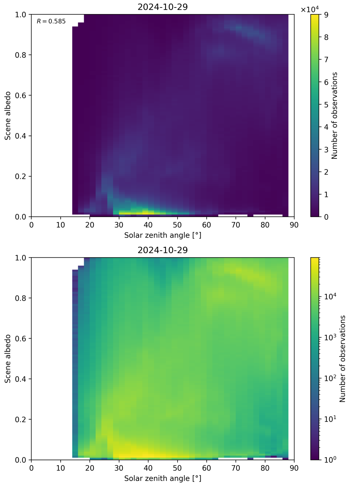
Figure 127: Scatter density plot of “Solar zenith angle” against “Scene albedo” for 2024-10-29 to 2024-10-30.
