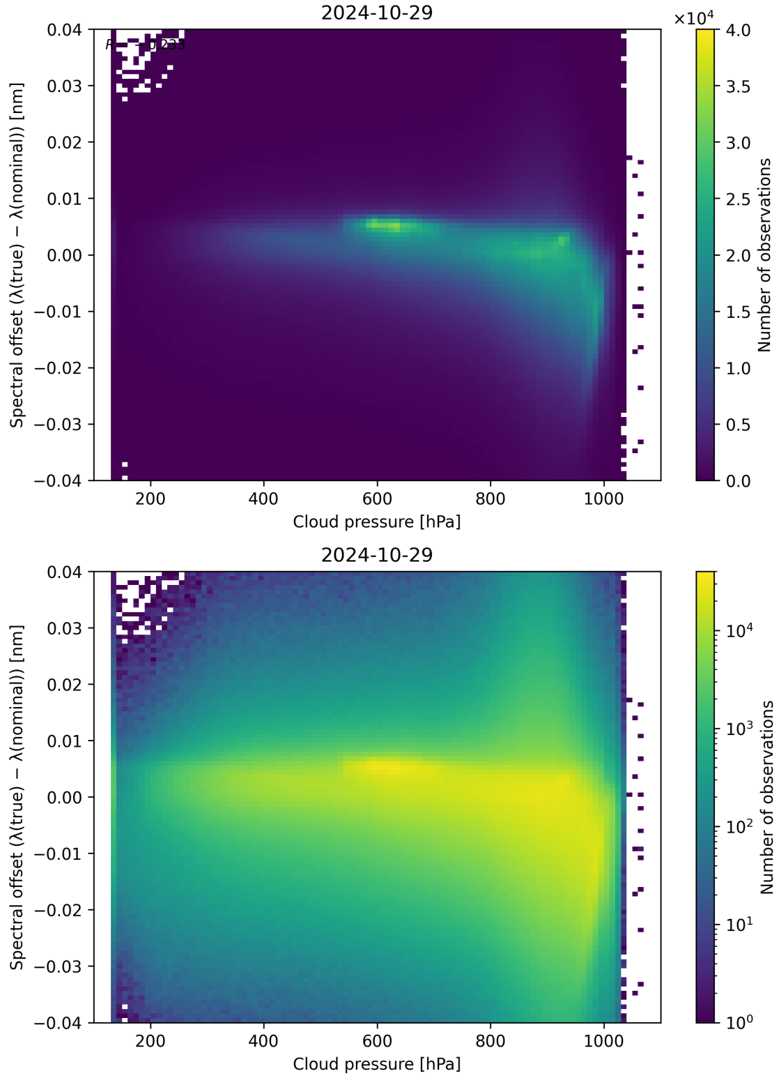
Figure 92: Scatter density plot of “Cloud pressure” against “Spectral offset ( \lambda_{\text{true}} - \lambda_{\text{nominal}} )” for 2024-10-29 to 2024-10-30.
