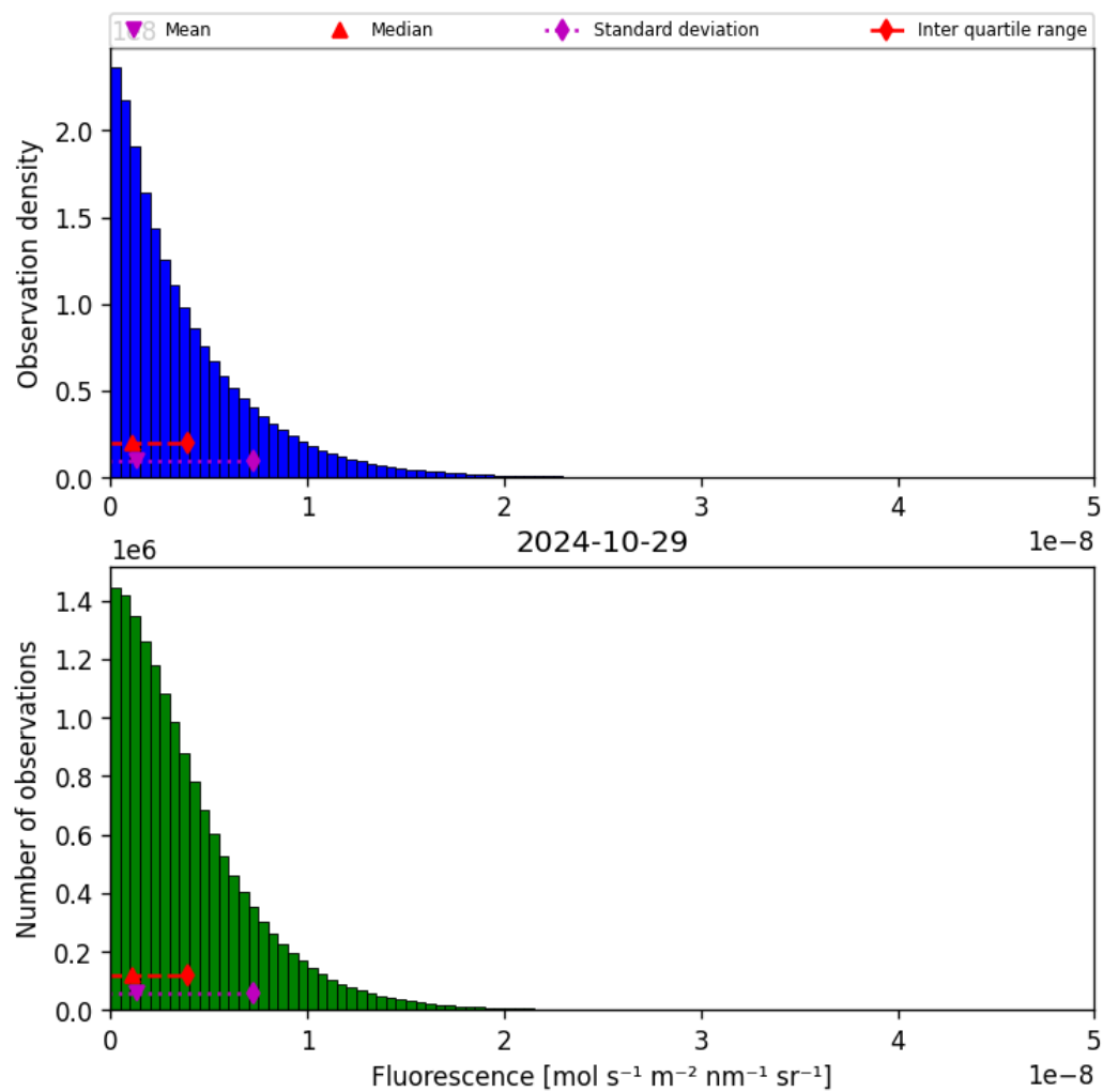
Figure 40: Histogram of “Fluorescence” for 2024-10-29 to 2024-10-30
