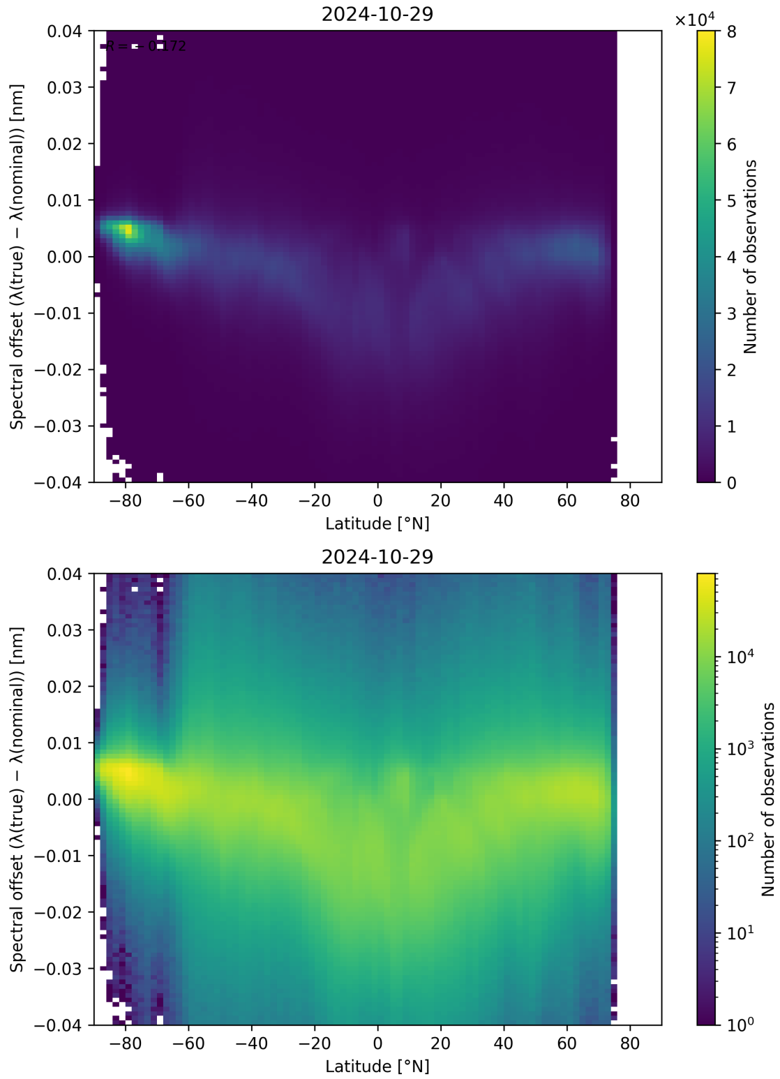
Figure 105: Scatter density plot of “Latitude” against “Spectral offset ( \lambda_{\text{true}} - \lambda_{\text{nominal}} )” for 2024-10-29 to 2024-10-30.
