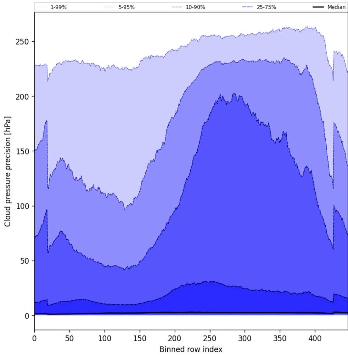
Figure 48: Along track statistics of “Cloud pressure precision” for 2024-10-29 to 2024-10-30
