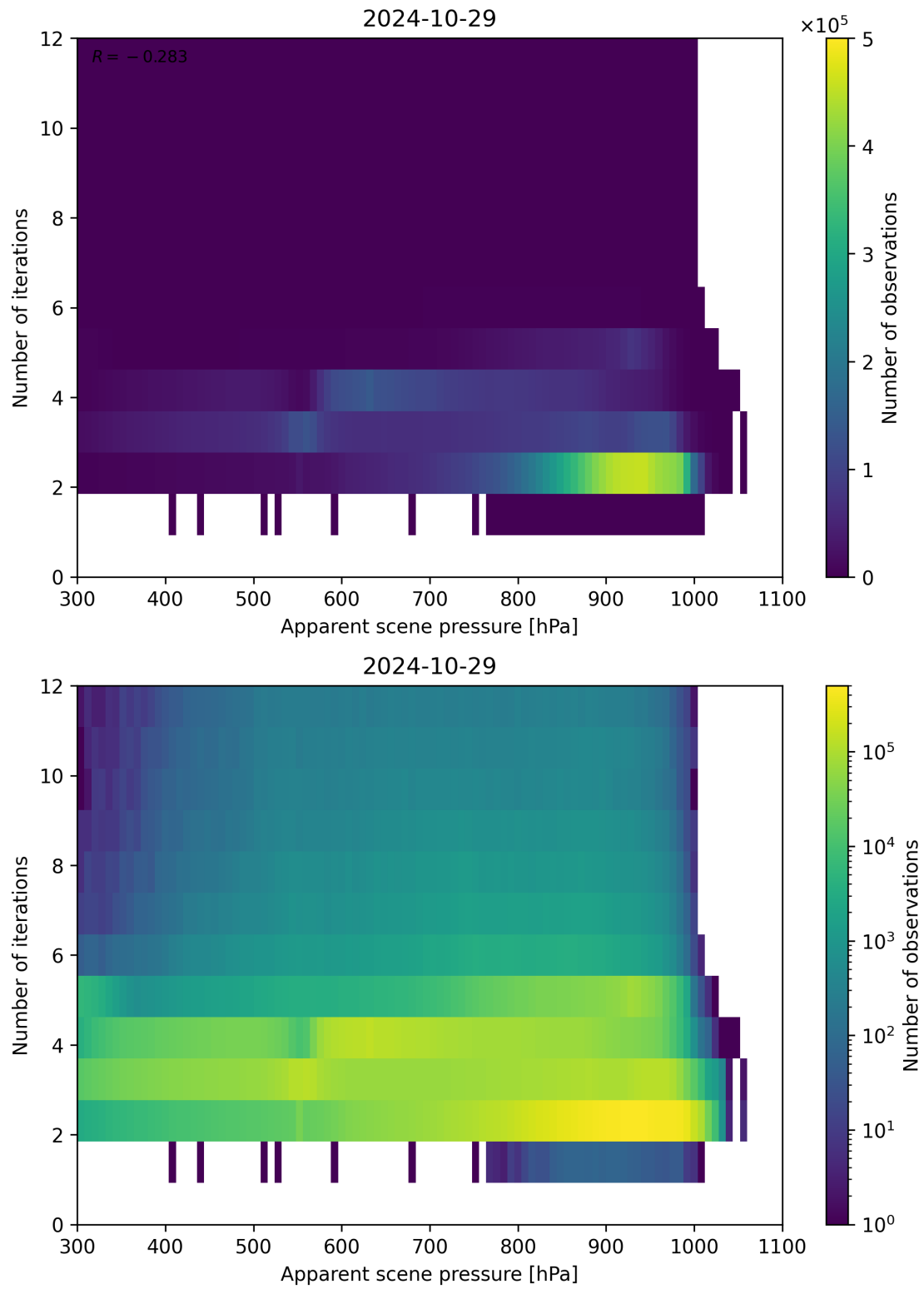
Figure 66: Scatter density plot of “Apparent scene pressure” against “Number of iterations” for 2024-10-29 to 2024-10-30.
