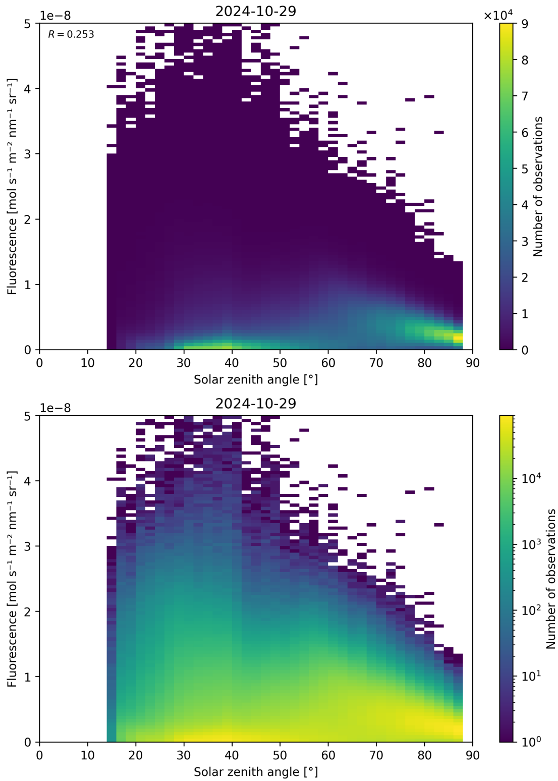
Figure 123: Scatter density plot of “Solar zenith angle” against “Fluorescence” for 2024-10-29 to 2024-10-30.
