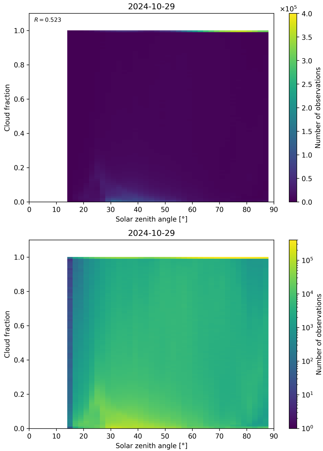
Figure 121: Scatter density plot of “Solar zenith angle” against “Cloud fraction” for 2024-10-29 to 2024-10-30.
