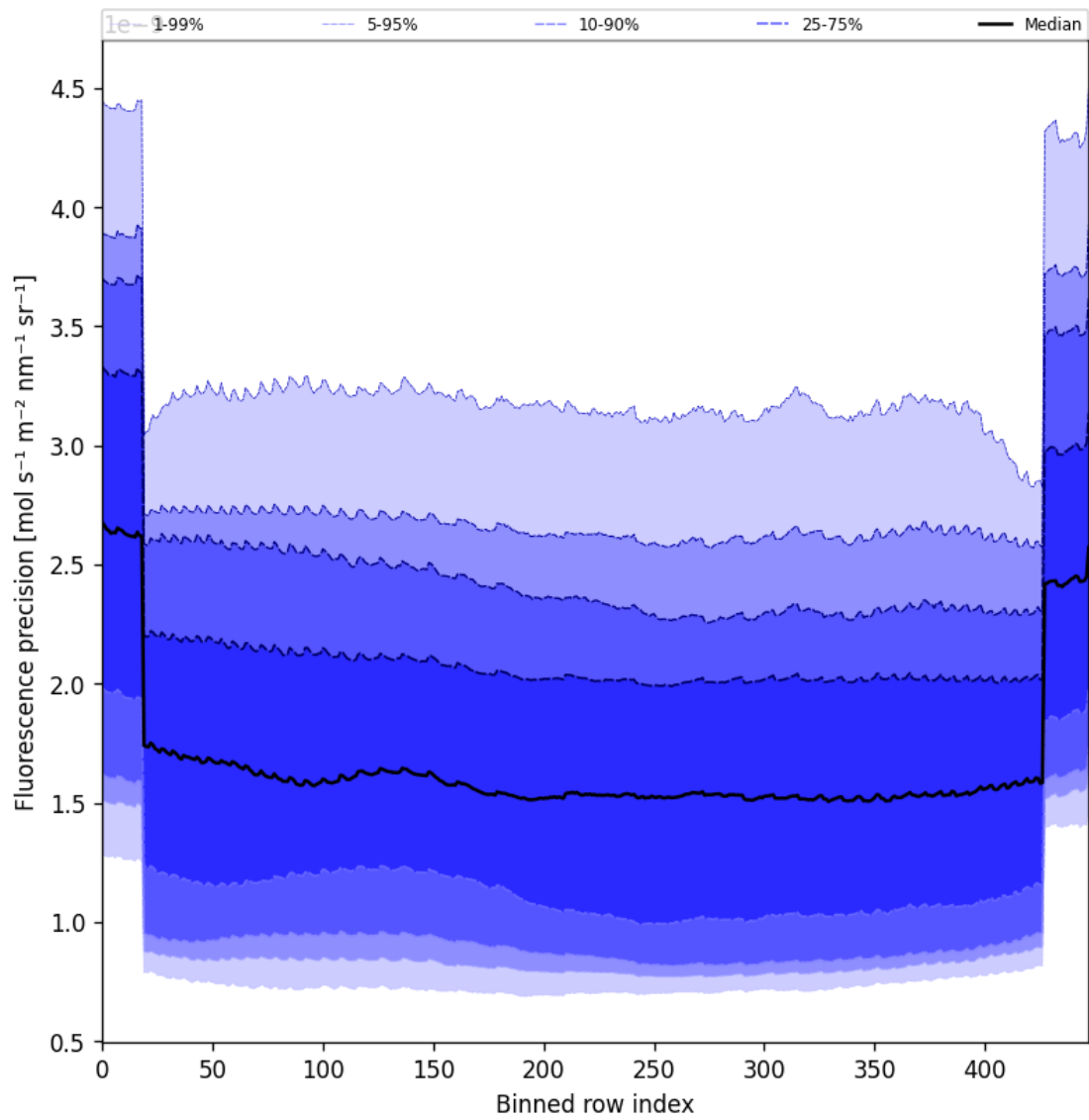
Figure 58: Along track statistics of "Fluorescence precision" for 2024-10-29 to 2024-10-30
