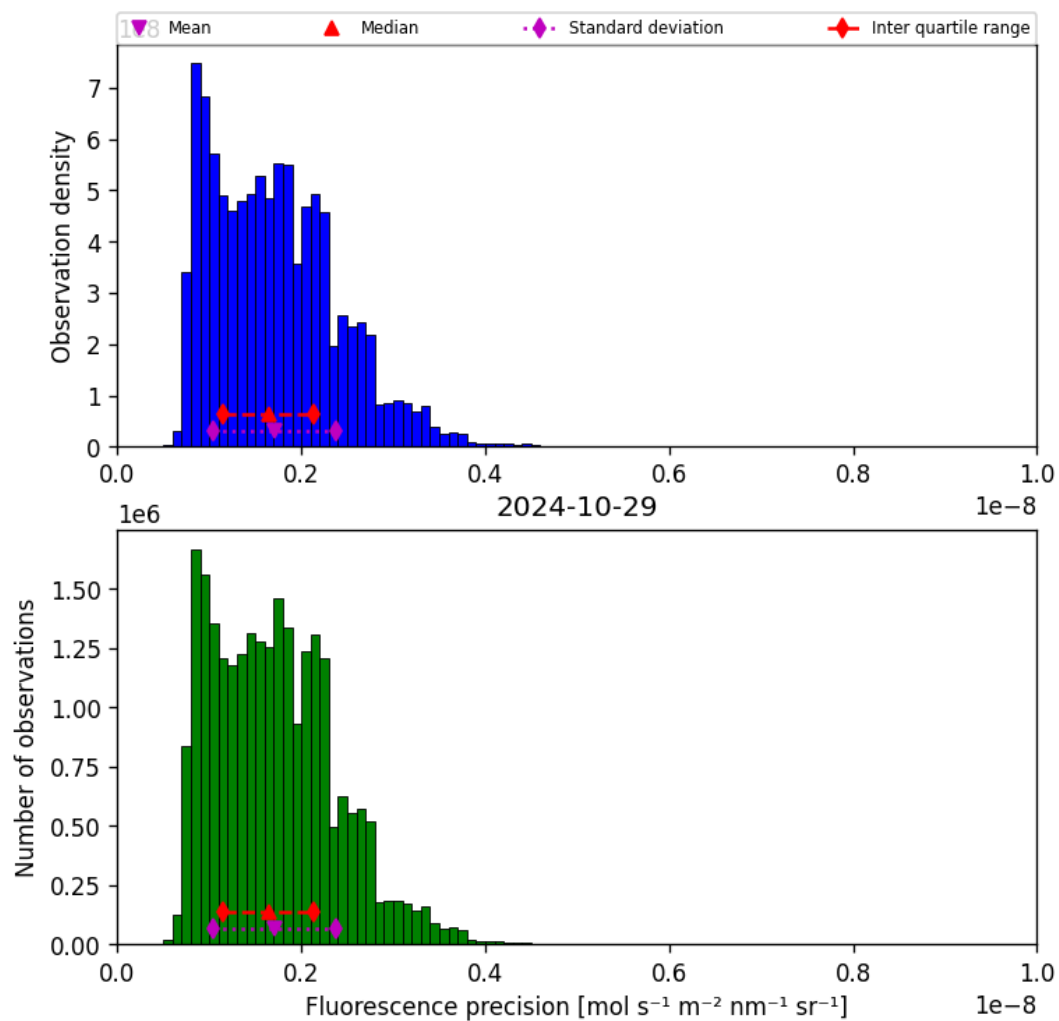
Figure 41: Histogram of “Fluorescence precision” for 2024-10-29 to 2024-10-30
