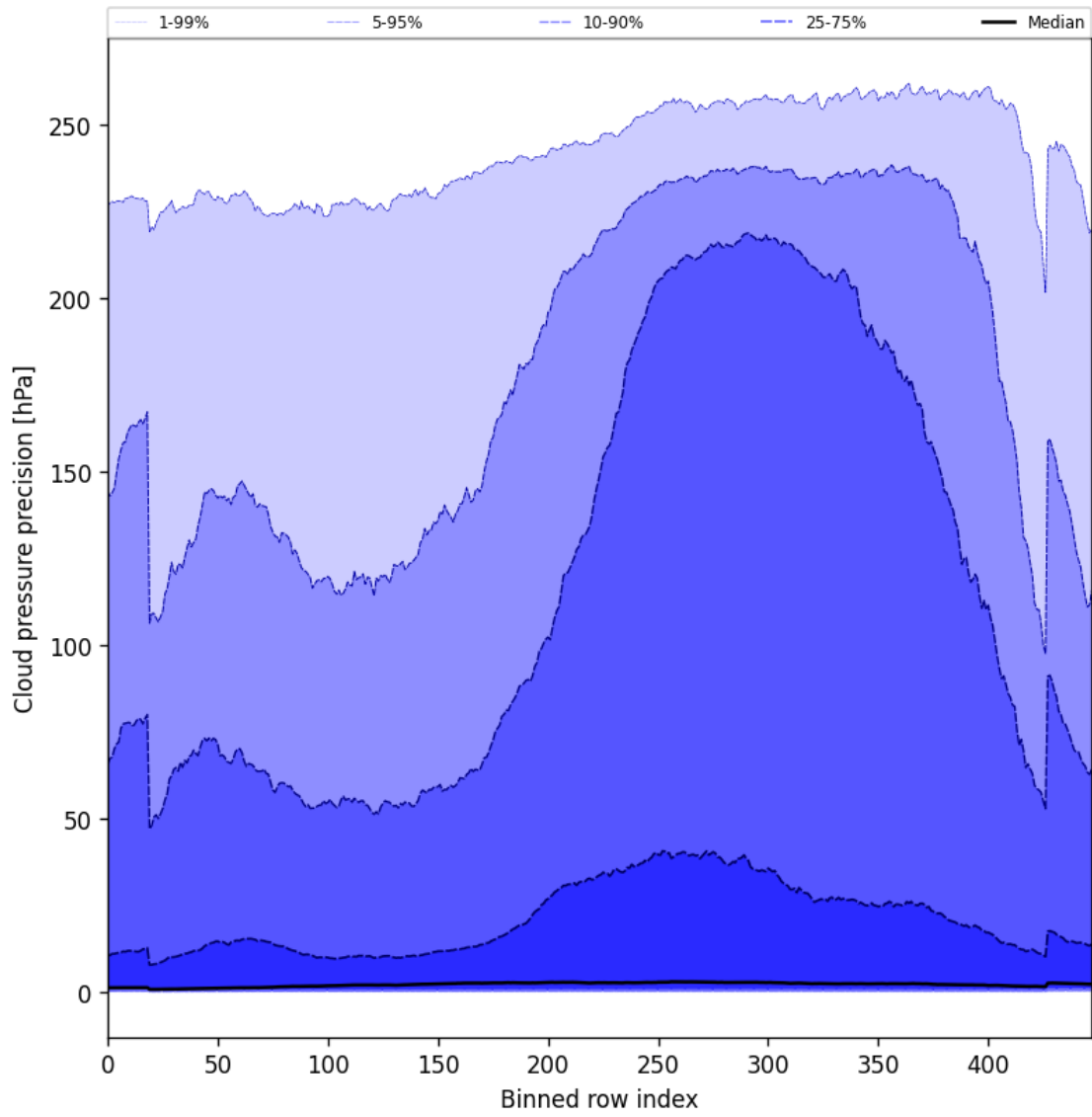
Figure 48: Along track statistics of “Cloud pressure precision” for 2024-10-30 to 2024-11-01
