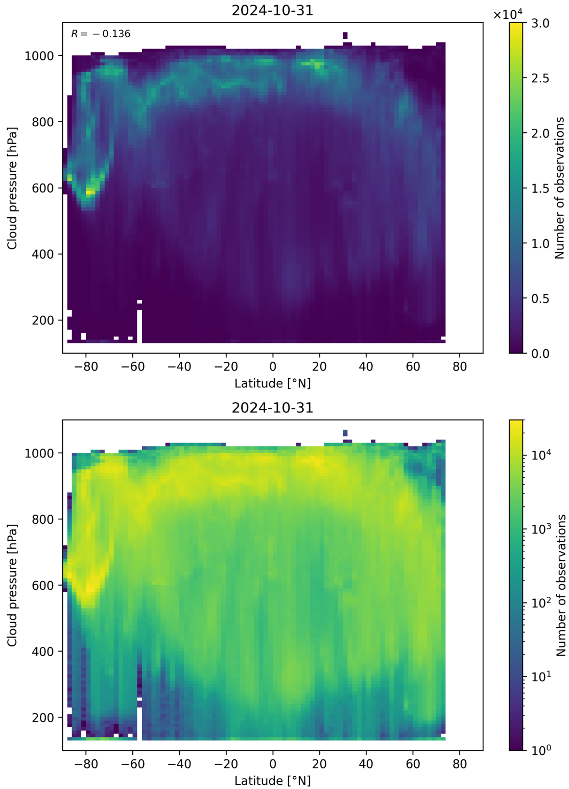
Figure 100: Scatter density plot of “Latitude” against “Cloud pressure” for 2024-10-30 to 2024-11-01.
