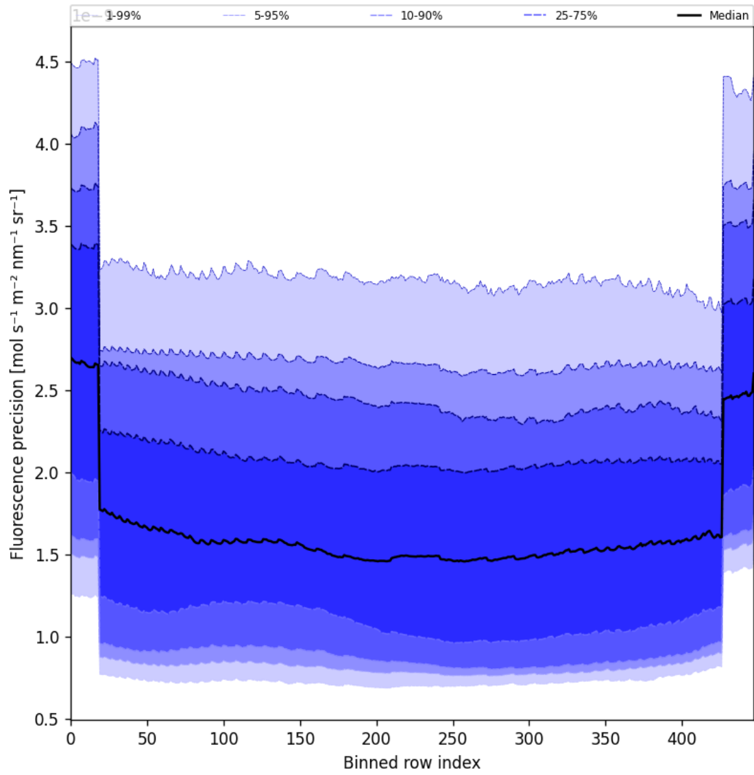
Figure 58: Along track statistics of “Fluorescence precision” for 2024-10-30 to 2024-11-01
