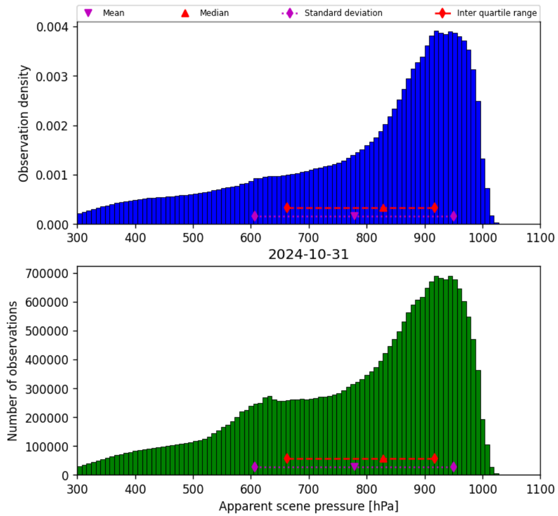
Figure 36: Histogram of “Apparent scene pressure” for 2024-10-30 to 2024-11-01
