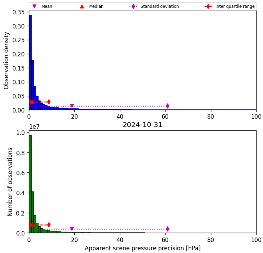
Figure 37: Histogram of “Apparent scene pressure precision” for 2024-10-30 to 2024-11-01
