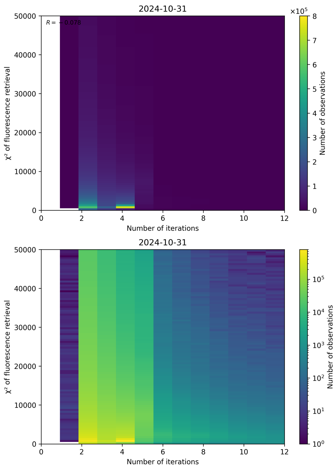
Figure 106: Scatter density plot of “Number of iterations” against “ \chi^2 of fluorescence retrieval” for 2024-10-30 to 2024-11-01.
