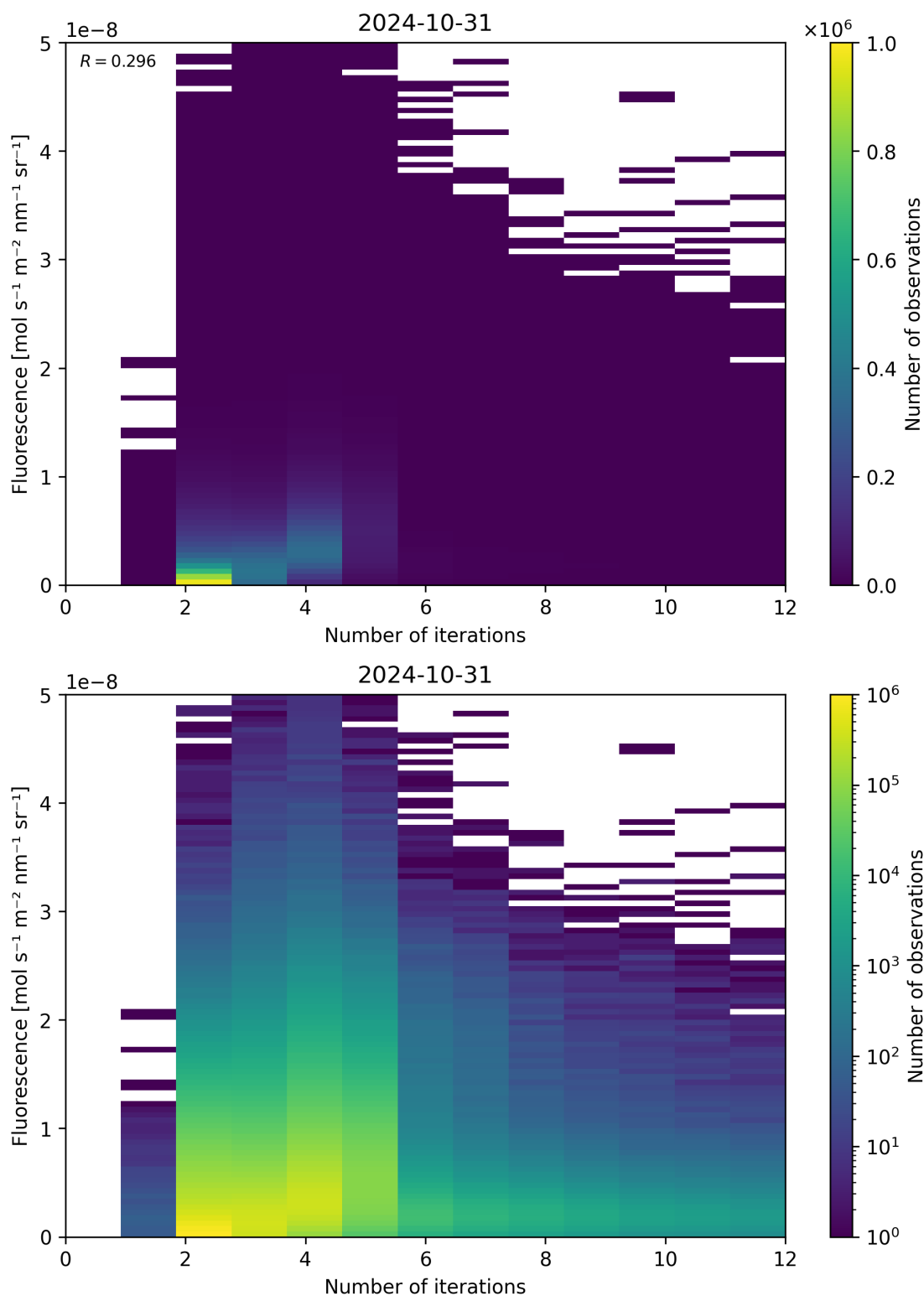
Figure 107: Scatter density plot of “Number of iterations” against “Fluorescence” for 2024-10-30 to 2024-11-01.
