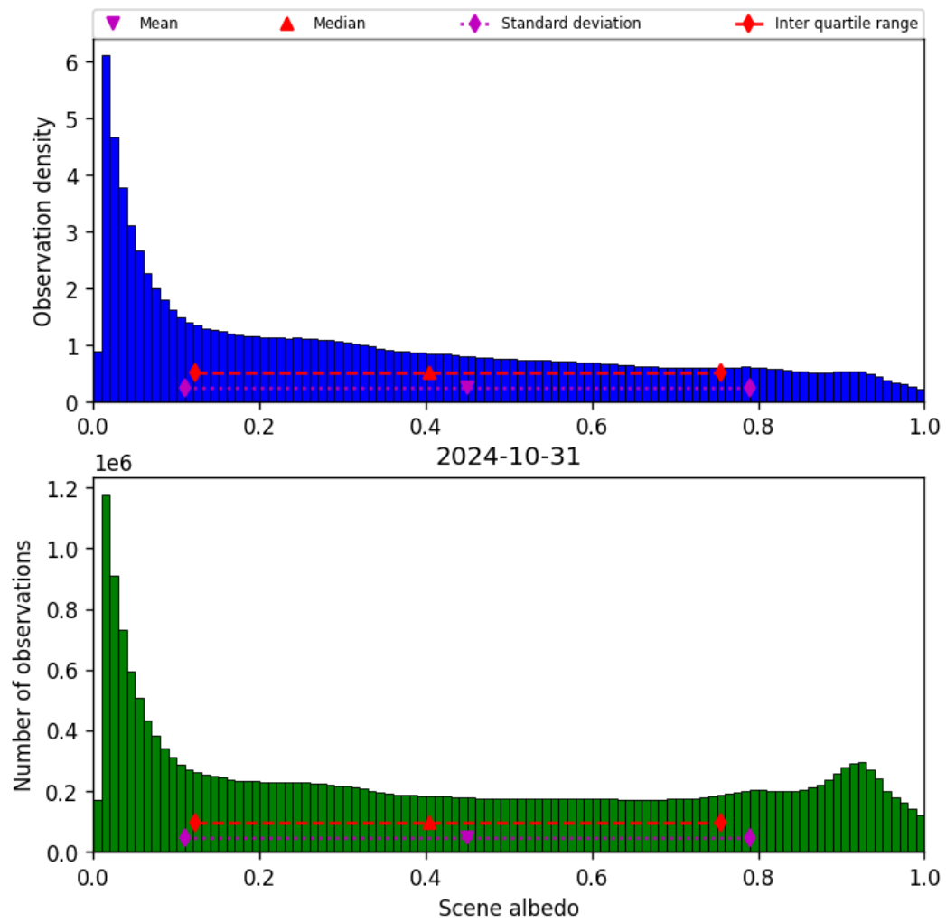
Figure 34: Histogram of “Scene albedo” for 2024-10-30 to 2024-11-01
