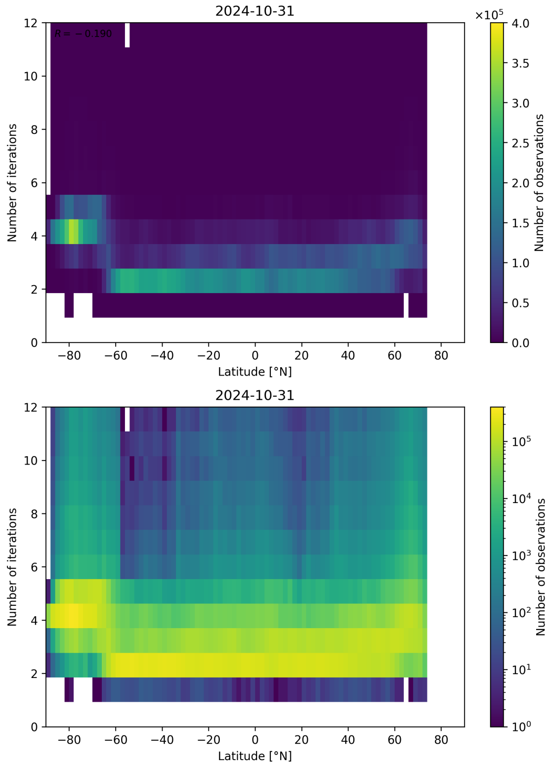
Figure 102: Scatter density plot of “Latitude” against “Number of iterations” for 2024-10-30 to 2024-11-01.
