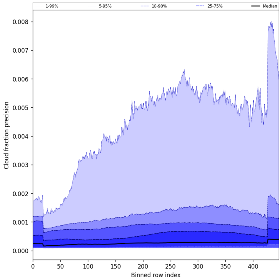
Figure 50: Along track statistics of “Cloud fraction precision” for 2024-10-30 to 2024-11-01
