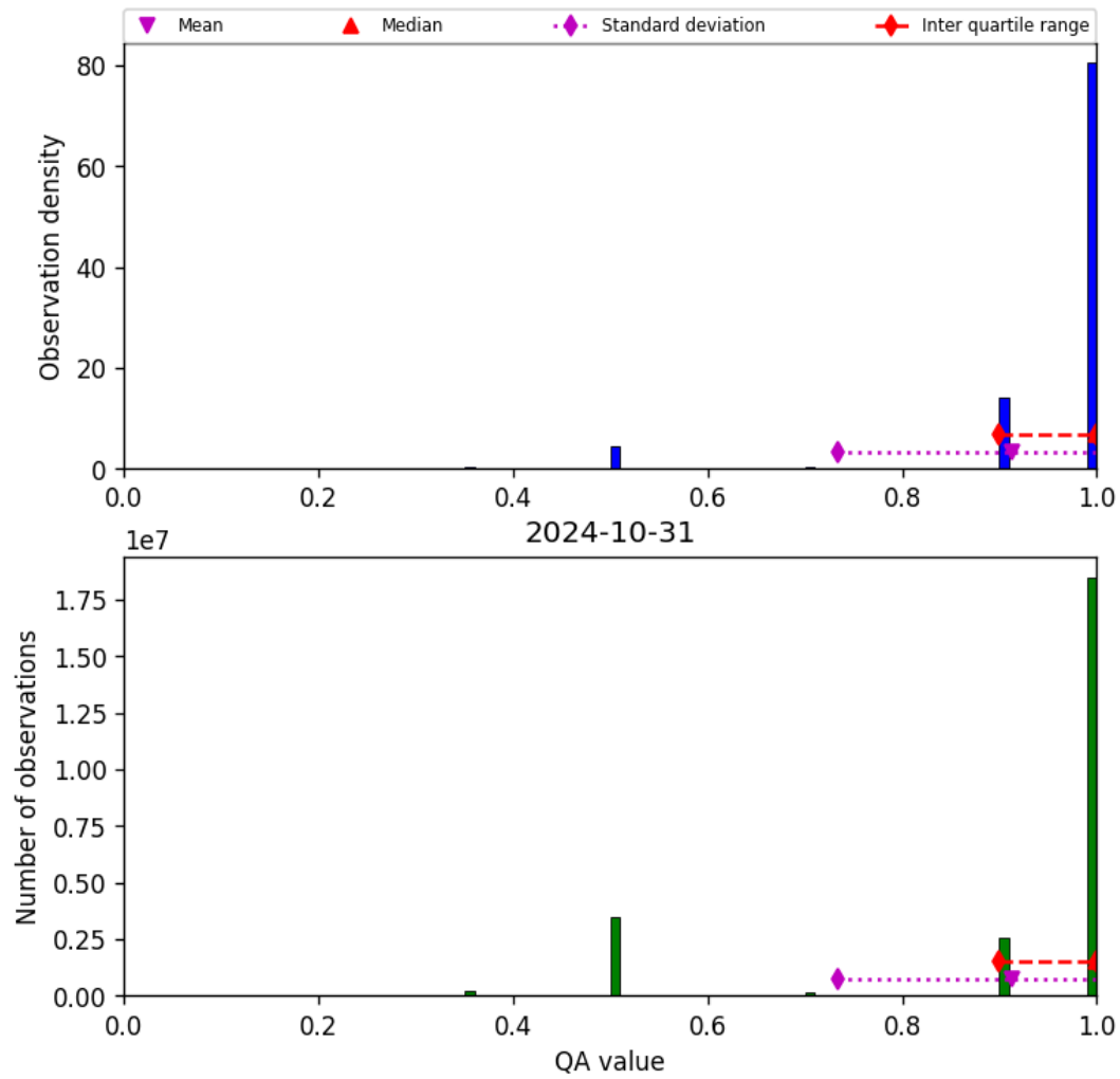
Figure 29: Histogram of “QA value” for 2024-10-30 to 2024-11-01
