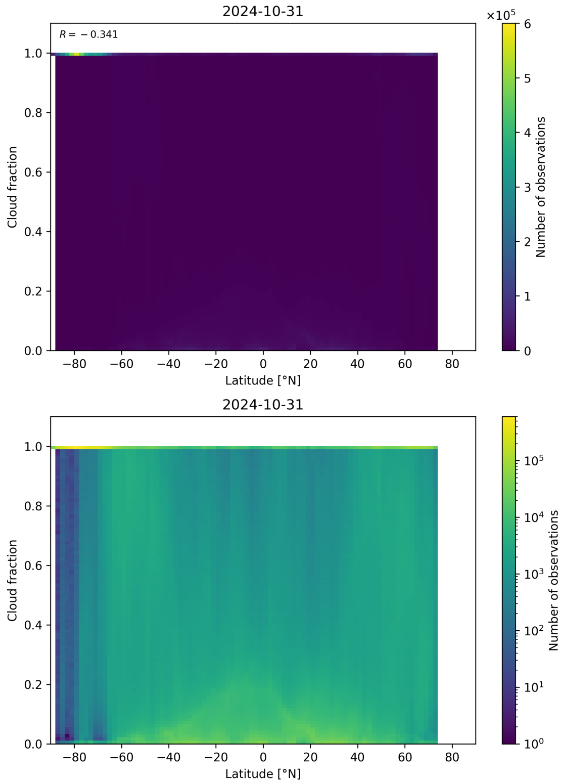
Figure 99: Scatter density plot of “Latitude” against “Cloud fraction” for 2024-10-30 to 2024-11-01.
