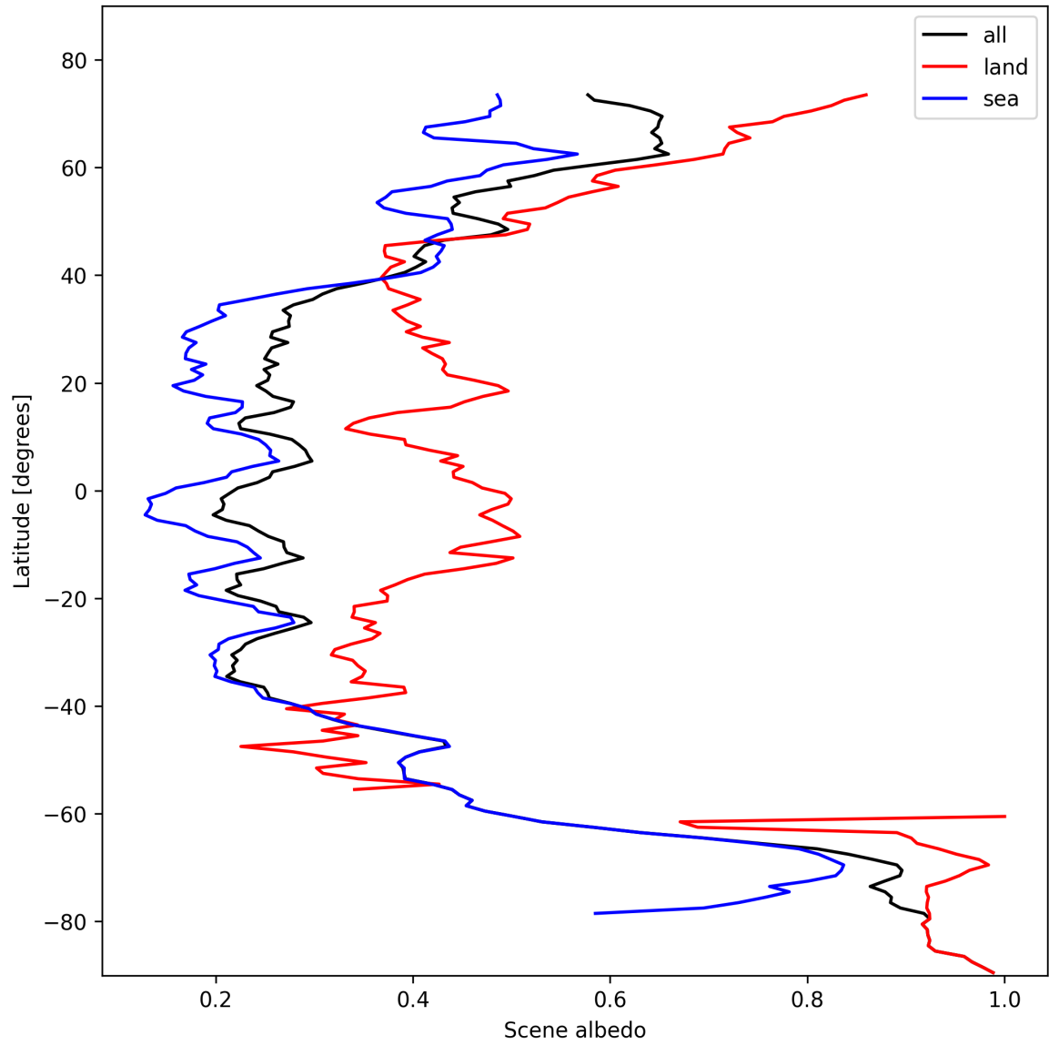
Figure 17: Zonal average of “Scene albedo” for 2024-10-30 to 2024-11-01.
