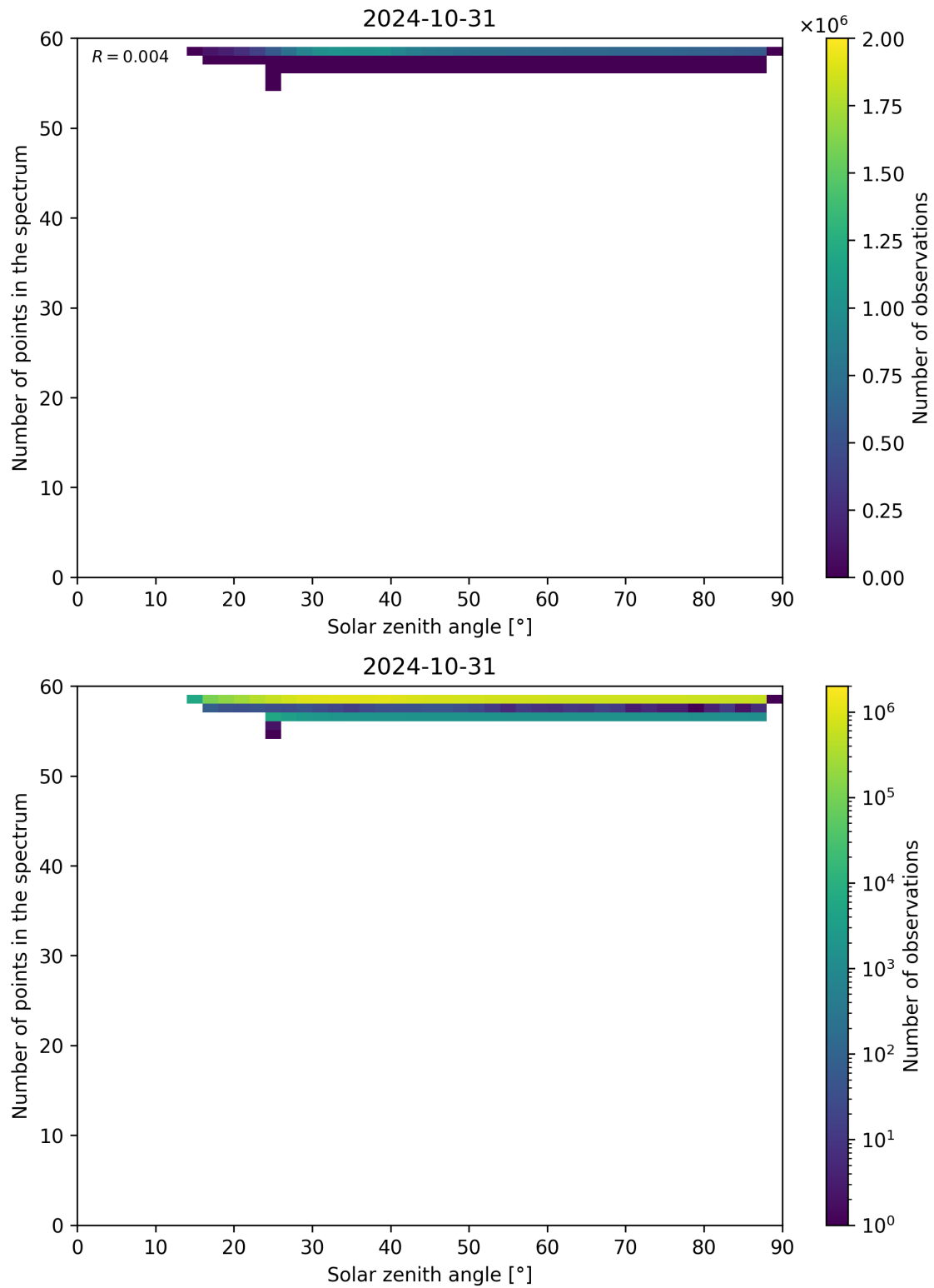
Figure 126: Scatter density plot of “Solar zenith angle” against “Number of points in the spectrum” for 2024-10-30 to 2024-11-01.
