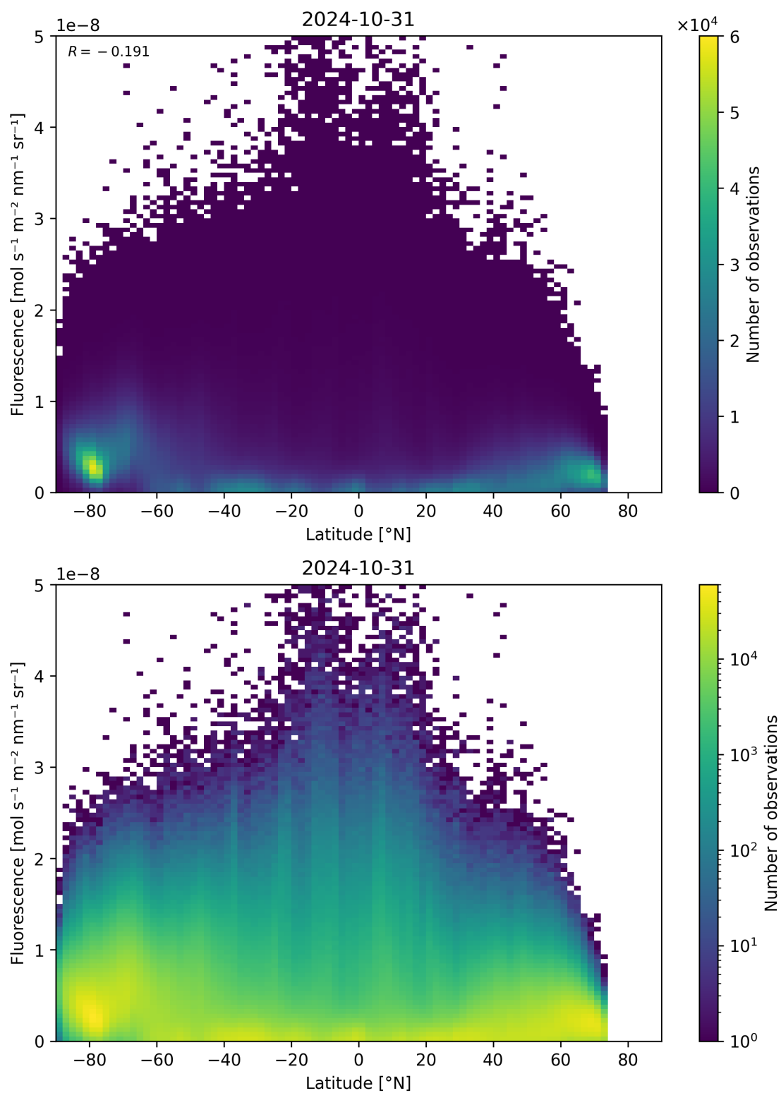
Figure 101: Scatter density plot of “Latitude” against “Fluorescence” for 2024-10-30 to 2024-11-01.
