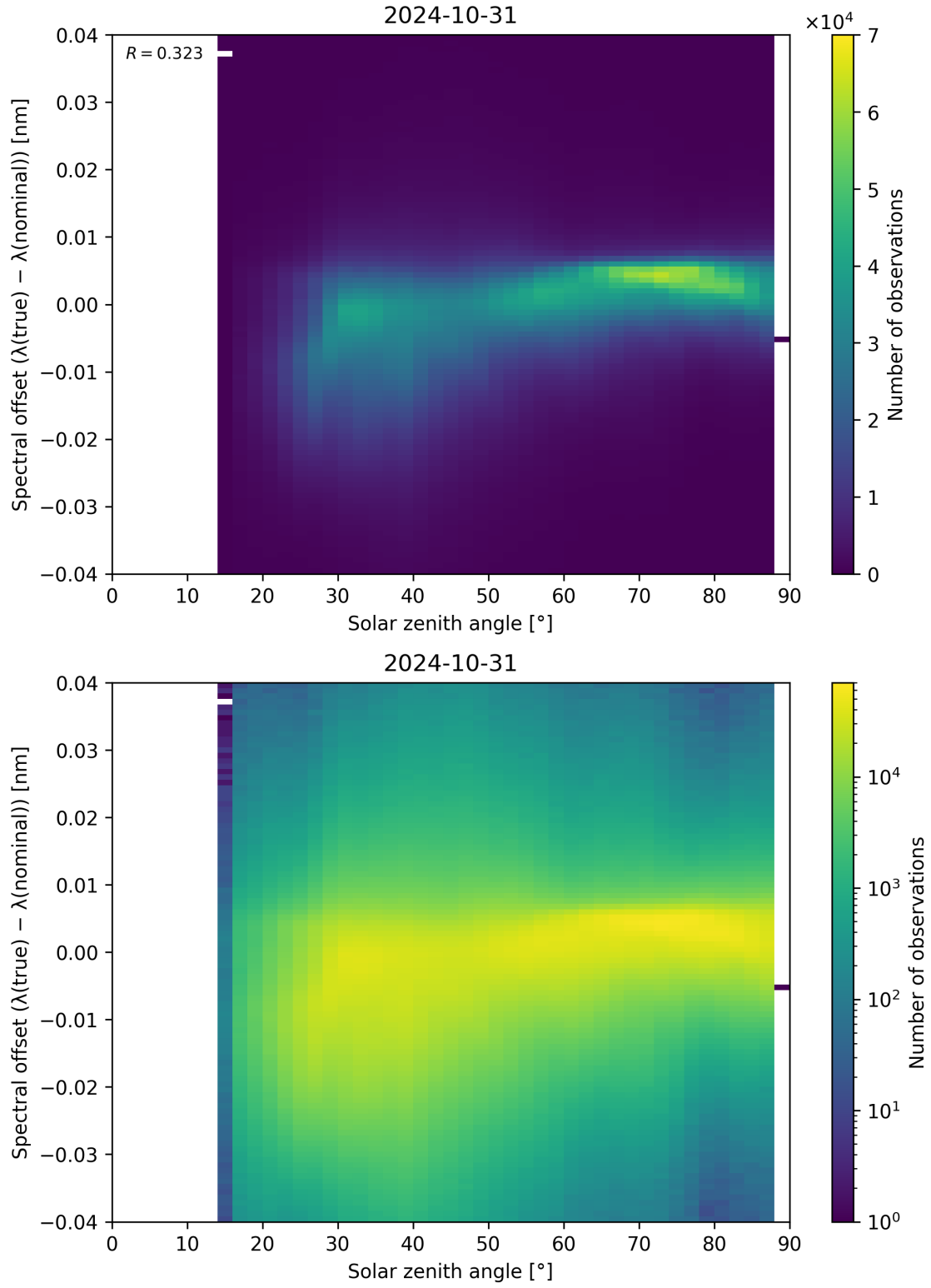
Figure 128: Scatter density plot of “Solar zenith angle” against “Spectral offset ( \lambda_{\text{true}} - \lambda_{\text{nominal}} )” for 2024-10-30 to 2024-11-01.
