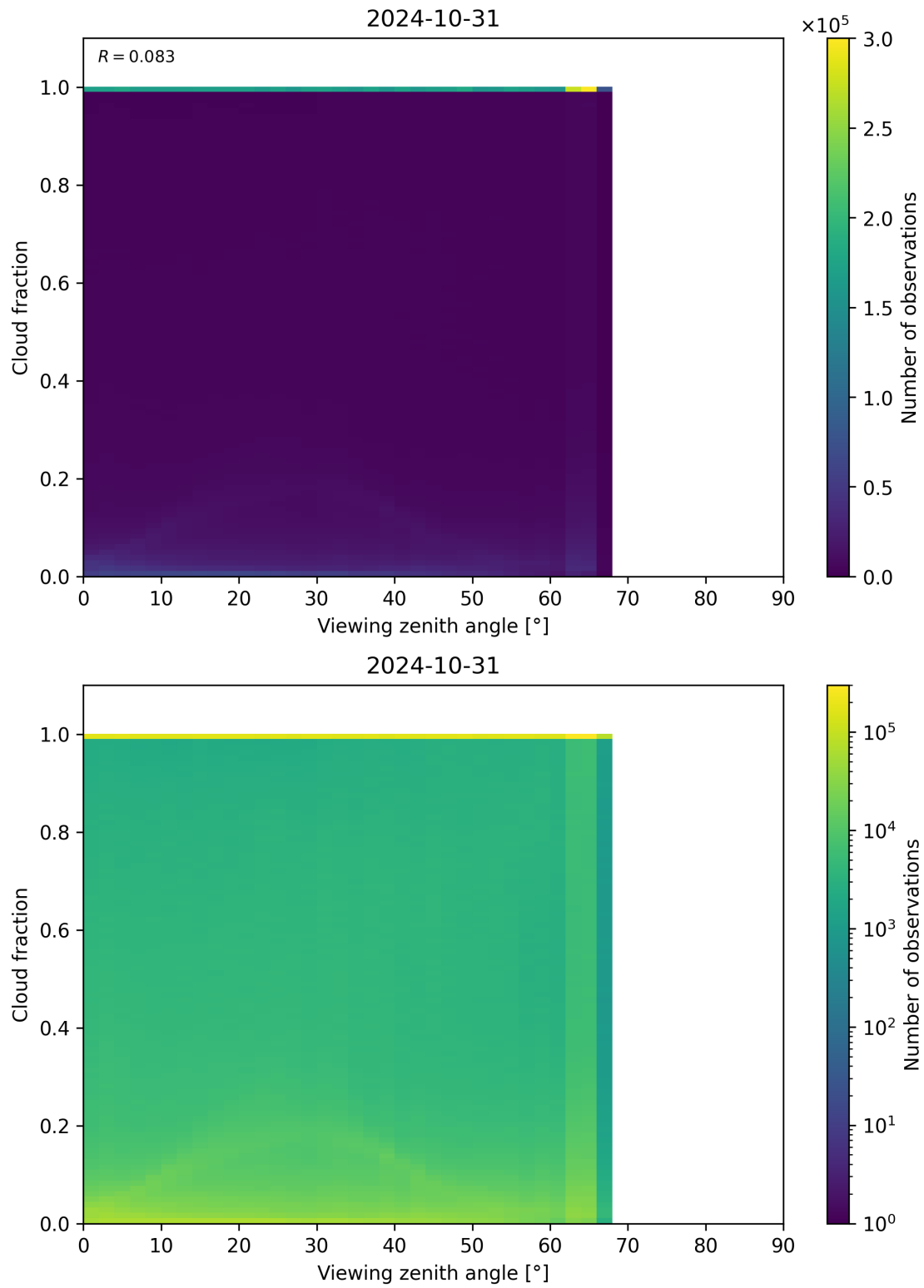
Figure 132: Scatter density plot of “Viewing zenith angle” against “Cloud fraction” for 2024-10-30 to 2024-11-01.
