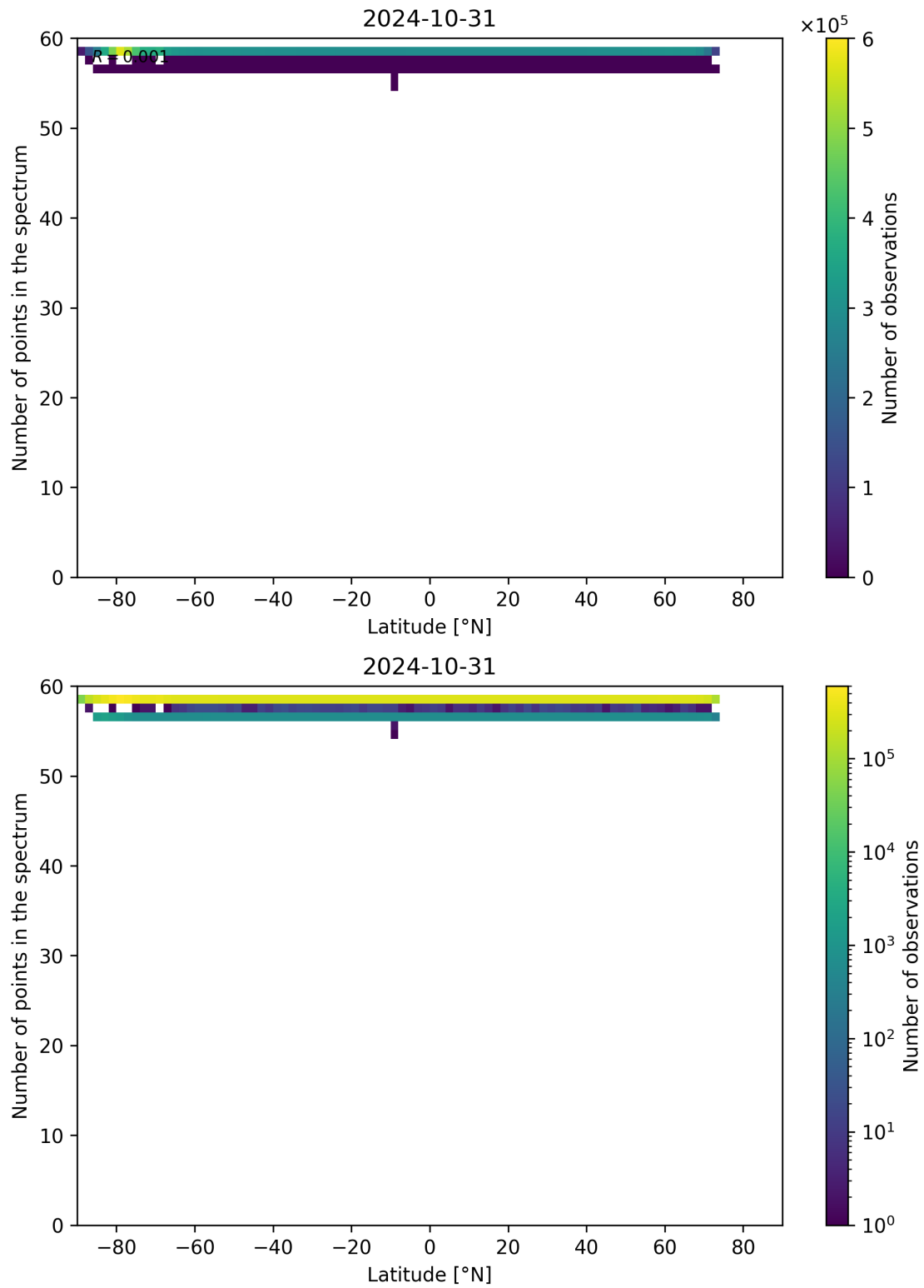
Figure 103: Scatter density plot of “Latitude” against “Number of points in the spectrum” for 2024-10-30 to 2024-11-01.
