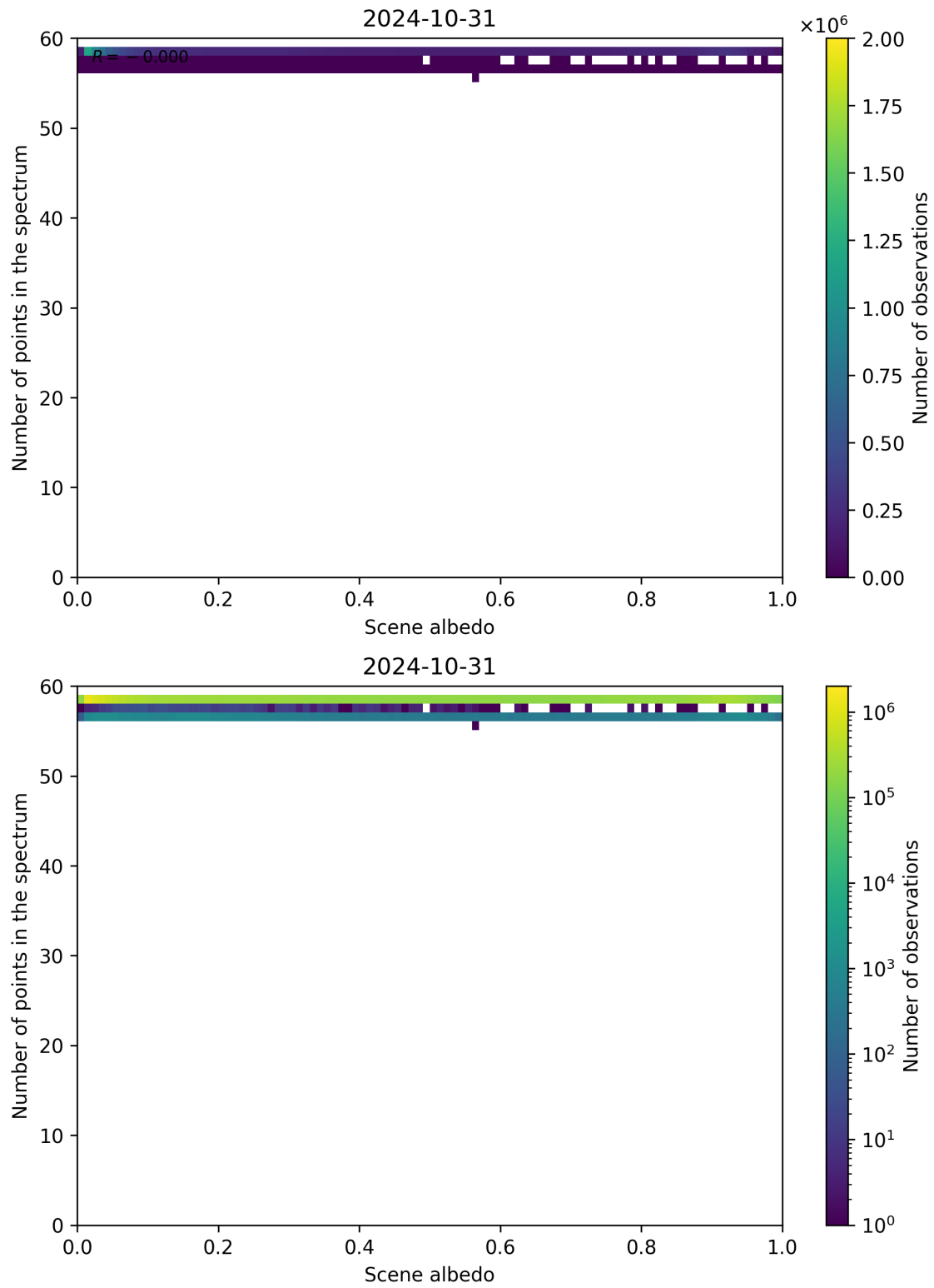
Figure 116: Scatter density plot of “Scene albedo” against “Number of points in the spectrum” for 2024-10-30 to 2024-11-01.
