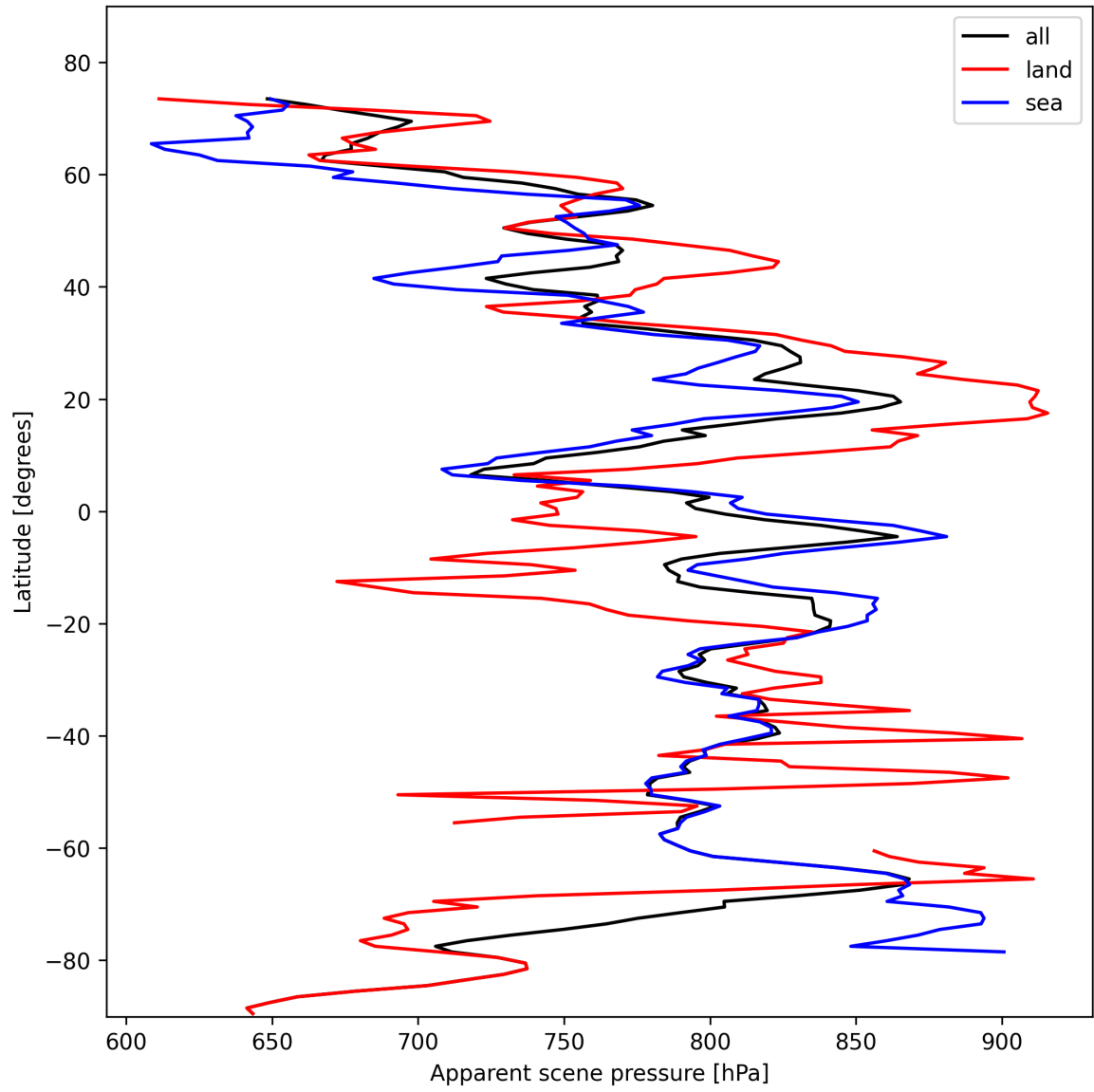
Figure 19: Zonal average of “Apparent scene pressure” for 2024-10-30 to 2024-11-01.
