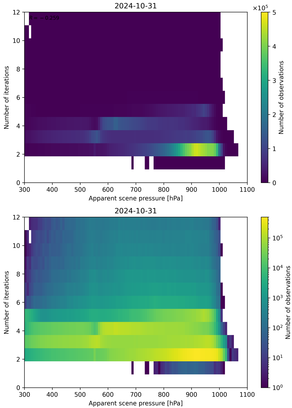
Figure 66: Scatter density plot of “Apparent scene pressure” against “Number of iterations” for 2024-10-30 to 2024-11-01.
