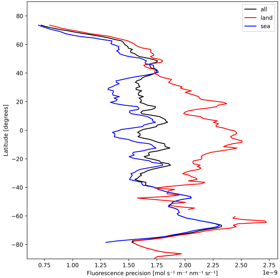
Figure 24: Zonal average of “Fluorescence precision” for 2024-10-30 to 2024-11-01.
