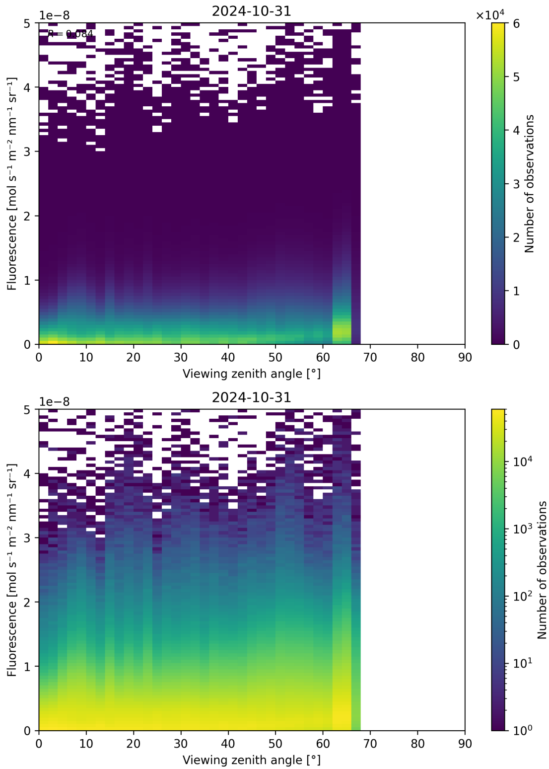
Figure 134: Scatter density plot of “Viewing zenith angle” against “Fluorescence” for 2024-10-30 to 2024-11-01.
