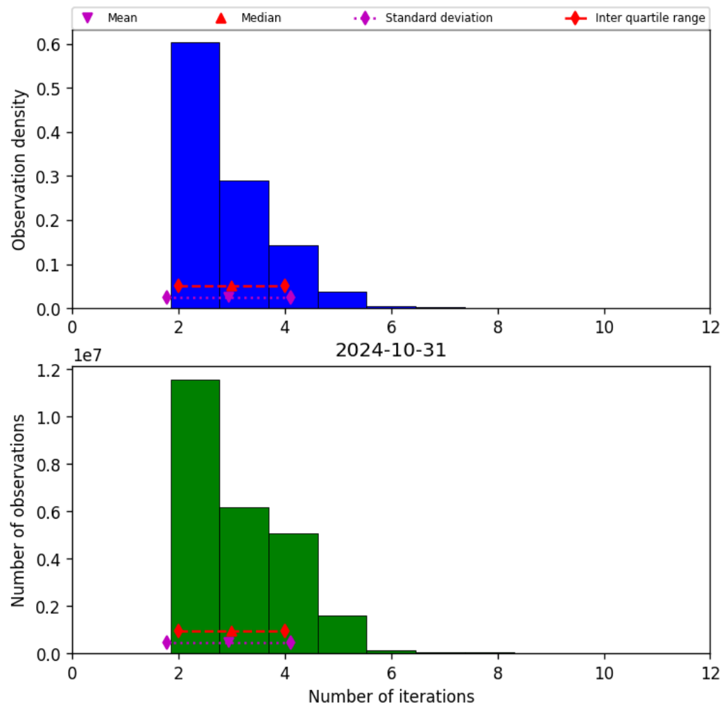
Figure 39: Histogram of “Number of iterations” for 2024-10-30 to 2024-11-01
