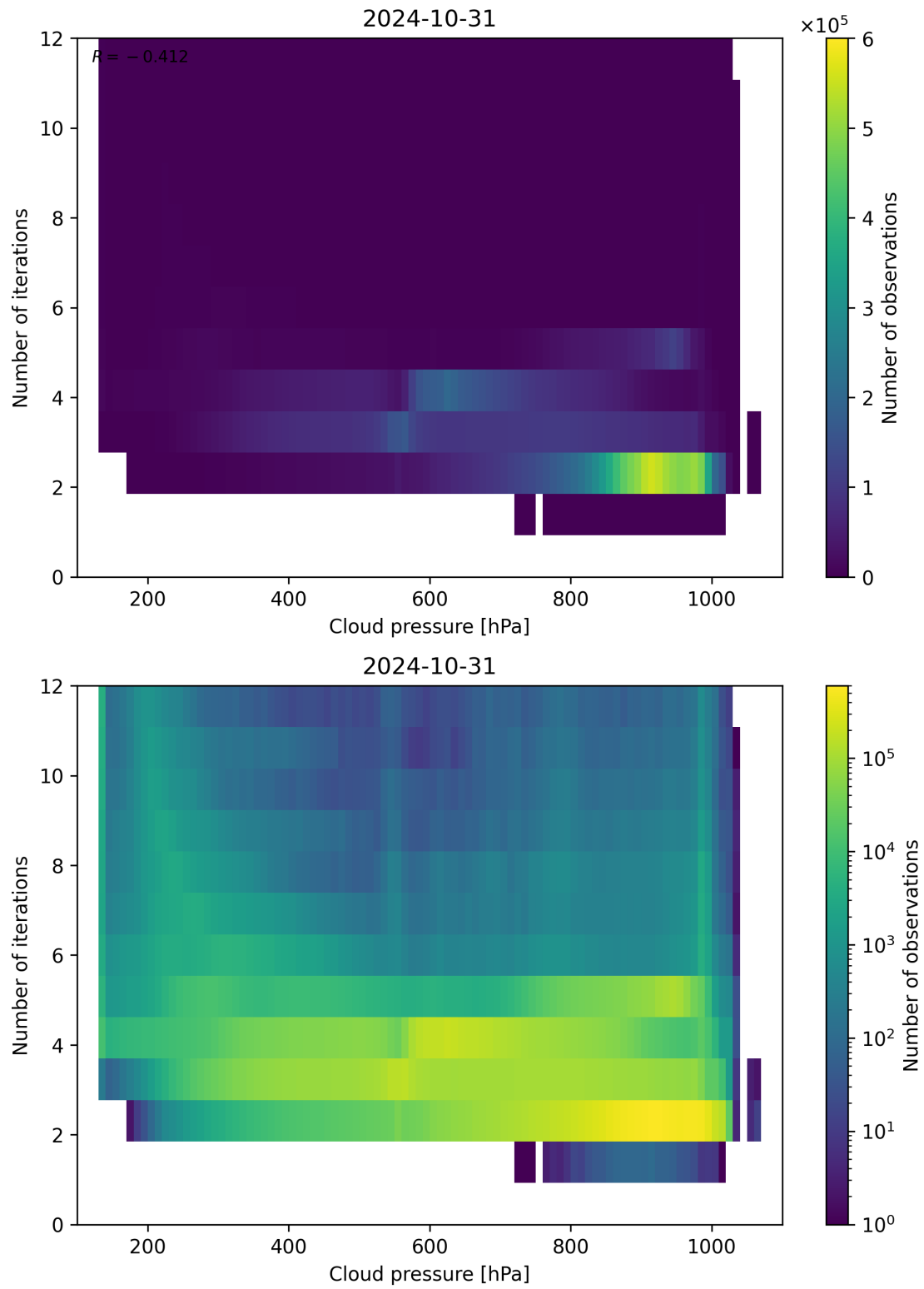
Figure 89: Scatter density plot of “Cloud pressure” against “Number of iterations” for 2024-10-30 to 2024-11-01.
