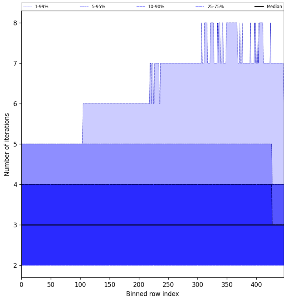
Figure 56: Along track statistics of “Number of iterations” for 2024-10-30 to 2024-11-01
