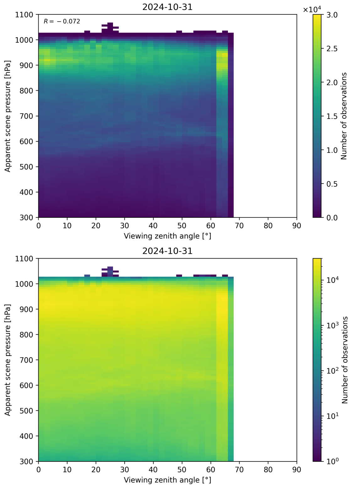
Figure 129: Scatter density plot of “Viewing zenith angle” against “Apparent scene pressure” for 2024-10-30 to 2024-11-01.
