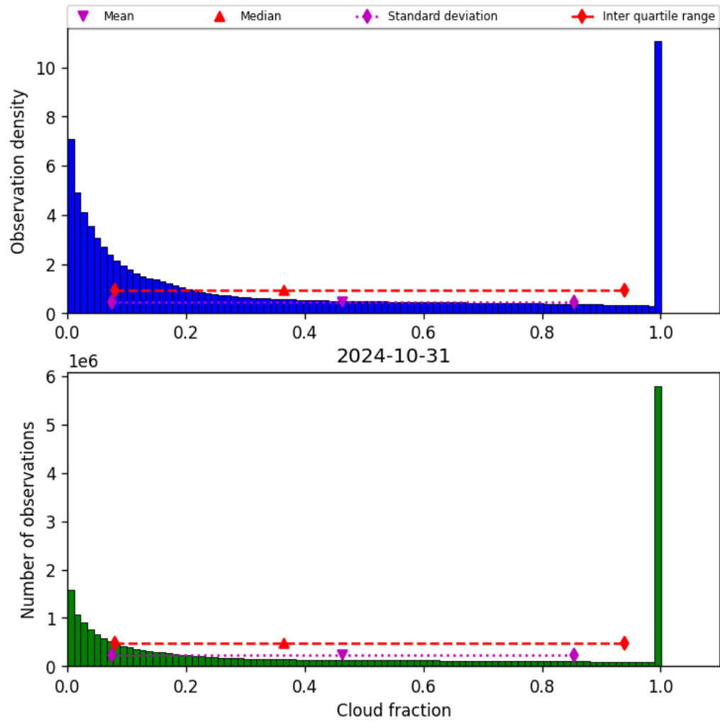
Figure 32: Histogram of “Cloud fraction” for 2024-10-30 to 2024-11-01
