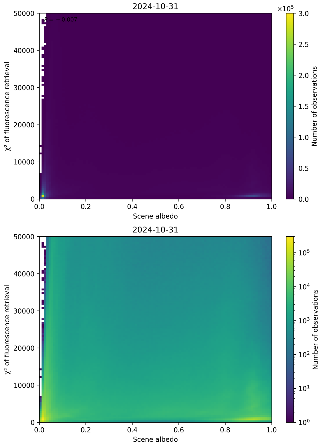
Figure 113: Scatter density plot of “Scene albedo” against “ \chi^2 of fluorescence retrieval” for 2024-10-30 to 2024-11-01.
