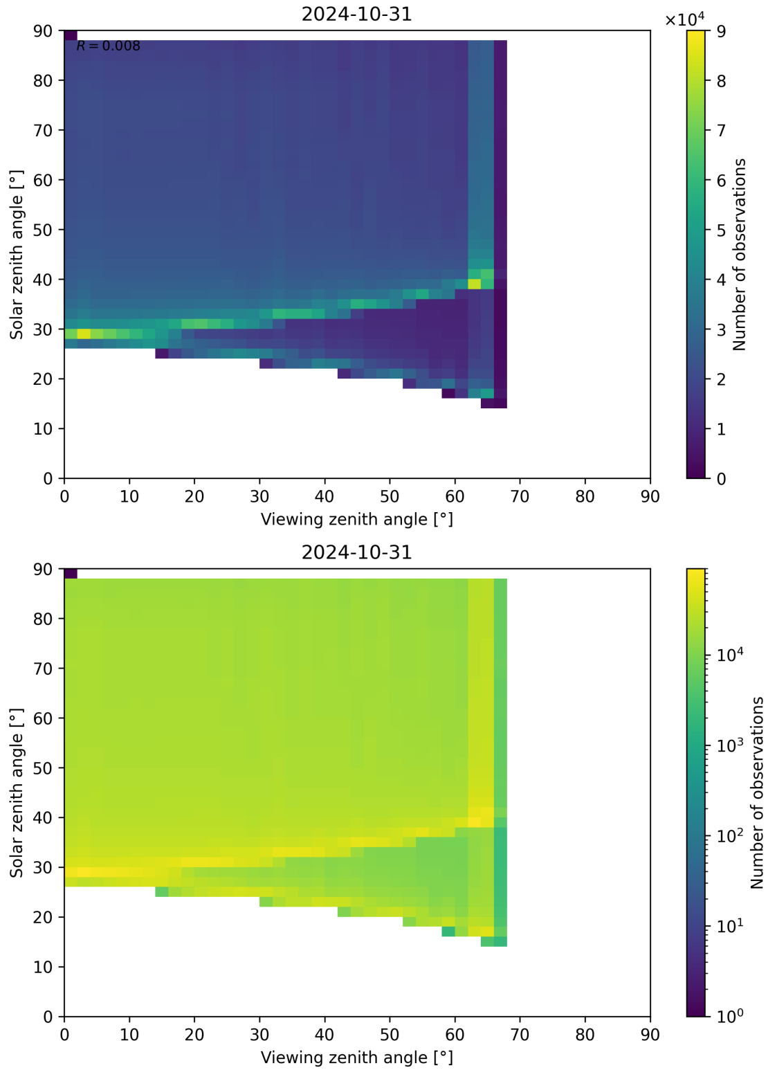
Figure 139: Scatter density plot of “Viewing zenith angle” against “Solar zenith angle” for 2024-10-30 to 2024-11-01.
