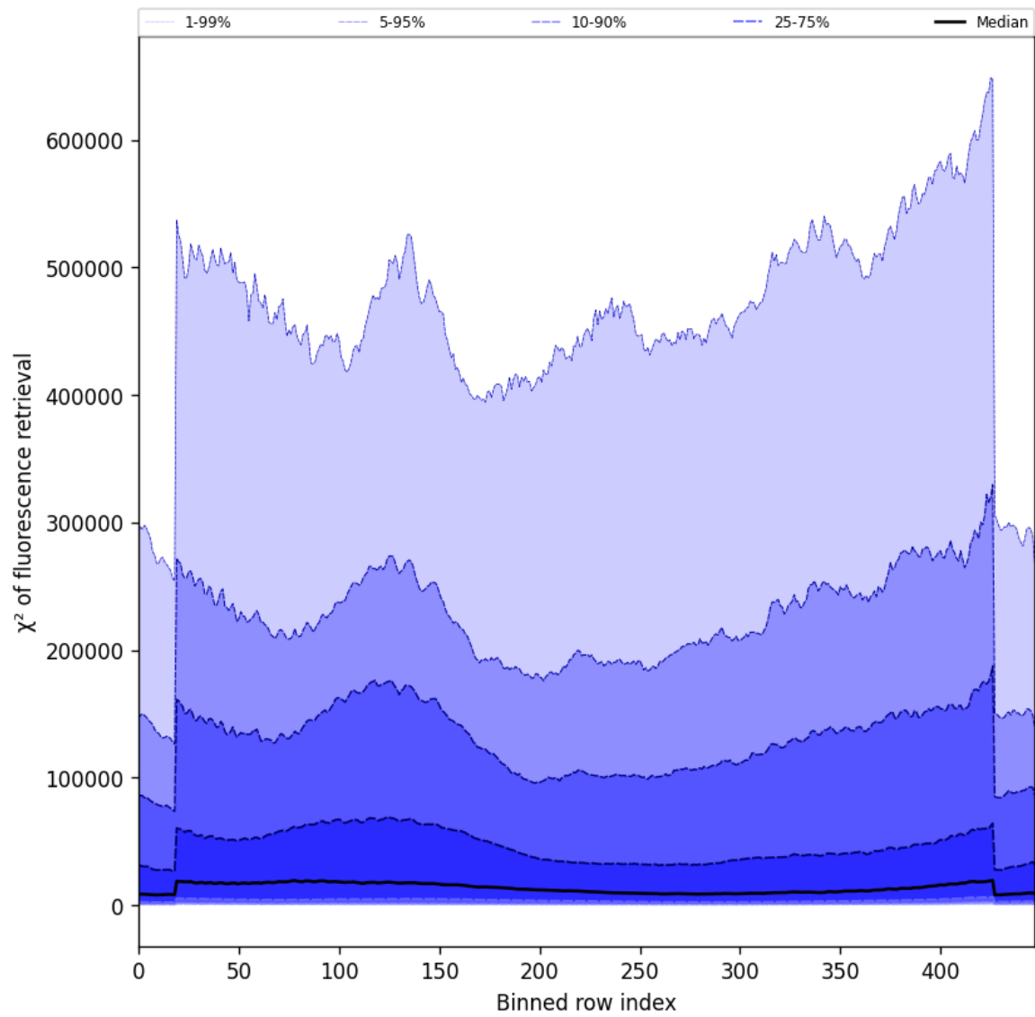
Figure 59: Along track statistics of " \chi^2 of fluorescence retrieval" for 2024-10-30 to 2024-11-01
