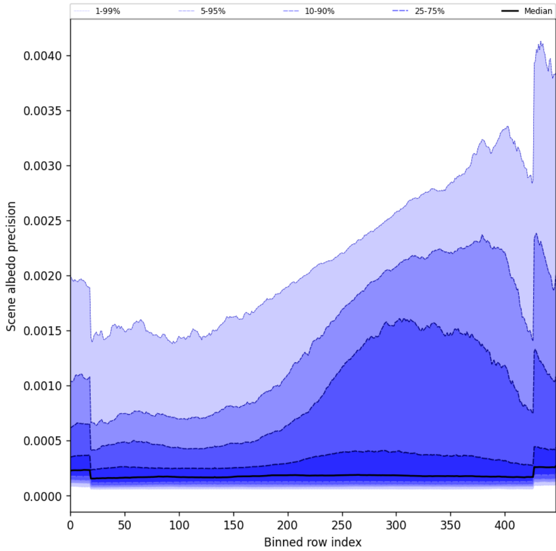
Figure 52: Along track statistics of “Scene albedo precision” for 2024-10-30 to 2024-11-01
