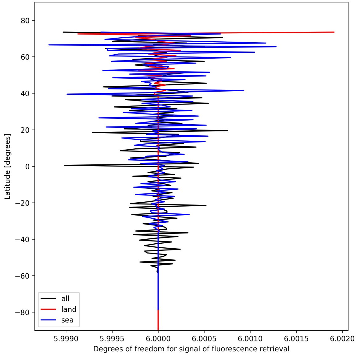
Figure 26: Zonal average of “Degrees of freedom for signal of fluorescence retrieval” for 2024-10-30 to 2024-11-01.
