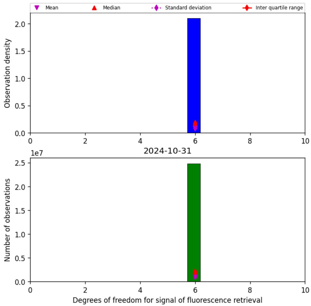
Figure 43: Histogram of “Degrees of freedom for signal of fluorescence retrieval” for 2024-10-30 to 2024-11-01
