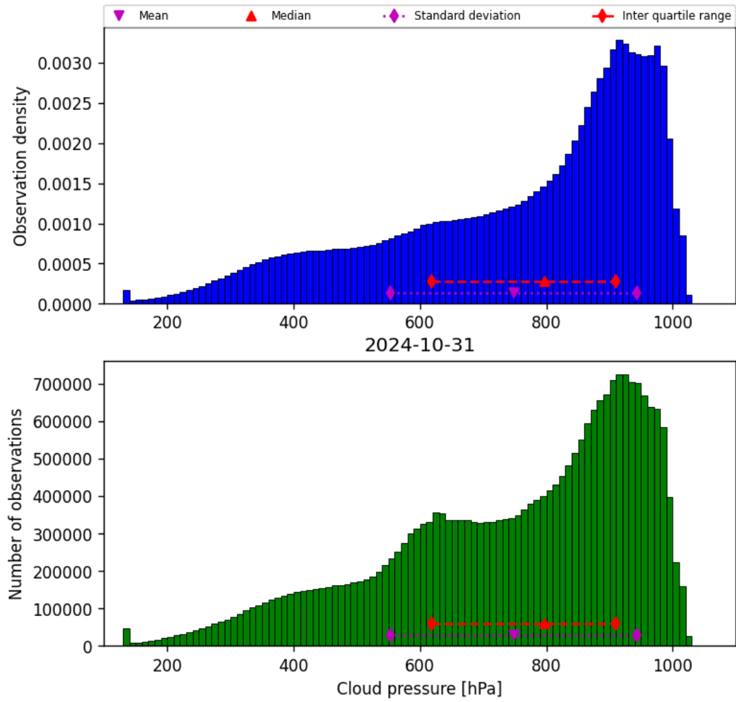
Figure 30: Histogram of “Cloud pressure” for 2024-10-30 to 2024-11-01
