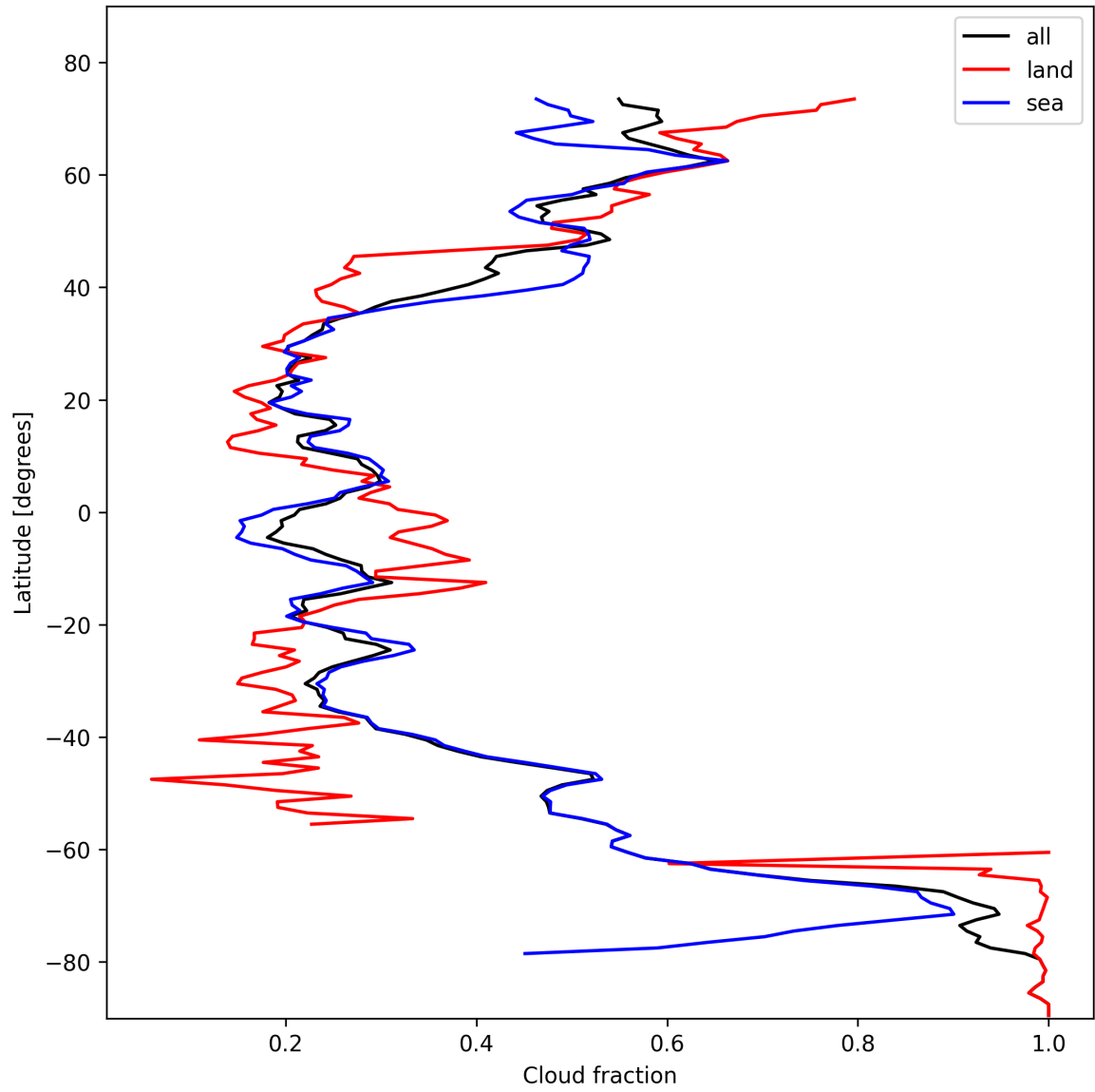
Figure 15: Zonal average of “Cloud fraction” for 2024-10-30 to 2024-11-01.
