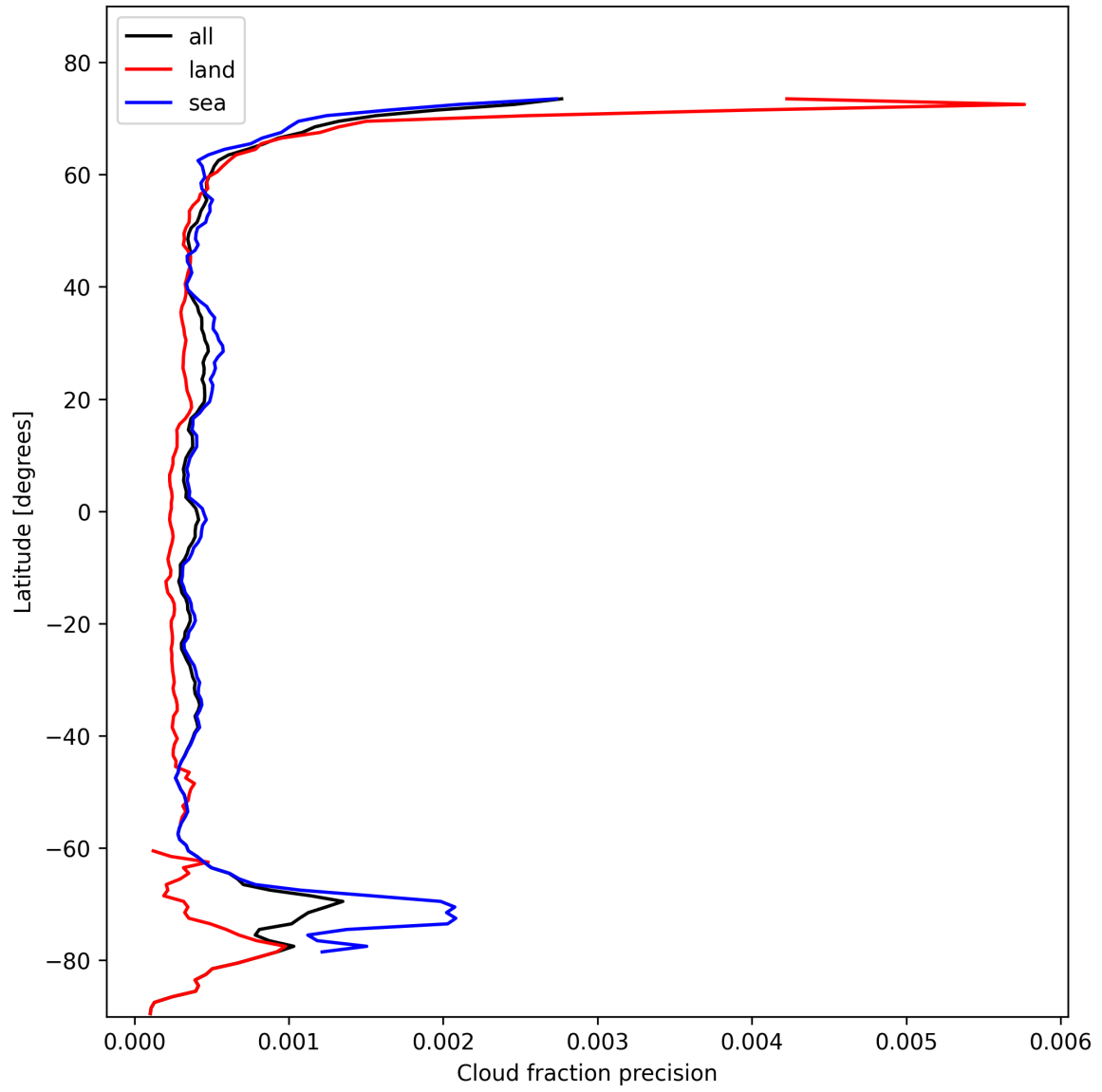
Figure 16: Zonal average of “Cloud fraction precision” for 2024-10-30 to 2024-11-01.
