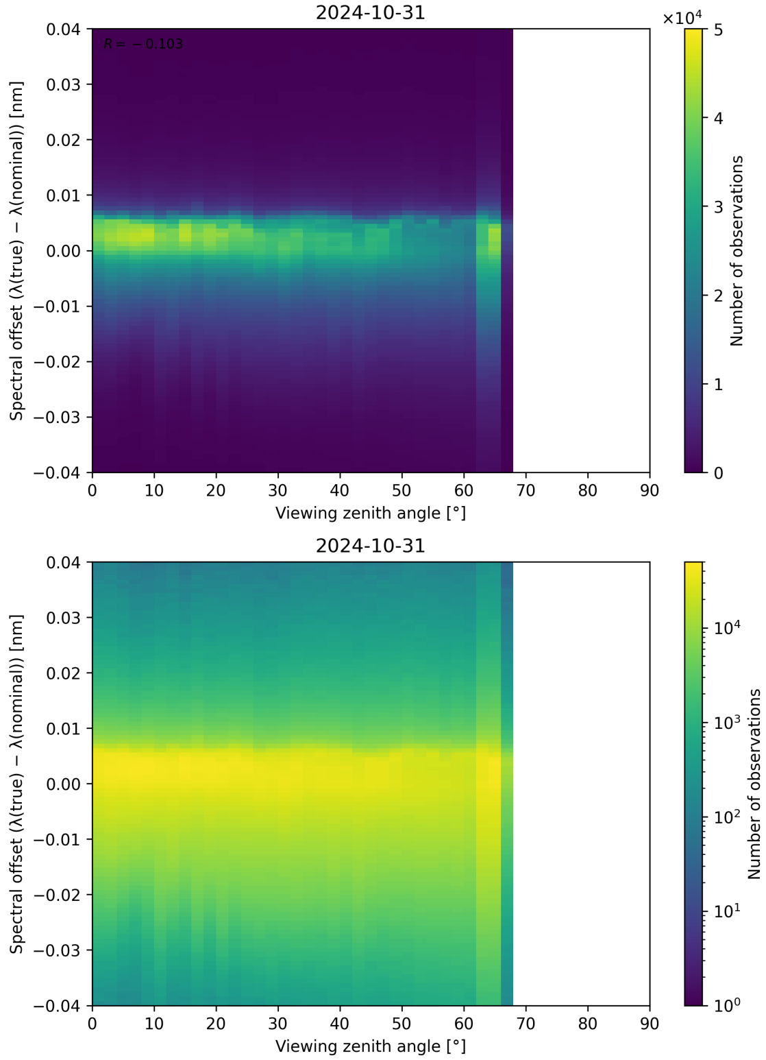
Figure 140: Scatter density plot of “Viewing zenith angle” against “Spectral offset ( \lambda_{\text{true}} - \lambda_{\text{nominal}} )” for 2024-10-30 to 2024-11-01.
