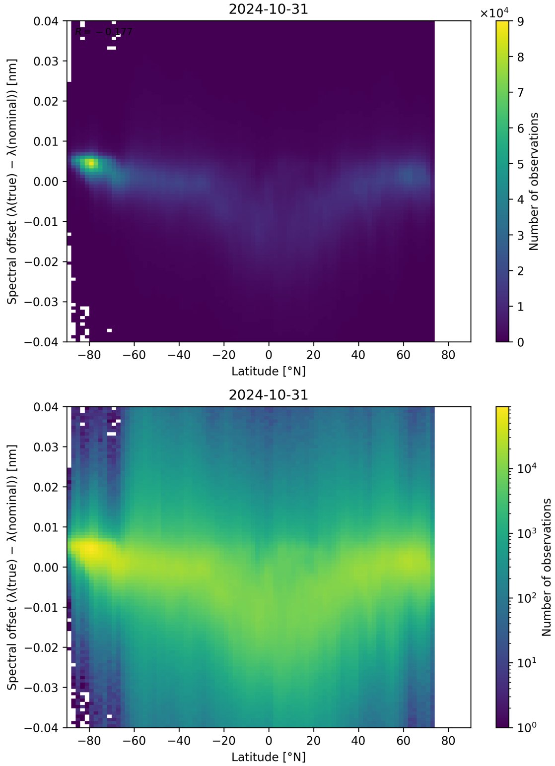
Figure 105: Scatter density plot of “Latitude” against “Spectral offset ( \lambda_{\text{true}} - \lambda_{\text{nominal}} )” for 2024-10-30 to 2024-11-01.
