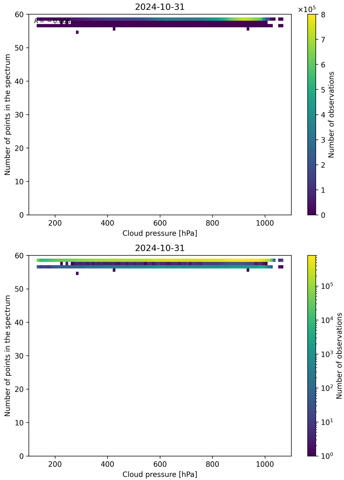
Figure 90: Scatter density plot of “Cloud pressure” against “Number of points in the spectrum” for 2024-10-30 to 2024-11-01.
