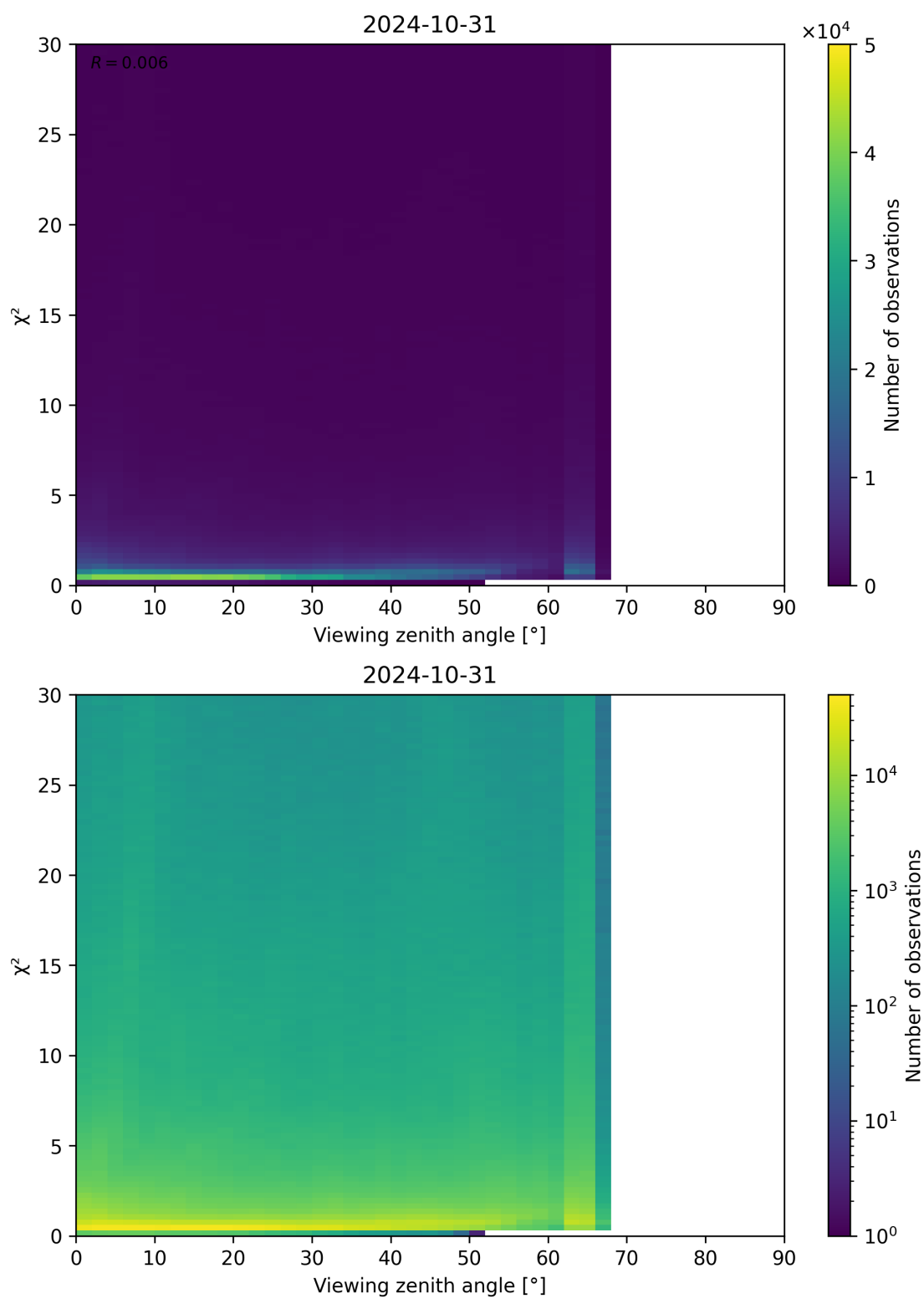
Figure 130: Scatter density plot of “Viewing zenith angle” against “ \chi^2 ” for 2024-10-30 to 2024-11-01.
