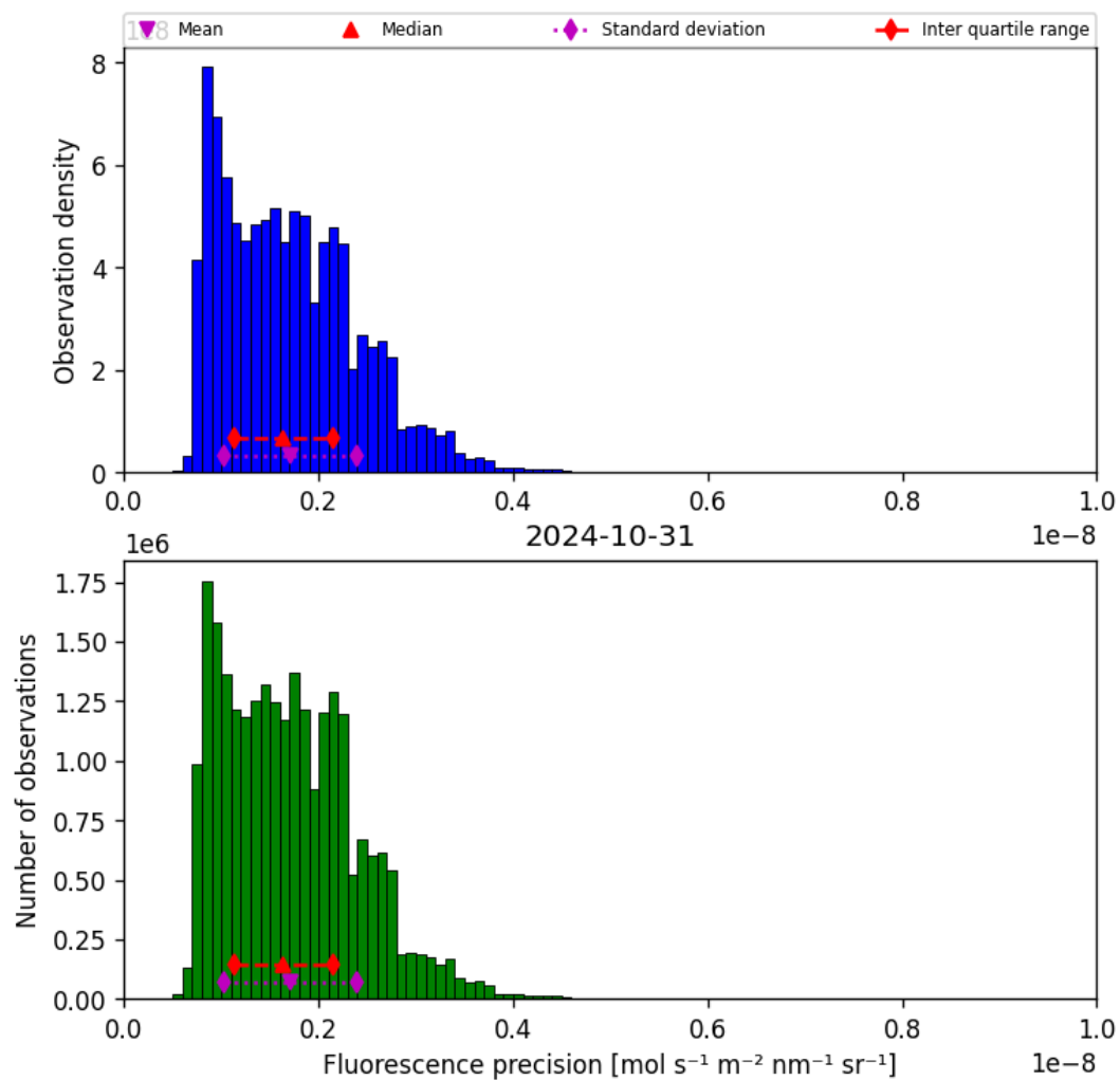
Figure 41: Histogram of “Fluorescence precision” for 2024-10-30 to 2024-11-01
