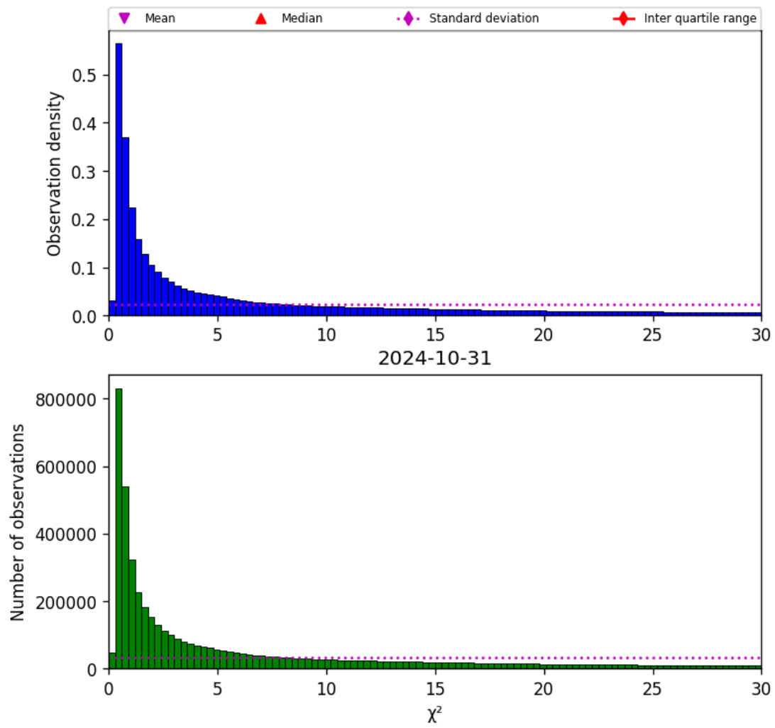
Figure 38: Histogram of " \chi^2 " for 2024-10-30 to 2024-11-01
