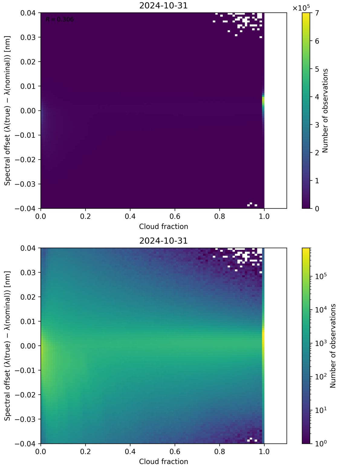
Figure 83: Scatter density plot of “Cloud fraction” against “Spectral offset ( \lambda_{\text{true}} - \lambda_{\text{nominal}} )” for 2024-10-30 to 2024-11-01.
