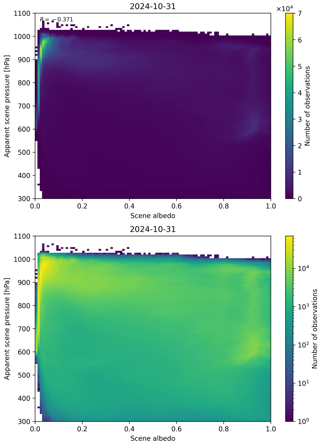
Figure 111: Scatter density plot of “Scene albedo” against “Apparent scene pressure” for 2024-10-30 to 2024-11-01.
