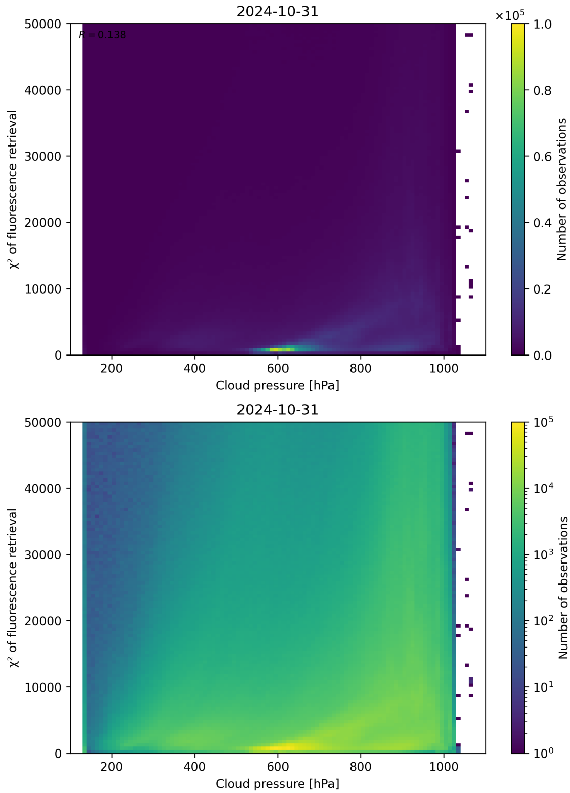
Figure 86: Scatter density plot of “Cloud pressure” against “ \chi^2 of fluorescence retrieval” for 2024-10-30 to 2024-11-01.
