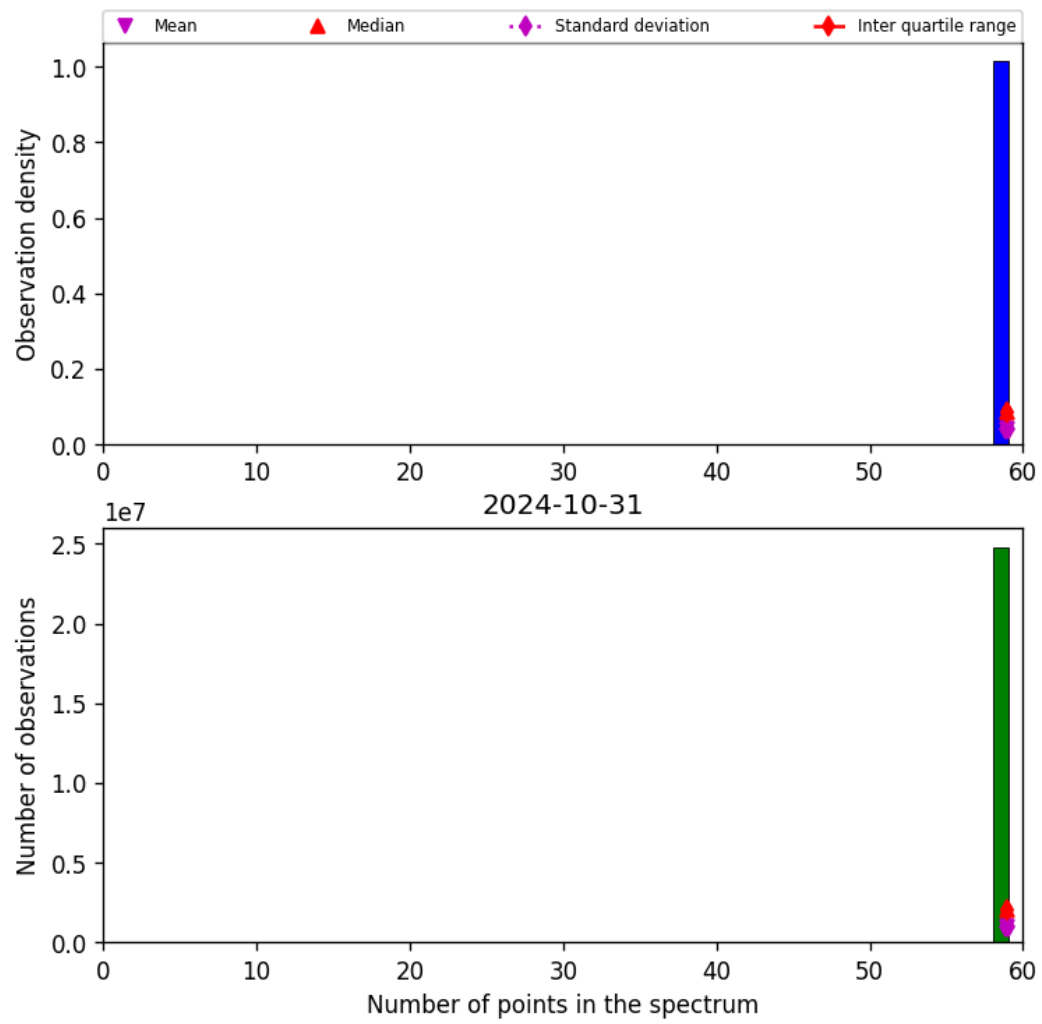
Figure 44: Histogram of “Number of points in the spectrum” for 2024-10-30 to 2024-11-01
