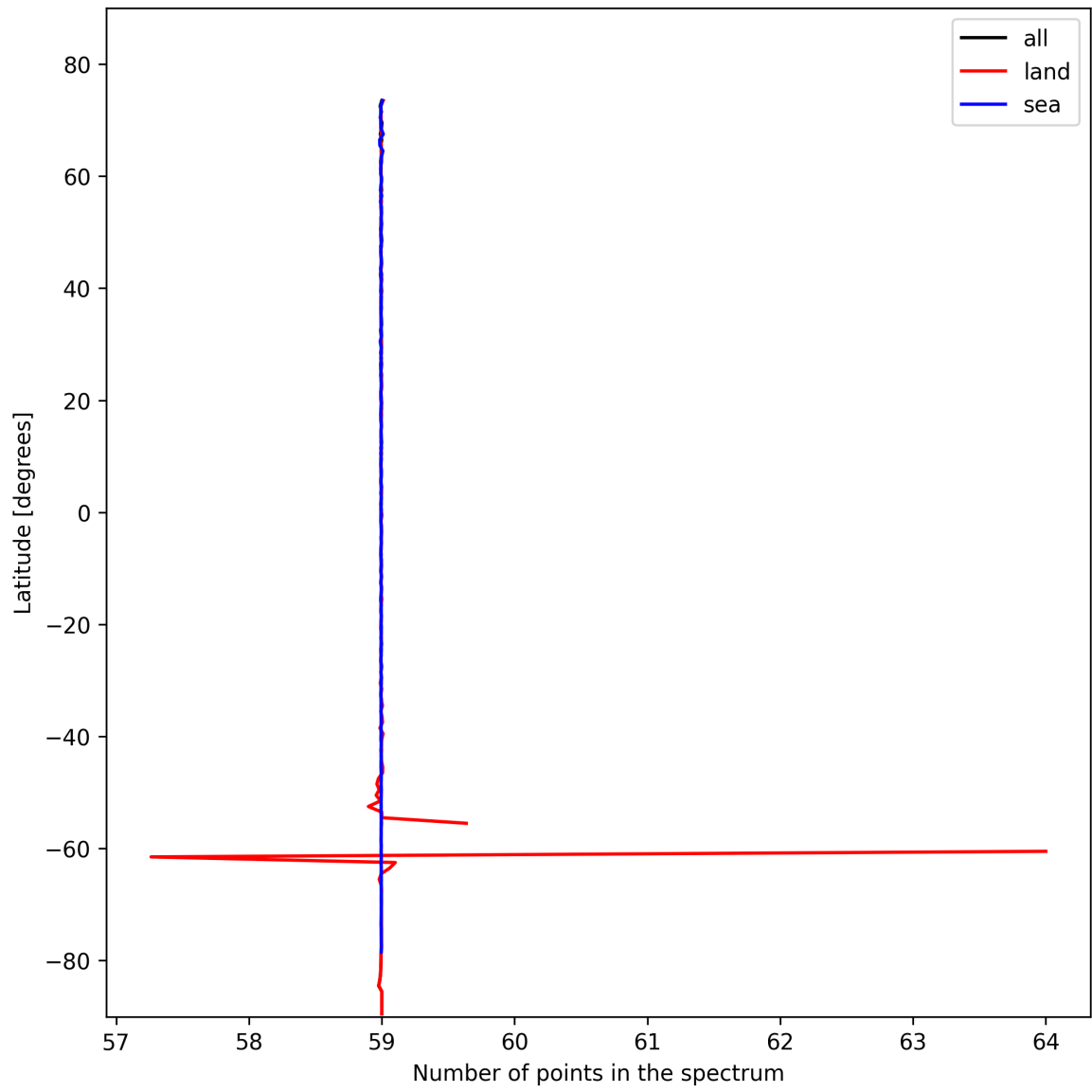
Figure 27: Zonal average of “Number of points in the spectrum” for 2024-10-30 to 2024-11-01.
