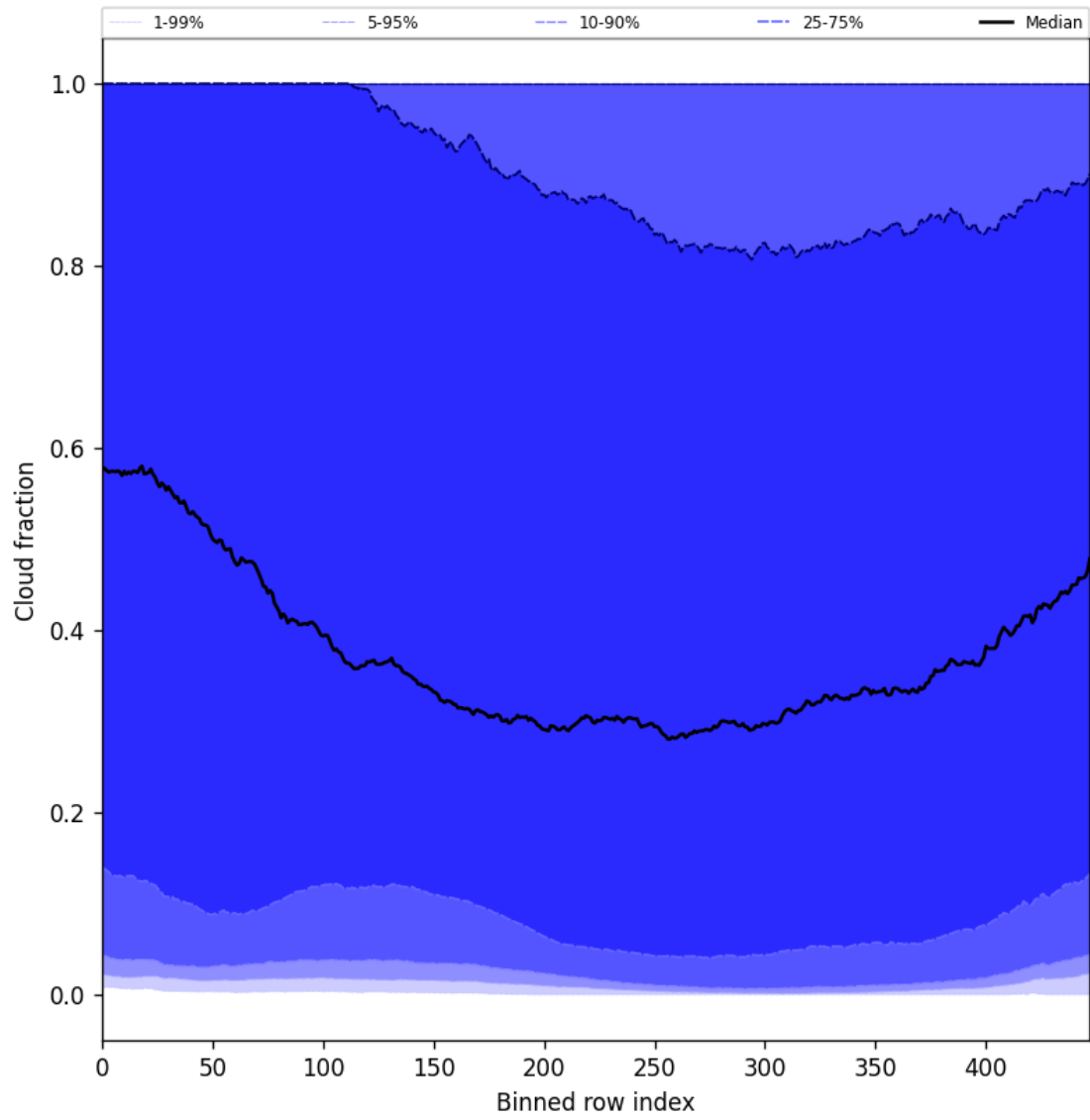
Figure 49: Along track statistics of “Cloud fraction” for 2024-10-30 to 2024-11-01
