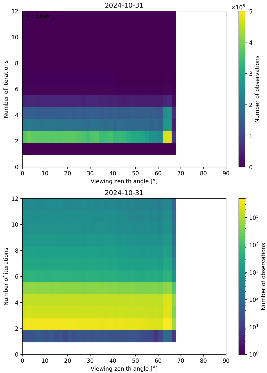
Figure 136: Scatter density plot of “Viewing zenith angle” against “Number of iterations” for 2024-10-30 to 2024-11-01.
