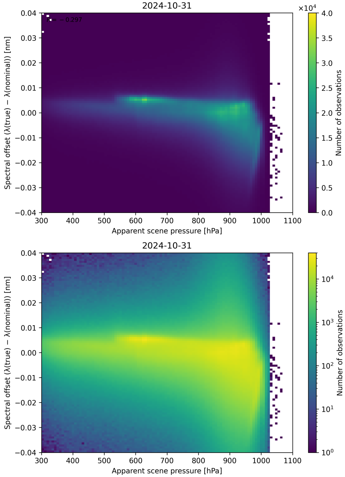
Figure 68: Scatter density plot of “Apparent scene pressure” against “Spectral offset ( \lambda_{\text{true}} - \lambda_{\text{nominal}} )” for 2024-10-30 to 2024-11-01.
