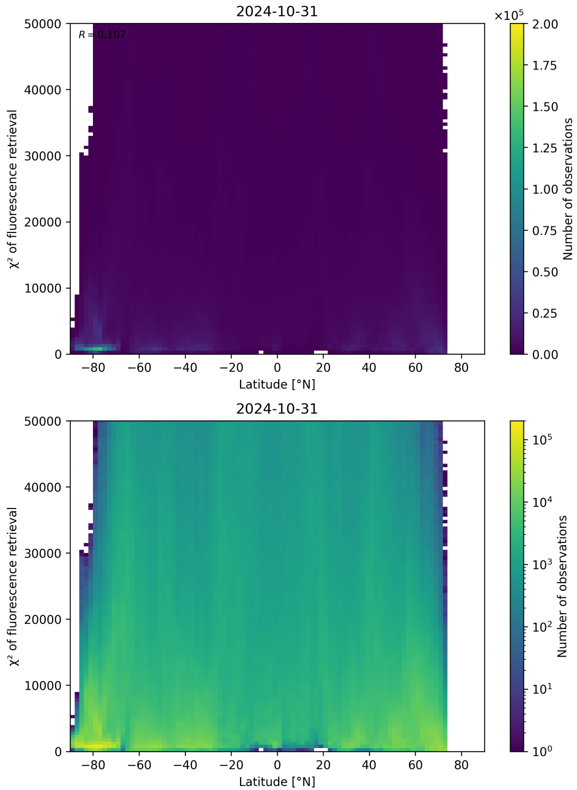
Figure 98: Scatter density plot of “Latitude” against “ \chi^2 of fluorescence retrieval” for 2024-10-30 to 2024-11-01.
