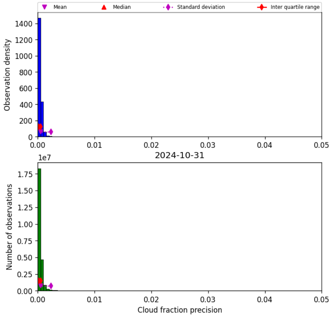
Figure 33: Histogram of “Cloud fraction precision” for 2024-10-30 to 2024-11-01
