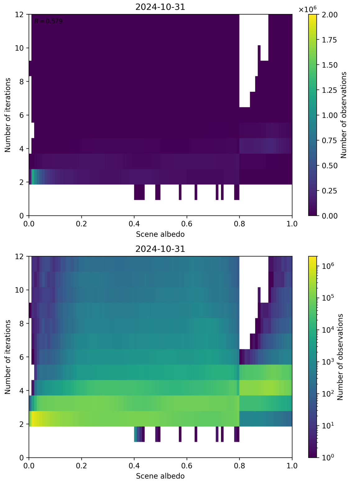
Figure 115: Scatter density plot of “Scene albedo” against “Number of iterations” for 2024-10-30 to 2024-11-01.
