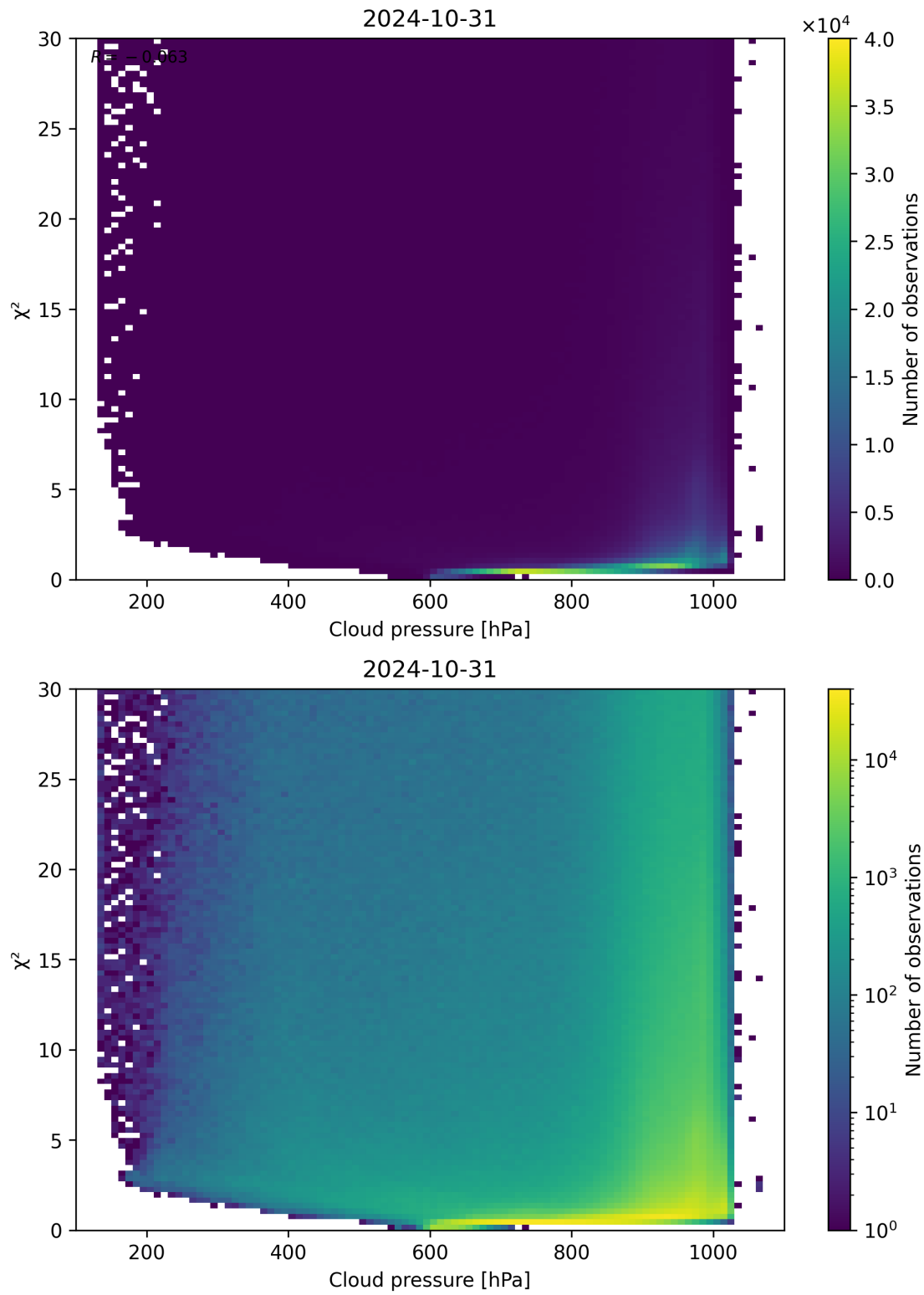
Figure 85: Scatter density plot of “Cloud pressure” against “ \chi^2 ” for 2024-10-30 to 2024-11-01.
