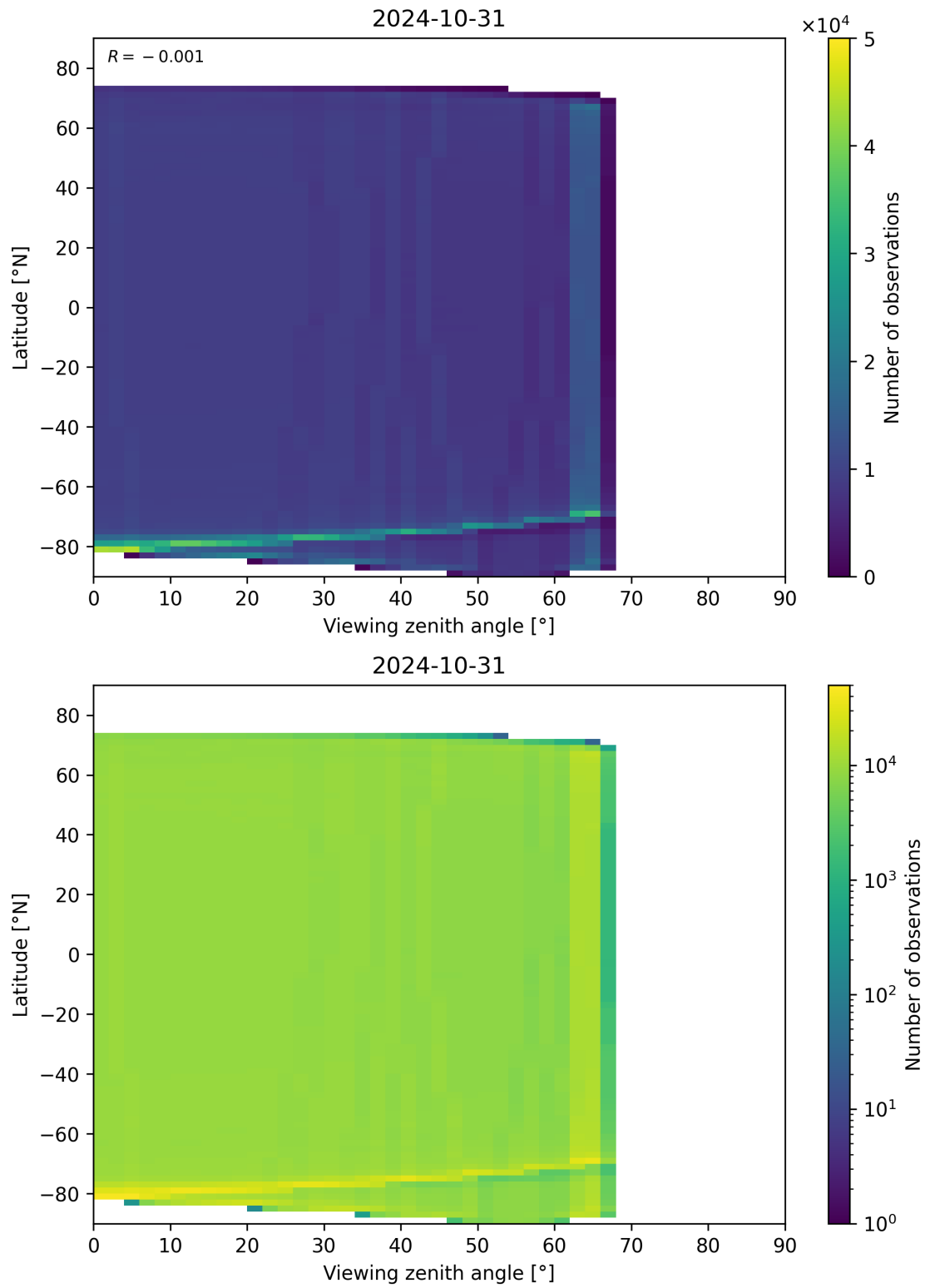
Figure 135: Scatter density plot of “Viewing zenith angle” against “Latitude” for 2024-10-30 to 2024-11-01.
