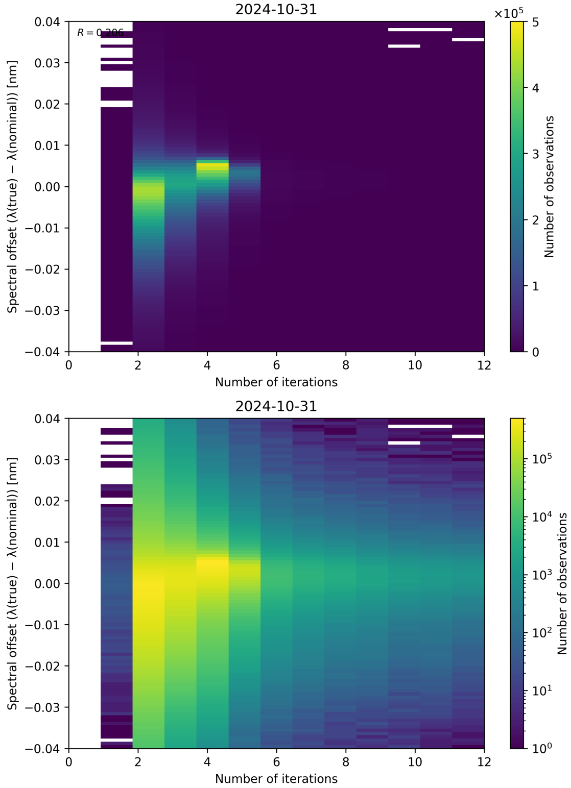
Figure 109: Scatter density plot of “Number of iterations” against “Spectral offset ( \lambda_{\text{true}} - \lambda_{\text{nominal}} )” for 2024-10-30 to 2024-11-01.
