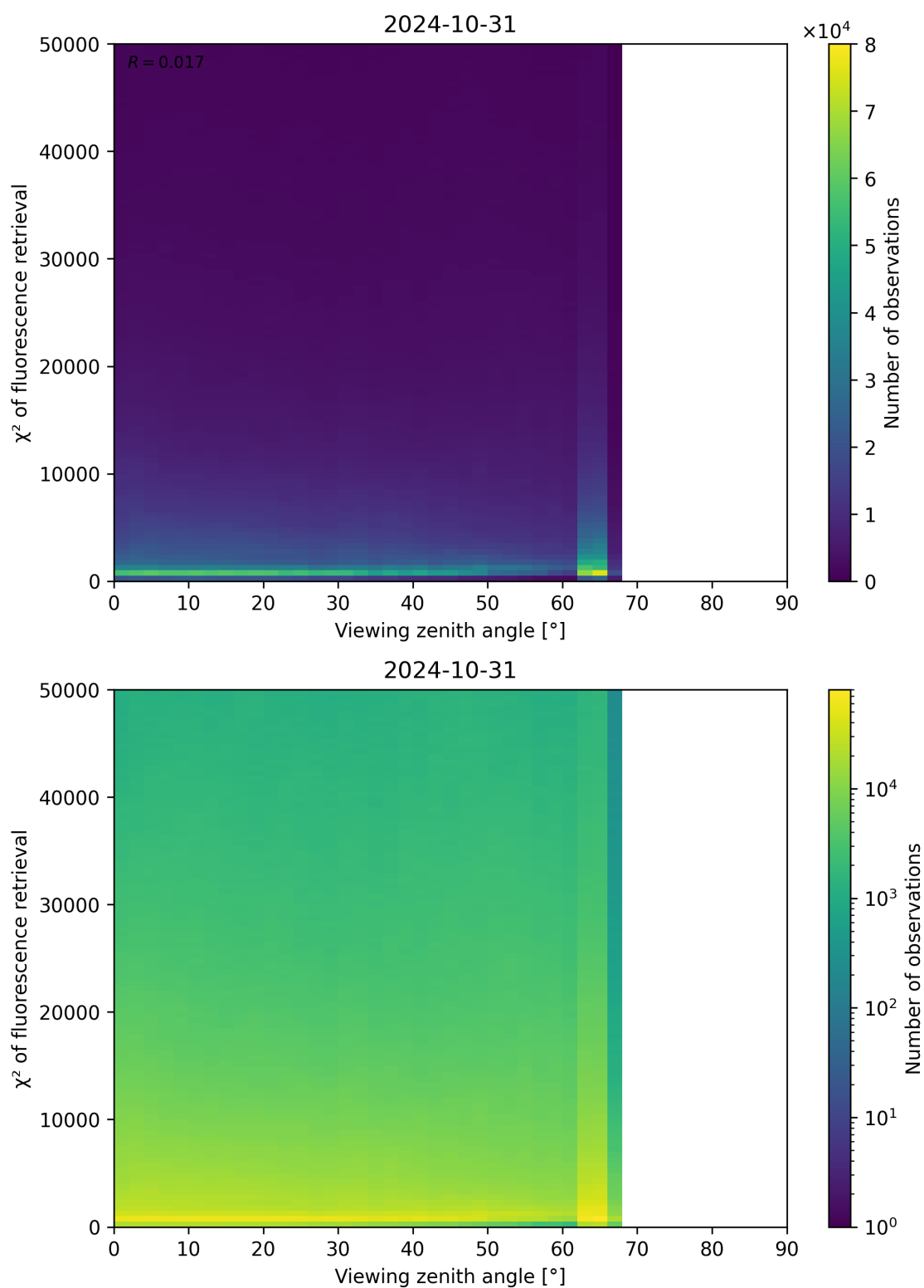
Figure 131: Scatter density plot of “Viewing zenith angle” against “ \chi^2 of fluorescence retrieval” for 2024-10-30 to 2024-11-01.
