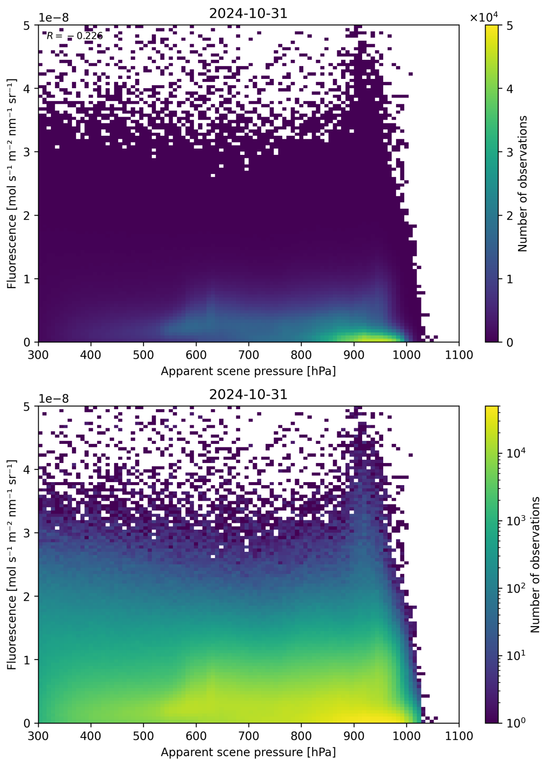
Figure 65: Scatter density plot of “Apparent scene pressure” against “Fluorescence” for 2024-10-30 to 2024-11-01.
