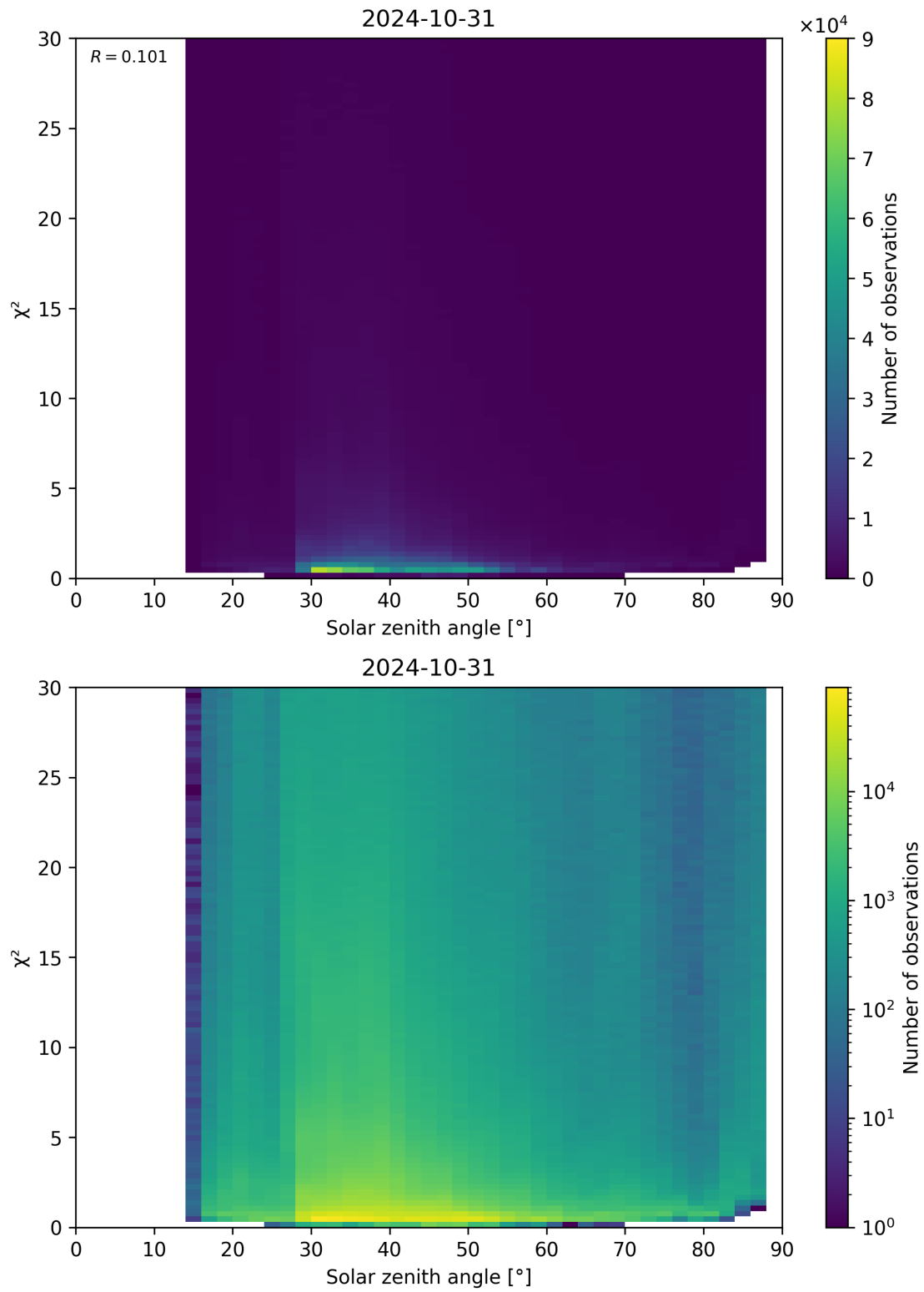
Figure 119: Scatter density plot of “Solar zenith angle” against “ \chi^2 ” for 2024-10-30 to 2024-11-01.
