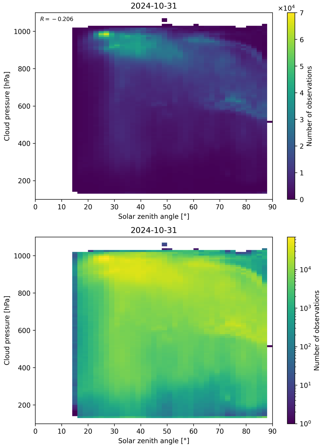
Figure 122: Scatter density plot of “Solar zenith angle” against “Cloud pressure” for 2024-10-30 to 2024-11-01.
