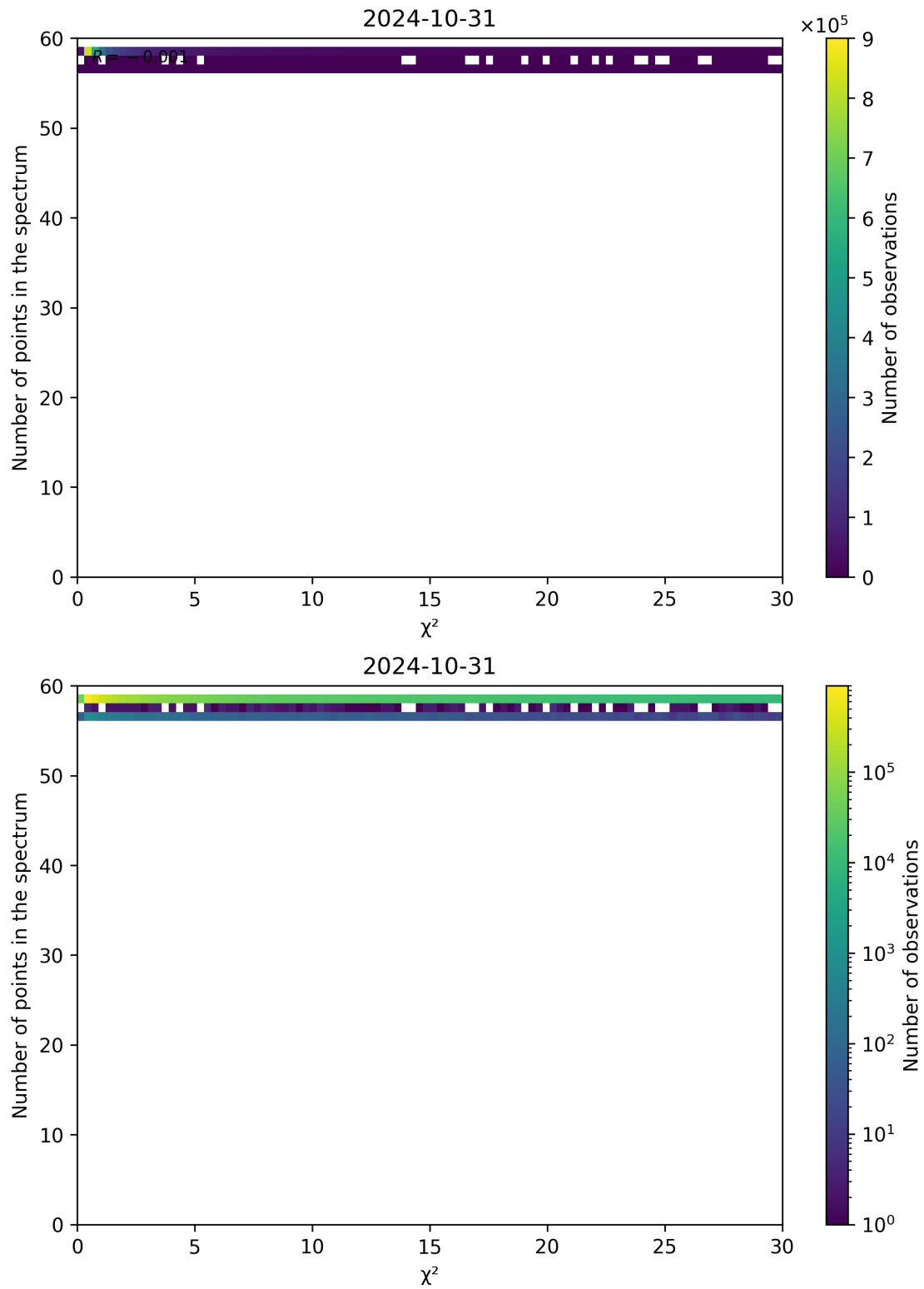
Figure 74: Scatter density plot of " \chi^2 " against "Number of points in the spectrum" for 2024-10-30 to 2024-11-01.
