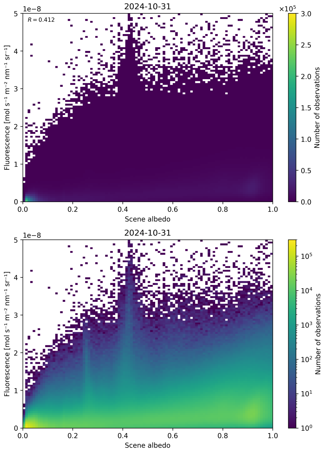
Figure 114: Scatter density plot of “Scene albedo” against “Fluorescence” for 2024-10-30 to 2024-11-01.
