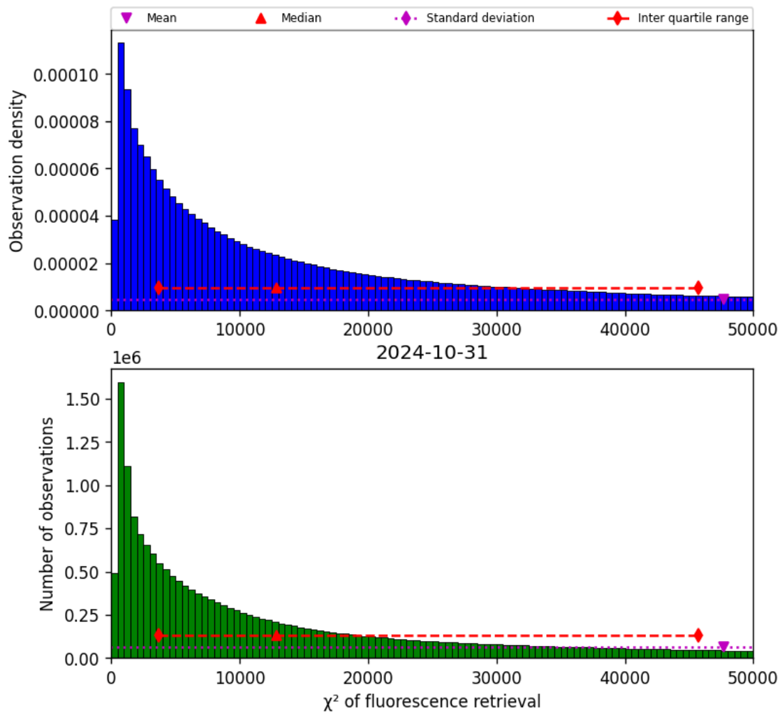
Figure 42: Histogram of “ \chi^2 of fluorescence retrieval” for 2024-10-30 to 2024-11-01
