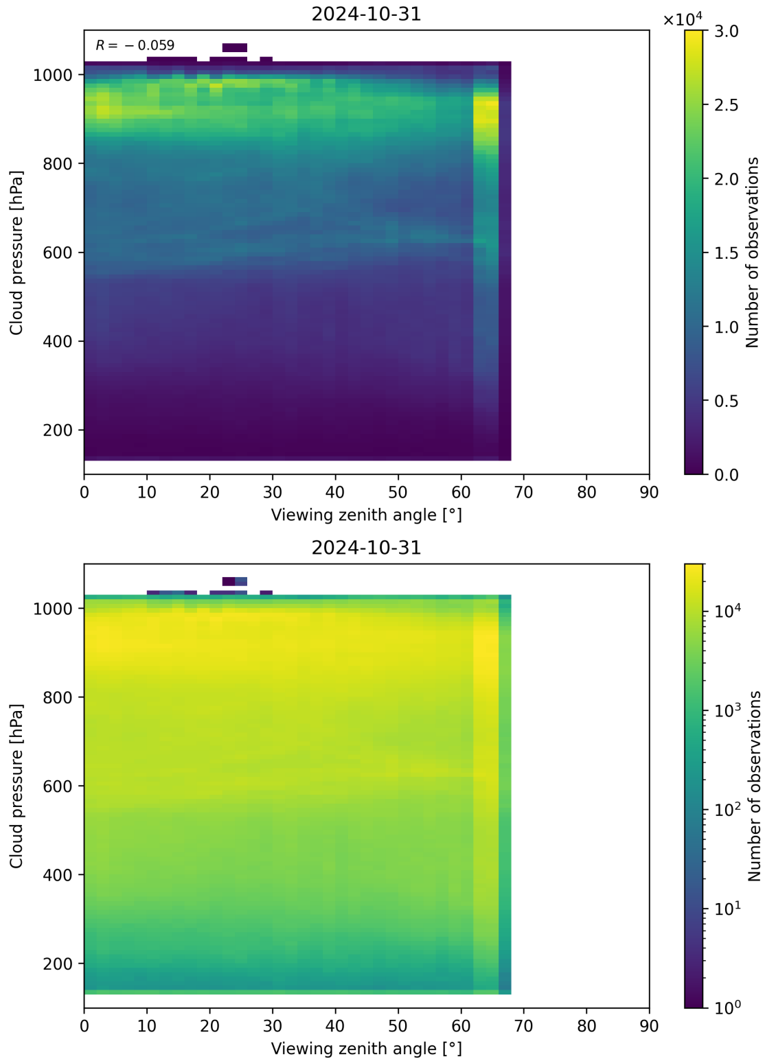
Figure 133: Scatter density plot of “Viewing zenith angle” against “Cloud pressure” for 2024-10-30 to 2024-11-01.
