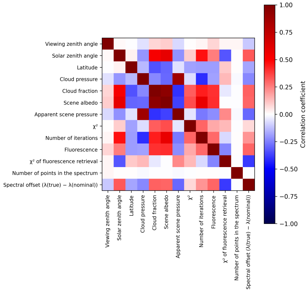
Figure 2: Map of correlation matrix for 2024-10-30 to 2024-11-01.
