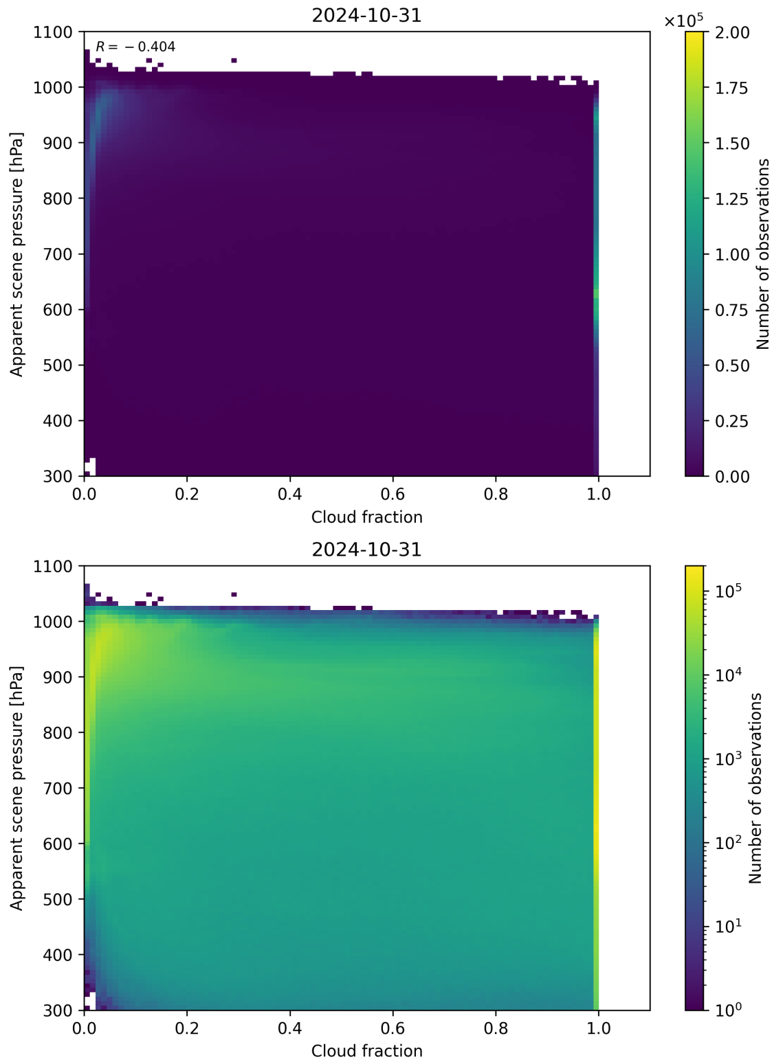
Figure 76: Scatter density plot of “Cloud fraction” against “Apparent scene pressure” for 2024-10-30 to 2024-11-01.
