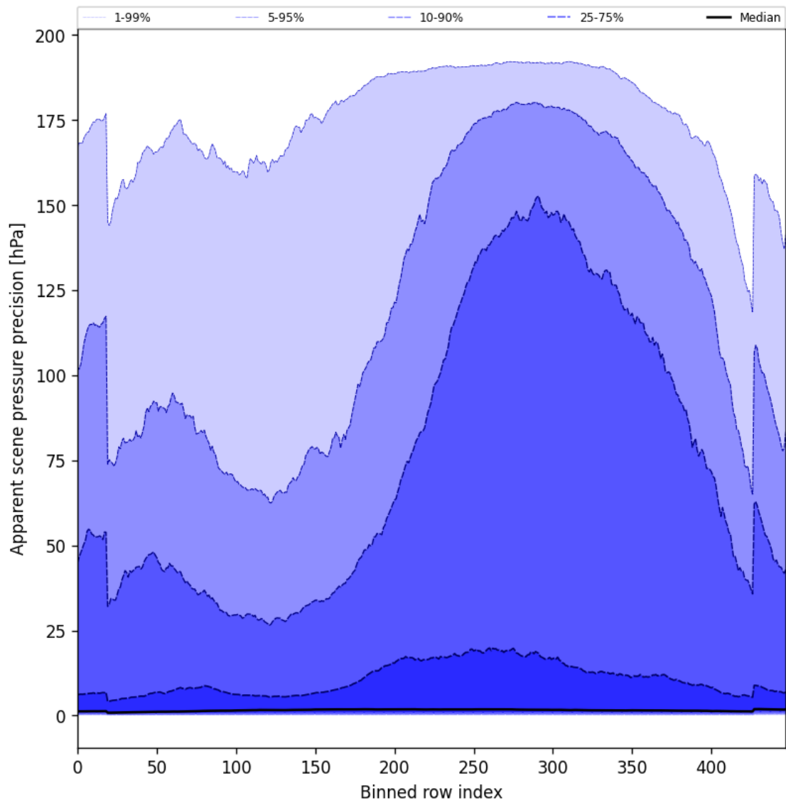
Figure 54: Along track statistics of “Apparent scene pressure precision” for 2024-10-30 to 2024-11-01
