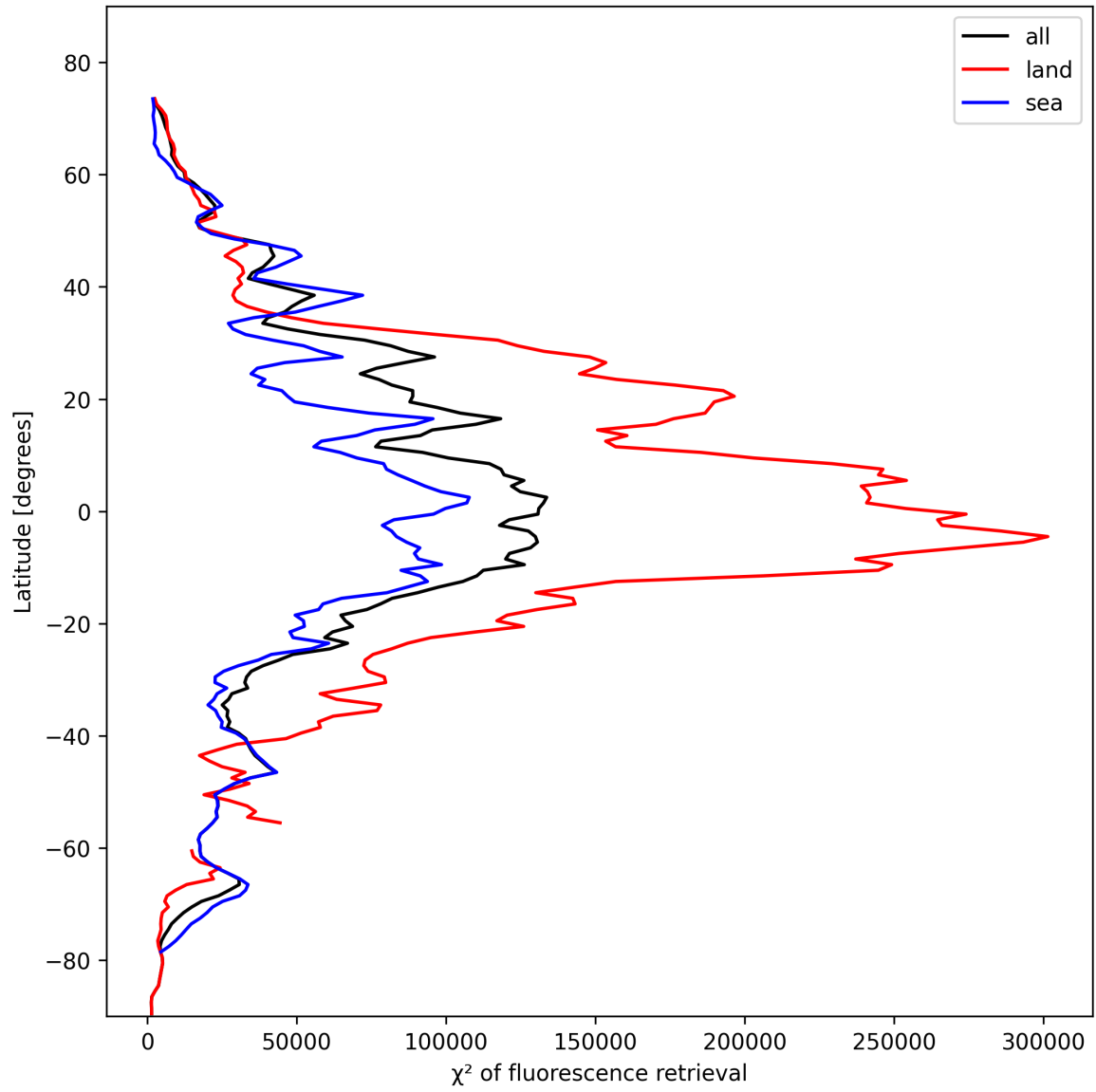
Figure 25: Zonal average of “ \chi^2 of fluorescence retrieval” for 2024-10-30 to 2024-11-01.
