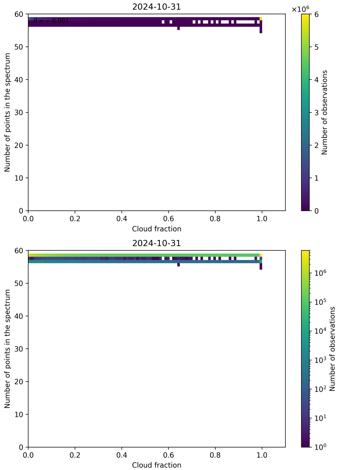
Figure 81: Scatter density plot of “Cloud fraction” against “Number of points in the spectrum” for 2024-10-30 to 2024-11-01.
