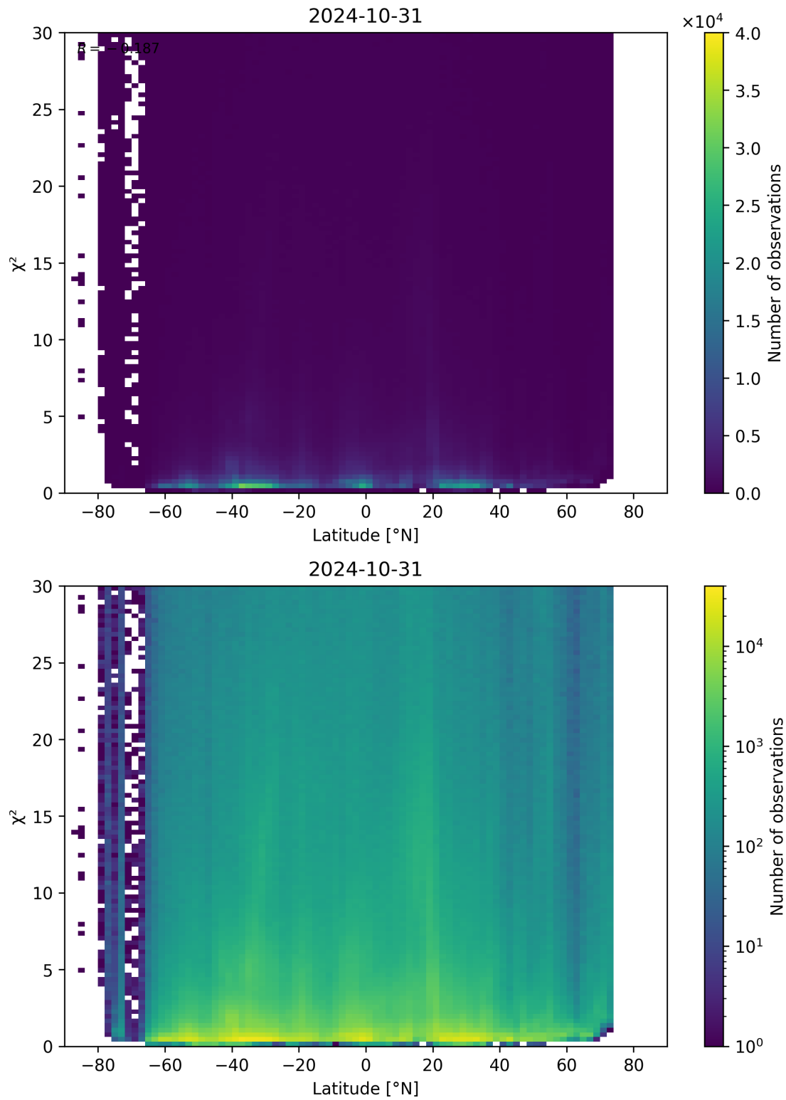
Figure 97: Scatter density plot of “Latitude” against “ \chi^2 ” for 2024-10-30 to 2024-11-01.
