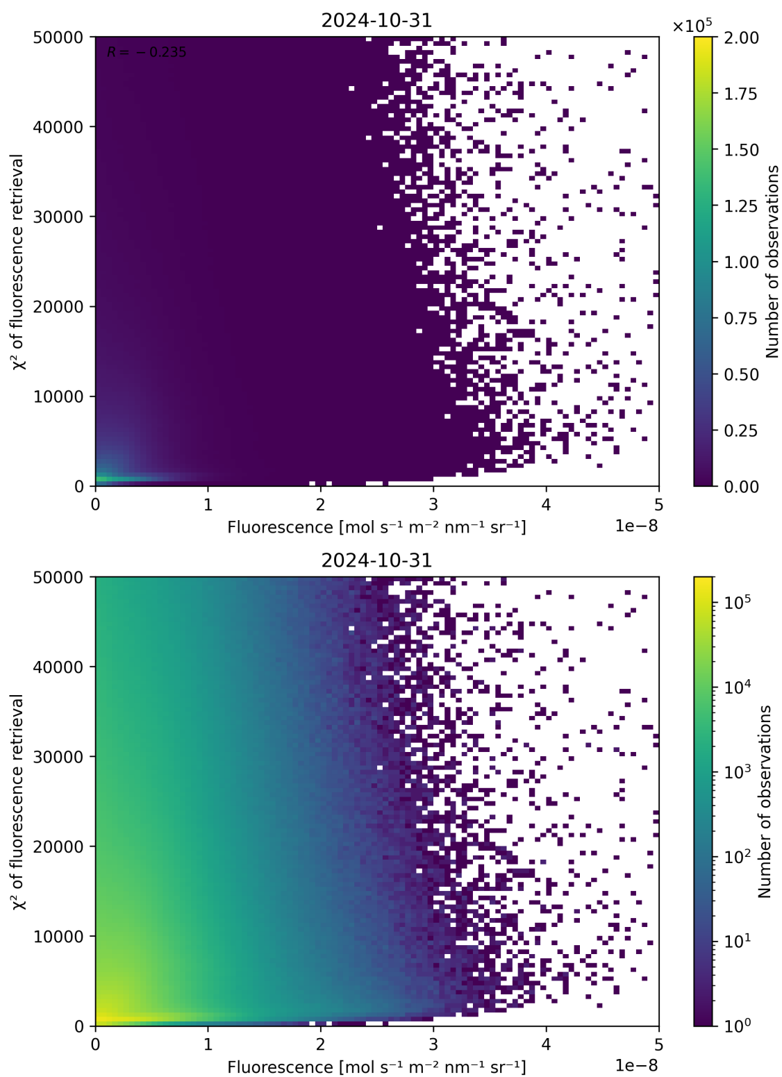
Figure 93: Scatter density plot of “Fluorescence” against “ \chi^2 of fluorescence retrieval” for 2024-10-30 to 2024-11-01.
