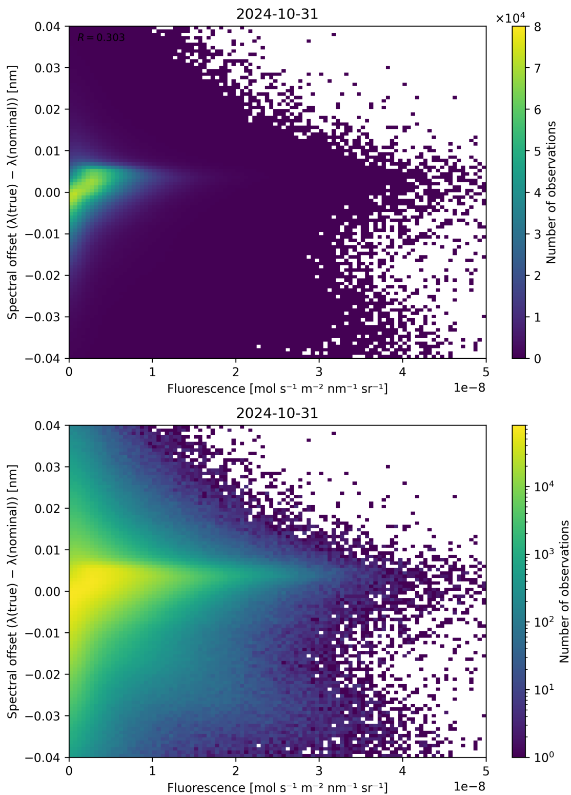
Figure 95: Scatter density plot of “Fluorescence” against “Spectral offset ( \lambda_{\text{true}} - \lambda_{\text{nominal}} )” for 2024-10-30 to 2024-11-01.
