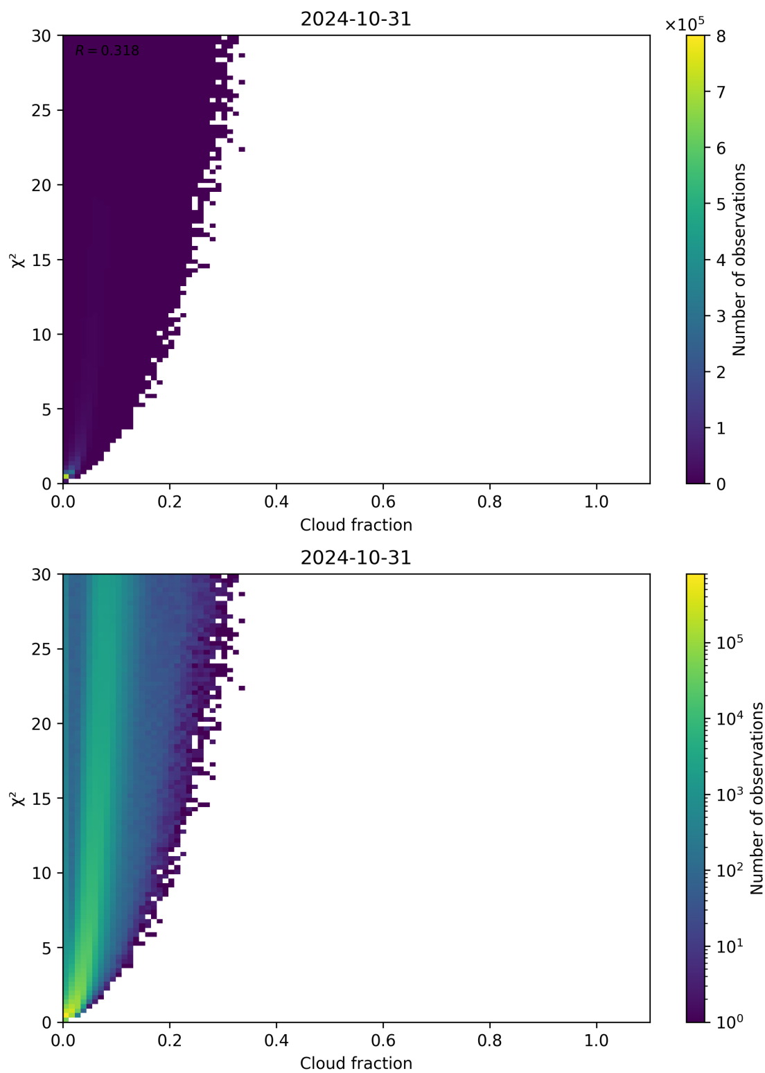
Figure 77: Scatter density plot of “Cloud fraction” against “ \chi^2 ” for 2024-10-30 to 2024-11-01.
