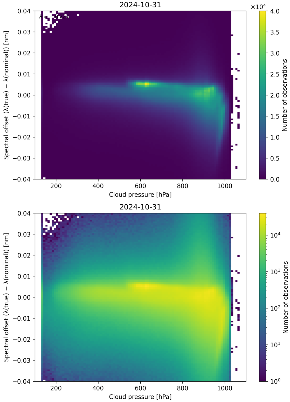
Figure 92: Scatter density plot of “Cloud pressure” against “Spectral offset ( \lambda_{\text{true}} - \lambda_{\text{nominal}} )” for 2024-10-30 to 2024-11-01.
