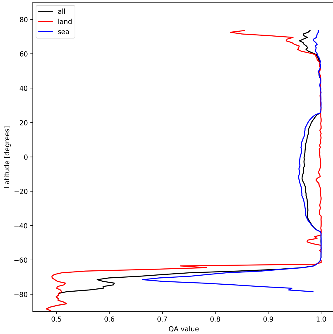
Figure 12: Zonal average of “QA value” for 2024-10-30 to 2024-11-01.
