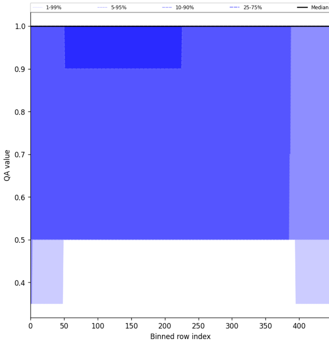
Figure 46: Along track statistics of “QA value” for 2024-10-30 to 2024-11-01
