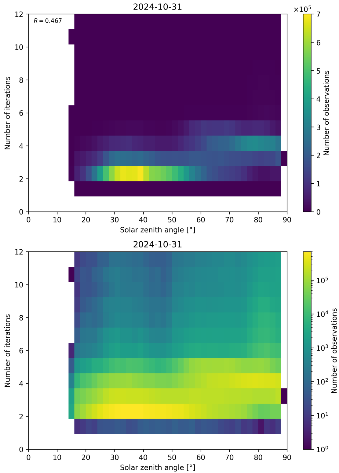
Figure 125: Scatter density plot of “Solar zenith angle” against “Number of iterations” for 2024-10-30 to 2024-11-01.
