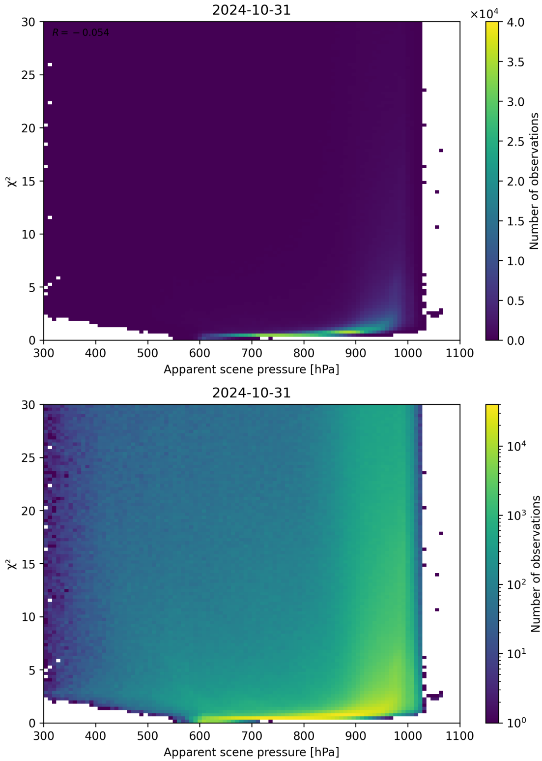
Figure 63: Scatter density plot of “Apparent scene pressure” against “ \chi^2 ” for 2024-10-30 to 2024-11-01.
