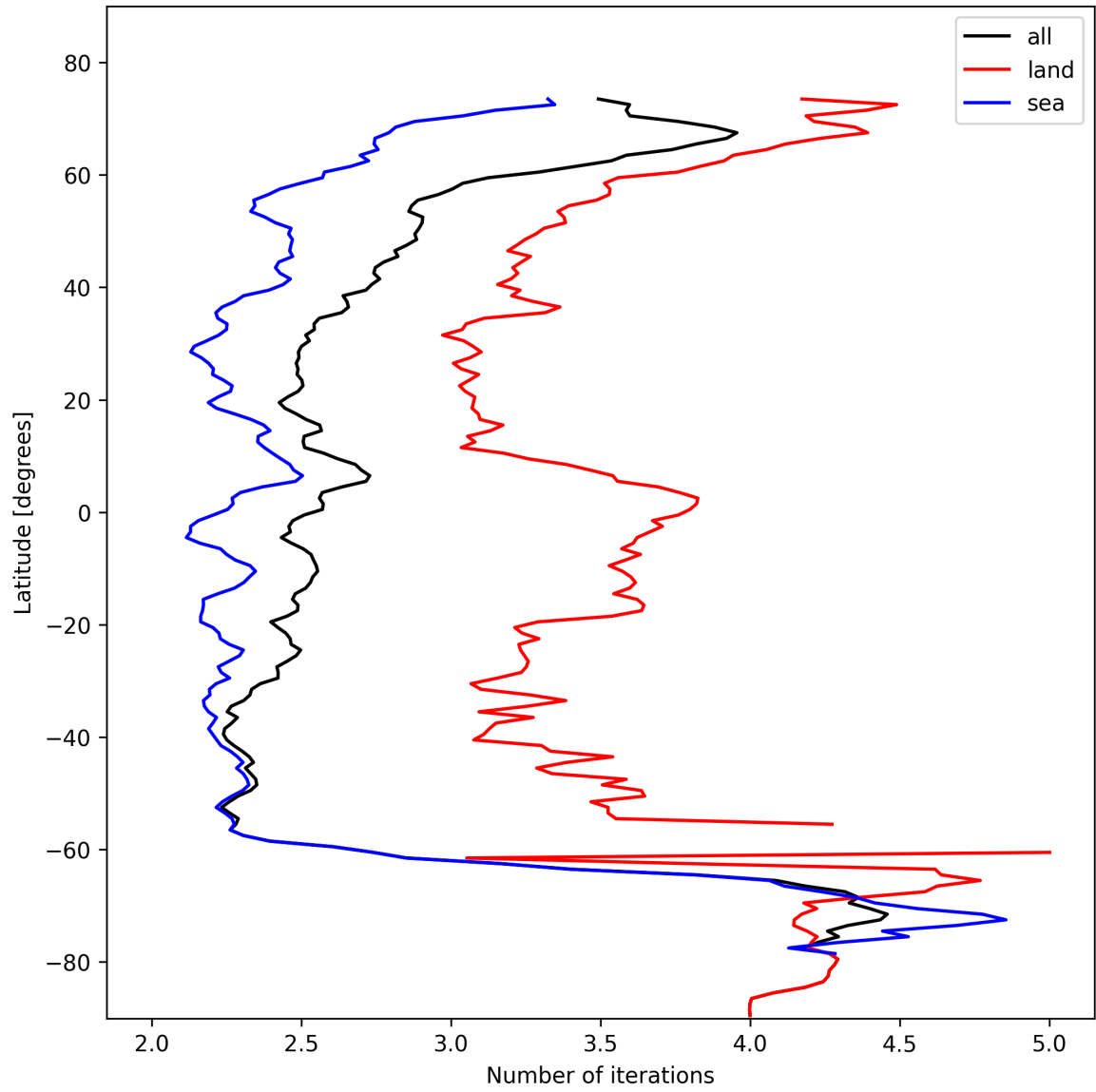
Figure 22: Zonal average of “Number of iterations” for 2024-10-30 to 2024-11-01.
