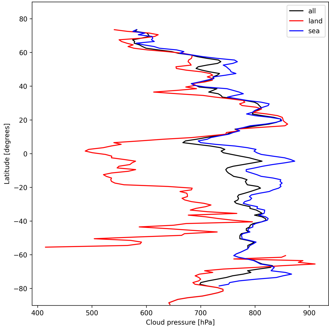
Figure 13: Zonal average of “Cloud pressure” for 2024-10-30 to 2024-11-01.
