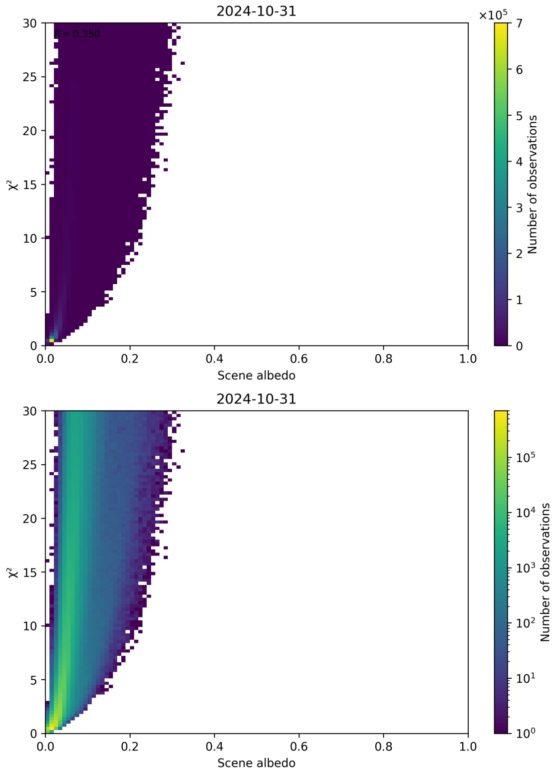
Figure 112: Scatter density plot of “Scene albedo” against “ \chi^2 ” for 2024-10-30 to 2024-11-01.
