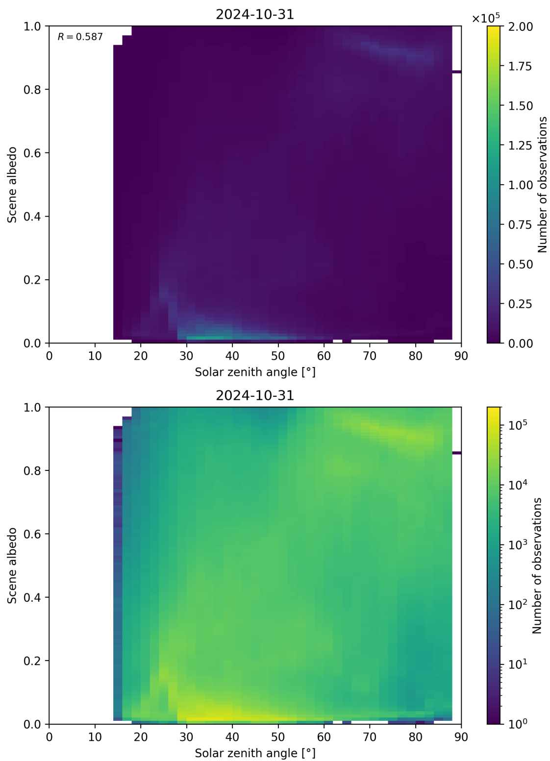
Figure 127: Scatter density plot of “Solar zenith angle” against “Scene albedo” for 2024-10-30 to 2024-11-01.
