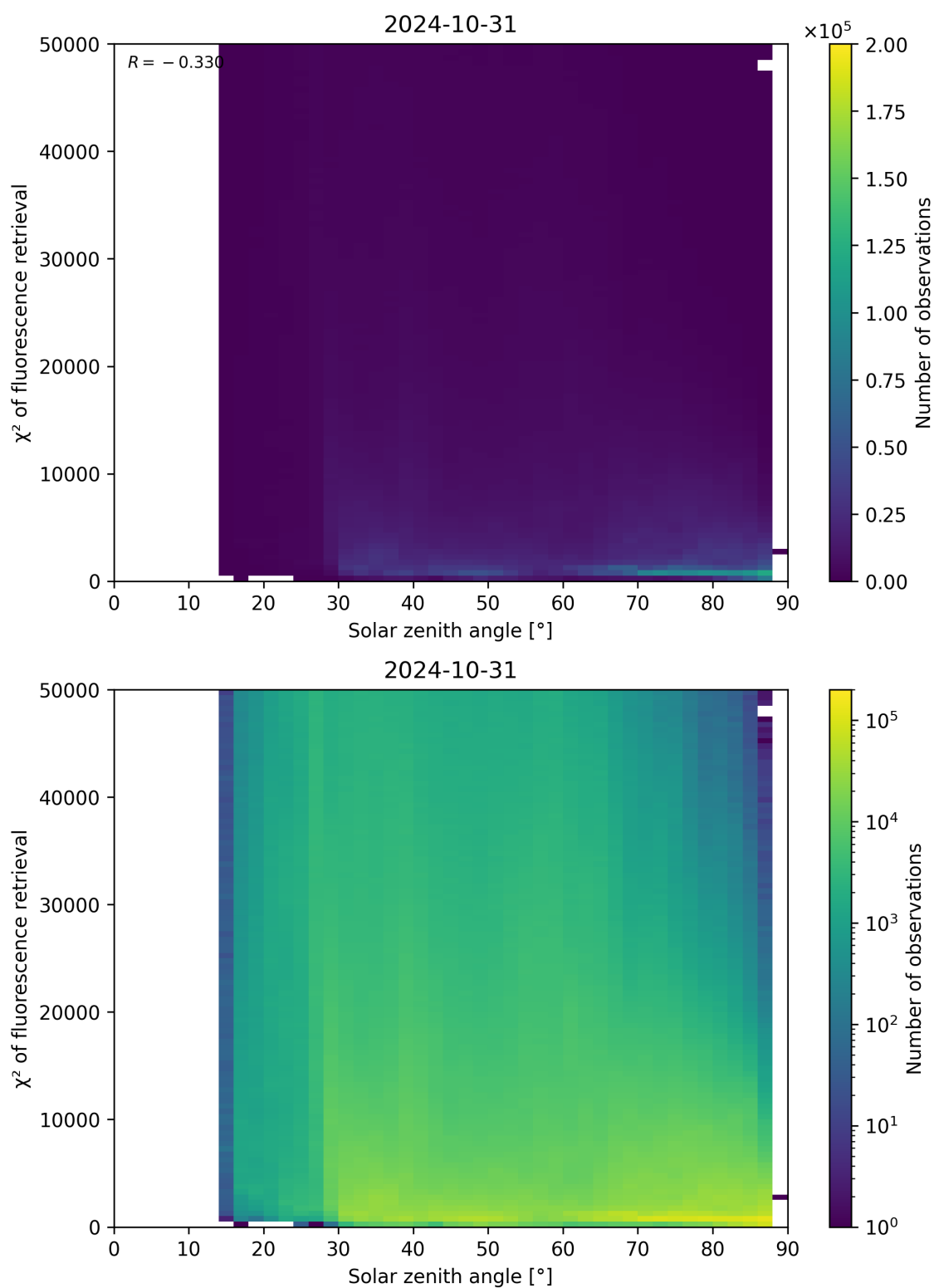
Figure 120: Scatter density plot of “Solar zenith angle” against “ \chi^2 of fluorescence retrieval” for 2024-10-30 to 2024-11-01.
