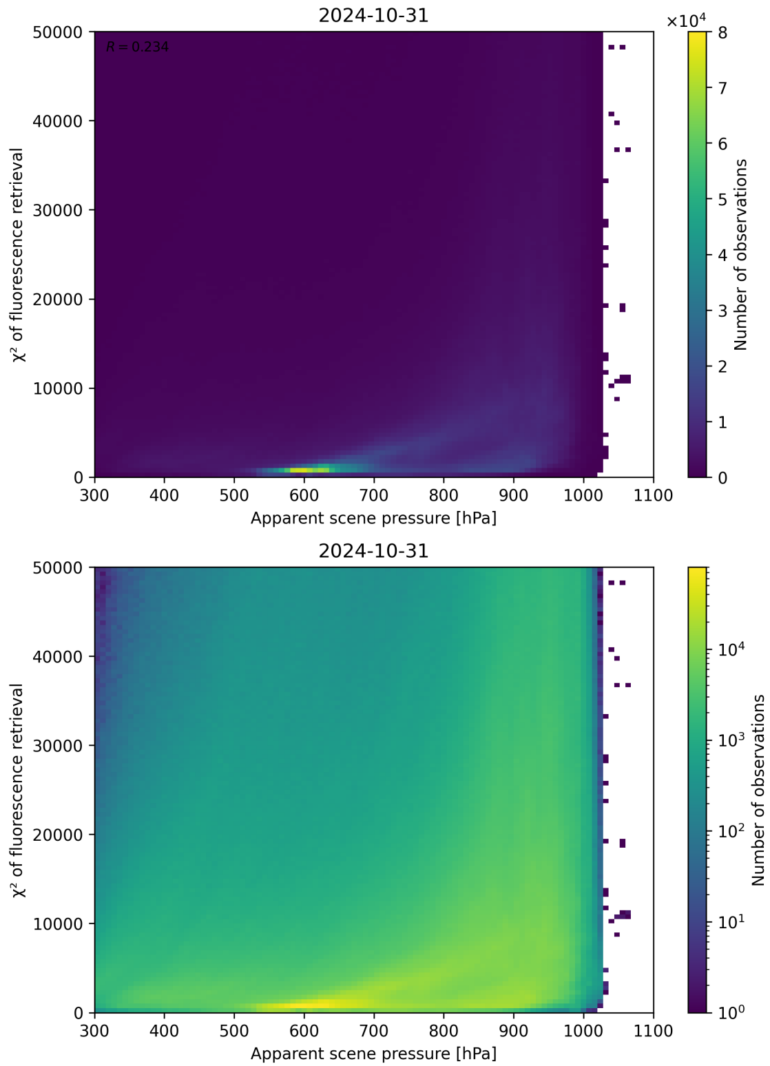
Figure 64: Scatter density plot of “Apparent scene pressure” against “ \chi^2 of fluorescence retrieval” for 2024-10-30 to 2024-11-01.
