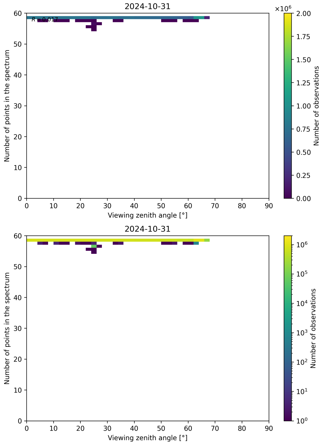
Figure 137: Scatter density plot of “Viewing zenith angle” against “Number of points in the spectrum” for 2024-10-30 to 2024-11-01.
