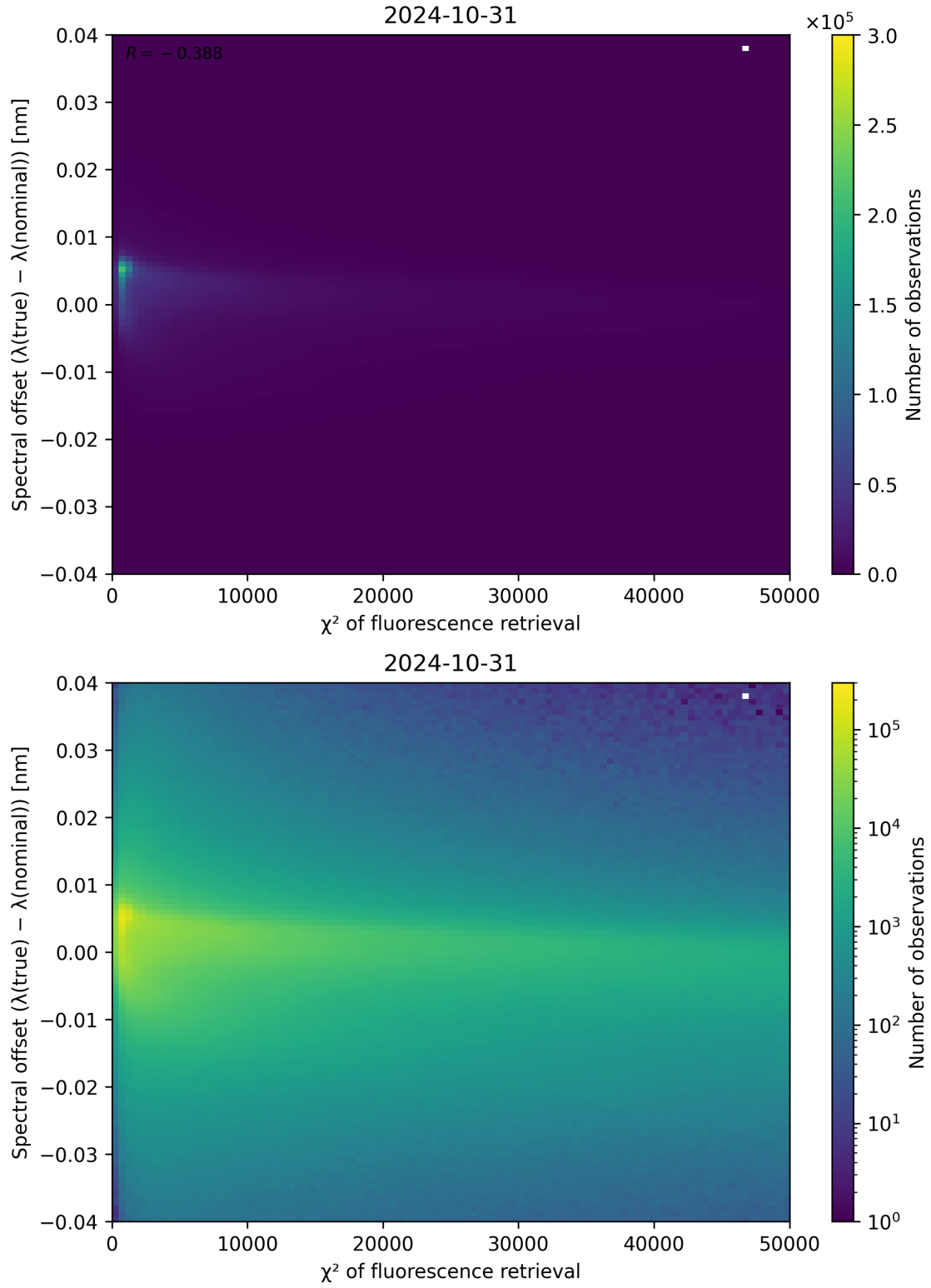
Figure 72: Scatter density plot of “ \chi^2 of fluorescence retrieval” against “Spectral offset ( \lambda_{\text{true}} - \lambda_{\text{nominal}} )” for 2024-10-30 to 2024-11-01.
