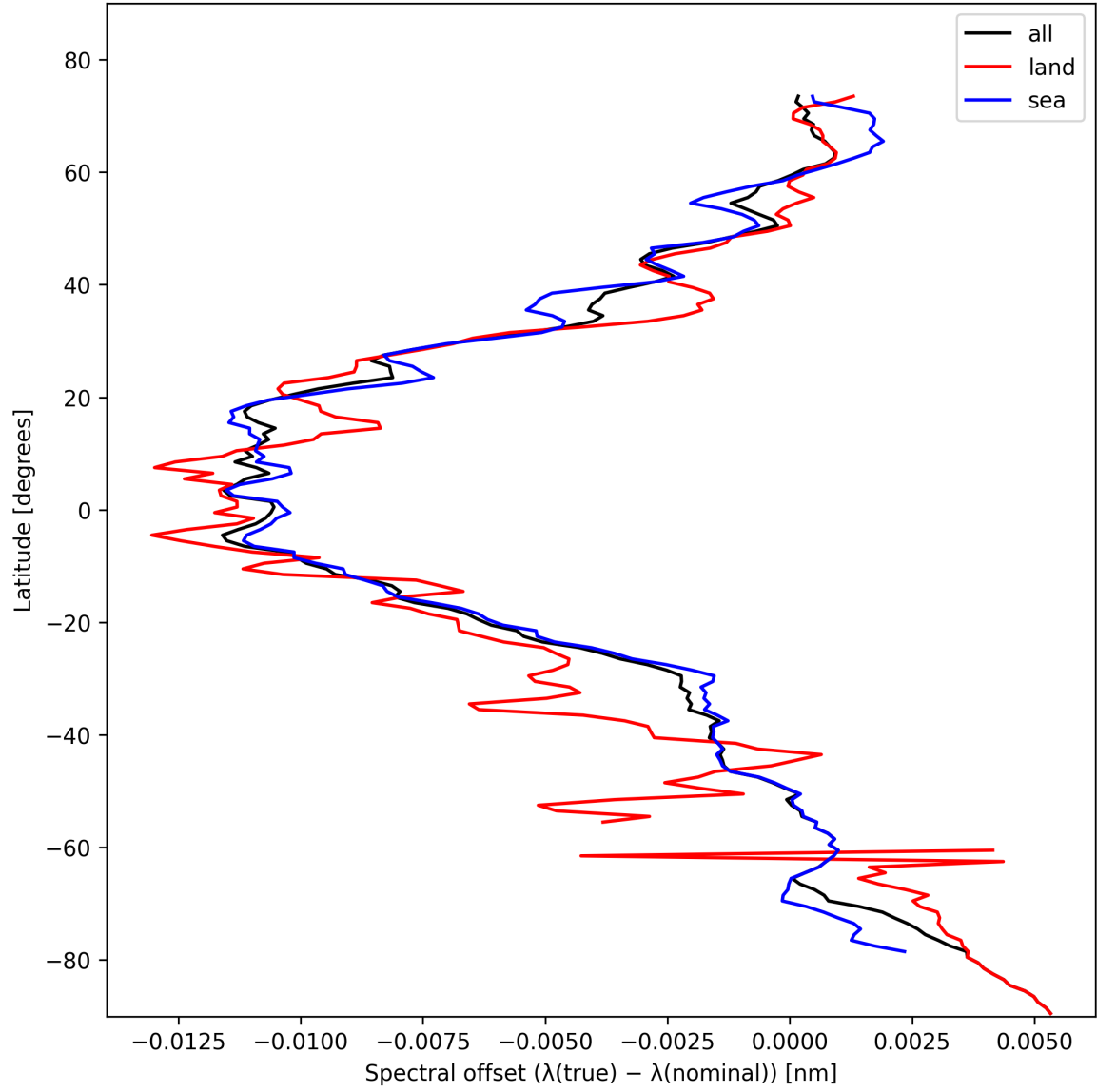
Figure 28: Zonal average of “Spectral offset ( \lambda_{\text{true}} - \lambda_{\text{nominal}} )” for 2024-10-30 to 2024-11-01.
