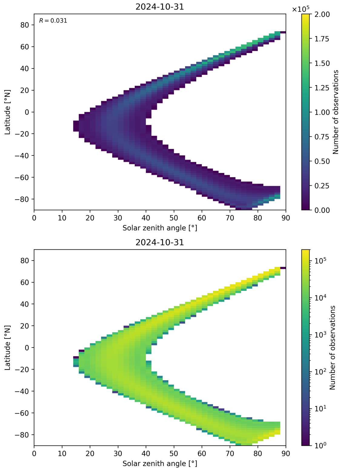
Figure 124: Scatter density plot of “Solar zenith angle” against “Latitude” for 2024-10-30 to 2024-11-01.
