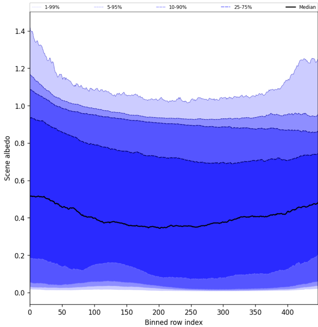
Figure 51: Along track statistics of “Scene albedo” for 2024-10-30 to 2024-11-01
