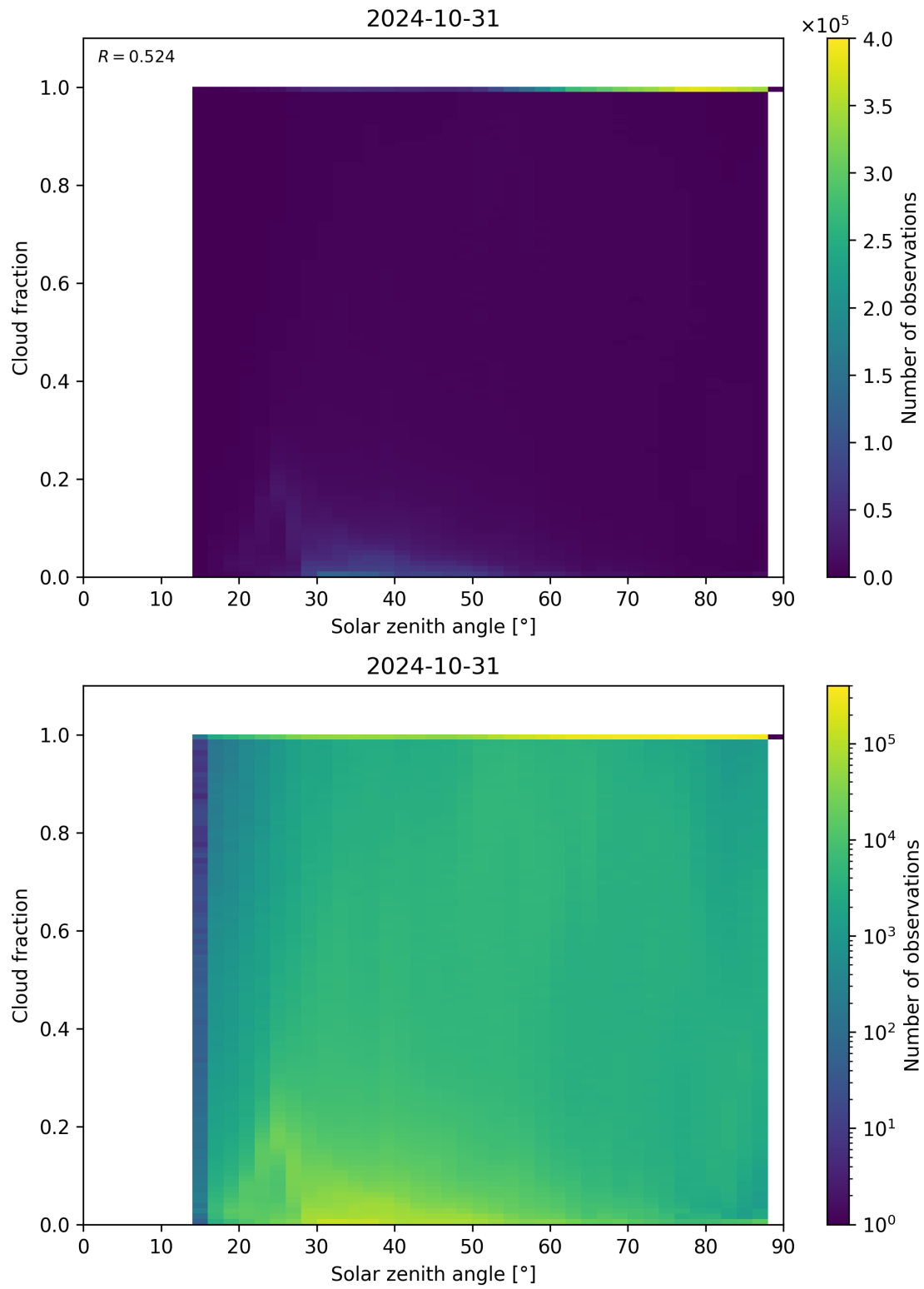
Figure 121: Scatter density plot of “Solar zenith angle” against “Cloud fraction” for 2024-10-30 to 2024-11-01.
