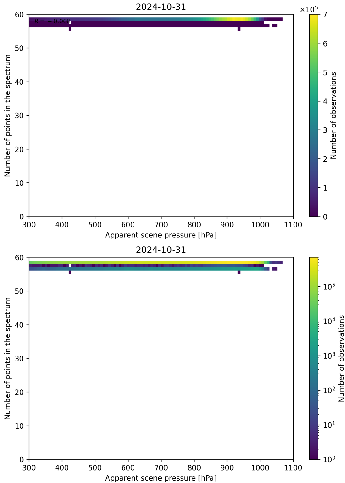
Figure 67: Scatter density plot of “Apparent scene pressure” against “Number of points in the spectrum” for 2024-10-30 to 2024-11-01.
