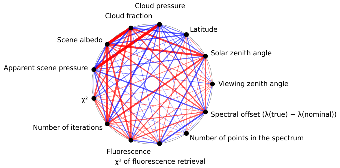
Figure 1: Map of correlation graph for 2024-10-30 to 2024-11-01.
