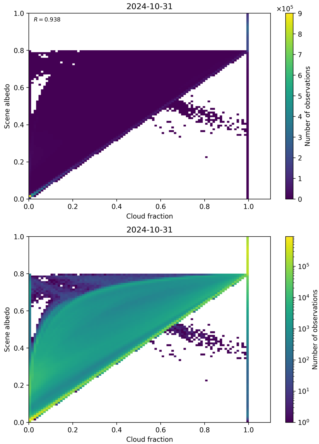
Figure 82: Scatter density plot of “Cloud fraction” against “Scene albedo” for 2024-10-30 to 2024-11-01.
