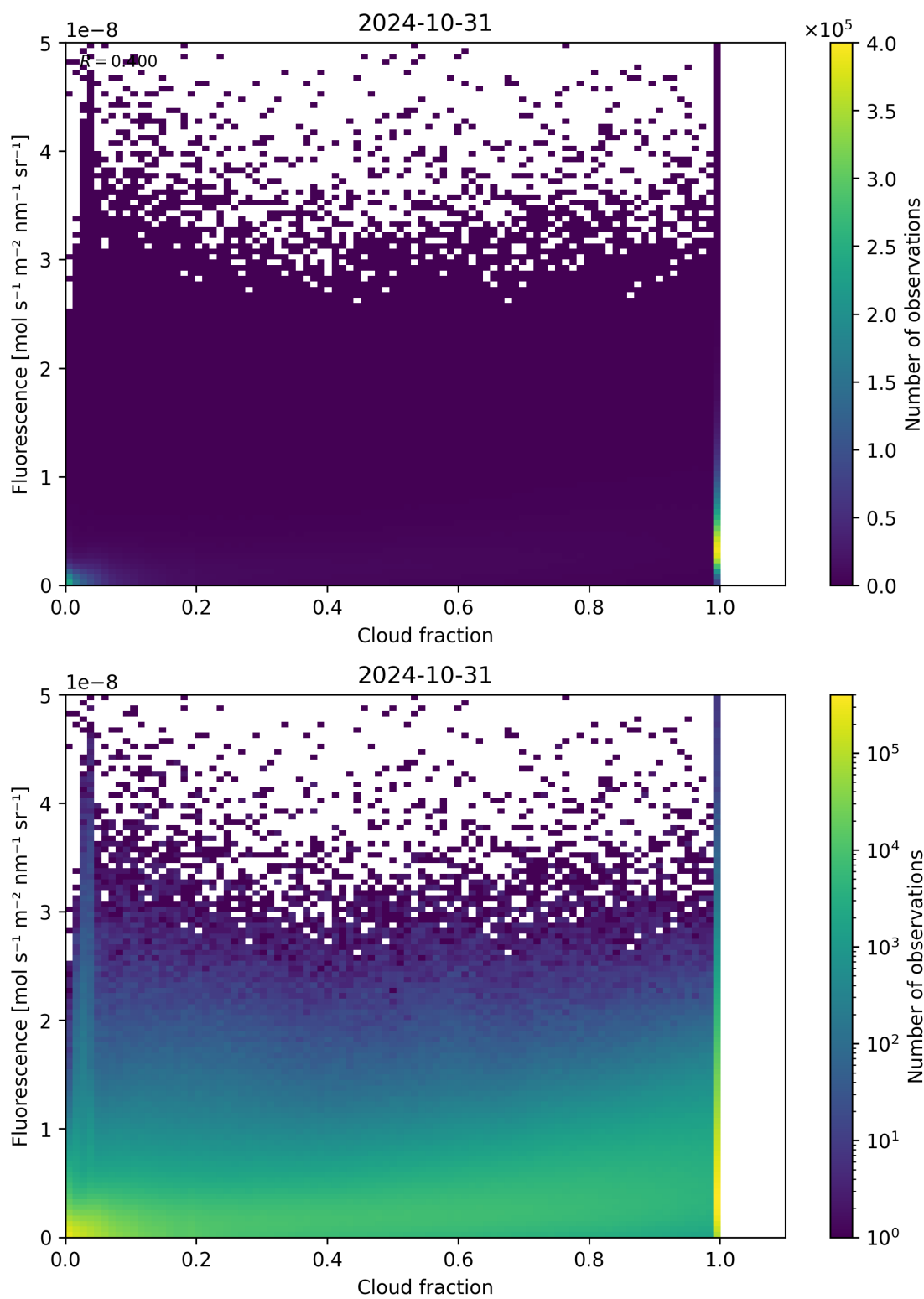
Figure 79: Scatter density plot of “Cloud fraction” against “Fluorescence” for 2024-10-30 to 2024-11-01.
