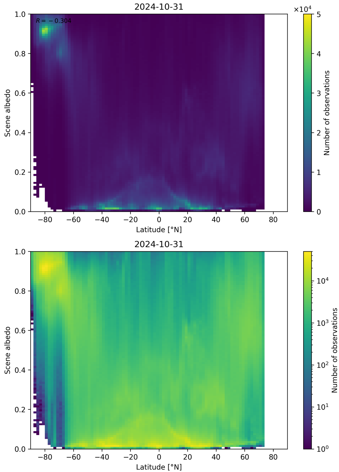
Figure 104: Scatter density plot of “Latitude” against “Scene albedo” for 2024-10-30 to 2024-11-01.
