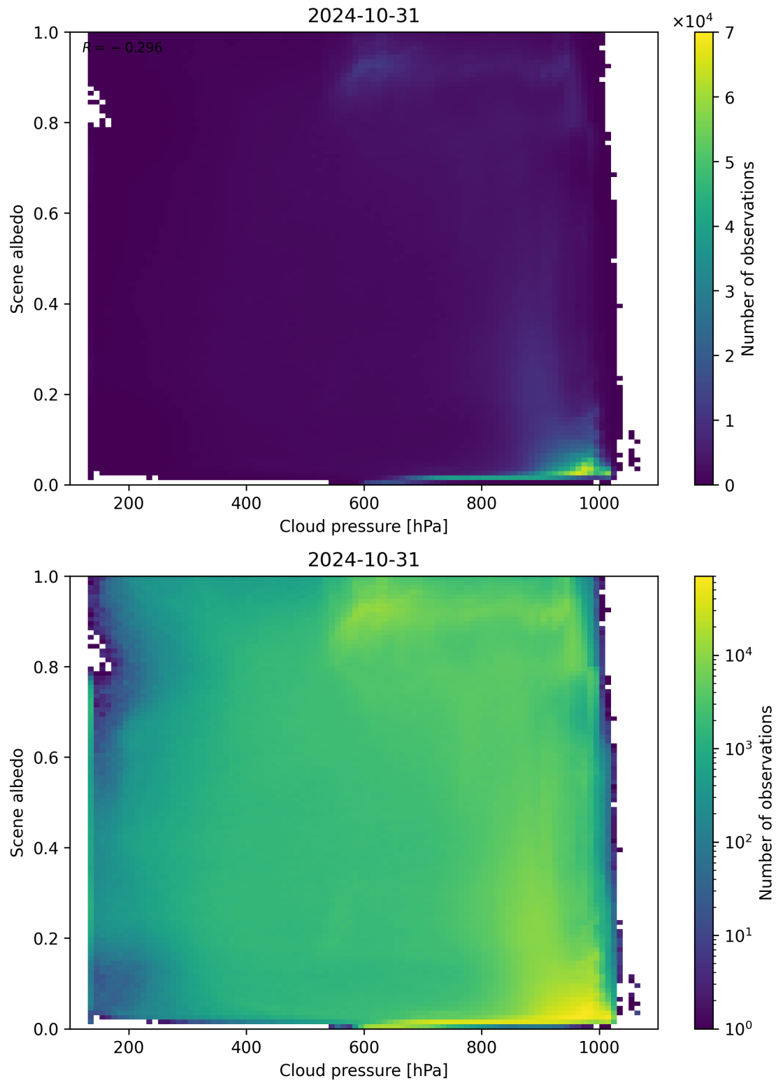
Figure 91: Scatter density plot of “Cloud pressure” against “Scene albedo” for 2024-10-30 to 2024-11-01.
