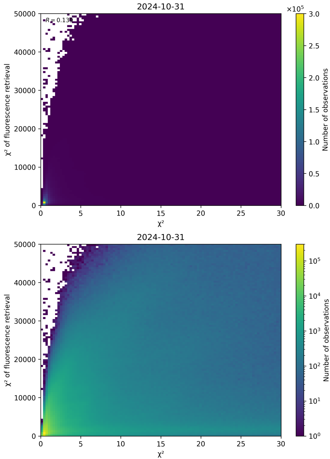
Figure 69: Scatter density plot of “ \chi^2 ” against “ \chi^2 of fluorescence retrieval” for 2024-10-30 to 2024-11-01.
