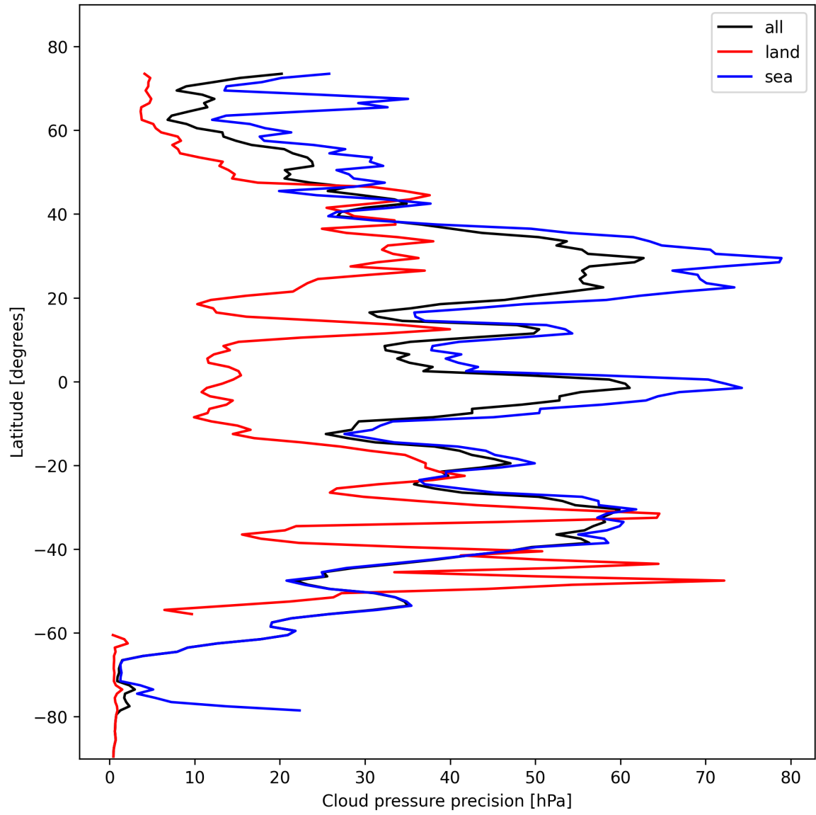
Figure 14: Zonal average of “Cloud pressure precision” for 2024-10-30 to 2024-11-01.
