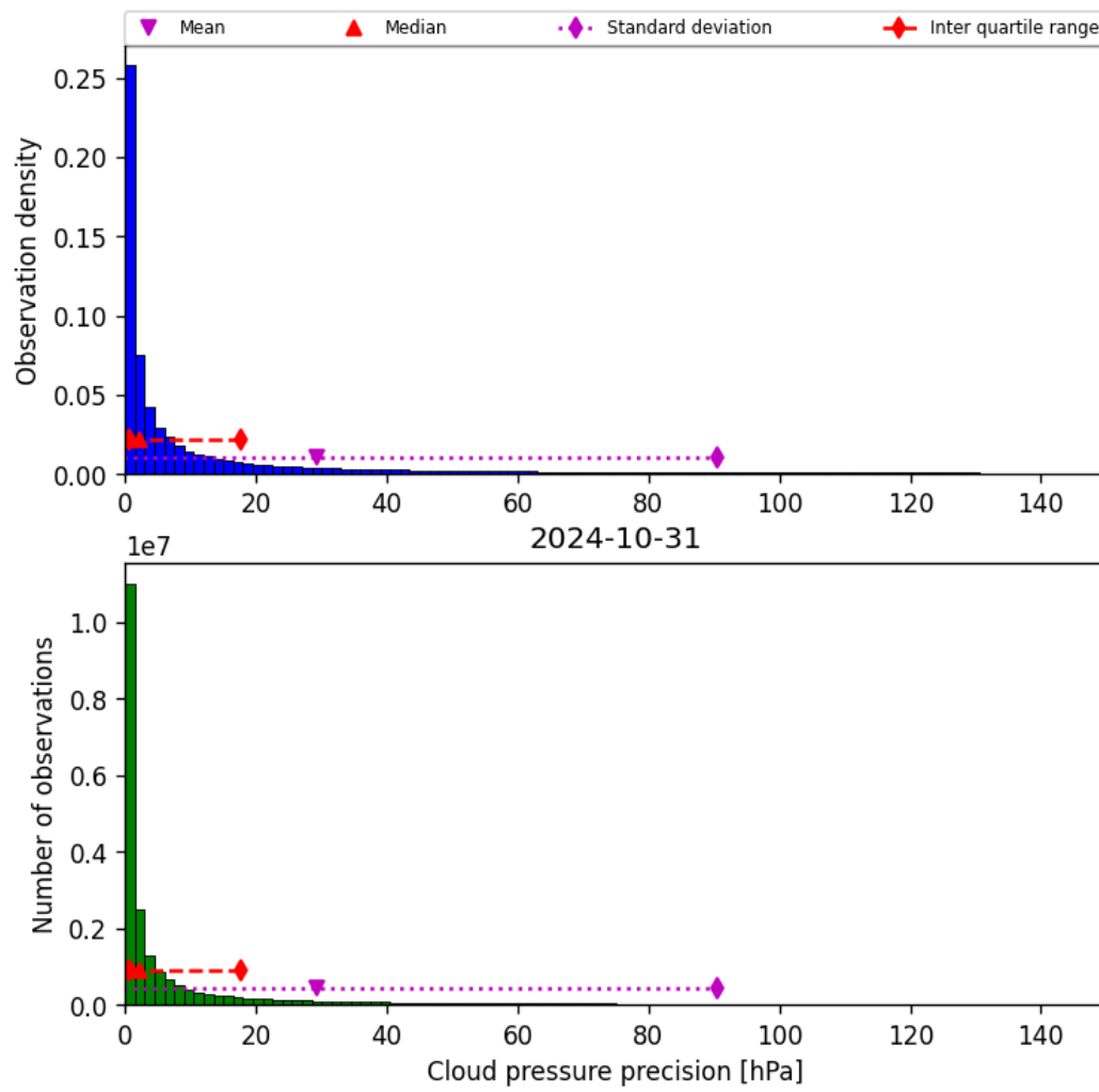
Figure 31: Histogram of “Cloud pressure precision” for 2024-10-30 to 2024-11-01
