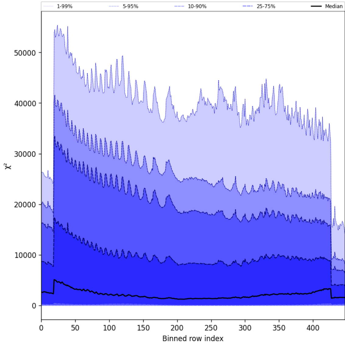
Figure 55: Along track statistics of “ \chi^2 ” for 2024-10-30 to 2024-11-01
