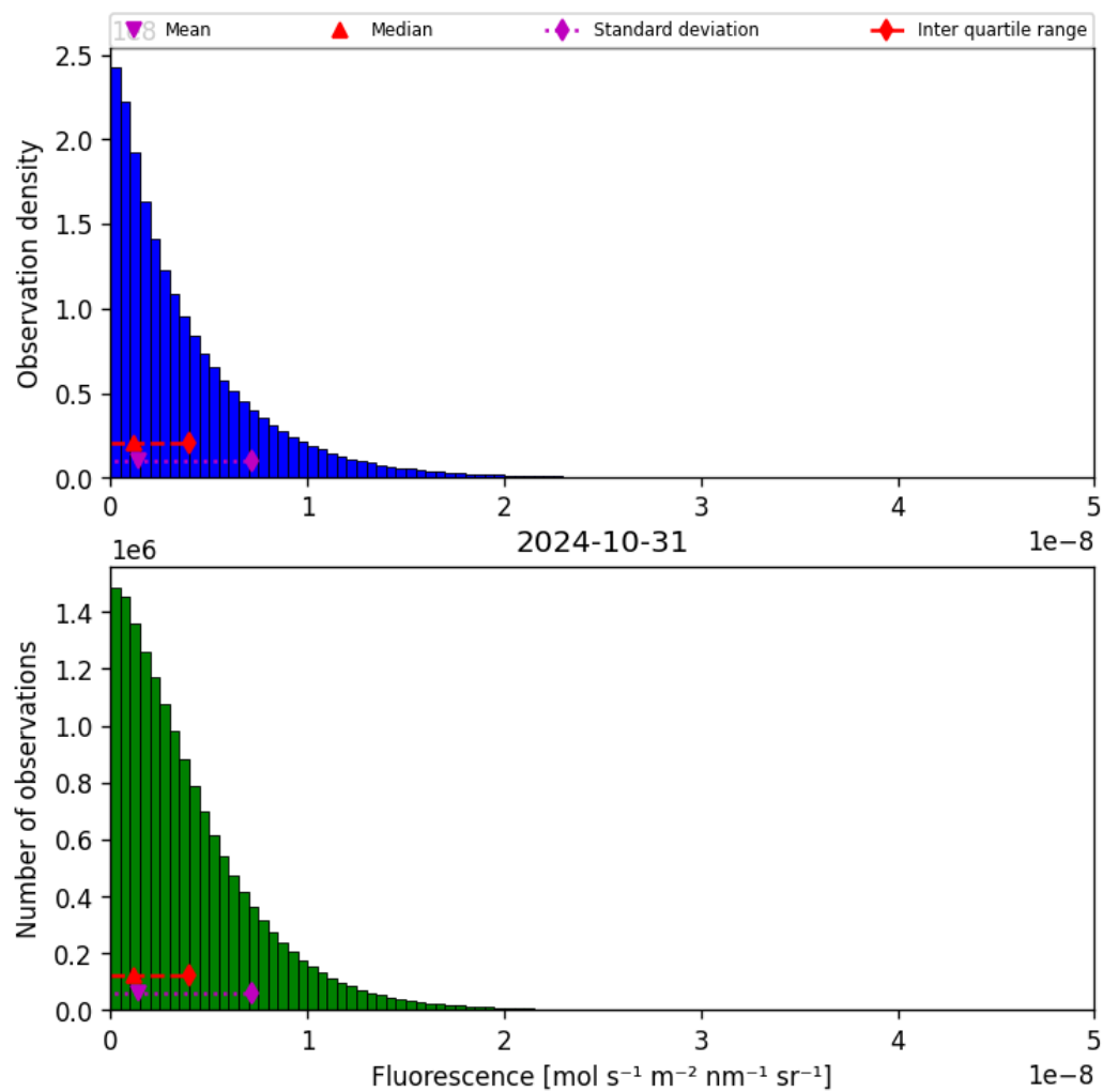
Figure 40: Histogram of “Fluorescence” for 2024-10-30 to 2024-11-01
