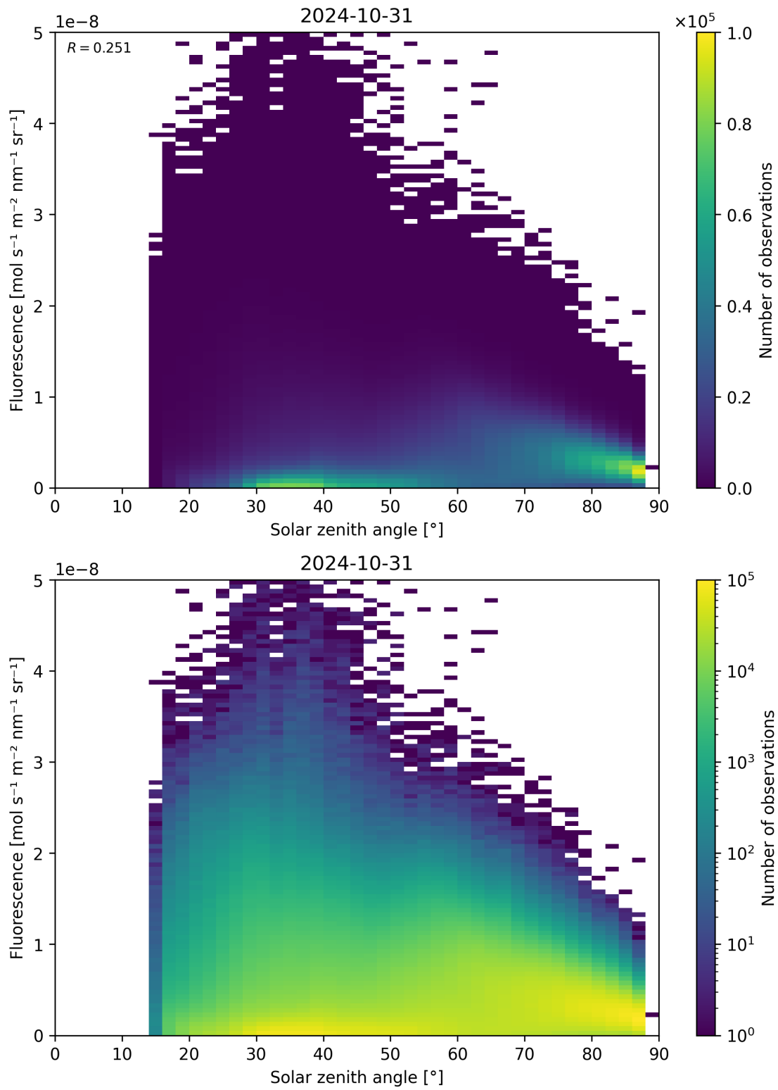
Figure 123: Scatter density plot of “Solar zenith angle” against “Fluorescence” for 2024-10-30 to 2024-11-01.
