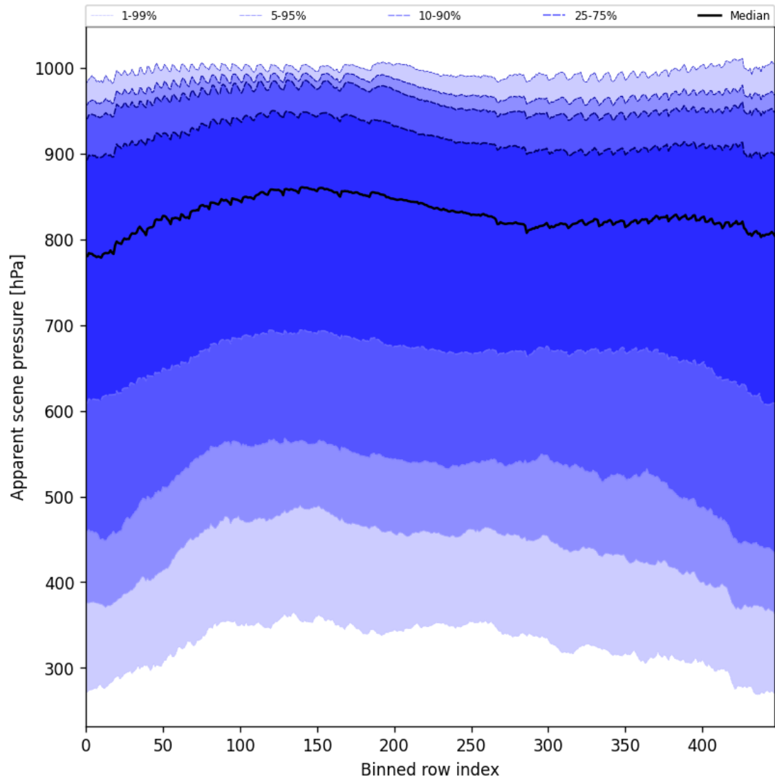
Figure 53: Along track statistics of “Apparent scene pressure” for 2024-10-30 to 2024-11-01
