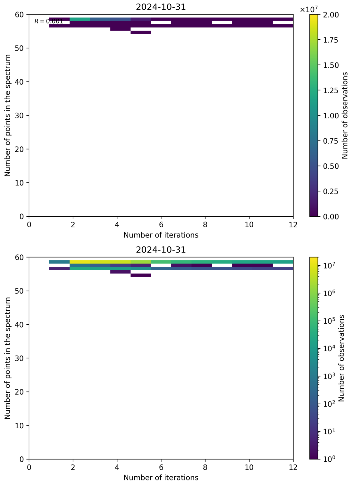
Figure 108: Scatter density plot of “Number of iterations” against “Number of points in the spectrum” for 2024-10-30 to 2024-11-01.
