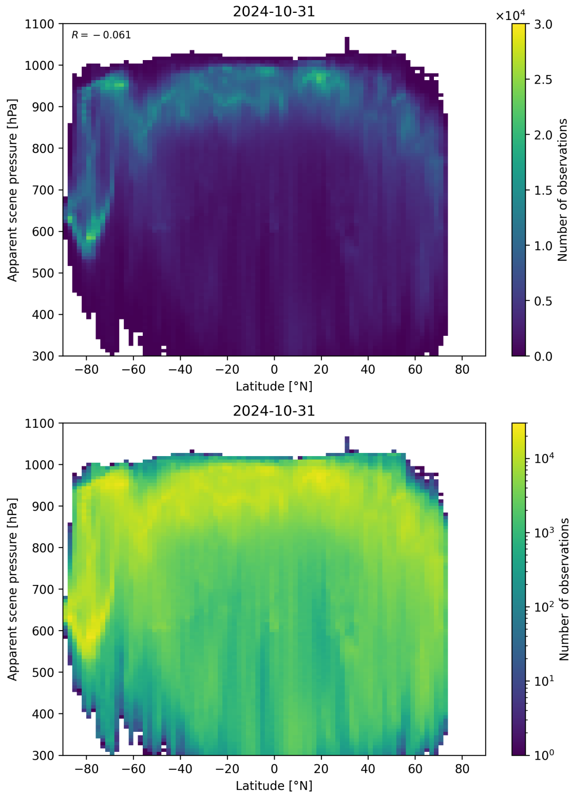
Figure 96: Scatter density plot of “Latitude” against “Apparent scene pressure” for 2024-10-30 to 2024-11-01.
