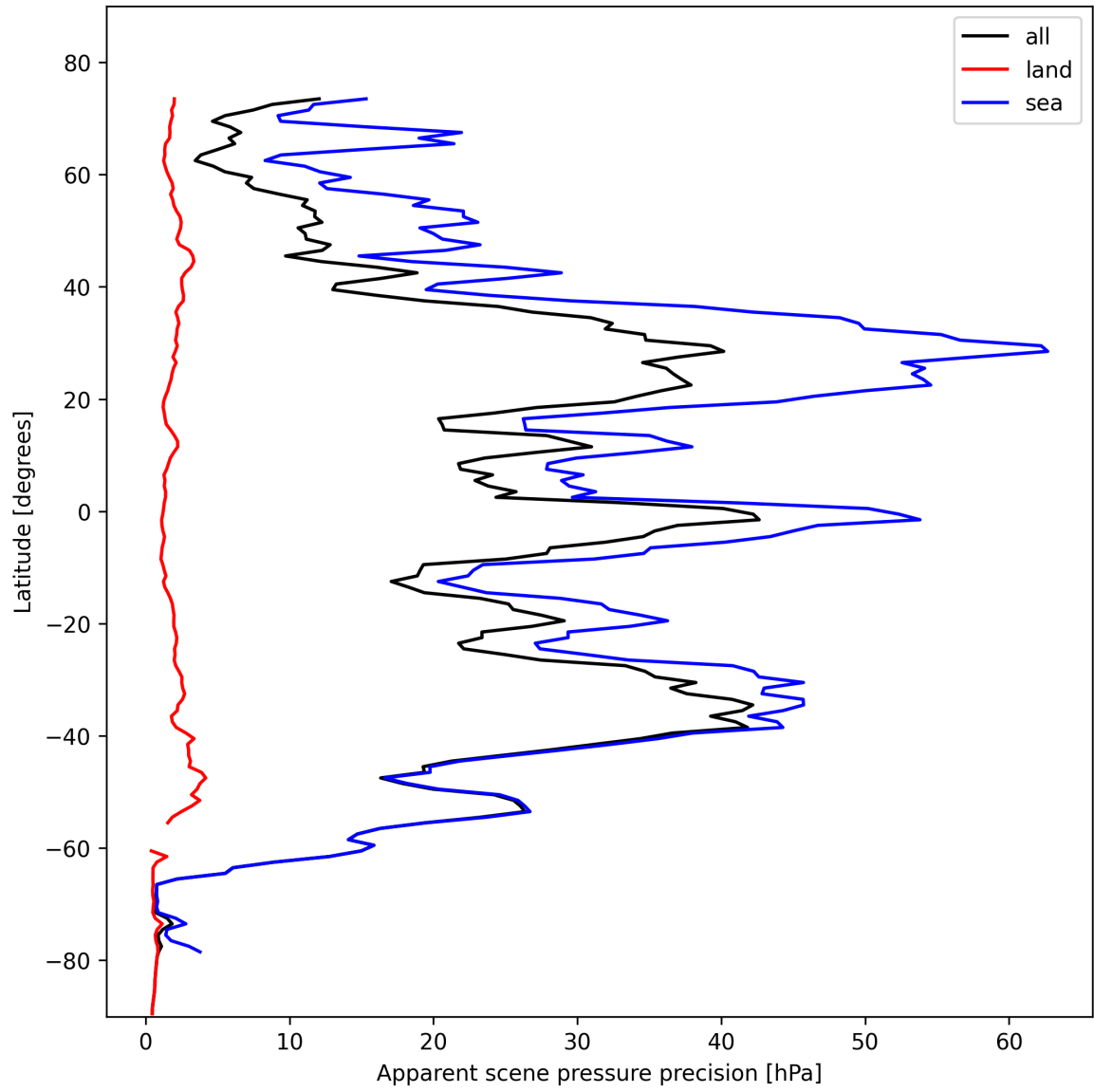
Figure 20: Zonal average of “Apparent scene pressure precision” for 2024-10-30 to 2024-11-01.
