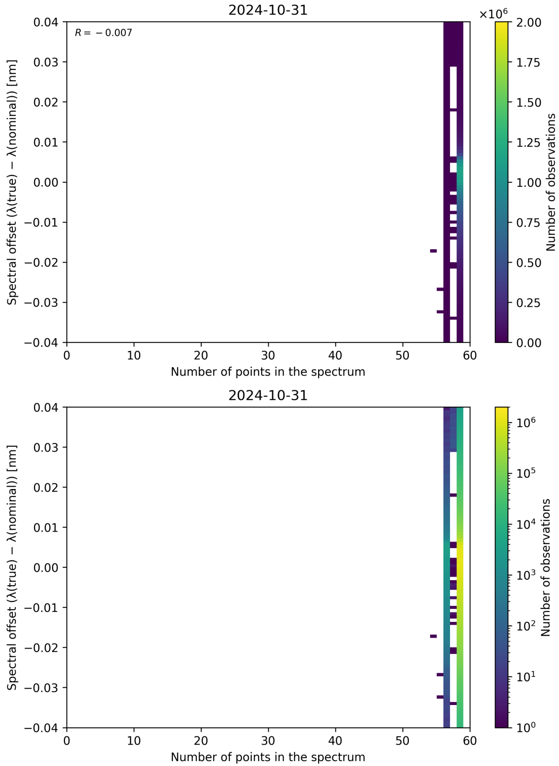
Figure 110: Scatter density plot of “Number of points in the spectrum” against “Spectral offset ( \lambda_{\text{true}} - \lambda_{\text{nominal}} )” for 2024-10-30 to 2024-11-01.
