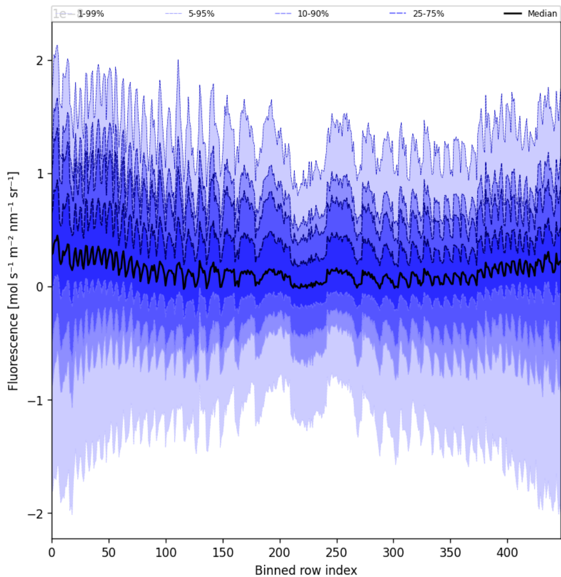
Figure 57: Along track statistics of “Fluorescence” for 2024-10-30 to 2024-11-01
