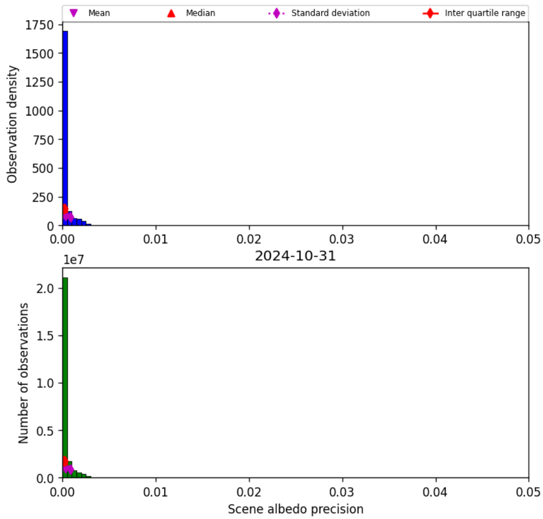
Figure 35: Histogram of “Scene albedo precision” for 2024-10-30 to 2024-11-01
