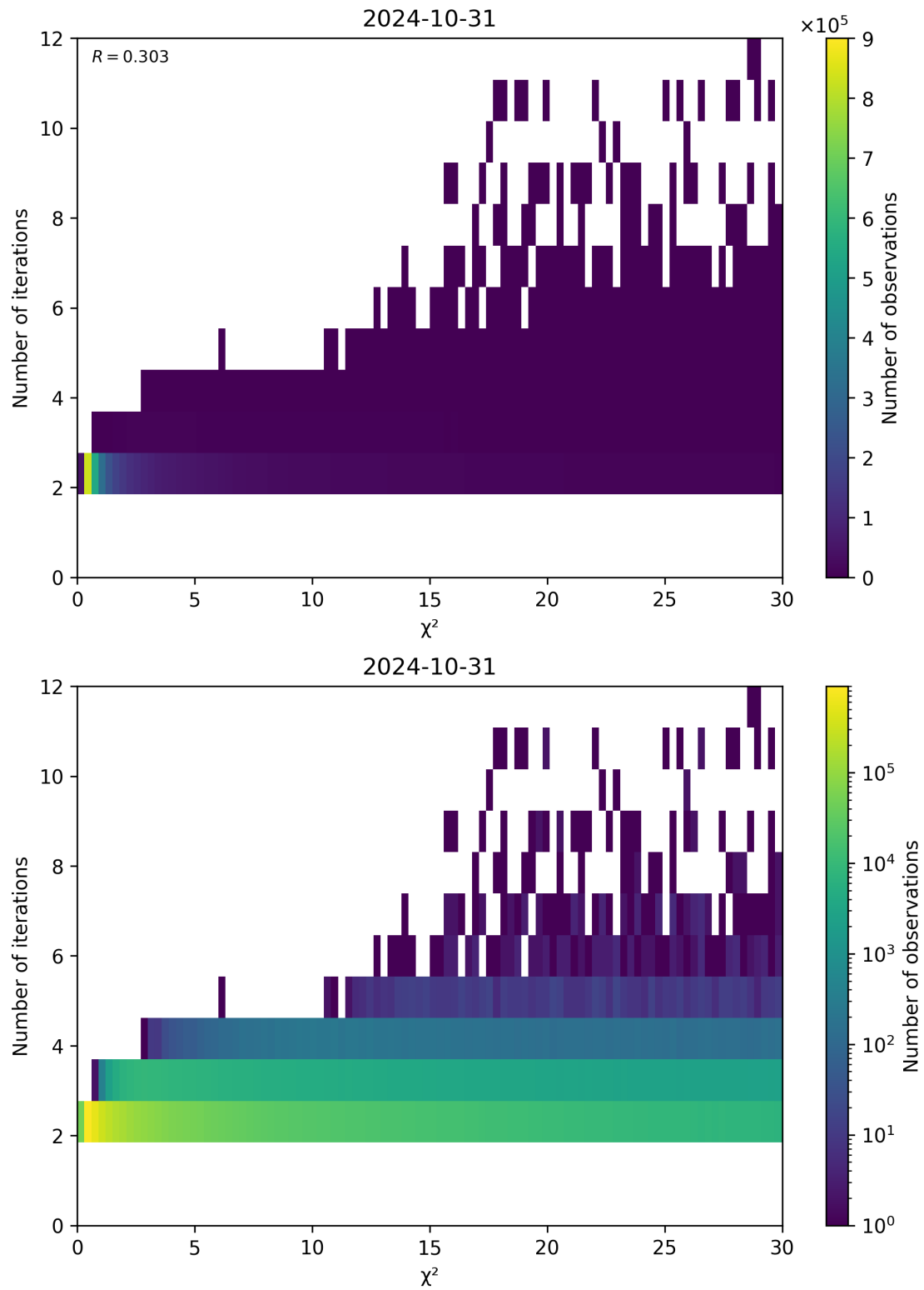
Figure 73: Scatter density plot of “ \chi^2 ” against “Number of iterations” for 2024-10-30 to 2024-11-01.
