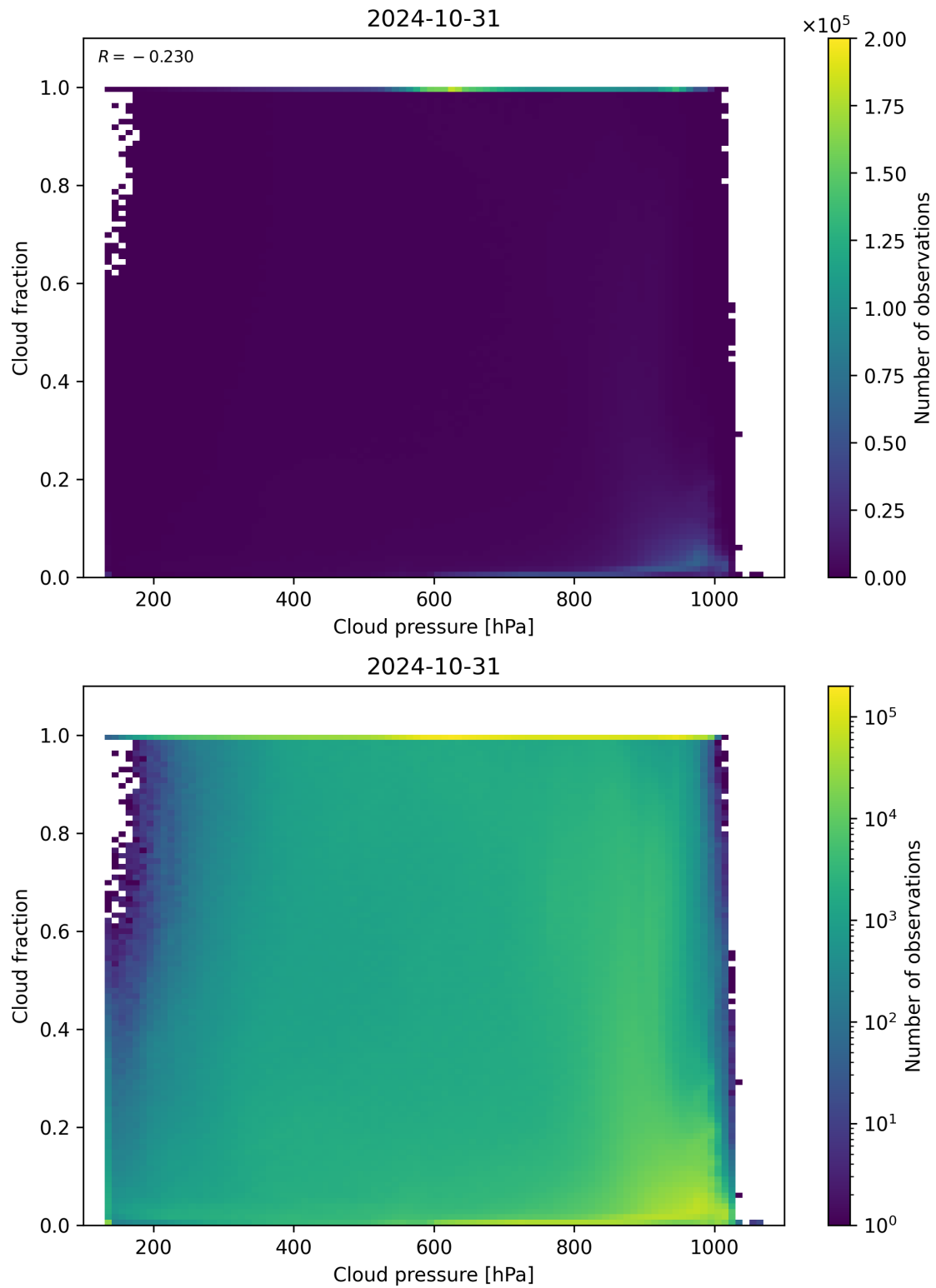
Figure 87: Scatter density plot of “Cloud pressure” against “Cloud fraction” for 2024-10-30 to 2024-11-01.
