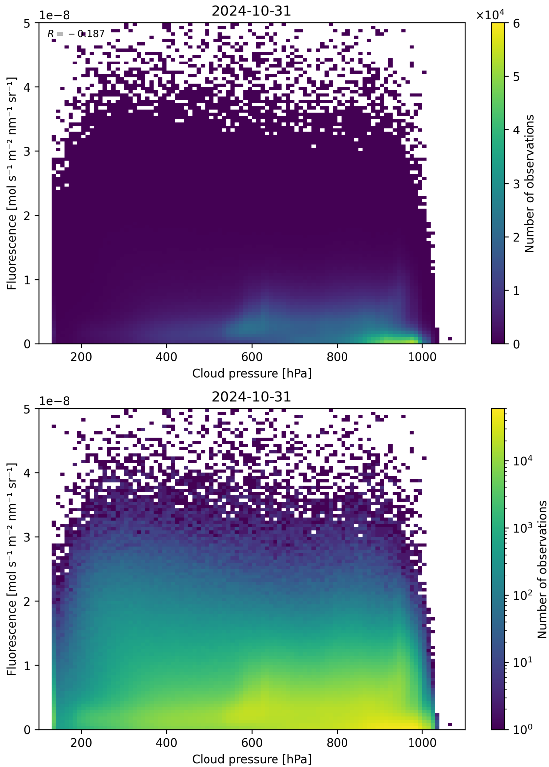
Figure 88: Scatter density plot of “Cloud pressure” against “Fluorescence” for 2024-10-30 to 2024-11-01.
