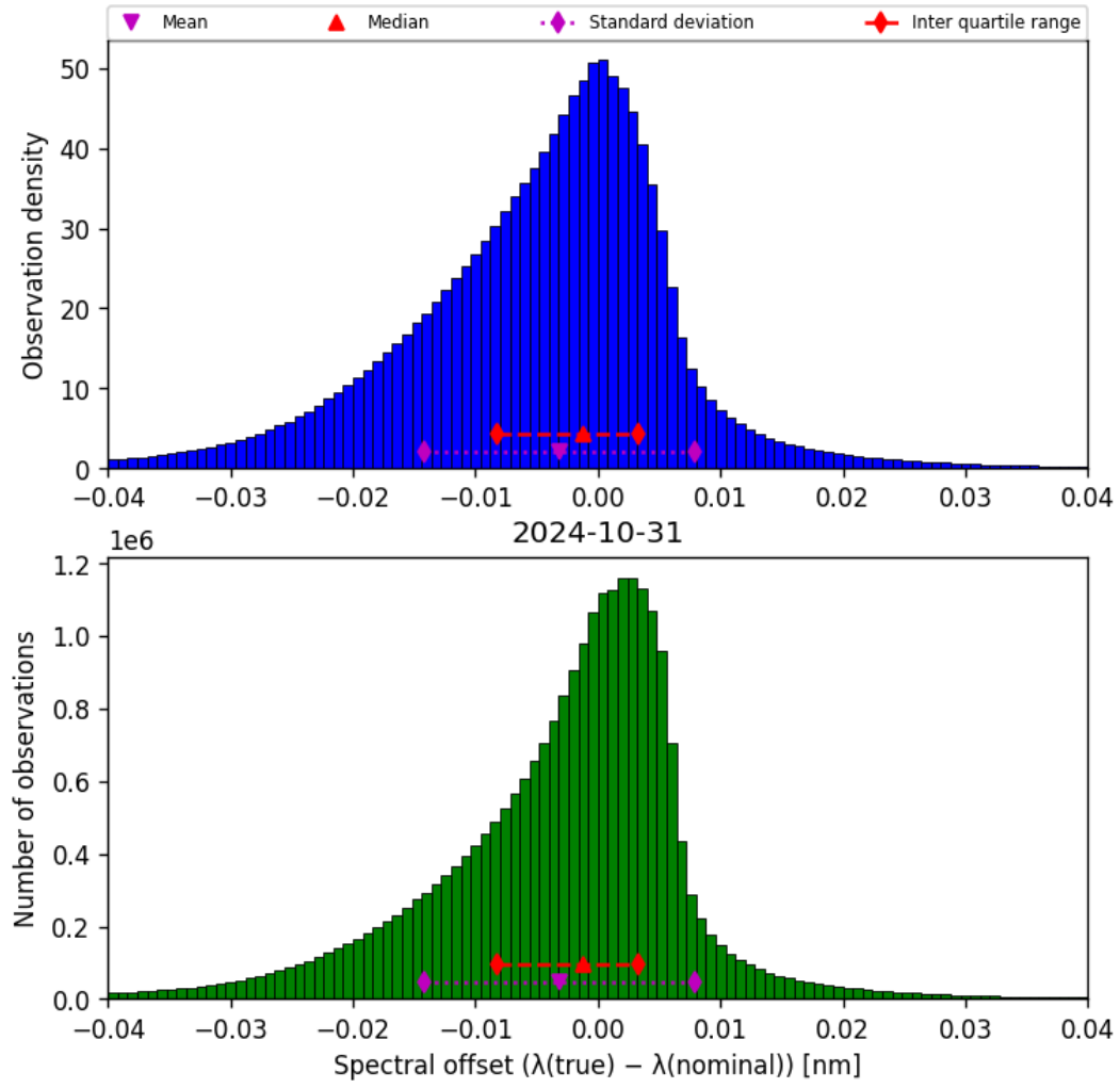
Figure 45: Histogram of “Spectral offset ( \lambda_{\text{true}} - \lambda_{\text{nominal}} )” for 2024-10-30 to 2024-11-01
