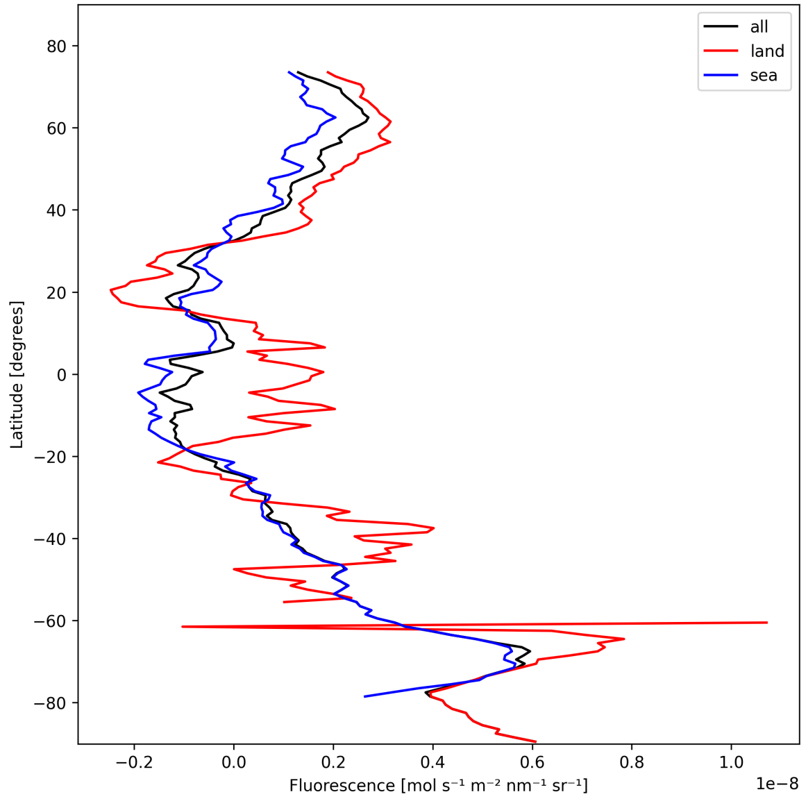
Figure 23: Zonal average of “Fluorescence” for 2024-10-30 to 2024-11-01.
