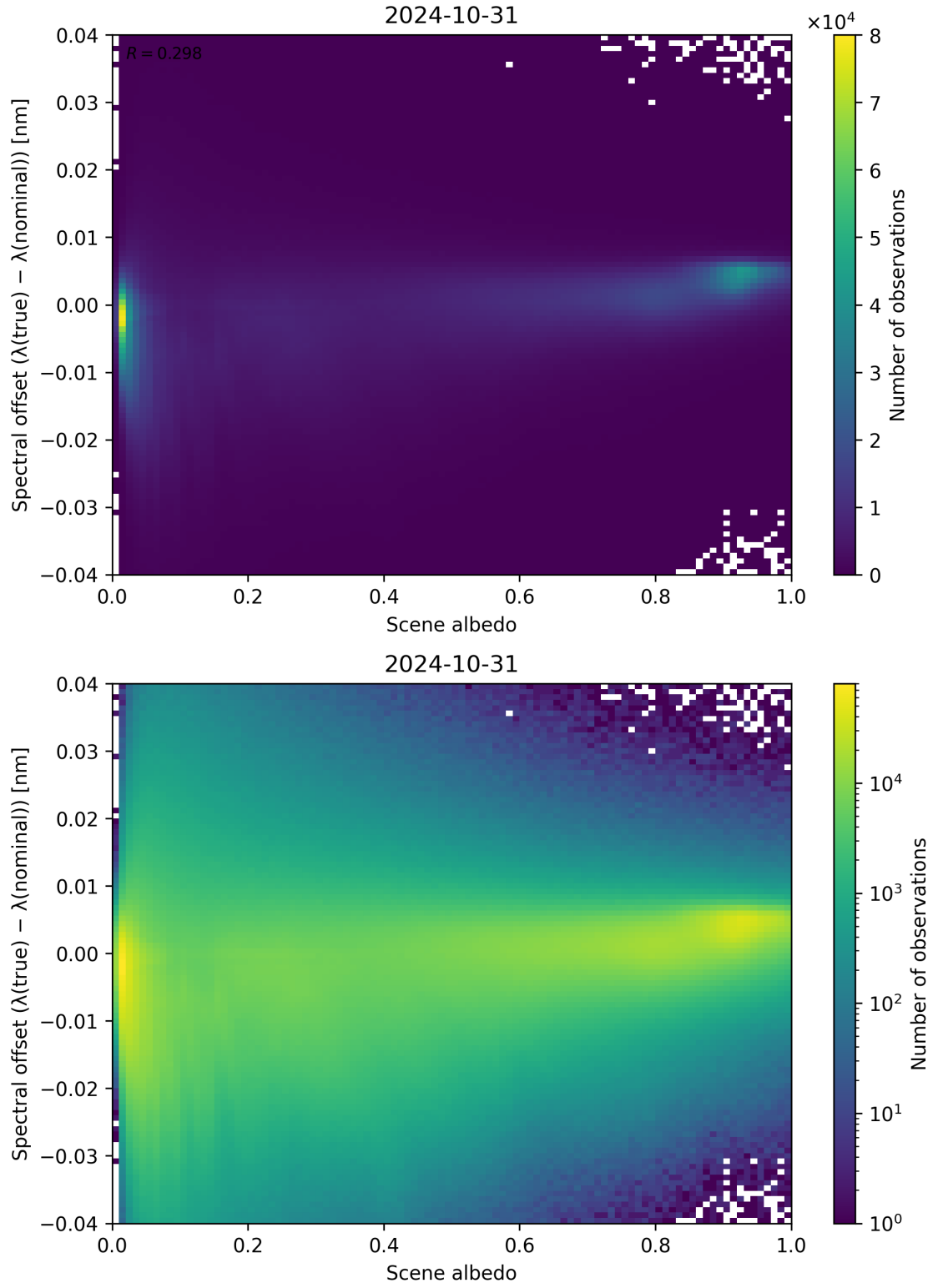
Figure 117: Scatter density plot of “Scene albedo” against “Spectral offset ( \lambda_{\text{true}} - \lambda_{\text{nominal}} )” for 2024-10-30 to 2024-11-01.
