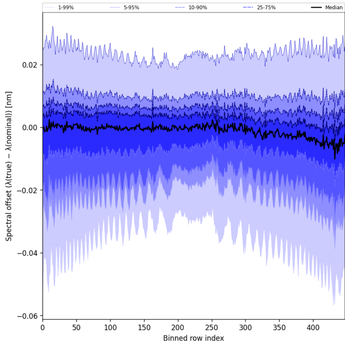
Figure 62: Along track statistics of “Spectral offset ( \lambda_{\text{true}} - \lambda_{\text{nominal}} )” for 2024-10-30 to 2024-11-01
