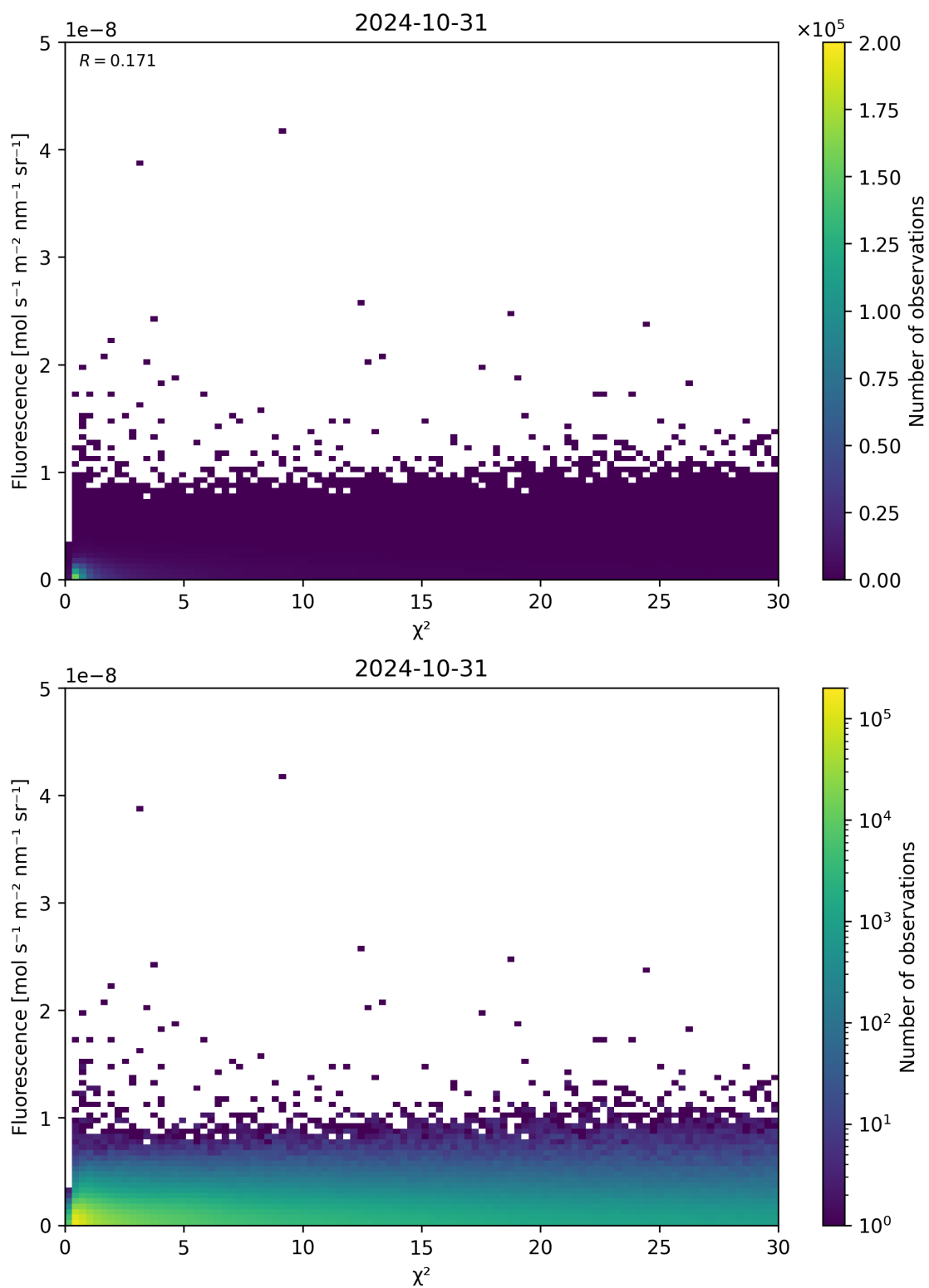
Figure 70: Scatter density plot of “ \chi^2 ” against “Fluorescence” for 2024-10-30 to 2024-11-01.
