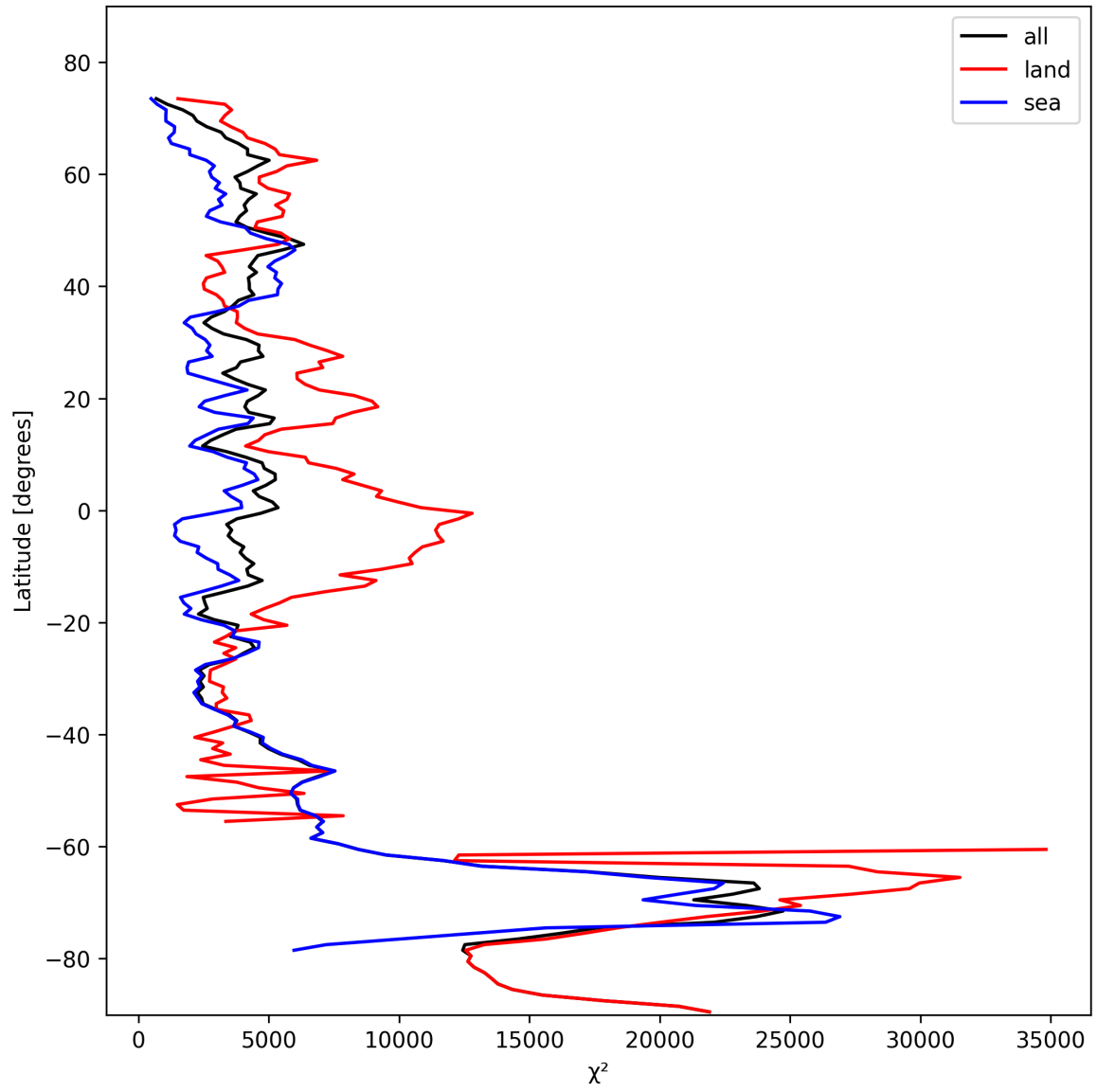
Figure 21: Zonal average of “ \chi^2 ” for 2024-10-30 to 2024-11-01.
