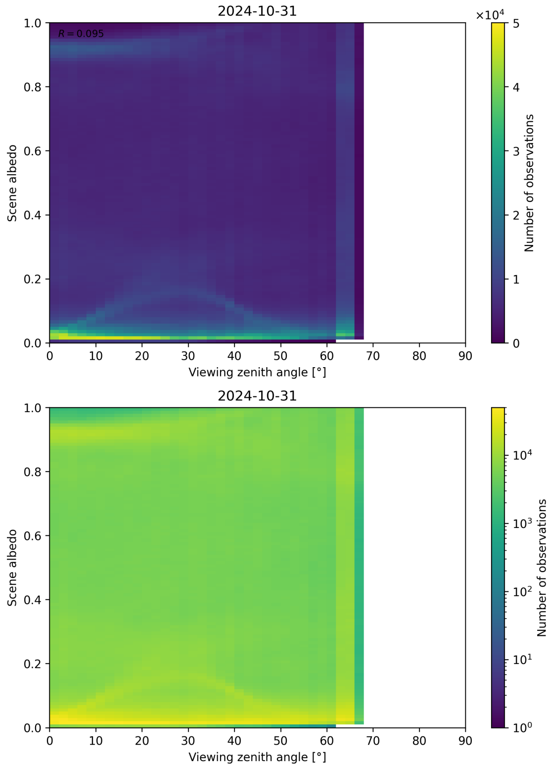
Figure 138: Scatter density plot of “Viewing zenith angle” against “Scene albedo” for 2024-10-30 to 2024-11-01.
