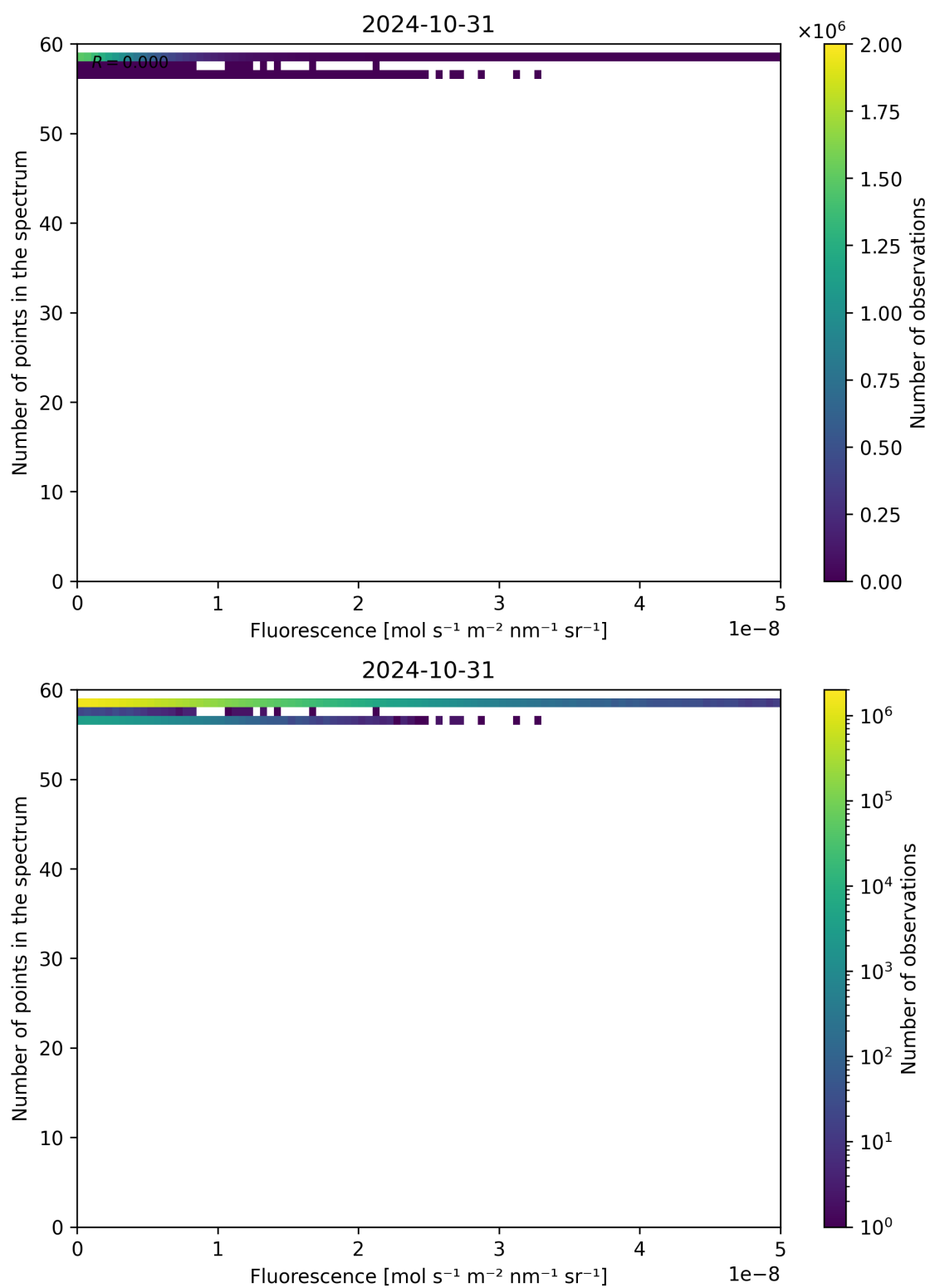
Figure 94: Scatter density plot of “Fluorescence” against “Number of points in the spectrum” for 2024-10-30 to 2024-11-01.
