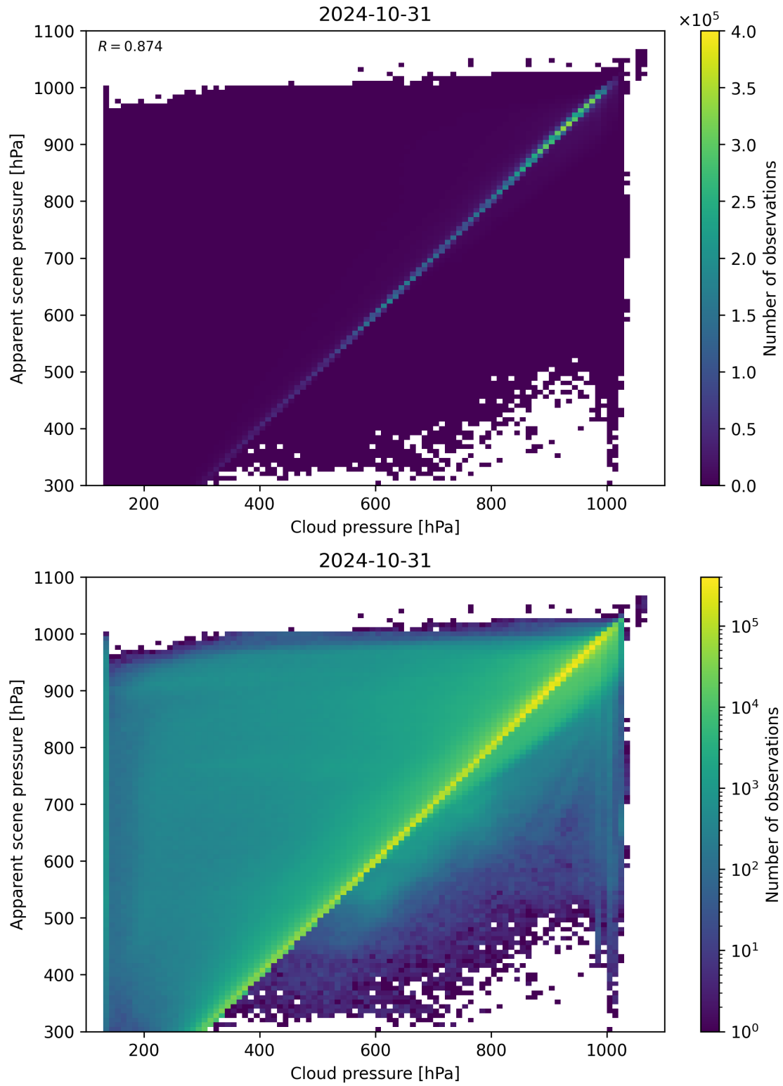
Figure 84: Scatter density plot of “Cloud pressure” against “Apparent scene pressure” for 2024-10-30 to 2024-11-01.
