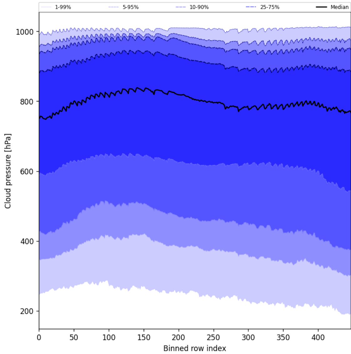
Figure 47: Along track statistics of “Cloud pressure” for 2024-10-30 to 2024-11-01
