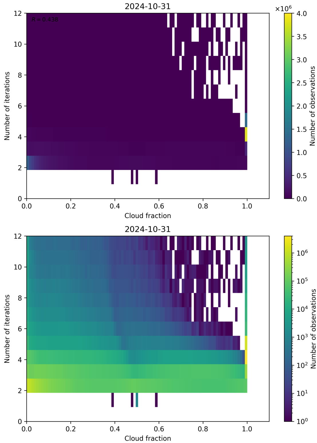
Figure 80: Scatter density plot of “Cloud fraction” against “Number of iterations” for 2024-10-30 to 2024-11-01.
