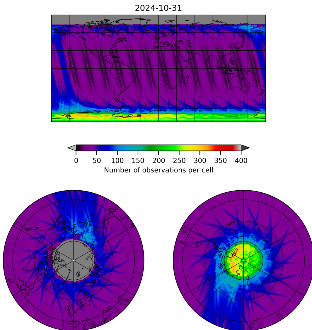
Figure 11: Map of the number of observations for 2024-10-30 to 2024-11-01
