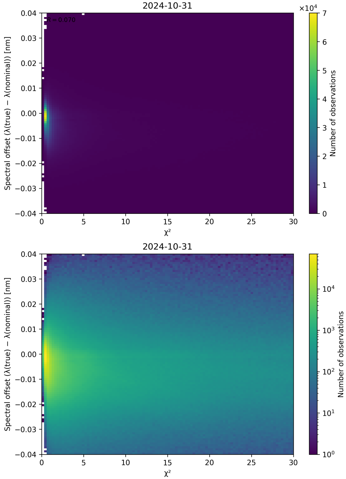
Figure 75: Scatter density plot of “ \chi^2 ” against “Spectral offset ( \lambda_{\text{true}} - \lambda_{\text{nominal}} )” for 2024-10-30 to 2024-11-01.
