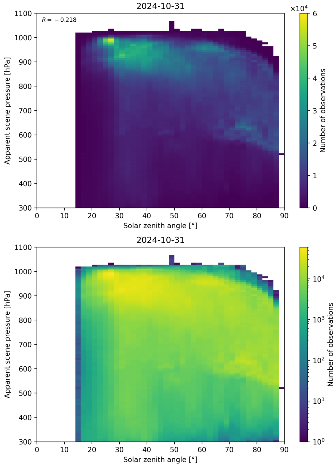
Figure 118: Scatter density plot of “Solar zenith angle” against “Apparent scene pressure” for 2024-10-30 to 2024-11-01.
