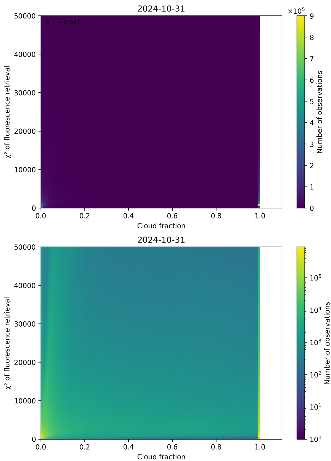
Figure 78: Scatter density plot of “Cloud fraction” against “ \chi^2 of fluorescence retrieval” for 2024-10-30 to 2024-11-01.
