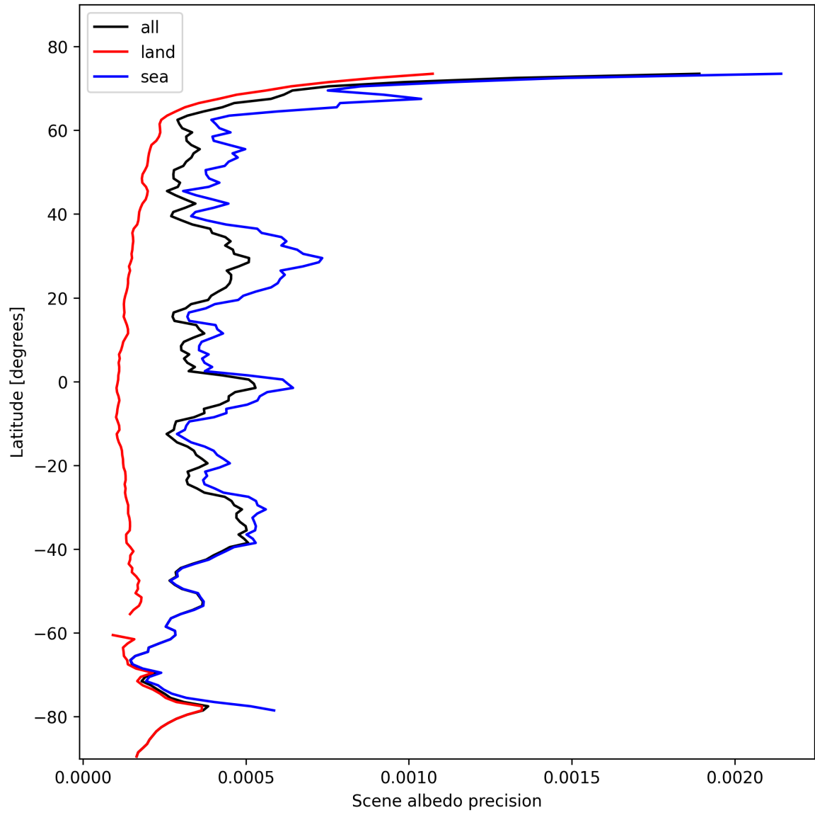
Figure 18: Zonal average of "Scene albedo precision" for 2024-10-30 to 2024-11-01.
