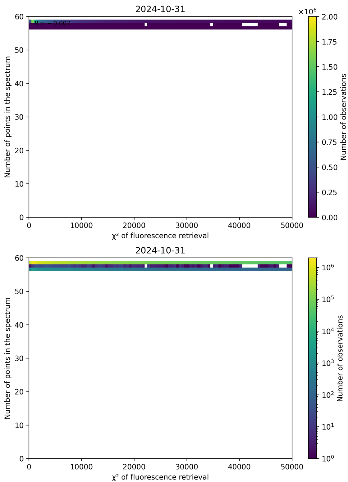
Figure 71: Scatter density plot of “ \chi^2 of fluorescence retrieval” against “Number of points in the spectrum” for 2024-10-30 to 2024-11-01.
