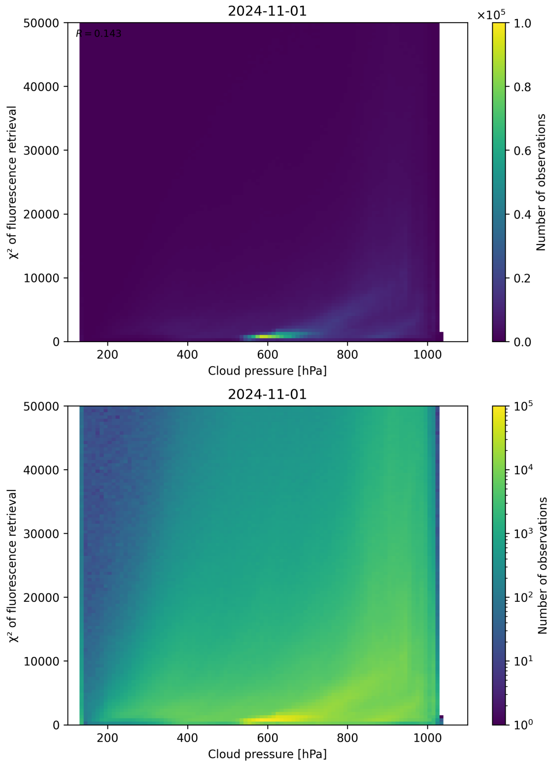
Figure 86: Scatter density plot of “Cloud pressure” against “ \chi^2 of fluorescence retrieval” for 2024-10-31 to 2024-11-02.
