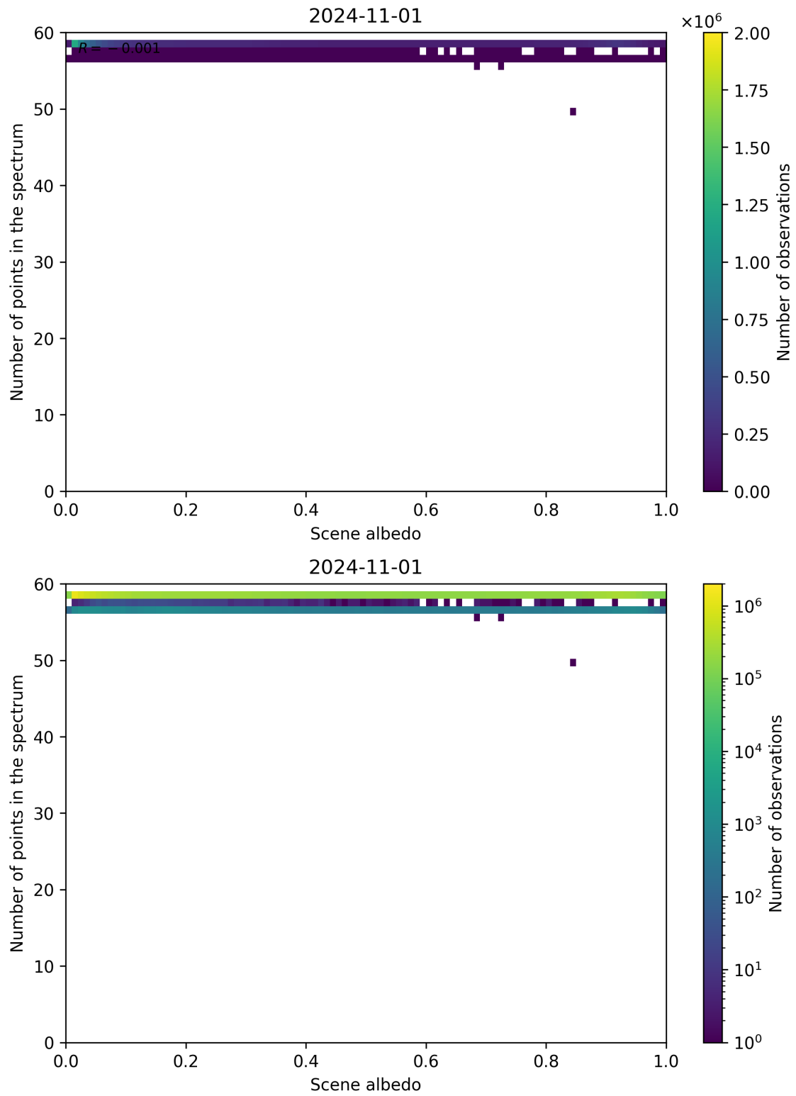
Figure 116: Scatter density plot of “Scene albedo” against “Number of points in the spectrum” for 2024-10-31 to 2024-11-02.
