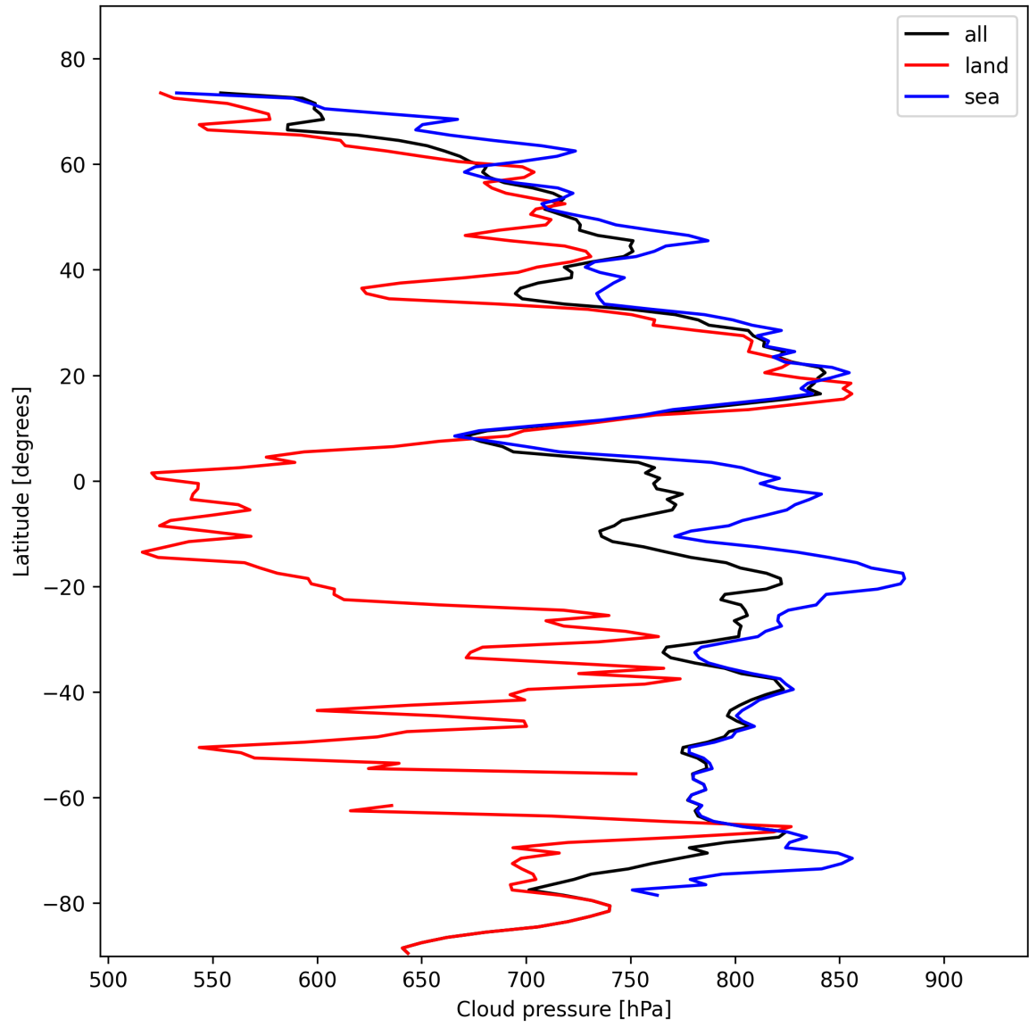
Figure 13: Zonal average of “Cloud pressure” for 2024-10-31 to 2024-11-02.
