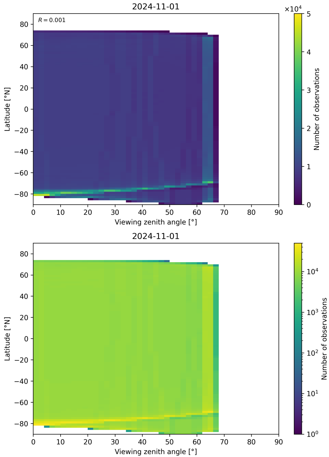
Figure 135: Scatter density plot of “Viewing zenith angle” against “Latitude” for 2024-10-31 to 2024-11-02.
