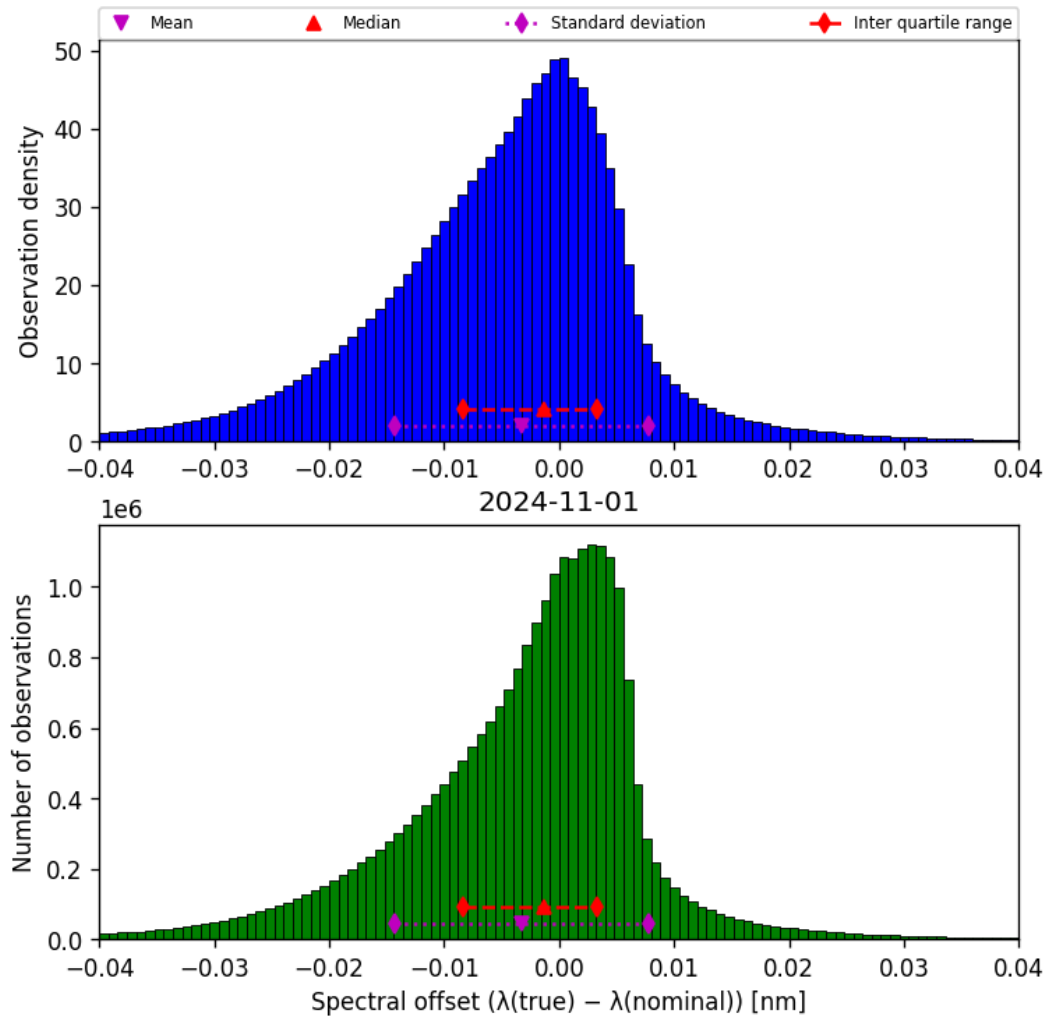
Figure 45: Histogram of “Spectral offset ( \lambda_{\text{true}} - \lambda_{\text{nominal}} )” for 2024-10-31 to 2024-11-02
