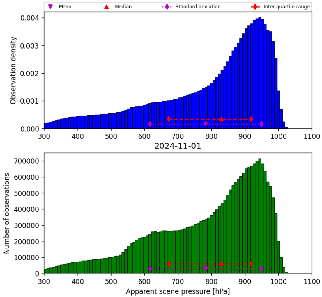
Figure 36: Histogram of “Apparent scene pressure” for 2024-10-31 to 2024-11-02
