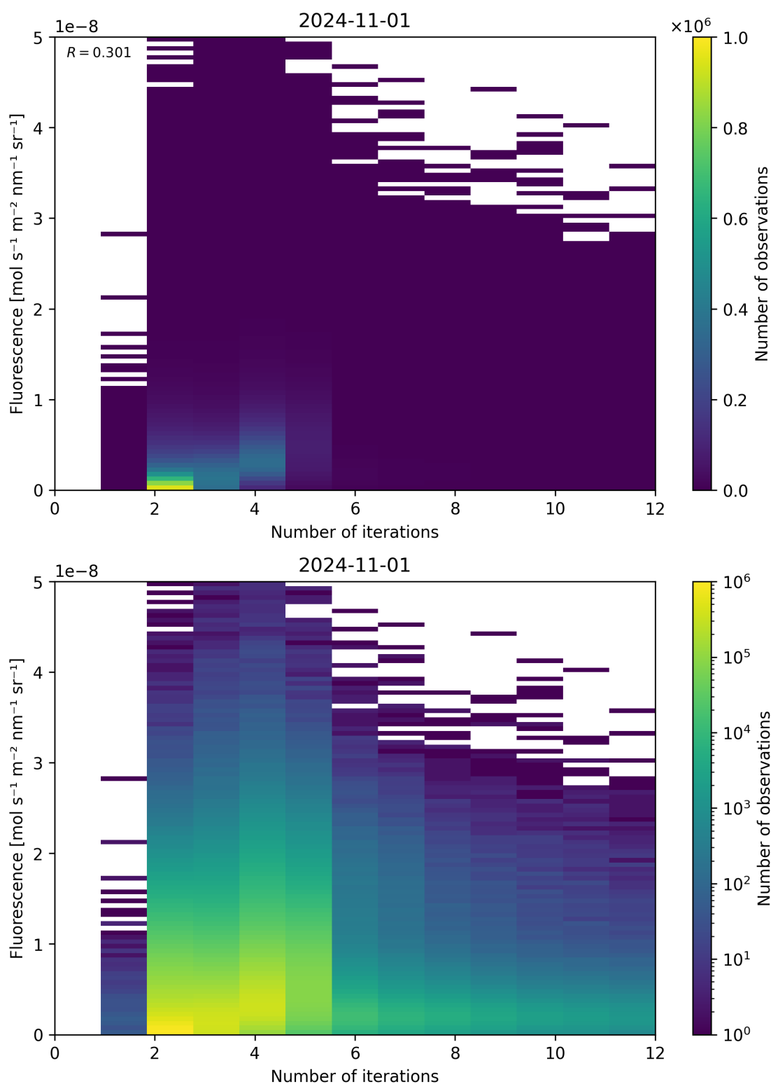
Figure 107: Scatter density plot of “Number of iterations” against “Fluorescence” for 2024-10-31 to 2024-11-02.
