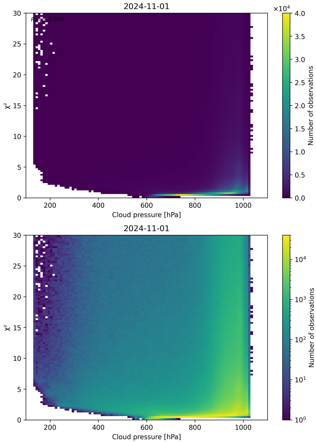
Figure 85: Scatter density plot of “Cloud pressure” against “ \chi^2 ” for 2024-10-31 to 2024-11-02.
