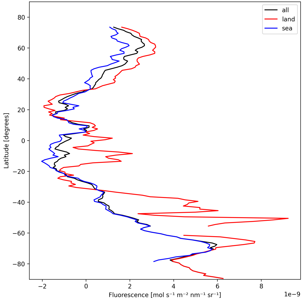
Figure 23: Zonal average of “Fluorescence” for 2024-10-31 to 2024-11-02.
