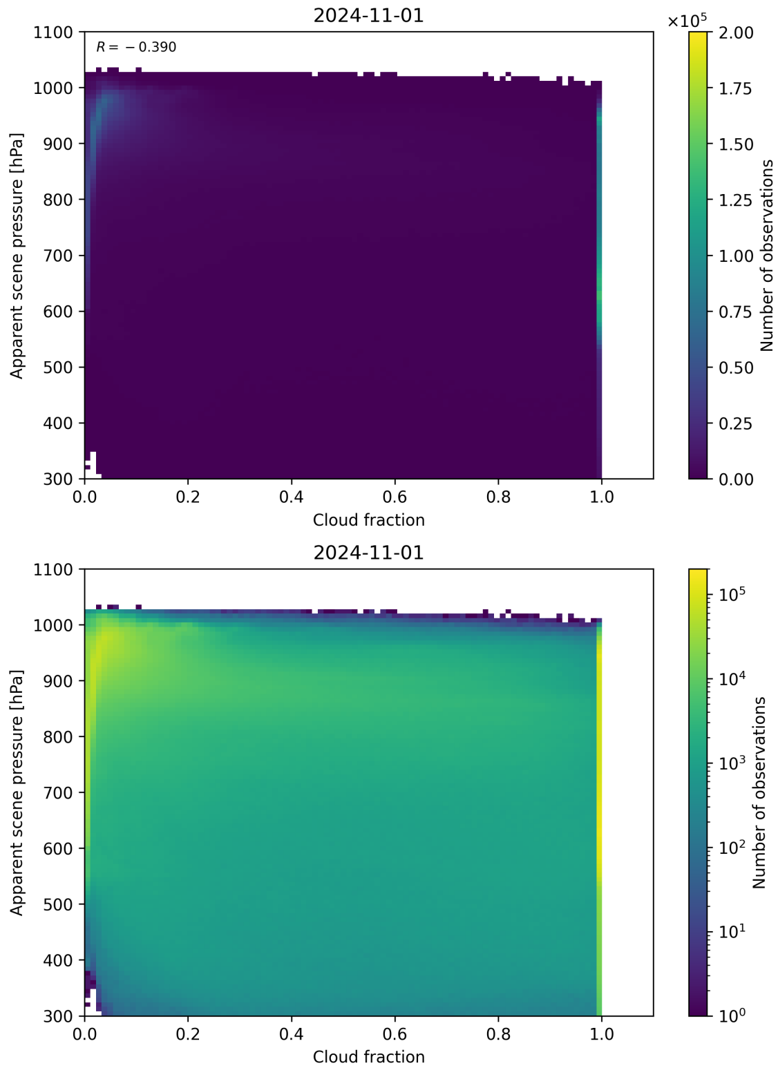
Figure 76: Scatter density plot of “Cloud fraction” against “Apparent scene pressure” for 2024-10-31 to 2024-11-02.
