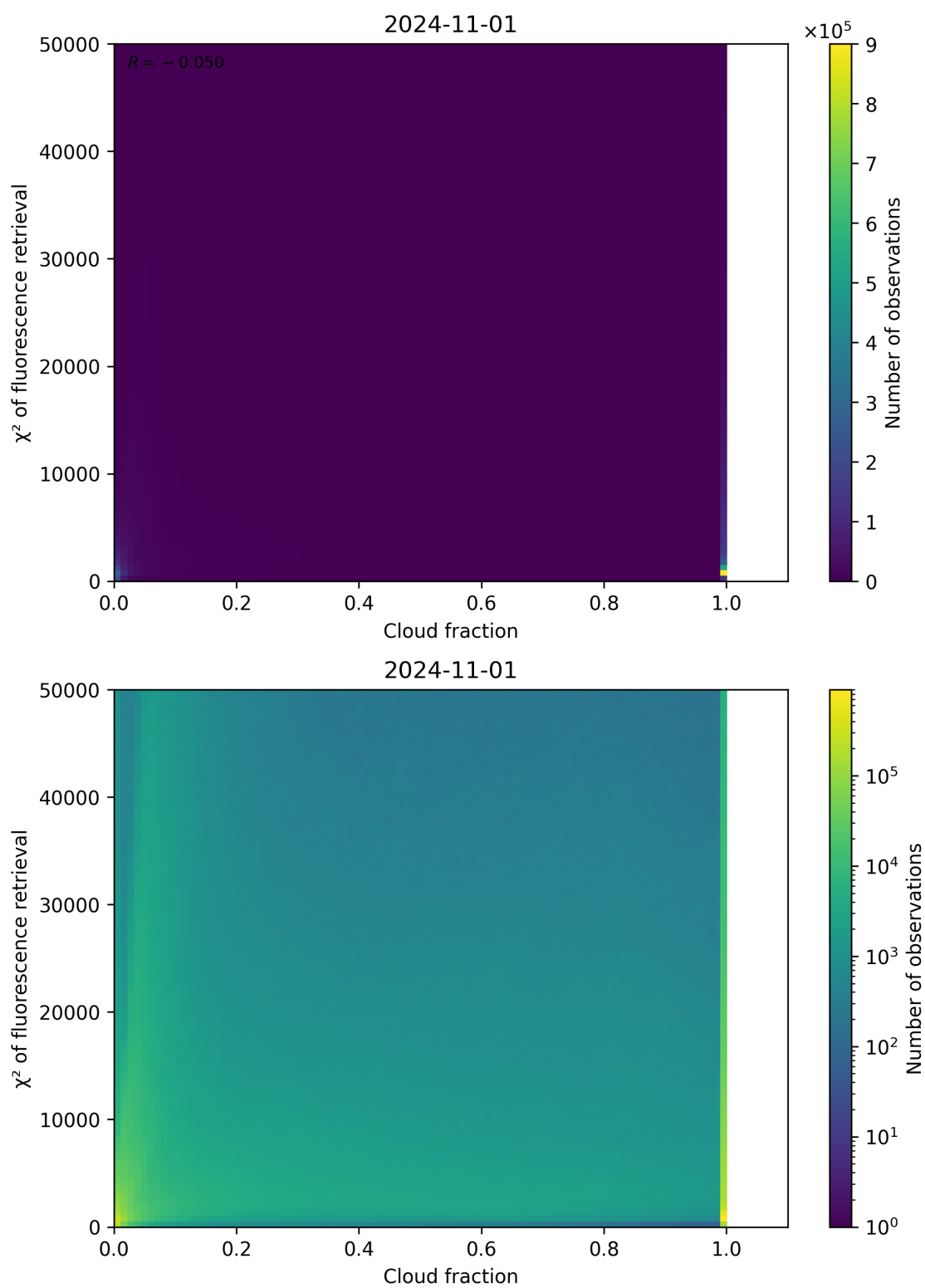
Figure 78: Scatter density plot of “Cloud fraction” against “ \chi^2 of fluorescence retrieval” for 2024-10-31 to 2024-11-02.
