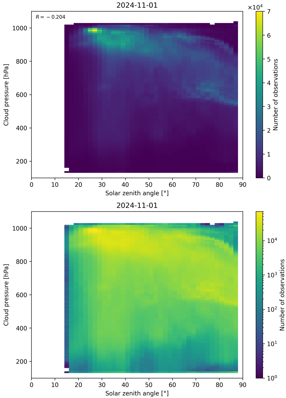
Figure 122: Scatter density plot of “Solar zenith angle” against “Cloud pressure” for 2024-10-31 to 2024-11-02.
