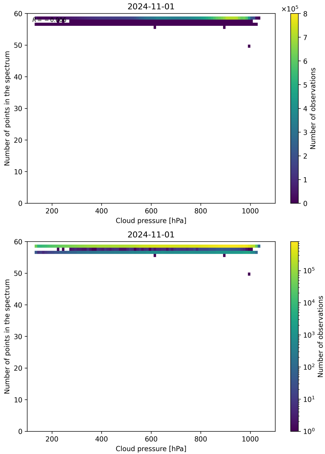
Figure 90: Scatter density plot of “Cloud pressure” against “Number of points in the spectrum” for 2024-10-31 to 2024-11-02.
