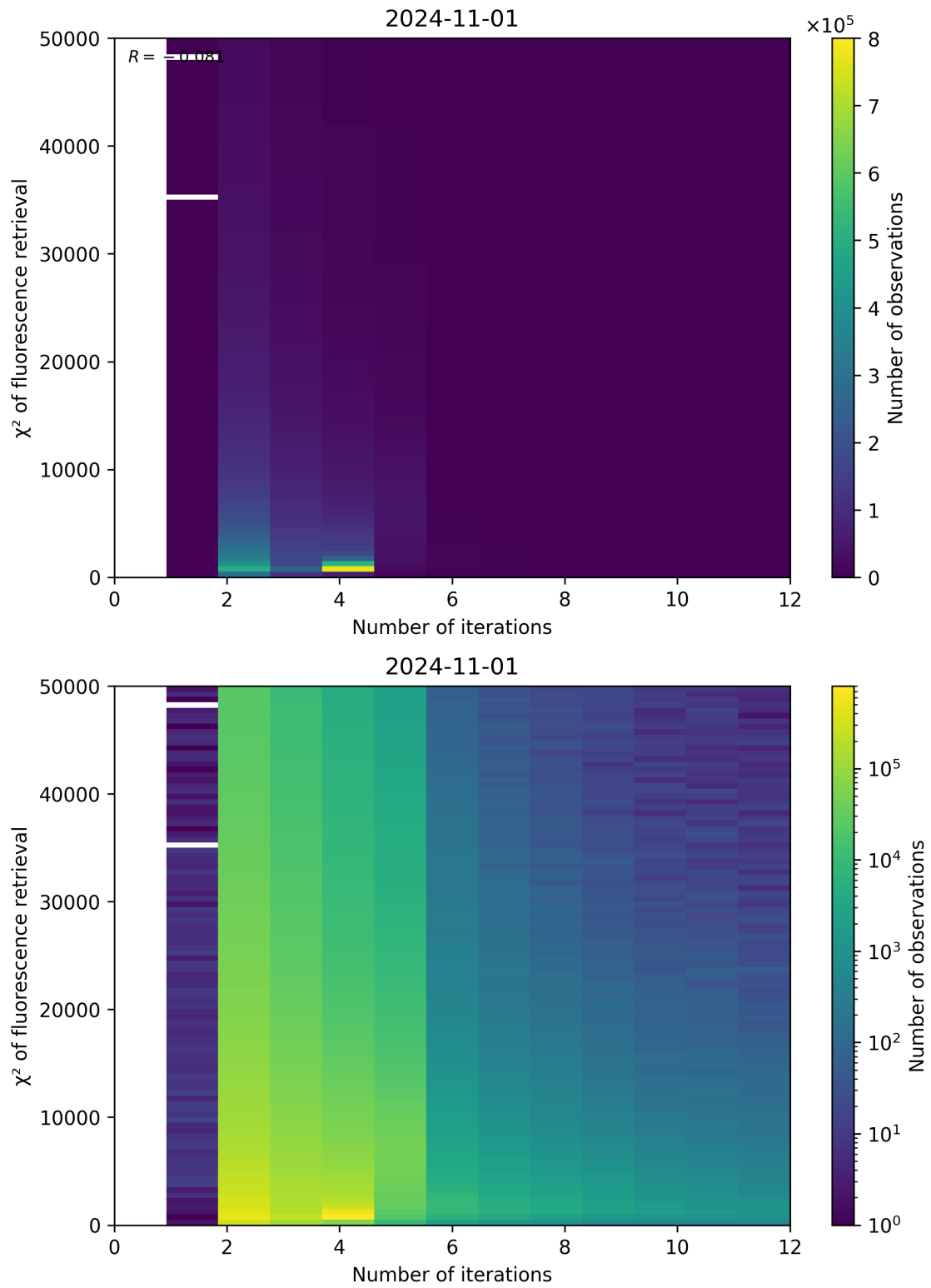
Figure 106: Scatter density plot of “Number of iterations” against “ \chi^2 of fluorescence retrieval” for 2024-10-31 to 2024-11-02.
