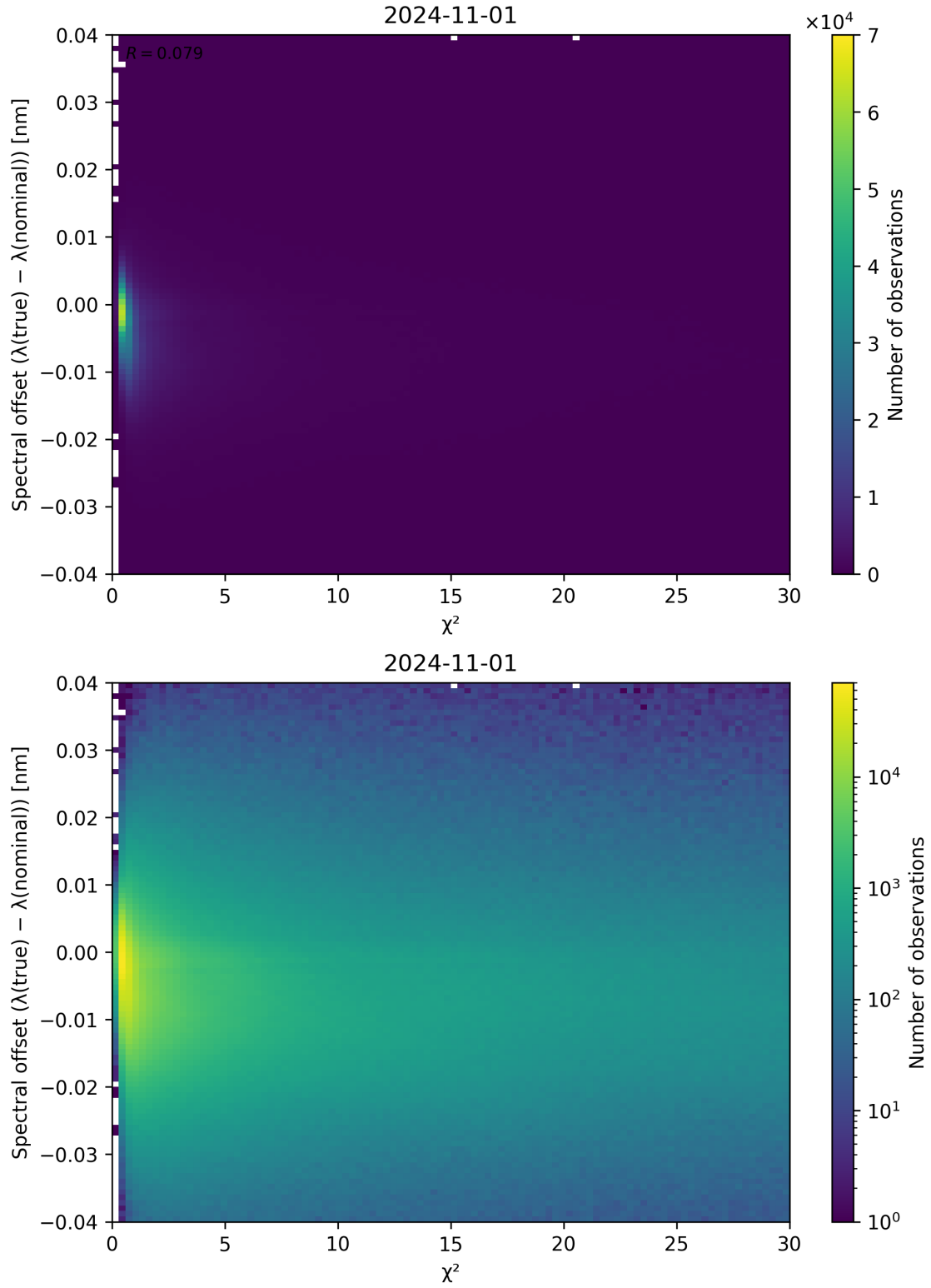
Figure 75: Scatter density plot of “ \chi^2 ” against “Spectral offset ( \lambda_{\text{true}} - \lambda_{\text{nominal}} )” for 2024-10-31 to 2024-11-02.
