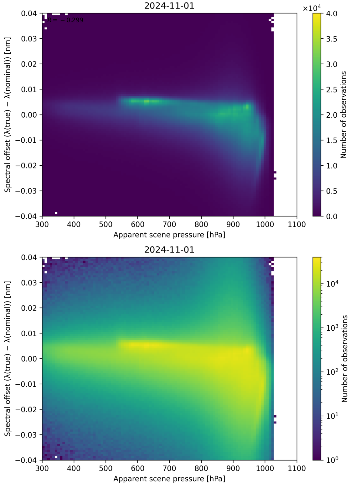
Figure 68: Scatter density plot of “Apparent scene pressure” against “Spectral offset ( \lambda_{\text{true}} - \lambda_{\text{nominal}} )” for 2024-10-31 to 2024-11-02.
