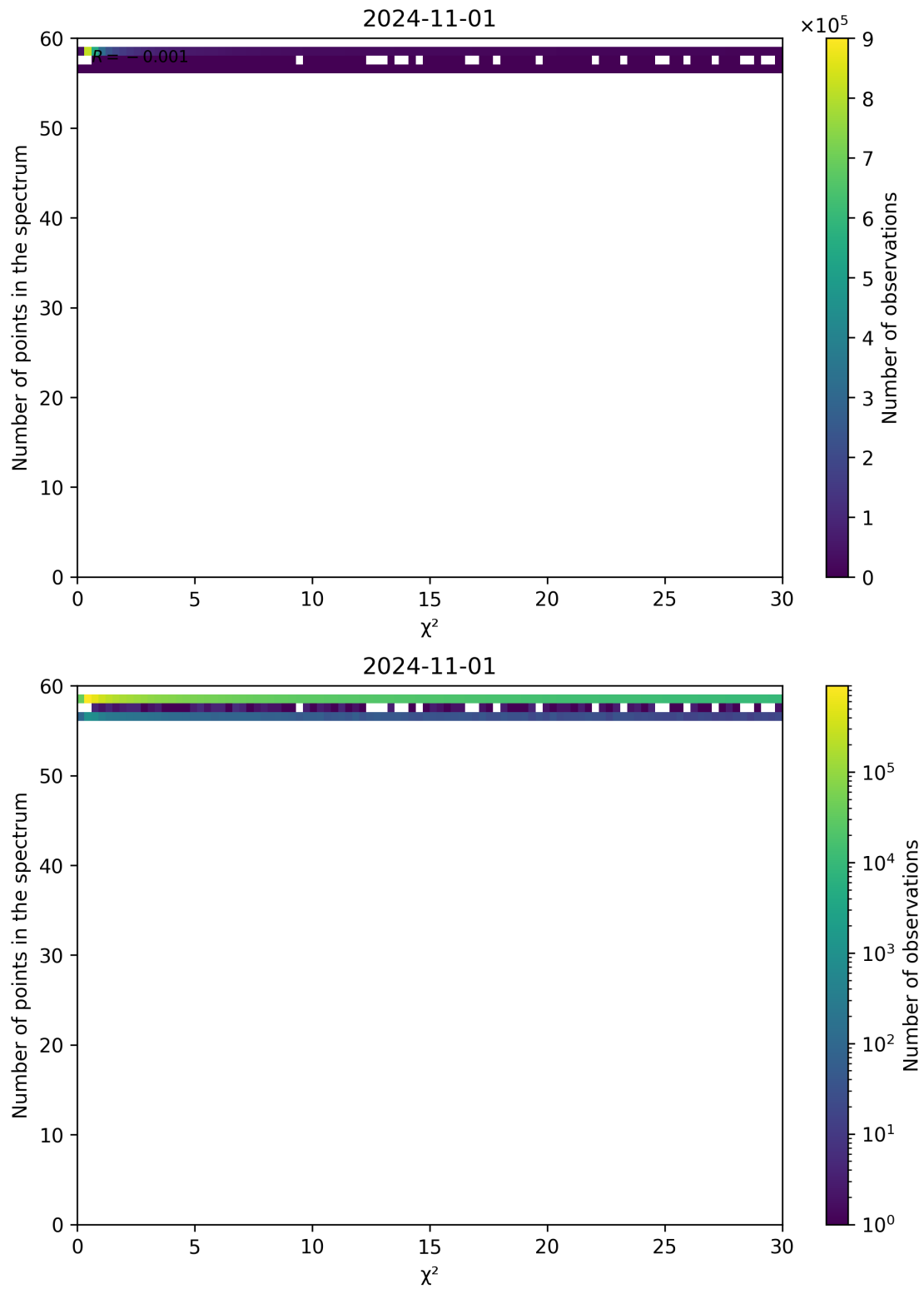
Figure 74: Scatter density plot of “ \chi^2 ” against “Number of points in the spectrum” for 2024-10-31 to 2024-11-02.
