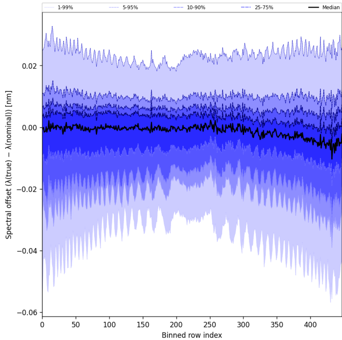
Figure 62: Along track statistics of “Spectral offset ( \lambda_{\text{true}} - \lambda_{\text{nominal}} )” for 2024-10-31 to 2024-11-02
