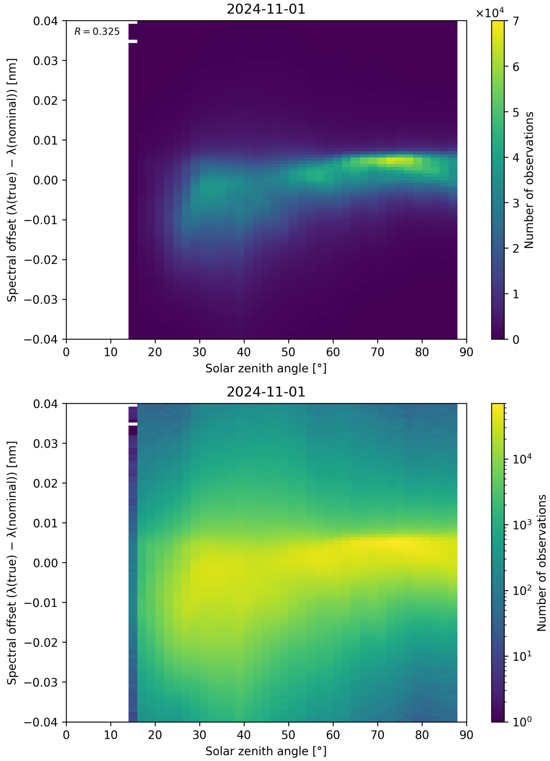
Figure 128: Scatter density plot of “Solar zenith angle” against “Spectral offset ( \lambda_{\text{true}} - \lambda_{\text{nominal}} )” for 2024-10-31 to 2024-11-02.
