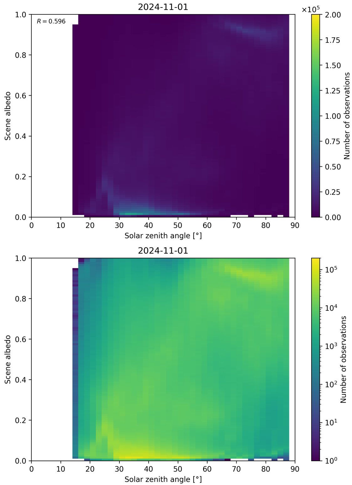
Figure 127: Scatter density plot of “Solar zenith angle” against “Scene albedo” for 2024-10-31 to 2024-11-02.
