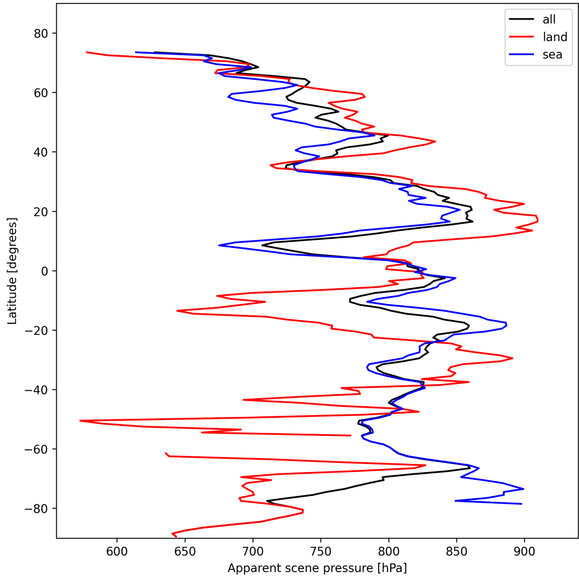
Figure 19: Zonal average of “Apparent scene pressure” for 2024-10-31 to 2024-11-02.
