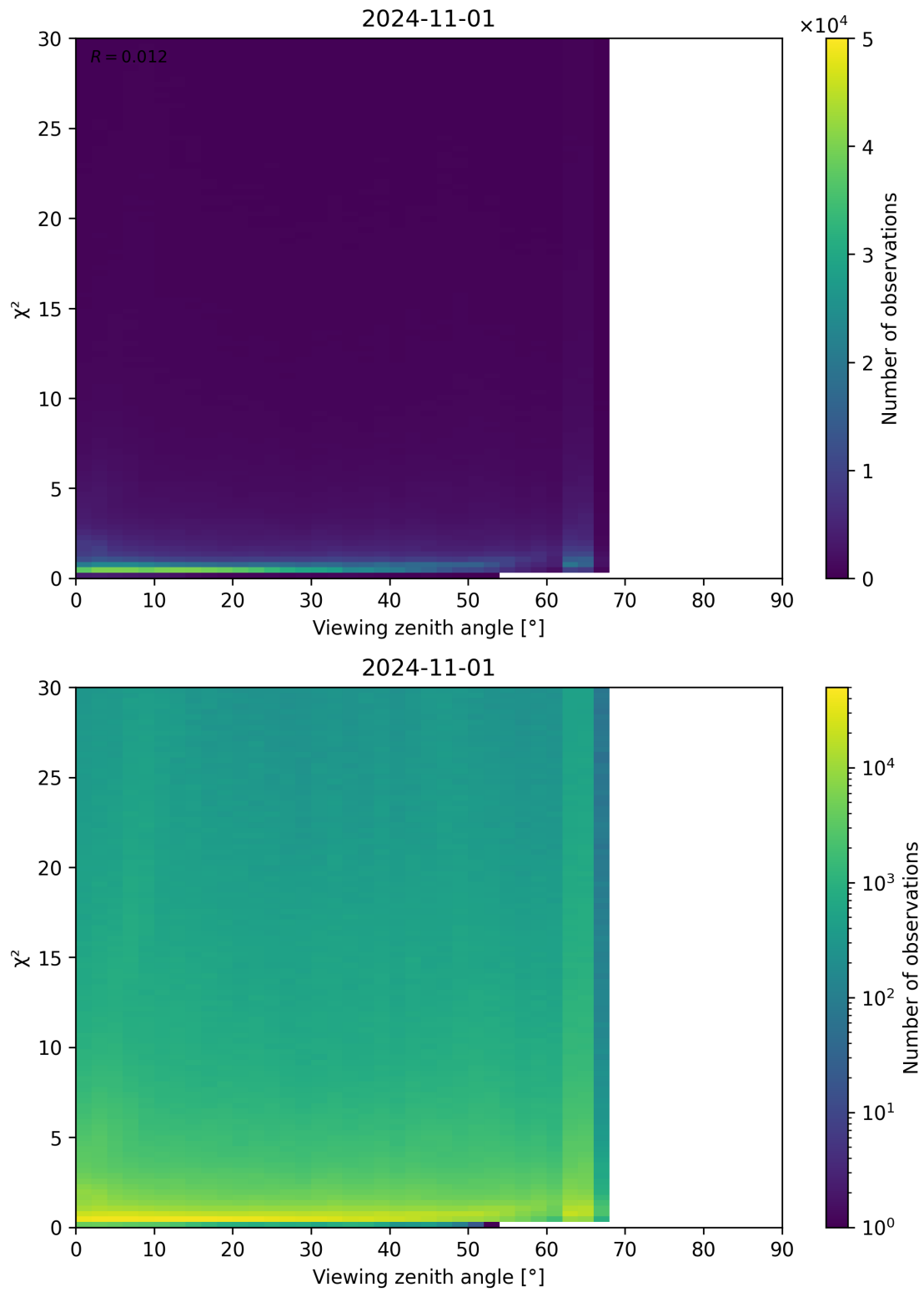
Figure 130: Scatter density plot of “Viewing zenith angle” against “ \chi^2 ” for 2024-10-31 to 2024-11-02.
