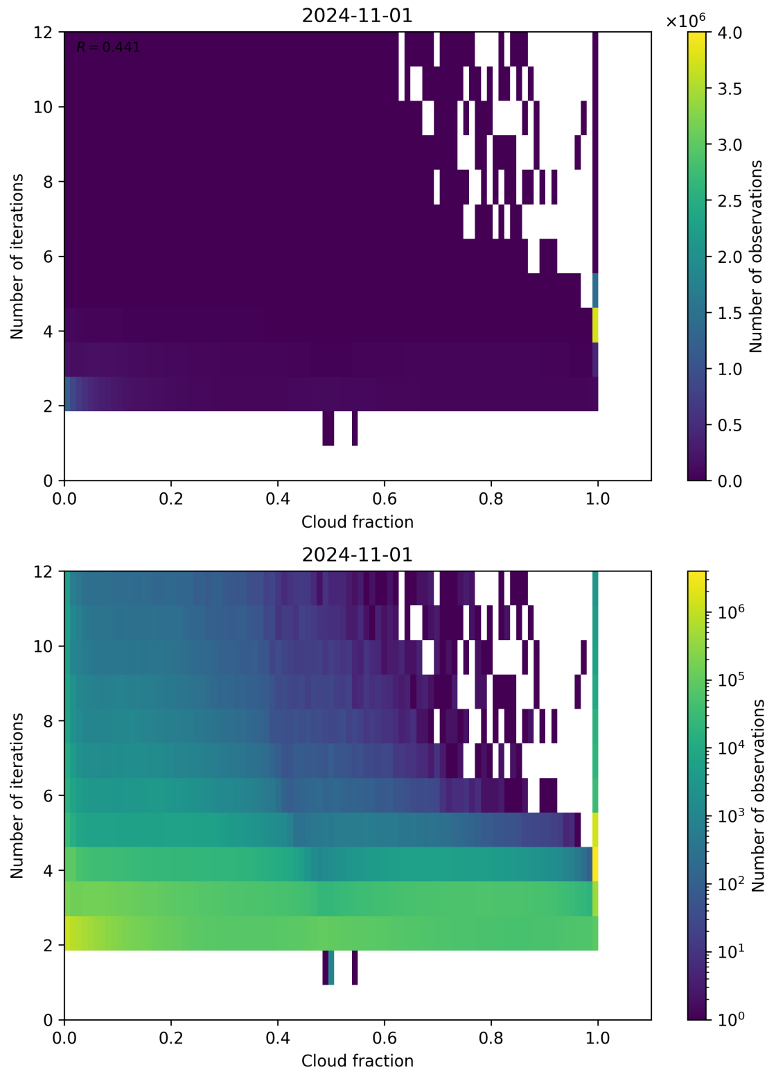
Figure 80: Scatter density plot of “Cloud fraction” against “Number of iterations” for 2024-10-31 to 2024-11-02.
