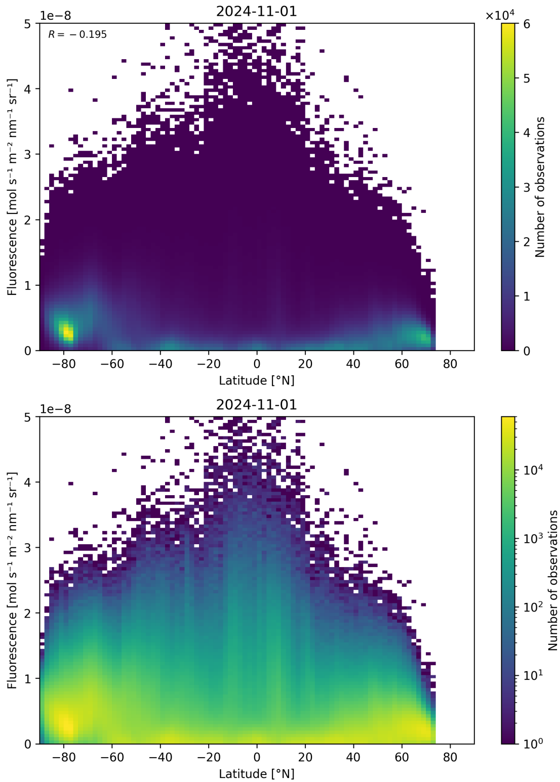
Figure 101: Scatter density plot of “Latitude” against “Fluorescence” for 2024-10-31 to 2024-11-02.
