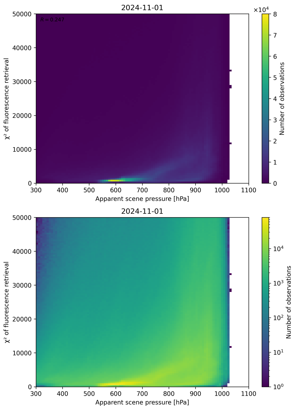
Figure 64: Scatter density plot of “Apparent scene pressure” against “ \chi^2 of fluorescence retrieval” for 2024-10-31 to 2024-11-02.
