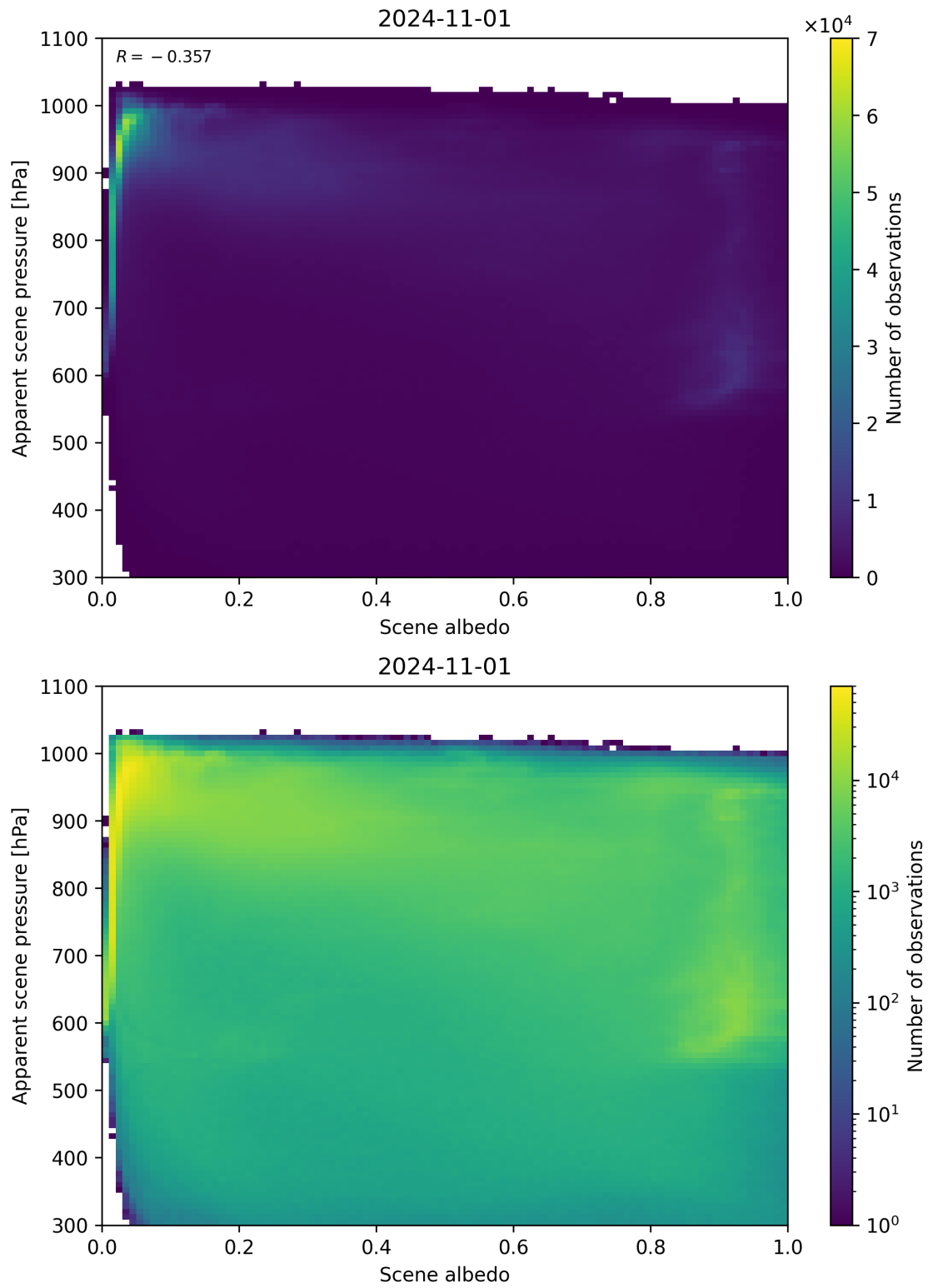
Figure 111: Scatter density plot of “Scene albedo” against “Apparent scene pressure” for 2024-10-31 to 2024-11-02.
