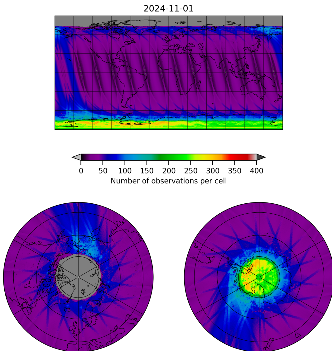
Figure 11: Map of the number of observations for 2024-10-31 to 2024-11-02
