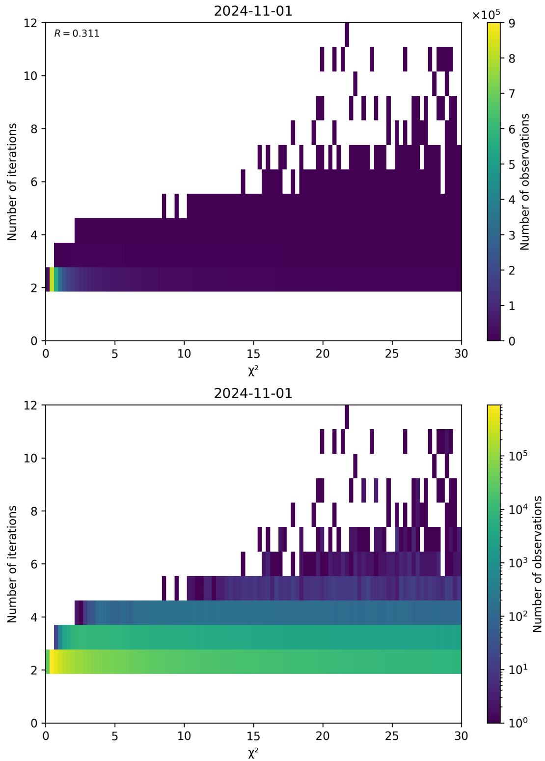
Figure 73: Scatter density plot of “ \chi^2 ” against “Number of iterations” for 2024-10-31 to 2024-11-02.
