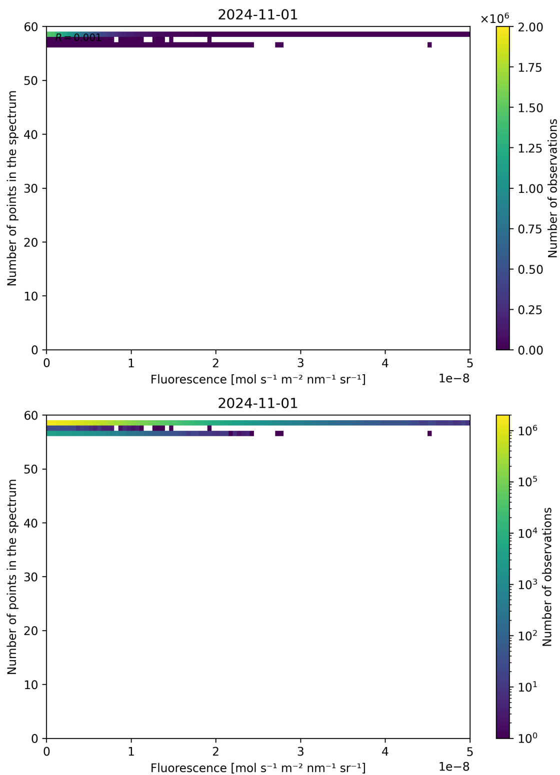
Figure 94: Scatter density plot of “Fluorescence” against “Number of points in the spectrum” for 2024-10-31 to 2024-11-02.
