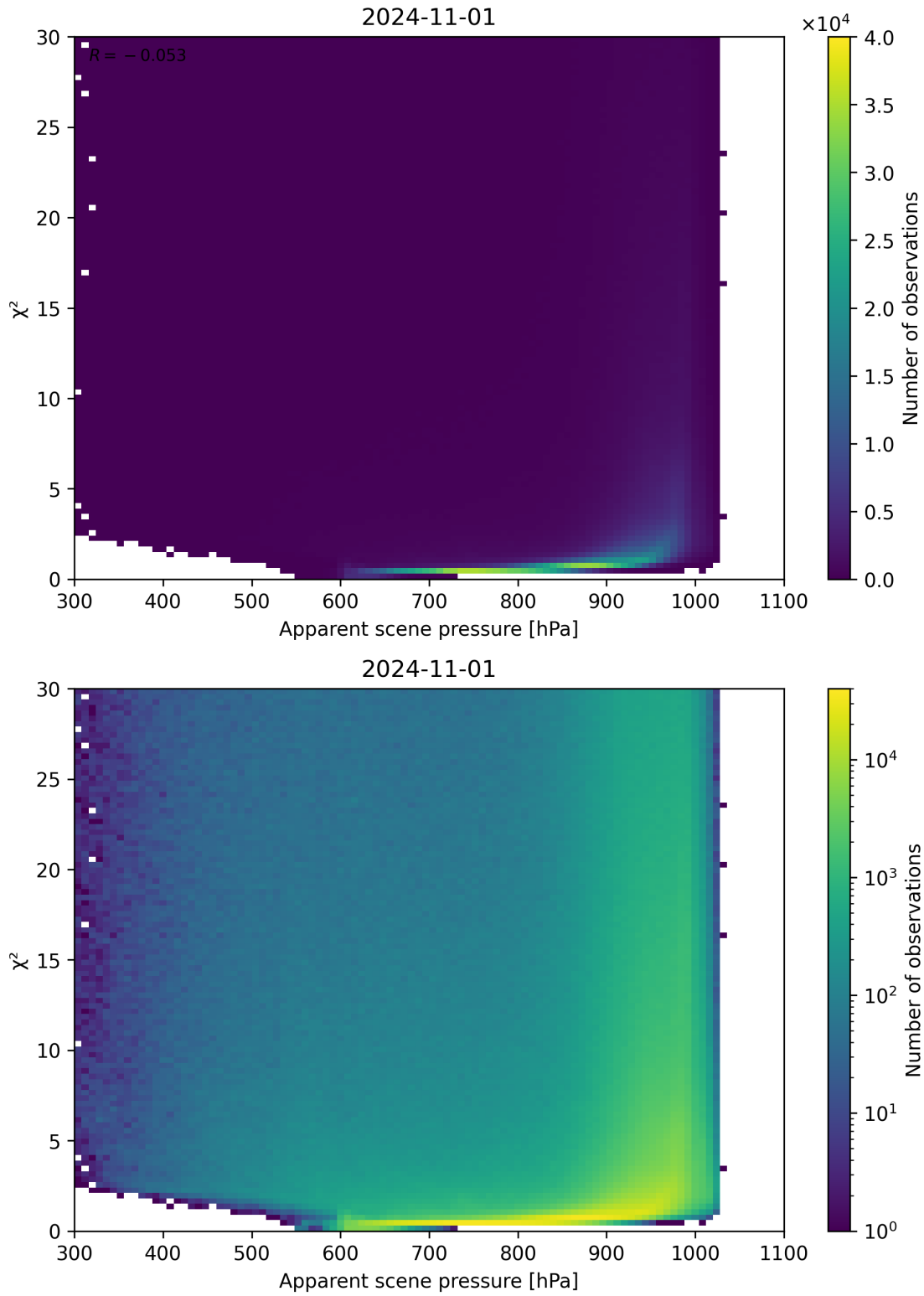
Figure 63: Scatter density plot of “Apparent scene pressure” against “ \chi^2 ” for 2024-10-31 to 2024-11-02.
