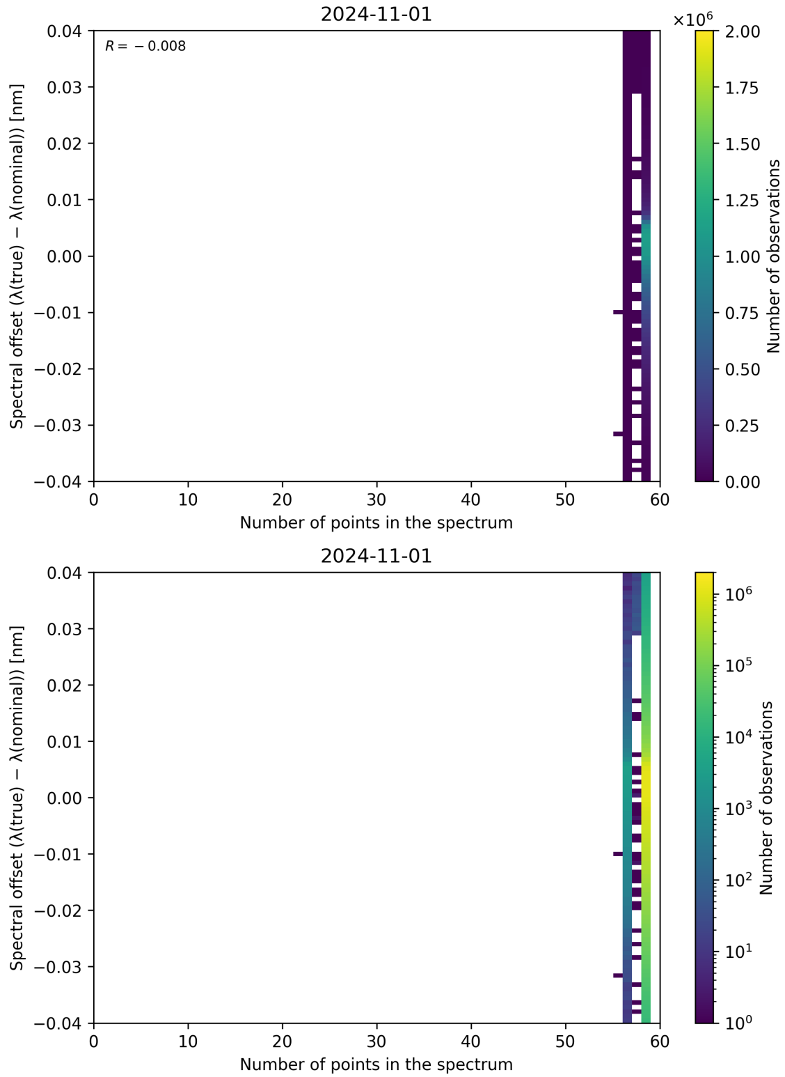
Figure 110: Scatter density plot of “Number of points in the spectrum” against “Spectral offset ( \lambda_{\text{true}} - \lambda_{\text{nominal}} )” for 2024-10-31 to 2024-11-02.
