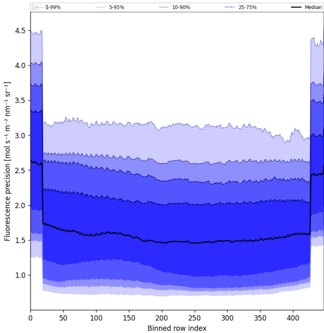
Figure 58: Along track statistics of “Fluorescence precision” for 2024-10-31 to 2024-11-02
