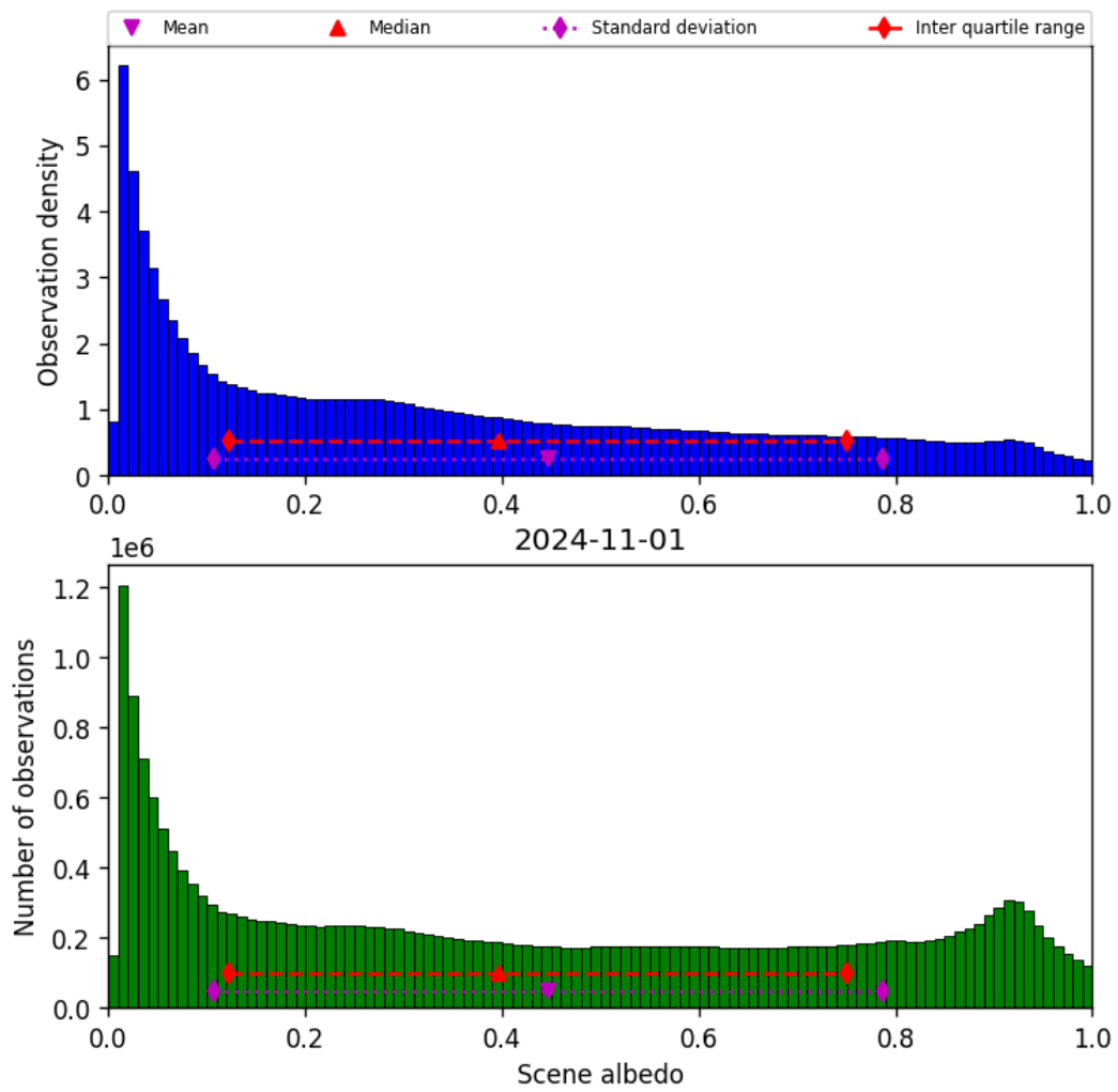
Figure 34: Histogram of “Scene albedo” for 2024-10-31 to 2024-11-02
