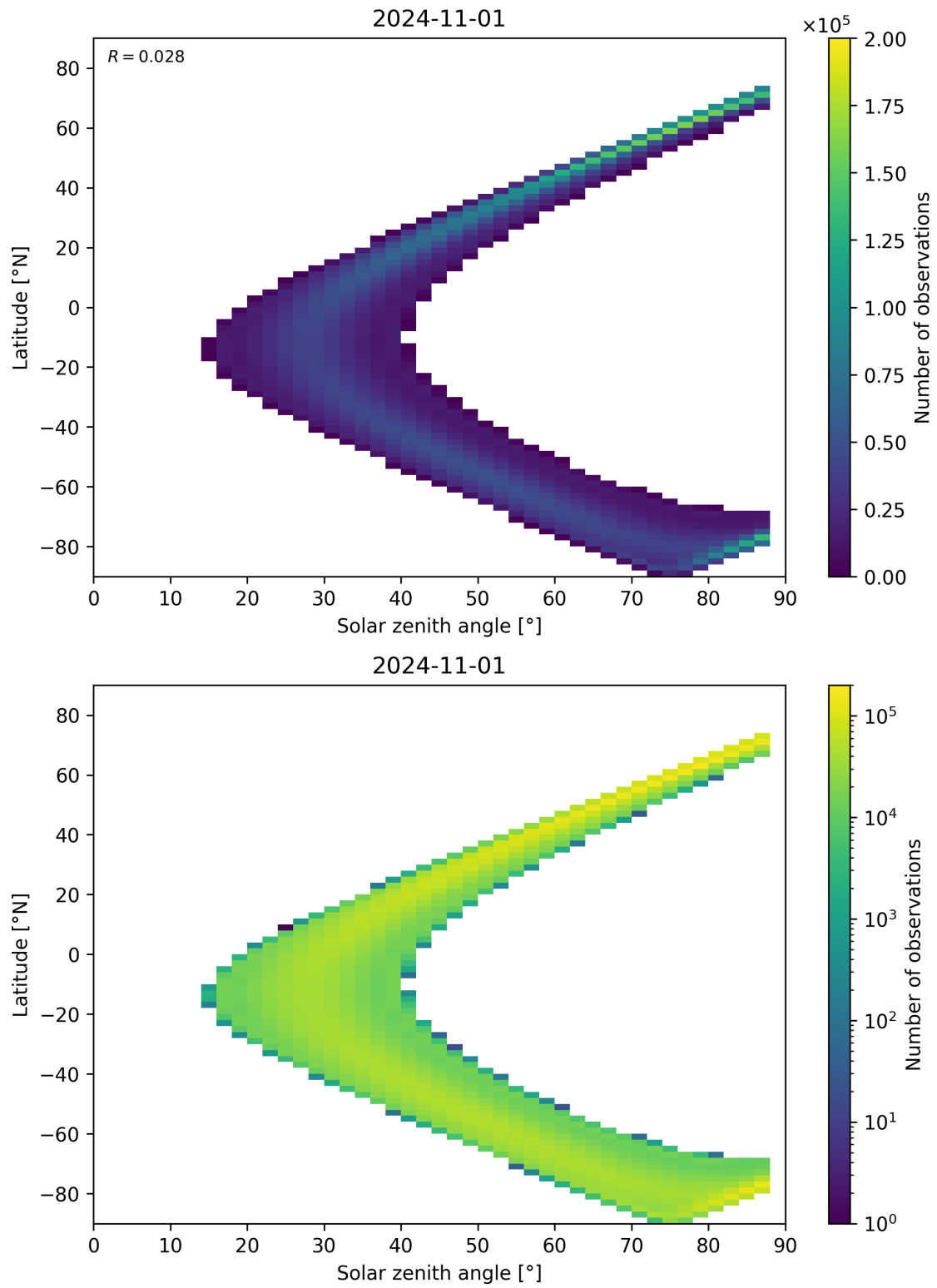
Figure 124: Scatter density plot of “Solar zenith angle” against “Latitude” for 2024-10-31 to 2024-11-02.
