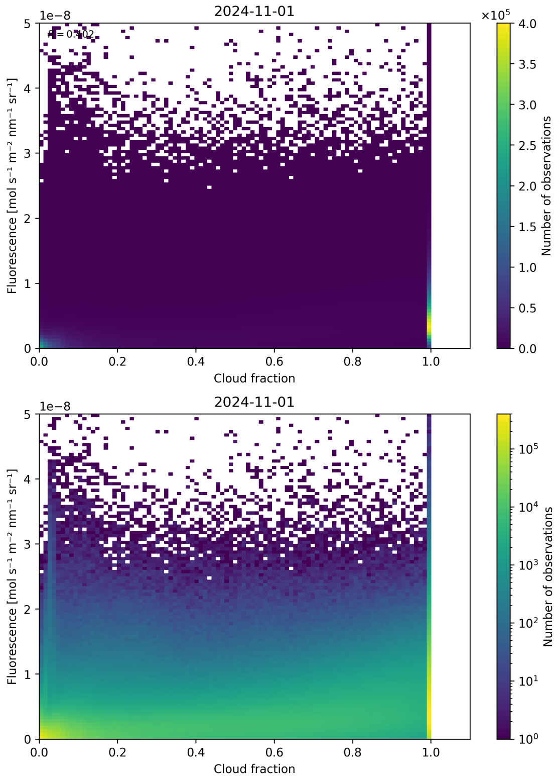
Figure 79: Scatter density plot of “Cloud fraction” against “Fluorescence” for 2024-10-31 to 2024-11-02.
