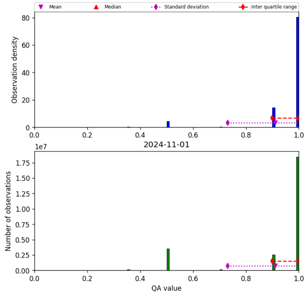
Figure 29: Histogram of “QA value” for 2024-10-31 to 2024-11-02
