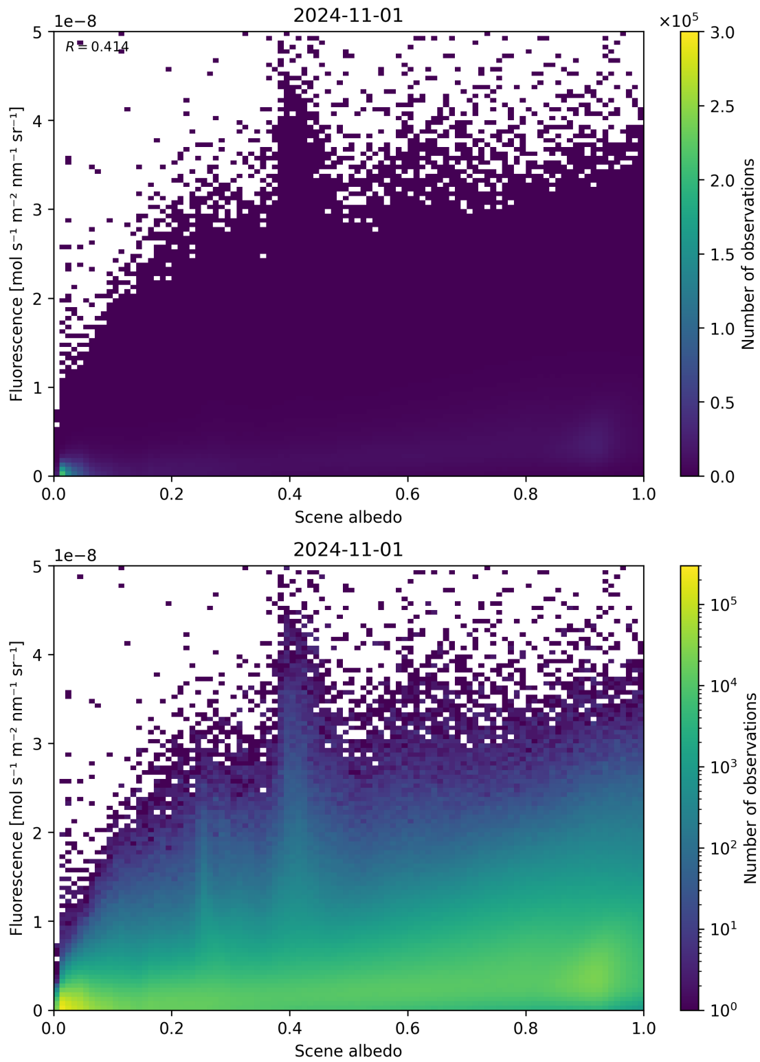
Figure 114: Scatter density plot of “Scene albedo” against “Fluorescence” for 2024-10-31 to 2024-11-02.
