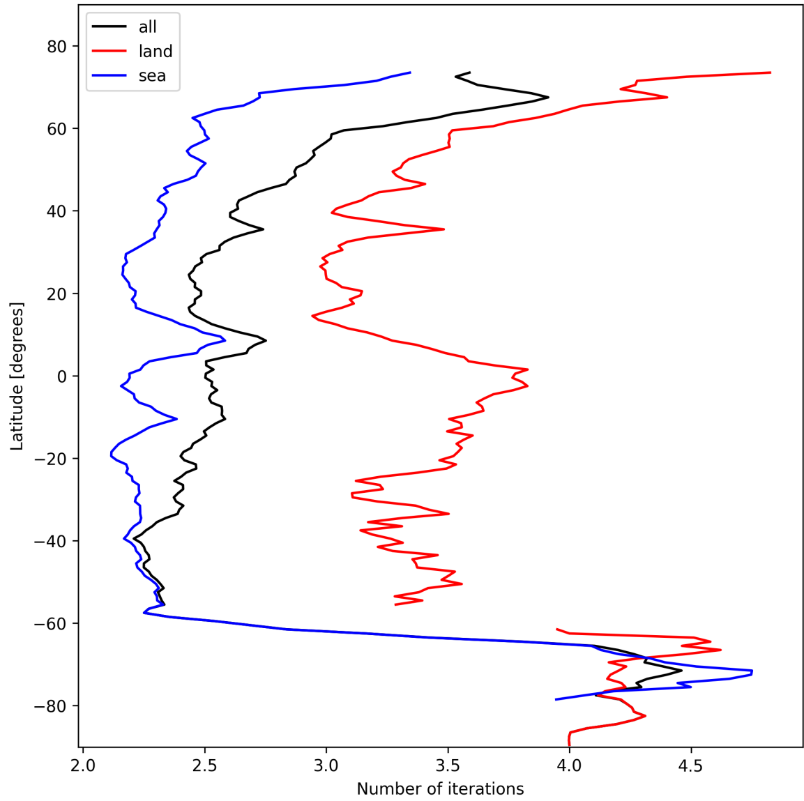
Figure 22: Zonal average of “Number of iterations” for 2024-10-31 to 2024-11-02.
