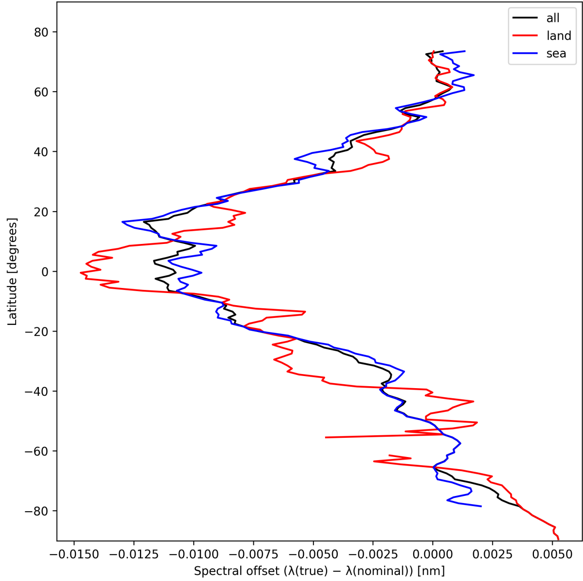
Figure 28: Zonal average of “Spectral offset ( \lambda_{\text{true}} - \lambda_{\text{nominal}} )” for 2024-10-31 to 2024-11-02.
