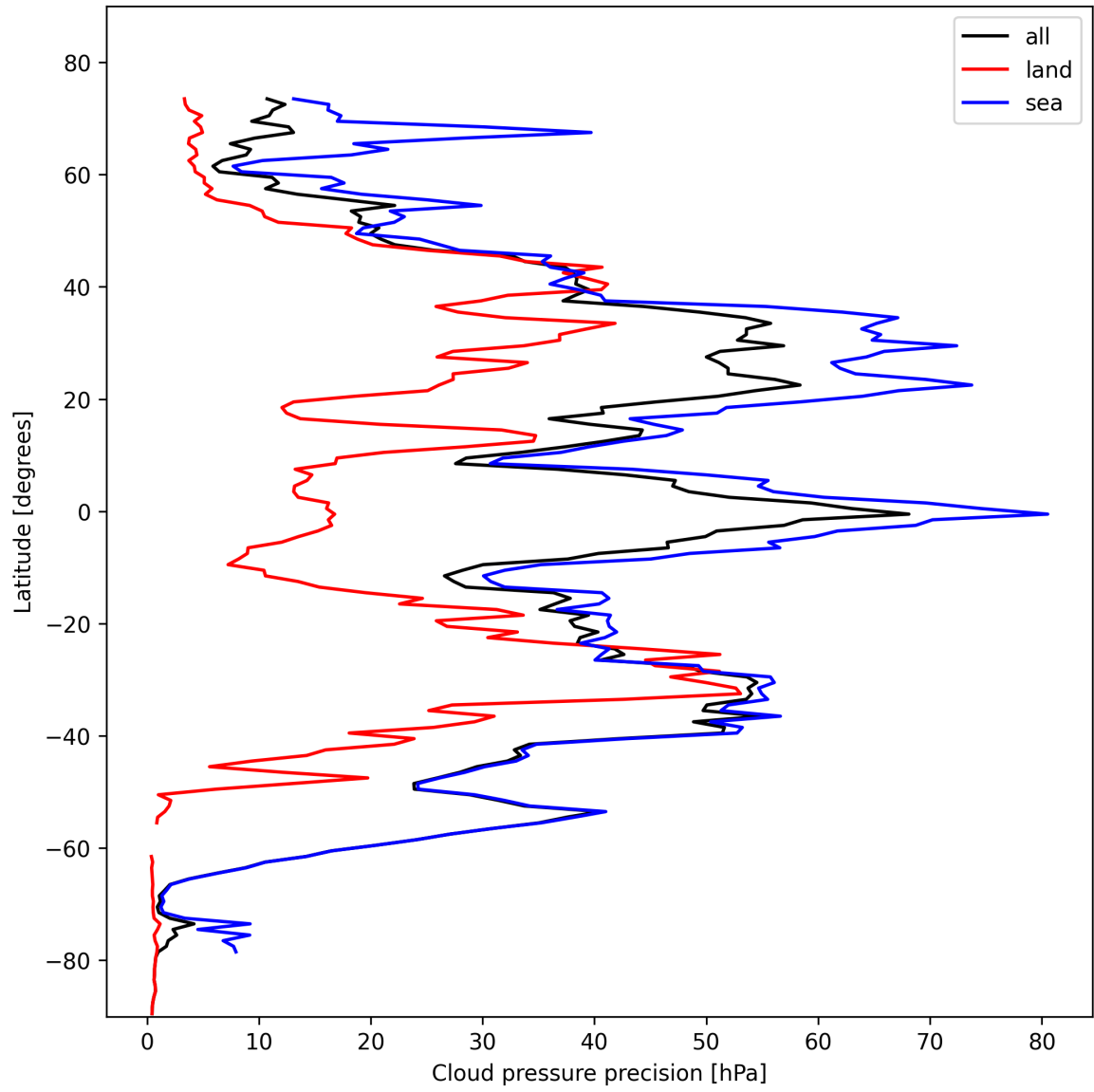
Figure 14: Zonal average of “Cloud pressure precision” for 2024-10-31 to 2024-11-02.
