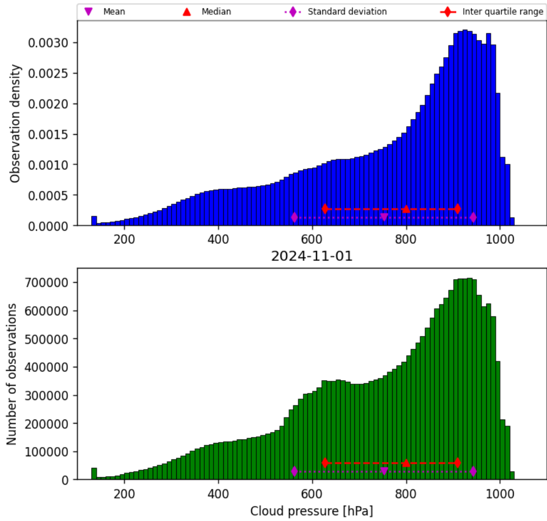
Figure 30: Histogram of “Cloud pressure” for 2024-10-31 to 2024-11-02
