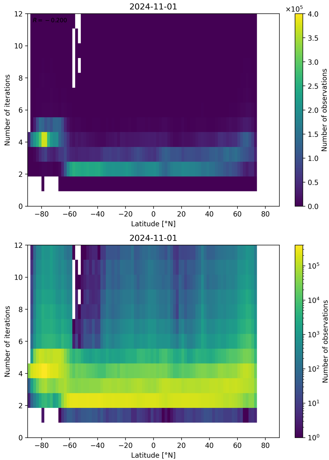
Figure 102: Scatter density plot of “Latitude” against “Number of iterations” for 2024-10-31 to 2024-11-02.
