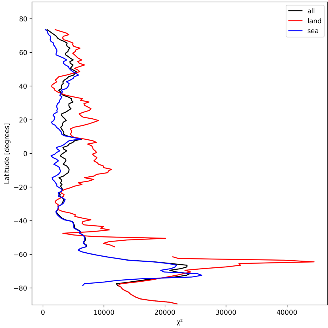
Figure 21: Zonal average of “ \chi^2 ” for 2024-10-31 to 2024-11-02.
