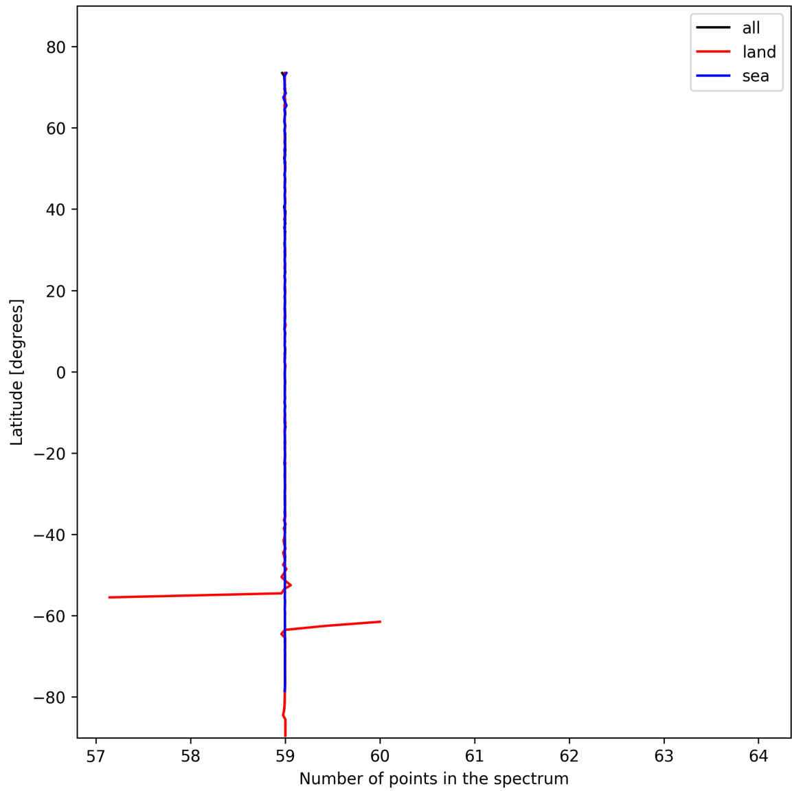
Figure 27: Zonal average of “Number of points in the spectrum” for 2024-10-31 to 2024-11-02.
