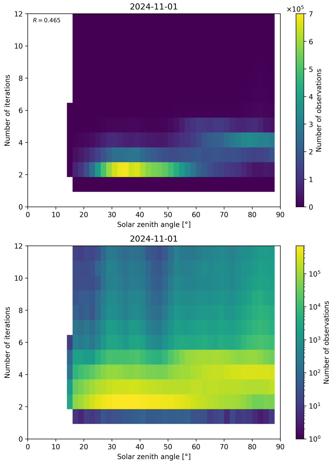
Figure 125: Scatter density plot of “Solar zenith angle” against “Number of iterations” for 2024-10-31 to 2024-11-02.
