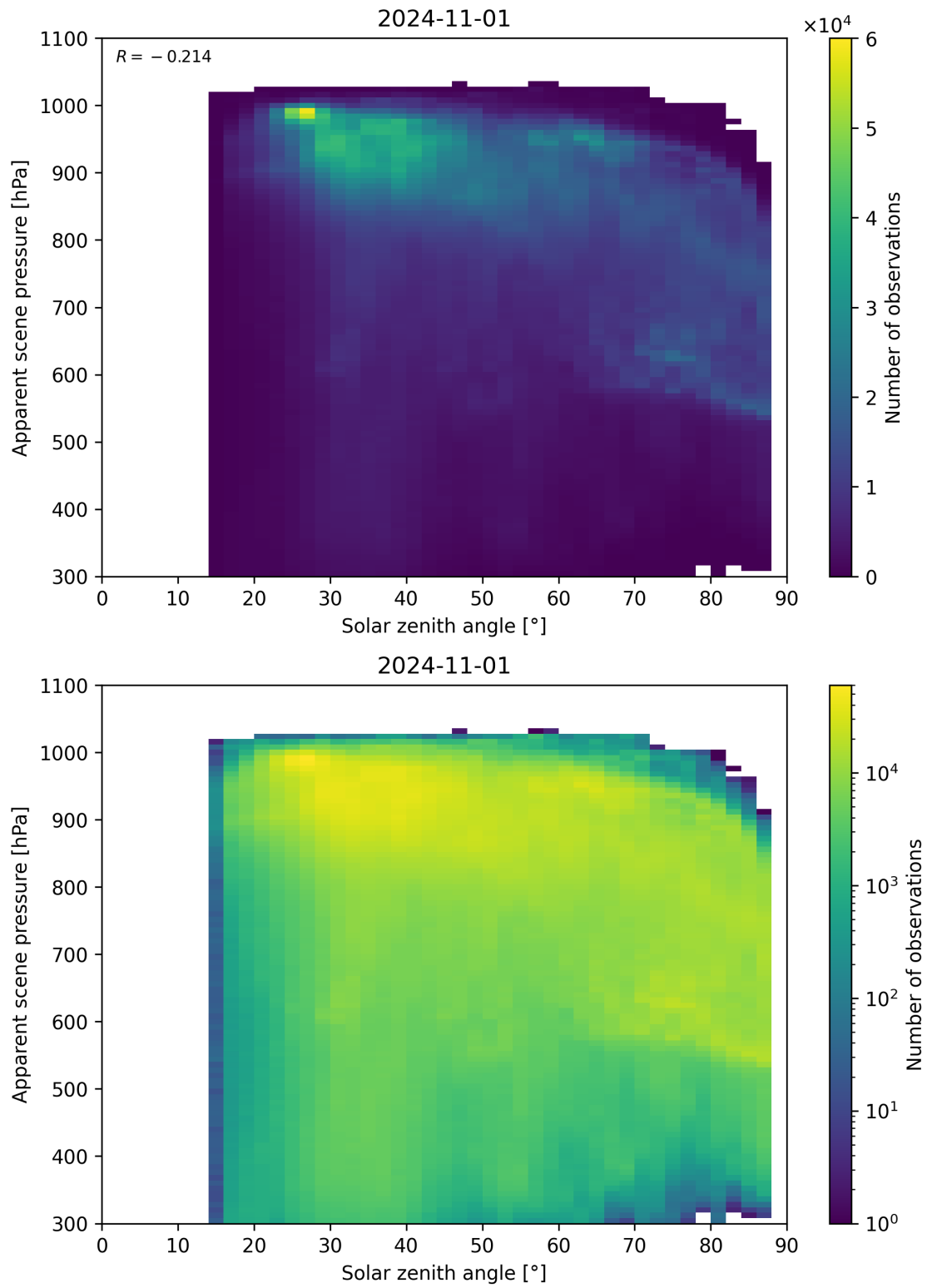
Figure 118: Scatter density plot of “Solar zenith angle” against “Apparent scene pressure” for 2024-10-31 to 2024-11-02.
