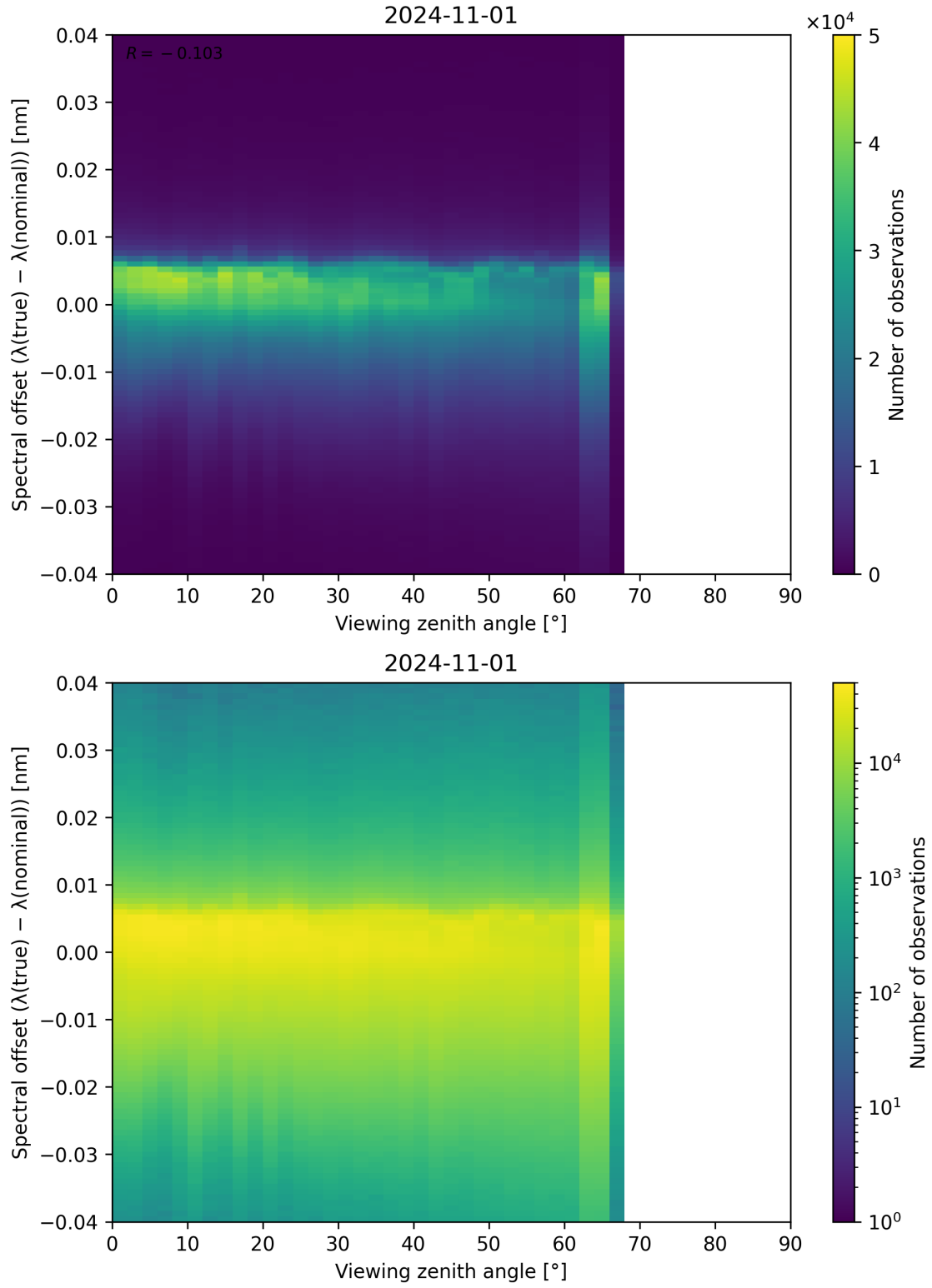
Figure 140: Scatter density plot of “Viewing zenith angle” against “Spectral offset ( \lambda_{\text{true}} - \lambda_{\text{nominal}} )” for 2024-10-31 to 2024-11-02.
