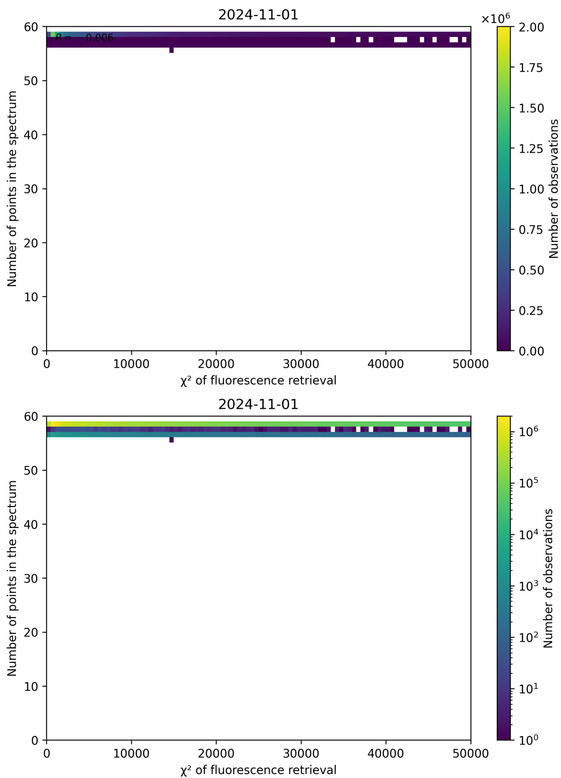
Figure 71: Scatter density plot of " \chi^2 of fluorescence retrieval" against "Number of points in the spectrum" for 2024-10-31 to 2024-11-02.
