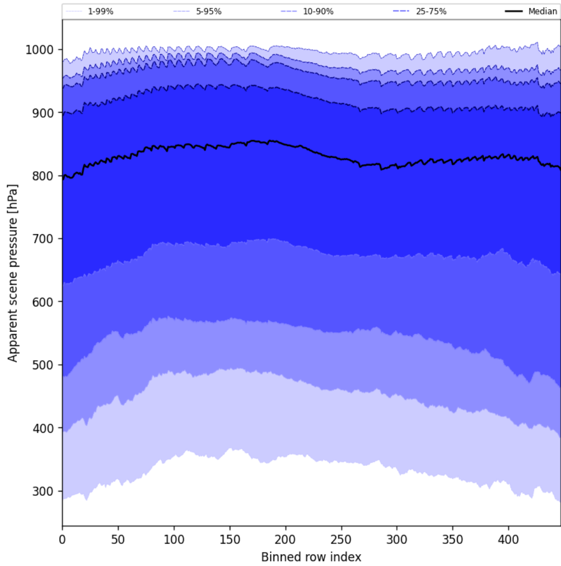
Figure 53: Along track statistics of “Apparent scene pressure” for 2024-10-31 to 2024-11-02
