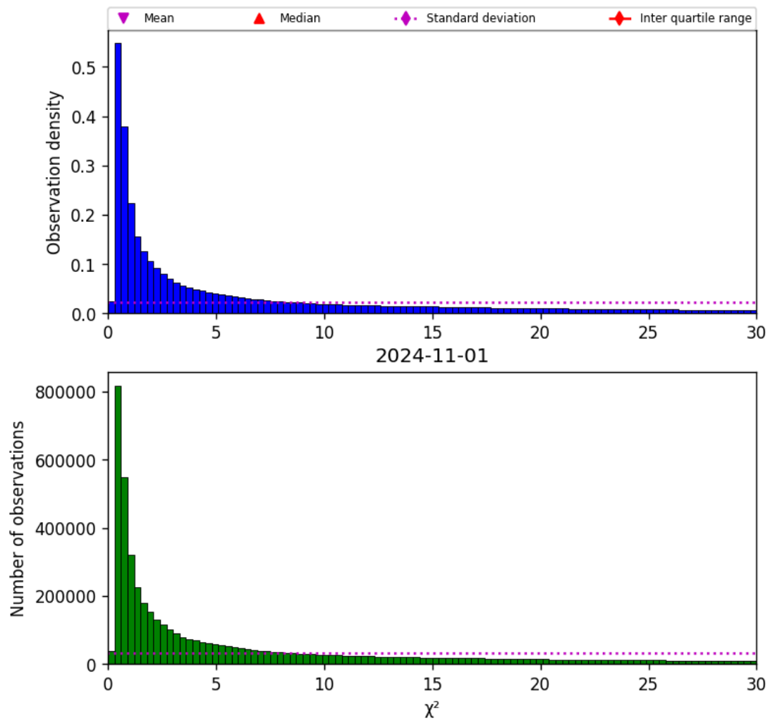
Figure 38: Histogram of “ \chi^2 ” for 2024-10-31 to 2024-11-02
