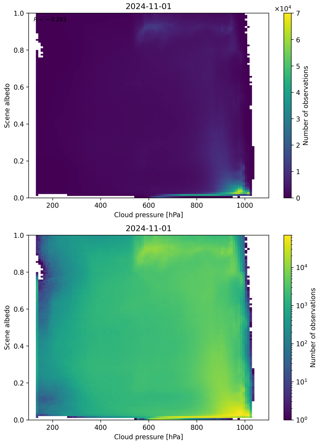
Figure 91: Scatter density plot of “Cloud pressure” against “Scene albedo” for 2024-10-31 to 2024-11-02.
