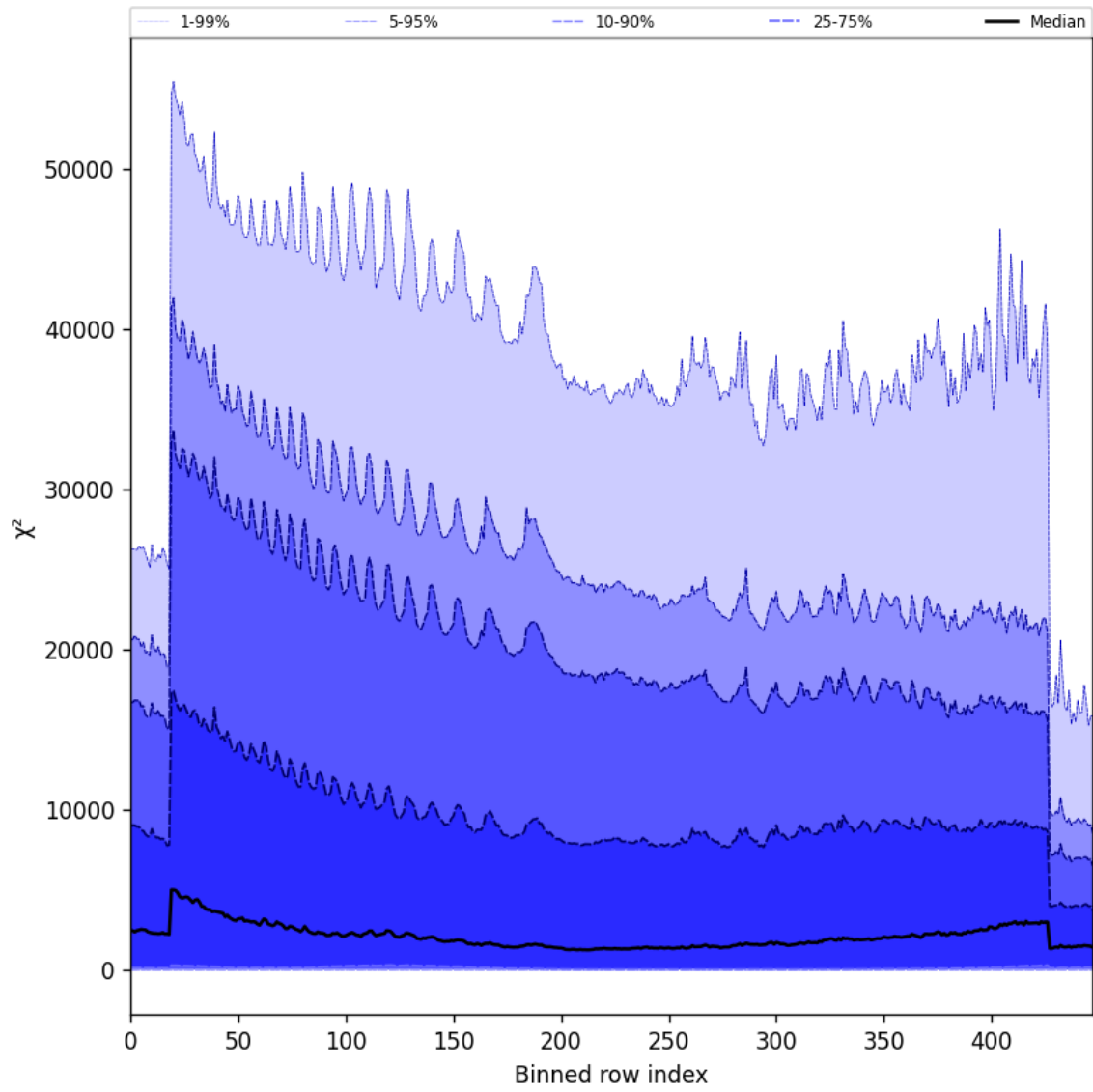
Figure 55: Along track statistics of “ \chi^2 ” for 2024-10-31 to 2024-11-02
