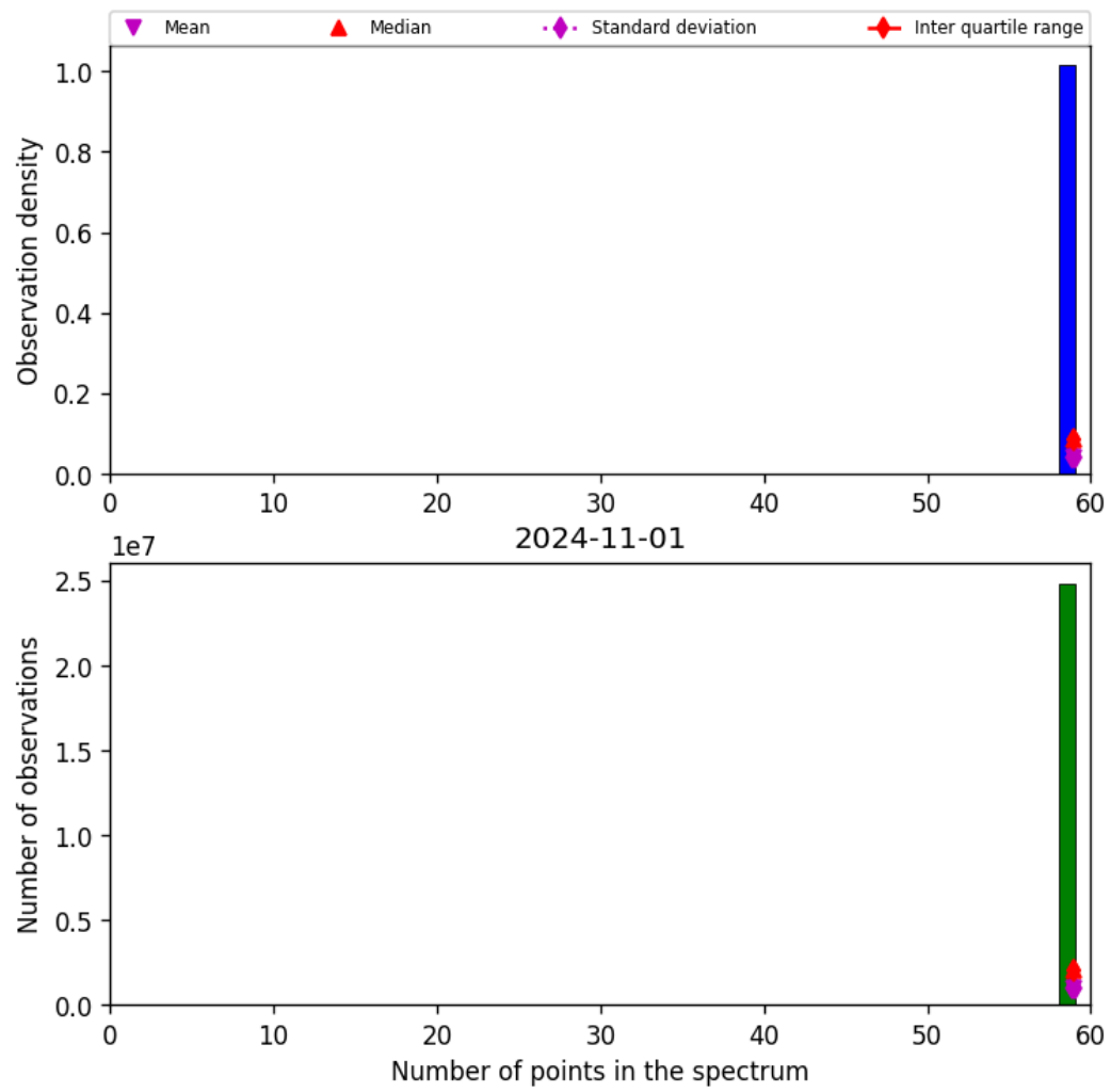
Figure 44: Histogram of “Number of points in the spectrum” for 2024-10-31 to 2024-11-02
