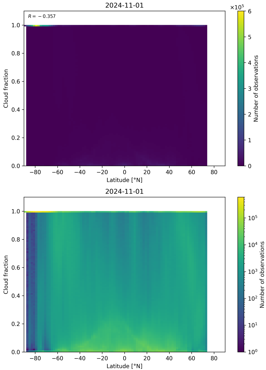
Figure 99: Scatter density plot of “Latitude” against “Cloud fraction” for 2024-10-31 to 2024-11-02.
