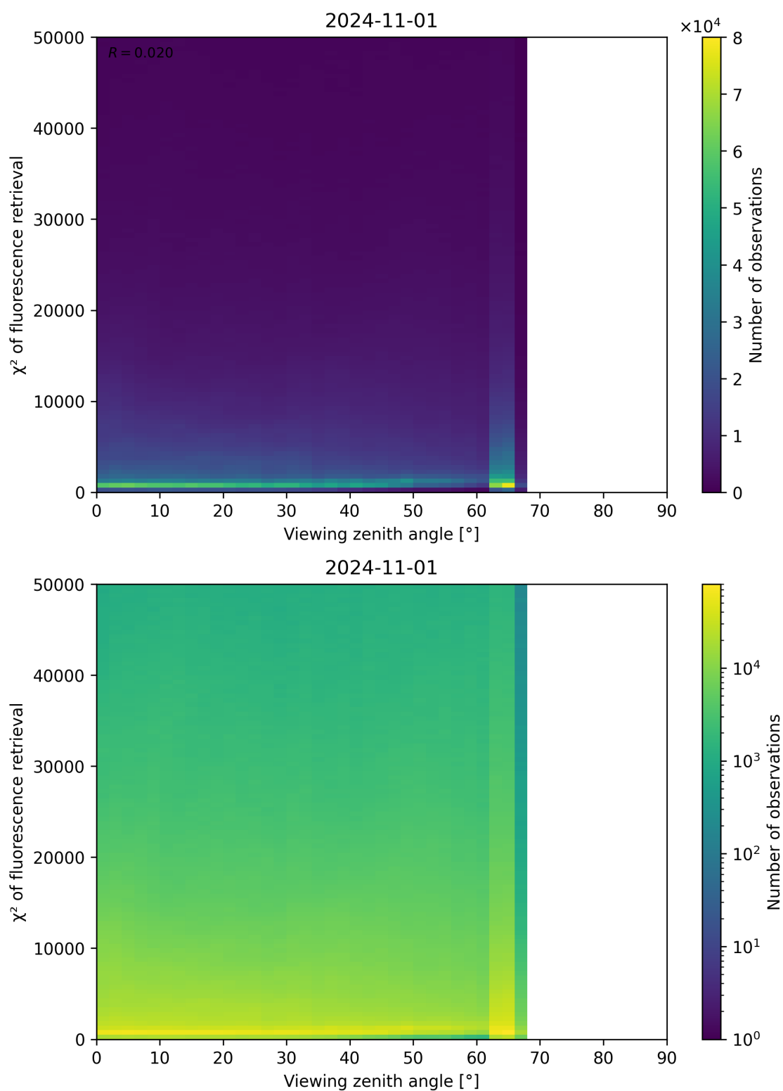
Figure 131: Scatter density plot of “Viewing zenith angle” against “ \chi^2 of fluorescence retrieval” for 2024-10-31 to 2024-11-02.
