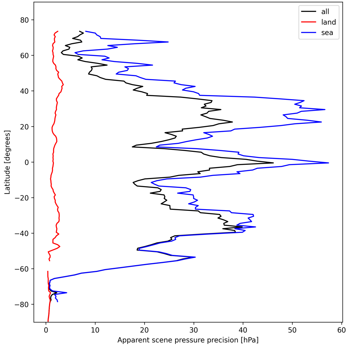
Figure 20: Zonal average of “Apparent scene pressure precision” for 2024-10-31 to 2024-11-02.
