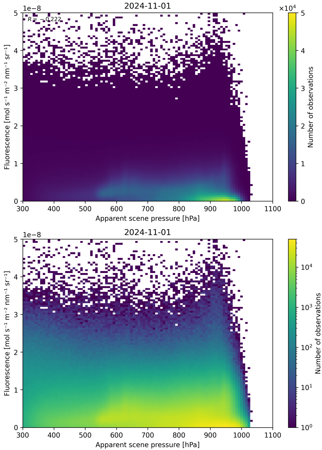
Figure 65: Scatter density plot of “Apparent scene pressure” against “Fluorescence” for 2024-10-31 to 2024-11-02.
