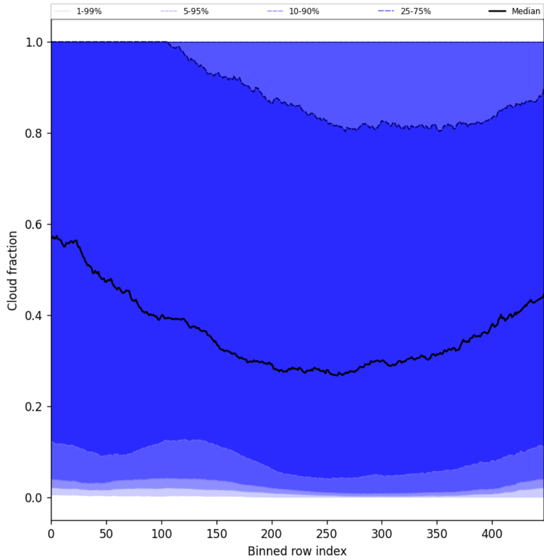
Figure 49: Along track statistics of “Cloud fraction” for 2024-10-31 to 2024-11-02
