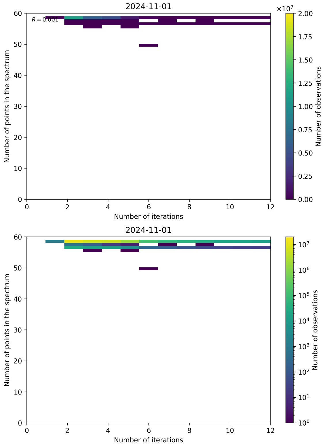
Figure 108: Scatter density plot of “Number of iterations” against “Number of points in the spectrum” for 2024-10-31 to 2024-11-02.
