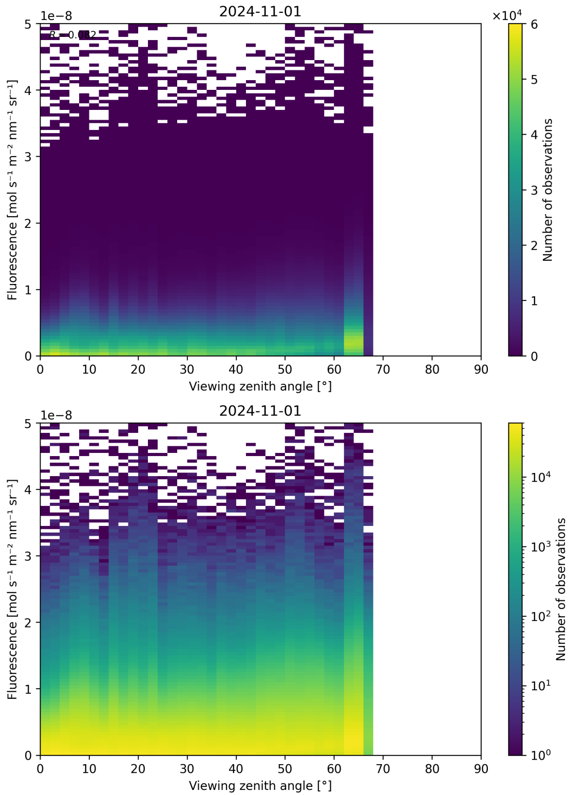
Figure 134: Scatter density plot of “Viewing zenith angle” against “Fluorescence” for 2024-10-31 to 2024-11-02.
