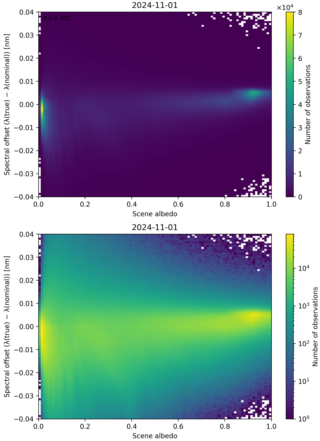
Figure 117: Scatter density plot of “Scene albedo” against “Spectral offset ( \lambda_{\text{true}} - \lambda_{\text{nominal}} )” for 2024-10-31 to 2024-11-02.
