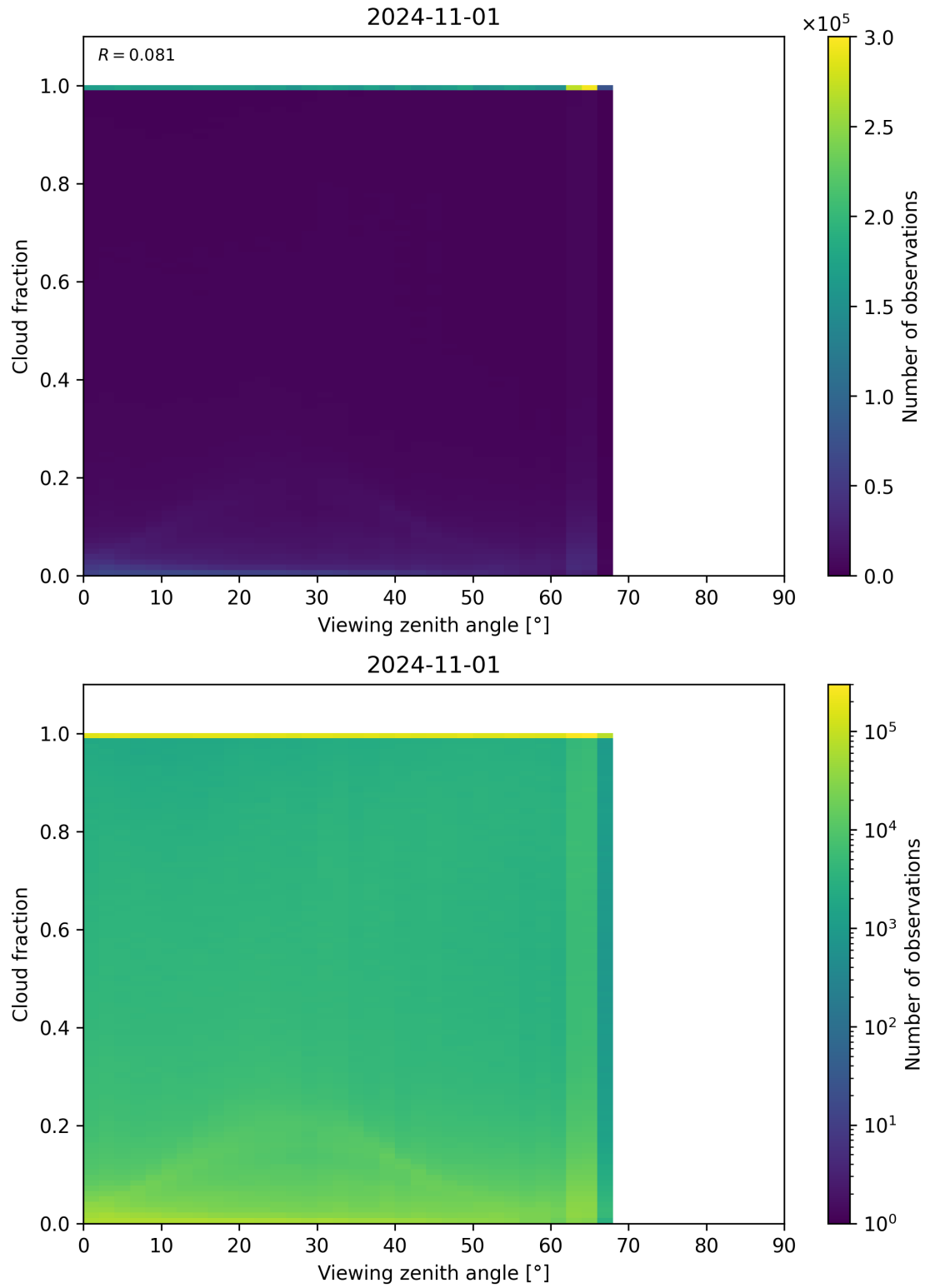
Figure 132: Scatter density plot of “Viewing zenith angle” against “Cloud fraction” for 2024-10-31 to 2024-11-02.
