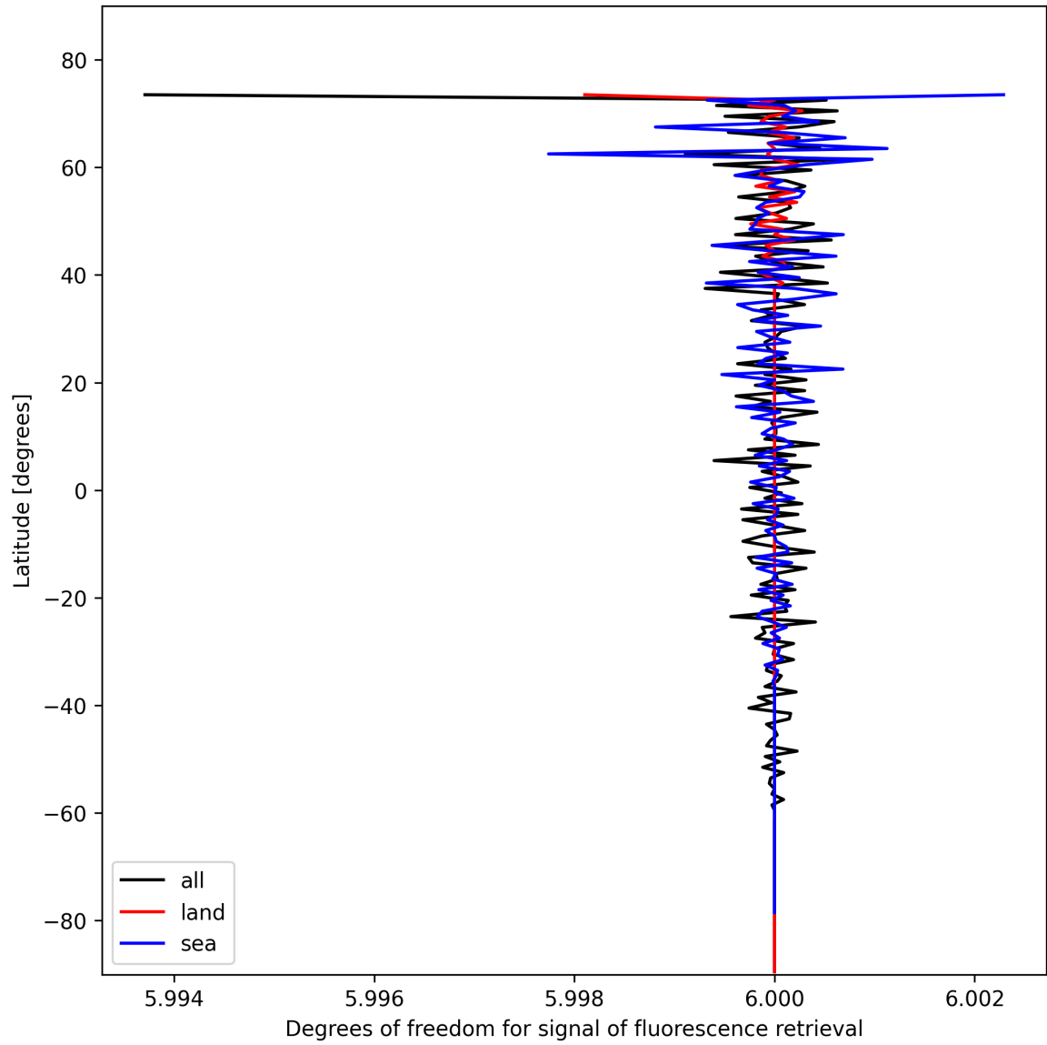
Figure 26: Zonal average of “Degrees of freedom for signal of fluorescence retrieval” for 2024-10-31 to 2024-11-02.
