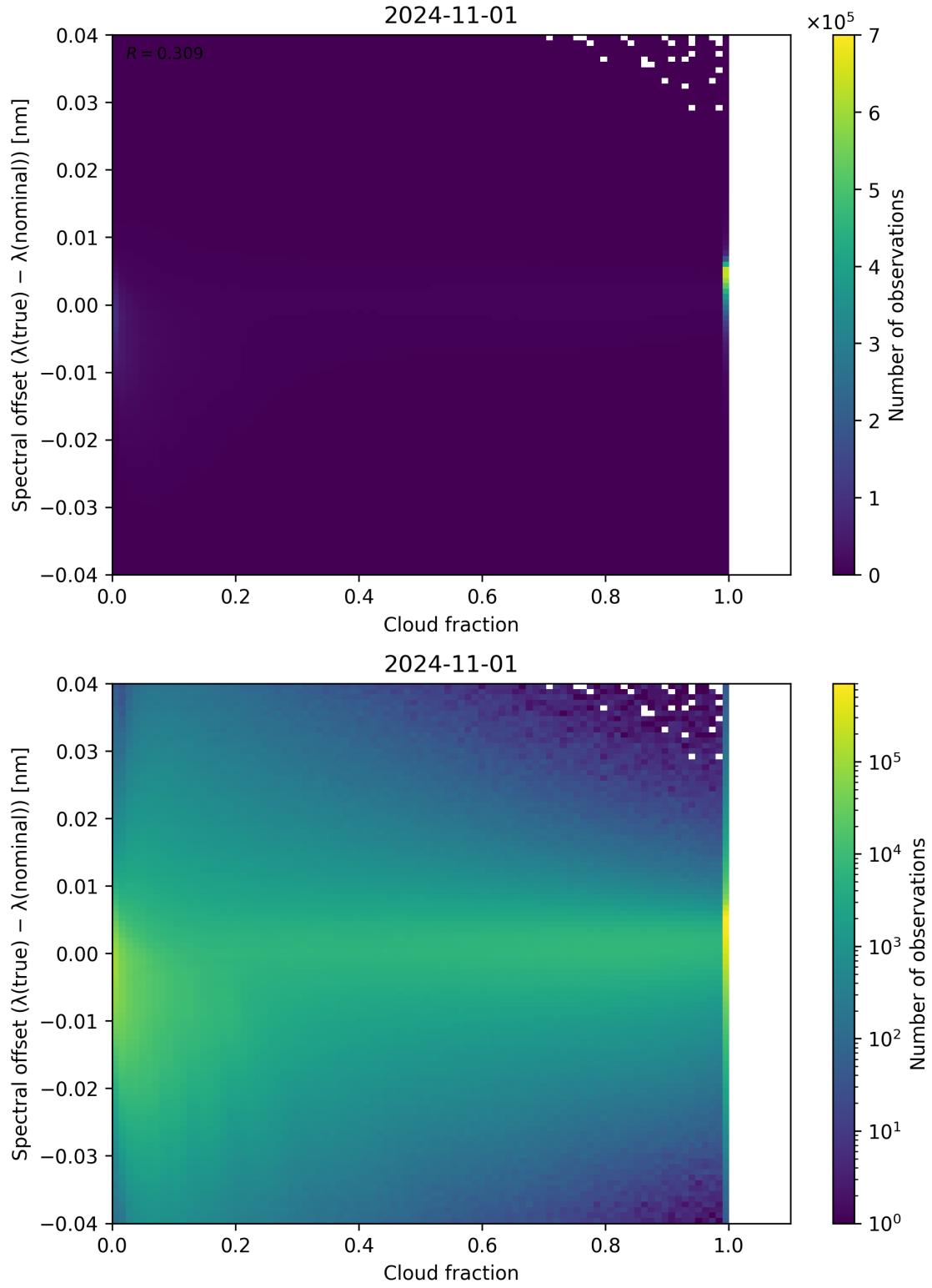
Figure 83: Scatter density plot of “Cloud fraction” against “Spectral offset ( \lambda_{\text{true}} - \lambda_{\text{nominal}} )” for 2024-10-31 to 2024-11-02.
