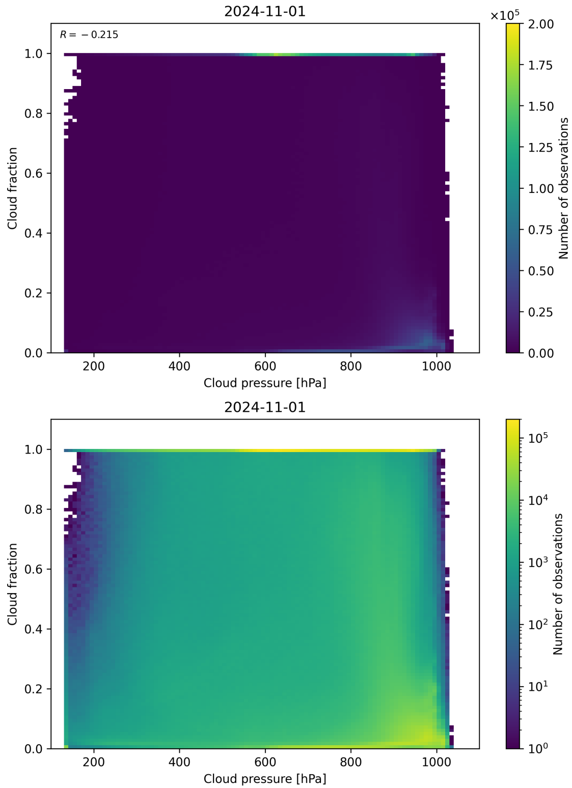
Figure 87: Scatter density plot of “Cloud pressure” against “Cloud fraction” for 2024-10-31 to 2024-11-02.
