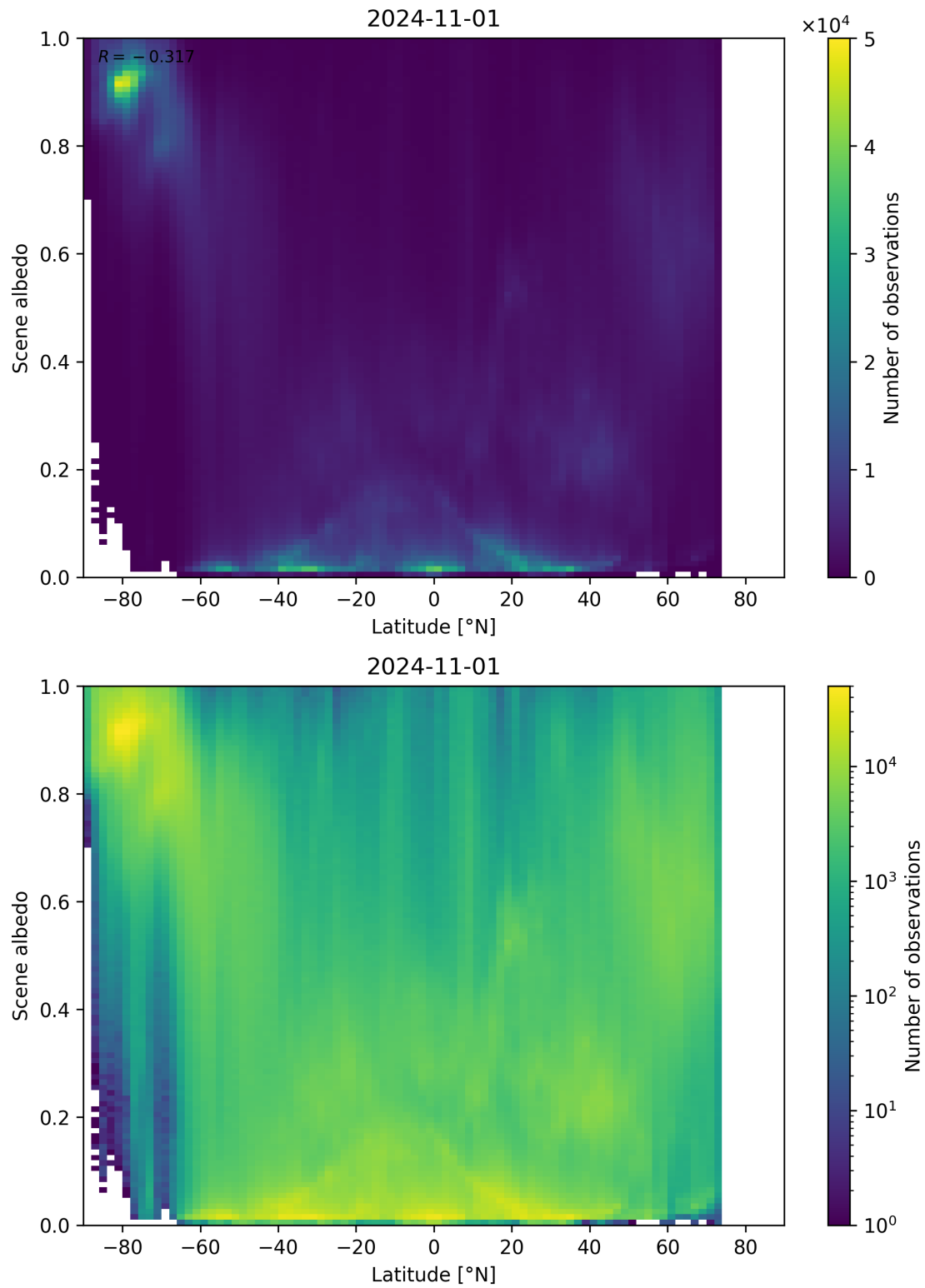
Figure 104: Scatter density plot of “Latitude” against “Scene albedo” for 2024-10-31 to 2024-11-02.
