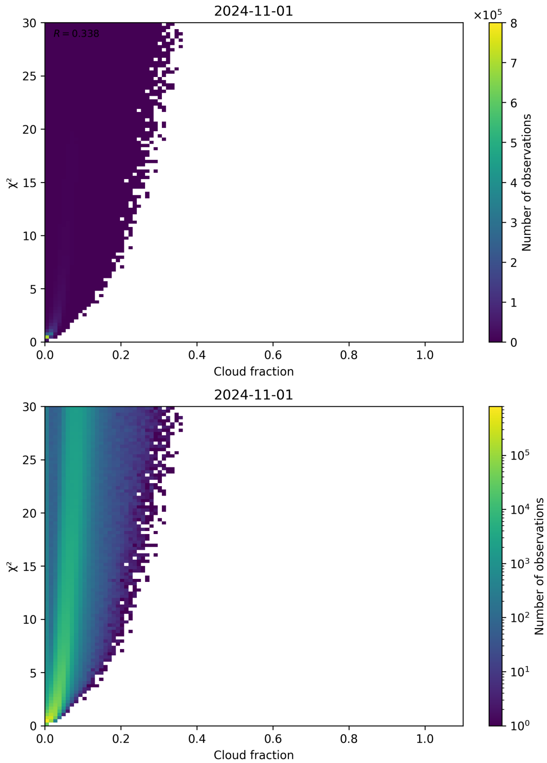
Figure 77: Scatter density plot of “Cloud fraction” against “ \chi^2 ” for 2024-10-31 to 2024-11-02.
