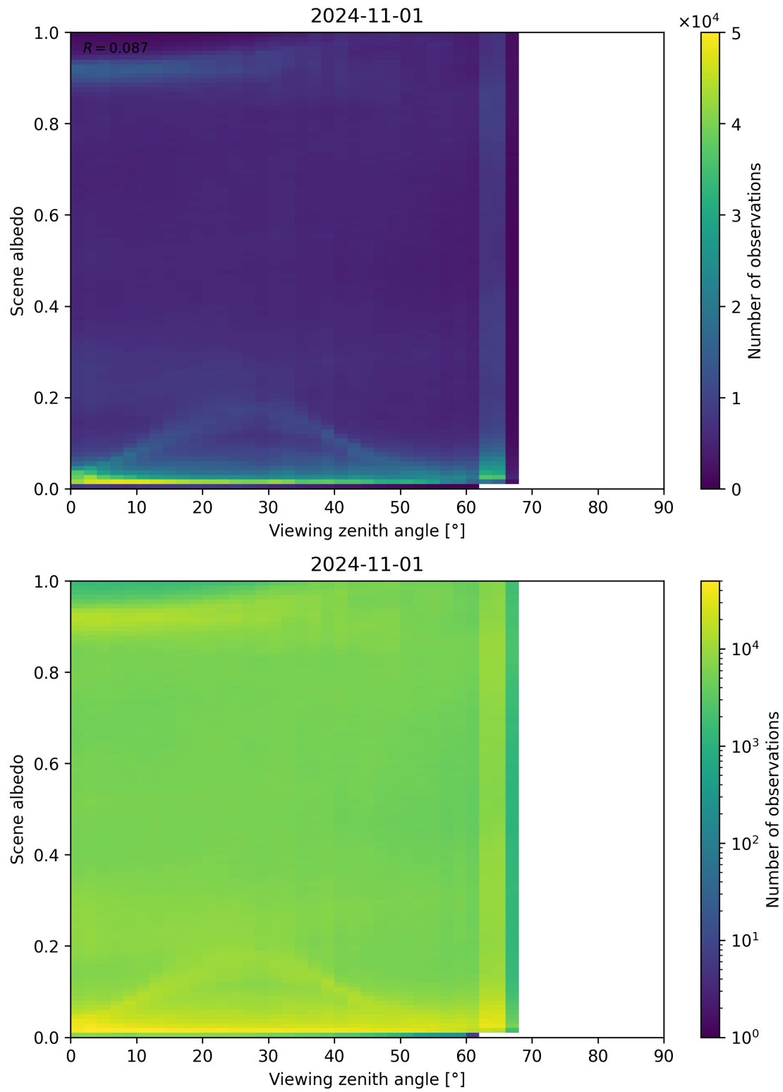
Figure 138: Scatter density plot of “Viewing zenith angle” against “Scene albedo” for 2024-10-31 to 2024-11-02.
