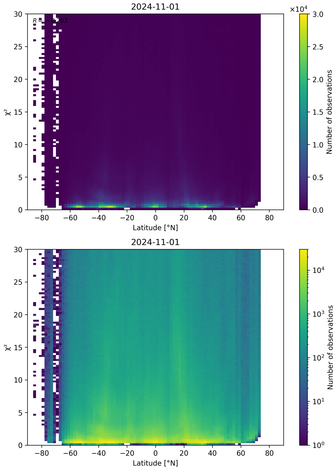
Figure 97: Scatter density plot of “Latitude” against “ \chi^2 ” for 2024-10-31 to 2024-11-02.
