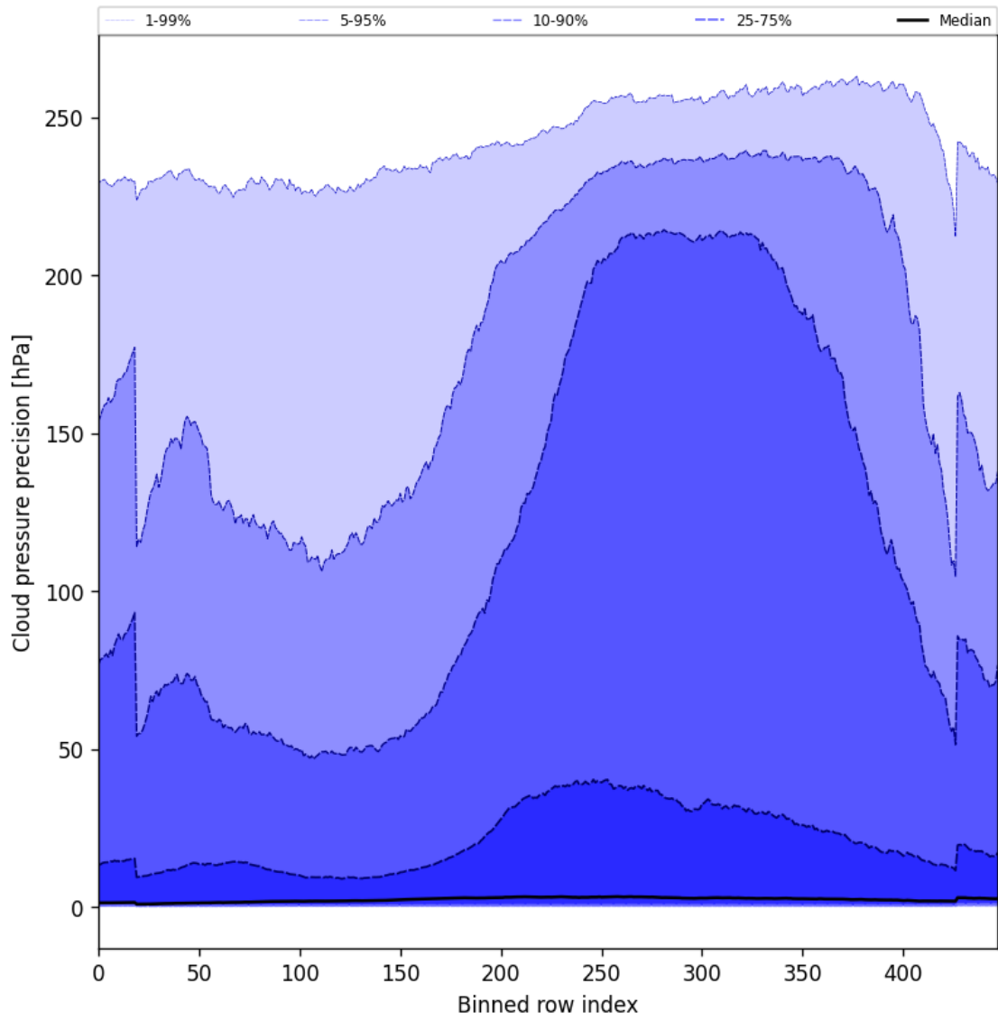
Figure 48: Along track statistics of “Cloud pressure precision” for 2024-10-31 to 2024-11-02
