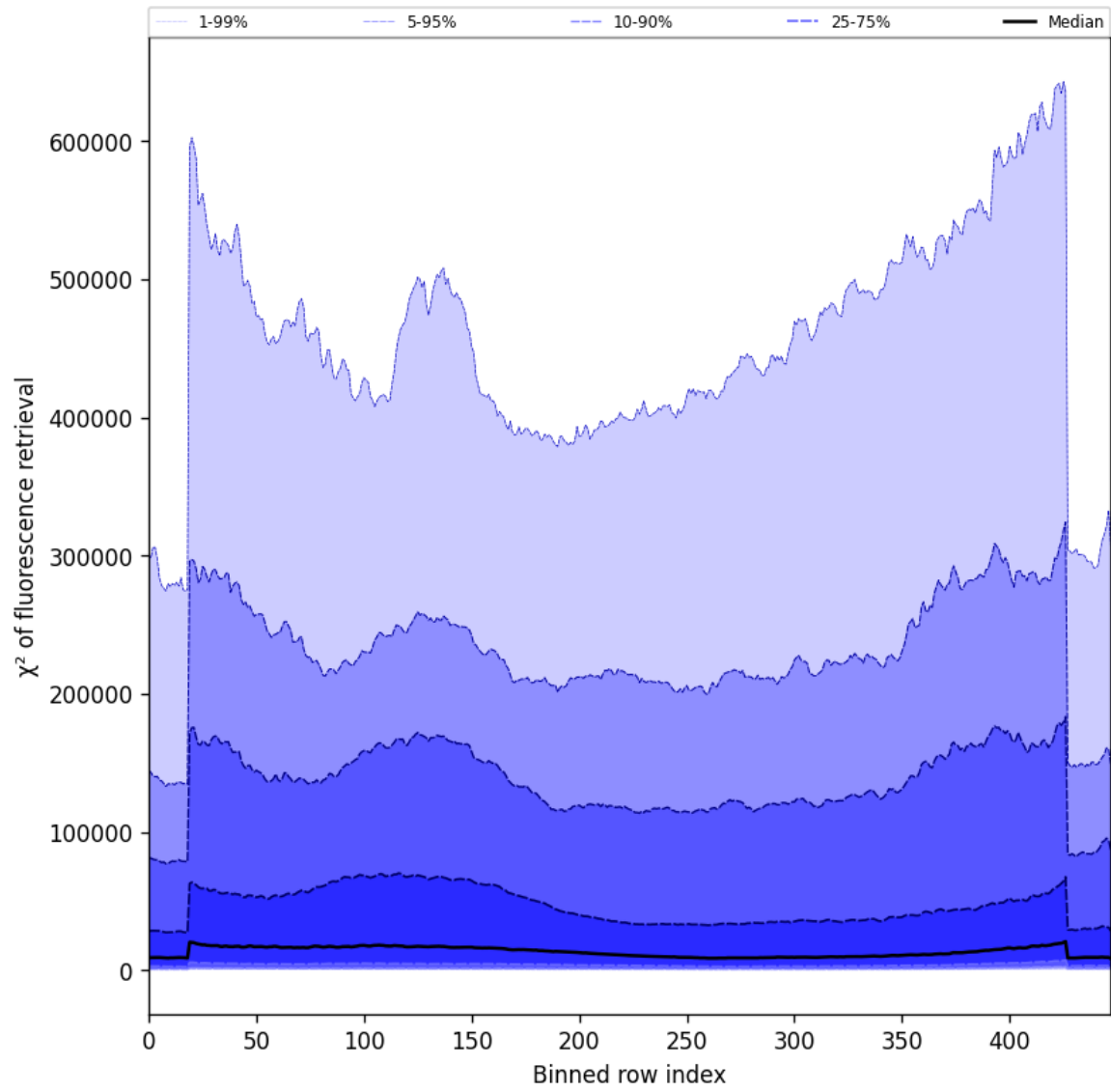
Figure 59: Along track statistics of “ \chi^2 of fluorescence retrieval” for 2024-10-31 to 2024-11-02
