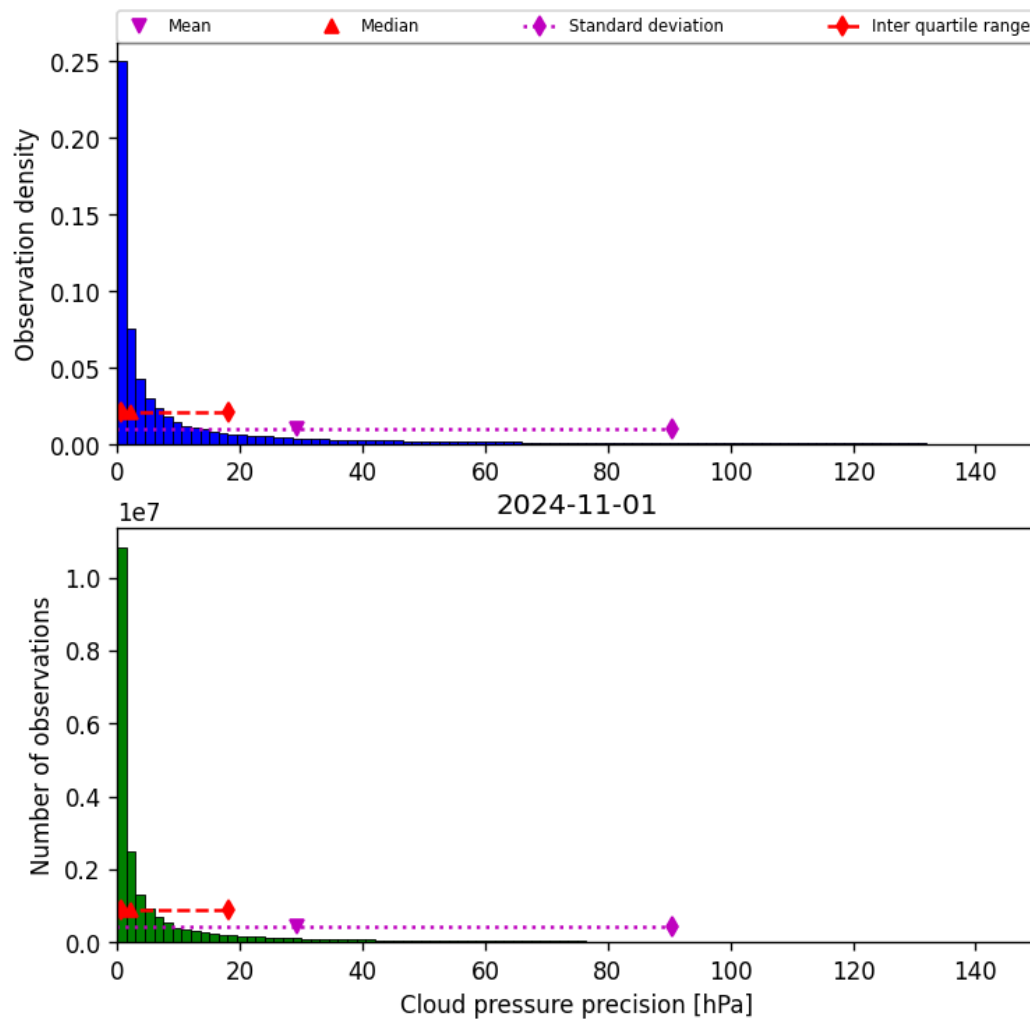
Figure 31: Histogram of “Cloud pressure precision” for 2024-10-31 to 2024-11-02
