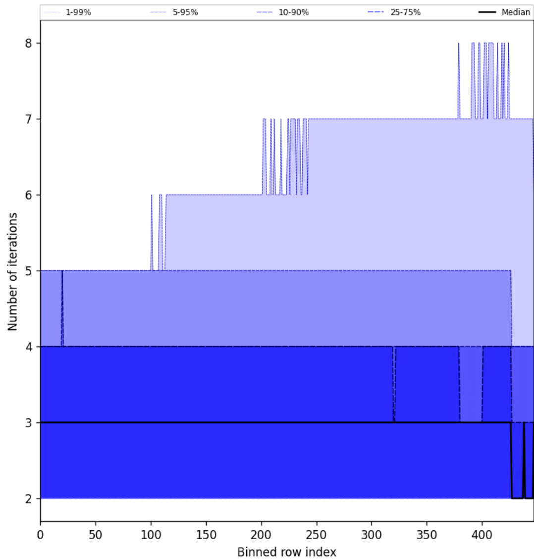
Figure 56: Along track statistics of “Number of iterations” for 2024-10-31 to 2024-11-02
