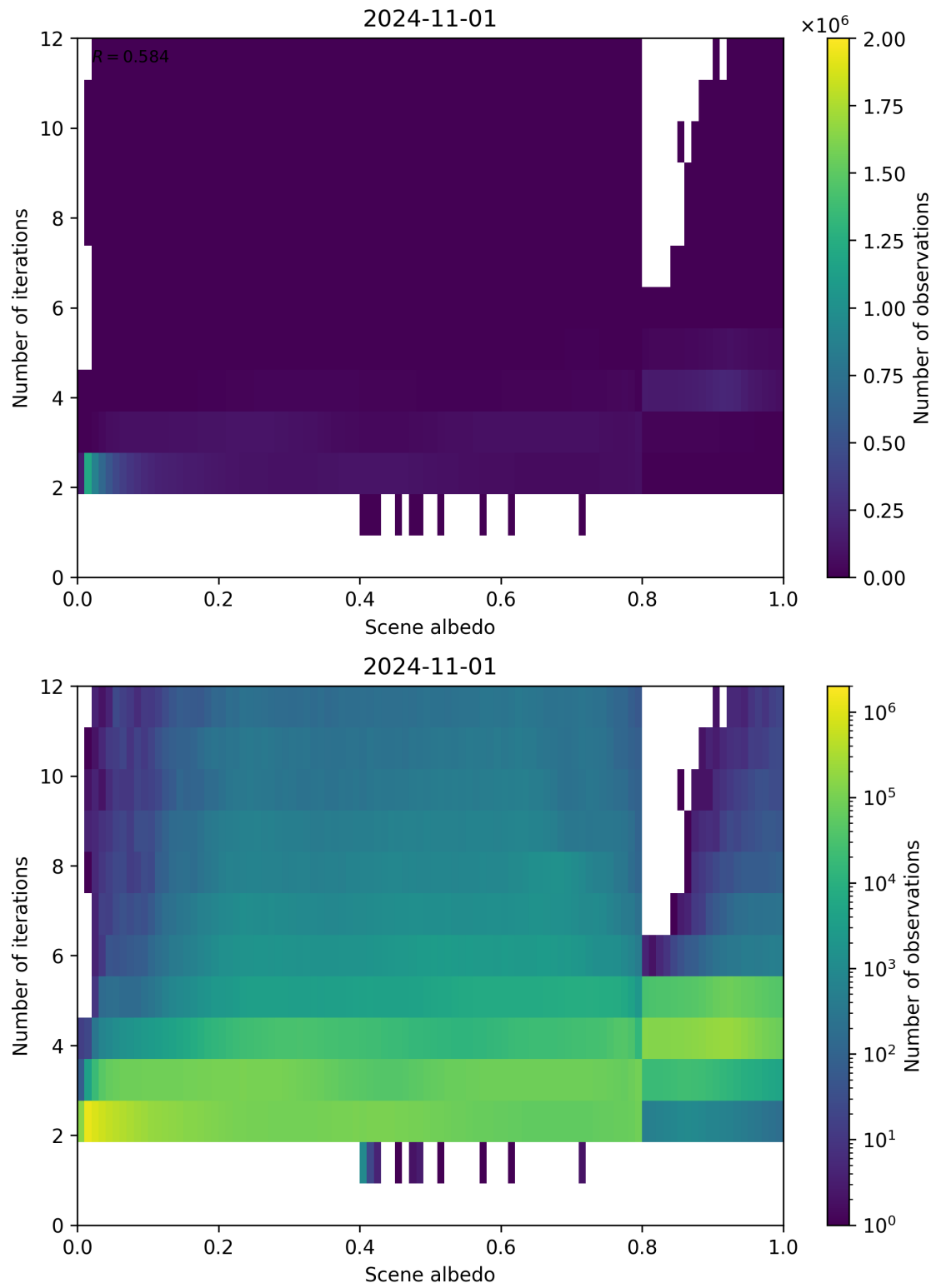
Figure 115: Scatter density plot of “Scene albedo” against “Number of iterations” for 2024-10-31 to 2024-11-02.
