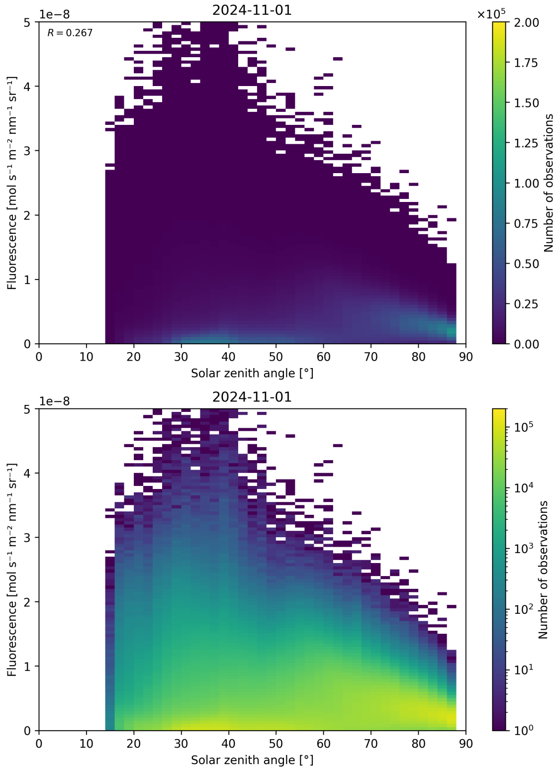
Figure 123: Scatter density plot of “Solar zenith angle” against “Fluorescence” for 2024-10-31 to 2024-11-02.
