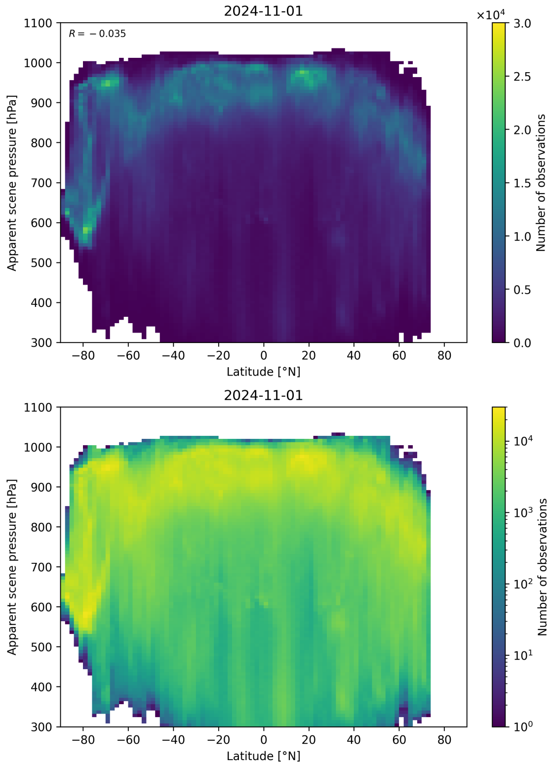
Figure 96: Scatter density plot of “Latitude” against “Apparent scene pressure” for 2024-10-31 to 2024-11-02.
