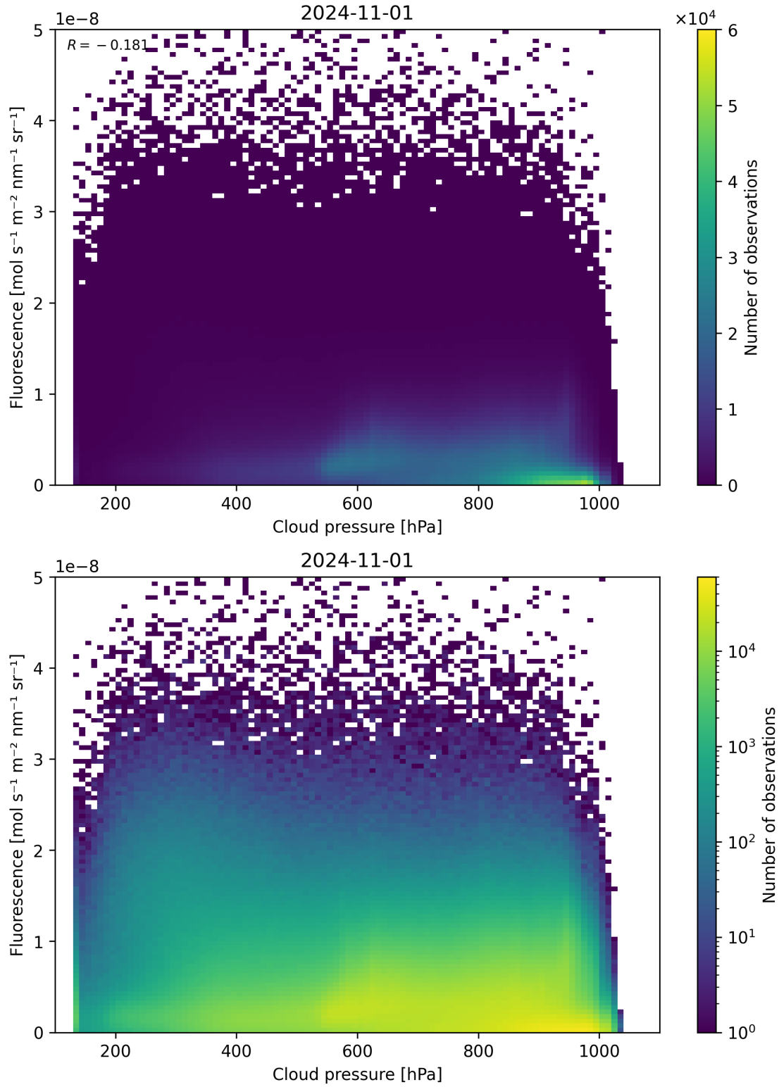
Figure 88: Scatter density plot of “Cloud pressure” against “Fluorescence” for 2024-10-31 to 2024-11-02.
