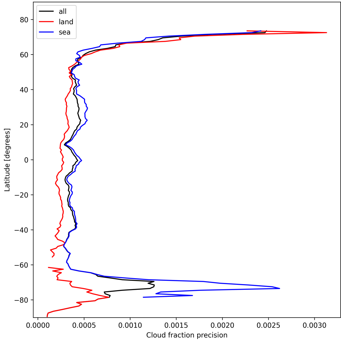
Figure 16: Zonal average of “Cloud fraction precision” for 2024-10-31 to 2024-11-02.
