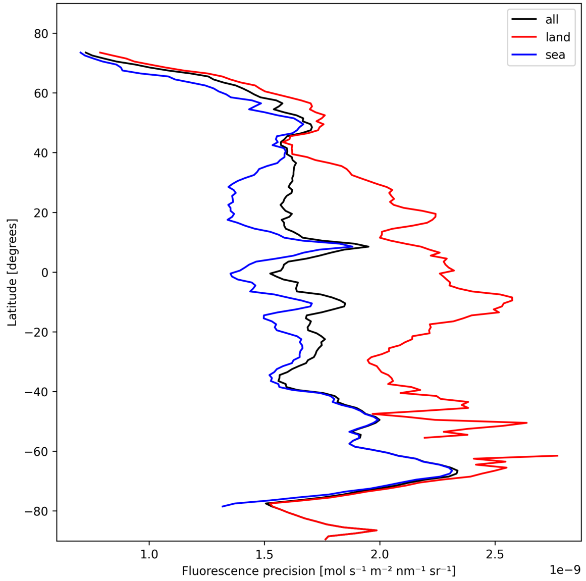
Figure 24: Zonal average of “Fluorescence precision” for 2024-10-31 to 2024-11-02.
