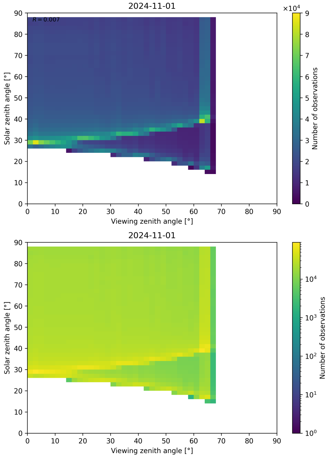
Figure 139: Scatter density plot of “Viewing zenith angle” against “Solar zenith angle” for 2024-10-31 to 2024-11-02.
