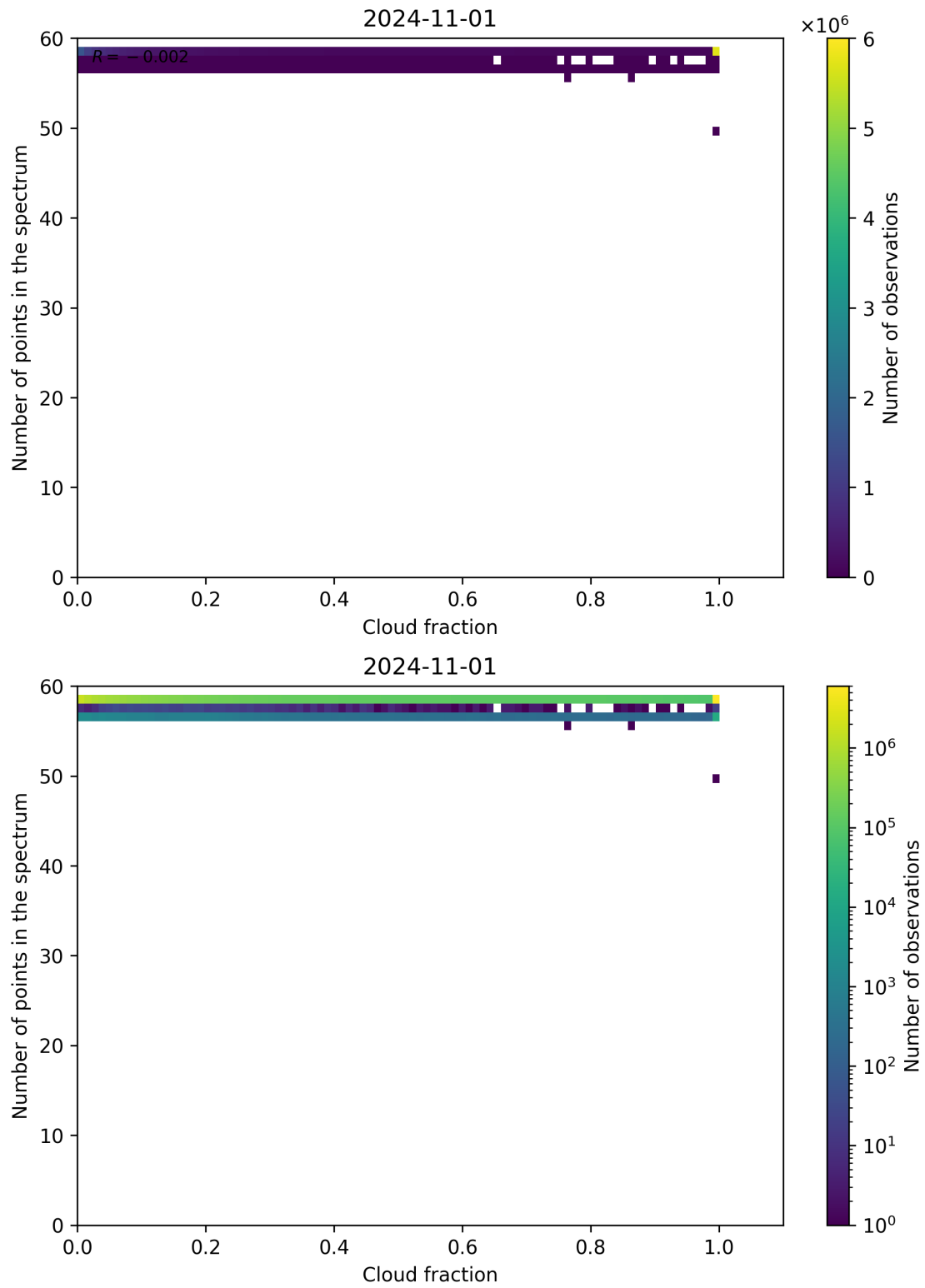
Figure 81: Scatter density plot of “Cloud fraction” against “Number of points in the spectrum” for 2024-10-31 to 2024-11-02.
