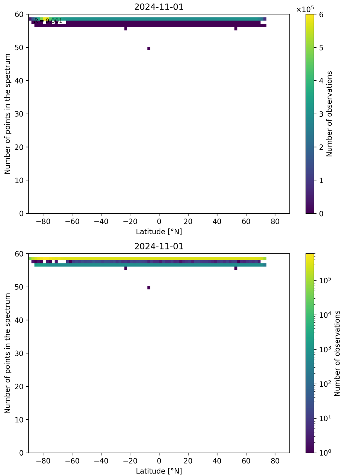
Figure 103: Scatter density plot of “Latitude” against “Number of points in the spectrum” for 2024-10-31 to 2024-11-02.
