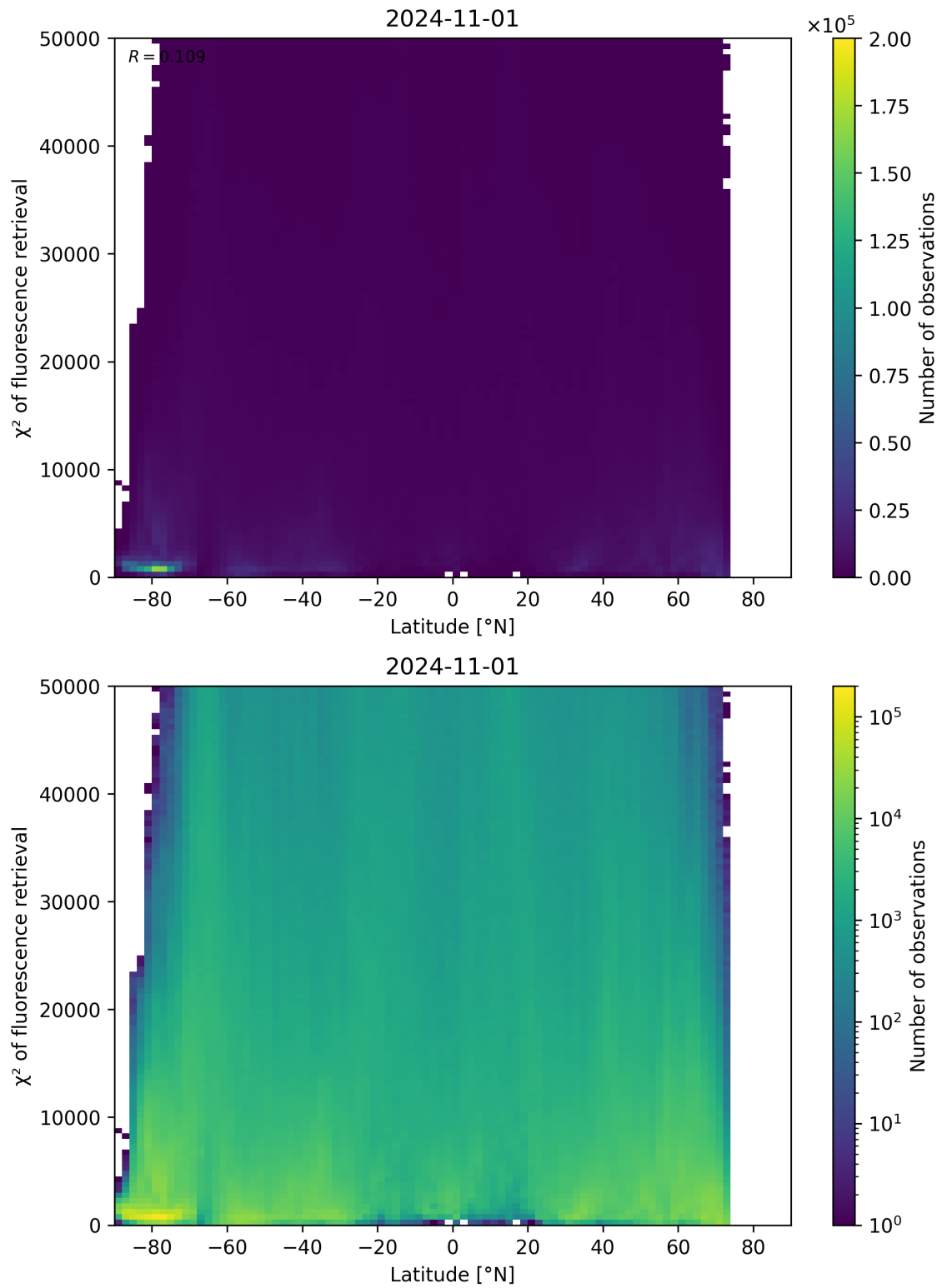
Figure 98: Scatter density plot of “Latitude” against “ \chi^2 of fluorescence retrieval” for 2024-10-31 to 2024-11-02.
