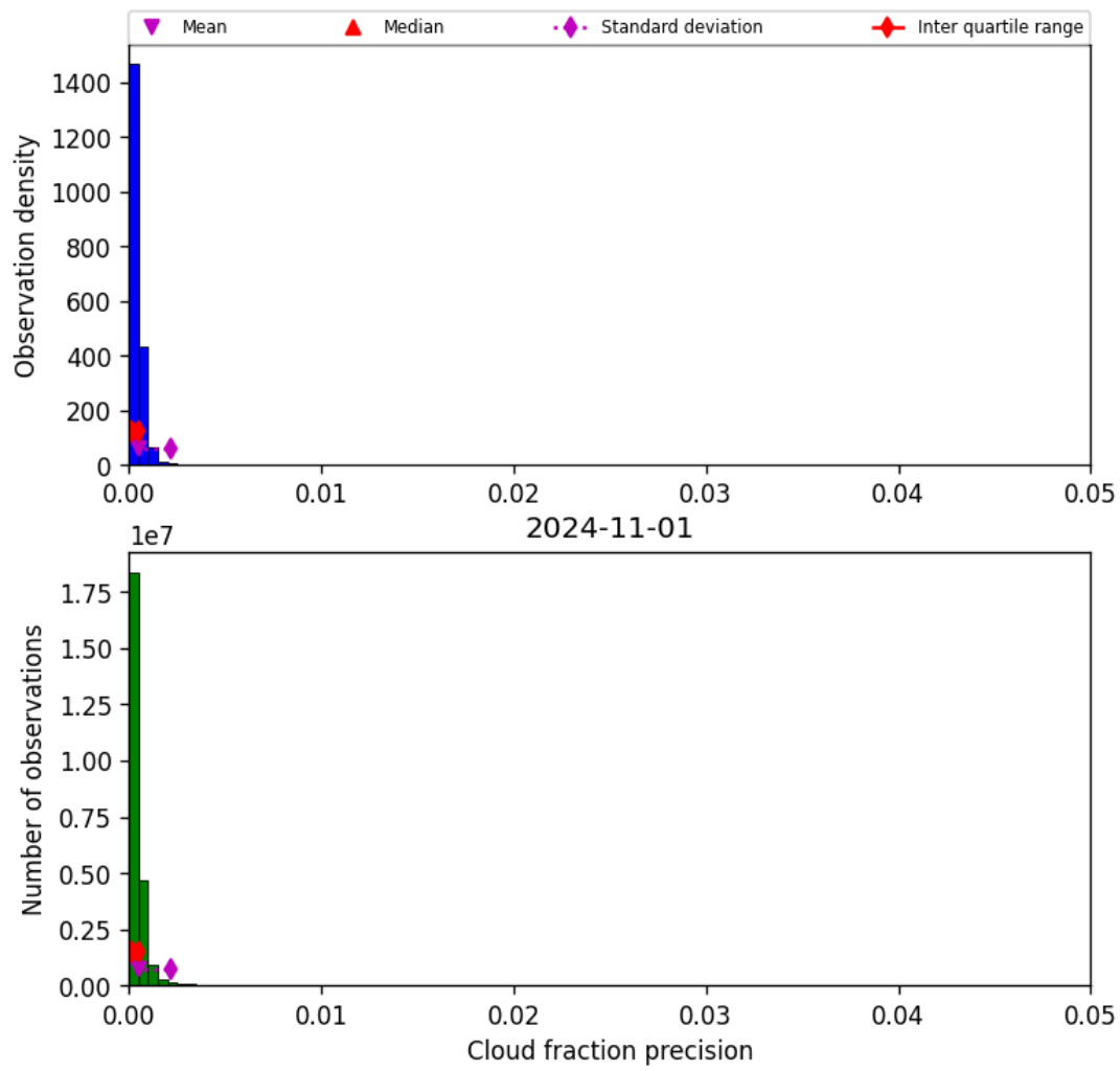
Figure 33: Histogram of “Cloud fraction precision” for 2024-10-31 to 2024-11-02
