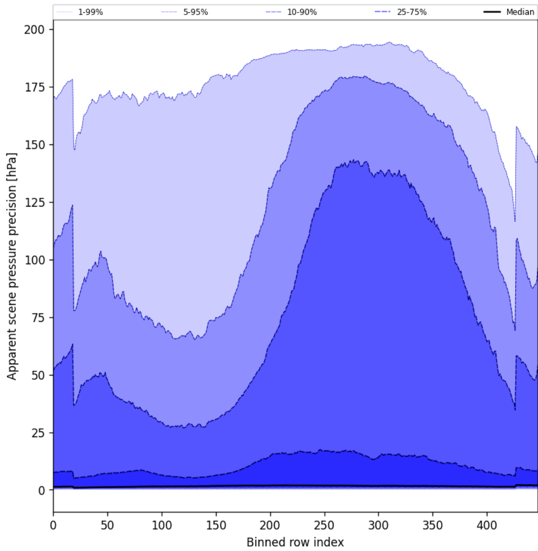
Figure 54: Along track statistics of “Apparent scene pressure precision” for 2024-10-31 to 2024-11-02
