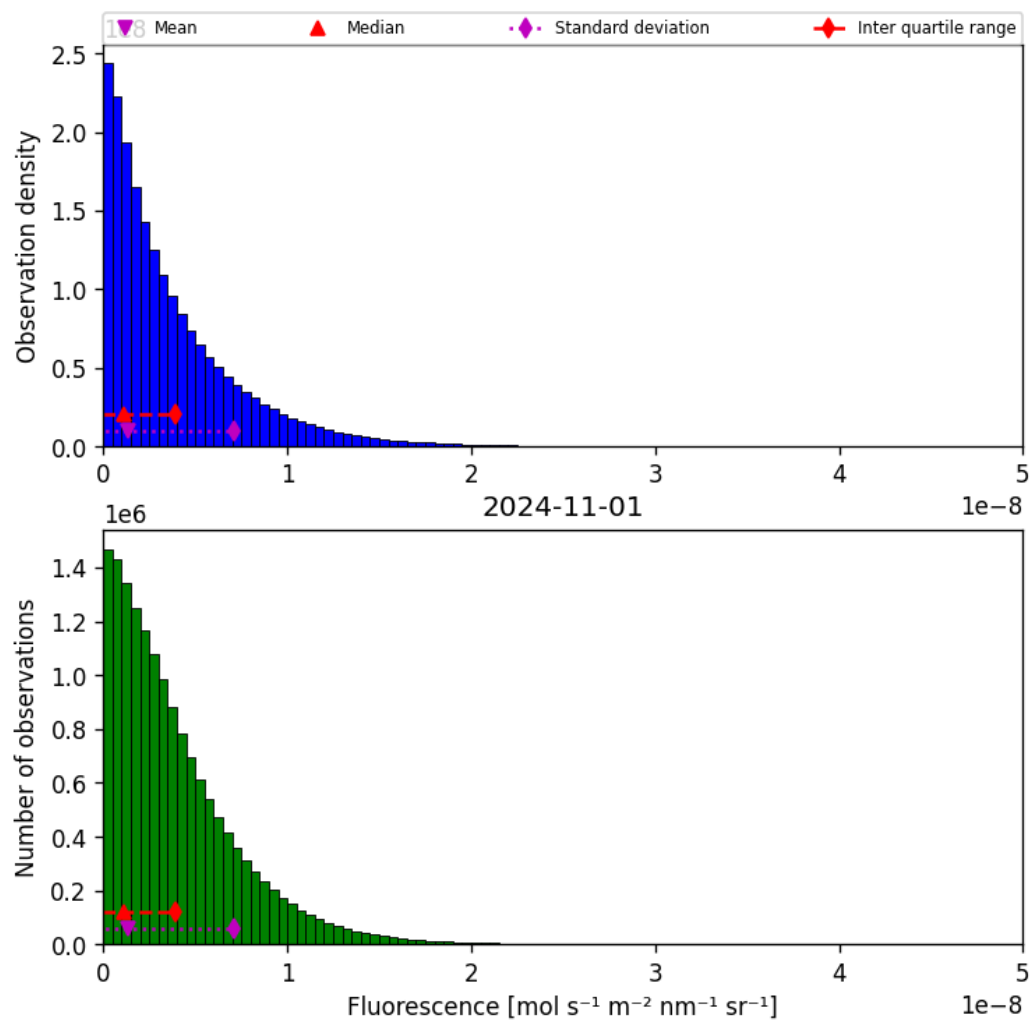
Figure 40: Histogram of “Fluorescence” for 2024-10-31 to 2024-11-02
