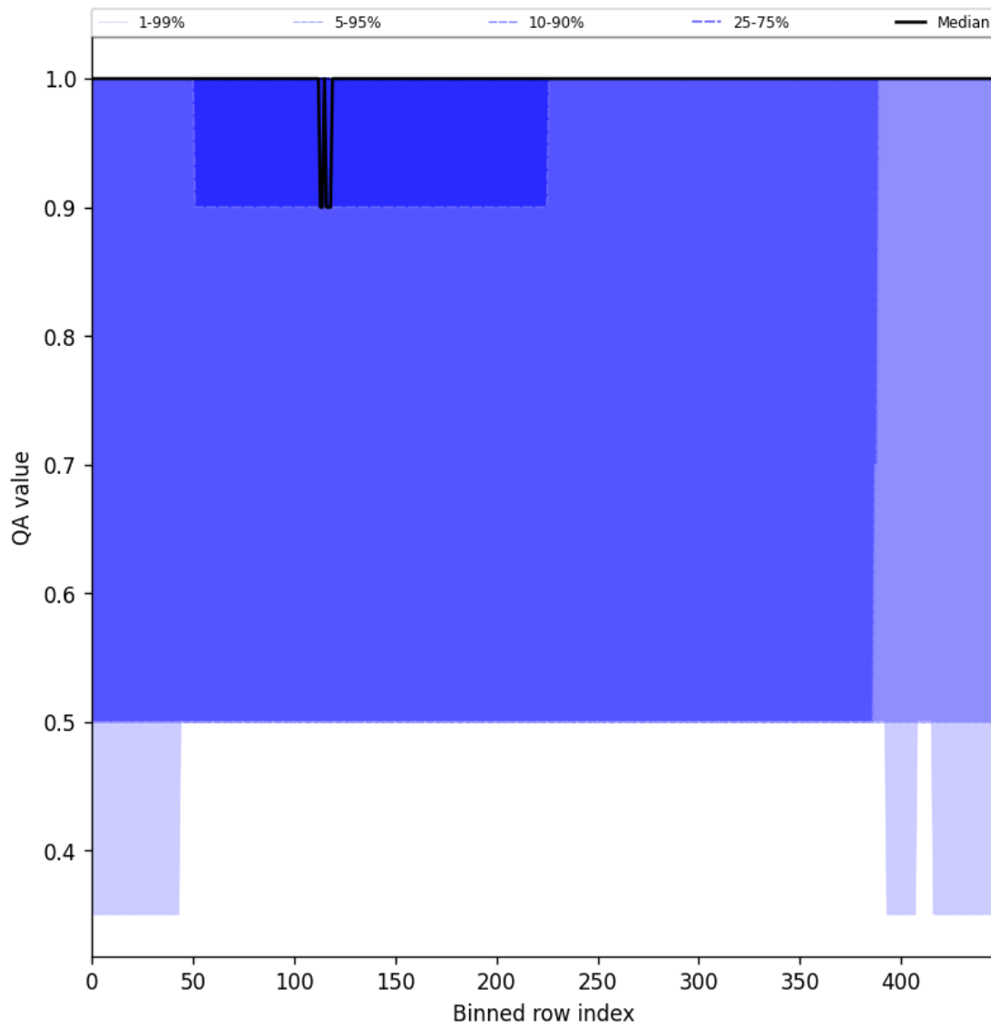
Figure 46: Along track statistics of “QA value” for 2024-10-31 to 2024-11-02
