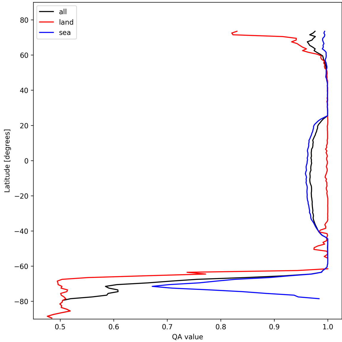
Figure 12: Zonal average of “QA value” for 2024-10-31 to 2024-11-02.
