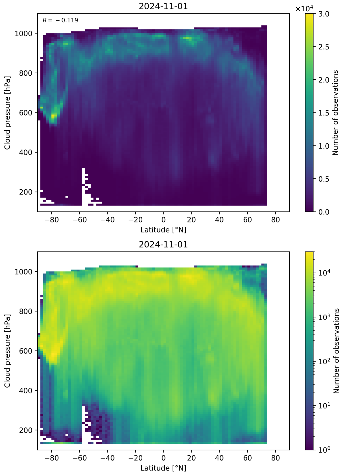
Figure 100: Scatter density plot of “Latitude” against “Cloud pressure” for 2024-10-31 to 2024-11-02.
