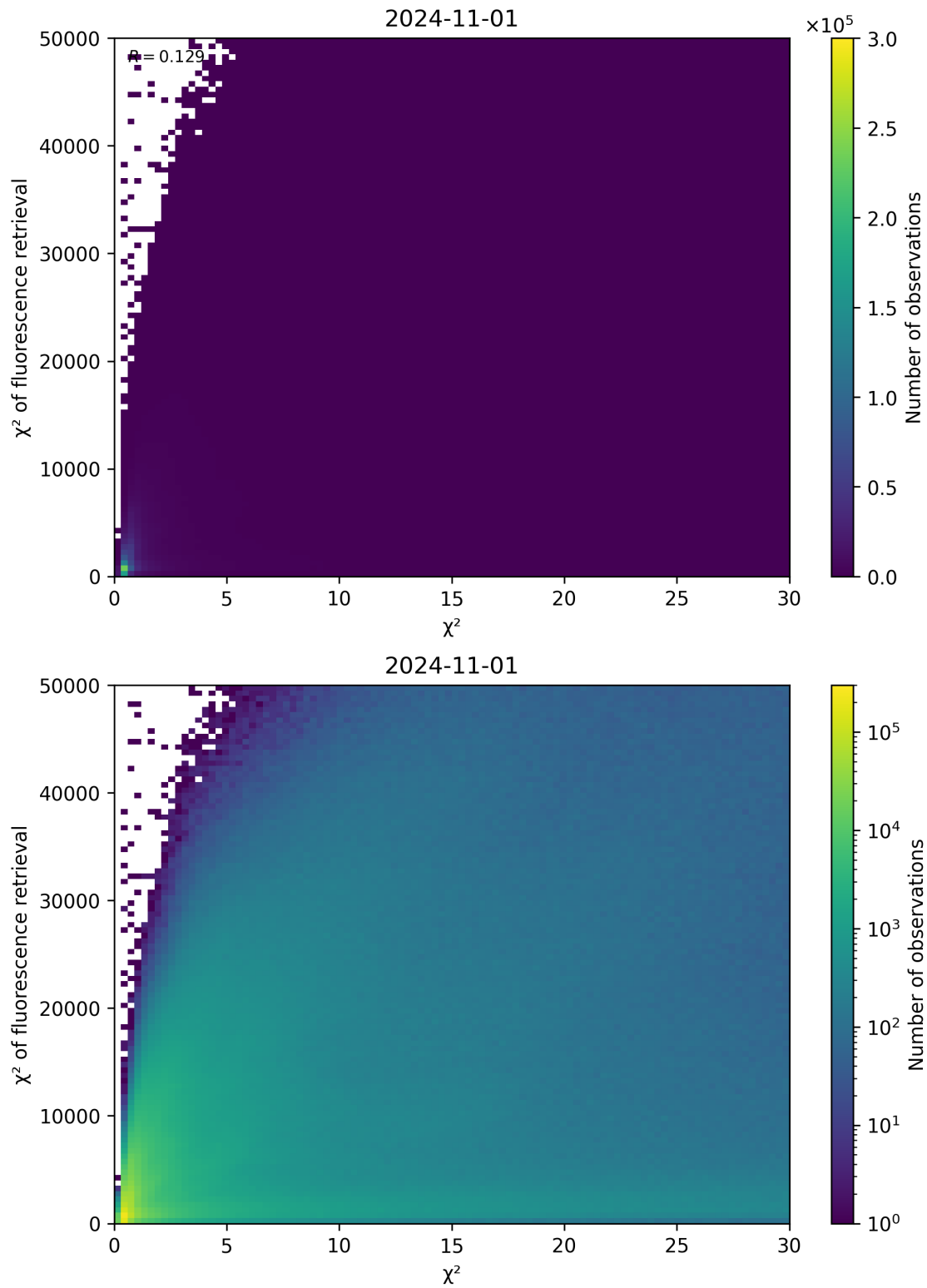
Figure 69: Scatter density plot of “ \chi^2 ” against “ \chi^2 of fluorescence retrieval” for 2024-10-31 to 2024-11-02.
