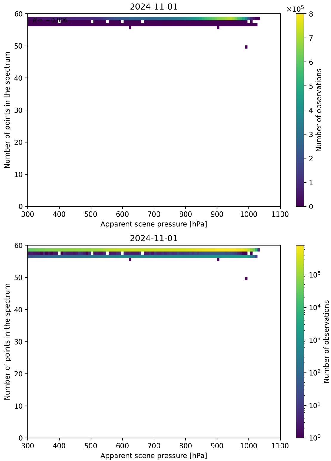
Figure 67: Scatter density plot of “Apparent scene pressure” against “Number of points in the spectrum” for 2024-10-31 to 2024-11-02.
