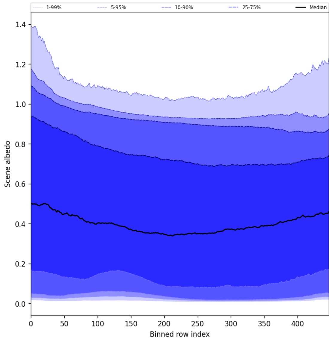
Figure 51: Along track statistics of “Scene albedo” for 2024-10-31 to 2024-11-02
