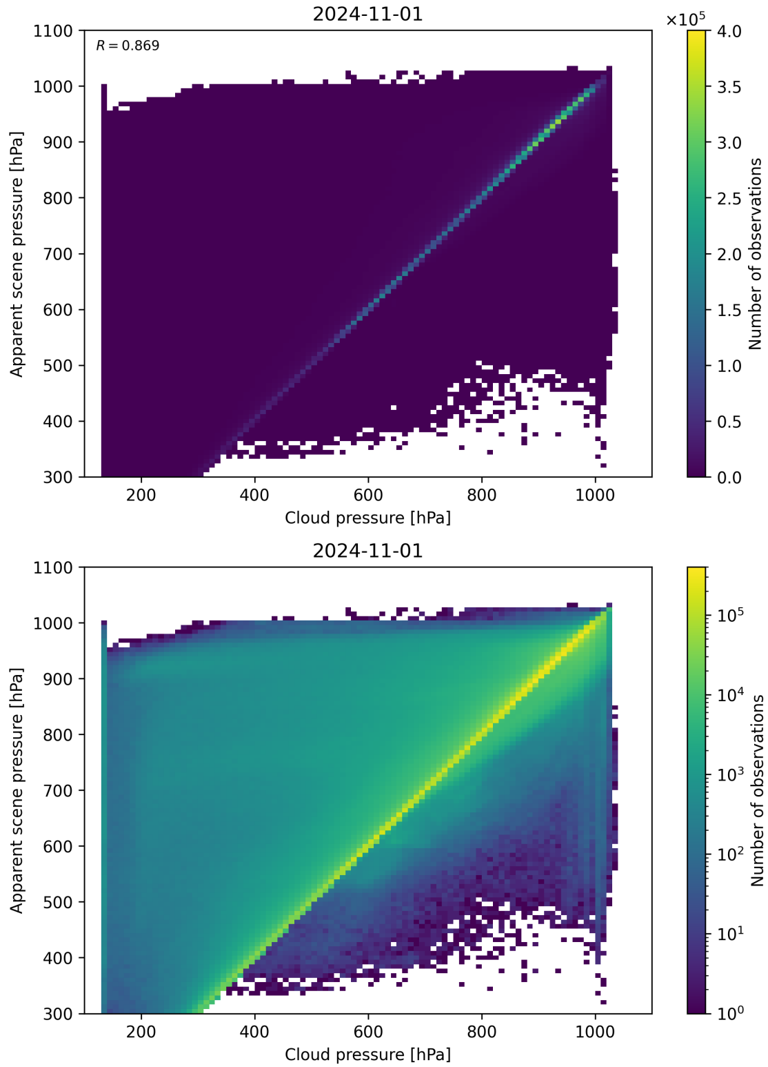
Figure 84: Scatter density plot of “Cloud pressure” against “Apparent scene pressure” for 2024-10-31 to 2024-11-02.
