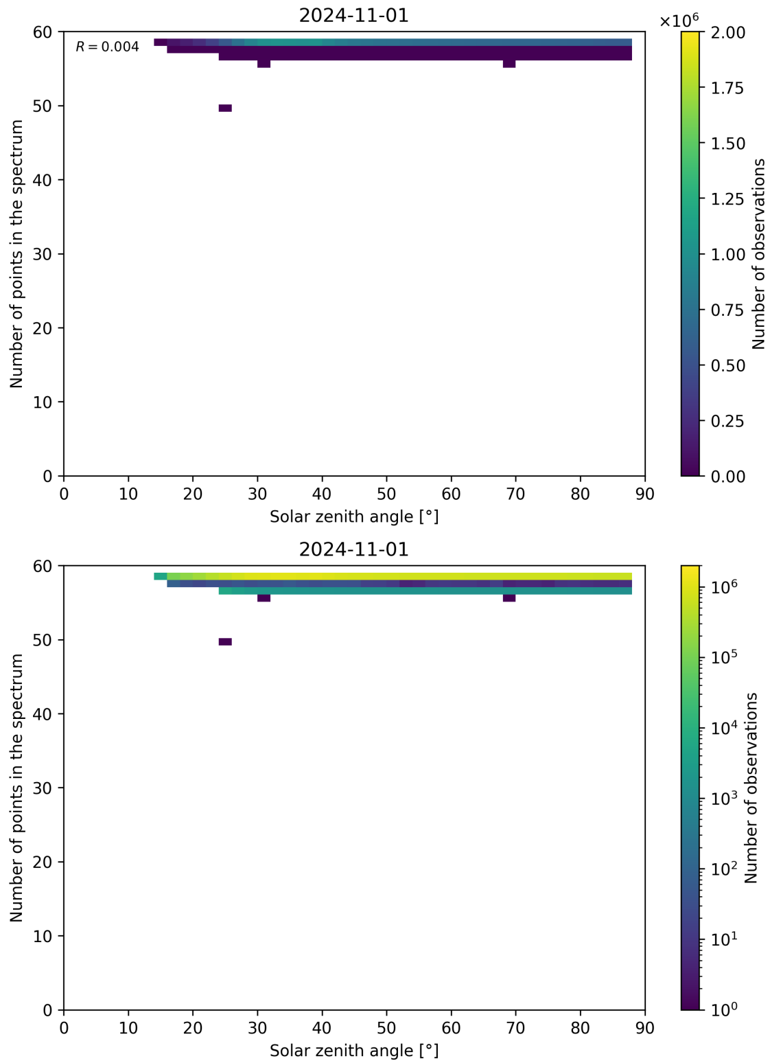
Figure 126: Scatter density plot of “Solar zenith angle” against “Number of points in the spectrum” for 2024-10-31 to 2024-11-02.
