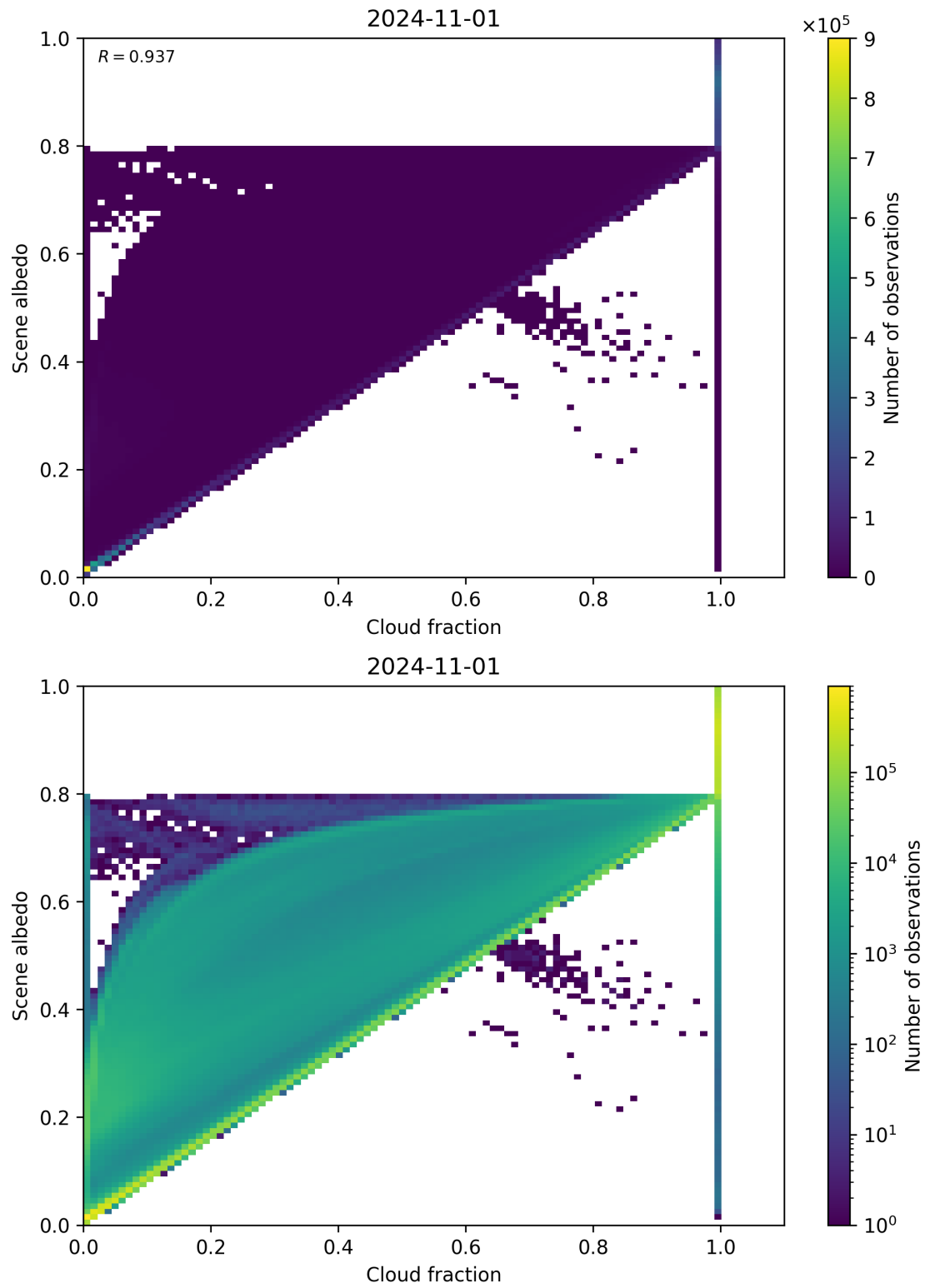
Figure 82: Scatter density plot of “Cloud fraction” against “Scene albedo” for 2024-10-31 to 2024-11-02.
