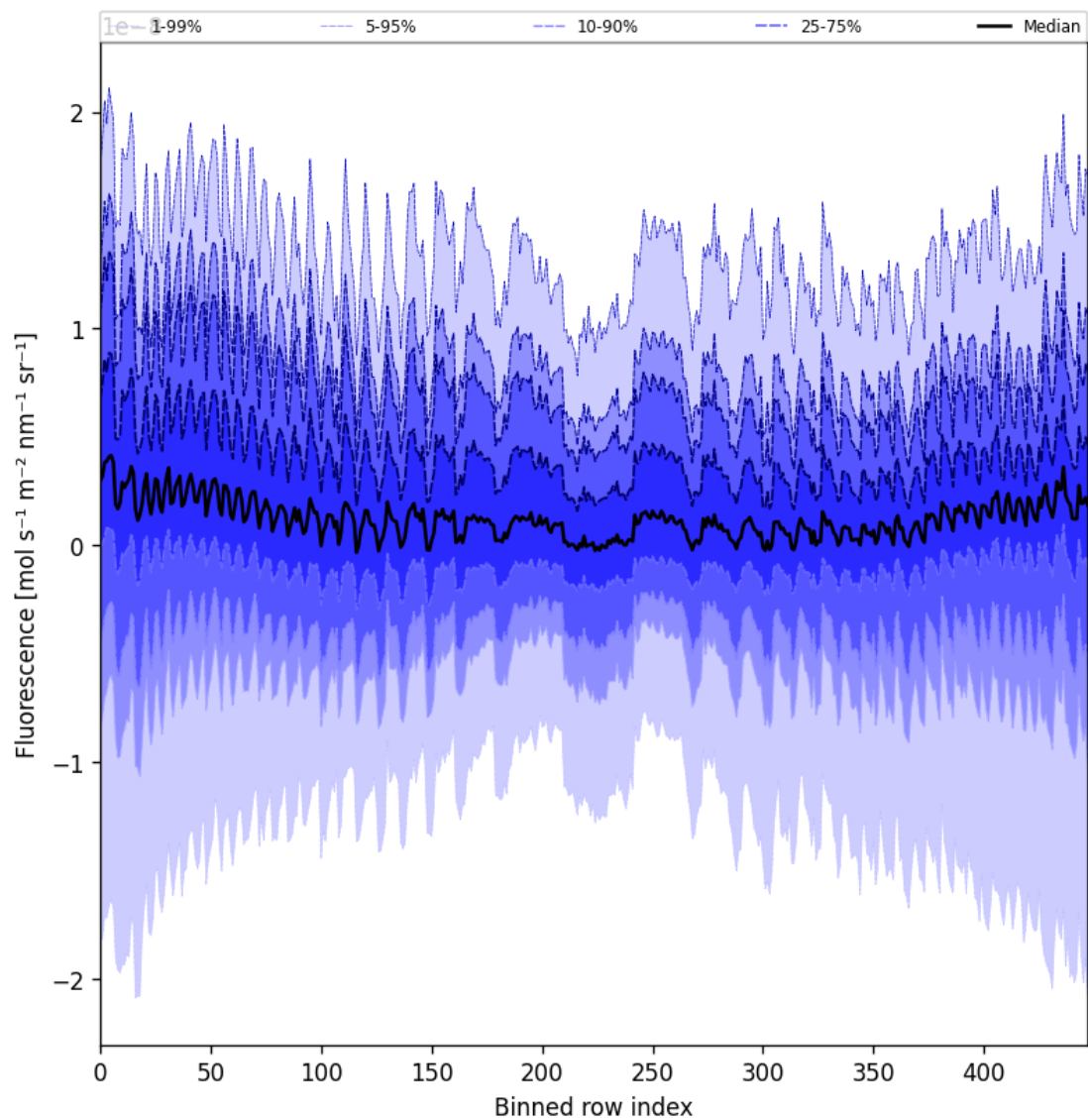
Figure 57: Along track statistics of “Fluorescence” for 2024-10-31 to 2024-11-02
