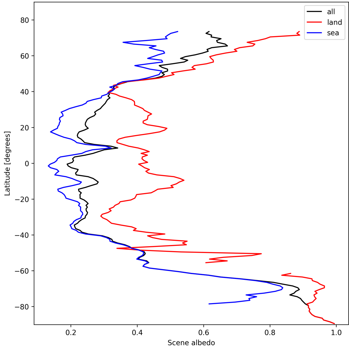
Figure 17: Zonal average of “Scene albedo” for 2024-10-31 to 2024-11-02.
