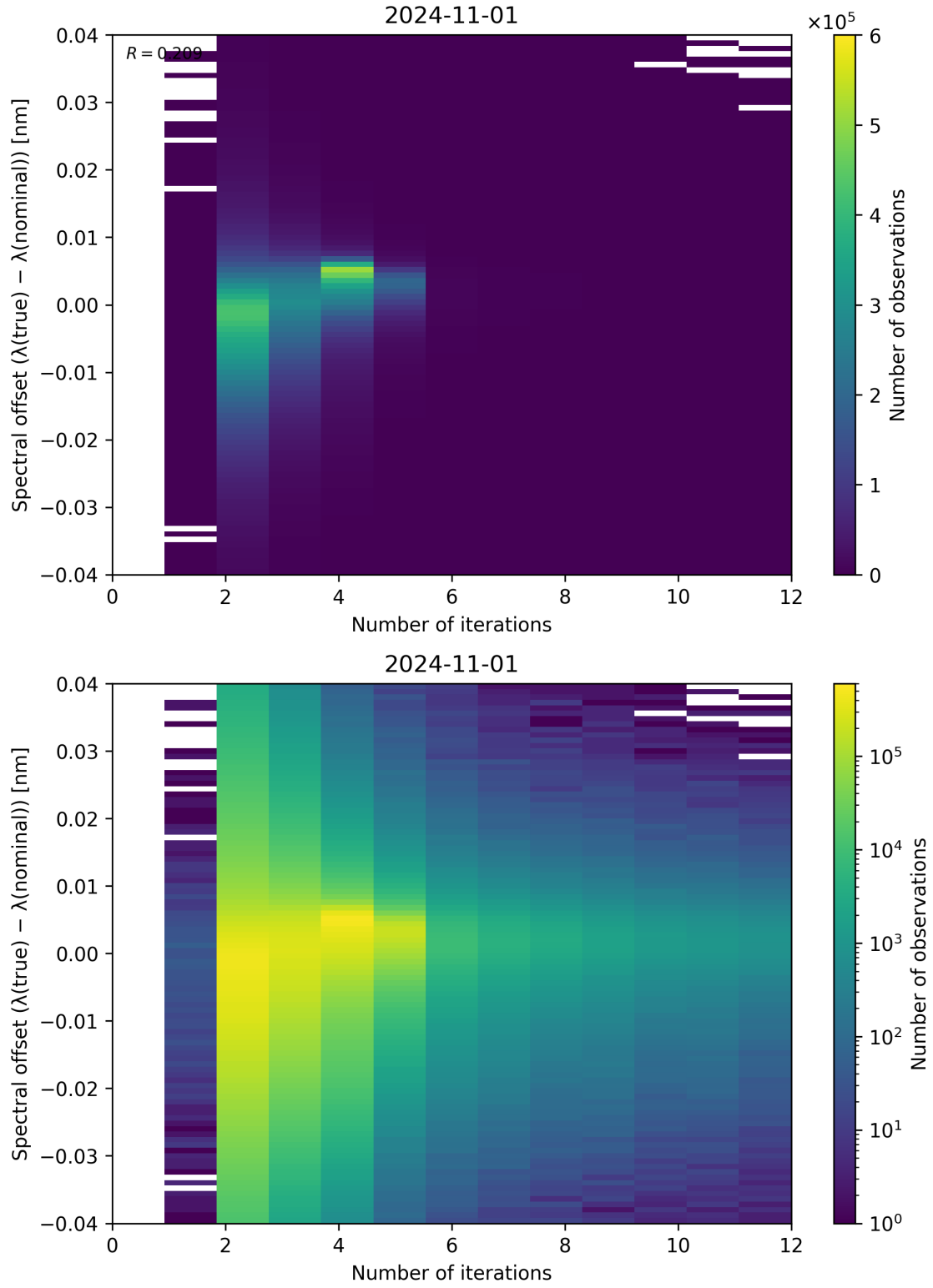
Figure 109: Scatter density plot of “Number of iterations” against “Spectral offset ( \lambda_{\text{true}} - \lambda_{\text{nominal}} )” for 2024-10-31 to 2024-11-02.
