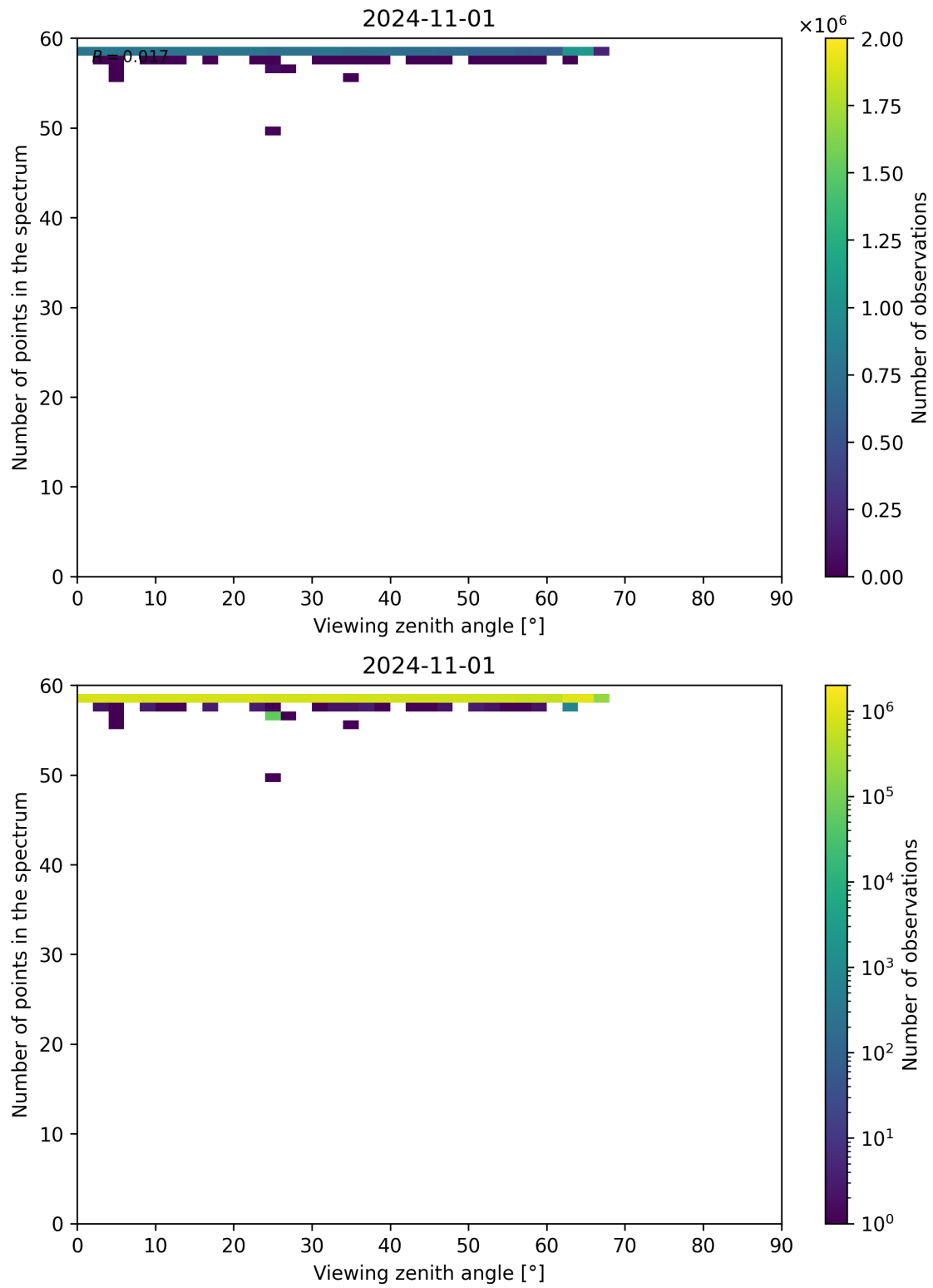
Figure 137: Scatter density plot of “Viewing zenith angle” against “Number of points in the spectrum” for 2024-10-31 to 2024-11-02.
