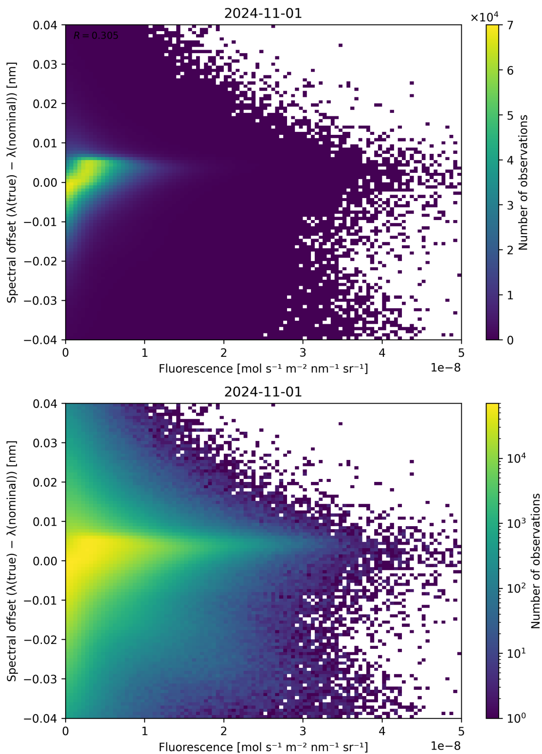
Figure 95: Scatter density plot of “Fluorescence” against “Spectral offset ( \lambda_{\text{true}} - \lambda_{\text{nominal}} )” for 2024-10-31 to 2024-11-02.
