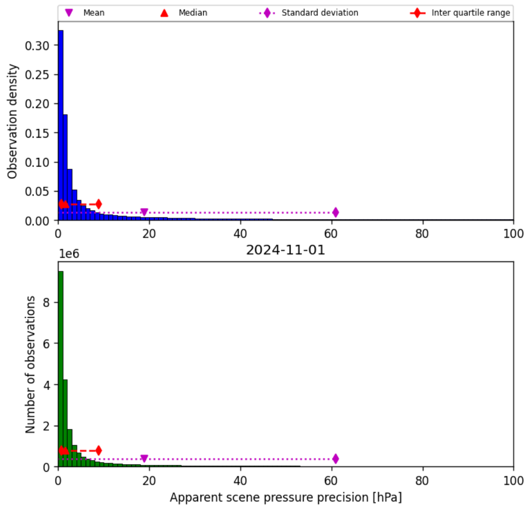
Figure 37: Histogram of “Apparent scene pressure precision” for 2024-10-31 to 2024-11-02
