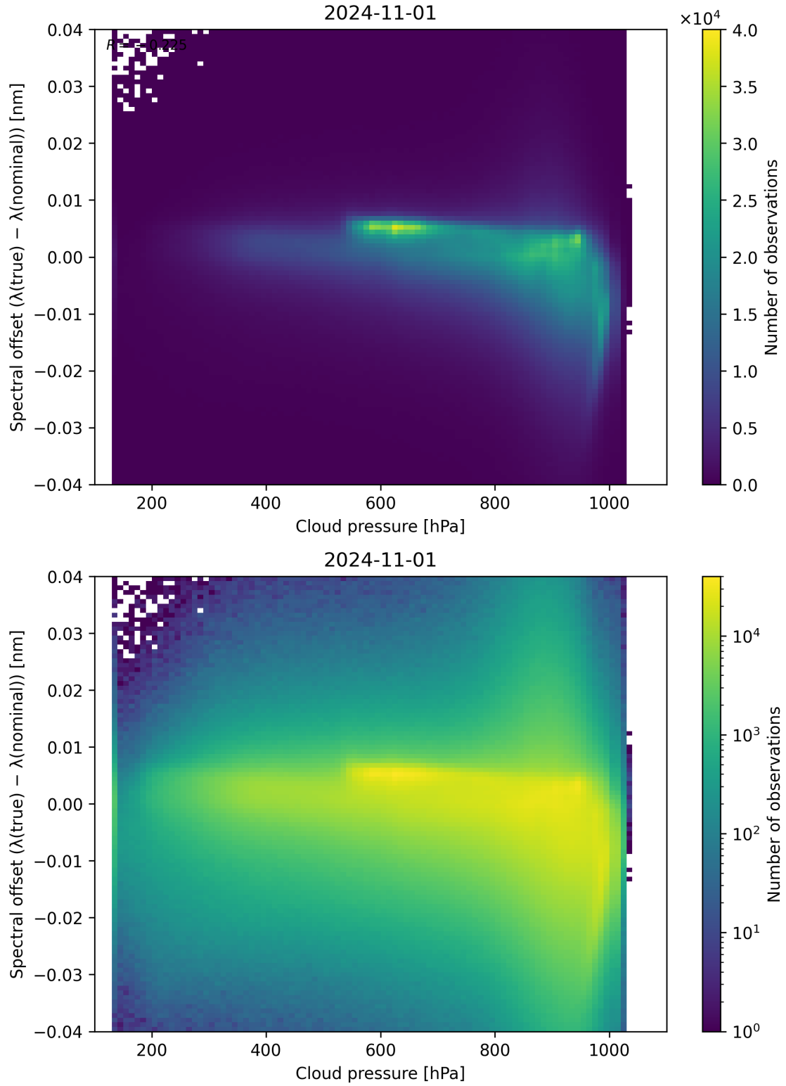
Figure 92: Scatter density plot of “Cloud pressure” against “Spectral offset ( \lambda_{\text{true}} - \lambda_{\text{nominal}} )” for 2024-10-31 to 2024-11-02.
