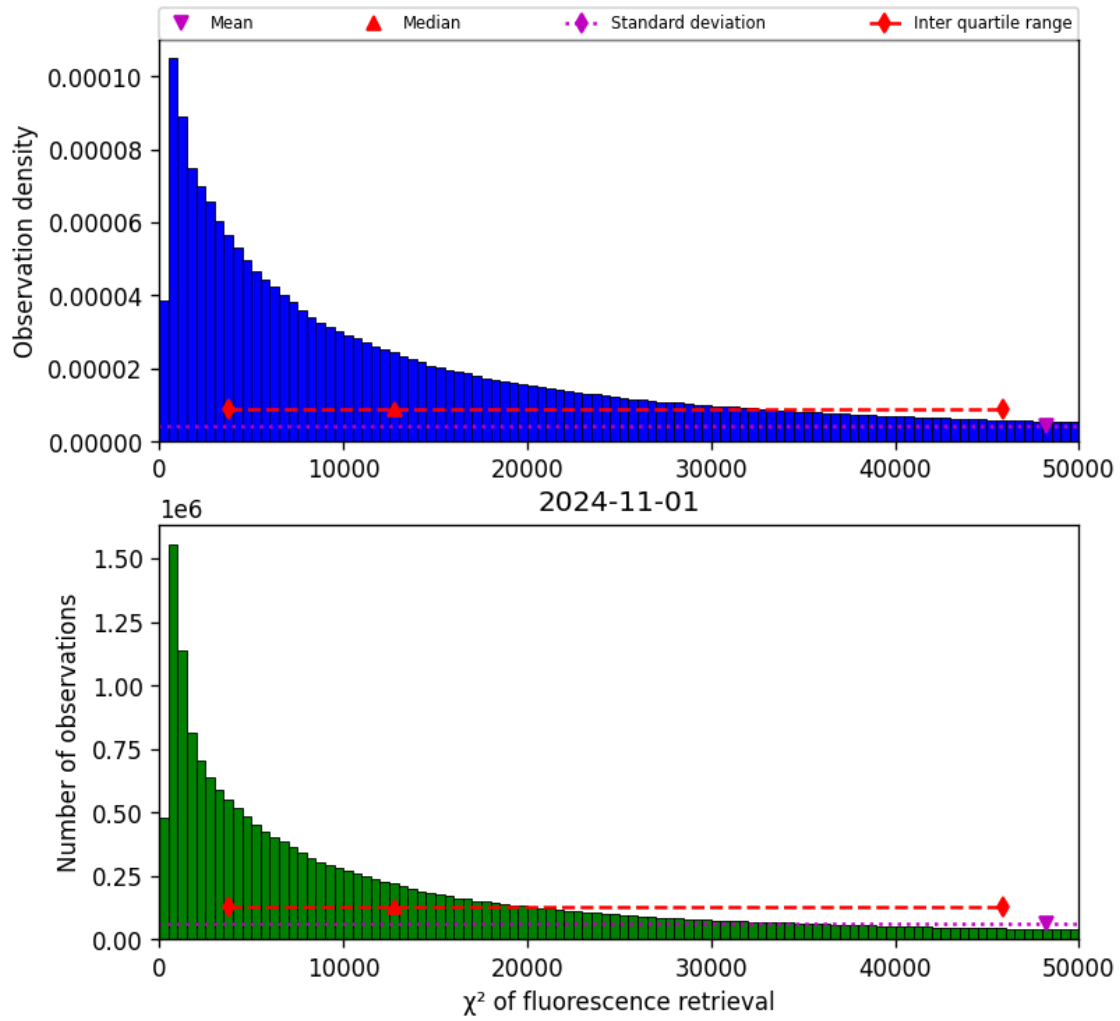
Figure 42: Histogram of “ \chi^2 of fluorescence retrieval” for 2024-10-31 to 2024-11-02
