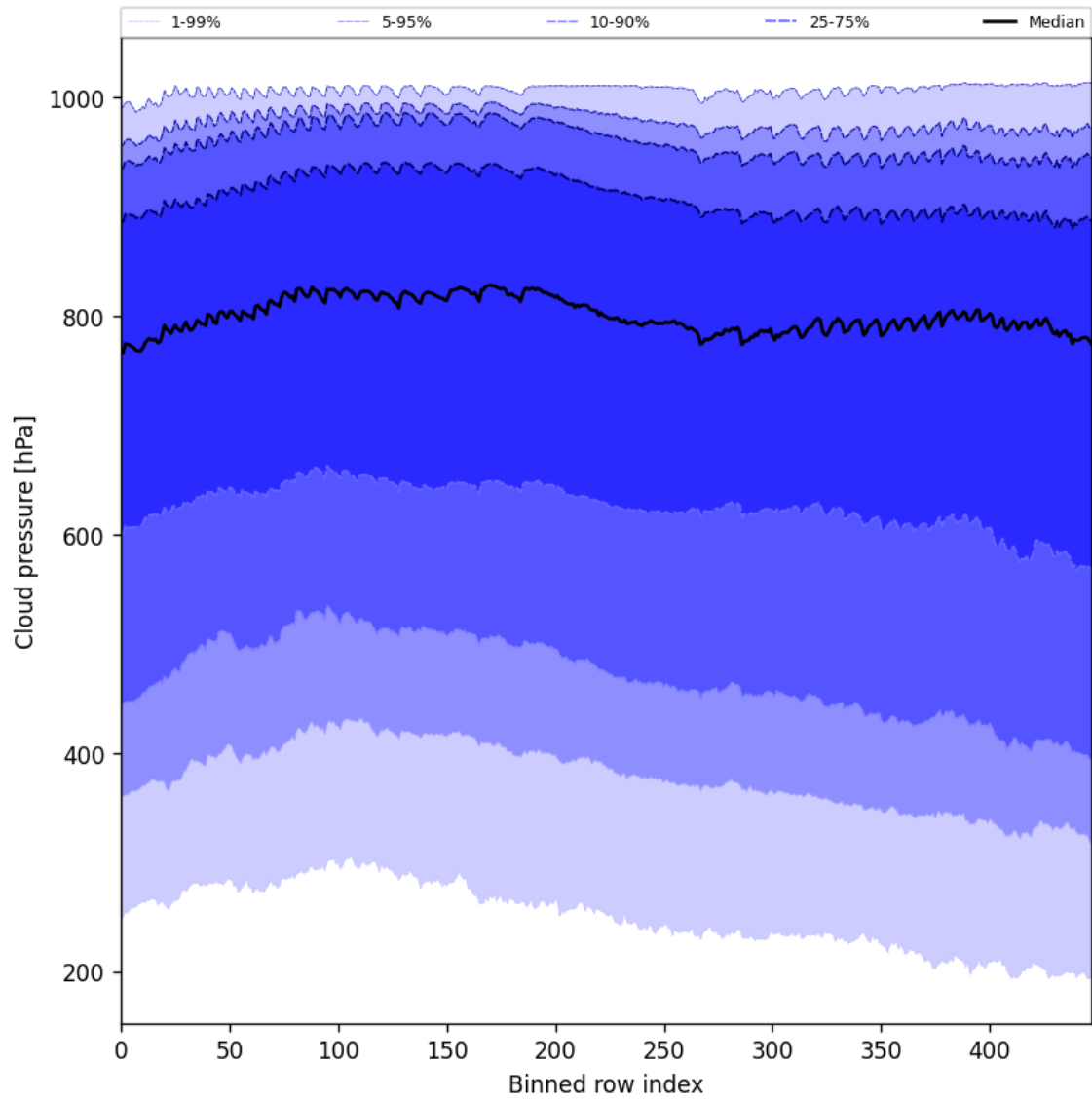
Figure 47: Along track statistics of “Cloud pressure” for 2024-10-31 to 2024-11-02
