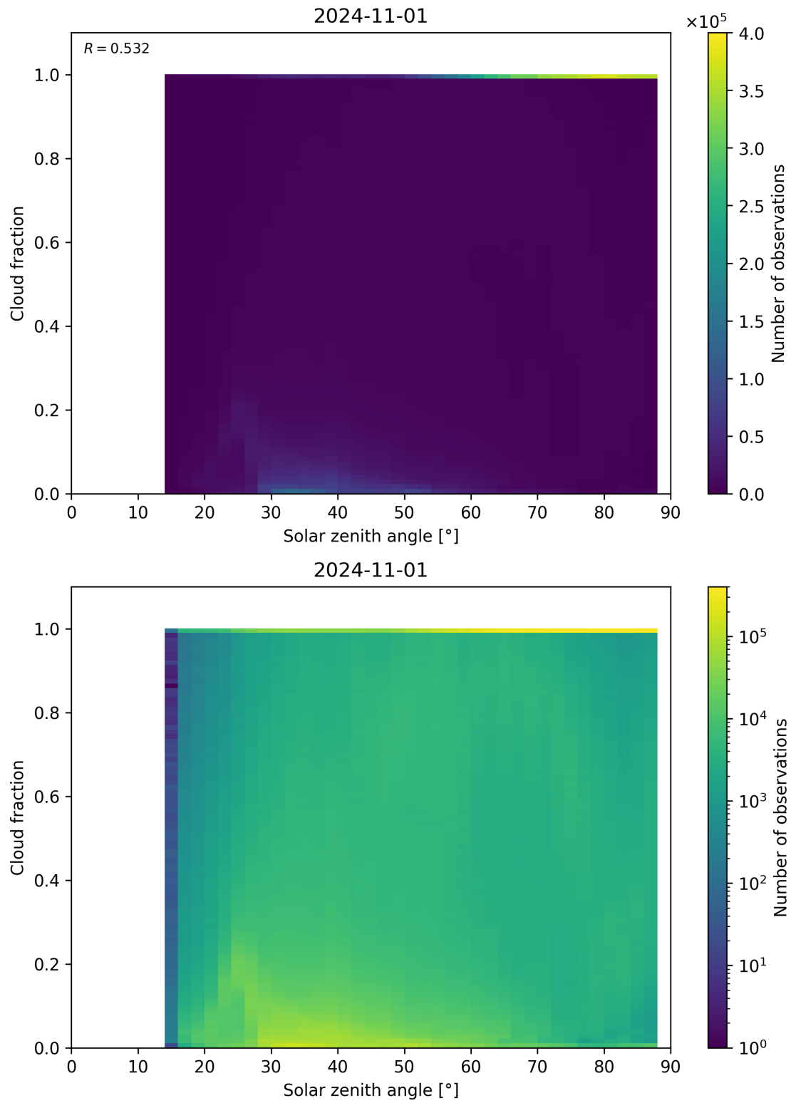
Figure 121: Scatter density plot of “Solar zenith angle” against “Cloud fraction” for 2024-10-31 to 2024-11-02.
