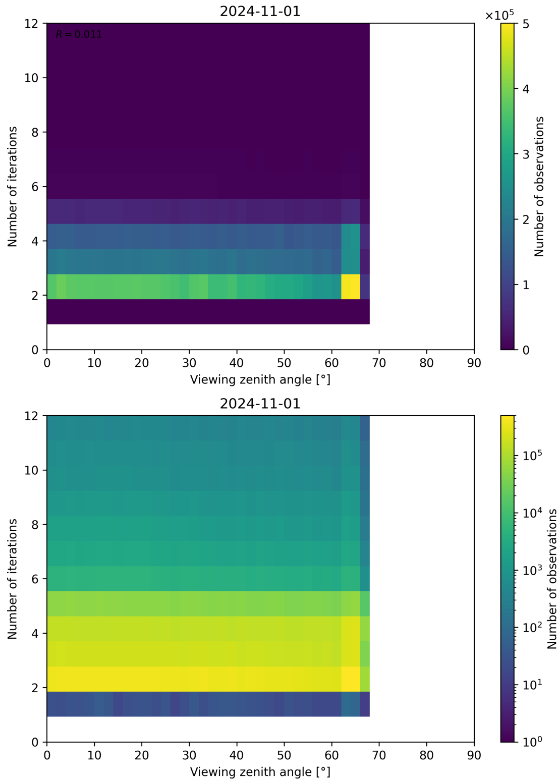
Figure 136: Scatter density plot of “Viewing zenith angle” against “Number of iterations” for 2024-10-31 to 2024-11-02.
