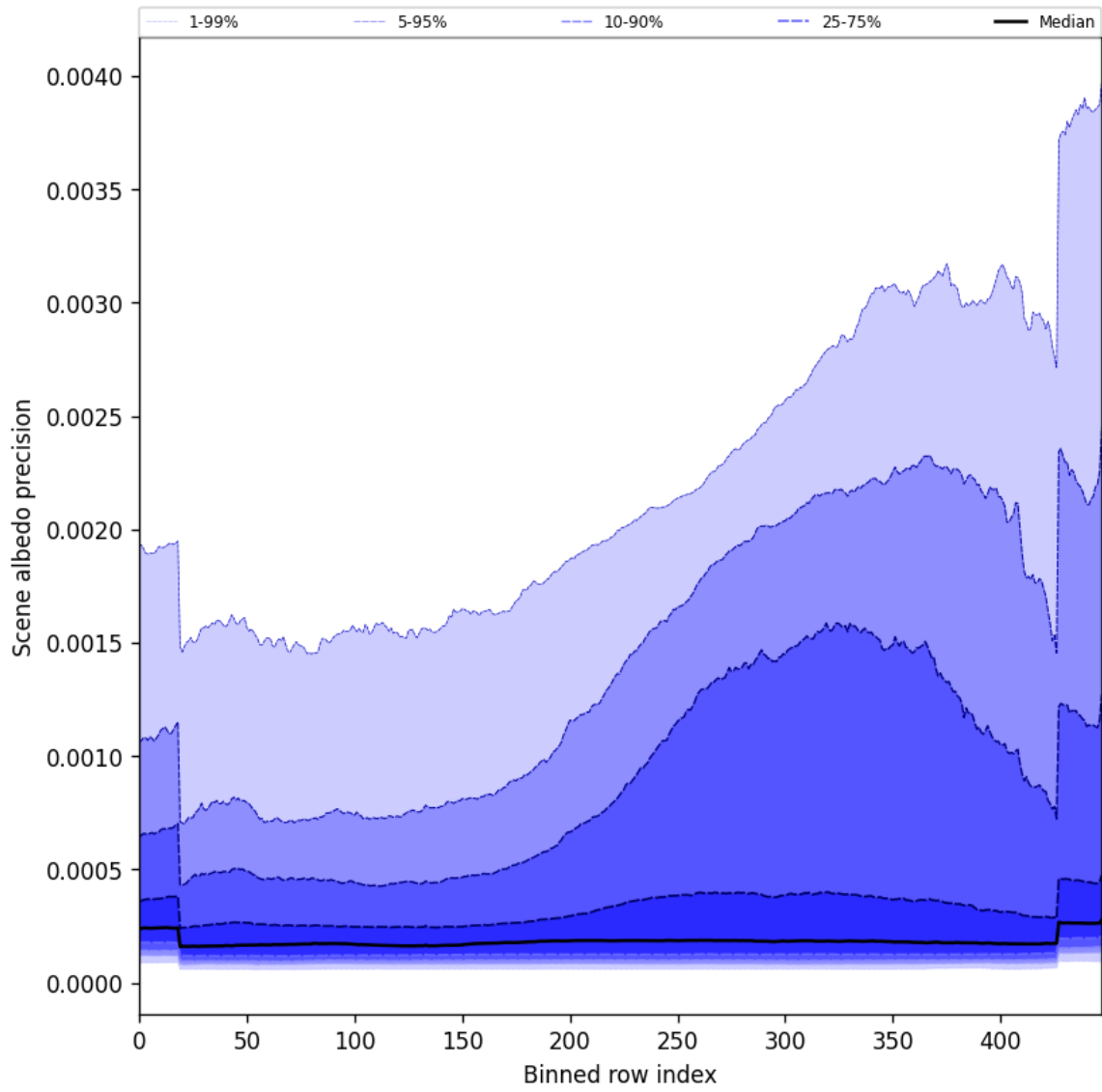
Figure 52: Along track statistics of “Scene albedo precision” for 2024-10-31 to 2024-11-02
