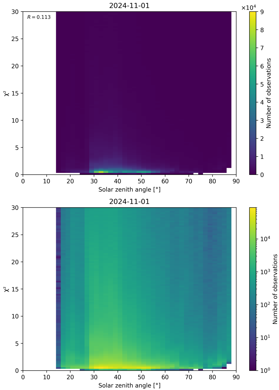
Figure 119: Scatter density plot of “Solar zenith angle” against “ \chi^2 ” for 2024-10-31 to 2024-11-02.
