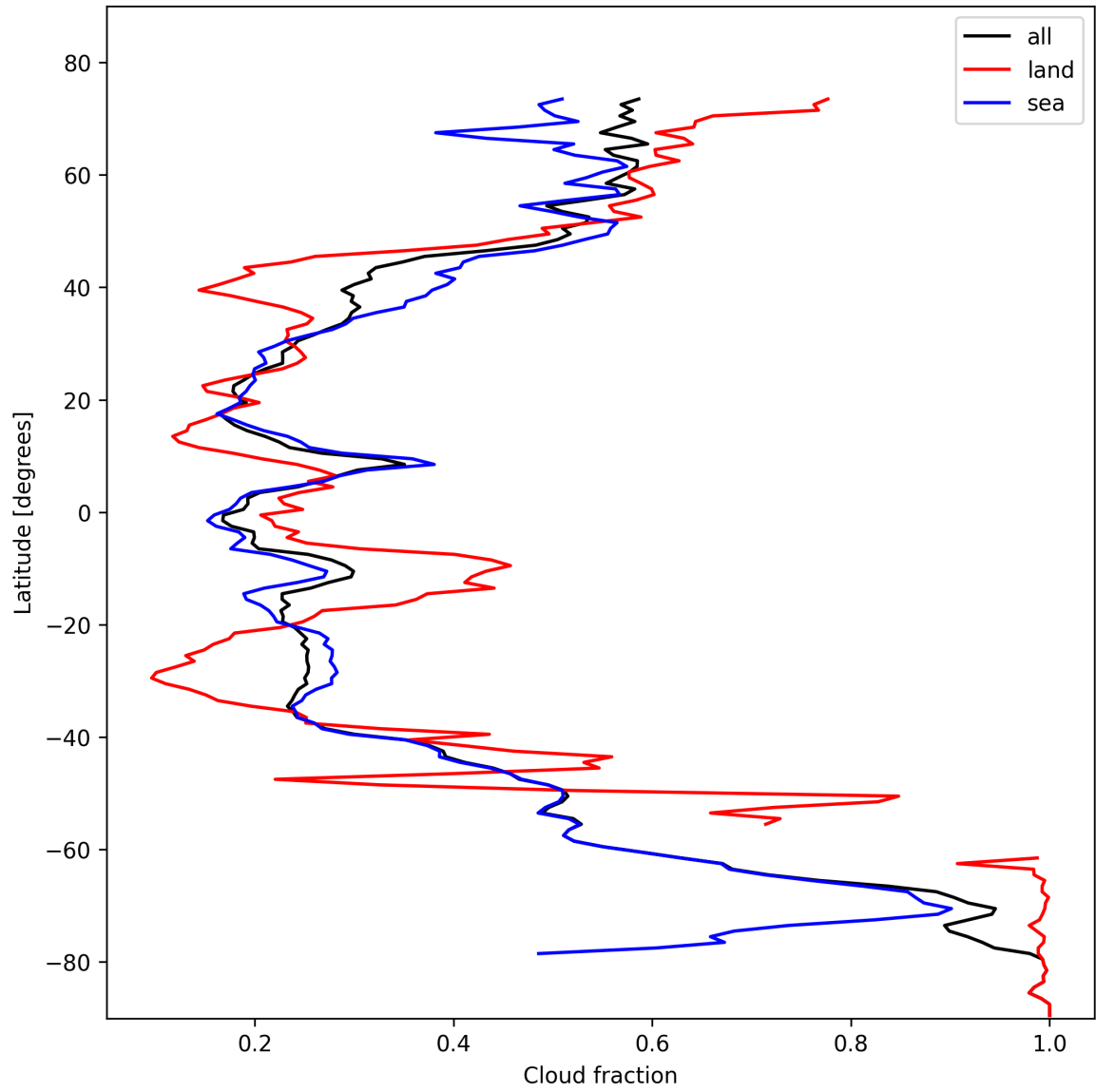
Figure 15: Zonal average of “Cloud fraction” for 2024-10-31 to 2024-11-02.
