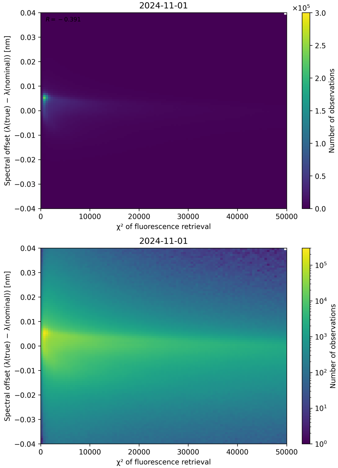
Figure 72: Scatter density plot of “ \chi^2 of fluorescence retrieval” against “Spectral offset ( \lambda_{\text{true}} - \lambda_{\text{nominal}} )” for 2024-10-31 to 2024-11-02.
