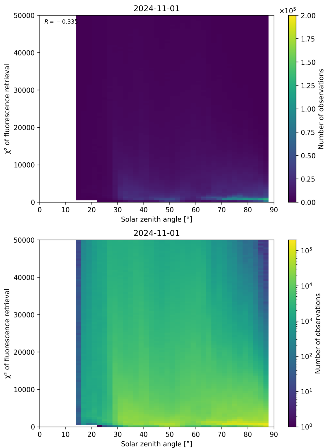
Figure 120: Scatter density plot of “Solar zenith angle” against “ \chi^2 of fluorescence retrieval” for 2024-10-31 to 2024-11-02.
