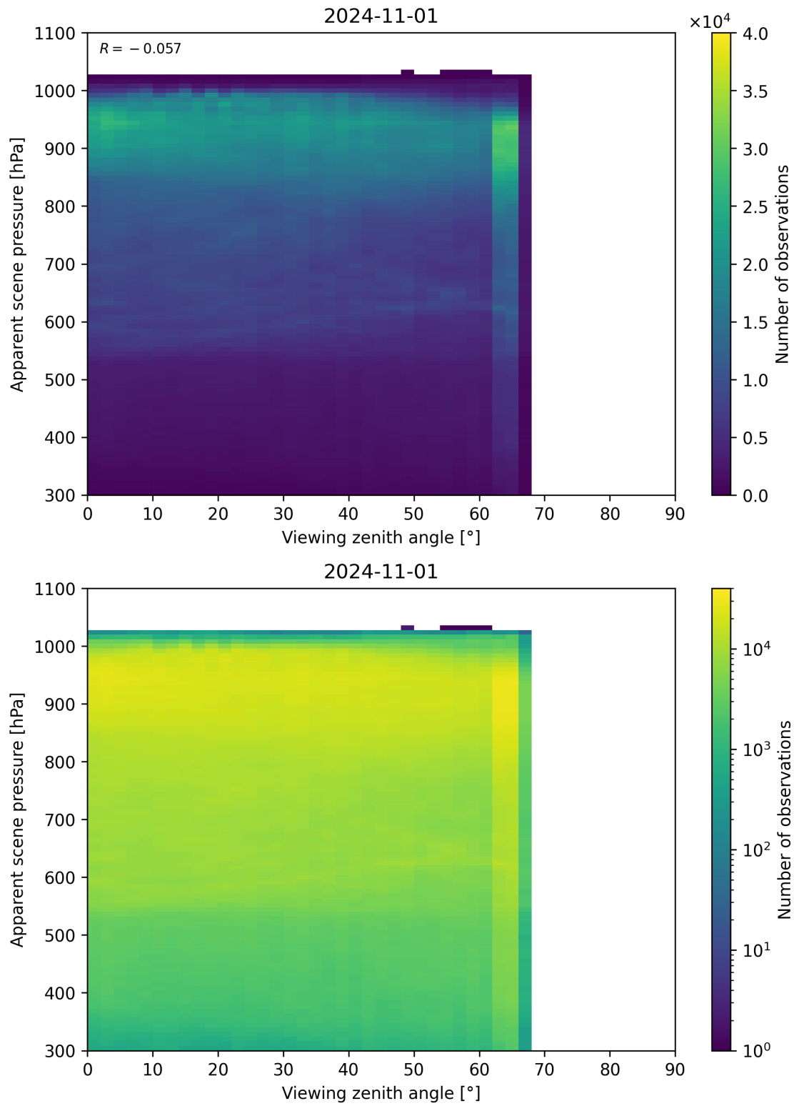
Figure 129: Scatter density plot of “Viewing zenith angle” against “Apparent scene pressure” for 2024-10-31 to 2024-11-02.
