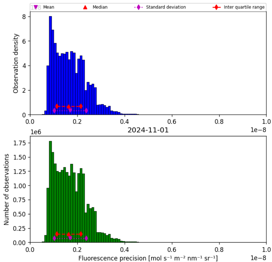
Figure 41: Histogram of “Fluorescence precision” for 2024-10-31 to 2024-11-02
