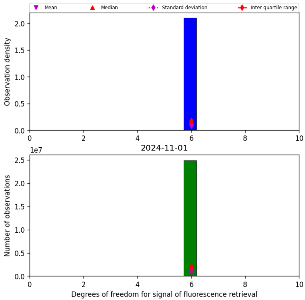
Figure 43: Histogram of "Degrees of freedom for signal of fluorescence retrieval" for 2024-10-31 to 2024-11-02
