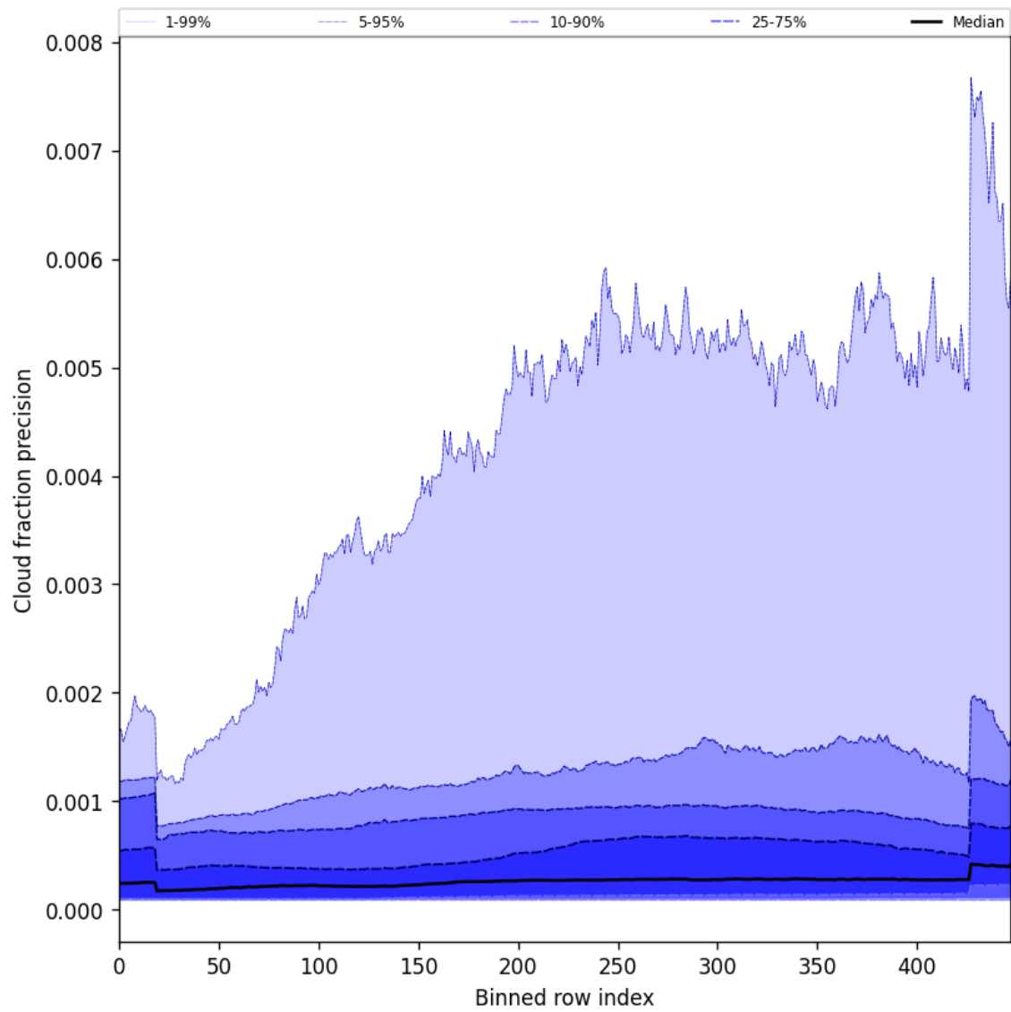
Figure 50: Along track statistics of “Cloud fraction precision” for 2024-10-31 to 2024-11-02
