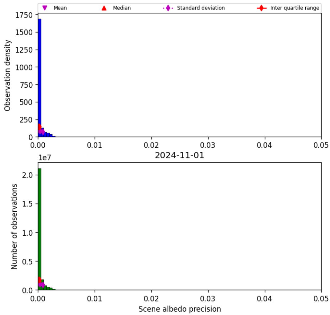
Figure 35: Histogram of “Scene albedo precision” for 2024-10-31 to 2024-11-02
