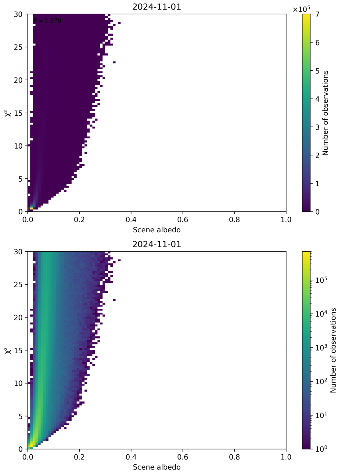
Figure 112: Scatter density plot of “Scene albedo” against “ \chi^2 ” for 2024-10-31 to 2024-11-02.
