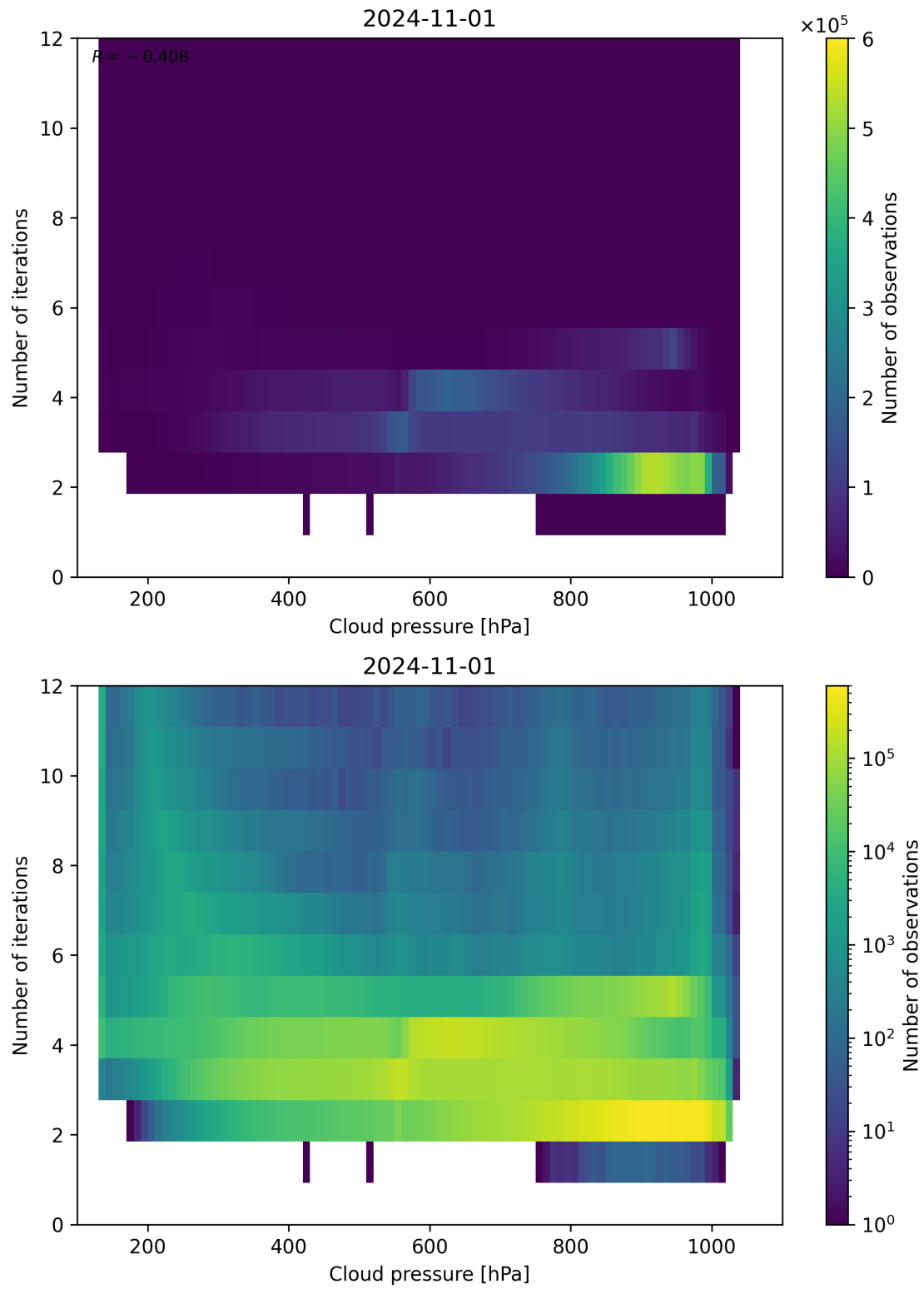
Figure 89: Scatter density plot of “Cloud pressure” against “Number of iterations” for 2024-10-31 to 2024-11-02.
