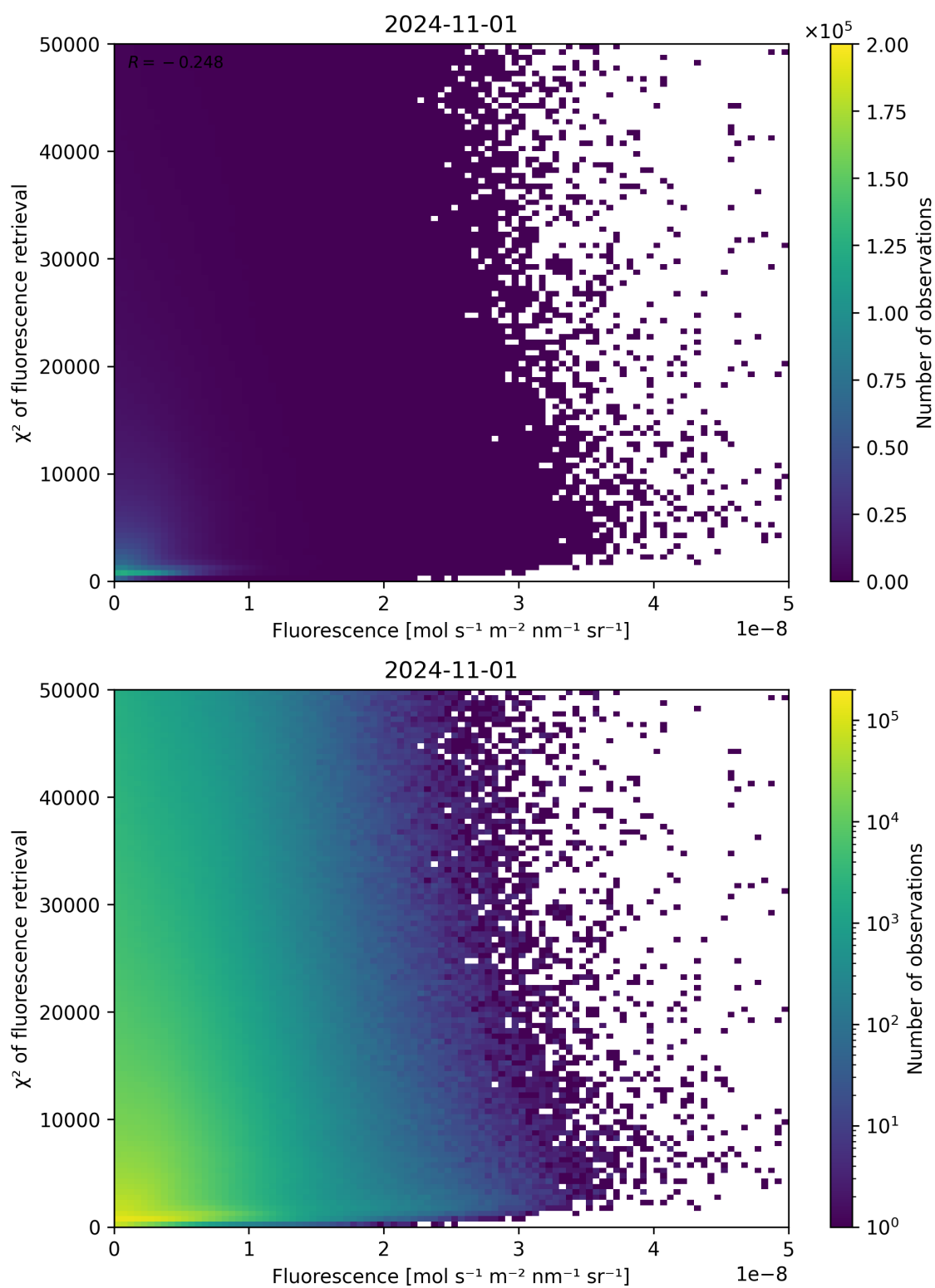
Figure 93: Scatter density plot of “Fluorescence” against “ \chi^2 of fluorescence retrieval” for 2024-10-31 to 2024-11-02.
