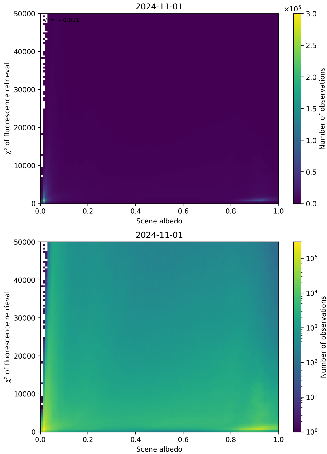
Figure 113: Scatter density plot of “Scene albedo” against “ \chi^2 of fluorescence retrieval” for 2024-10-31 to 2024-11-02.
