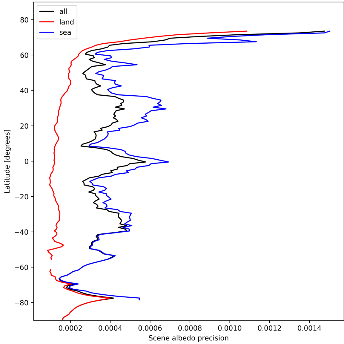
Figure 18: Zonal average of “Scene albedo precision” for 2024-10-31 to 2024-11-02.
