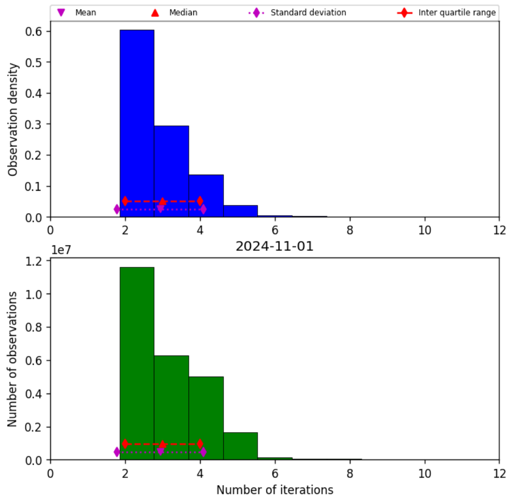
Figure 39: Histogram of “Number of iterations” for 2024-10-31 to 2024-11-02
