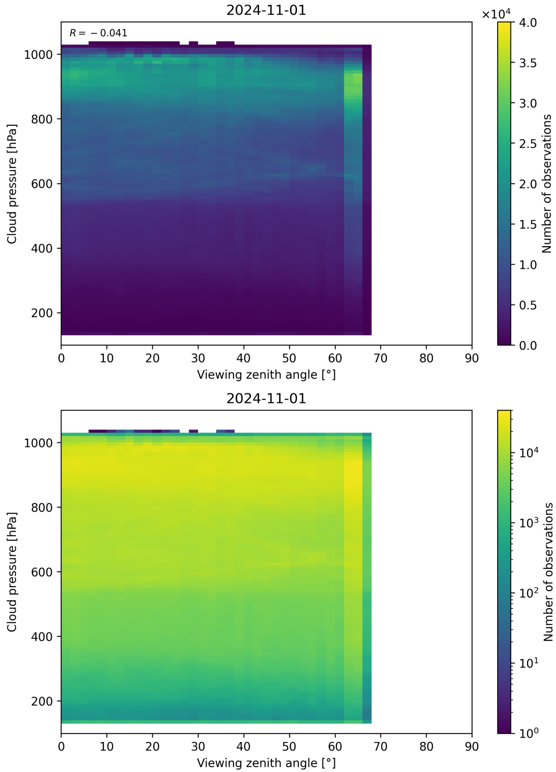
Figure 133: Scatter density plot of “Viewing zenith angle” against “Cloud pressure” for 2024-10-31 to 2024-11-02.
