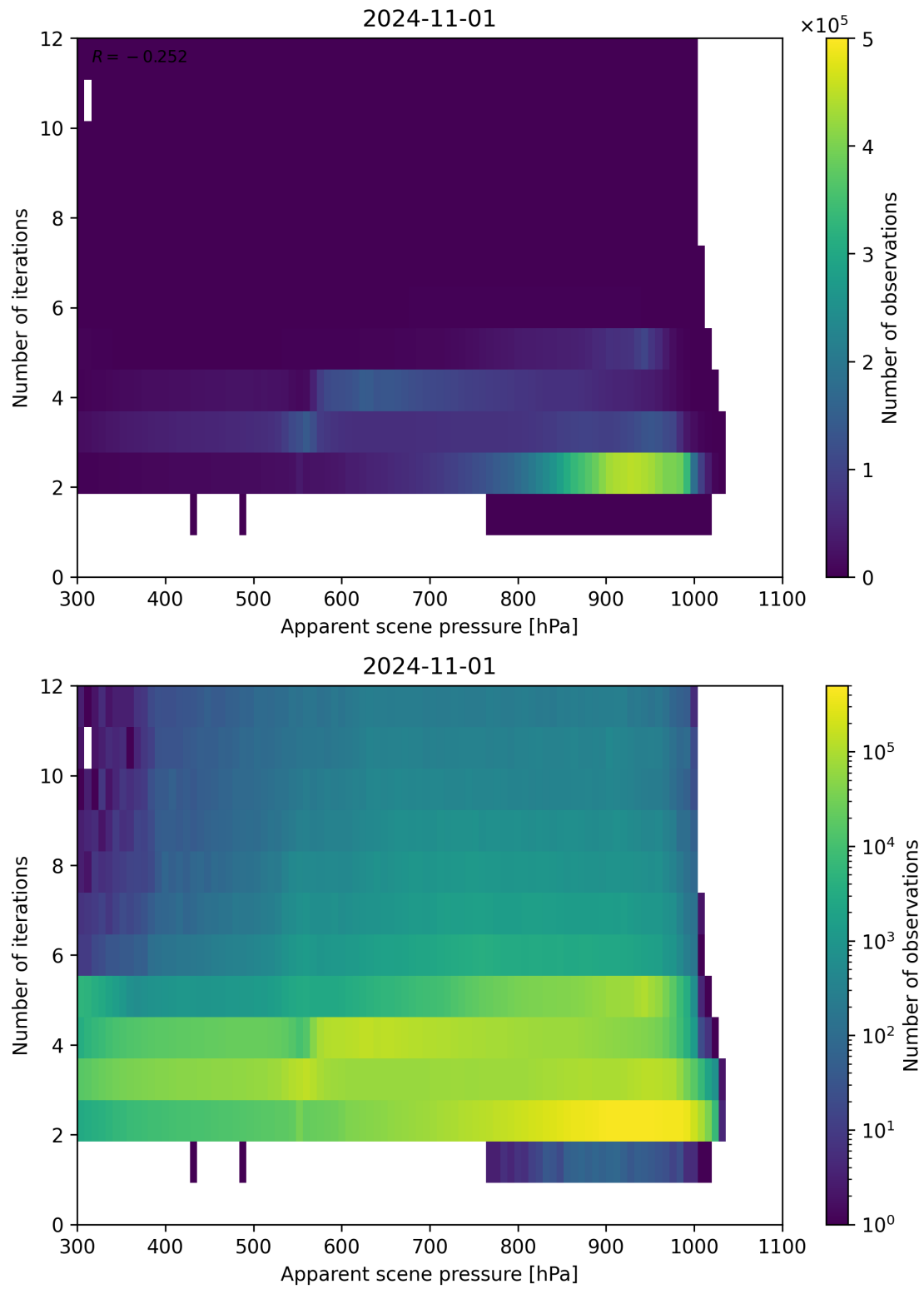
Figure 66: Scatter density plot of “Apparent scene pressure” against “Number of iterations” for 2024-10-31 to 2024-11-02.
