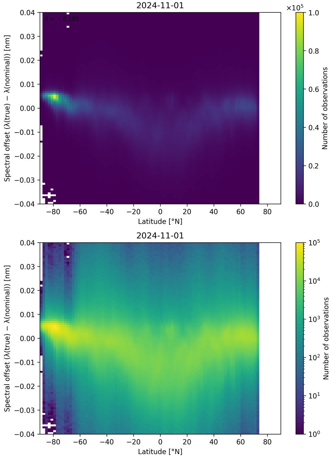
Figure 105: Scatter density plot of “Latitude” against “Spectral offset ( \lambda_{\text{true}} - \lambda_{\text{nominal}} )” for 2024-10-31 to 2024-11-02.
