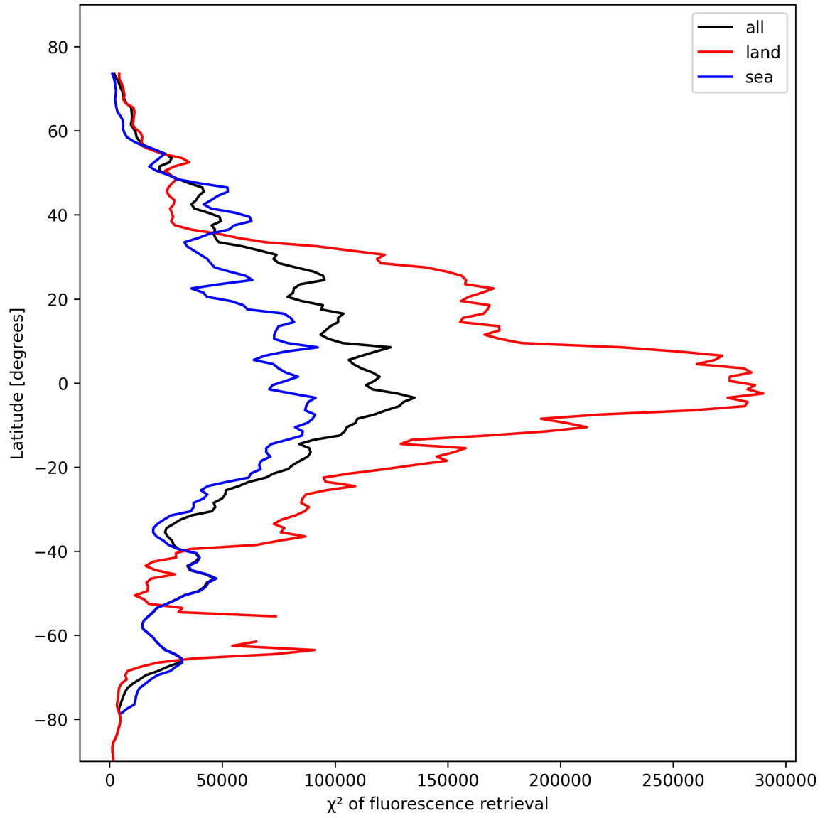
Figure 25: Zonal average of “ \chi^2 of fluorescence retrieval” for 2024-10-31 to 2024-11-02.
