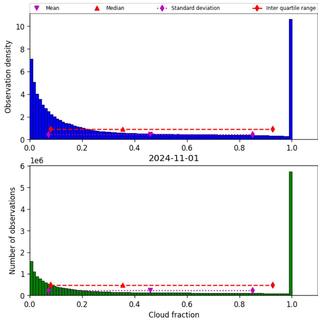
Figure 32: Histogram of “Cloud fraction” for 2024-10-31 to 2024-11-02
