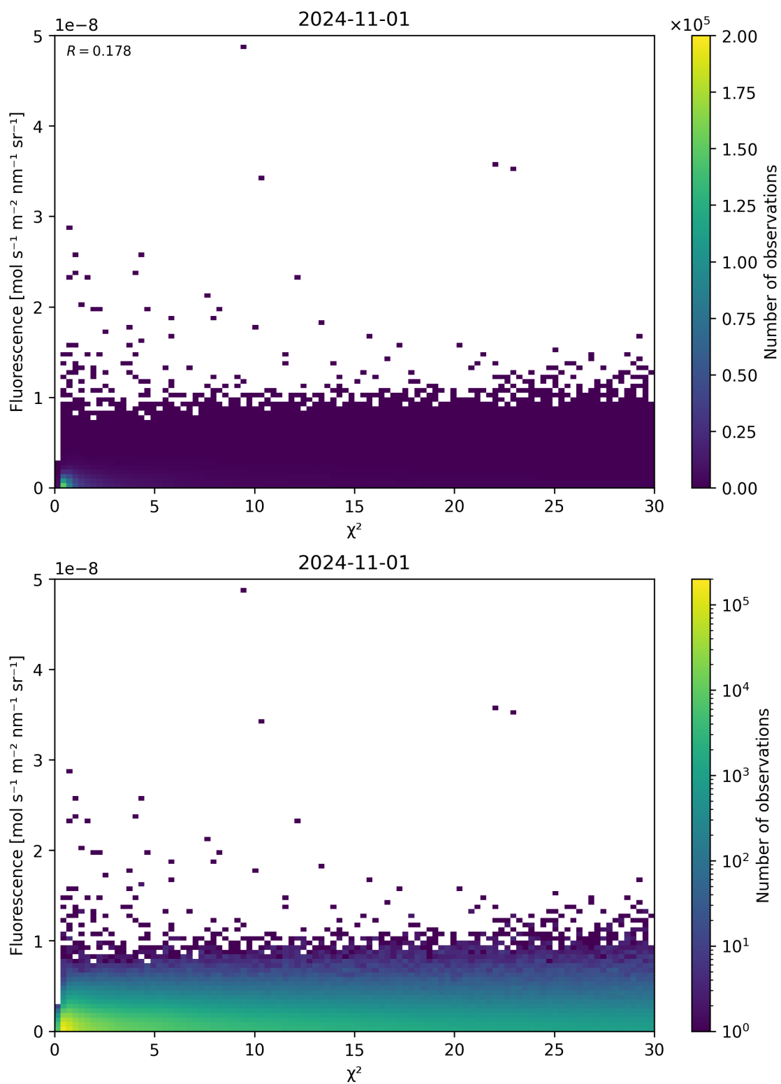
Figure 70: Scatter density plot of “ \chi^2 ” against “Fluorescence” for 2024-10-31 to 2024-11-02.
