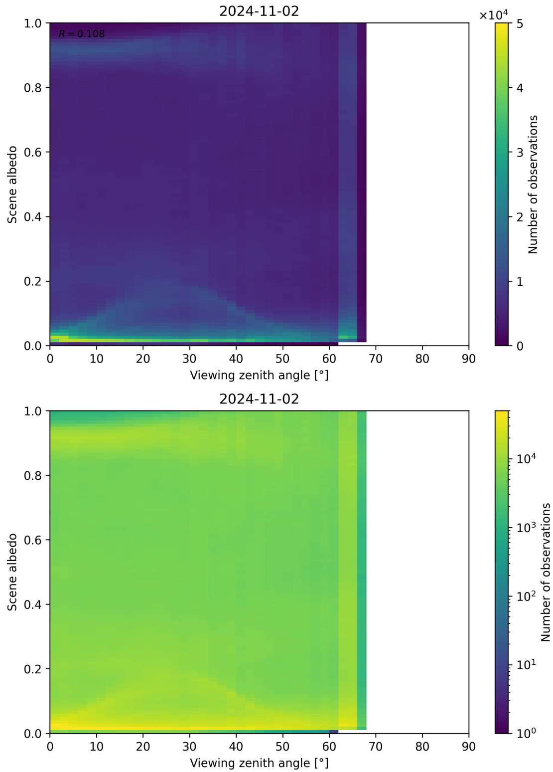
Figure 138: Scatter density plot of “Viewing zenith angle” against “Scene albedo” for 2024-11-01 to 2024-11-03.
