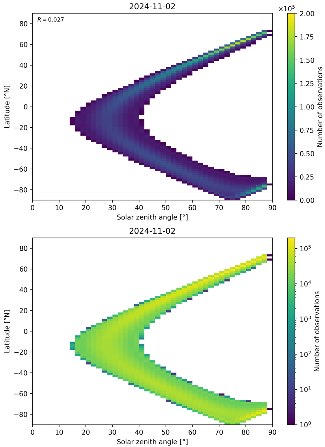
Figure 124: Scatter density plot of “Solar zenith angle” against “Latitude” for 2024-11-01 to 2024-11-03.
