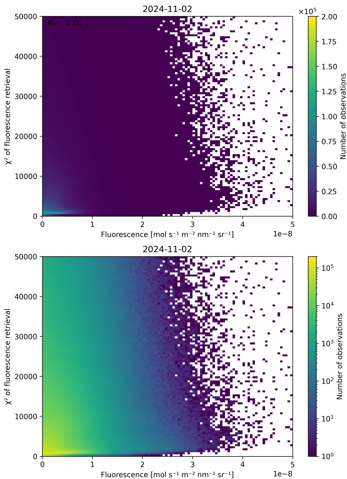
Figure 93: Scatter density plot of “Fluorescence” against “ \chi^2 of fluorescence retrieval” for 2024-11-01 to 2024-11-03.
