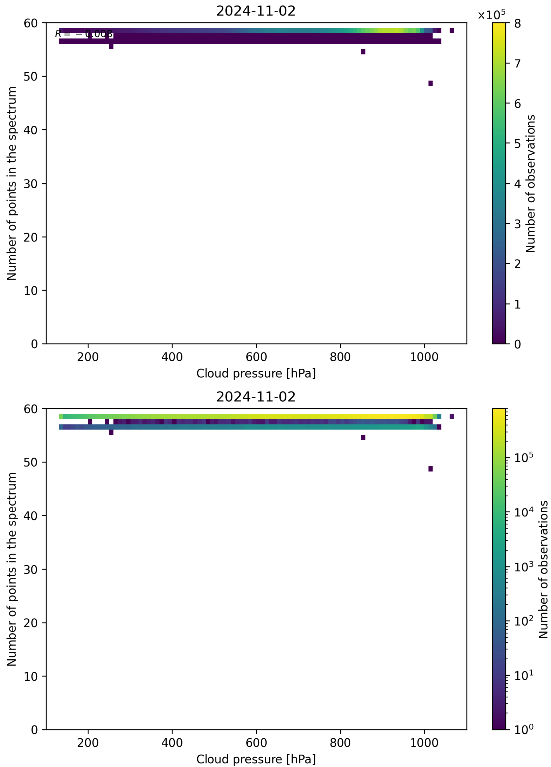
Figure 90: Scatter density plot of “Cloud pressure” against “Number of points in the spectrum” for 2024-11-01 to 2024-11-03.
