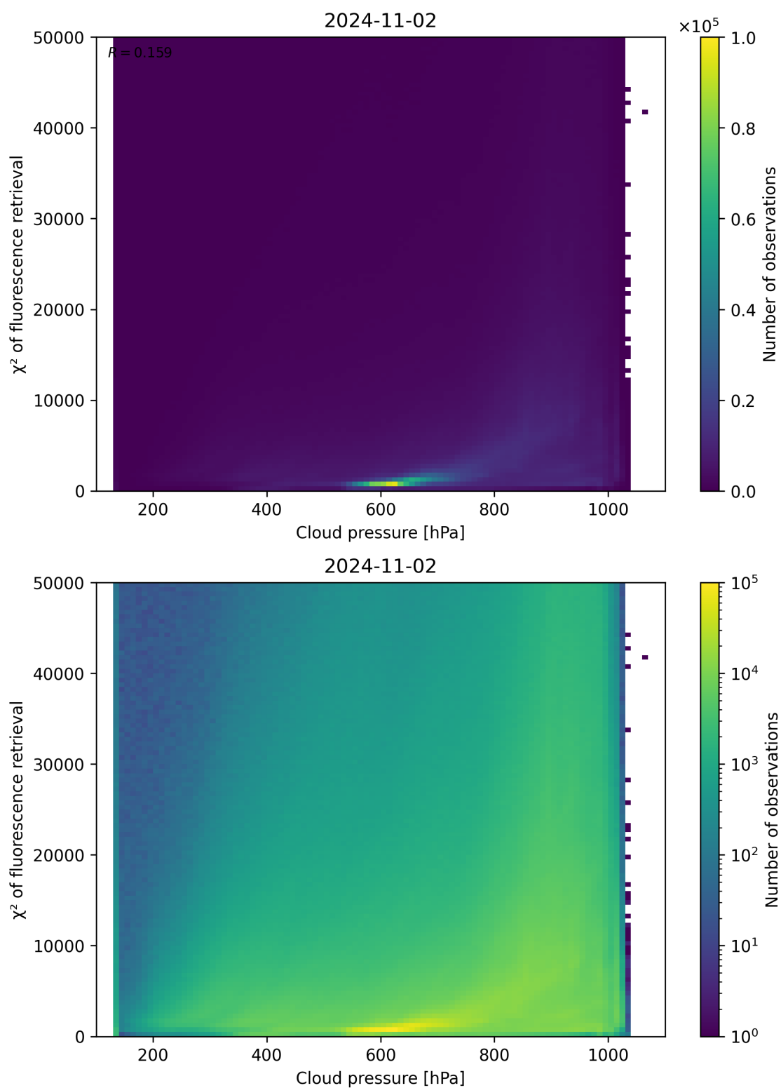
Figure 86: Scatter density plot of “Cloud pressure” against “ \chi^2 of fluorescence retrieval” for 2024-11-01 to 2024-11-03.
