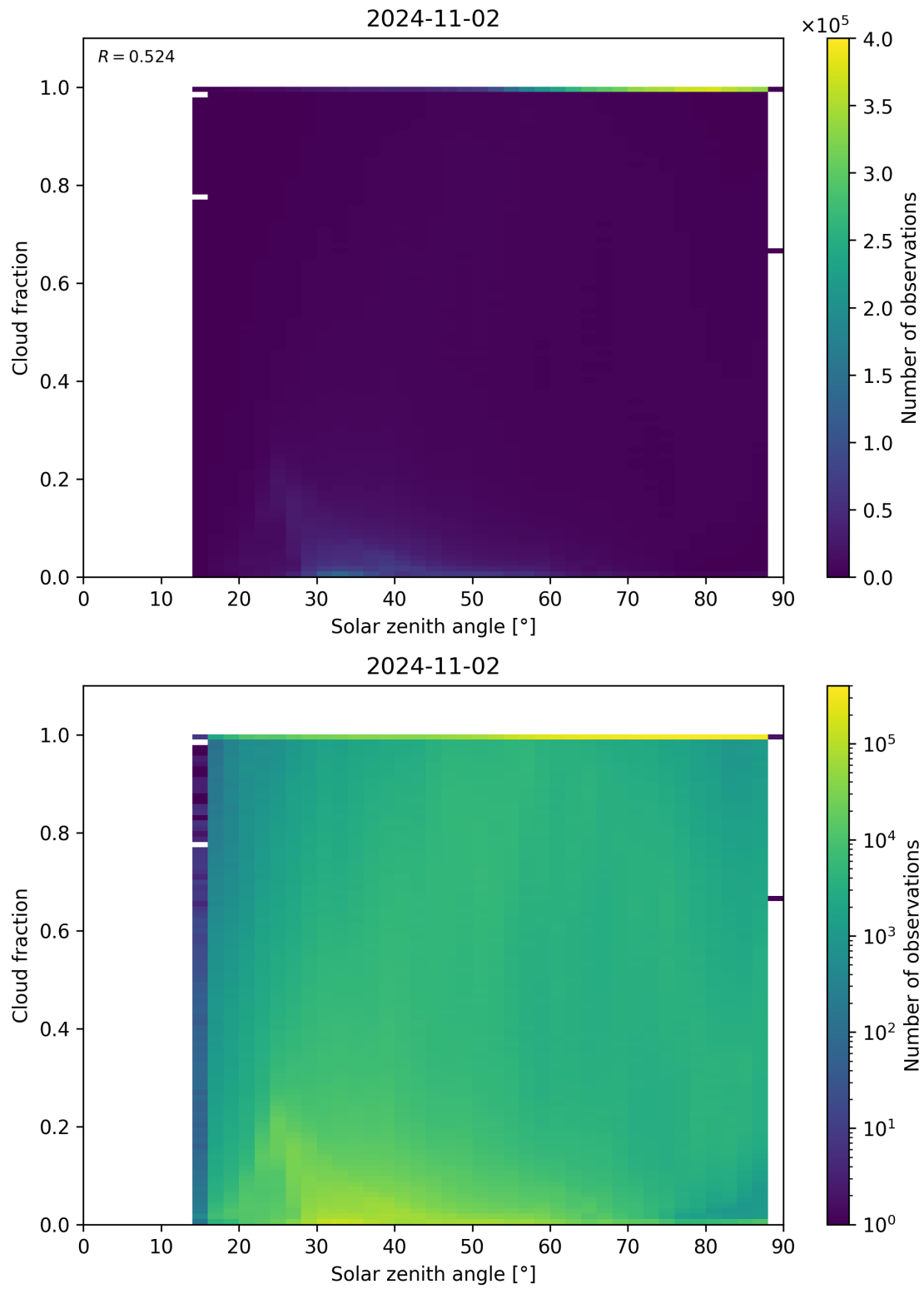
Figure 121: Scatter density plot of “Solar zenith angle” against “Cloud fraction” for 2024-11-01 to 2024-11-03.
