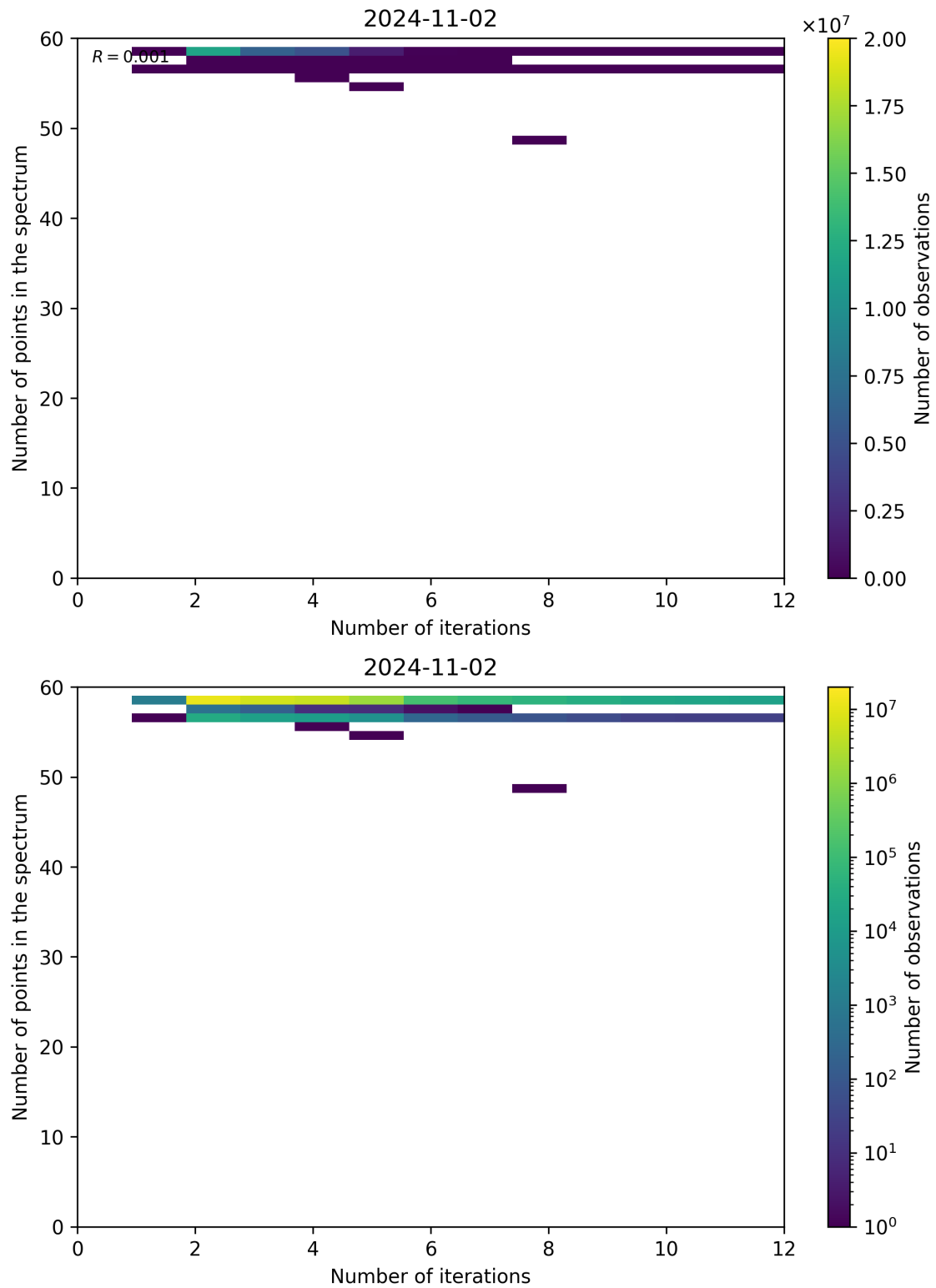
Figure 108: Scatter density plot of “Number of iterations” against “Number of points in the spectrum” for 2024-11-01 to 2024-11-03.
