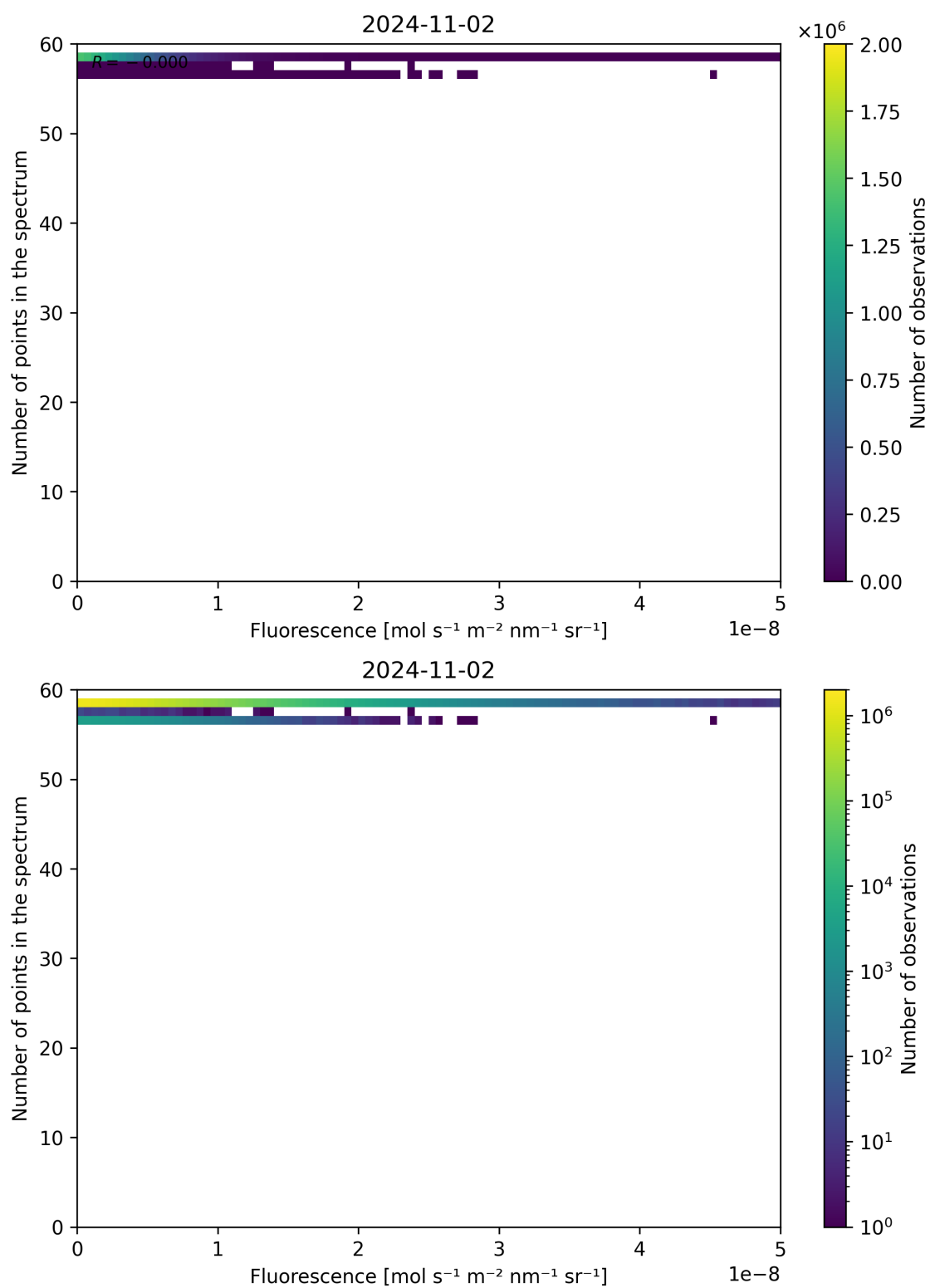
Figure 94: Scatter density plot of “Fluorescence” against “Number of points in the spectrum” for 2024-11-01 to 2024-11-03.
