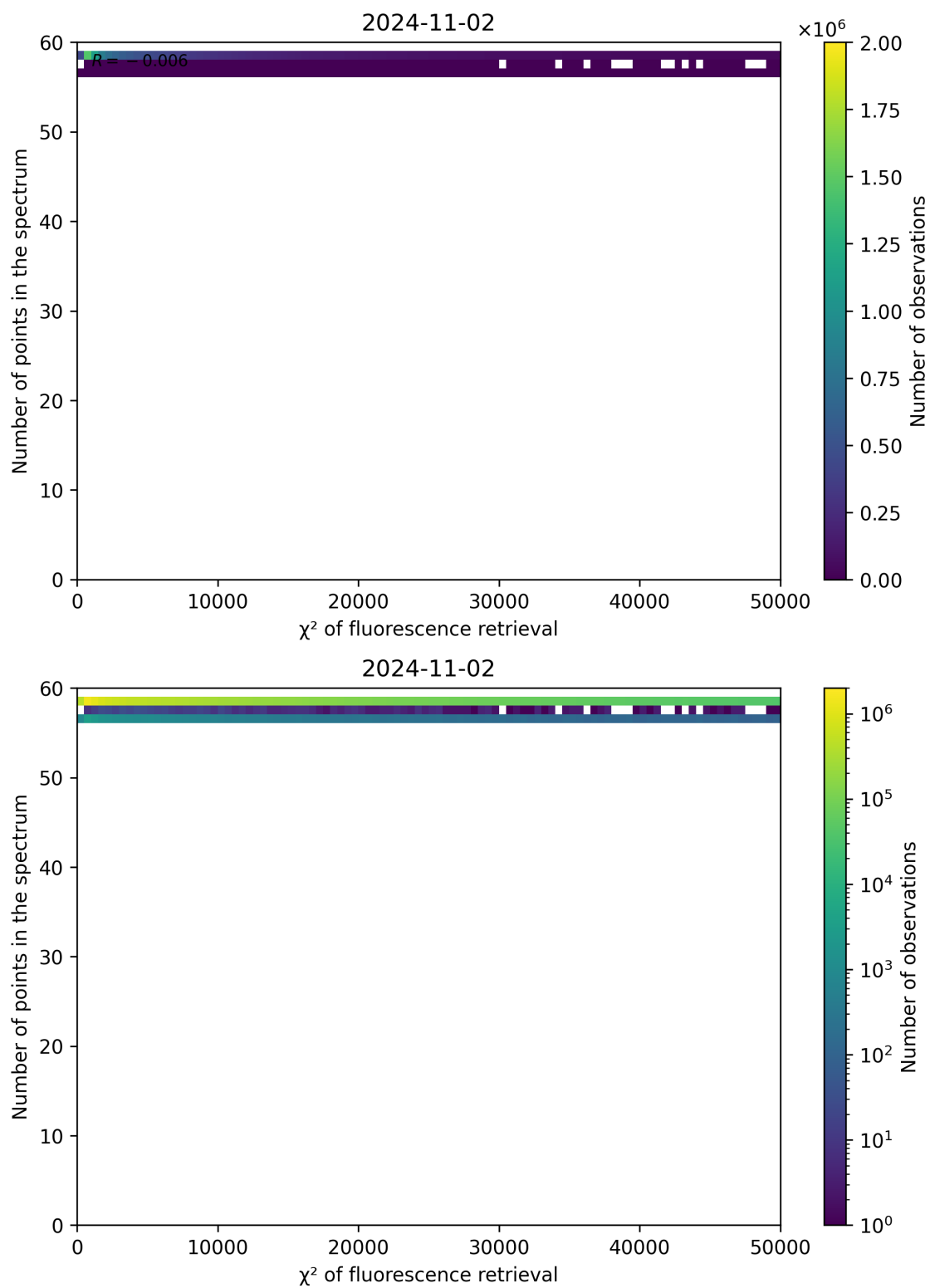
Figure 71: Scatter density plot of " \chi^2 of fluorescence retrieval" against "Number of points in the spectrum" for 2024-11-01 to 2024-11-03.
