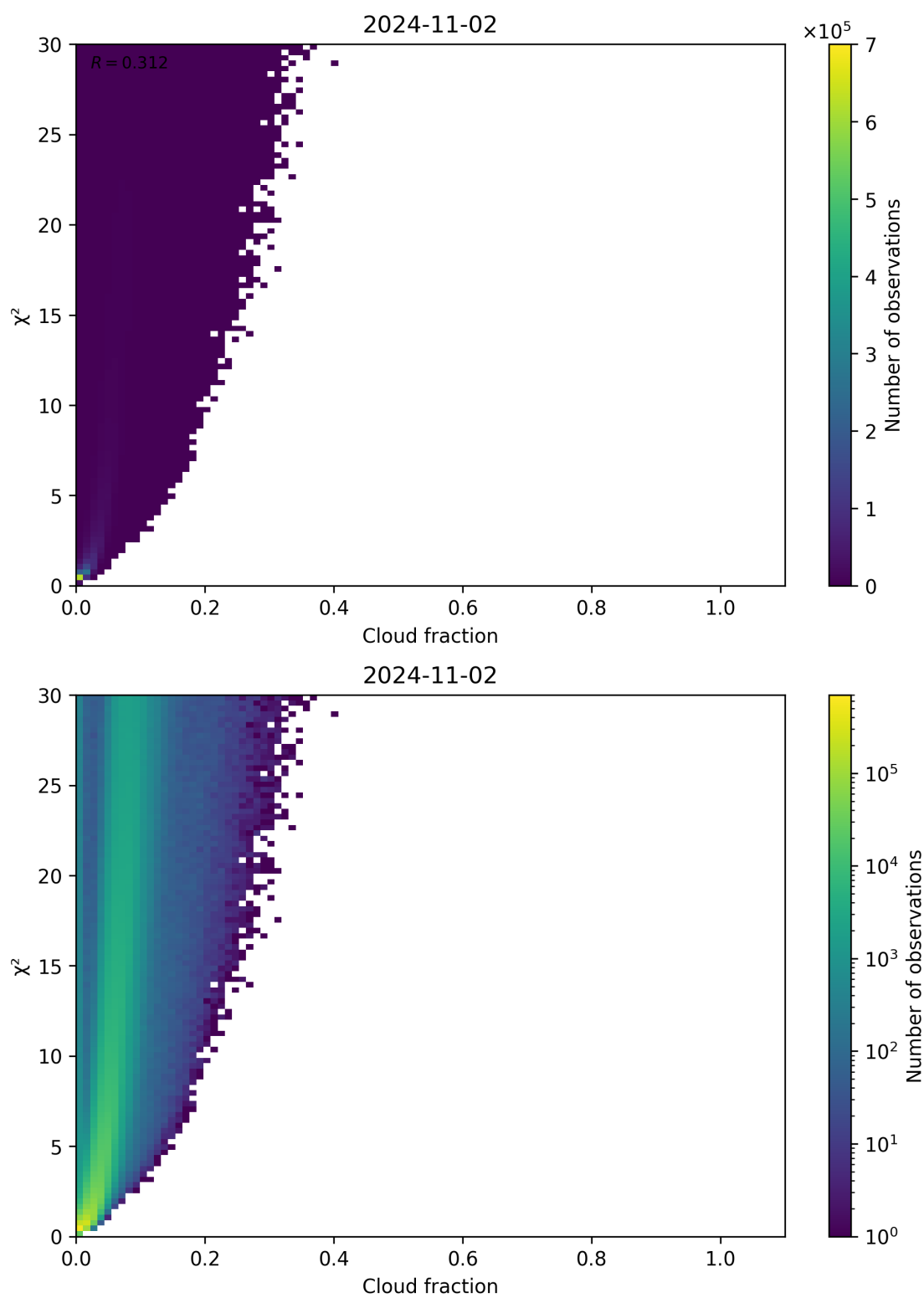
Figure 77: Scatter density plot of “Cloud fraction” against “ \chi^2 ” for 2024-11-01 to 2024-11-03.
