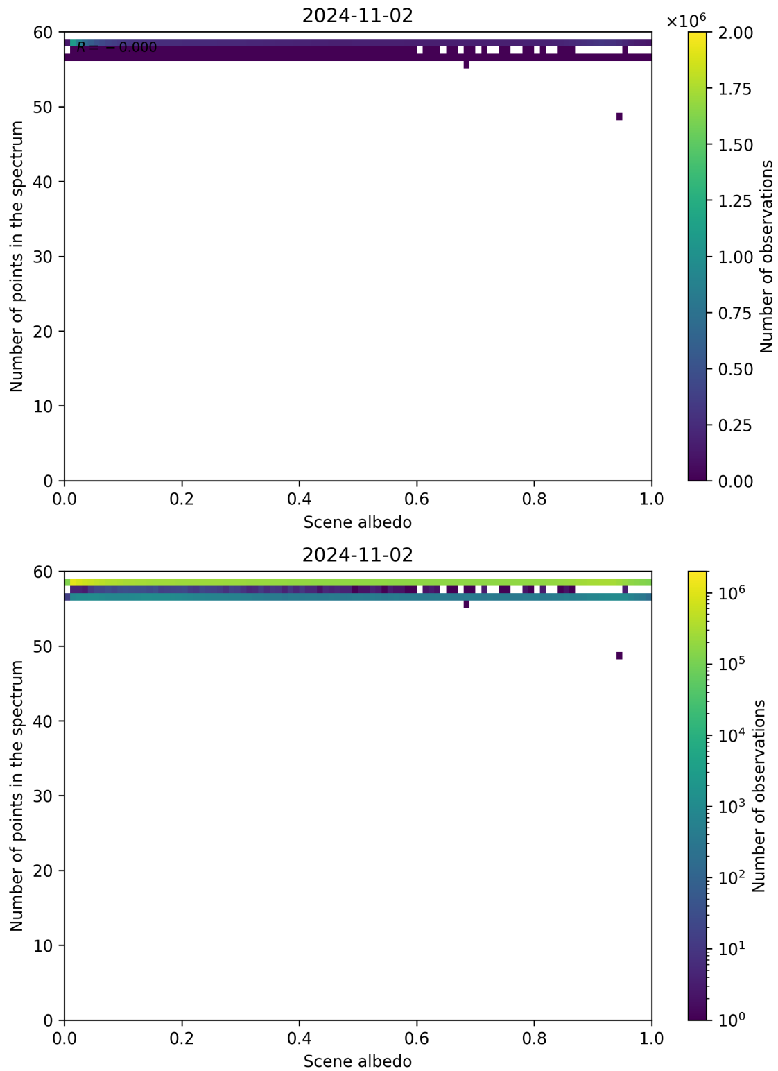
Figure 116: Scatter density plot of “Scene albedo” against “Number of points in the spectrum” for 2024-11-01 to 2024-11-03.
