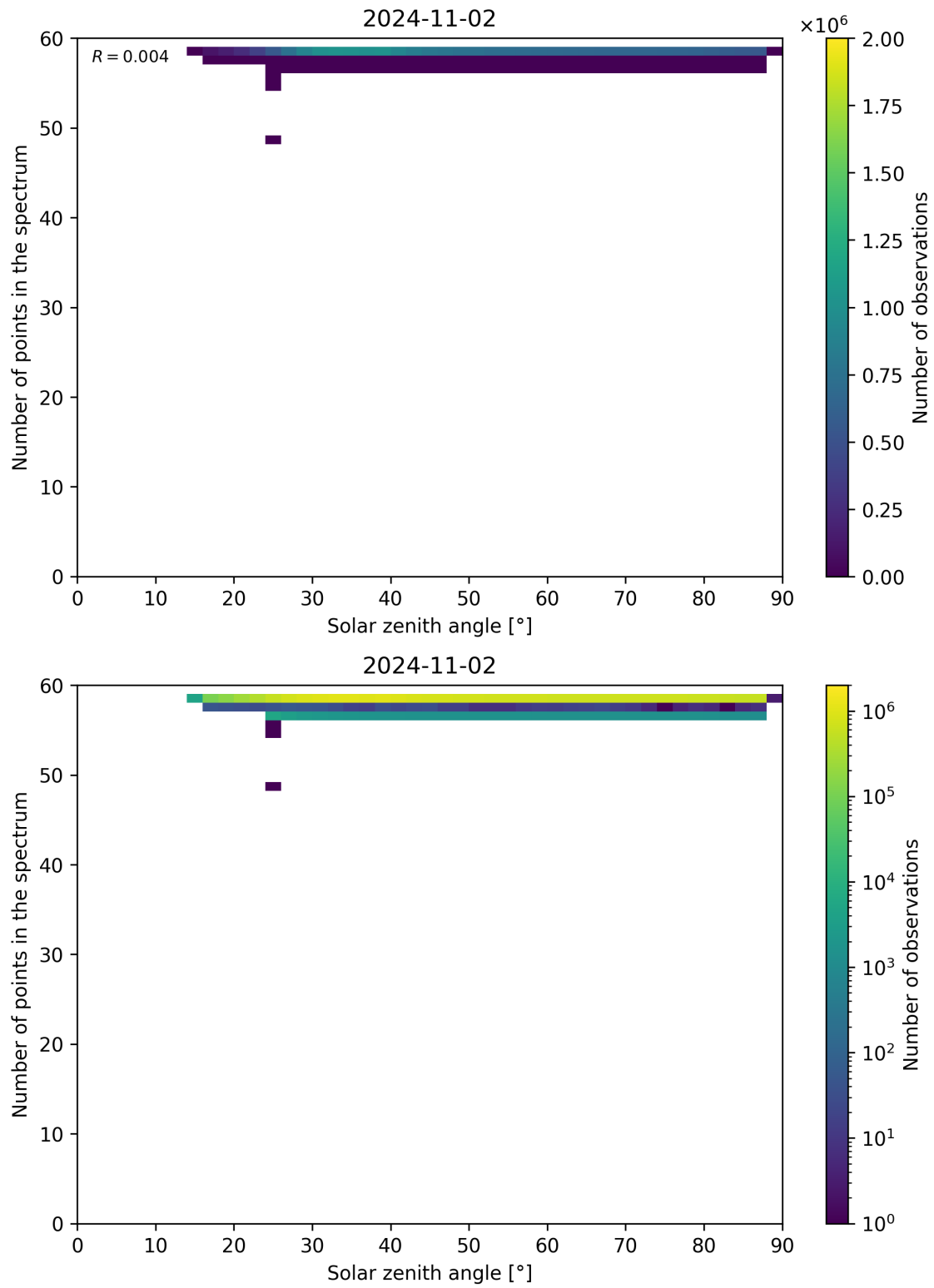
Figure 126: Scatter density plot of “Solar zenith angle” against “Number of points in the spectrum” for 2024-11-01 to 2024-11-03.
