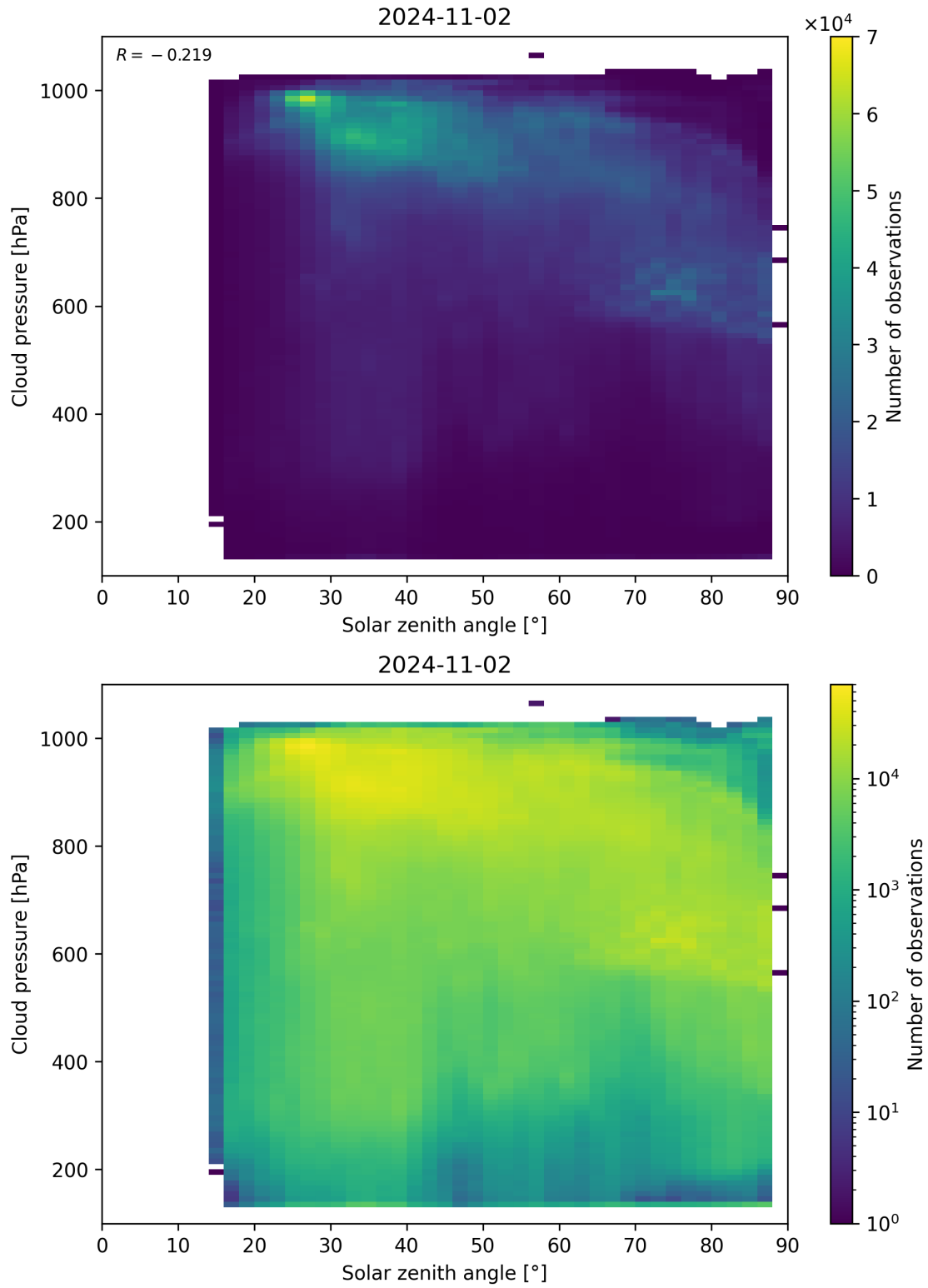
Figure 122: Scatter density plot of “Solar zenith angle” against “Cloud pressure” for 2024-11-01 to 2024-11-03.
