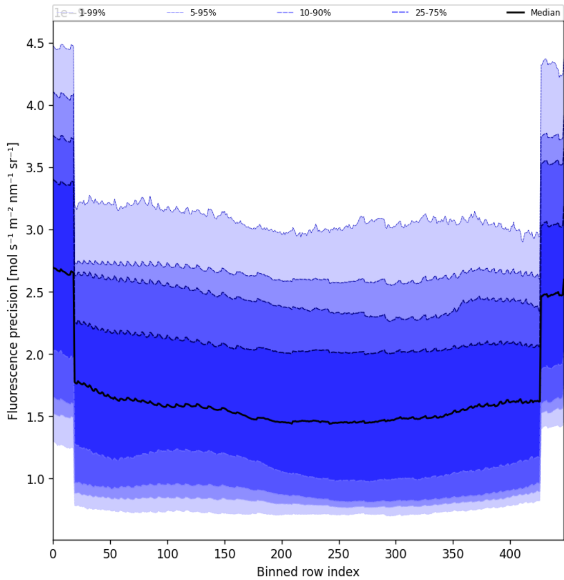
Figure 58: Along track statistics of "Fluorescence precision" for 2024-11-01 to 2024-11-03
