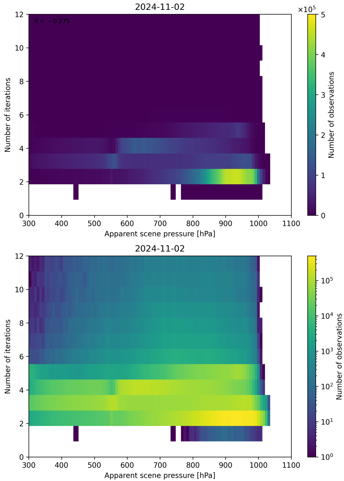
Figure 66: Scatter density plot of “Apparent scene pressure” against “Number of iterations” for 2024-11-01 to 2024-11-03.
