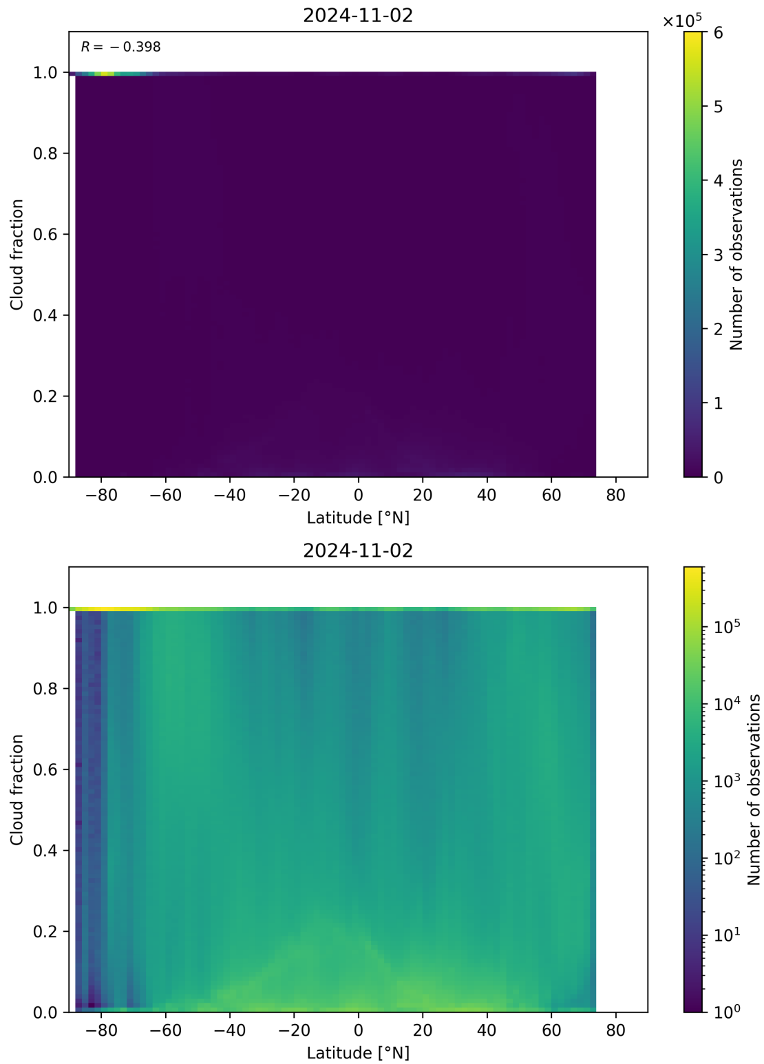
Figure 99: Scatter density plot of “Latitude” against “Cloud fraction” for 2024-11-01 to 2024-11-03.
