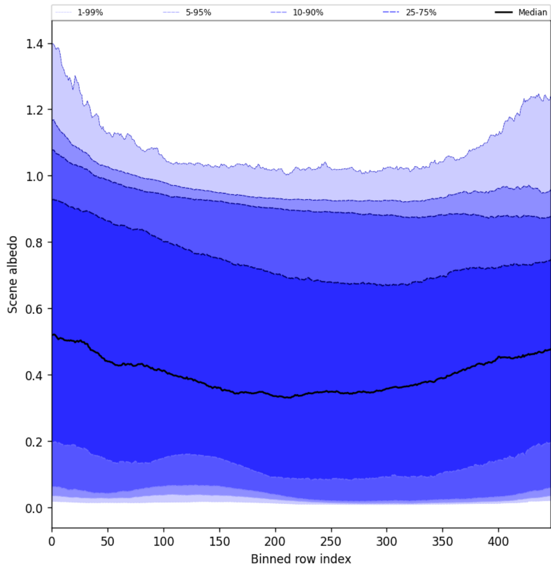
Figure 51: Along track statistics of “Scene albedo” for 2024-11-01 to 2024-11-03
