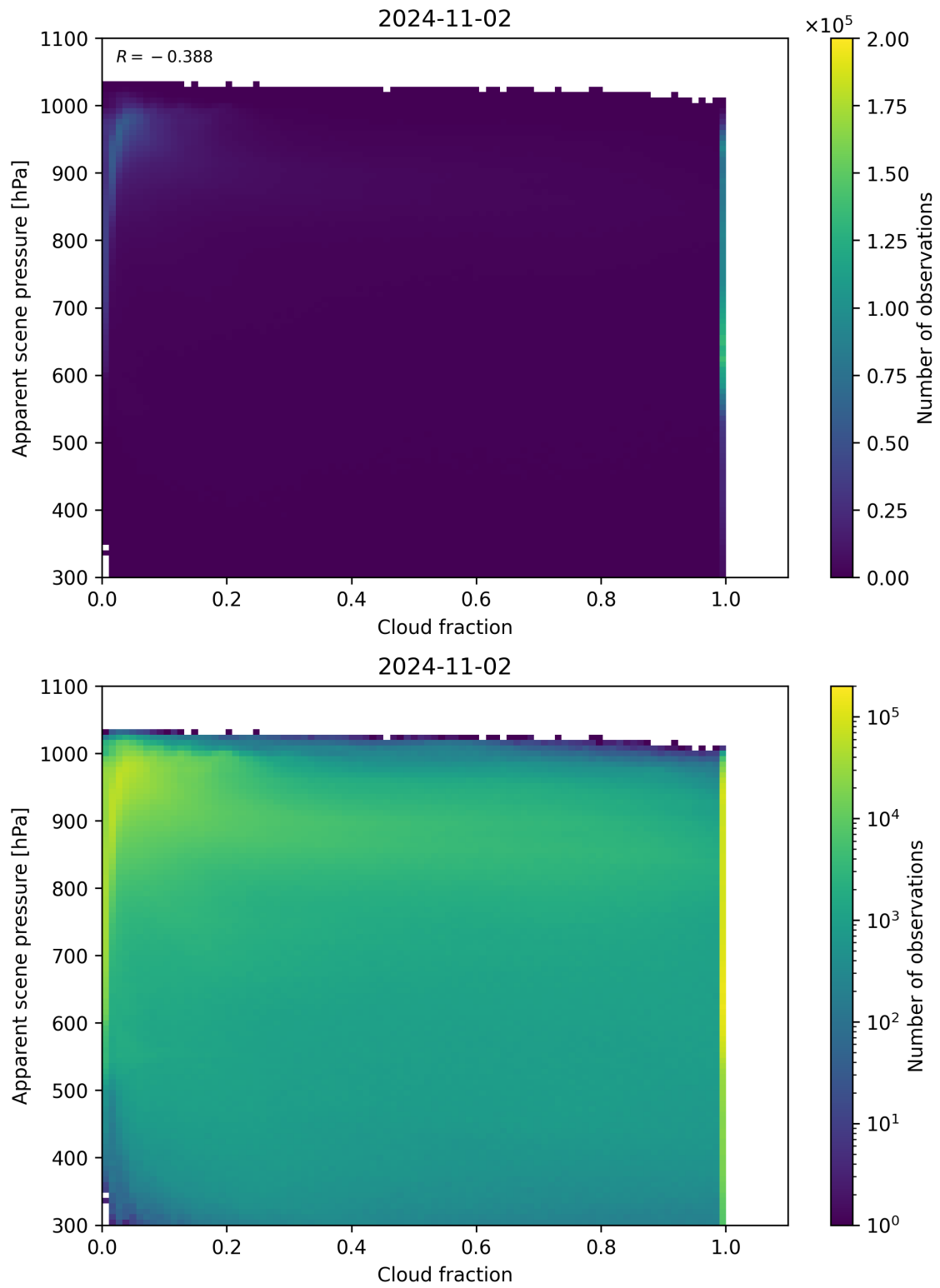
Figure 76: Scatter density plot of “Cloud fraction” against “Apparent scene pressure” for 2024-11-01 to 2024-11-03.
