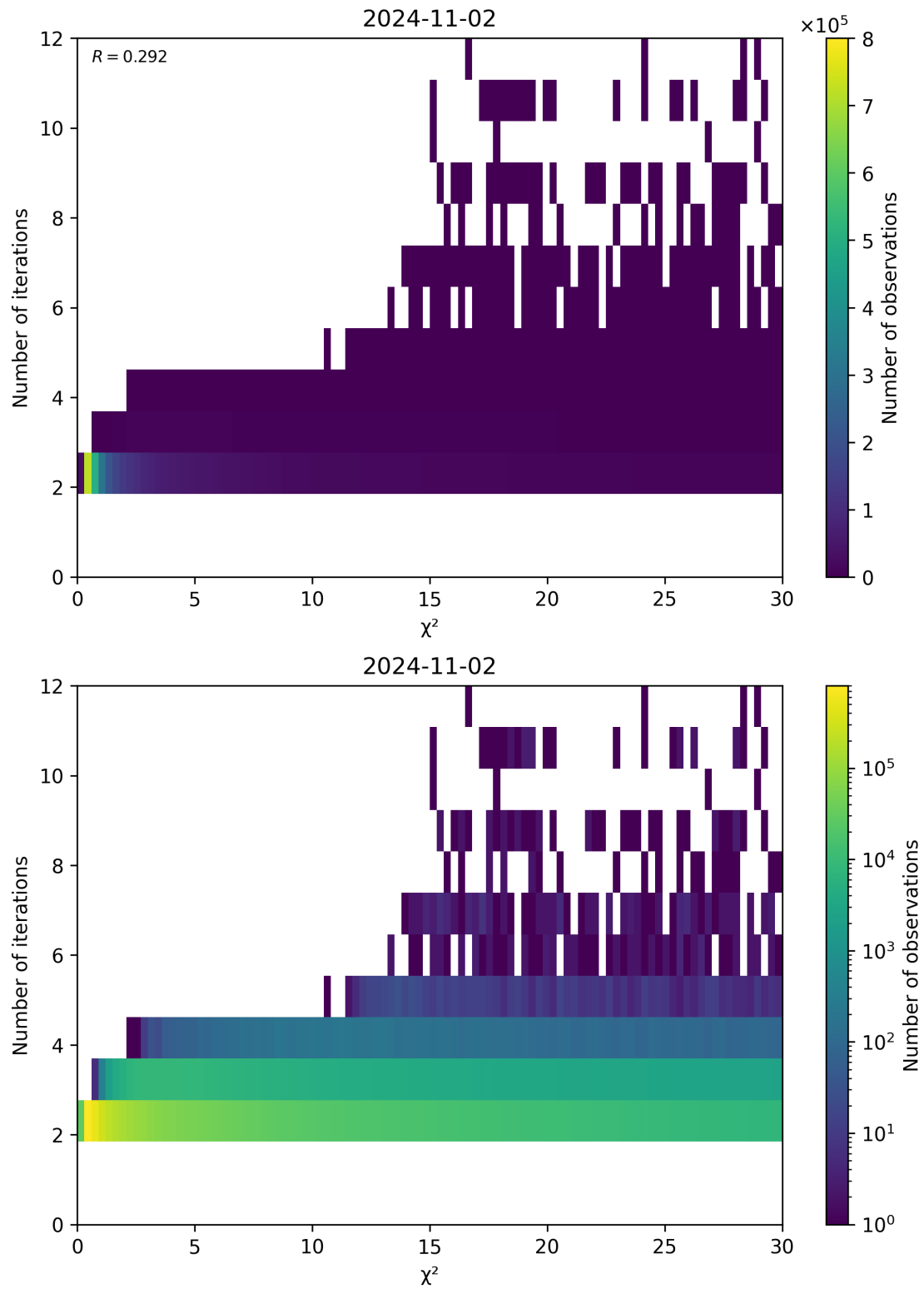
Figure 73: Scatter density plot of “ \chi^2 ” against “Number of iterations” for 2024-11-01 to 2024-11-03.
