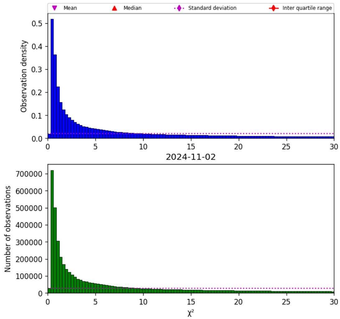
Figure 38: Histogram of “ \chi^2 ” for 2024-11-01 to 2024-11-03
