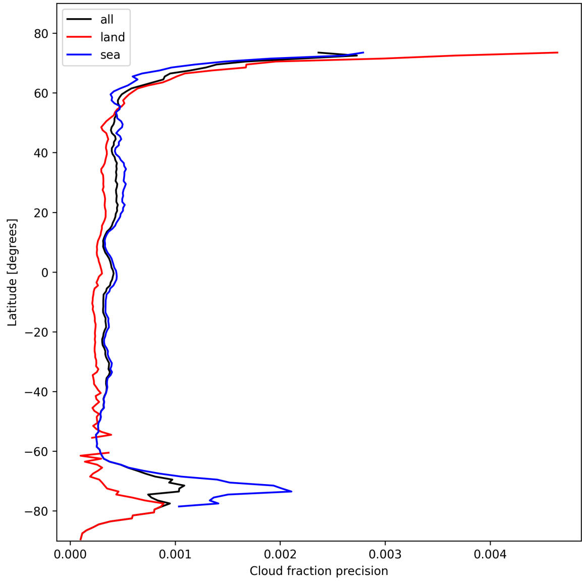
Figure 16: Zonal average of “Cloud fraction precision” for 2024-11-01 to 2024-11-03.
