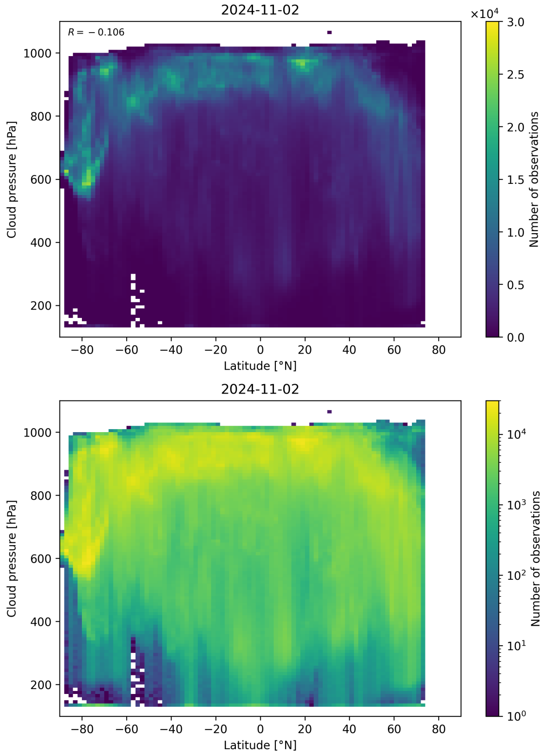
Figure 100: Scatter density plot of “Latitude” against “Cloud pressure” for 2024-11-01 to 2024-11-03.
