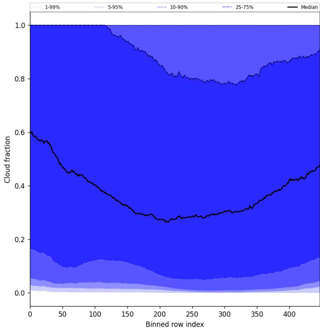
Figure 49: Along track statistics of “Cloud fraction” for 2024-11-01 to 2024-11-03
