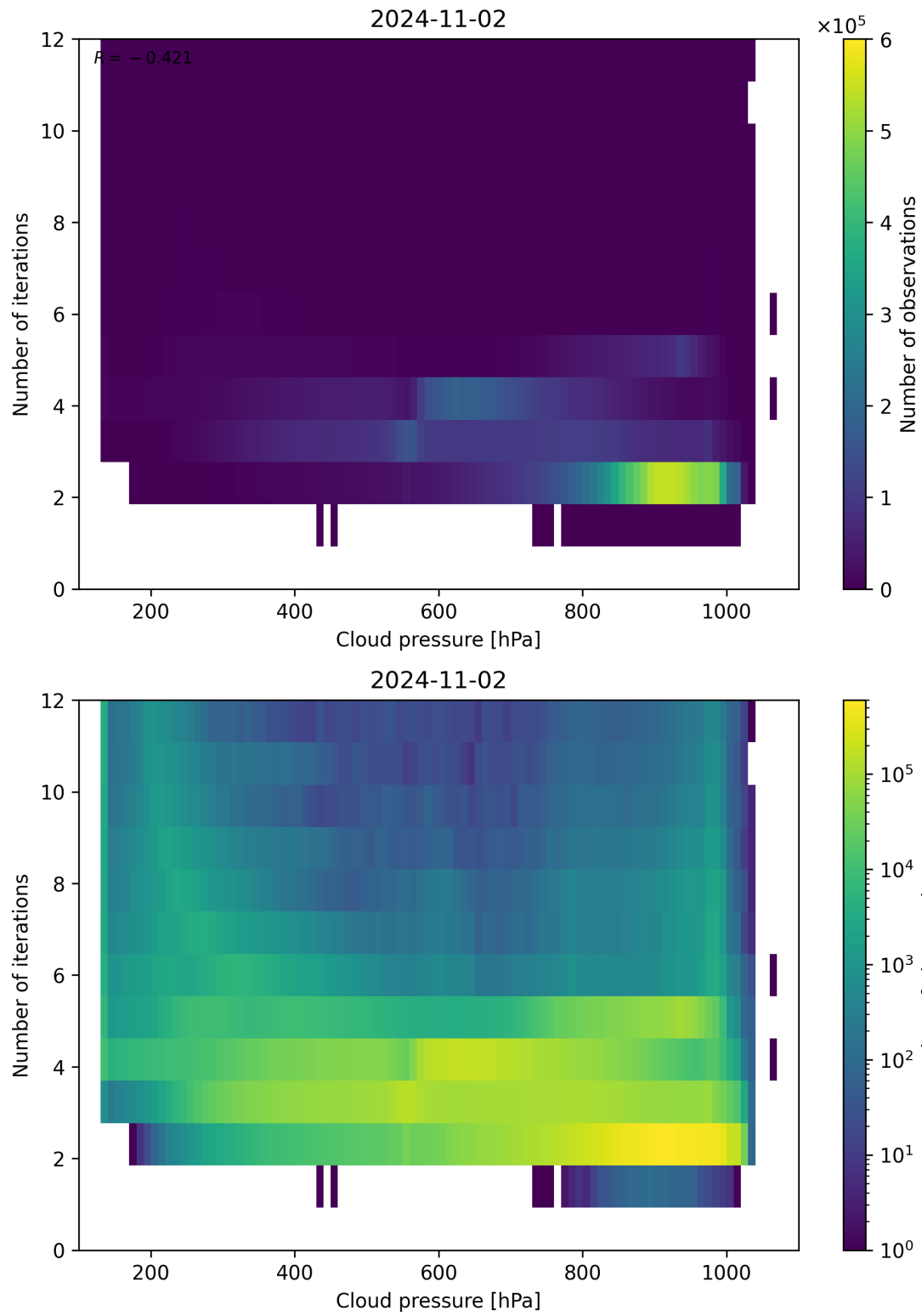
Figure 89: Scatter density plot of “Cloud pressure” against “Number of iterations” for 2024-11-01 to 2024-11-03.
