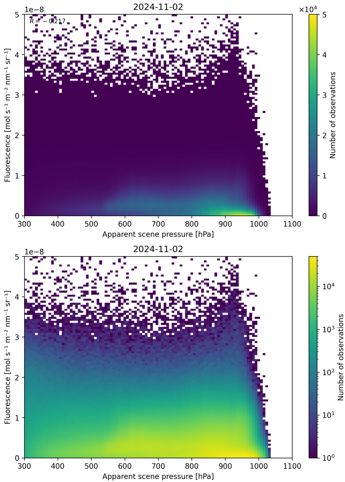
Figure 65: Scatter density plot of “Apparent scene pressure” against “Fluorescence” for 2024-11-01 to 2024-11-03.
