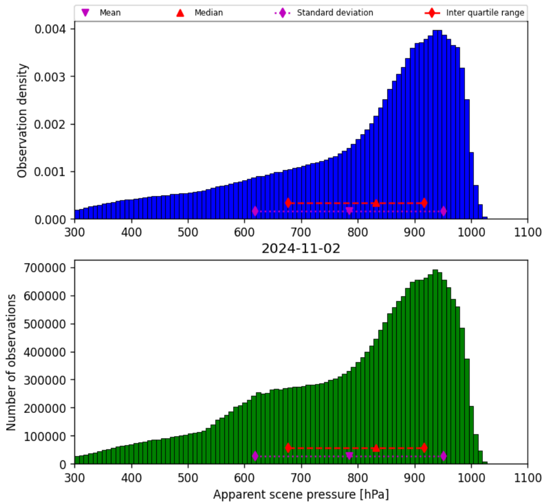
Figure 36: Histogram of “Apparent scene pressure” for 2024-11-01 to 2024-11-03
