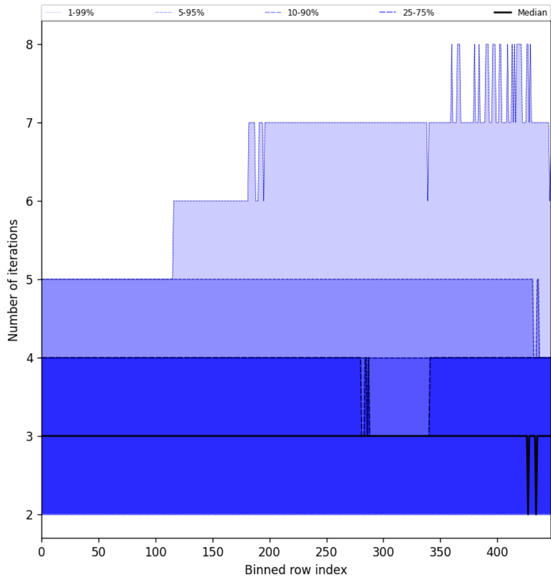
Figure 56: Along track statistics of “Number of iterations” for 2024-11-01 to 2024-11-03
