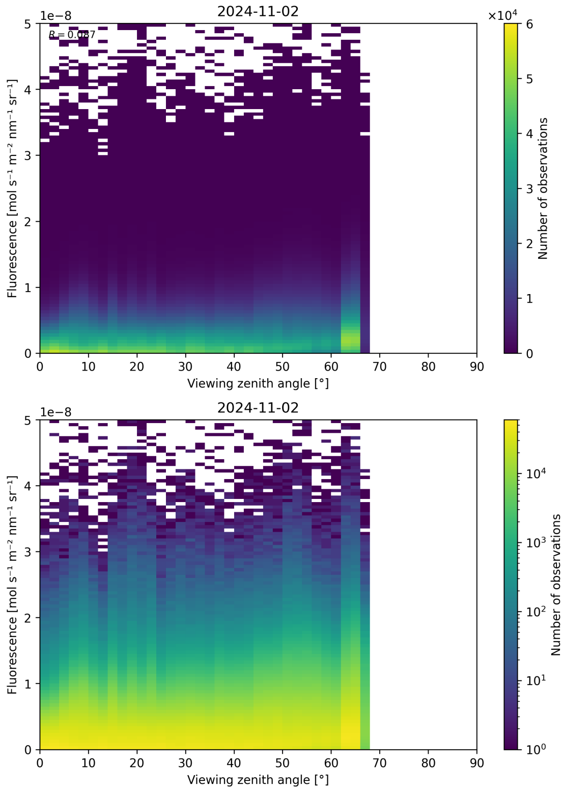
Figure 134: Scatter density plot of “Viewing zenith angle” against “Fluorescence” for 2024-11-01 to 2024-11-03.
