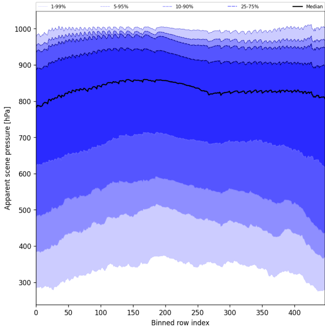
Figure 53: Along track statistics of “Apparent scene pressure” for 2024-11-01 to 2024-11-03
