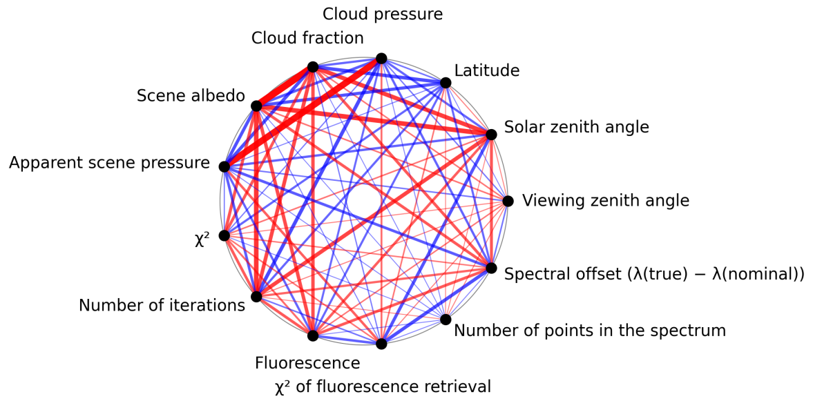
Figure 1: Map of correlation graph for 2024-11-01 to 2024-11-03.
