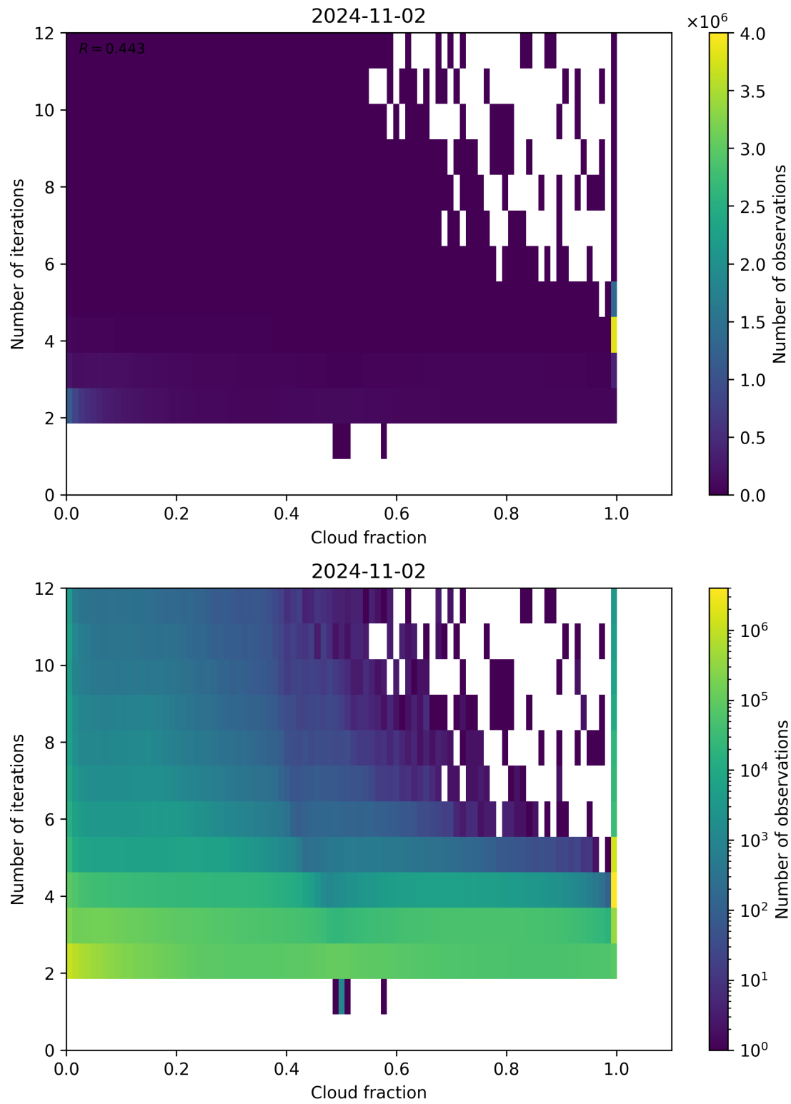
Figure 80: Scatter density plot of “Cloud fraction” against “Number of iterations” for 2024-11-01 to 2024-11-03.
