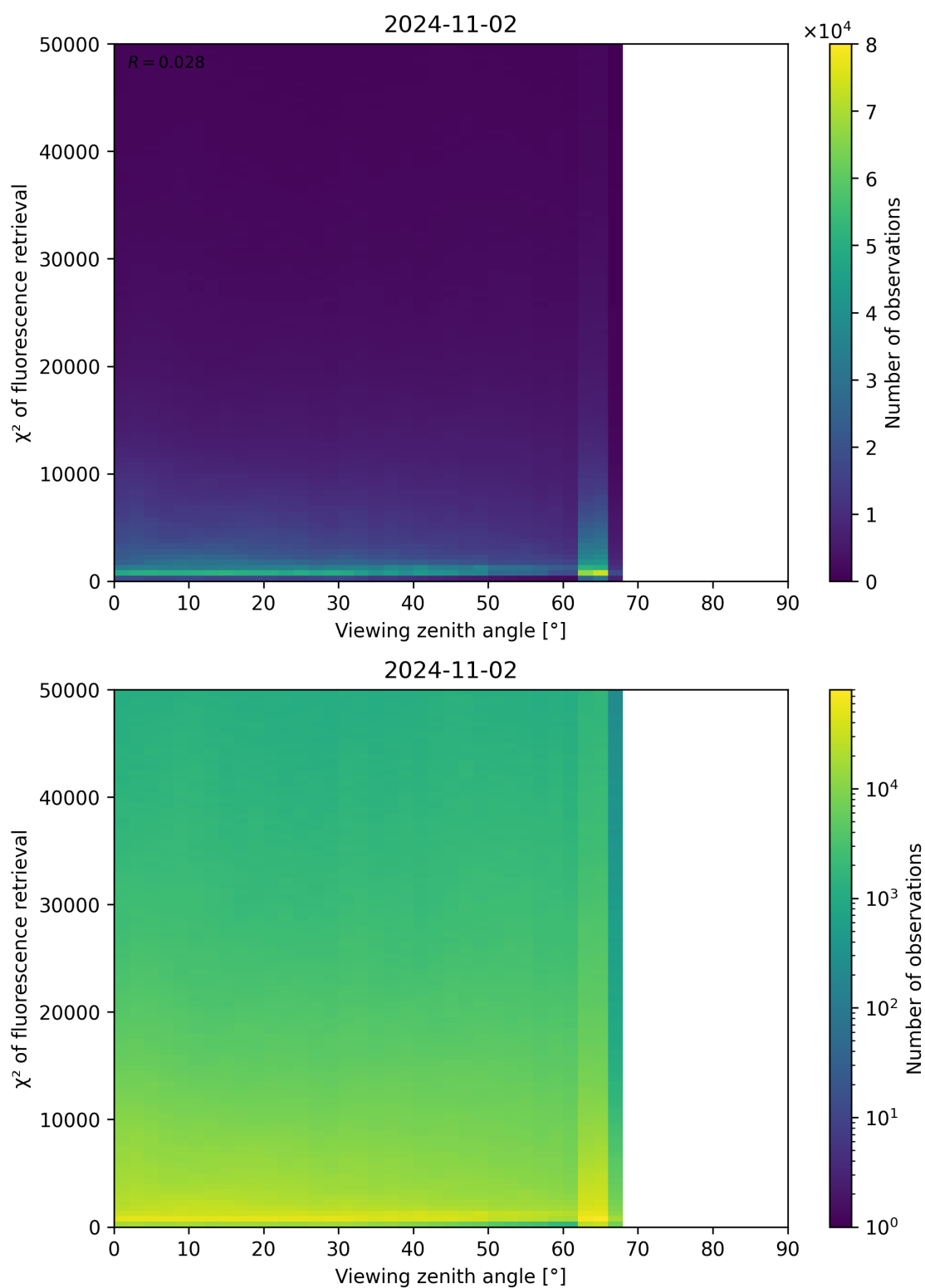
Figure 131: Scatter density plot of “Viewing zenith angle” against “ \chi^2 of fluorescence retrieval” for 2024-11-01 to 2024-11-03.
