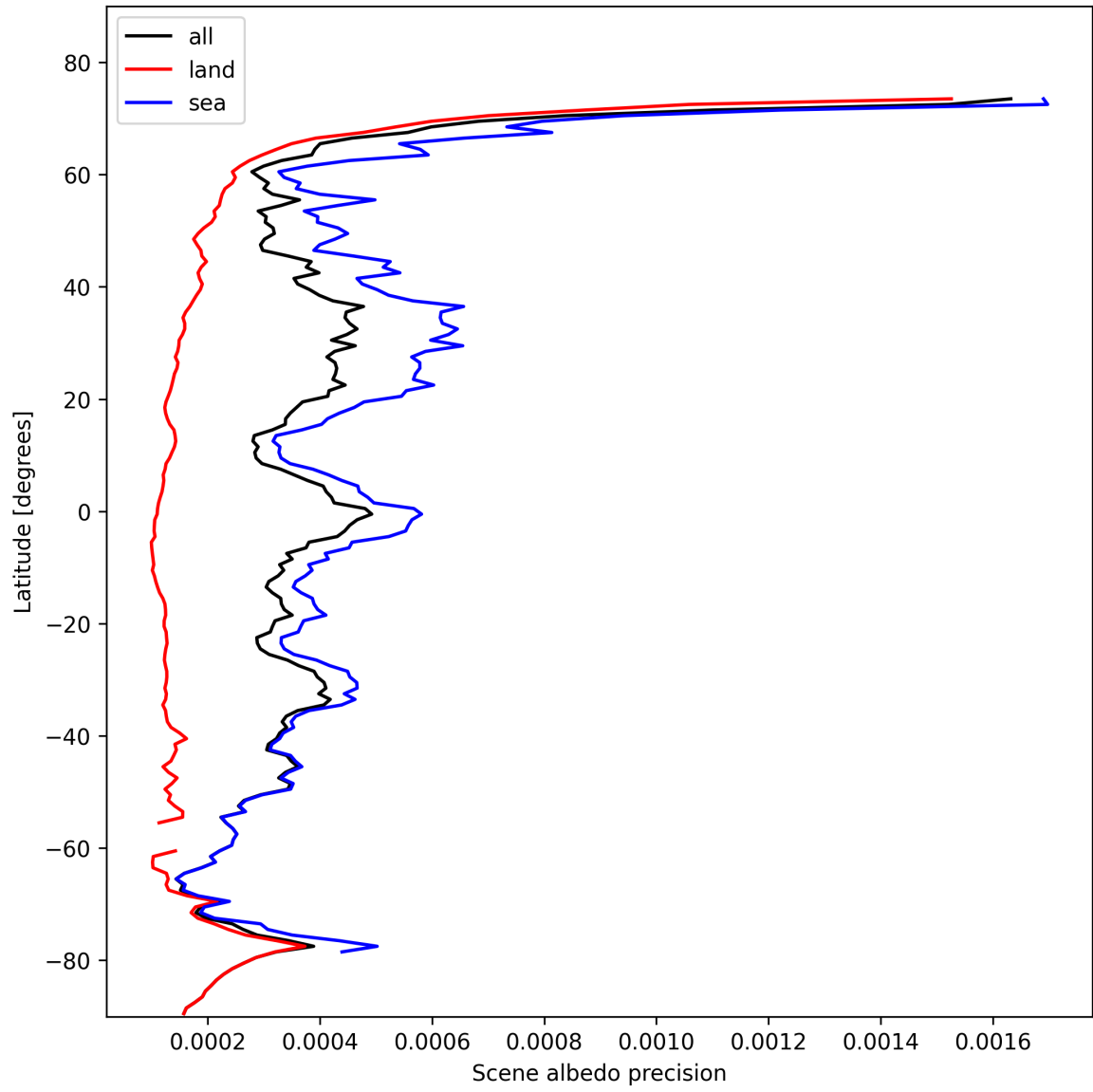
Figure 18: Zonal average of "Scene albedo precision" for 2024-11-01 to 2024-11-03.
