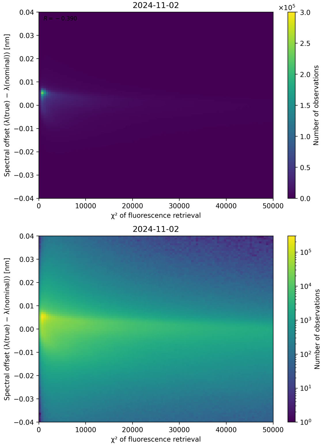
Figure 72: Scatter density plot of “ \chi^2 of fluorescence retrieval” against “Spectral offset ( \lambda_{\text{true}} - \lambda_{\text{nominal}} )” for 2024-11-01 to 2024-11-03.
