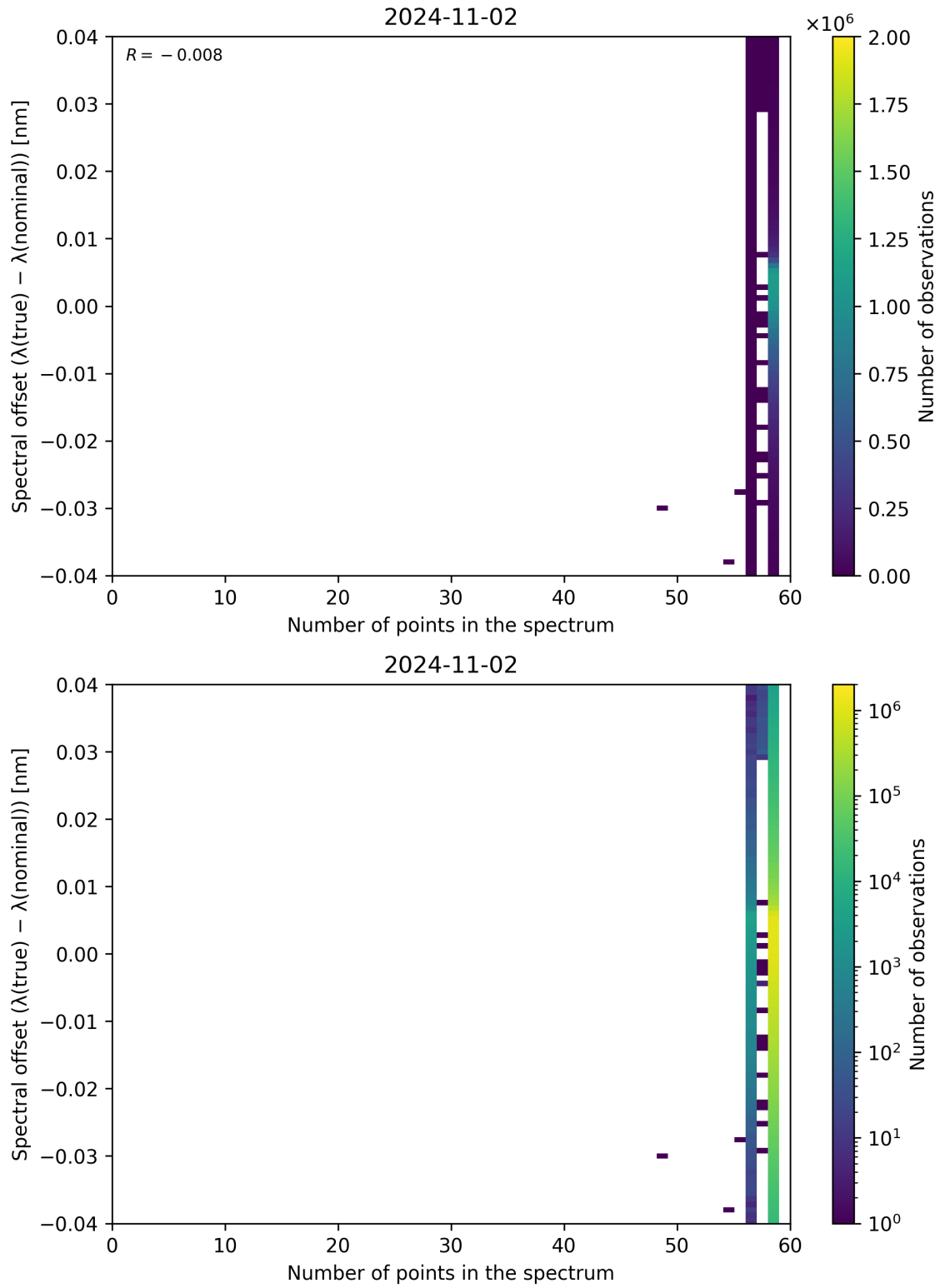
Figure 110: Scatter density plot of “Number of points in the spectrum” against “Spectral offset ( \lambda_{\text{true}} - \lambda_{\text{nominal}} )” for 2024-11-01 to 2024-11-03.
