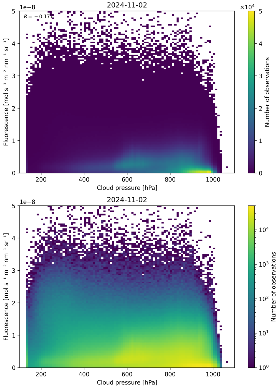
Figure 88: Scatter density plot of “Cloud pressure” against “Fluorescence” for 2024-11-01 to 2024-11-03.
