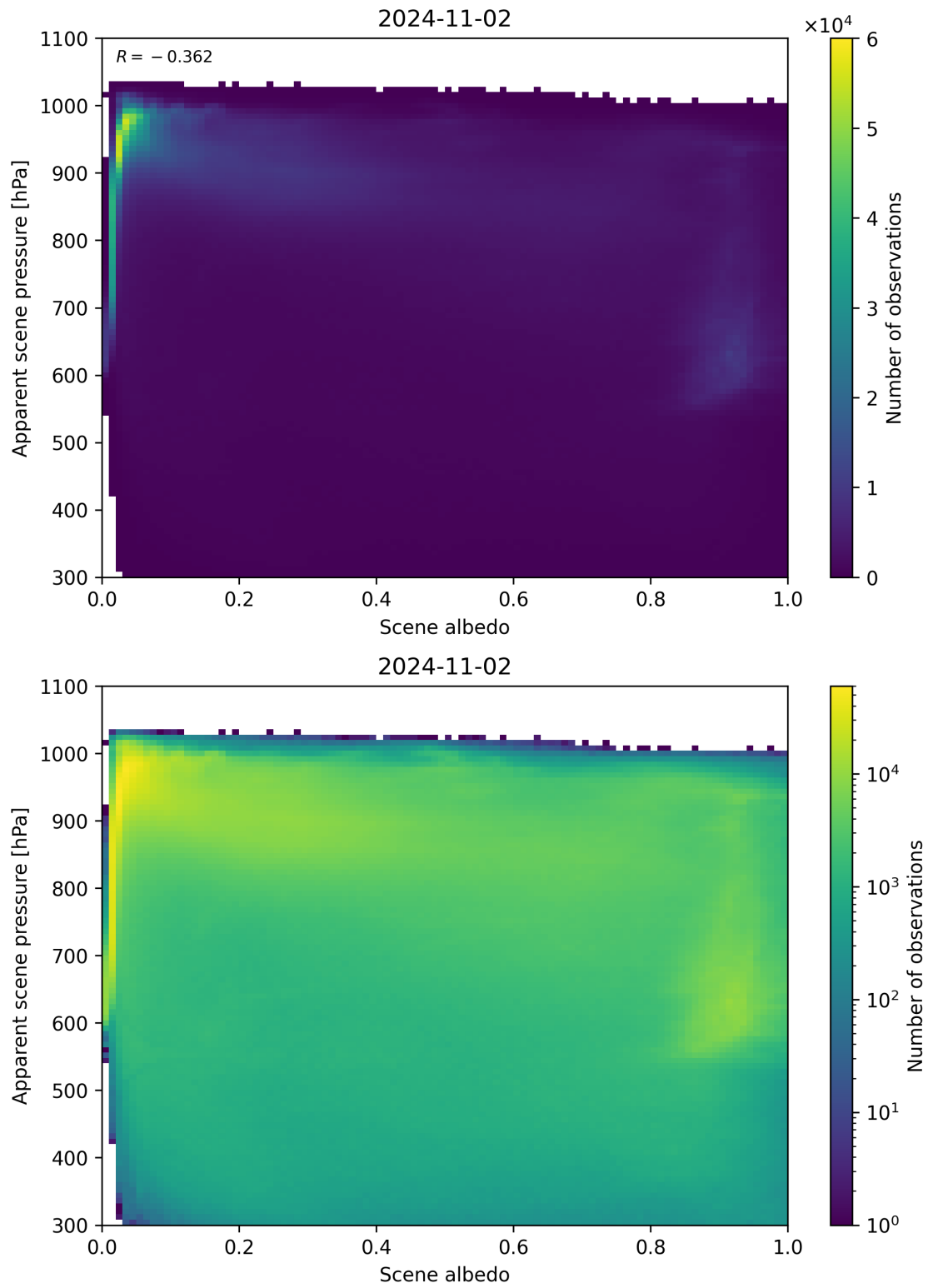
Figure 111: Scatter density plot of “Scene albedo” against “Apparent scene pressure” for 2024-11-01 to 2024-11-03.
