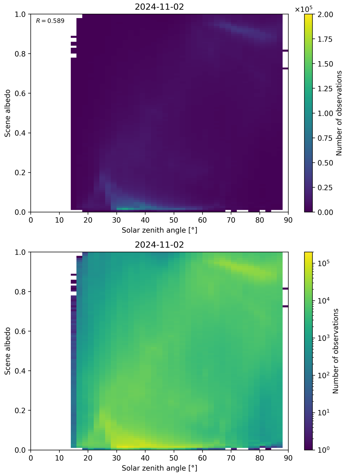
Figure 127: Scatter density plot of “Solar zenith angle” against “Scene albedo” for 2024-11-01 to 2024-11-03.
