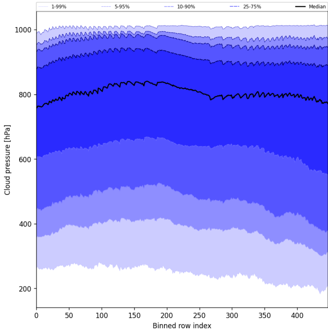
Figure 47: Along track statistics of “Cloud pressure” for 2024-11-01 to 2024-11-03
