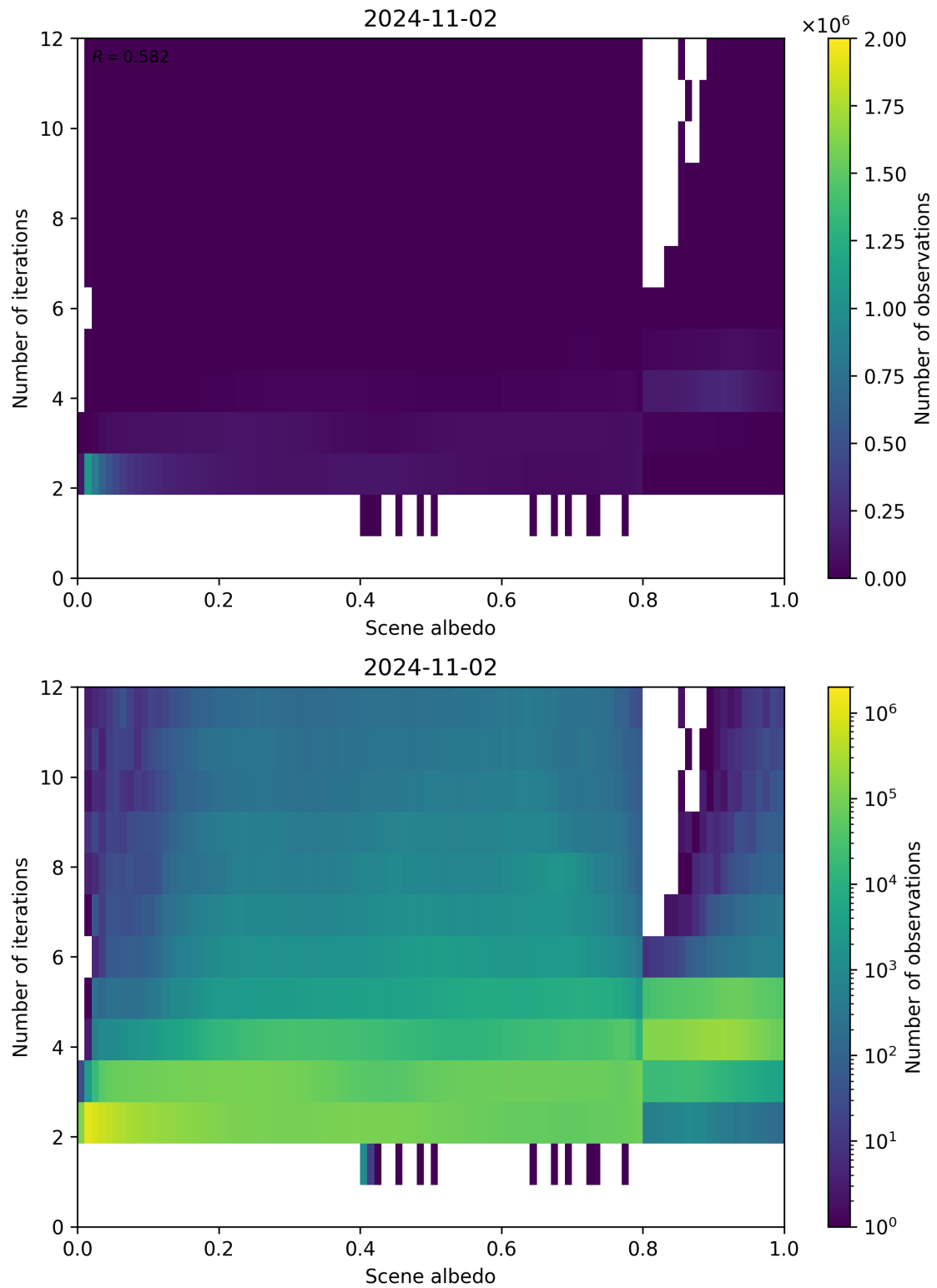
Figure 115: Scatter density plot of “Scene albedo” against “Number of iterations” for 2024-11-01 to 2024-11-03.
