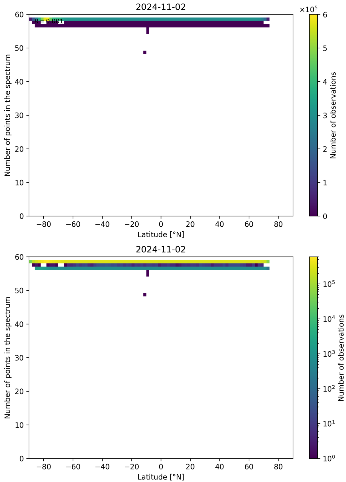
Figure 103: Scatter density plot of “Latitude” against “Number of points in the spectrum” for 2024-11-01 to 2024-11-03.
