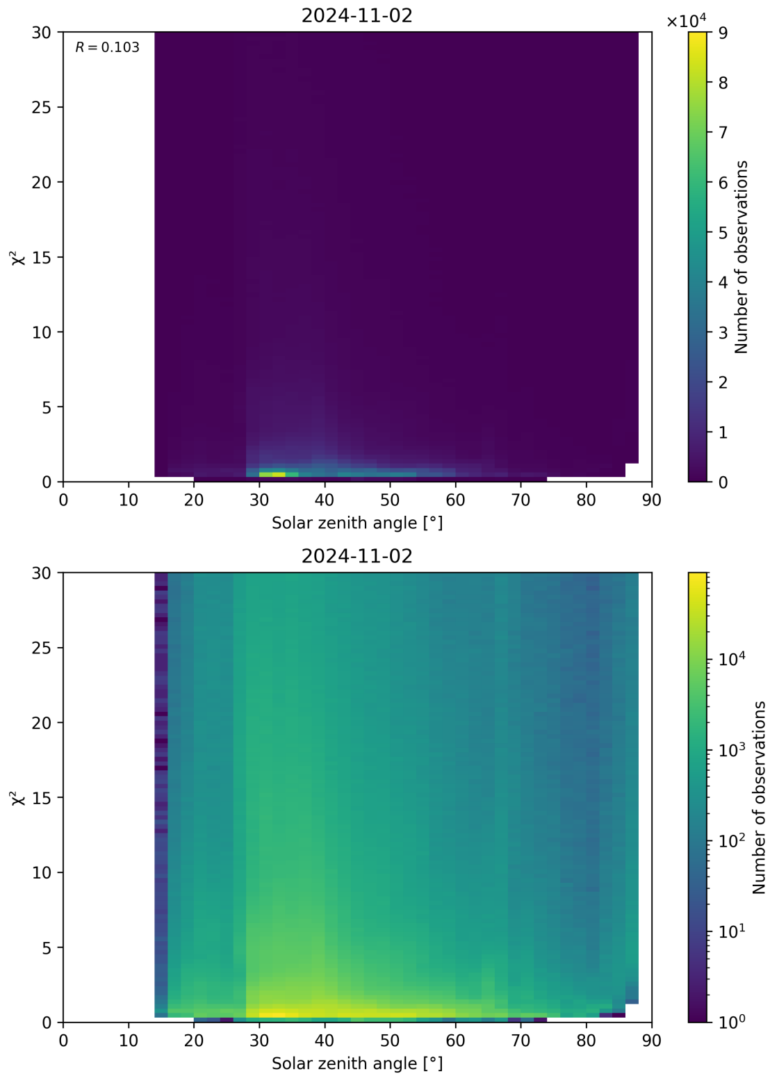
Figure 119: Scatter density plot of “Solar zenith angle” against “ \chi^2 ” for 2024-11-01 to 2024-11-03.
