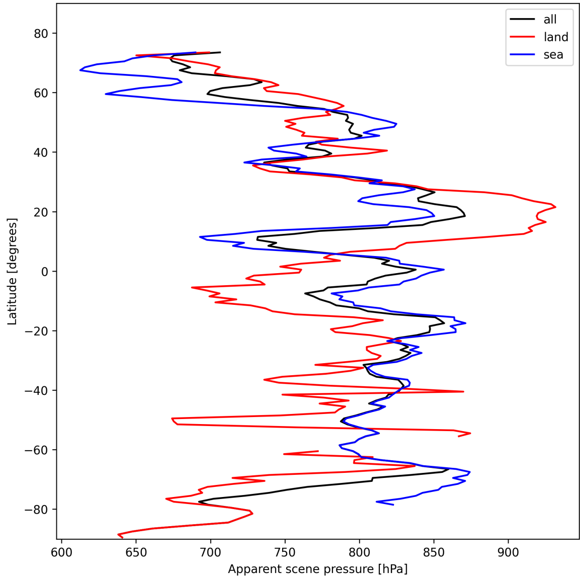
Figure 19: Zonal average of “Apparent scene pressure” for 2024-11-01 to 2024-11-03.
