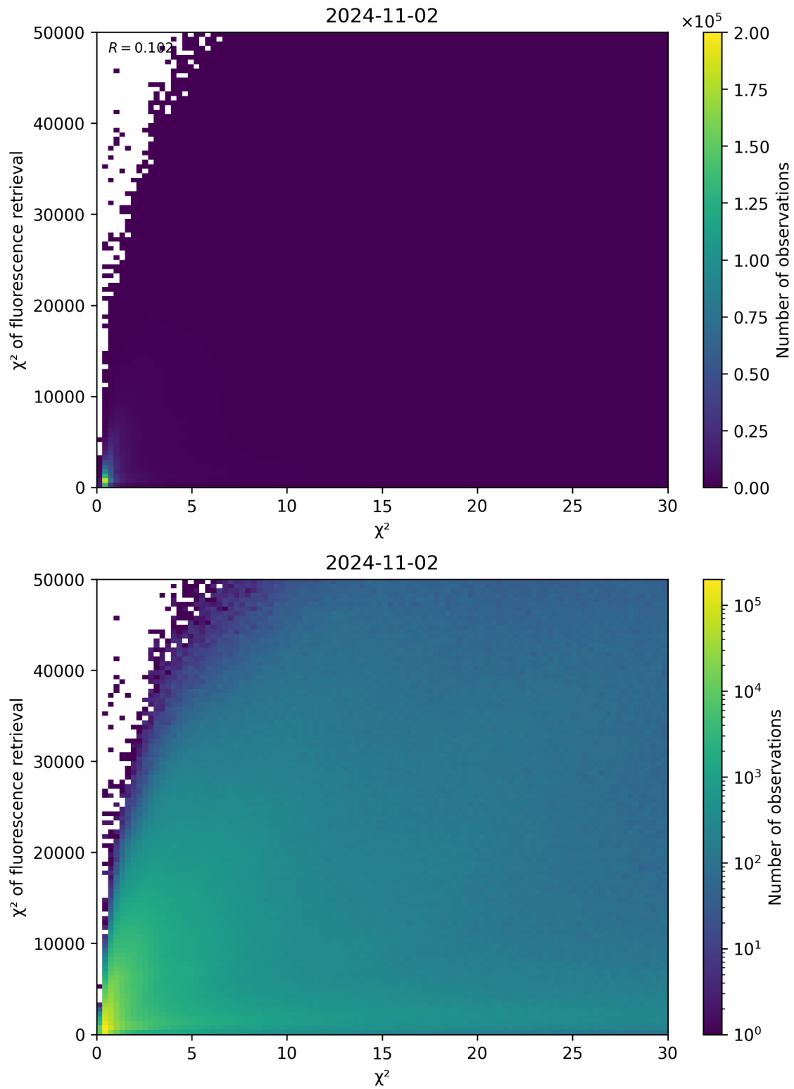
Figure 69: Scatter density plot of “ \chi^2 ” against “ \chi^2 of fluorescence retrieval” for 2024-11-01 to 2024-11-03.
