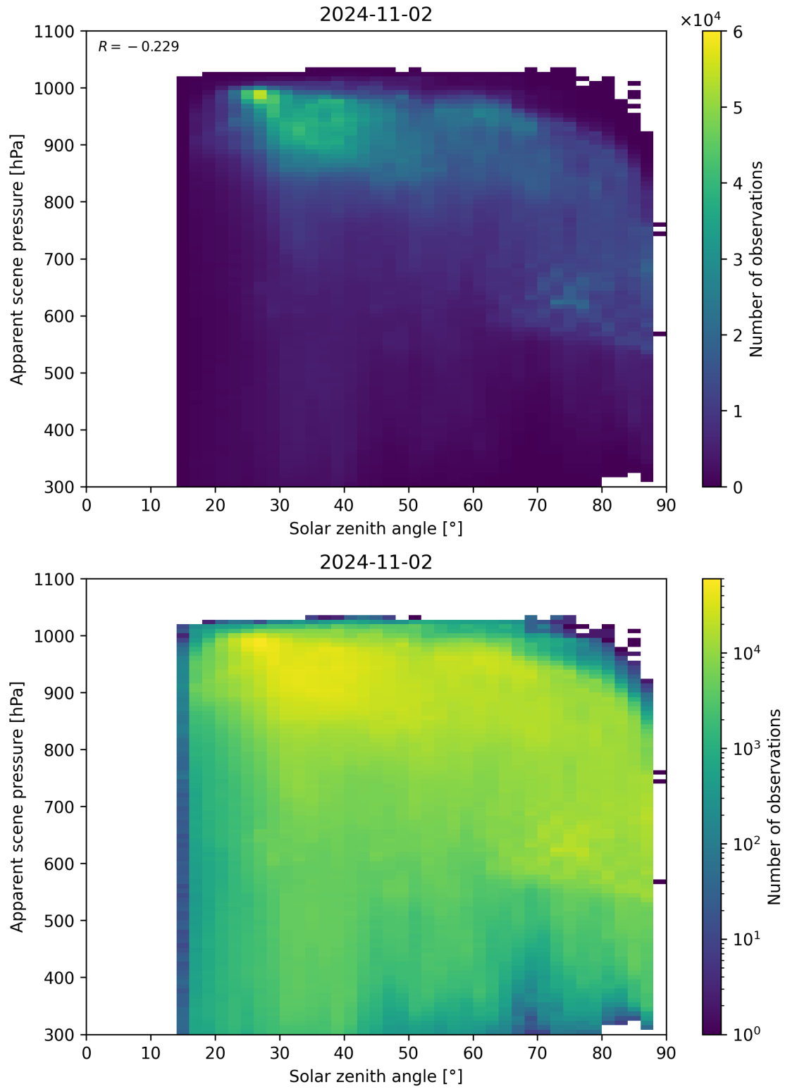
Figure 118: Scatter density plot of “Solar zenith angle” against “Apparent scene pressure” for 2024-11-01 to 2024-11-03.
