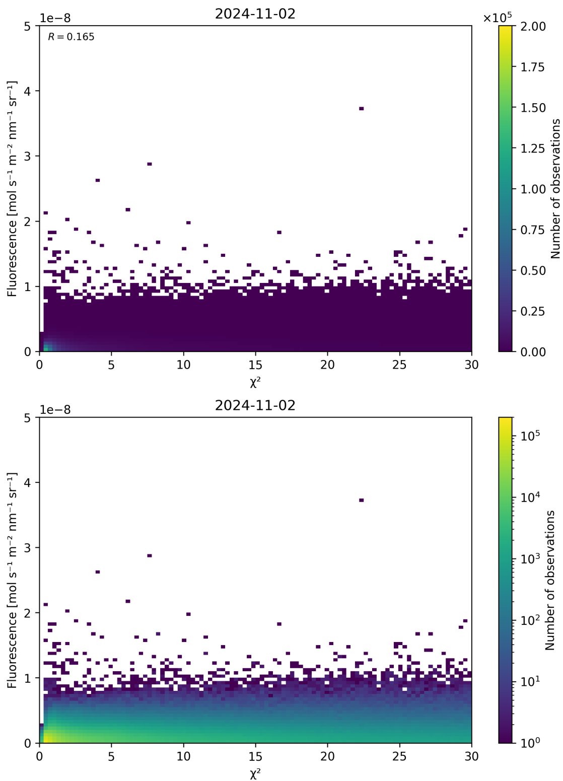
Figure 70: Scatter density plot of “ \chi^2 ” against “Fluorescence” for 2024-11-01 to 2024-11-03.
