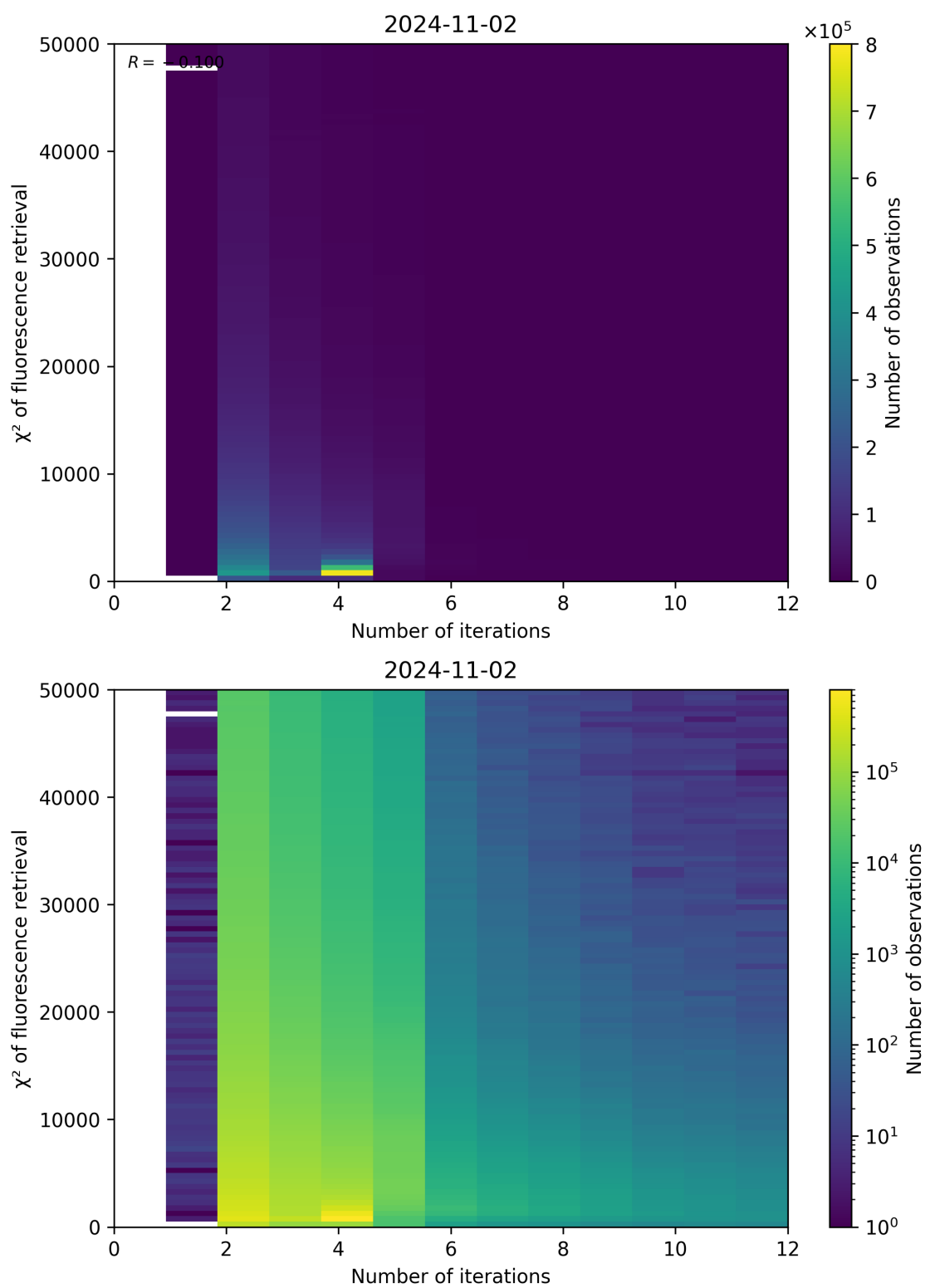
Figure 106: Scatter density plot of “Number of iterations” against “ \chi^2 of fluorescence retrieval” for 2024-11-01 to 2024-11-03.
