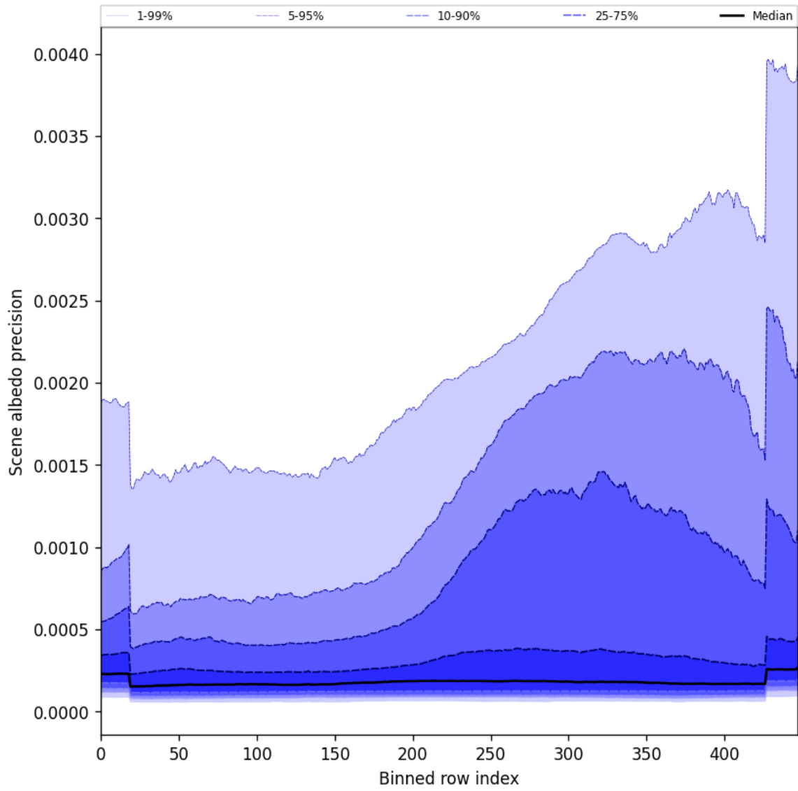
Figure 52: Along track statistics of “Scene albedo precision” for 2024-11-01 to 2024-11-03
