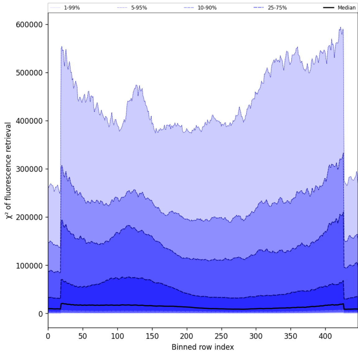
Figure 59: Along track statistics of “ \chi^2 of fluorescence retrieval” for 2024-11-01 to 2024-11-03
