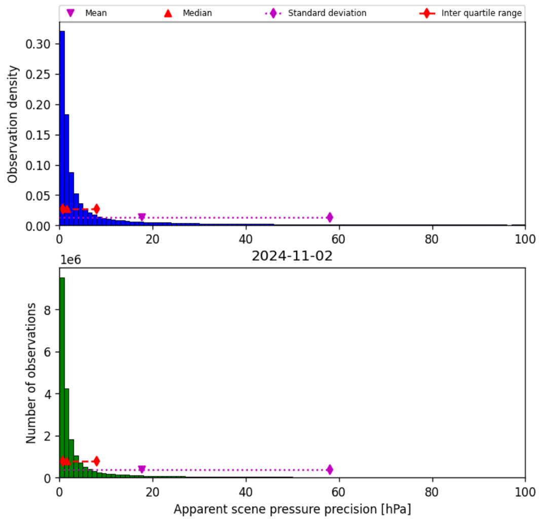
Figure 37: Histogram of “Apparent scene pressure precision” for 2024-11-01 to 2024-11-03
