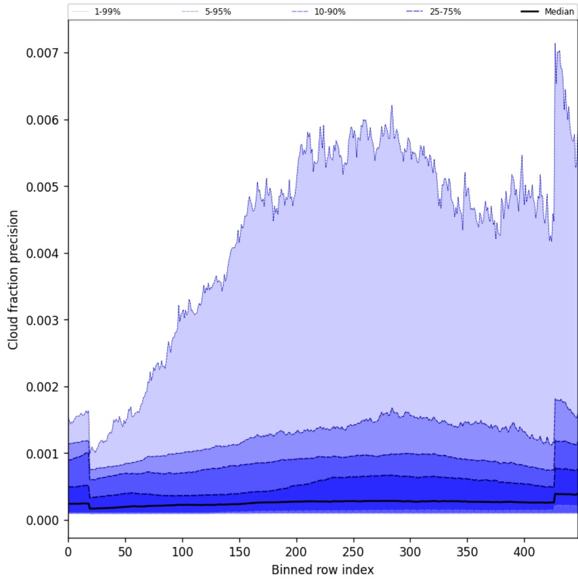
Figure 50: Along track statistics of “Cloud fraction precision” for 2024-11-01 to 2024-11-03
