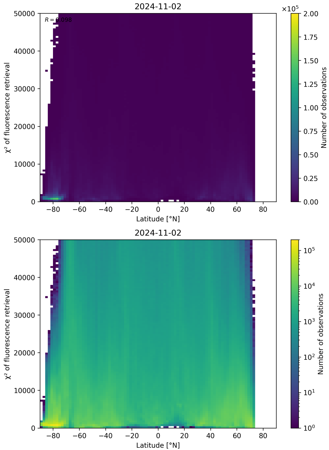
Figure 98: Scatter density plot of “Latitude” against “ \chi^2 of fluorescence retrieval” for 2024-11-01 to 2024-11-03.
