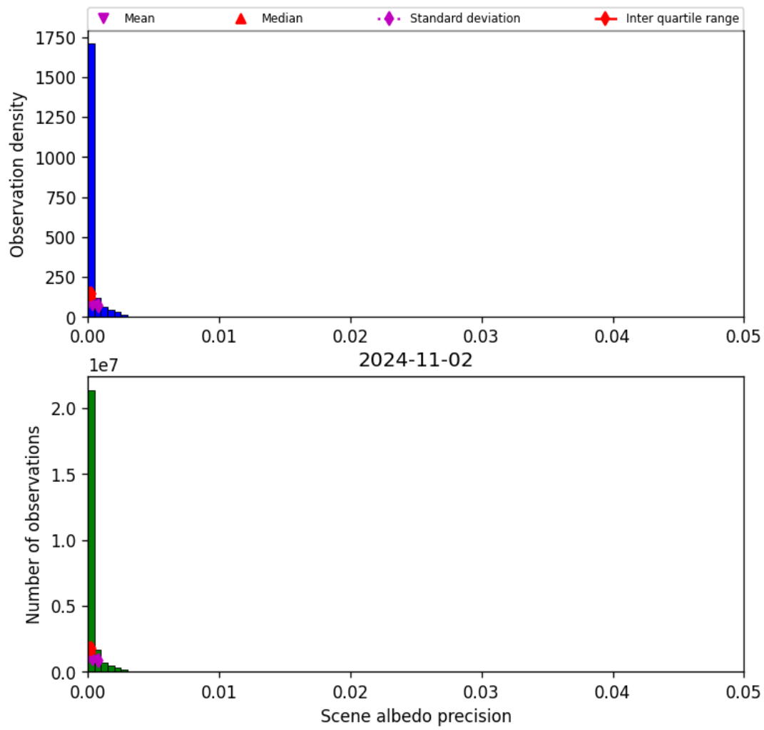
Figure 35: Histogram of “Scene albedo precision” for 2024-11-01 to 2024-11-03
