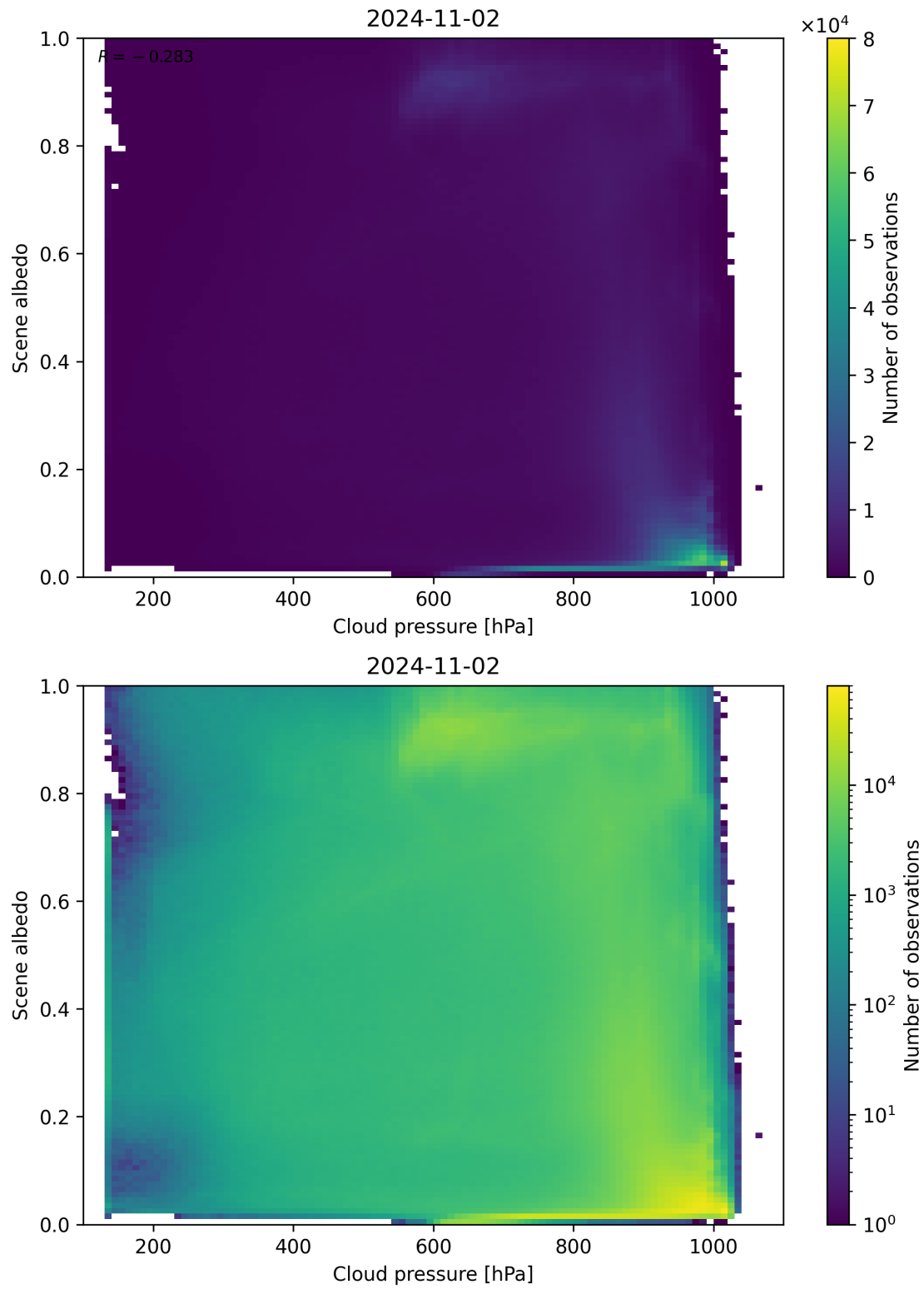
Figure 91: Scatter density plot of “Cloud pressure” against “Scene albedo” for 2024-11-01 to 2024-11-03.
