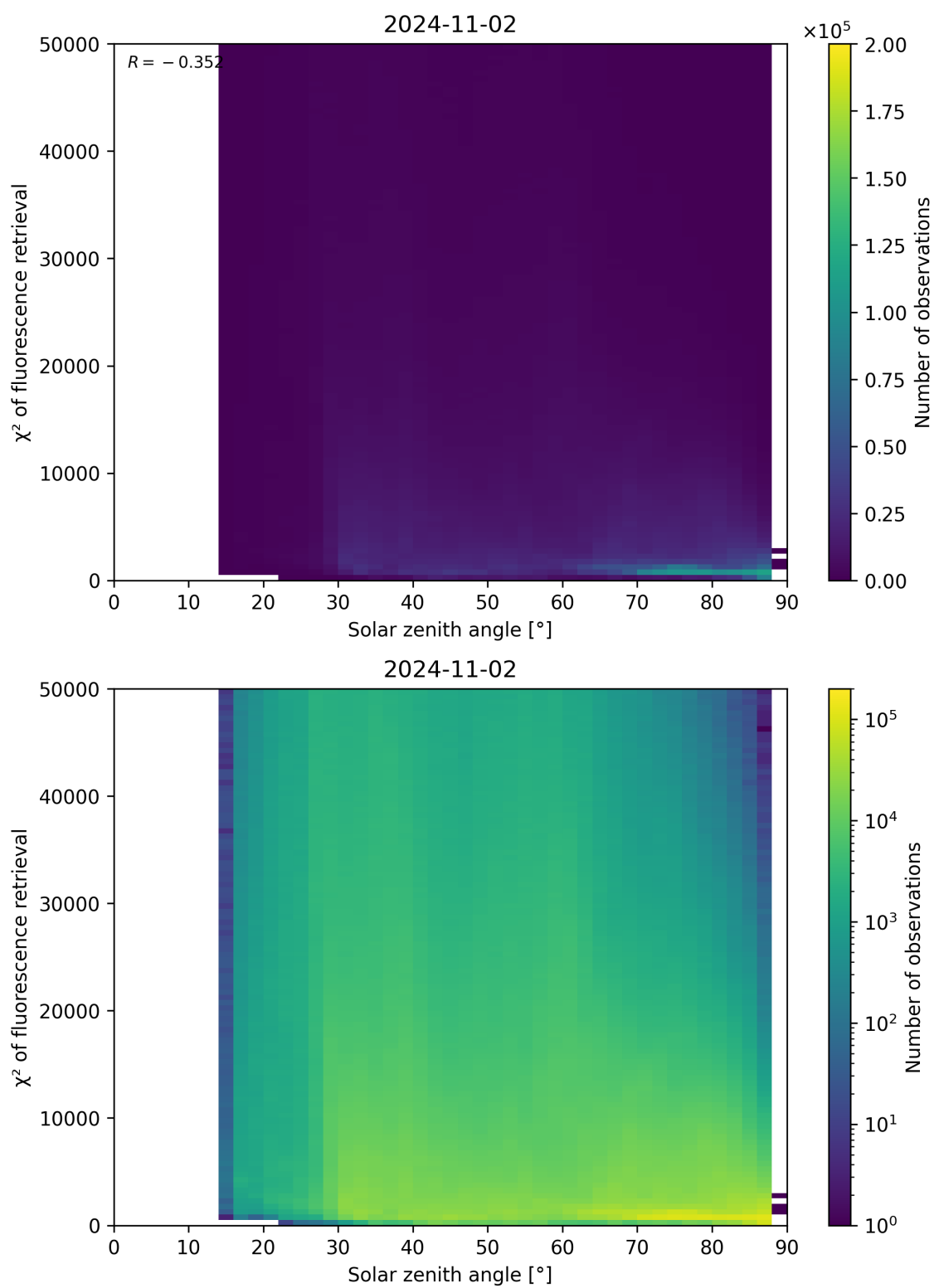
Figure 120: Scatter density plot of “Solar zenith angle” against “ \chi^2 of fluorescence retrieval” for 2024-11-01 to 2024-11-03.
