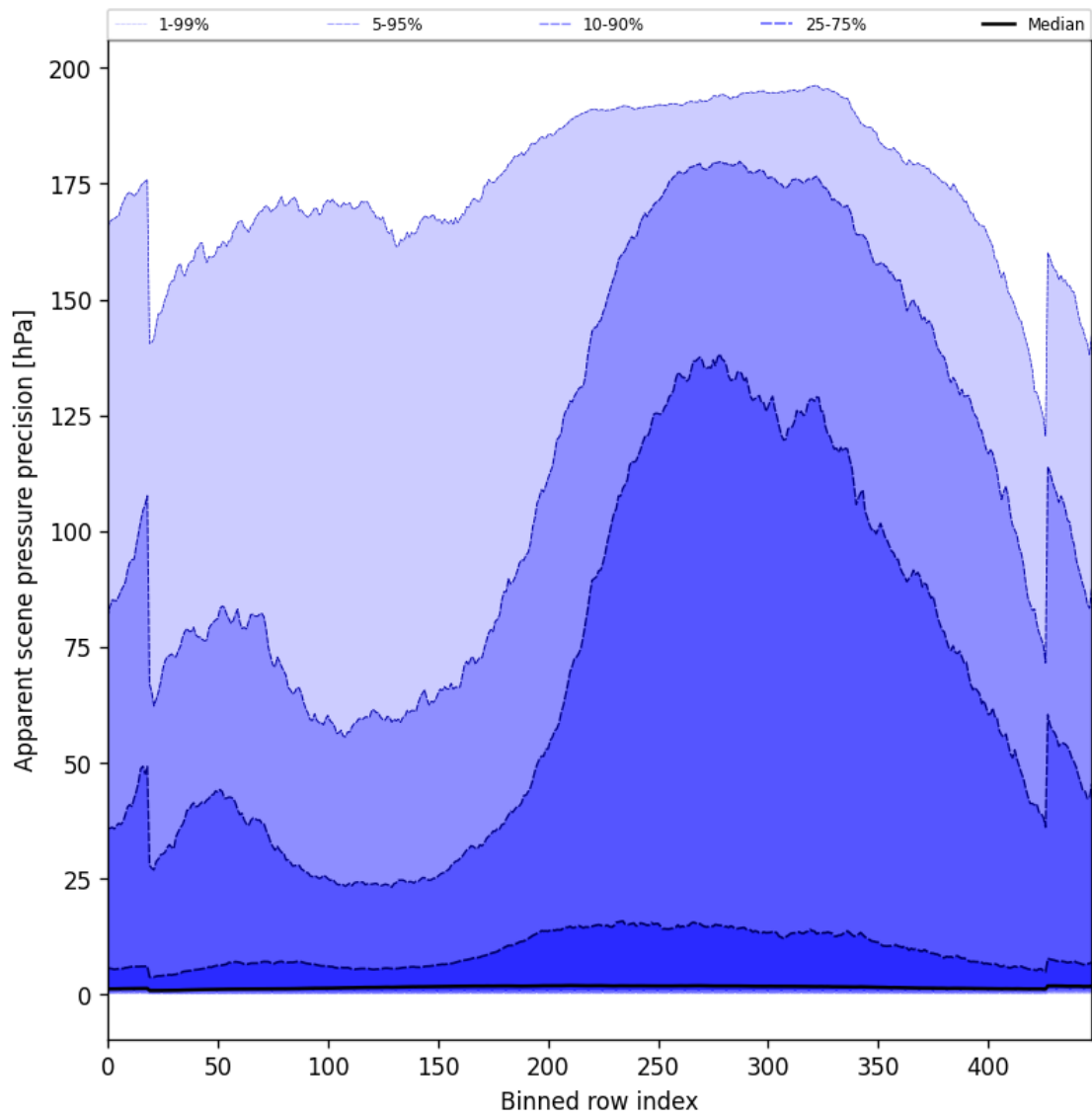
Figure 54: Along track statistics of “Apparent scene pressure precision” for 2024-11-01 to 2024-11-03
