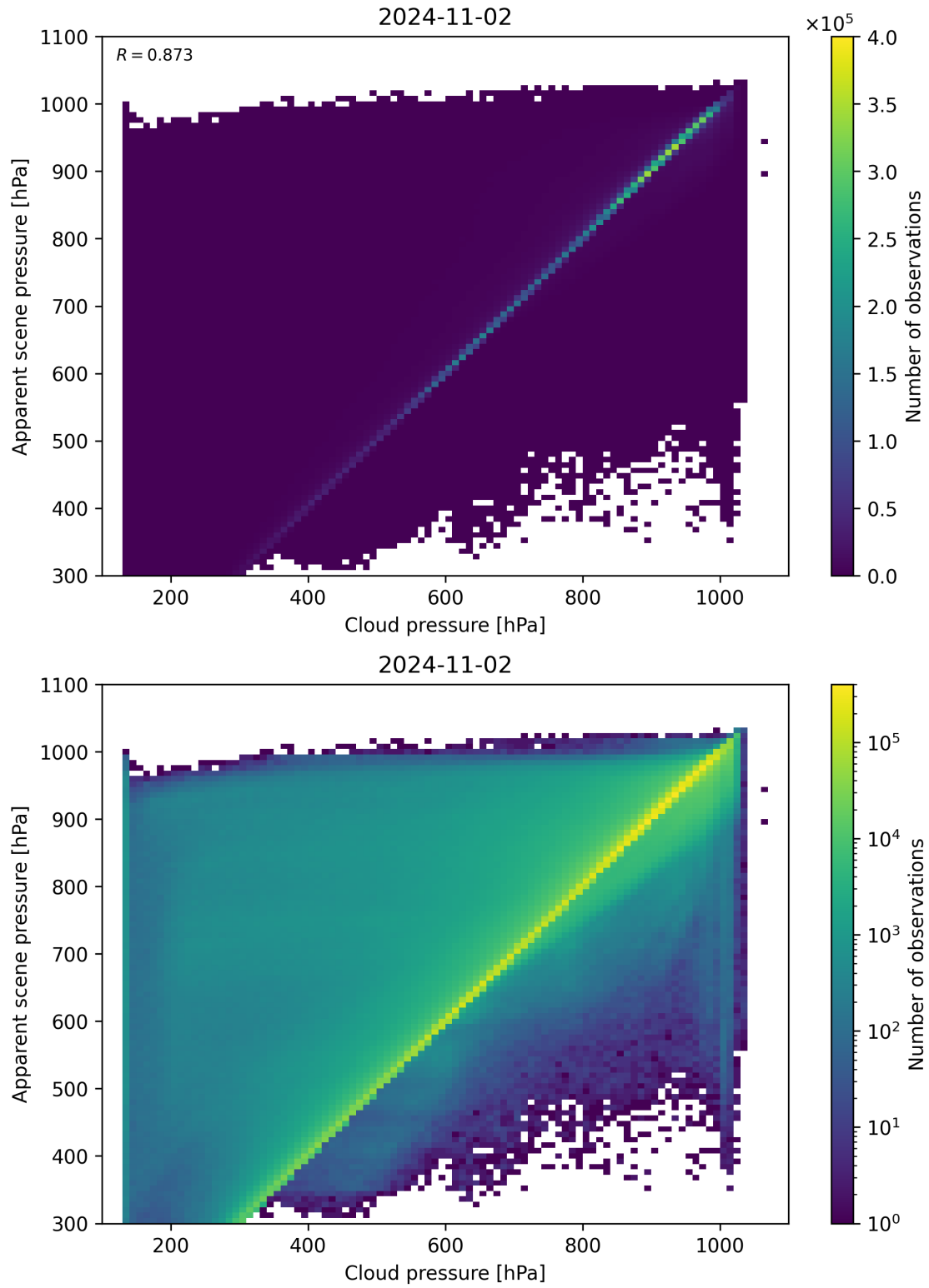
Figure 84: Scatter density plot of “Cloud pressure” against “Apparent scene pressure” for 2024-11-01 to 2024-11-03.
