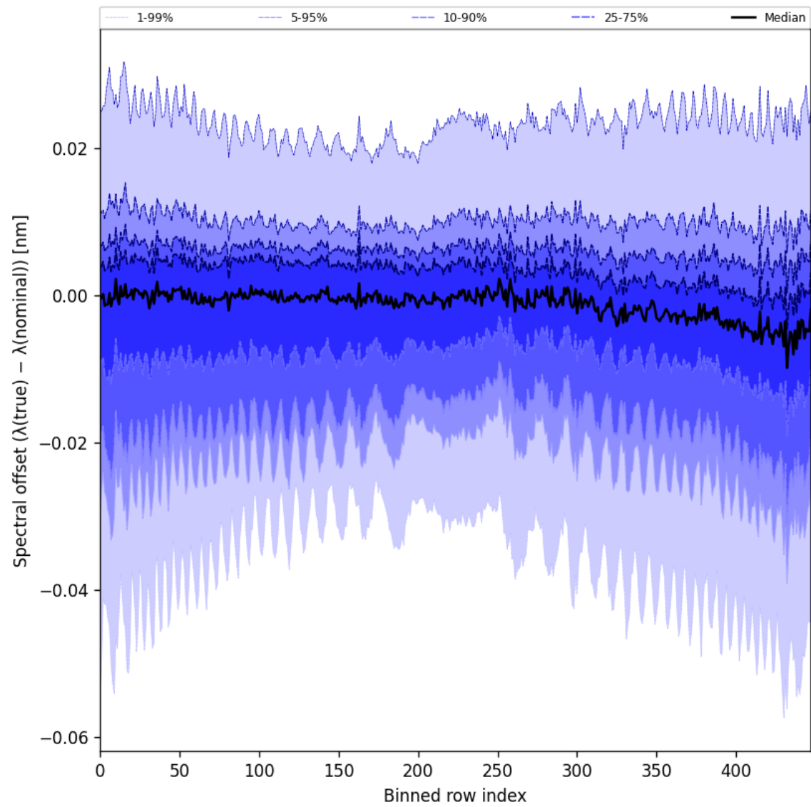
Figure 62: Along track statistics of “Spectral offset ( \lambda_{\text{true}} - \lambda_{\text{nominal}} )” for 2024-11-01 to 2024-11-03
