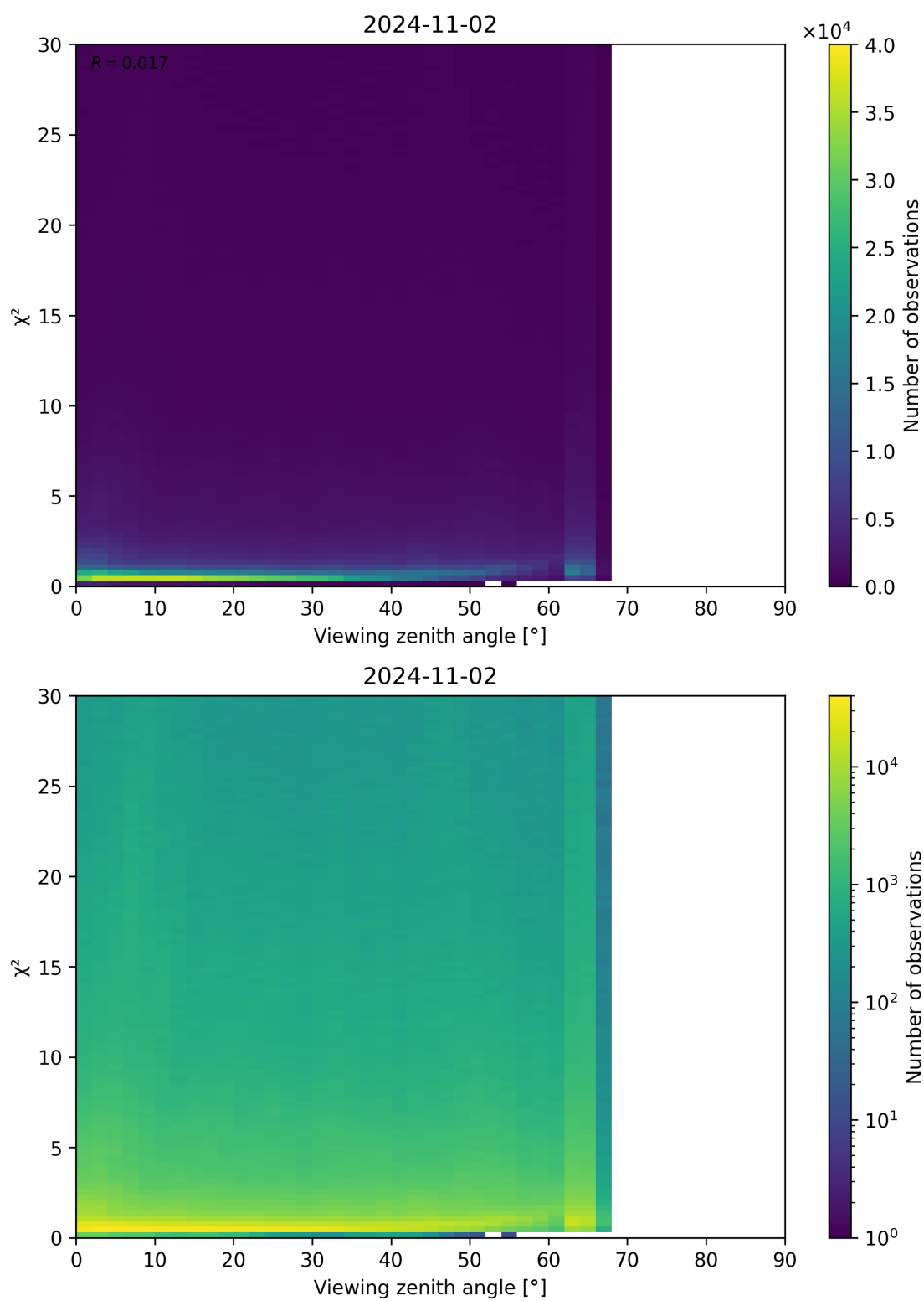
Figure 130: Scatter density plot of “Viewing zenith angle” against “ \chi^2 ” for 2024-11-01 to 2024-11-03.
