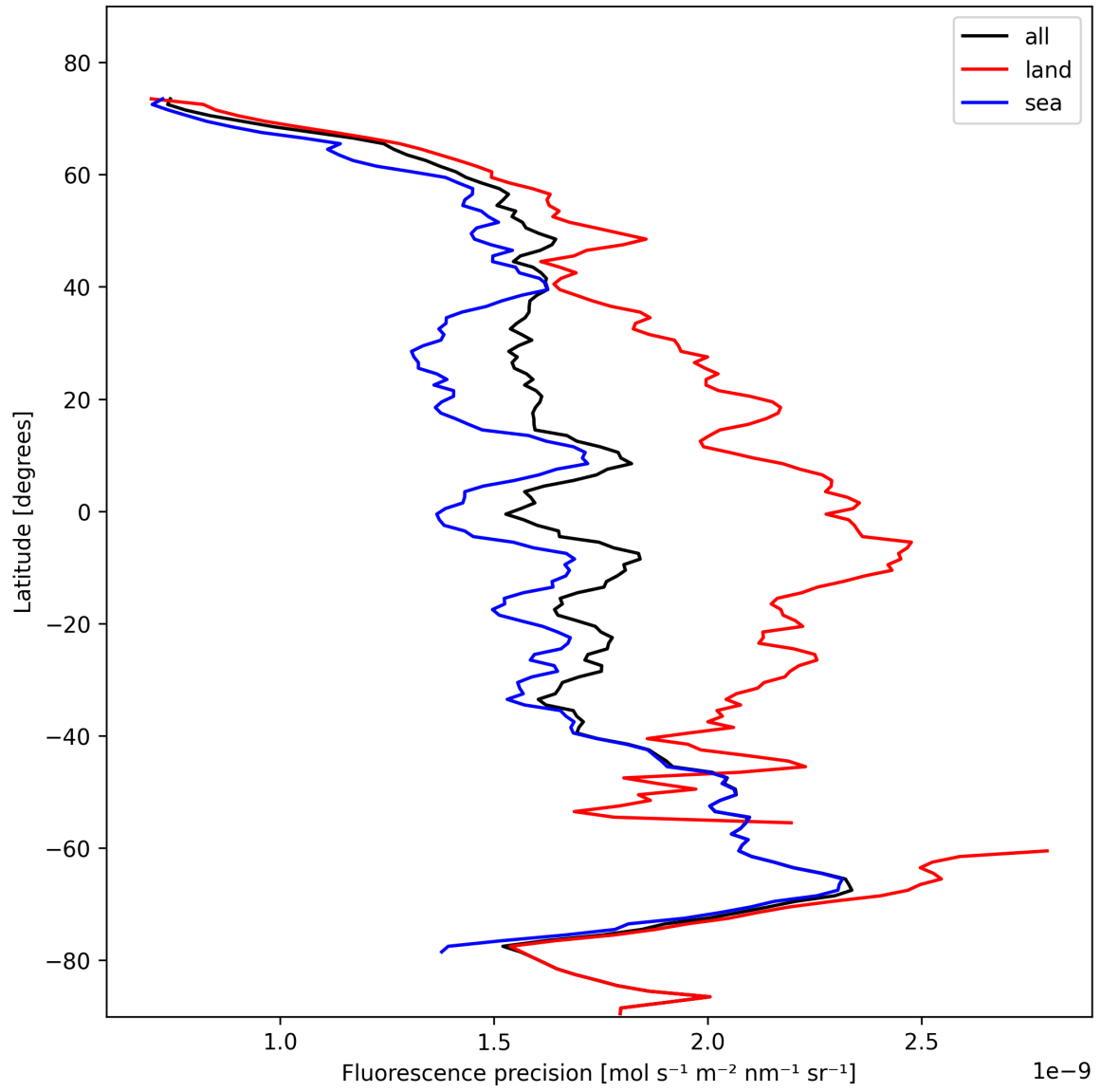
Figure 24: Zonal average of “Fluorescence precision” for 2024-11-01 to 2024-11-03.
