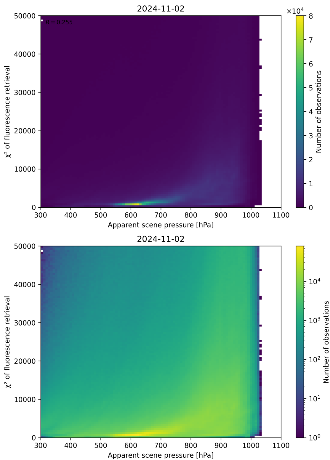
Figure 64: Scatter density plot of “Apparent scene pressure” against “ \chi^2 of fluorescence retrieval” for 2024-11-01 to 2024-11-03.
