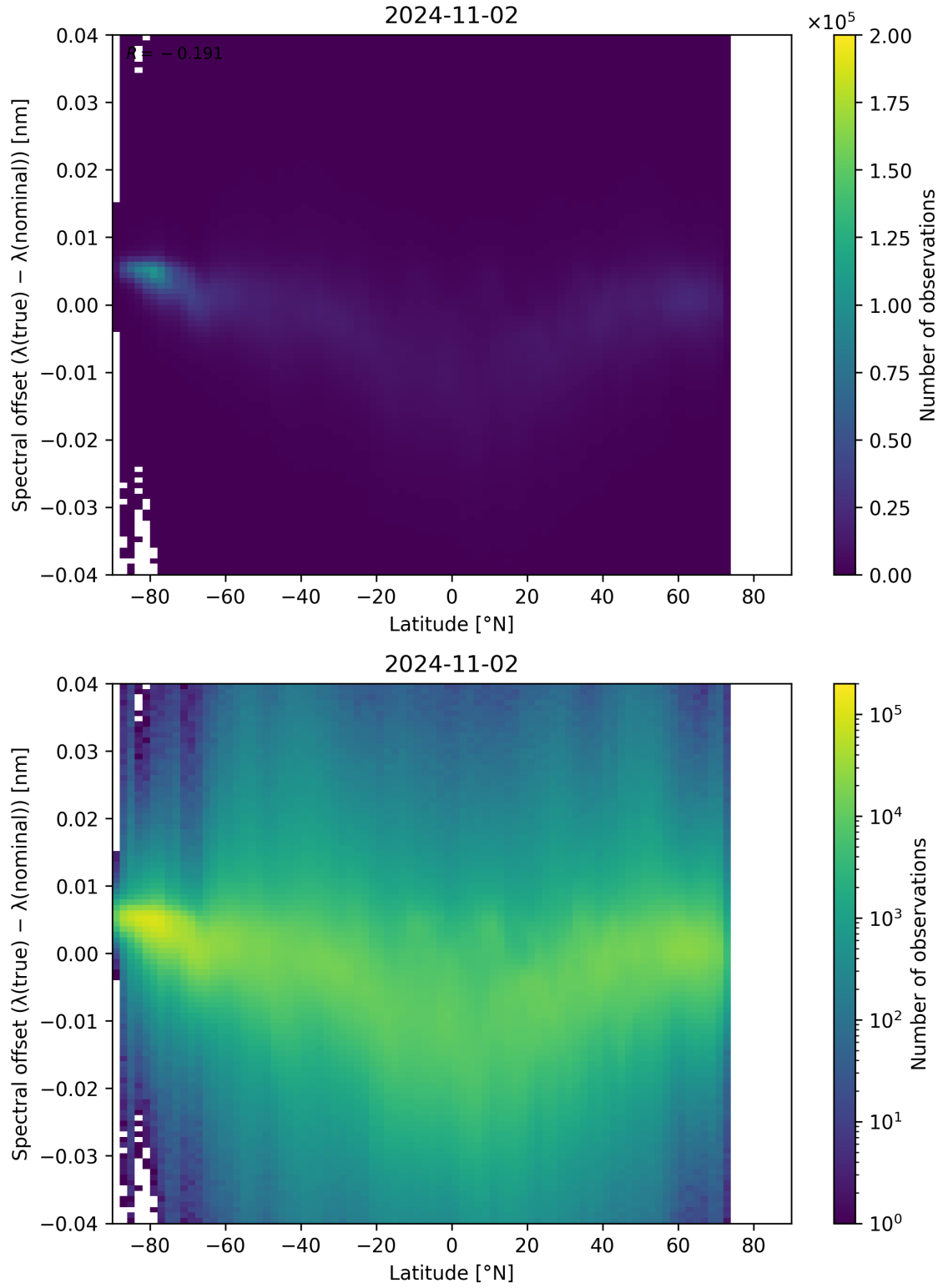
Figure 105: Scatter density plot of “Latitude” against “Spectral offset ( \lambda_{\text{true}} - \lambda_{\text{nominal}} )” for 2024-11-01 to 2024-11-03.
