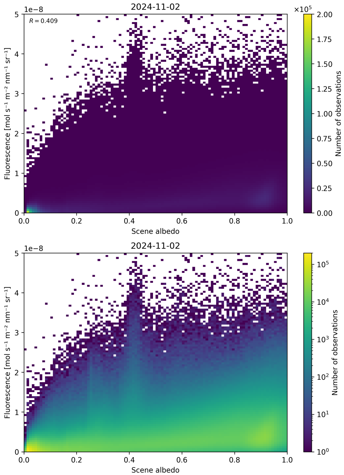
Figure 114: Scatter density plot of "Scene albedo" against "Fluorescence" for 2024-11-01 to 2024-11-03.
