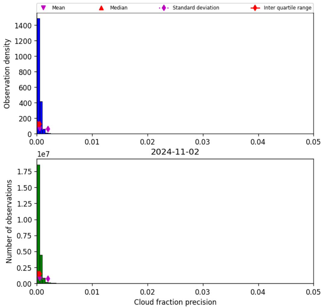
Figure 33: Histogram of “Cloud fraction precision” for 2024-11-01 to 2024-11-03
