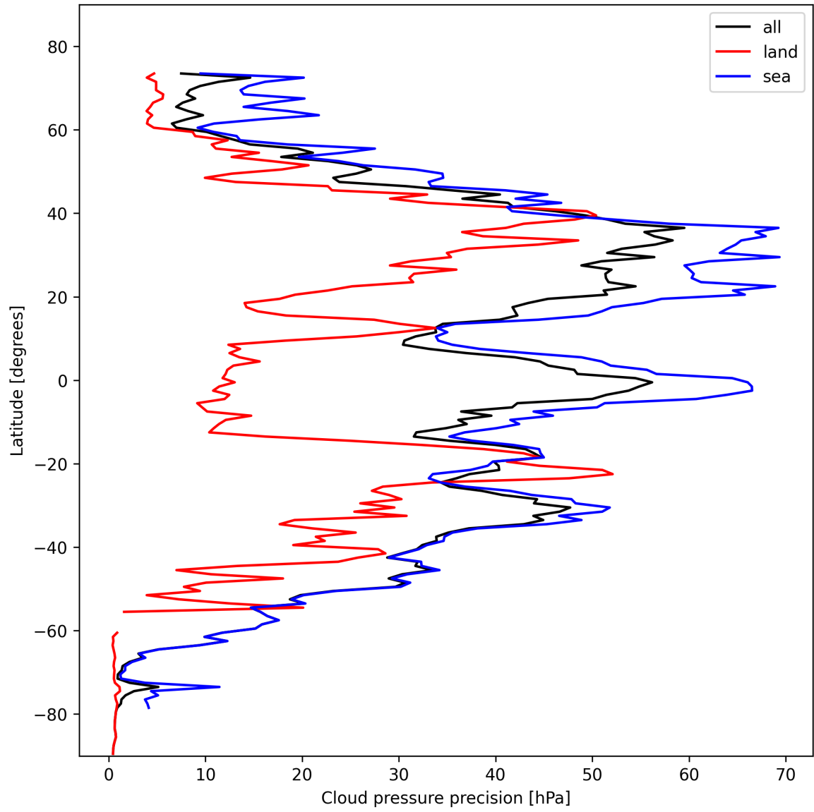
Figure 14: Zonal average of “Cloud pressure precision” for 2024-11-01 to 2024-11-03.
