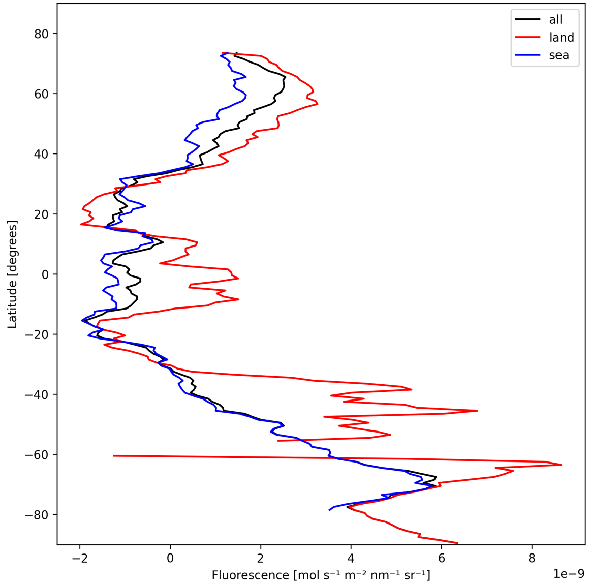
Figure 23: Zonal average of “Fluorescence” for 2024-11-01 to 2024-11-03.
