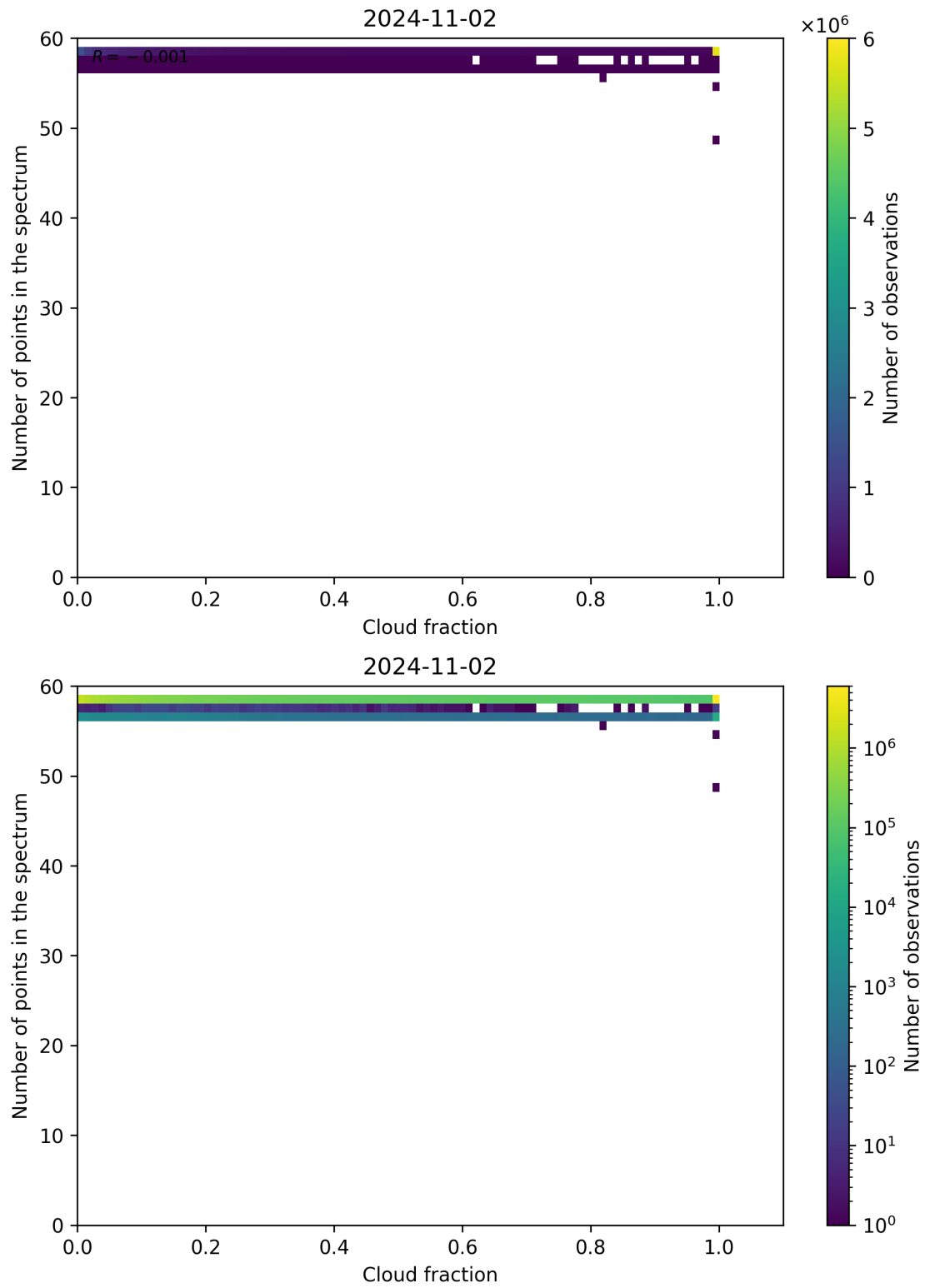
Figure 81: Scatter density plot of “Cloud fraction” against “Number of points in the spectrum” for 2024-11-01 to 2024-11-03.
