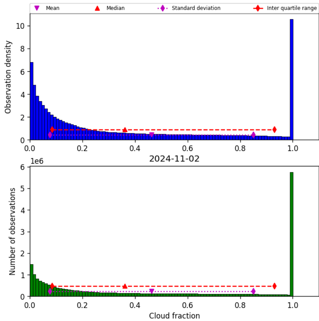
Figure 32: Histogram of "Cloud fraction" for 2024-11-01 to 2024-11-03
