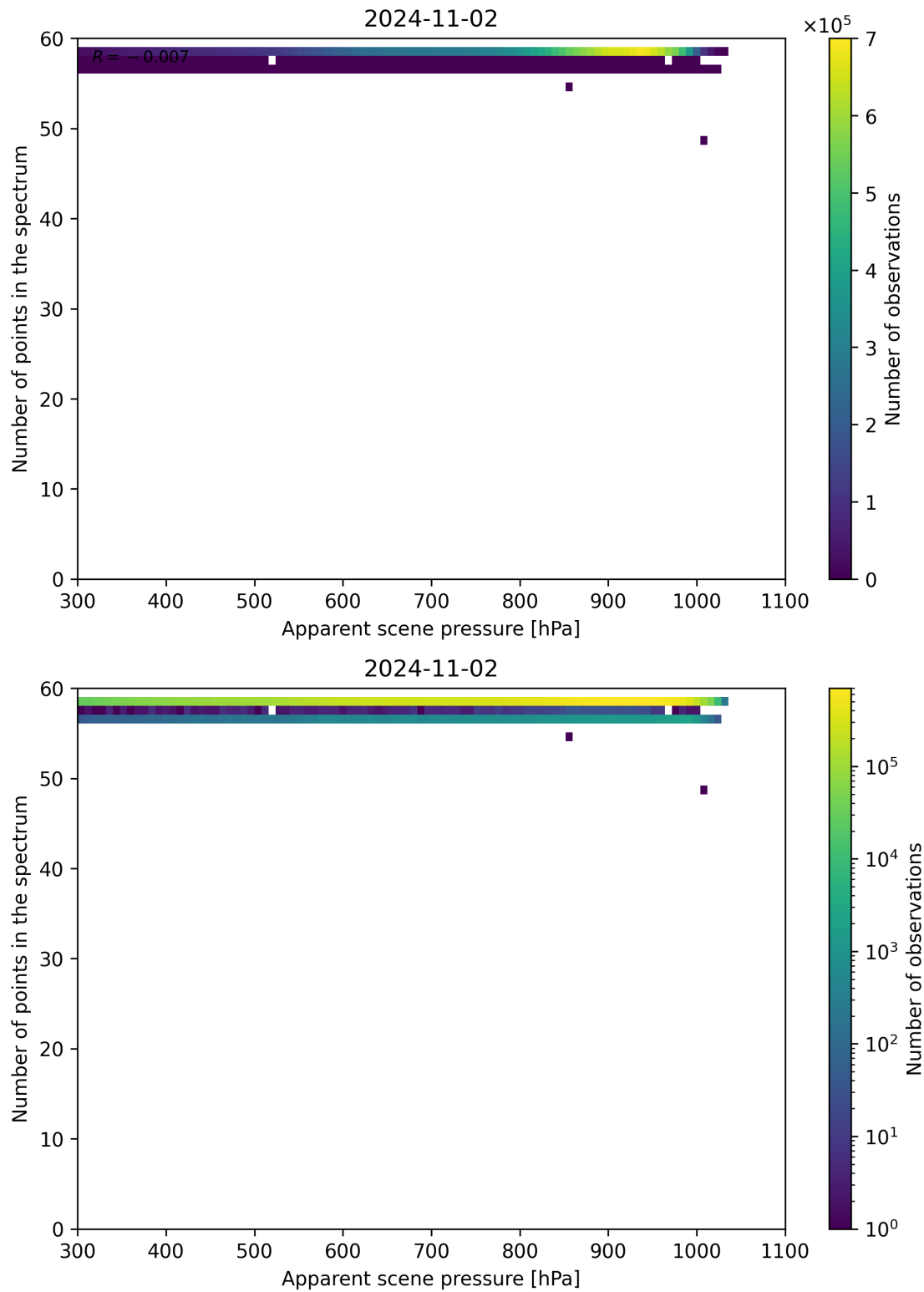
Figure 67: Scatter density plot of “Apparent scene pressure” against “Number of points in the spectrum” for 2024-11-01 to 2024-11-03.
