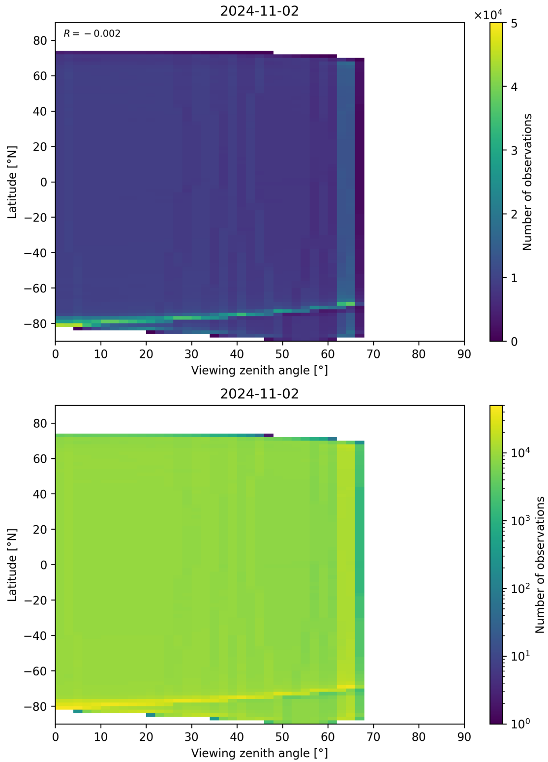
Figure 135: Scatter density plot of “Viewing zenith angle” against “Latitude” for 2024-11-01 to 2024-11-03.
