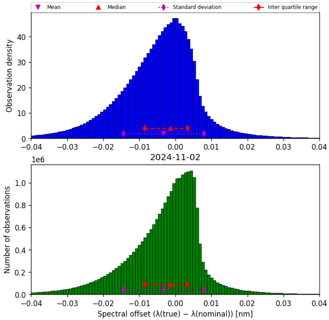
Figure 45: Histogram of “Spectral offset ( \lambda_{\text{true}} - \lambda_{\text{nominal}} )” for 2024-11-01 to 2024-11-03
