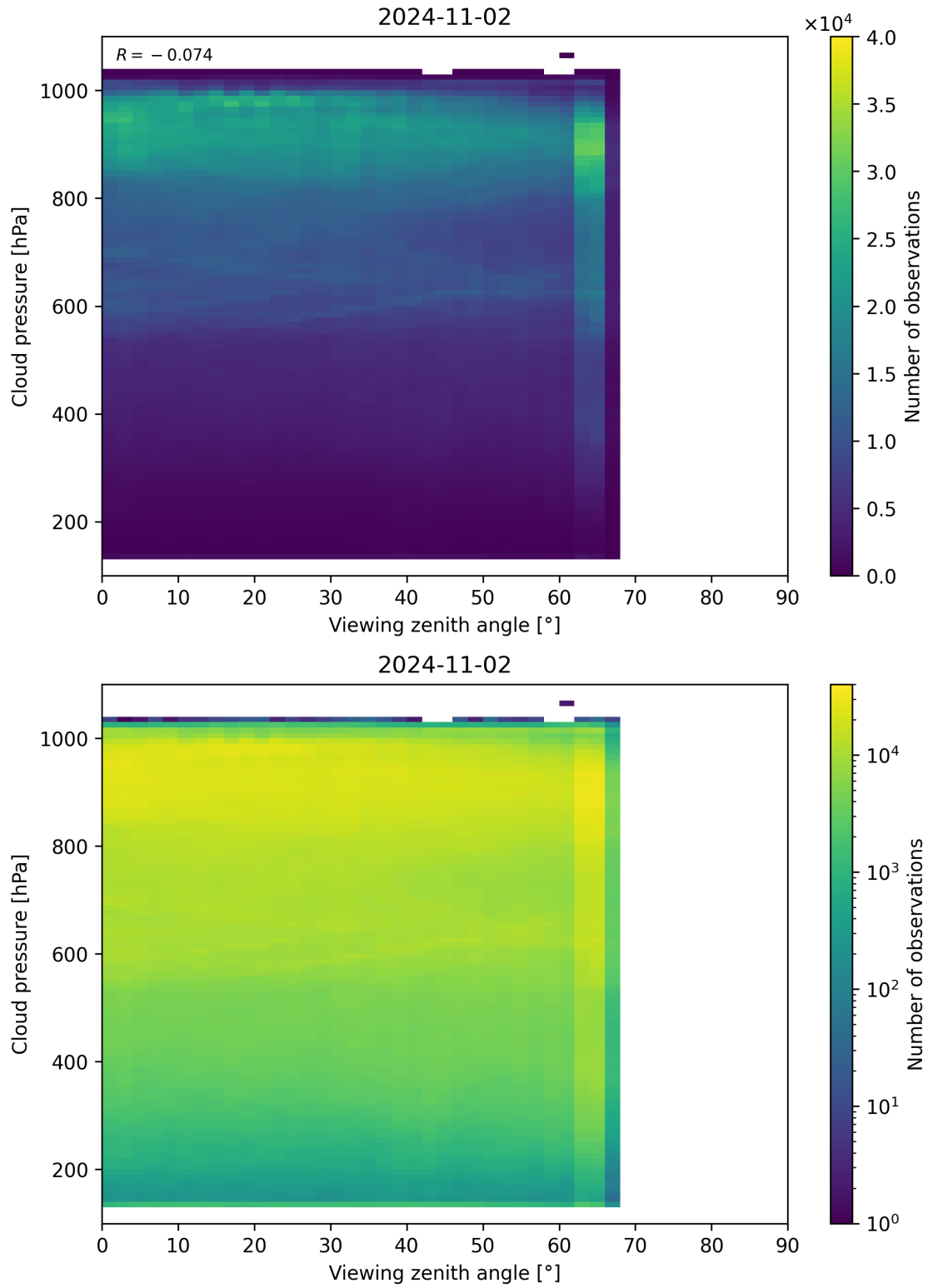
Figure 133: Scatter density plot of “Viewing zenith angle” against “Cloud pressure” for 2024-11-01 to 2024-11-03.
