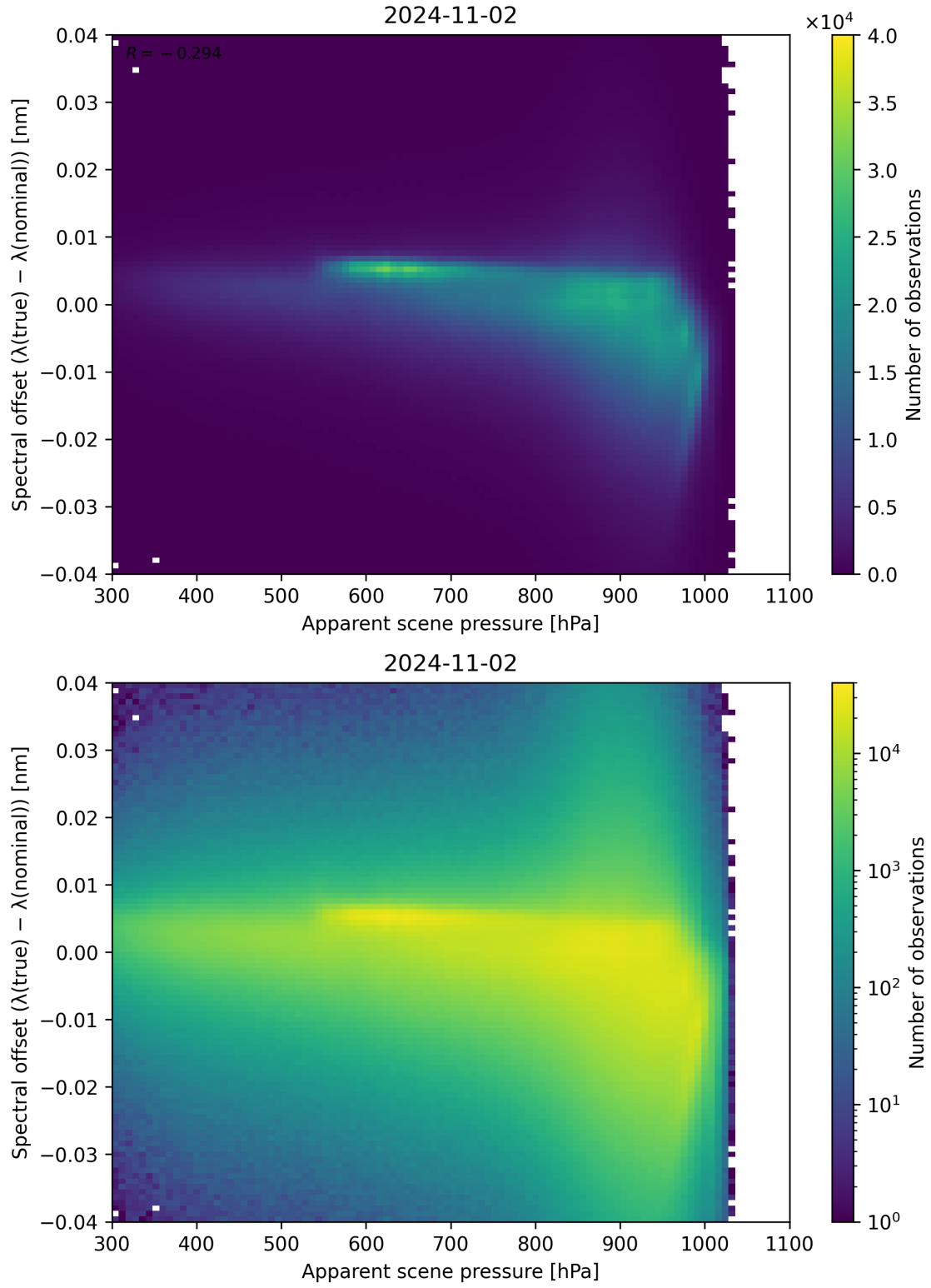
Figure 68: Scatter density plot of “Apparent scene pressure” against “Spectral offset ( \lambda_{\text{true}} - \lambda_{\text{nominal}} )” for 2024-11-01 to 2024-11-03.
