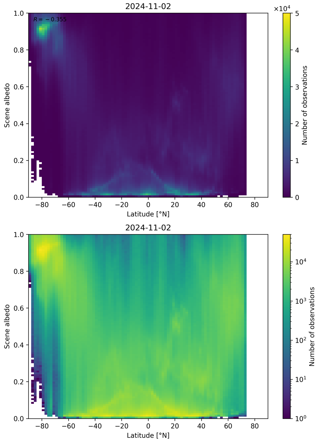
Figure 104: Scatter density plot of “Latitude” against “Scene albedo” for 2024-11-01 to 2024-11-03.
