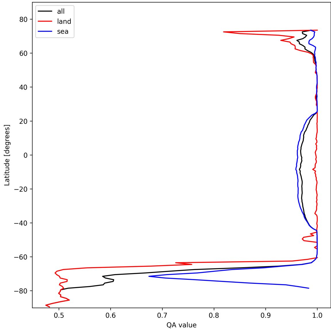
Figure 12: Zonal average of “QA value” for 2024-11-01 to 2024-11-03.
