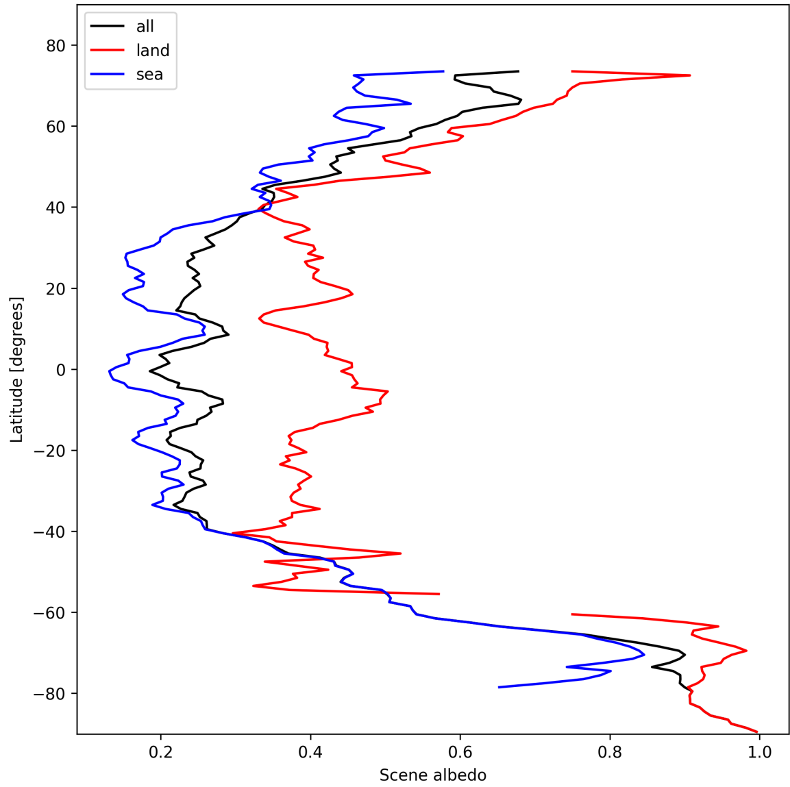
Figure 17: Zonal average of “Scene albedo” for 2024-11-01 to 2024-11-03.
