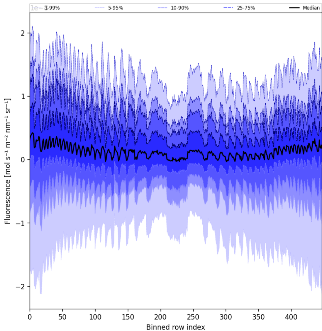
Figure 57: Along track statistics of “Fluorescence” for 2024-11-01 to 2024-11-03
