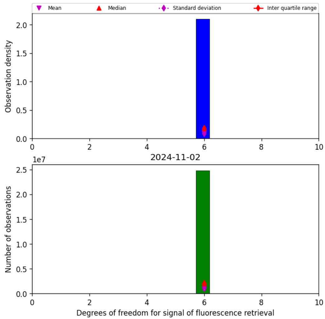
Figure 43: Histogram of “Degrees of freedom for signal of fluorescence retrieval” for 2024-11-01 to 2024-11-03
