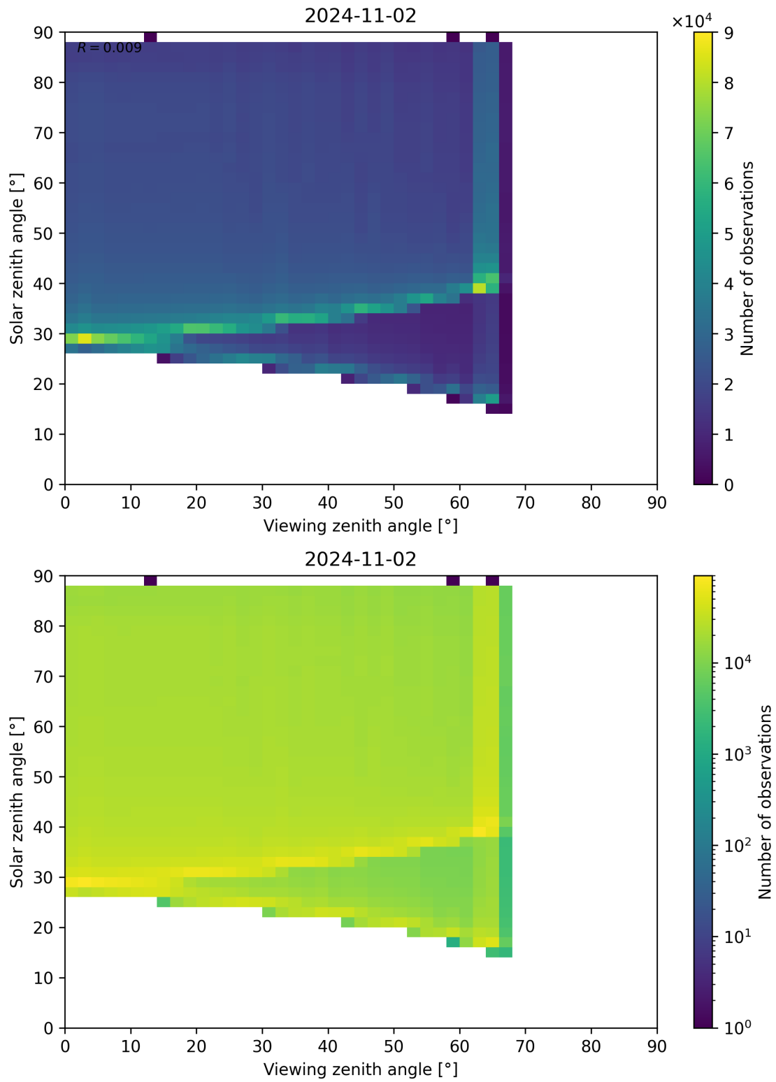
Figure 139: Scatter density plot of “Viewing zenith angle” against “Solar zenith angle” for 2024-11-01 to 2024-11-03.
