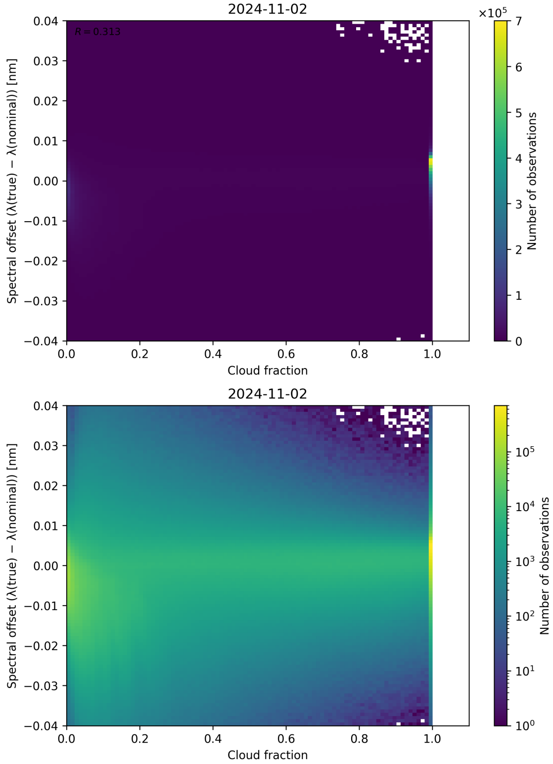
Figure 83: Scatter density plot of “Cloud fraction” against “Spectral offset ( \lambda_{\text{true}} - \lambda_{\text{nominal}} )” for 2024-11-01 to 2024-11-03.
