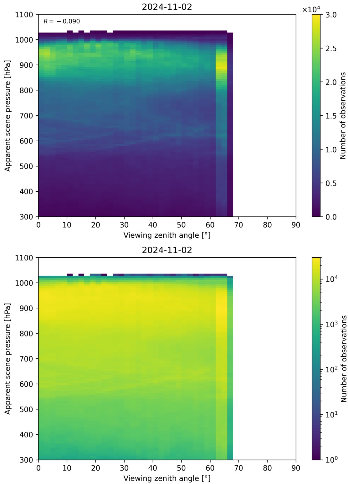
Figure 129: Scatter density plot of “Viewing zenith angle” against “Apparent scene pressure” for 2024-11-01 to 2024-11-03.
