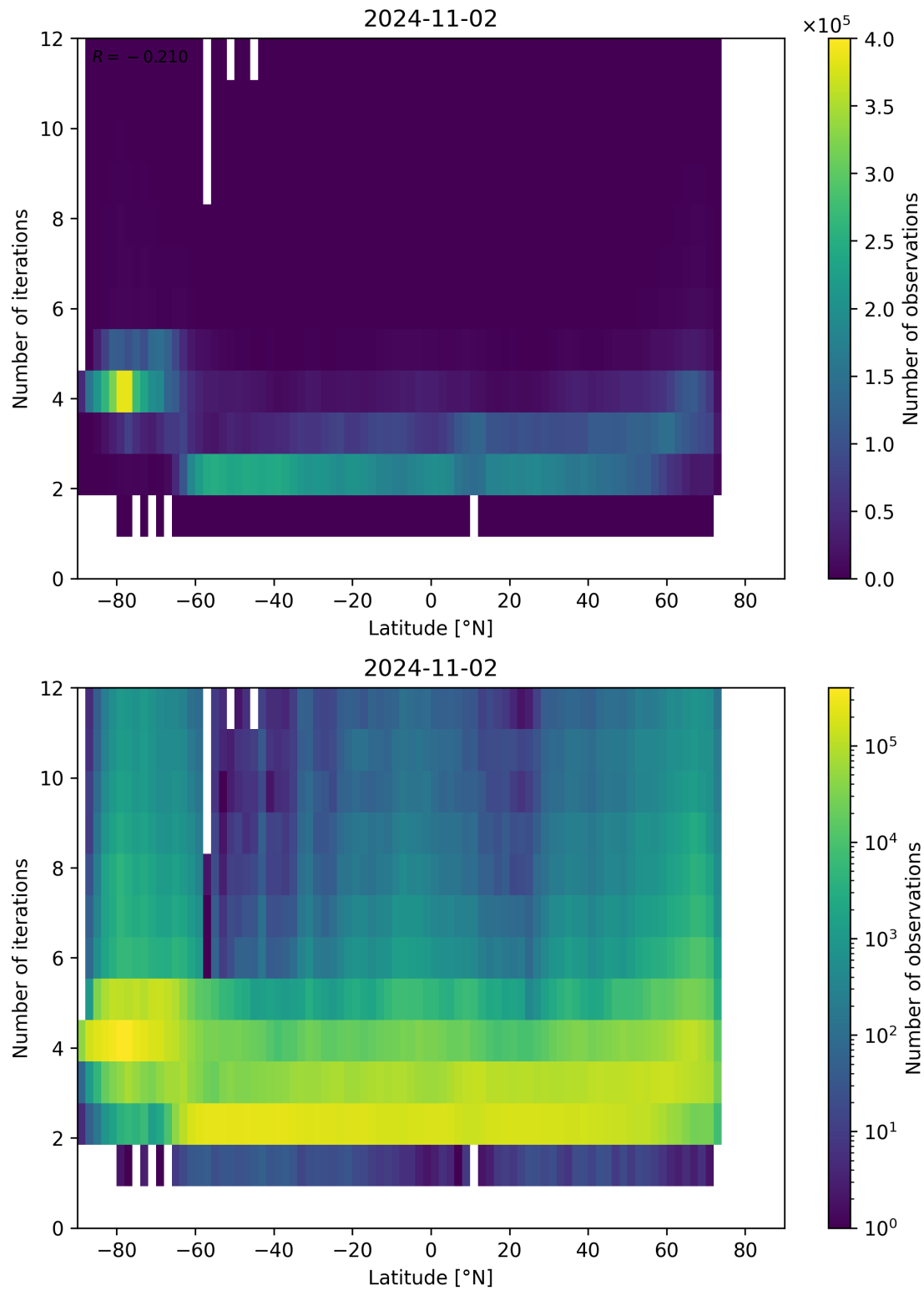
Figure 102: Scatter density plot of “Latitude” against “Number of iterations” for 2024-11-01 to 2024-11-03.
