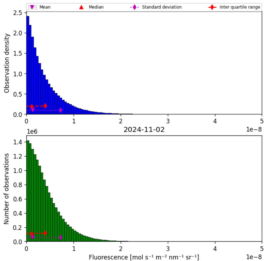
Figure 40: Histogram of “Fluorescence” for 2024-11-01 to 2024-11-03
