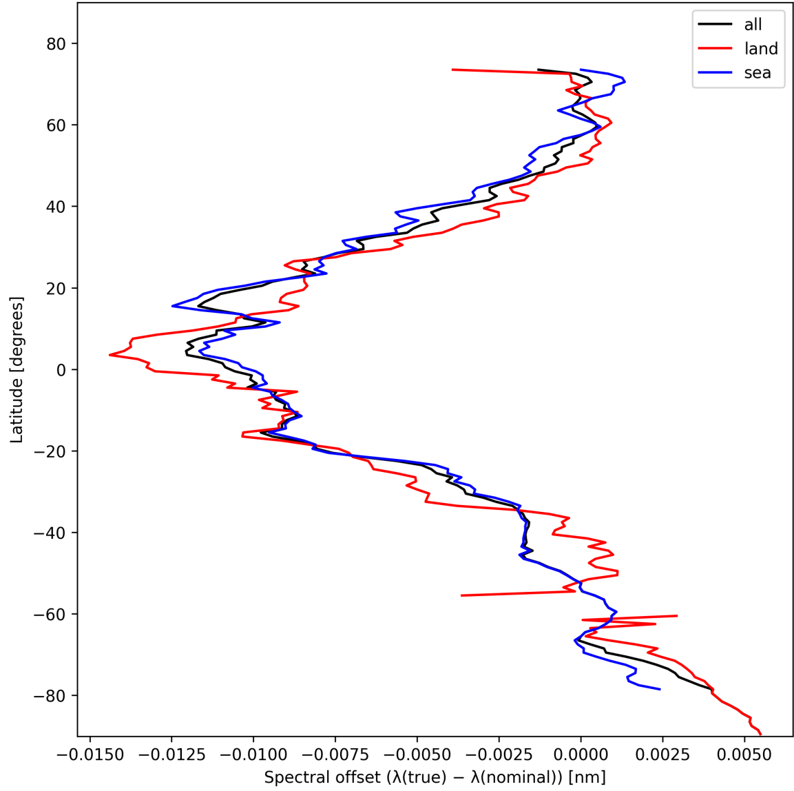
Figure 28: Zonal average of “Spectral offset ( \lambda_{\text{true}} - \lambda_{\text{nominal}} )” for 2024-11-01 to 2024-11-03.
