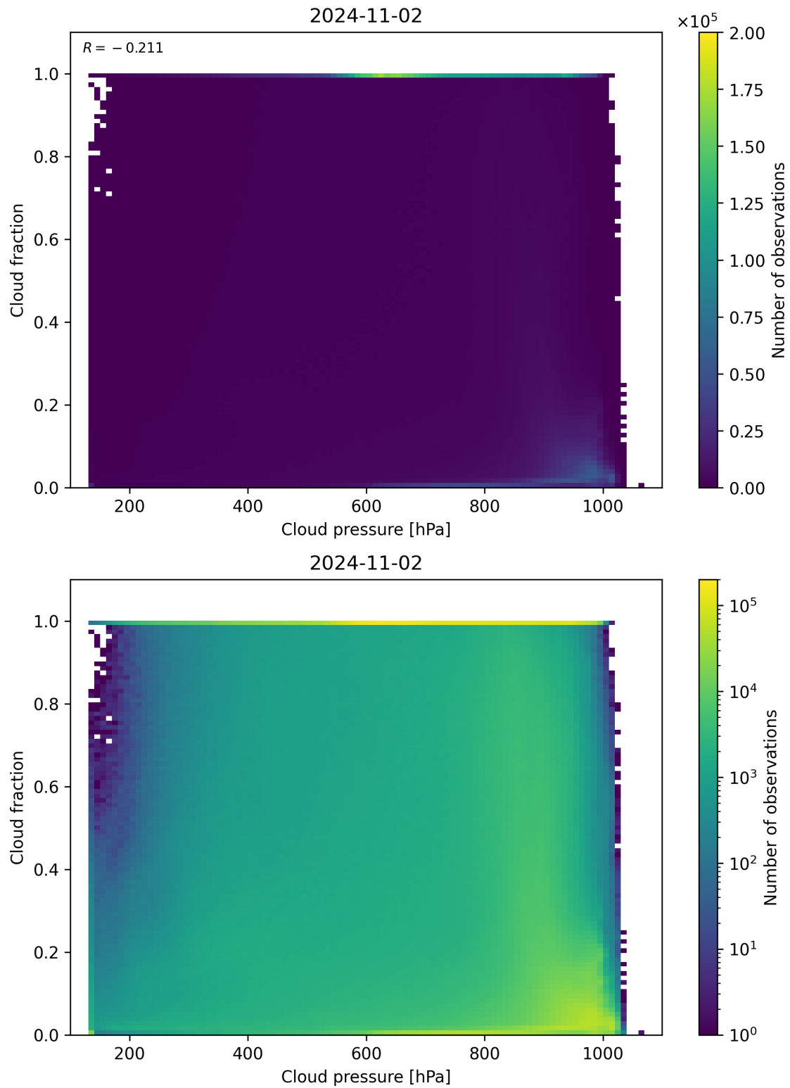
Figure 87: Scatter density plot of “Cloud pressure” against “Cloud fraction” for 2024-11-01 to 2024-11-03.
