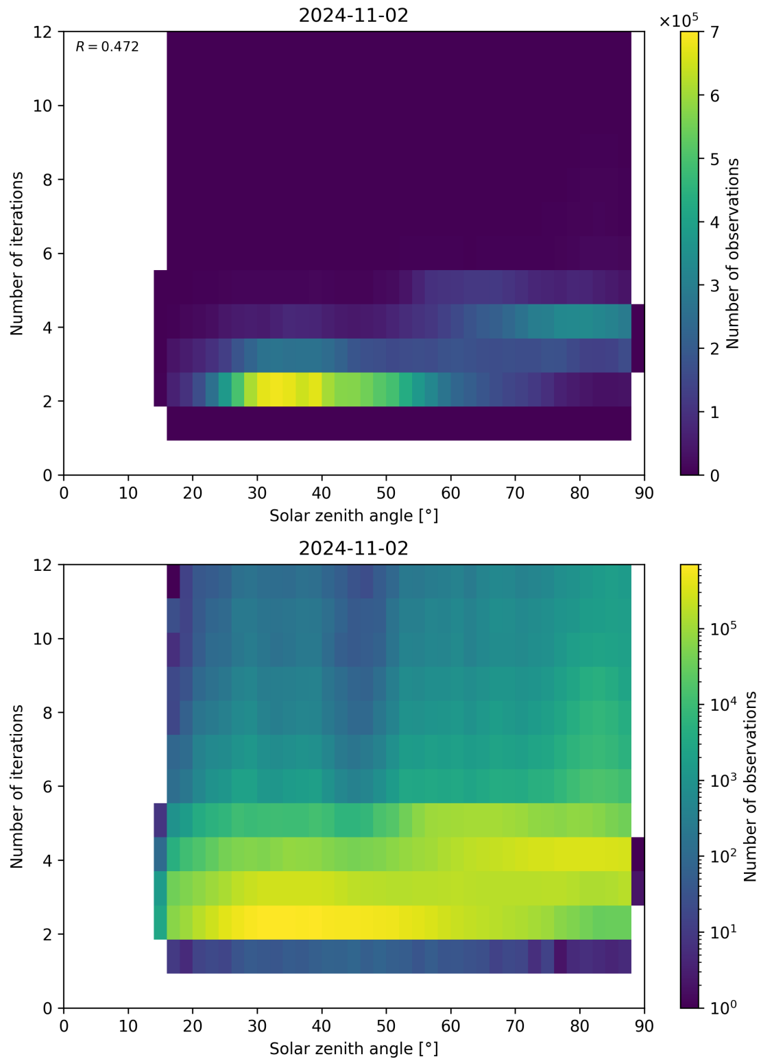
Figure 125: Scatter density plot of “Solar zenith angle” against “Number of iterations” for 2024-11-01 to 2024-11-03.
