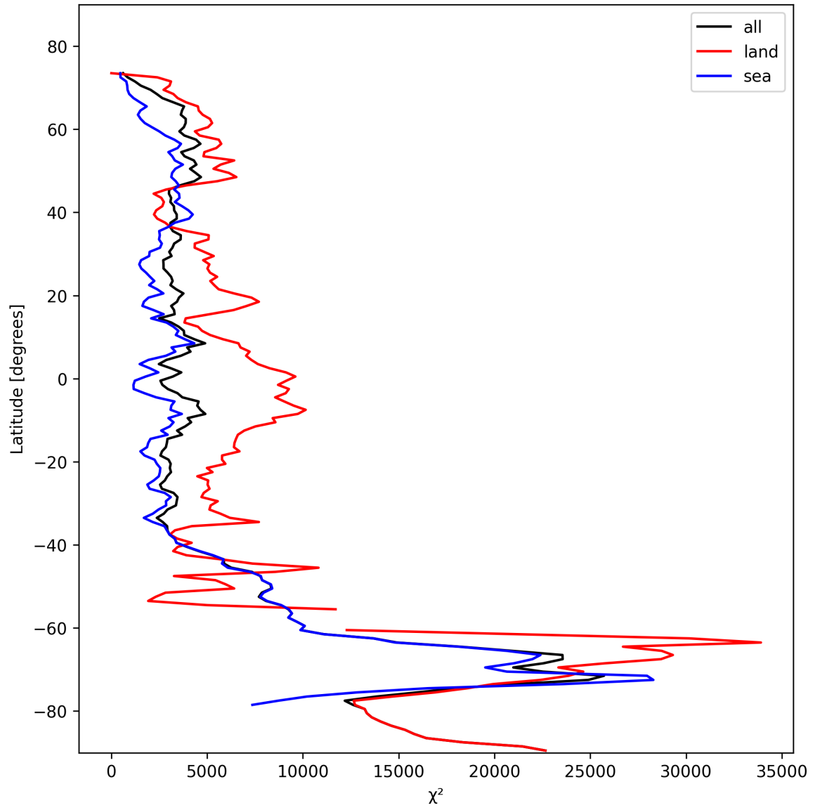
Figure 21: Zonal average of “ \chi^2 ” for 2024-11-01 to 2024-11-03.
