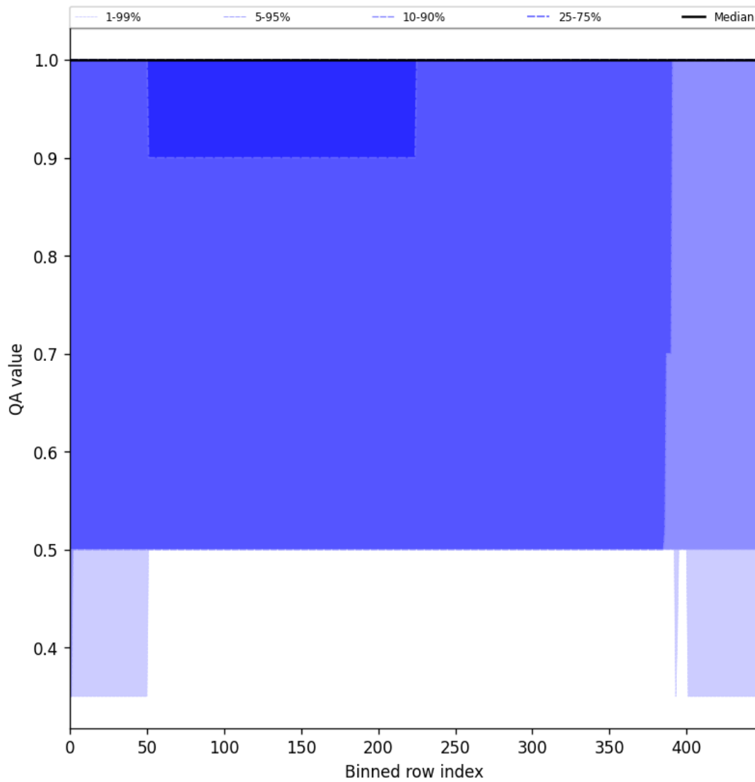
Figure 46: Along track statistics of “QA value” for 2024-11-01 to 2024-11-03
