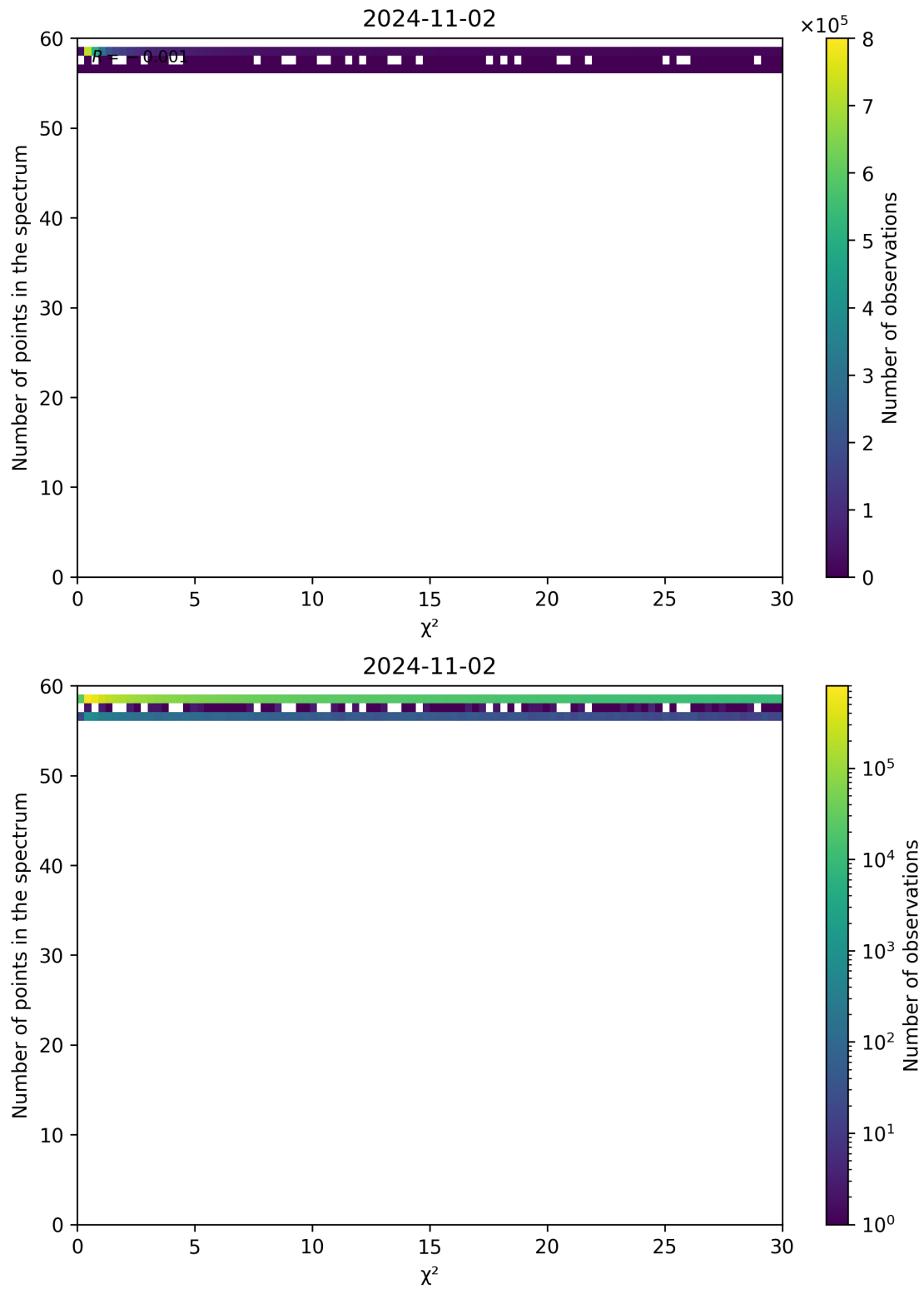
Figure 74: Scatter density plot of " \chi^2 " against "Number of points in the spectrum" for 2024-11-01 to 2024-11-03.
