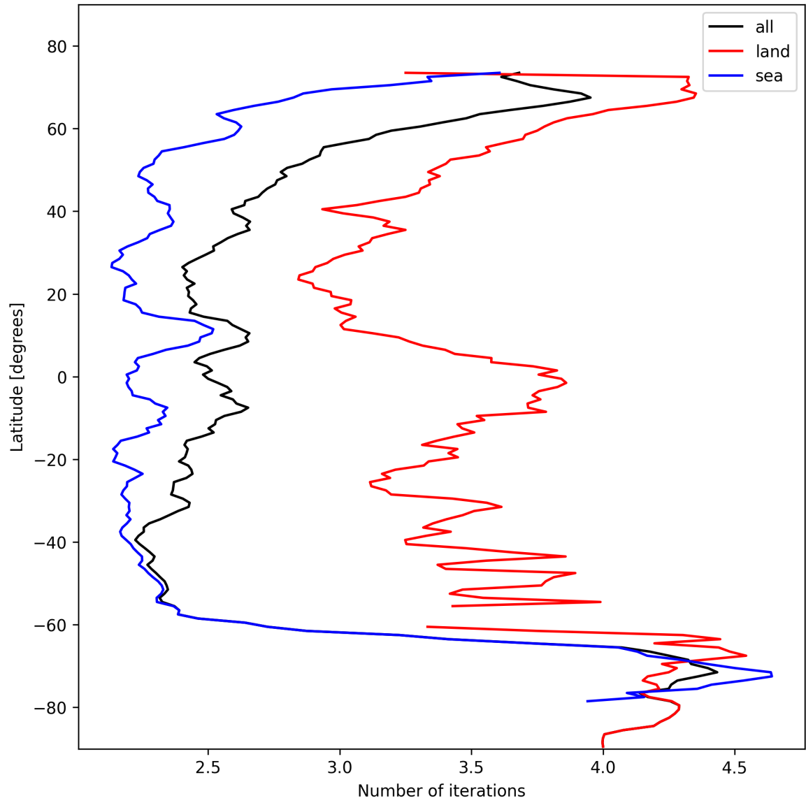
Figure 22: Zonal average of “Number of iterations” for 2024-11-01 to 2024-11-03.
