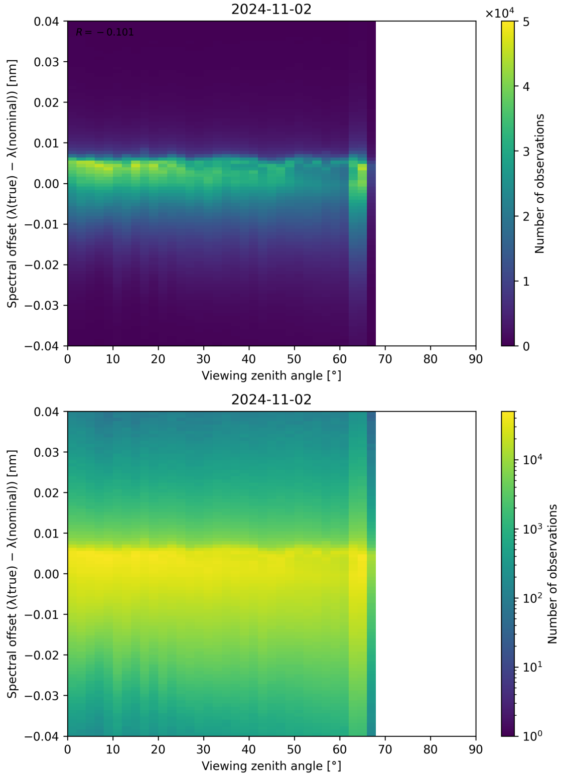
Figure 140: Scatter density plot of “Viewing zenith angle” against “Spectral offset ( \lambda_{\text{true}} - \lambda_{\text{nominal}} )” for 2024-11-01 to 2024-11-03.
