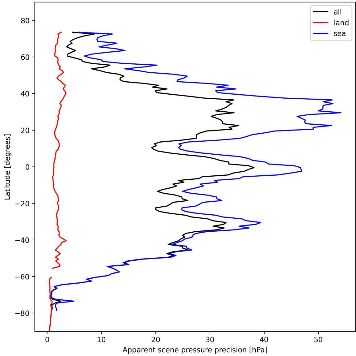
Figure 20: Zonal average of “Apparent scene pressure precision” for 2024-11-01 to 2024-11-03.
