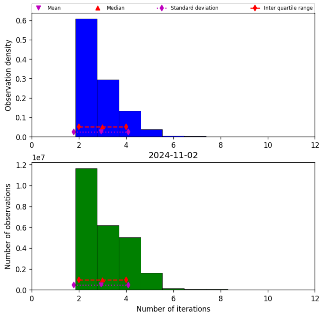
Figure 39: Histogram of “Number of iterations” for 2024-11-01 to 2024-11-03
