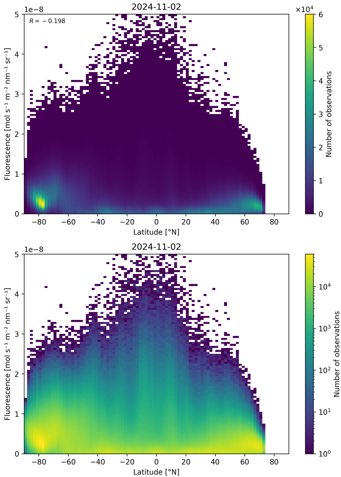
Figure 101: Scatter density plot of “Latitude” against “Fluorescence” for 2024-11-01 to 2024-11-03.
