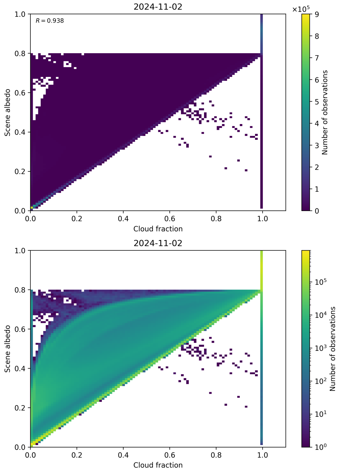
Figure 82: Scatter density plot of “Cloud fraction” against “Scene albedo” for 2024-11-01 to 2024-11-03.
