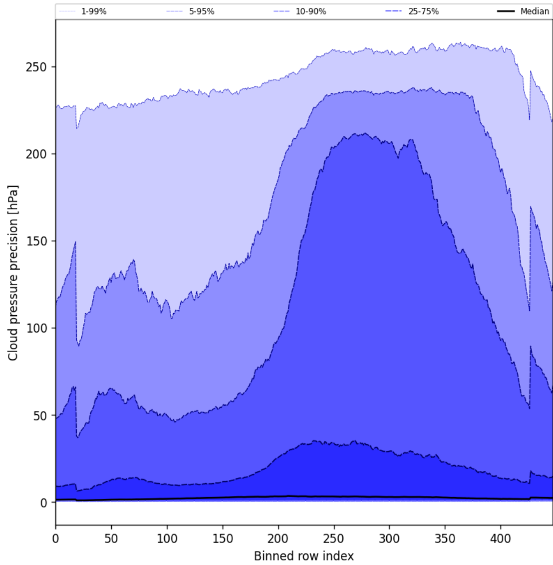
Figure 48: Along track statistics of “Cloud pressure precision” for 2024-11-01 to 2024-11-03
