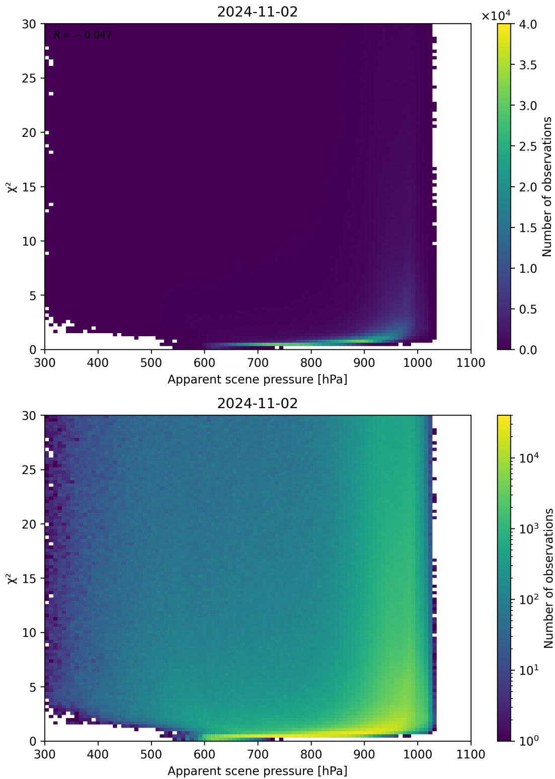
Figure 63: Scatter density plot of “Apparent scene pressure” against “ \chi^2 ” for 2024-11-01 to 2024-11-03.
