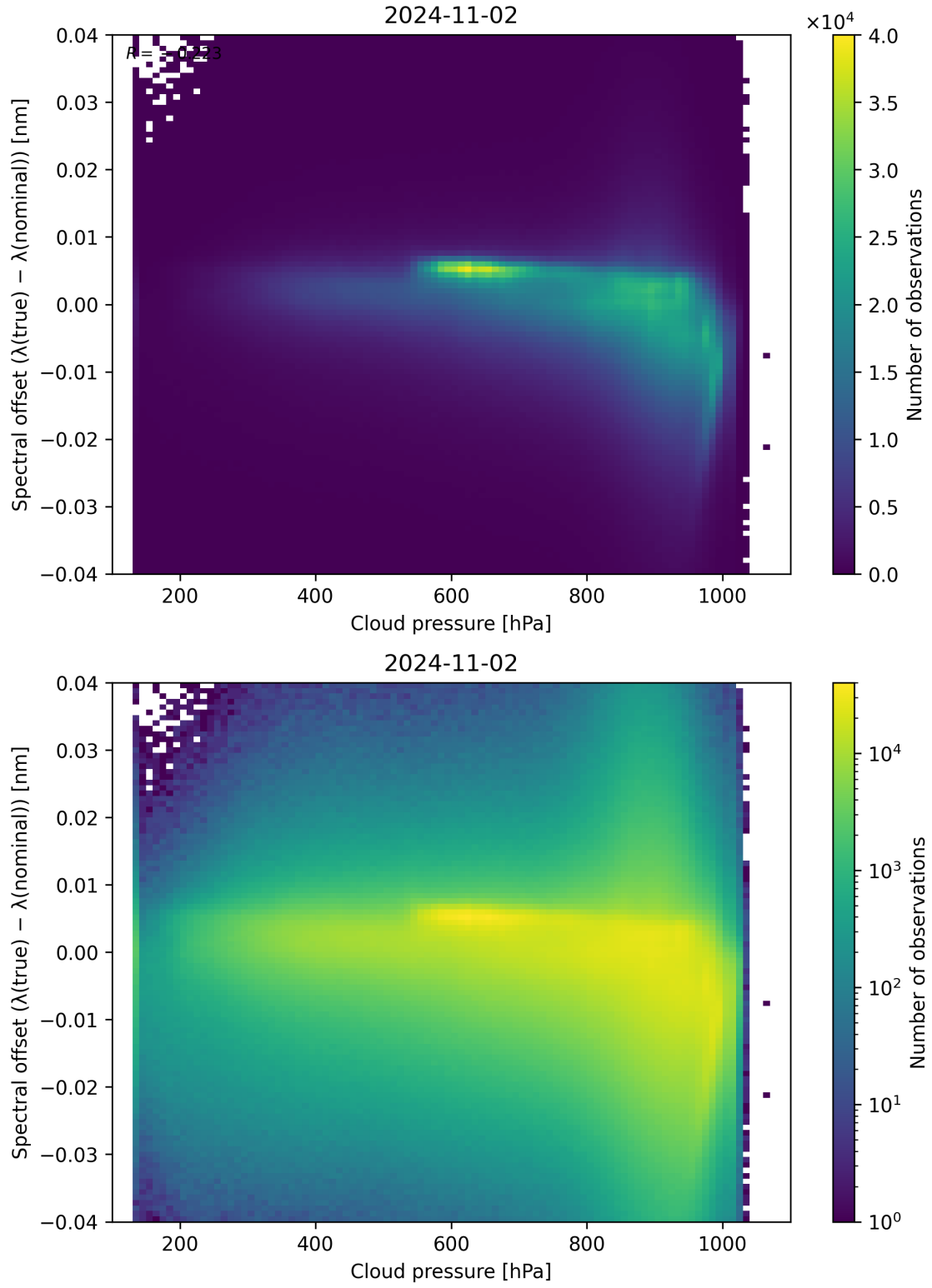
Figure 92: Scatter density plot of “Cloud pressure” against “Spectral offset ( \lambda_{\text{true}} - \lambda_{\text{nominal}} )” for 2024-11-01 to 2024-11-03.
