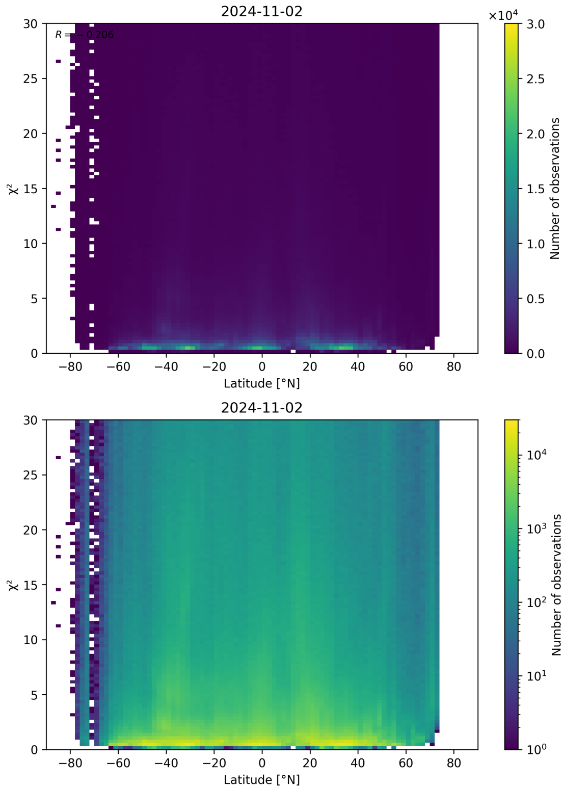
Figure 97: Scatter density plot of “Latitude” against “ \chi^2 ” for 2024-11-01 to 2024-11-03.
