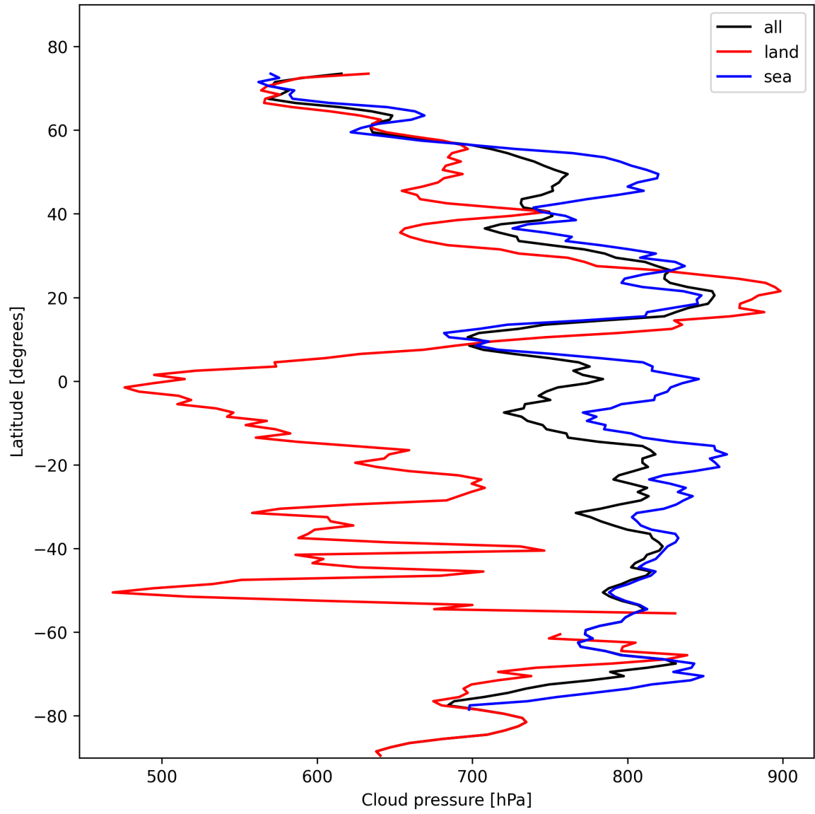
Figure 13: Zonal average of “Cloud pressure” for 2024-11-01 to 2024-11-03.
