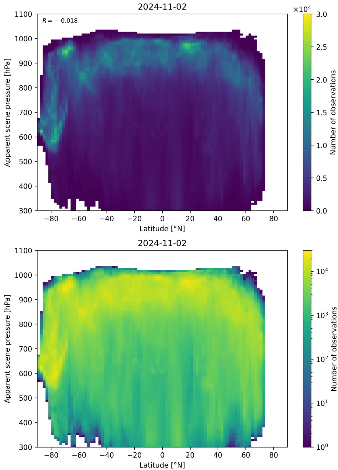
Figure 96: Scatter density plot of “Latitude” against “Apparent scene pressure” for 2024-11-01 to 2024-11-03.
