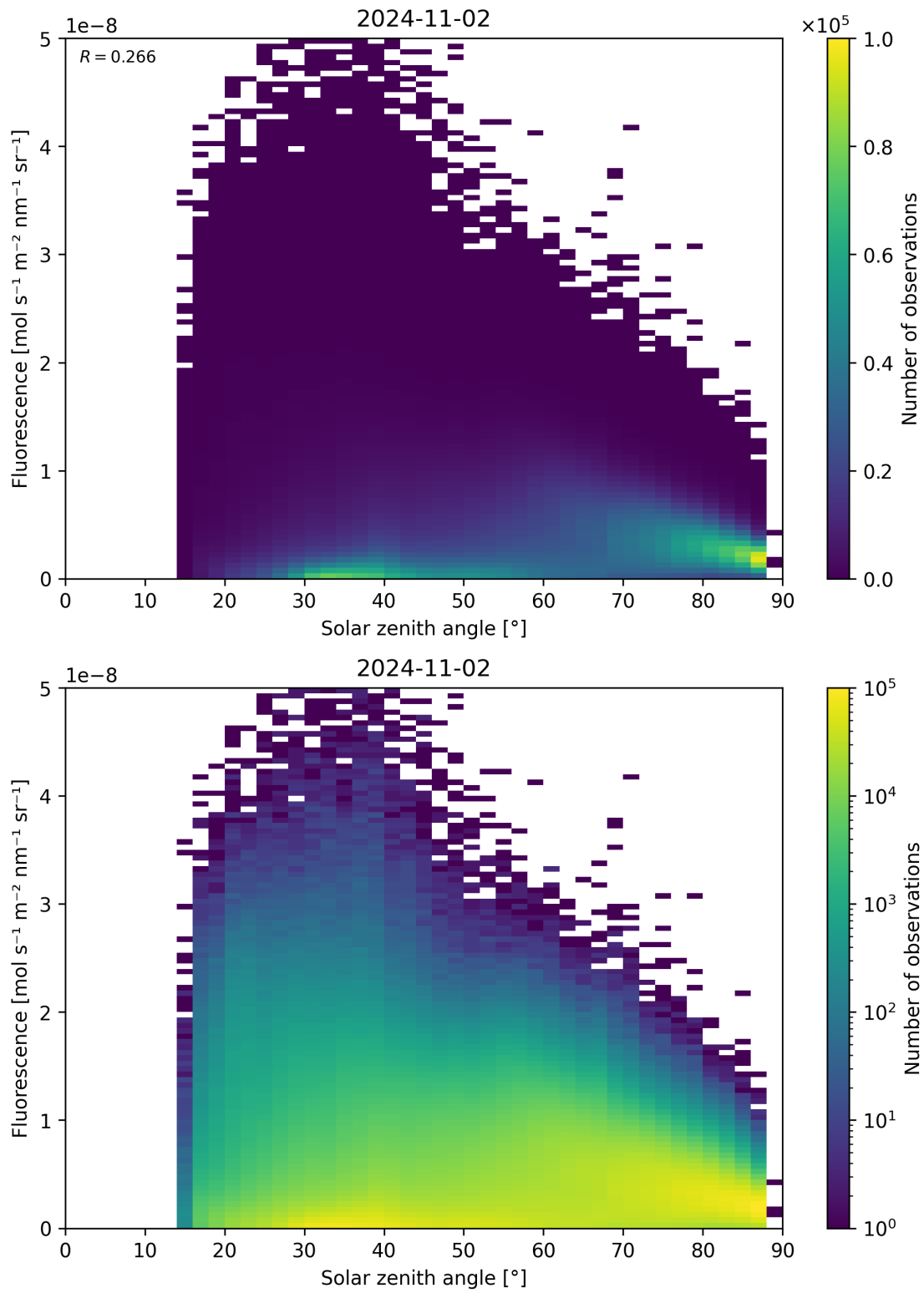
Figure 123: Scatter density plot of “Solar zenith angle” against “Fluorescence” for 2024-11-01 to 2024-11-03.
