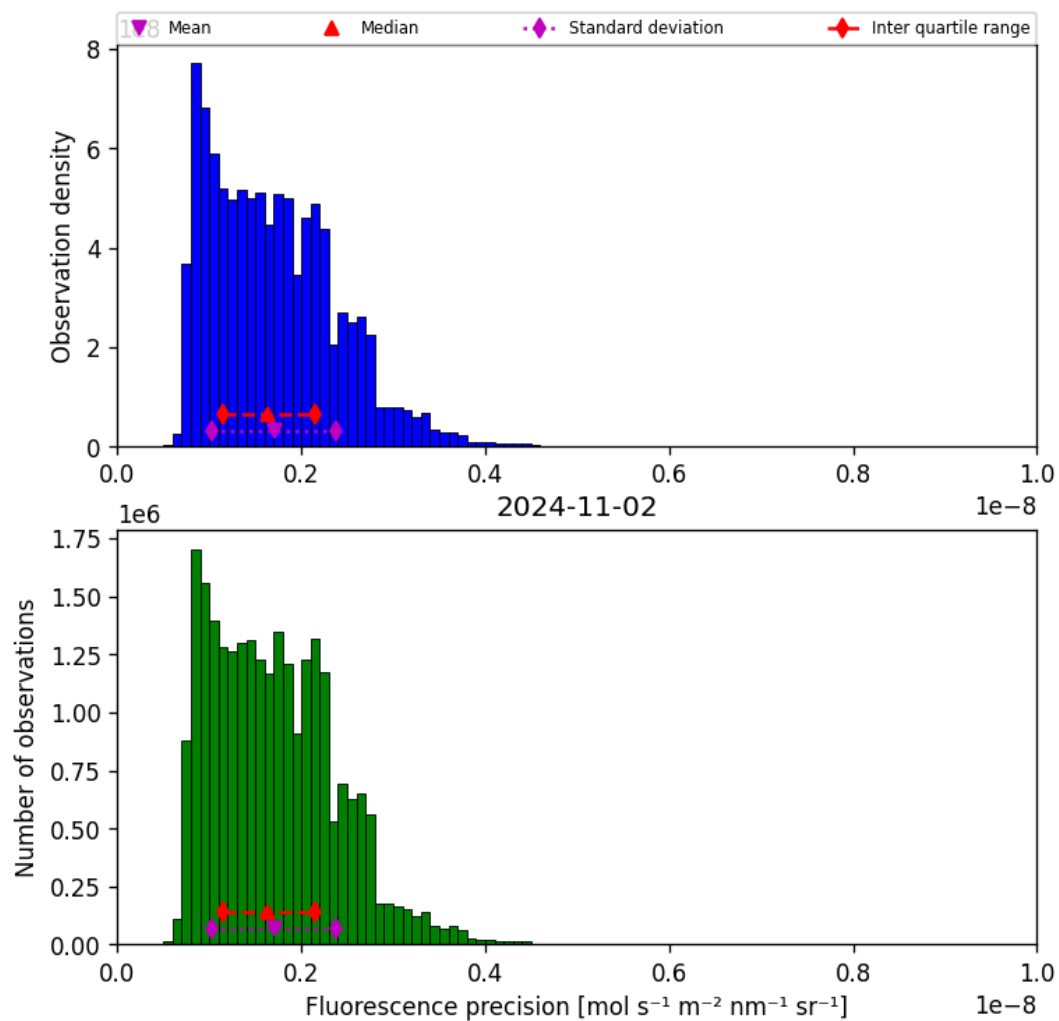
Figure 41: Histogram of “Fluorescence precision” for 2024-11-01 to 2024-11-03
