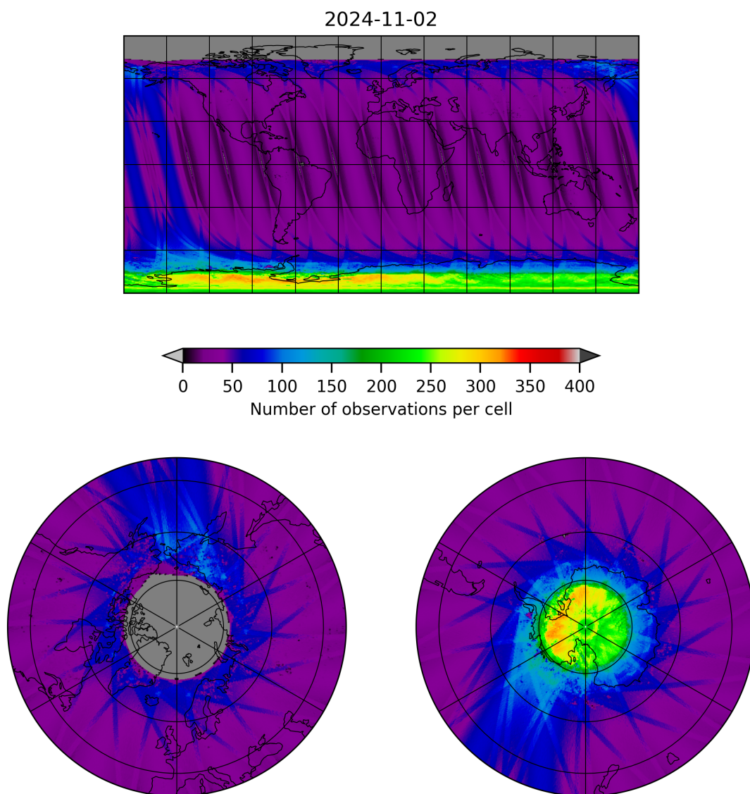
Figure 11: Map of the number of observations for 2024-11-01 to 2024-11-03
