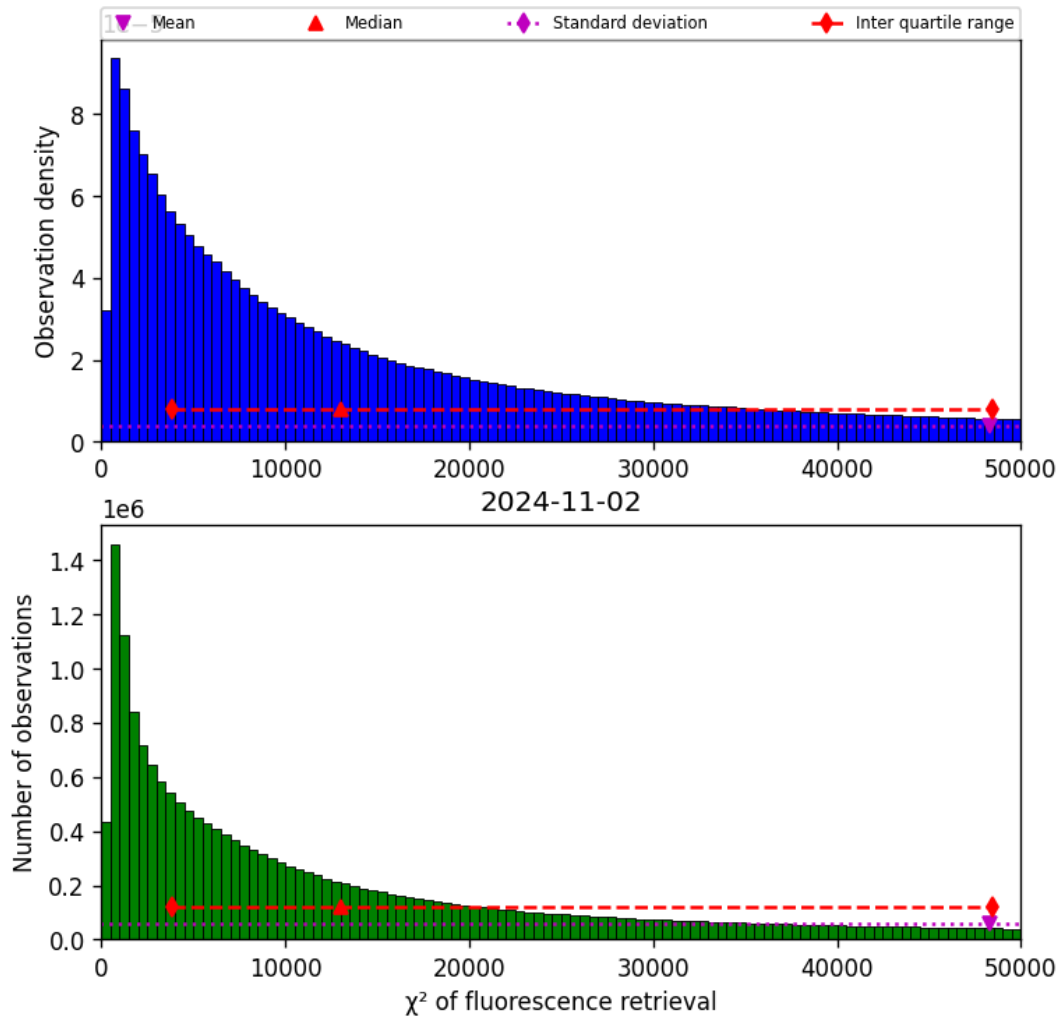
Figure 42: Histogram of “ \chi^2 of fluorescence retrieval” for 2024-11-01 to 2024-11-03
