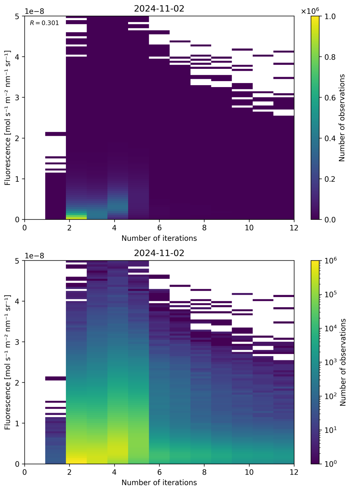
Figure 107: Scatter density plot of “Number of iterations” against “Fluorescence” for 2024-11-01 to 2024-11-03.
