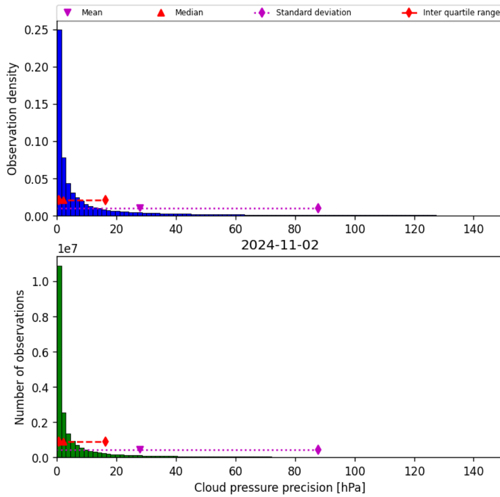
Figure 31: Histogram of “Cloud pressure precision” for 2024-11-01 to 2024-11-03
