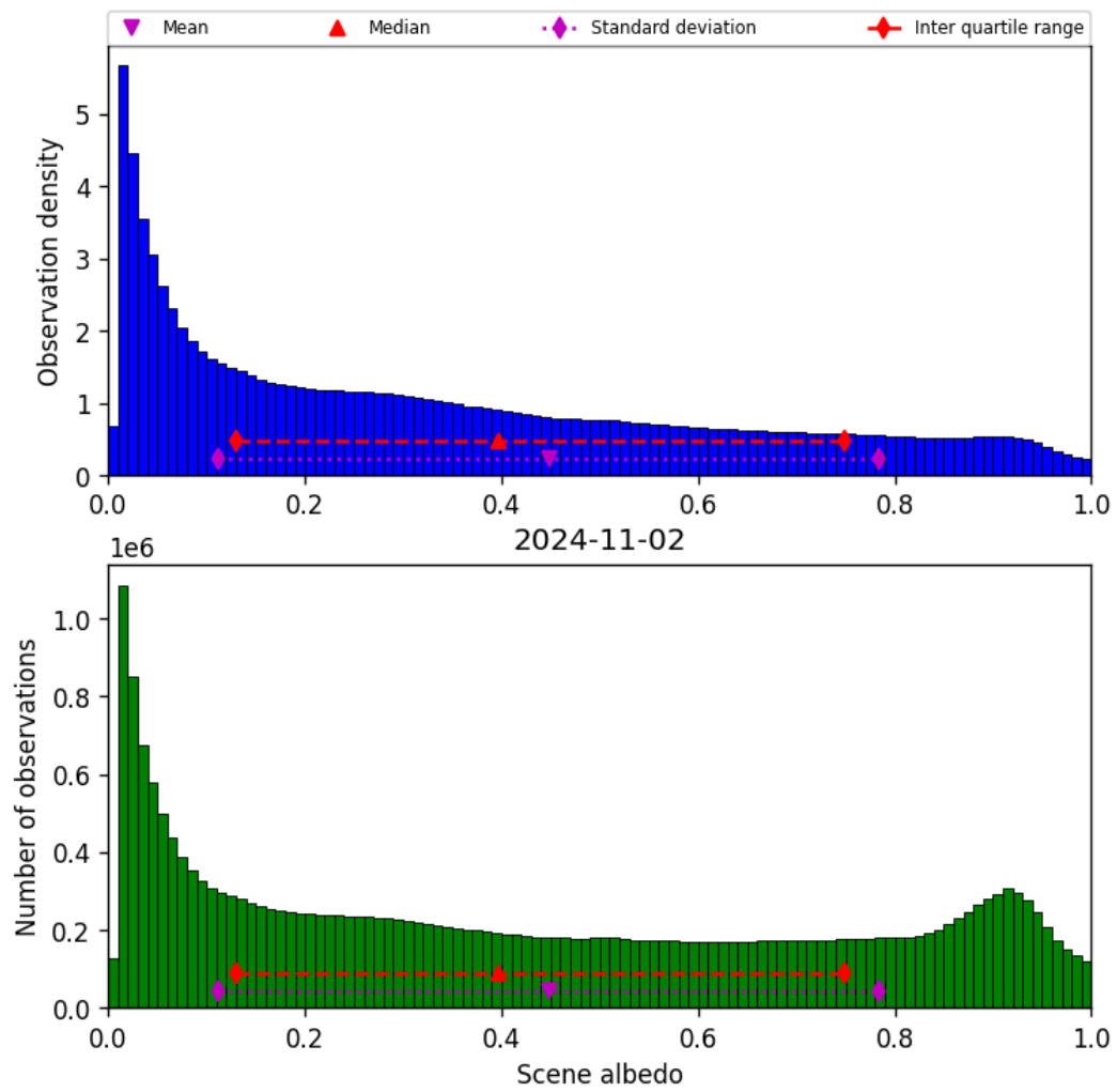
Figure 34: Histogram of “Scene albedo” for 2024-11-01 to 2024-11-03
