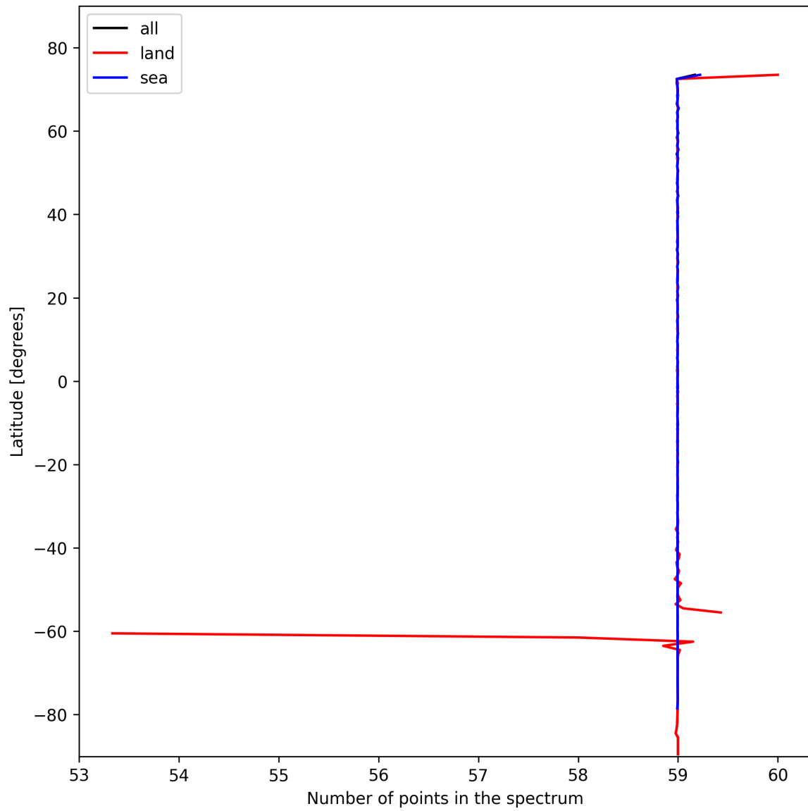
Figure 27: Zonal average of “Number of points in the spectrum” for 2024-11-01 to 2024-11-03.
