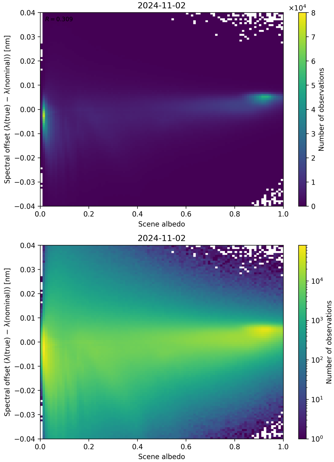
Figure 117: Scatter density plot of “Scene albedo” against “Spectral offset ( \lambda_{\text{true}} - \lambda_{\text{nominal}} )” for 2024-11-01 to 2024-11-03.
