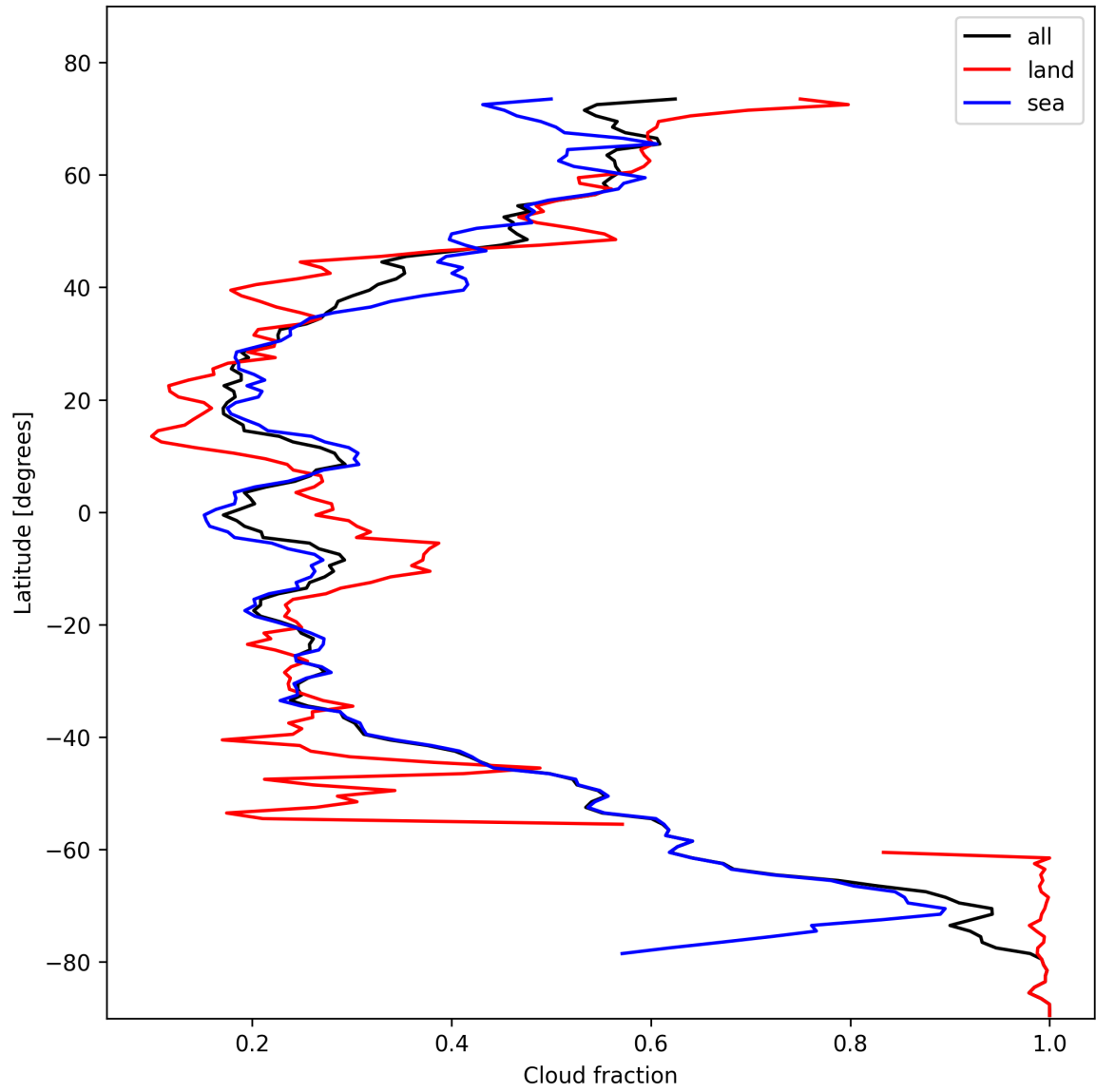
Figure 15: Zonal average of “Cloud fraction” for 2024-11-01 to 2024-11-03.
