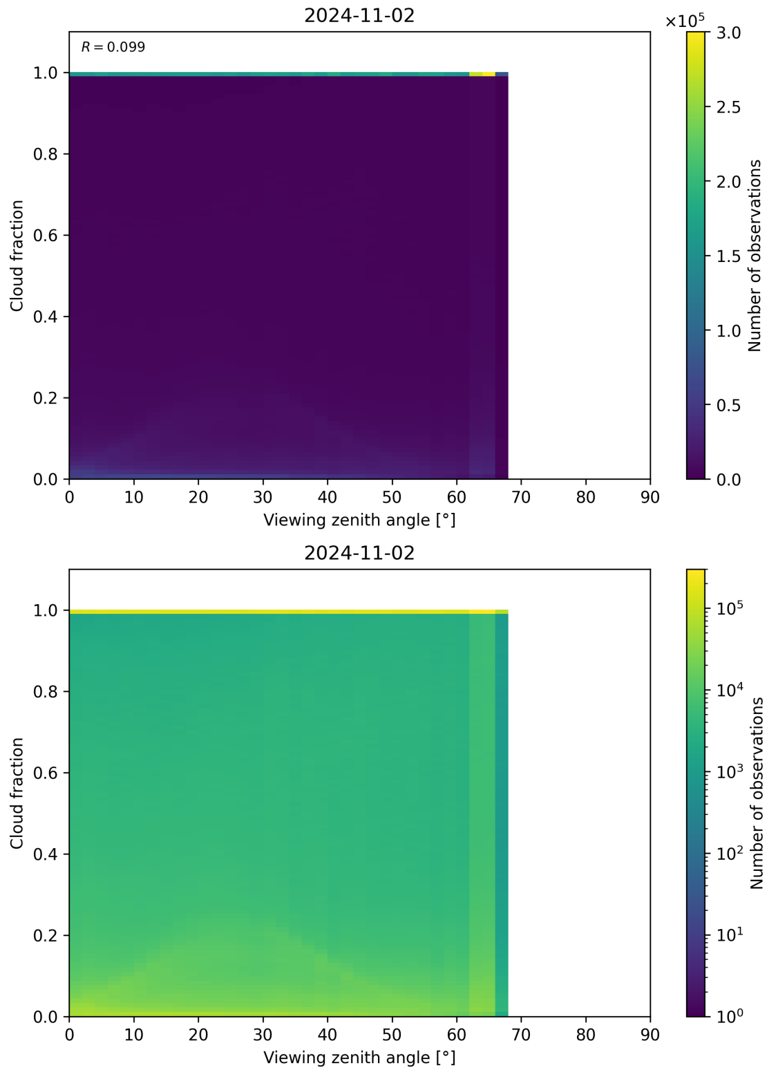
Figure 132: Scatter density plot of “Viewing zenith angle” against “Cloud fraction” for 2024-11-01 to 2024-11-03.
