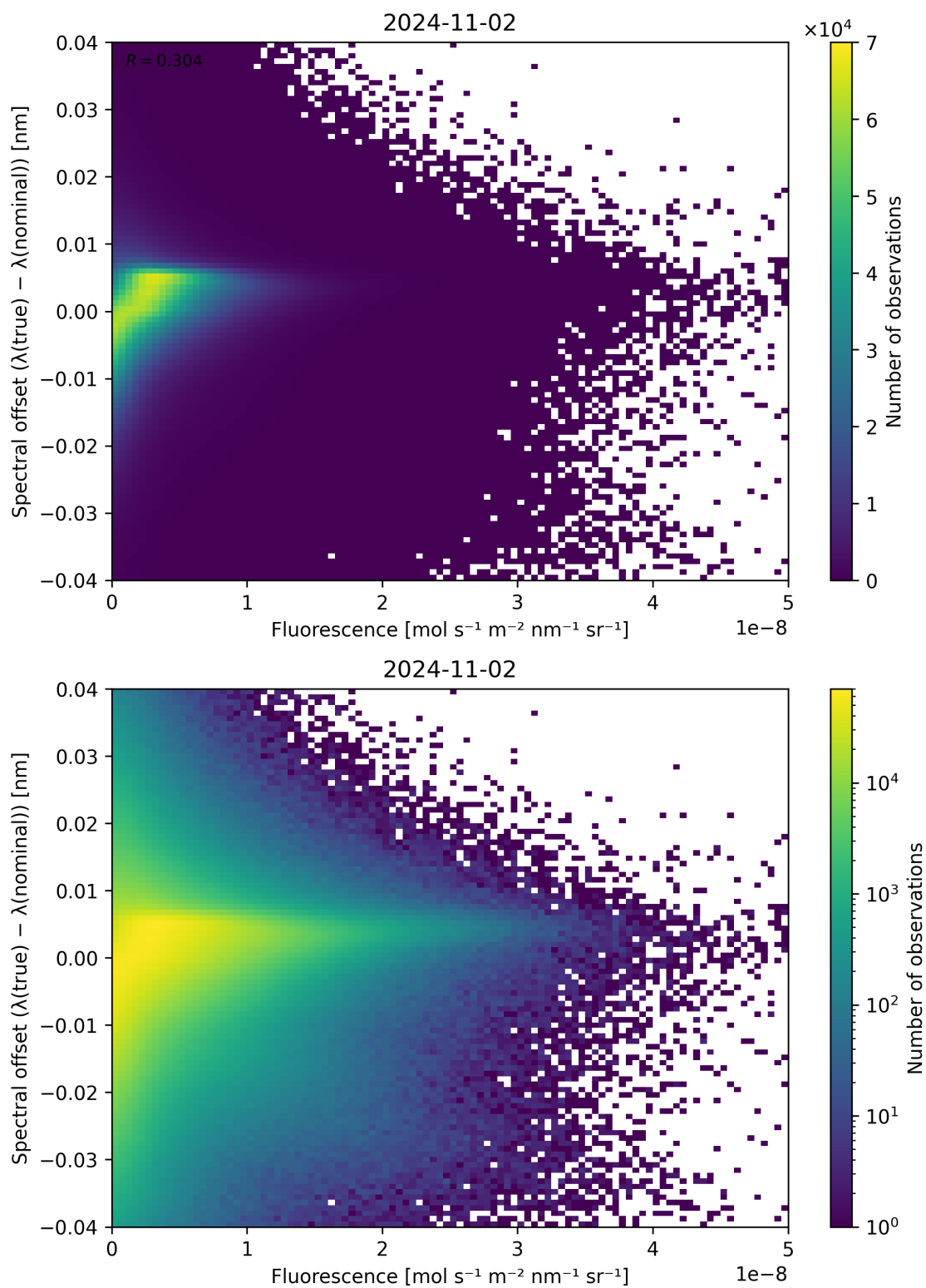
Figure 95: Scatter density plot of “Fluorescence” against “Spectral offset ( \lambda_{\text{true}} - \lambda_{\text{nominal}} )” for 2024-11-01 to 2024-11-03.
