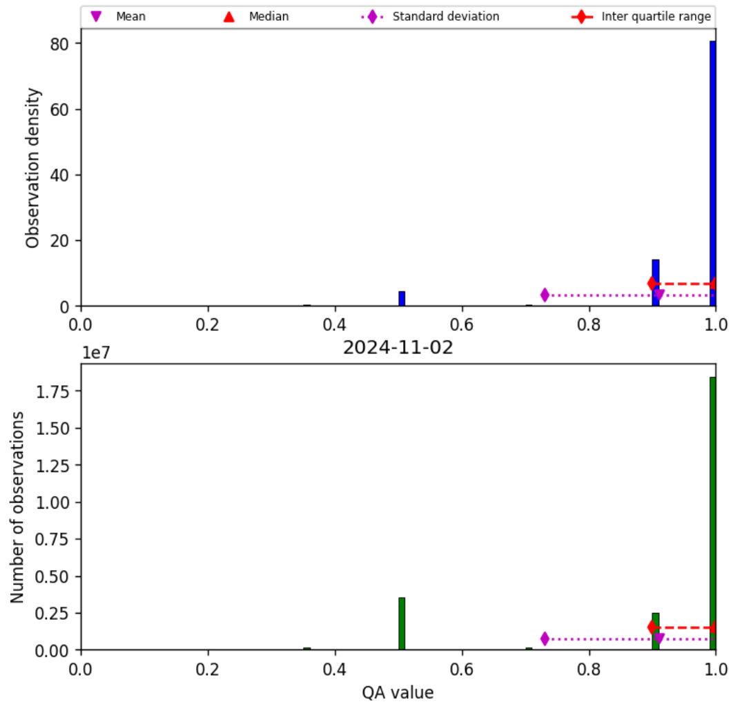
Figure 29: Histogram of “QA value” for 2024-11-01 to 2024-11-03
