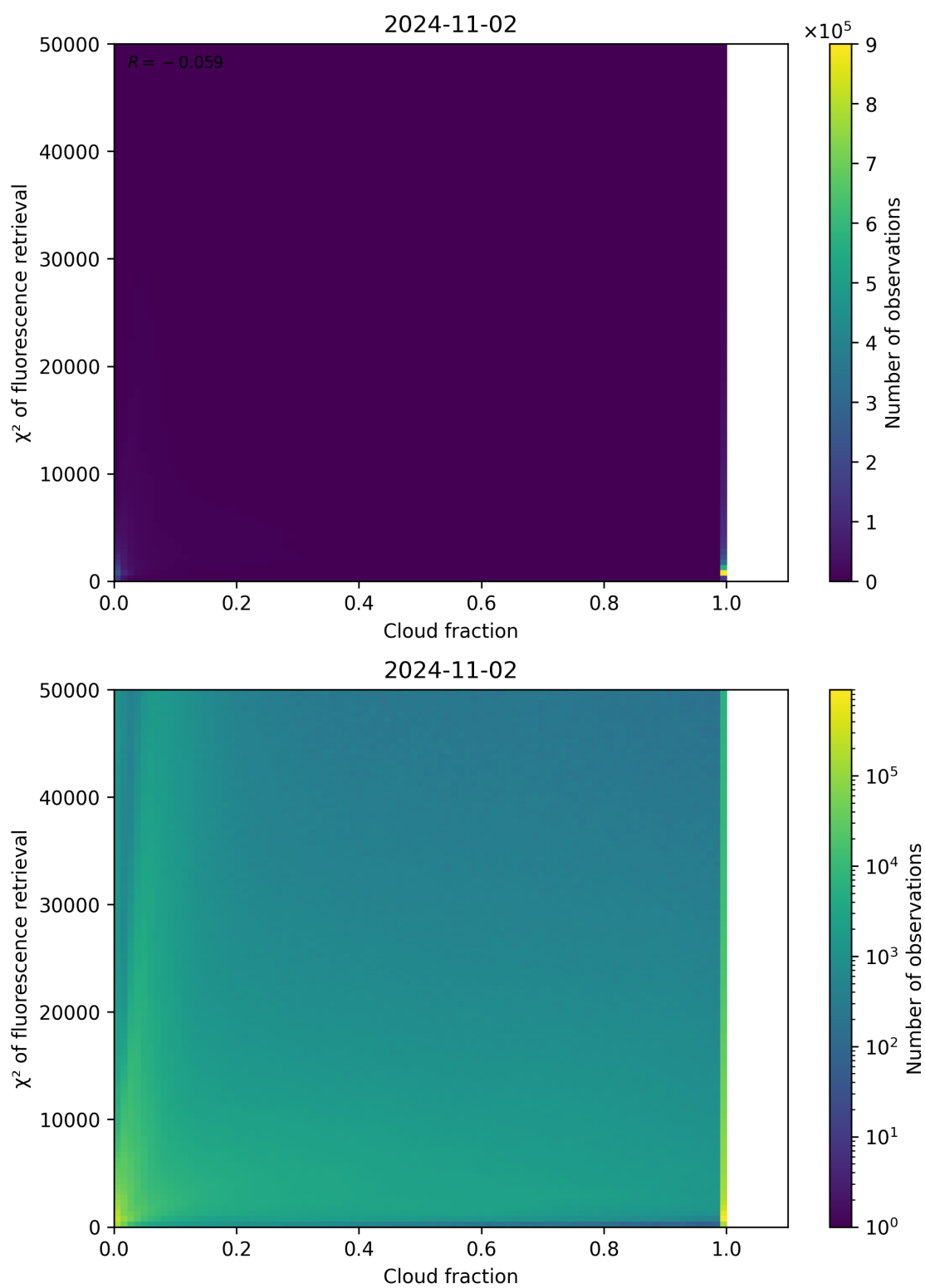
Figure 78: Scatter density plot of “Cloud fraction” against “ \chi^2 of fluorescence retrieval” for 2024-11-01 to 2024-11-03.
