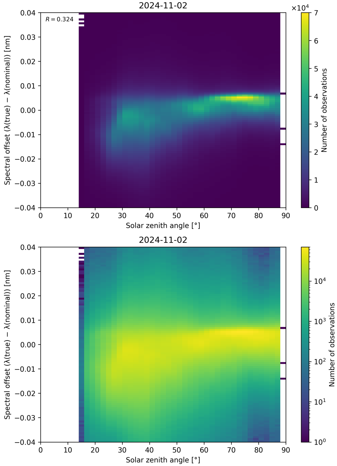
Figure 128: Scatter density plot of “Solar zenith angle” against “Spectral offset ( \lambda_{\text{true}} - \lambda_{\text{nominal}} )” for 2024-11-01 to 2024-11-03.
