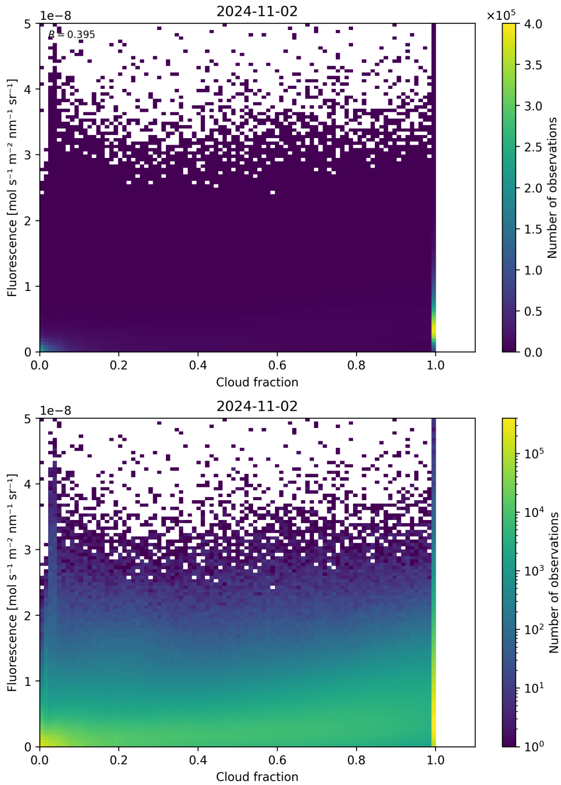
Figure 79: Scatter density plot of “Cloud fraction” against “Fluorescence” for 2024-11-01 to 2024-11-03.
