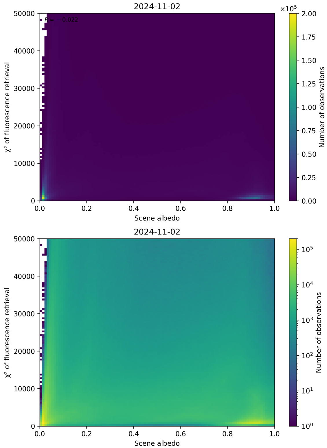
Figure 113: Scatter density plot of “Scene albedo” against “ \chi^2 of fluorescence retrieval” for 2024-11-01 to 2024-11-03.
