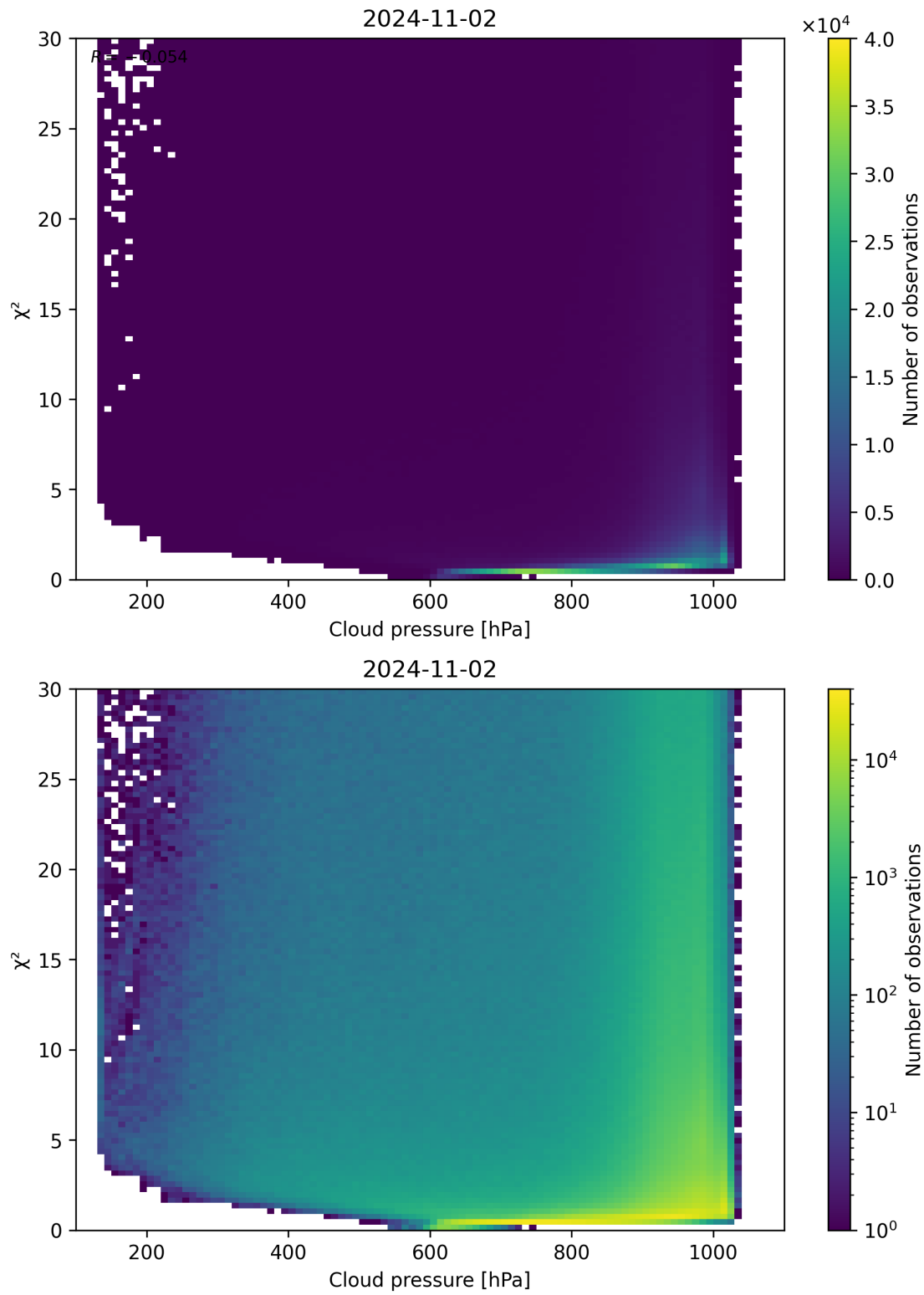
Figure 85: Scatter density plot of “Cloud pressure” against “ \chi^2 ” for 2024-11-01 to 2024-11-03.
