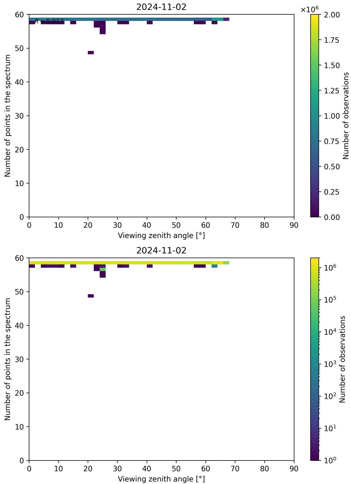
Figure 137: Scatter density plot of “Viewing zenith angle” against “Number of points in the spectrum” for 2024-11-01 to 2024-11-03.
