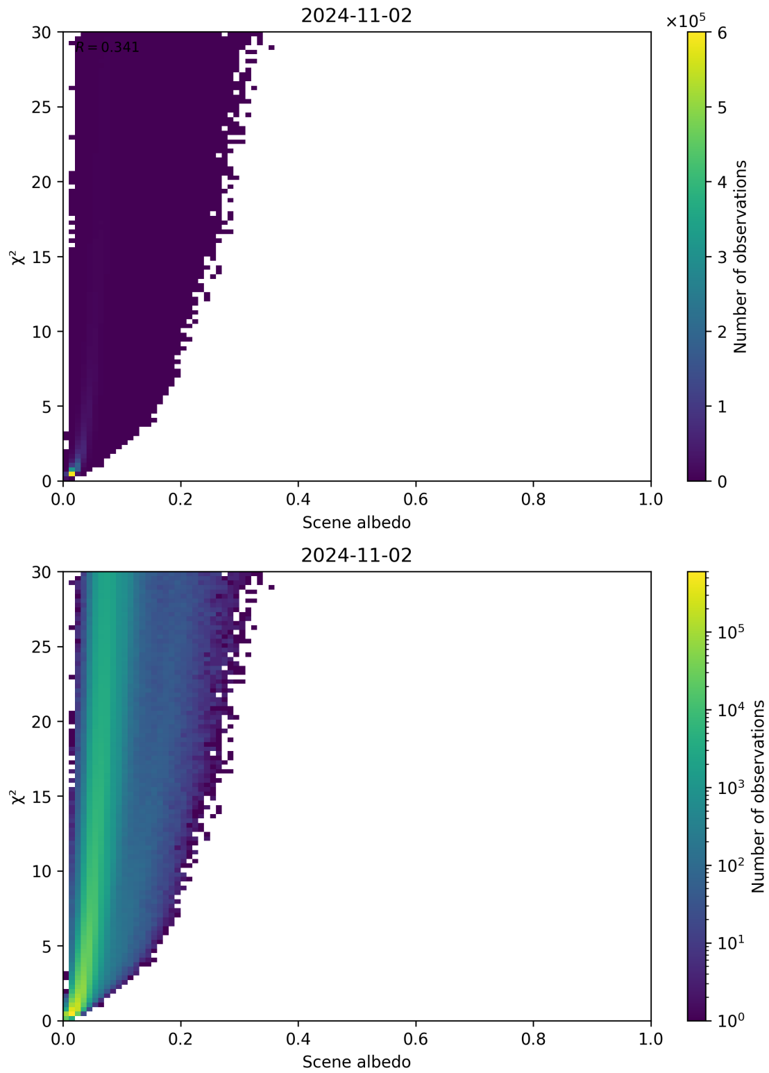
Figure 112: Scatter density plot of “Scene albedo” against “ \chi^2 ” for 2024-11-01 to 2024-11-03.
