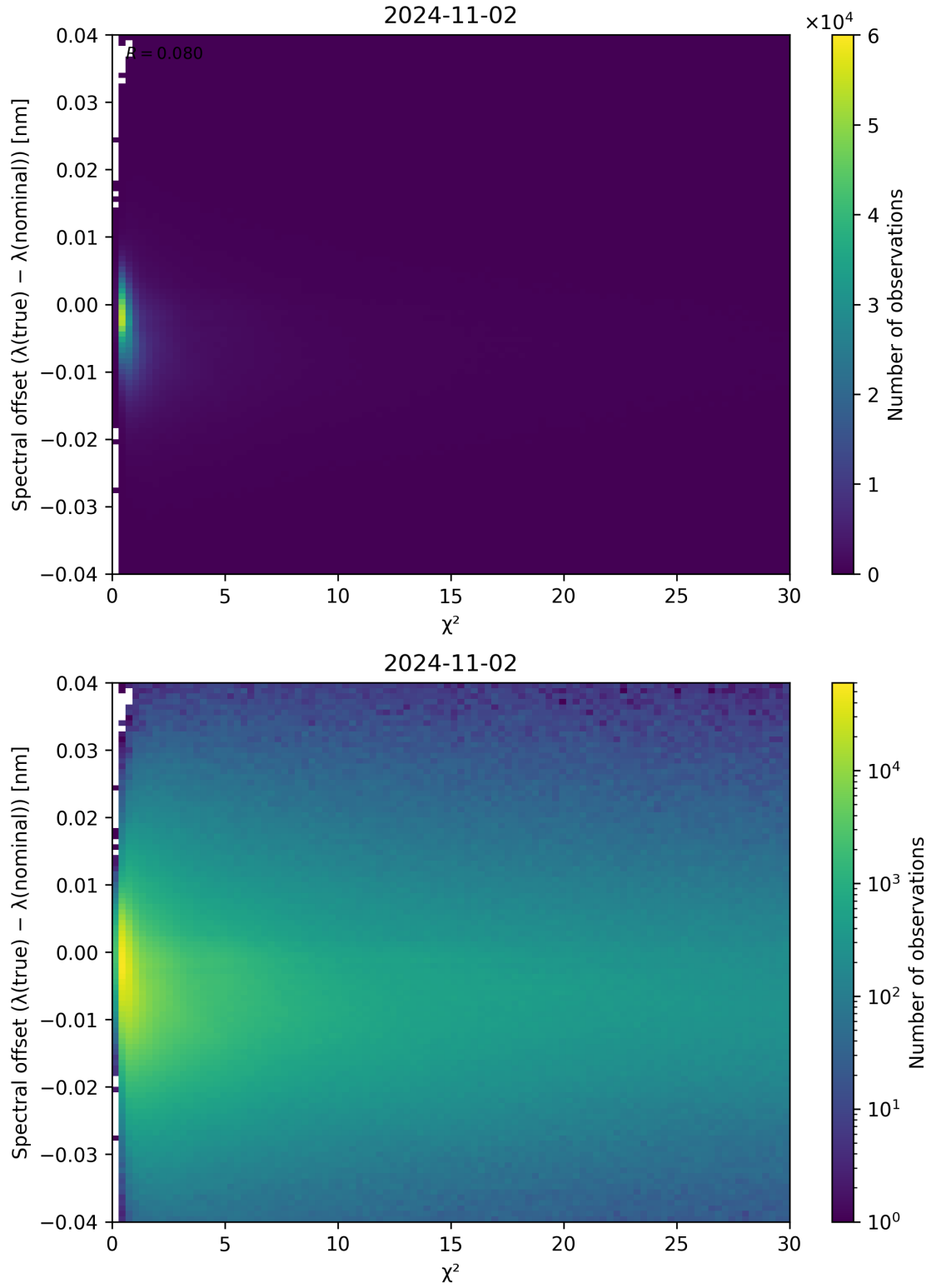
Figure 75: Scatter density plot of “ \chi^2 ” against “Spectral offset ( \lambda_{\text{true}} - \lambda_{\text{nominal}} )” for 2024-11-01 to 2024-11-03.
