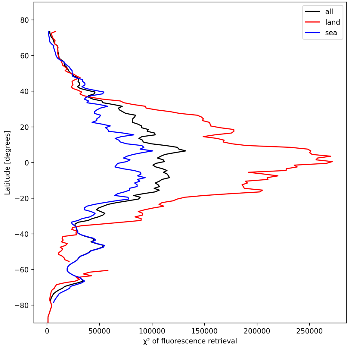
Figure 25: Zonal average of “ \chi^2 of fluorescence retrieval” for 2024-11-01 to 2024-11-03.
