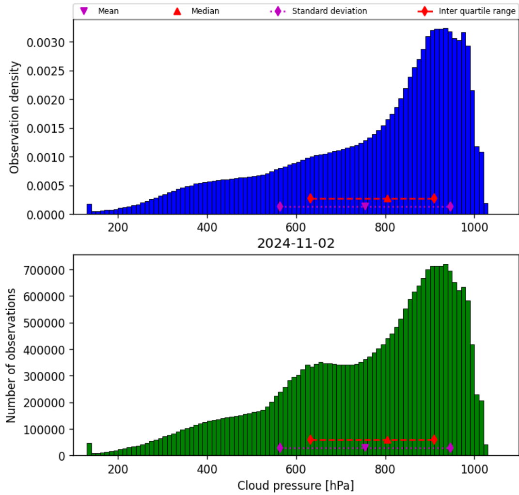
Figure 30: Histogram of “Cloud pressure” for 2024-11-01 to 2024-11-03
