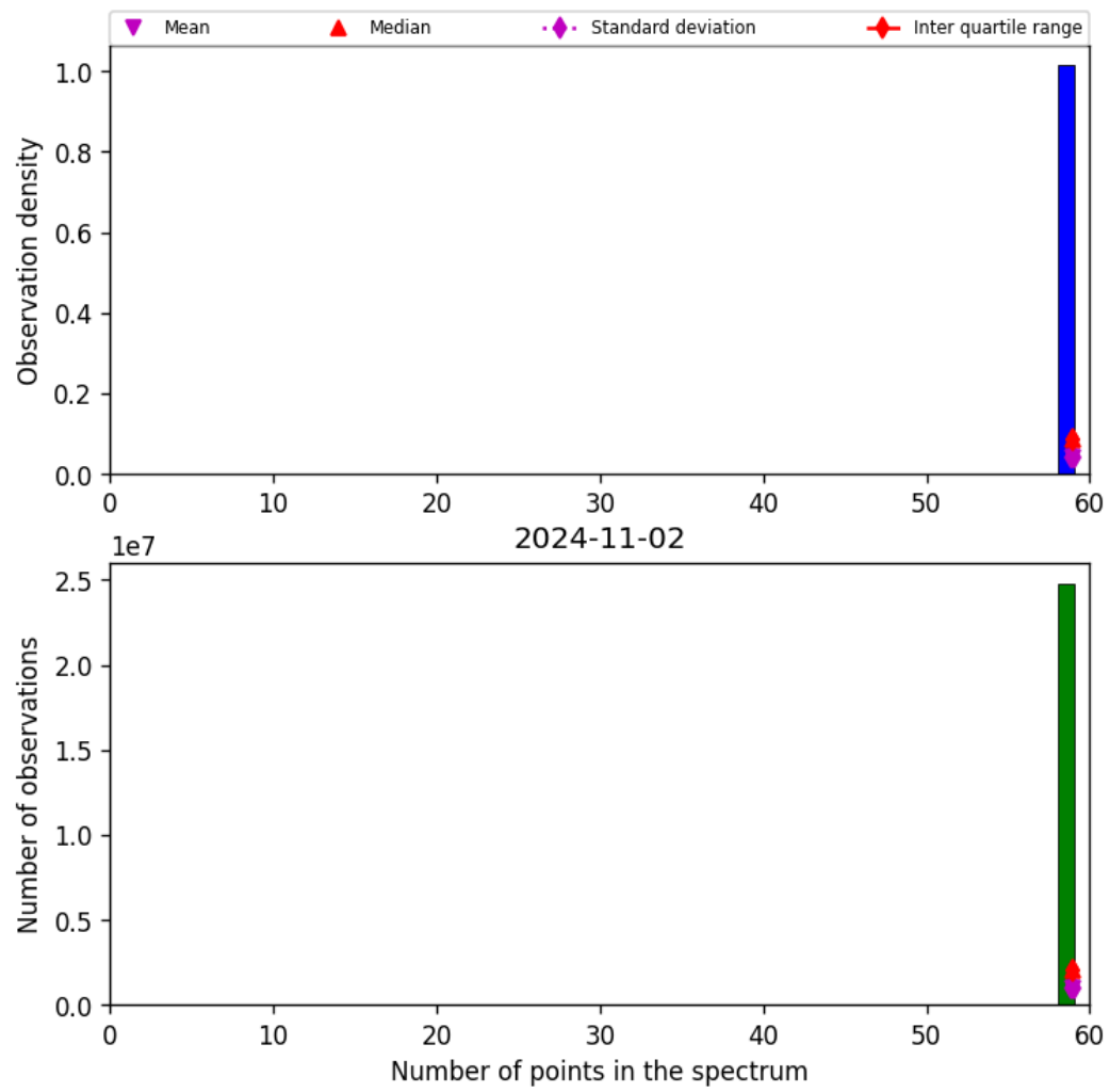
Figure 44: Histogram of “Number of points in the spectrum” for 2024-11-01 to 2024-11-03
