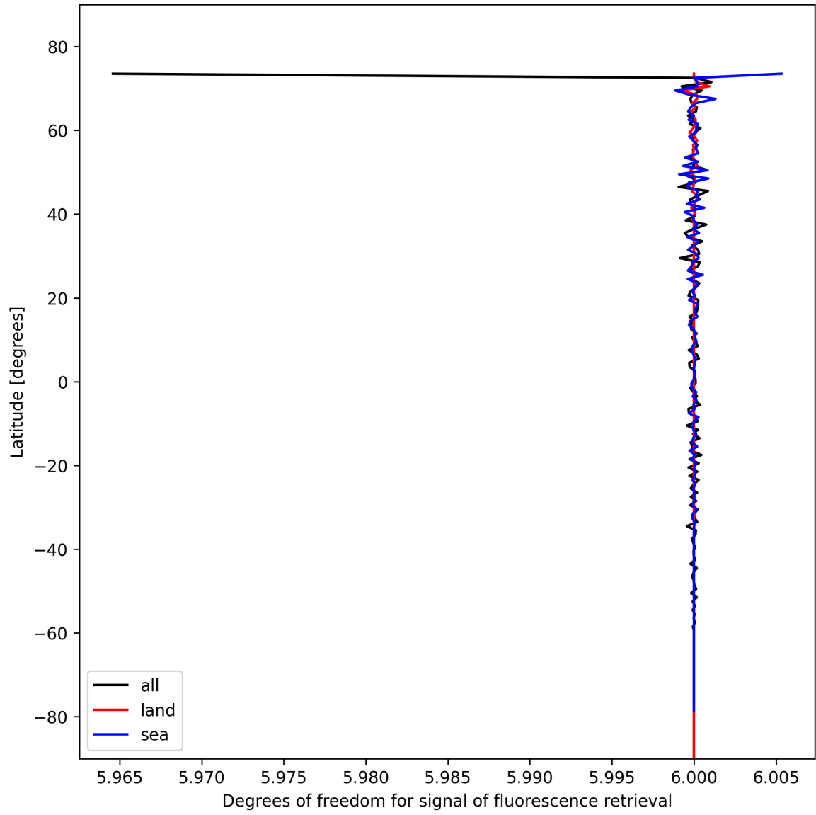
Figure 26: Zonal average of “Degrees of freedom for signal of fluorescence retrieval” for 2024-11-01 to 2024-11-03.
