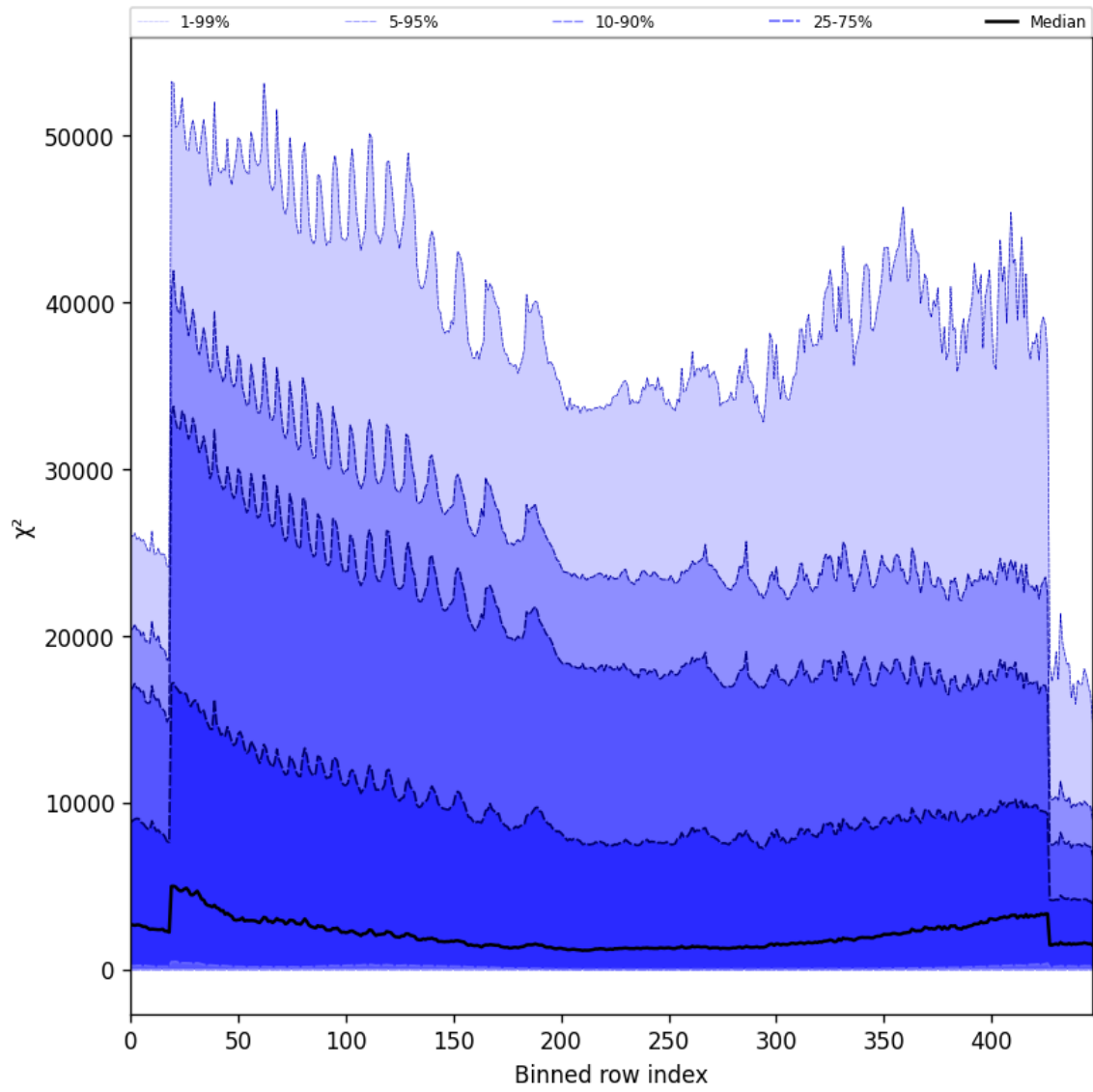
Figure 55: Along track statistics of “ \chi^2 ” for 2024-11-01 to 2024-11-03
