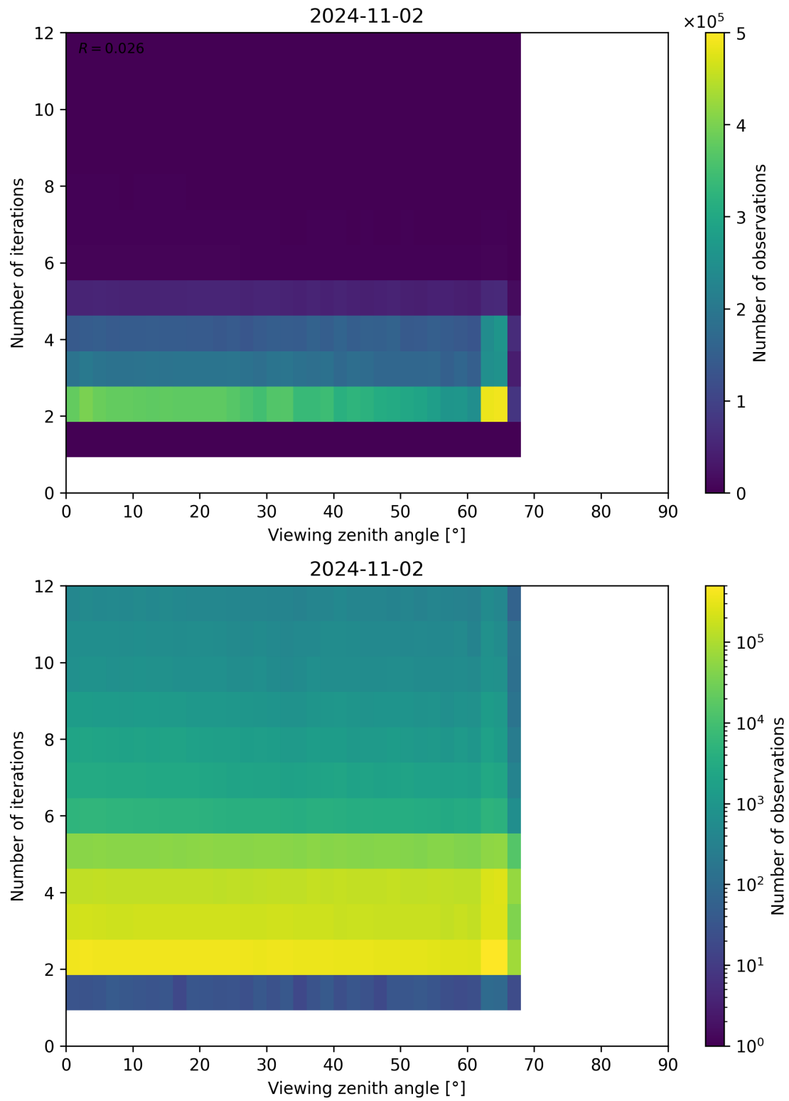
Figure 136: Scatter density plot of “Viewing zenith angle” against “Number of iterations” for 2024-11-01 to 2024-11-03.
