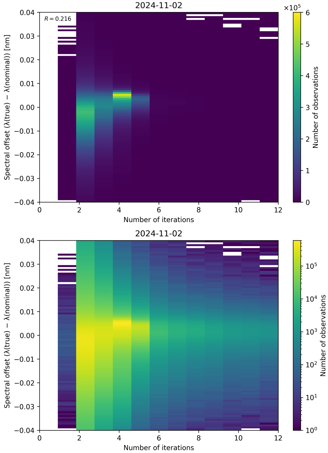
Figure 109: Scatter density plot of “Number of iterations” against “Spectral offset ( \lambda_{\text{true}} - \lambda_{\text{nominal}} )” for 2024-11-01 to 2024-11-03.
