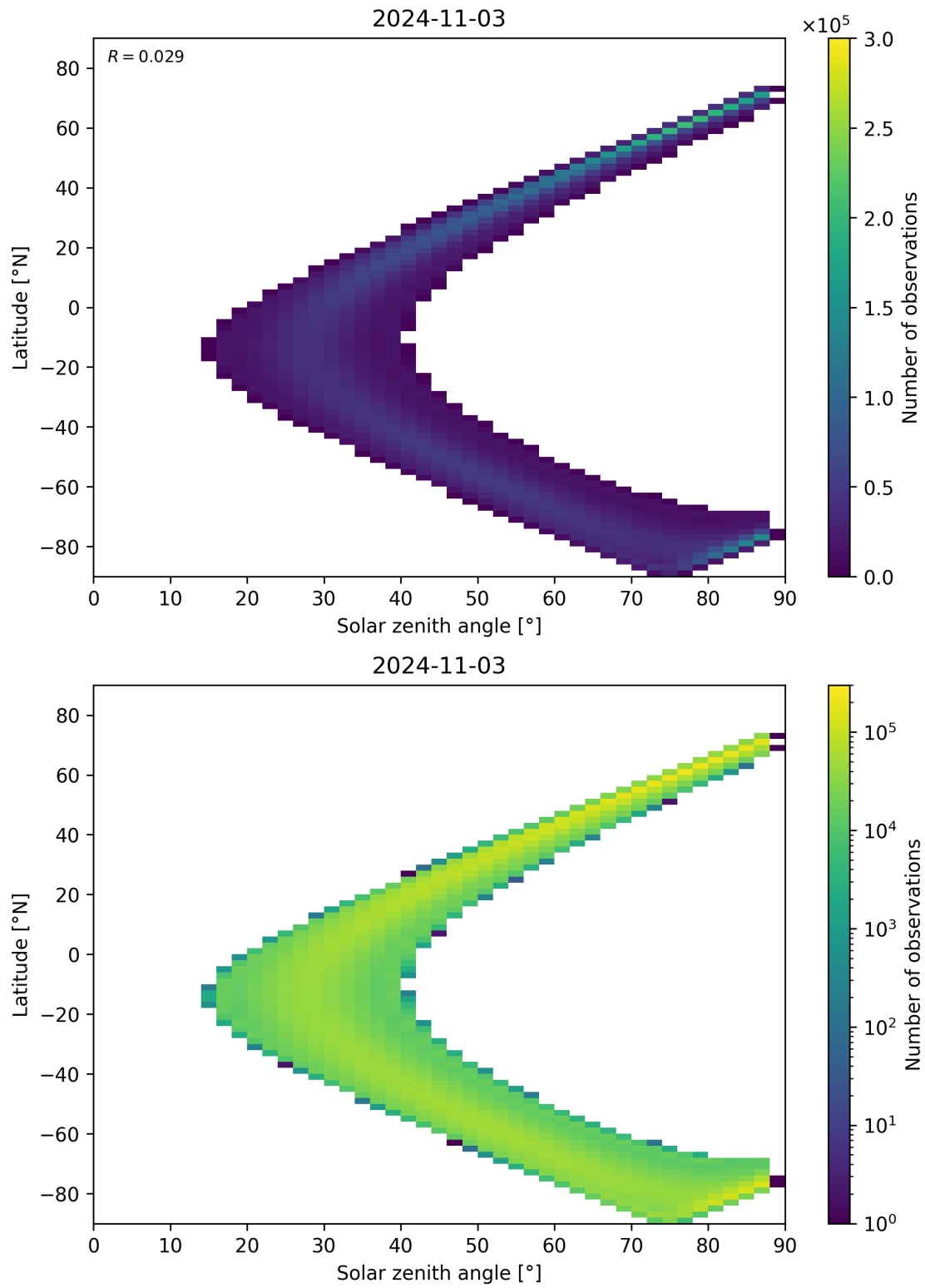
Figure 124: Scatter density plot of “Solar zenith angle” against “Latitude” for 2024-11-02 to 2024-11-04.
