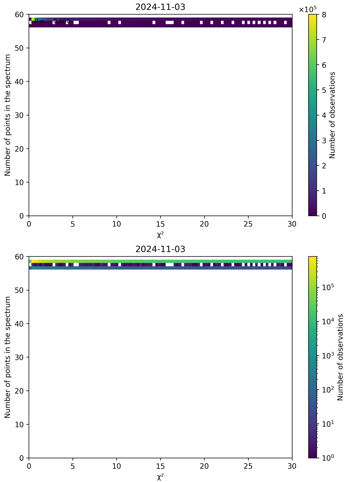
Figure 74: Scatter density plot of “ \chi^2 ” against “Number of points in the spectrum” for 2024-11-02 to 2024-11-04.
