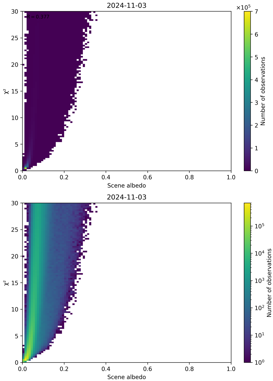
Figure 112: Scatter density plot of “Scene albedo” against “ \chi^2 ” for 2024-11-02 to 2024-11-04.
