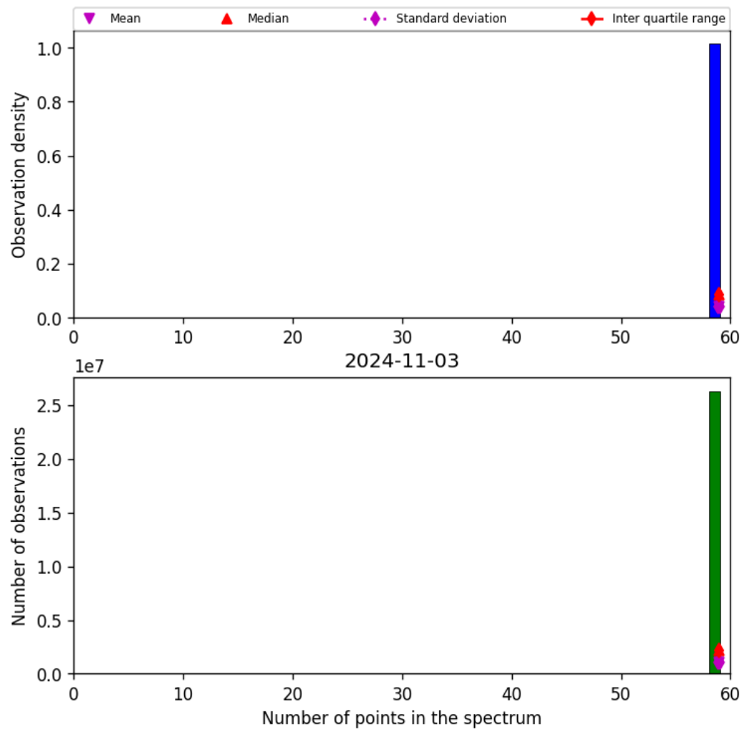
Figure 44: Histogram of “Number of points in the spectrum” for 2024-11-02 to 2024-11-04
