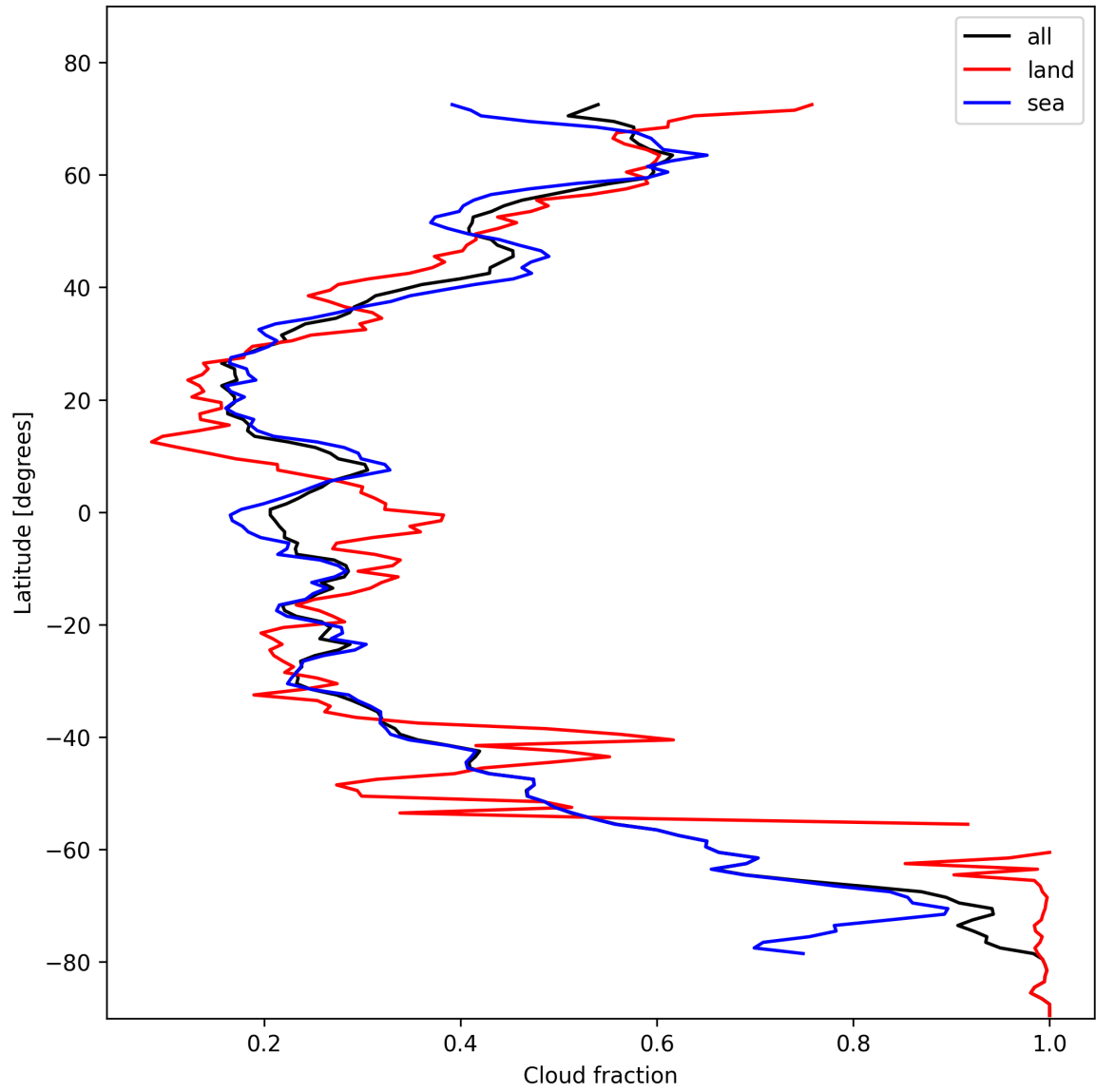
Figure 15: Zonal average of “Cloud fraction” for 2024-11-02 to 2024-11-04.
