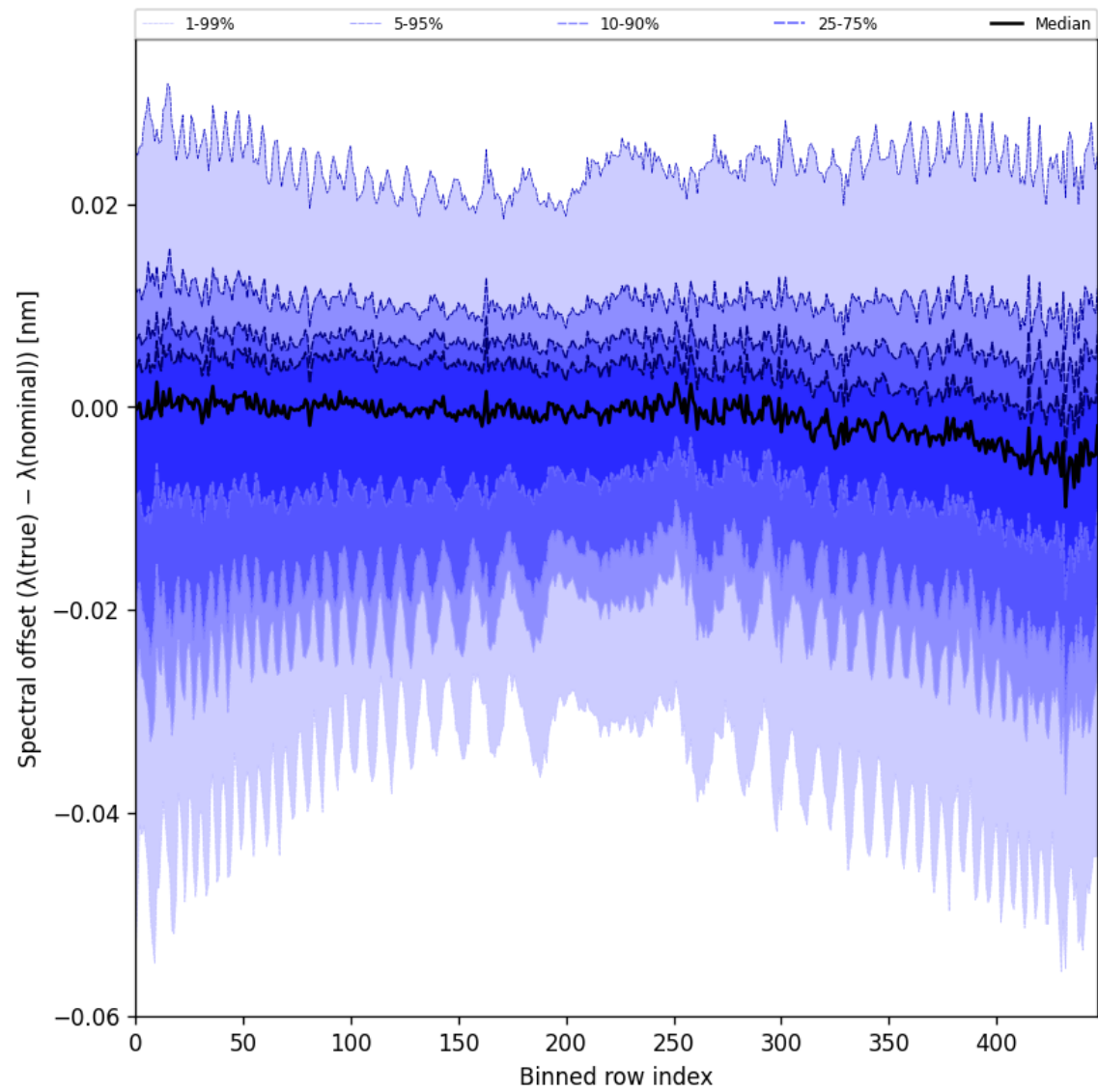
Figure 62: Along track statistics of “Spectral offset ( \lambda_{\text{true}} - \lambda_{\text{nominal}} )” for 2024-11-02 to 2024-11-04
