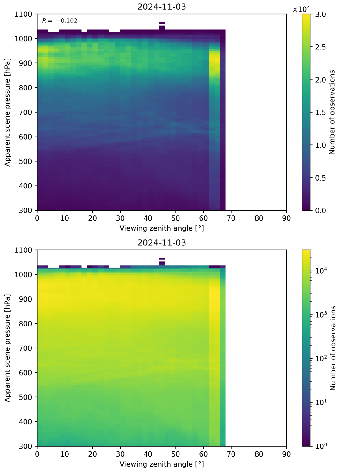
Figure 129: Scatter density plot of “Viewing zenith angle” against “Apparent scene pressure” for 2024-11-02 to 2024-11-04.
