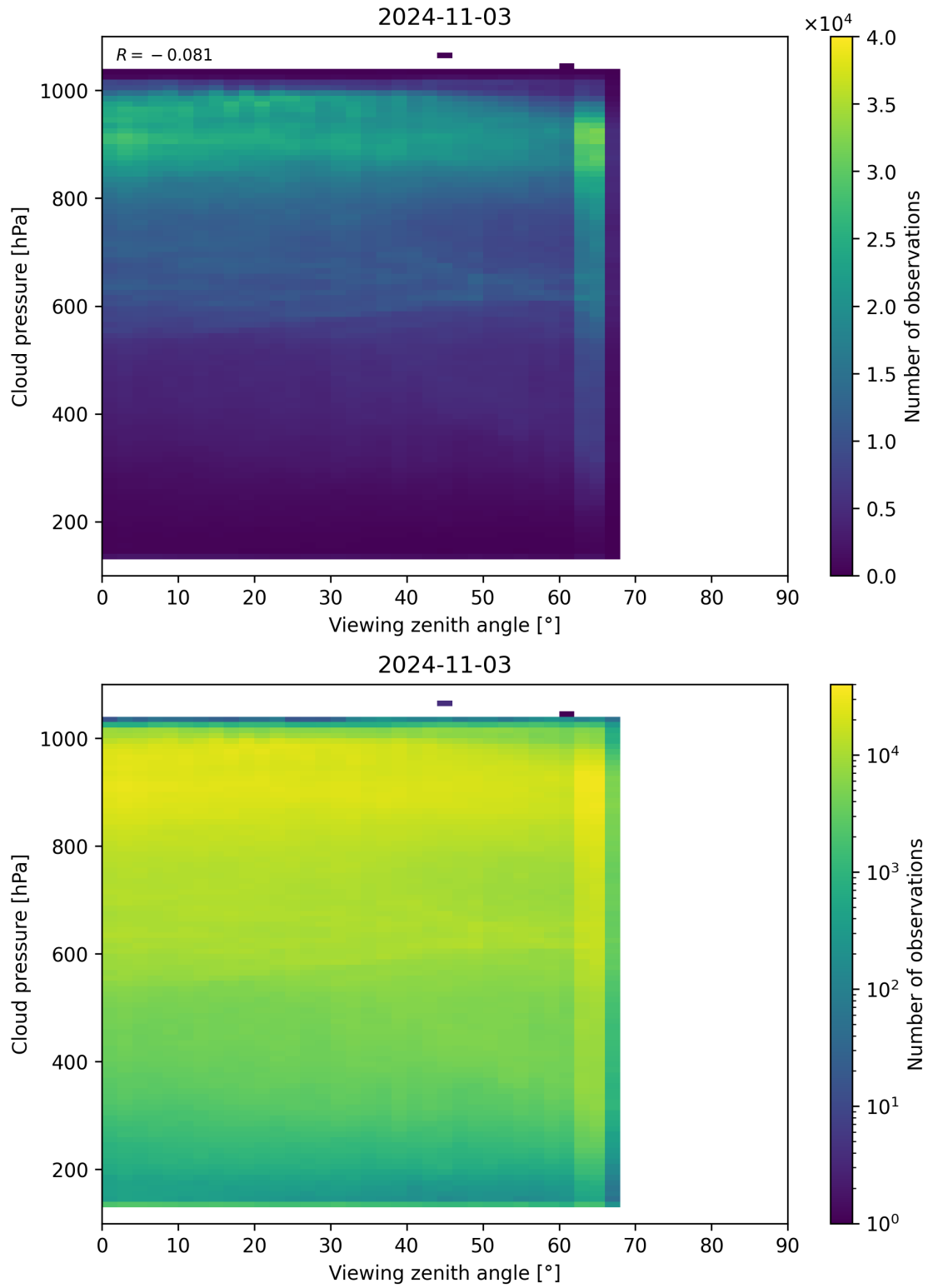
Figure 133: Scatter density plot of “Viewing zenith angle” against “Cloud pressure” for 2024-11-02 to 2024-11-04.
