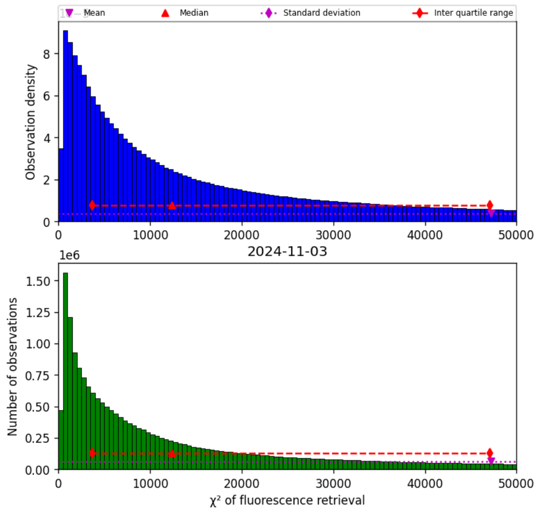
Figure 42: Histogram of “ \chi^2 of fluorescence retrieval” for 2024-11-02 to 2024-11-04
