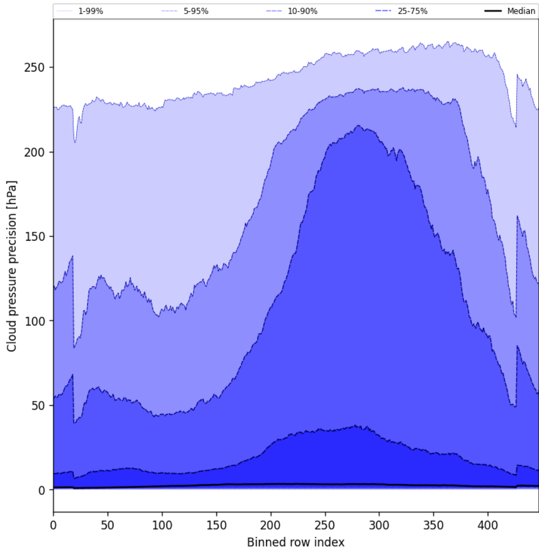
Figure 48: Along track statistics of “Cloud pressure precision” for 2024-11-02 to 2024-11-04
