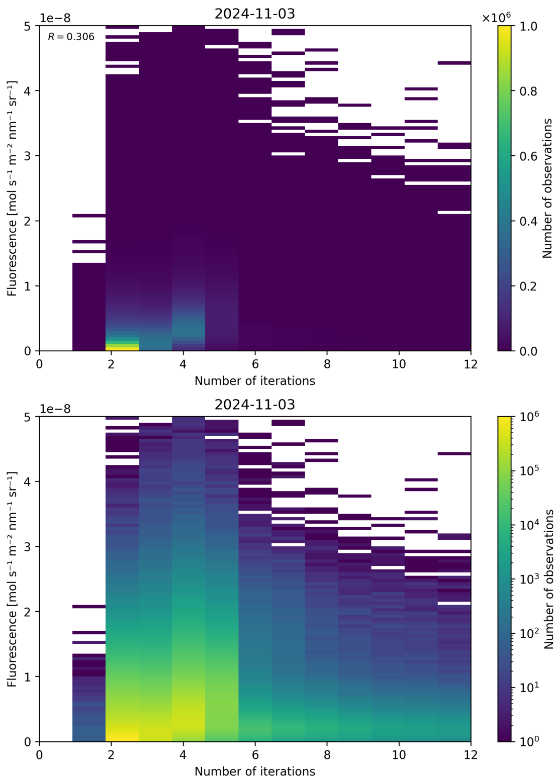
Figure 107: Scatter density plot of “Number of iterations” against “Fluorescence” for 2024-11-02 to 2024-11-04.
