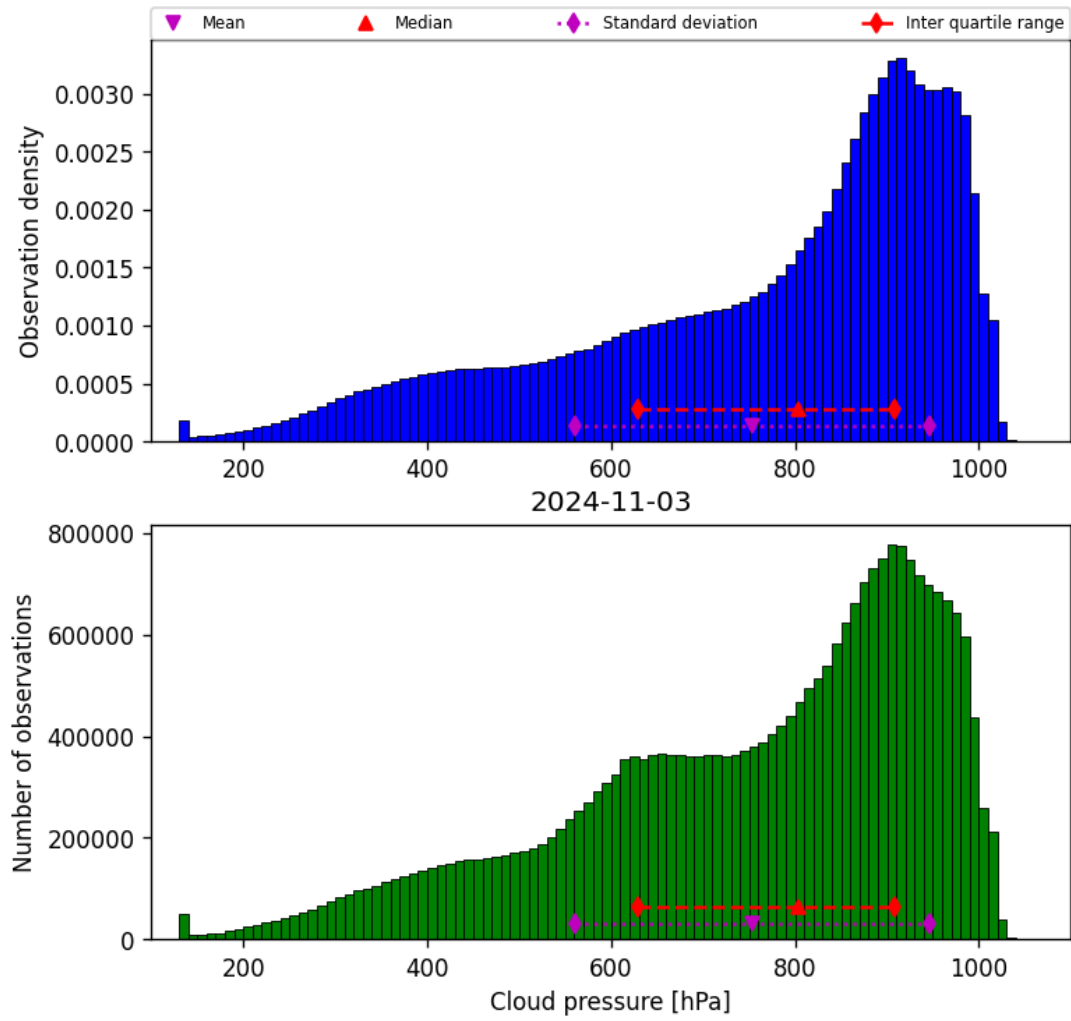
Figure 30: Histogram of “Cloud pressure” for 2024-11-02 to 2024-11-04
