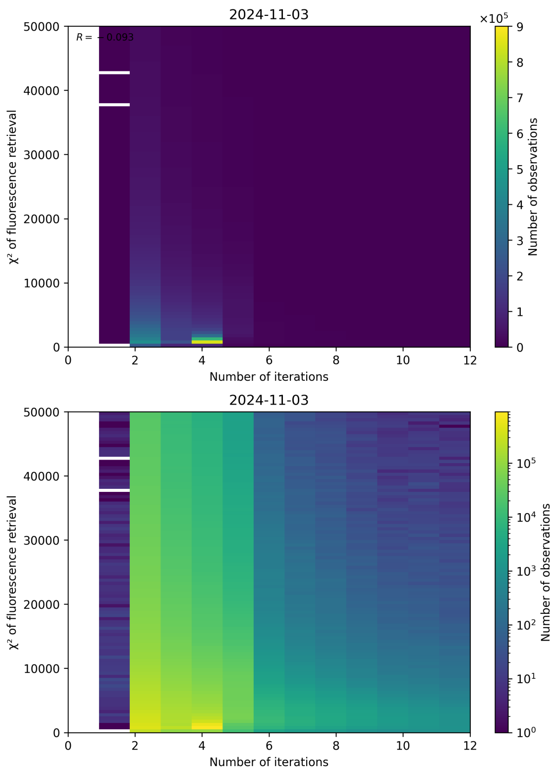
Figure 106: Scatter density plot of “Number of iterations” against “ \chi^2 of fluorescence retrieval” for 2024-11-02 to 2024-11-04.
