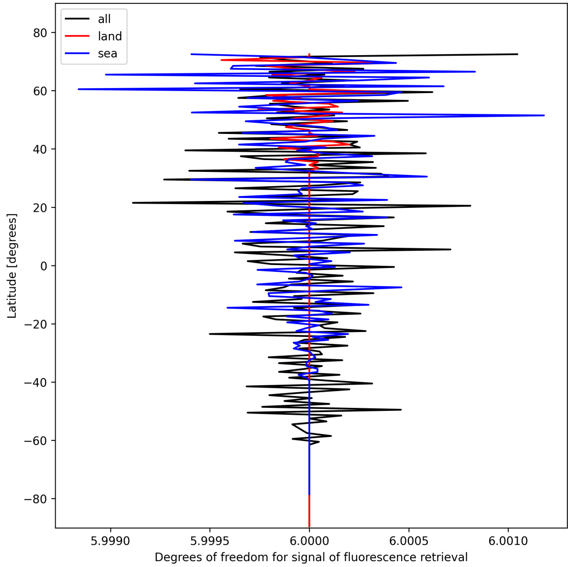
Figure 26: Zonal average of “Degrees of freedom for signal of fluorescence retrieval” for 2024-11-02 to 2024-11-04.
