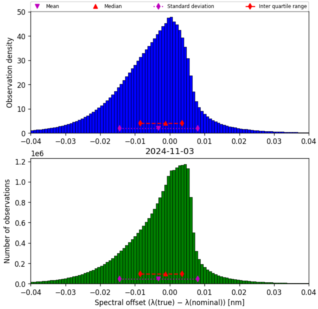
Figure 45: Histogram of “Spectral offset ( \lambda_{\text{true}} - \lambda_{\text{nominal}} )” for 2024-11-02 to 2024-11-04
