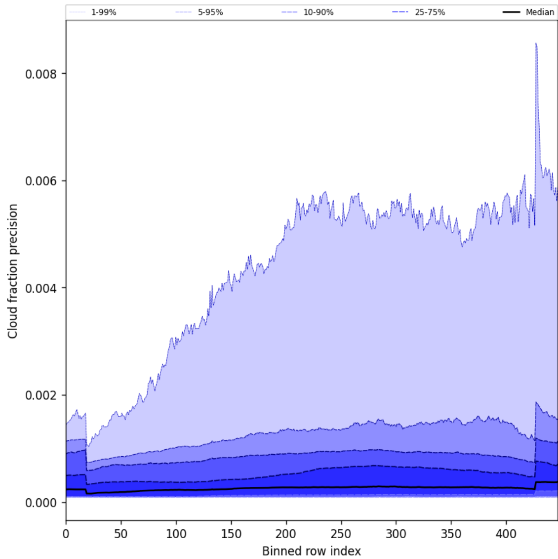
Figure 50: Along track statistics of “Cloud fraction precision” for 2024-11-02 to 2024-11-04
