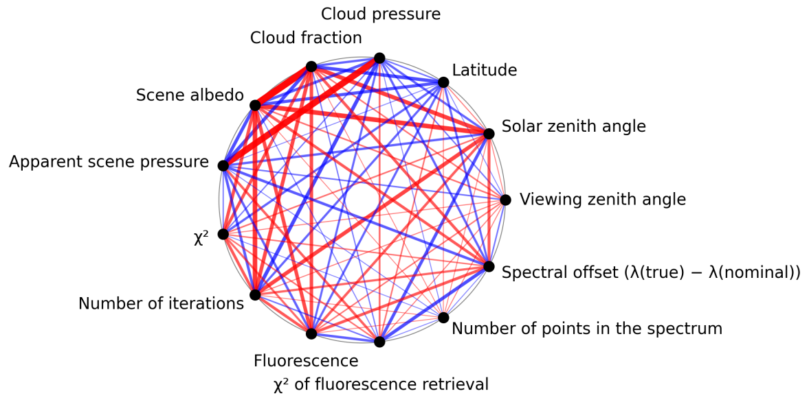
Figure 1: Map of correlation graph for 2024-11-02 to 2024-11-04.
