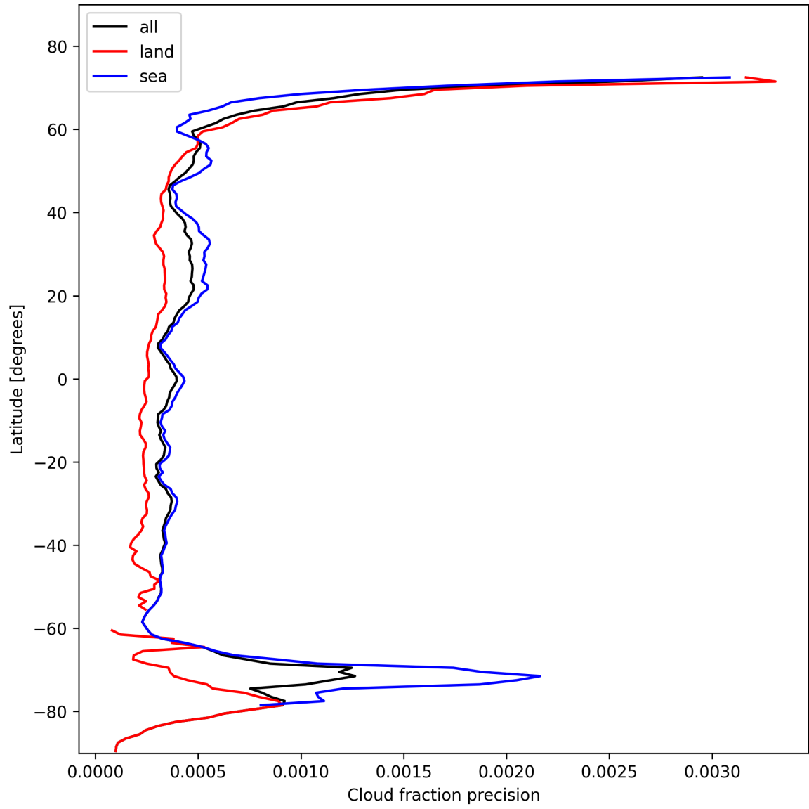
Figure 16: Zonal average of “Cloud fraction precision” for 2024-11-02 to 2024-11-04.
