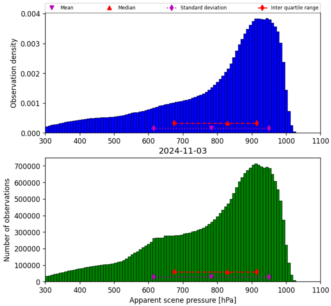
Figure 36: Histogram of “Apparent scene pressure” for 2024-11-02 to 2024-11-04
