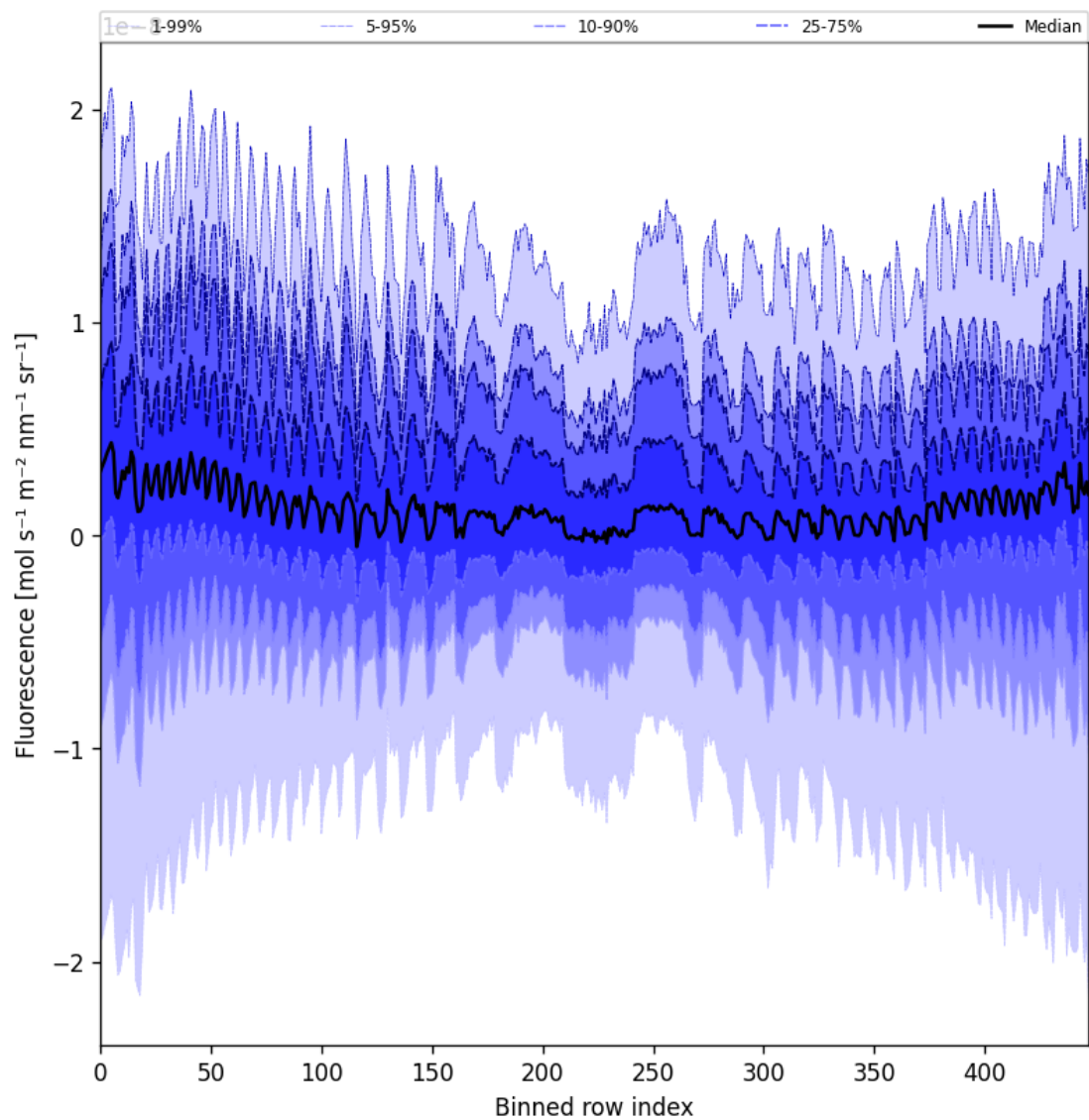
Figure 57: Along track statistics of “Fluorescence” for 2024-11-02 to 2024-11-04
