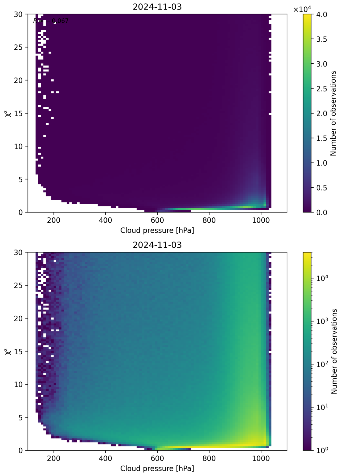
Figure 85: Scatter density plot of “Cloud pressure” against “ \chi^2 ” for 2024-11-02 to 2024-11-04.
