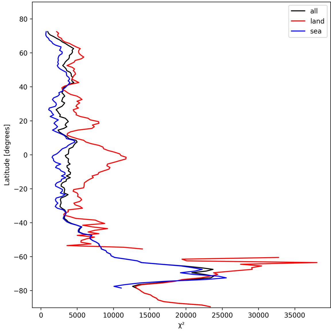
Figure 21: Zonal average of “ \chi^2 ” for 2024-11-02 to 2024-11-04.
