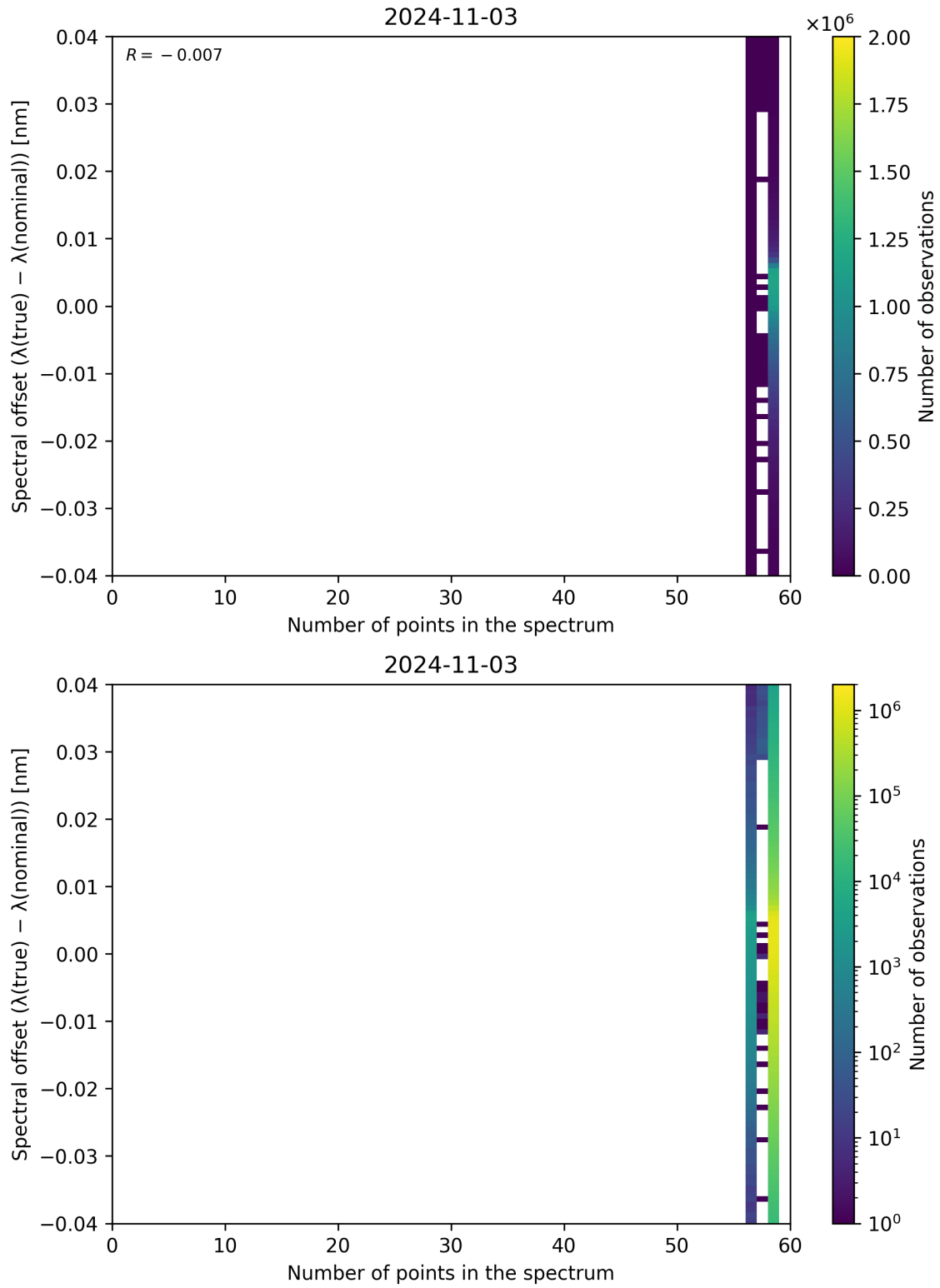
Figure 110: Scatter density plot of “Number of points in the spectrum” against “Spectral offset ( \lambda_{\text{true}} - \lambda_{\text{nominal}} )” for 2024-11-02 to 2024-11-04.
