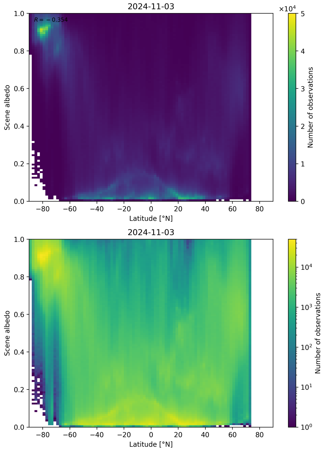
Figure 104: Scatter density plot of “Latitude” against “Scene albedo” for 2024-11-02 to 2024-11-04.
