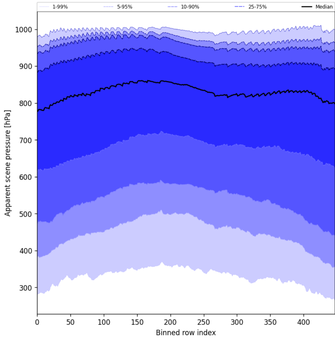
Figure 53: Along track statistics of “Apparent scene pressure” for 2024-11-02 to 2024-11-04
