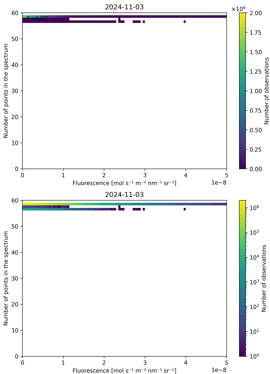
Figure 94: Scatter density plot of “Fluorescence” against “Number of points in the spectrum” for 2024-11-02 to 2024-11-04.
