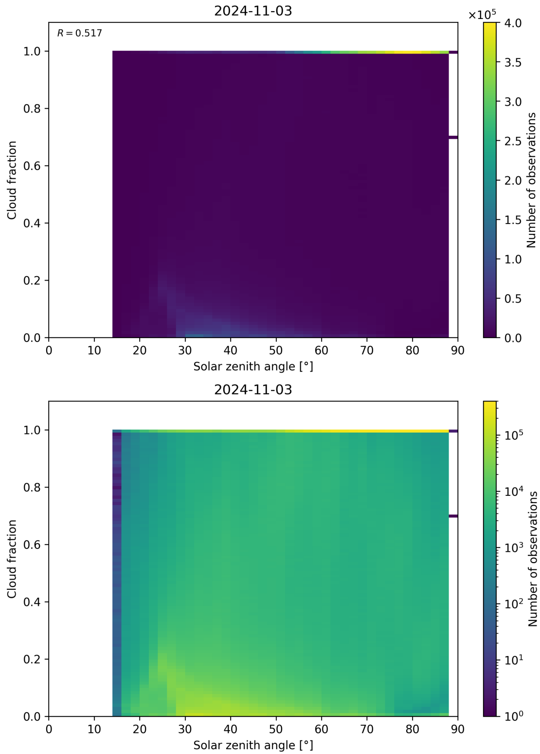
Figure 121: Scatter density plot of “Solar zenith angle” against “Cloud fraction” for 2024-11-02 to 2024-11-04.
