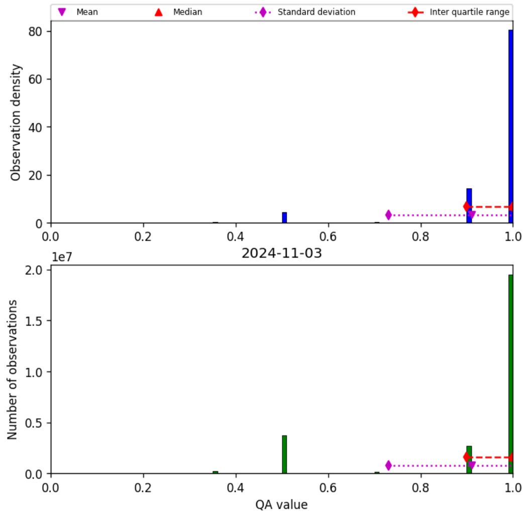
Figure 29: Histogram of “QA value” for 2024-11-02 to 2024-11-04
