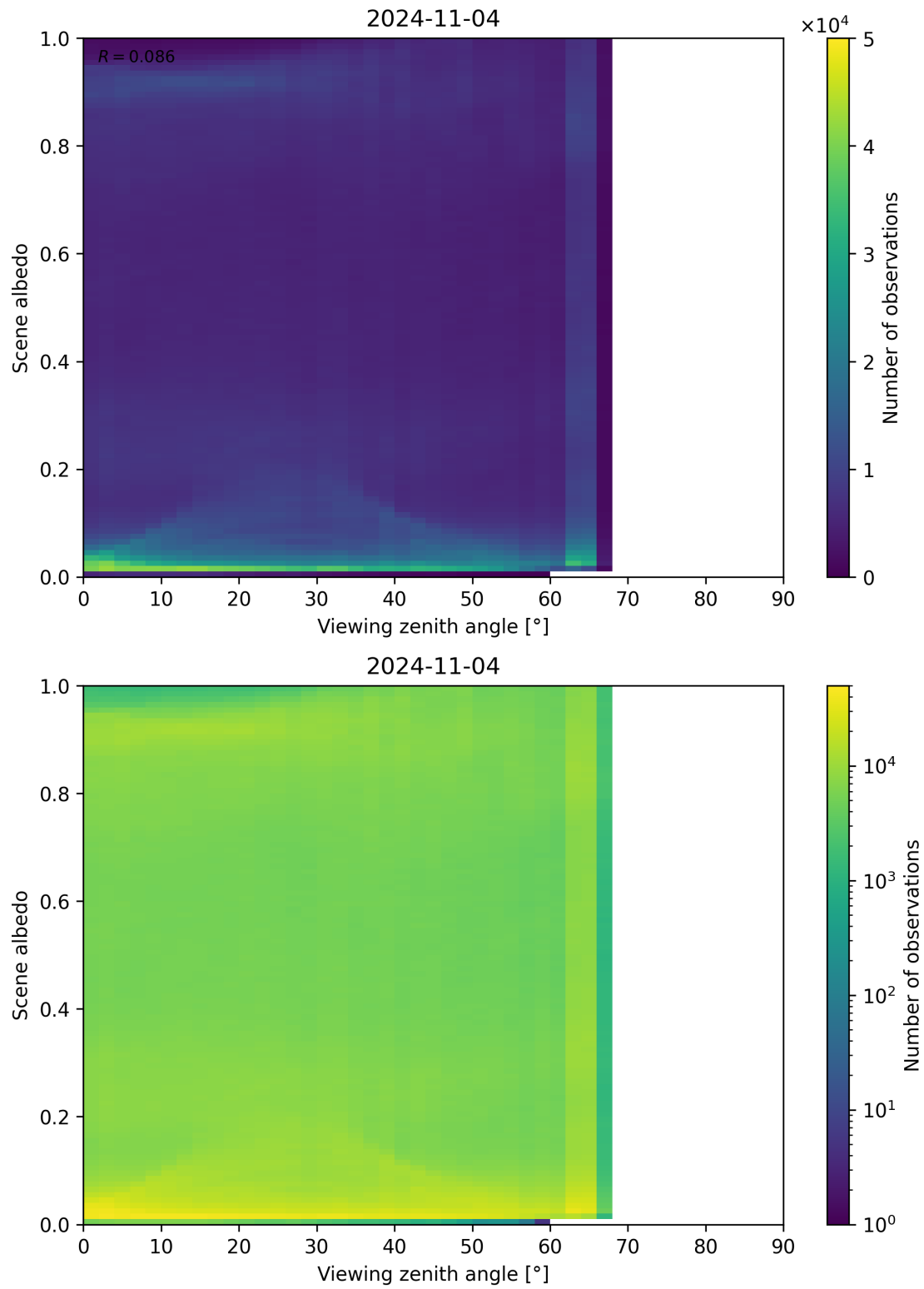
Figure 138: Scatter density plot of “Viewing zenith angle” against “Scene albedo” for 2024-11-04 to 2024-11-05.
