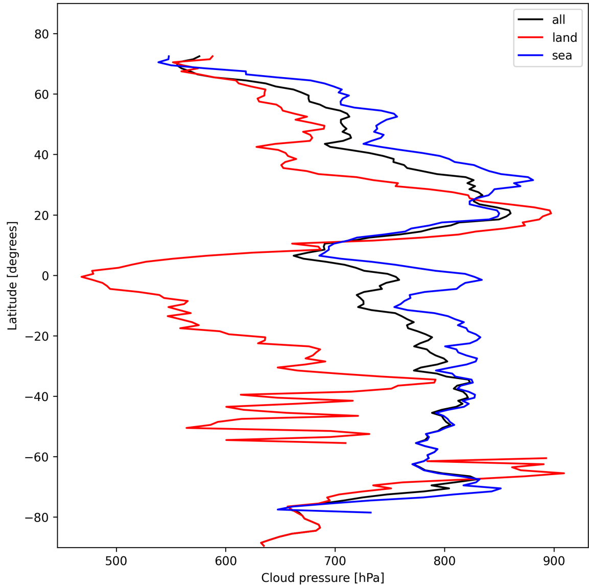
Figure 13: Zonal average of “Cloud pressure” for 2024-11-04 to 2024-11-05.
