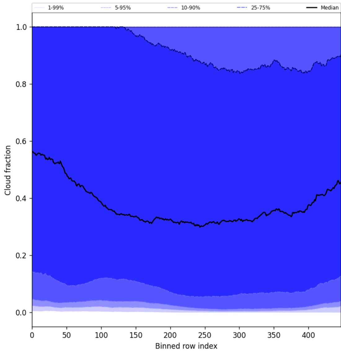
Figure 49: Along track statistics of “Cloud fraction” for 2024-11-04 to 2024-11-05
