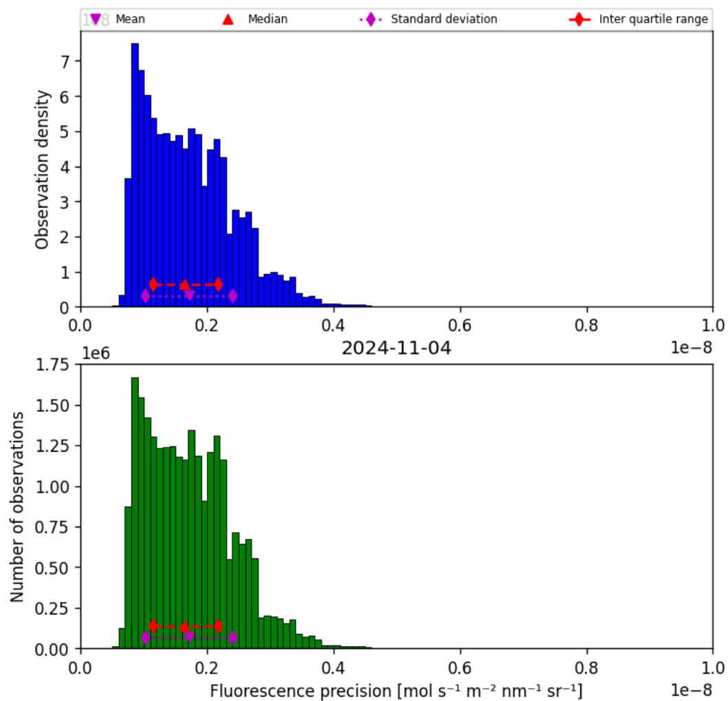
Figure 41: Histogram of “Fluorescence precision” for 2024-11-04 to 2024-11-05
