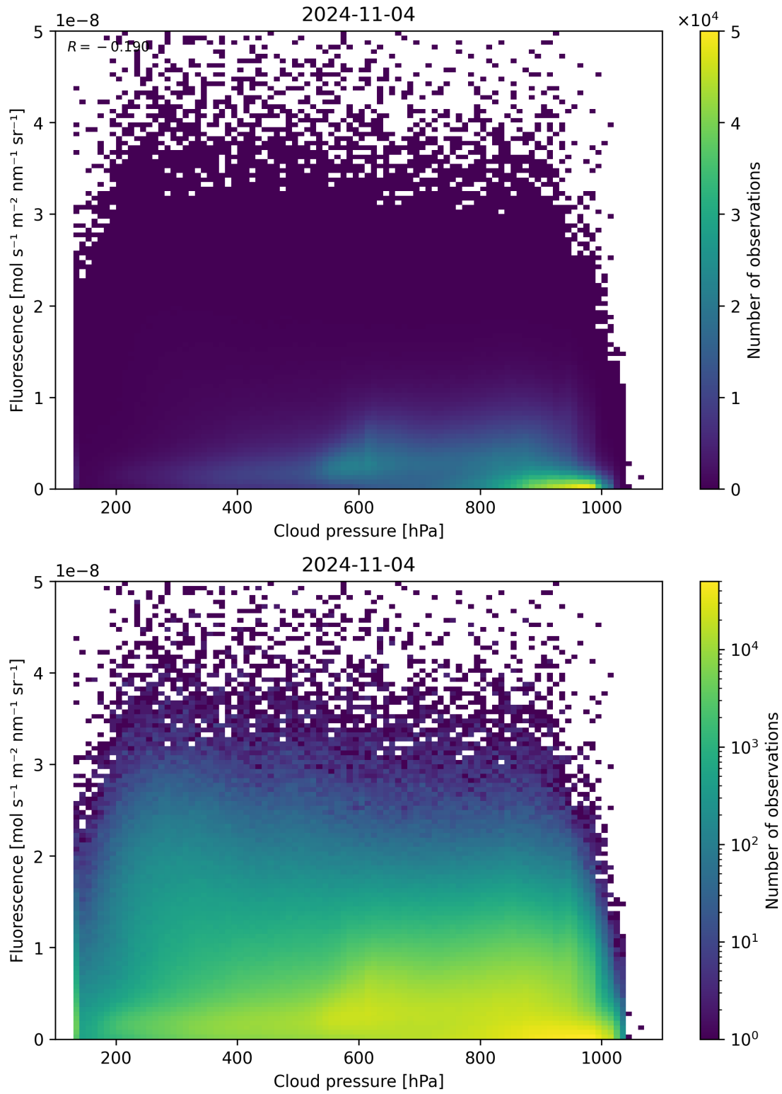
Figure 88: Scatter density plot of “Cloud pressure” against “Fluorescence” for 2024-11-04 to 2024-11-05.
