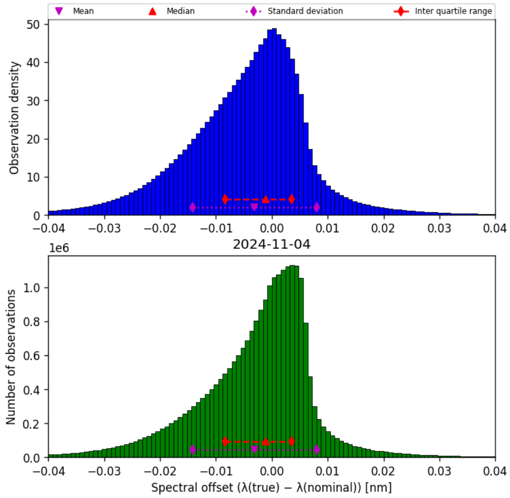
Figure 45: Histogram of “Spectral offset ( \lambda_{\text{true}} - \lambda_{\text{nominal}} )” for 2024-11-04 to 2024-11-05
