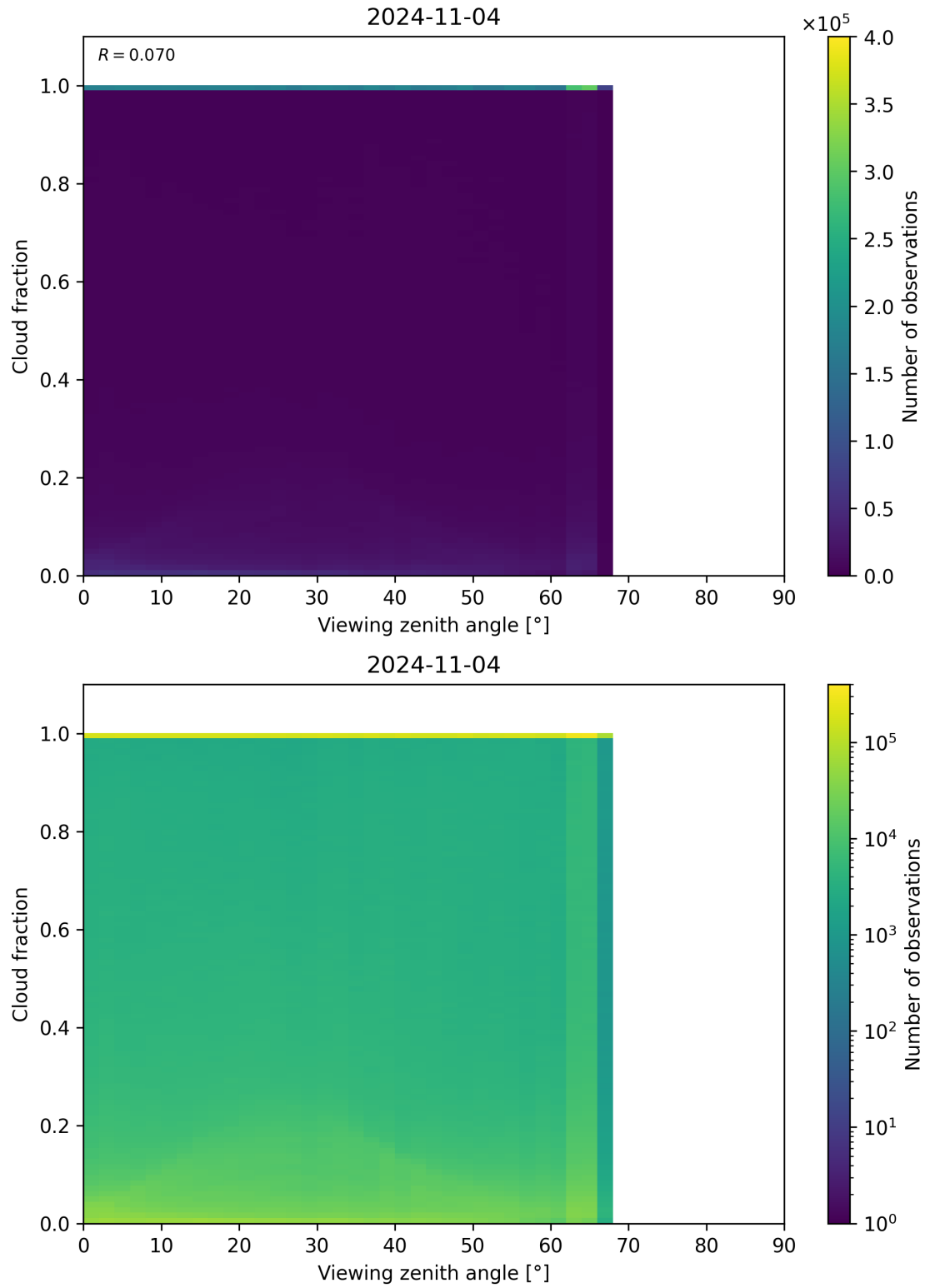
Figure 132: Scatter density plot of “Viewing zenith angle” against “Cloud fraction” for 2024-11-04 to 2024-11-05.
