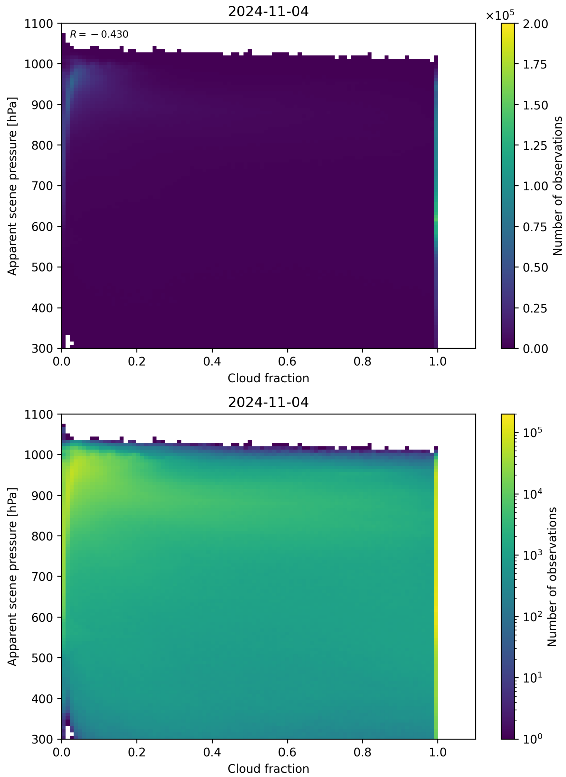
Figure 76: Scatter density plot of “Cloud fraction” against “Apparent scene pressure” for 2024-11-04 to 2024-11-05.
