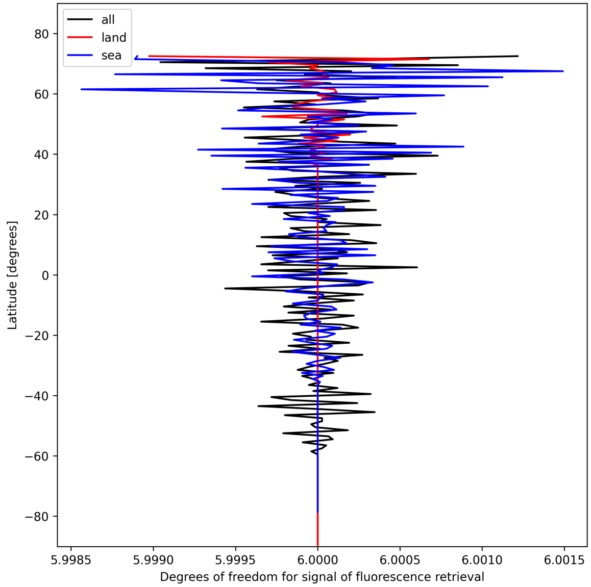
Figure 26: Zonal average of “Degrees of freedom for signal of fluorescence retrieval” for 2024-11-04 to 2024-11-05.
