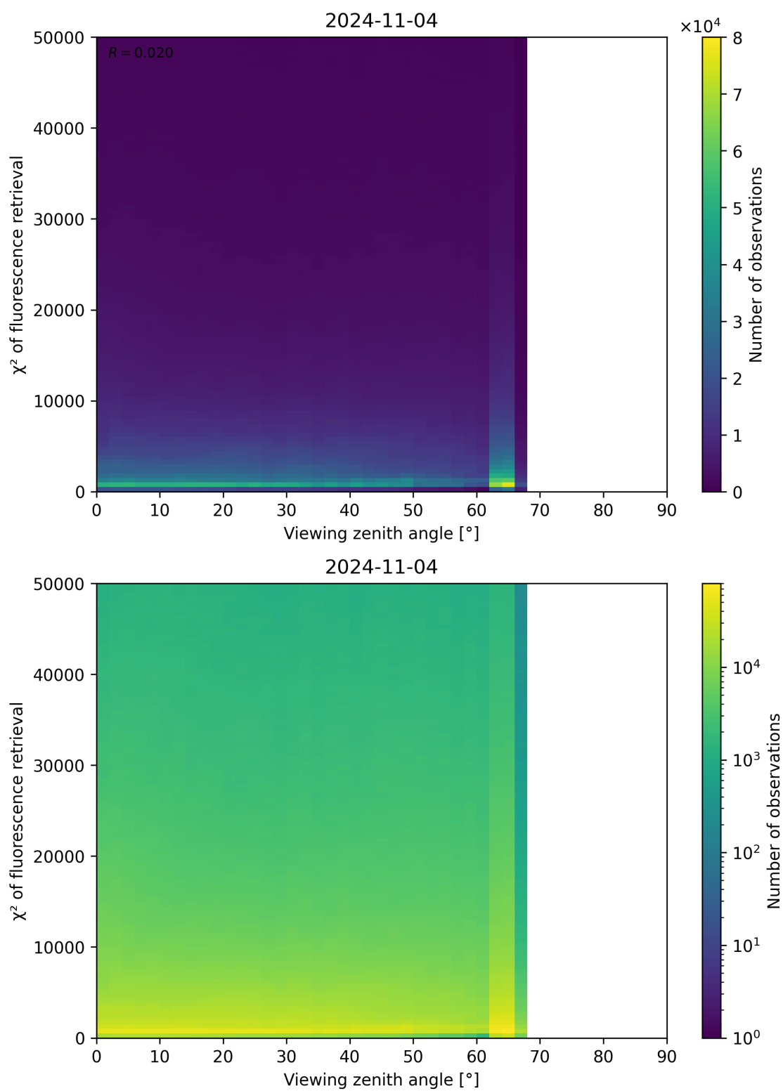
Figure 131: Scatter density plot of “Viewing zenith angle” against “ \chi^2 of fluorescence retrieval” for 2024-11-04 to 2024-11-05.
