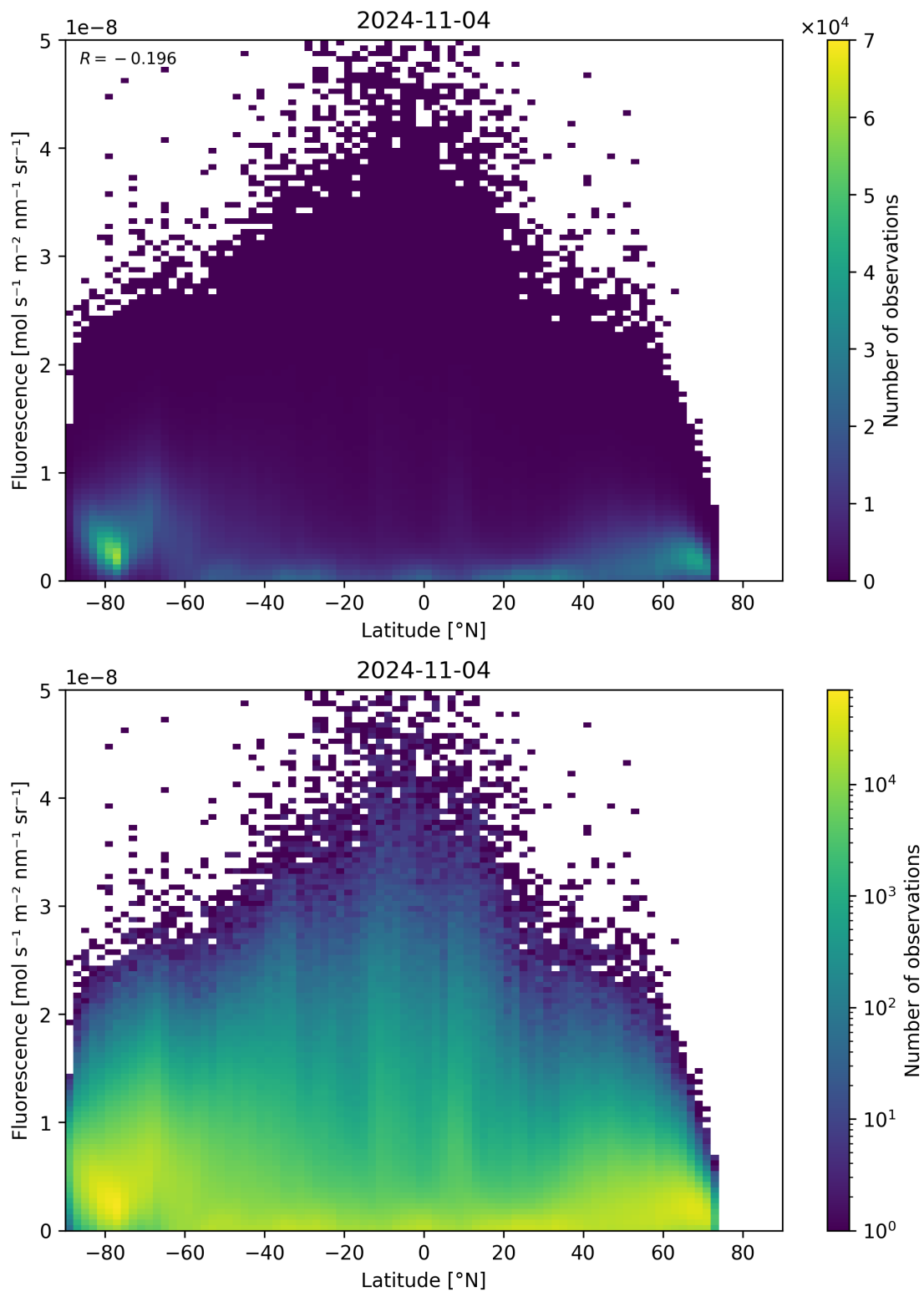
Figure 101: Scatter density plot of “Latitude” against “Fluorescence” for 2024-11-04 to 2024-11-05.
