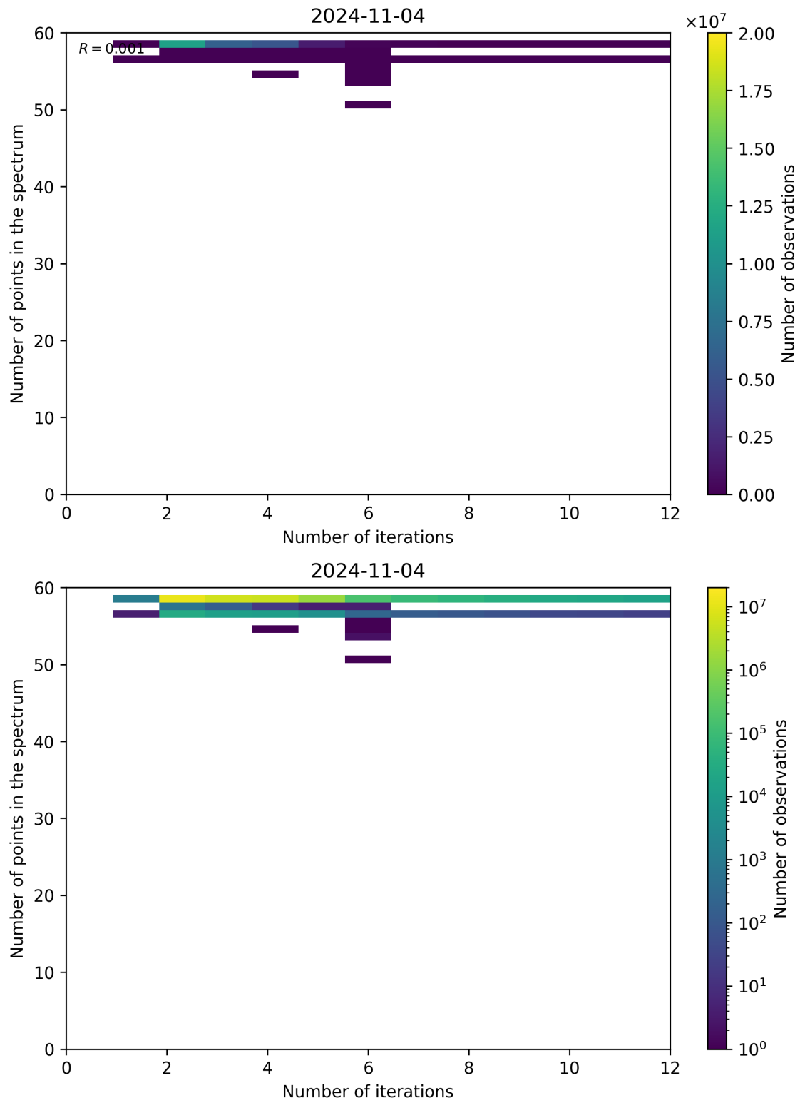
Figure 108: Scatter density plot of “Number of iterations” against “Number of points in the spectrum” for 2024-11-04 to 2024-11-05.
