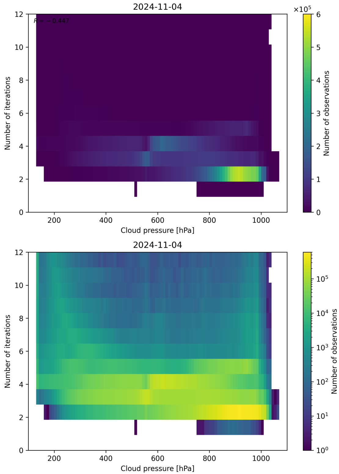
Figure 89: Scatter density plot of “Cloud pressure” against “Number of iterations” for 2024-11-04 to 2024-11-05.
