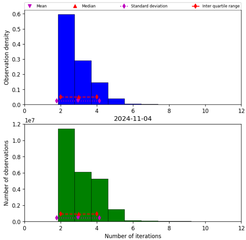
Figure 39: Histogram of “Number of iterations” for 2024-11-04 to 2024-11-05
