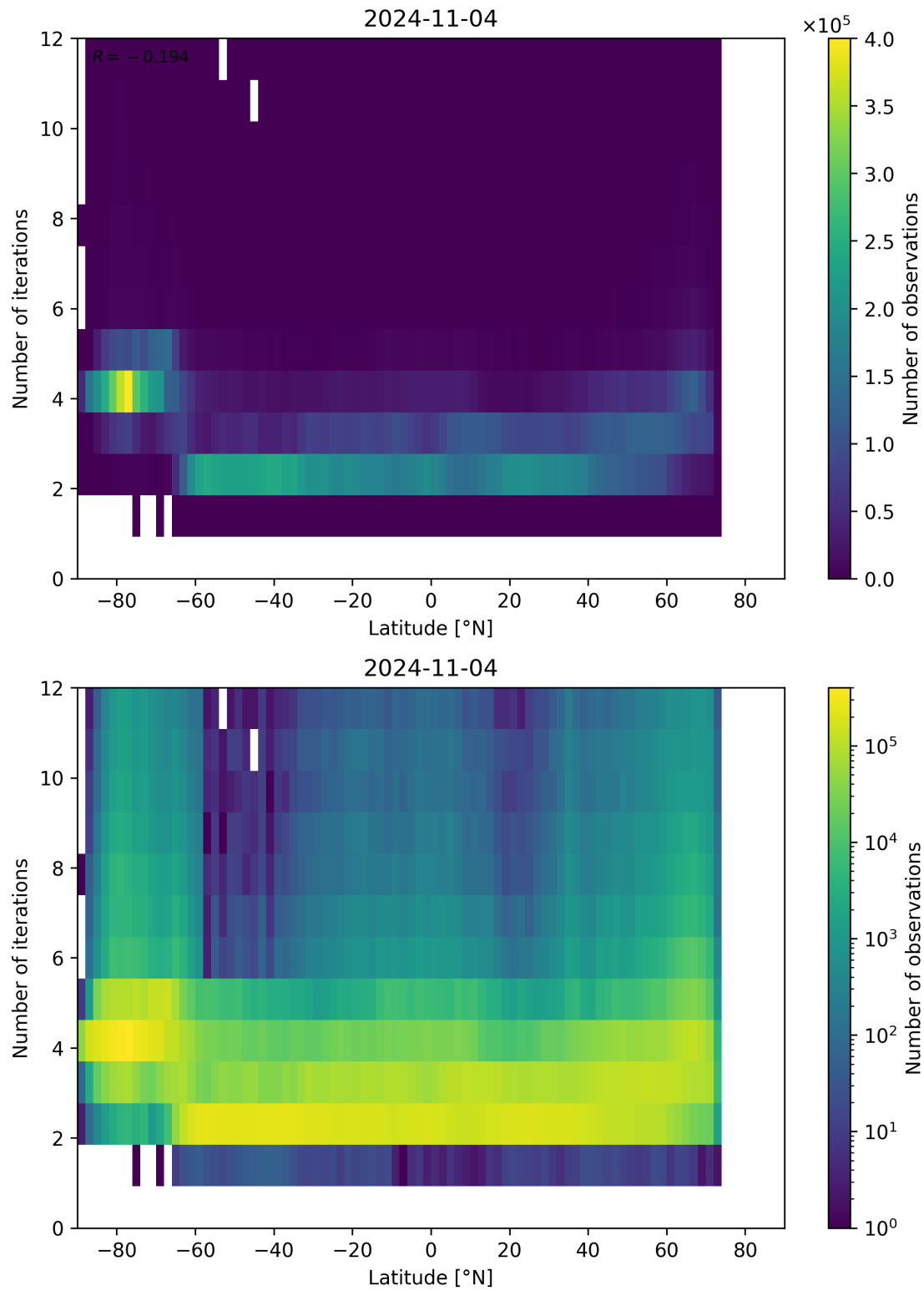
Figure 102: Scatter density plot of “Latitude” against “Number of iterations” for 2024-11-04 to 2024-11-05.
