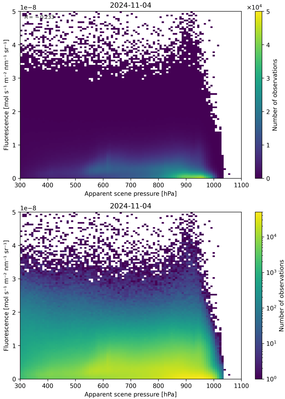
Figure 65: Scatter density plot of “Apparent scene pressure” against “Fluorescence” for 2024-11-04 to 2024-11-05.
