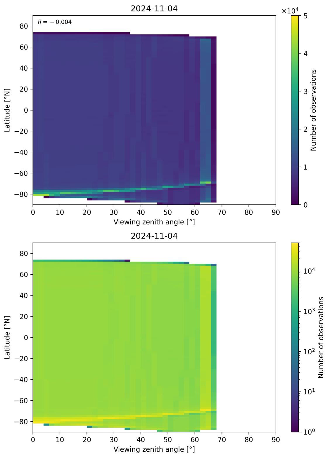
Figure 135: Scatter density plot of “Viewing zenith angle” against “Latitude” for 2024-11-04 to 2024-11-05.
