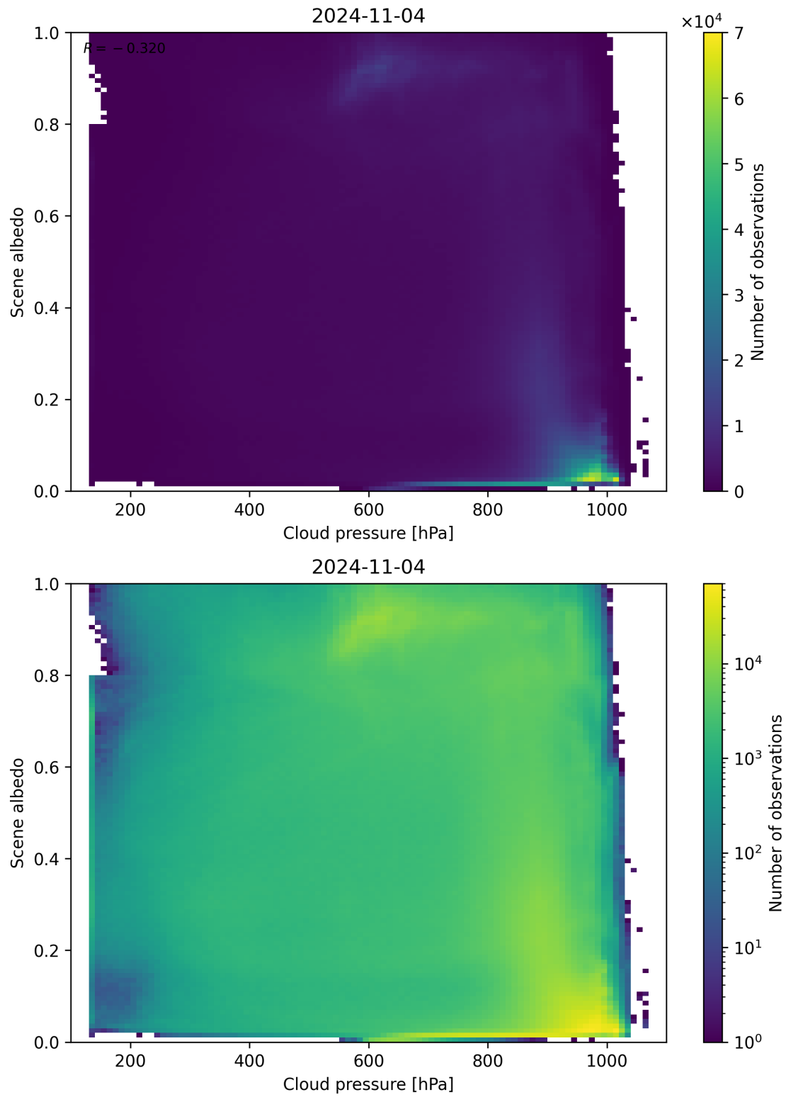
Figure 91: Scatter density plot of “Cloud pressure” against “Scene albedo” for 2024-11-04 to 2024-11-05.
