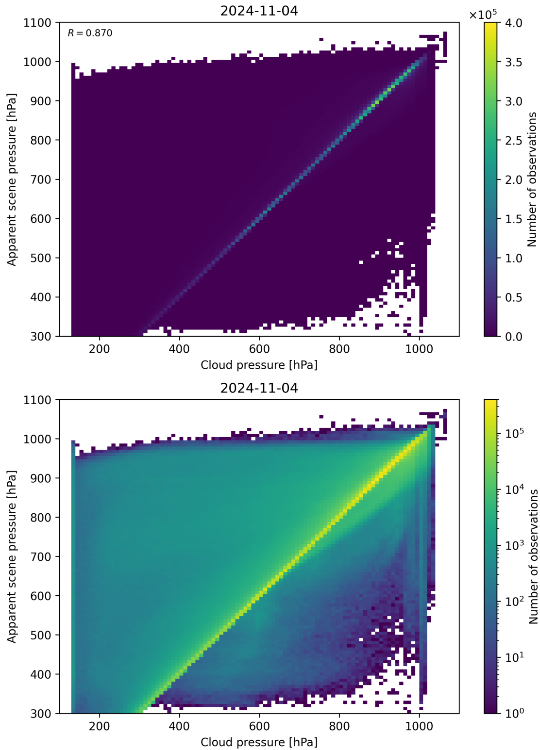
Figure 84: Scatter density plot of “Cloud pressure” against “Apparent scene pressure” for 2024-11-04 to 2024-11-05.
