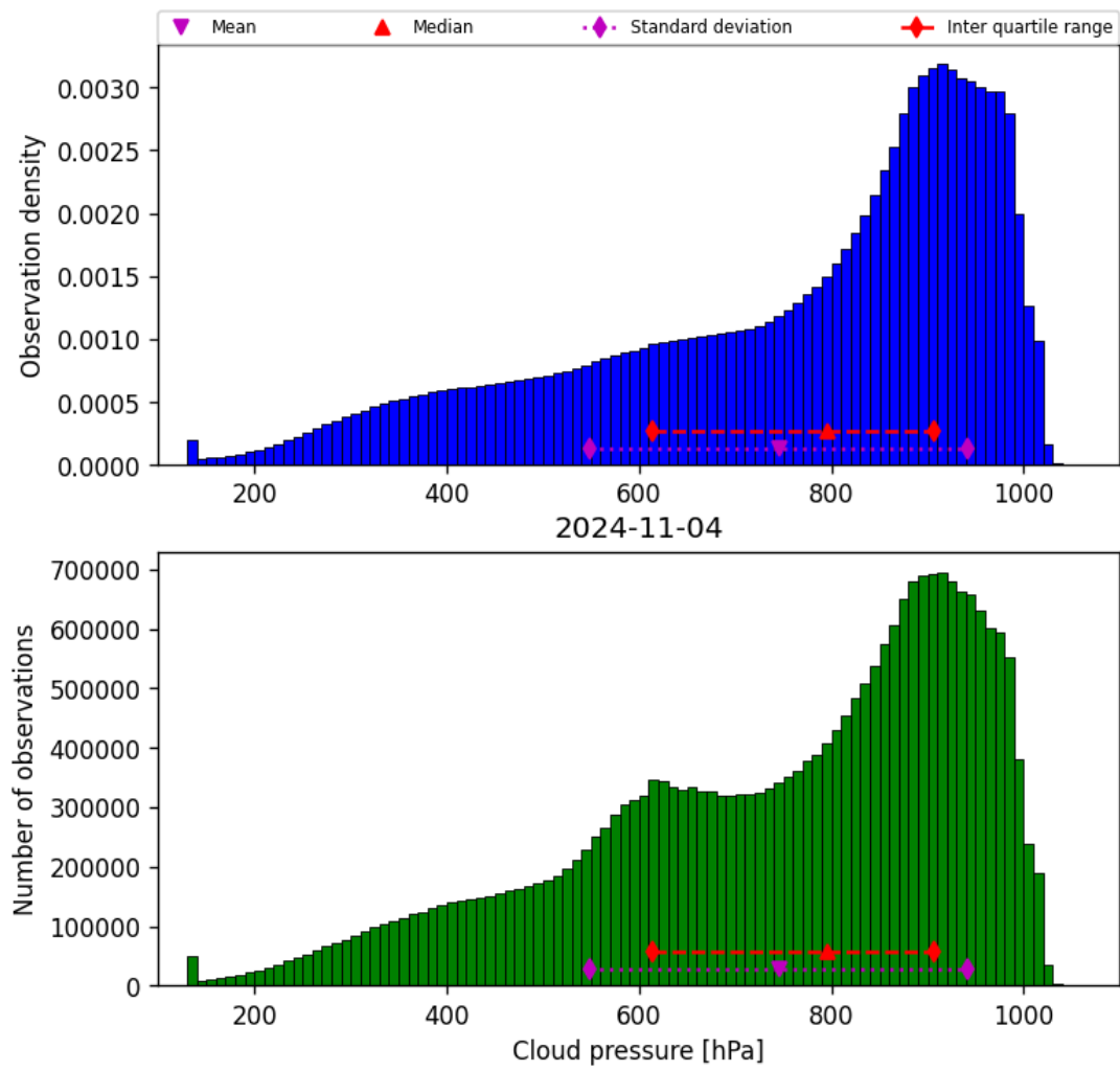
Figure 30: Histogram of “Cloud pressure” for 2024-11-04 to 2024-11-05
