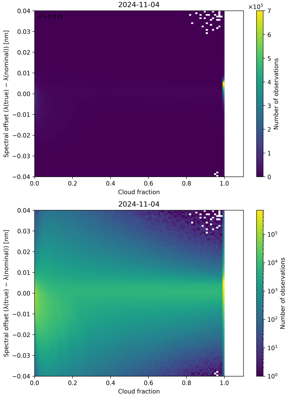
Figure 83: Scatter density plot of “Cloud fraction” against “Spectral offset ( \lambda_{\text{true}} - \lambda_{\text{nominal}} )” for 2024-11-04 to 2024-11-05.
