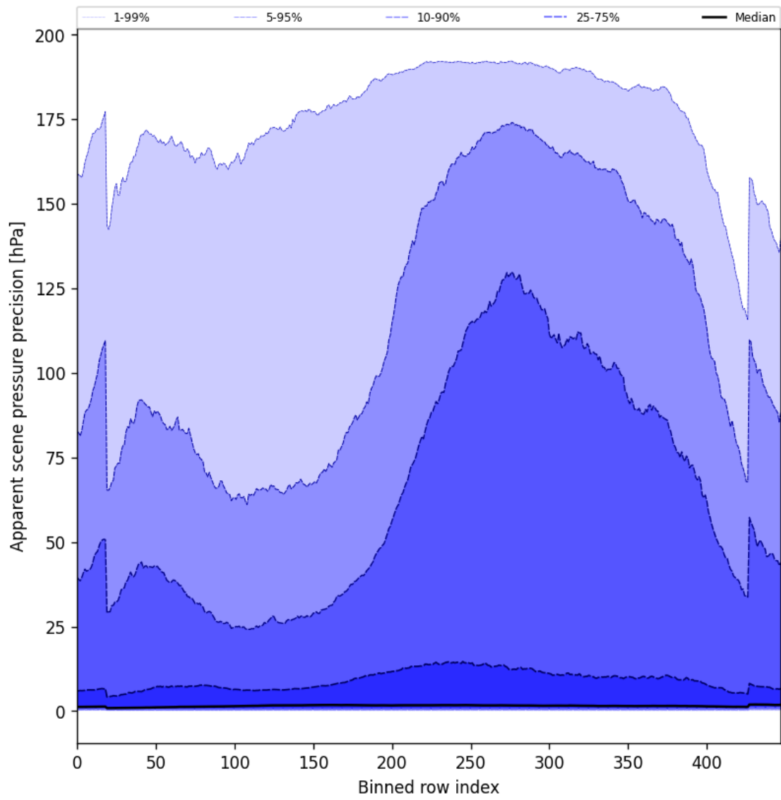
Figure 54: Along track statistics of “Apparent scene pressure precision” for 2024-11-04 to 2024-11-05
