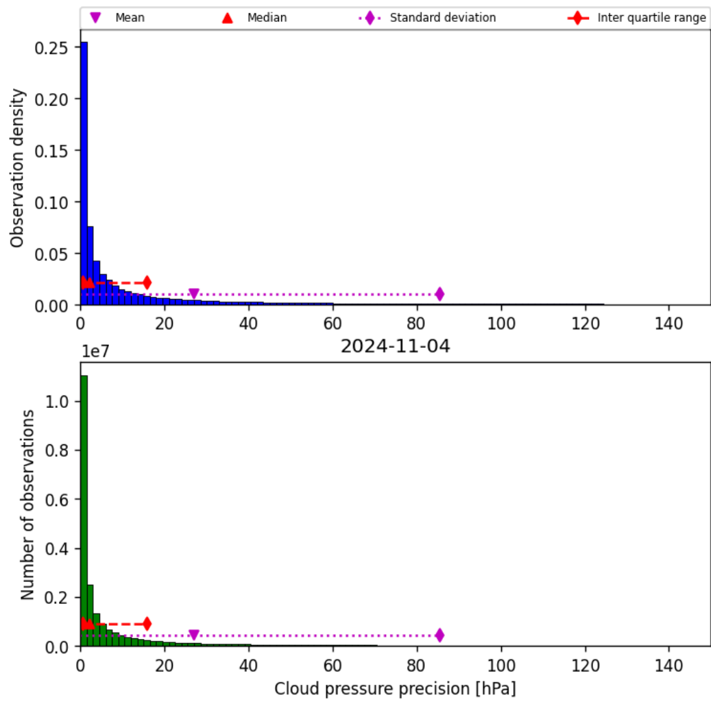
Figure 31: Histogram of “Cloud pressure precision” for 2024-11-04 to 2024-11-05
