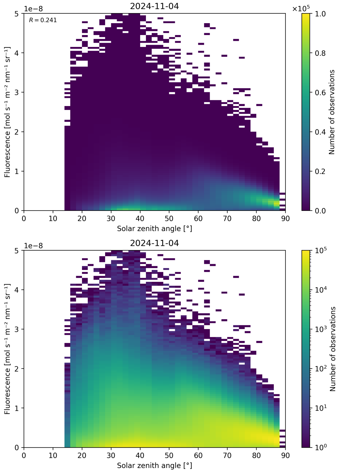
Figure 123: Scatter density plot of “Solar zenith angle” against “Fluorescence” for 2024-11-04 to 2024-11-05.
