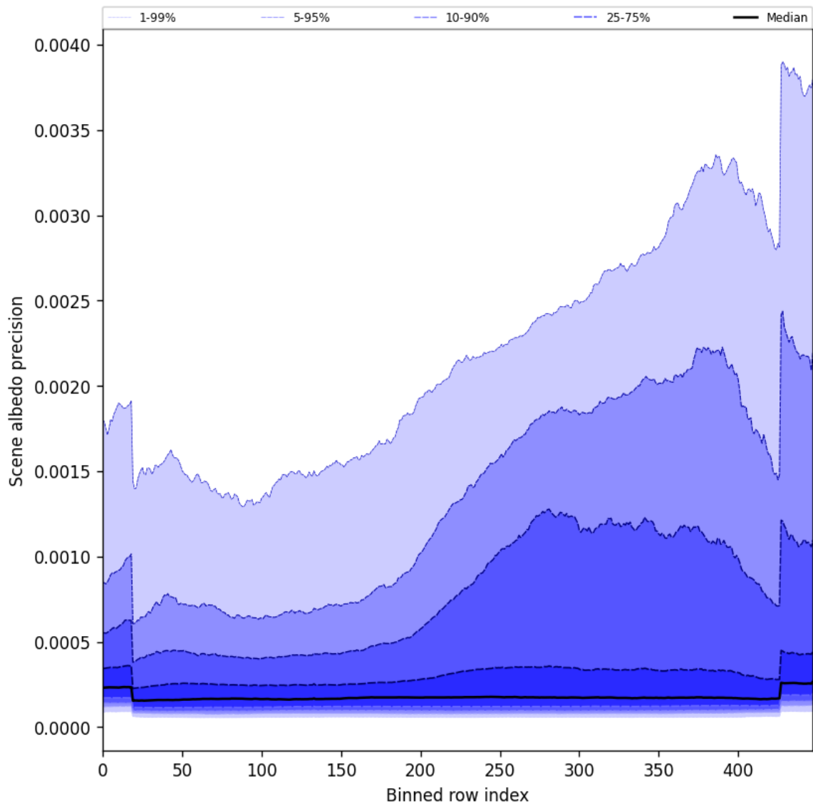
Figure 52: Along track statistics of “Scene albedo precision” for 2024-11-04 to 2024-11-05
