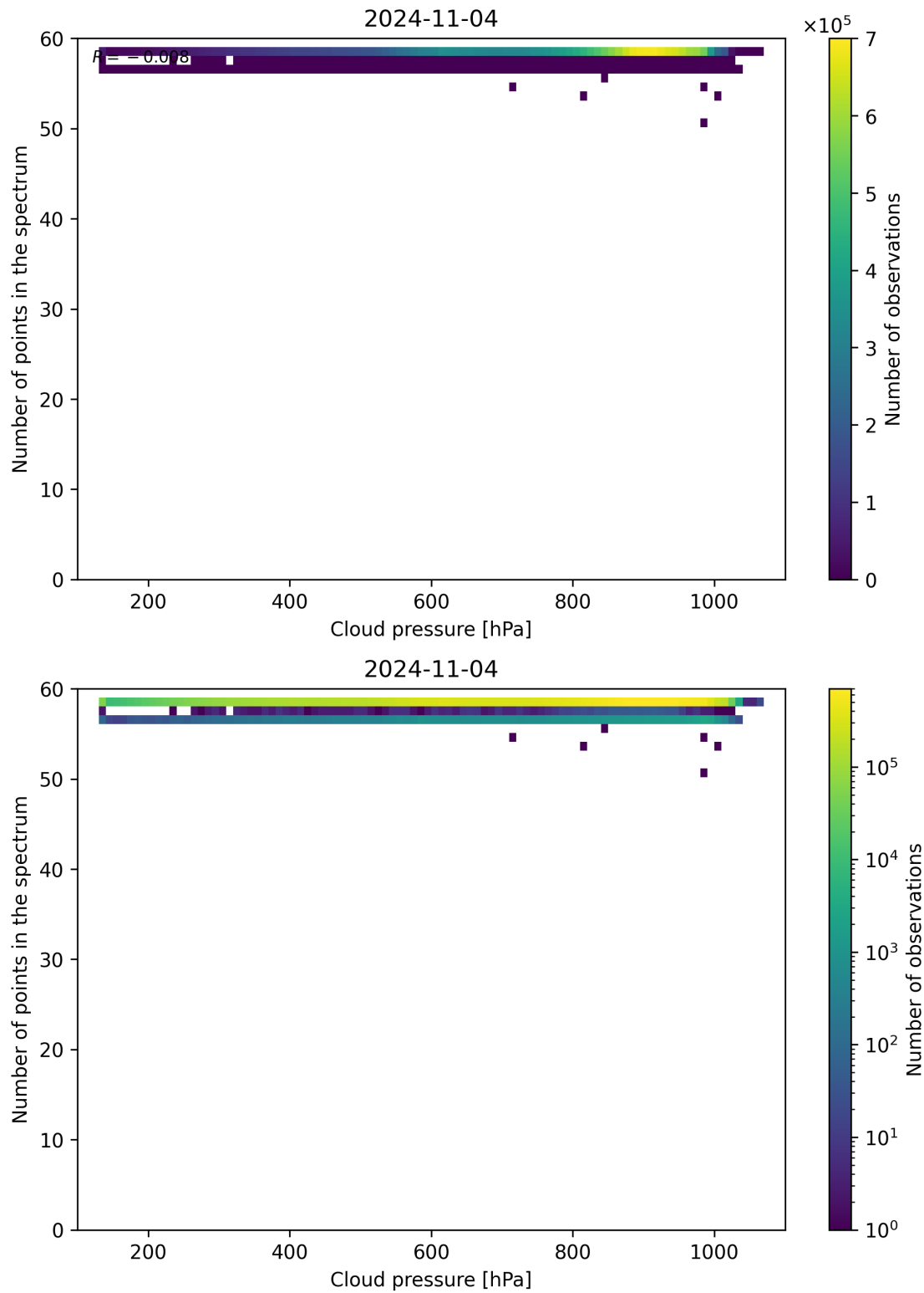
Figure 90: Scatter density plot of “Cloud pressure” against “Number of points in the spectrum” for 2024-11-04 to 2024-11-05.
