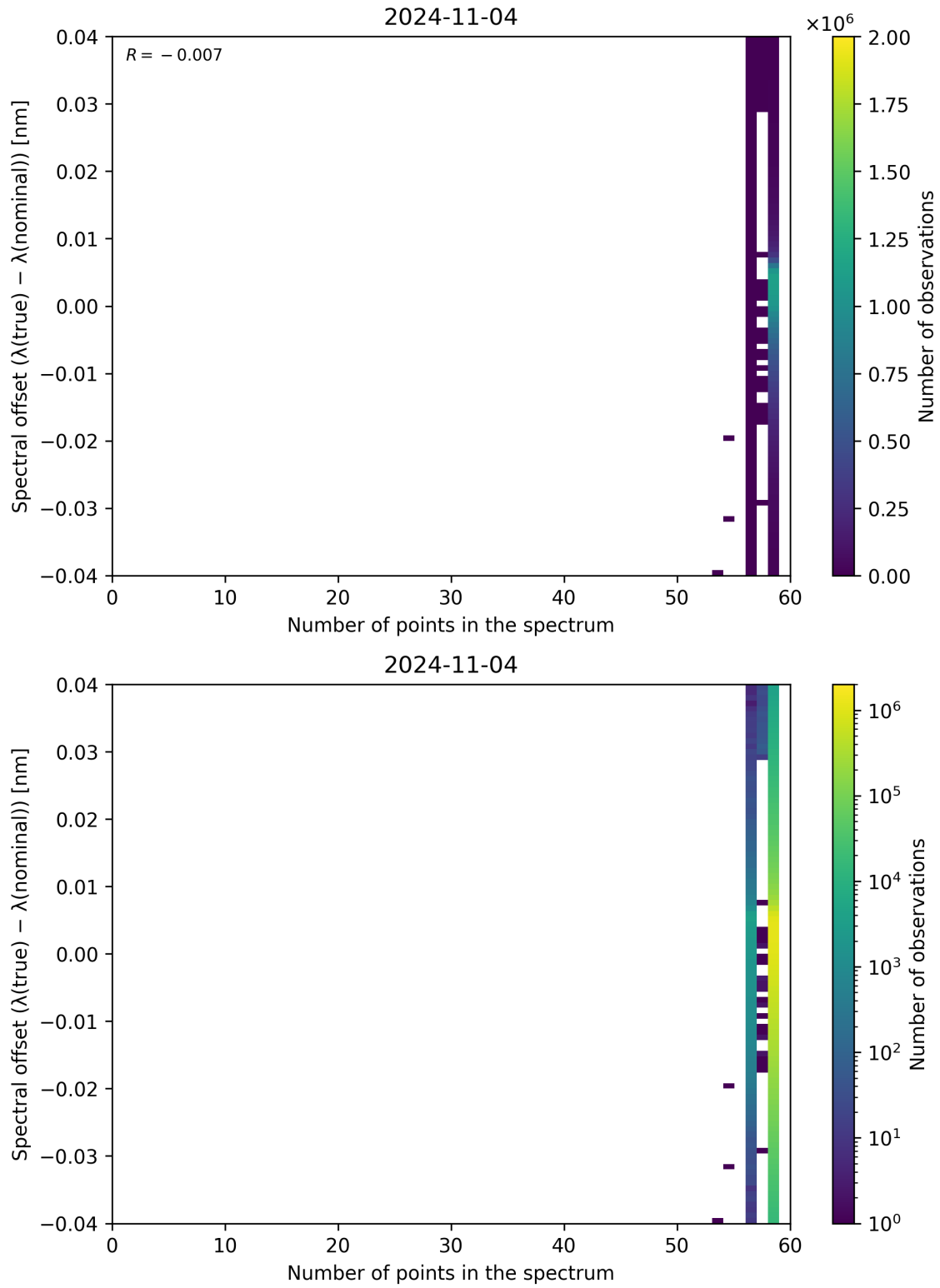
Figure 110: Scatter density plot of “Number of points in the spectrum” against “Spectral offset ( \lambda_{\text{true}} - \lambda_{\text{nominal}} )” for 2024-11-04 to 2024-11-05.
