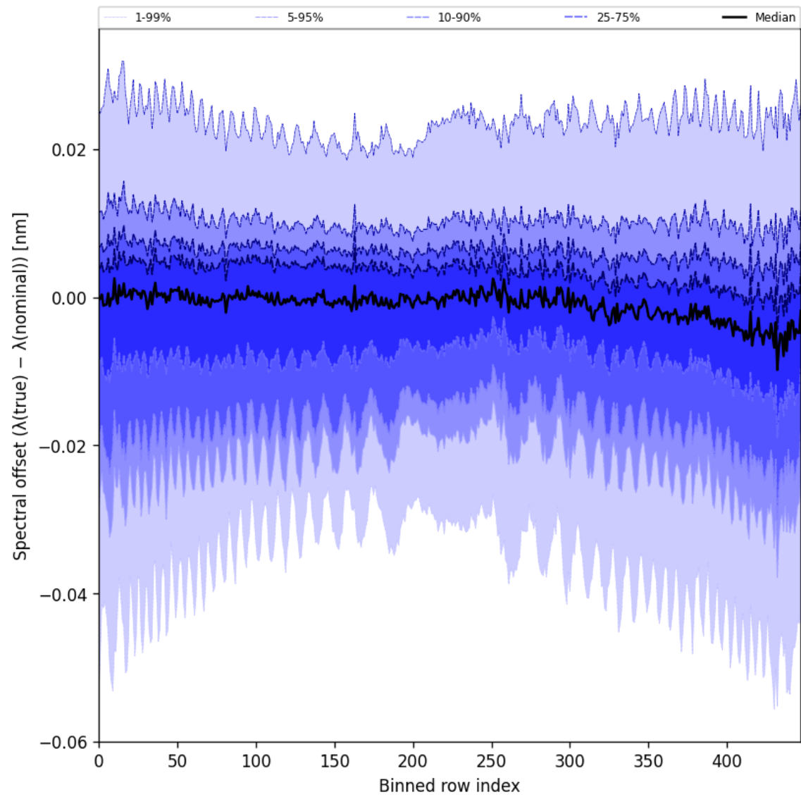
Figure 62: Along track statistics of “Spectral offset ( \lambda_{\text{true}} - \lambda_{\text{nominal}} )” for 2024-11-04 to 2024-11-05
