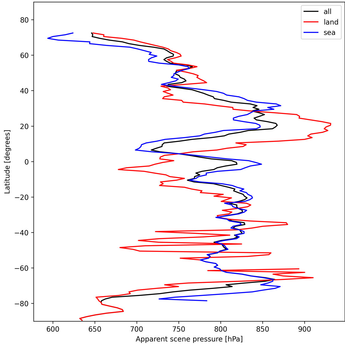
Figure 19: Zonal average of “Apparent scene pressure” for 2024-11-04 to 2024-11-05.
