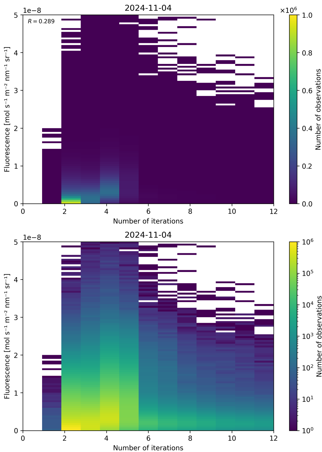
Figure 107: Scatter density plot of “Number of iterations” against “Fluorescence” for 2024-11-04 to 2024-11-05.
