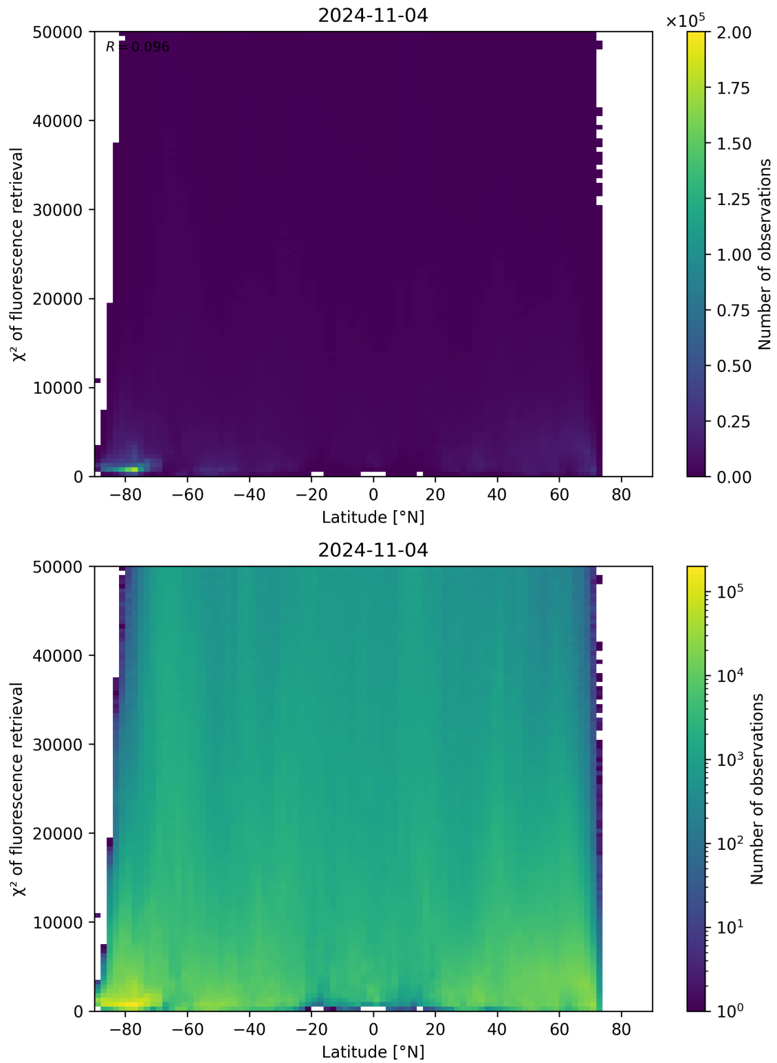
Figure 98: Scatter density plot of “Latitude” against “ \chi^2 of fluorescence retrieval” for 2024-11-04 to 2024-11-05.
