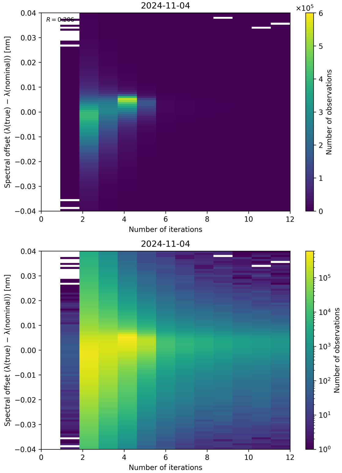
Figure 109: Scatter density plot of “Number of iterations” against “Spectral offset ( \lambda_{\text{true}} - \lambda_{\text{nominal}} )” for 2024-11-04 to 2024-11-05.
