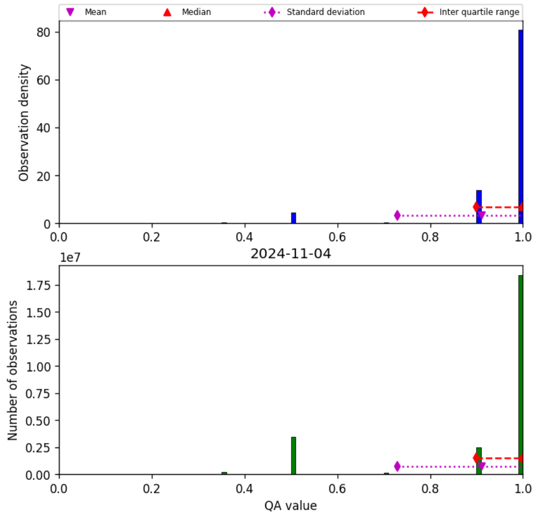
Figure 29: Histogram of “QA value” for 2024-11-04 to 2024-11-05
