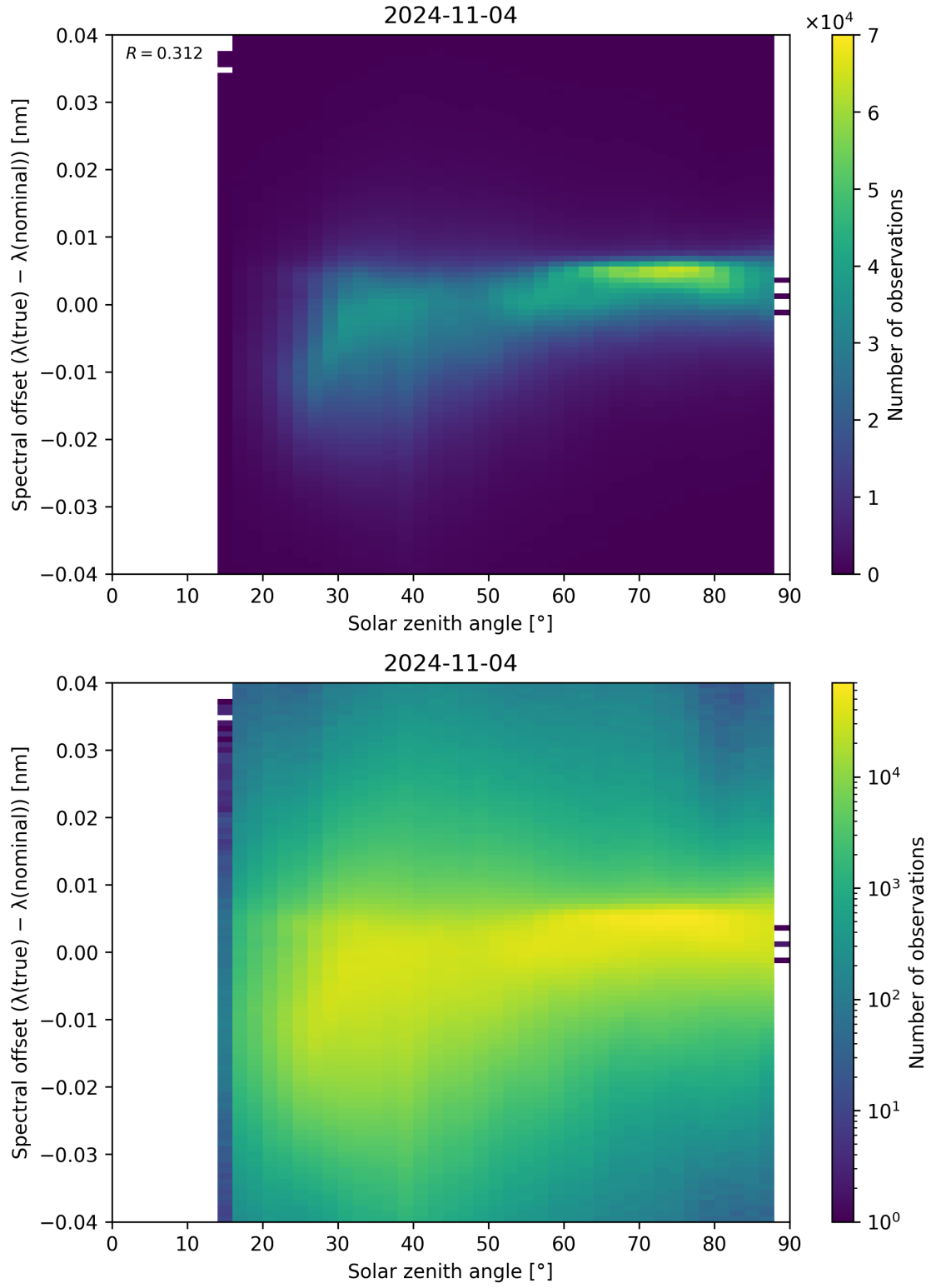
Figure 128: Scatter density plot of “Solar zenith angle” against “Spectral offset ( \lambda_{\text{true}} - \lambda_{\text{nominal}} )” for 2024-11-04 to 2024-11-05.
