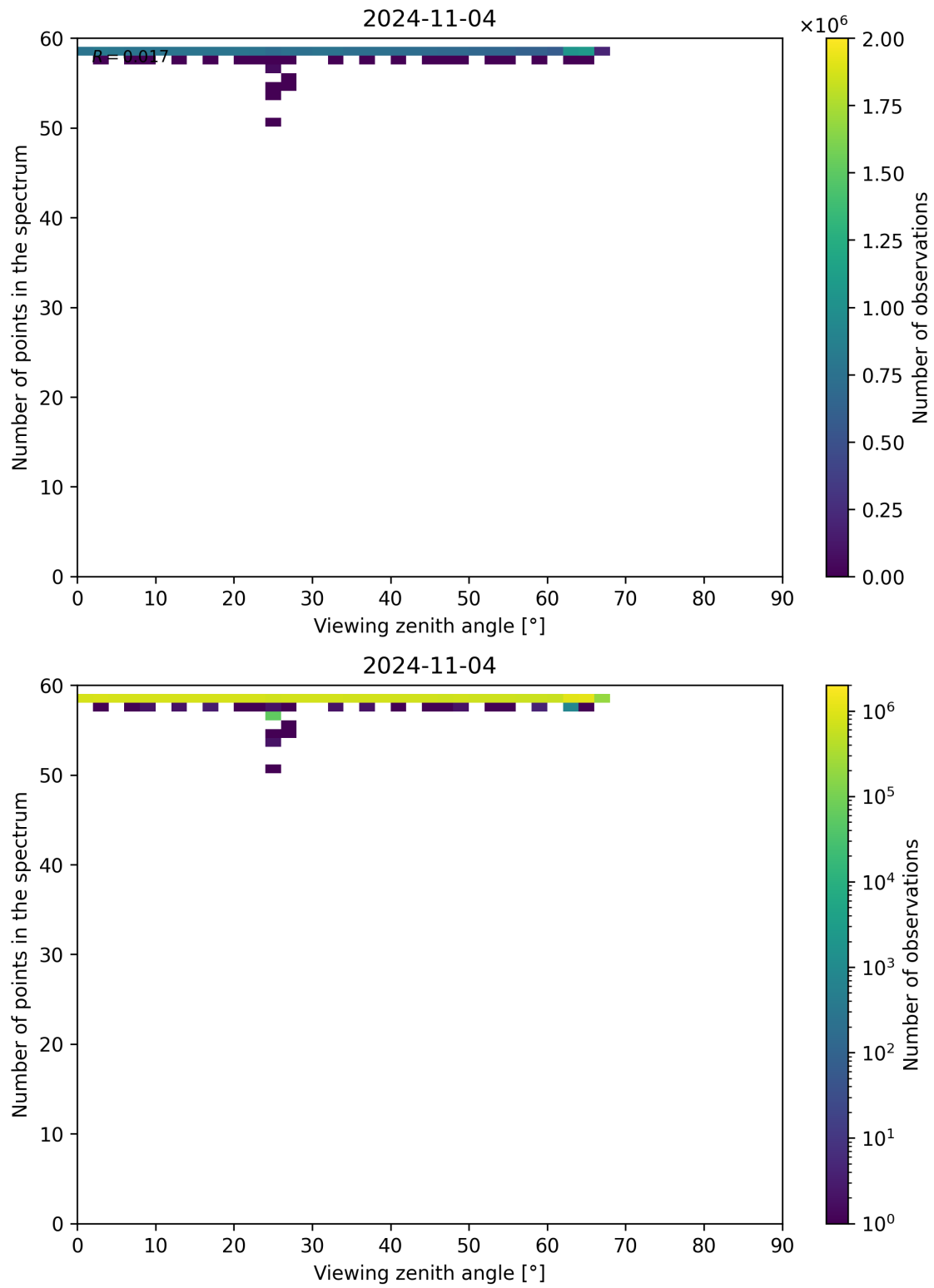
Figure 137: Scatter density plot of “Viewing zenith angle” against “Number of points in the spectrum” for 2024-11-04 to 2024-11-05.
