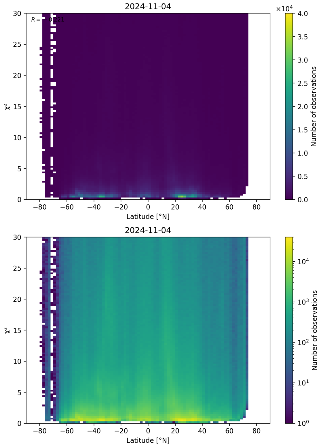
Figure 97: Scatter density plot of “Latitude” against “ \chi^2 ” for 2024-11-04 to 2024-11-05.
