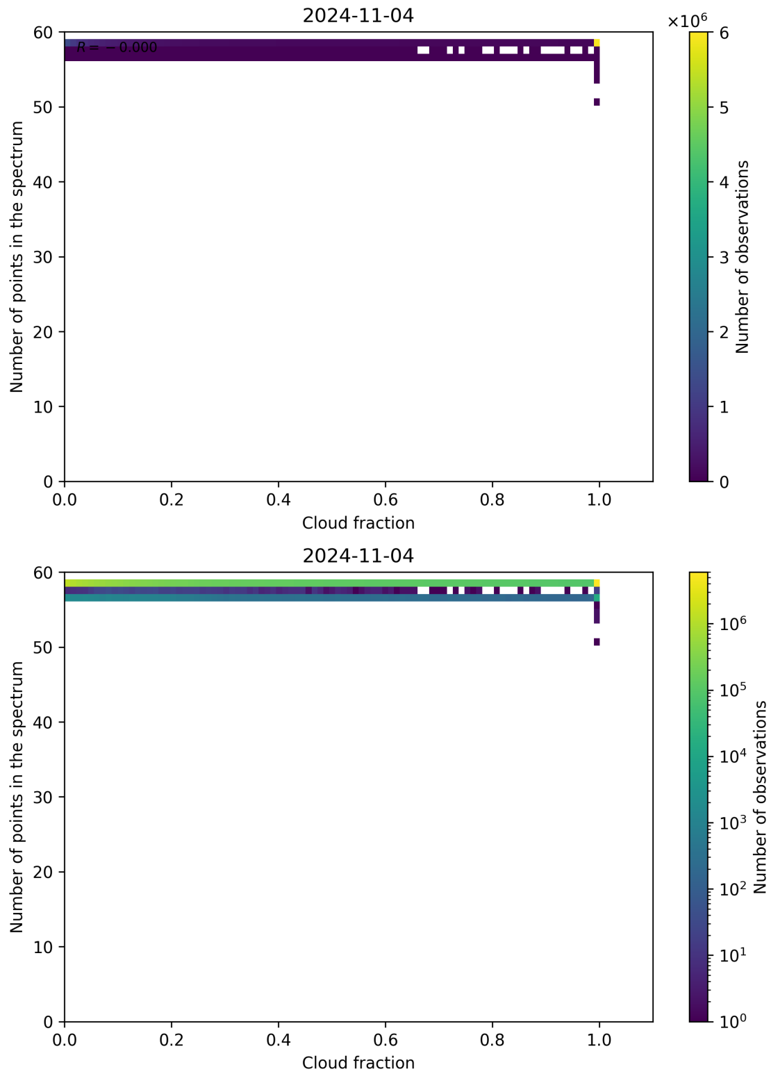
Figure 81: Scatter density plot of “Cloud fraction” against “Number of points in the spectrum” for 2024-11-04 to 2024-11-05.
