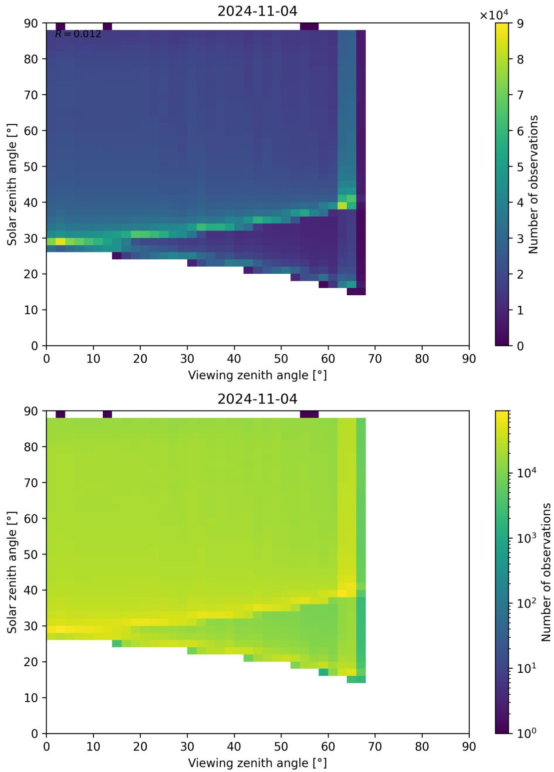
Figure 139: Scatter density plot of “Viewing zenith angle” against “Solar zenith angle” for 2024-11-04 to 2024-11-05.
