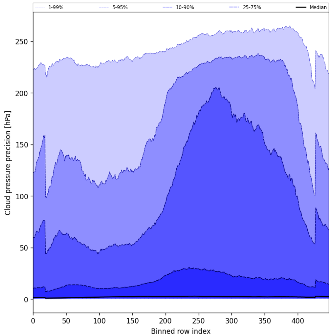
Figure 48: Along track statistics of “Cloud pressure precision” for 2024-11-04 to 2024-11-05
