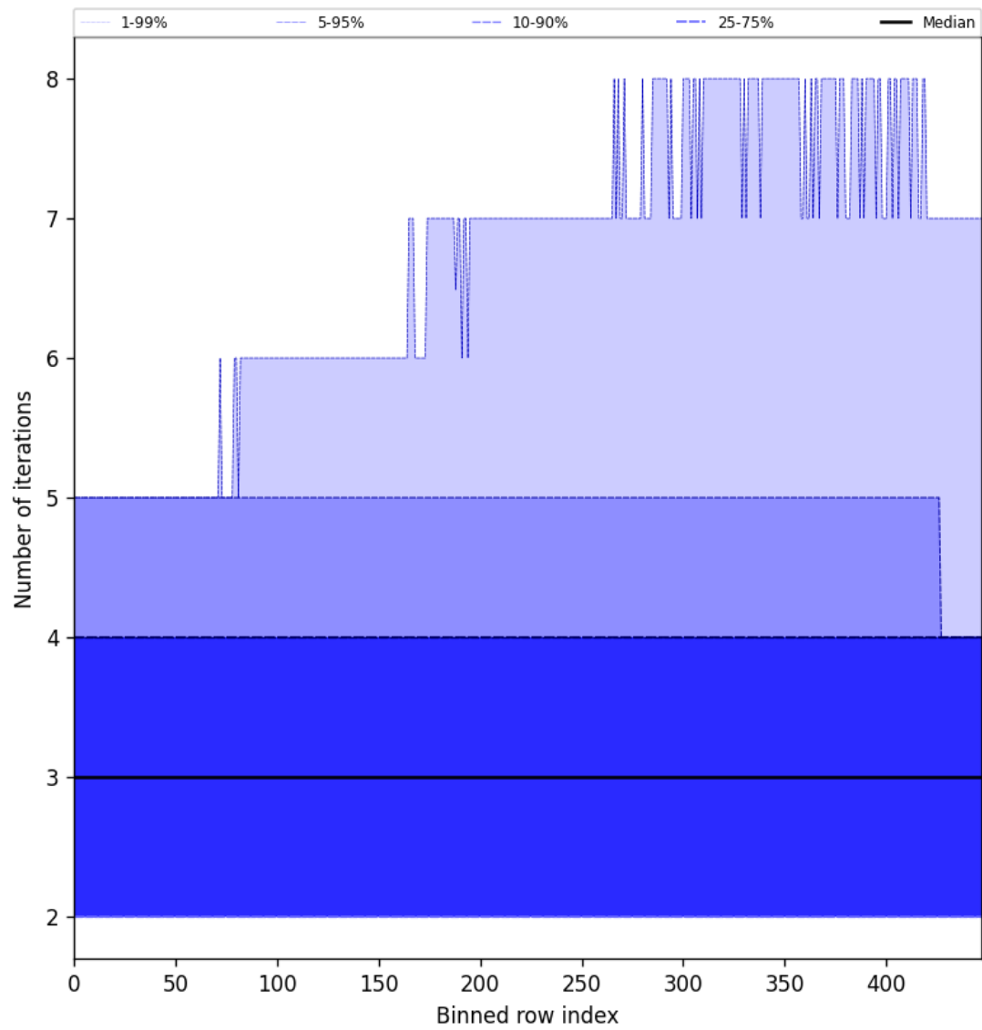
Figure 56: Along track statistics of “Number of iterations” for 2024-11-04 to 2024-11-05
