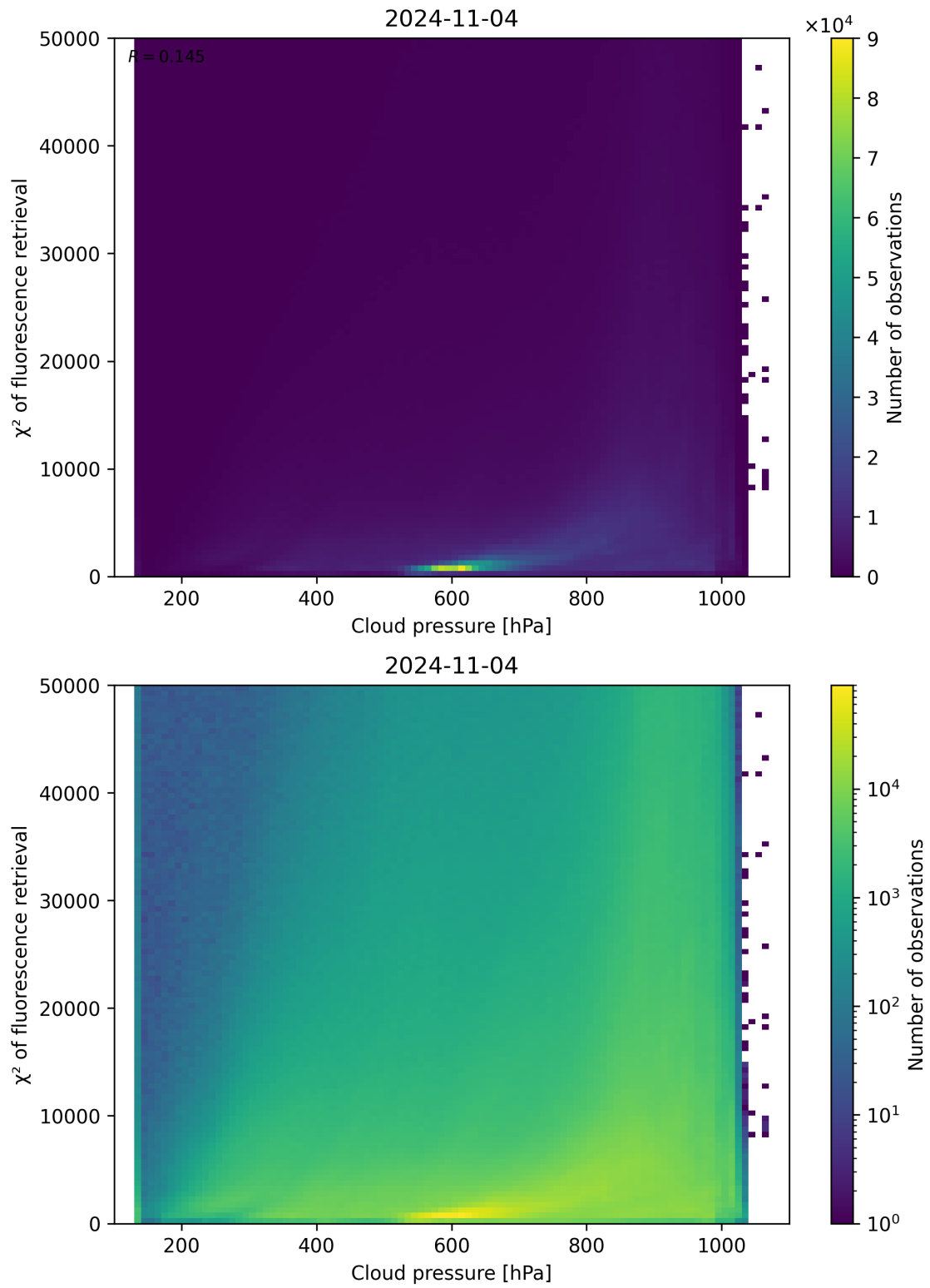
Figure 86: Scatter density plot of “Cloud pressure” against “ \chi^2 of fluorescence retrieval” for 2024-11-04 to 2024-11-05.
