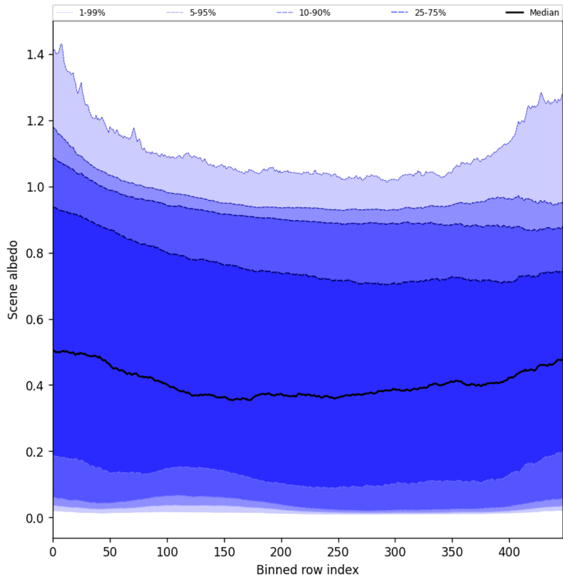
Figure 51: Along track statistics of “Scene albedo” for 2024-11-04 to 2024-11-05
