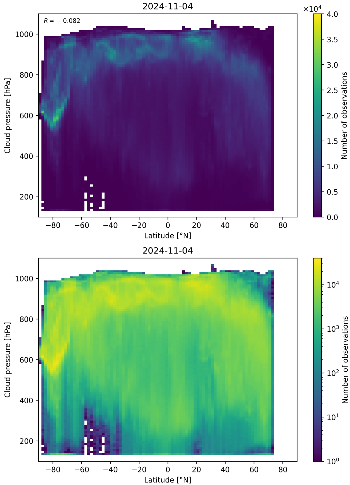
Figure 100: Scatter density plot of “Latitude” against “Cloud pressure” for 2024-11-04 to 2024-11-05.
