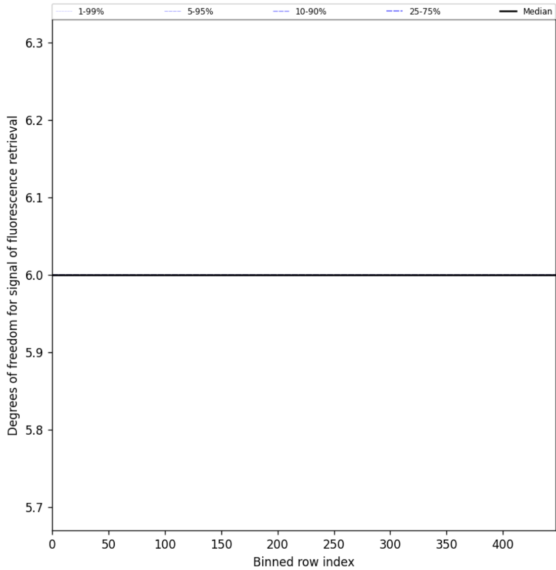
Figure 60: Along track statistics of “Degrees of freedom for signal of fluorescence retrieval” for 2024-11-04 to 2024-11-05
