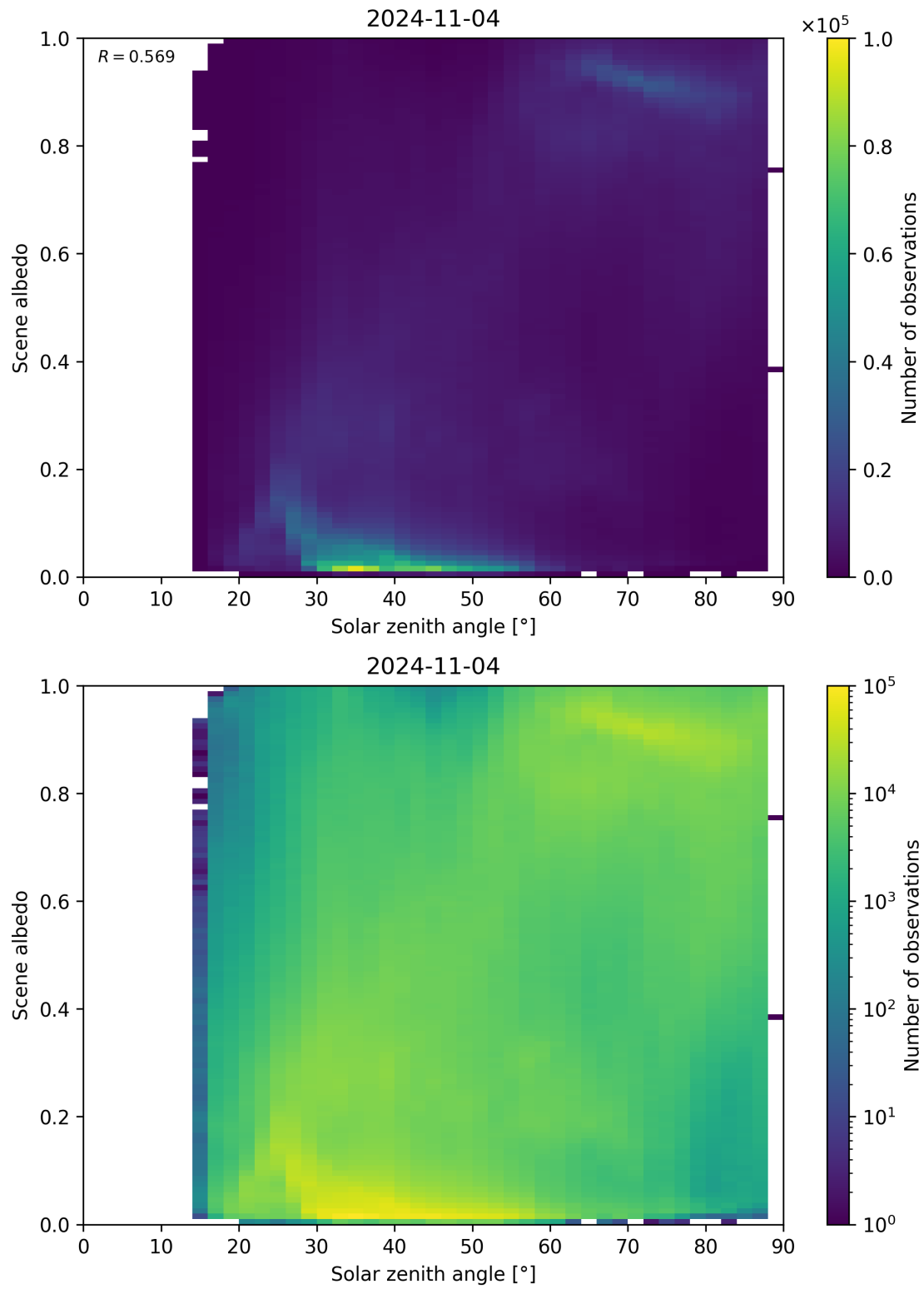
Figure 127: Scatter density plot of “Solar zenith angle” against “Scene albedo” for 2024-11-04 to 2024-11-05.
