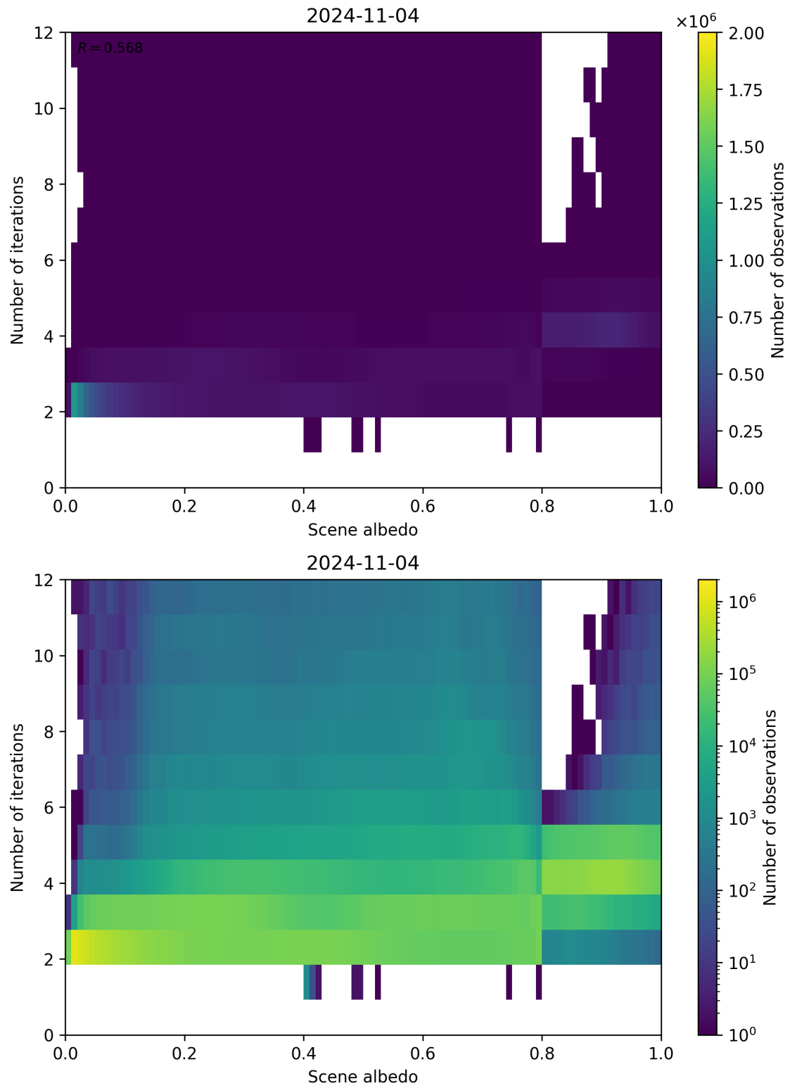
Figure 115: Scatter density plot of “Scene albedo” against “Number of iterations” for 2024-11-04 to 2024-11-05.
