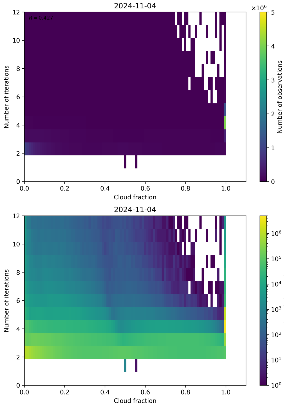
Figure 80: Scatter density plot of “Cloud fraction” against “Number of iterations” for 2024-11-04 to 2024-11-05.
