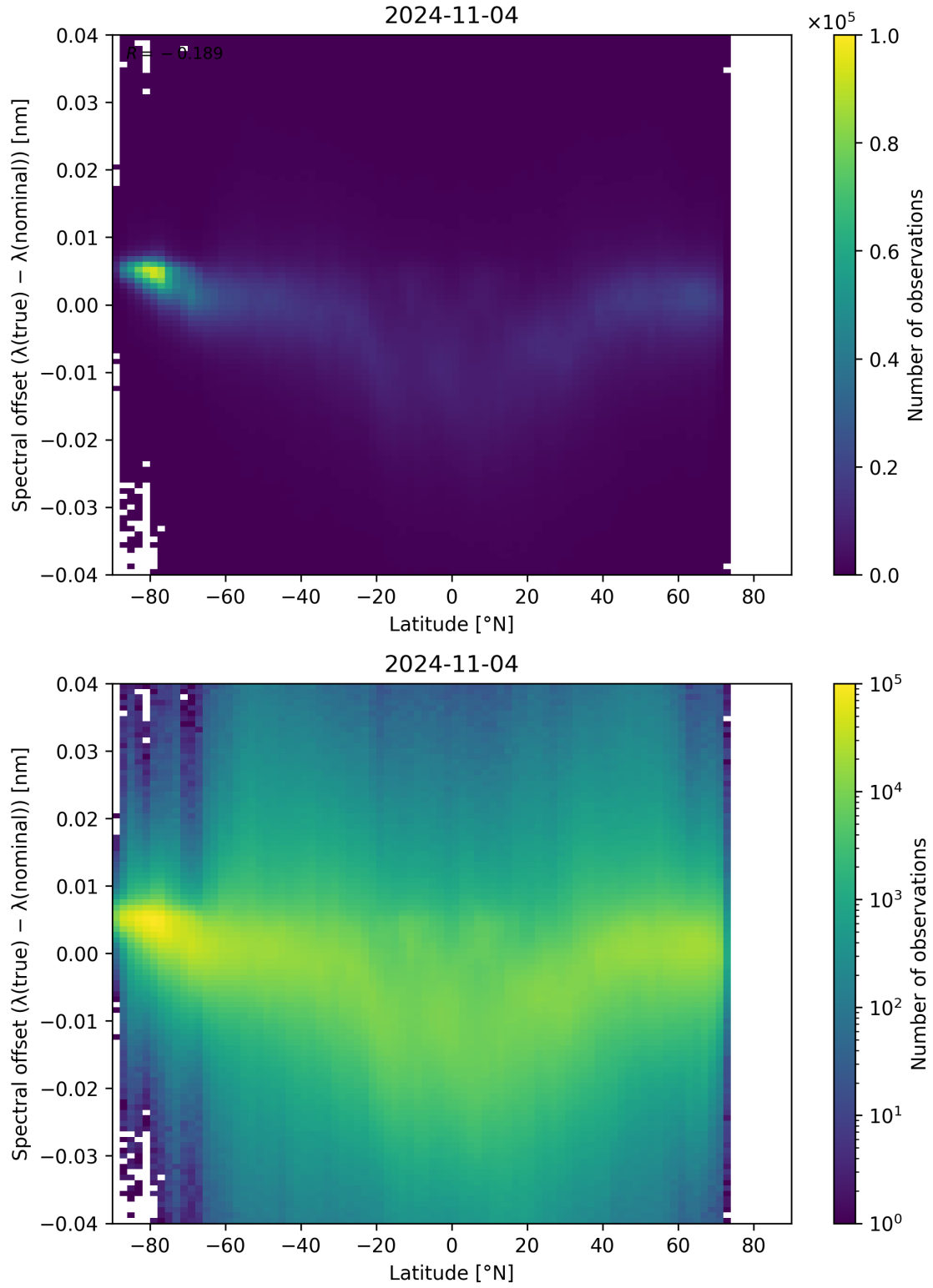
Figure 105: Scatter density plot of “Latitude” against “Spectral offset ( \lambda_{\text{true}} - \lambda_{\text{nominal}} )” for 2024-11-04 to 2024-11-05.
