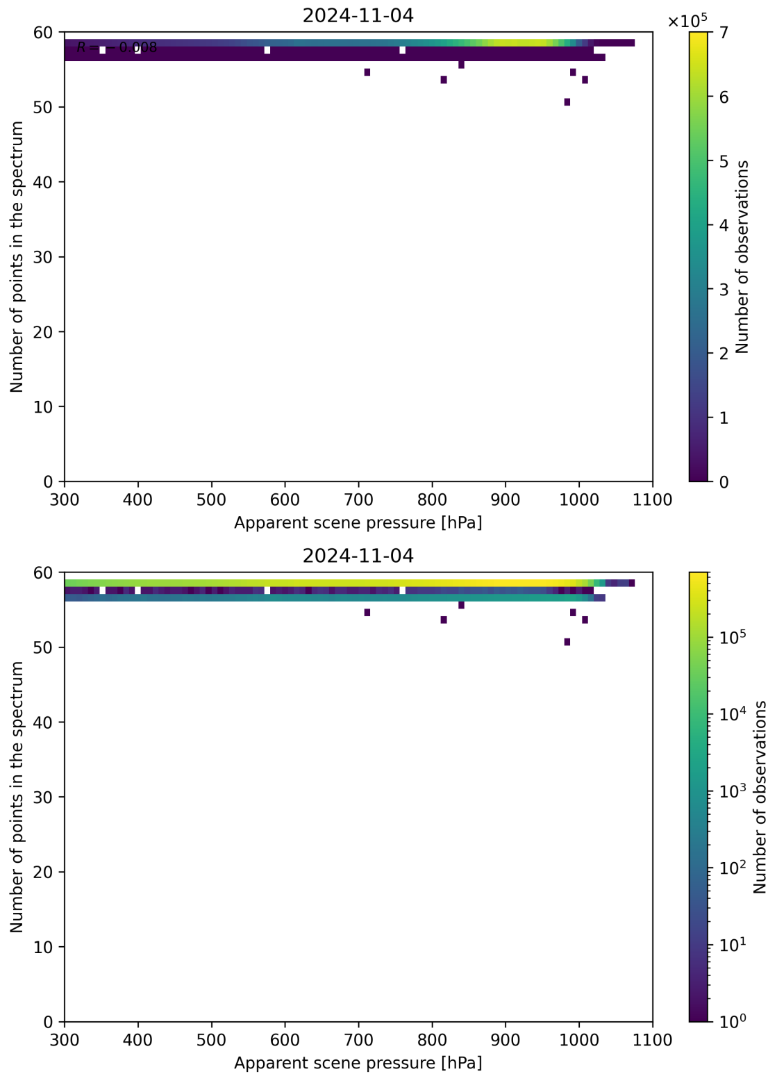
Figure 67: Scatter density plot of “Apparent scene pressure” against “Number of points in the spectrum” for 2024-11-04 to 2024-11-05.
