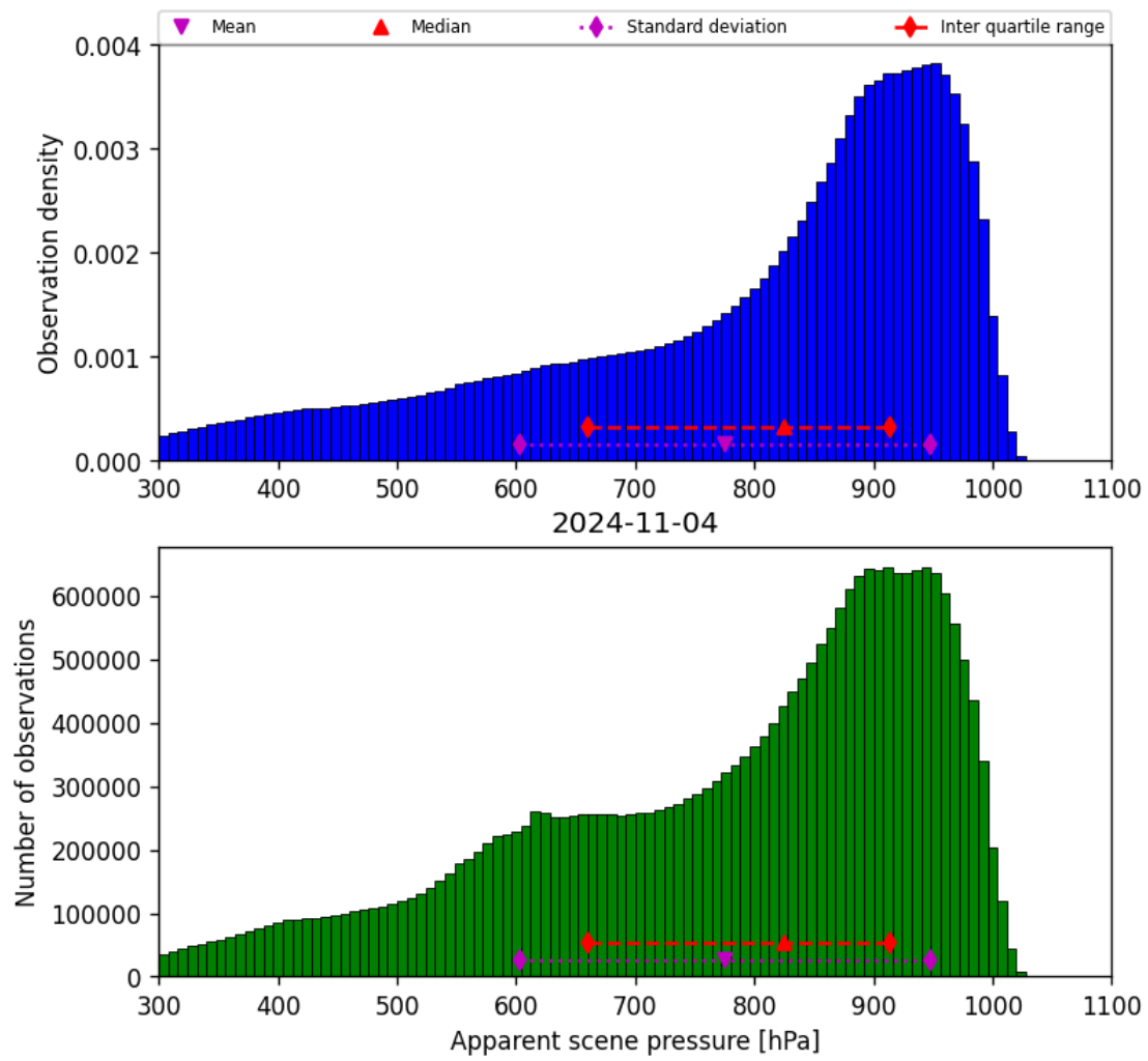
Figure 36: Histogram of “Apparent scene pressure” for 2024-11-04 to 2024-11-05
