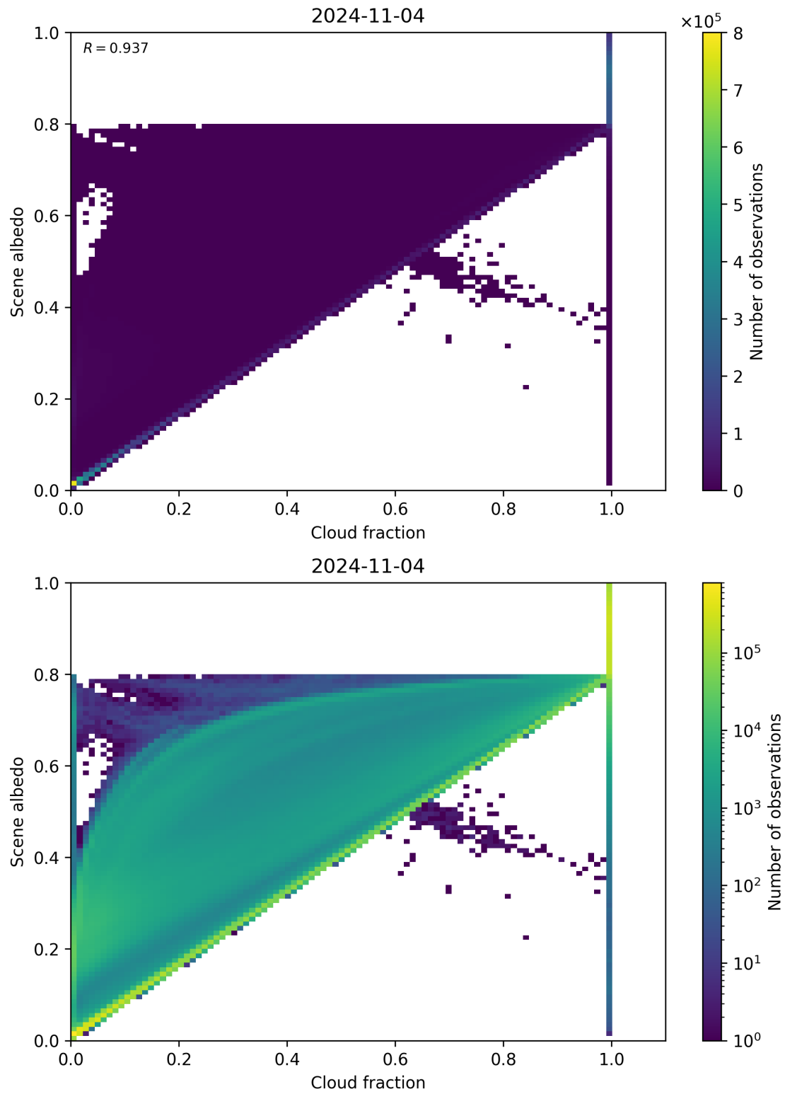
Figure 82: Scatter density plot of “Cloud fraction” against “Scene albedo” for 2024-11-04 to 2024-11-05.
