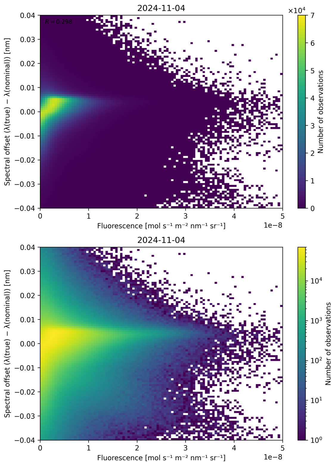
Figure 95: Scatter density plot of “Fluorescence” against “Spectral offset ( \lambda_{\text{true}} - \lambda_{\text{nominal}} )” for 2024-11-04 to 2024-11-05.
