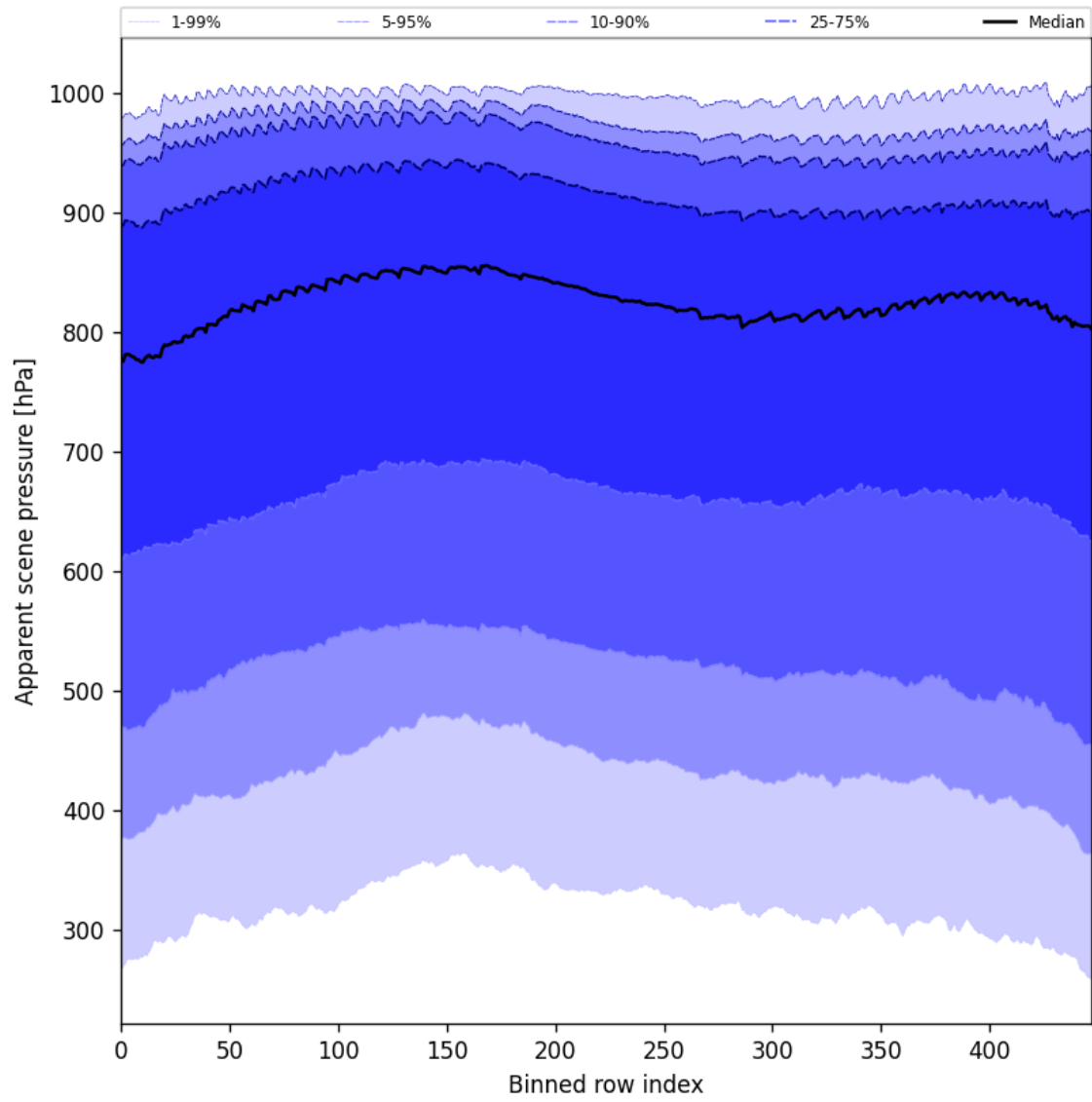
Figure 53: Along track statistics of “Apparent scene pressure” for 2024-11-04 to 2024-11-05
