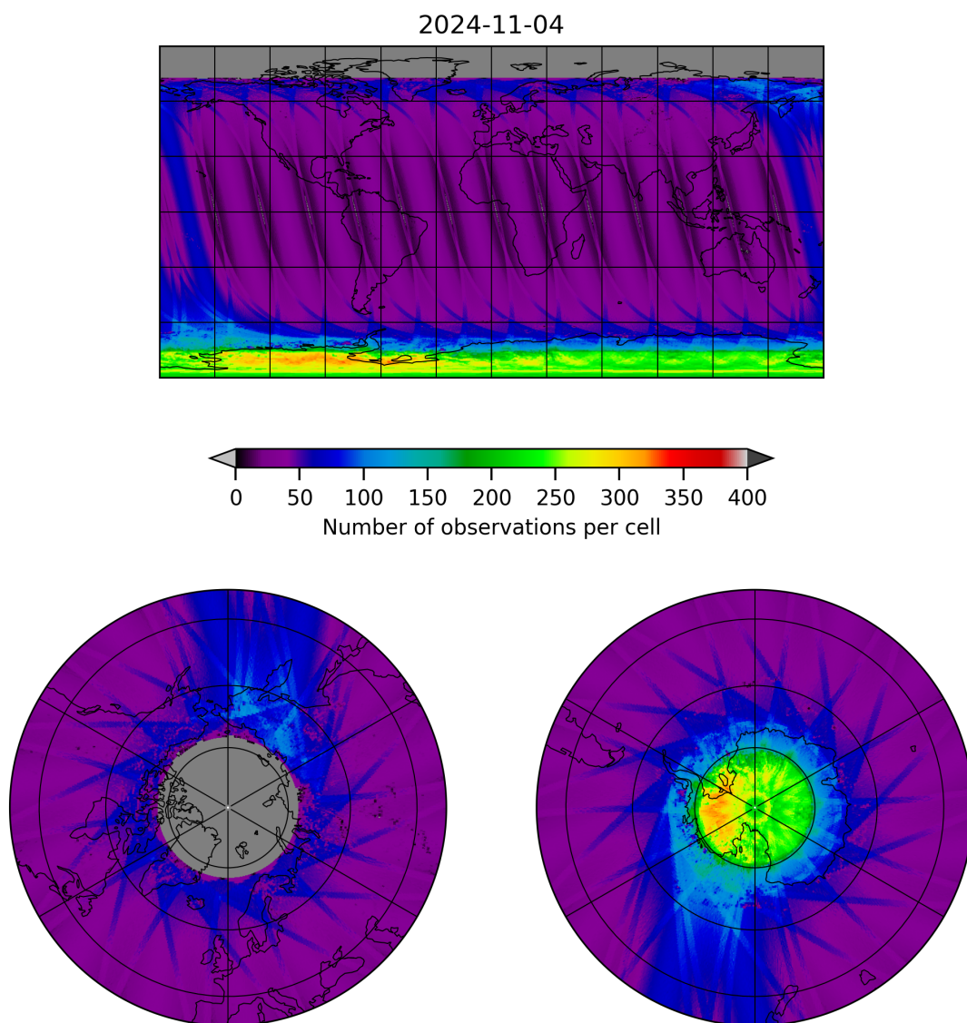
Figure 11: Map of the number of observations for 2024-11-04 to 2024-11-05
