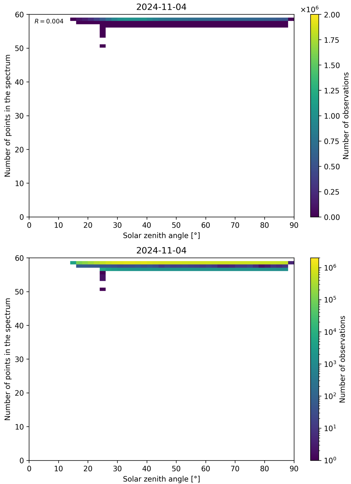
Figure 126: Scatter density plot of “Solar zenith angle” against “Number of points in the spectrum” for 2024-11-04 to 2024-11-05.
