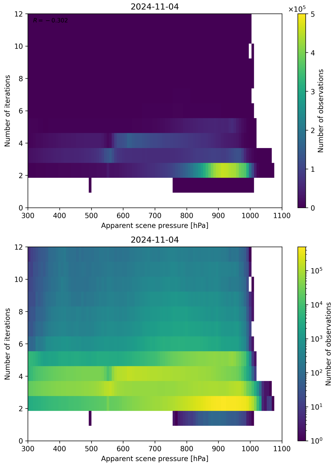
Figure 66: Scatter density plot of “Apparent scene pressure” against “Number of iterations” for 2024-11-04 to 2024-11-05.
