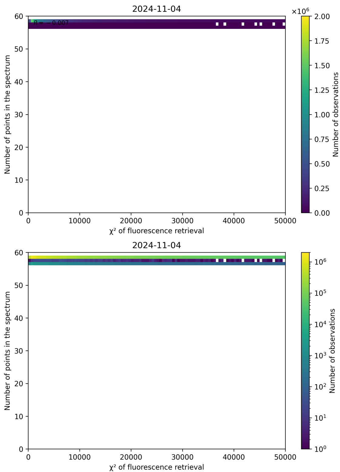
Figure 71: Scatter density plot of " \chi^2 of fluorescence retrieval" against "Number of points in the spectrum" for 2024-11-04 to 2024-11-05.
