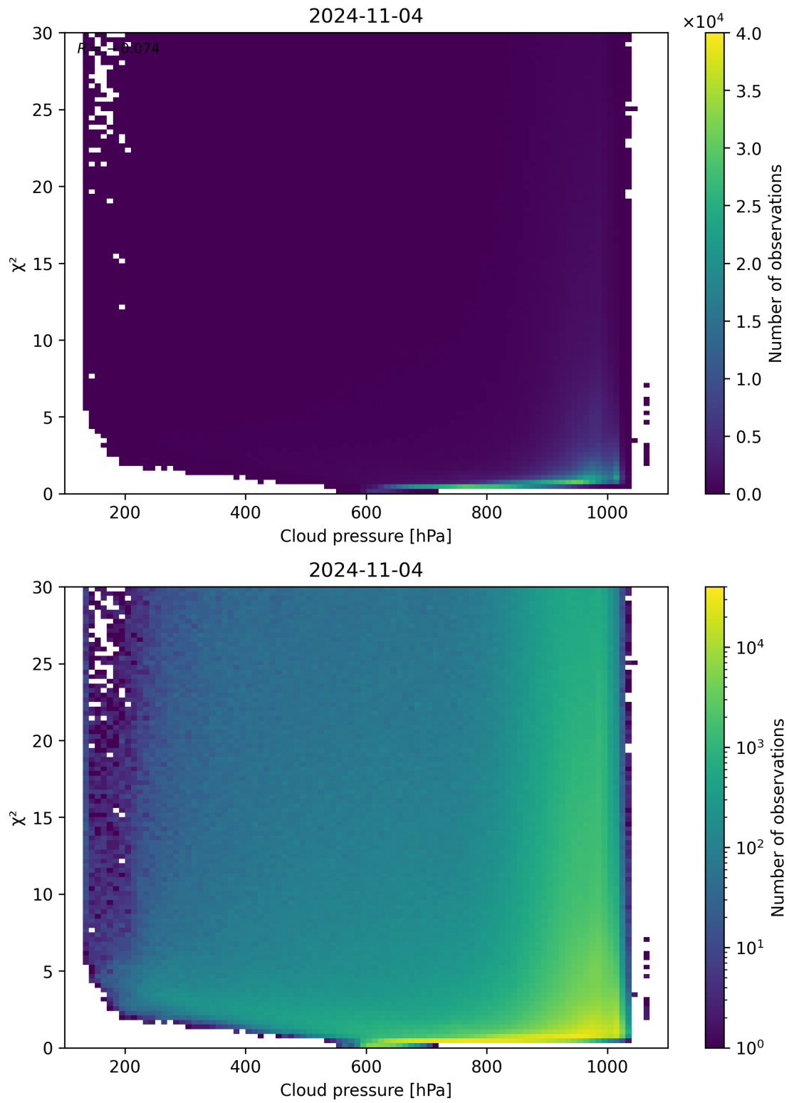
Figure 85: Scatter density plot of “Cloud pressure” against “ \chi^2 ” for 2024-11-04 to 2024-11-05.
