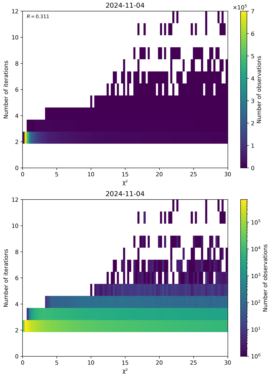
Figure 73: Scatter density plot of “ \chi^2 ” against “Number of iterations” for 2024-11-04 to 2024-11-05.
