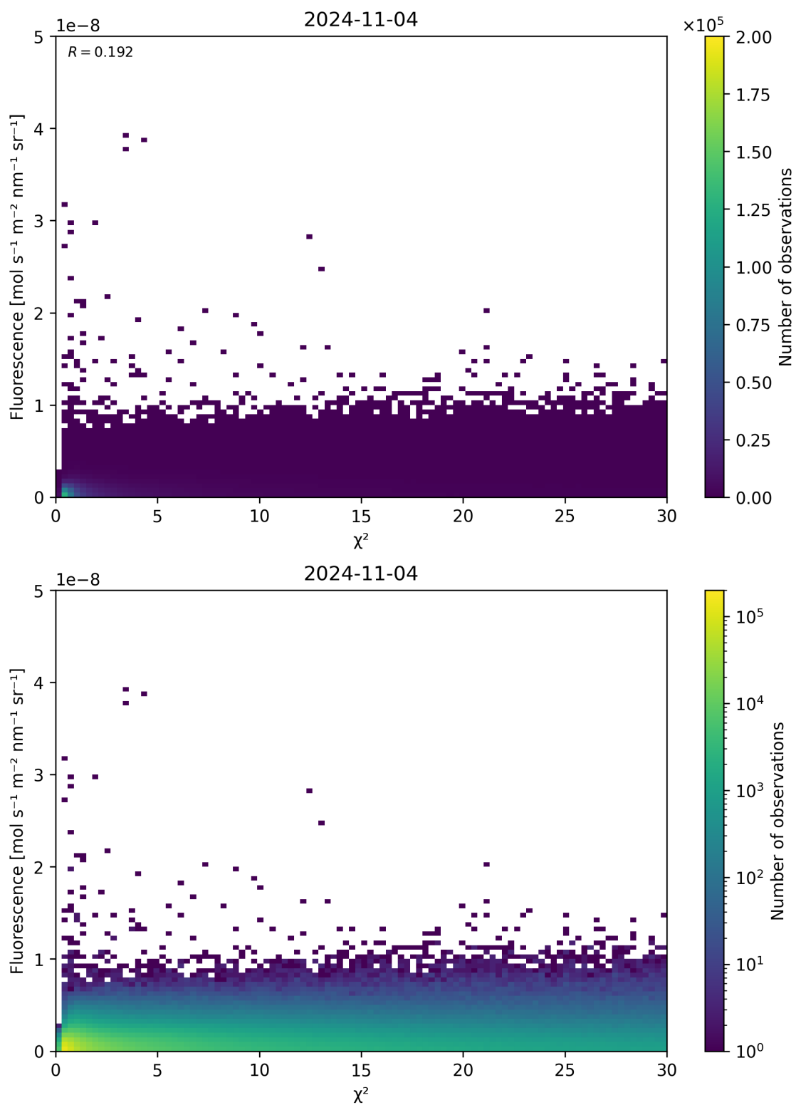
Figure 70: Scatter density plot of “ \chi^2 ” against “Fluorescence” for 2024-11-04 to 2024-11-05.
