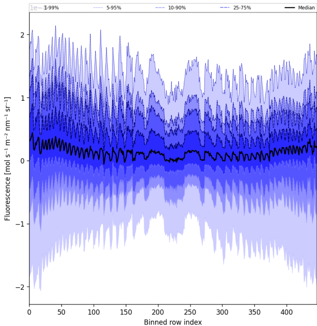
Figure 57: Along track statistics of “Fluorescence” for 2024-11-04 to 2024-11-05
