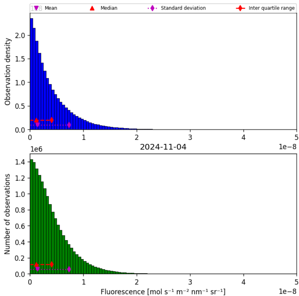
Figure 40: Histogram of “Fluorescence” for 2024-11-04 to 2024-11-05
