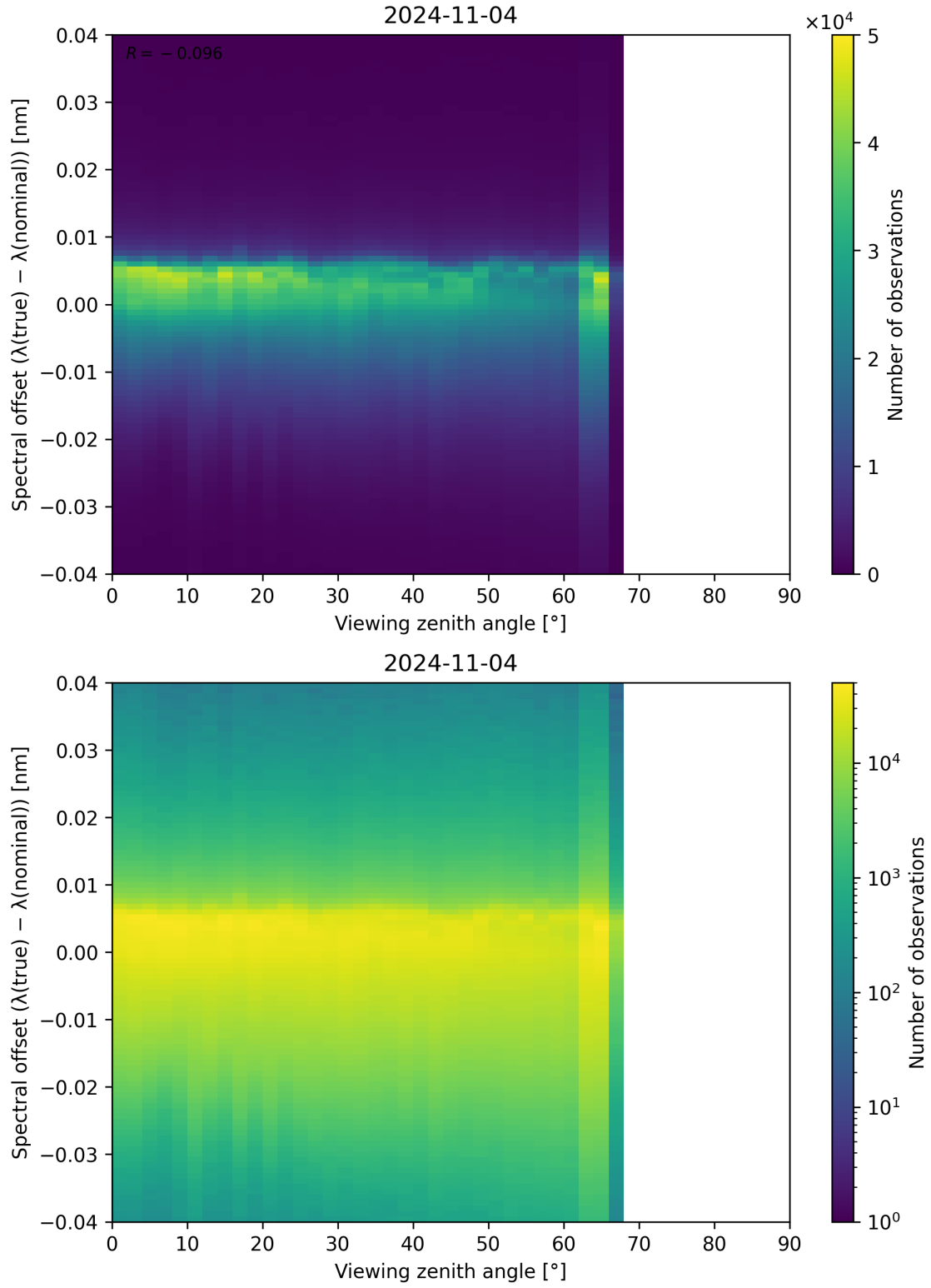
Figure 140: Scatter density plot of “Viewing zenith angle” against “Spectral offset ( \lambda_{\text{true}} - \lambda_{\text{nominal}} )” for 2024-11-04 to 2024-11-05.
