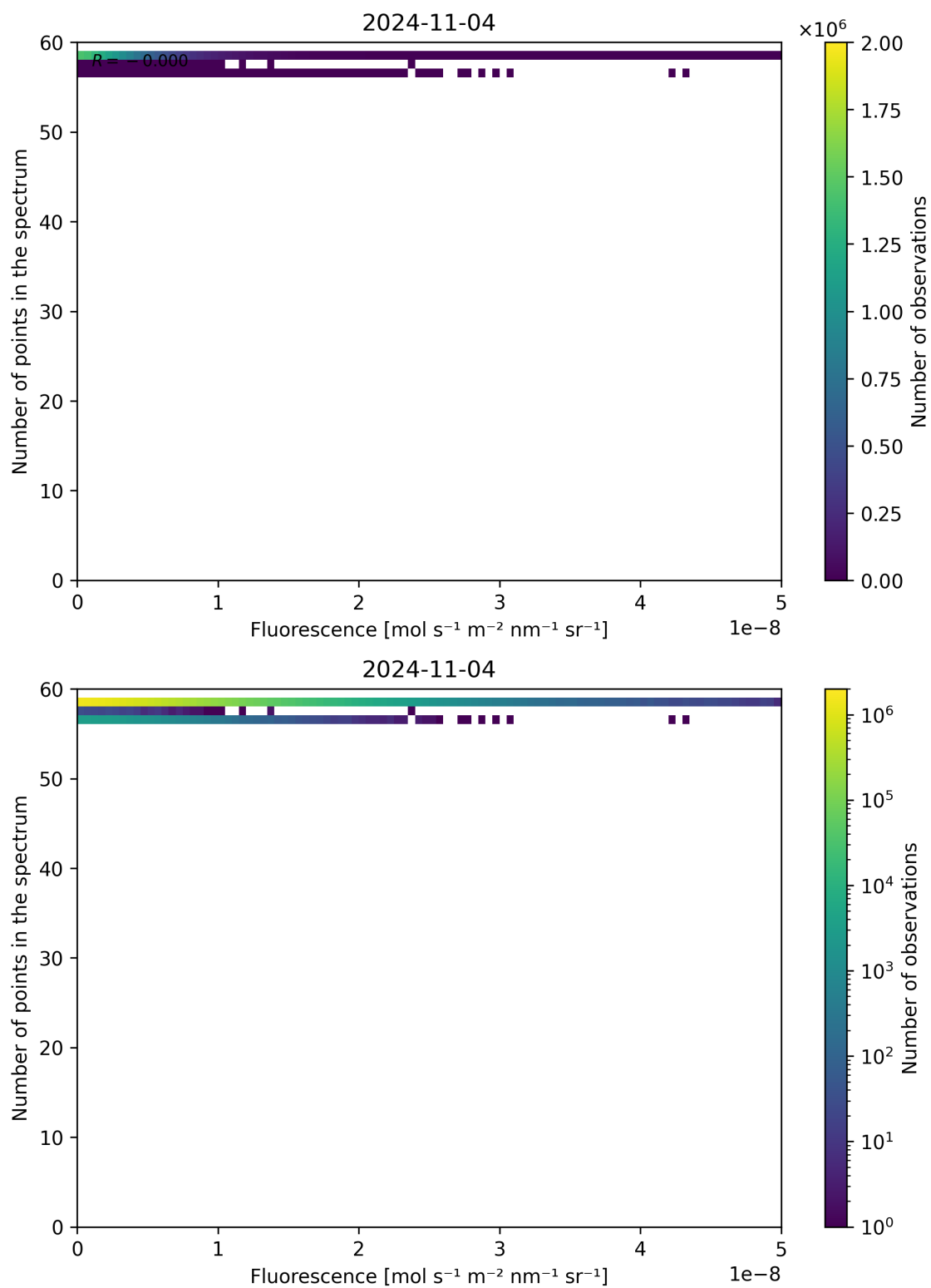
Figure 94: Scatter density plot of “Fluorescence” against “Number of points in the spectrum” for 2024-11-04 to 2024-11-05.
