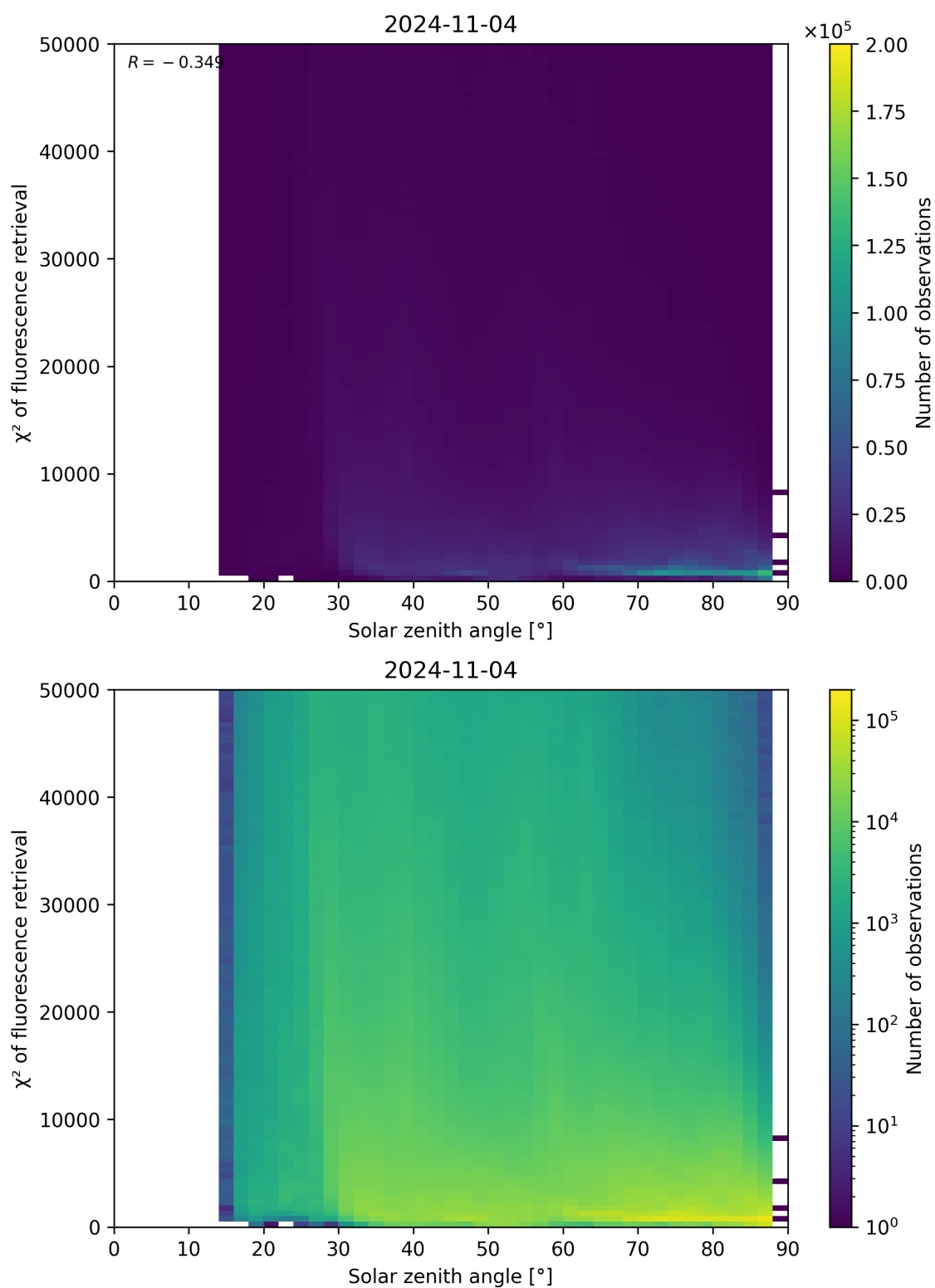
Figure 120: Scatter density plot of “Solar zenith angle” against “ \chi^2 of fluorescence retrieval” for 2024-11-04 to 2024-11-05.
