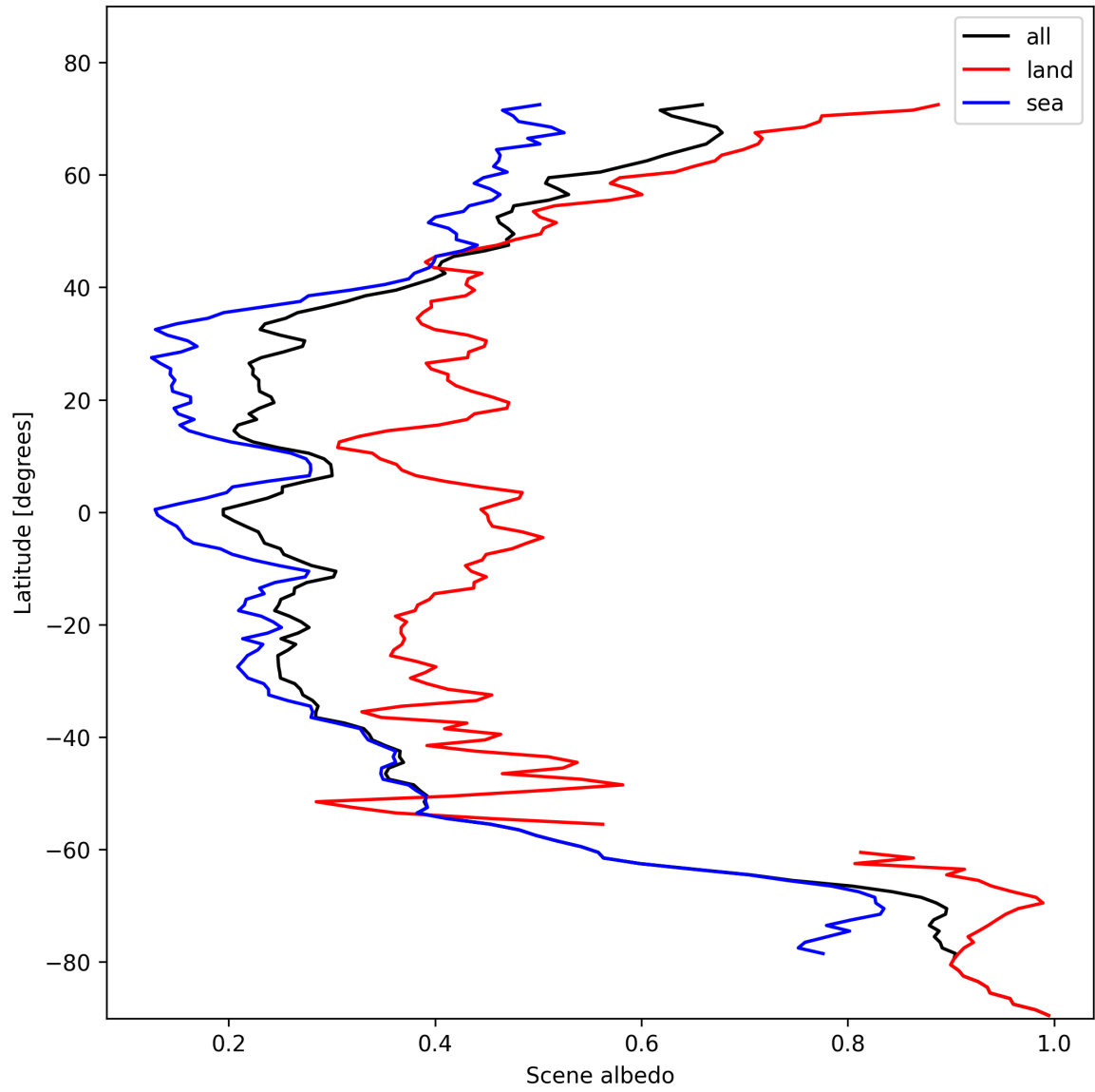
Figure 17: Zonal average of “Scene albedo” for 2024-11-04 to 2024-11-05.
