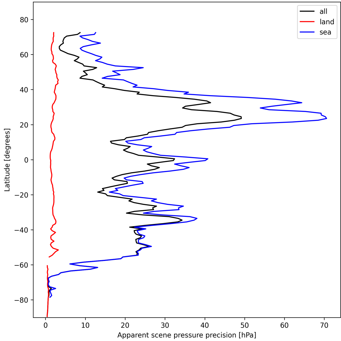
Figure 20: Zonal average of “Apparent scene pressure precision” for 2024-11-04 to 2024-11-05.
