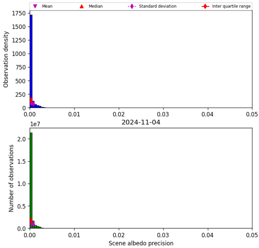
Figure 35: Histogram of “Scene albedo precision” for 2024-11-04 to 2024-11-05
