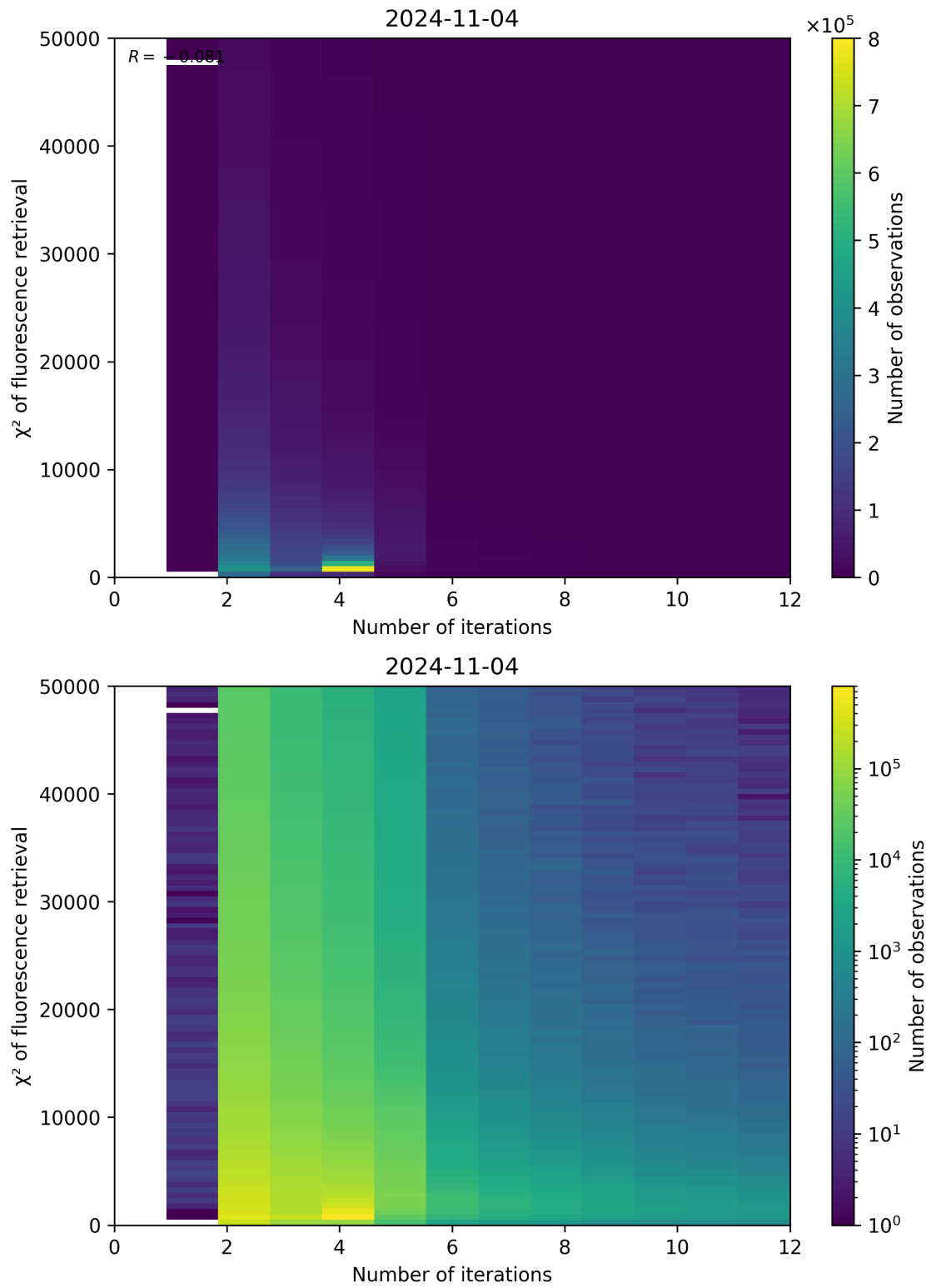
Figure 106: Scatter density plot of “Number of iterations” against “ \chi^2 of fluorescence retrieval” for 2024-11-04 to 2024-11-05.
