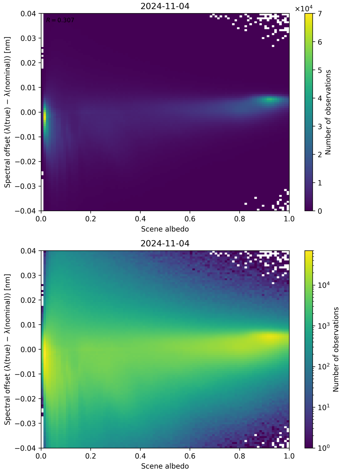
Figure 117: Scatter density plot of “Scene albedo” against “Spectral offset ( \lambda_{\text{true}} - \lambda_{\text{nominal}} )” for 2024-11-04 to 2024-11-05.
