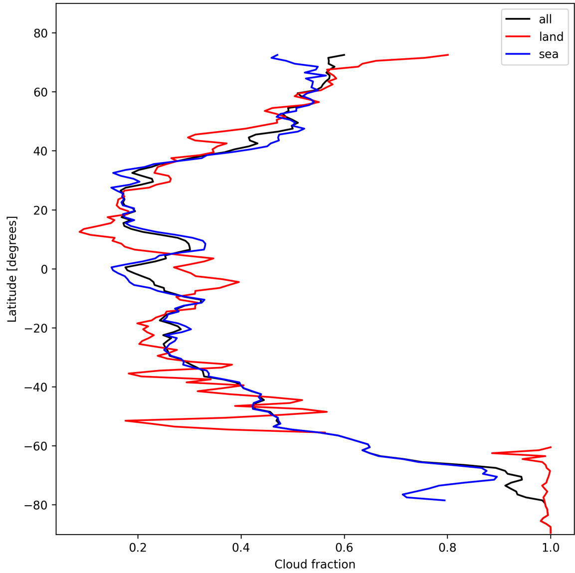
Figure 15: Zonal average of “Cloud fraction” for 2024-11-04 to 2024-11-05.
