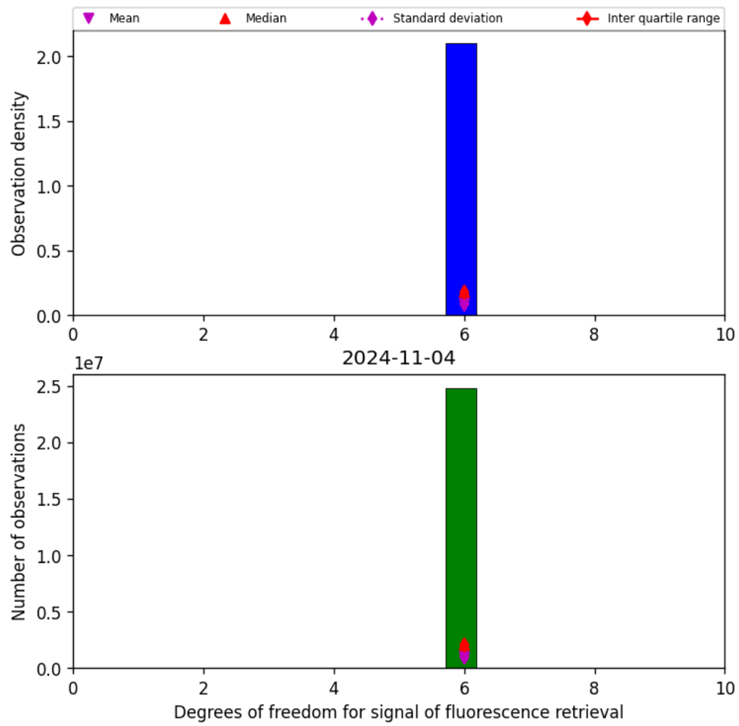
Figure 43: Histogram of “Degrees of freedom for signal of fluorescence retrieval” for 2024-11-04 to 2024-11-05
