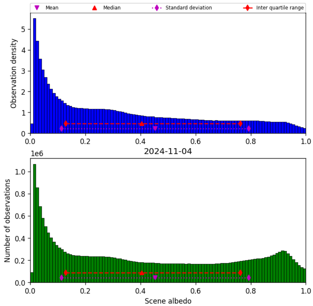
Figure 34: Histogram of “Scene albedo” for 2024-11-04 to 2024-11-05
