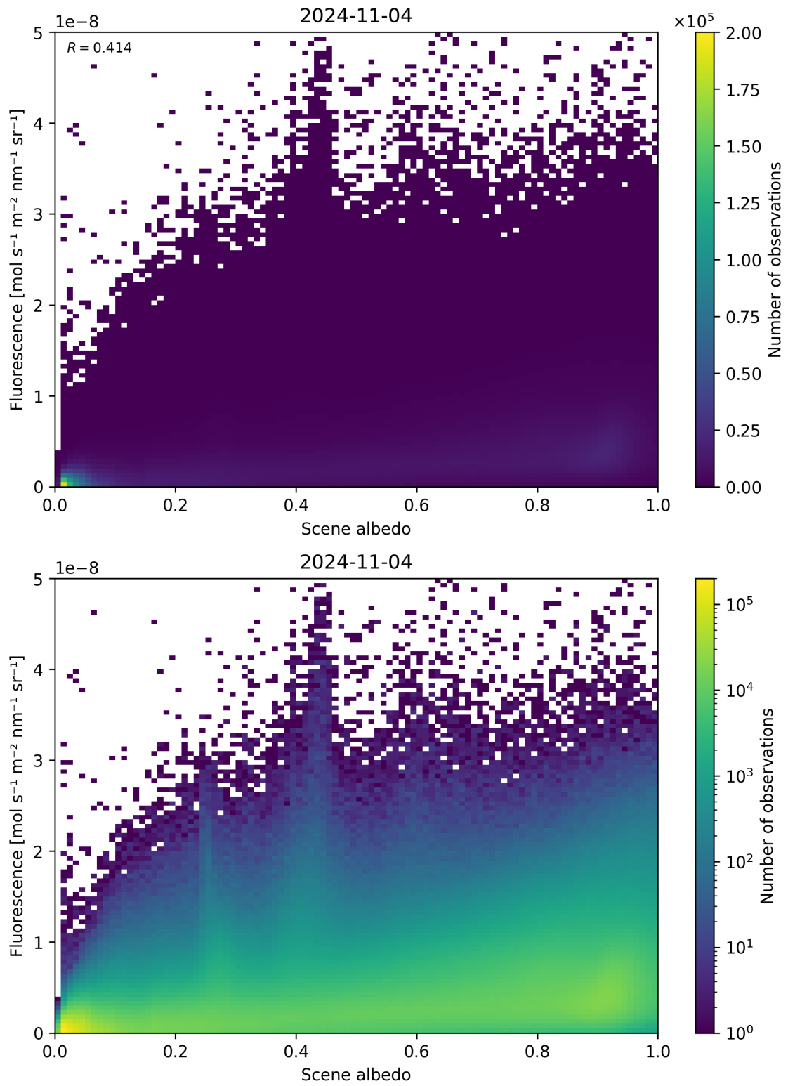
Figure 114: Scatter density plot of “Scene albedo” against “Fluorescence” for 2024-11-04 to 2024-11-05.
