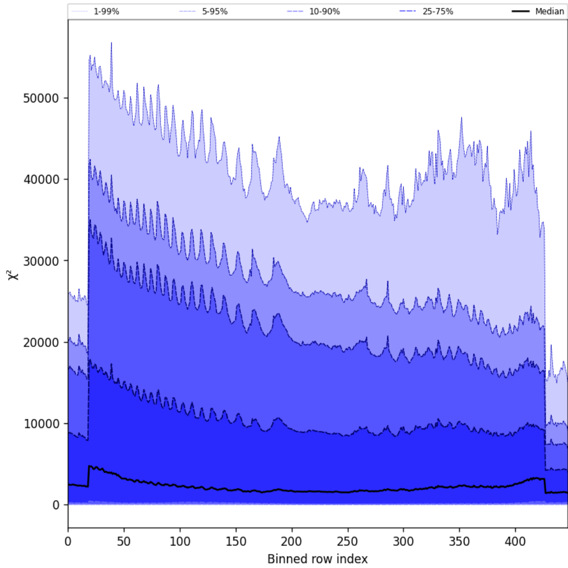
Figure 55: Along track statistics of “ \chi^2 ” for 2024-11-04 to 2024-11-05
