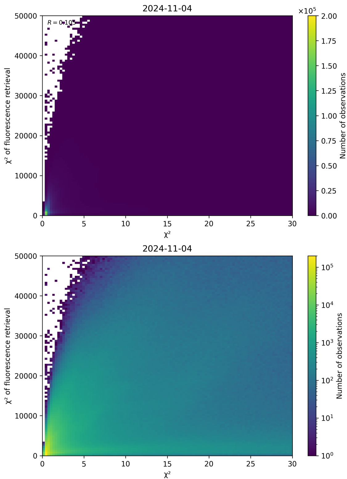
Figure 69: Scatter density plot of “ \chi^2 ” against “ \chi^2 of fluorescence retrieval” for 2024-11-04 to 2024-11-05.
