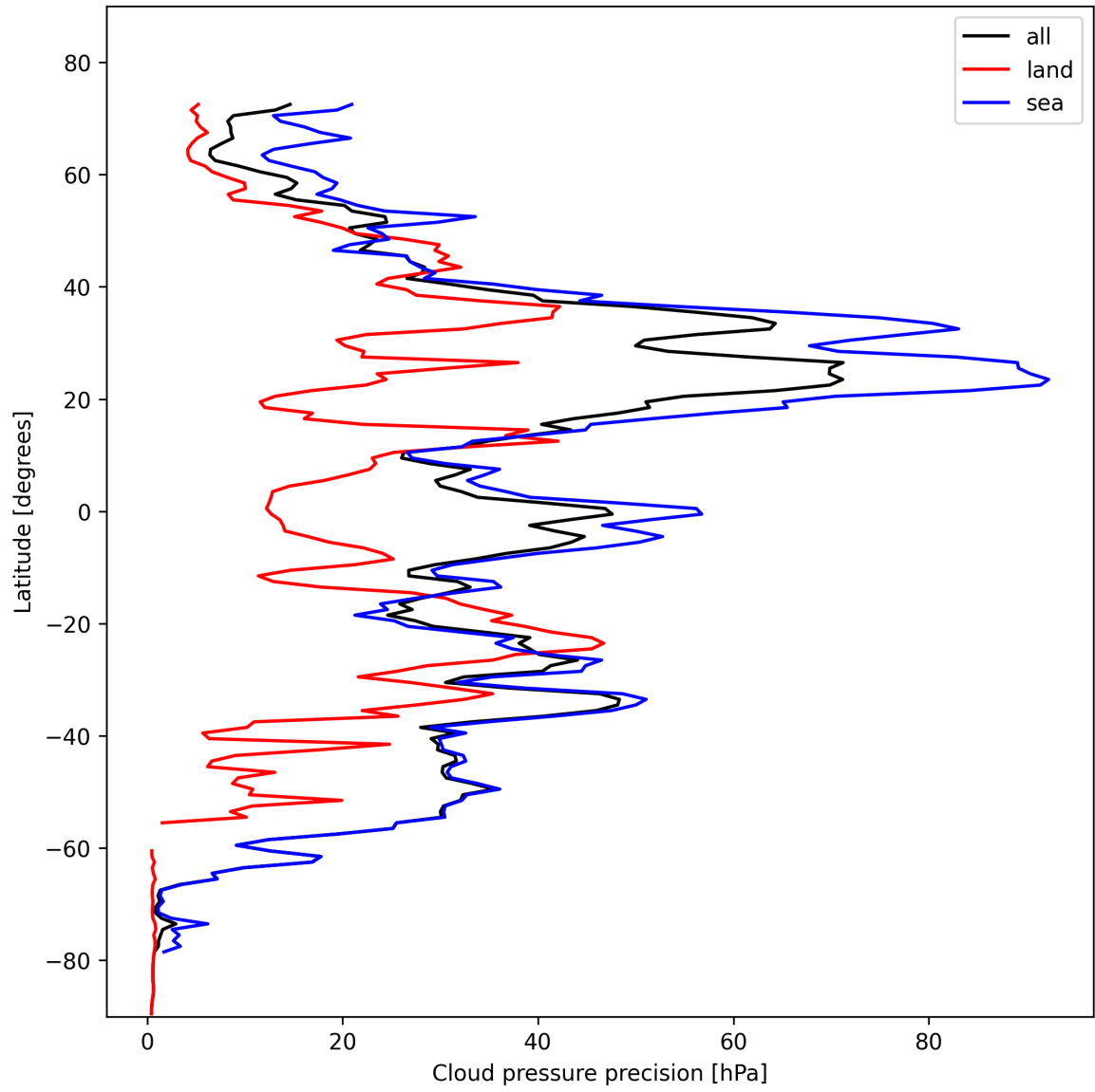
Figure 14: Zonal average of “Cloud pressure precision” for 2024-11-04 to 2024-11-05.
