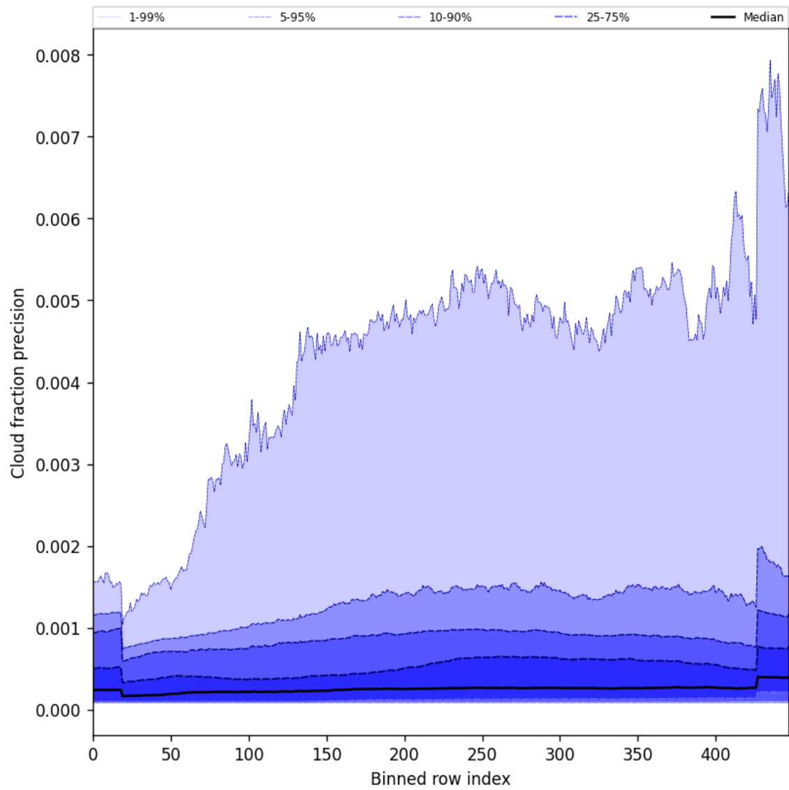
Figure 50: Along track statistics of “Cloud fraction precision” for 2024-11-04 to 2024-11-05
