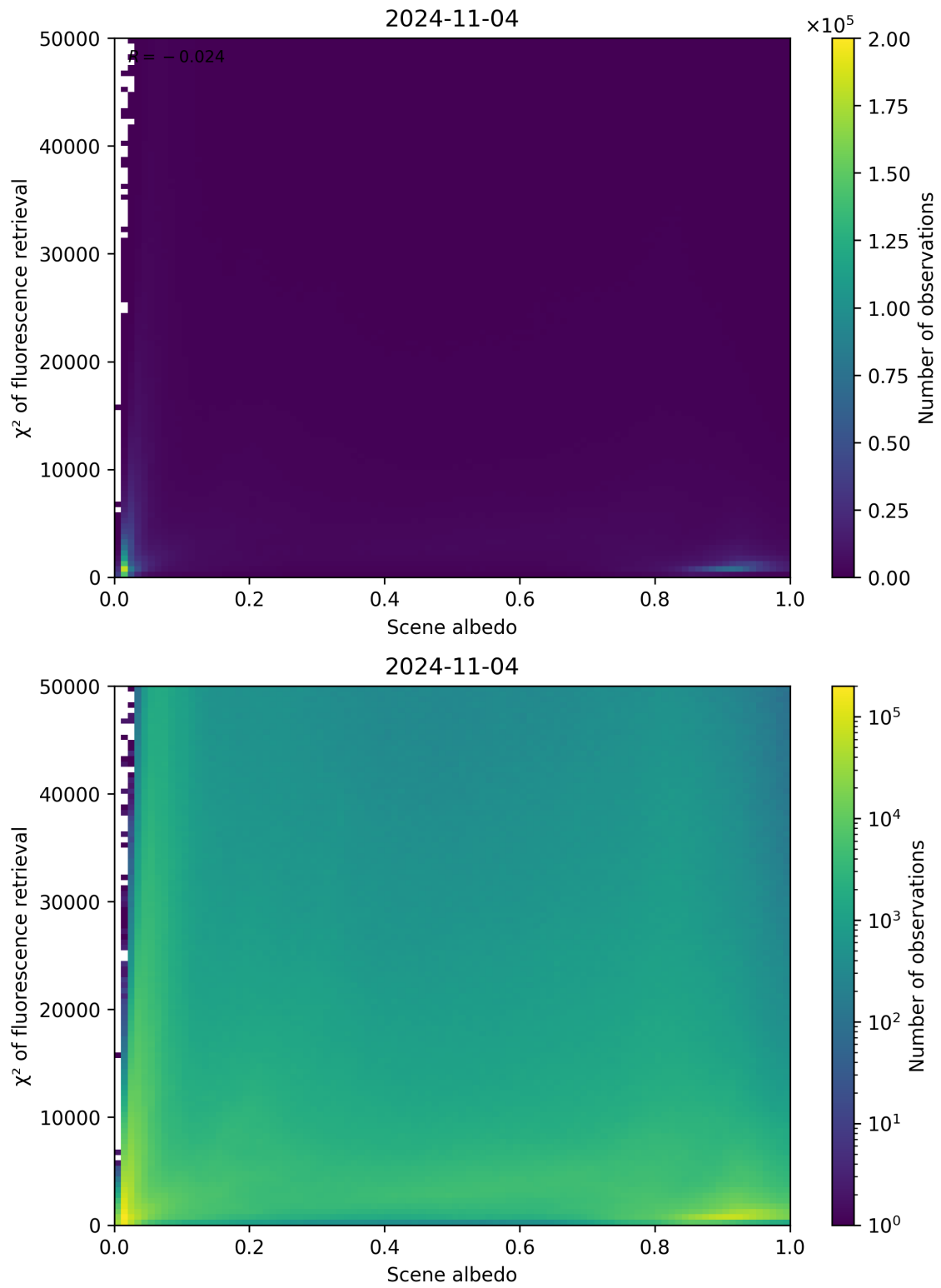
Figure 113: Scatter density plot of “Scene albedo” against “ \chi^2 of fluorescence retrieval” for 2024-11-04 to 2024-11-05.
