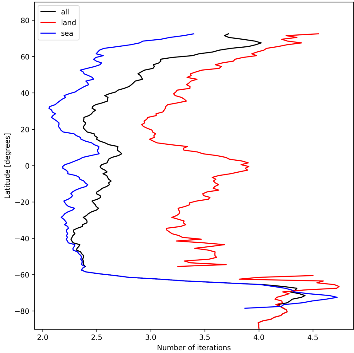
Figure 22: Zonal average of “Number of iterations” for 2024-11-04 to 2024-11-05.
