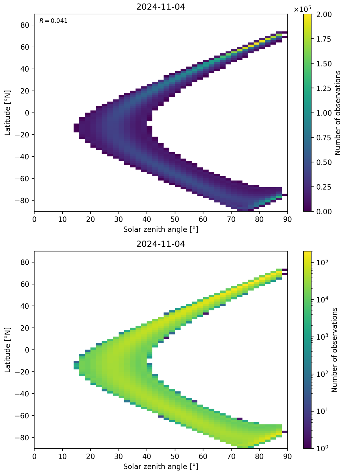
Figure 124: Scatter density plot of “Solar zenith angle” against “Latitude” for 2024-11-04 to 2024-11-05.
