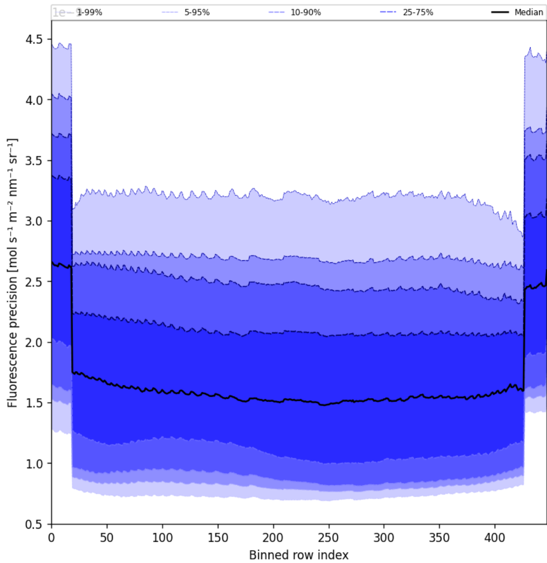
Figure 58: Along track statistics of “Fluorescence precision” for 2024-11-04 to 2024-11-05
