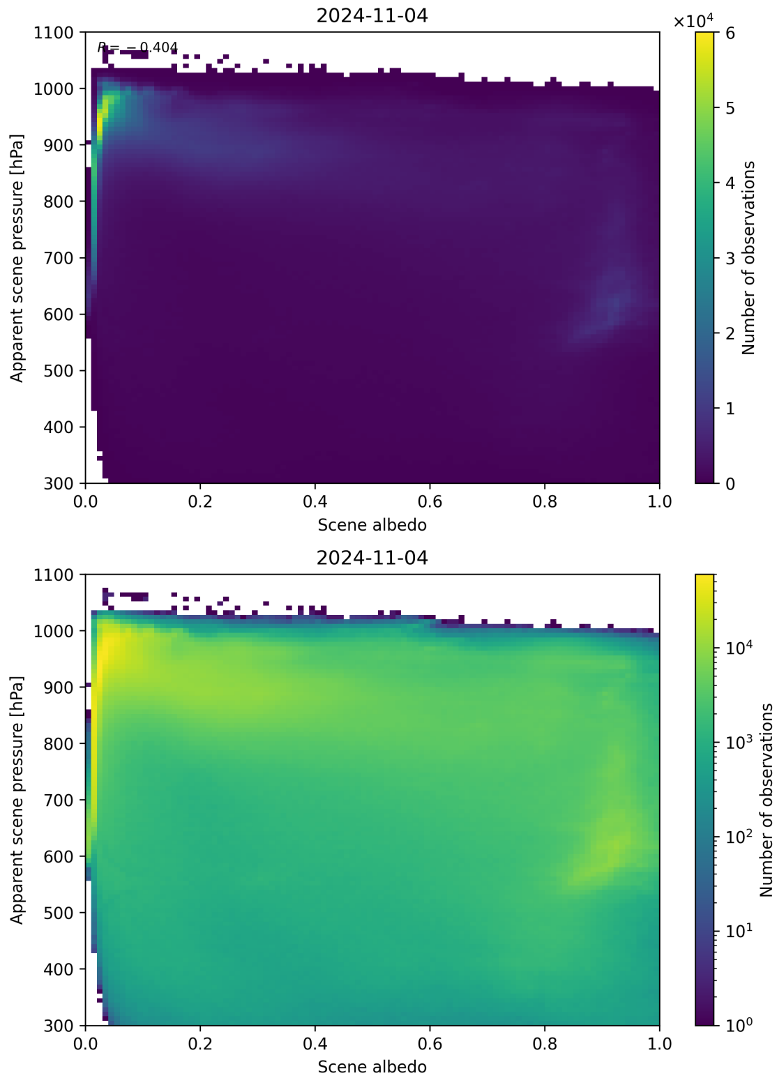
Figure 111: Scatter density plot of “Scene albedo” against “Apparent scene pressure” for 2024-11-04 to 2024-11-05.
