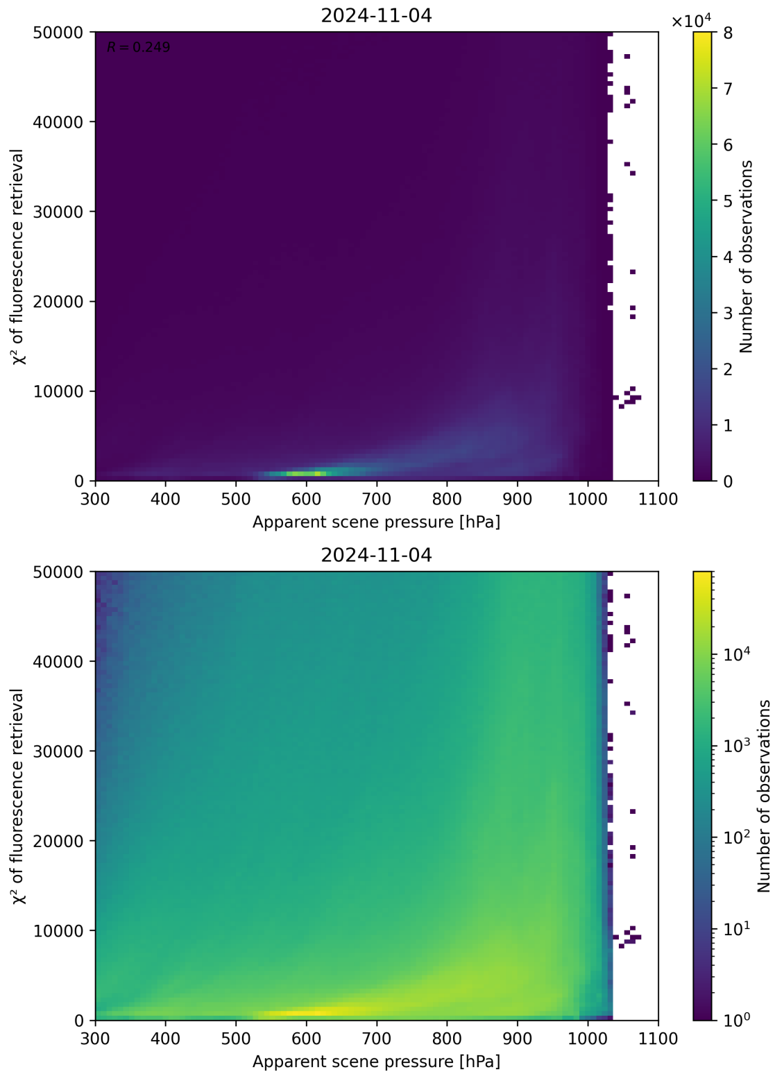
Figure 64: Scatter density plot of “Apparent scene pressure” against “ \chi^2 of fluorescence retrieval” for 2024-11-04 to 2024-11-05.
