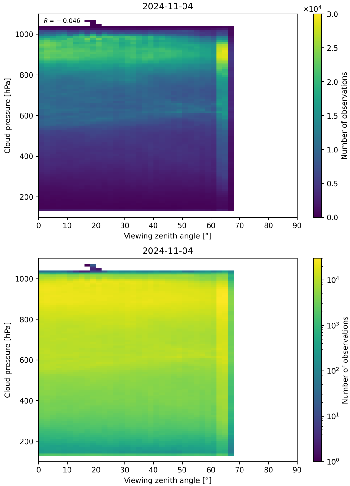
Figure 133: Scatter density plot of “Viewing zenith angle” against “Cloud pressure” for 2024-11-04 to 2024-11-05.
