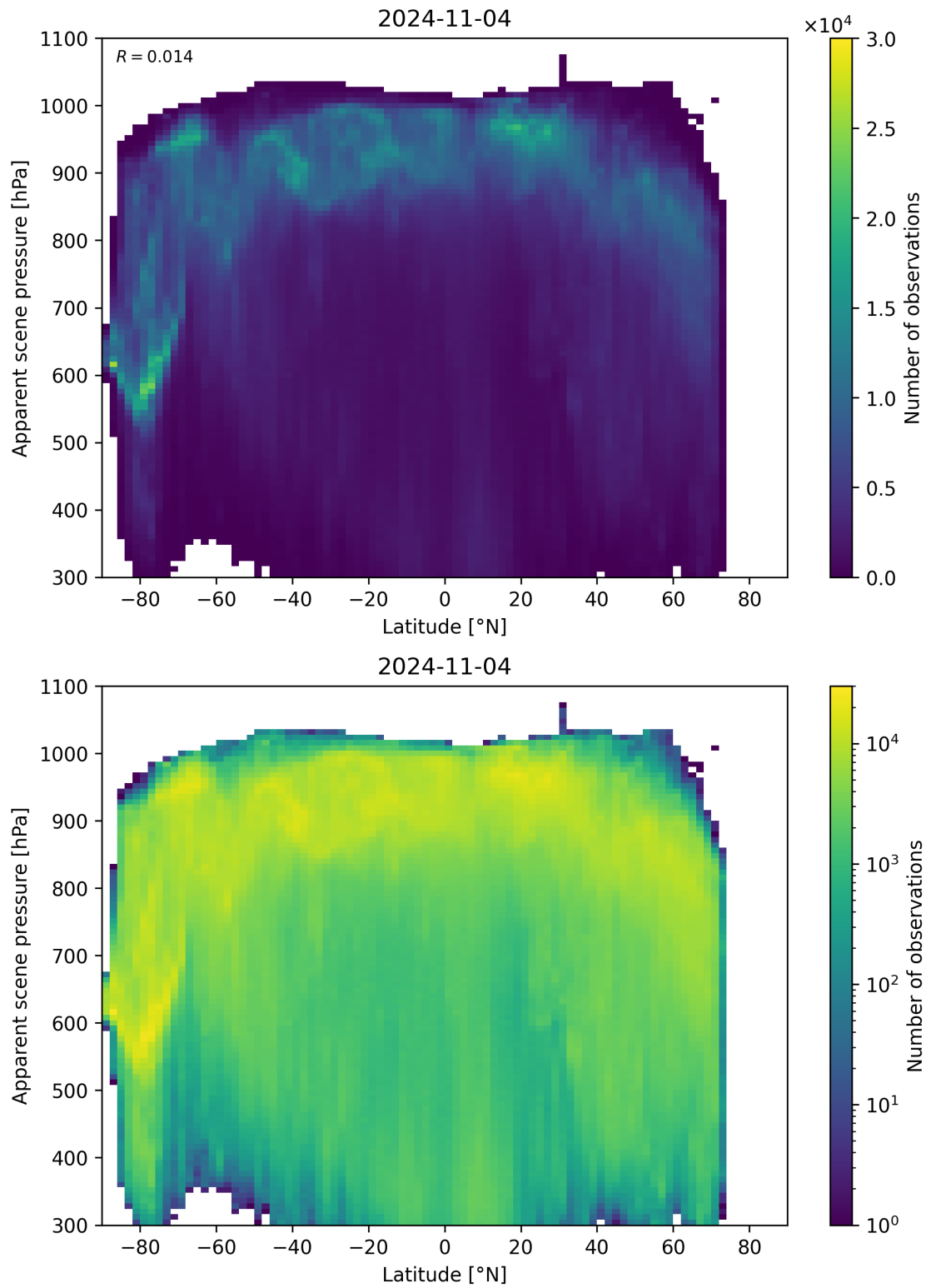
Figure 96: Scatter density plot of “Latitude” against “Apparent scene pressure” for 2024-11-04 to 2024-11-05.
