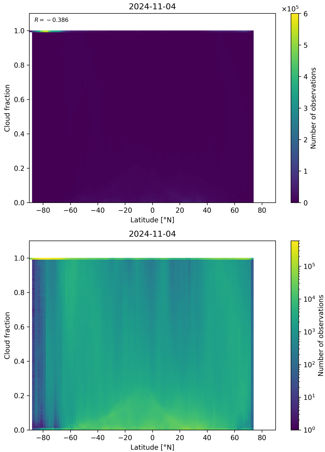
Figure 99: Scatter density plot of “Latitude” against “Cloud fraction” for 2024-11-04 to 2024-11-05.
