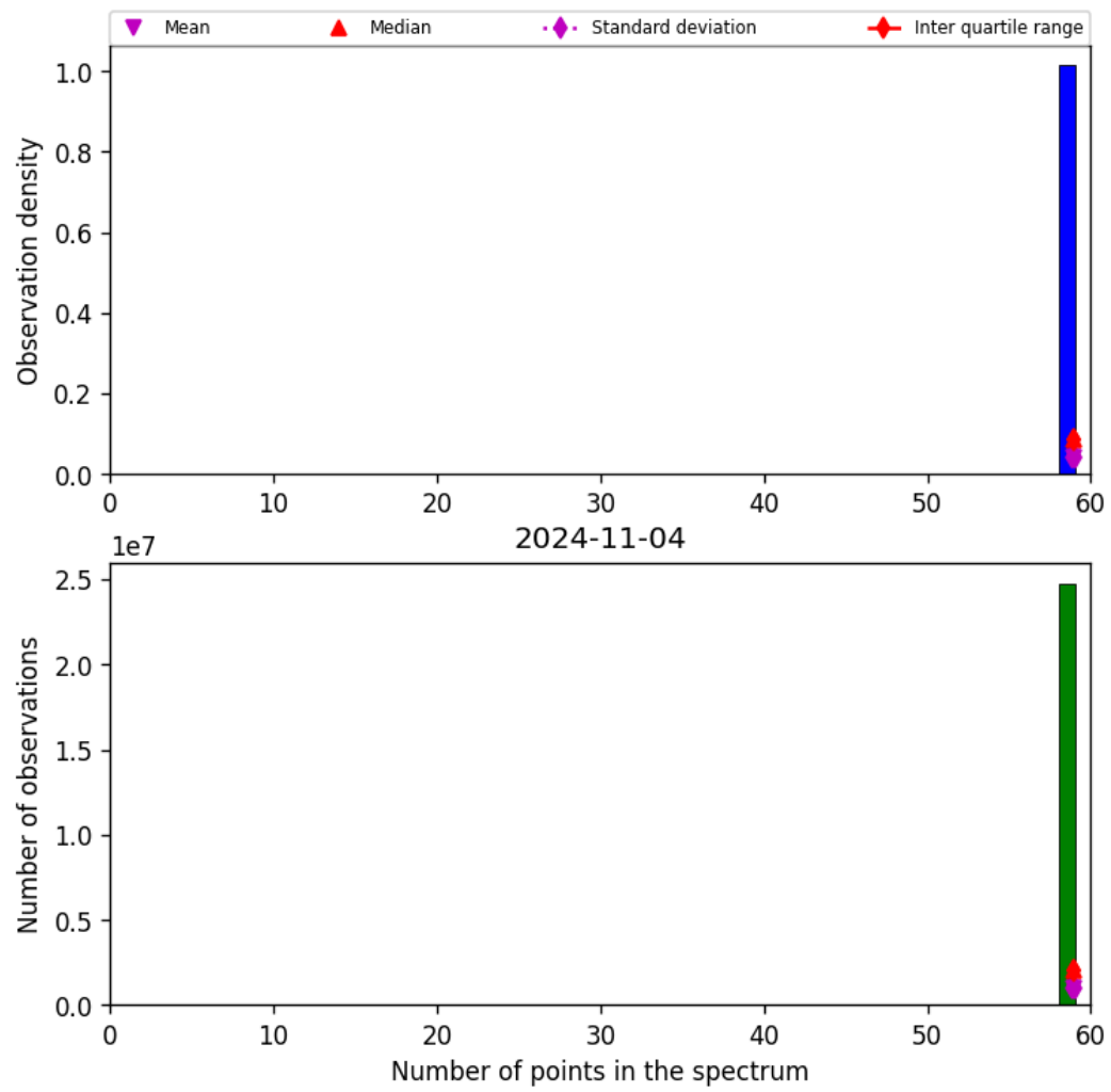
Figure 44: Histogram of “Number of points in the spectrum” for 2024-11-04 to 2024-11-05
