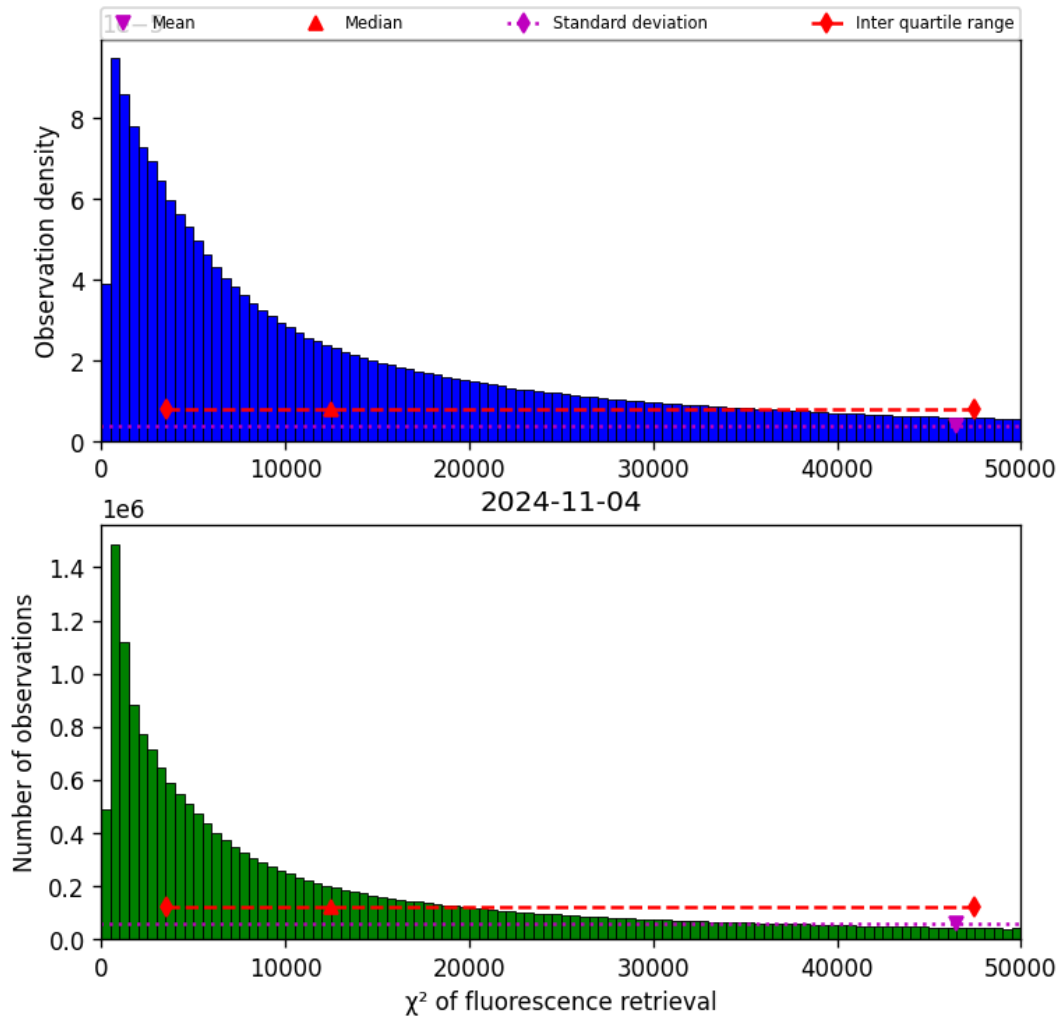
Figure 42: Histogram of “ \chi^2 of fluorescence retrieval” for 2024-11-04 to 2024-11-05
