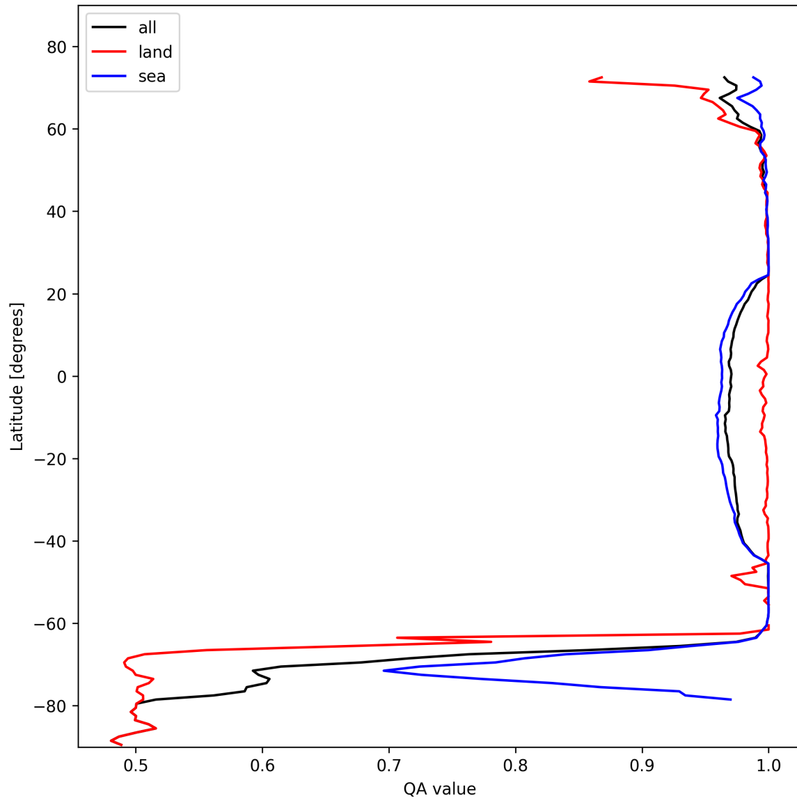
Figure 12: Zonal average of “QA value” for 2024-11-04 to 2024-11-05.
