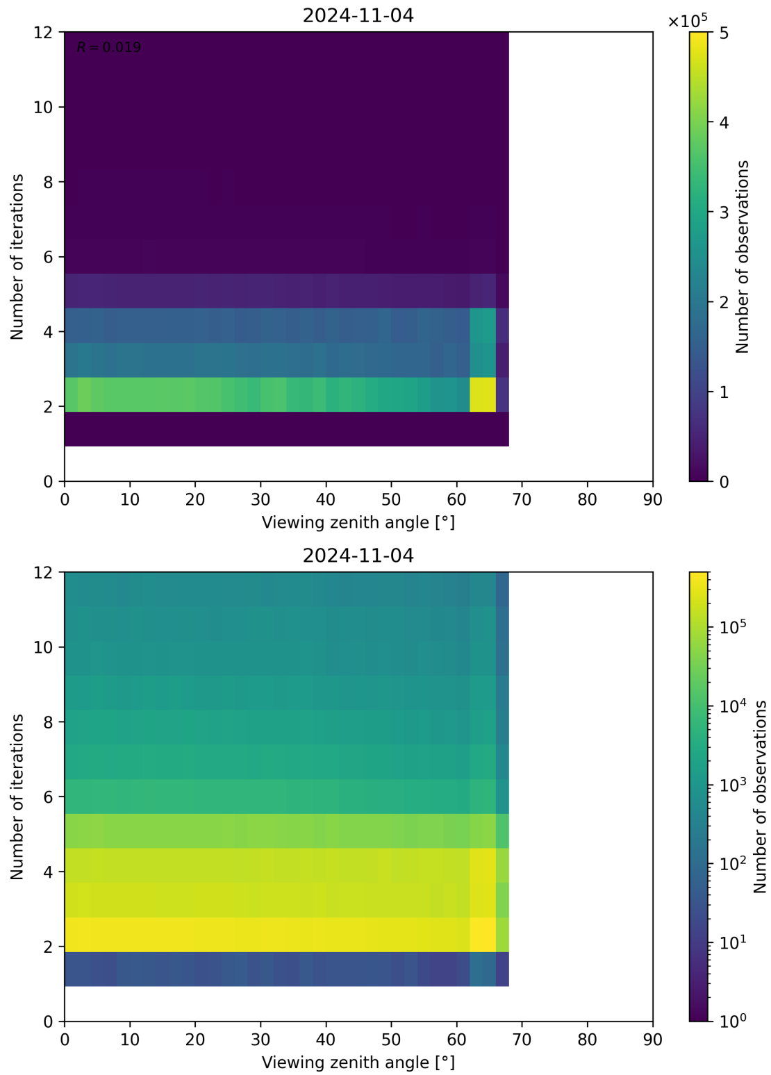
Figure 136: Scatter density plot of “Viewing zenith angle” against “Number of iterations” for 2024-11-04 to 2024-11-05.
