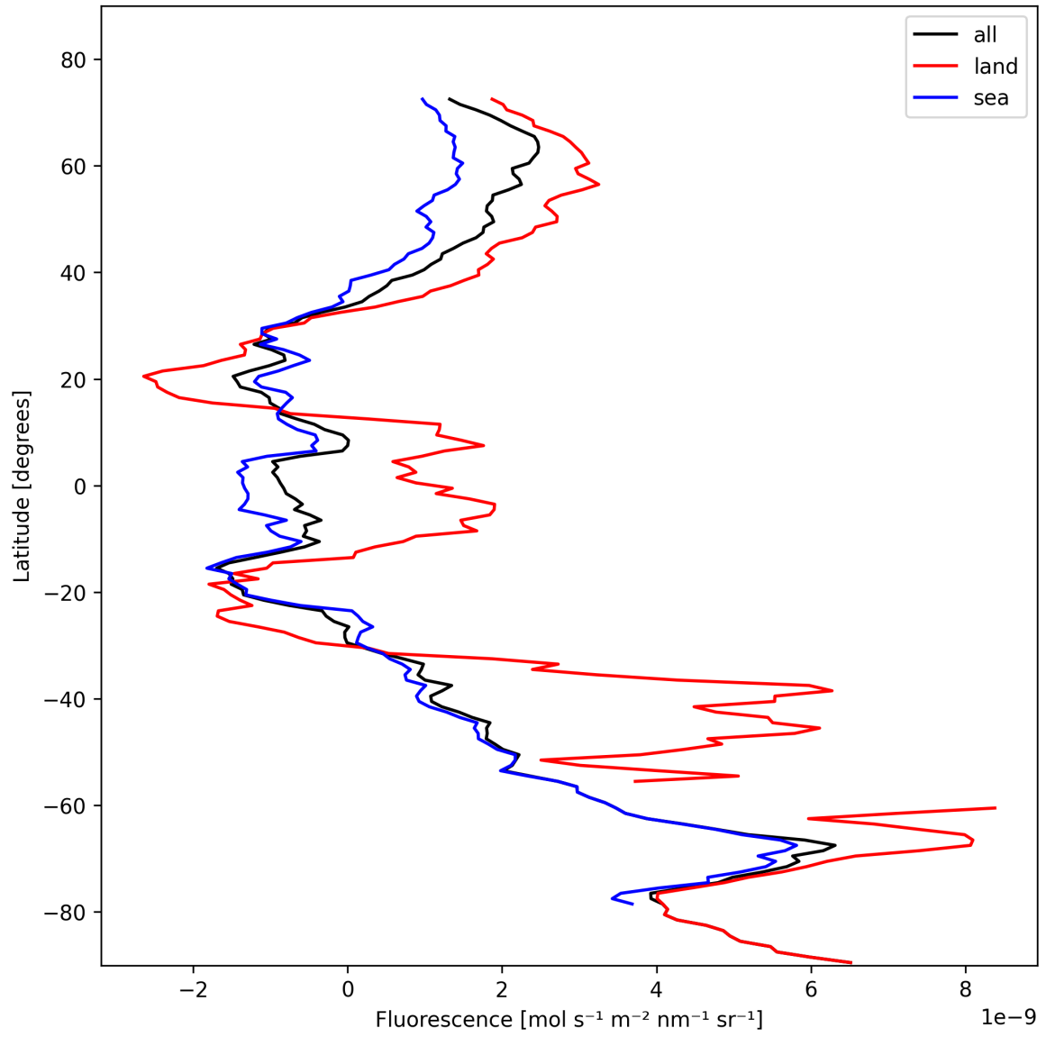
Figure 23: Zonal average of “Fluorescence” for 2024-11-04 to 2024-11-05.
