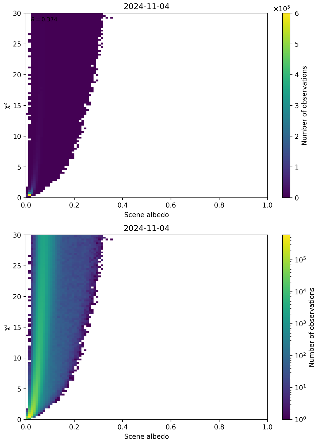
Figure 112: Scatter density plot of “Scene albedo” against “ \chi^2 ” for 2024-11-04 to 2024-11-05.
