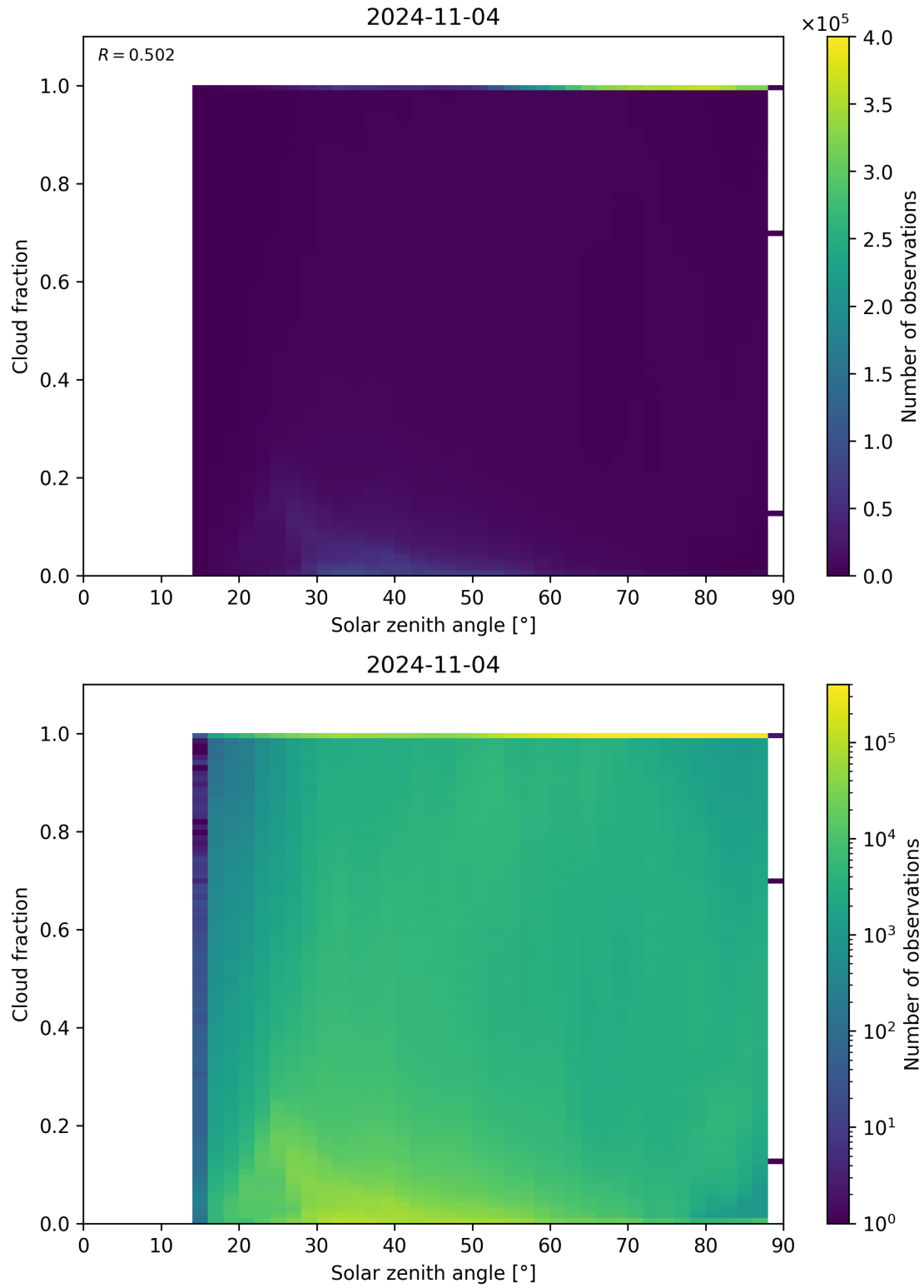
Figure 121: Scatter density plot of “Solar zenith angle” against “Cloud fraction” for 2024-11-04 to 2024-11-05.
