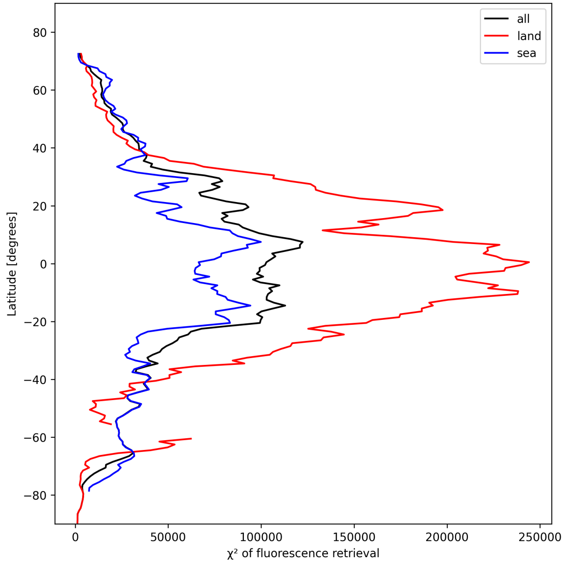
Figure 25: Zonal average of “ \chi^2 of fluorescence retrieval” for 2024-11-04 to 2024-11-05.
