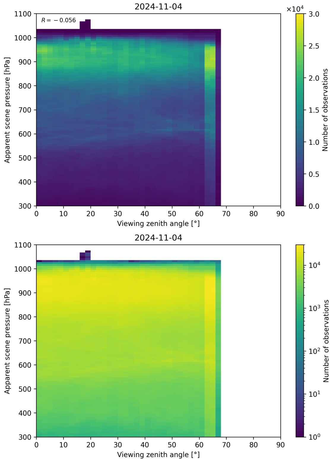
Figure 129: Scatter density plot of “Viewing zenith angle” against “Apparent scene pressure” for 2024-11-04 to 2024-11-05.
