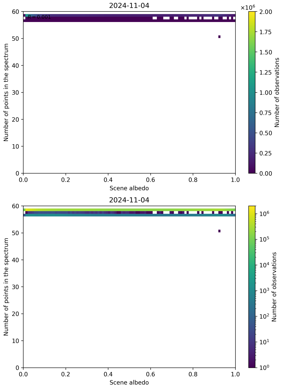
Figure 116: Scatter density plot of “Scene albedo” against “Number of points in the spectrum” for 2024-11-04 to 2024-11-05.
