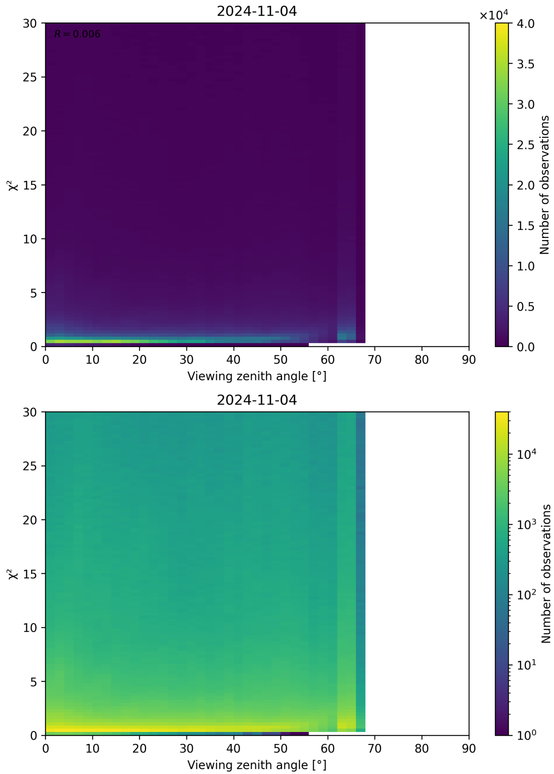
Figure 130: Scatter density plot of “Viewing zenith angle” against “ \chi^2 ” for 2024-11-04 to 2024-11-05.
