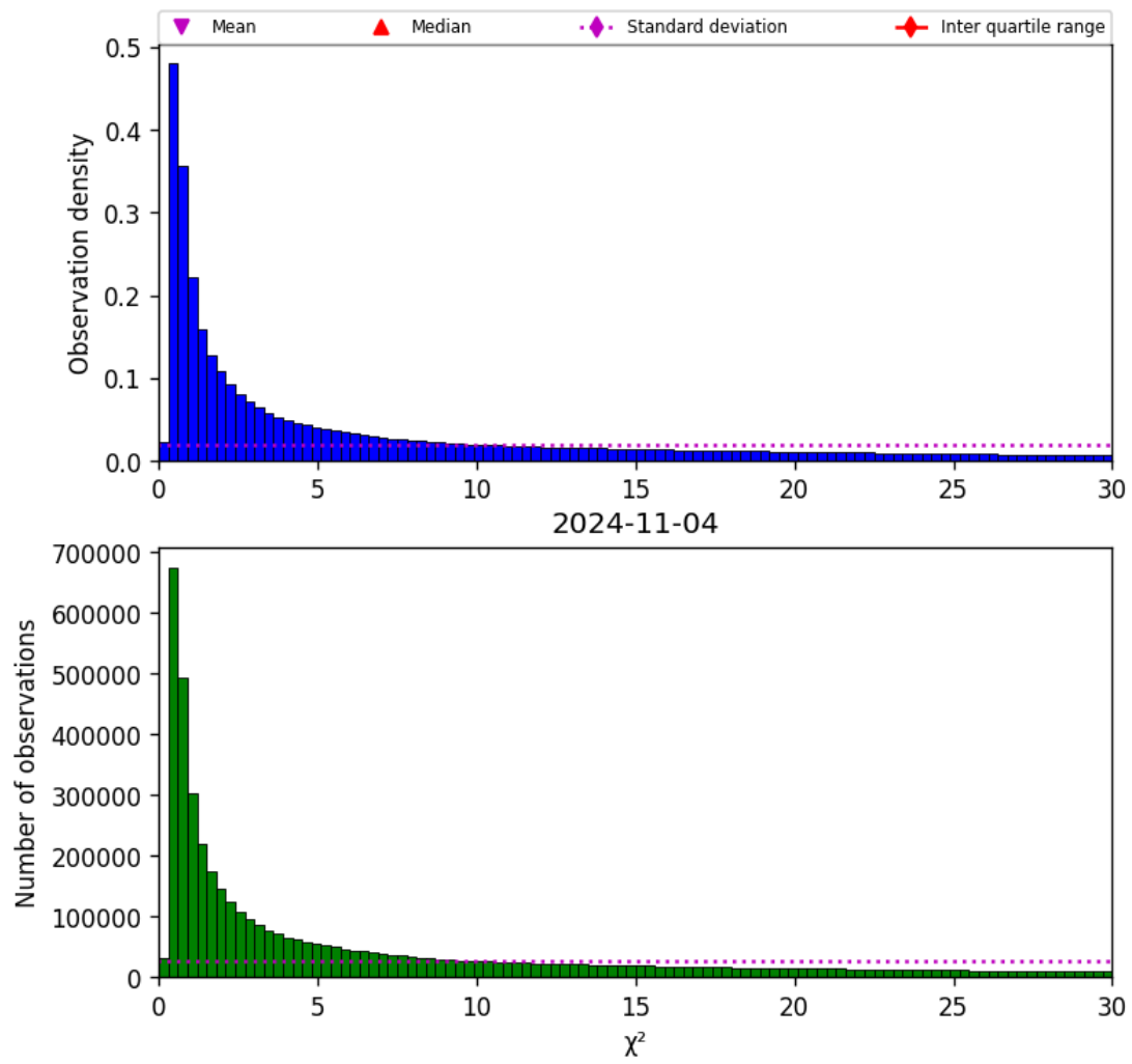
Figure 38: Histogram of “ \chi^2 ” for 2024-11-04 to 2024-11-05
