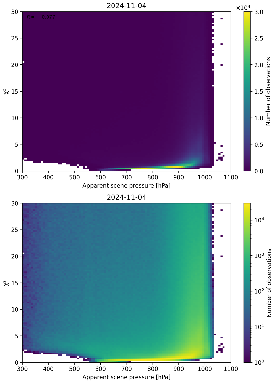
Figure 63: Scatter density plot of “Apparent scene pressure” against “ \chi^2 ” for 2024-11-04 to 2024-11-05.
