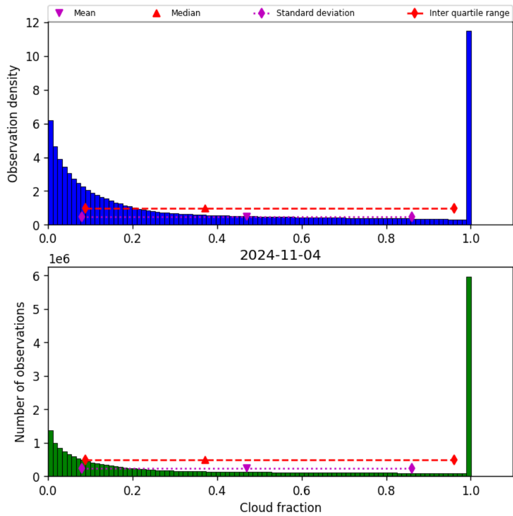
Figure 32: Histogram of “Cloud fraction” for 2024-11-04 to 2024-11-05
