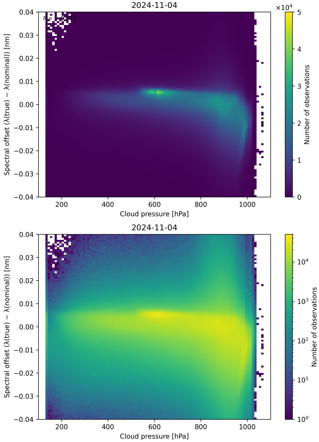
Figure 92: Scatter density plot of “Cloud pressure” against “Spectral offset ( \lambda_{\text{true}} - \lambda_{\text{nominal}} )” for 2024-11-04 to 2024-11-05.
