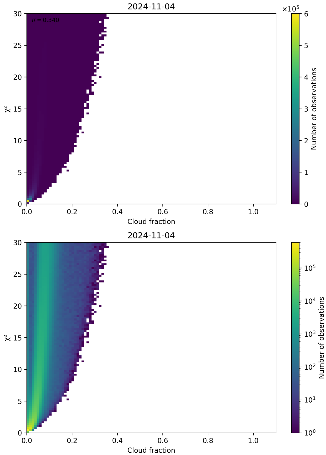
Figure 77: Scatter density plot of “Cloud fraction” against “ \chi^2 ” for 2024-11-04 to 2024-11-05.
