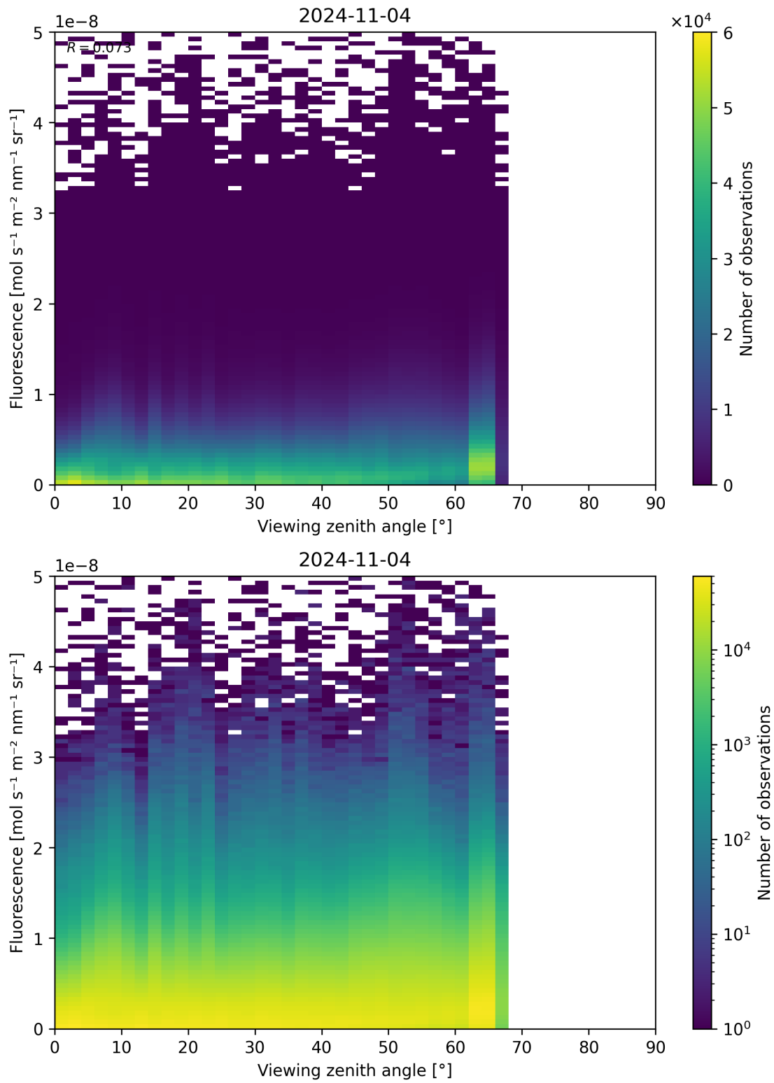
Figure 134: Scatter density plot of “Viewing zenith angle” against “Fluorescence” for 2024-11-04 to 2024-11-05.
