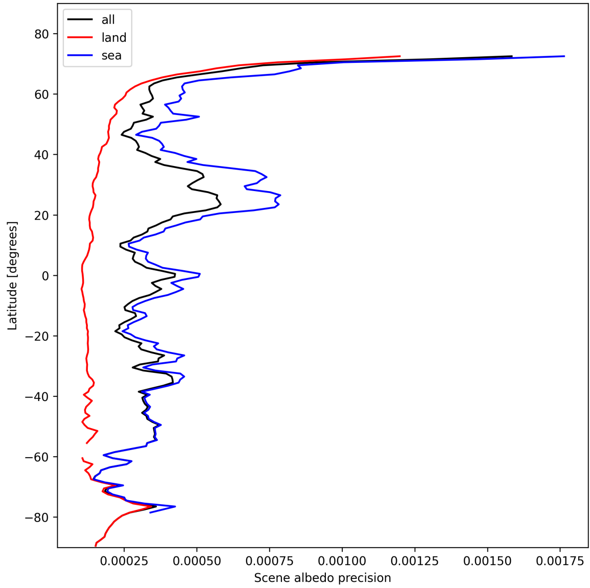
Figure 18: Zonal average of "Scene albedo precision" for 2024-11-04 to 2024-11-05.
