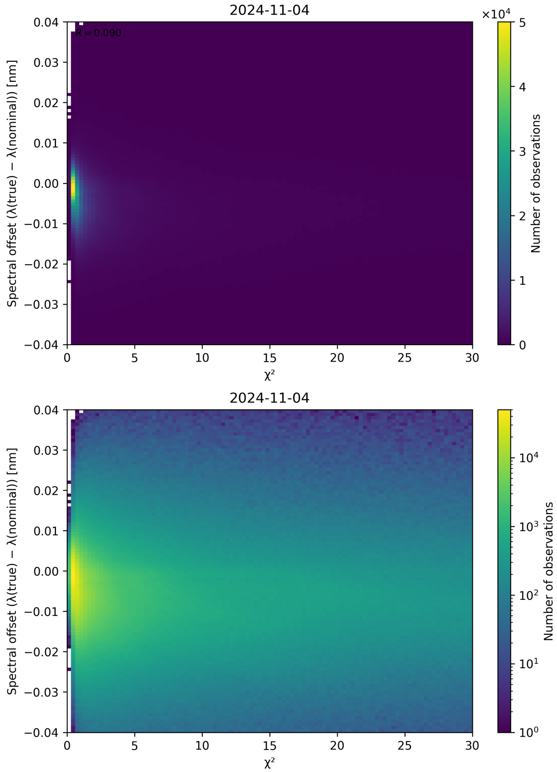
Figure 75: Scatter density plot of “ \chi^2 ” against “Spectral offset ( \lambda_{\text{true}} - \lambda_{\text{nominal}} )” for 2024-11-04 to 2024-11-05.
