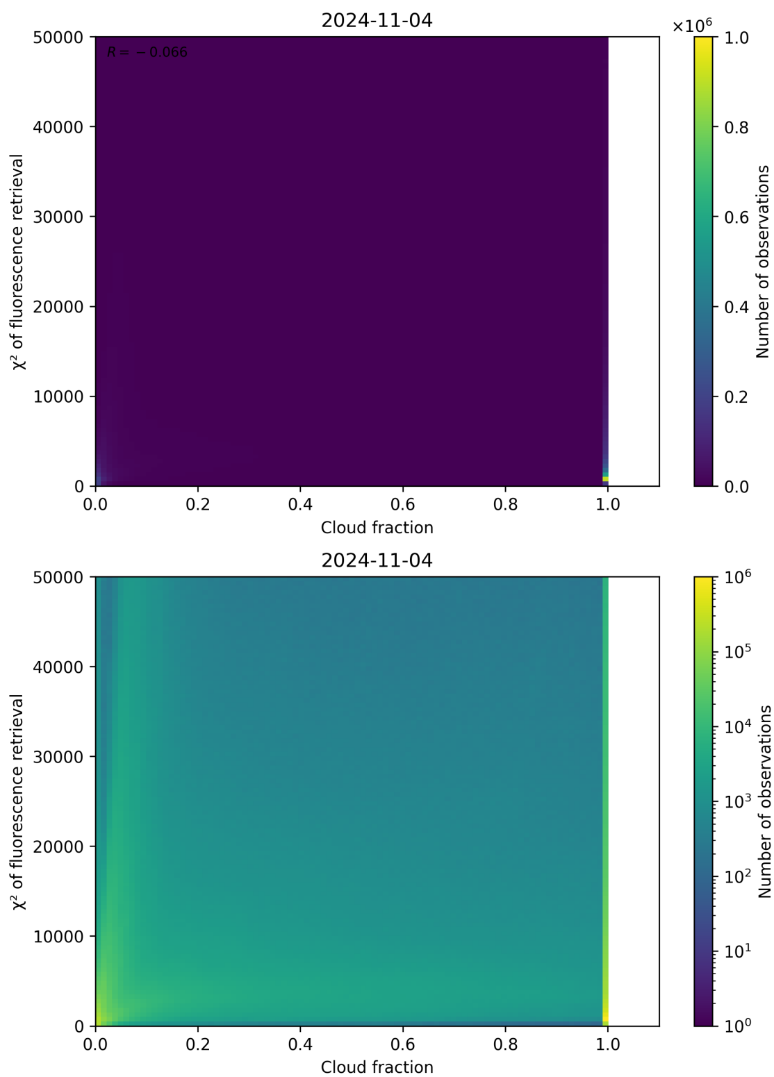
Figure 78: Scatter density plot of “Cloud fraction” against “ \chi^2 of fluorescence retrieval” for 2024-11-04 to 2024-11-05.
