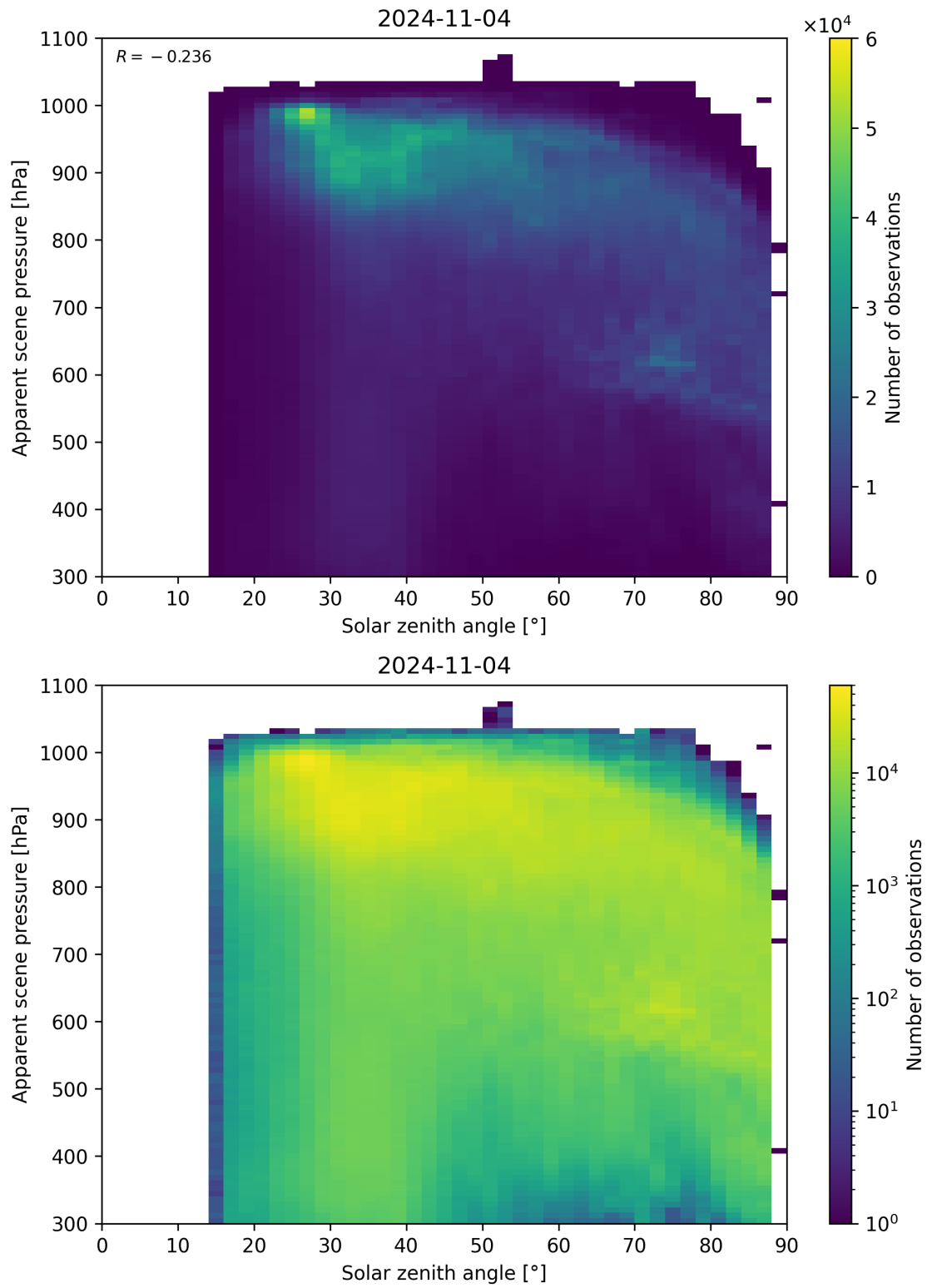
Figure 118: Scatter density plot of “Solar zenith angle” against “Apparent scene pressure” for 2024-11-04 to 2024-11-05.
