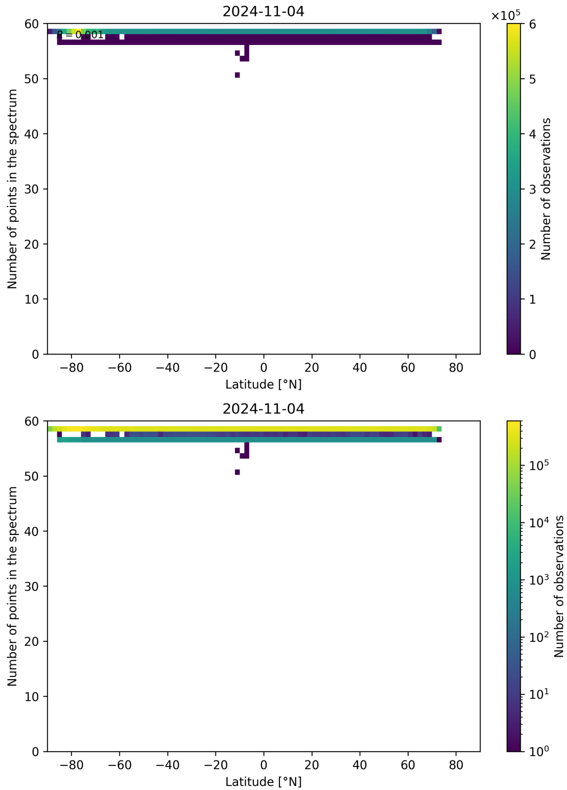
Figure 103: Scatter density plot of “Latitude” against “Number of points in the spectrum” for 2024-11-04 to 2024-11-05.
