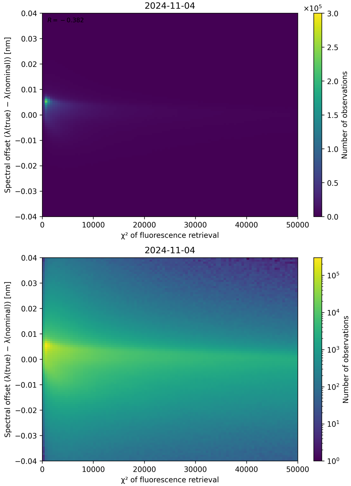
Figure 72: Scatter density plot of “ \chi^2 of fluorescence retrieval” against “Spectral offset ( \lambda_{\text{true}} - \lambda_{\text{nominal}} )” for 2024-11-04 to 2024-11-05.
