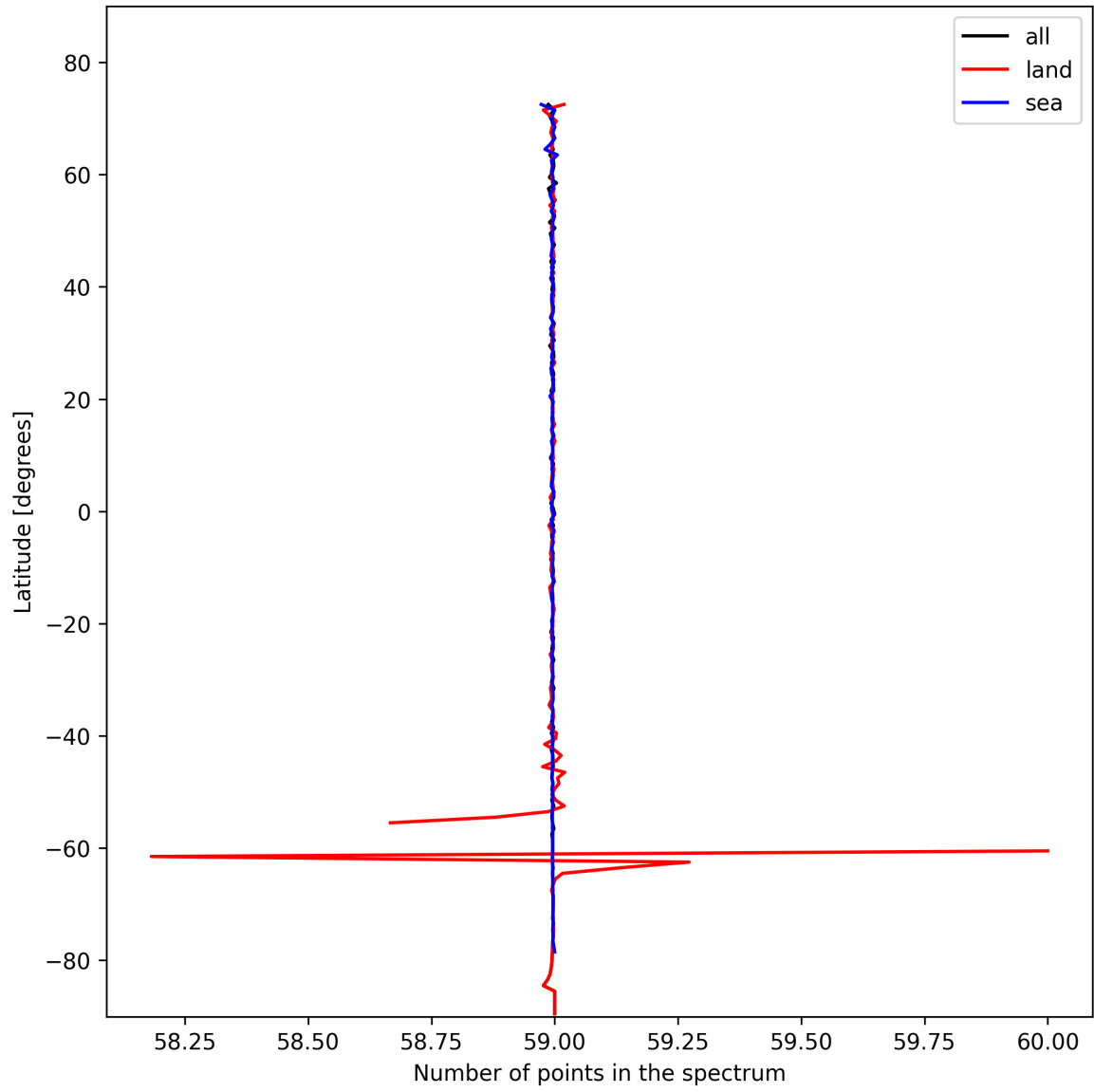
Figure 27: Zonal average of “Number of points in the spectrum” for 2024-11-04 to 2024-11-05.
