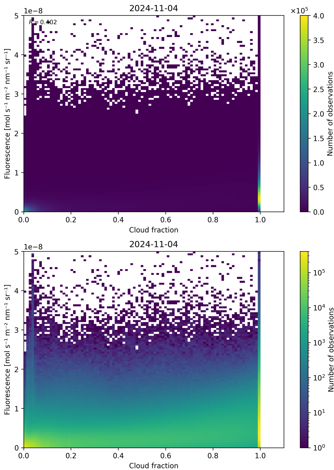
Figure 79: Scatter density plot of “Cloud fraction” against “Fluorescence” for 2024-11-04 to 2024-11-05.
