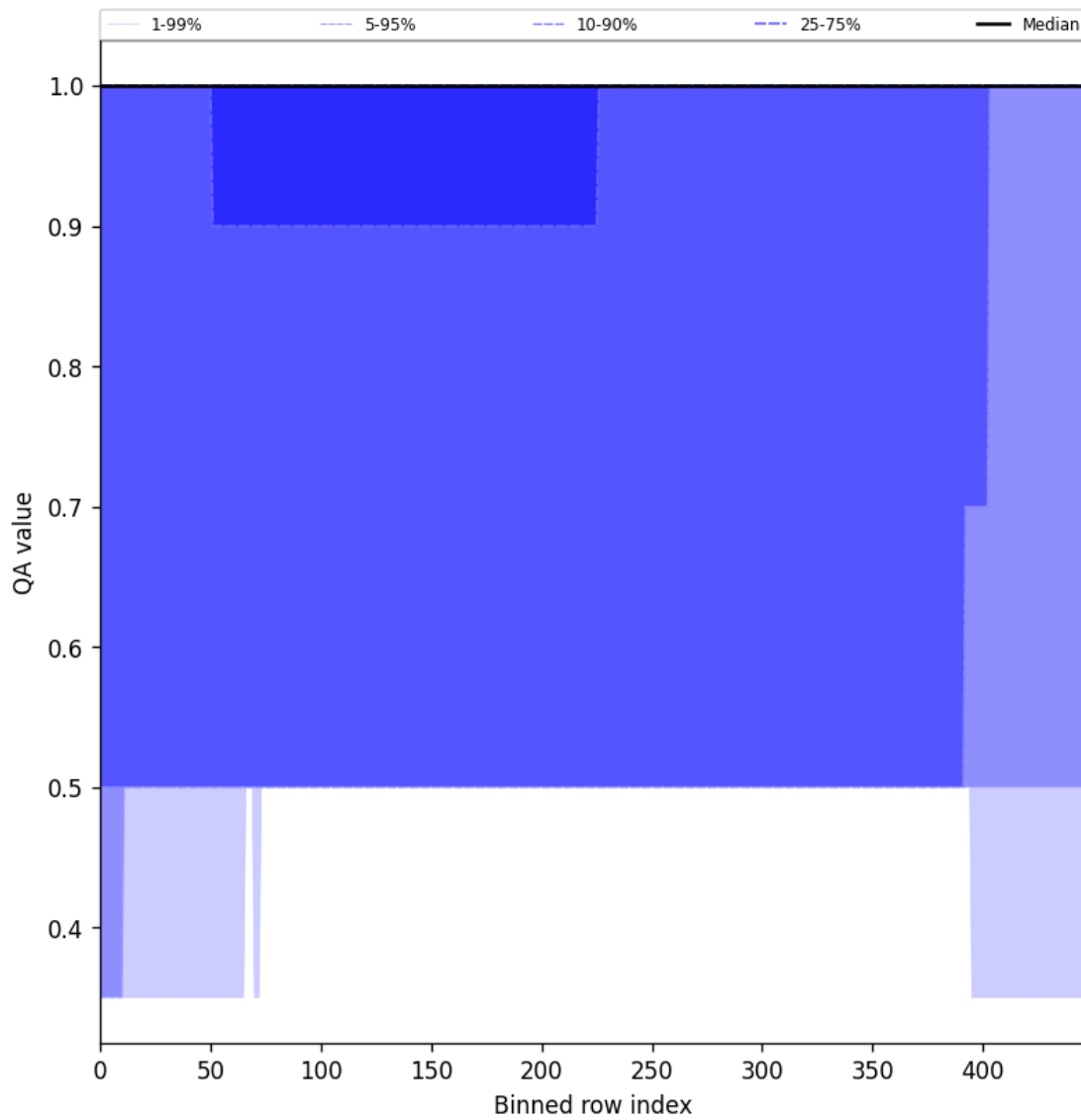
Figure 46: Along track statistics of “QA value” for 2024-11-04 to 2024-11-05
