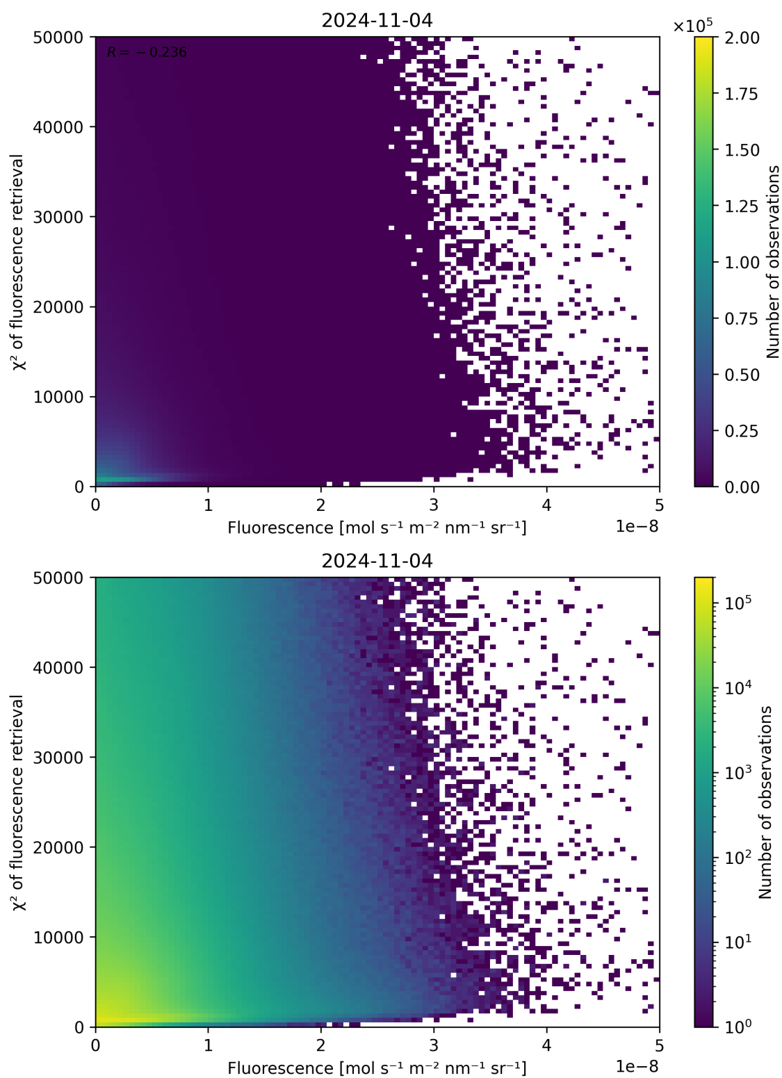
Figure 93: Scatter density plot of “Fluorescence” against “ \chi^2 of fluorescence retrieval” for 2024-11-04 to 2024-11-05.
