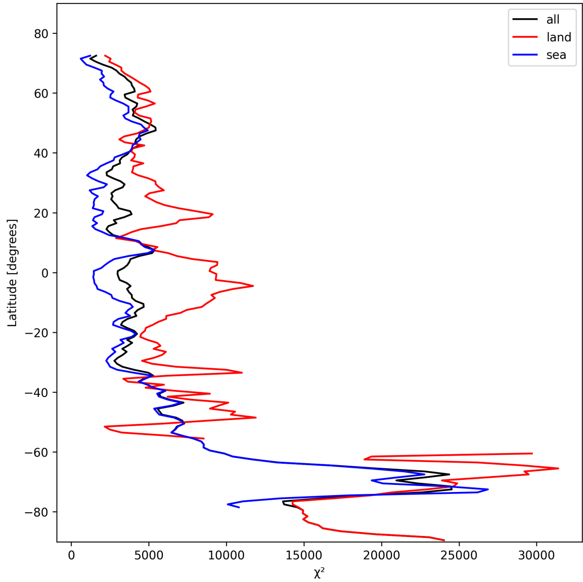
Figure 21: Zonal average of “ \chi^2 ” for 2024-11-04 to 2024-11-05.
