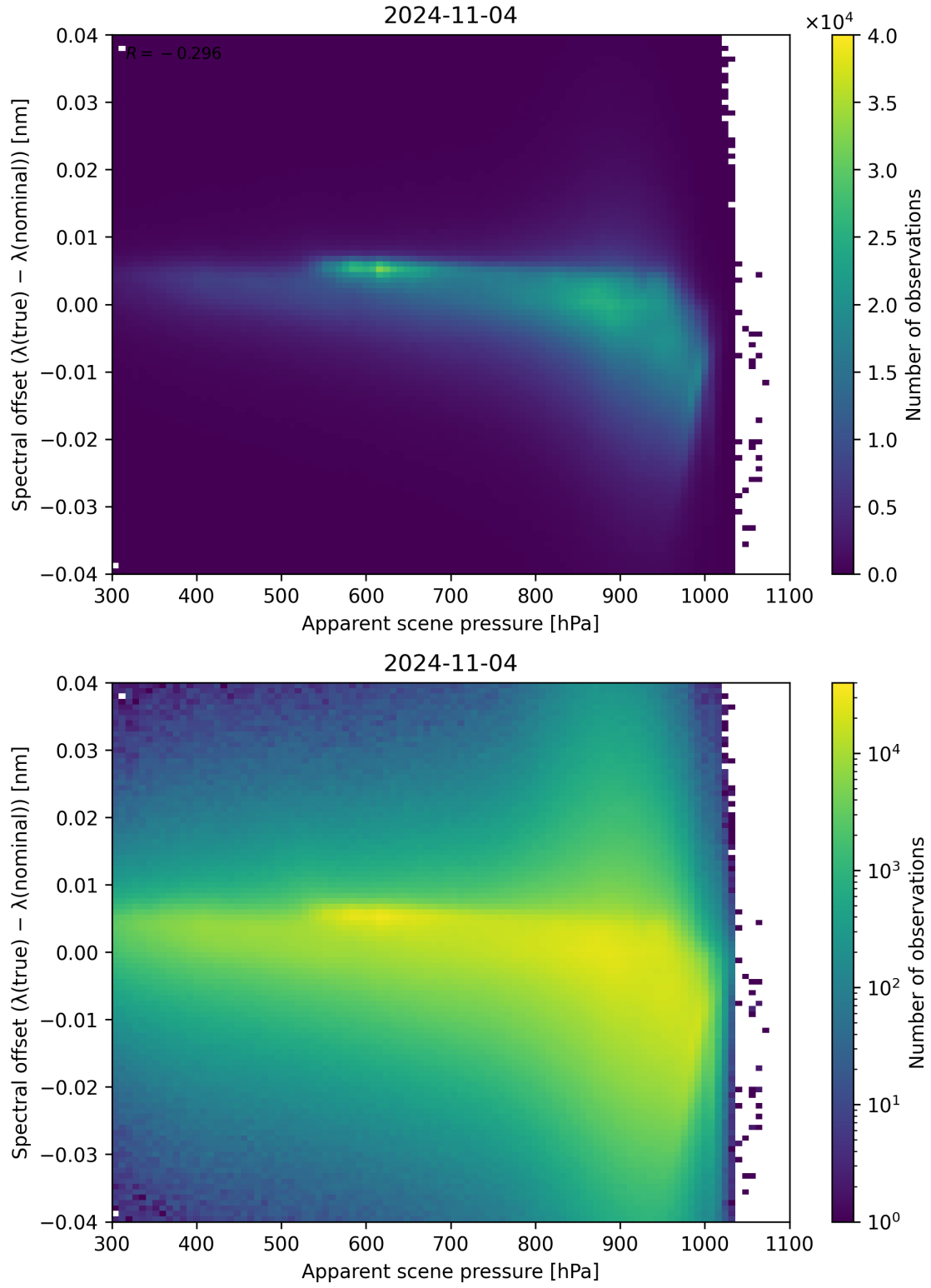
Figure 68: Scatter density plot of “Apparent scene pressure” against “Spectral offset ( \lambda_{\text{true}} - \lambda_{\text{nominal}} )” for 2024-11-04 to 2024-11-05.
