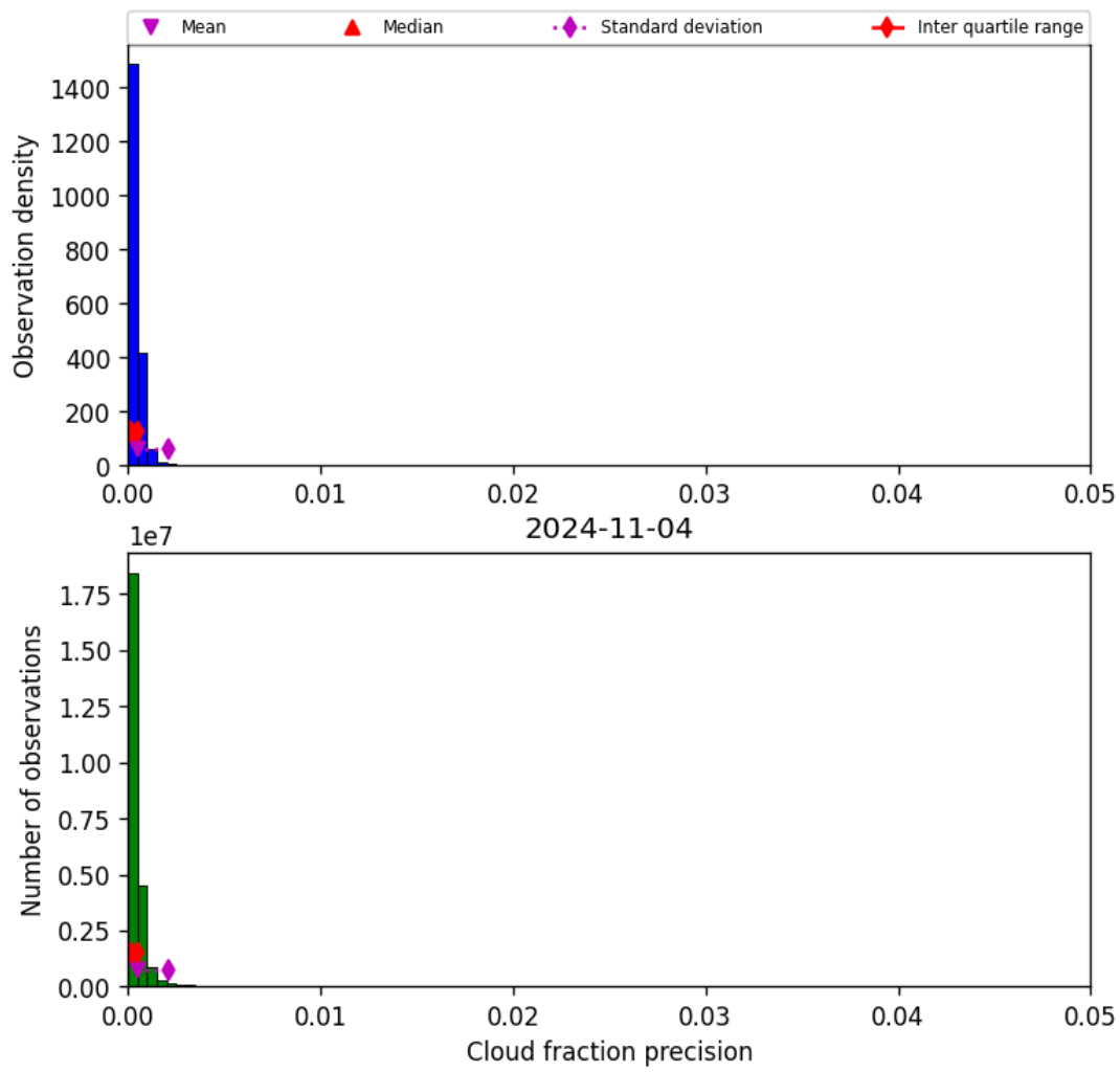
Figure 33: Histogram of “Cloud fraction precision” for 2024-11-04 to 2024-11-05
