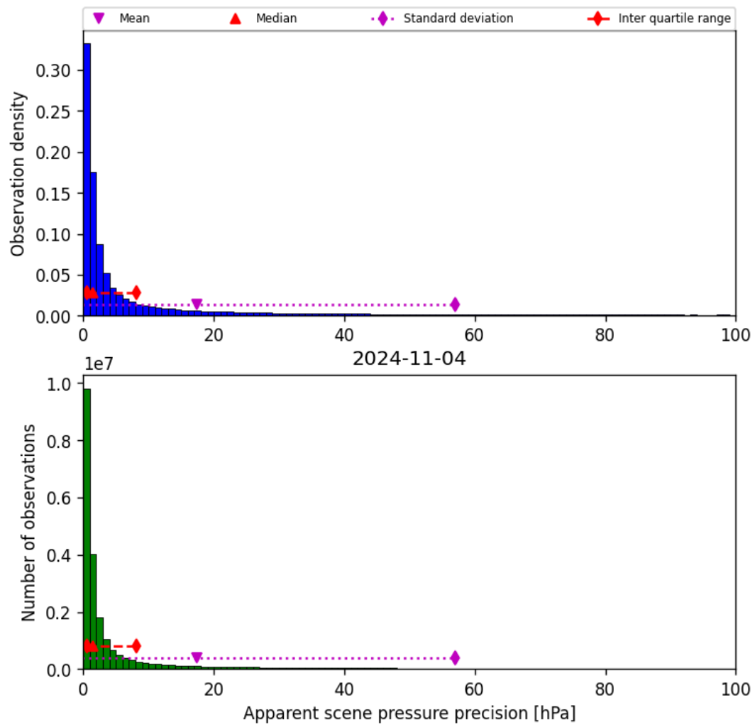
Figure 37: Histogram of “Apparent scene pressure precision” for 2024-11-04 to 2024-11-05
