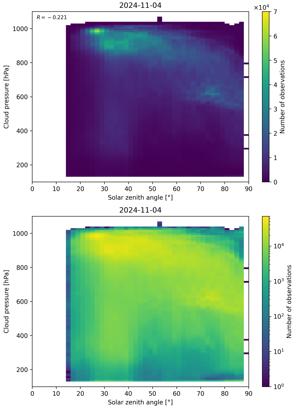
Figure 122: Scatter density plot of “Solar zenith angle” against “Cloud pressure” for 2024-11-04 to 2024-11-05.
