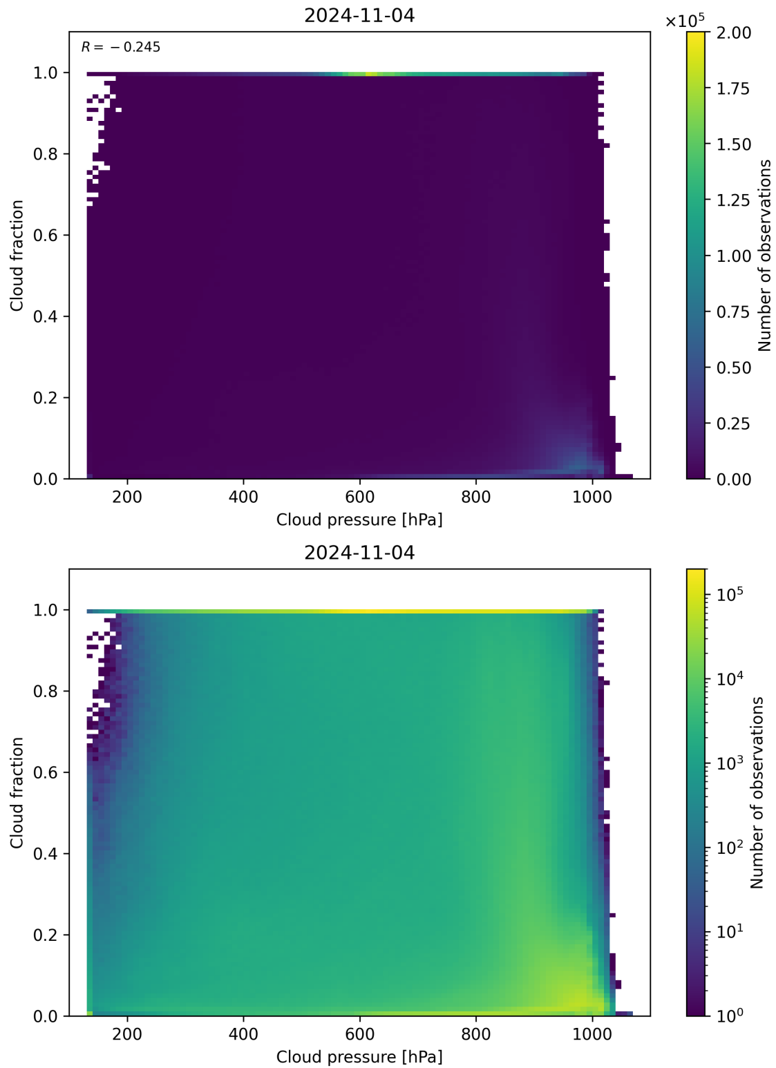
Figure 87: Scatter density plot of “Cloud pressure” against “Cloud fraction” for 2024-11-04 to 2024-11-05.
