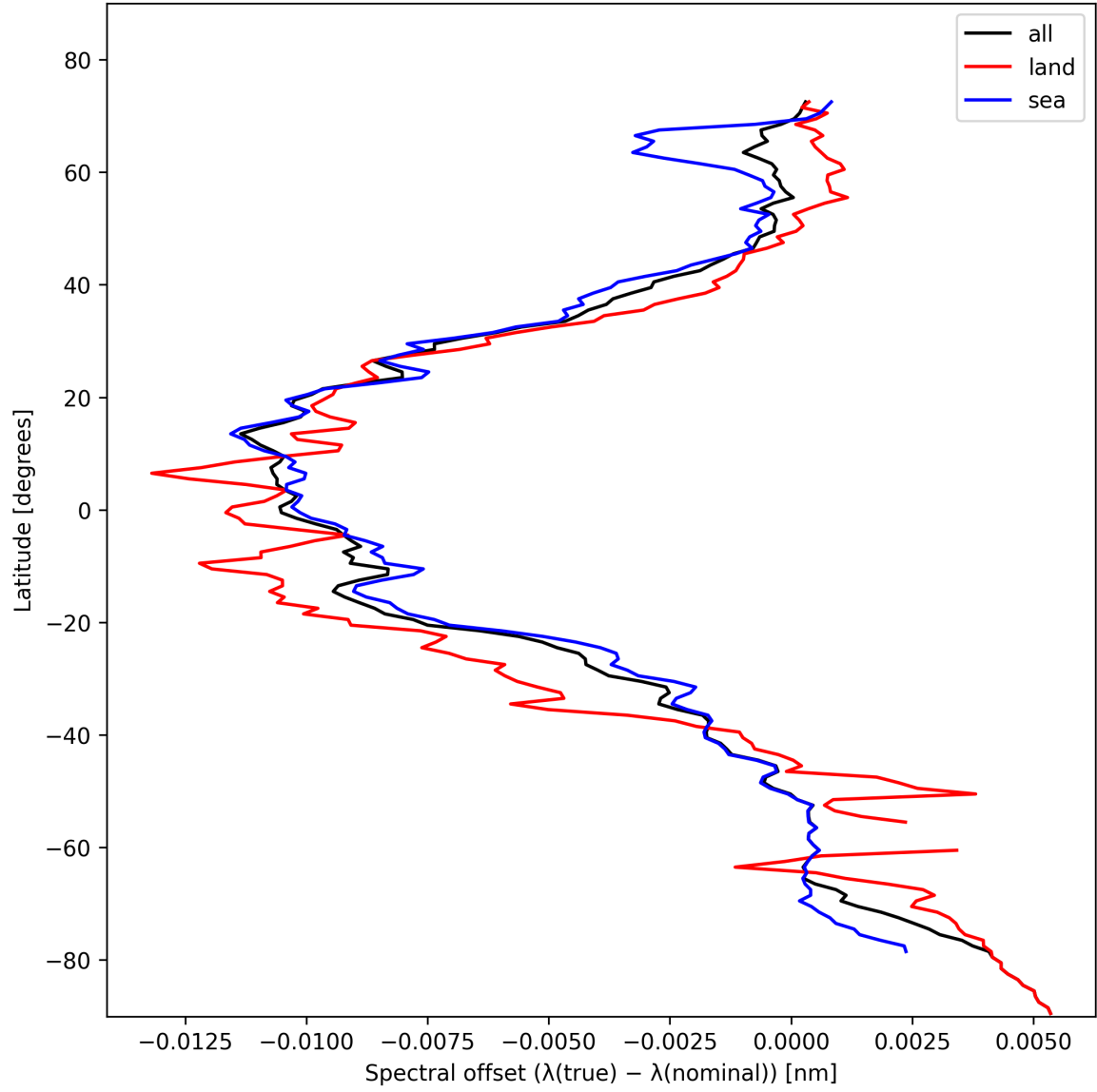
Figure 28: Zonal average of “Spectral offset ( \lambda_{\text{true}} - \lambda_{\text{nominal}} )” for 2024-11-04 to 2024-11-05.
