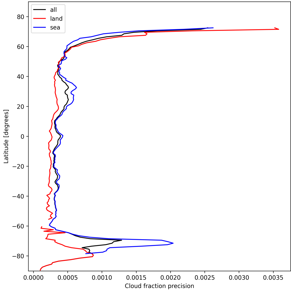
Figure 16: Zonal average of “Cloud fraction precision” for 2024-11-04 to 2024-11-05.
