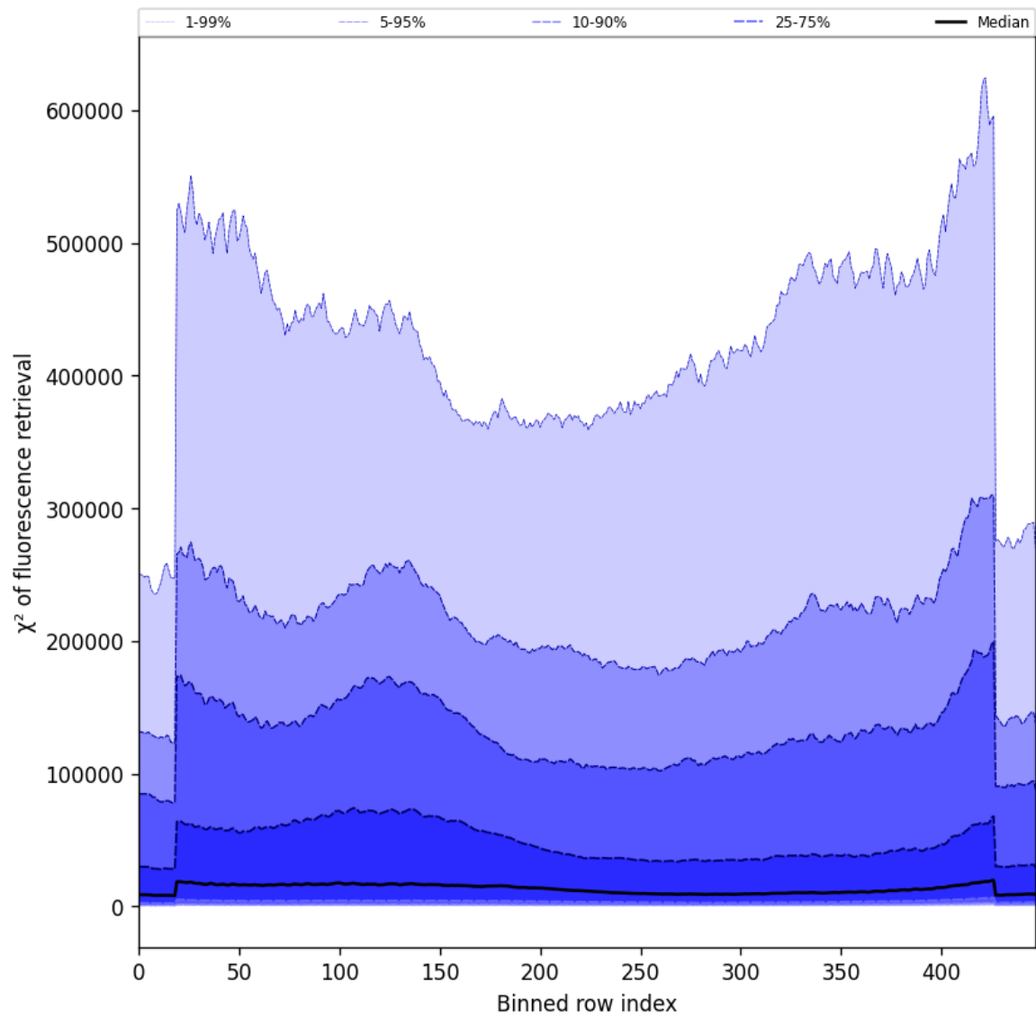
Figure 59: Along track statistics of “ \chi^2 of fluorescence retrieval” for 2024-11-04 to 2024-11-05
