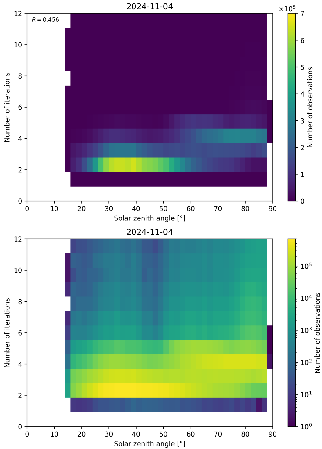
Figure 125: Scatter density plot of “Solar zenith angle” against “Number of iterations” for 2024-11-04 to 2024-11-05.
