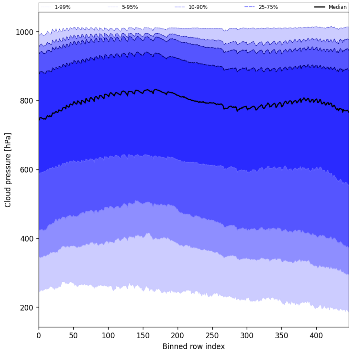
Figure 47: Along track statistics of “Cloud pressure” for 2024-11-04 to 2024-11-05
