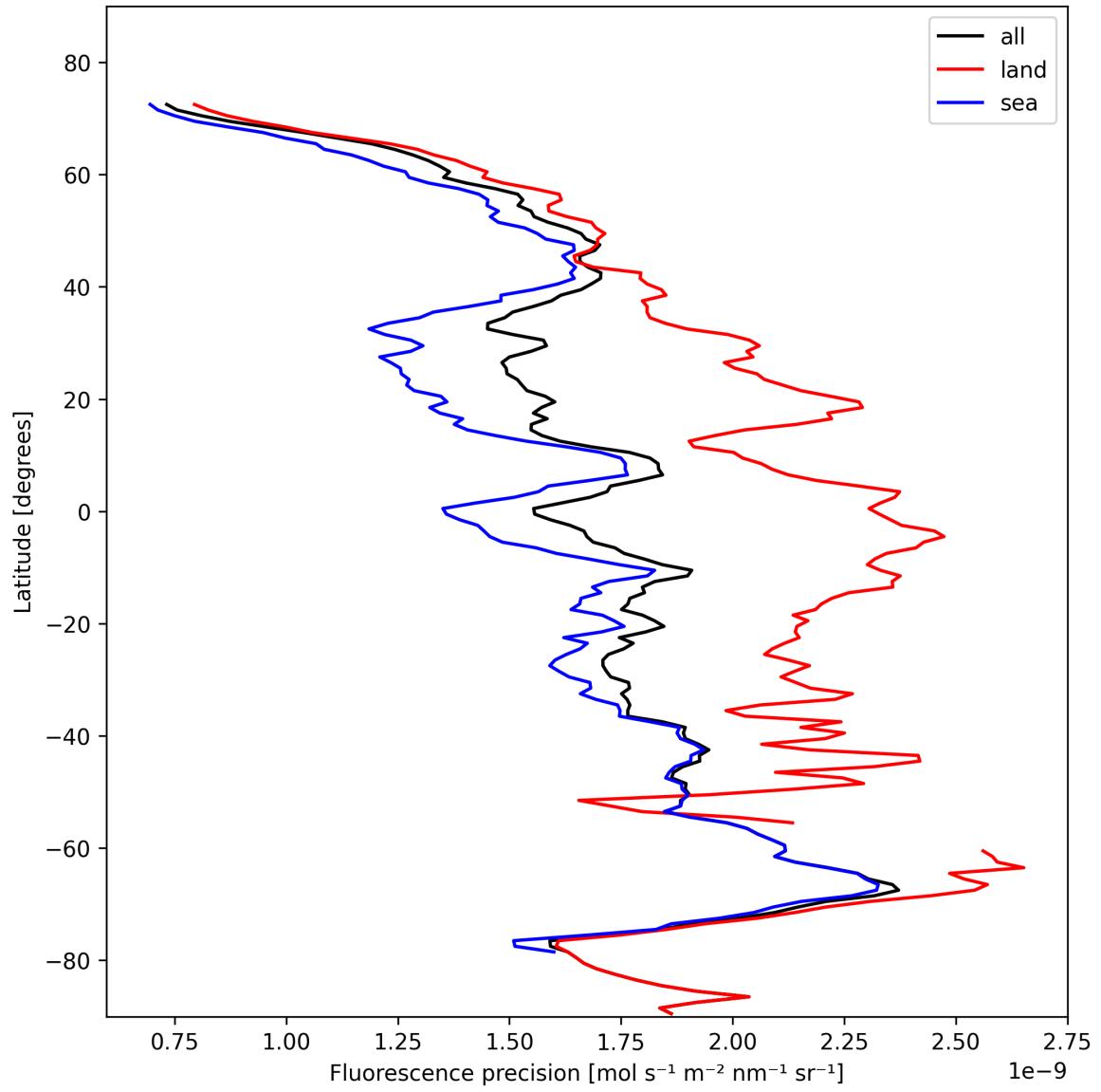
Figure 24: Zonal average of “Fluorescence precision” for 2024-11-04 to 2024-11-05.
