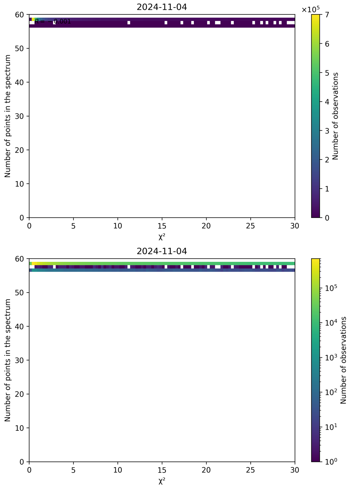
Figure 74: Scatter density plot of “ \chi^2 ” against “Number of points in the spectrum” for 2024-11-04 to 2024-11-05.
