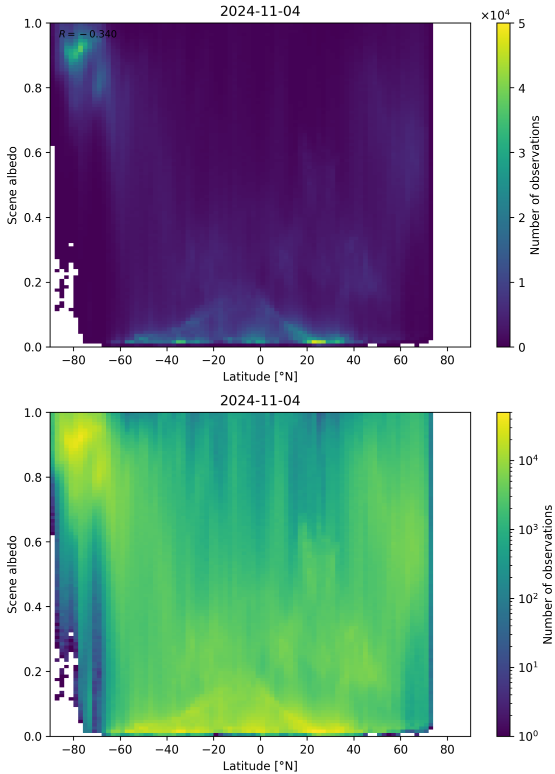
Figure 104: Scatter density plot of “Latitude” against “Scene albedo” for 2024-11-04 to 2024-11-05.
