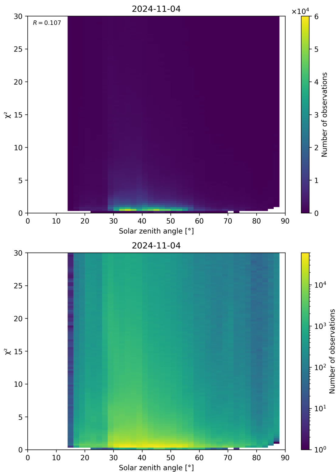
Figure 119: Scatter density plot of “Solar zenith angle” against “ \chi^2 ” for 2024-11-04 to 2024-11-05.
