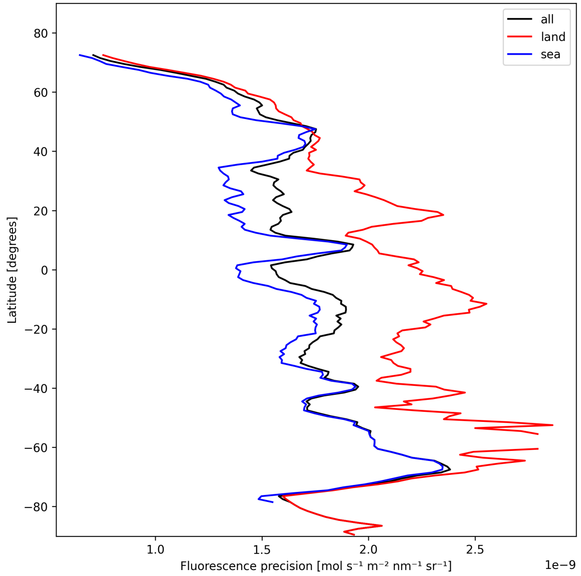
Figure 24: Zonal average of “Fluorescence precision” for 2024-11-04 to 2024-11-06.
