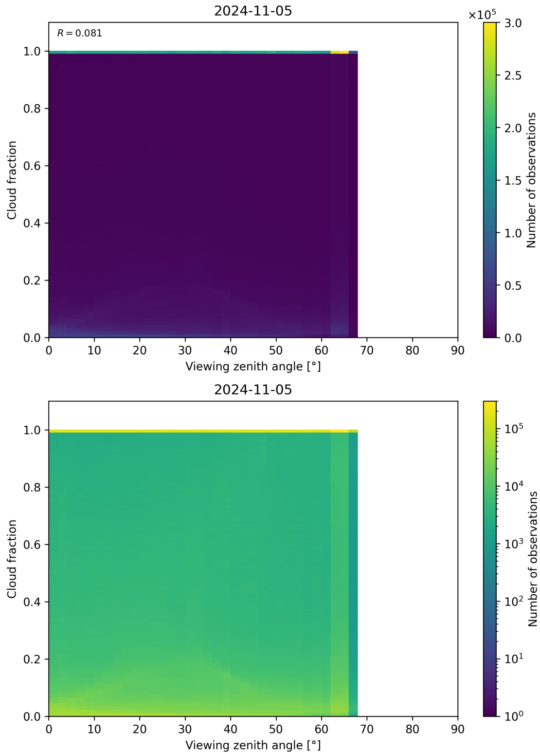
Figure 132: Scatter density plot of “Viewing zenith angle” against “Cloud fraction” for 2024-11-04 to 2024-11-06.
