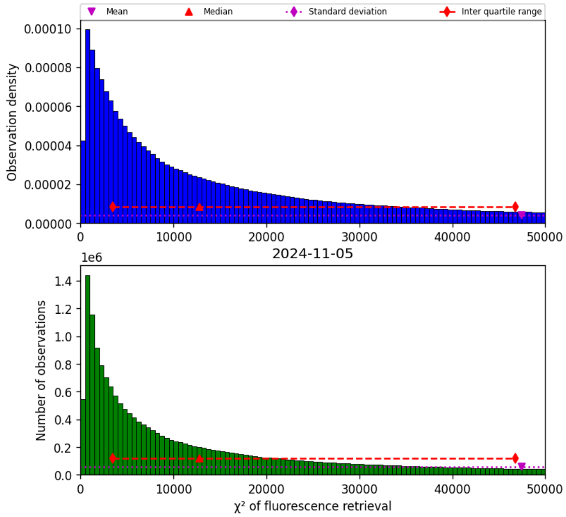
Figure 42: Histogram of “ \chi^2 of fluorescence retrieval” for 2024-11-04 to 2024-11-06
