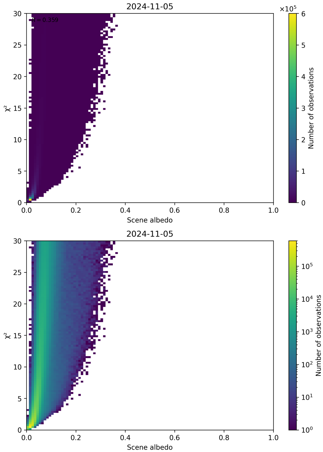
Figure 112: Scatter density plot of “Scene albedo” against “ \chi^2 ” for 2024-11-04 to 2024-11-06.
