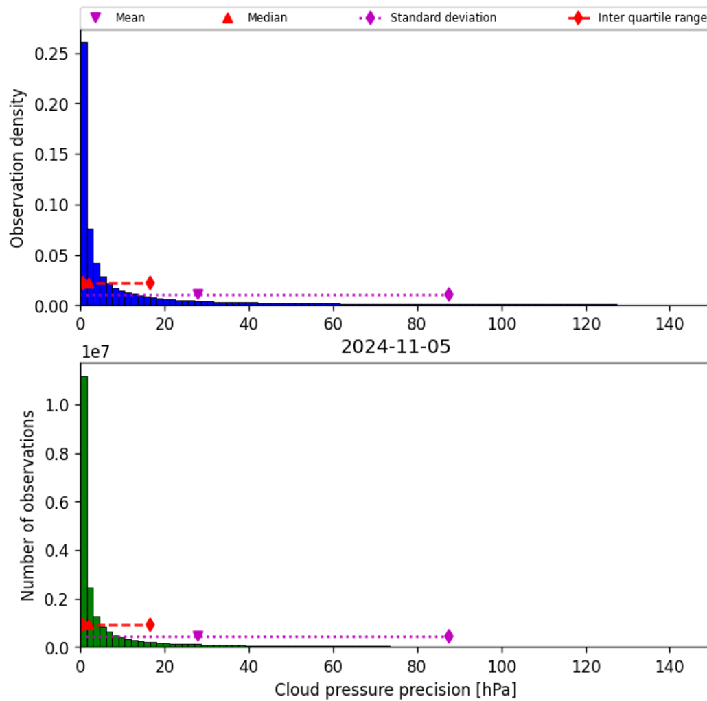
Figure 31: Histogram of “Cloud pressure precision” for 2024-11-04 to 2024-11-06
