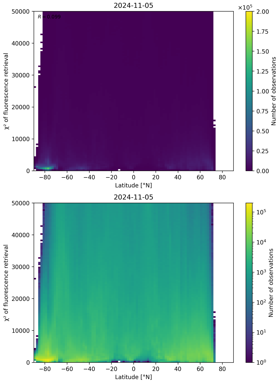
Figure 98: Scatter density plot of “Latitude” against “ \chi^2 of fluorescence retrieval” for 2024-11-04 to 2024-11-06.
