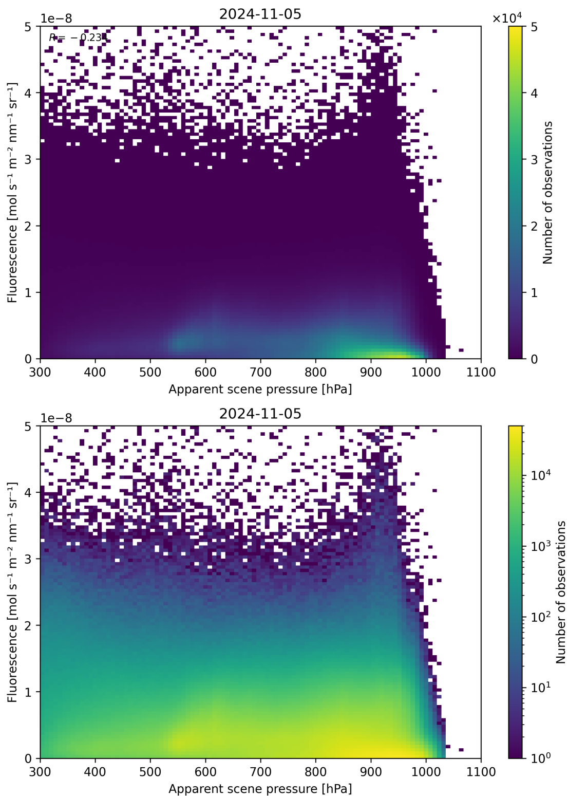
Figure 65: Scatter density plot of “Apparent scene pressure” against “Fluorescence” for 2024-11-04 to 2024-11-06.
