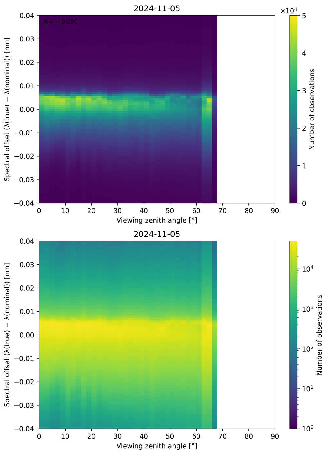
Figure 140: Scatter density plot of “Viewing zenith angle” against “Spectral offset ( \lambda_{\text{true}} - \lambda_{\text{nominal}} )” for 2024-11-04 to 2024-11-06.
