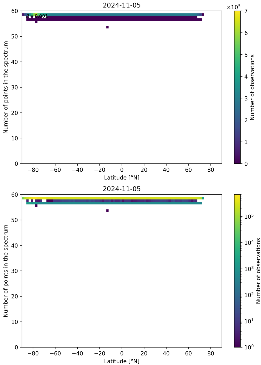
Figure 103: Scatter density plot of “Latitude” against “Number of points in the spectrum” for 2024-11-04 to 2024-11-06.
