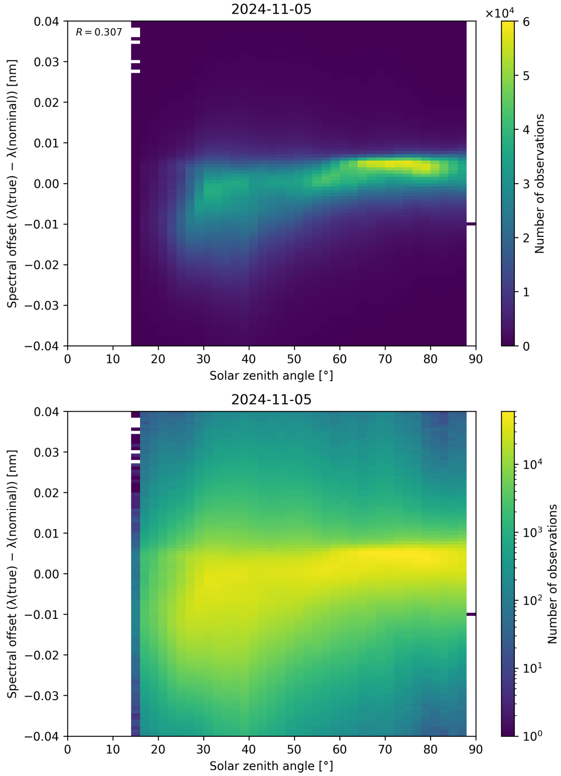
Figure 128: Scatter density plot of “Solar zenith angle” against “Spectral offset ( \lambda_{\text{true}} - \lambda_{\text{nominal}} )” for 2024-11-04 to 2024-11-06.
