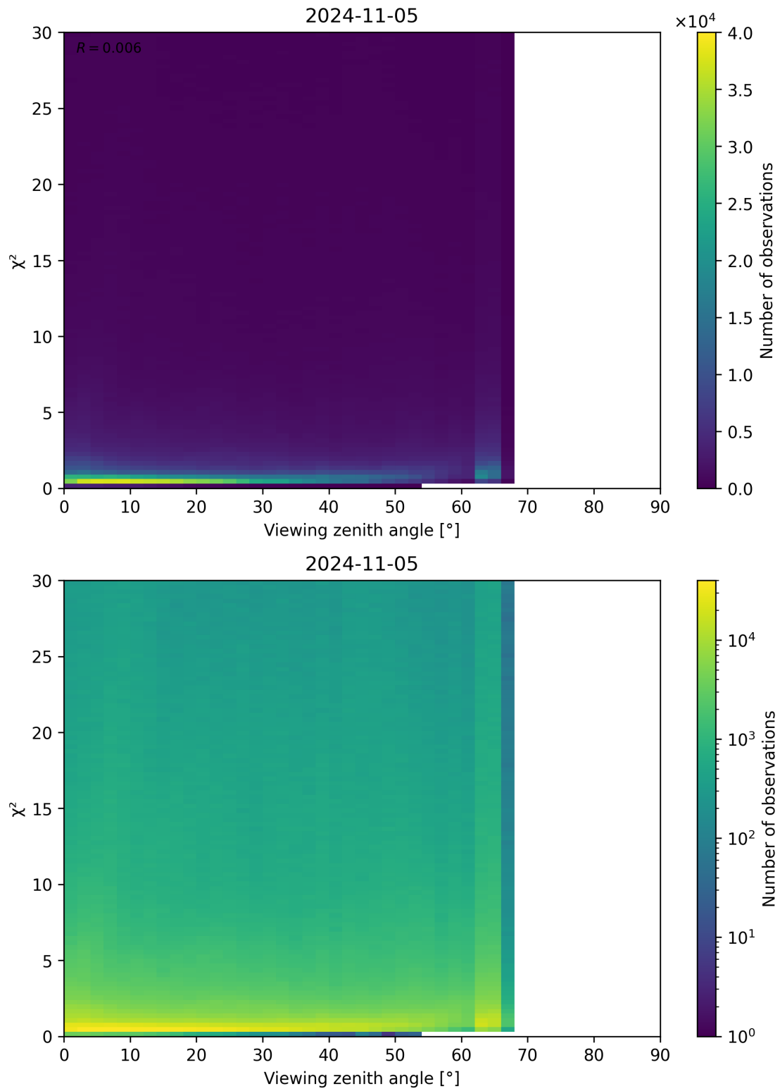
Figure 130: Scatter density plot of “Viewing zenith angle” against “ \chi^2 ” for 2024-11-04 to 2024-11-06.
