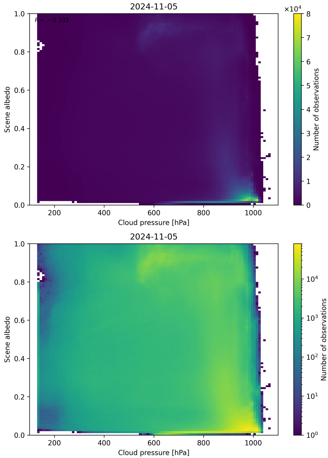
Figure 91: Scatter density plot of “Cloud pressure” against “Scene albedo” for 2024-11-04 to 2024-11-06.
