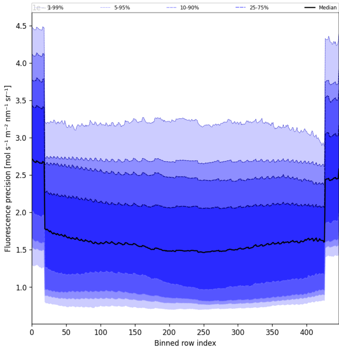
Figure 58: Along track statistics of “Fluorescence precision” for 2024-11-04 to 2024-11-06
