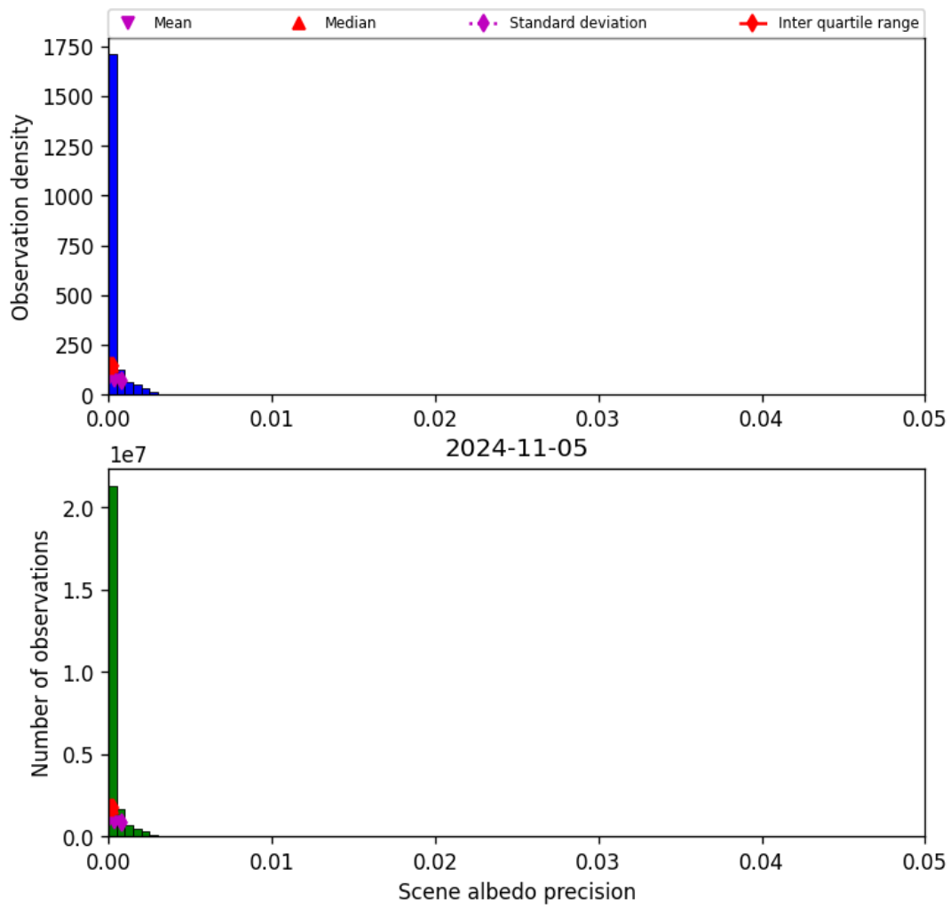
Figure 35: Histogram of “Scene albedo precision” for 2024-11-04 to 2024-11-06
