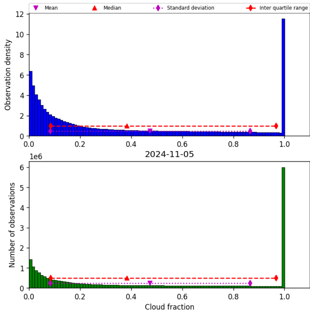
Figure 32: Histogram of “Cloud fraction” for 2024-11-04 to 2024-11-06
