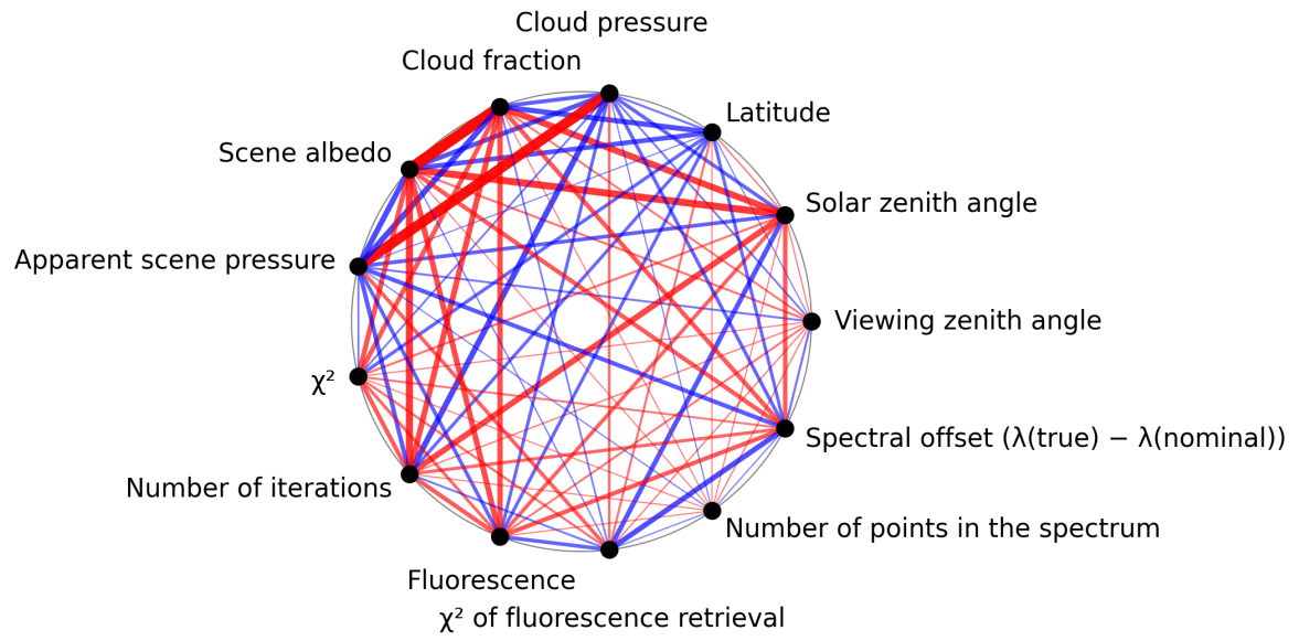
Figure 1: Map of correlation graph for 2024-11-04 to 2024-11-06.
