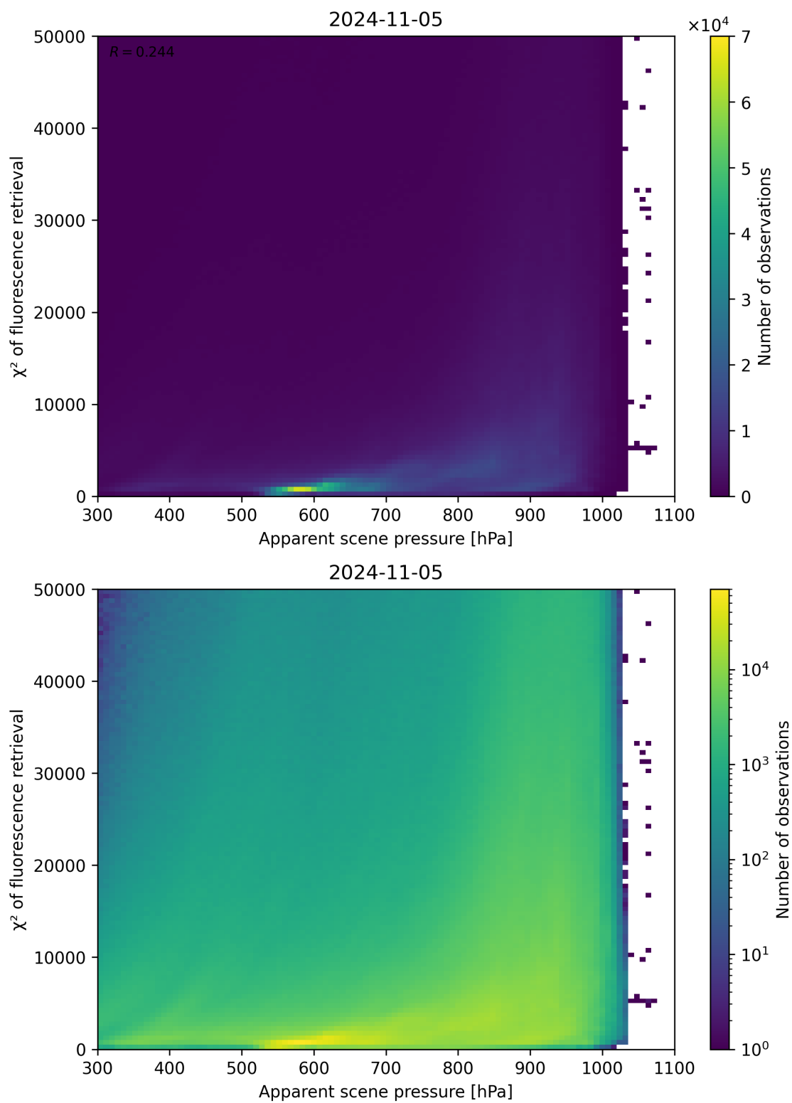
Figure 64: Scatter density plot of “Apparent scene pressure” against “ \chi^2 of fluorescence retrieval” for 2024-11-04 to 2024-11-06.
