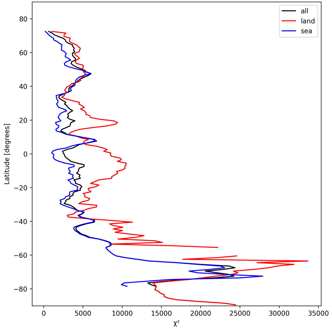
Figure 21: Zonal average of “ \chi^2 ” for 2024-11-04 to 2024-11-06.
