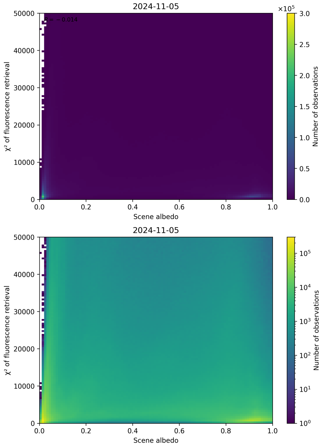
Figure 113: Scatter density plot of “Scene albedo” against “ \chi^2 of fluorescence retrieval” for 2024-11-04 to 2024-11-06.
