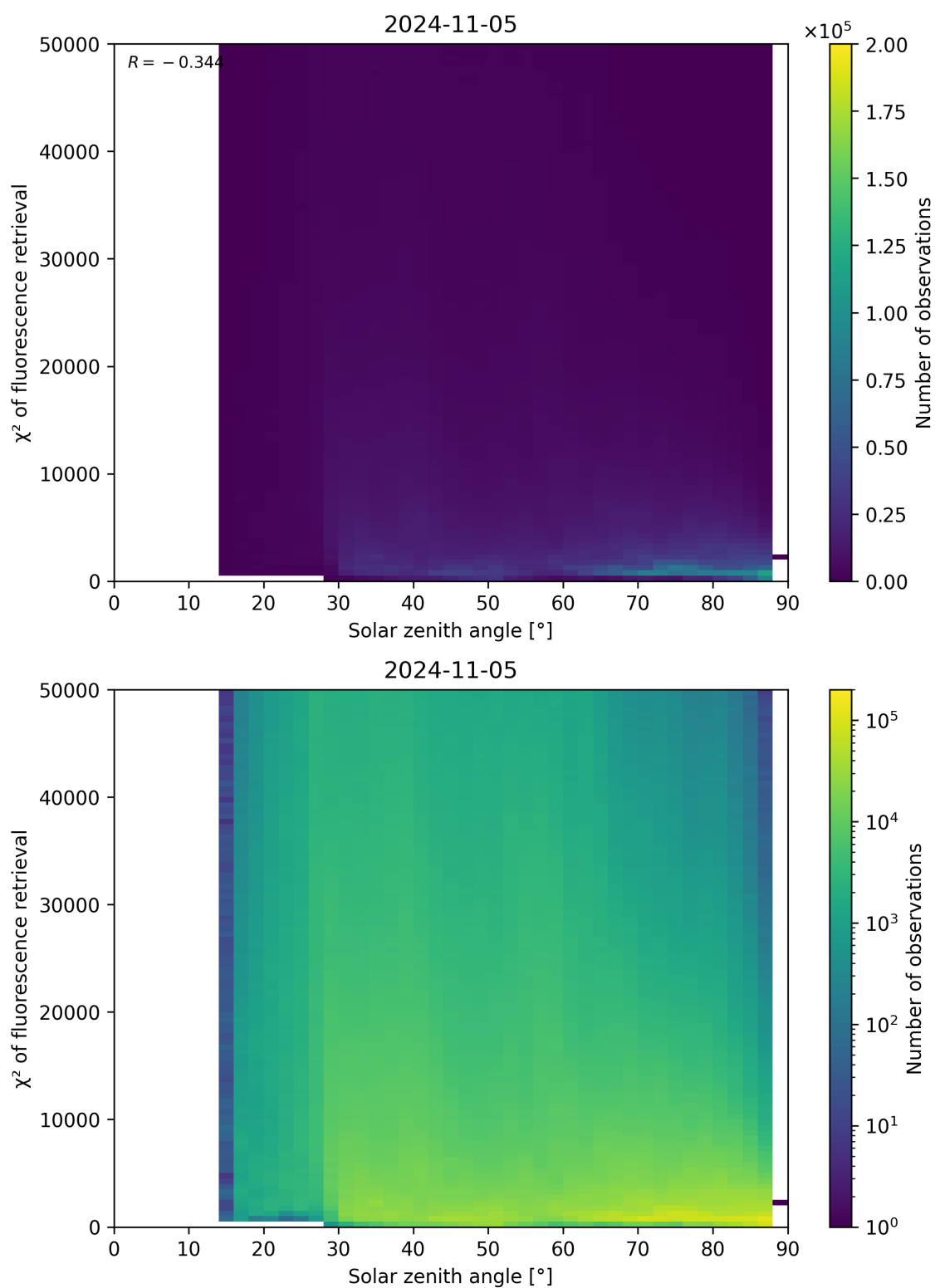
Figure 120: Scatter density plot of “Solar zenith angle” against “ \chi^2 of fluorescence retrieval” for 2024-11-04 to 2024-11-06.
