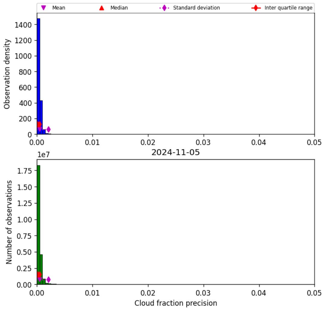
Figure 33: Histogram of “Cloud fraction precision” for 2024-11-04 to 2024-11-06
