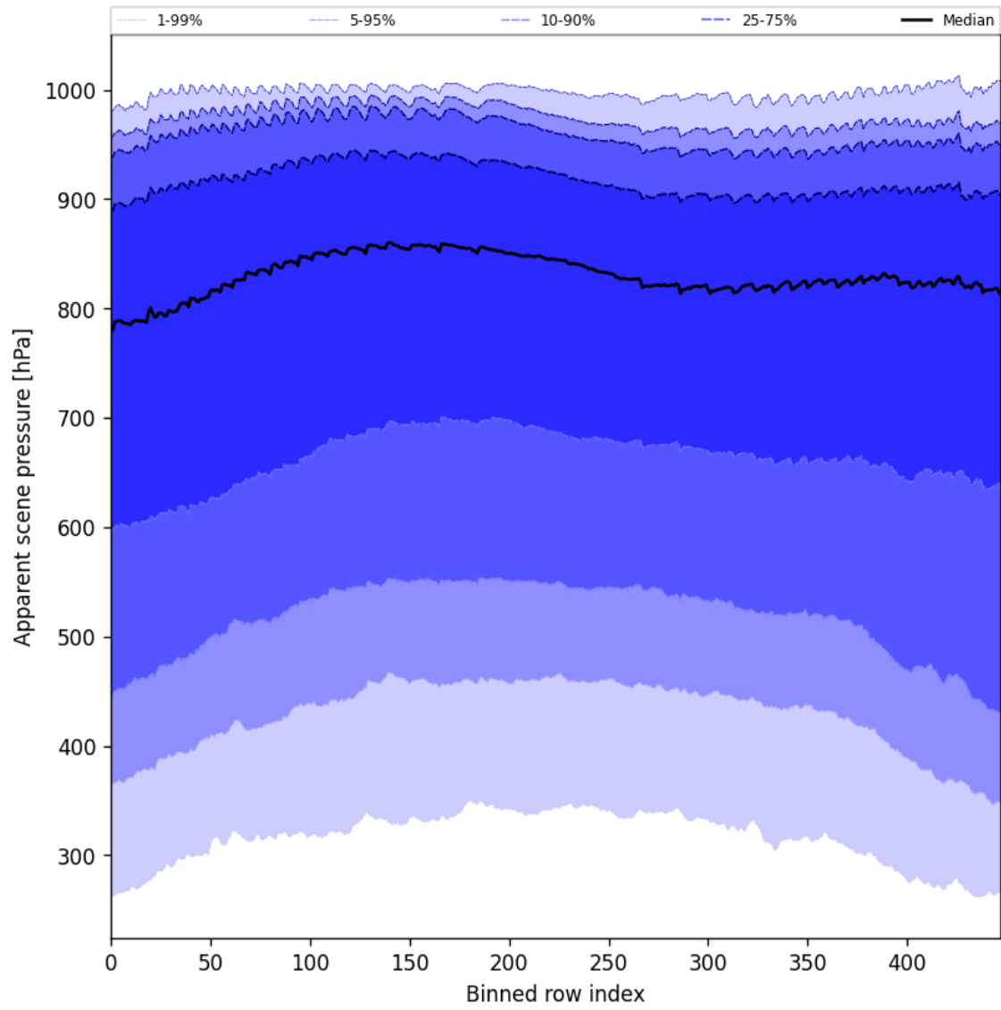
Figure 53: Along track statistics of “Apparent scene pressure” for 2024-11-04 to 2024-11-06
