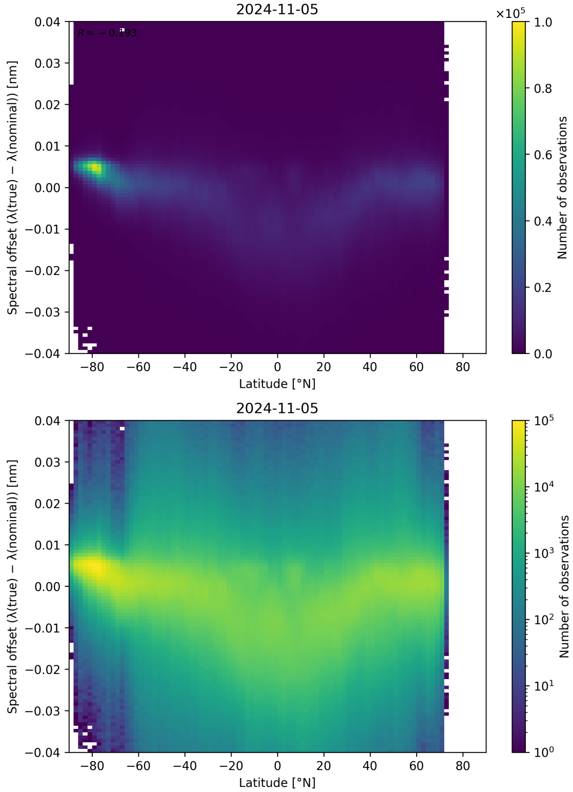
Figure 105: Scatter density plot of “Latitude” against “Spectral offset ( \lambda_{\text{true}} - \lambda_{\text{nominal}} )” for 2024-11-04 to 2024-11-06.
