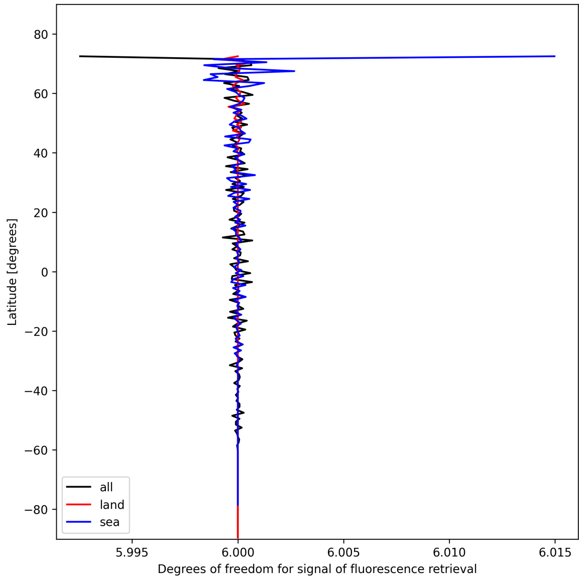
Figure 26: Zonal average of “Degrees of freedom for signal of fluorescence retrieval” for 2024-11-04 to 2024-11-06.
