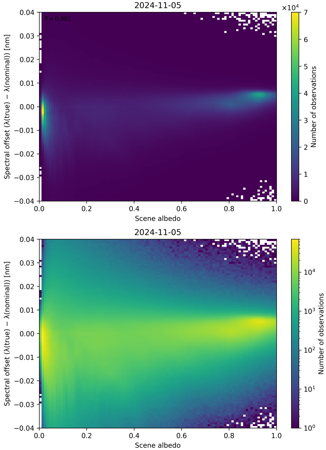
Figure 117: Scatter density plot of “Scene albedo” against “Spectral offset ( \lambda_{\text{true}} - \lambda_{\text{nominal}} )” for 2024-11-04 to 2024-11-06.
