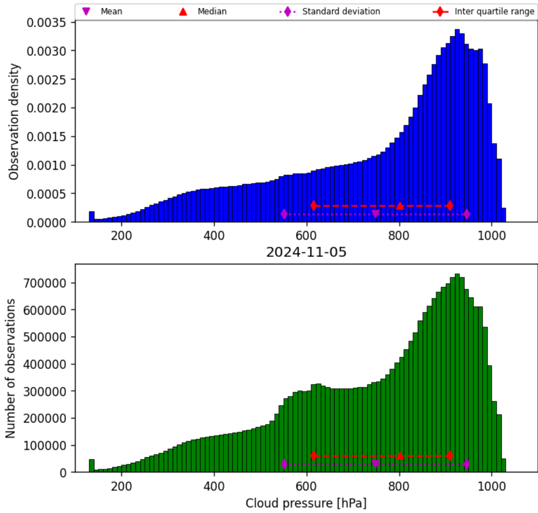
Figure 30: Histogram of “Cloud pressure” for 2024-11-04 to 2024-11-06
