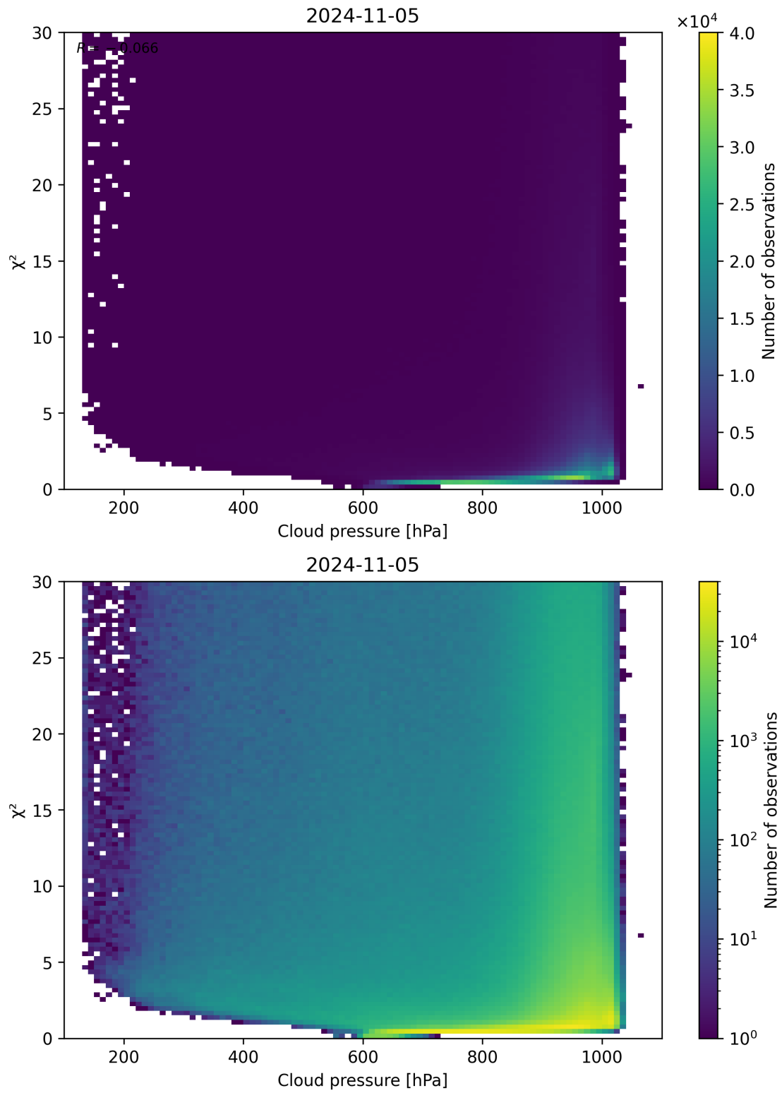
Figure 85: Scatter density plot of “Cloud pressure” against “ \chi^2 ” for 2024-11-04 to 2024-11-06.
