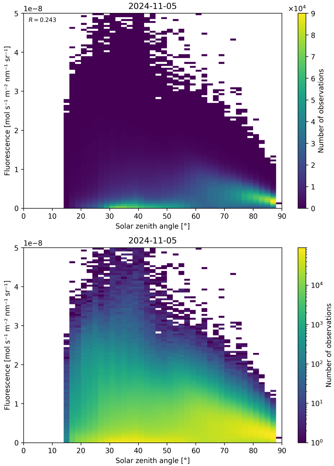
Figure 123: Scatter density plot of “Solar zenith angle” against “Fluorescence” for 2024-11-04 to 2024-11-06.
