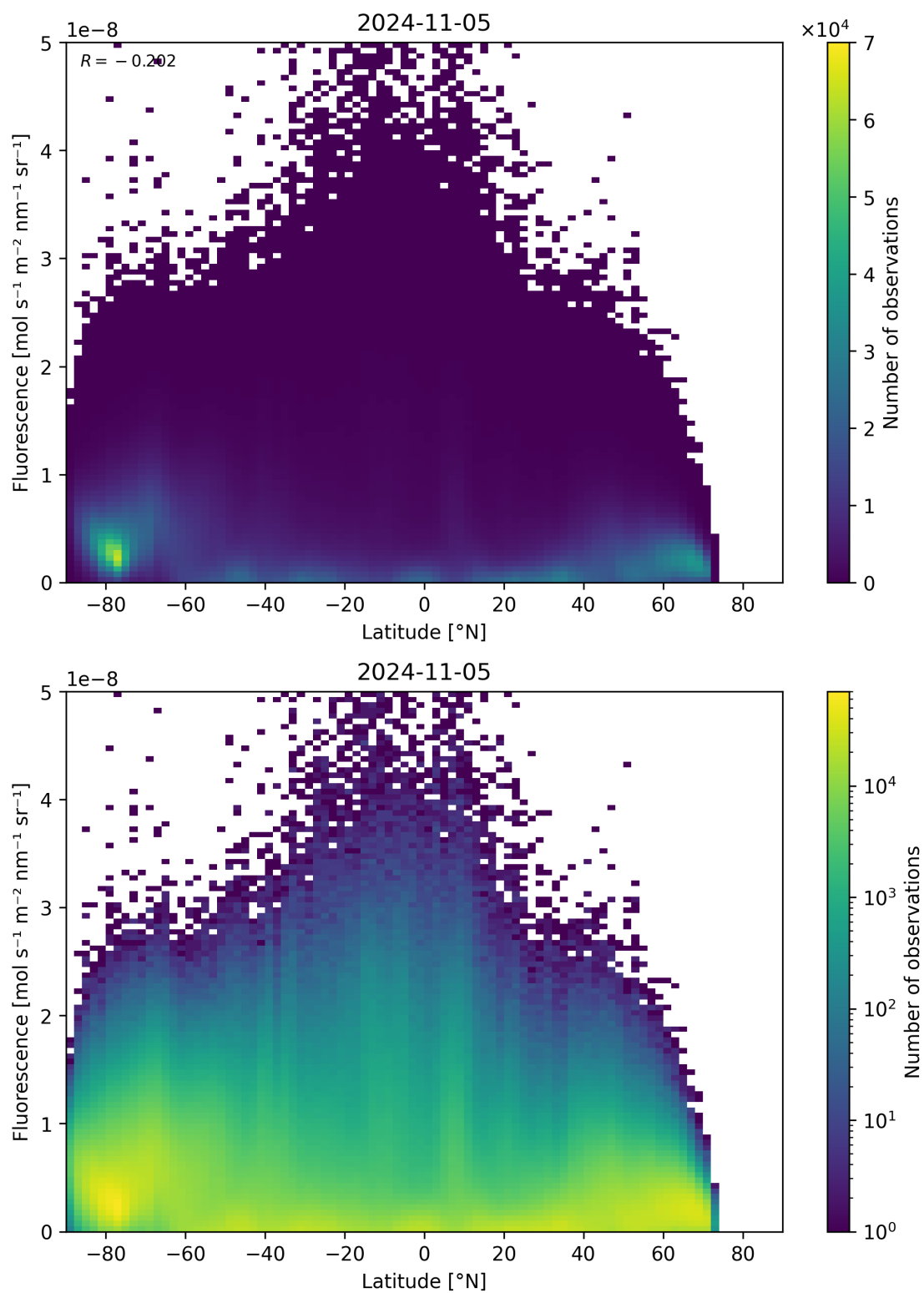
Figure 101: Scatter density plot of “Latitude” against “Fluorescence” for 2024-11-04 to 2024-11-06.
