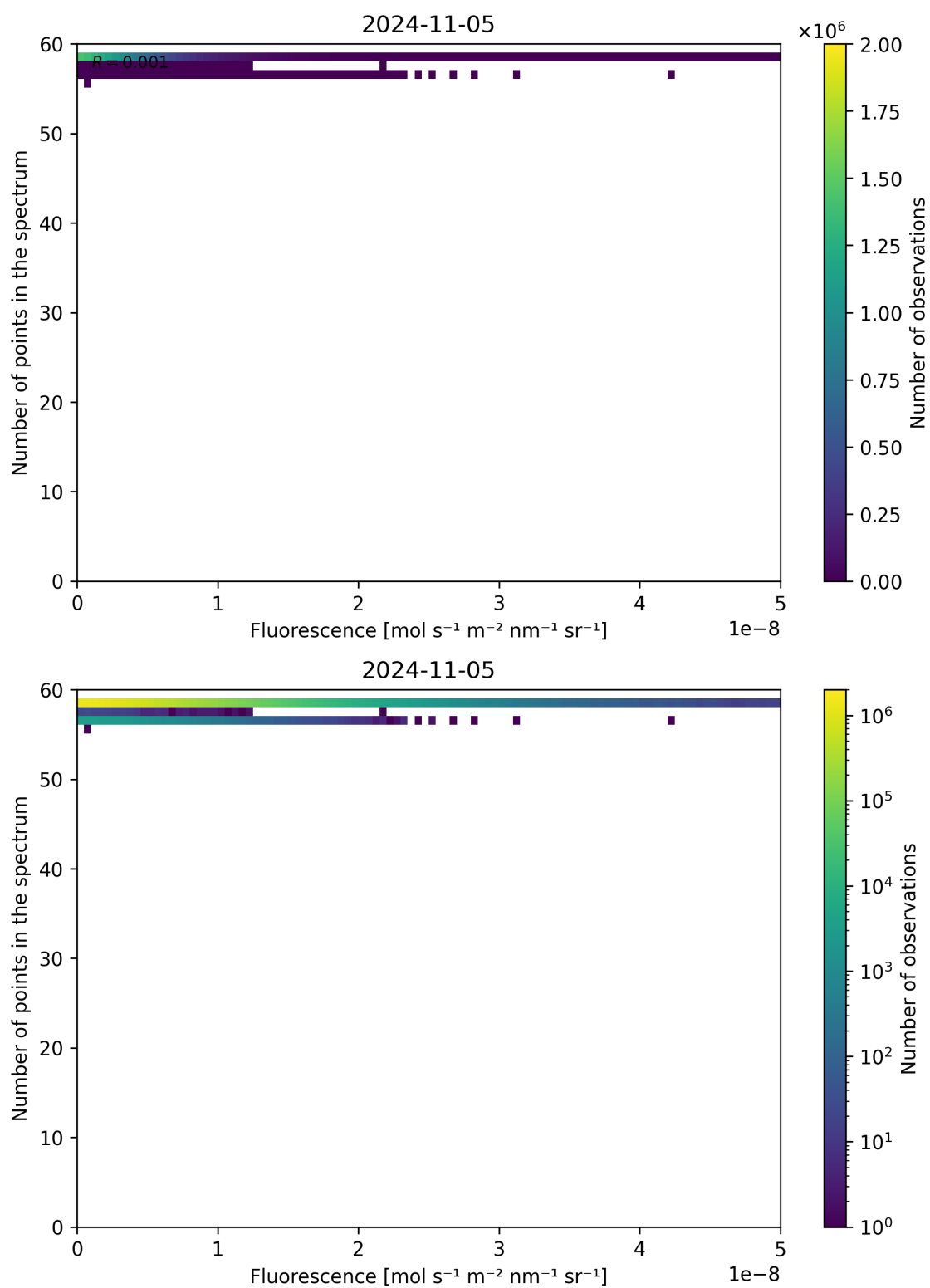
Figure 94: Scatter density plot of “Fluorescence” against “Number of points in the spectrum” for 2024-11-04 to 2024-11-06.
