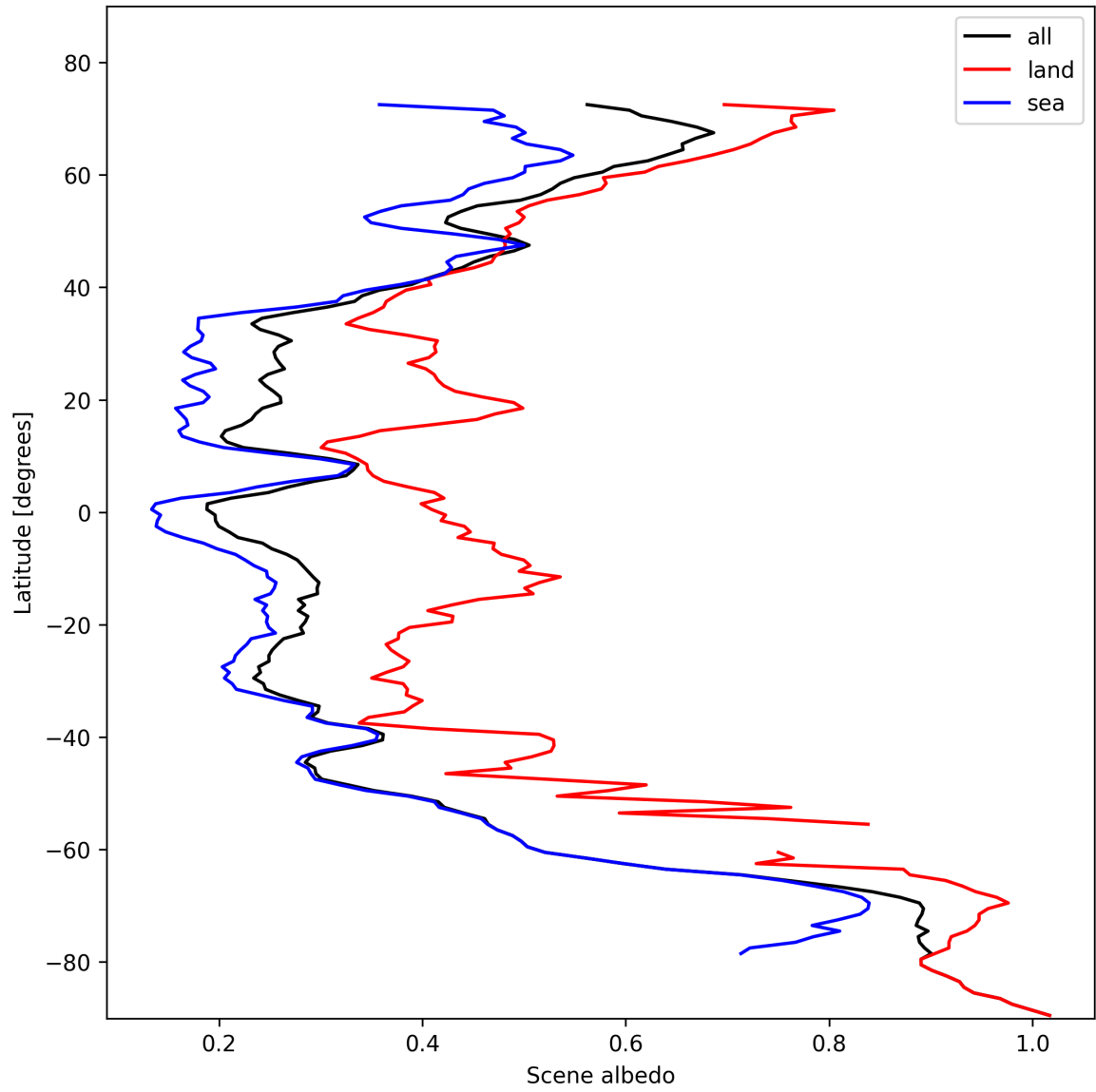
Figure 17: Zonal average of “Scene albedo” for 2024-11-04 to 2024-11-06.
