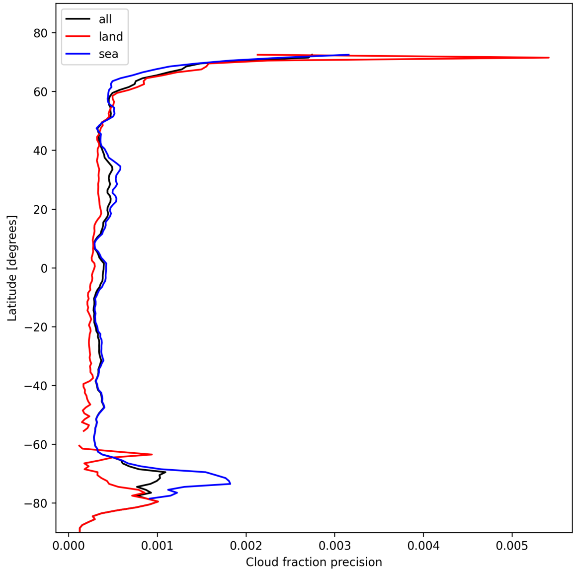
Figure 16: Zonal average of “Cloud fraction precision” for 2024-11-04 to 2024-11-06.
