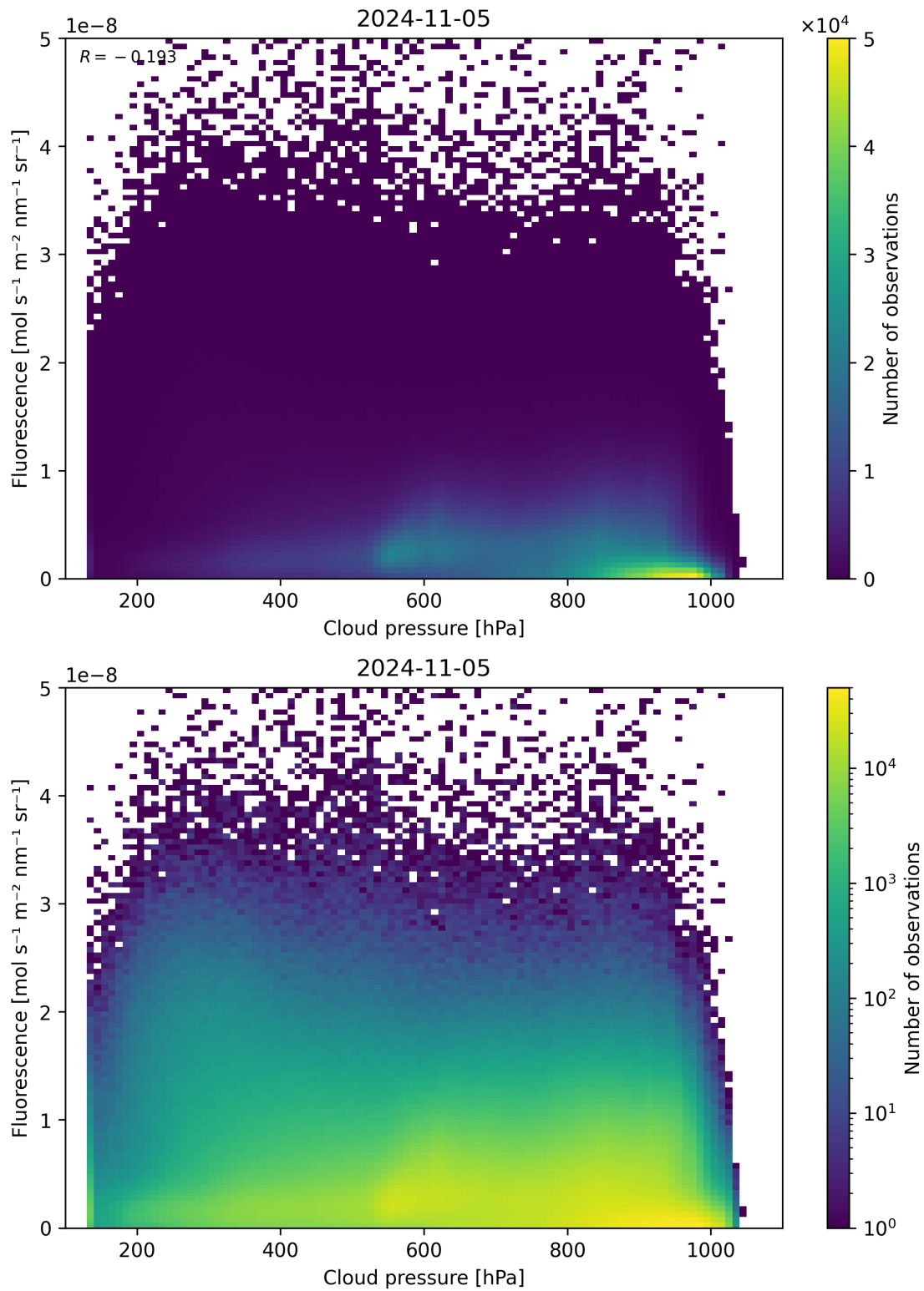
Figure 88: Scatter density plot of “Cloud pressure” against “Fluorescence” for 2024-11-04 to 2024-11-06.
