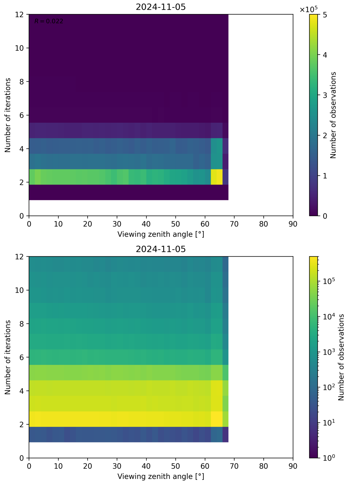
Figure 136: Scatter density plot of “Viewing zenith angle” against “Number of iterations” for 2024-11-04 to 2024-11-06.
