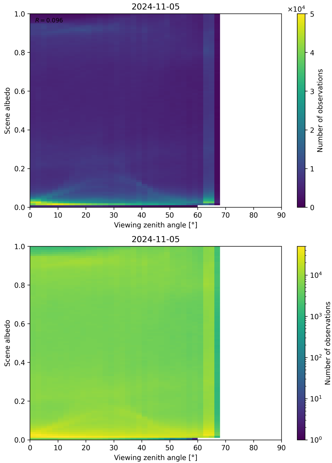
Figure 138: Scatter density plot of “Viewing zenith angle” against “Scene albedo” for 2024-11-04 to 2024-11-06.
