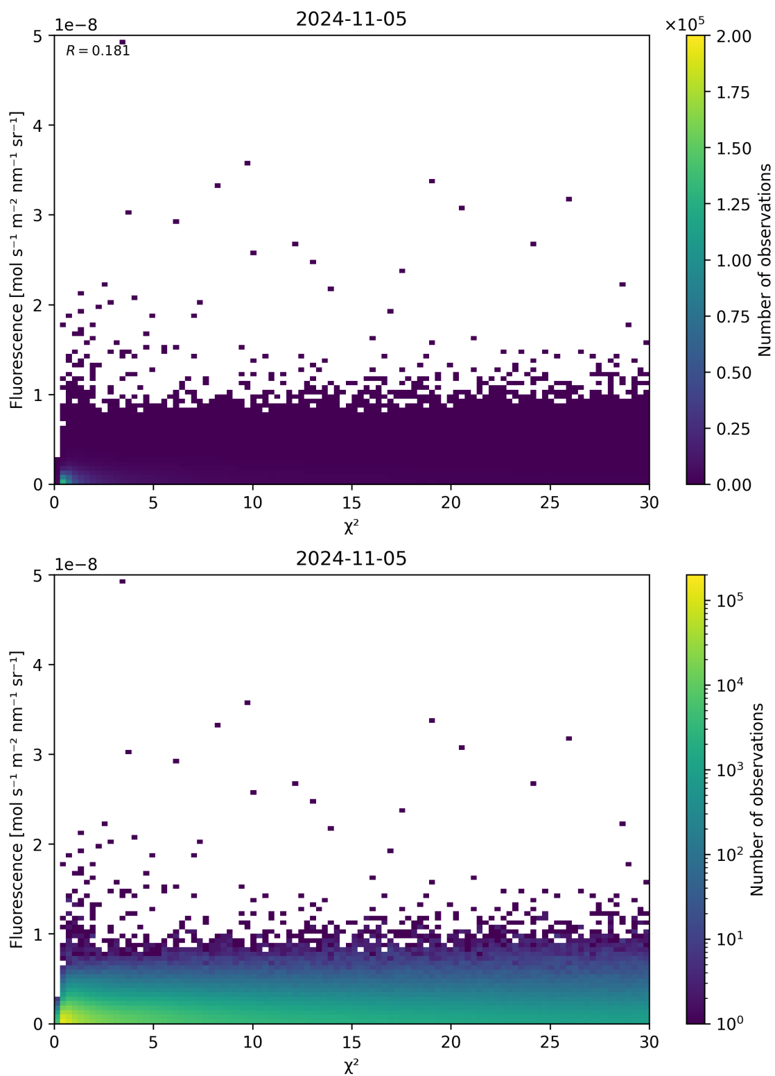
Figure 70: Scatter density plot of “ \chi^2 ” against “Fluorescence” for 2024-11-04 to 2024-11-06.
