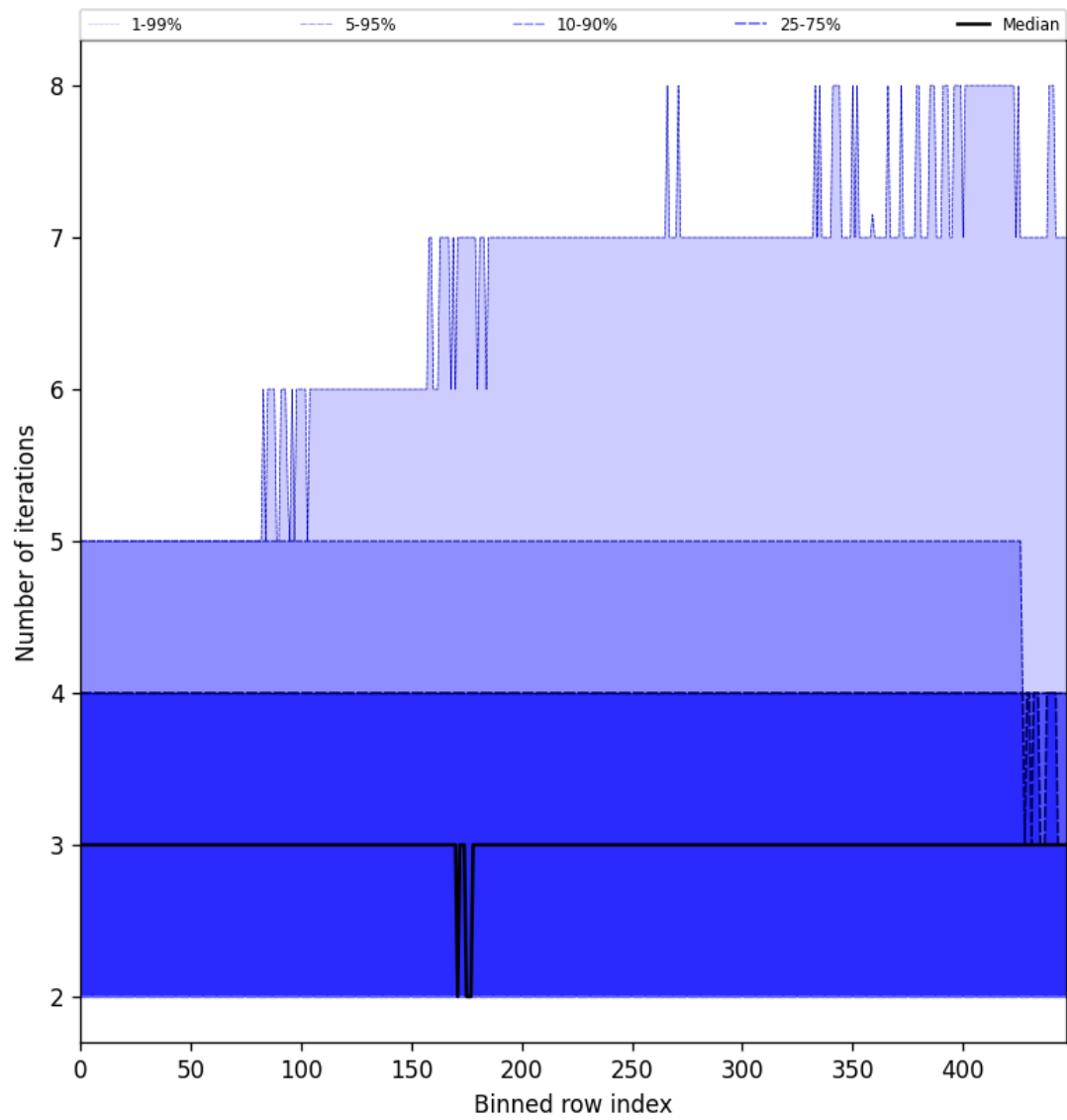
Figure 56: Along track statistics of “Number of iterations” for 2024-11-04 to 2024-11-06
