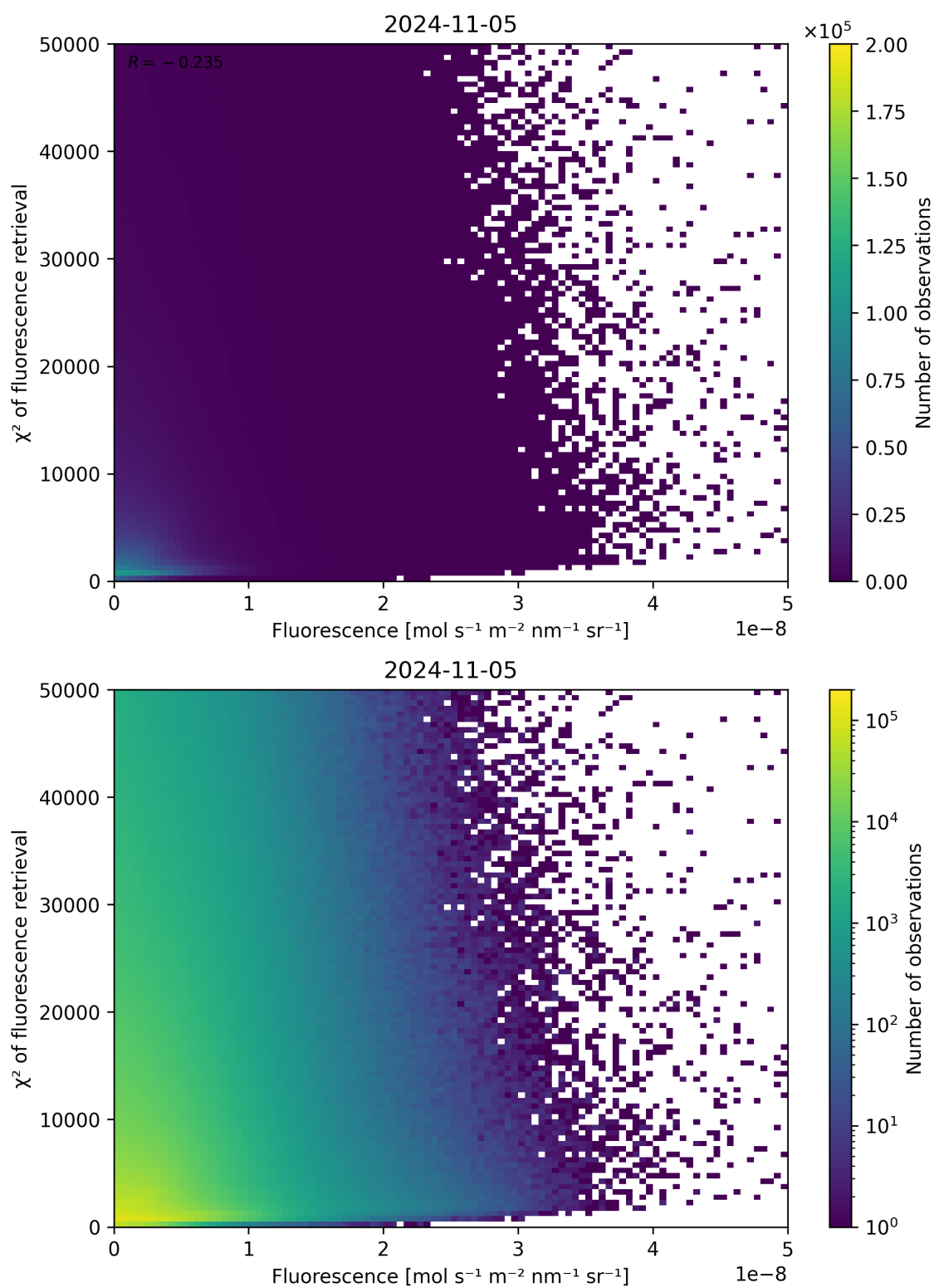
Figure 93: Scatter density plot of “Fluorescence” against “ \chi^2 of fluorescence retrieval” for 2024-11-04 to 2024-11-06.
