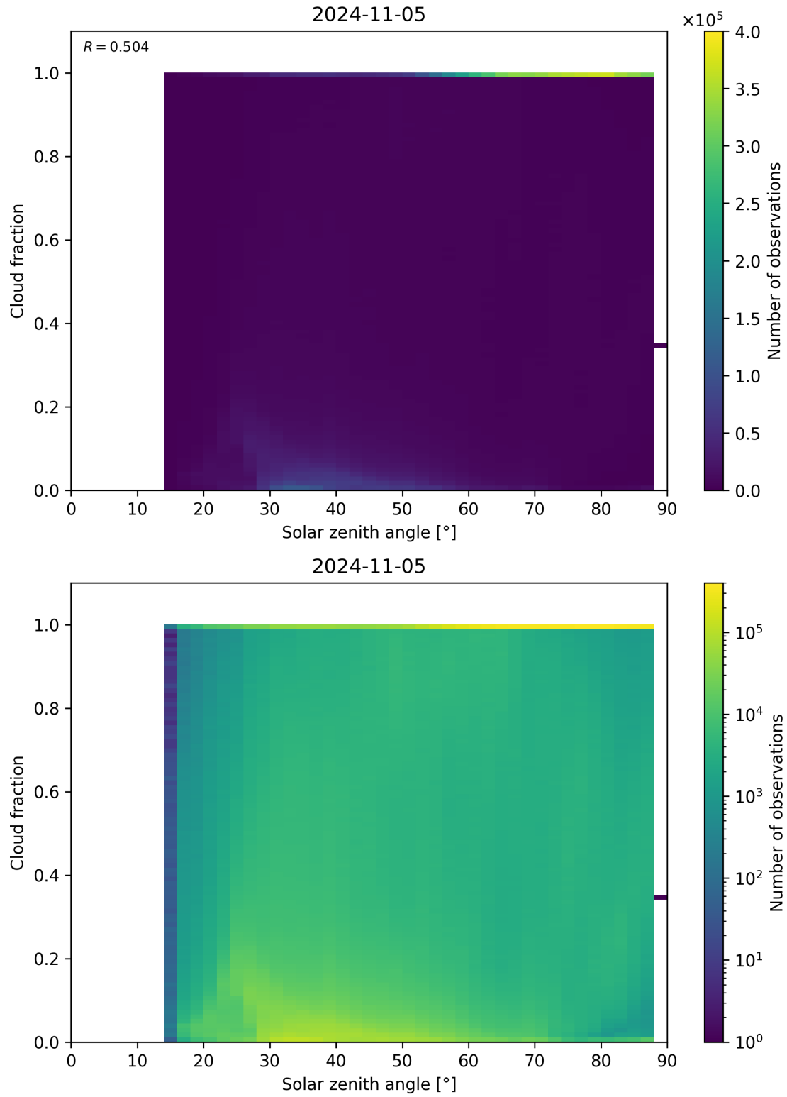
Figure 121: Scatter density plot of “Solar zenith angle” against “Cloud fraction” for 2024-11-04 to 2024-11-06.
