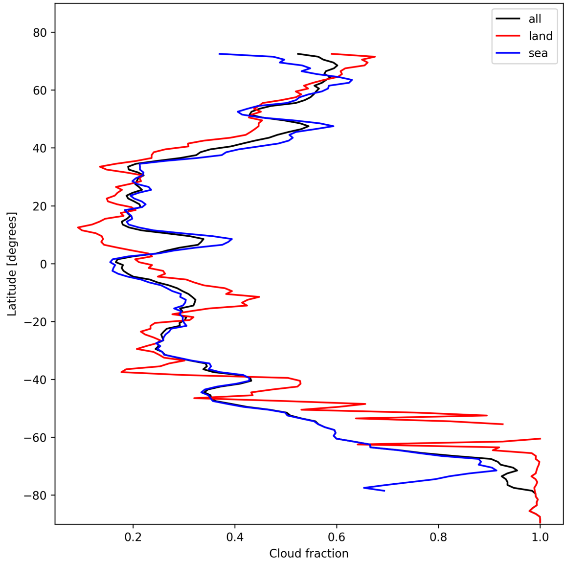
Figure 15: Zonal average of “Cloud fraction” for 2024-11-04 to 2024-11-06.
