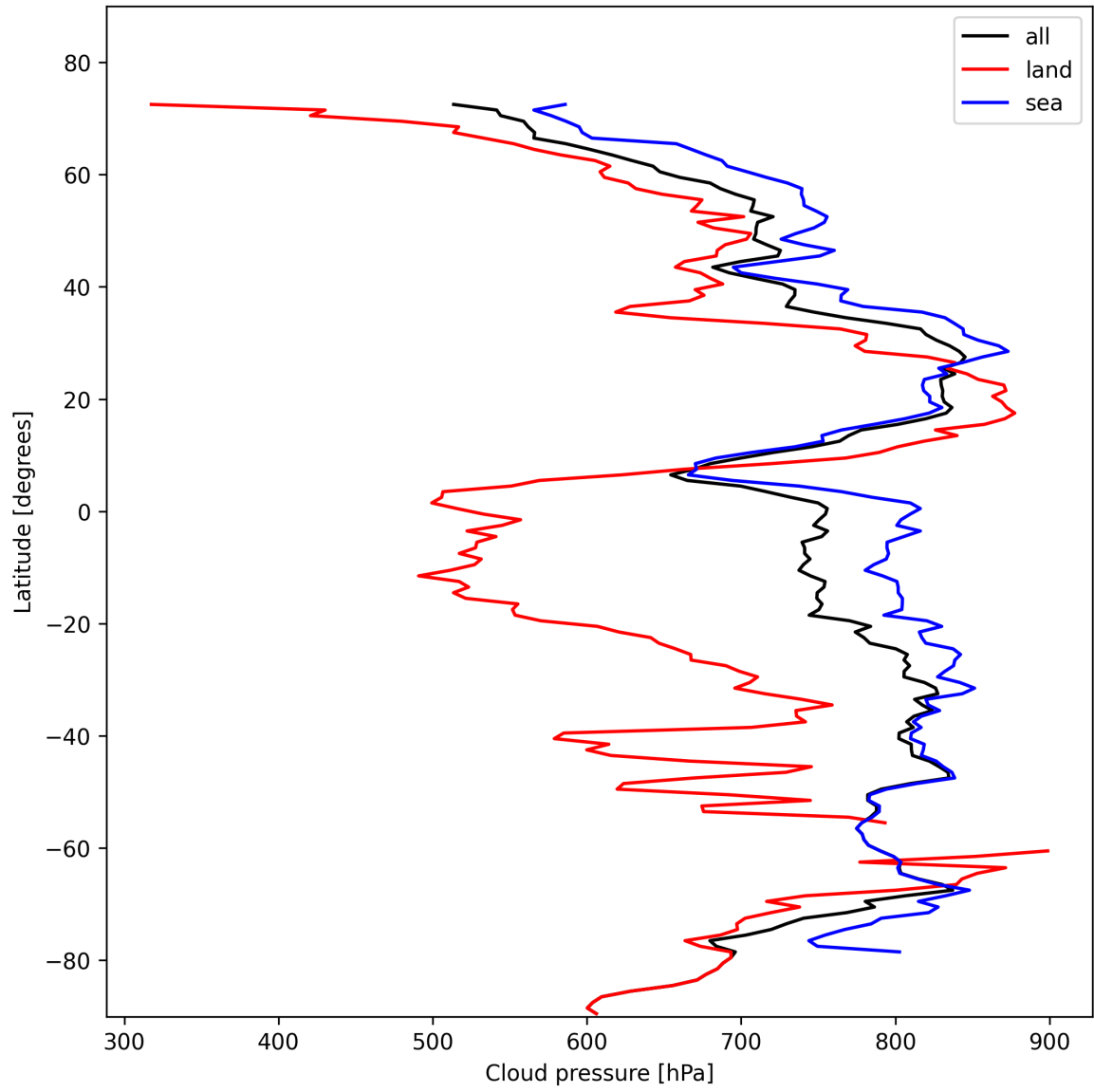
Figure 13: Zonal average of “Cloud pressure” for 2024-11-04 to 2024-11-06.
