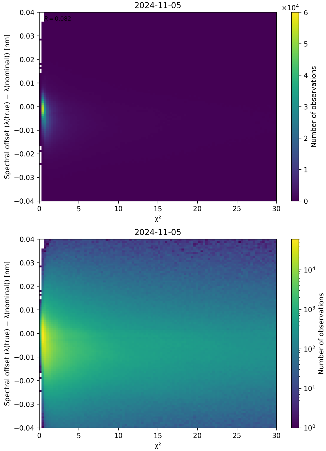
Figure 75: Scatter density plot of “ \chi^2 ” against “Spectral offset ( \lambda_{\text{true}} - \lambda_{\text{nominal}} )” for 2024-11-04 to 2024-11-06.
