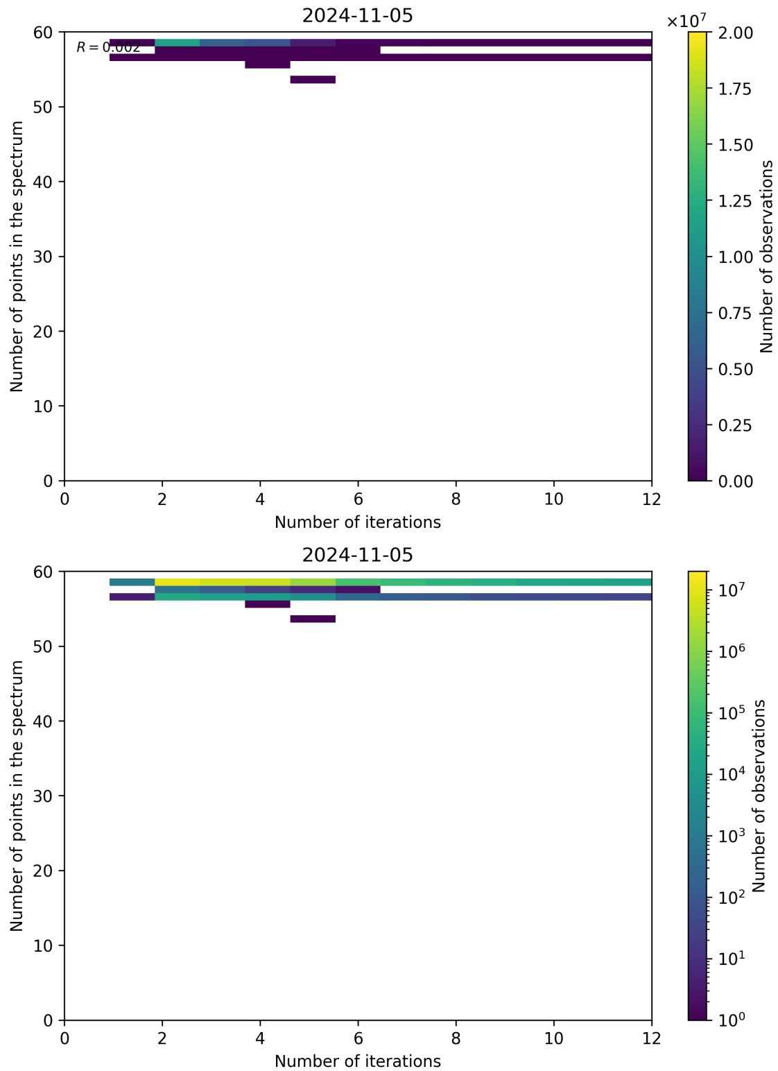
Figure 108: Scatter density plot of “Number of iterations” against “Number of points in the spectrum” for 2024-11-04 to 2024-11-06.
