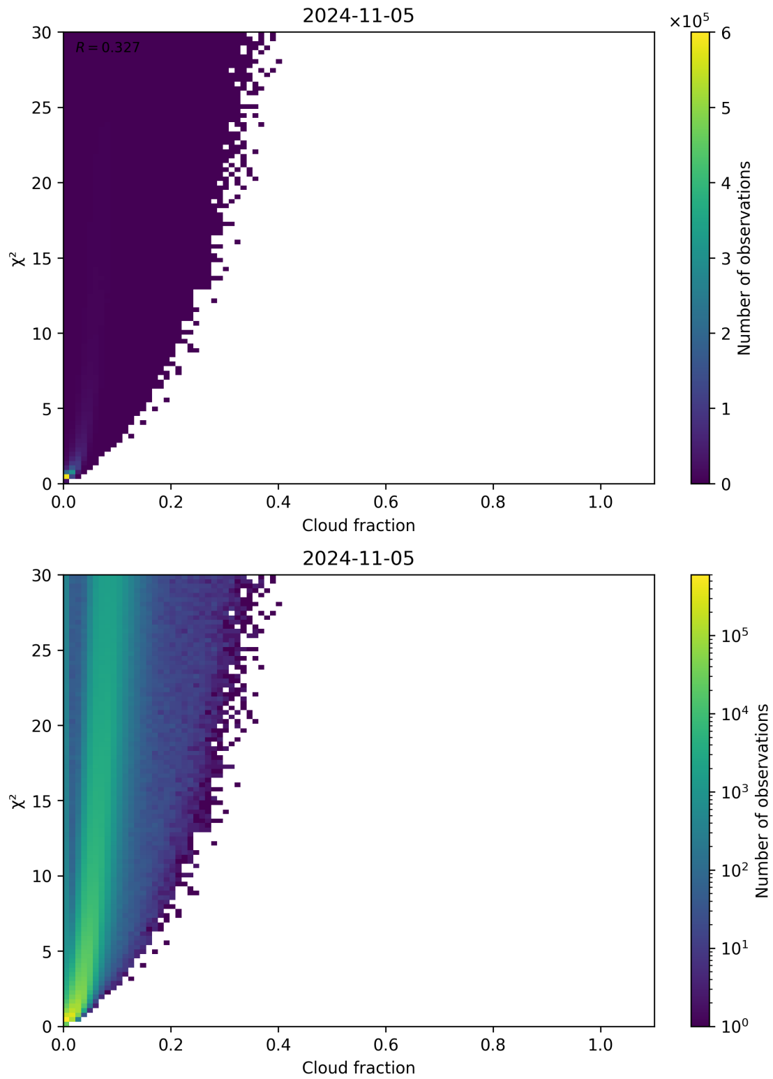
Figure 77: Scatter density plot of “Cloud fraction” against “ \chi^2 ” for 2024-11-04 to 2024-11-06.
