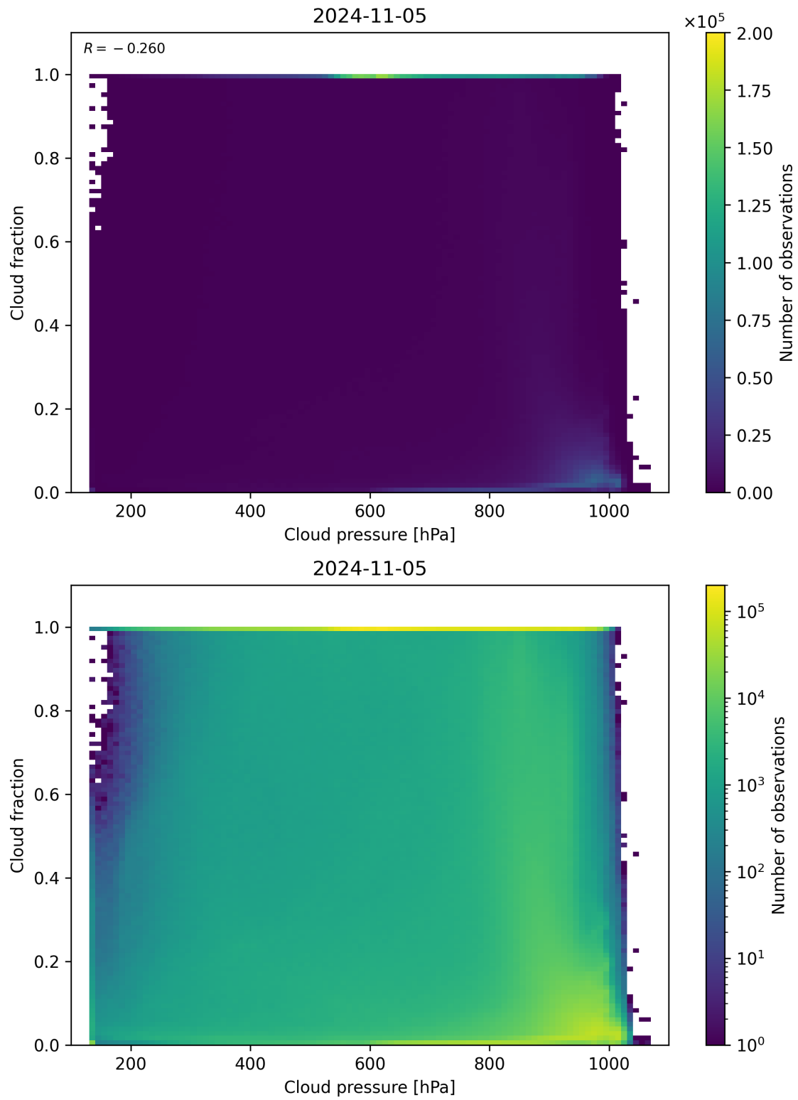
Figure 87: Scatter density plot of “Cloud pressure” against “Cloud fraction” for 2024-11-04 to 2024-11-06.
