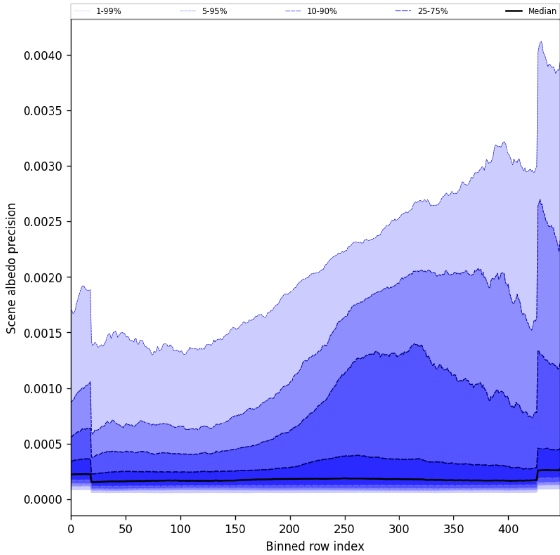
Figure 52: Along track statistics of “Scene albedo precision” for 2024-11-04 to 2024-11-06
