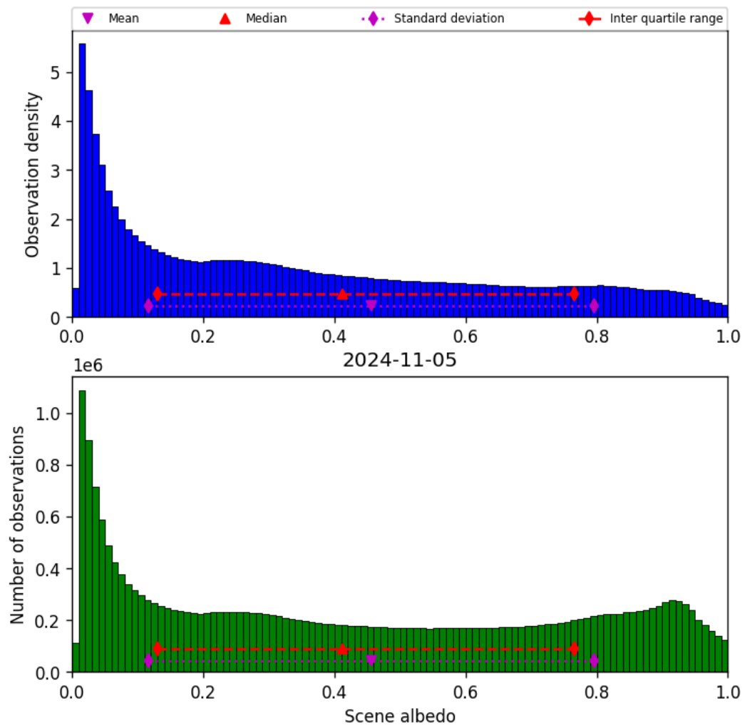
Figure 34: Histogram of “Scene albedo” for 2024-11-04 to 2024-11-06
