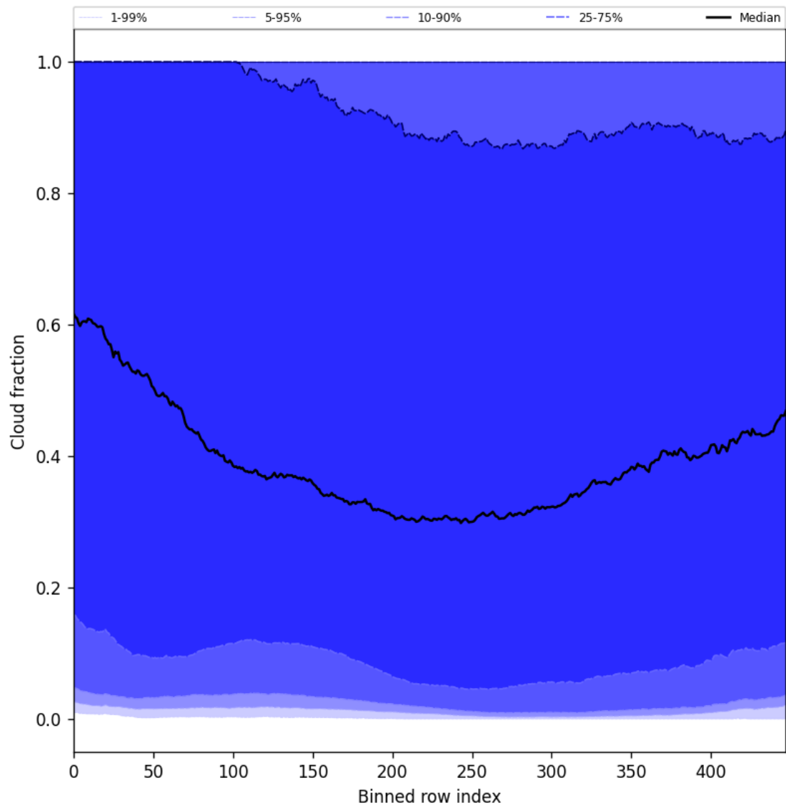
Figure 49: Along track statistics of “Cloud fraction” for 2024-11-04 to 2024-11-06
