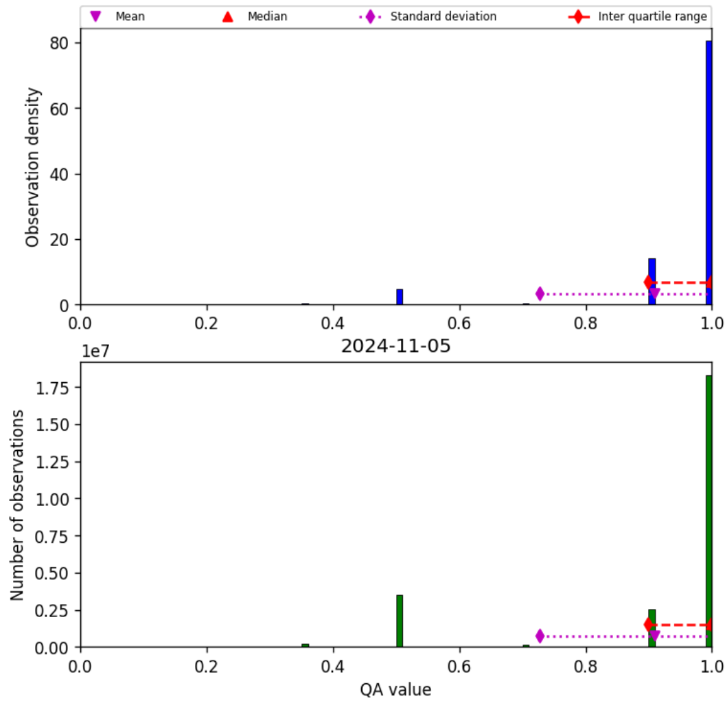
Figure 29: Histogram of “QA value” for 2024-11-04 to 2024-11-06
