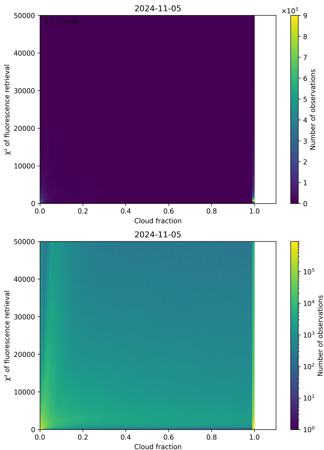
Figure 78: Scatter density plot of “Cloud fraction” against “ \chi^2 of fluorescence retrieval” for 2024-11-04 to 2024-11-06.
