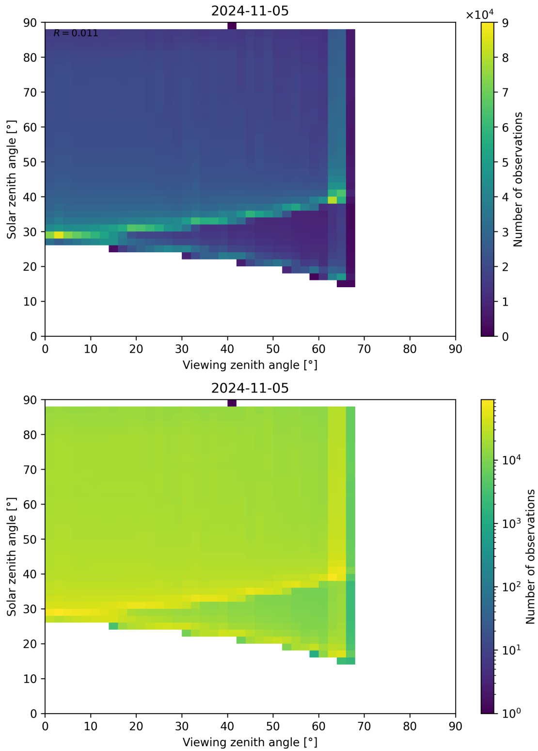
Figure 139: Scatter density plot of “Viewing zenith angle” against “Solar zenith angle” for 2024-11-04 to 2024-11-06.
