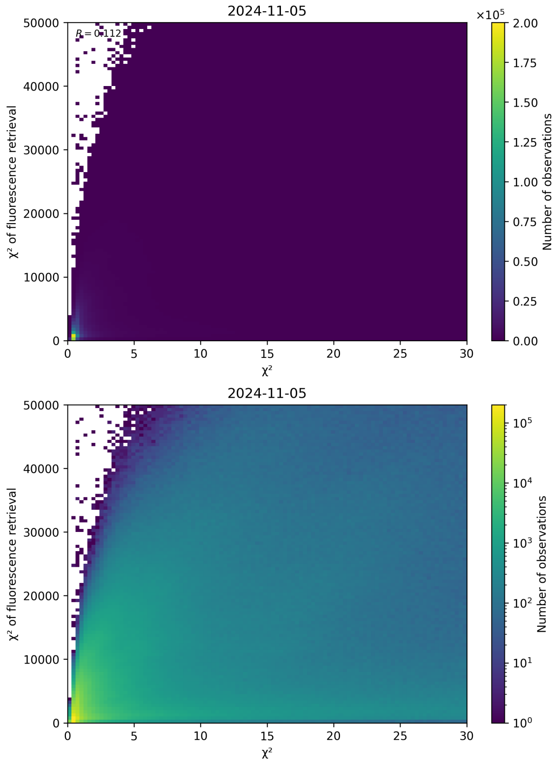
Figure 69: Scatter density plot of “ \chi^2 ” against “ \chi^2 of fluorescence retrieval” for 2024-11-04 to 2024-11-06.
