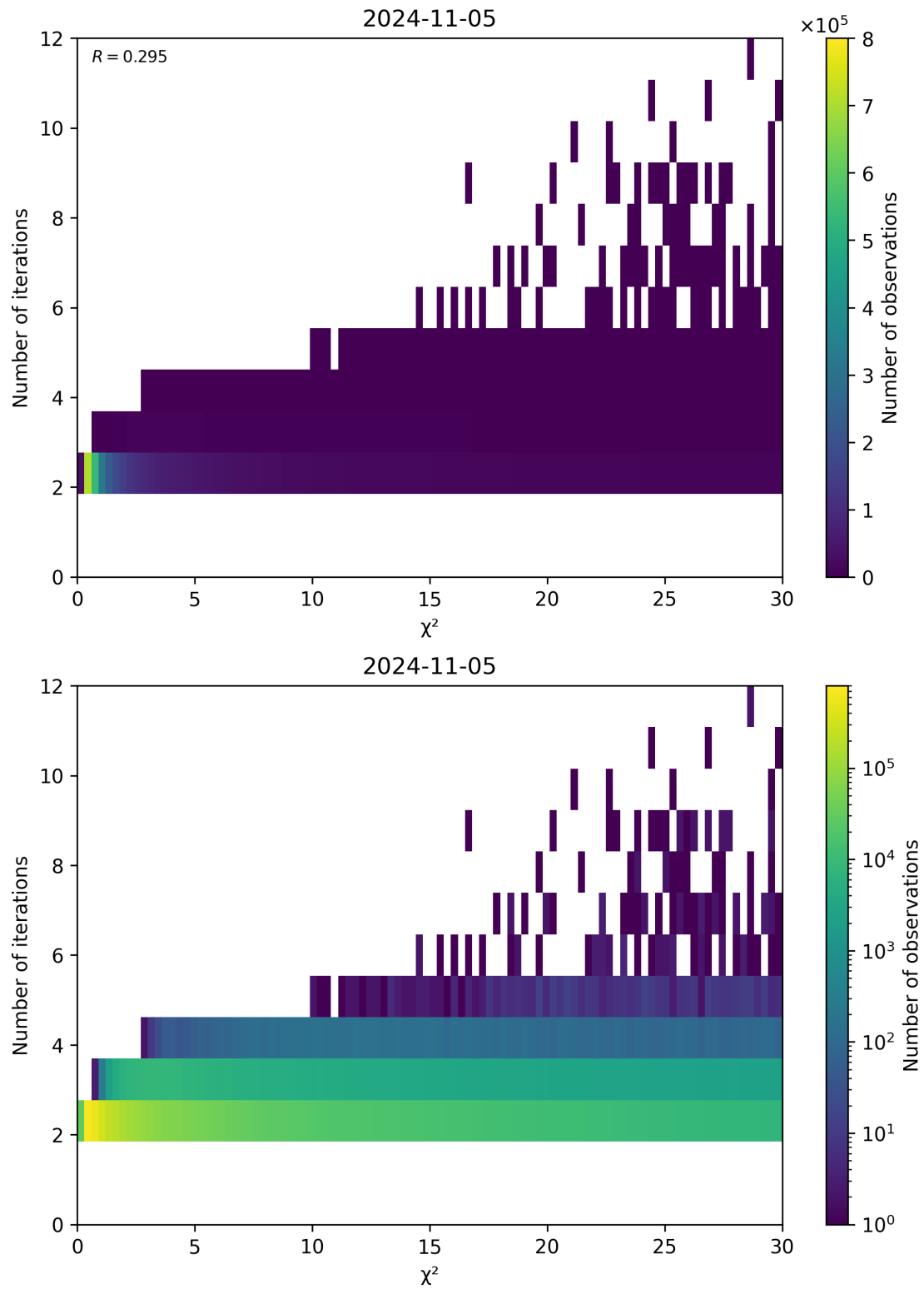
Figure 73: Scatter density plot of “ \chi^2 ” against “Number of iterations” for 2024-11-04 to 2024-11-06.
