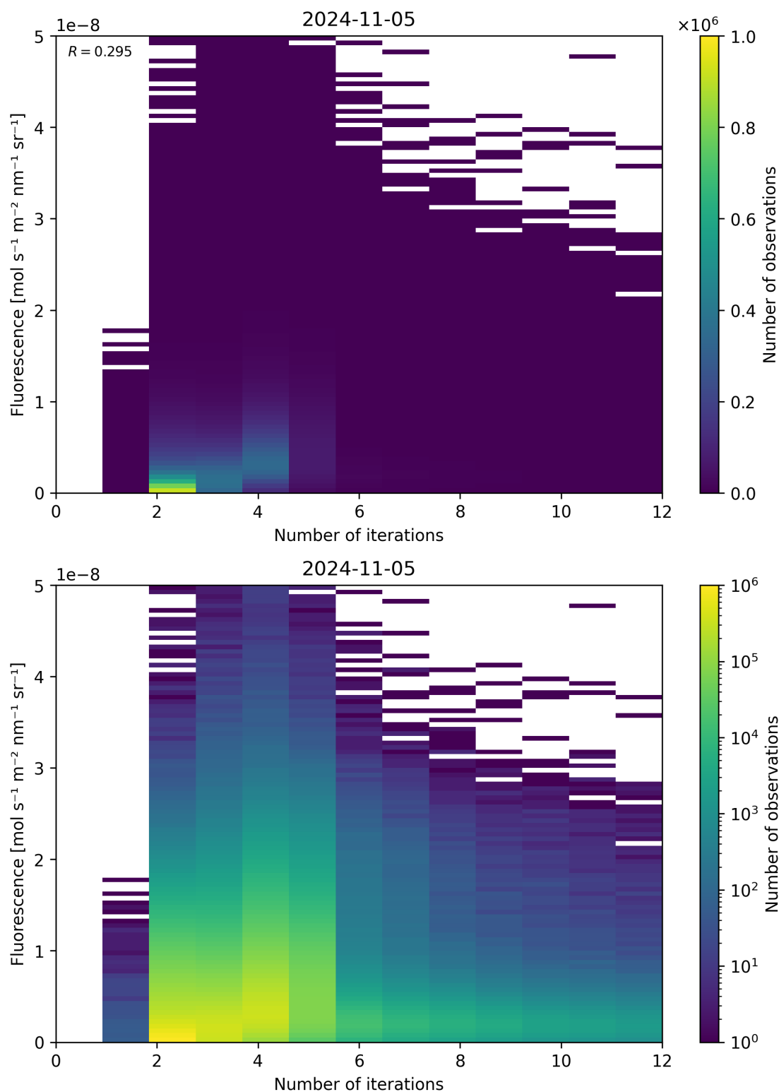
Figure 107: Scatter density plot of "Number of iterations" against "Fluorescence" for 2024-11-04 to 2024-11-06.
