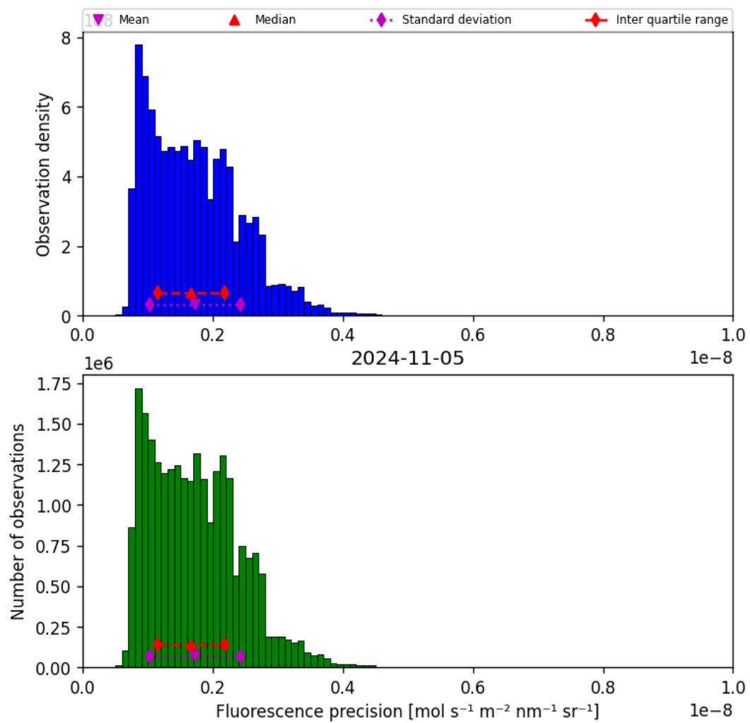
Figure 41: Histogram of “Fluorescence precision” for 2024-11-04 to 2024-11-06
