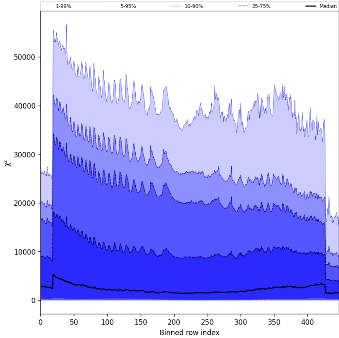
Figure 55: Along track statistics of “ \chi^2 ” for 2024-11-04 to 2024-11-06
