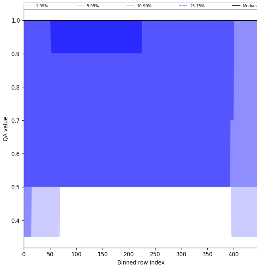
Figure 46: Along track statistics of “QA value” for 2024-11-04 to 2024-11-06
