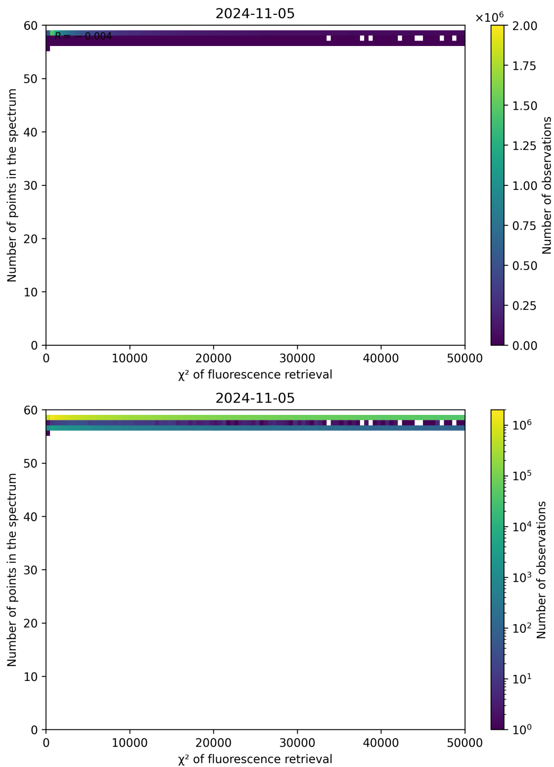
Figure 71: Scatter density plot of " \chi^2 of fluorescence retrieval" against "Number of points in the spectrum" for 2024-11-04 to 2024-11-06.
