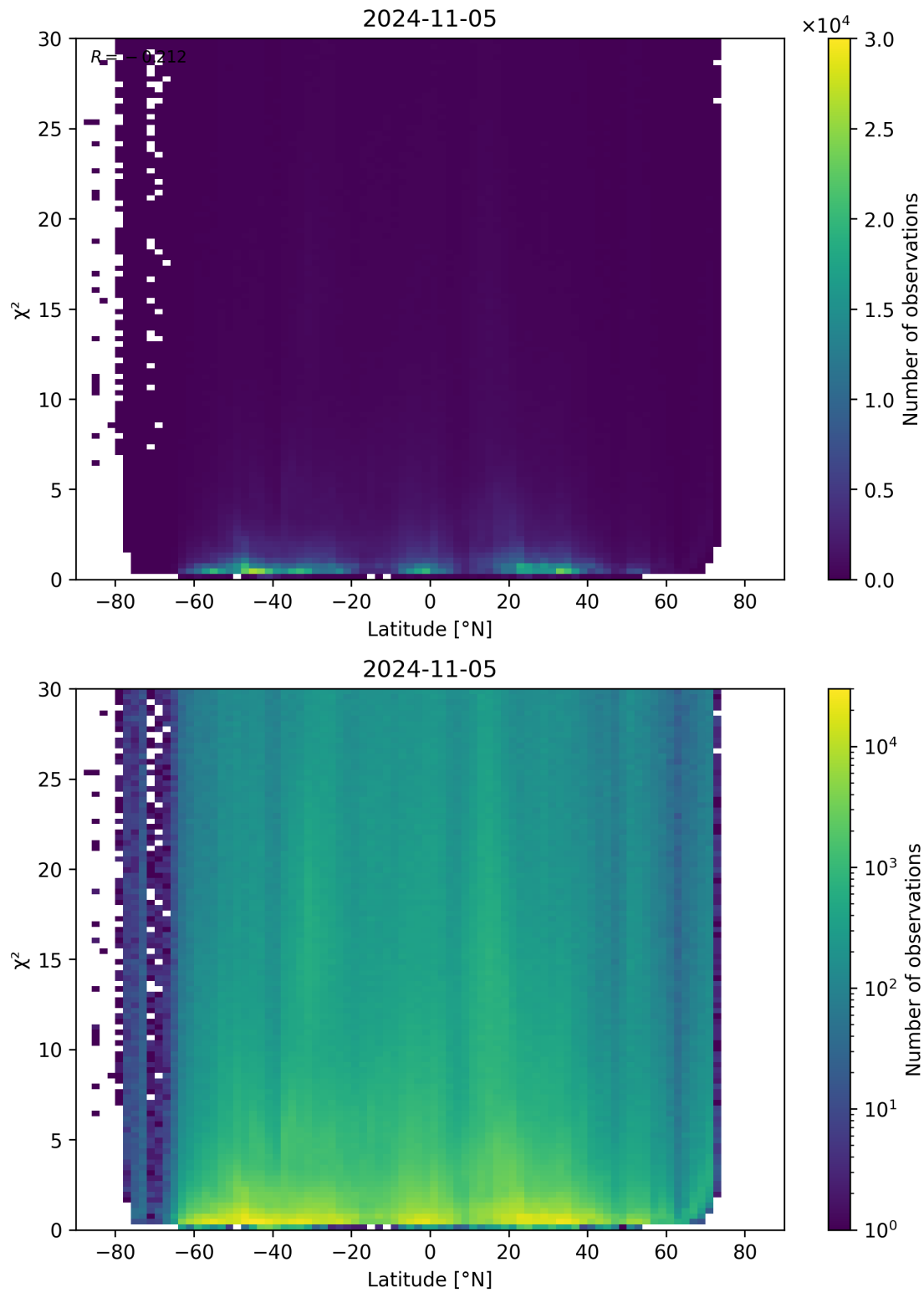
Figure 97: Scatter density plot of “Latitude” against “ \chi^2 ” for 2024-11-04 to 2024-11-06.
