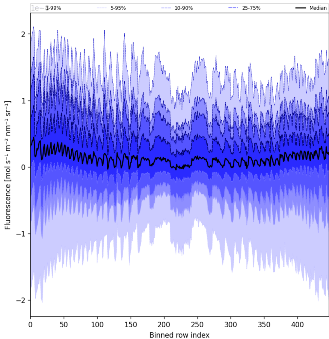
Figure 57: Along track statistics of “Fluorescence” for 2024-11-04 to 2024-11-06
