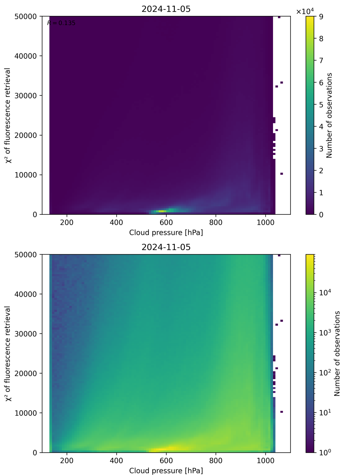
Figure 86: Scatter density plot of “Cloud pressure” against “ \chi^2 of fluorescence retrieval” for 2024-11-04 to 2024-11-06.
