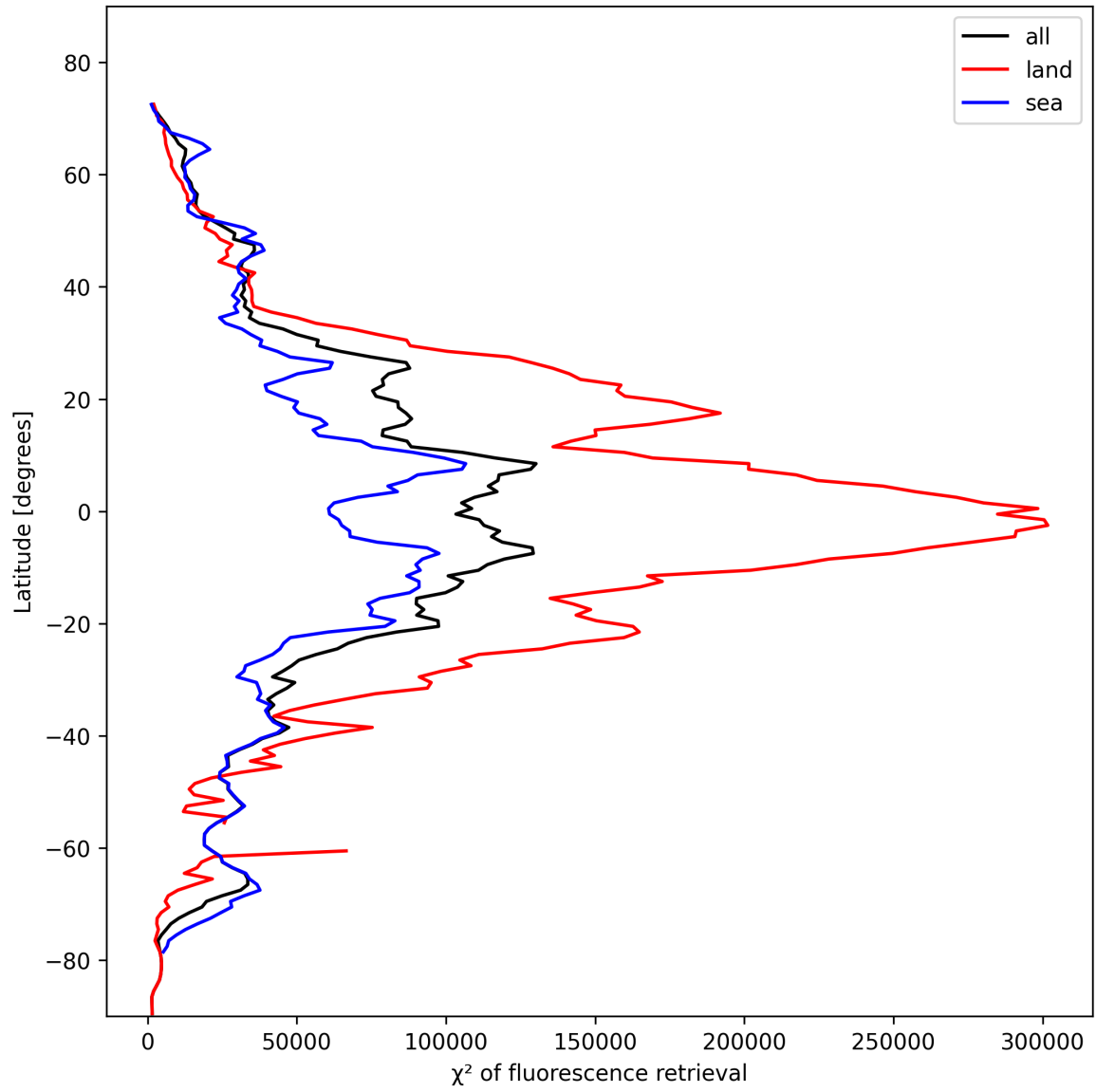
Figure 25: Zonal average of “ \chi^2 of fluorescence retrieval” for 2024-11-04 to 2024-11-06.
