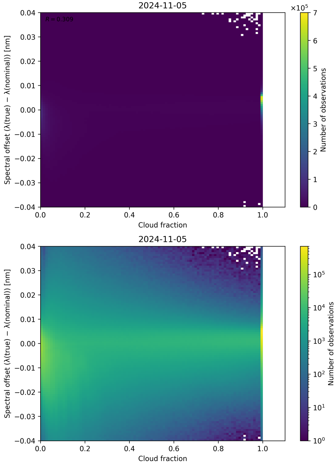
Figure 83: Scatter density plot of “Cloud fraction” against “Spectral offset ( \lambda_{\text{true}} - \lambda_{\text{nominal}} )” for 2024-11-04 to 2024-11-06.
