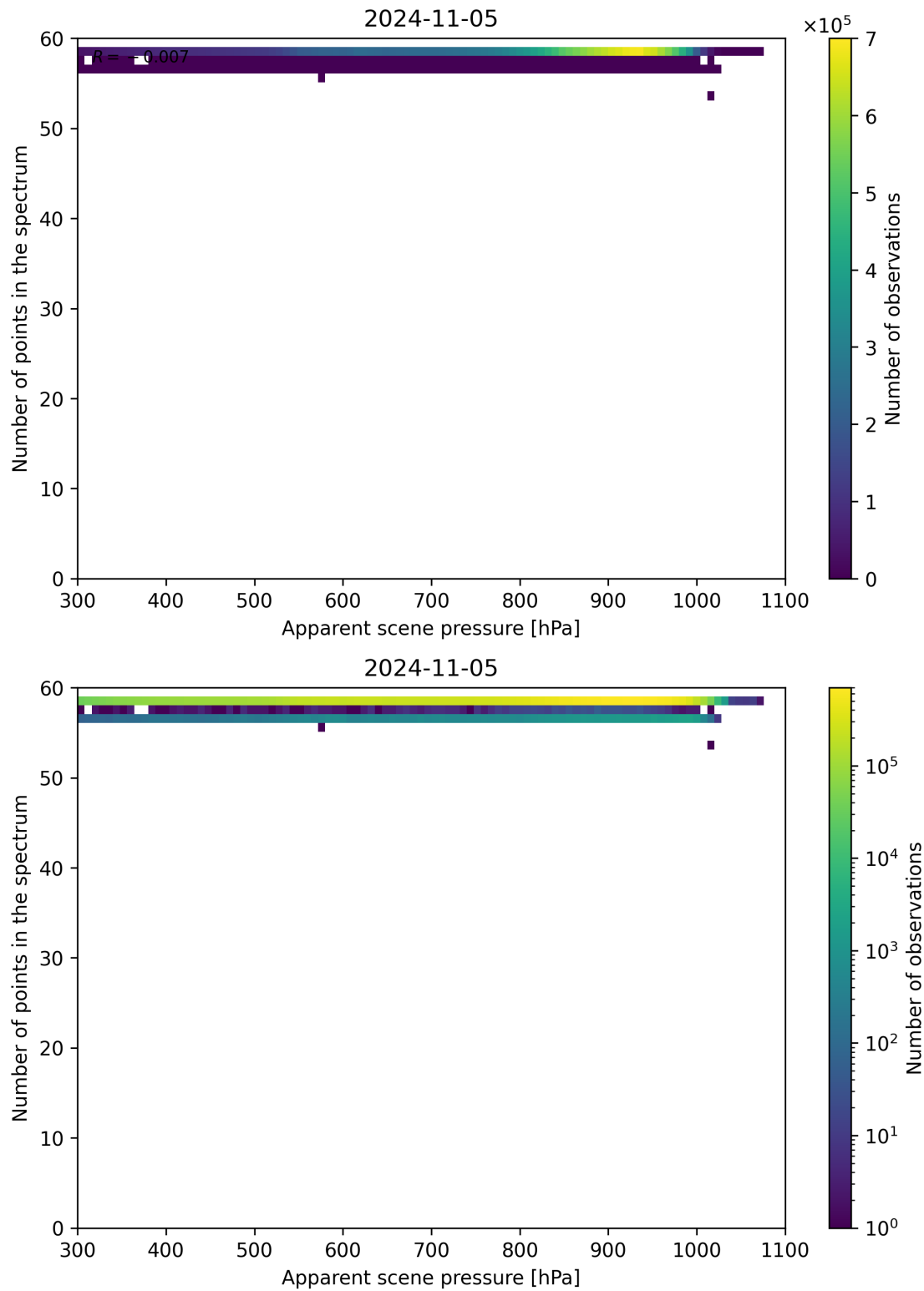
Figure 67: Scatter density plot of “Apparent scene pressure” against “Number of points in the spectrum” for 2024-11-04 to 2024-11-06.
