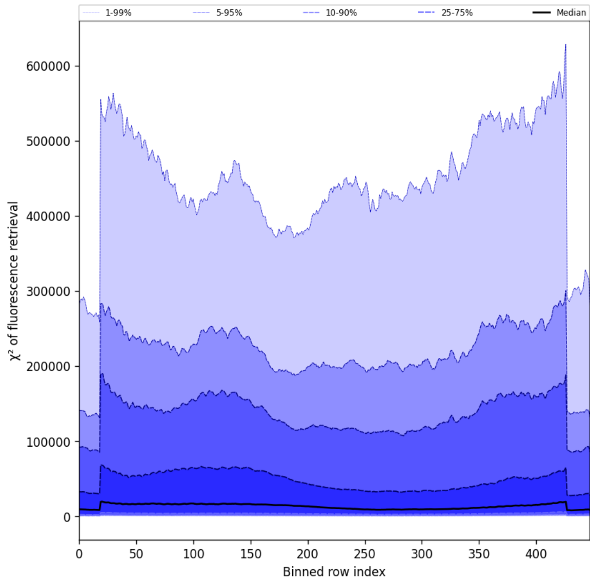
Figure 59: Along track statistics of “ \chi^2 of fluorescence retrieval” for 2024-11-04 to 2024-11-06
