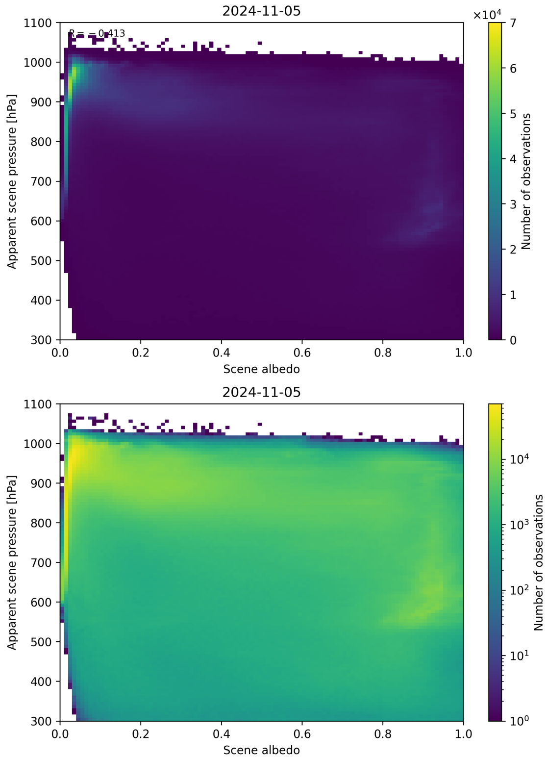
Figure 111: Scatter density plot of “Scene albedo” against “Apparent scene pressure” for 2024-11-04 to 2024-11-06.
