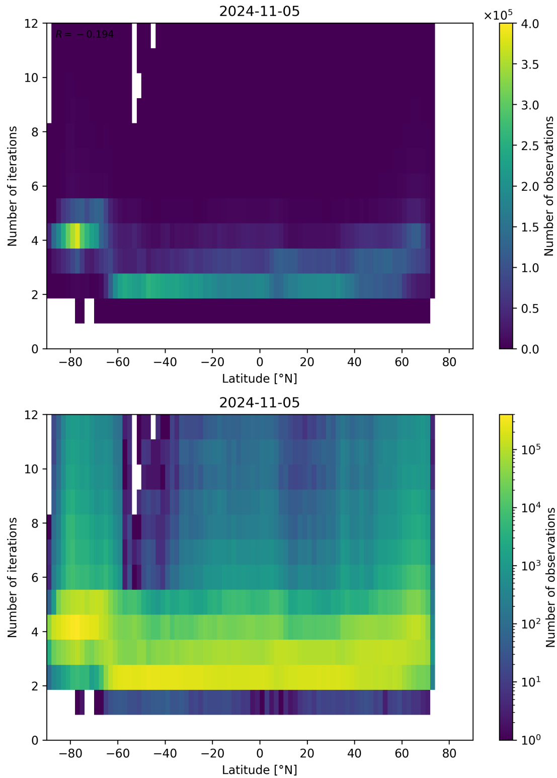
Figure 102: Scatter density plot of “Latitude” against “Number of iterations” for 2024-11-04 to 2024-11-06.
