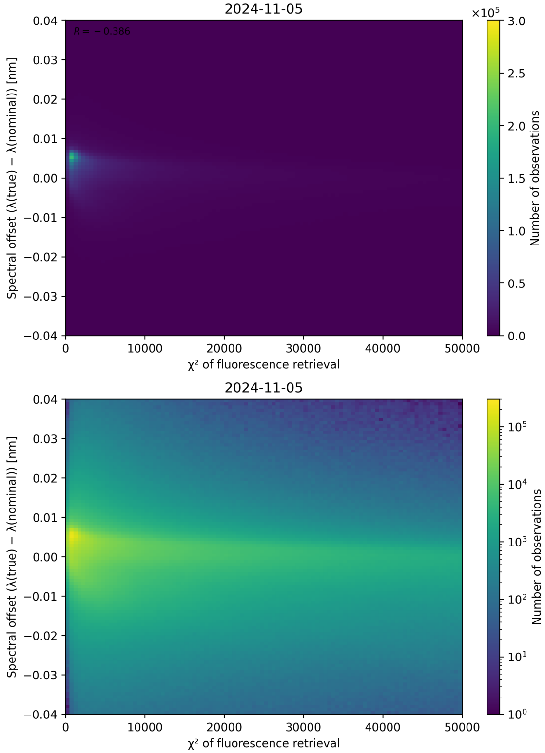
Figure 72: Scatter density plot of “ \chi^2 of fluorescence retrieval” against “Spectral offset ( \lambda_{\text{true}} - \lambda_{\text{nominal}} )” for 2024-11-04 to 2024-11-06.
