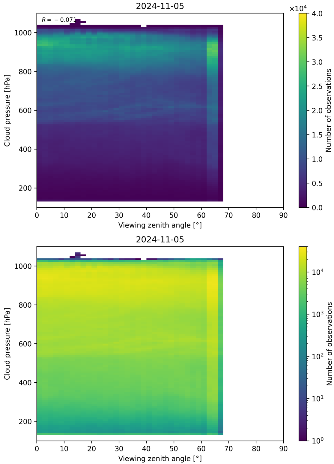
Figure 133: Scatter density plot of “Viewing zenith angle” against “Cloud pressure” for 2024-11-04 to 2024-11-06.
