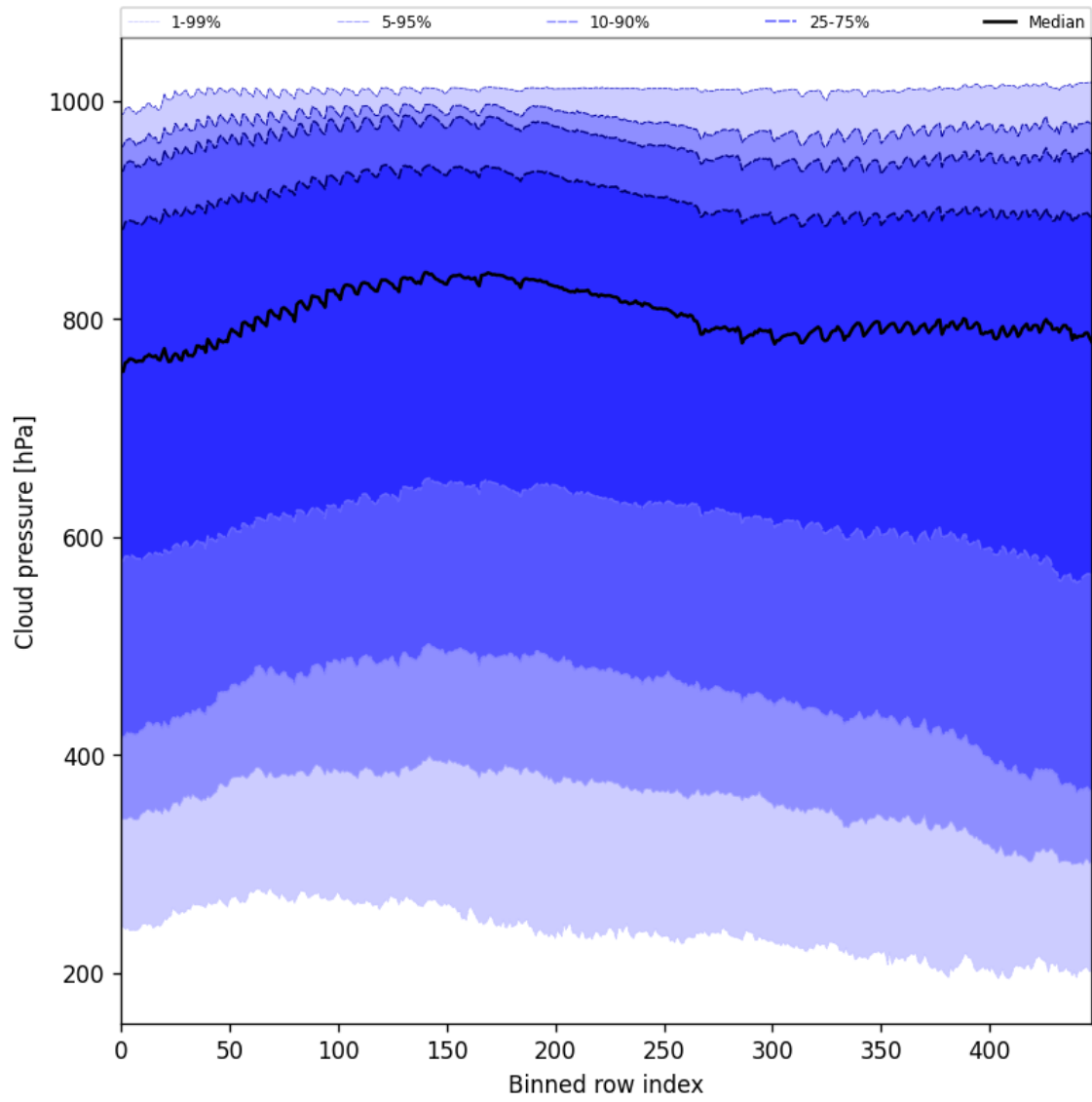
Figure 47: Along track statistics of “Cloud pressure” for 2024-11-04 to 2024-11-06
