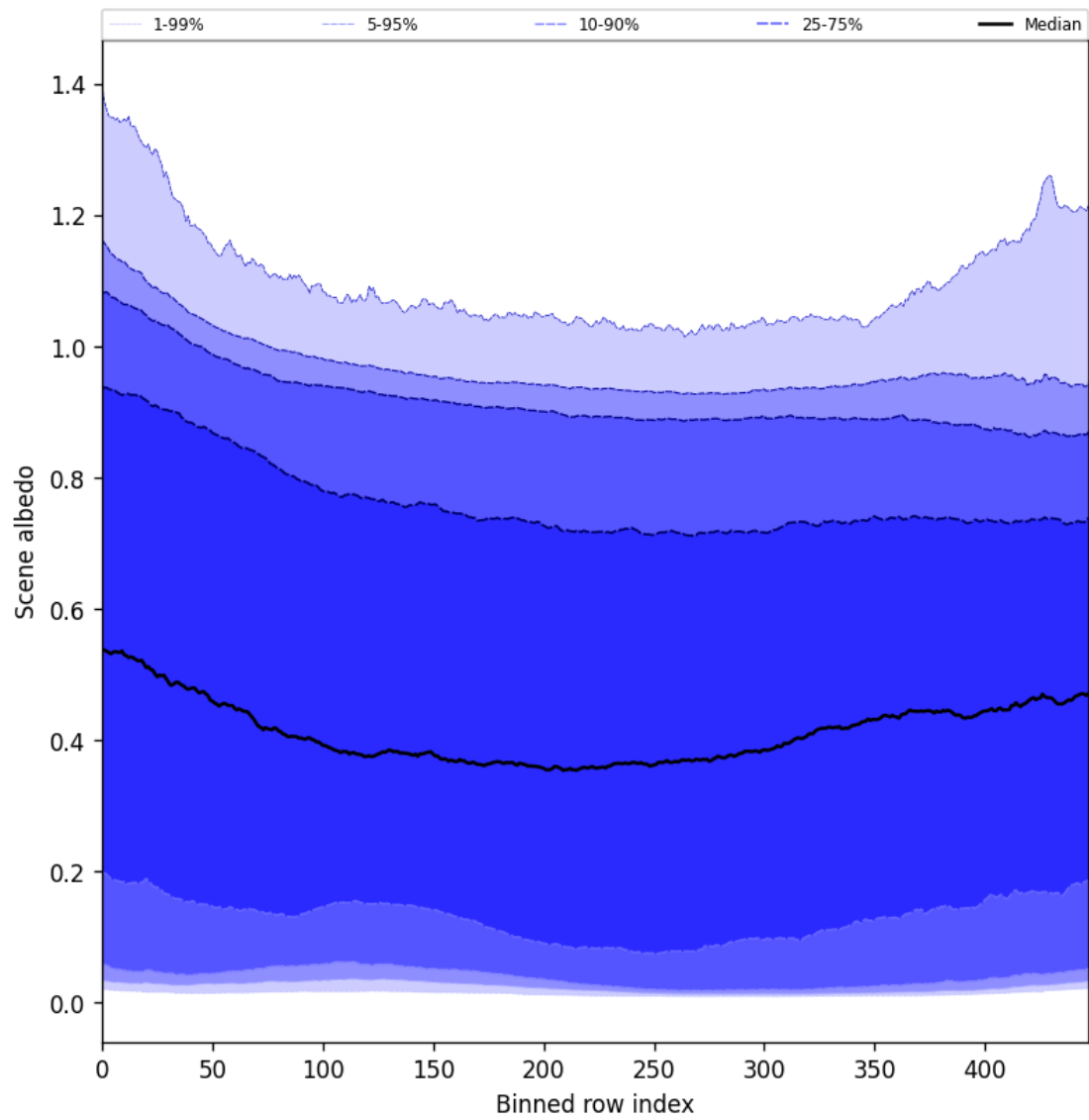
Figure 51: Along track statistics of “Scene albedo” for 2024-11-04 to 2024-11-06
