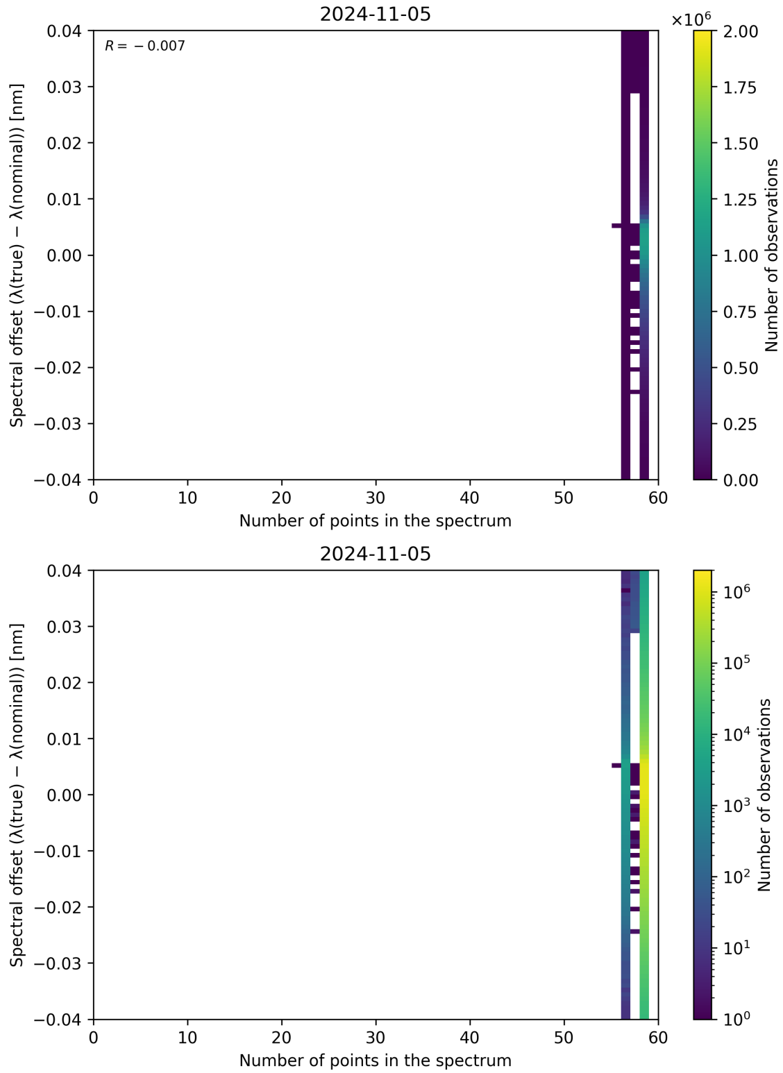
Figure 110: Scatter density plot of “Number of points in the spectrum” against “Spectral offset ( \lambda_{\text{true}} - \lambda_{\text{nominal}} )” for 2024-11-04 to 2024-11-06.
