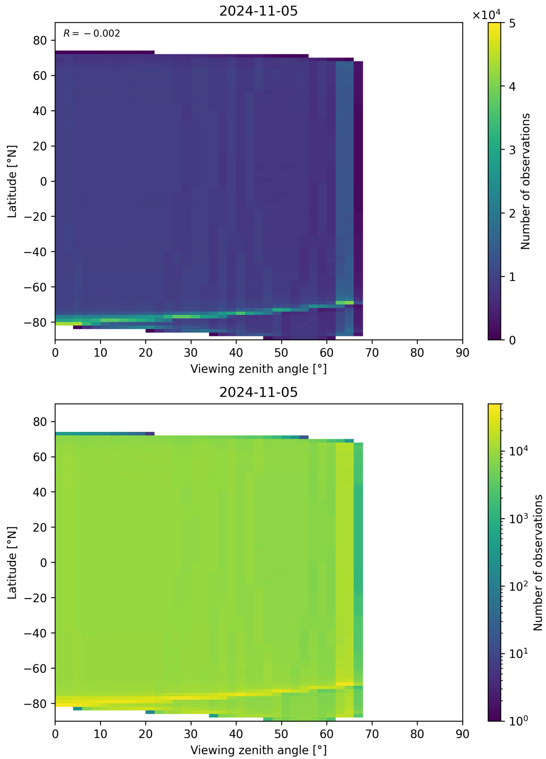
Figure 135: Scatter density plot of “Viewing zenith angle” against “Latitude” for 2024-11-04 to 2024-11-06.
