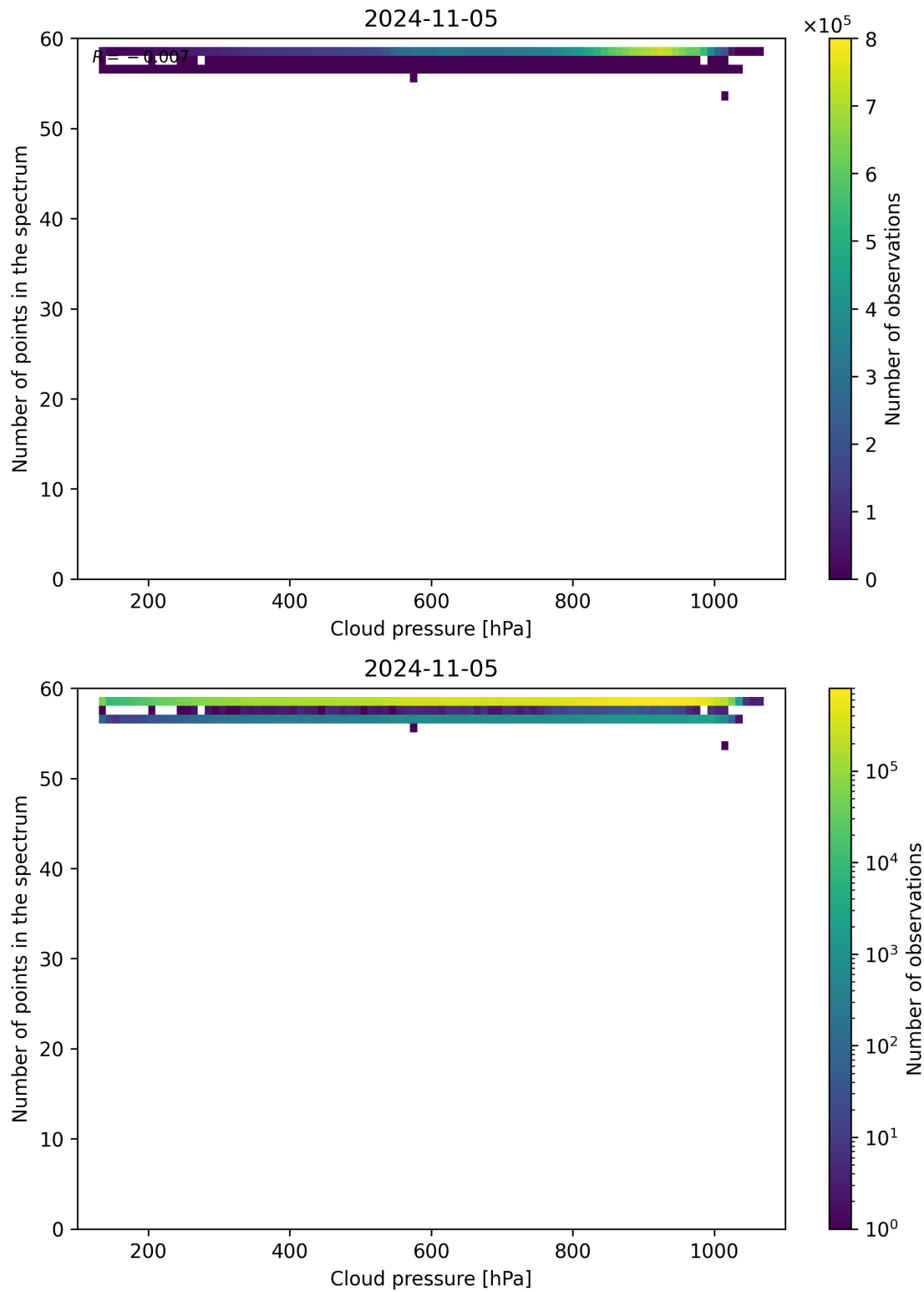
Figure 90: Scatter density plot of “Cloud pressure” against “Number of points in the spectrum” for 2024-11-04 to 2024-11-06.
