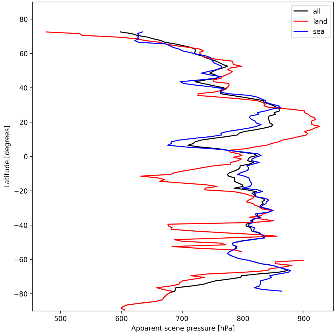
Figure 19: Zonal average of “Apparent scene pressure” for 2024-11-04 to 2024-11-06.
