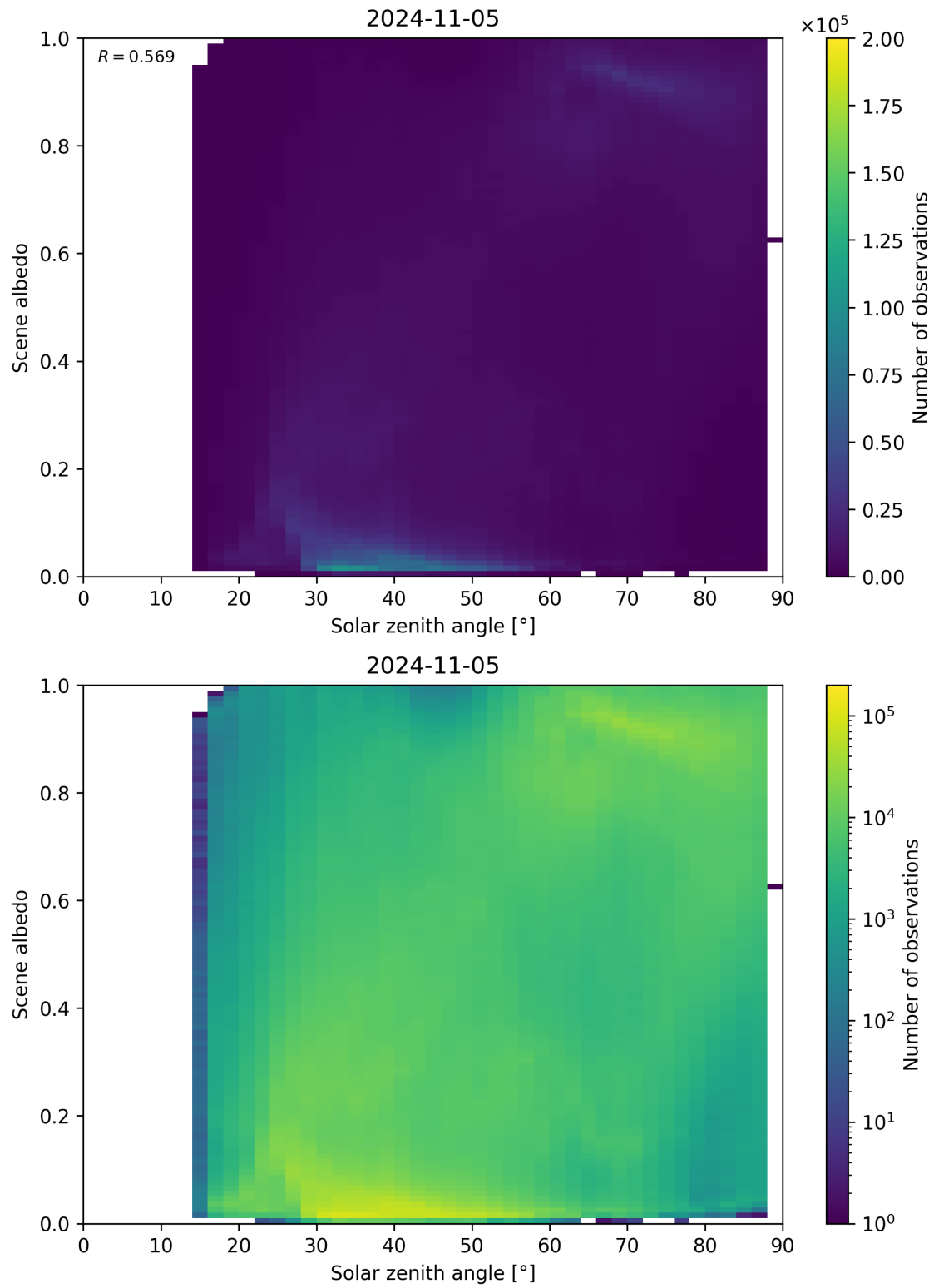
Figure 127: Scatter density plot of “Solar zenith angle” against “Scene albedo” for 2024-11-04 to 2024-11-06.
