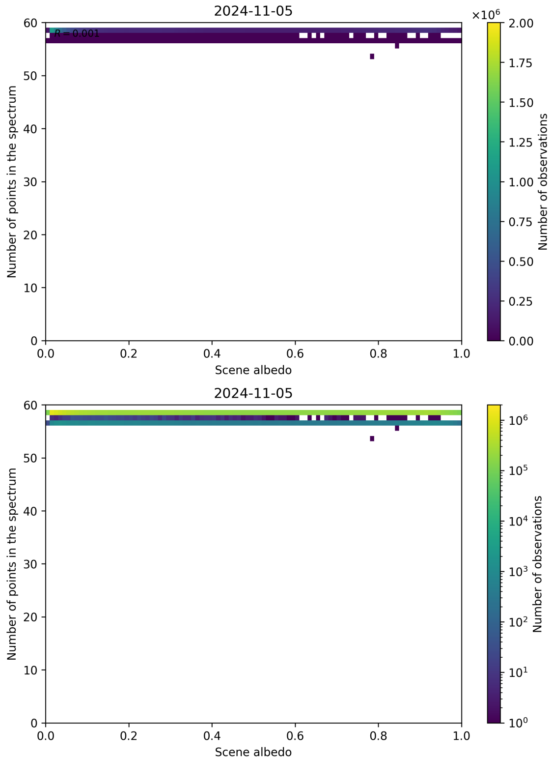
Figure 116: Scatter density plot of “Scene albedo” against “Number of points in the spectrum” for 2024-11-04 to 2024-11-06.
