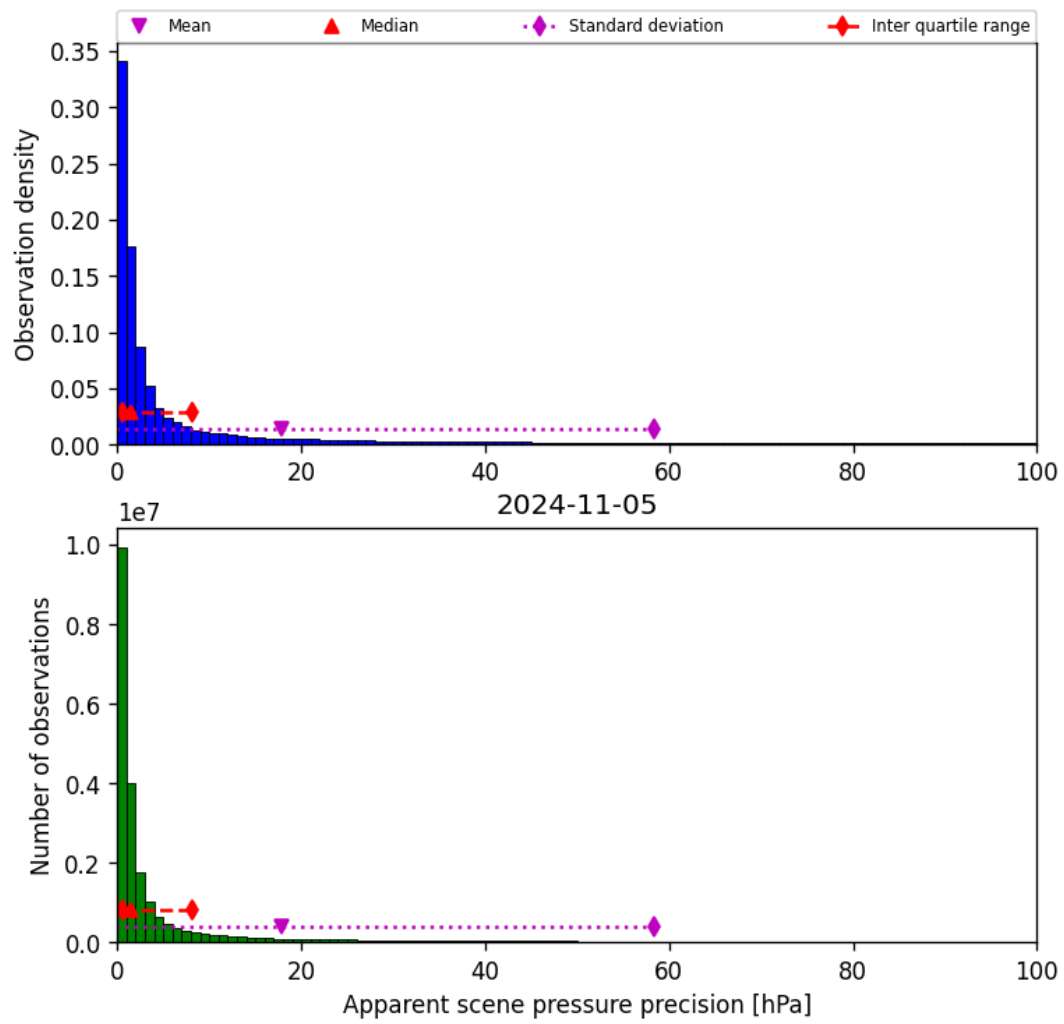
Figure 37: Histogram of “Apparent scene pressure precision” for 2024-11-04 to 2024-11-06
