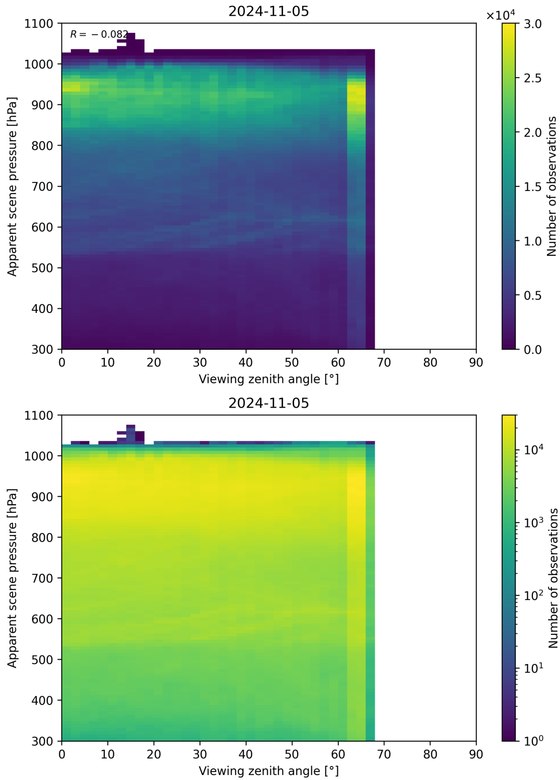
Figure 129: Scatter density plot of “Viewing zenith angle” against “Apparent scene pressure” for 2024-11-04 to 2024-11-06.
