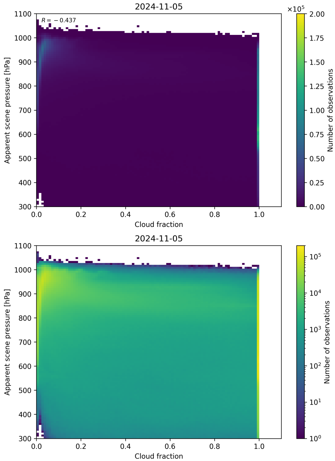
Figure 76: Scatter density plot of “Cloud fraction” against “Apparent scene pressure” for 2024-11-04 to 2024-11-06.
