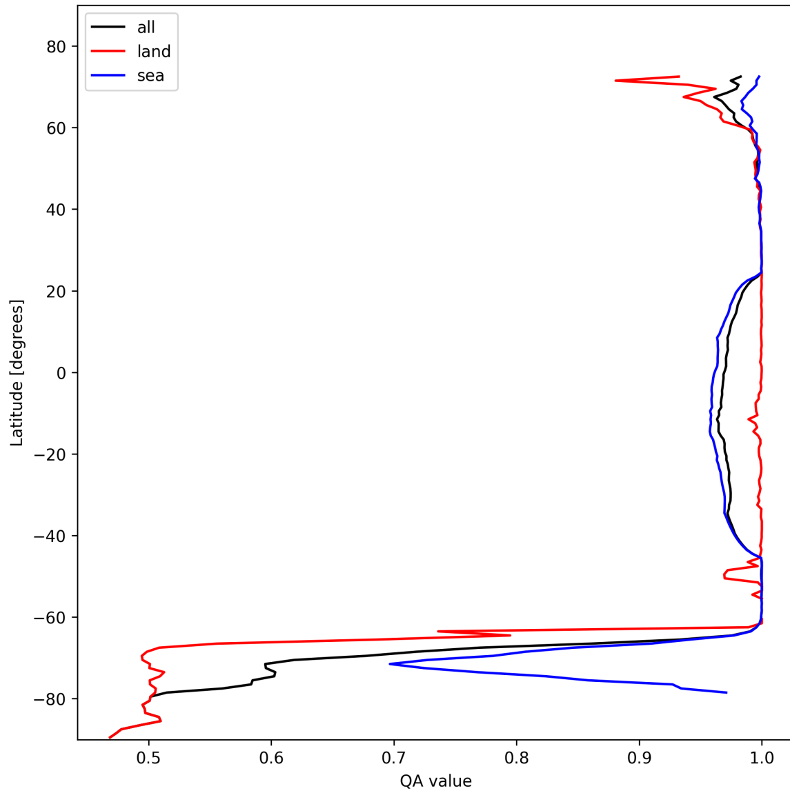
Figure 12: Zonal average of “QA value” for 2024-11-04 to 2024-11-06.
