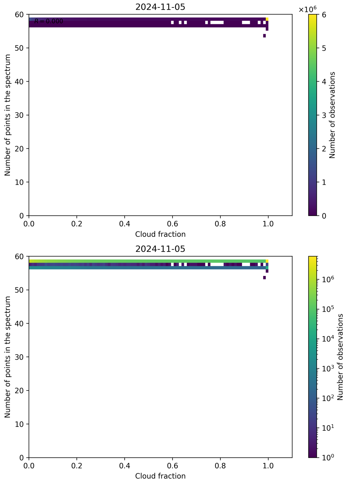
Figure 81: Scatter density plot of “Cloud fraction” against “Number of points in the spectrum” for 2024-11-04 to 2024-11-06.
