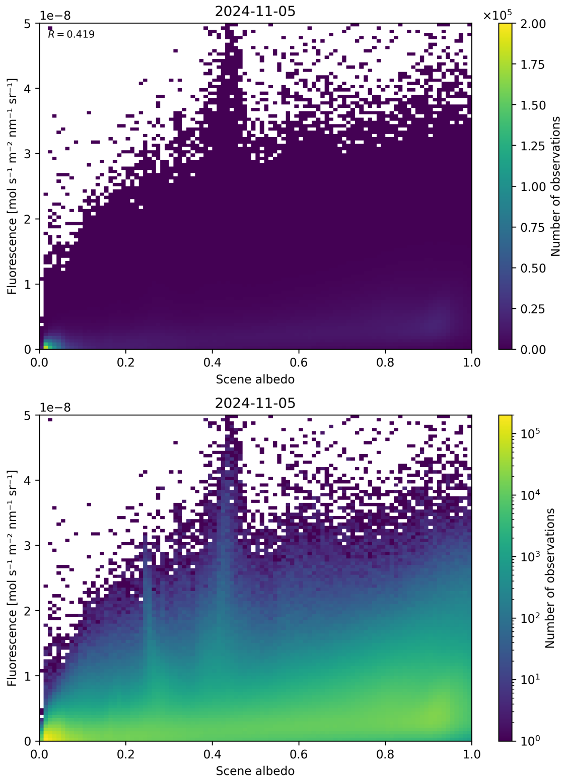
Figure 114: Scatter density plot of “Scene albedo” against “Fluorescence” for 2024-11-04 to 2024-11-06.
