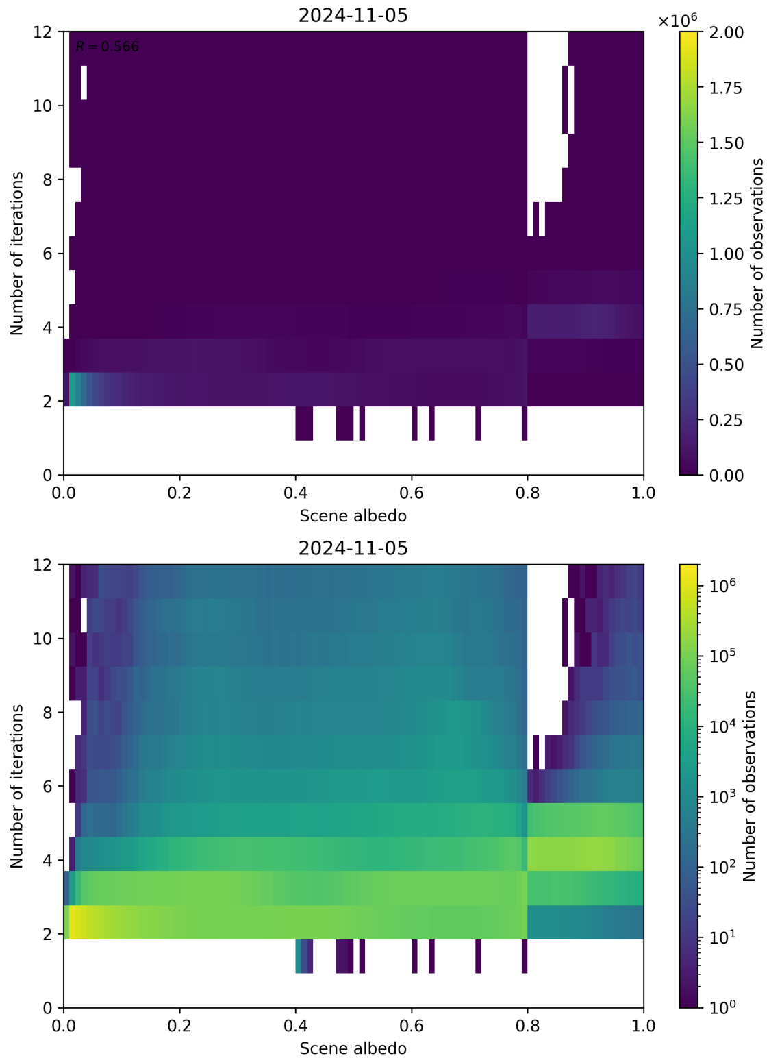
Figure 115: Scatter density plot of “Scene albedo” against “Number of iterations” for 2024-11-04 to 2024-11-06.
