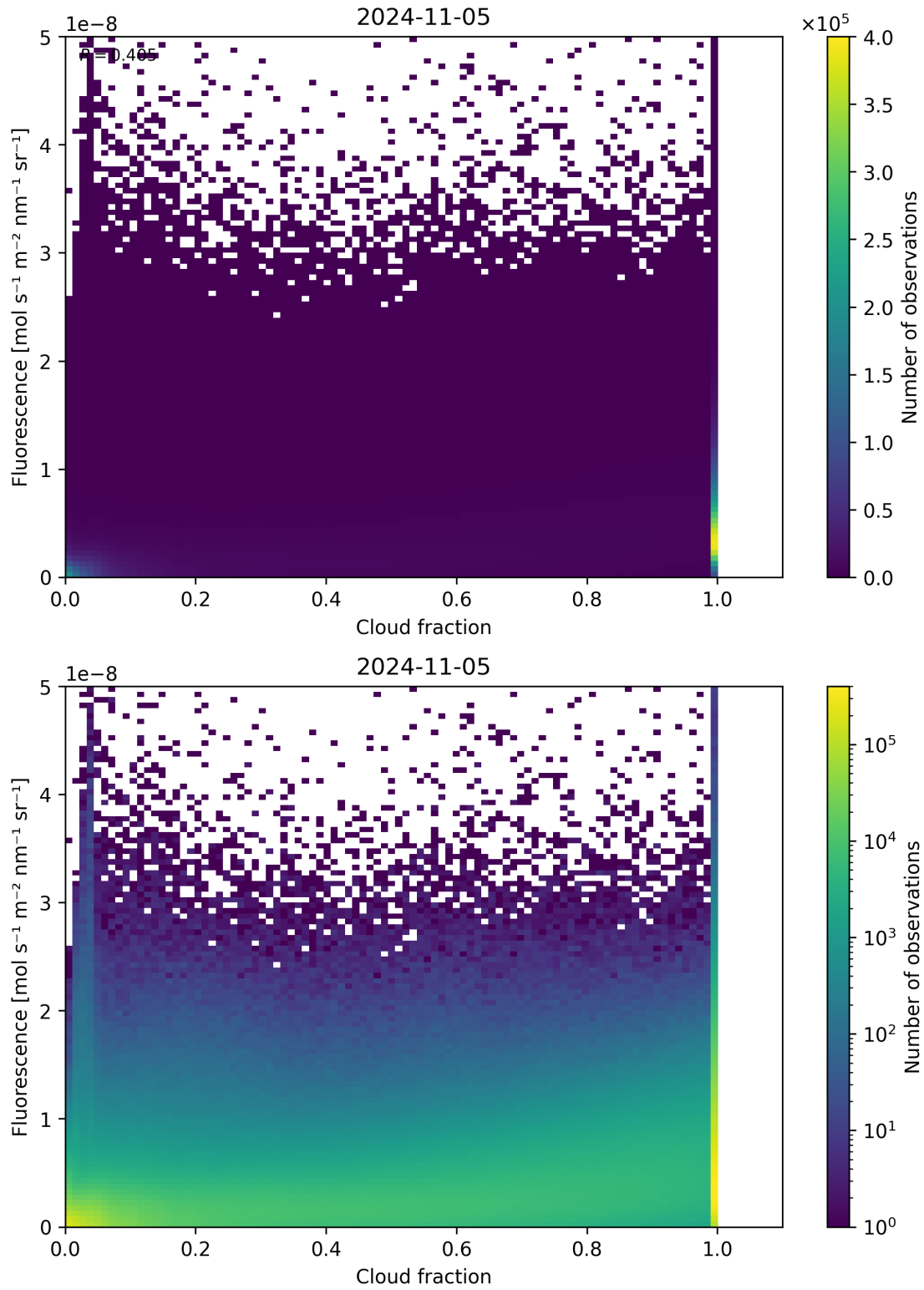
Figure 79: Scatter density plot of “Cloud fraction” against “Fluorescence” for 2024-11-04 to 2024-11-06.
