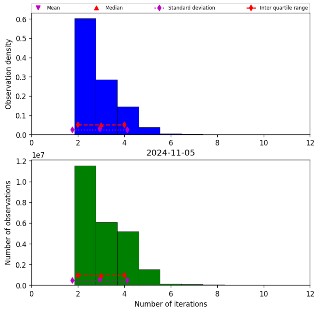
Figure 39: Histogram of “Number of iterations” for 2024-11-04 to 2024-11-06
