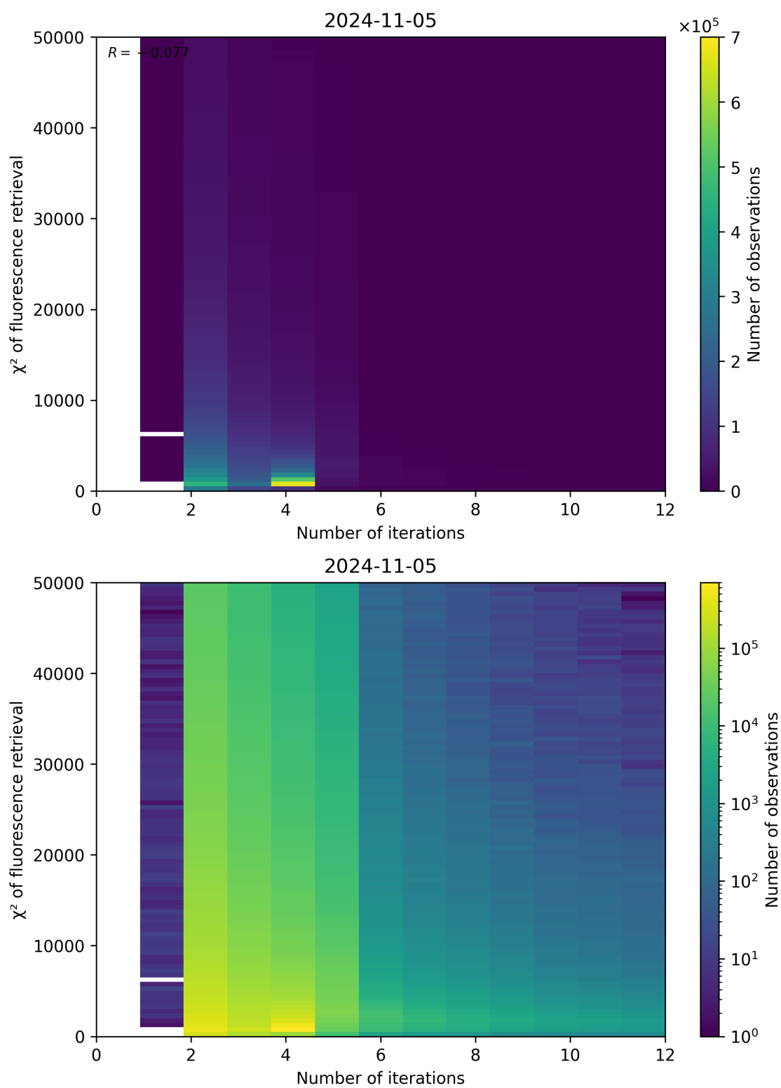
Figure 106: Scatter density plot of “Number of iterations” against “ \chi^2 of fluorescence retrieval” for 2024-11-04 to 2024-11-06.
