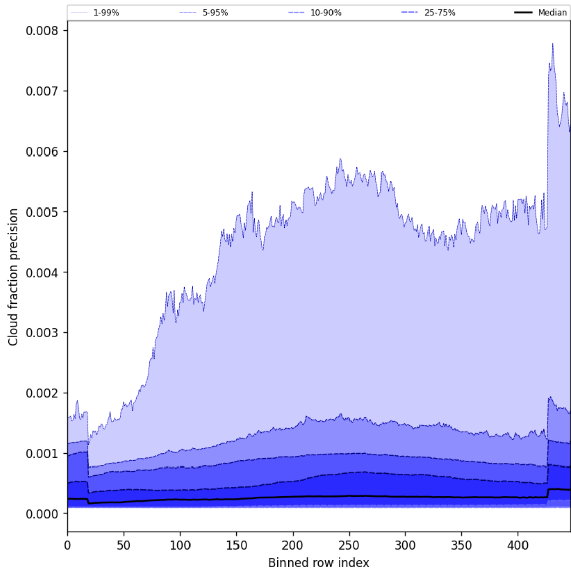
Figure 50: Along track statistics of “Cloud fraction precision” for 2024-11-04 to 2024-11-06
