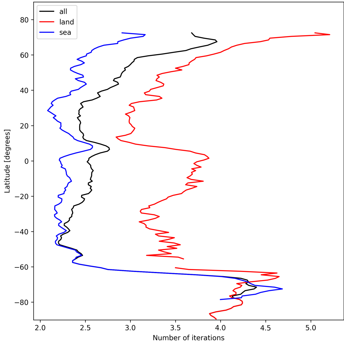
Figure 22: Zonal average of “Number of iterations” for 2024-11-04 to 2024-11-06.
