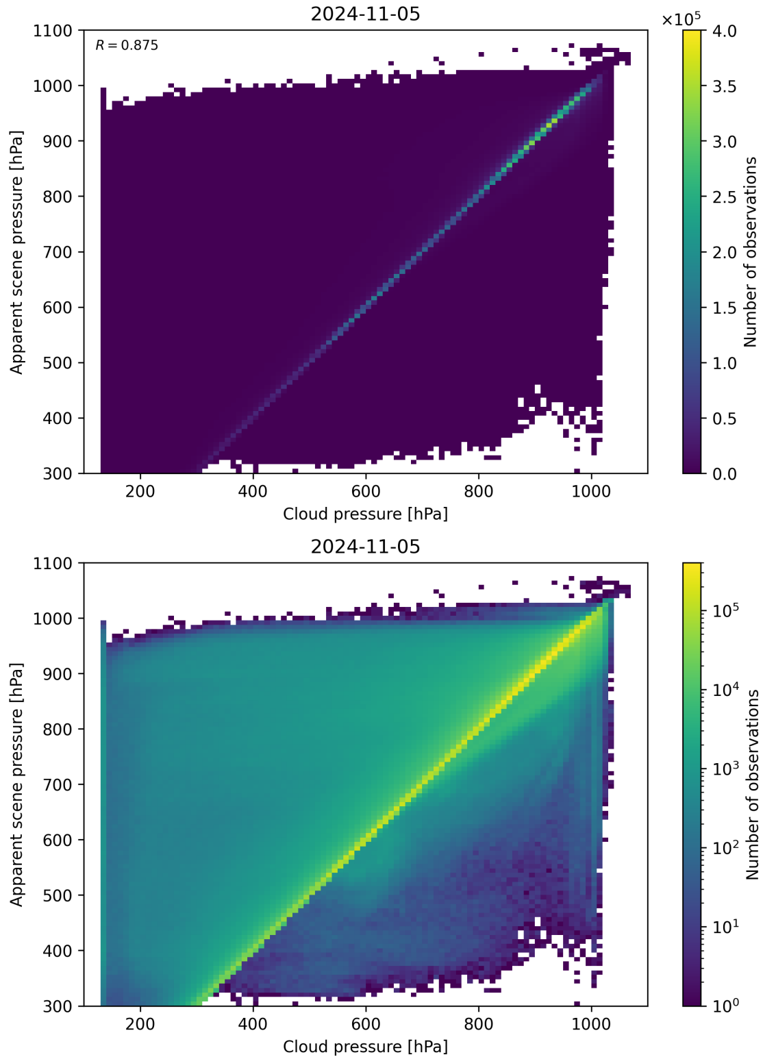
Figure 84: Scatter density plot of “Cloud pressure” against “Apparent scene pressure” for 2024-11-04 to 2024-11-06.
