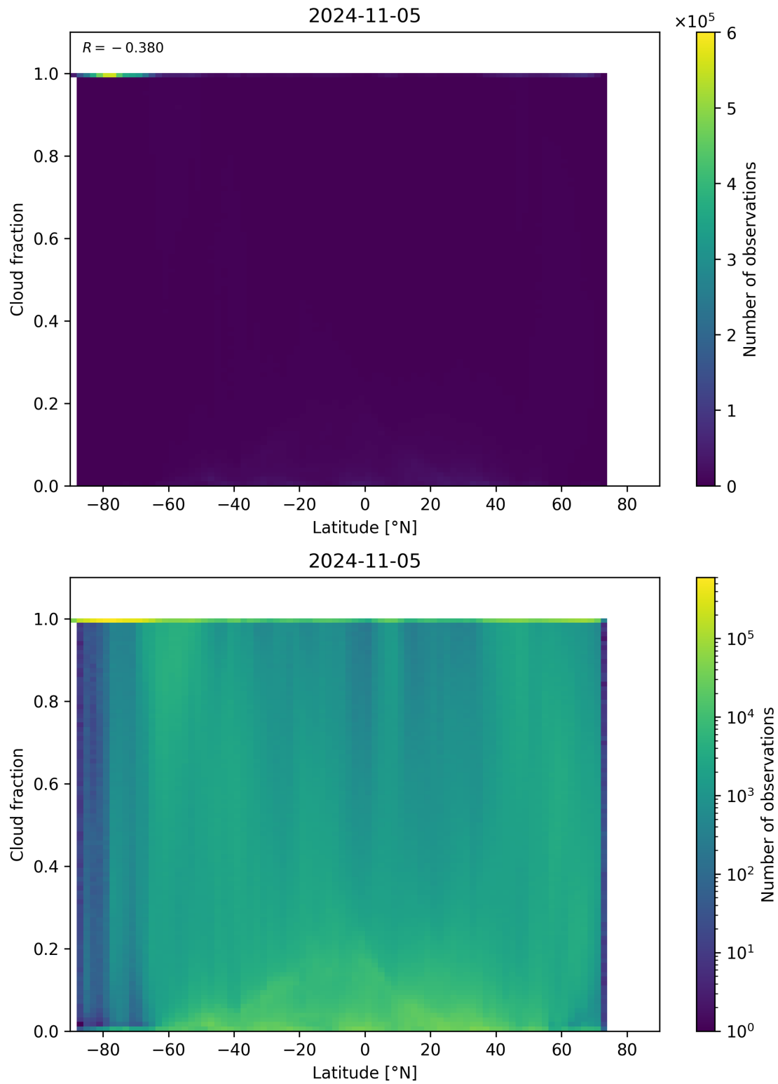
Figure 99: Scatter density plot of “Latitude” against “Cloud fraction” for 2024-11-04 to 2024-11-06.
