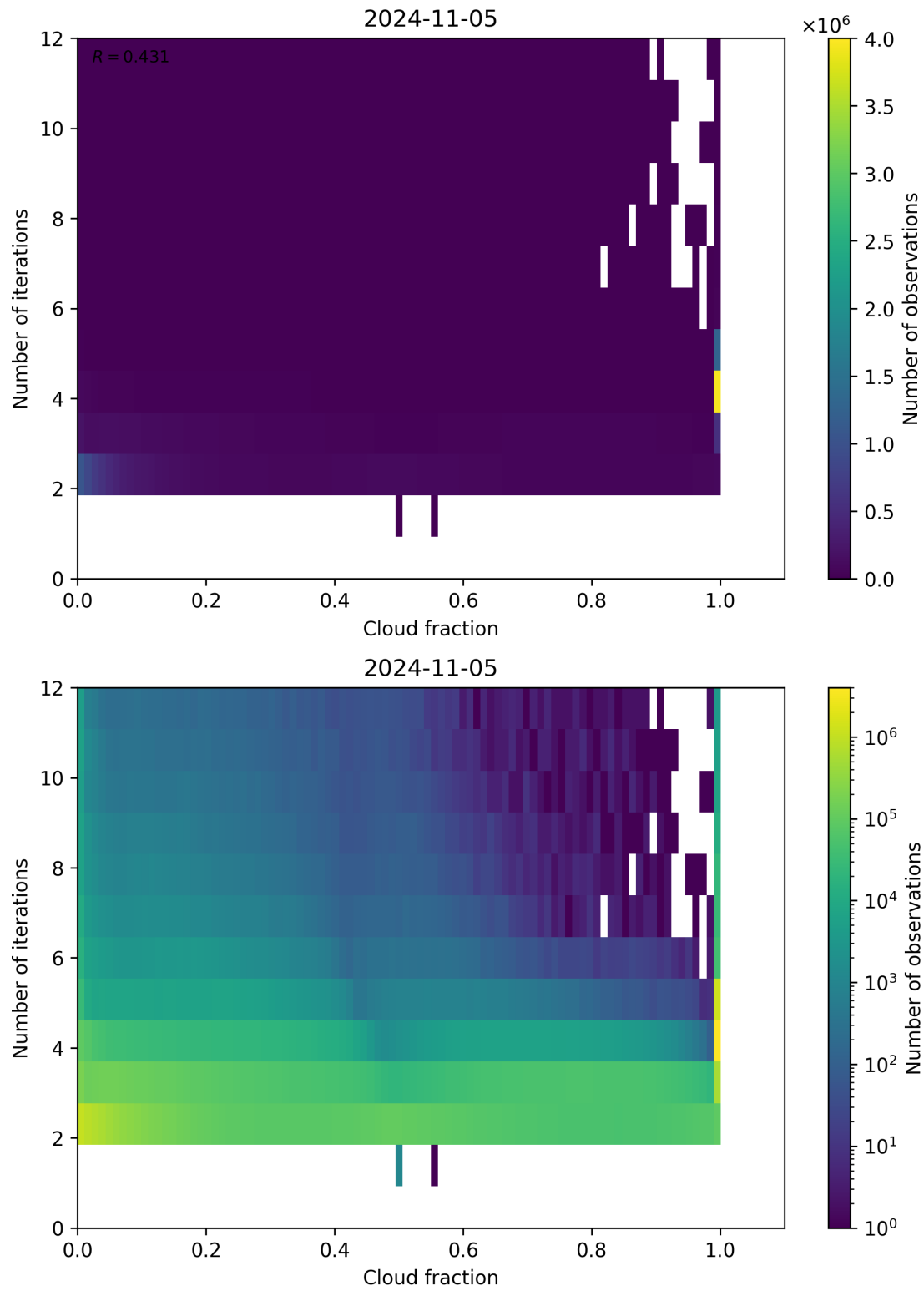
Figure 80: Scatter density plot of “Cloud fraction” against “Number of iterations” for 2024-11-04 to 2024-11-06.
