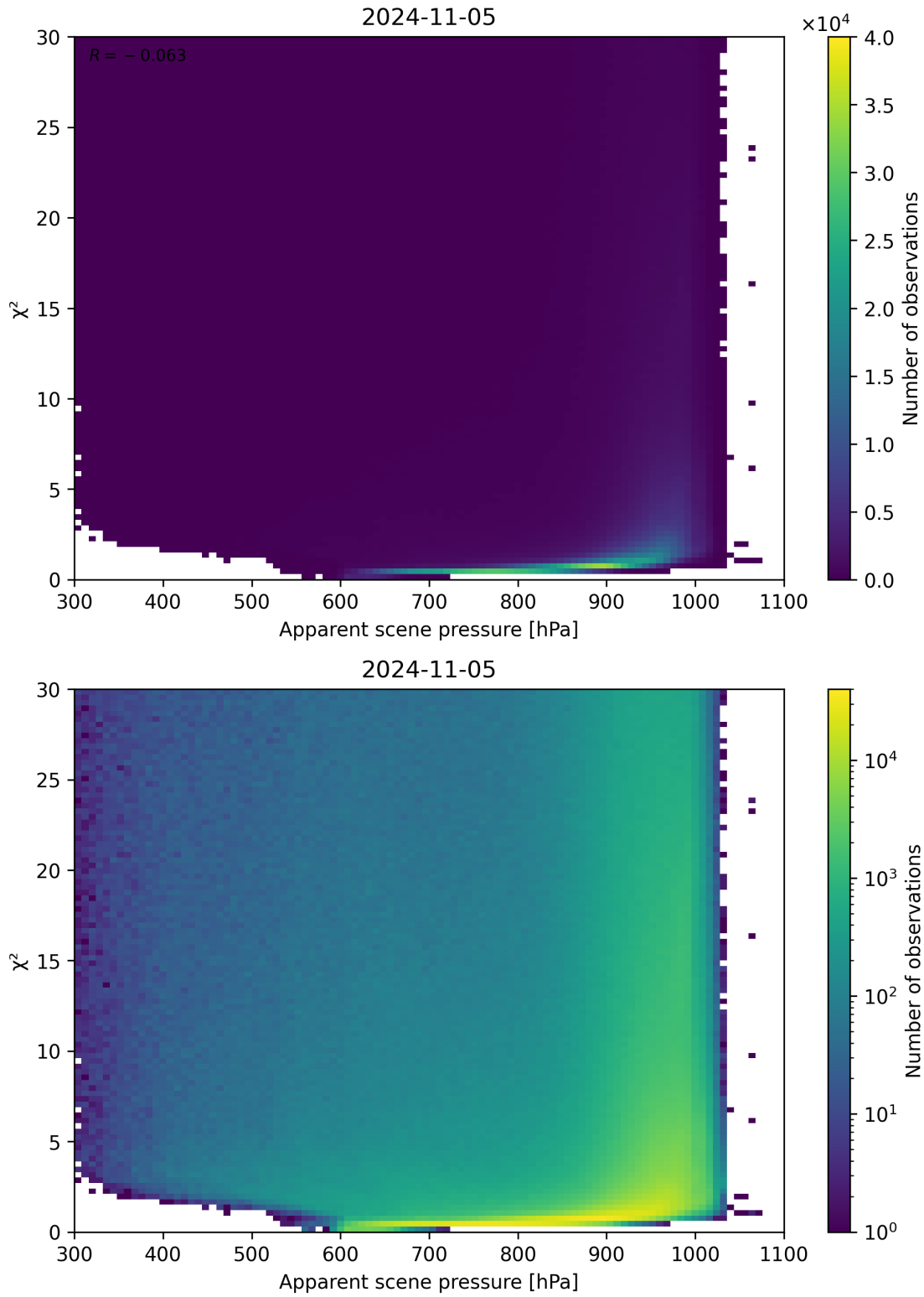
Figure 63: Scatter density plot of “Apparent scene pressure” against “ \chi^2 ” for 2024-11-04 to 2024-11-06.
