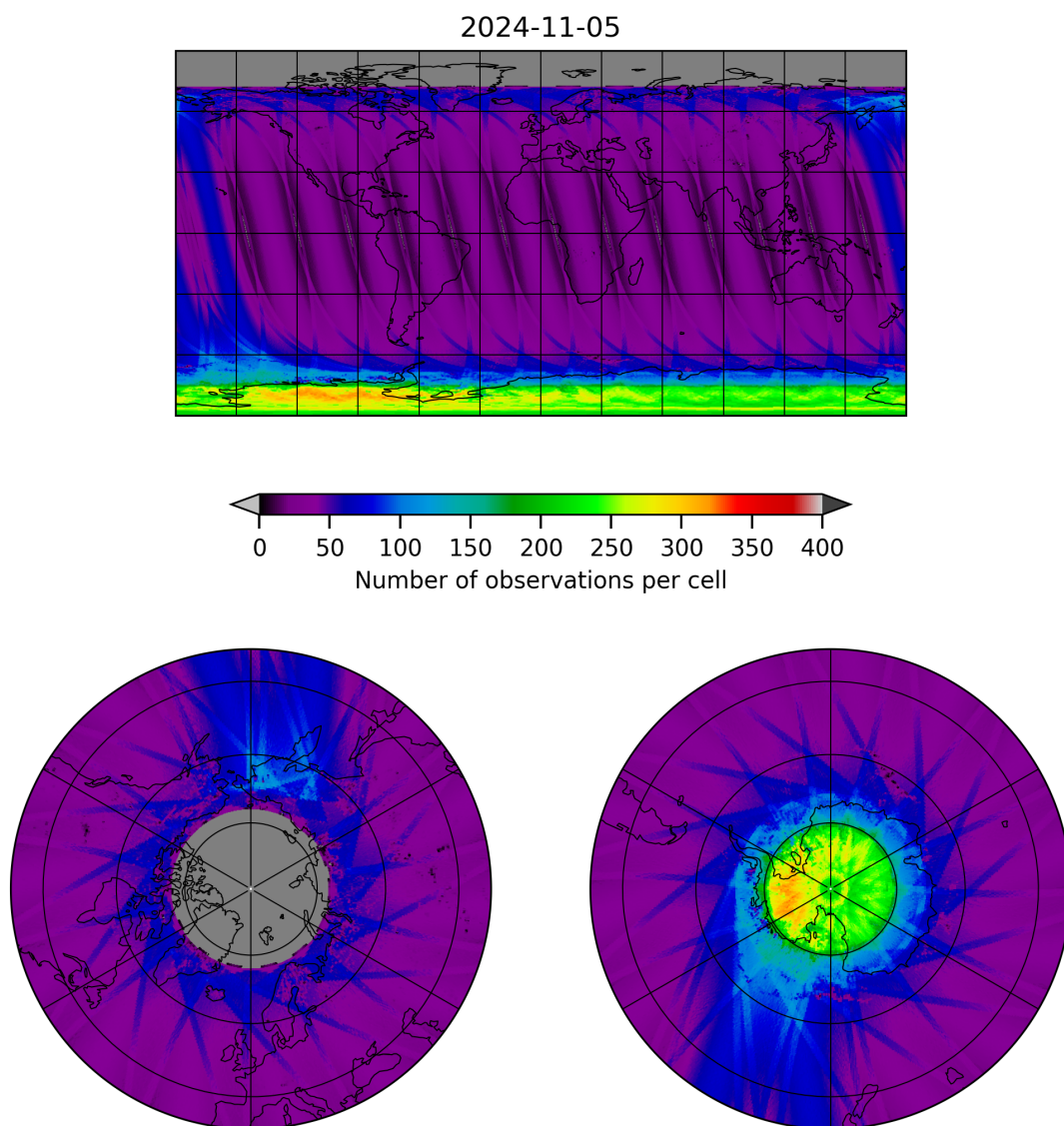
Figure 11: Map of the number of observations for 2024-11-04 to 2024-11-06
