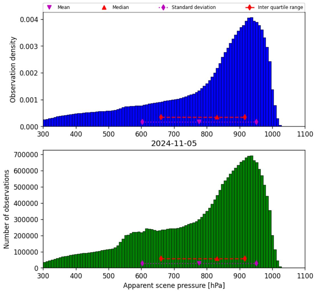
Figure 36: Histogram of “Apparent scene pressure” for 2024-11-04 to 2024-11-06
