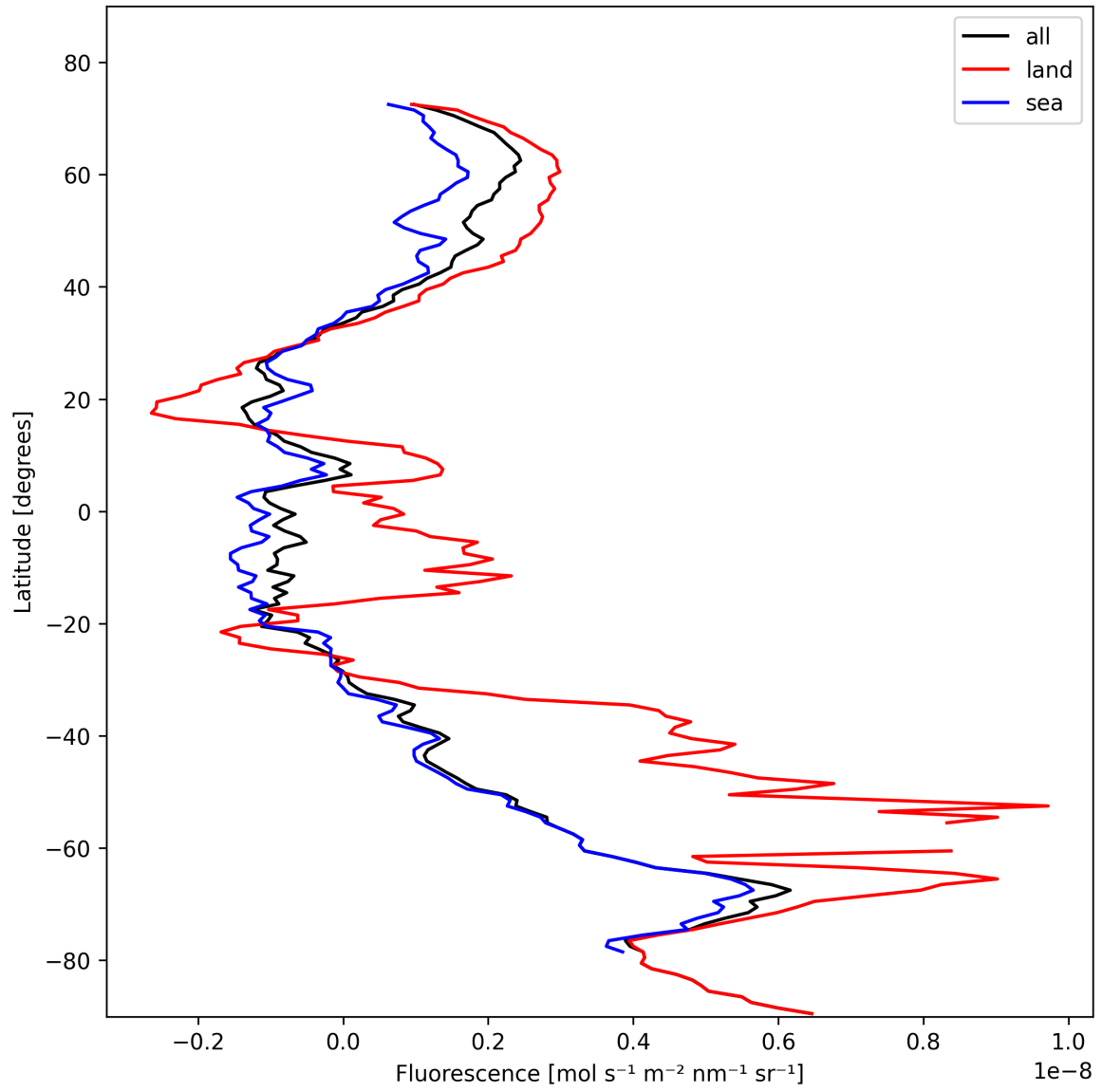
Figure 23: Zonal average of “Fluorescence” for 2024-11-04 to 2024-11-06.
