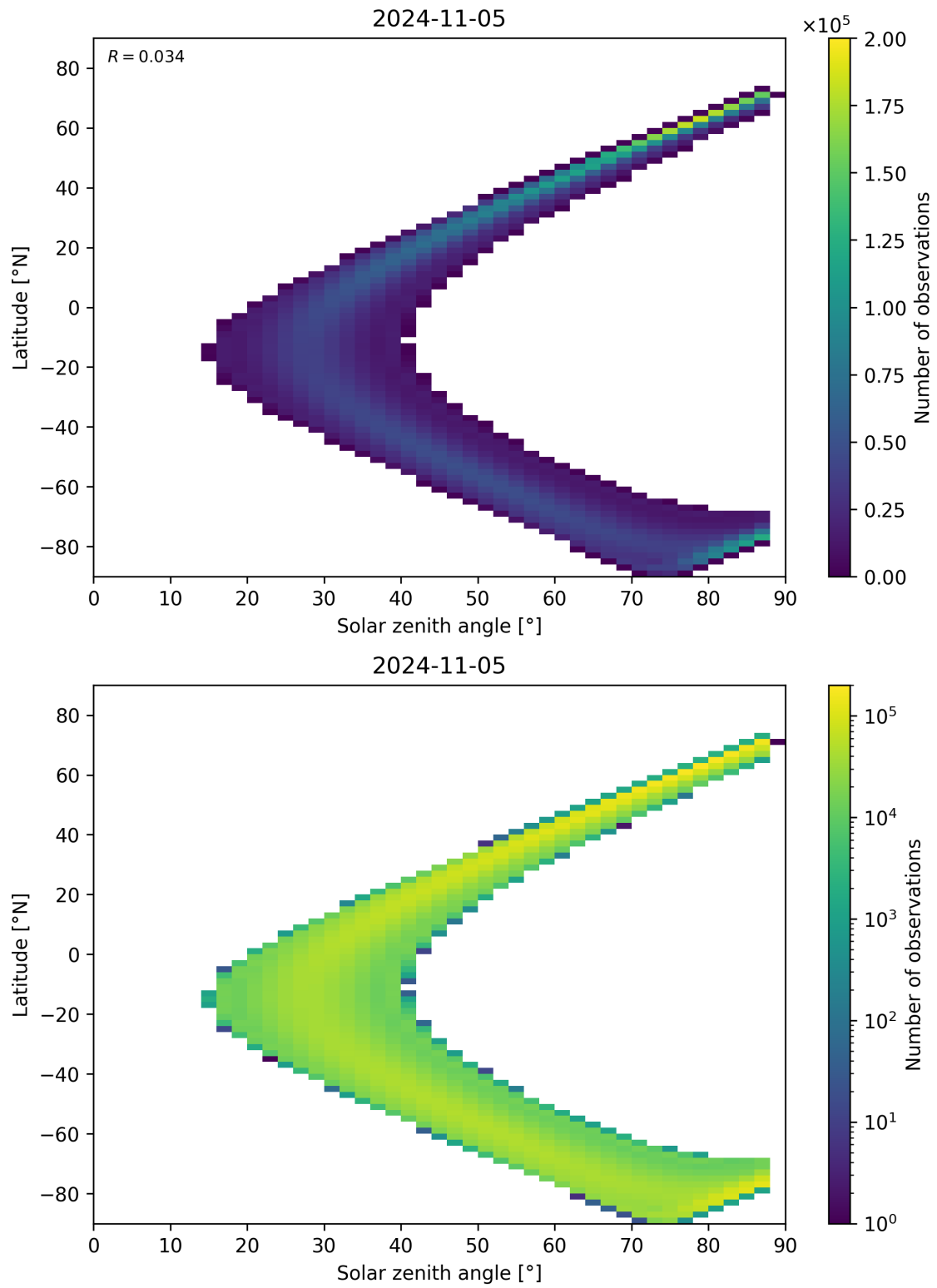
Figure 124: Scatter density plot of “Solar zenith angle” against “Latitude” for 2024-11-04 to 2024-11-06.
