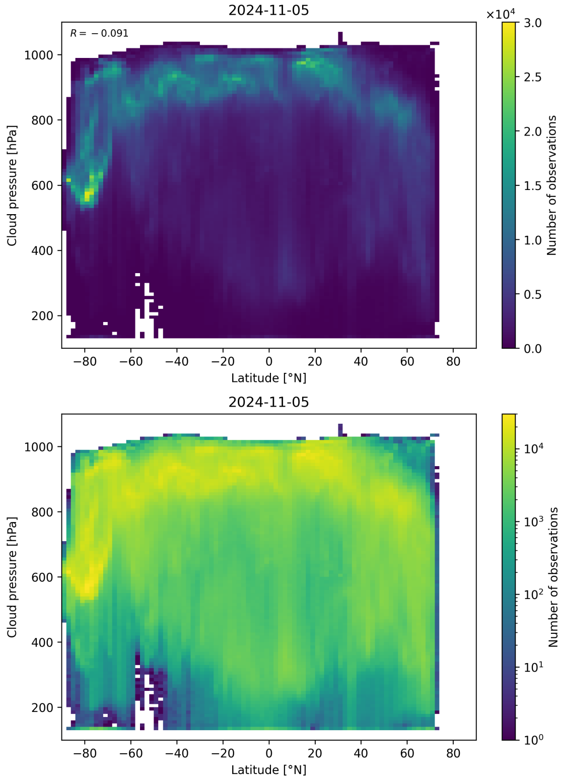
Figure 100: Scatter density plot of “Latitude” against “Cloud pressure” for 2024-11-04 to 2024-11-06.
