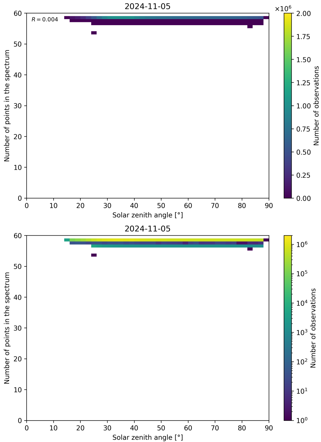
Figure 126: Scatter density plot of “Solar zenith angle” against “Number of points in the spectrum” for 2024-11-04 to 2024-11-06.
