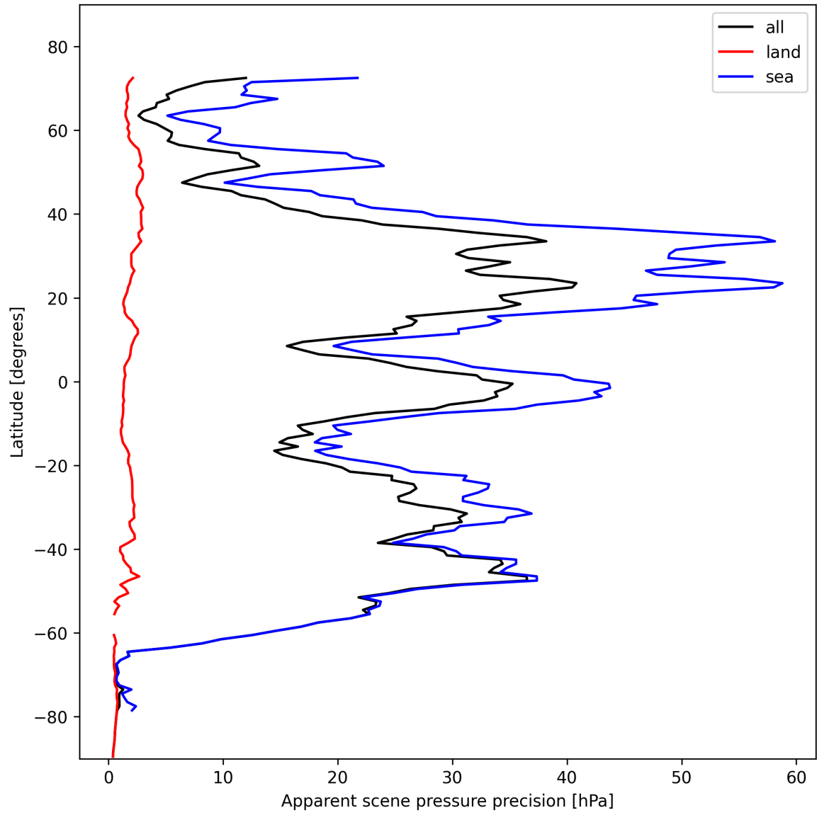
Figure 20: Zonal average of “Apparent scene pressure precision” for 2024-11-04 to 2024-11-06.
