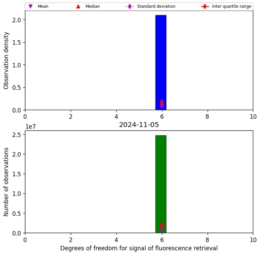
Figure 43: Histogram of "Degrees of freedom for signal of fluorescence retrieval" for 2024-11-04 to 2024-11-06
