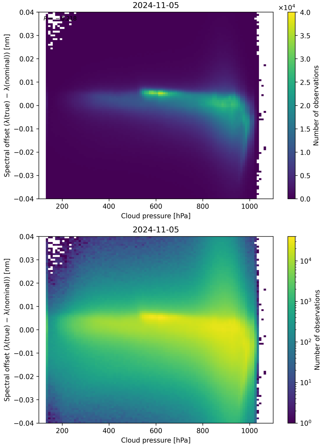
Figure 92: Scatter density plot of “Cloud pressure” against “Spectral offset ( \lambda_{\text{true}} - \lambda_{\text{nominal}} )” for 2024-11-04 to 2024-11-06.
