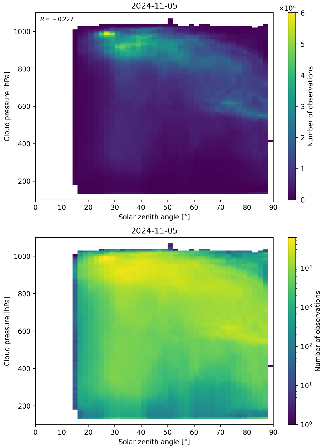
Figure 122: Scatter density plot of “Solar zenith angle” against “Cloud pressure” for 2024-11-04 to 2024-11-06.
