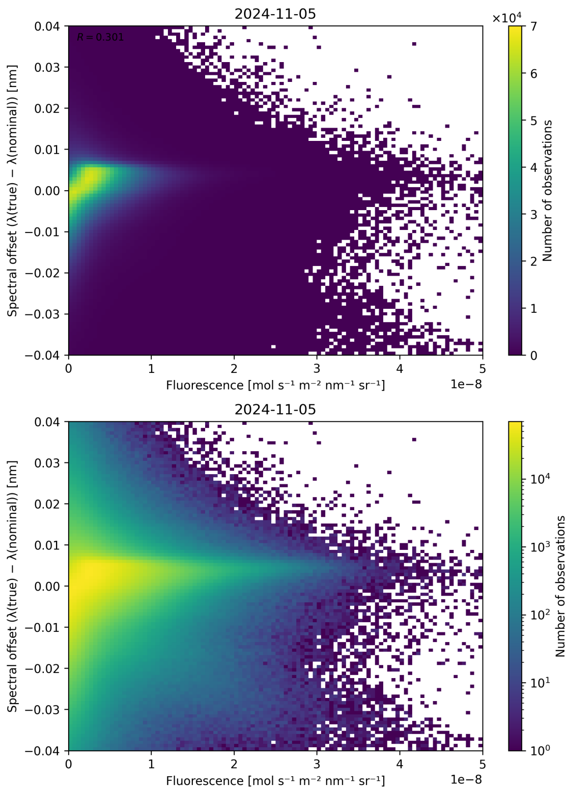
Figure 95: Scatter density plot of “Fluorescence” against “Spectral offset ( \lambda_{\text{true}} - \lambda_{\text{nominal}} )” for 2024-11-04 to 2024-11-06.
