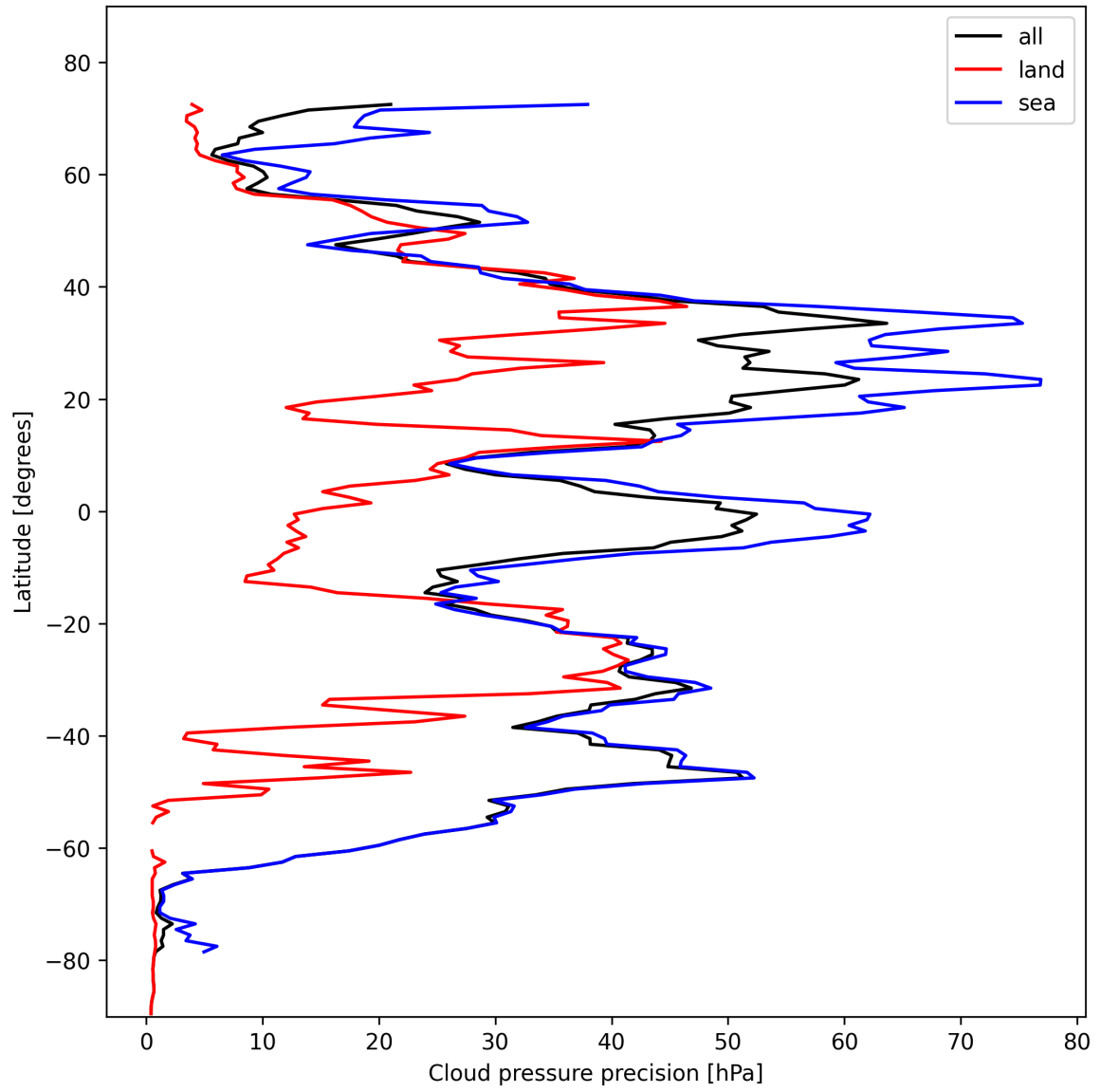
Figure 14: Zonal average of “Cloud pressure precision” for 2024-11-04 to 2024-11-06.
