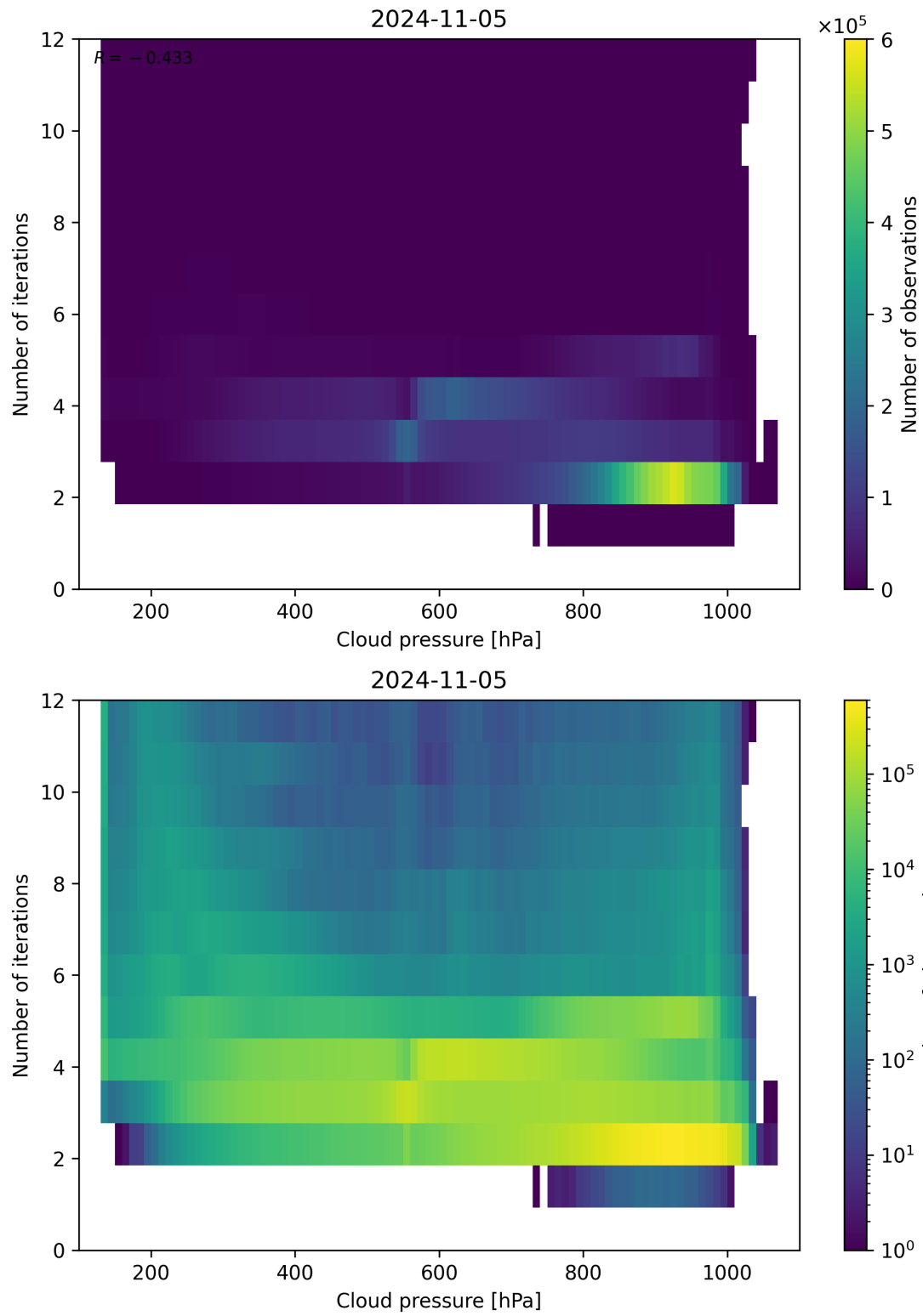
Figure 89: Scatter density plot of “Cloud pressure” against “Number of iterations” for 2024-11-04 to 2024-11-06.
