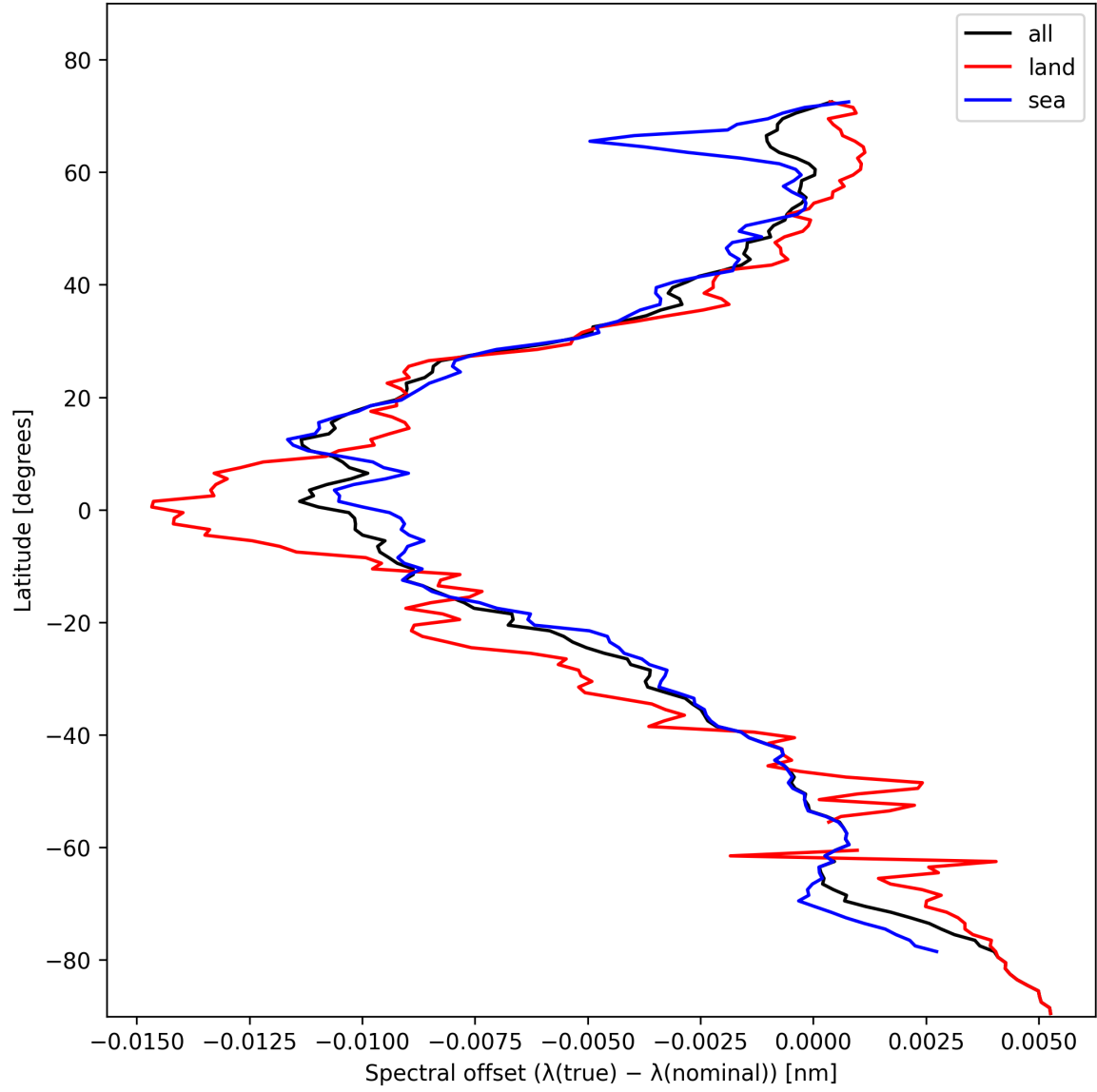
Figure 28: Zonal average of “Spectral offset ( \lambda_{\text{true}} - \lambda_{\text{nominal}} )” for 2024-11-04 to 2024-11-06.
