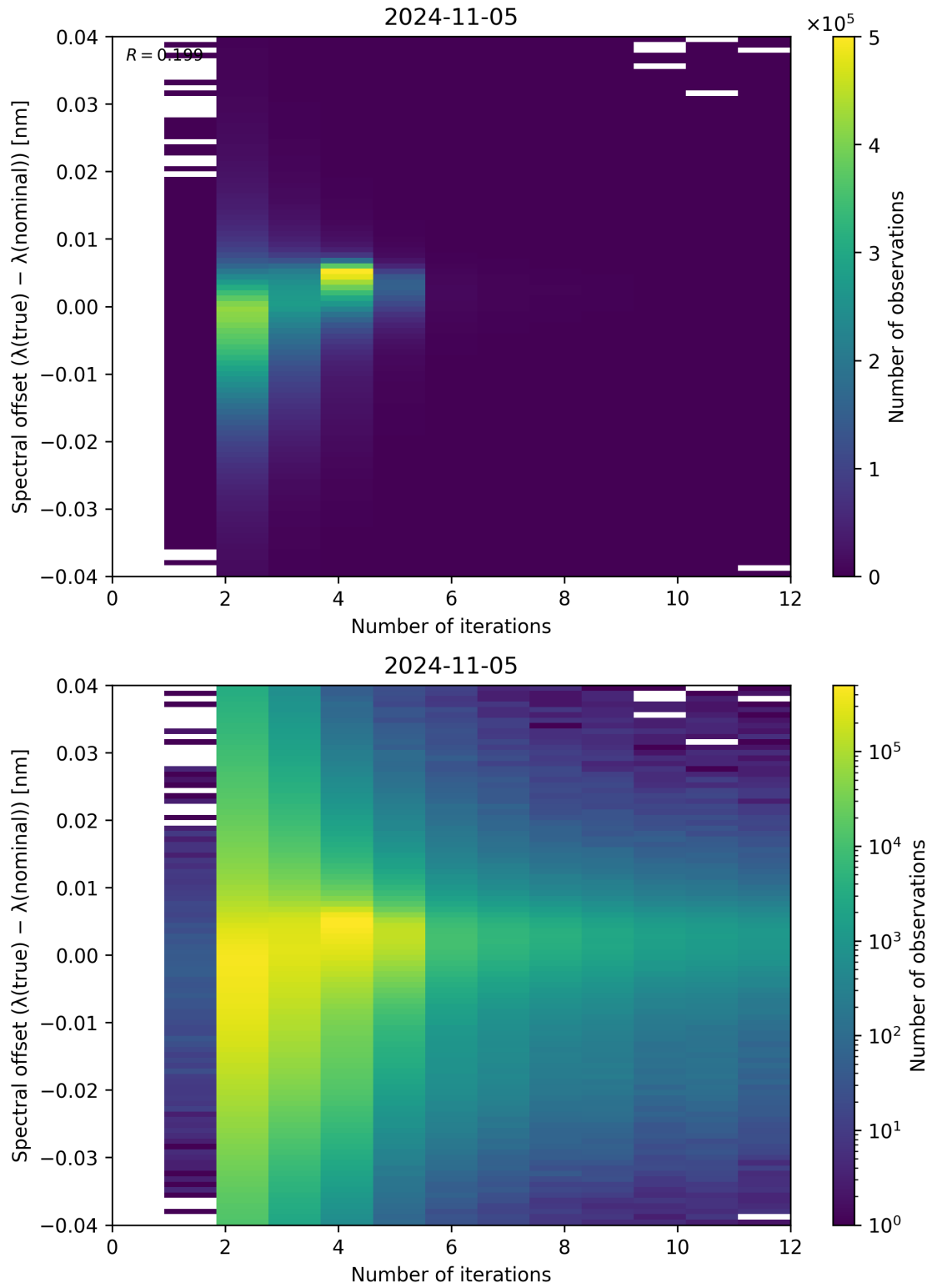
Figure 109: Scatter density plot of “Number of iterations” against “Spectral offset ( \lambda_{\text{true}} - \lambda_{\text{nominal}} )” for 2024-11-04 to 2024-11-06.
