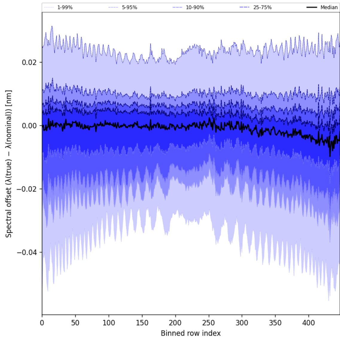
Figure 62: Along track statistics of “Spectral offset ( \lambda_{\text{true}} - \lambda_{\text{nominal}} )” for 2024-11-04 to 2024-11-06
