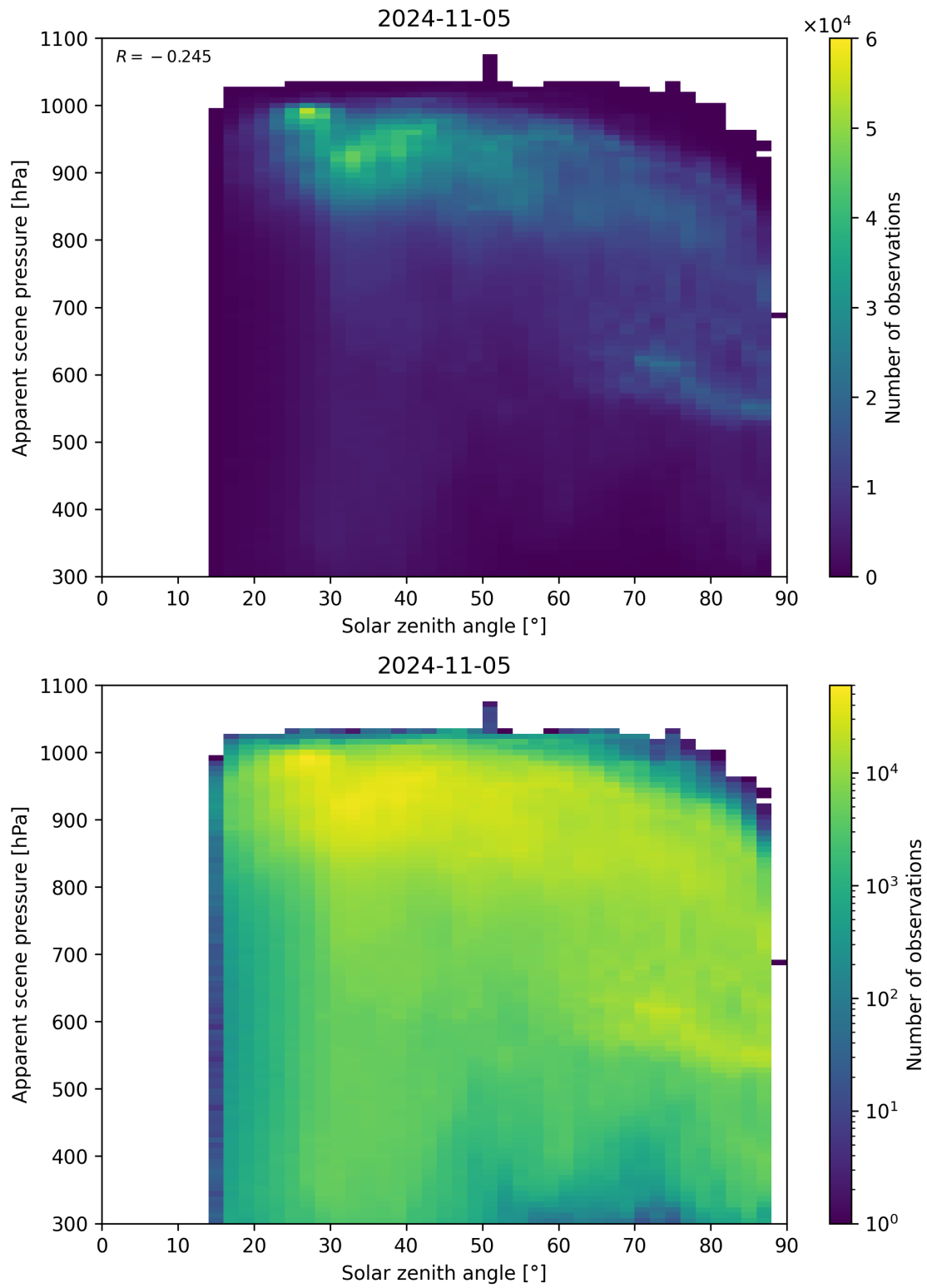
Figure 118: Scatter density plot of “Solar zenith angle” against “Apparent scene pressure” for 2024-11-04 to 2024-11-06.
