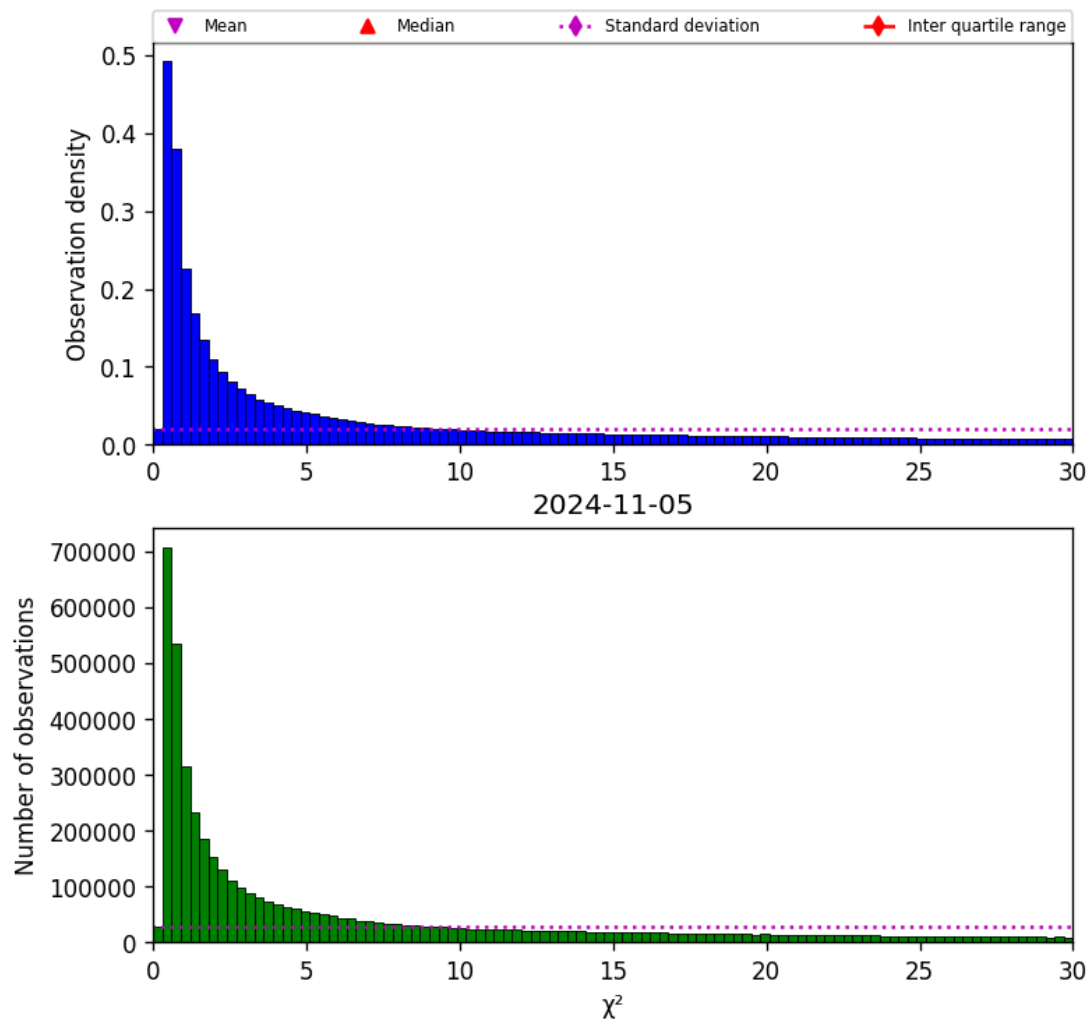
Figure 38: Histogram of " \chi^2 " for 2024-11-04 to 2024-11-06
