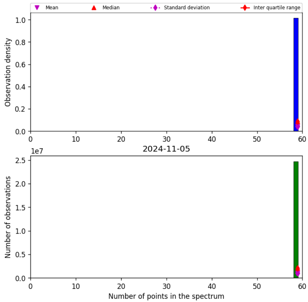
Figure 44: Histogram of “Number of points in the spectrum” for 2024-11-04 to 2024-11-06
