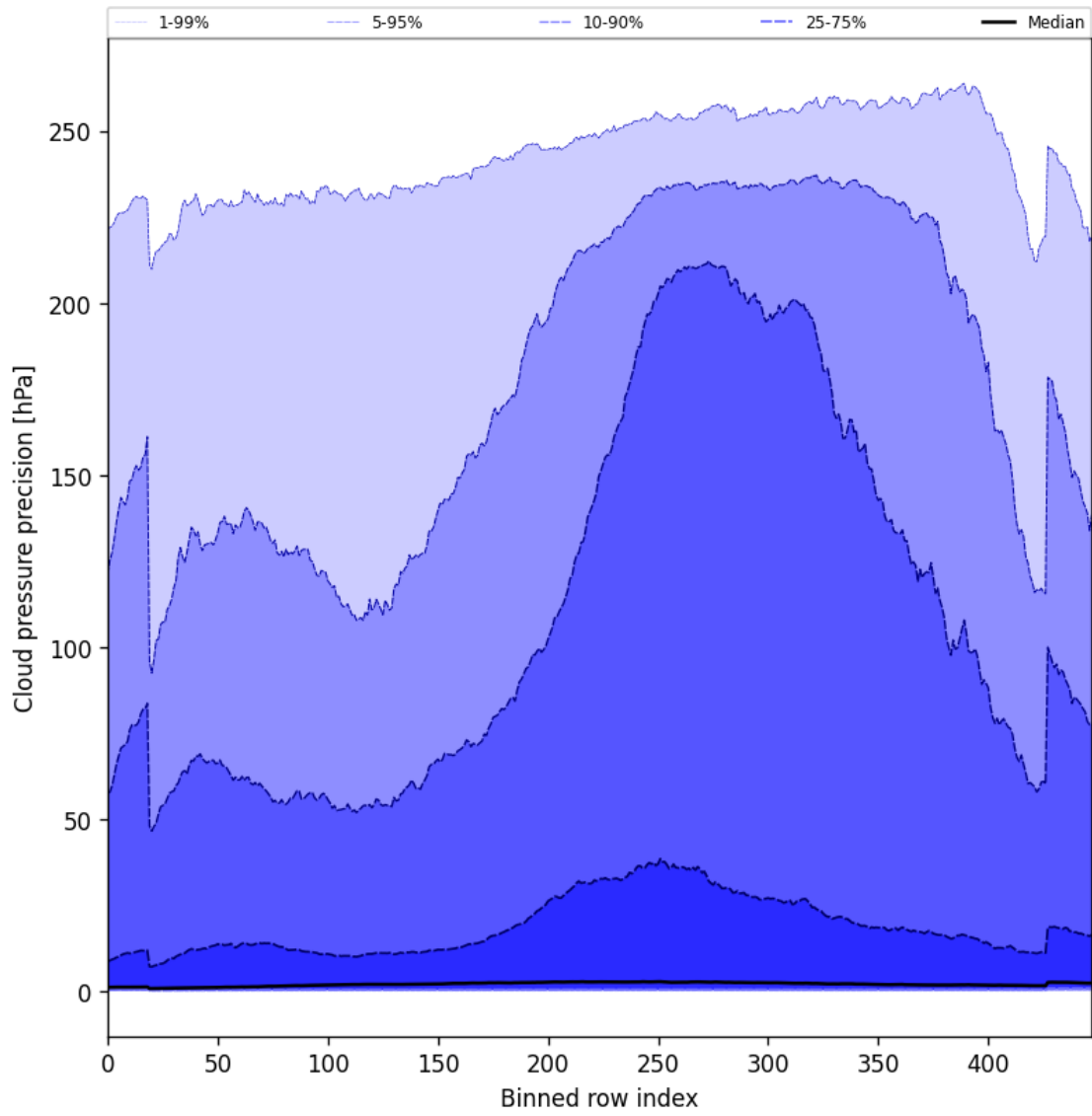
Figure 48: Along track statistics of “Cloud pressure precision” for 2024-11-04 to 2024-11-06
