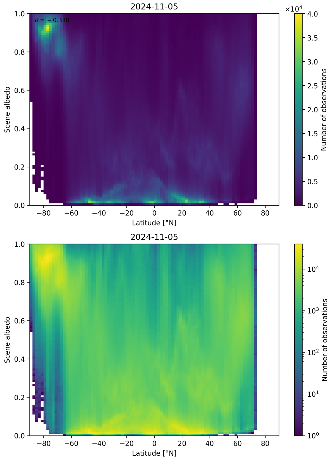
Figure 104: Scatter density plot of “Latitude” against “Scene albedo” for 2024-11-04 to 2024-11-06.
