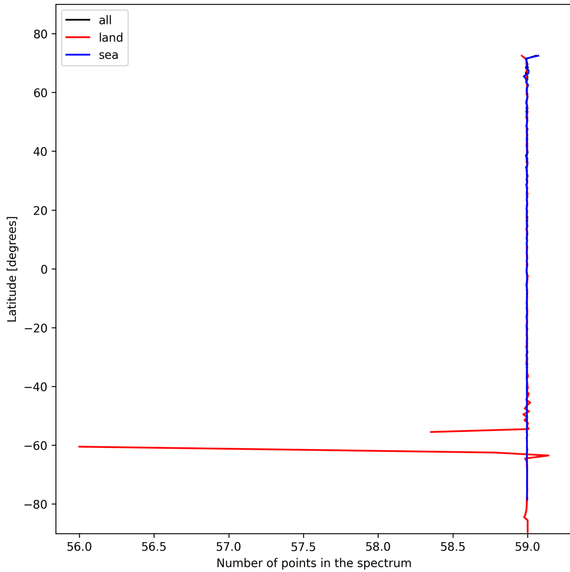
Figure 27: Zonal average of “Number of points in the spectrum” for 2024-11-04 to 2024-11-06.
