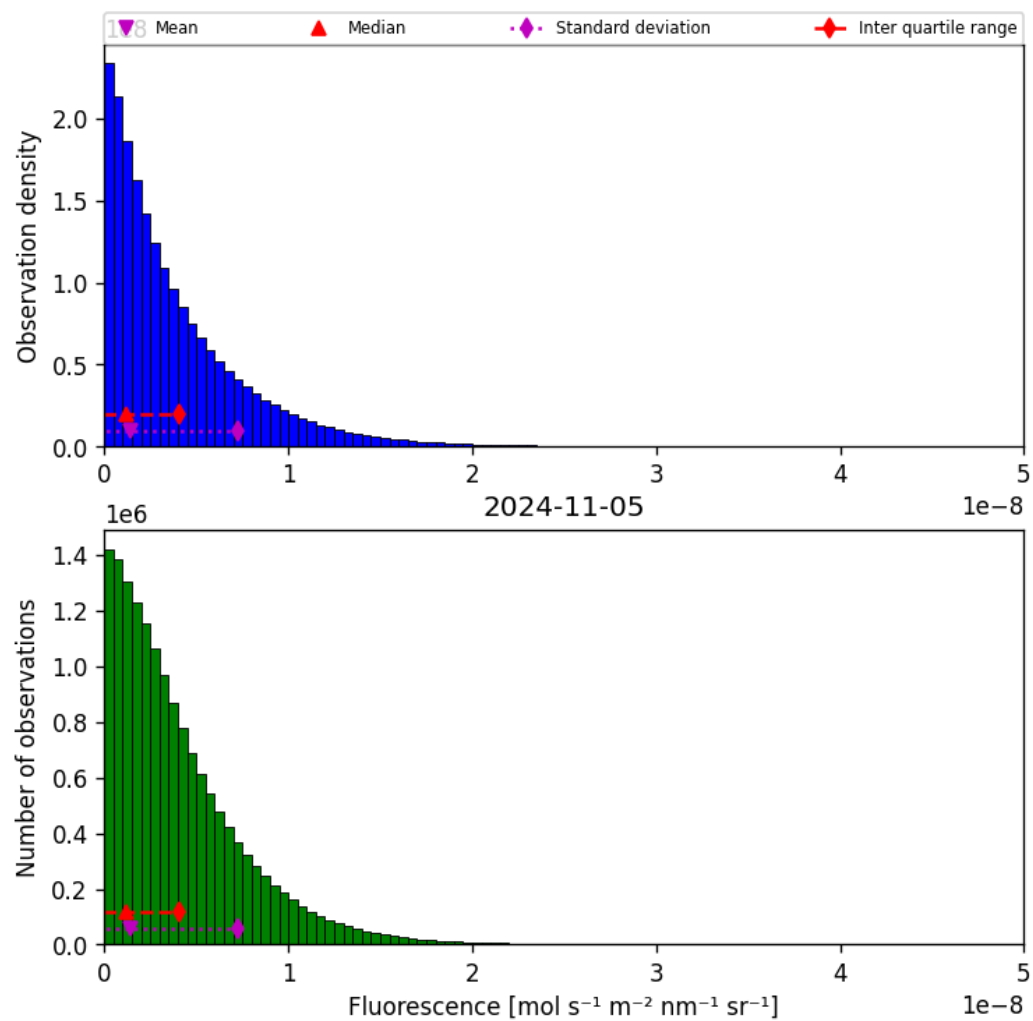
Figure 40: Histogram of “Fluorescence” for 2024-11-04 to 2024-11-06
