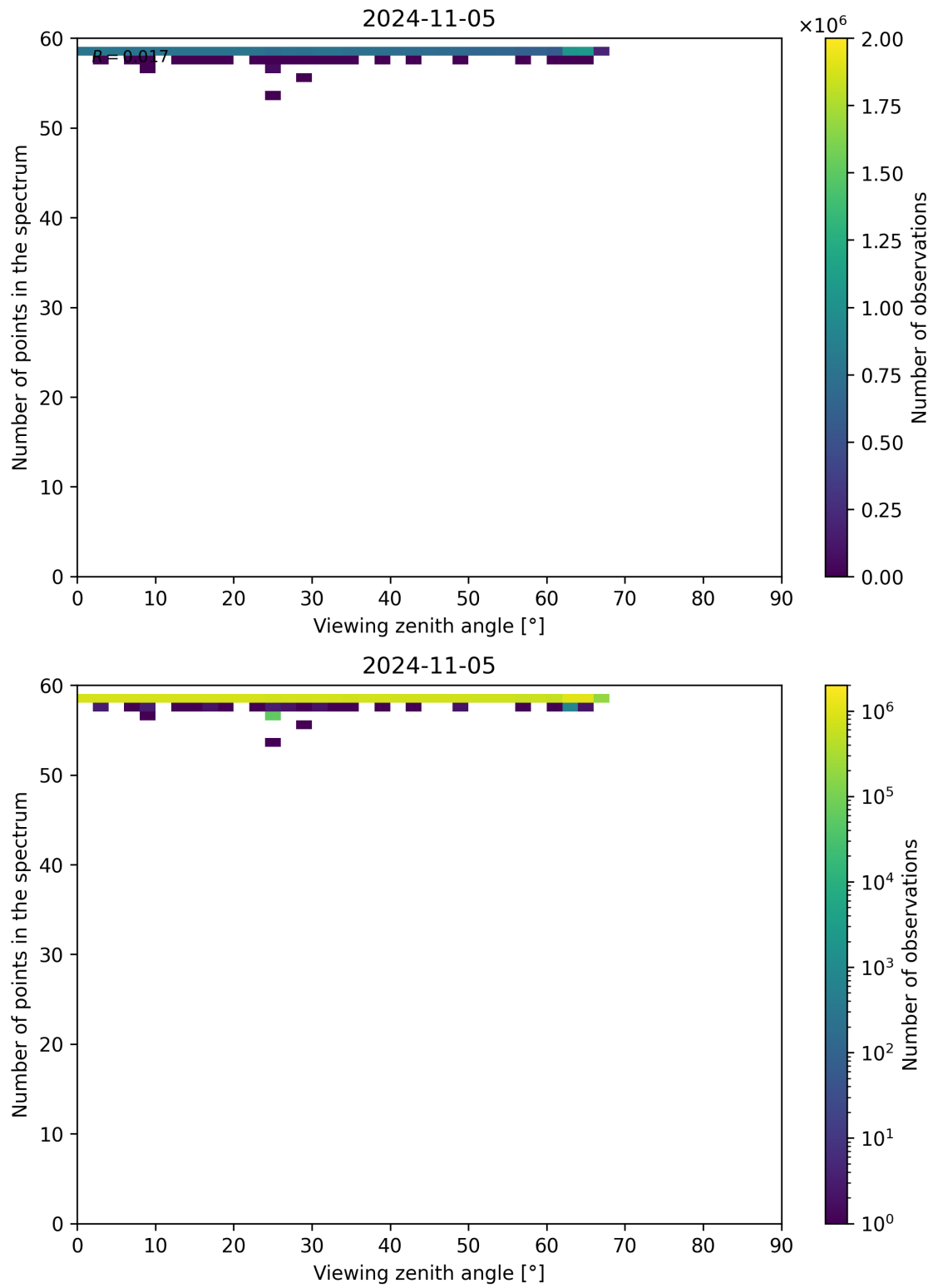
Figure 137: Scatter density plot of “Viewing zenith angle” against “Number of points in the spectrum” for 2024-11-04 to 2024-11-06.
