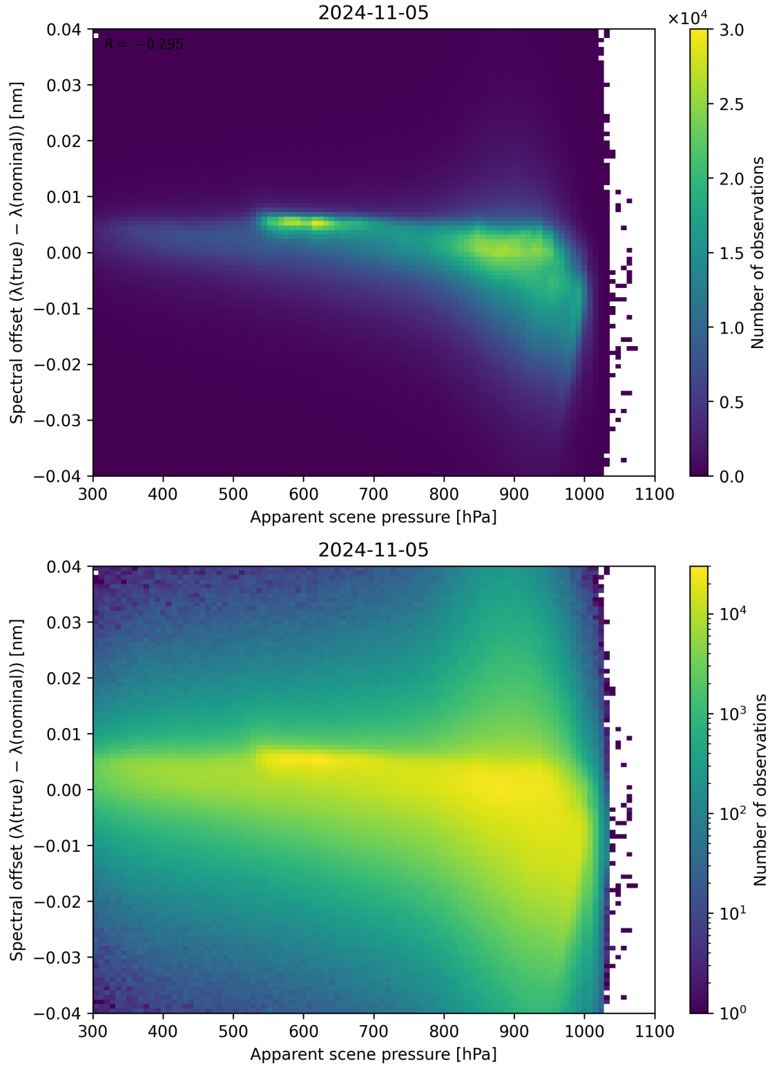
Figure 68: Scatter density plot of “Apparent scene pressure” against “Spectral offset ( \lambda_{\text{true}} - \lambda_{\text{nominal}} )” for 2024-11-04 to 2024-11-06.
