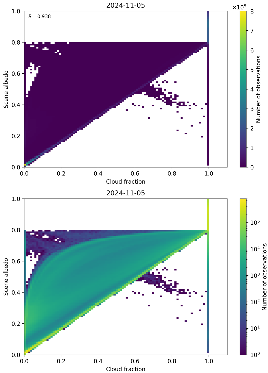
Figure 82: Scatter density plot of “Cloud fraction” against “Scene albedo” for 2024-11-04 to 2024-11-06.
