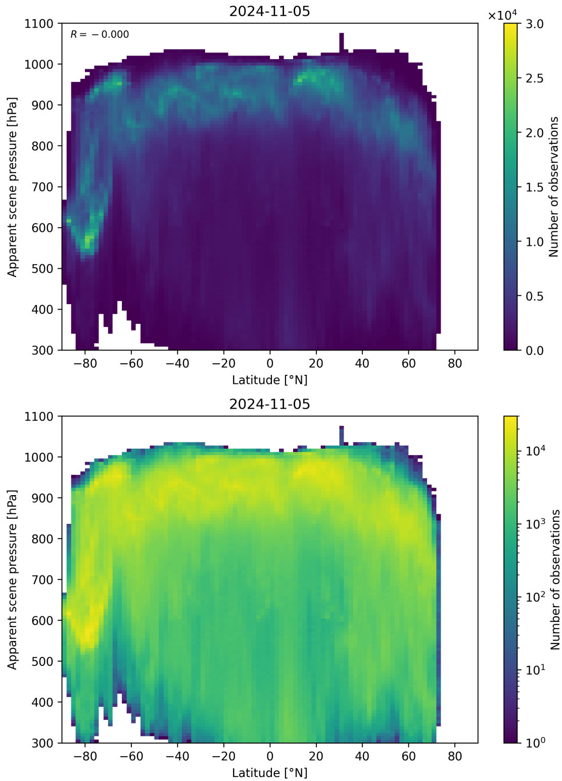
Figure 96: Scatter density plot of “Latitude” against “Apparent scene pressure” for 2024-11-04 to 2024-11-06.
