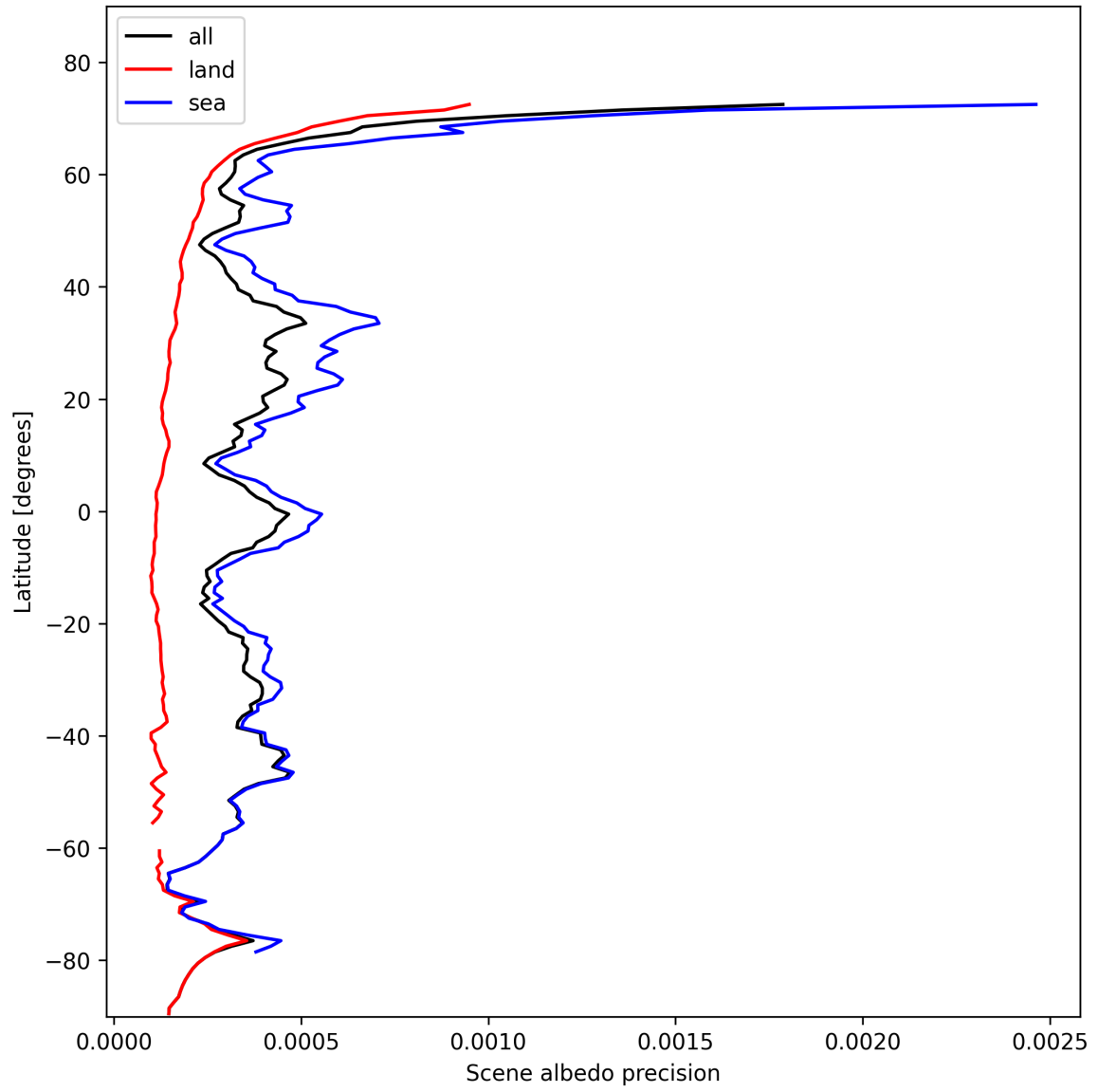
Figure 18: Zonal average of “Scene albedo precision” for 2024-11-04 to 2024-11-06.
