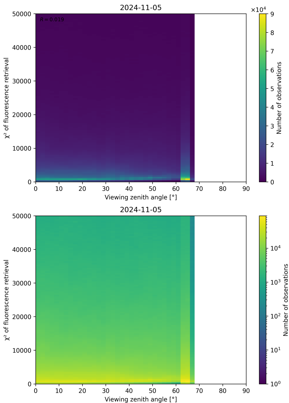
Figure 131: Scatter density plot of “Viewing zenith angle” against “ \chi^2 of fluorescence retrieval” for 2024-11-04 to 2024-11-06.
