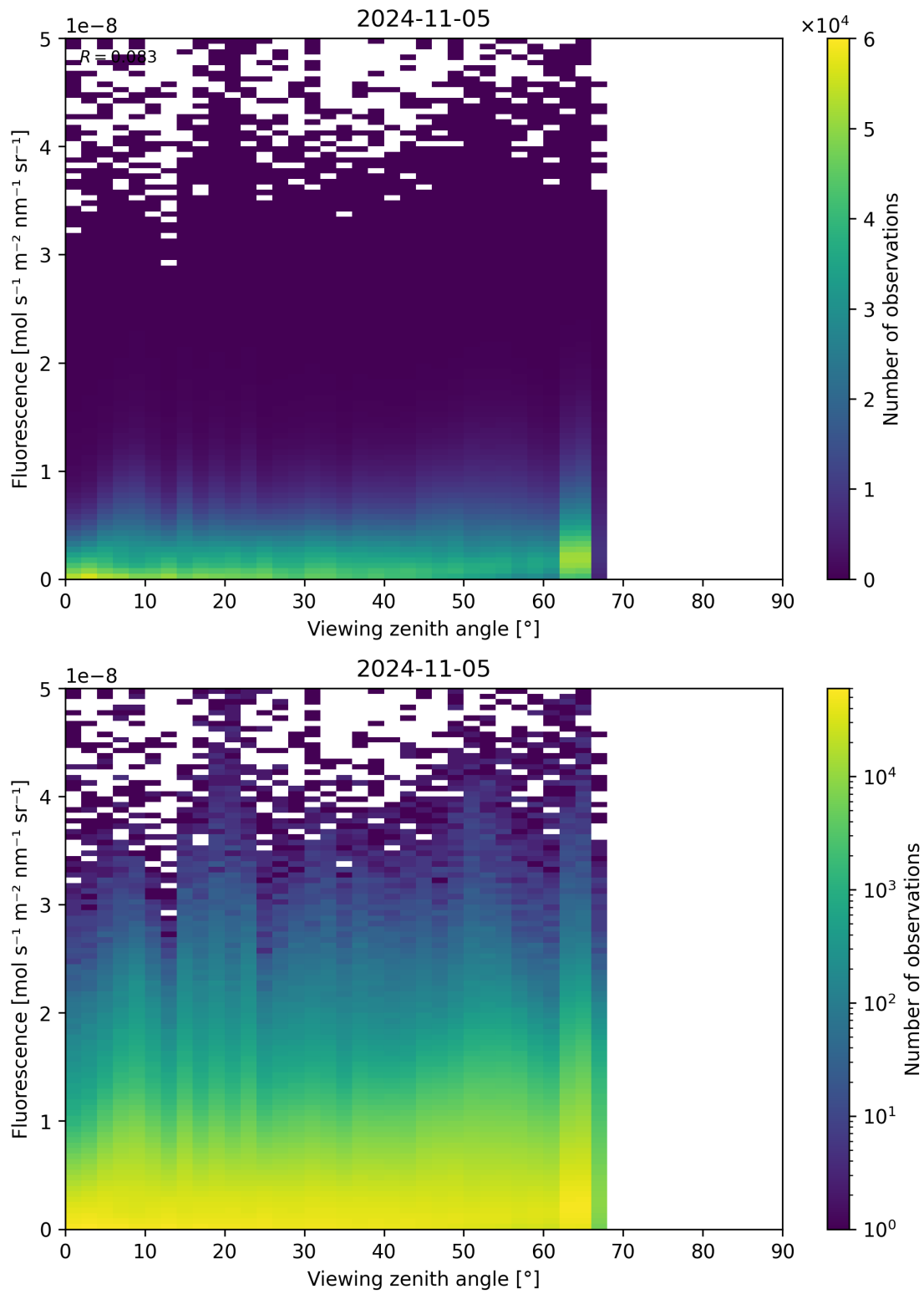
Figure 134: Scatter density plot of “Viewing zenith angle” against “Fluorescence” for 2024-11-04 to 2024-11-06.
