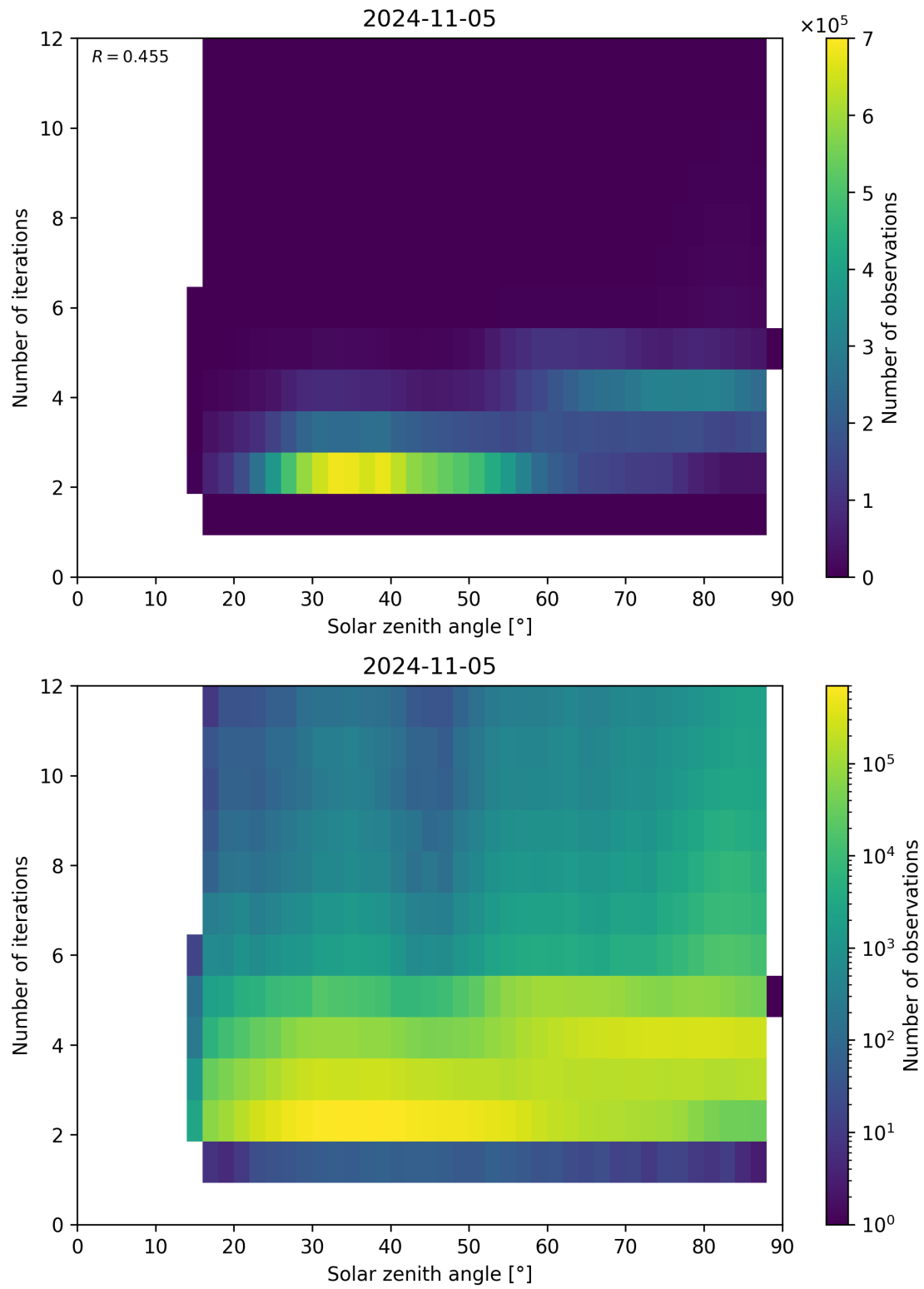
Figure 125: Scatter density plot of “Solar zenith angle” against “Number of iterations” for 2024-11-04 to 2024-11-06.
