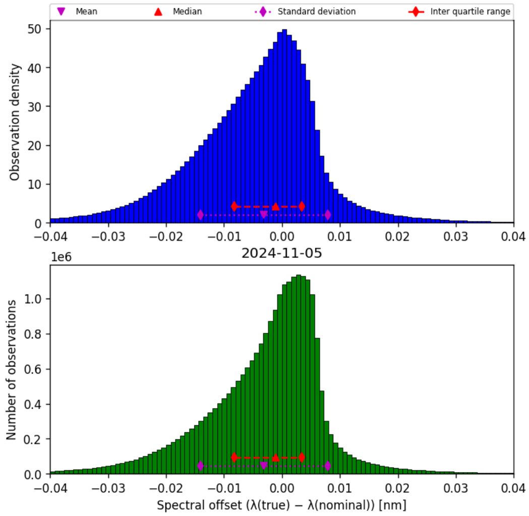
Figure 45: Histogram of “Spectral offset ( \lambda_{\text{true}} - \lambda_{\text{nominal}} )” for 2024-11-04 to 2024-11-06
