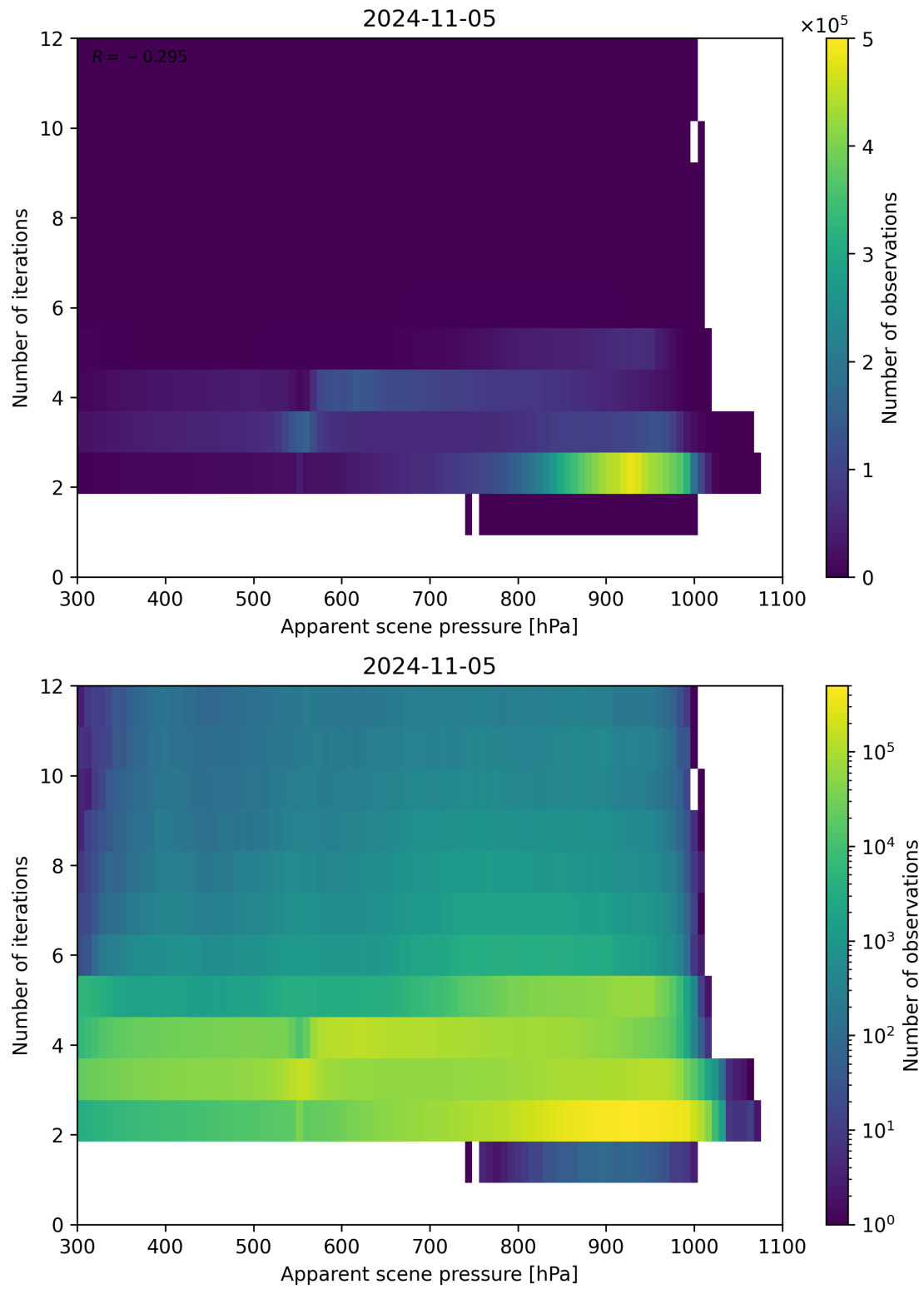
Figure 66: Scatter density plot of “Apparent scene pressure” against “Number of iterations” for 2024-11-04 to 2024-11-06.
