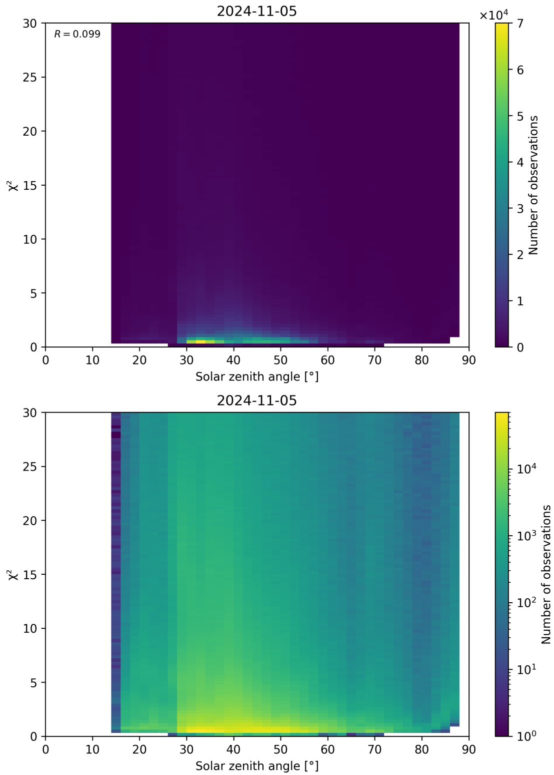
Figure 119: Scatter density plot of “Solar zenith angle” against “ \chi^2 ” for 2024-11-04 to 2024-11-06.
