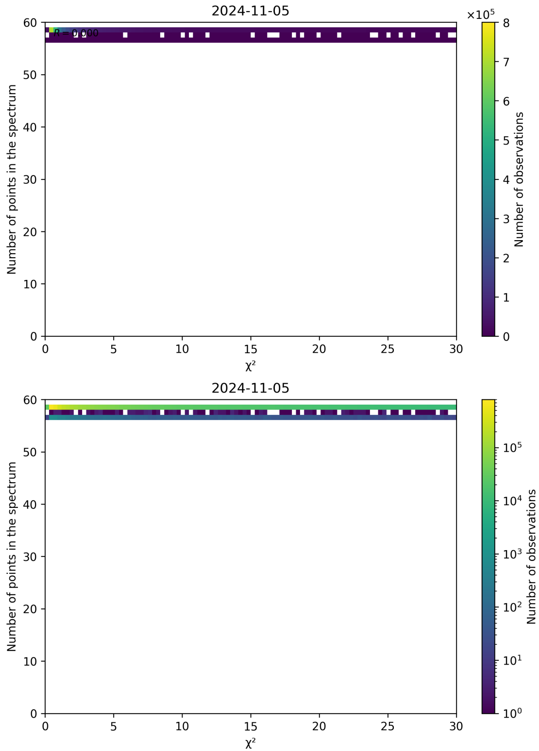
Figure 74: Scatter density plot of " \chi^2 " against "Number of points in the spectrum" for 2024-11-04 to 2024-11-06.
