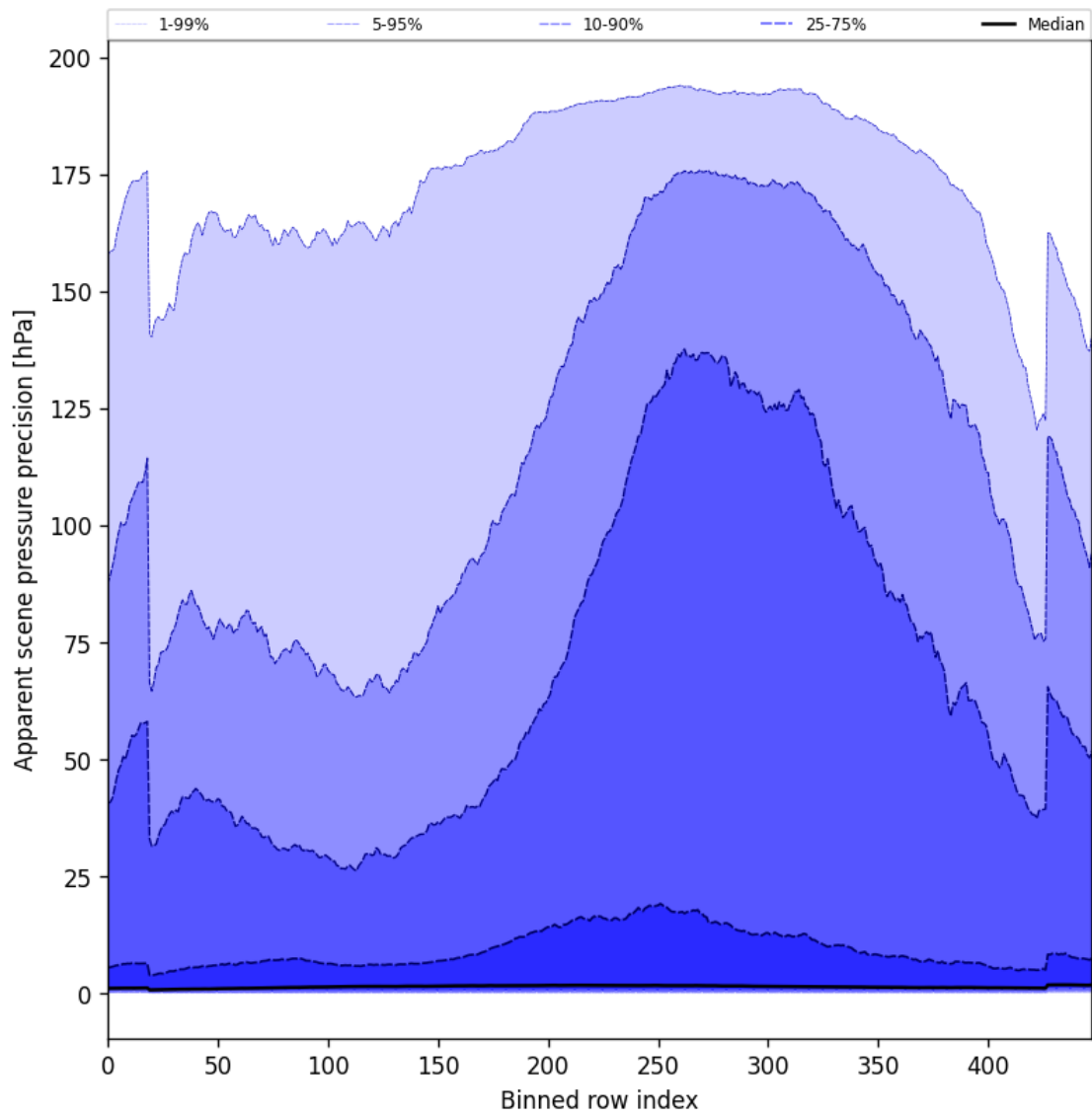
Figure 54: Along track statistics of “Apparent scene pressure precision” for 2024-11-04 to 2024-11-06
