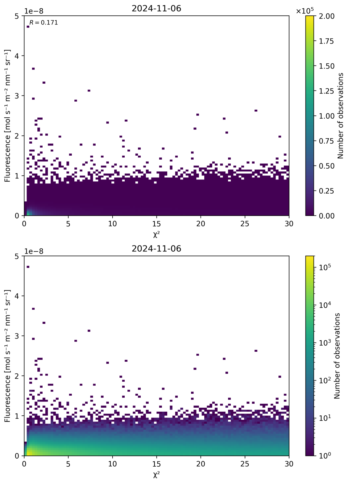
Figure 70: Scatter density plot of “ \chi^2 ” against “Fluorescence” for 2024-11-05 to 2024-11-07.
