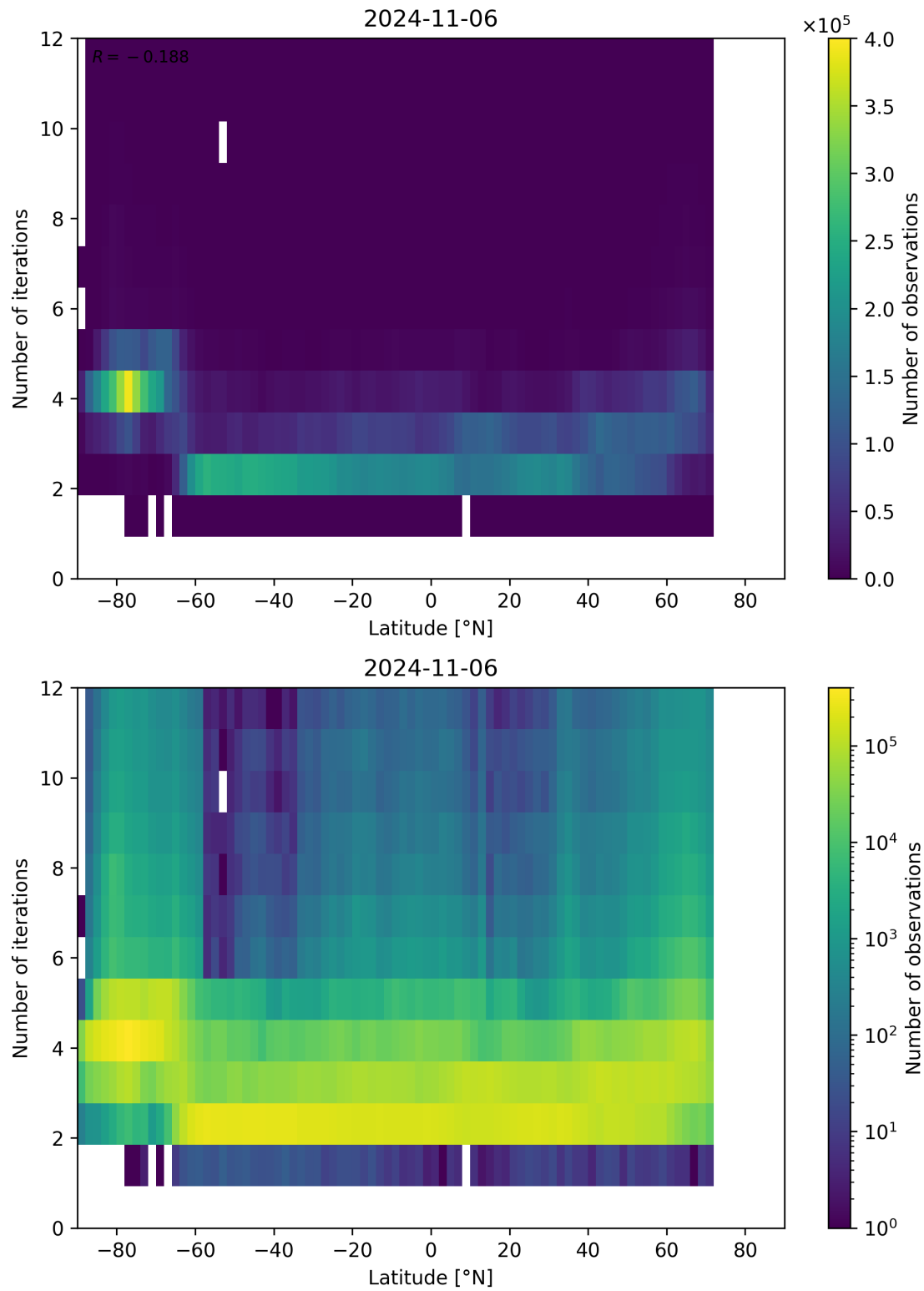
Figure 102: Scatter density plot of “Latitude” against “Number of iterations” for 2024-11-05 to 2024-11-07.
