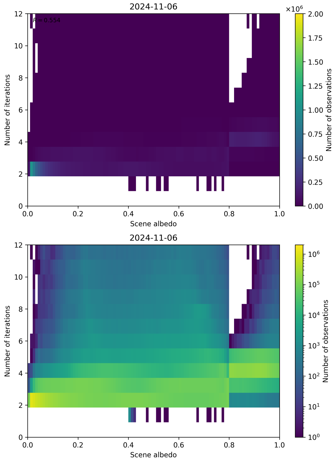
Figure 115: Scatter density plot of “Scene albedo” against “Number of iterations” for 2024-11-05 to 2024-11-07.
