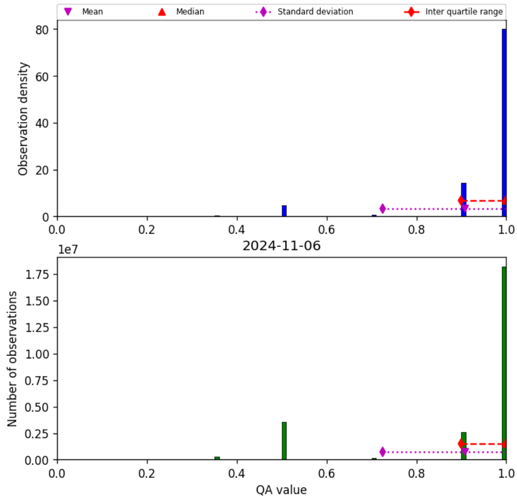
Figure 29: Histogram of “QA value” for 2024-11-05 to 2024-11-07
