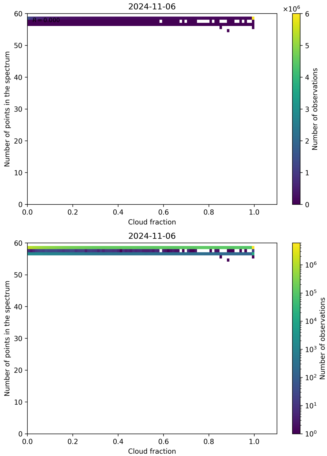
Figure 81: Scatter density plot of “Cloud fraction” against “Number of points in the spectrum” for 2024-11-05 to 2024-11-07.
