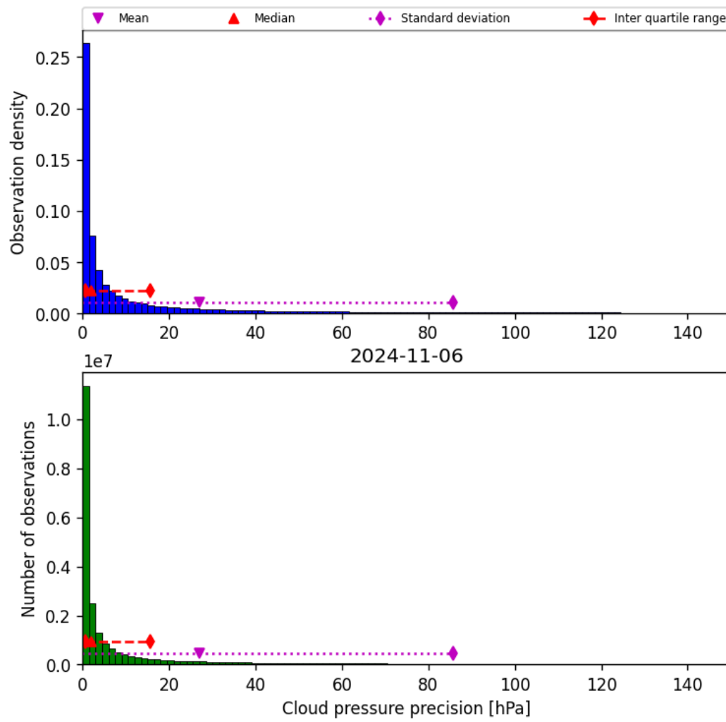
Figure 31: Histogram of “Cloud pressure precision” for 2024-11-05 to 2024-11-07
