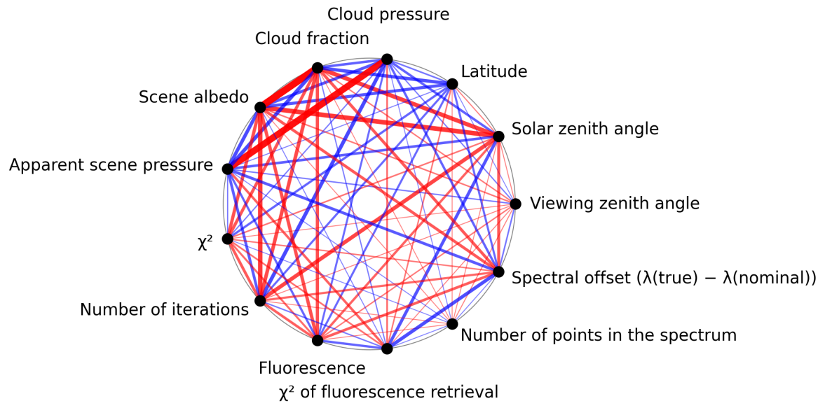
Figure 1: Map of correlation graph for 2024-11-05 to 2024-11-07.
