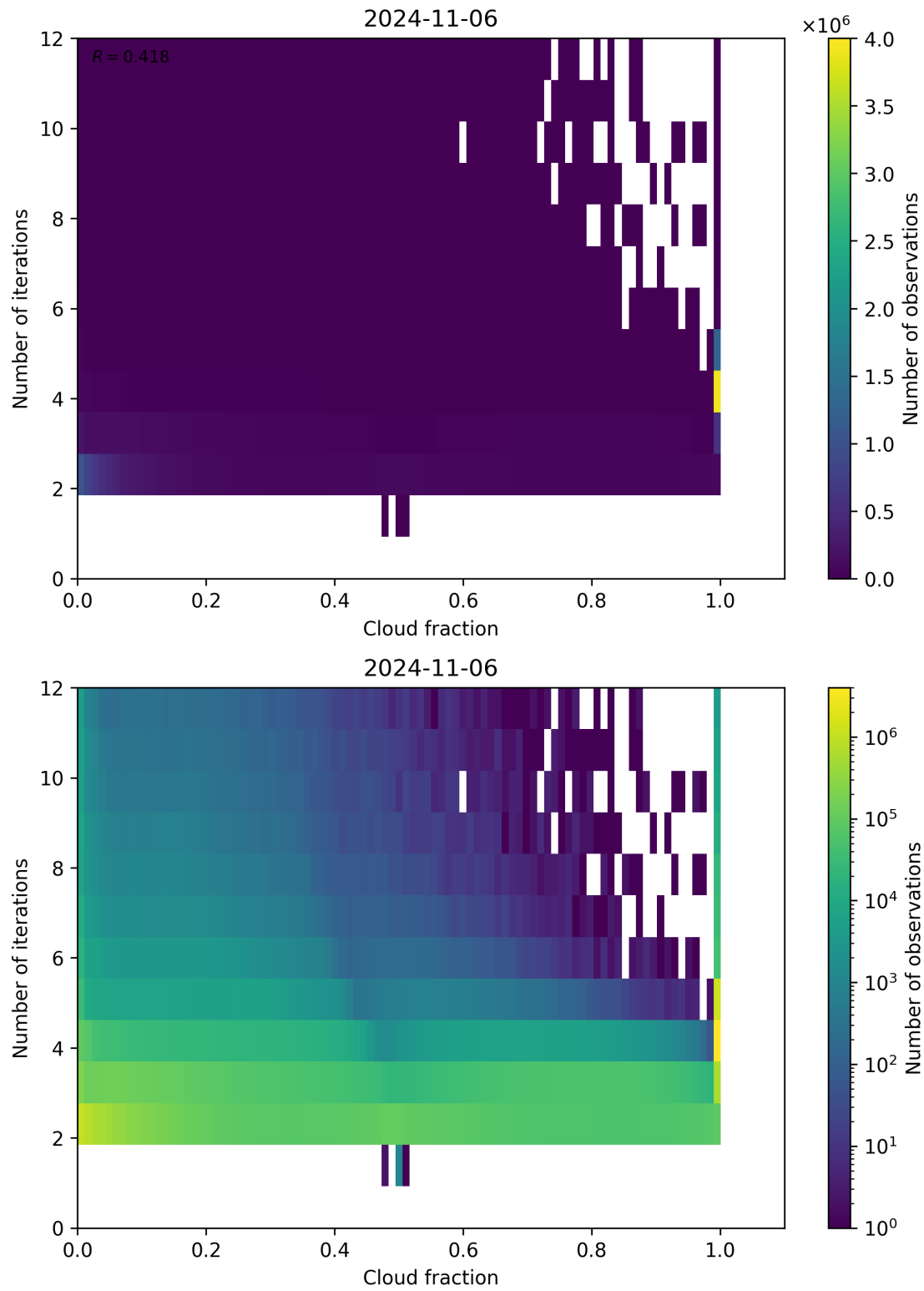
Figure 80: Scatter density plot of “Cloud fraction” against “Number of iterations” for 2024-11-05 to 2024-11-07.
