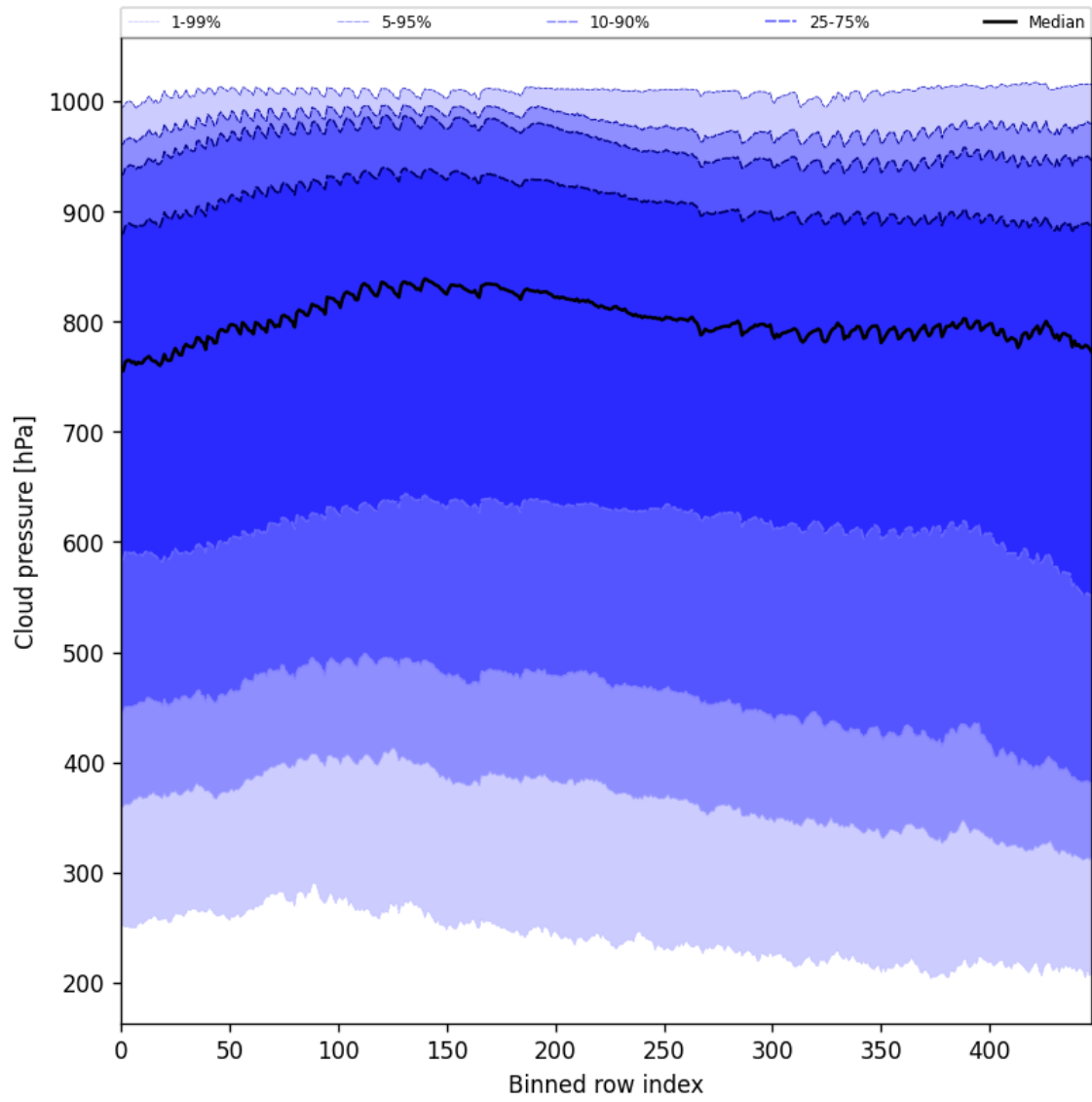
Figure 47: Along track statistics of “Cloud pressure” for 2024-11-05 to 2024-11-07
