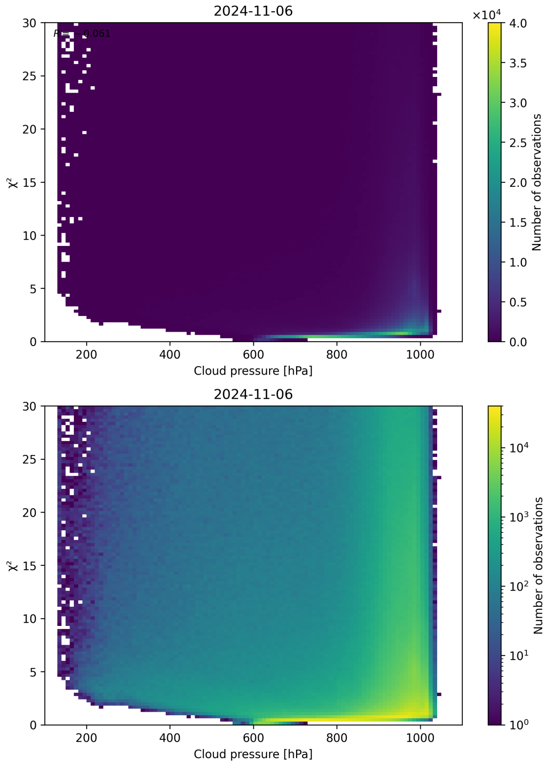
Figure 85: Scatter density plot of “Cloud pressure” against “ \chi^2 ” for 2024-11-05 to 2024-11-07.
