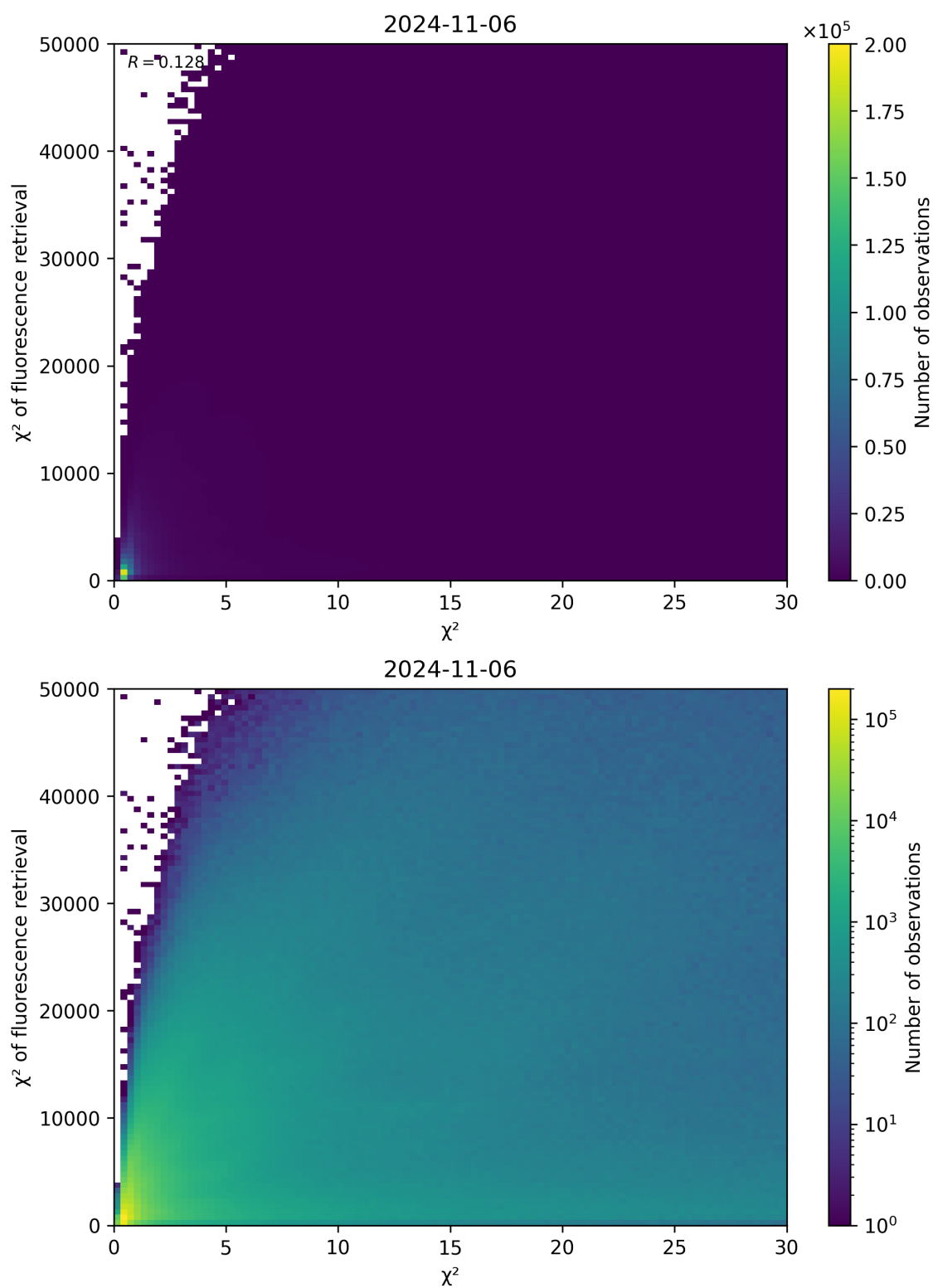
Figure 69: Scatter density plot of “ \chi^2 ” against “ \chi^2 of fluorescence retrieval” for 2024-11-05 to 2024-11-07.
