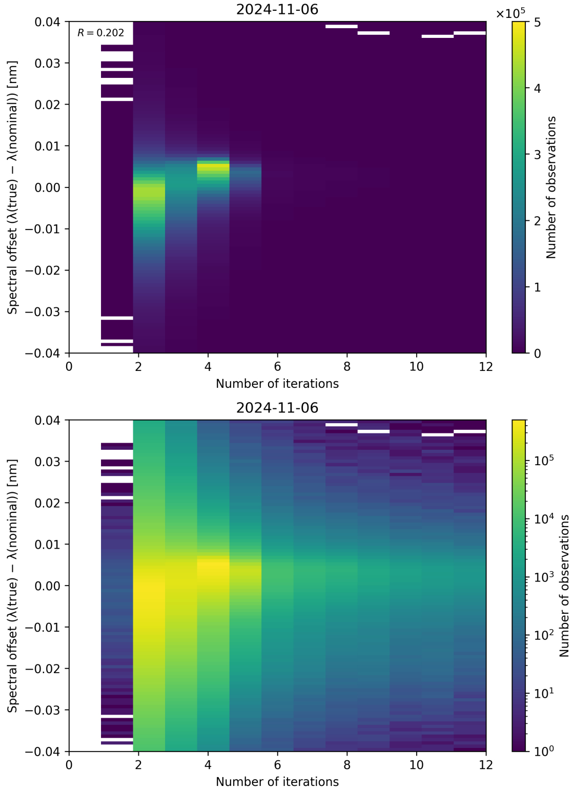
Figure 109: Scatter density plot of “Number of iterations” against “Spectral offset ( \lambda_{\text{true}} - \lambda_{\text{nominal}} )” for 2024-11-05 to 2024-11-07.
