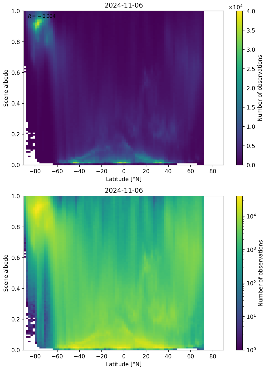
Figure 104: Scatter density plot of “Latitude” against “Scene albedo” for 2024-11-05 to 2024-11-07.
