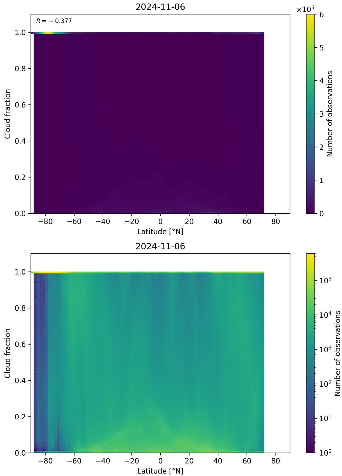
Figure 99: Scatter density plot of “Latitude” against “Cloud fraction” for 2024-11-05 to 2024-11-07.
