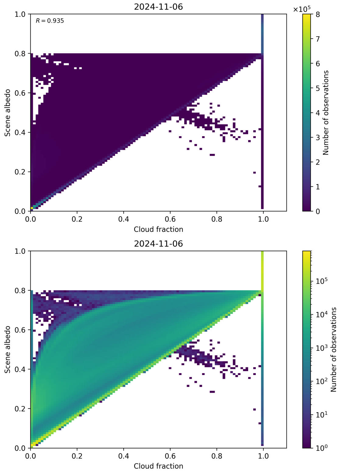
Figure 82: Scatter density plot of “Cloud fraction” against “Scene albedo” for 2024-11-05 to 2024-11-07.
