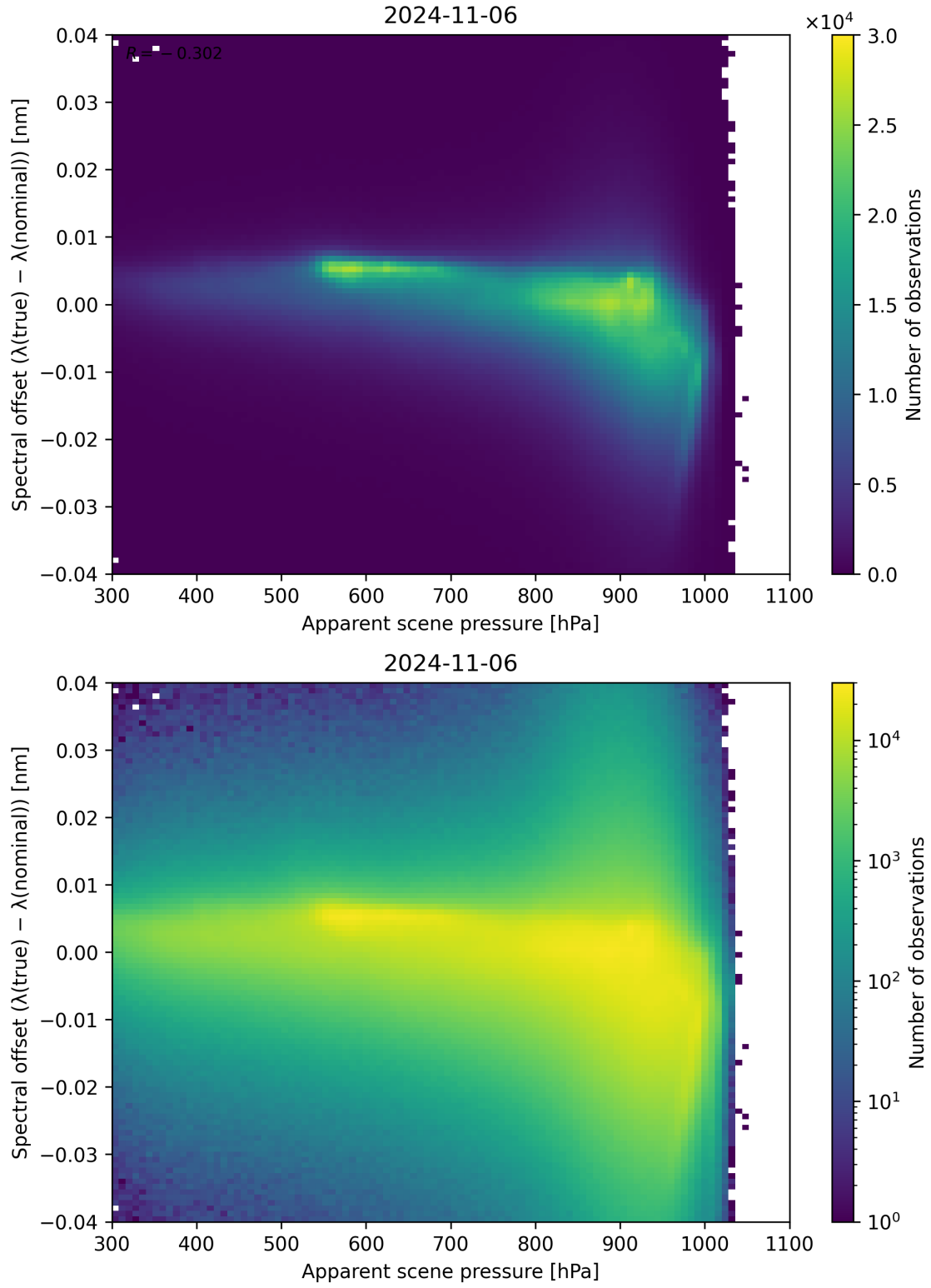
Figure 68: Scatter density plot of “Apparent scene pressure” against “Spectral offset ( \lambda_{\text{true}} - \lambda_{\text{nominal}} )” for 2024-11-05 to 2024-11-07.
