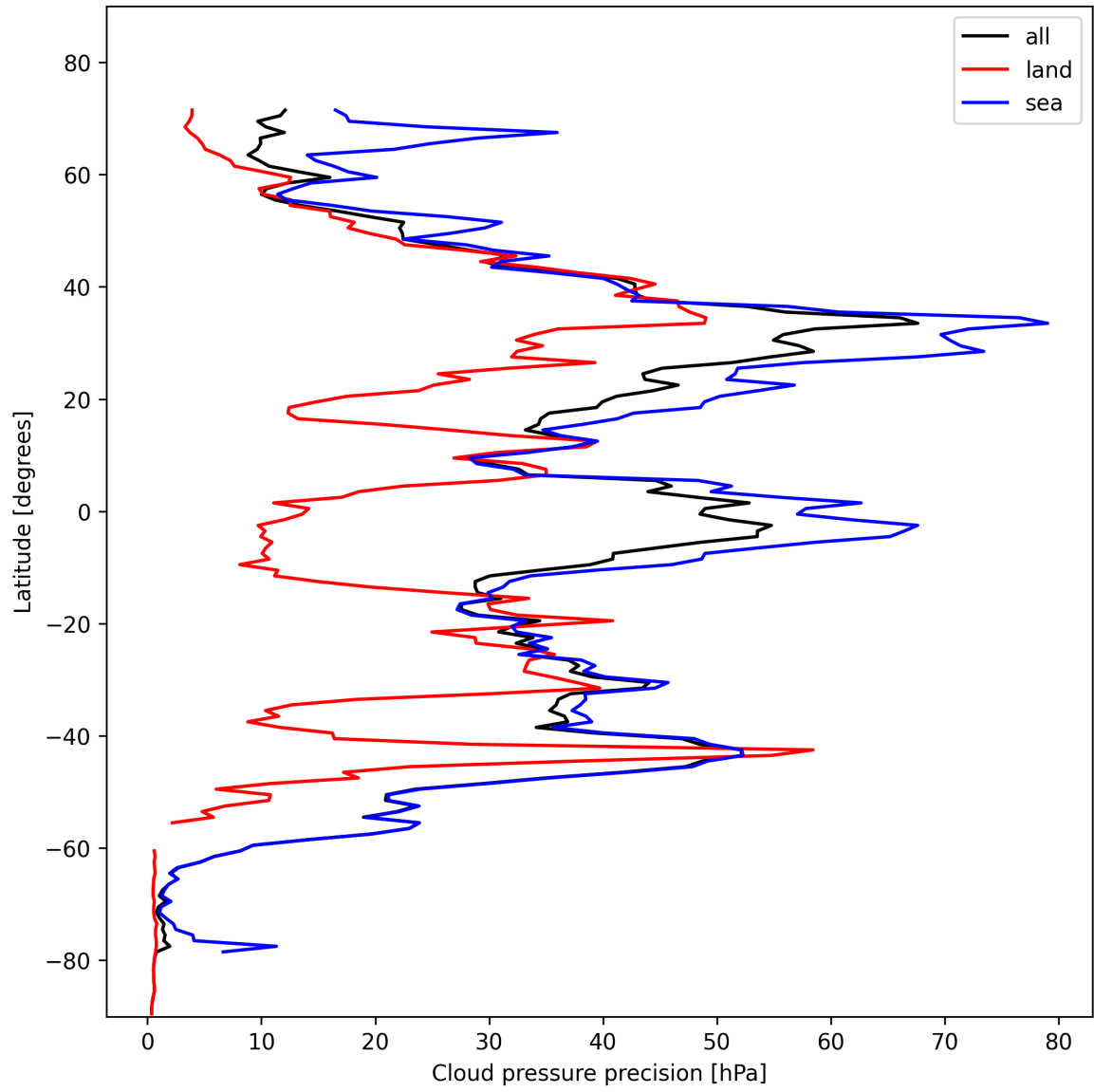
Figure 14: Zonal average of “Cloud pressure precision” for 2024-11-05 to 2024-11-07.
