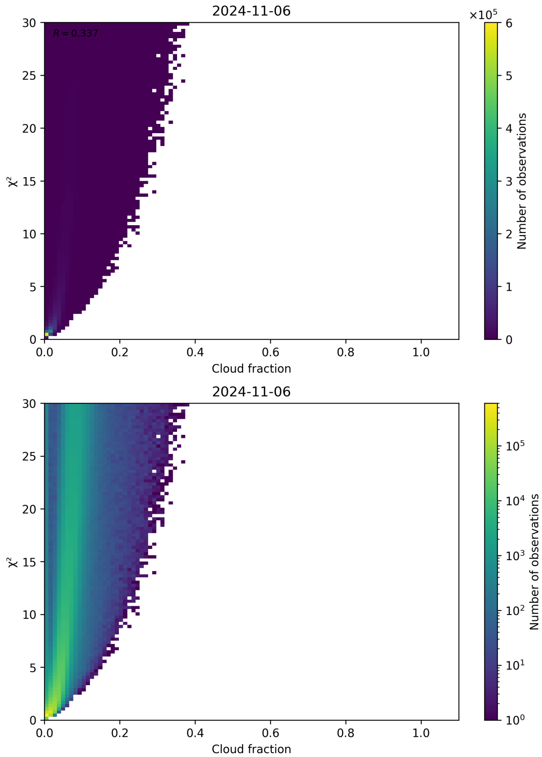
Figure 77: Scatter density plot of “Cloud fraction” against “ \chi^2 ” for 2024-11-05 to 2024-11-07.
