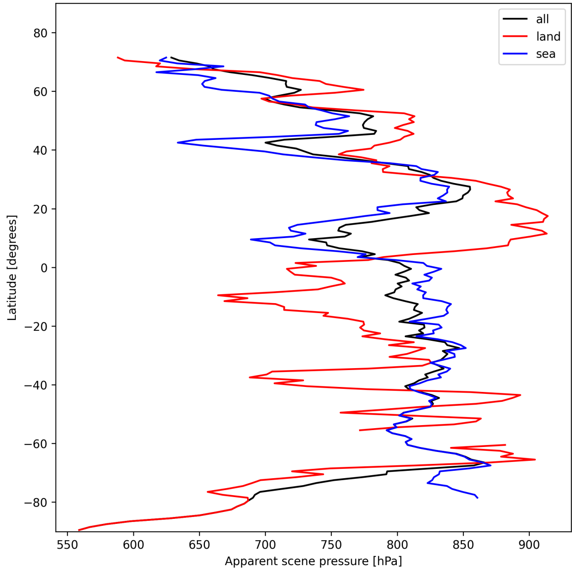
Figure 19: Zonal average of “Apparent scene pressure” for 2024-11-05 to 2024-11-07.
