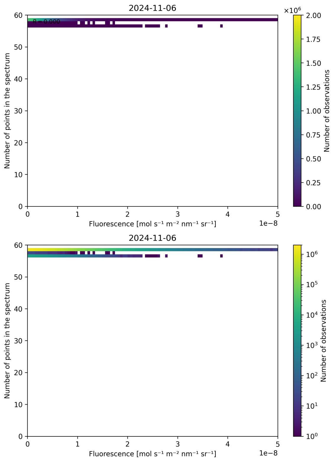
Figure 94: Scatter density plot of “Fluorescence” against “Number of points in the spectrum” for 2024-11-05 to 2024-11-07.
