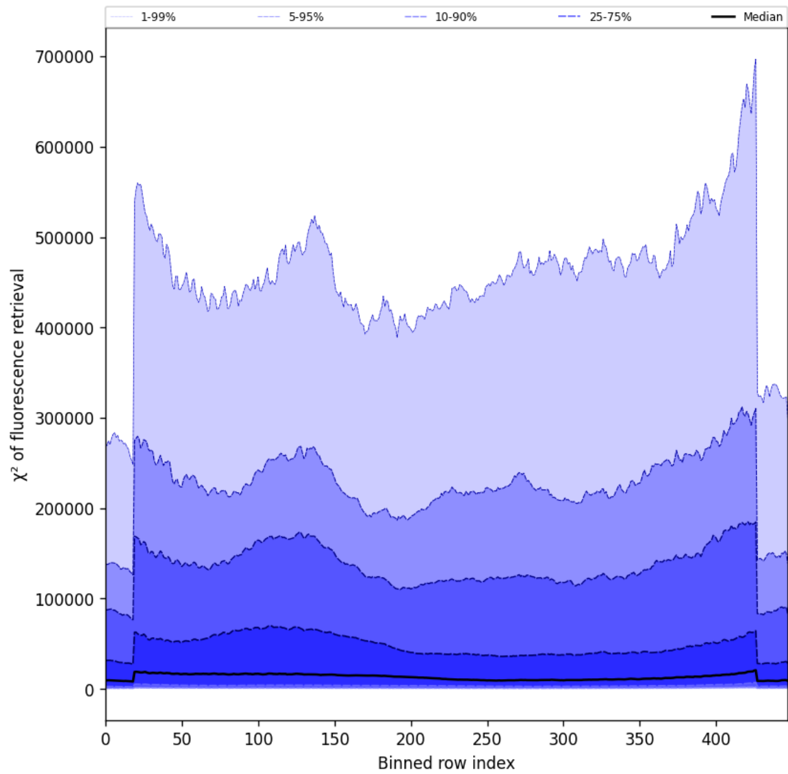
Figure 59: Along track statistics of “ \chi^2 of fluorescence retrieval” for 2024-11-05 to 2024-11-07
