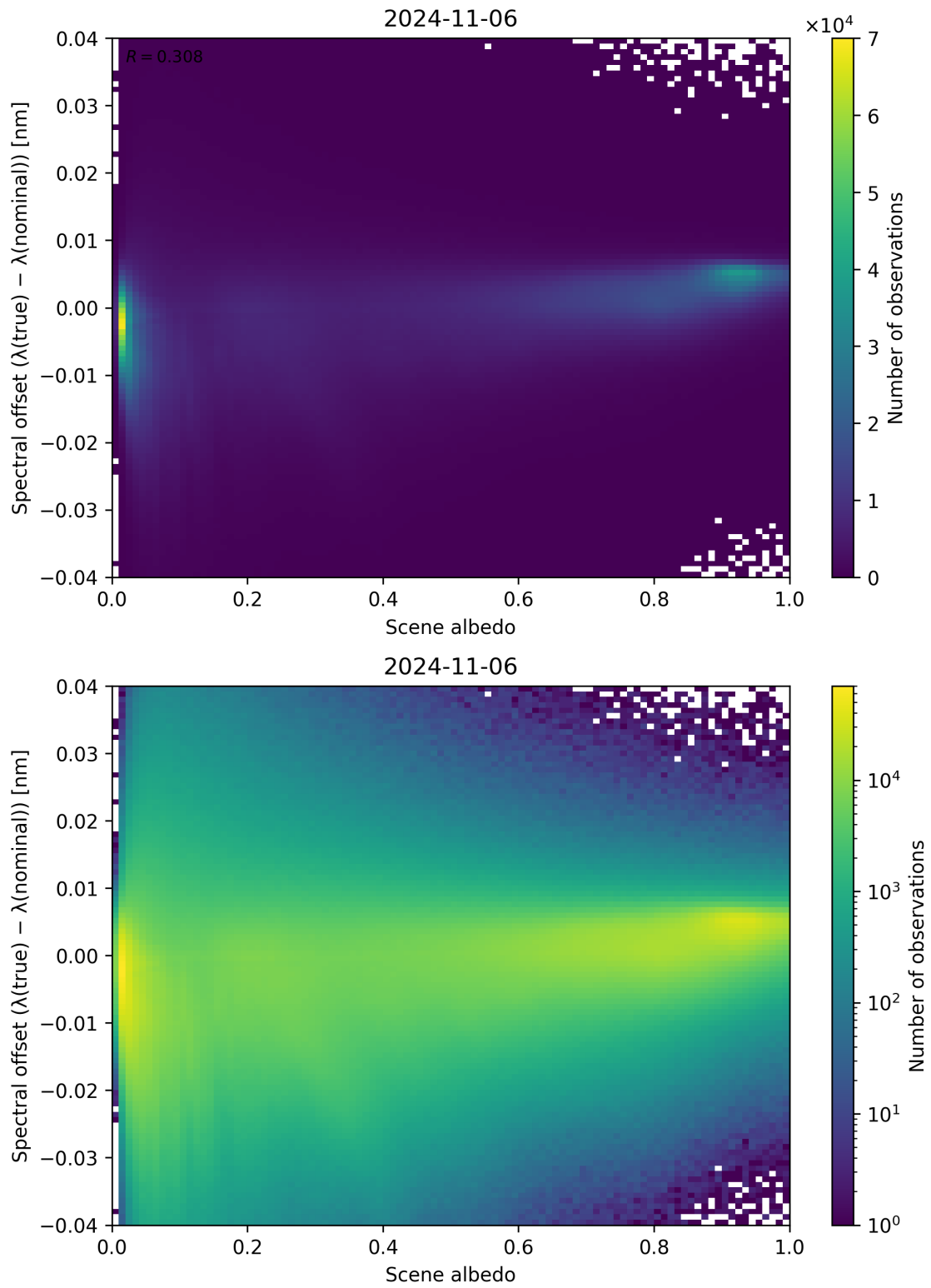
Figure 117: Scatter density plot of “Scene albedo” against “Spectral offset ( \lambda_{\text{true}} - \lambda_{\text{nominal}} )” for 2024-11-05 to 2024-11-07.
