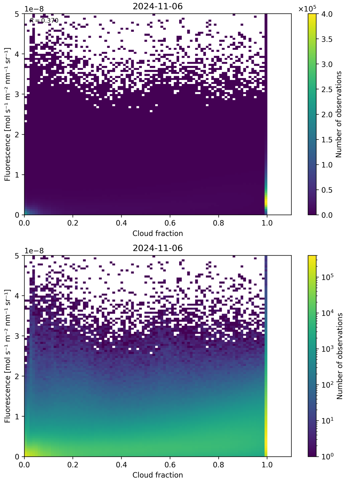
Figure 79: Scatter density plot of “Cloud fraction” against “Fluorescence” for 2024-11-05 to 2024-11-07.
