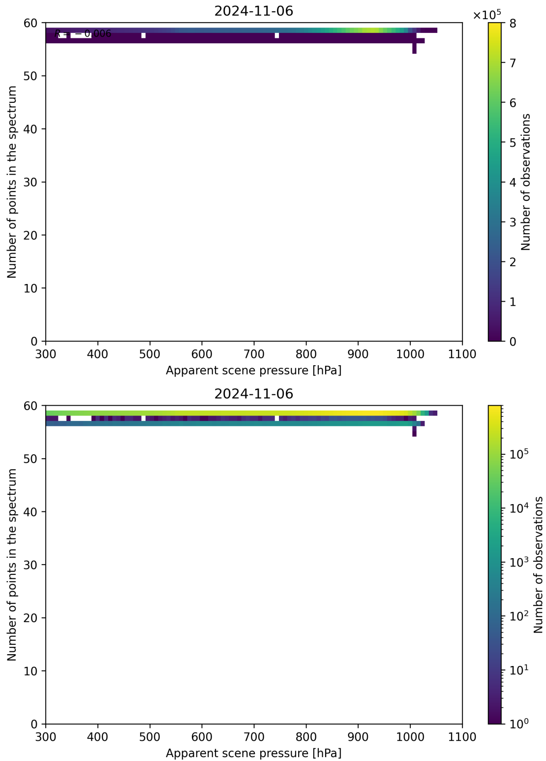
Figure 67: Scatter density plot of “Apparent scene pressure” against “Number of points in the spectrum” for 2024-11-05 to 2024-11-07.
