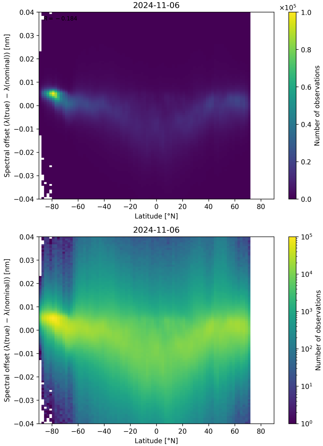
Figure 105: Scatter density plot of “Latitude” against “Spectral offset ( \lambda_{\text{true}} - \lambda_{\text{nominal}} )” for 2024-11-05 to 2024-11-07.
