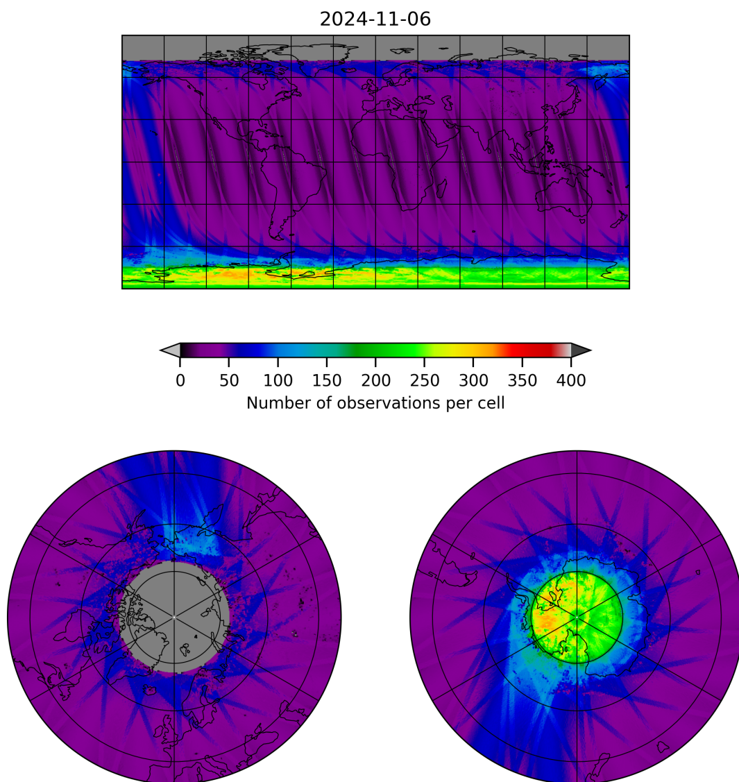
Figure 11: Map of the number of observations for 2024-11-05 to 2024-11-07
