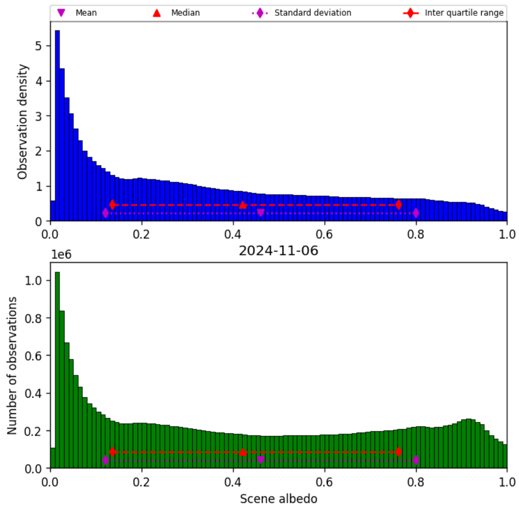
Figure 34: Histogram of “Scene albedo” for 2024-11-05 to 2024-11-07
