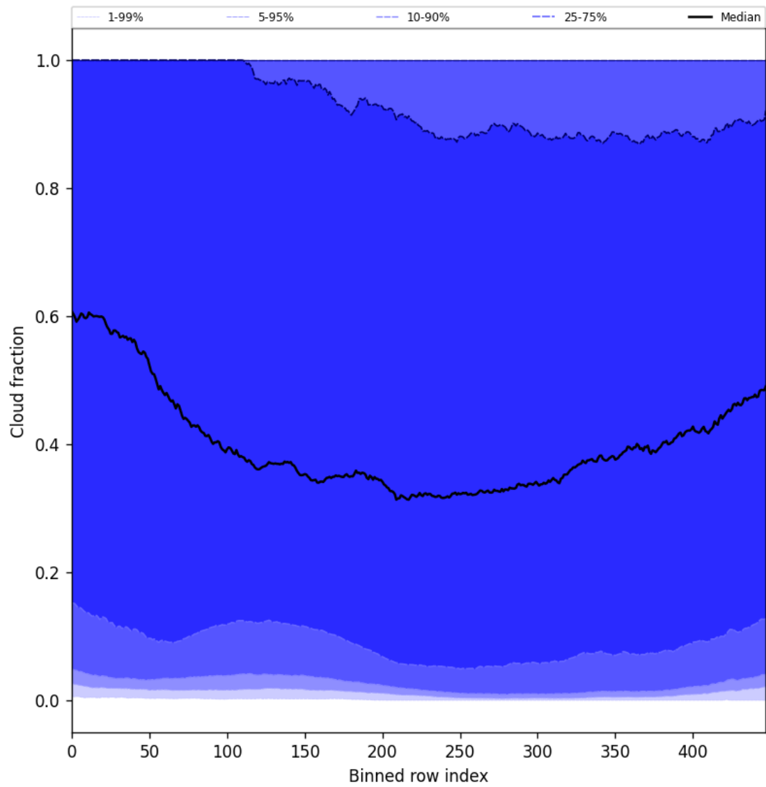
Figure 49: Along track statistics of “Cloud fraction” for 2024-11-05 to 2024-11-07
