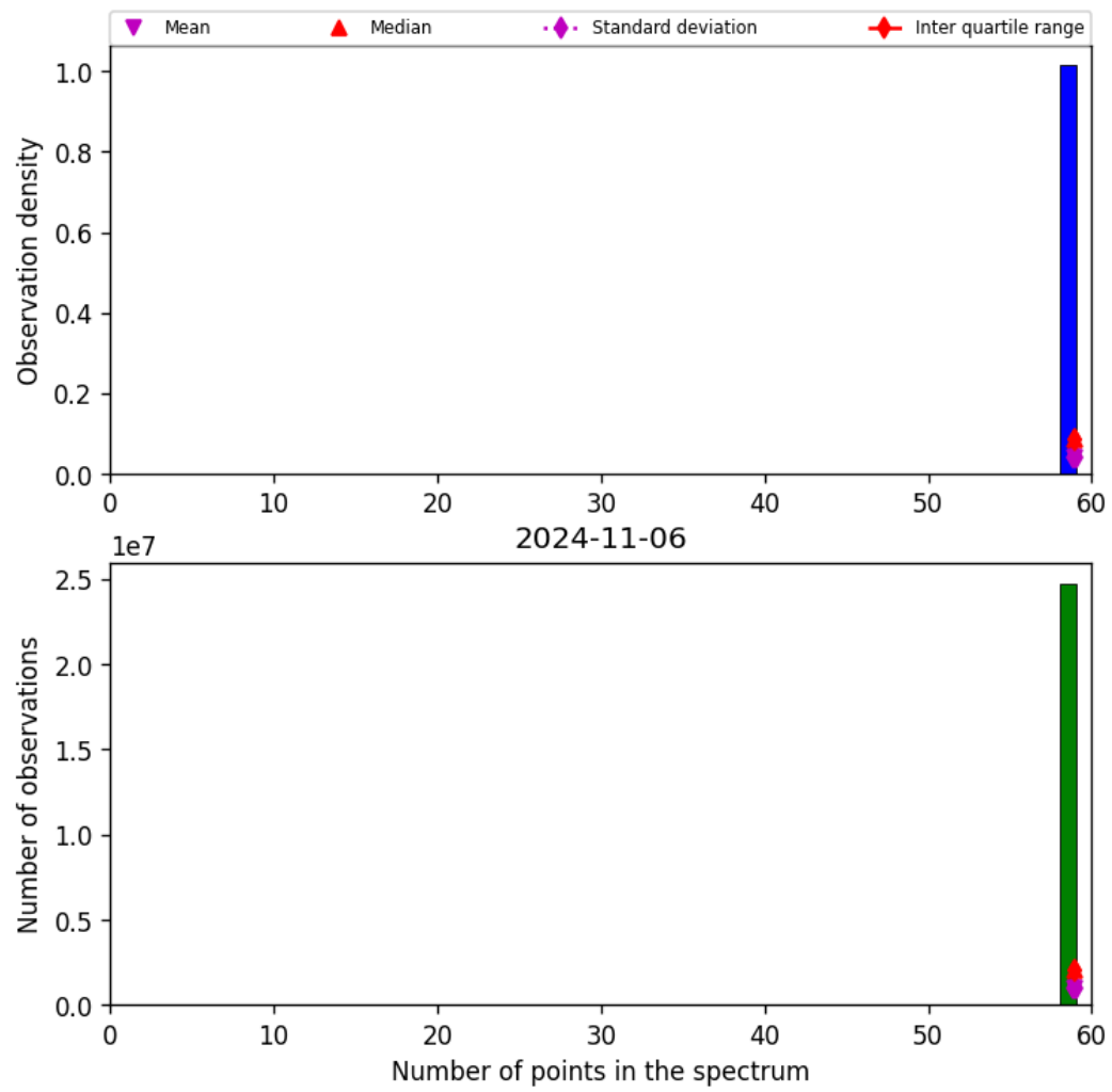
Figure 44: Histogram of “Number of points in the spectrum” for 2024-11-05 to 2024-11-07
