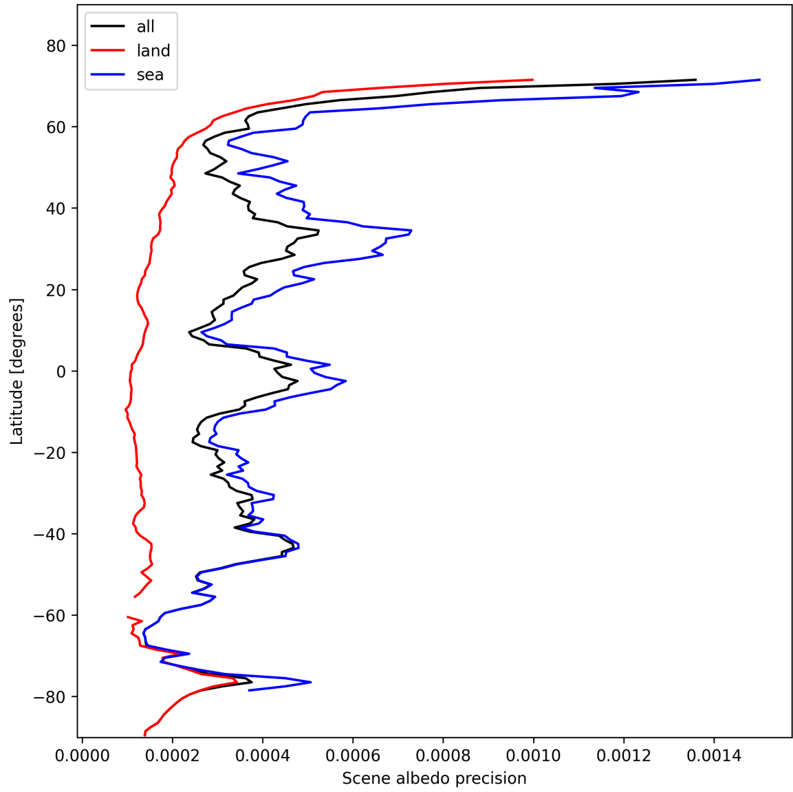
Figure 18: Zonal average of “Scene albedo precision” for 2024-11-05 to 2024-11-07.
