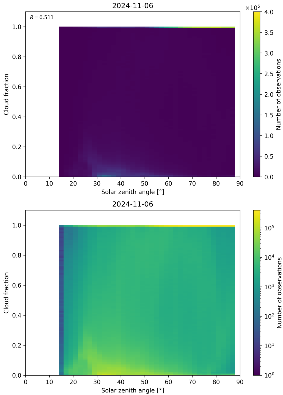
Figure 121: Scatter density plot of “Solar zenith angle” against “Cloud fraction” for 2024-11-05 to 2024-11-07.
