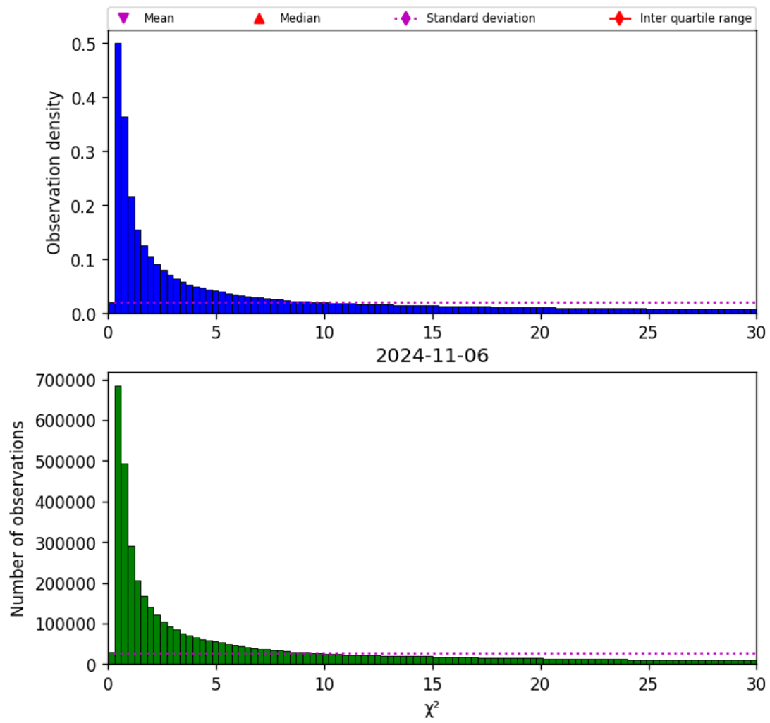
Figure 38: Histogram of “ \chi^2 ” for 2024-11-05 to 2024-11-07
