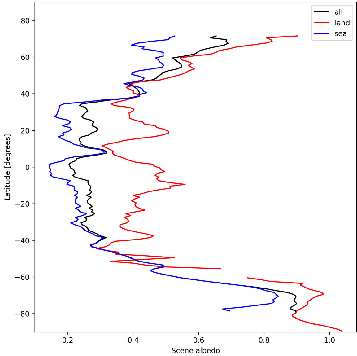
Figure 17: Zonal average of “Scene albedo” for 2024-11-05 to 2024-11-07.
