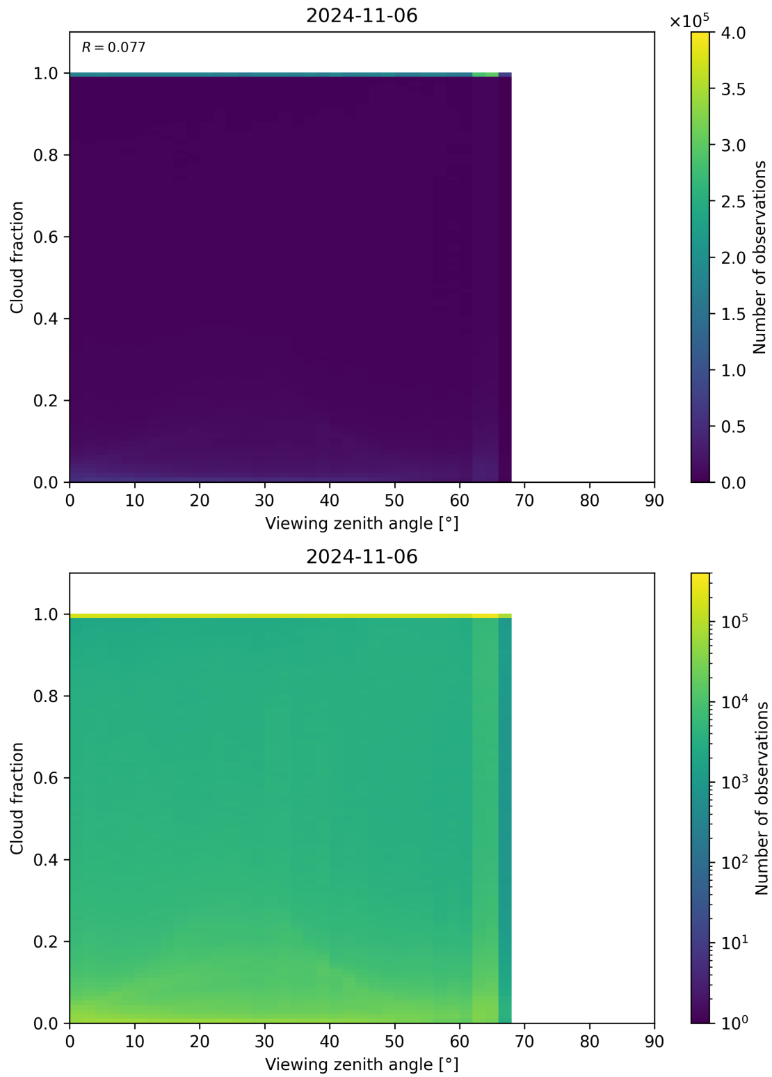
Figure 132: Scatter density plot of “Viewing zenith angle” against “Cloud fraction” for 2024-11-05 to 2024-11-07.
