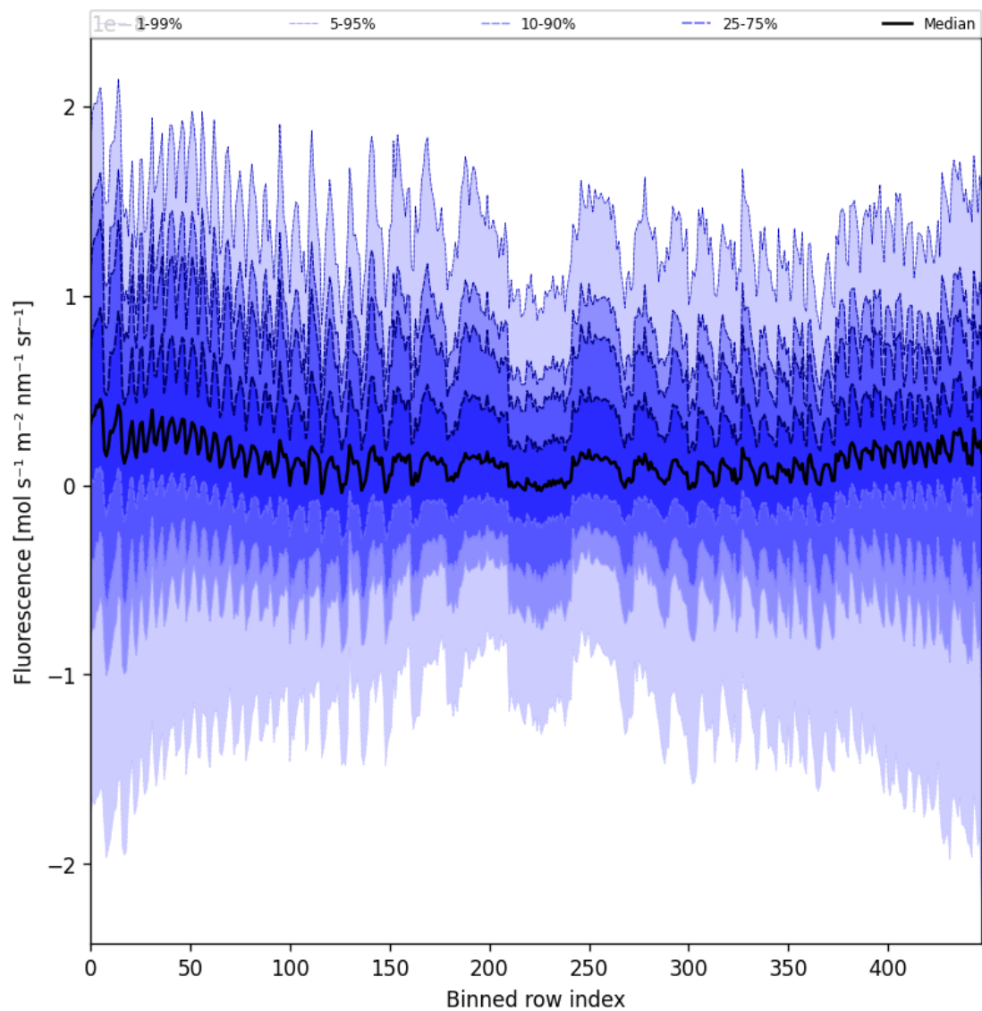
Figure 57: Along track statistics of "Fluorescence" for 2024-11-05 to 2024-11-07
