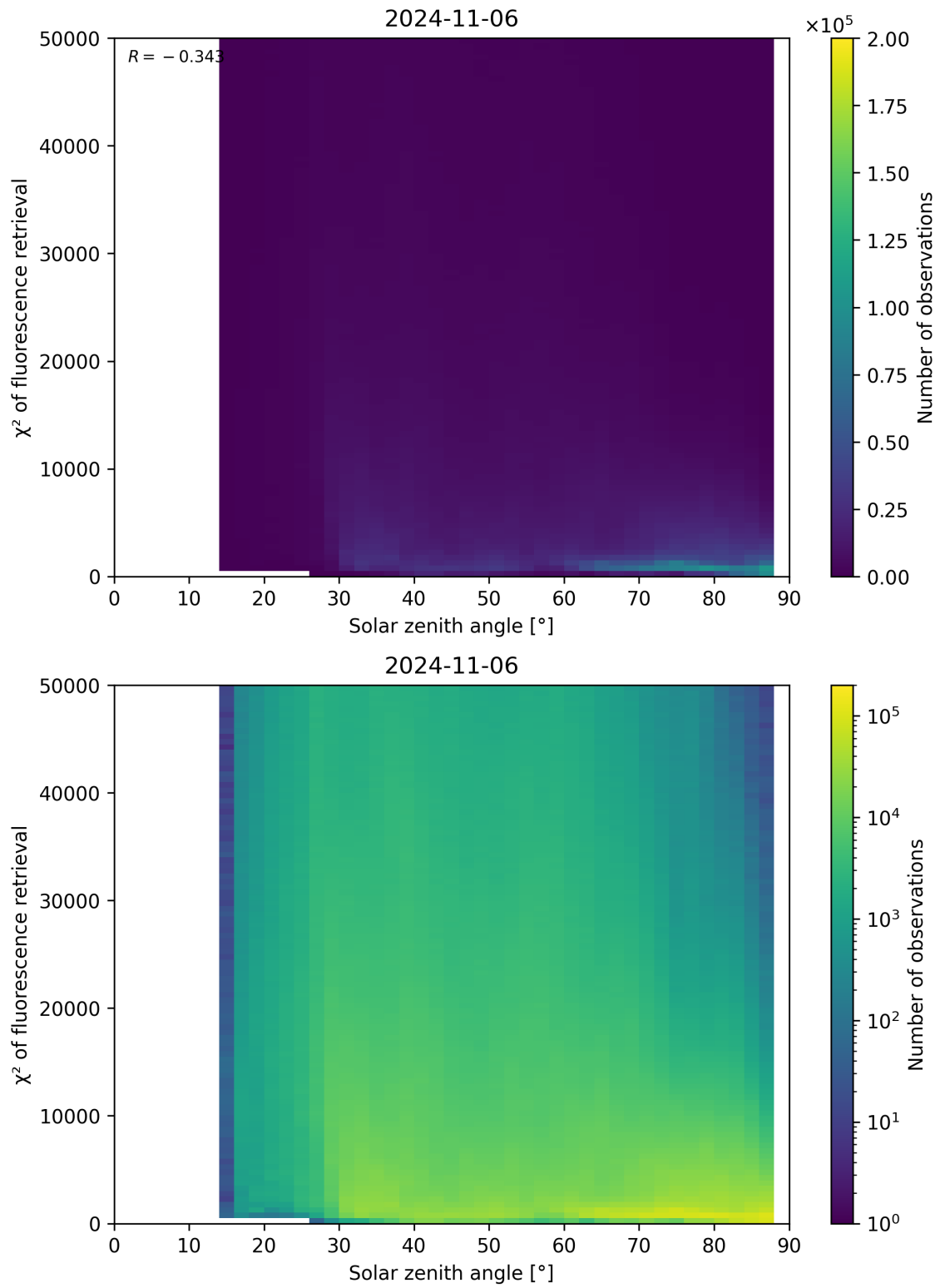
Figure 120: Scatter density plot of “Solar zenith angle” against “ \chi^2 of fluorescence retrieval” for 2024-11-05 to 2024-11-07.
