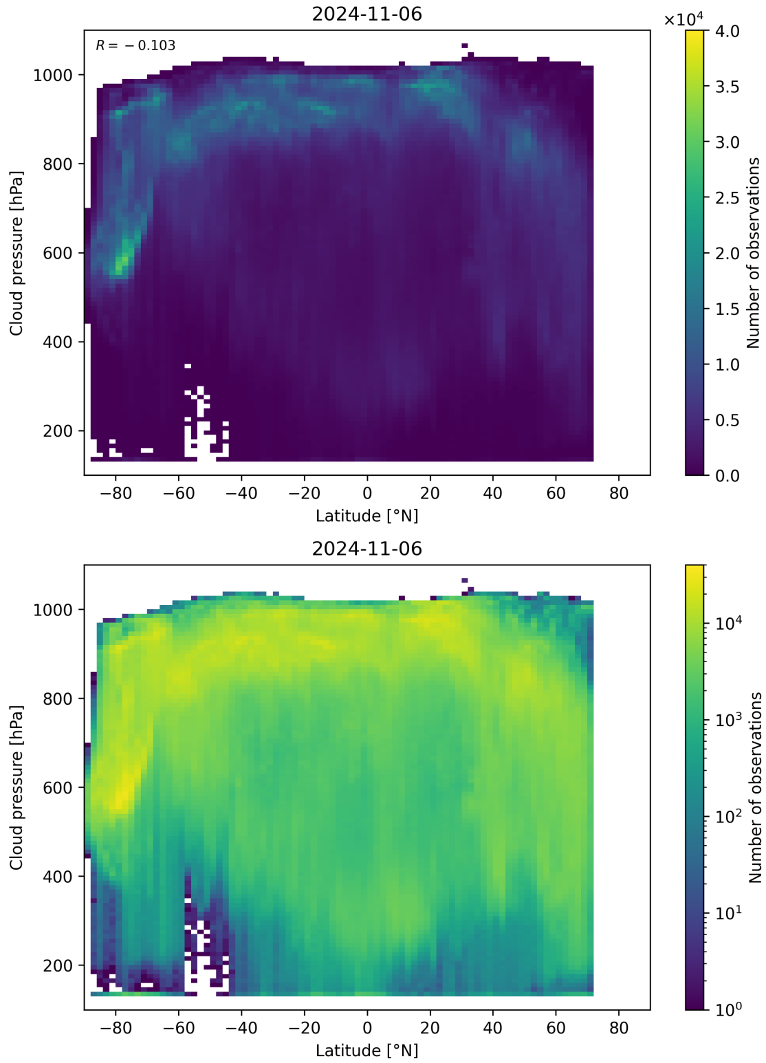
Figure 100: Scatter density plot of “Latitude” against “Cloud pressure” for 2024-11-05 to 2024-11-07.
