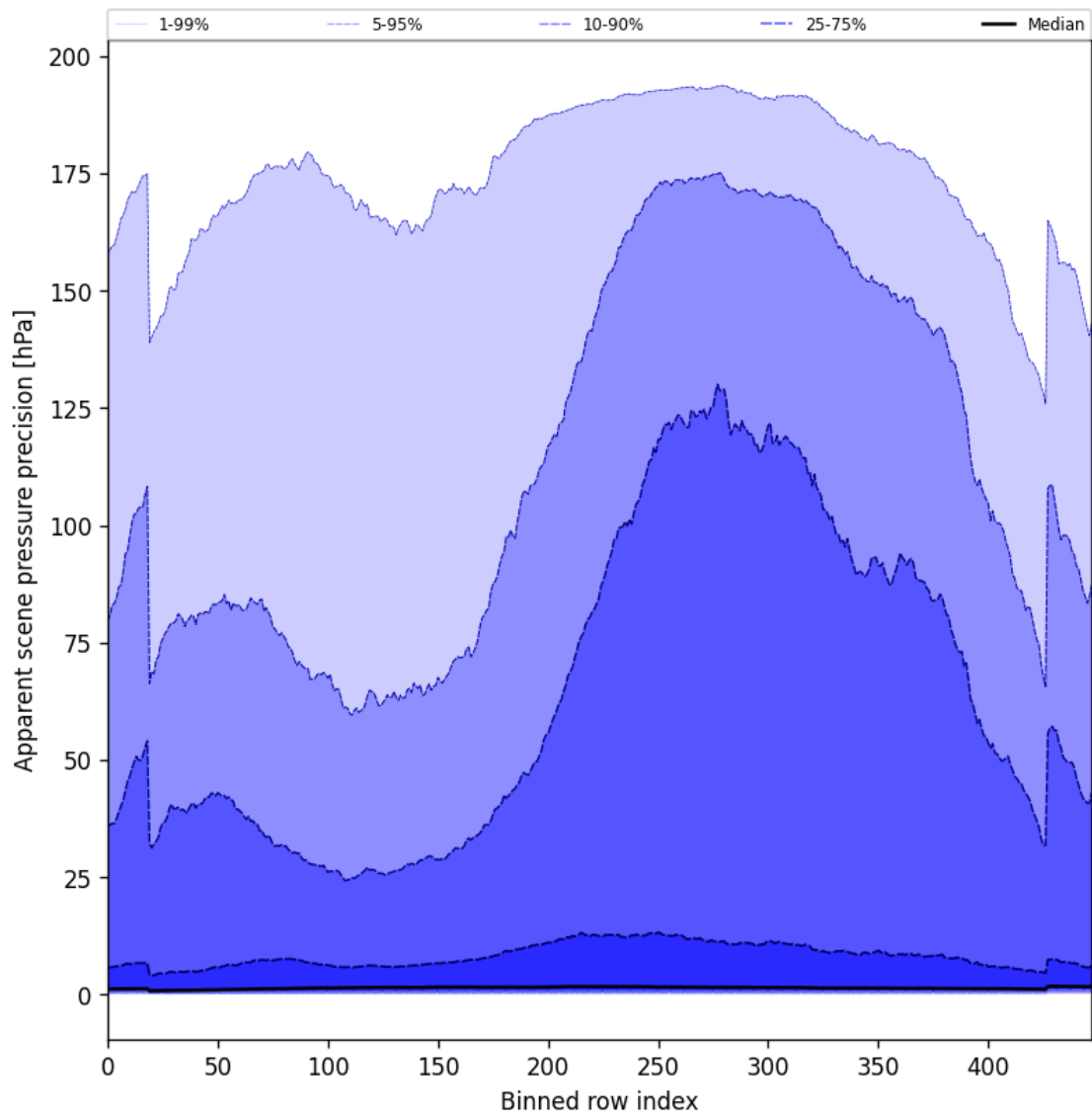
Figure 54: Along track statistics of “Apparent scene pressure precision” for 2024-11-05 to 2024-11-07
