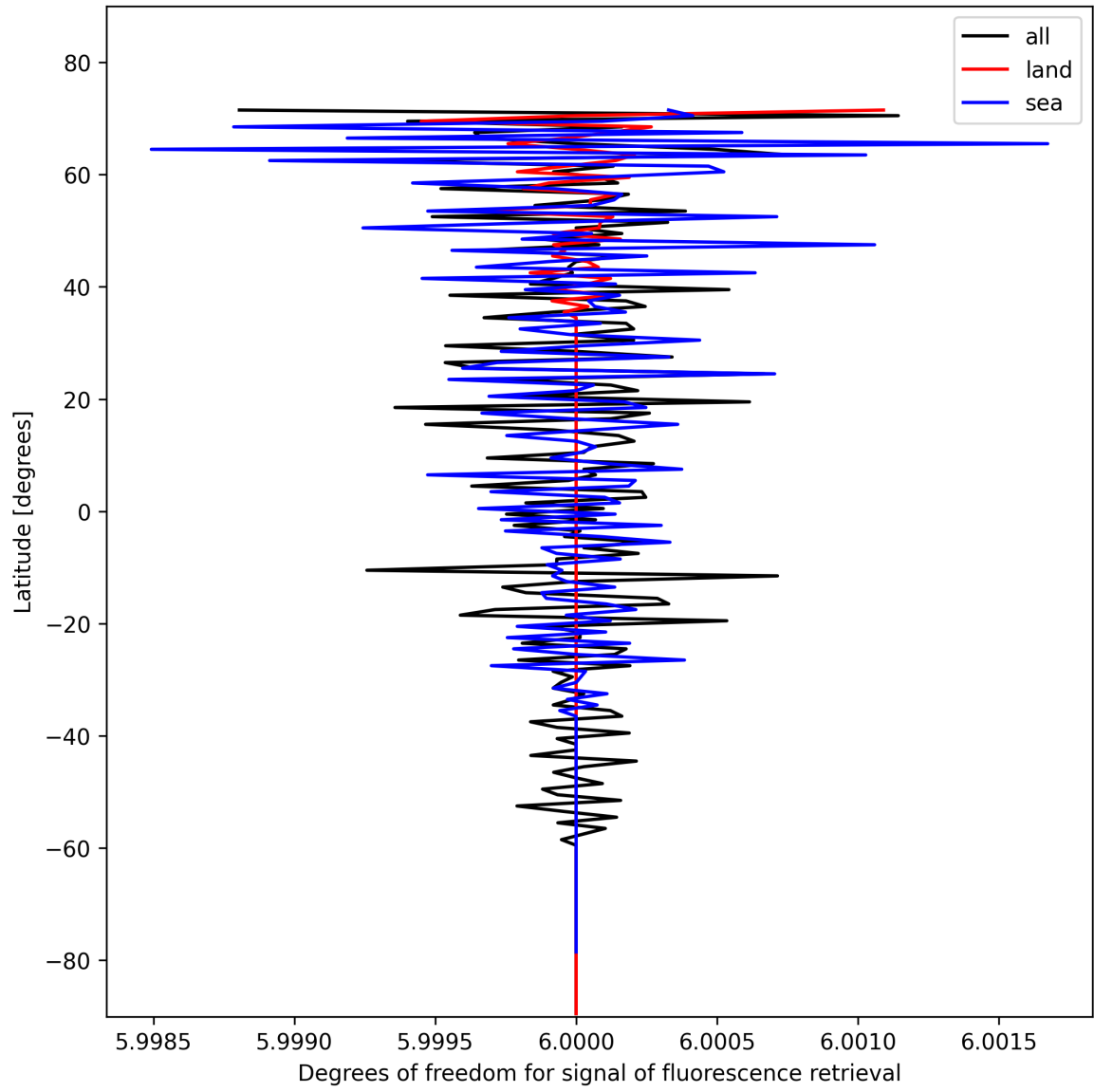
Figure 26: Zonal average of “Degrees of freedom for signal of fluorescence retrieval” for 2024-11-05 to 2024-11-07.
