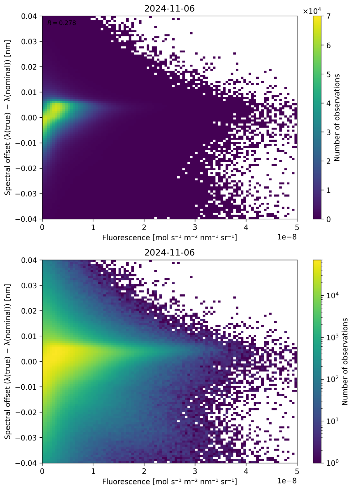
Figure 95: Scatter density plot of “Fluorescence” against “Spectral offset ( \lambda_{\text{true}} - \lambda_{\text{nominal}} )” for 2024-11-05 to 2024-11-07.
