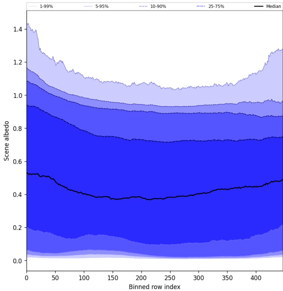
Figure 51: Along track statistics of “Scene albedo” for 2024-11-05 to 2024-11-07
