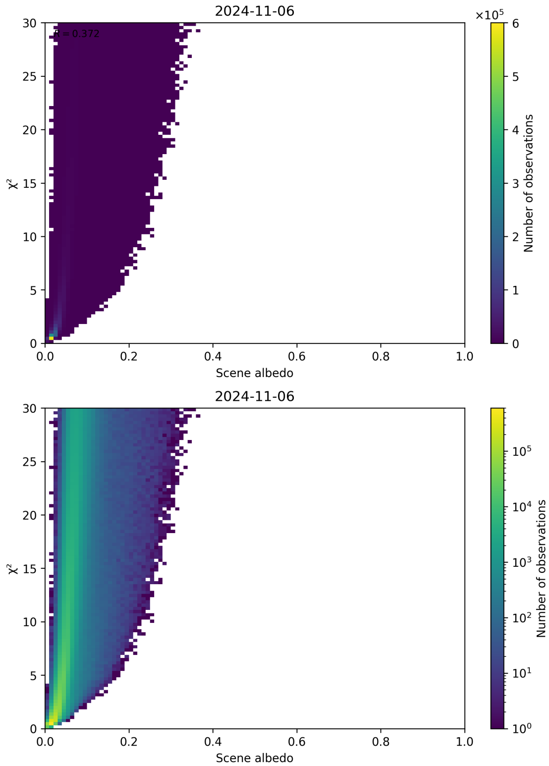
Figure 112: Scatter density plot of “Scene albedo” against “ \chi^2 ” for 2024-11-05 to 2024-11-07.
