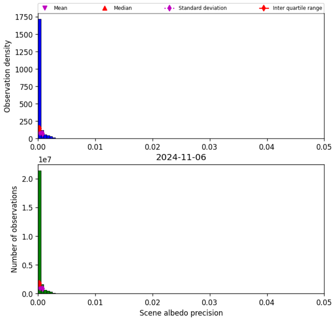
Figure 35: Histogram of “Scene albedo precision” for 2024-11-05 to 2024-11-07
