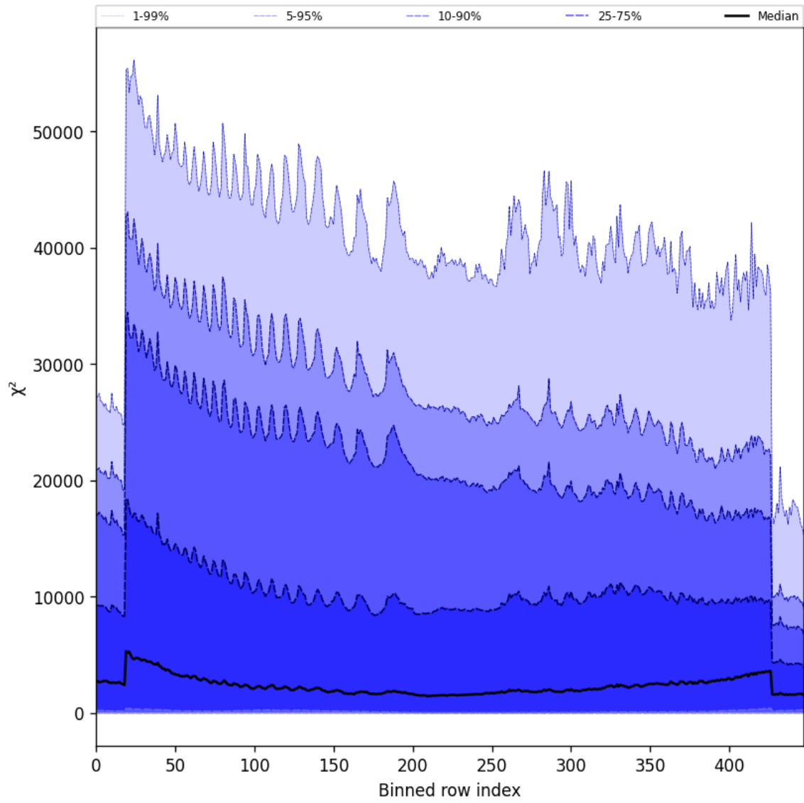
Figure 55: Along track statistics of “ \chi^2 ” for 2024-11-05 to 2024-11-07
