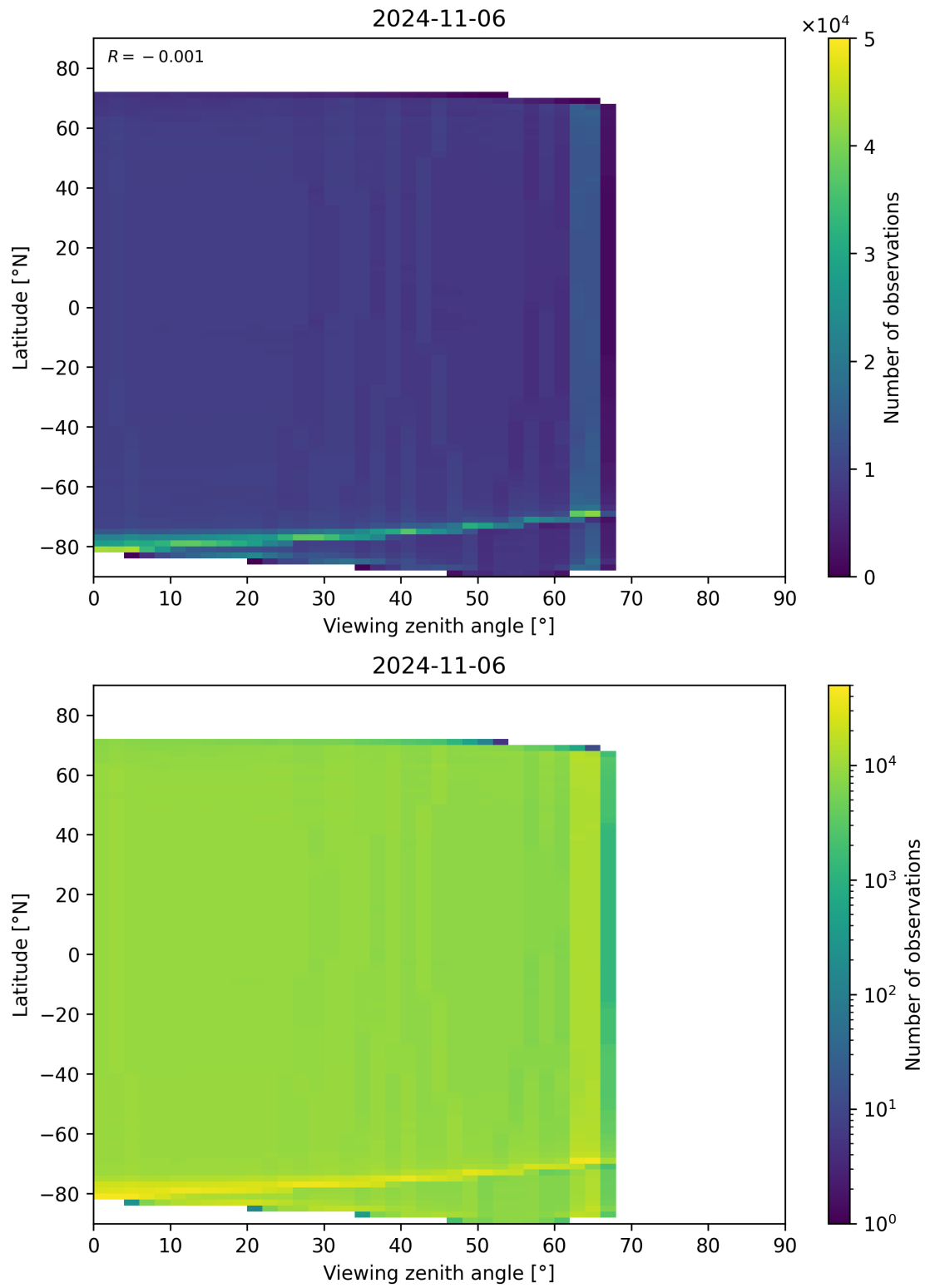
Figure 135: Scatter density plot of “Viewing zenith angle” against “Latitude” for 2024-11-05 to 2024-11-07.
