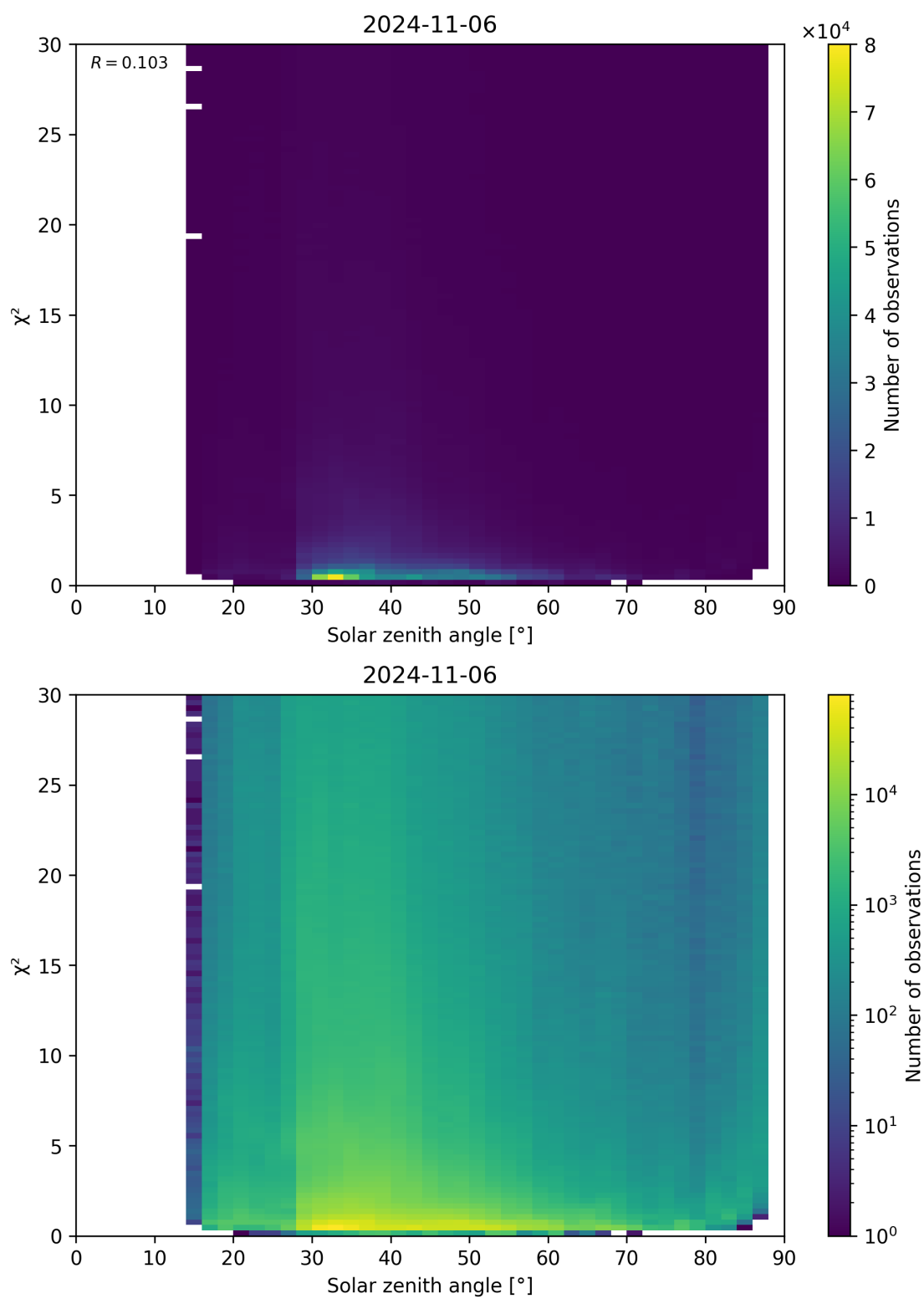
Figure 119: Scatter density plot of “Solar zenith angle” against “ \chi^2 ” for 2024-11-05 to 2024-11-07.
