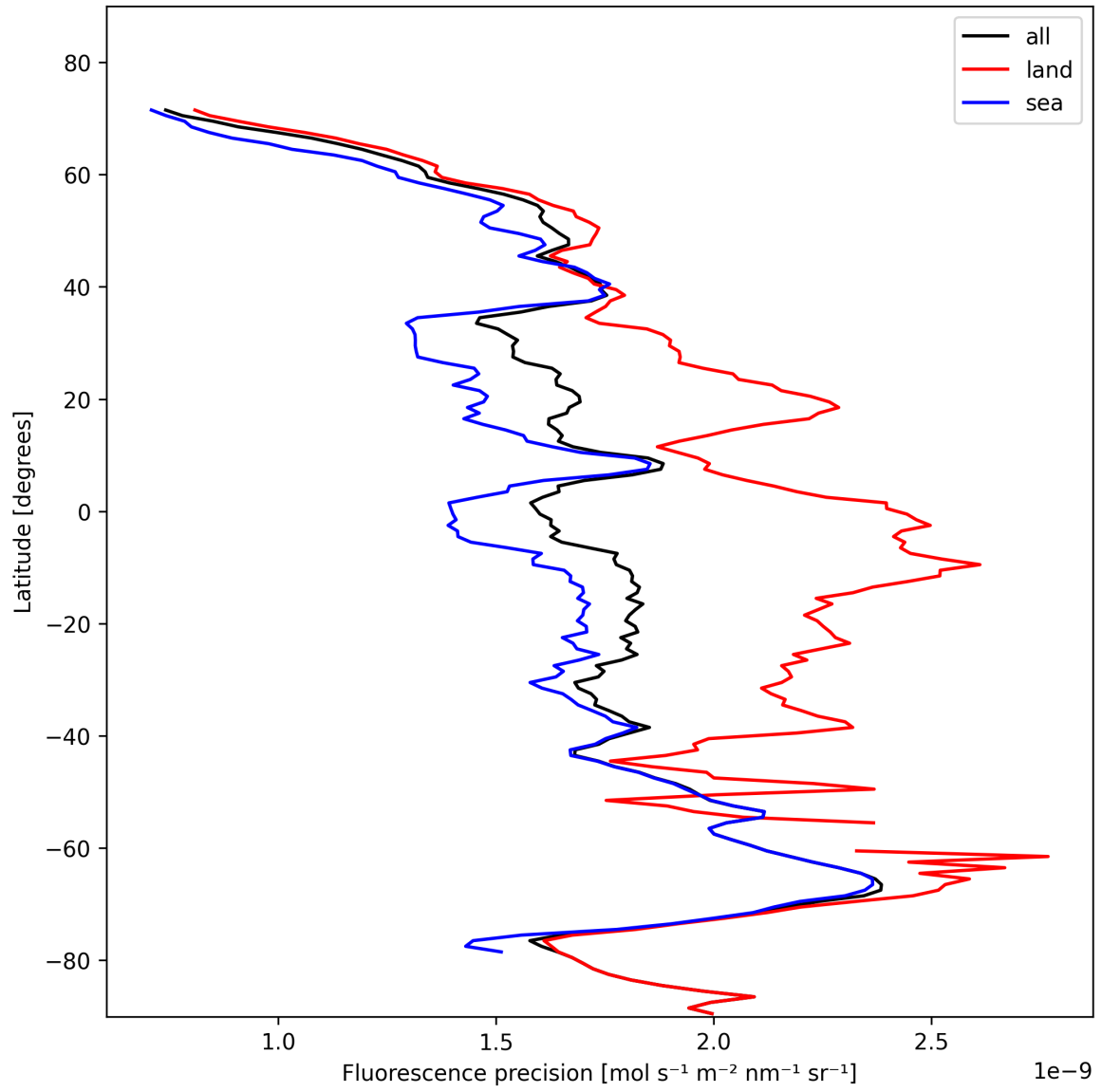
Figure 24: Zonal average of “Fluorescence precision” for 2024-11-05 to 2024-11-07.
