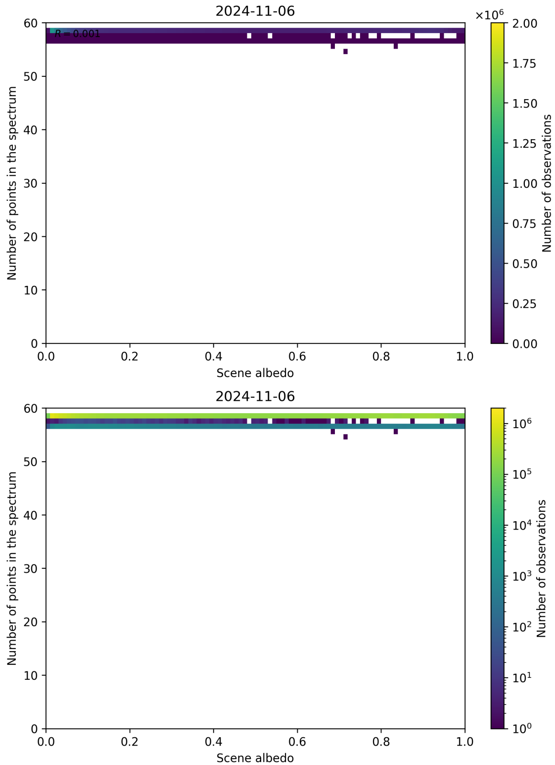
Figure 116: Scatter density plot of “Scene albedo” against “Number of points in the spectrum” for 2024-11-05 to 2024-11-07.
