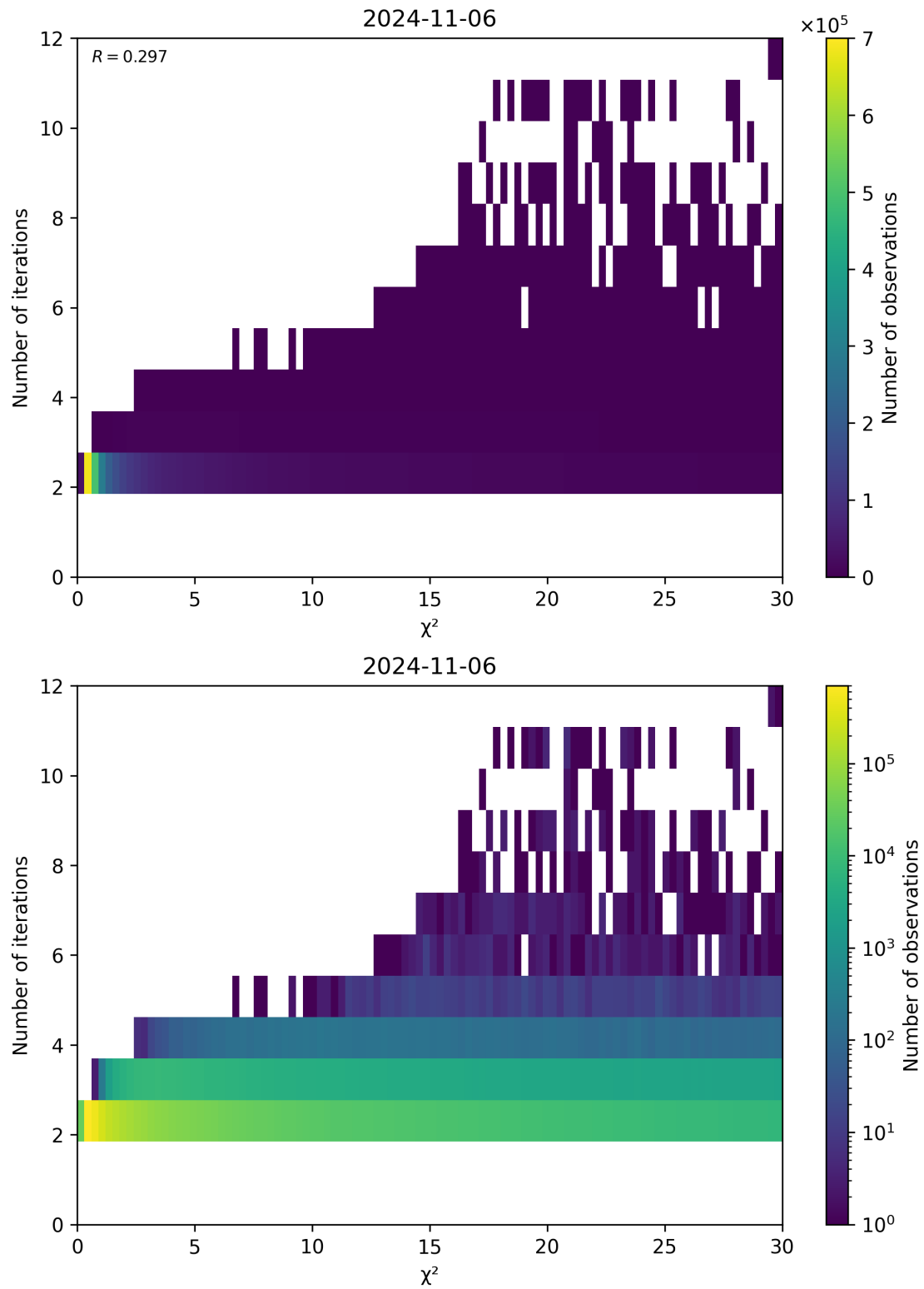
Figure 73: Scatter density plot of “ \chi^2 ” against “Number of iterations” for 2024-11-05 to 2024-11-07.
