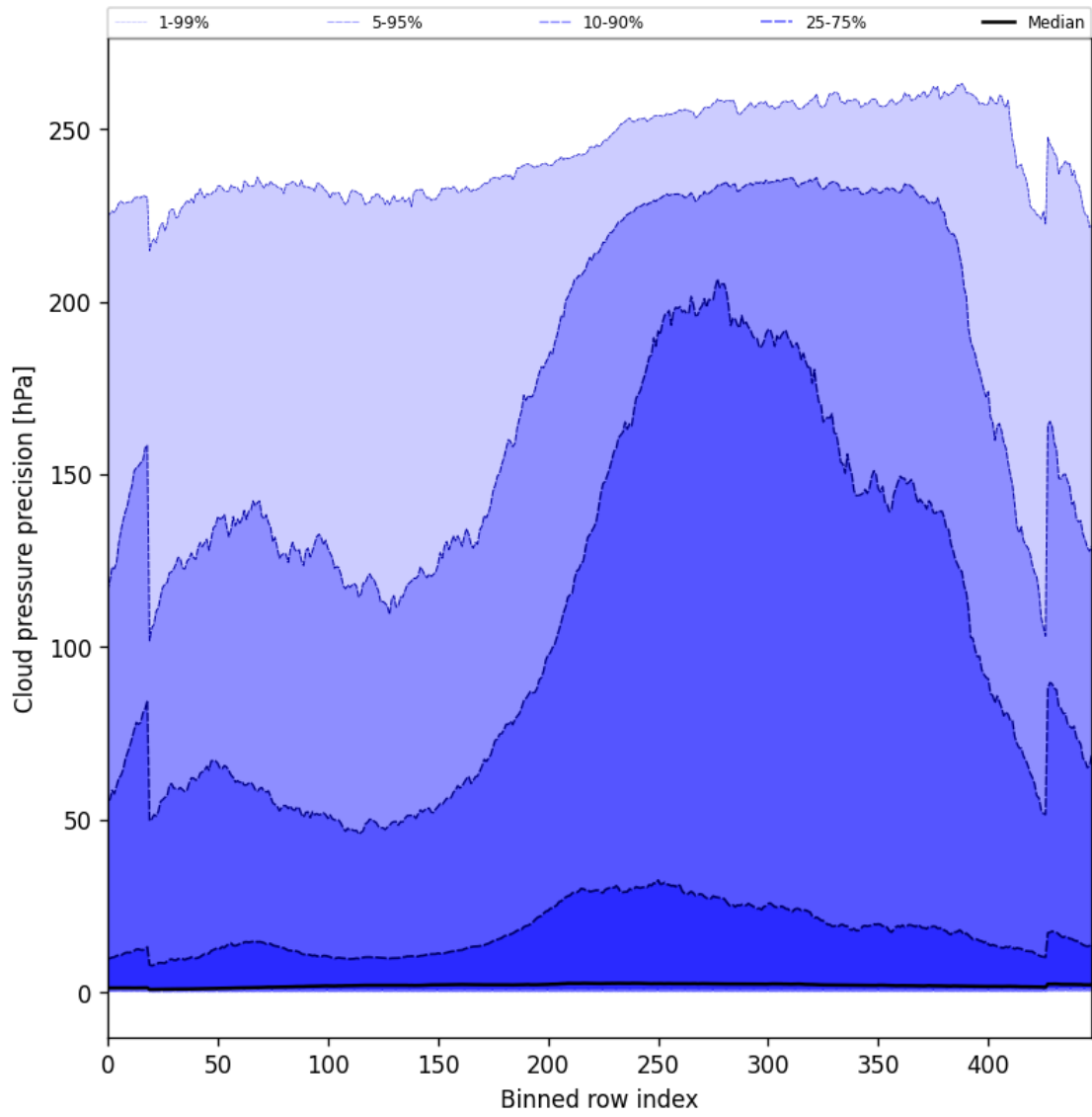
Figure 48: Along track statistics of “Cloud pressure precision” for 2024-11-05 to 2024-11-07
