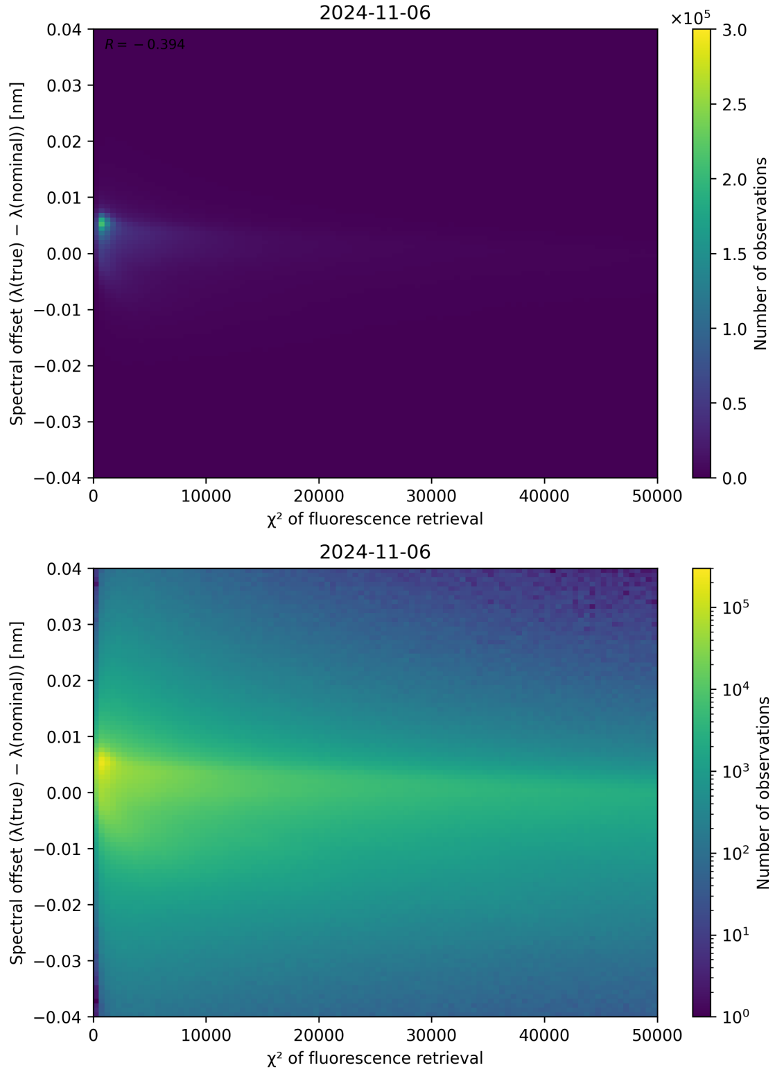
Figure 72: Scatter density plot of “ \chi^2 of fluorescence retrieval” against “Spectral offset ( \lambda_{\text{true}} - \lambda_{\text{nominal}} )” for 2024-11-05 to 2024-11-07.
