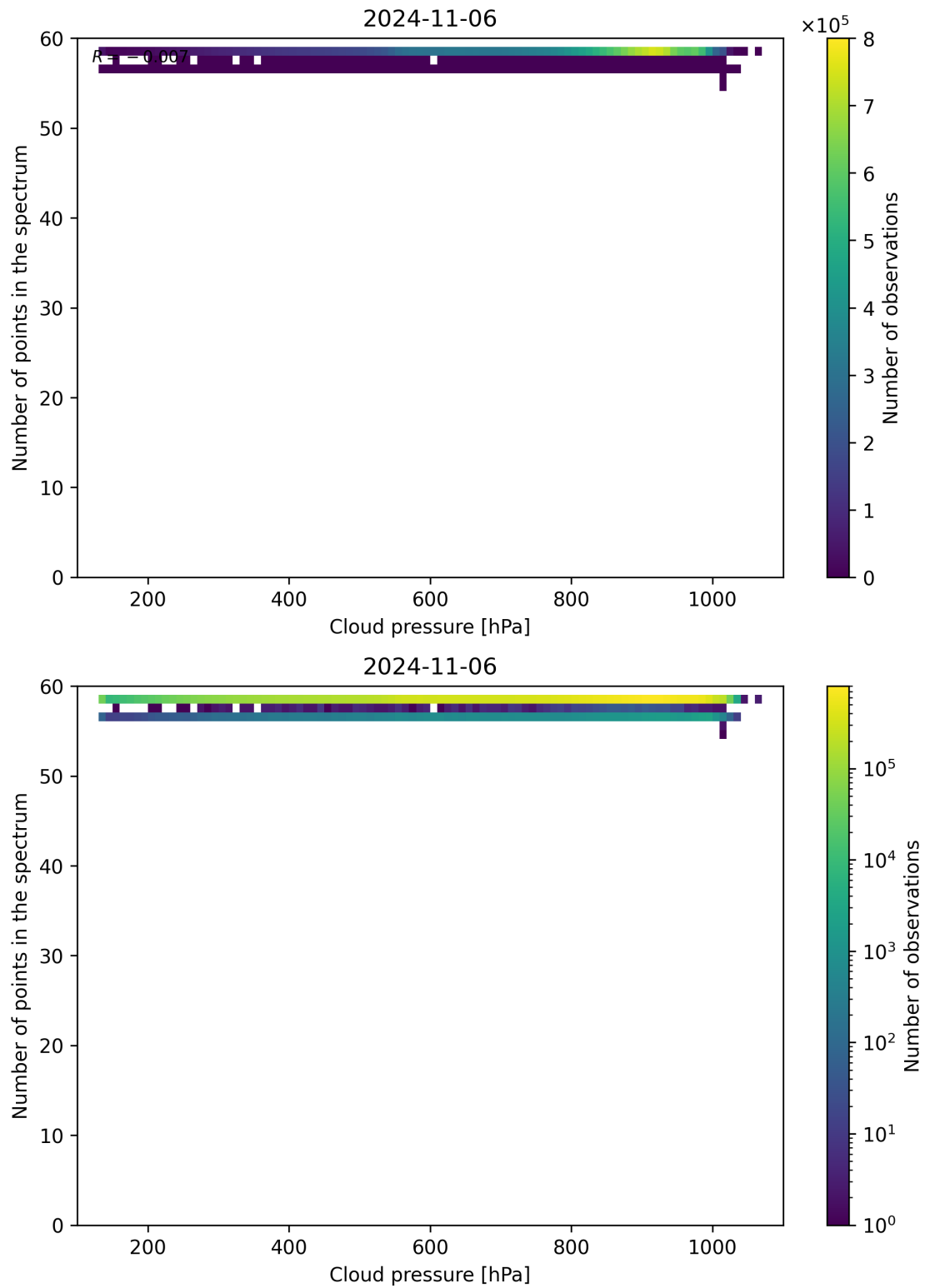
Figure 90: Scatter density plot of “Cloud pressure” against “Number of points in the spectrum” for 2024-11-05 to 2024-11-07.
