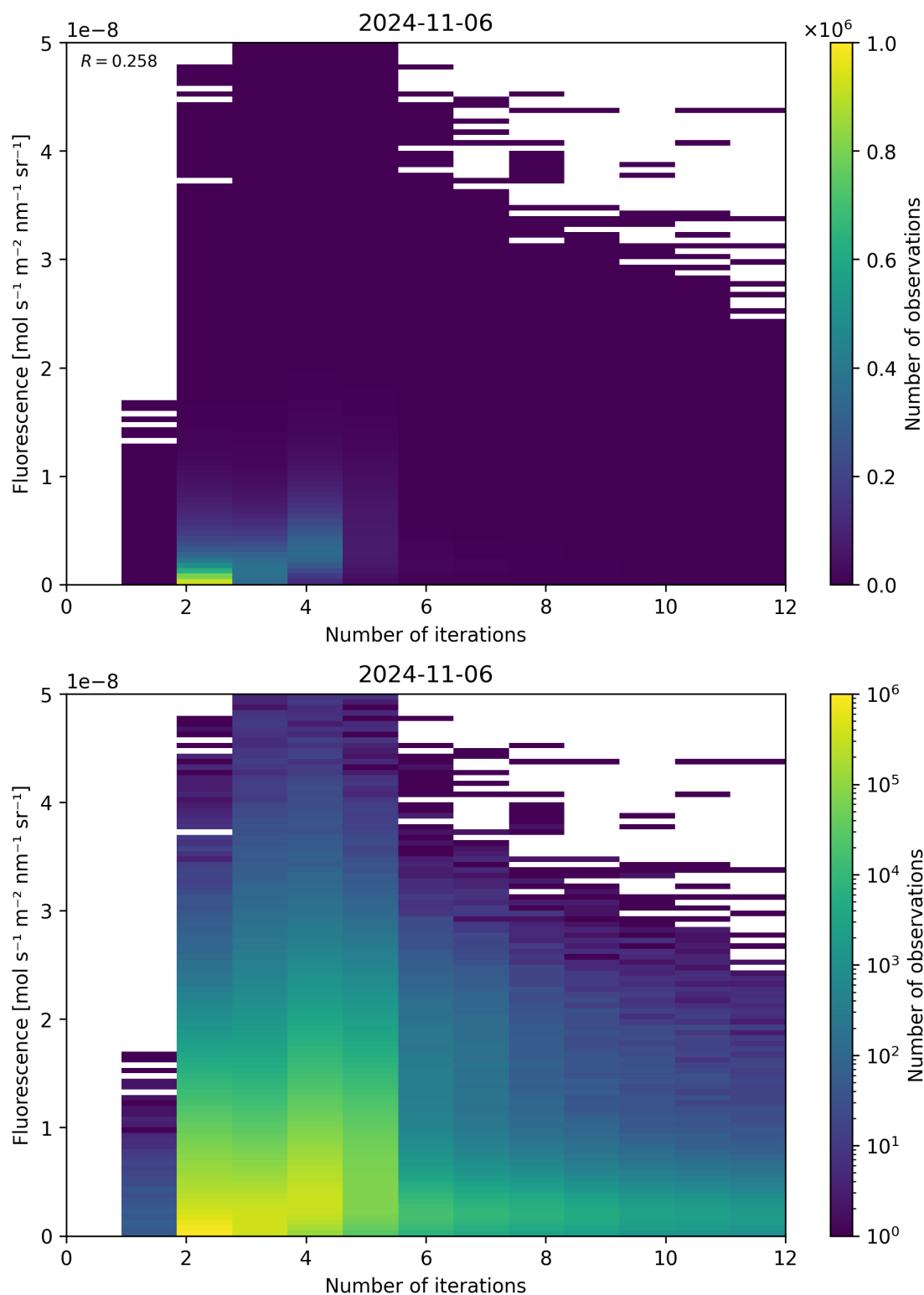
Figure 107: Scatter density plot of “Number of iterations” against “Fluorescence” for 2024-11-05 to 2024-11-07.
