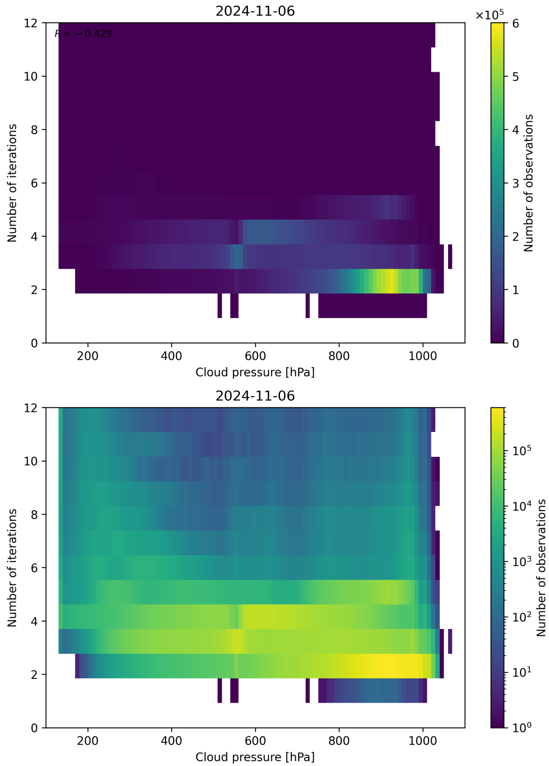
Figure 89: Scatter density plot of “Cloud pressure” against “Number of iterations” for 2024-11-05 to 2024-11-07.
