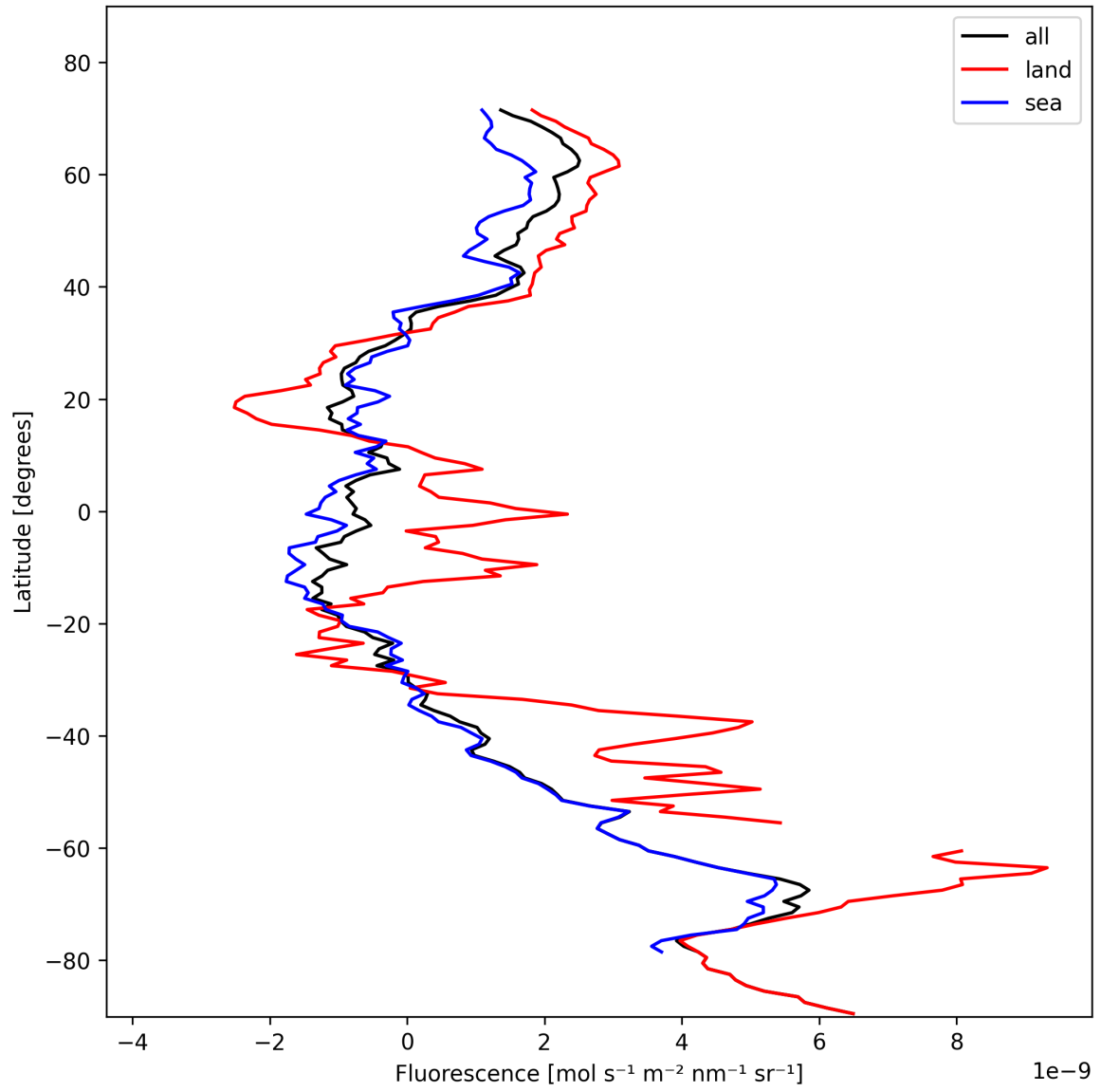
Figure 23: Zonal average of “Fluorescence” for 2024-11-05 to 2024-11-07.
