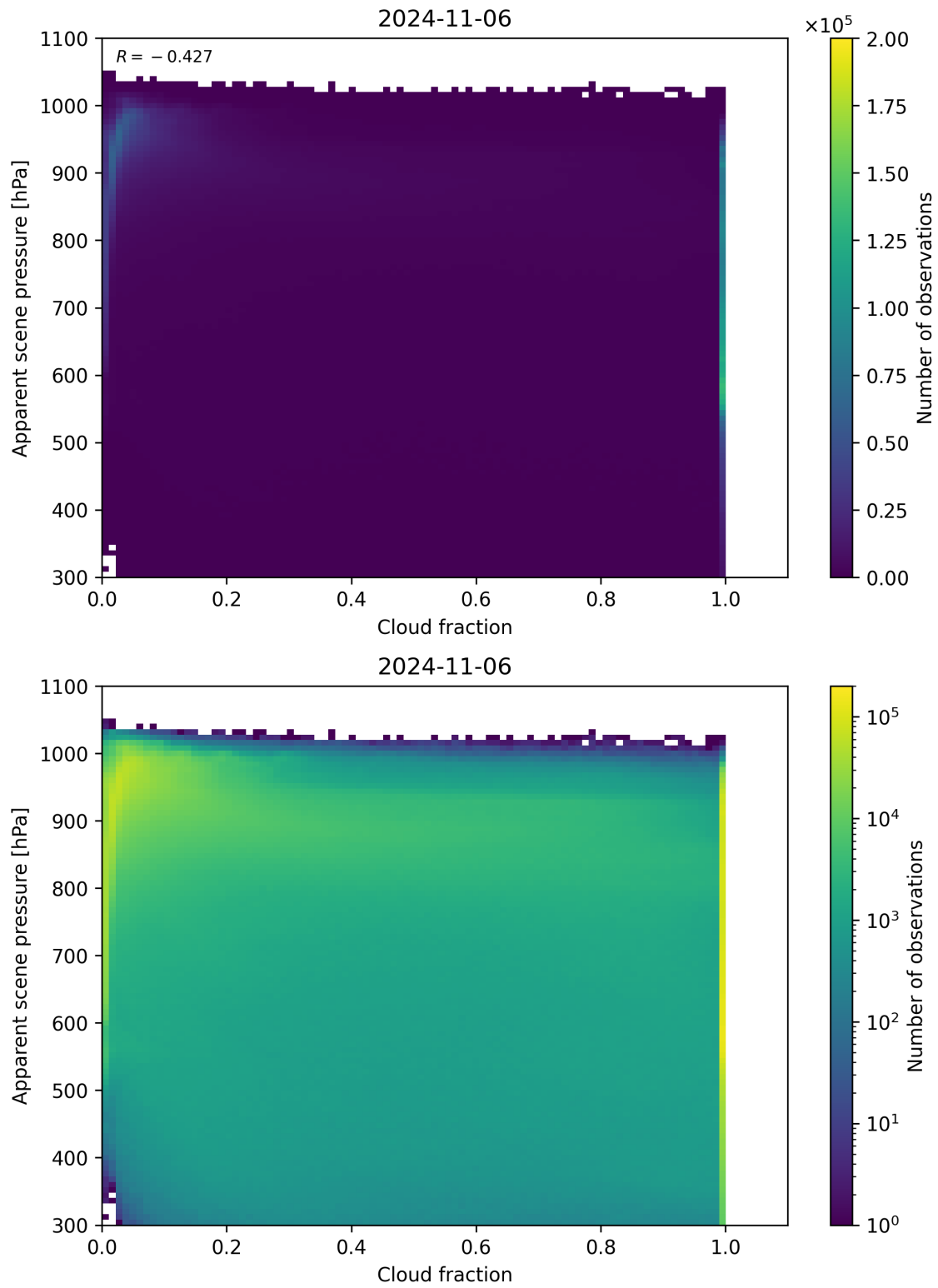
Figure 76: Scatter density plot of “Cloud fraction” against “Apparent scene pressure” for 2024-11-05 to 2024-11-07.
