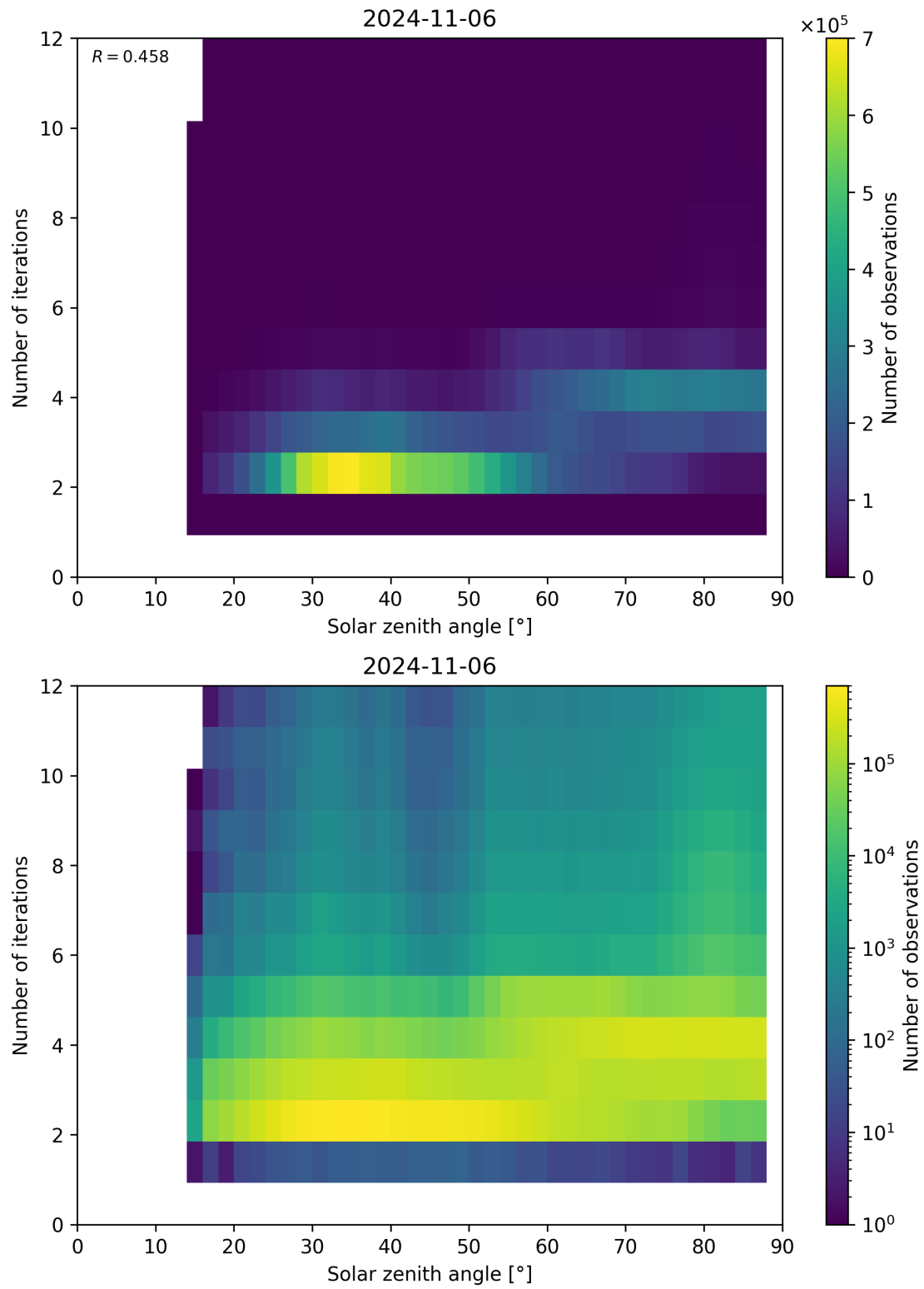
Figure 125: Scatter density plot of “Solar zenith angle” against “Number of iterations” for 2024-11-05 to 2024-11-07.
