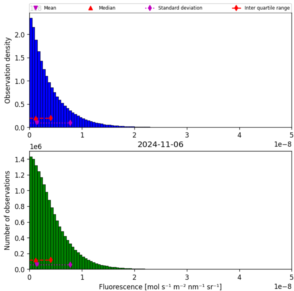
Figure 40: Histogram of “Fluorescence” for 2024-11-05 to 2024-11-07
