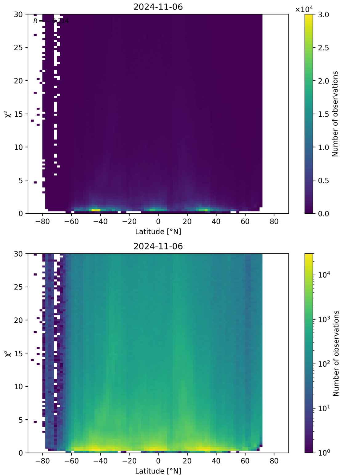
Figure 97: Scatter density plot of “Latitude” against “ \chi^2 ” for 2024-11-05 to 2024-11-07.
