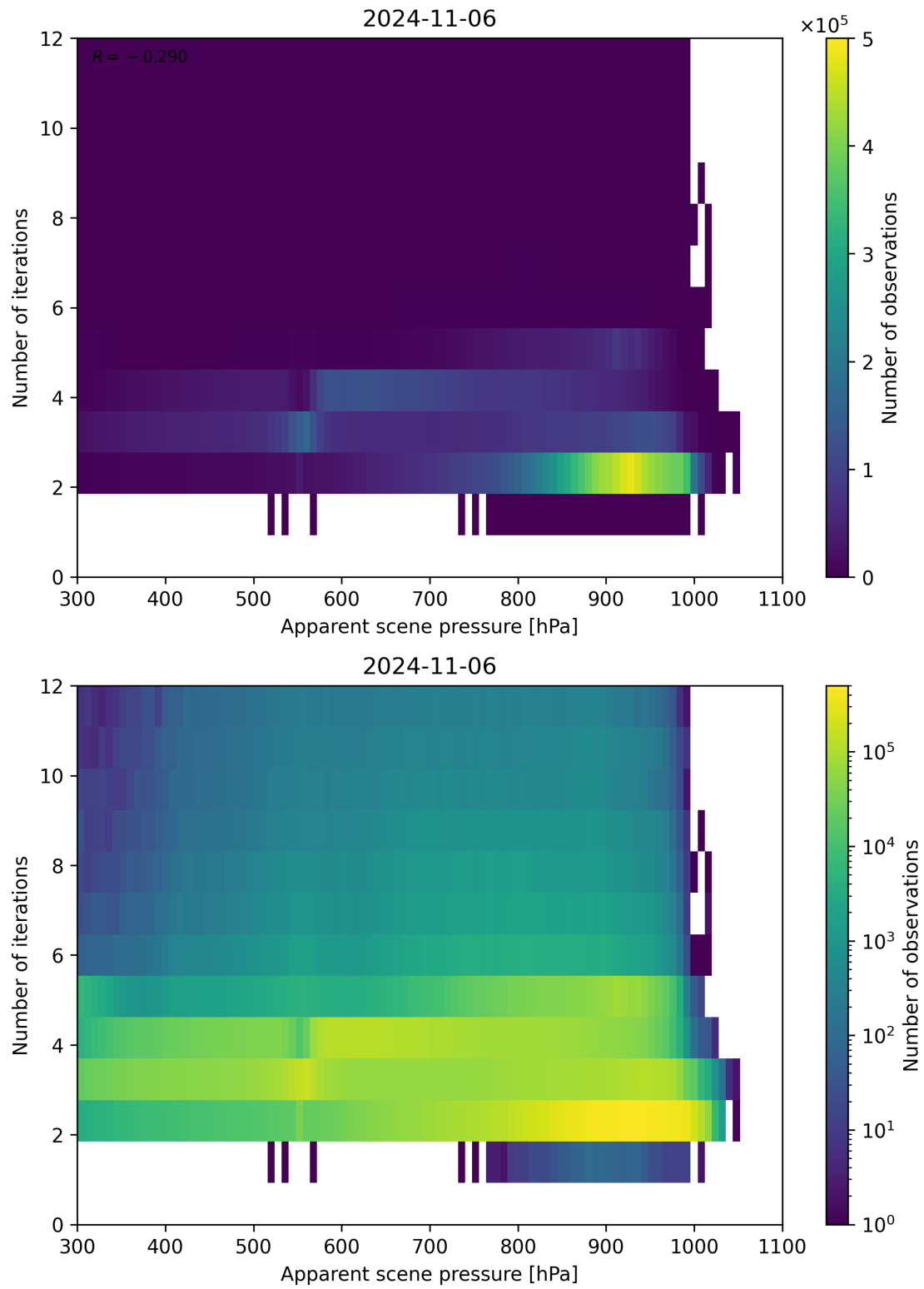
Figure 66: Scatter density plot of “Apparent scene pressure” against “Number of iterations” for 2024-11-05 to 2024-11-07.
