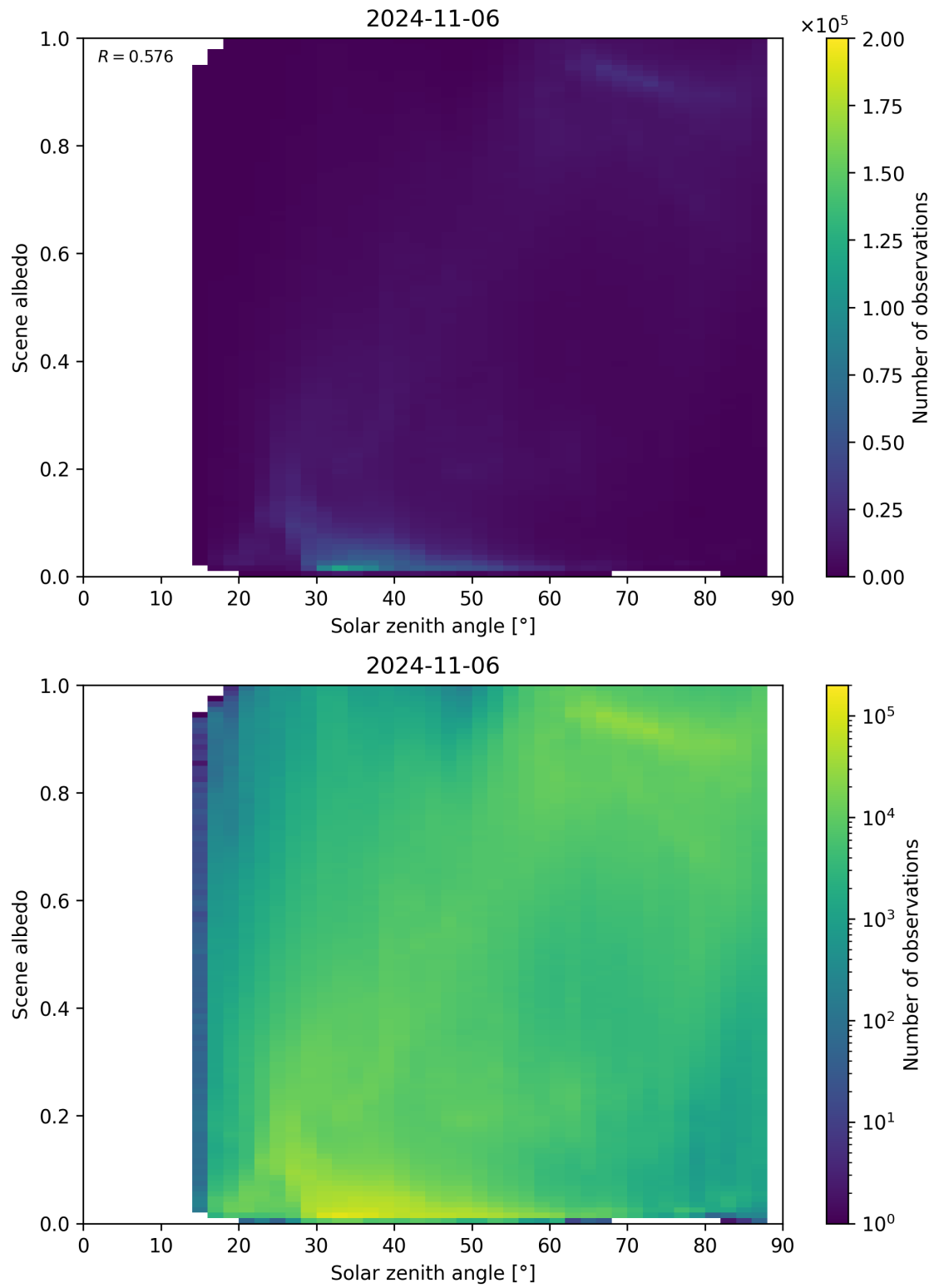
Figure 127: Scatter density plot of “Solar zenith angle” against “Scene albedo” for 2024-11-05 to 2024-11-07.
