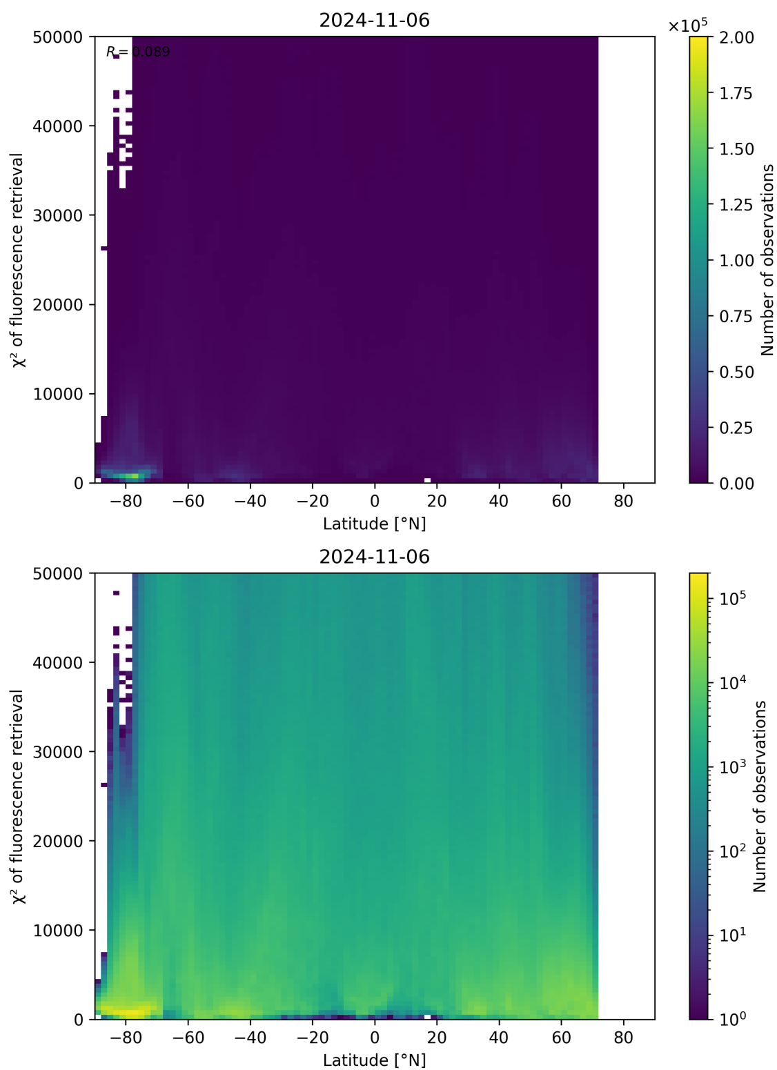
Figure 98: Scatter density plot of “Latitude” against “ \chi^2 of fluorescence retrieval” for 2024-11-05 to 2024-11-07.
