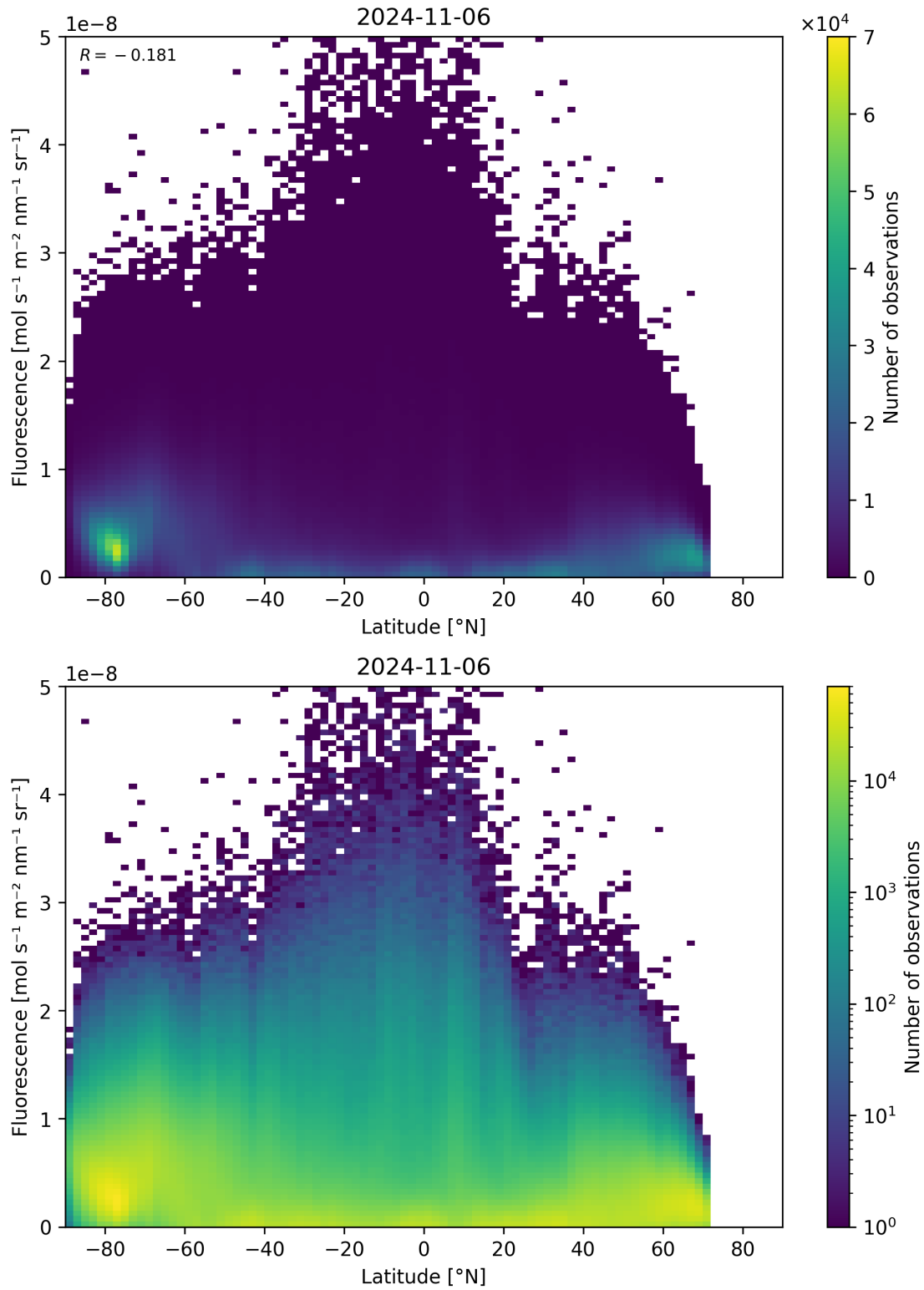
Figure 101: Scatter density plot of “Latitude” against “Fluorescence” for 2024-11-05 to 2024-11-07.
