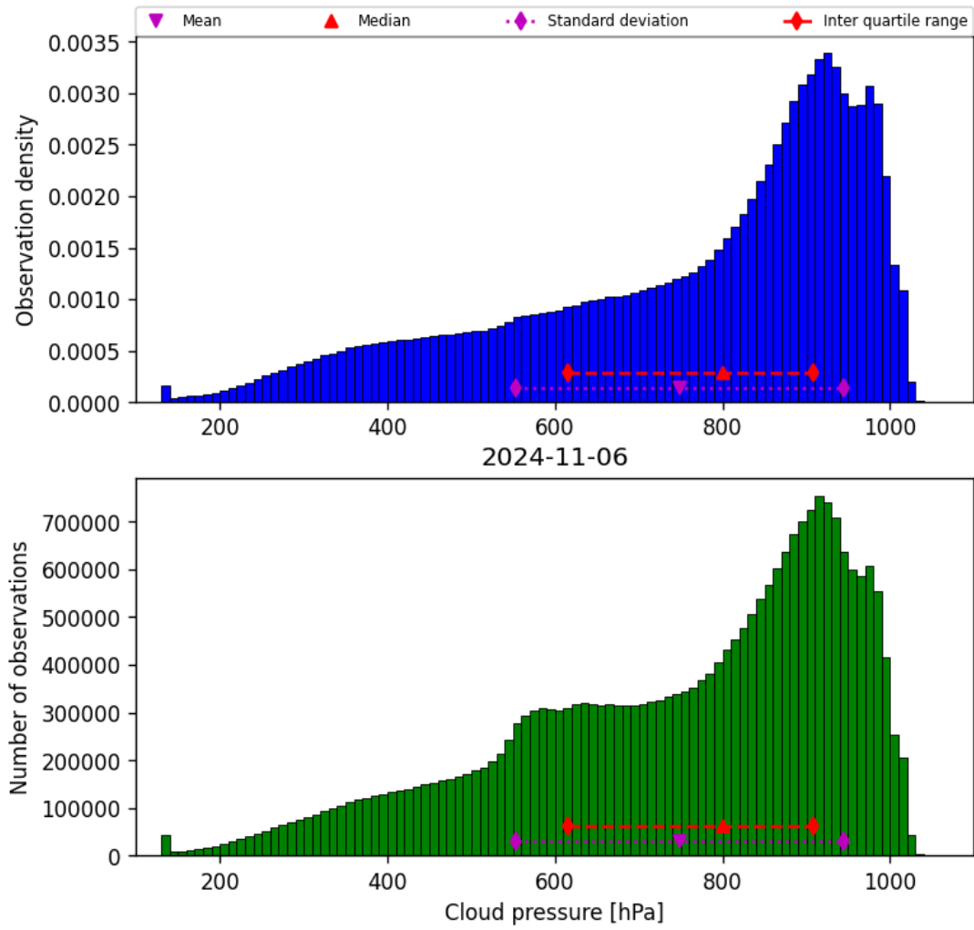
Figure 30: Histogram of “Cloud pressure” for 2024-11-05 to 2024-11-07
