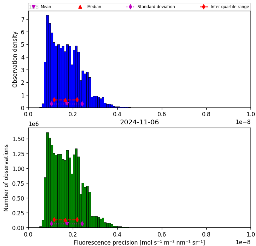
Figure 41: Histogram of “Fluorescence precision” for 2024-11-05 to 2024-11-07
