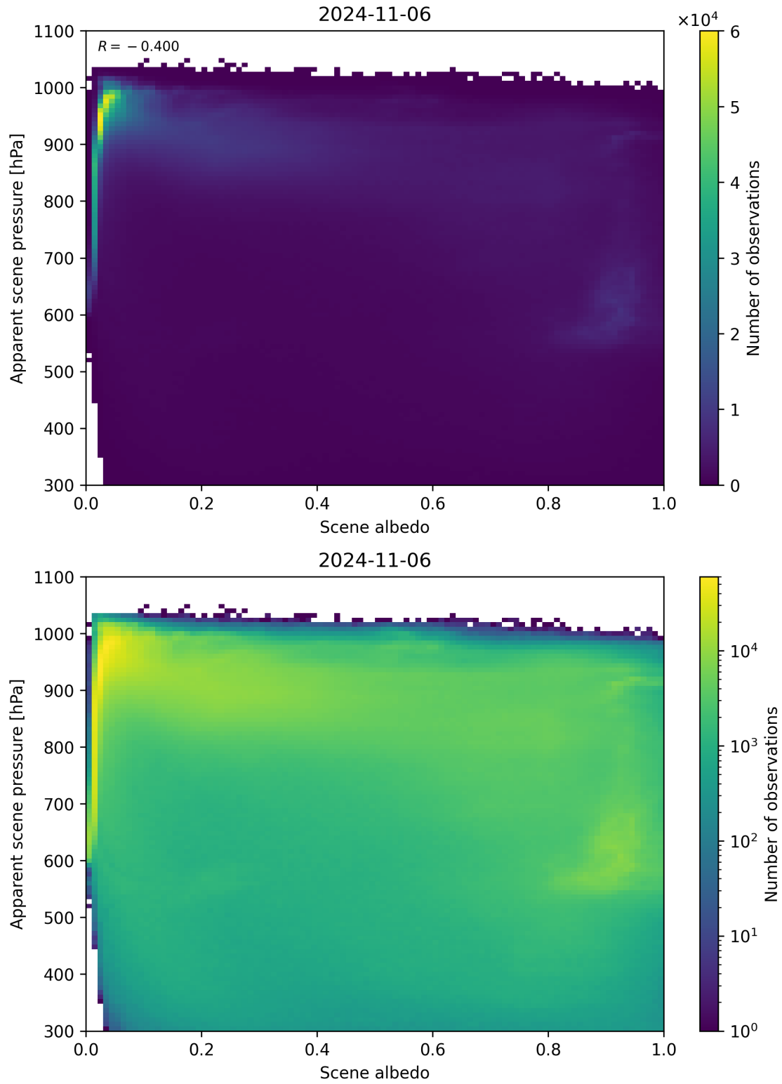
Figure 111: Scatter density plot of “Scene albedo” against “Apparent scene pressure” for 2024-11-05 to 2024-11-07.
