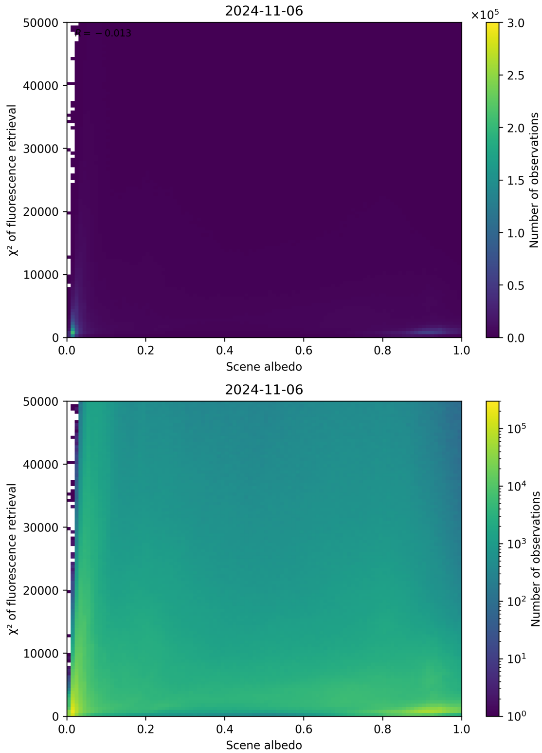
Figure 113: Scatter density plot of “Scene albedo” against “ \chi^2 of fluorescence retrieval” for 2024-11-05 to 2024-11-07.
