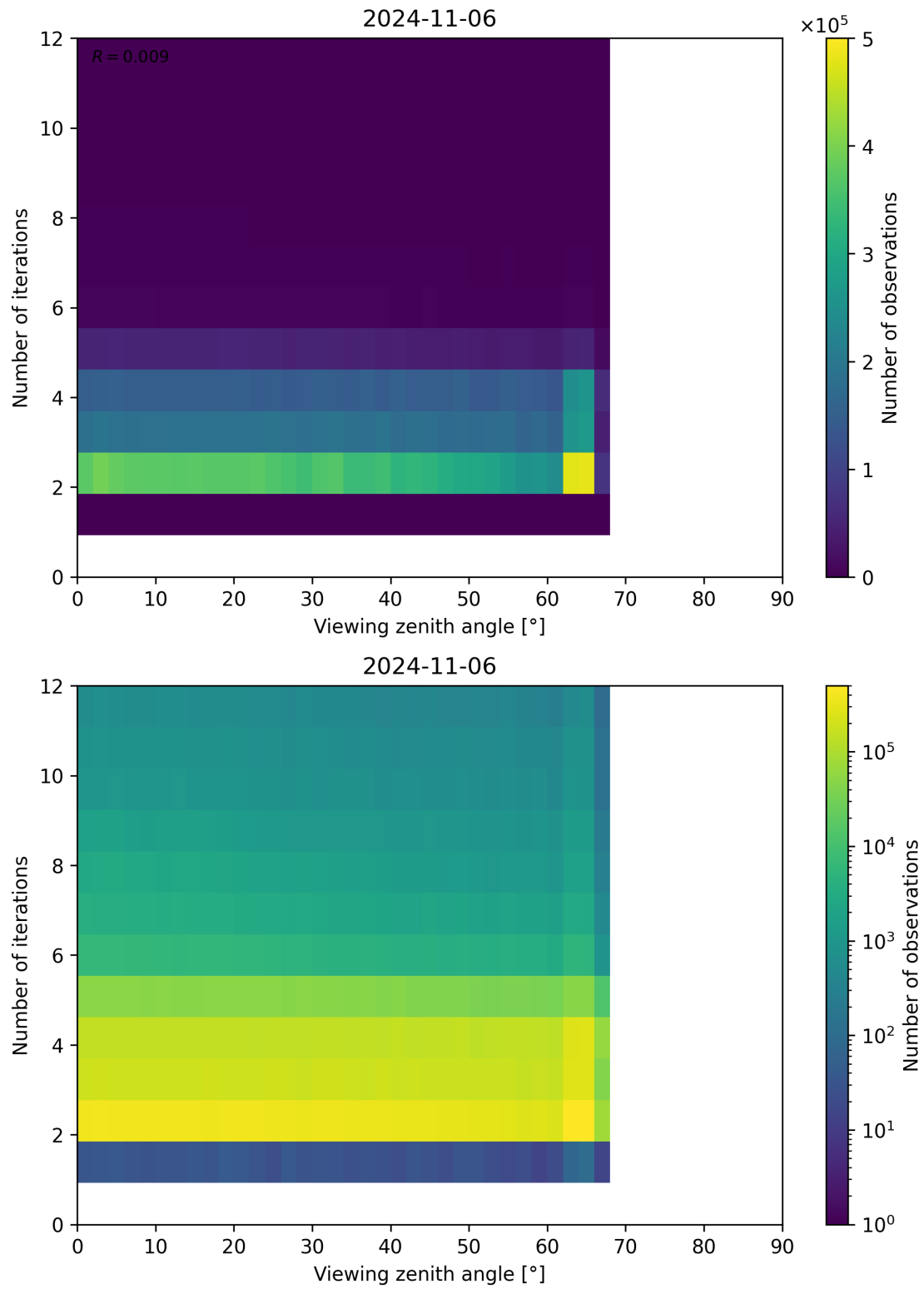
Figure 136: Scatter density plot of “Viewing zenith angle” against “Number of iterations” for 2024-11-05 to 2024-11-07.
