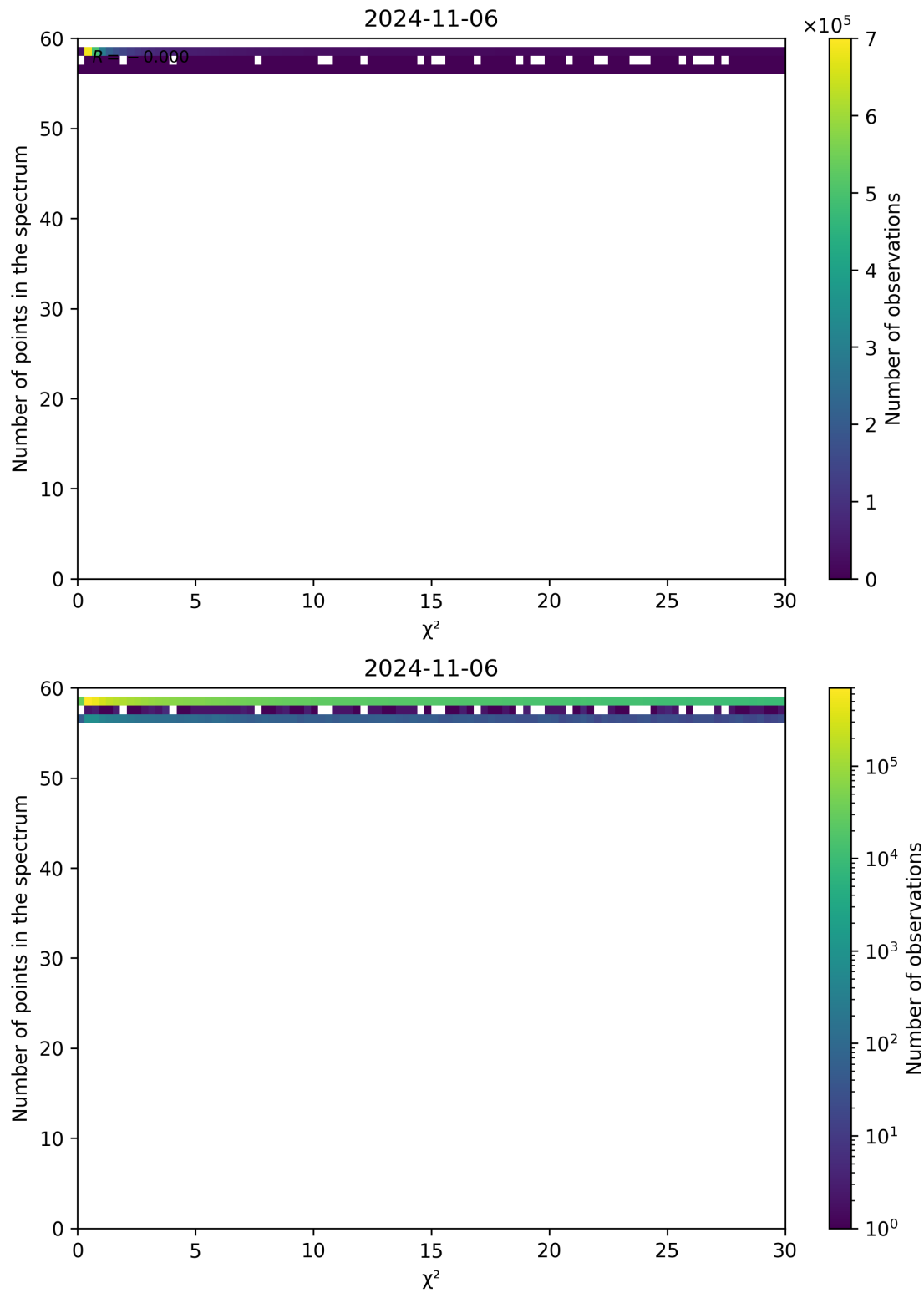
Figure 74: Scatter density plot of “ \chi^2 ” against “Number of points in the spectrum” for 2024-11-05 to 2024-11-07.
