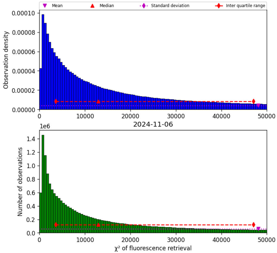
Figure 42: Histogram of “ \chi^2 of fluorescence retrieval” for 2024-11-05 to 2024-11-07
