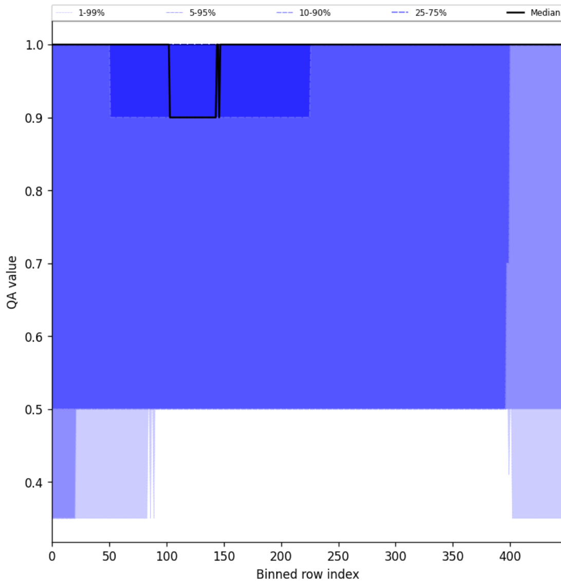
Figure 46: Along track statistics of “QA value” for 2024-11-05 to 2024-11-07
