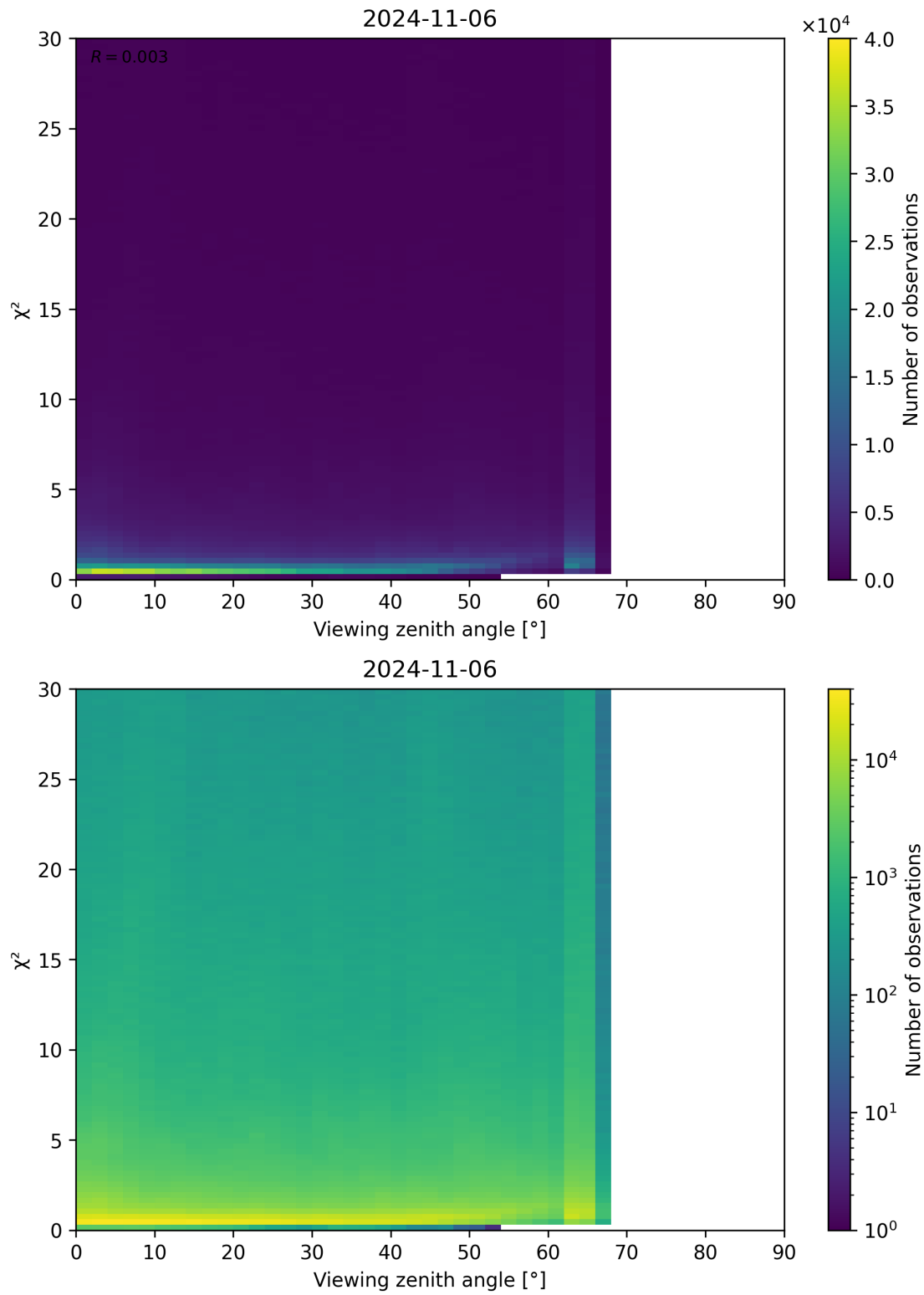
Figure 130: Scatter density plot of “Viewing zenith angle” against “ \chi^2 ” for 2024-11-05 to 2024-11-07.
