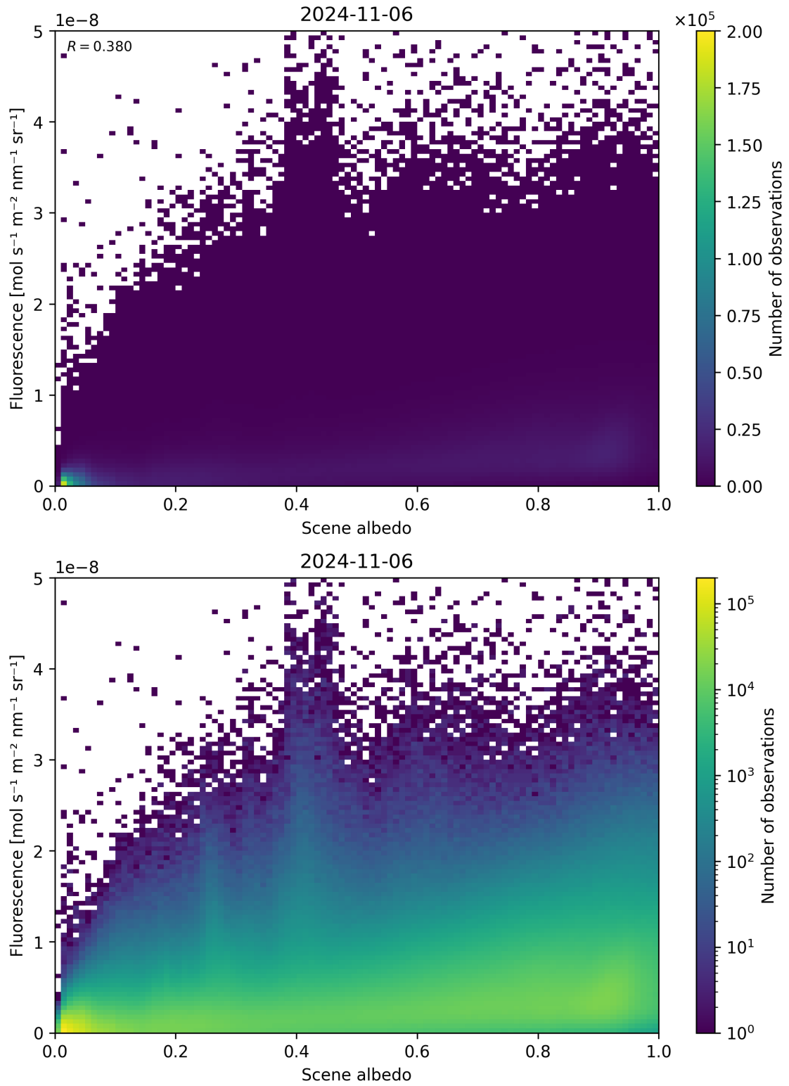
Figure 114: Scatter density plot of “Scene albedo” against “Fluorescence” for 2024-11-05 to 2024-11-07.
