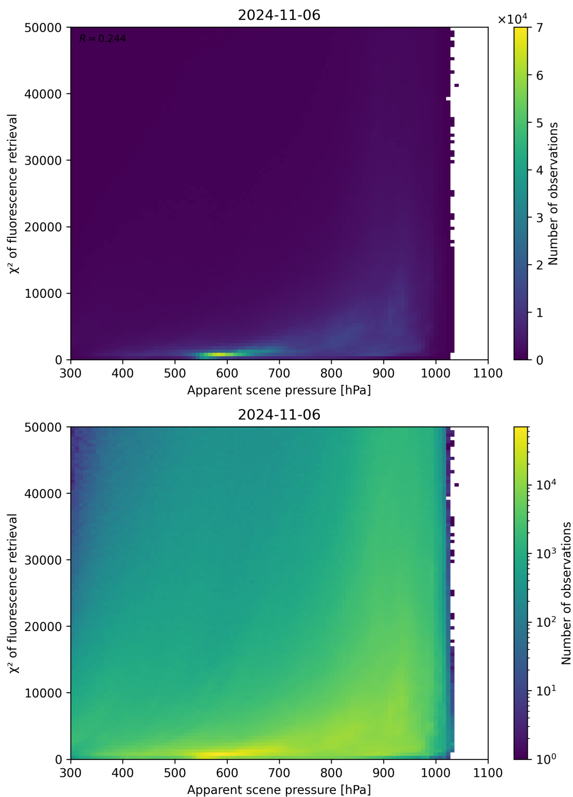
Figure 64: Scatter density plot of “Apparent scene pressure” against “ \chi^2 of fluorescence retrieval” for 2024-11-05 to 2024-11-07.
