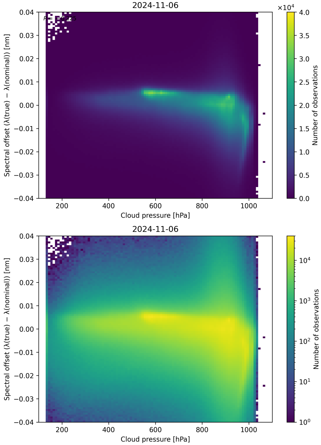
Figure 92: Scatter density plot of “Cloud pressure” against “Spectral offset ( \lambda_{\text{true}} - \lambda_{\text{nominal}} )” for 2024-11-05 to 2024-11-07.
