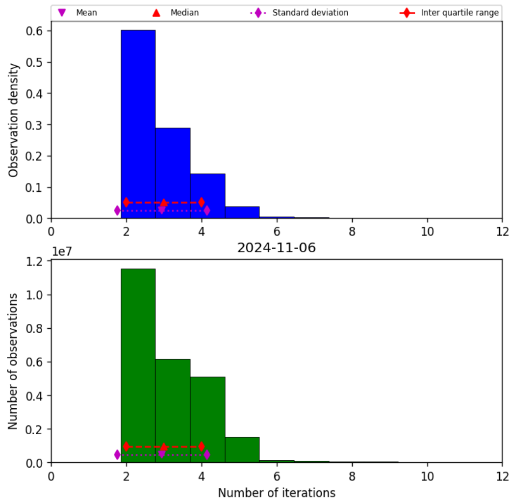
Figure 39: Histogram of “Number of iterations” for 2024-11-05 to 2024-11-07
