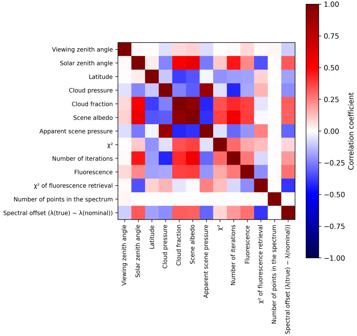
Figure 2: Map of correlation matrix for 2024-11-05 to 2024-11-07.
