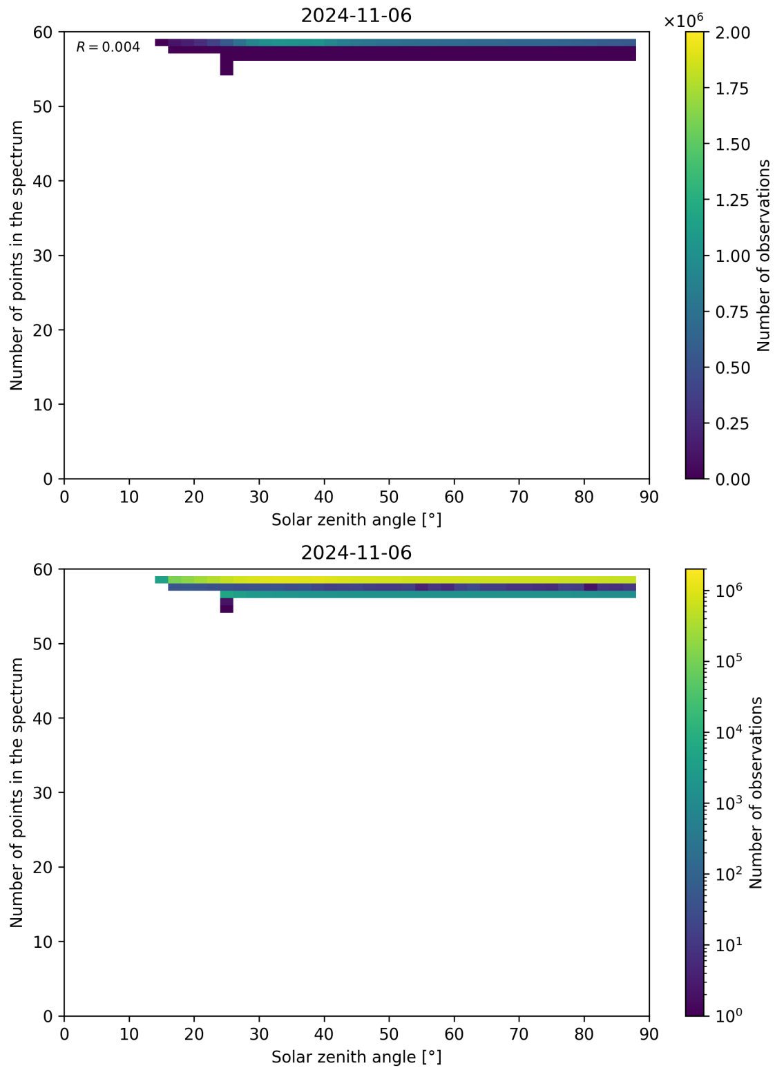
Figure 126: Scatter density plot of “Solar zenith angle” against “Number of points in the spectrum” for 2024-11-05 to 2024-11-07.
