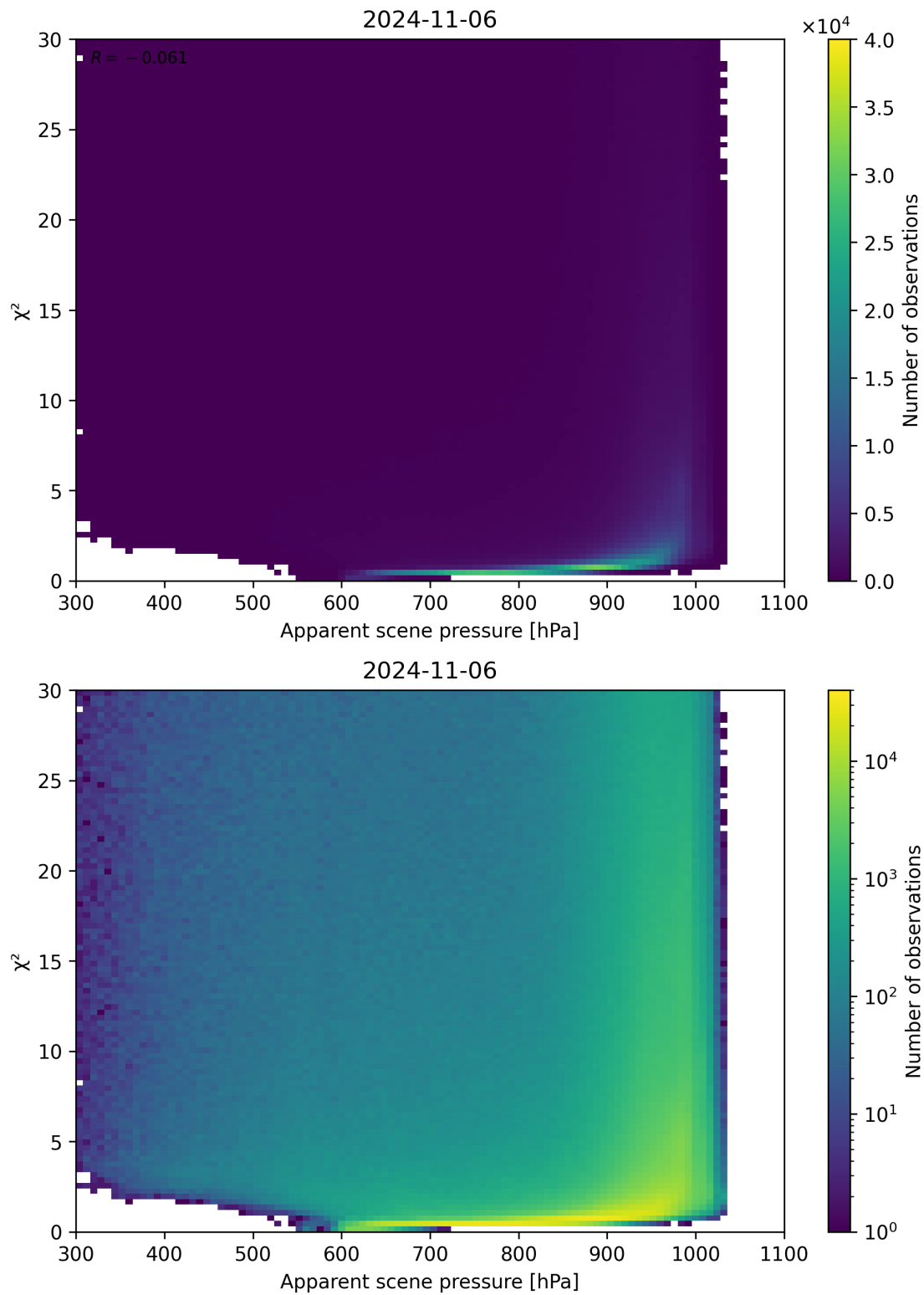
Figure 63: Scatter density plot of “Apparent scene pressure” against “ \chi^2 ” for 2024-11-05 to 2024-11-07.
