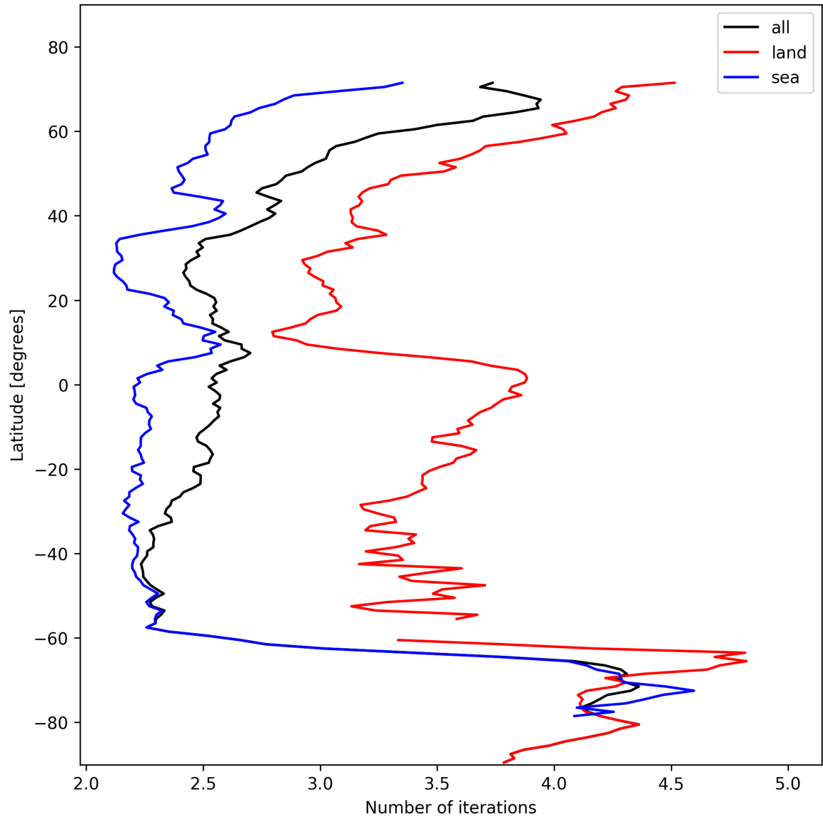
Figure 22: Zonal average of “Number of iterations” for 2024-11-05 to 2024-11-07.
