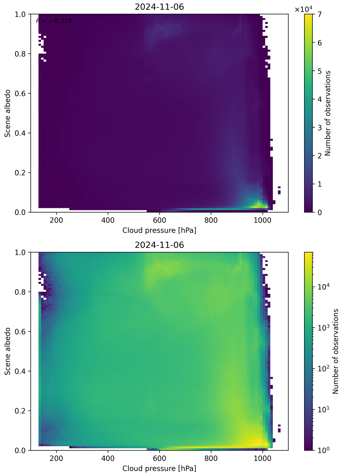
Figure 91: Scatter density plot of “Cloud pressure” against “Scene albedo” for 2024-11-05 to 2024-11-07.
