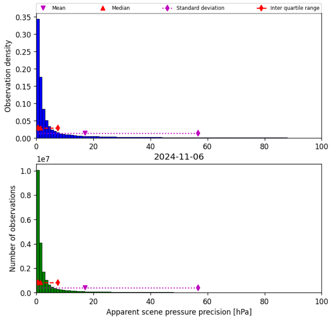
Figure 37: Histogram of “Apparent scene pressure precision” for 2024-11-05 to 2024-11-07
