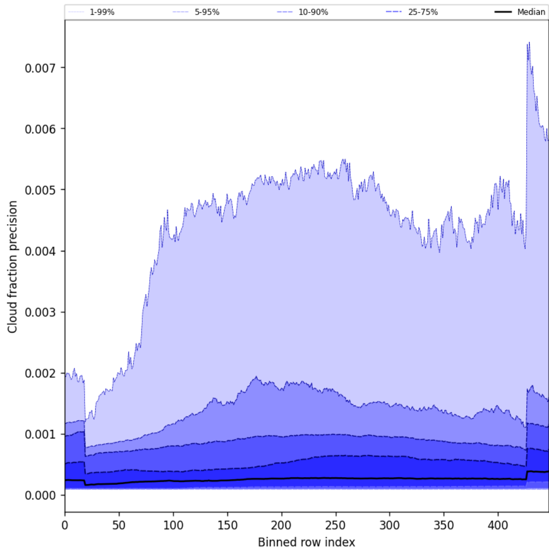
Figure 50: Along track statistics of “Cloud fraction precision” for 2024-11-05 to 2024-11-07
