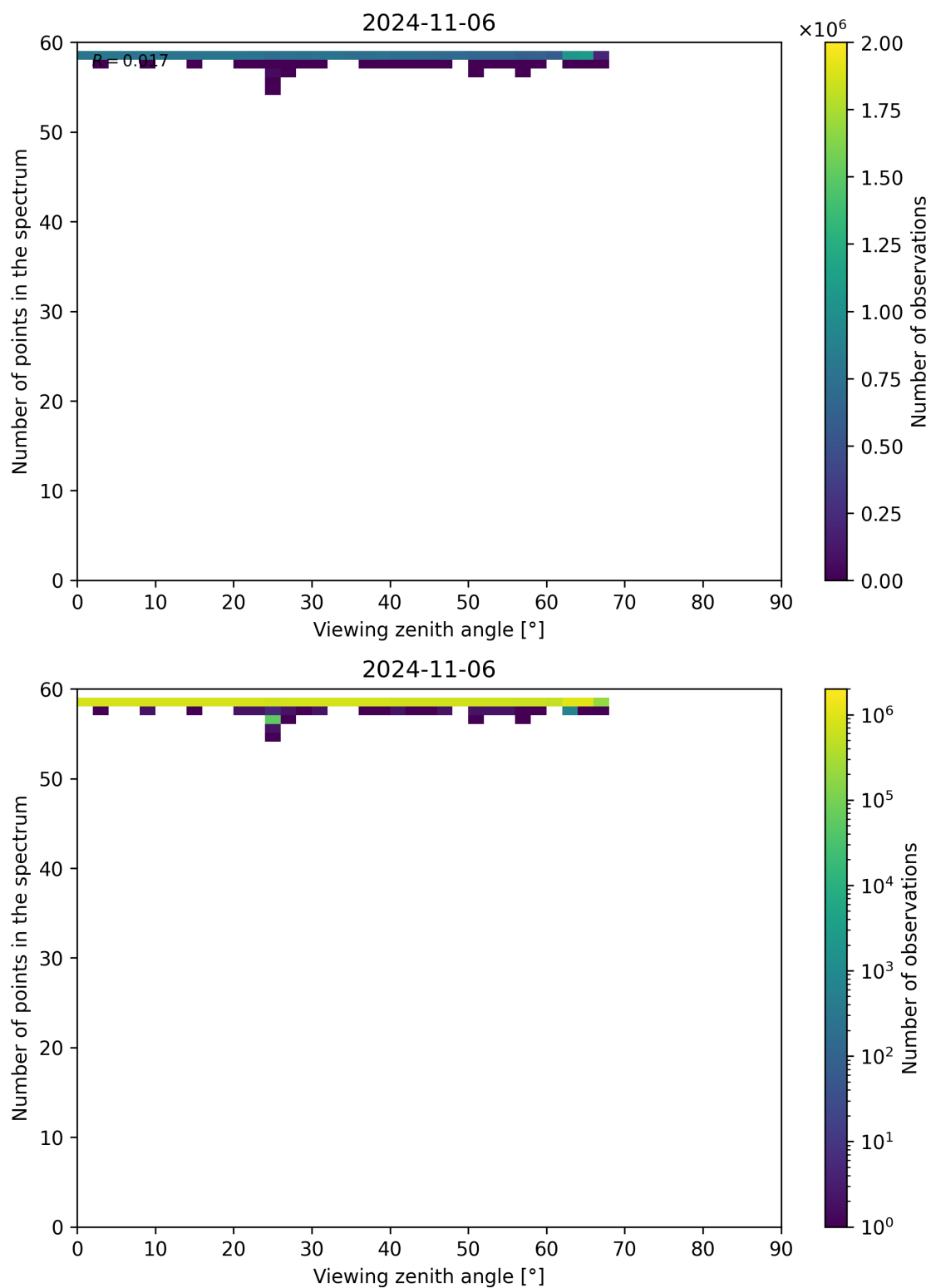
Figure 137: Scatter density plot of “Viewing zenith angle” against “Number of points in the spectrum” for 2024-11-05 to 2024-11-07.
