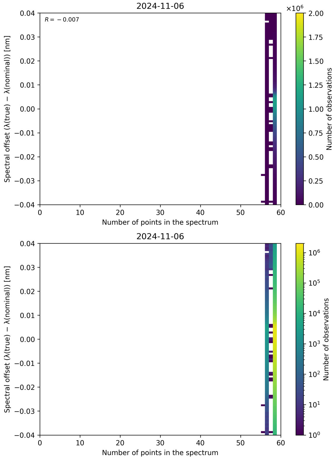
Figure 110: Scatter density plot of “Number of points in the spectrum” against “Spectral offset ( \lambda_{\text{true}} - \lambda_{\text{nominal}} )” for 2024-11-05 to 2024-11-07.
