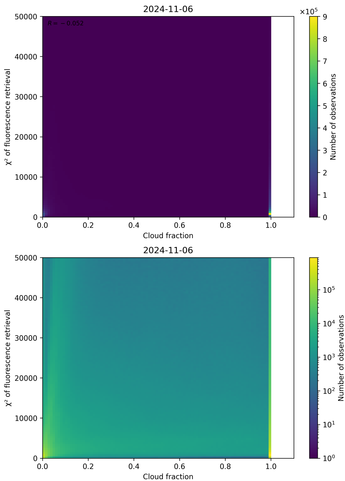
Figure 78: Scatter density plot of “Cloud fraction” against “ \chi^2 of fluorescence retrieval” for 2024-11-05 to 2024-11-07.
