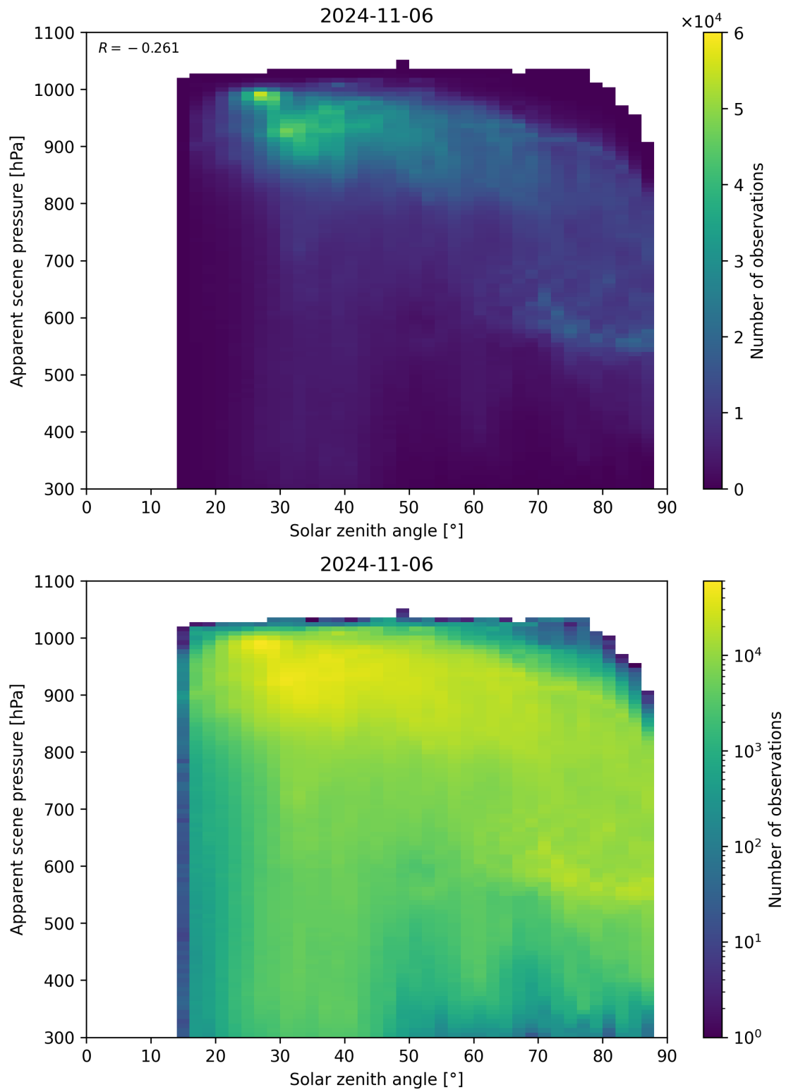
Figure 118: Scatter density plot of “Solar zenith angle” against “Apparent scene pressure” for 2024-11-05 to 2024-11-07.
