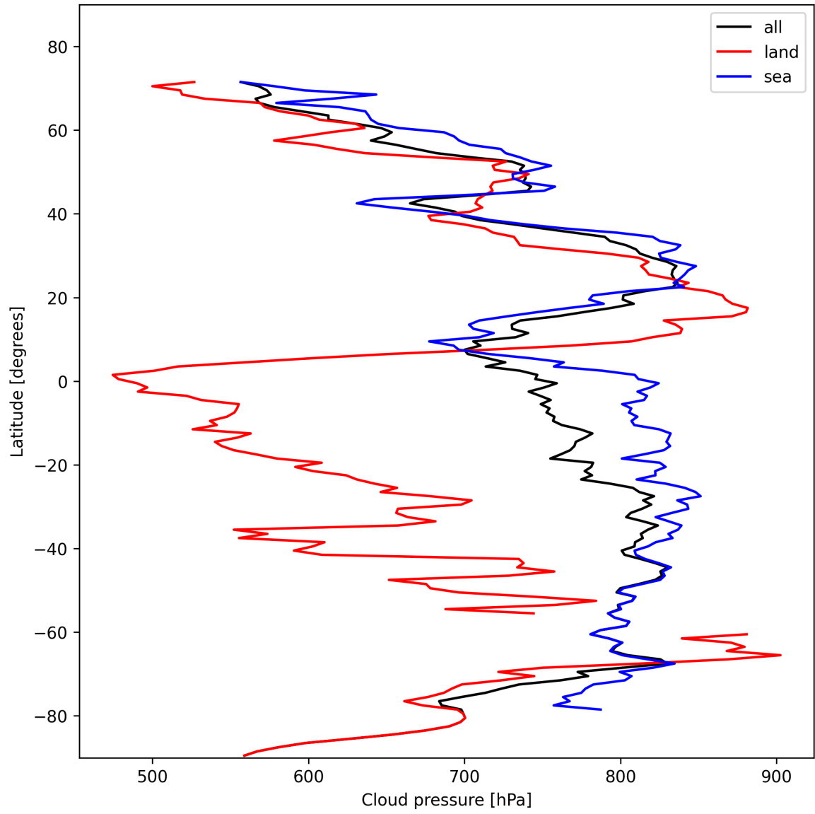
Figure 13: Zonal average of “Cloud pressure” for 2024-11-05 to 2024-11-07.
