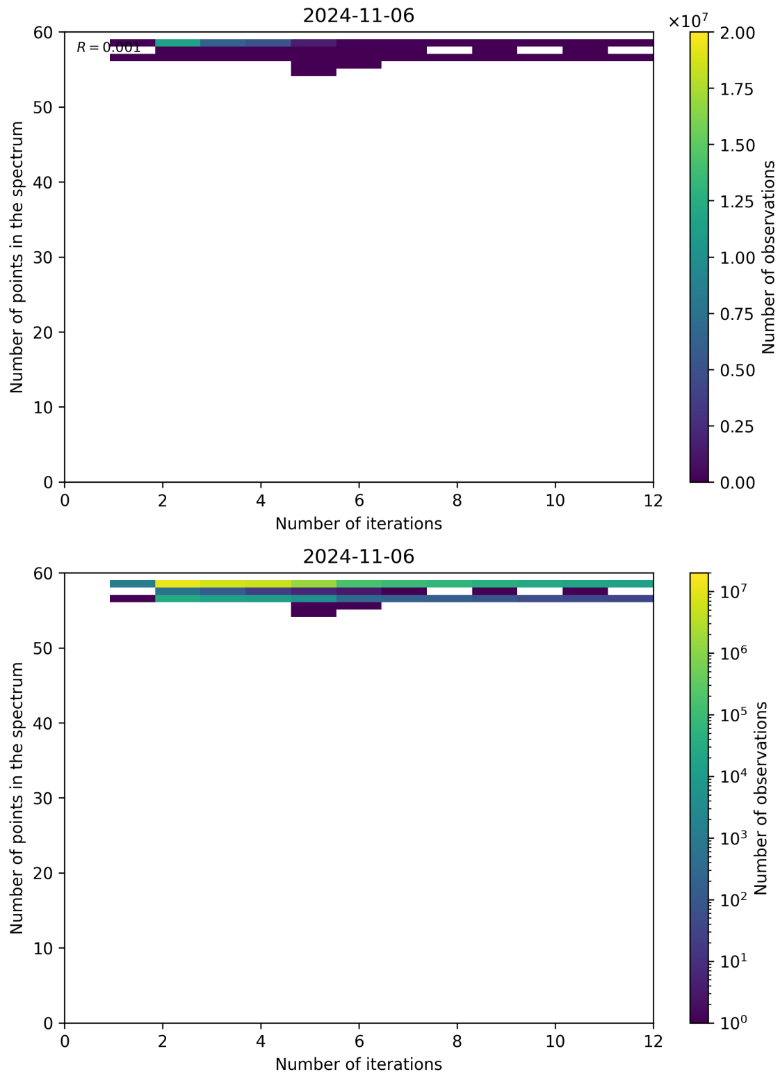
Figure 108: Scatter density plot of “Number of iterations” against “Number of points in the spectrum” for 2024-11-05 to 2024-11-07.
