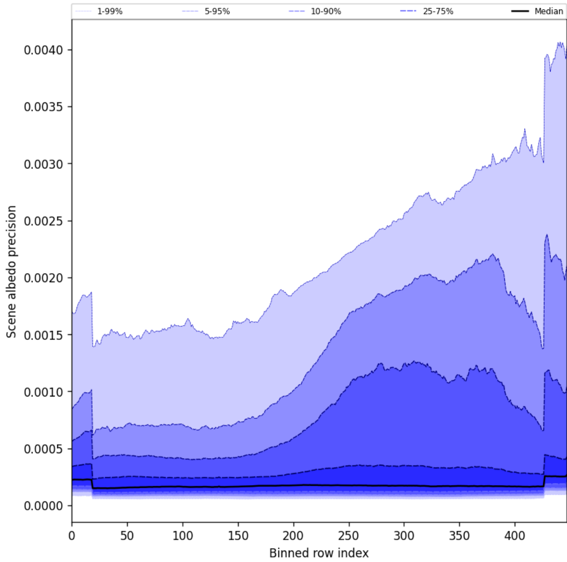
Figure 52: Along track statistics of “Scene albedo precision” for 2024-11-05 to 2024-11-07
