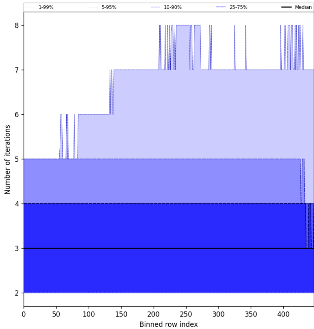
Figure 56: Along track statistics of “Number of iterations” for 2024-11-05 to 2024-11-07
