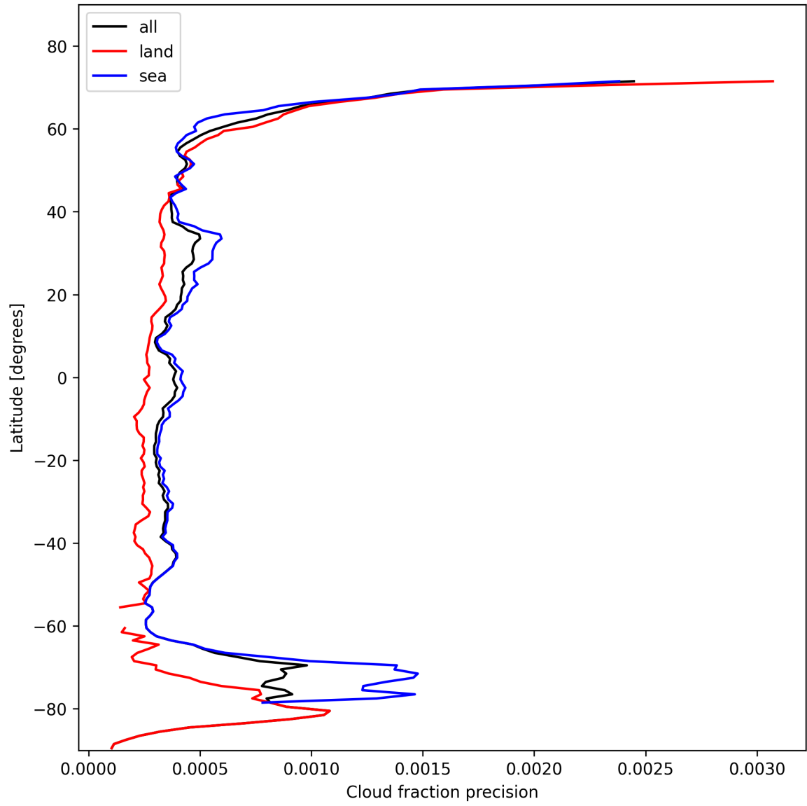
Figure 16: Zonal average of “Cloud fraction precision” for 2024-11-05 to 2024-11-07.
