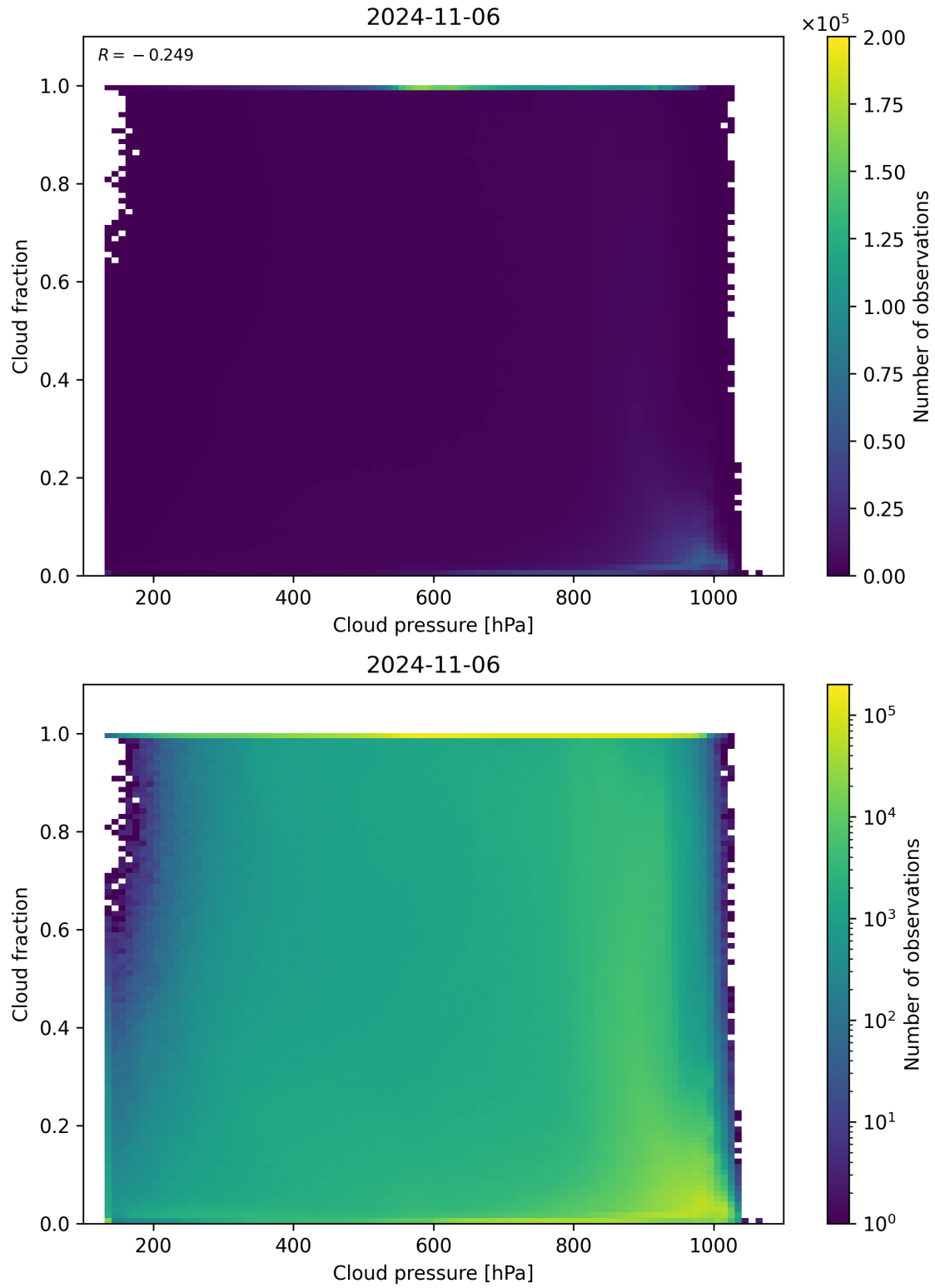
Figure 87: Scatter density plot of “Cloud pressure” against “Cloud fraction” for 2024-11-05 to 2024-11-07.
