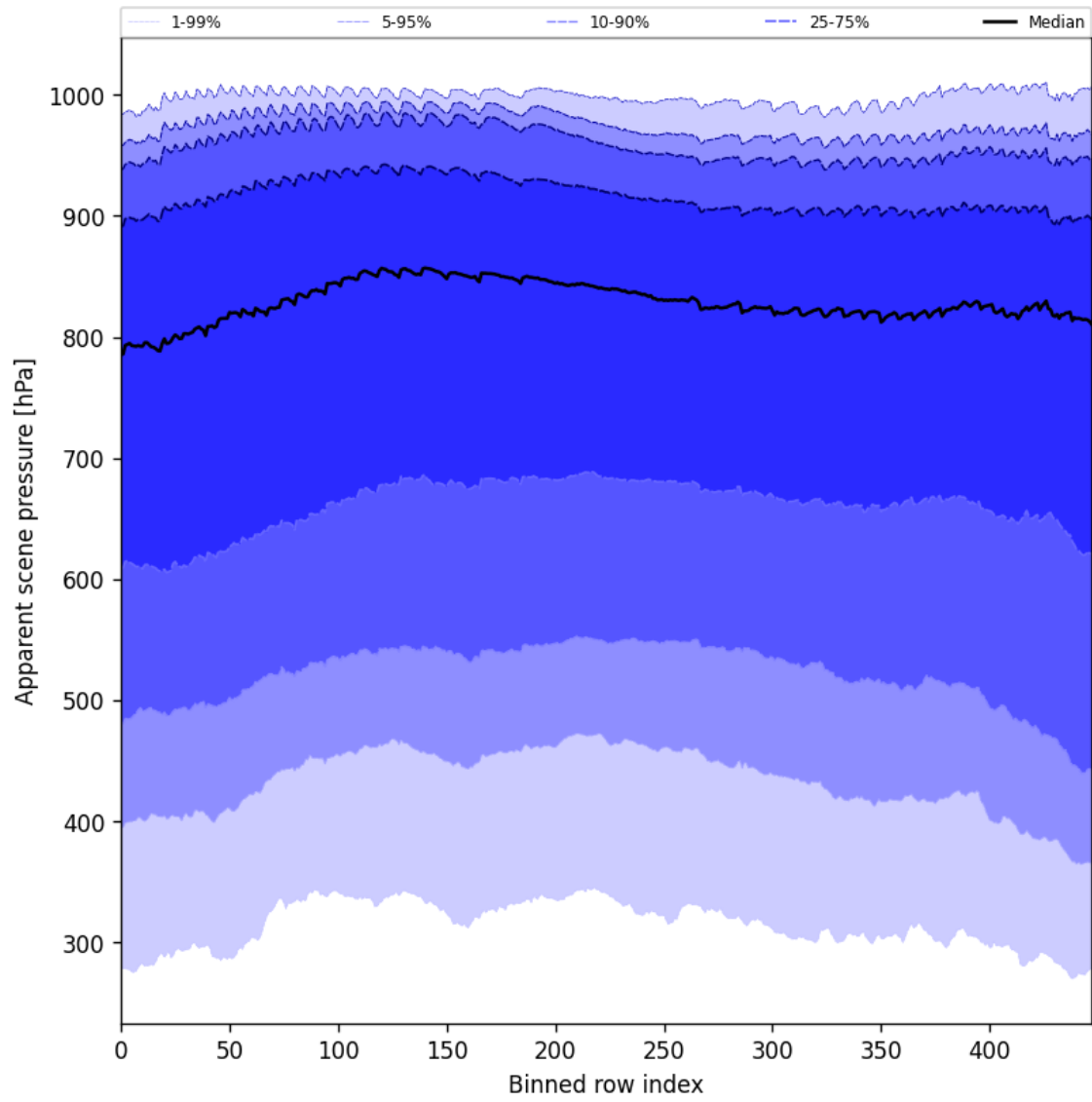
Figure 53: Along track statistics of “Apparent scene pressure” for 2024-11-05 to 2024-11-07
