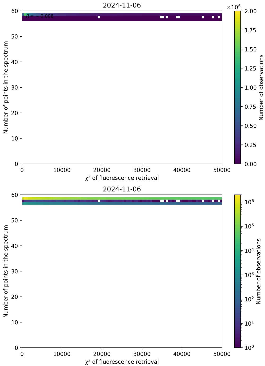
Figure 71: Scatter density plot of " \chi^2 of fluorescence retrieval" against "Number of points in the spectrum" for 2024-11-05 to 2024-11-07.
