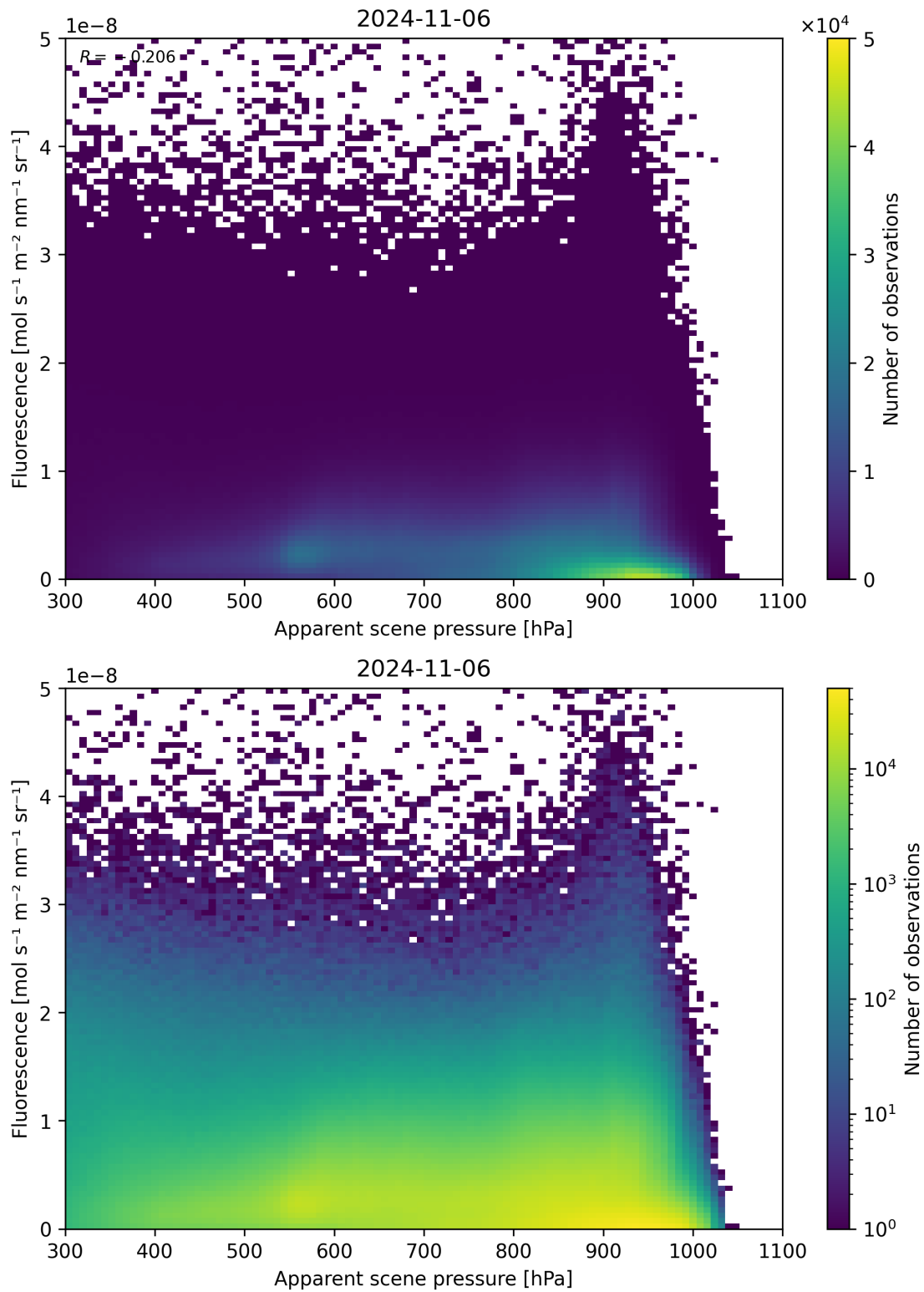
Figure 65: Scatter density plot of “Apparent scene pressure” against “Fluorescence” for 2024-11-05 to 2024-11-07.
