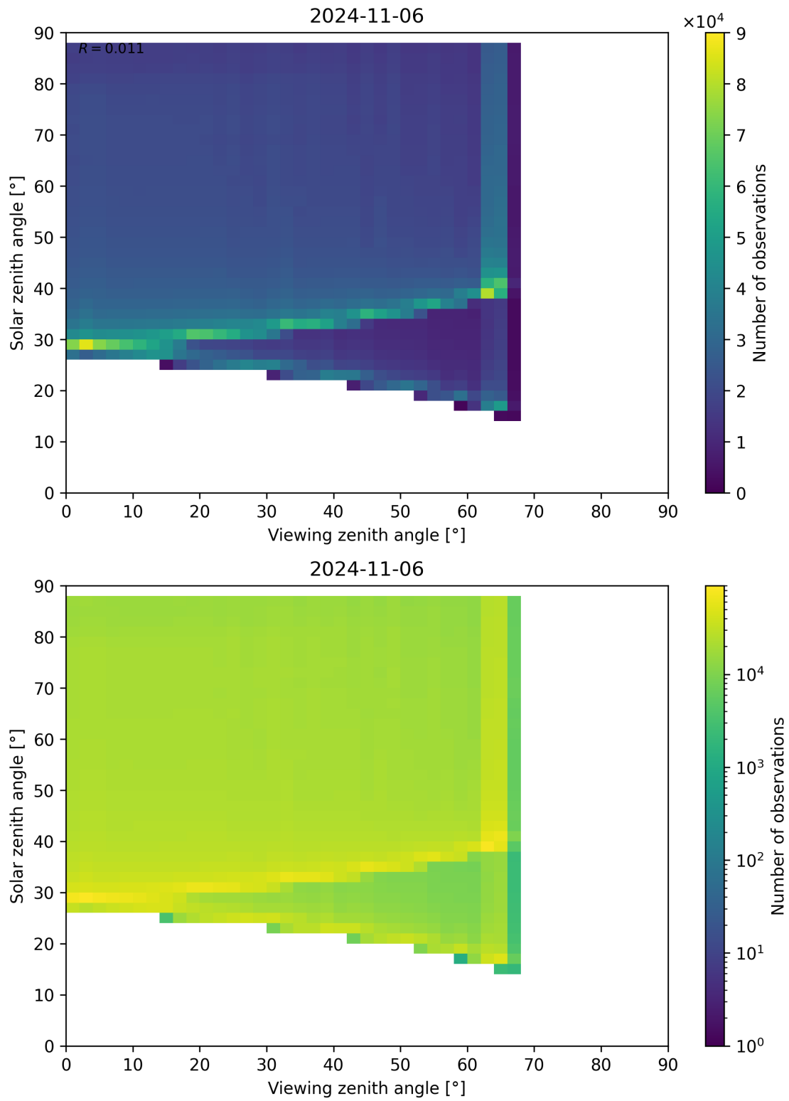
Figure 139: Scatter density plot of “Viewing zenith angle” against “Solar zenith angle” for 2024-11-05 to 2024-11-07.
