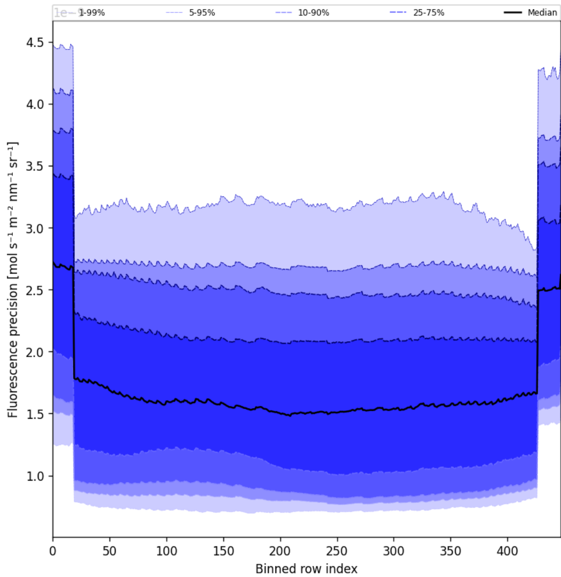
Figure 58: Along track statistics of “Fluorescence precision” for 2024-11-05 to 2024-11-07
