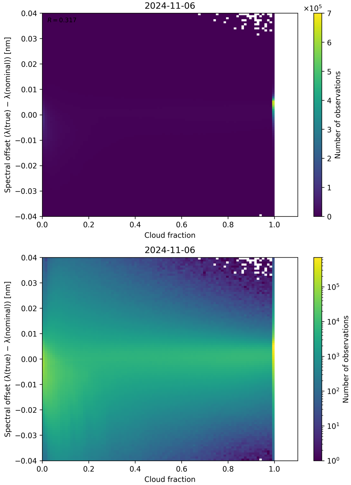
Figure 83: Scatter density plot of “Cloud fraction” against “Spectral offset ( \lambda_{\text{true}} - \lambda_{\text{nominal}} )” for 2024-11-05 to 2024-11-07.
