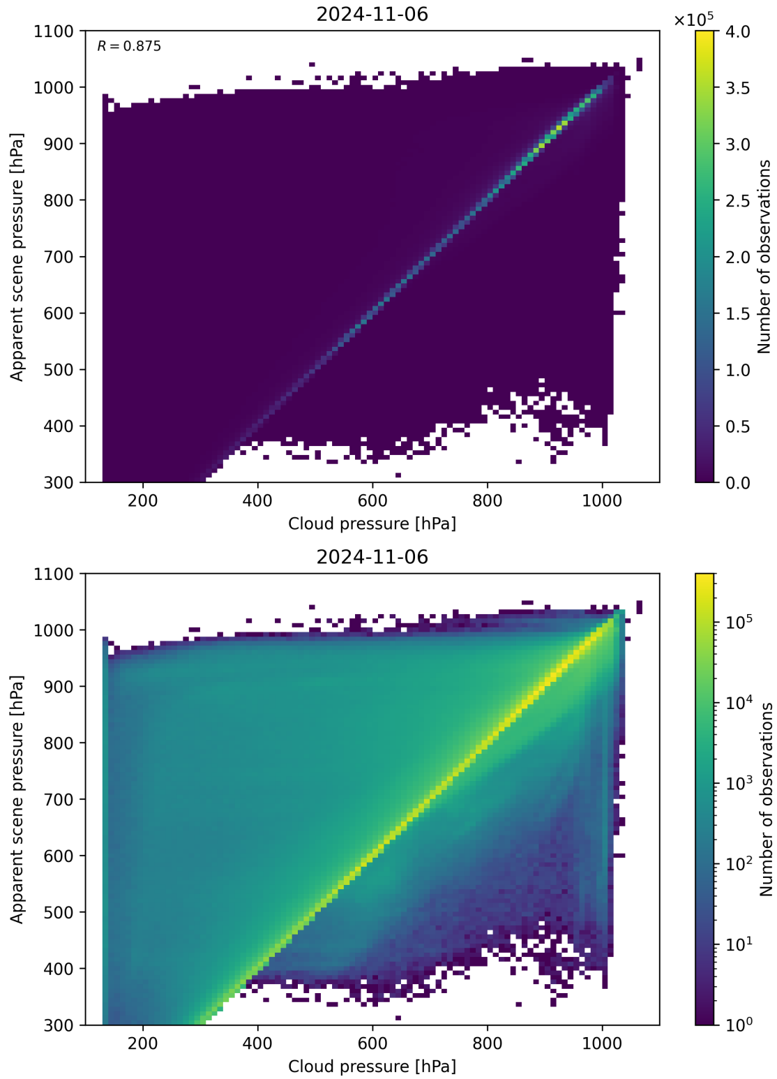
Figure 84: Scatter density plot of “Cloud pressure” against “Apparent scene pressure” for 2024-11-05 to 2024-11-07.
