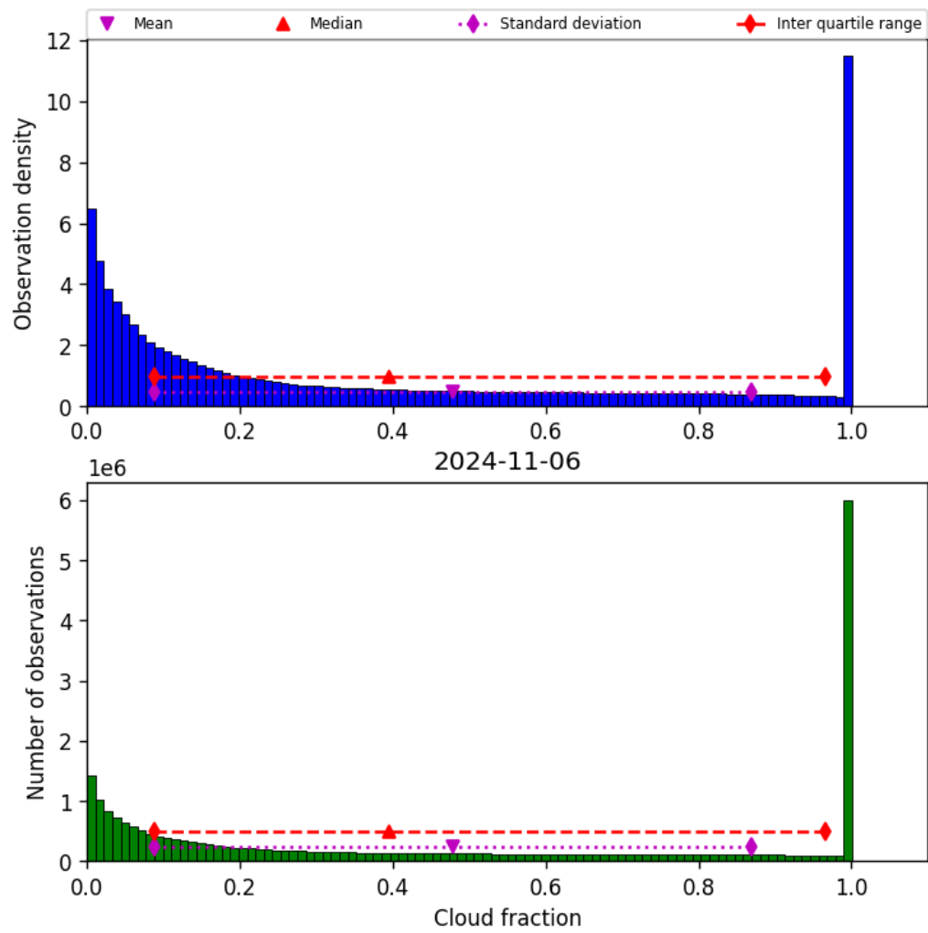
Figure 32: Histogram of “Cloud fraction” for 2024-11-05 to 2024-11-07
