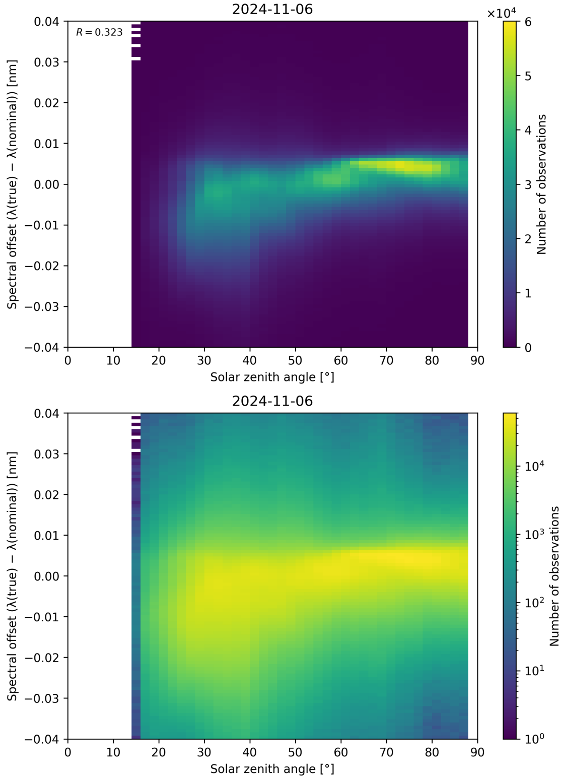
Figure 128: Scatter density plot of “Solar zenith angle” against “Spectral offset ( \lambda_{\text{true}} - \lambda_{\text{nominal}} )” for 2024-11-05 to 2024-11-07.
