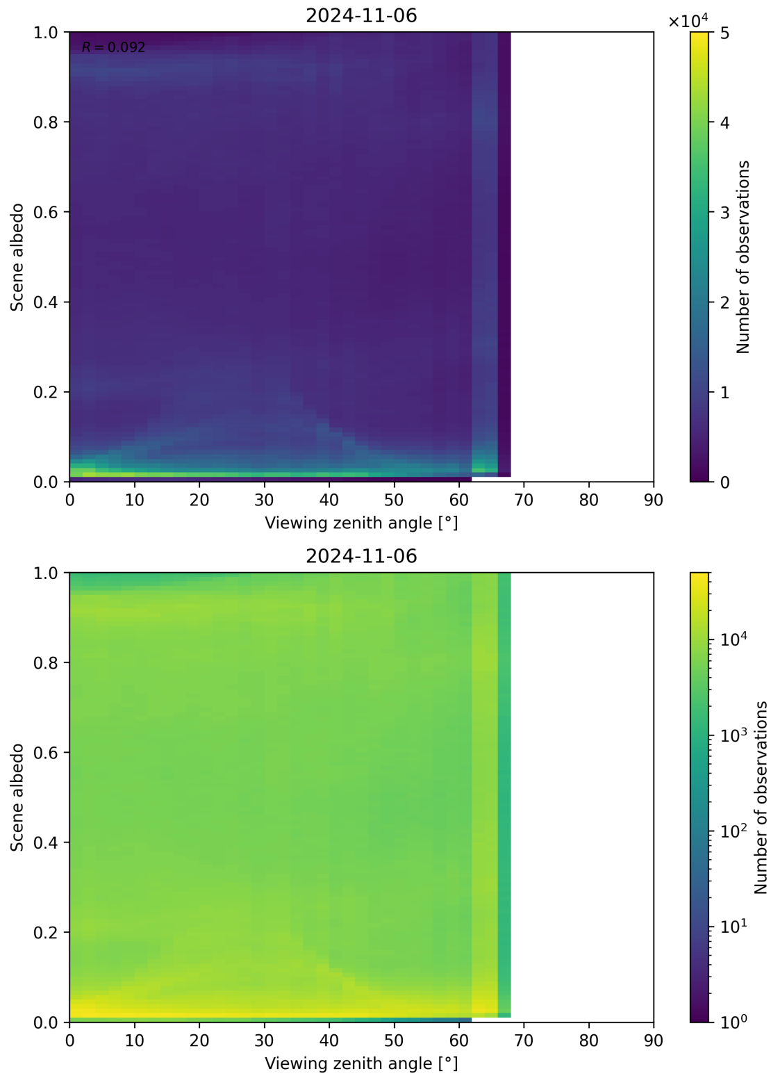
Figure 138: Scatter density plot of “Viewing zenith angle” against “Scene albedo” for 2024-11-05 to 2024-11-07.
