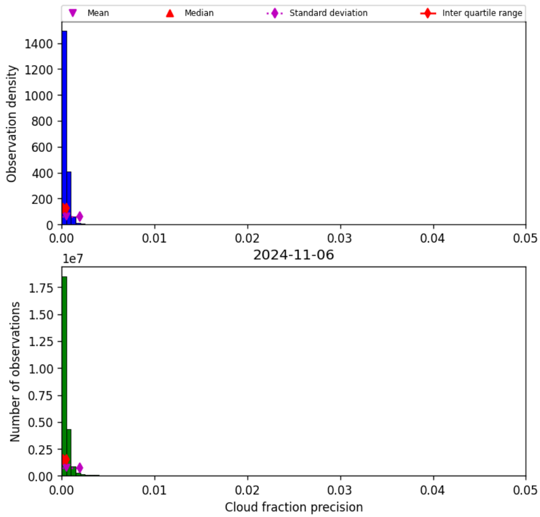
Figure 33: Histogram of “Cloud fraction precision” for 2024-11-05 to 2024-11-07
