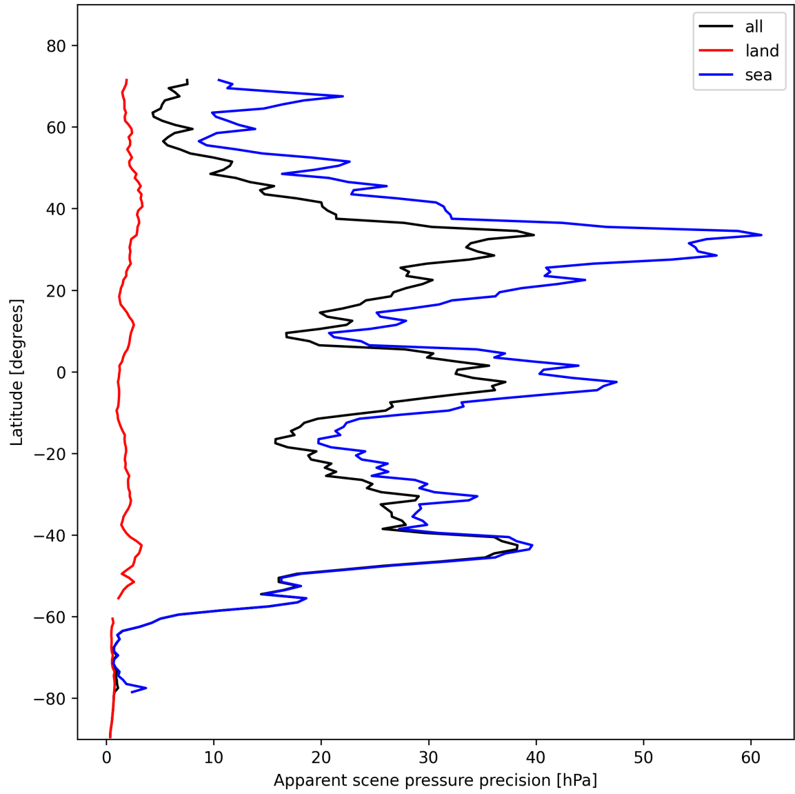
Figure 20: Zonal average of “Apparent scene pressure precision” for 2024-11-05 to 2024-11-07.
