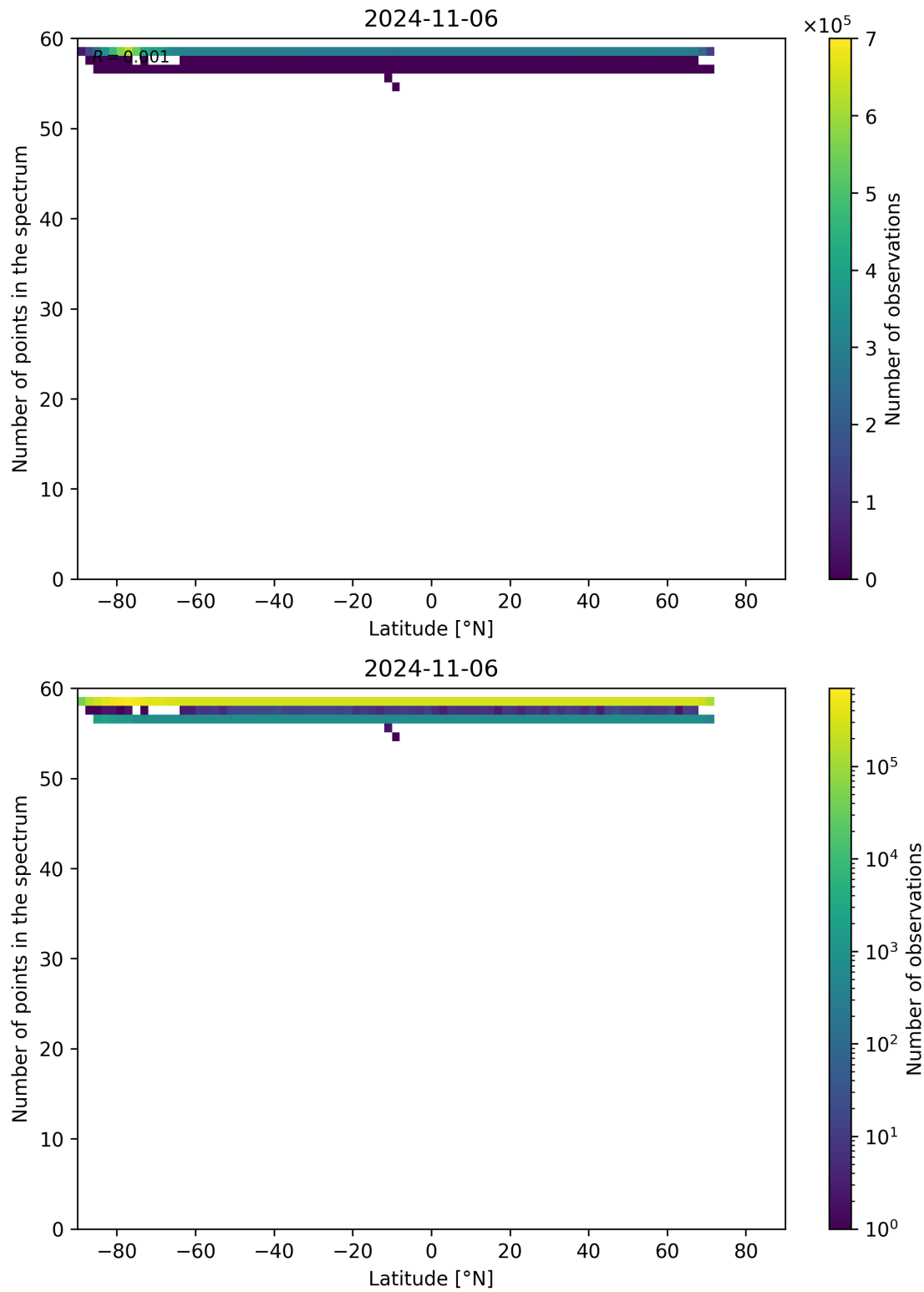
Figure 103: Scatter density plot of “Latitude” against “Number of points in the spectrum” for 2024-11-05 to 2024-11-07.
