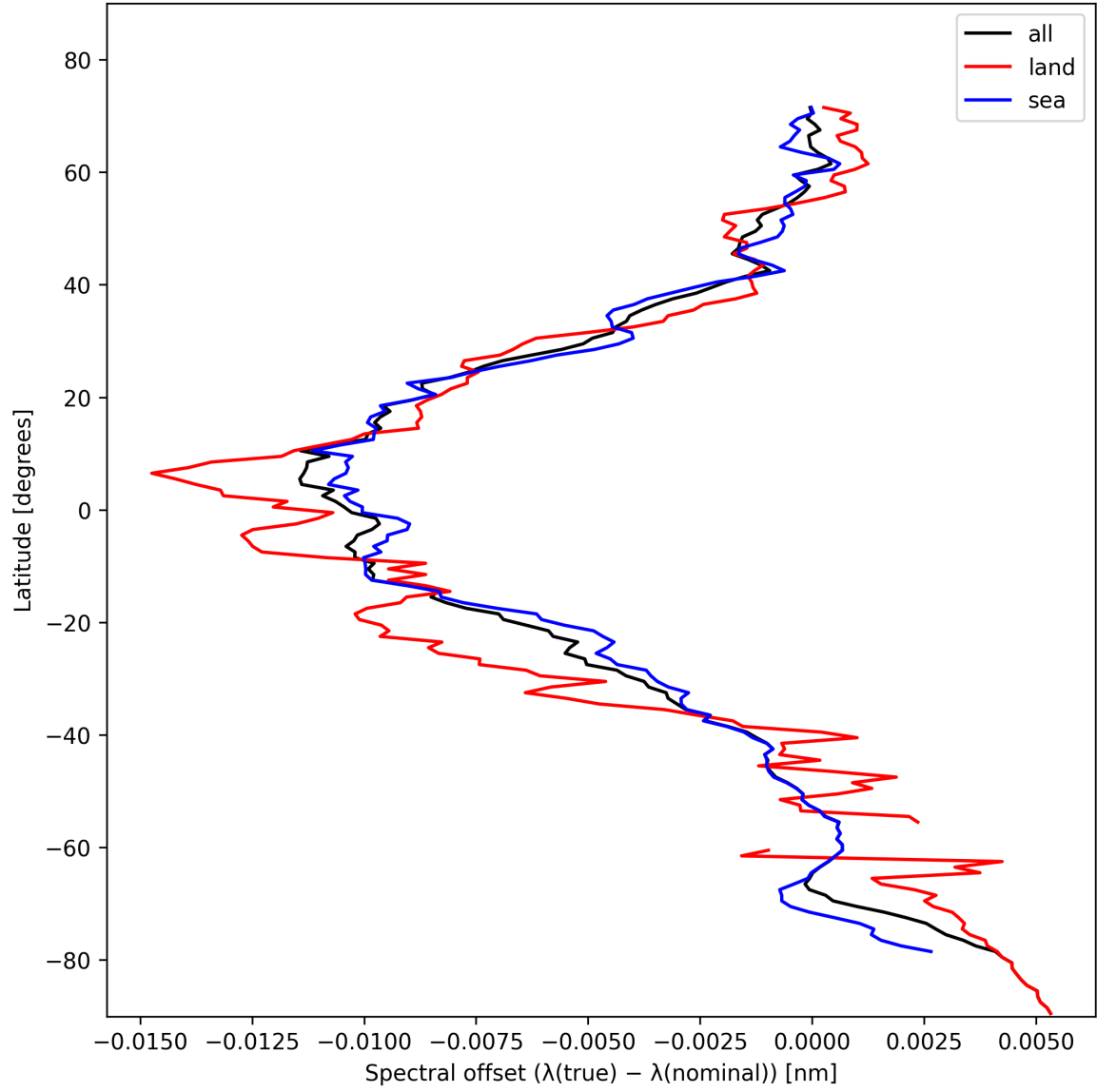
Figure 28: Zonal average of “Spectral offset ( \lambda_{\text{true}} - \lambda_{\text{nominal}} )” for 2024-11-05 to 2024-11-07.
