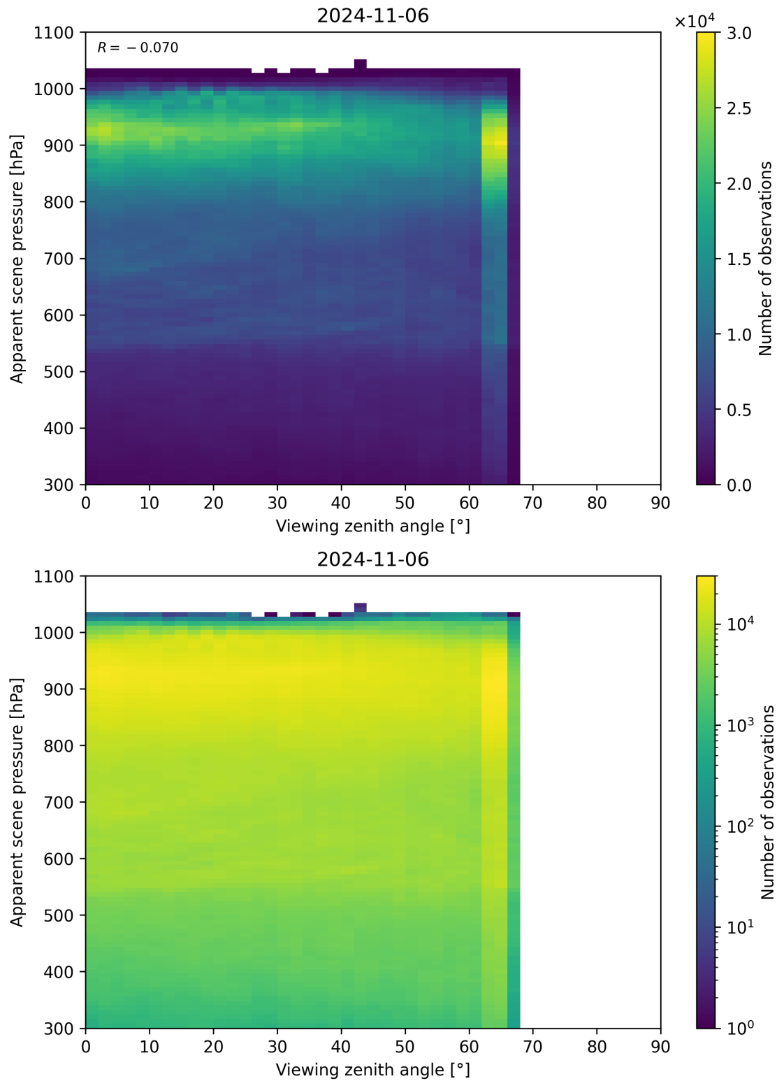
Figure 129: Scatter density plot of “Viewing zenith angle” against “Apparent scene pressure” for 2024-11-05 to 2024-11-07.
