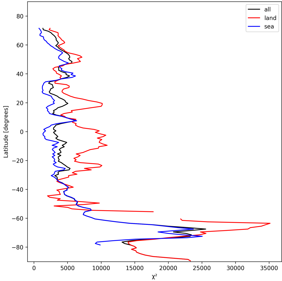
Figure 21: Zonal average of “ \chi^2 ” for 2024-11-05 to 2024-11-07.
