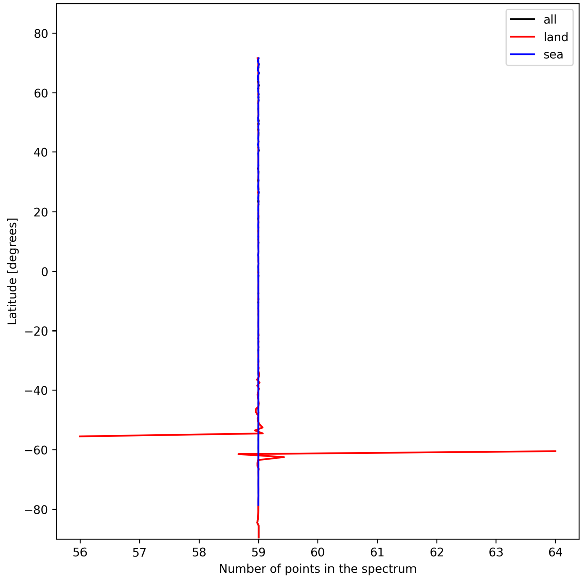
Figure 27: Zonal average of “Number of points in the spectrum” for 2024-11-05 to 2024-11-07.
