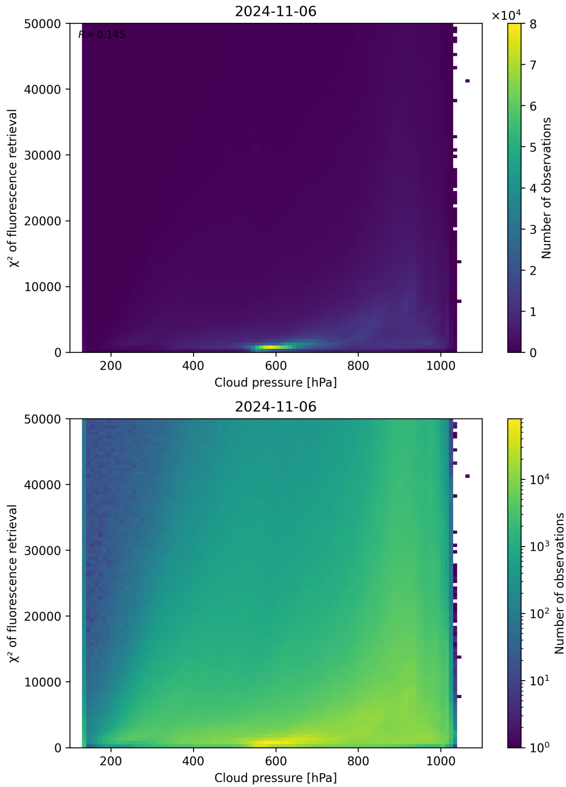
Figure 86: Scatter density plot of “Cloud pressure” against “ \chi^2 of fluorescence retrieval” for 2024-11-05 to 2024-11-07.
