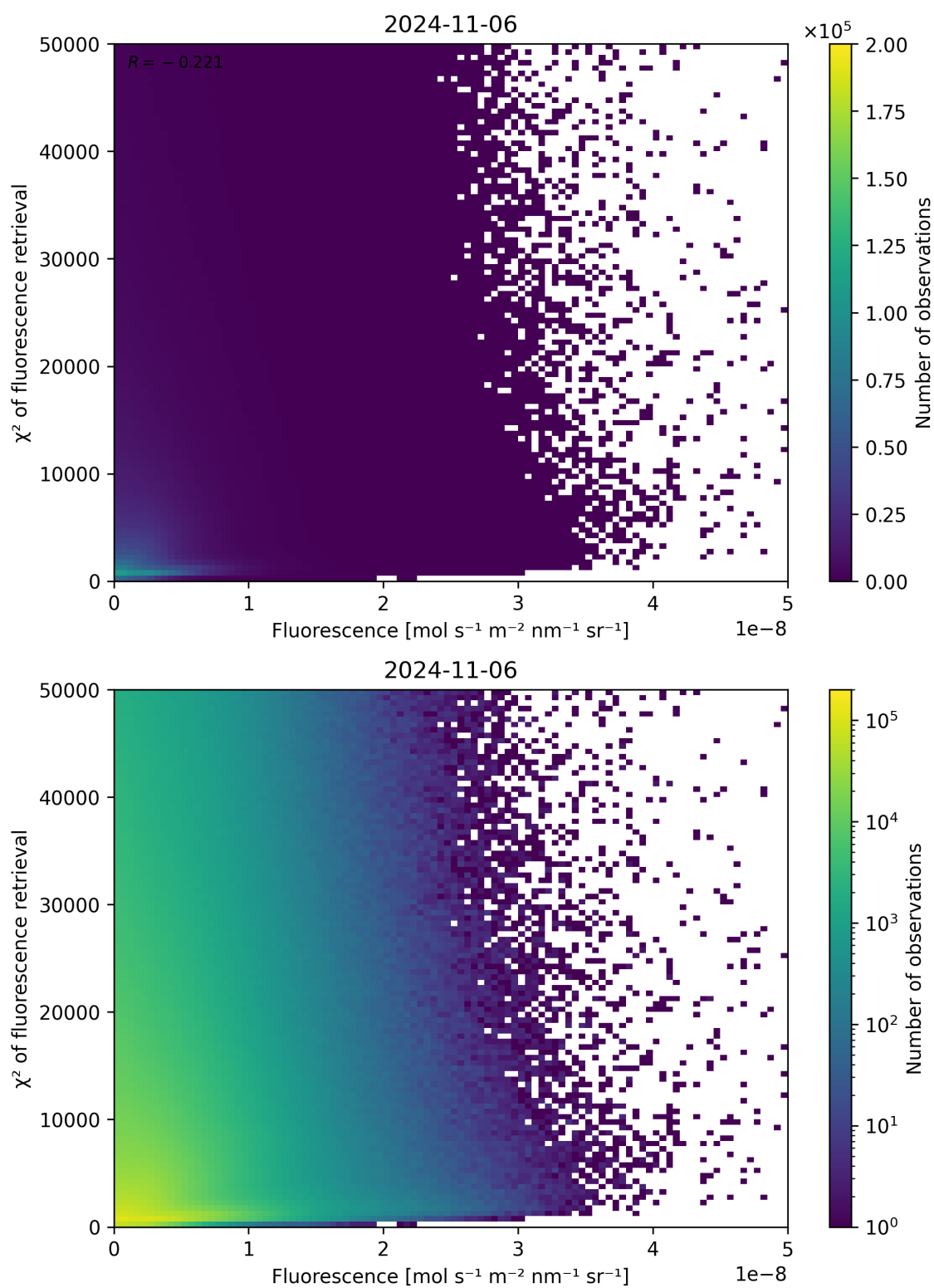
Figure 93: Scatter density plot of “Fluorescence” against “ \chi^2 of fluorescence retrieval” for 2024-11-05 to 2024-11-07.
