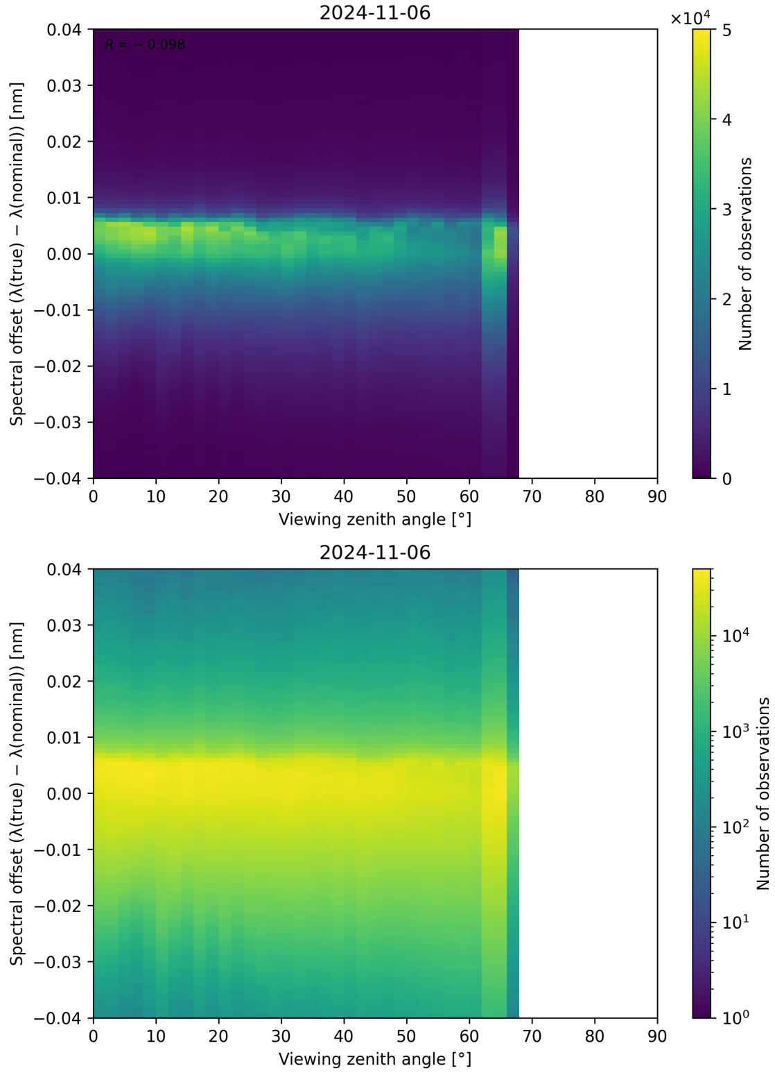
Figure 140: Scatter density plot of “Viewing zenith angle” against “Spectral offset ( \lambda_{\text{true}} - \lambda_{\text{nominal}} )” for 2024-11-05 to 2024-11-07.
