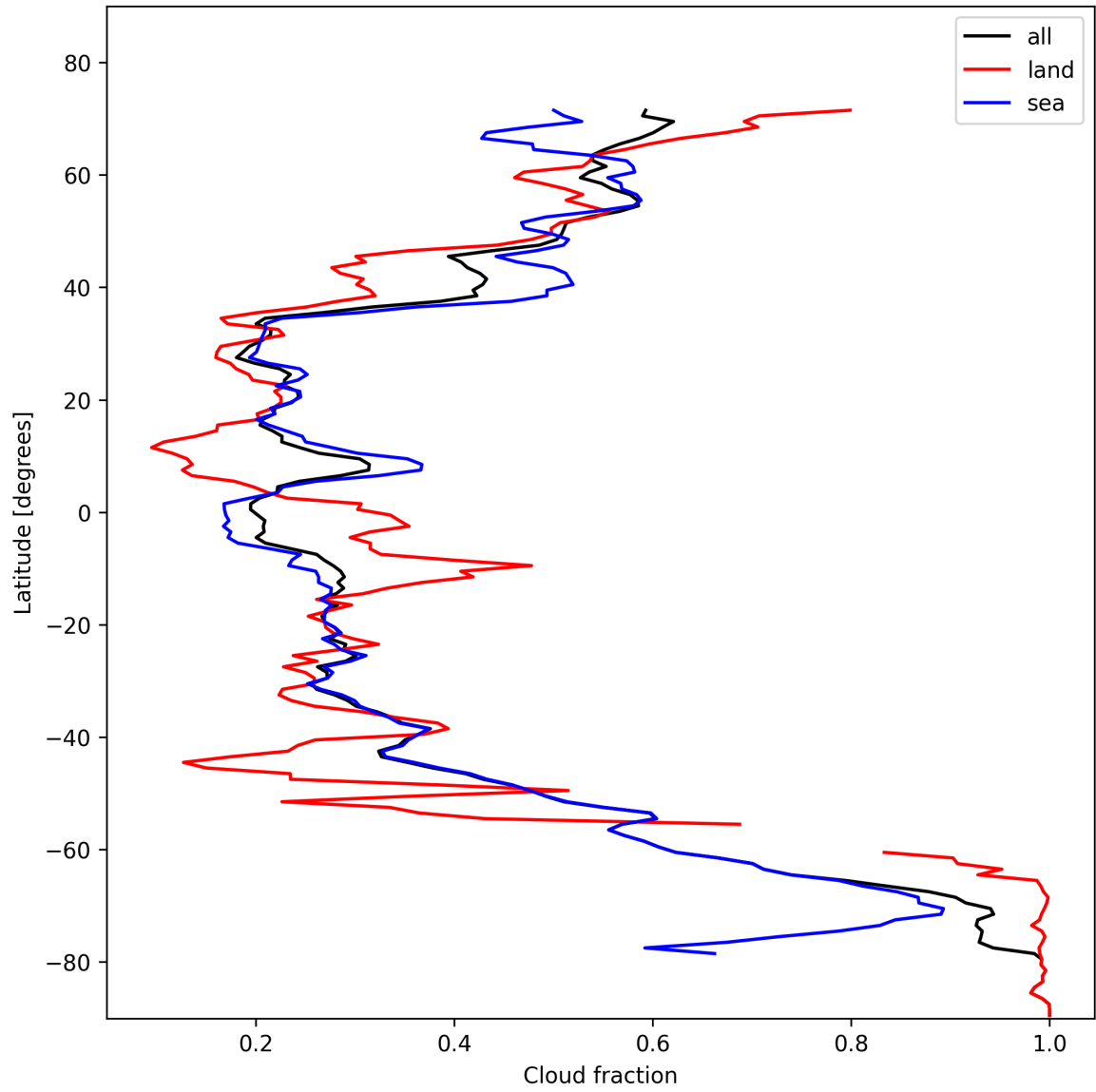
Figure 15: Zonal average of “Cloud fraction” for 2024-11-05 to 2024-11-07.
