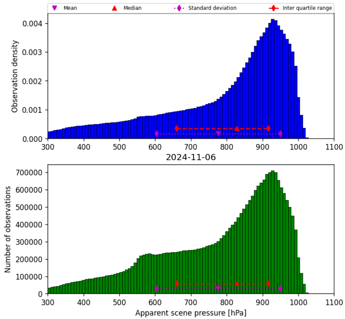
Figure 36: Histogram of “Apparent scene pressure” for 2024-11-05 to 2024-11-07
