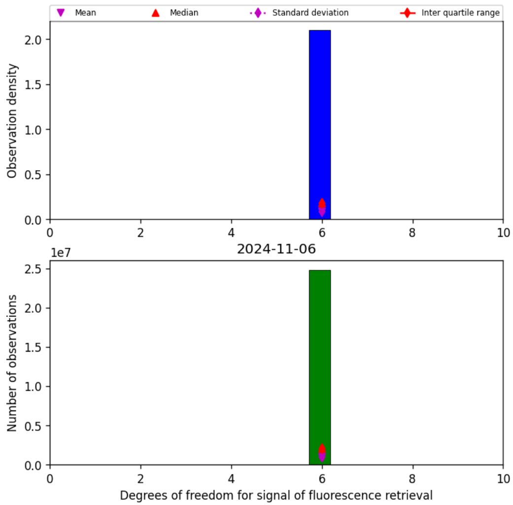
Figure 43: Histogram of "Degrees of freedom for signal of fluorescence retrieval" for 2024-11-05 to 2024-11-07
