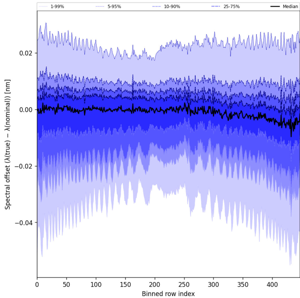
Figure 62: Along track statistics of “Spectral offset ( \lambda_{\text{true}} - \lambda_{\text{nominal}} )” for 2024-11-05 to 2024-11-07
