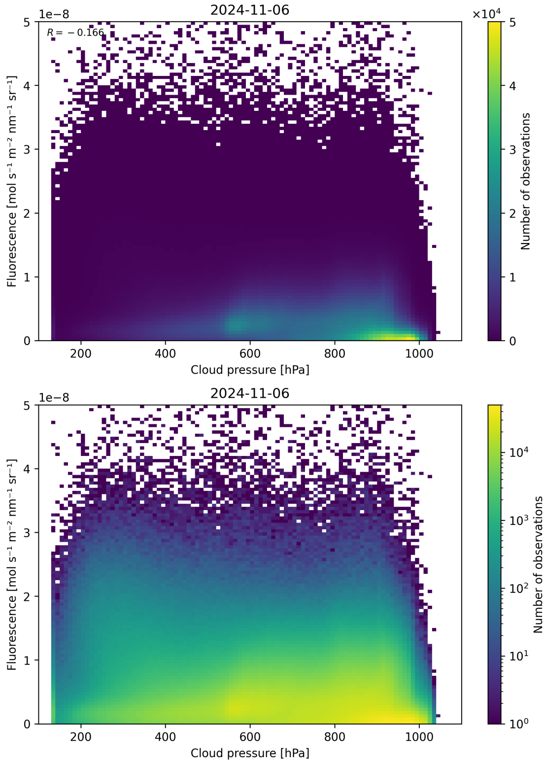
Figure 88: Scatter density plot of “Cloud pressure” against “Fluorescence” for 2024-11-05 to 2024-11-07.
