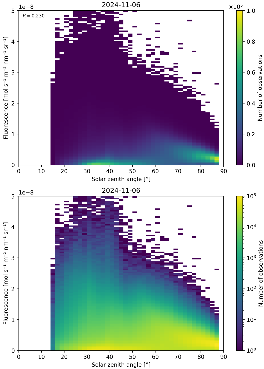
Figure 123: Scatter density plot of “Solar zenith angle” against “Fluorescence” for 2024-11-05 to 2024-11-07.
