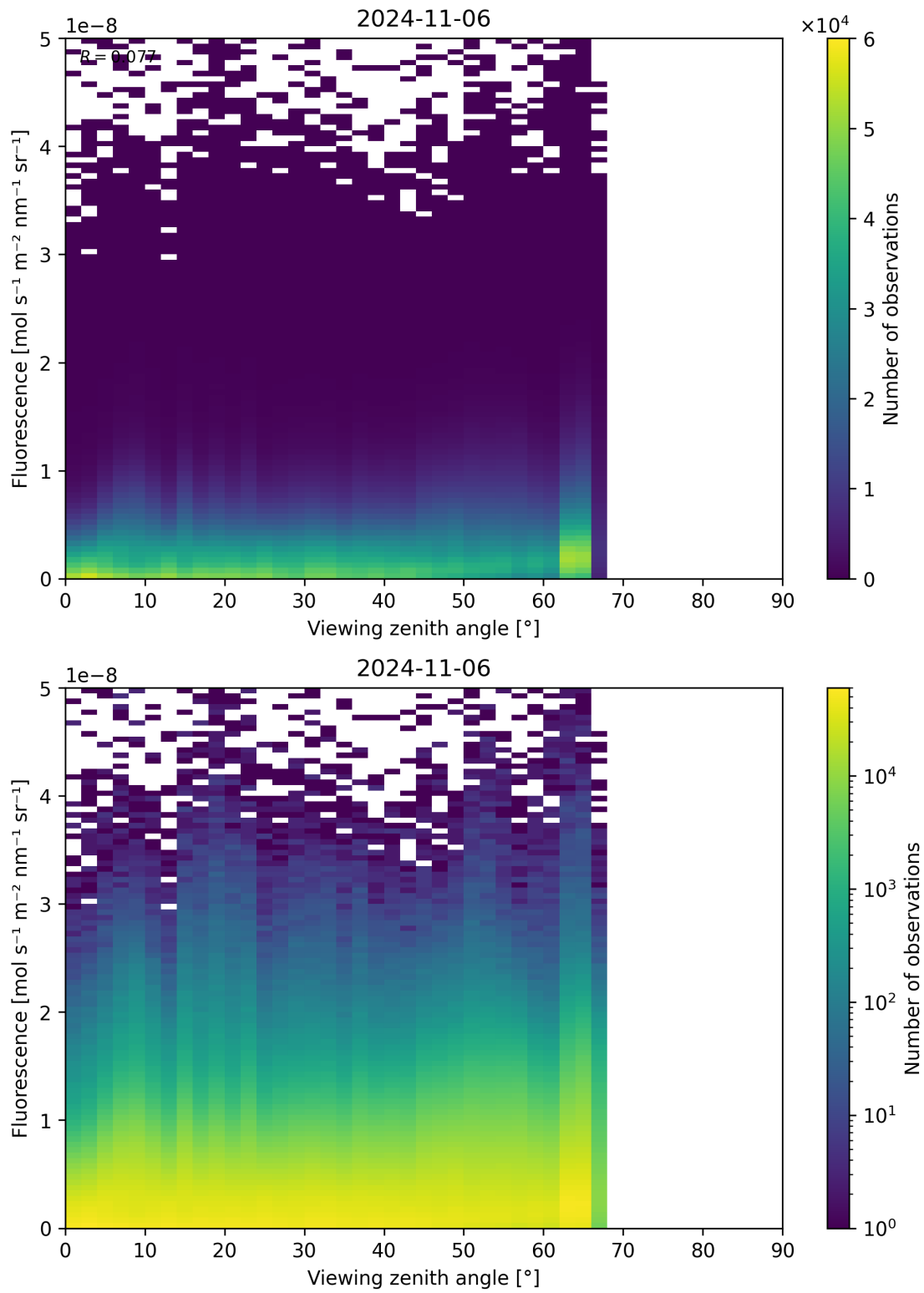
Figure 134: Scatter density plot of “Viewing zenith angle” against “Fluorescence” for 2024-11-05 to 2024-11-07.
