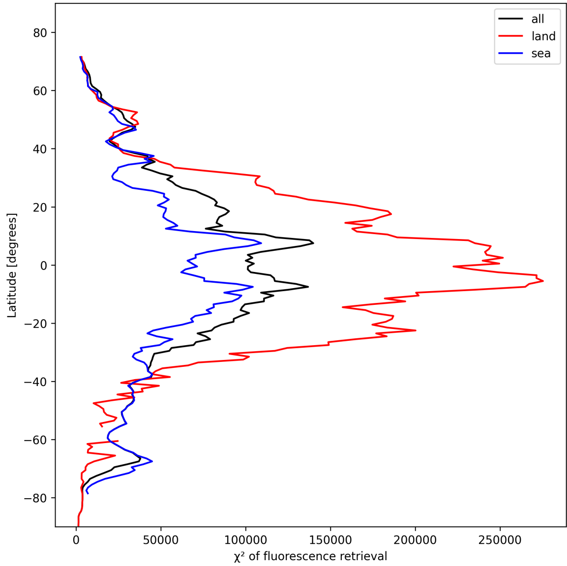
Figure 25: Zonal average of “ \chi^2 of fluorescence retrieval” for 2024-11-05 to 2024-11-07.
