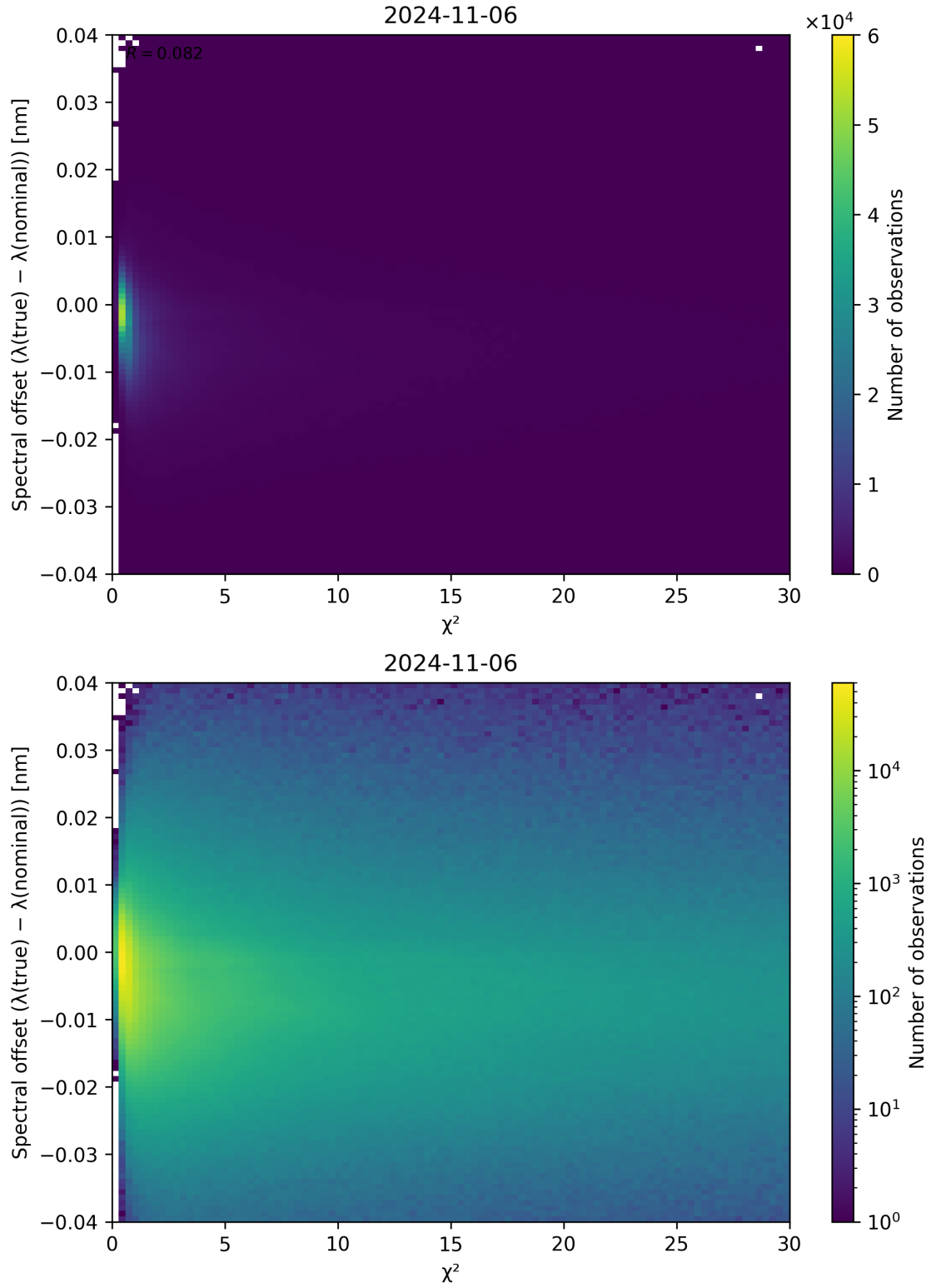
Figure 75: Scatter density plot of “ \chi^2 ” against “Spectral offset ( \lambda_{\text{true}} - \lambda_{\text{nominal}} )” for 2024-11-05 to 2024-11-07.
