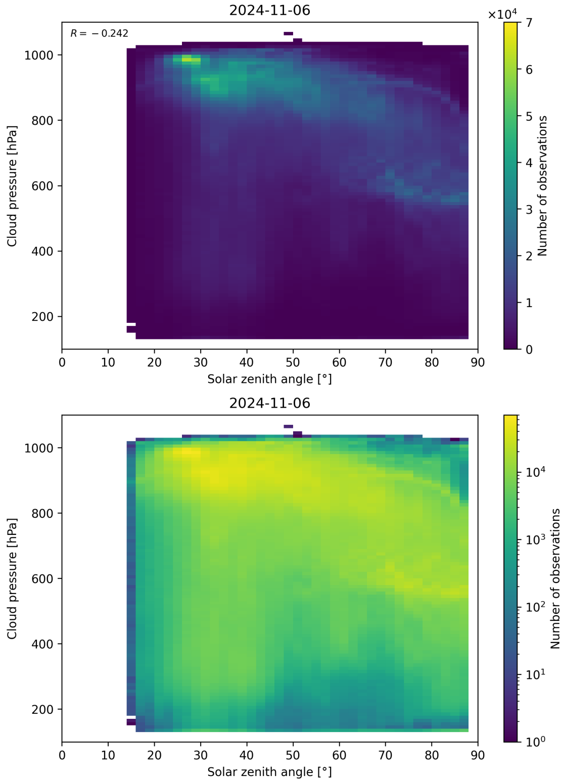
Figure 122: Scatter density plot of “Solar zenith angle” against “Cloud pressure” for 2024-11-05 to 2024-11-07.
