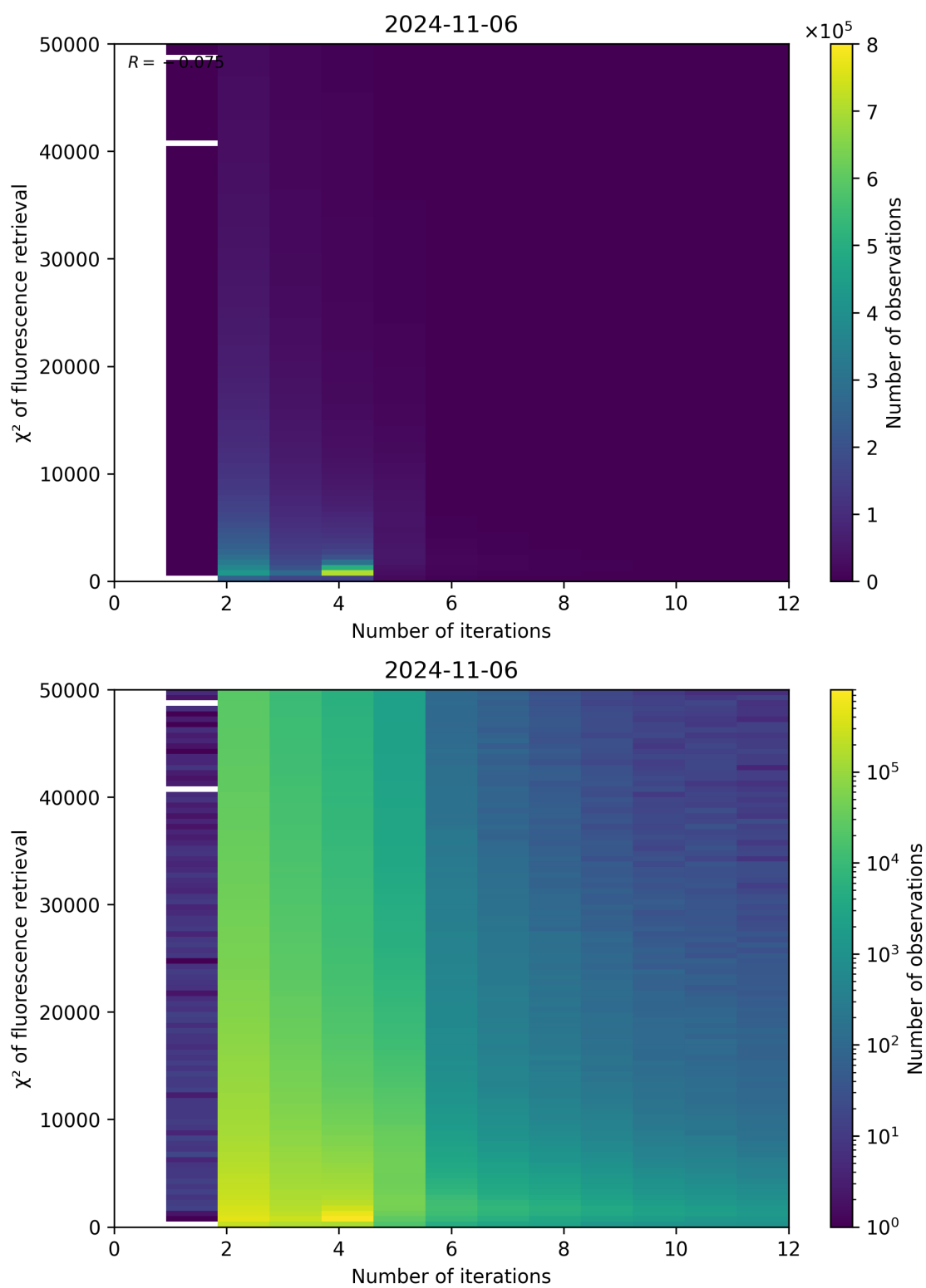
Figure 106: Scatter density plot of “Number of iterations” against “ \chi^2 of fluorescence retrieval” for 2024-11-05 to 2024-11-07.
