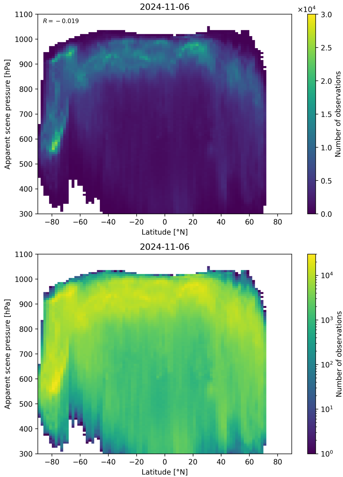
Figure 96: Scatter density plot of “Latitude” against “Apparent scene pressure” for 2024-11-05 to 2024-11-07.
