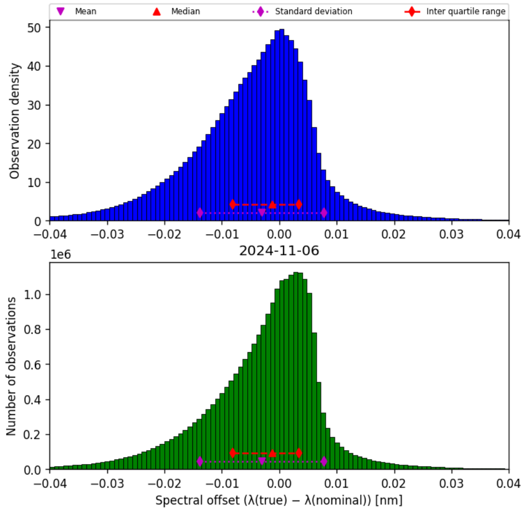
Figure 45: Histogram of “Spectral offset ( \lambda_{\text{true}} - \lambda_{\text{nominal}} )” for 2024-11-05 to 2024-11-07
