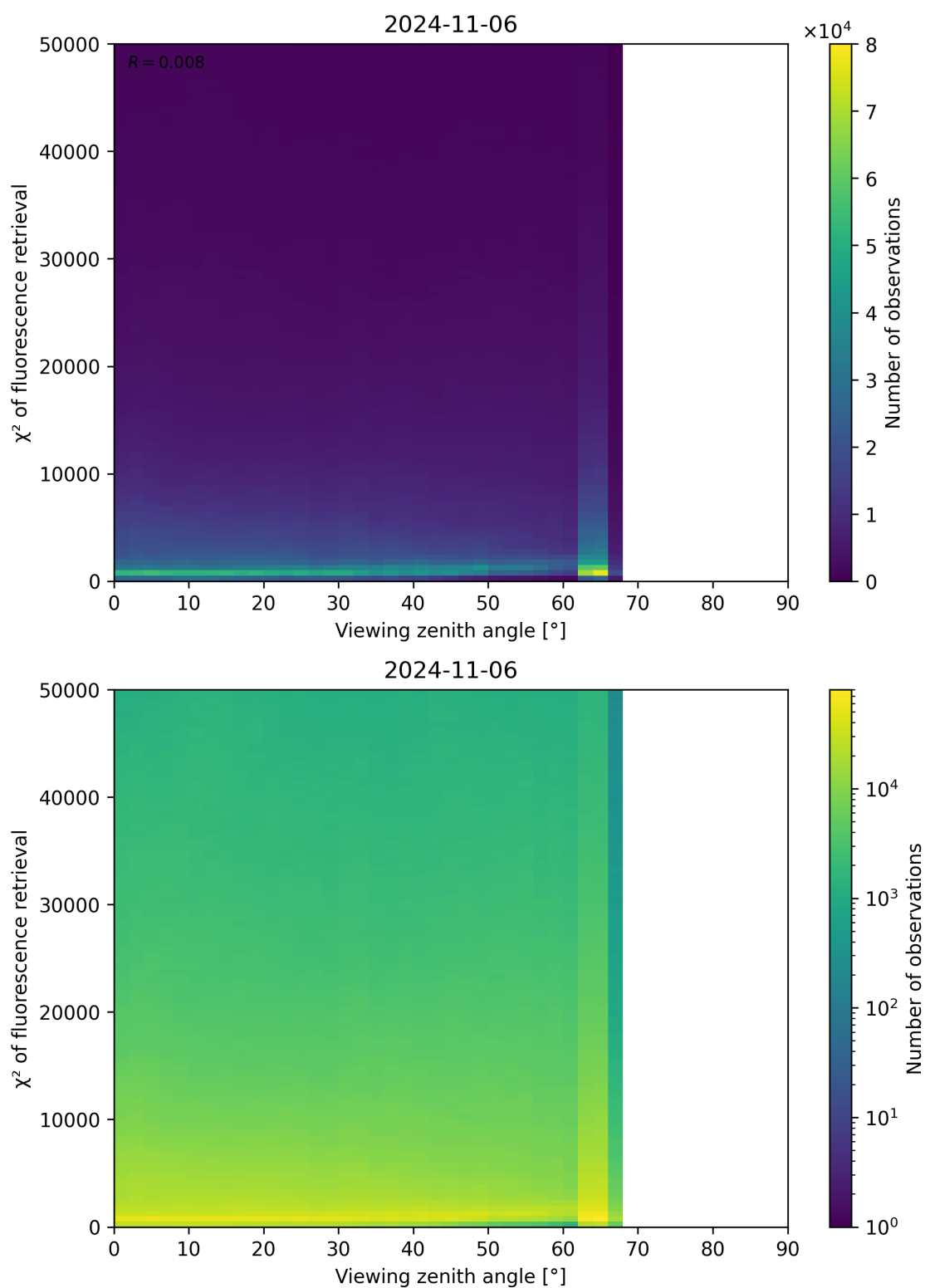
Figure 131: Scatter density plot of “Viewing zenith angle” against “ \chi^2 of fluorescence retrieval” for 2024-11-05 to 2024-11-07.
