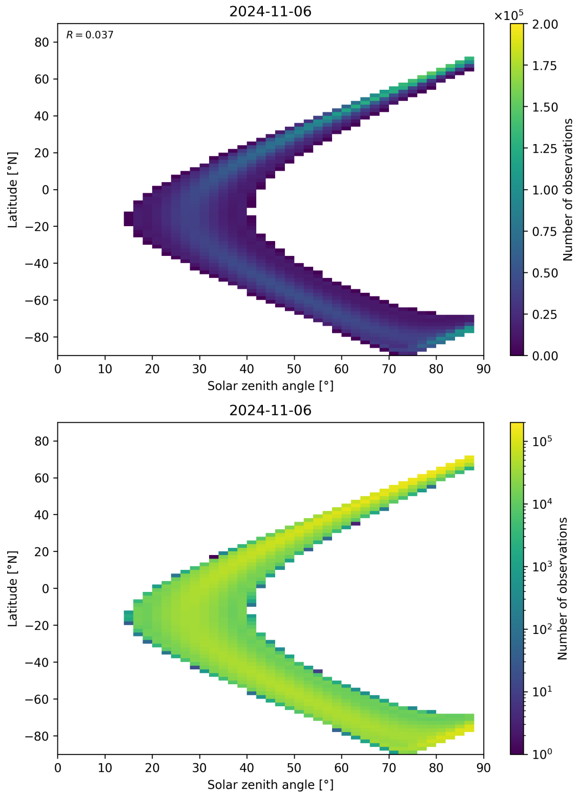
Figure 124: Scatter density plot of “Solar zenith angle” against “Latitude” for 2024-11-05 to 2024-11-07.
