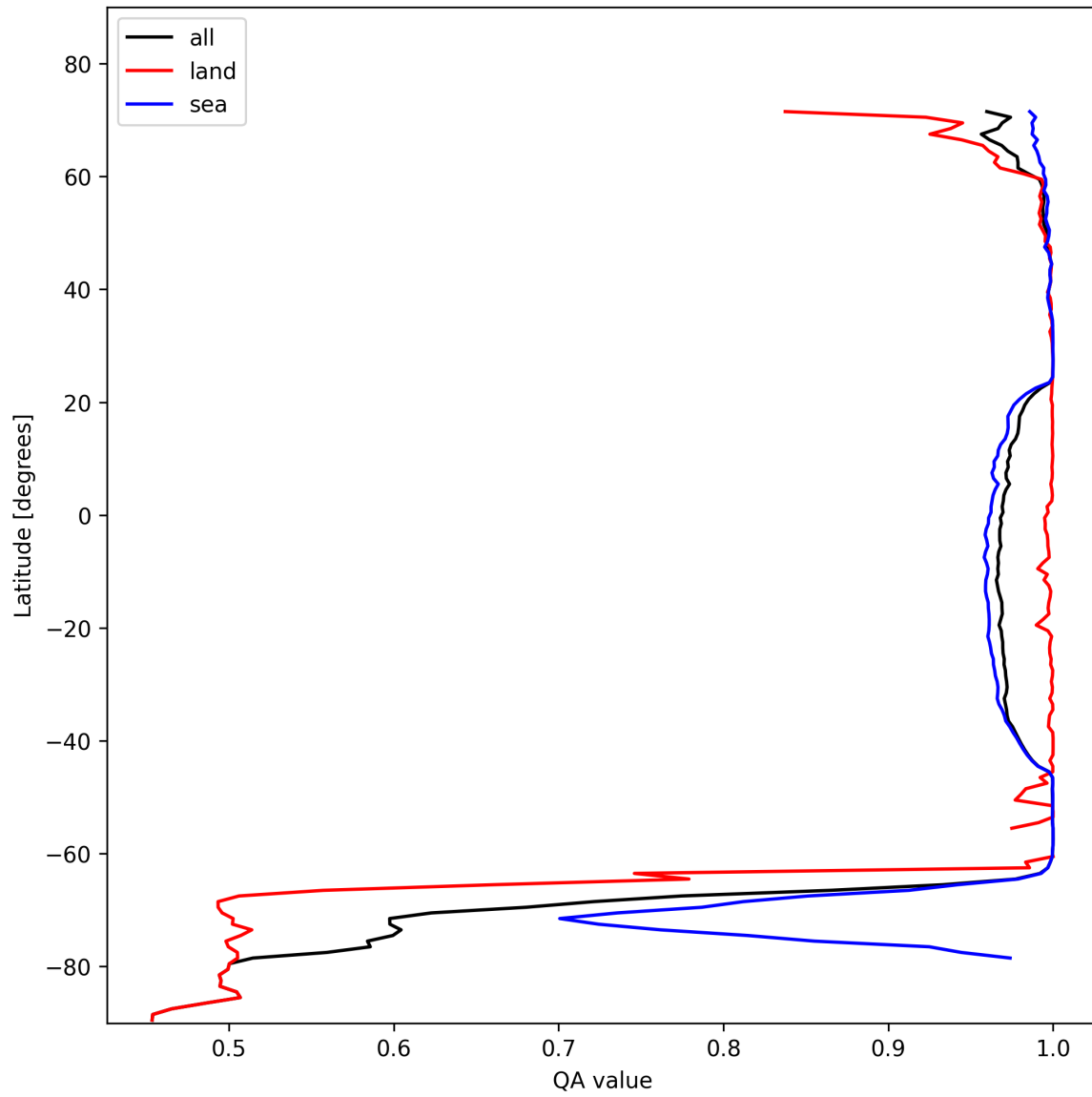
Figure 12: Zonal average of “QA value” for 2024-11-05 to 2024-11-07.
