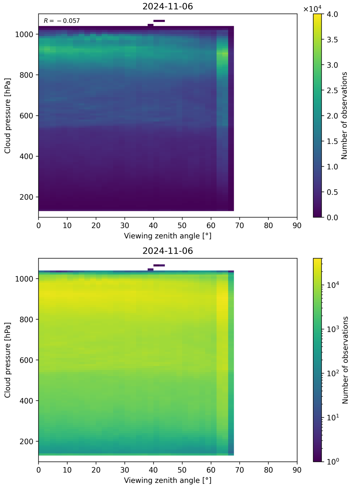
Figure 133: Scatter density plot of “Viewing zenith angle” against “Cloud pressure” for 2024-11-05 to 2024-11-07.
