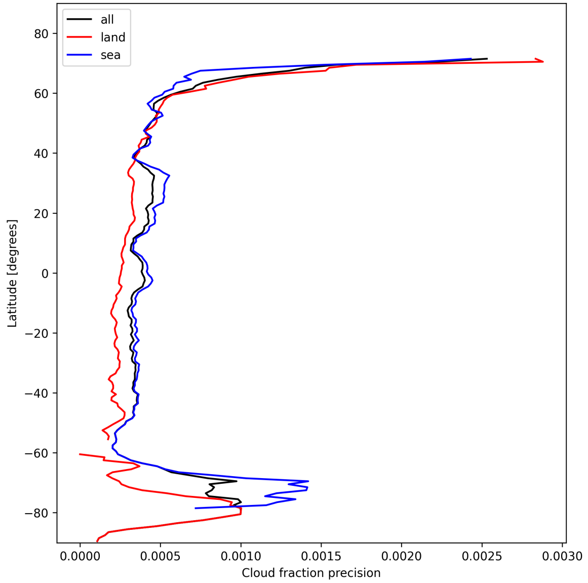
Figure 16: Zonal average of “Cloud fraction precision” for 2024-11-06 to 2024-11-08.
