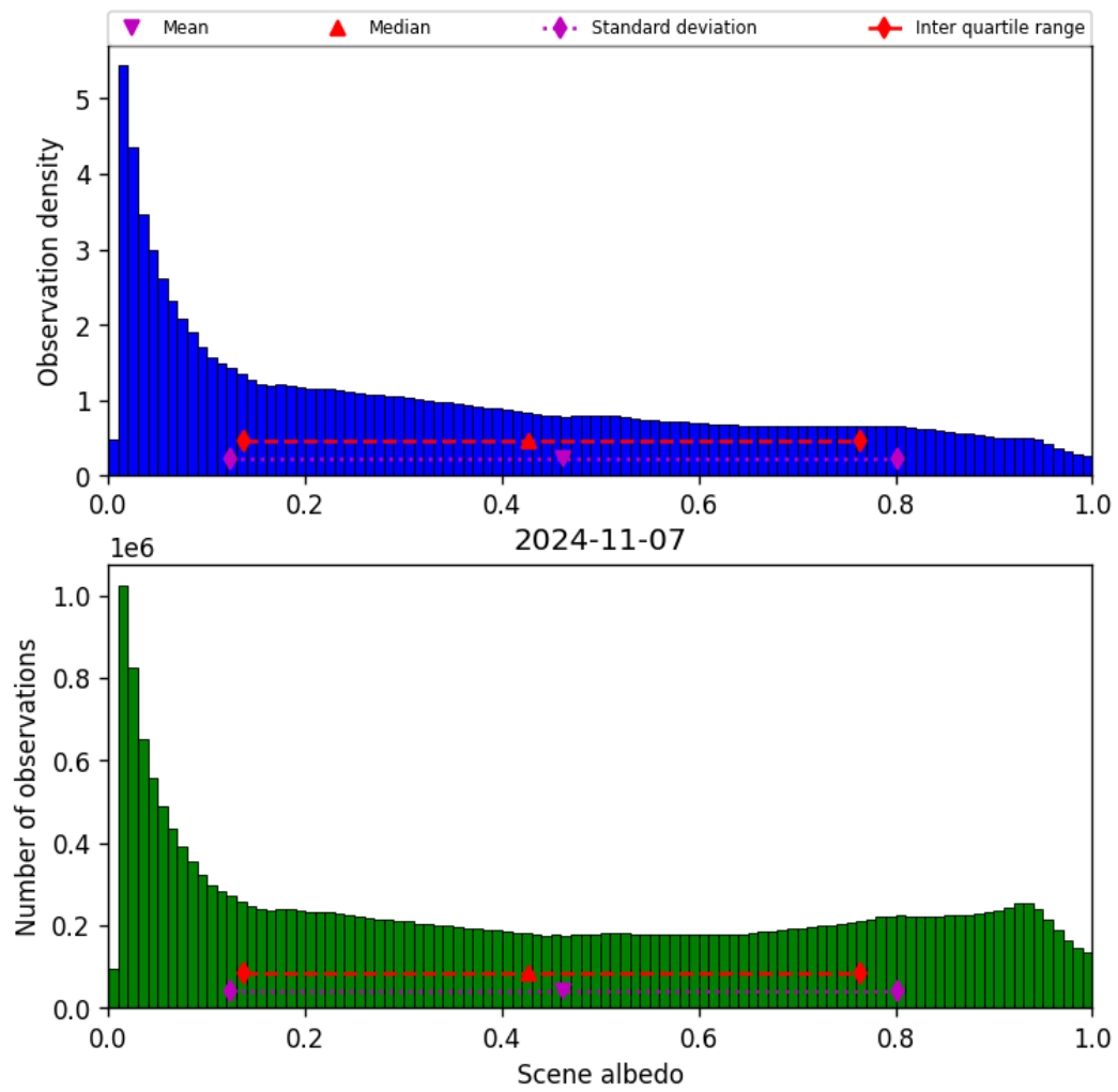
Figure 34: Histogram of “Scene albedo” for 2024-11-06 to 2024-11-08
