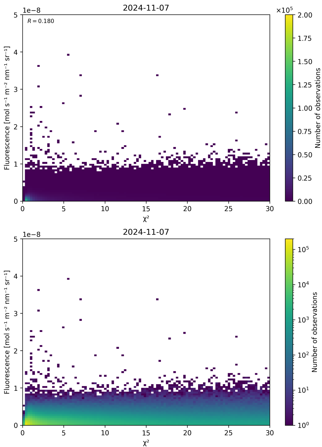
Figure 70: Scatter density plot of “ \chi^2 ” against “Fluorescence” for 2024-11-06 to 2024-11-08.
