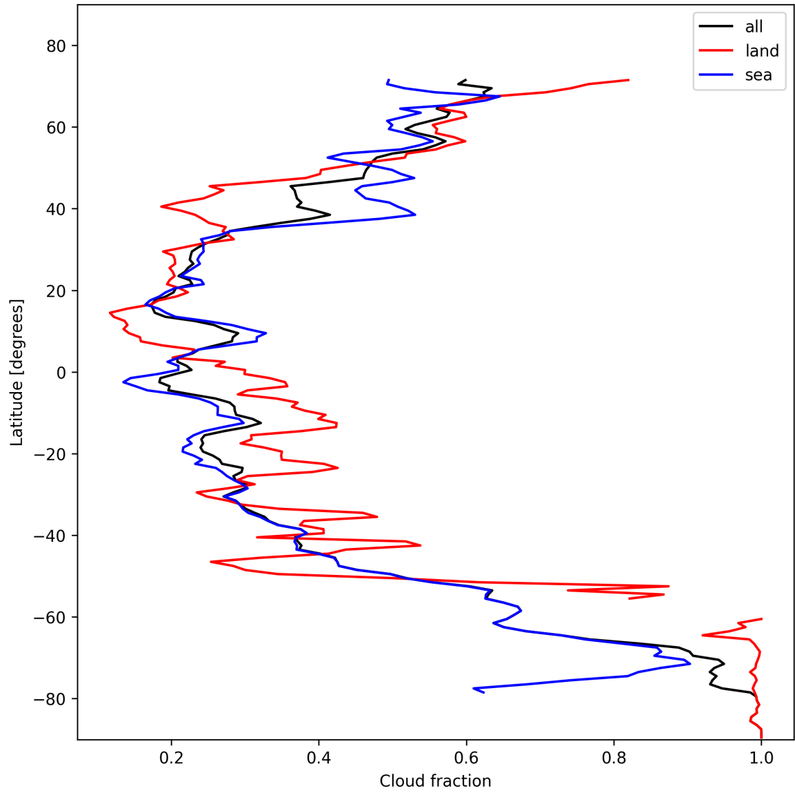
Figure 15: Zonal average of “Cloud fraction” for 2024-11-06 to 2024-11-08.
