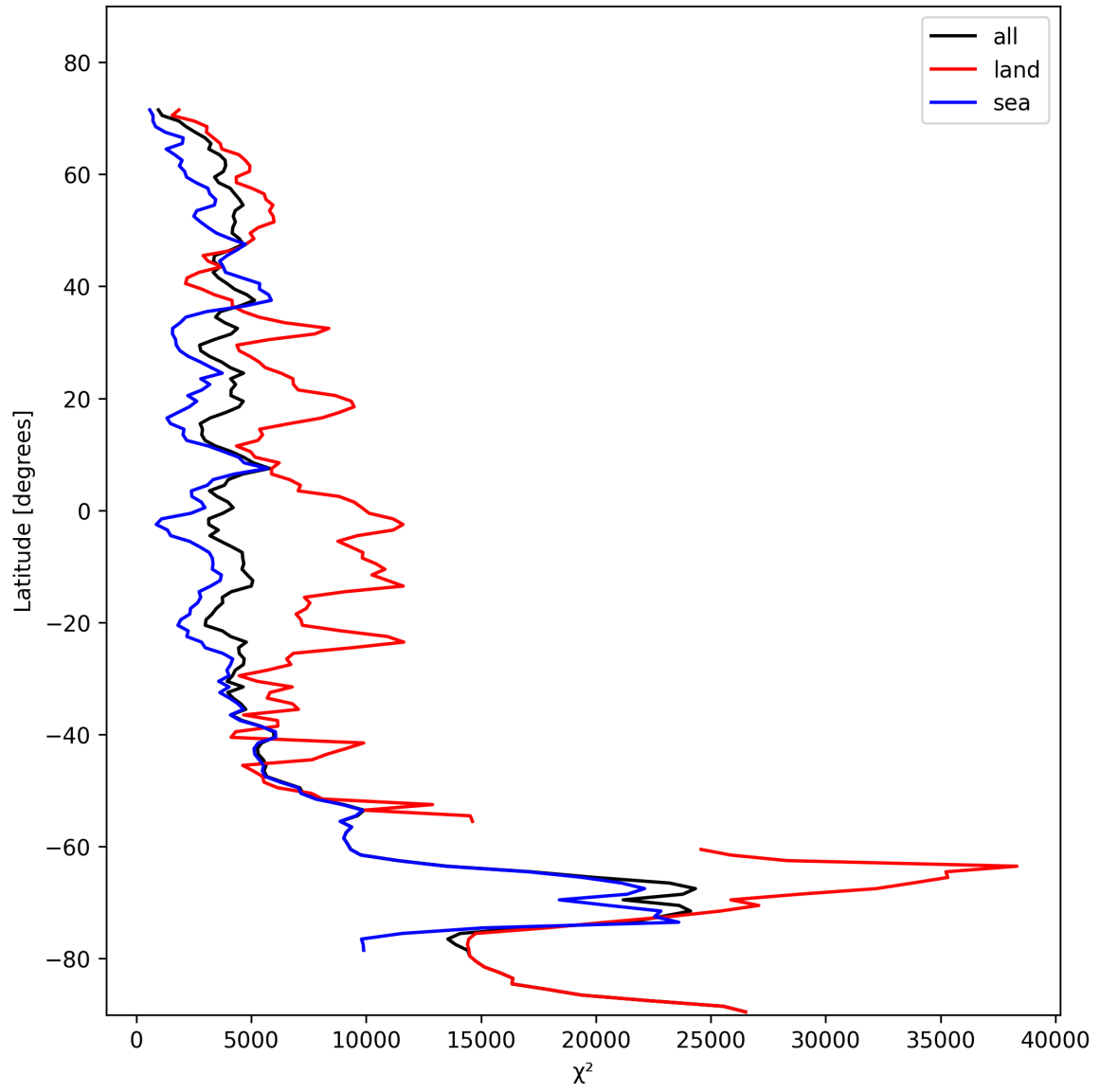
Figure 21: Zonal average of “ \chi^2 ” for 2024-11-06 to 2024-11-08.
