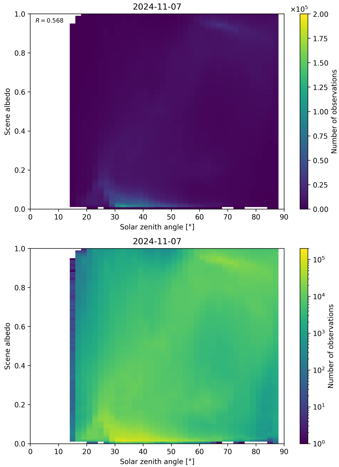
Figure 127: Scatter density plot of “Solar zenith angle” against “Scene albedo” for 2024-11-06 to 2024-11-08.
