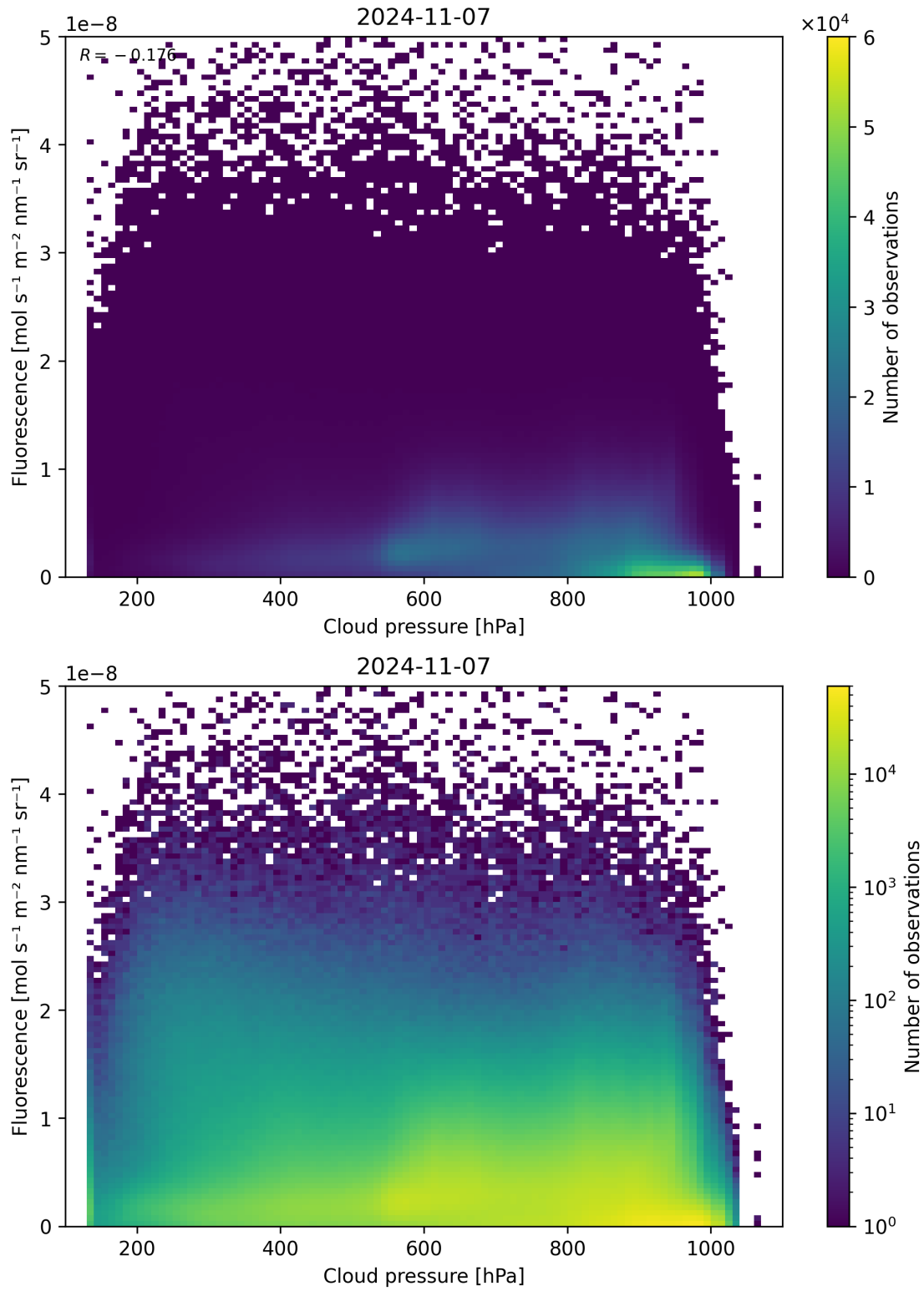
Figure 88: Scatter density plot of “Cloud pressure” against “Fluorescence” for 2024-11-06 to 2024-11-08.
