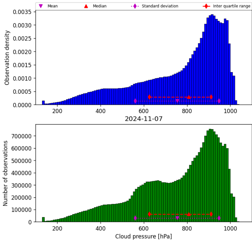
Figure 30: Histogram of “Cloud pressure” for 2024-11-06 to 2024-11-08
