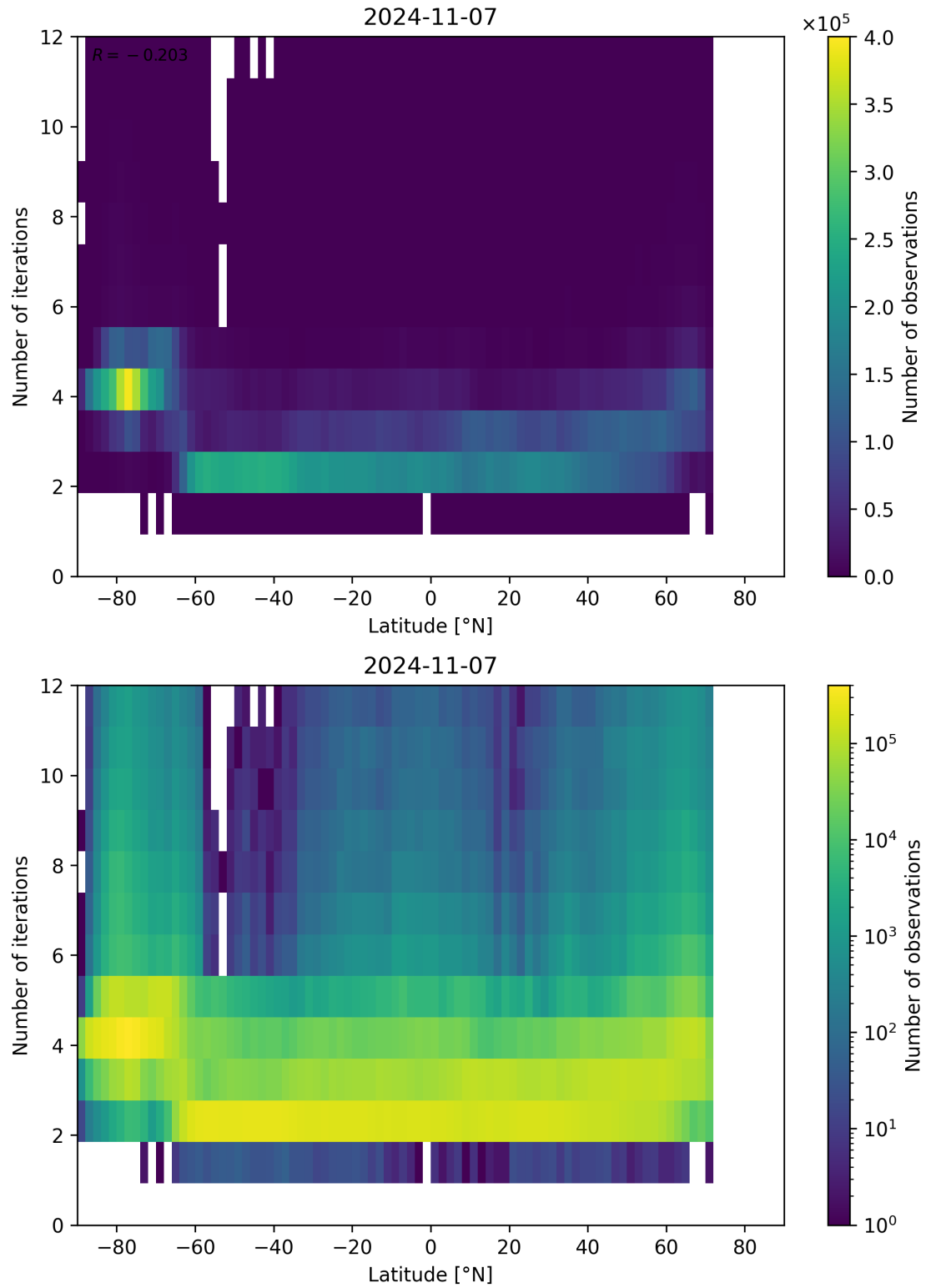
Figure 102: Scatter density plot of “Latitude” against “Number of iterations” for 2024-11-06 to 2024-11-08.
