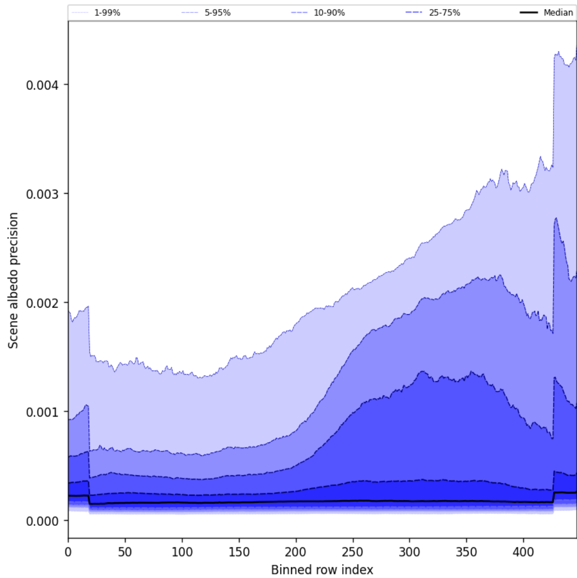
Figure 52: Along track statistics of “Scene albedo precision” for 2024-11-06 to 2024-11-08
