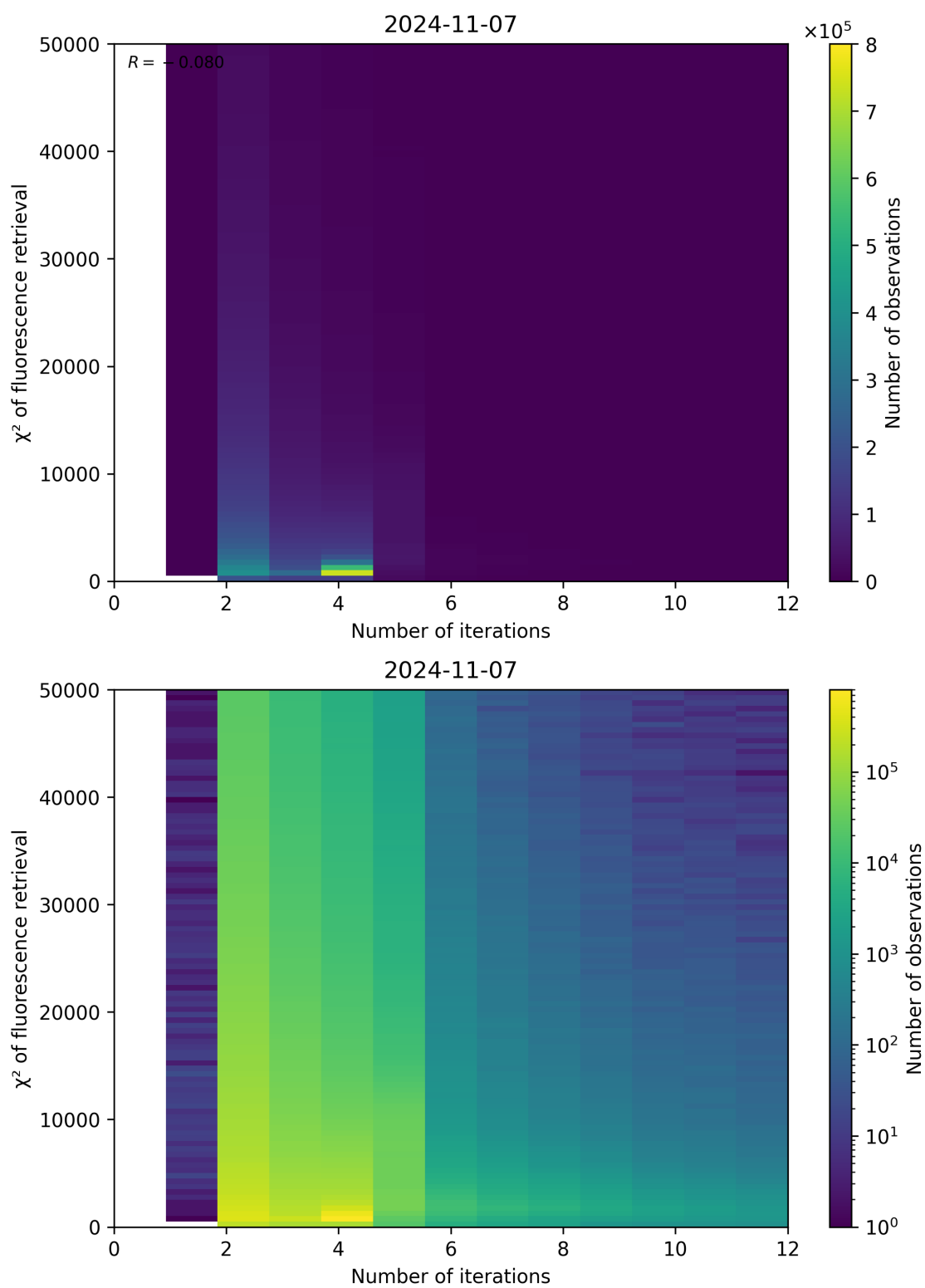
Figure 106: Scatter density plot of “Number of iterations” against “ \chi^2 of fluorescence retrieval” for 2024-11-06 to 2024-11-08.
