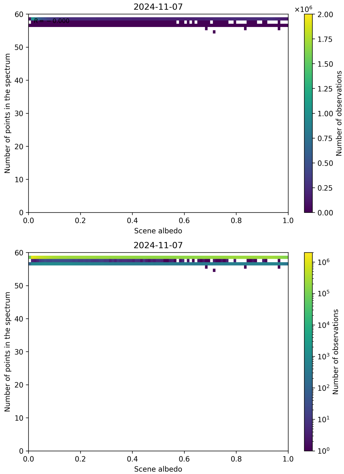
Figure 116: Scatter density plot of “Scene albedo” against “Number of points in the spectrum” for 2024-11-06 to 2024-11-08.
