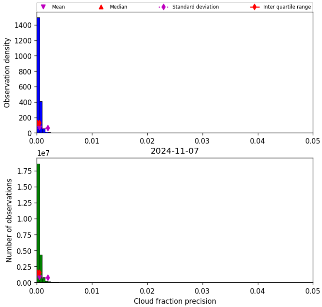
Figure 33: Histogram of “Cloud fraction precision” for 2024-11-06 to 2024-11-08
