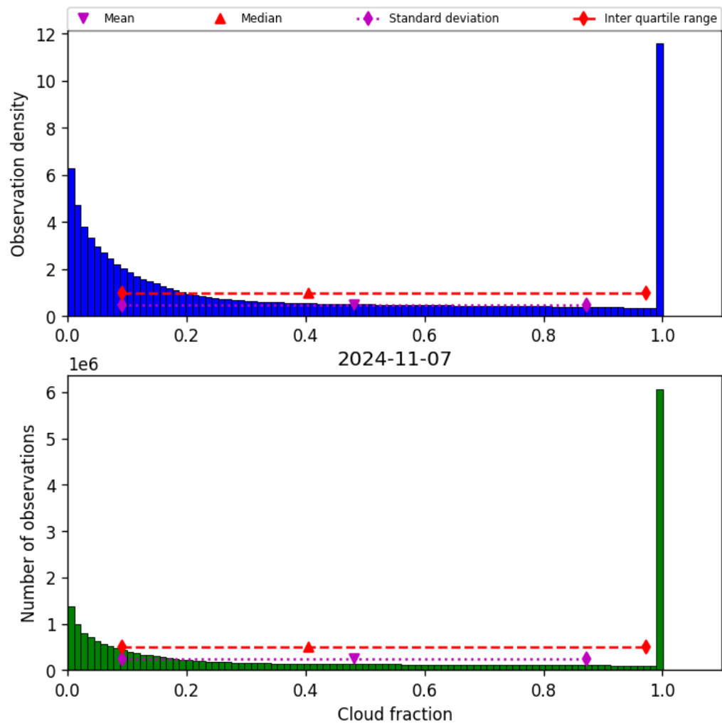
Figure 32: Histogram of “Cloud fraction” for 2024-11-06 to 2024-11-08
