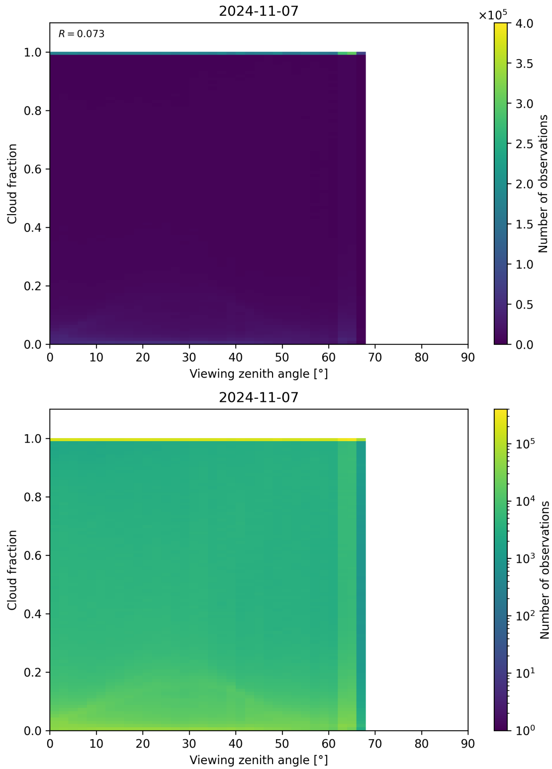
Figure 132: Scatter density plot of “Viewing zenith angle” against “Cloud fraction” for 2024-11-06 to 2024-11-08.
