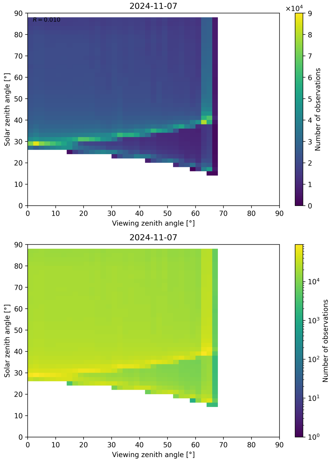
Figure 139: Scatter density plot of “Viewing zenith angle” against “Solar zenith angle” for 2024-11-06 to 2024-11-08.
