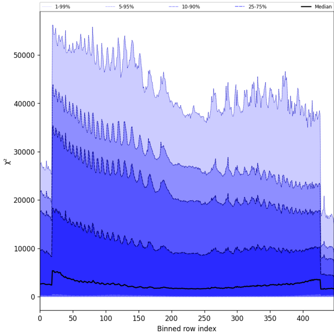
Figure 55: Along track statistics of “ \chi^2 ” for 2024-11-06 to 2024-11-08
