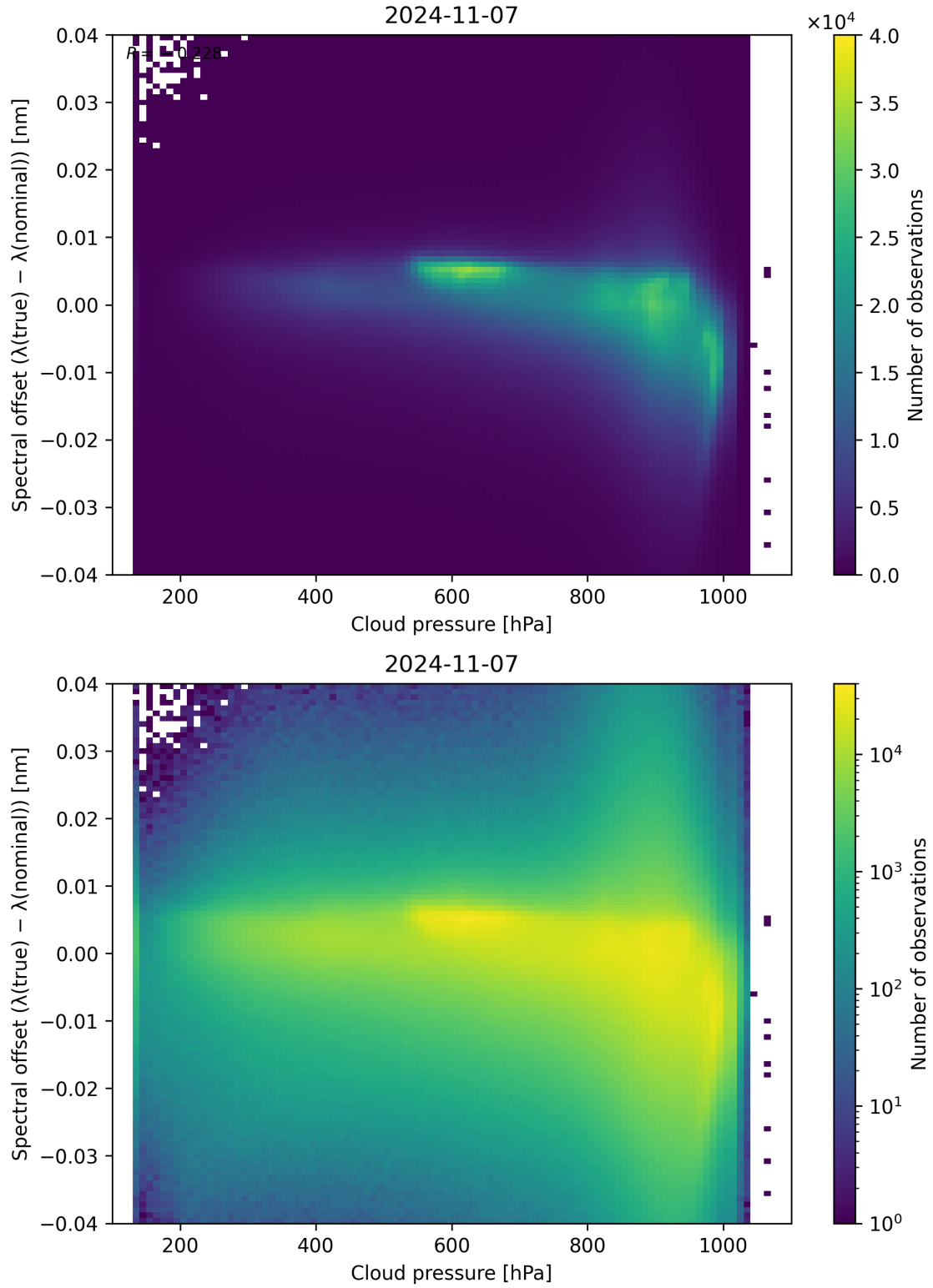
Figure 92: Scatter density plot of “Cloud pressure” against “Spectral offset ( \lambda_{\text{true}} - \lambda_{\text{nominal}} )” for 2024-11-06 to 2024-11-08.
