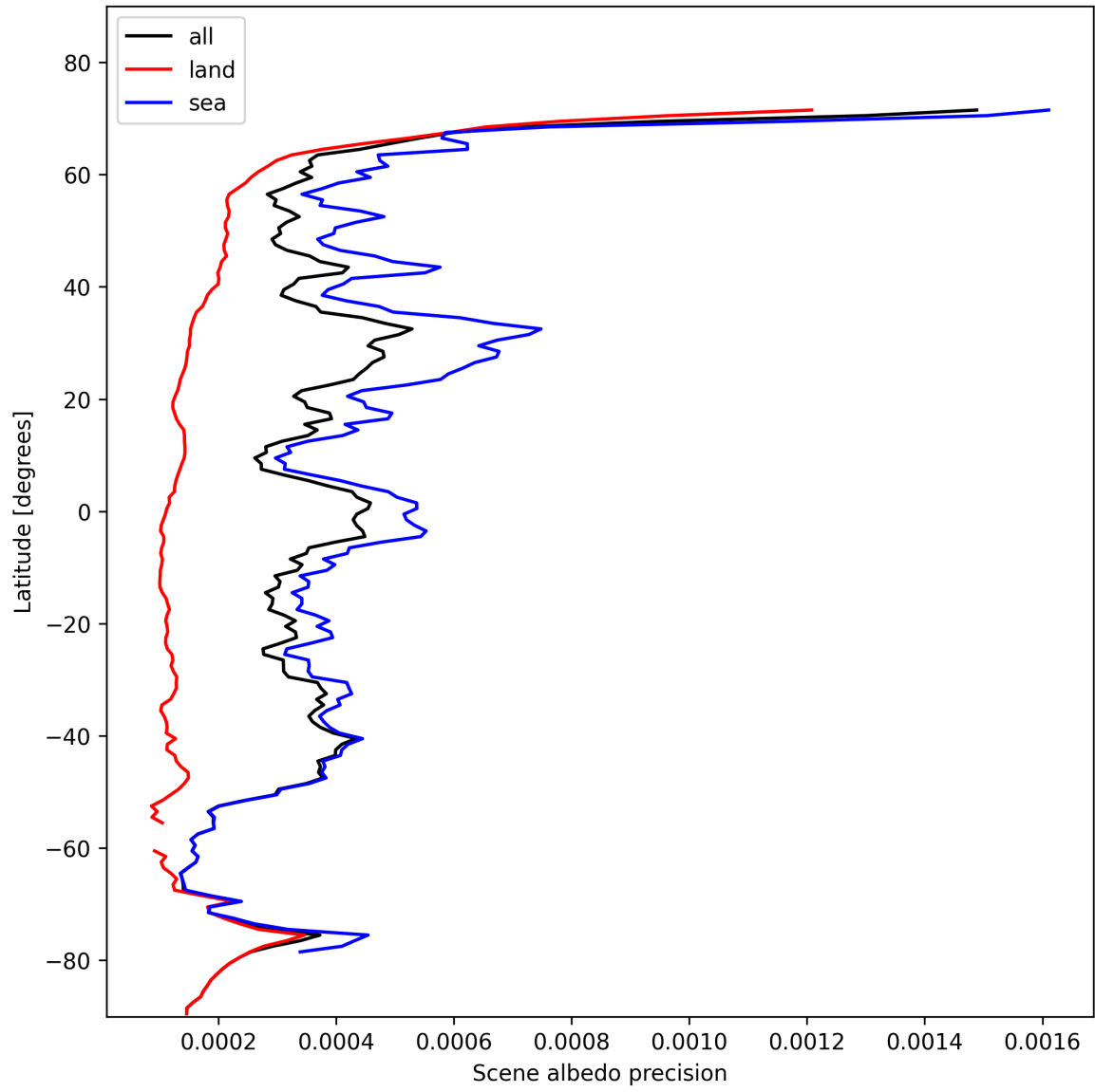
Figure 18: Zonal average of “Scene albedo precision” for 2024-11-06 to 2024-11-08.
