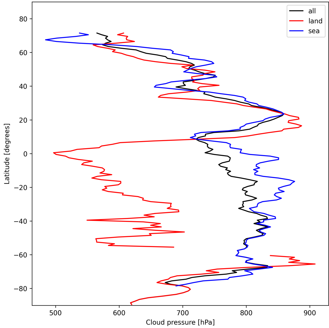
Figure 13: Zonal average of “Cloud pressure” for 2024-11-06 to 2024-11-08.
