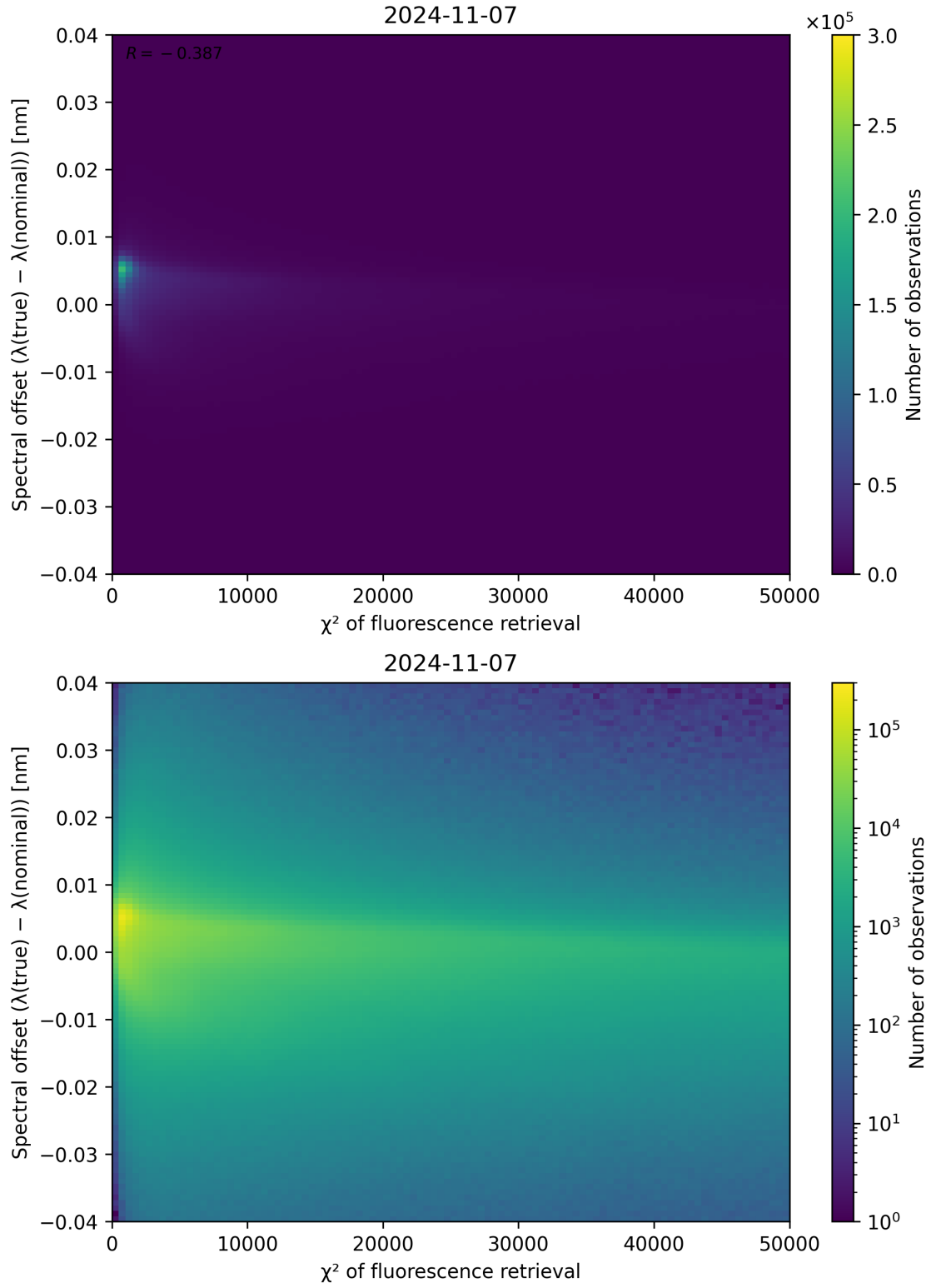
Figure 72: Scatter density plot of “ \chi^2 of fluorescence retrieval” against “Spectral offset ( \lambda_{\text{true}} - \lambda_{\text{nominal}} )” for 2024-11-06 to 2024-11-08.
