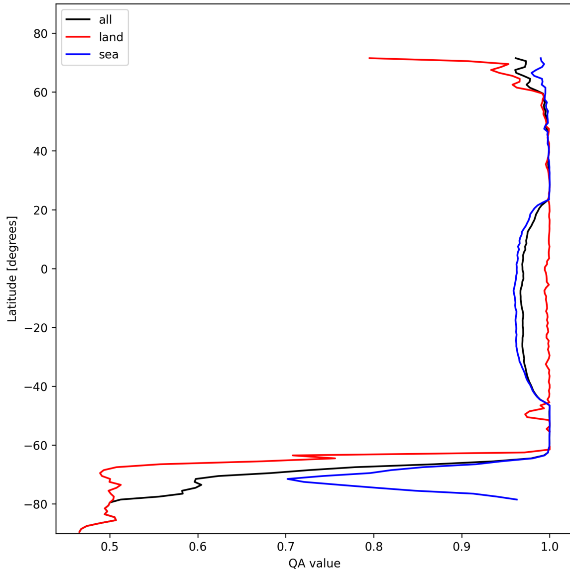
Figure 12: Zonal average of “QA value” for 2024-11-06 to 2024-11-08.
