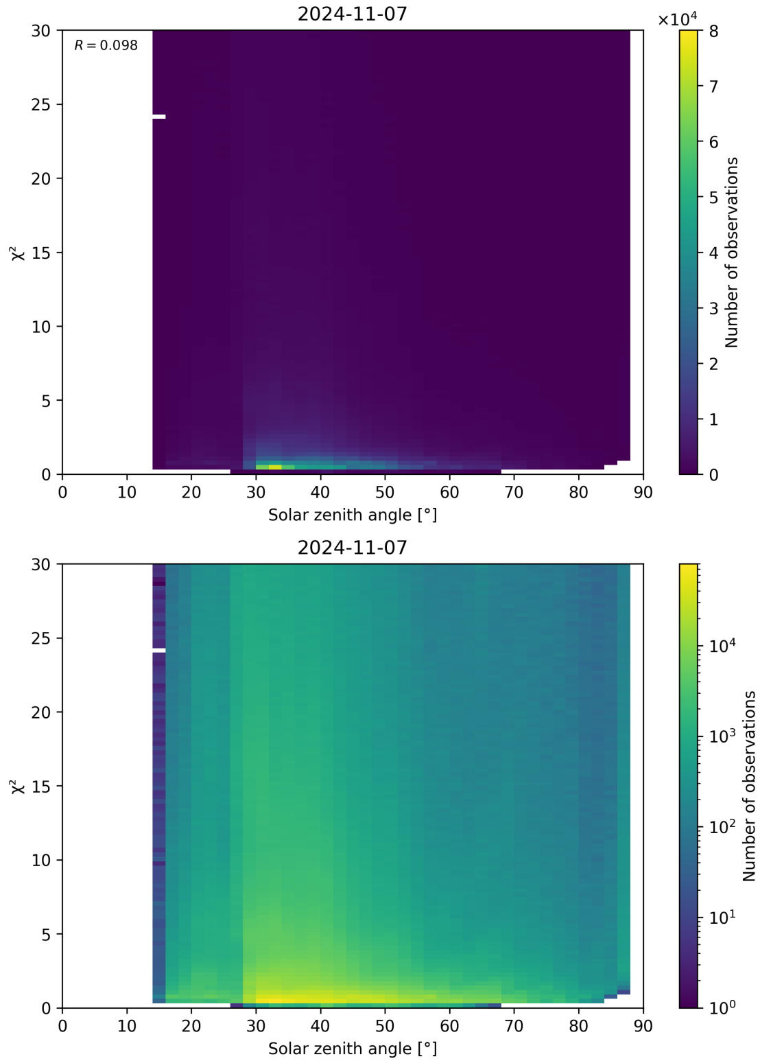
Figure 119: Scatter density plot of “Solar zenith angle” against “ \chi^2 ” for 2024-11-06 to 2024-11-08.
