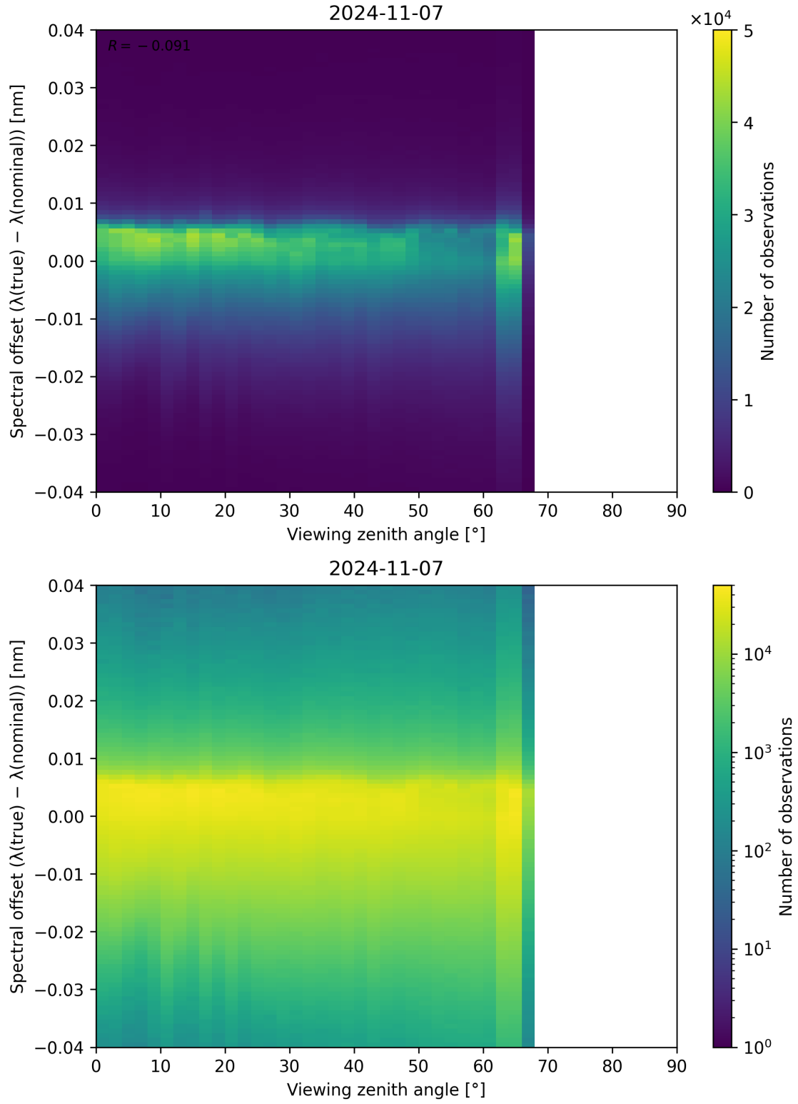
Figure 140: Scatter density plot of “Viewing zenith angle” against “Spectral offset ( \lambda_{\text{true}} - \lambda_{\text{nominal}} )” for 2024-11-06 to 2024-11-08.
