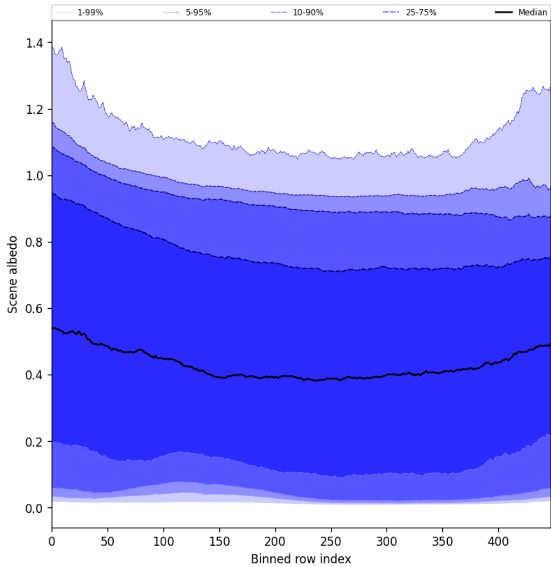
Figure 51: Along track statistics of “Scene albedo” for 2024-11-06 to 2024-11-08
