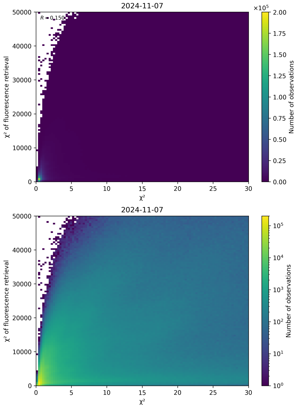
Figure 69: Scatter density plot of “ \chi^2 ” against “ \chi^2 of fluorescence retrieval” for 2024-11-06 to 2024-11-08.
