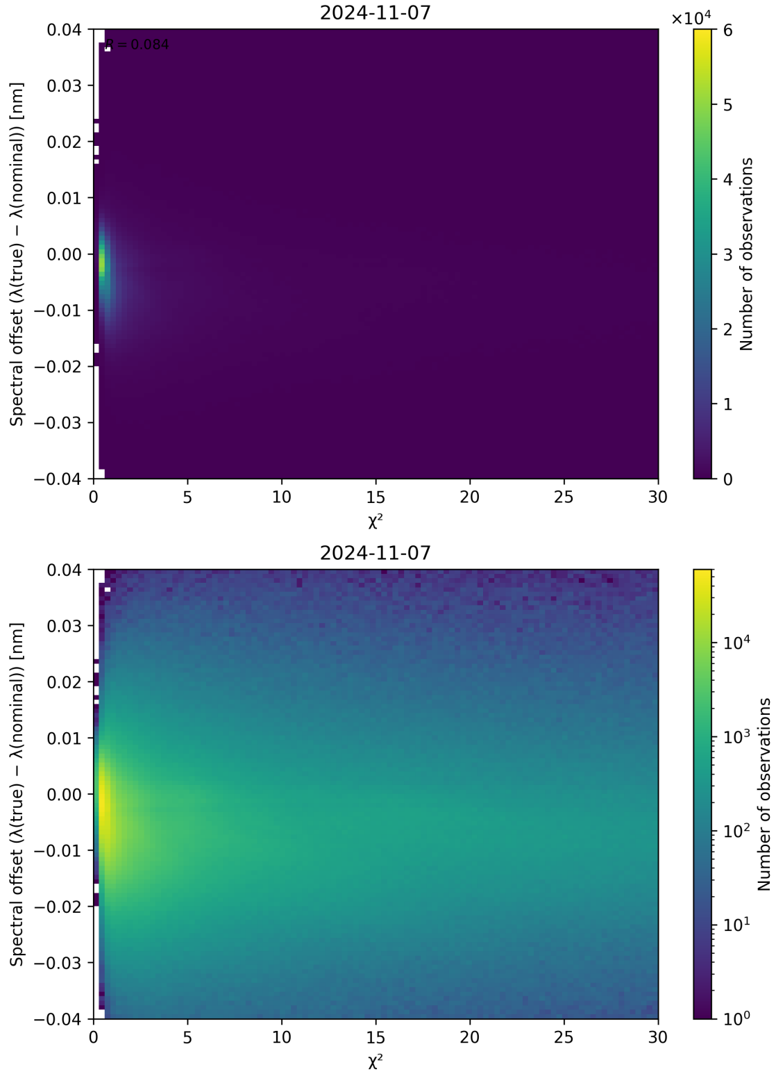
Figure 75: Scatter density plot of “ \chi^2 ” against “Spectral offset ( \lambda_{\text{true}} - \lambda_{\text{nominal}} )” for 2024-11-06 to 2024-11-08.
