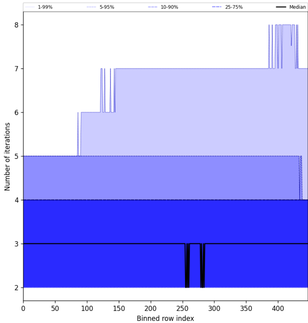
Figure 56: Along track statistics of “Number of iterations” for 2024-11-06 to 2024-11-08
