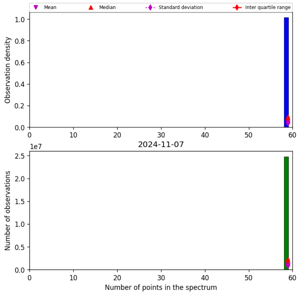
Figure 44: Histogram of “Number of points in the spectrum” for 2024-11-06 to 2024-11-08
