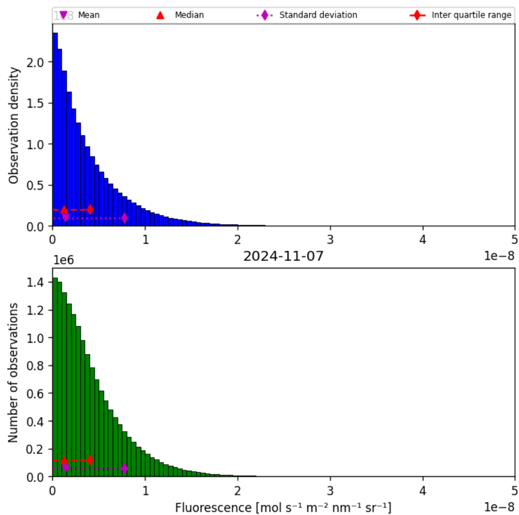
Figure 40: Histogram of “Fluorescence” for 2024-11-06 to 2024-11-08
