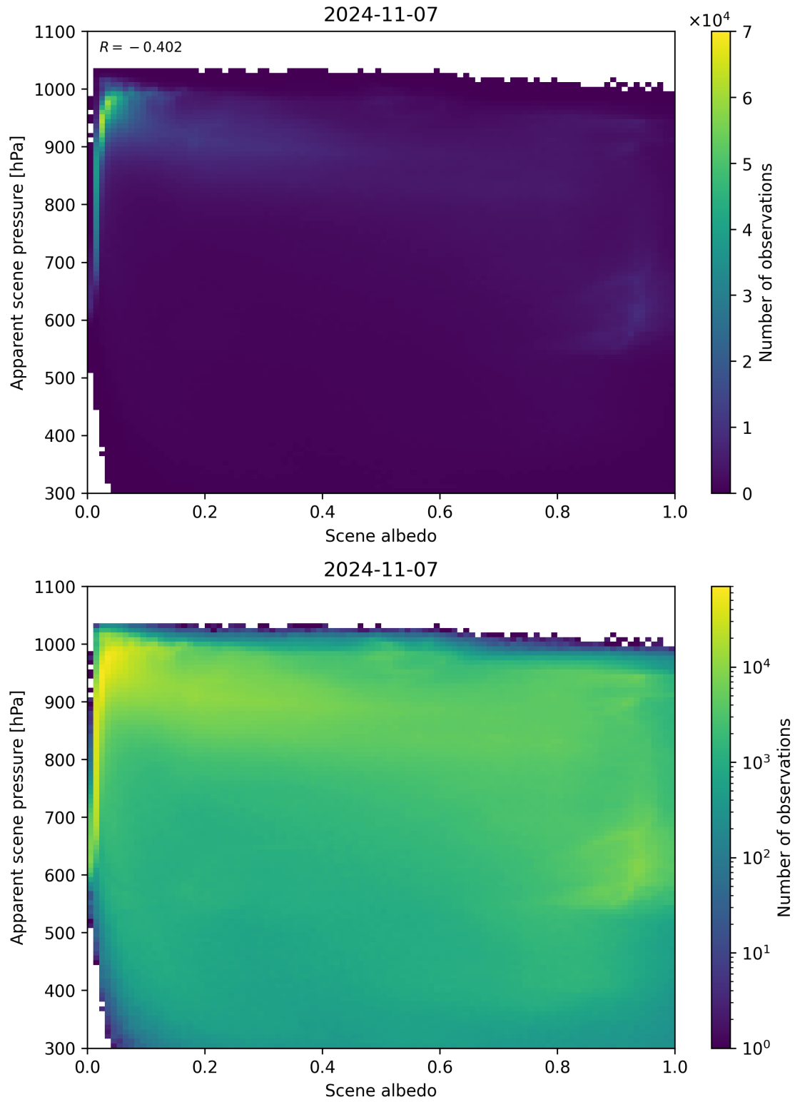
Figure 111: Scatter density plot of “Scene albedo” against “Apparent scene pressure” for 2024-11-06 to 2024-11-08.
