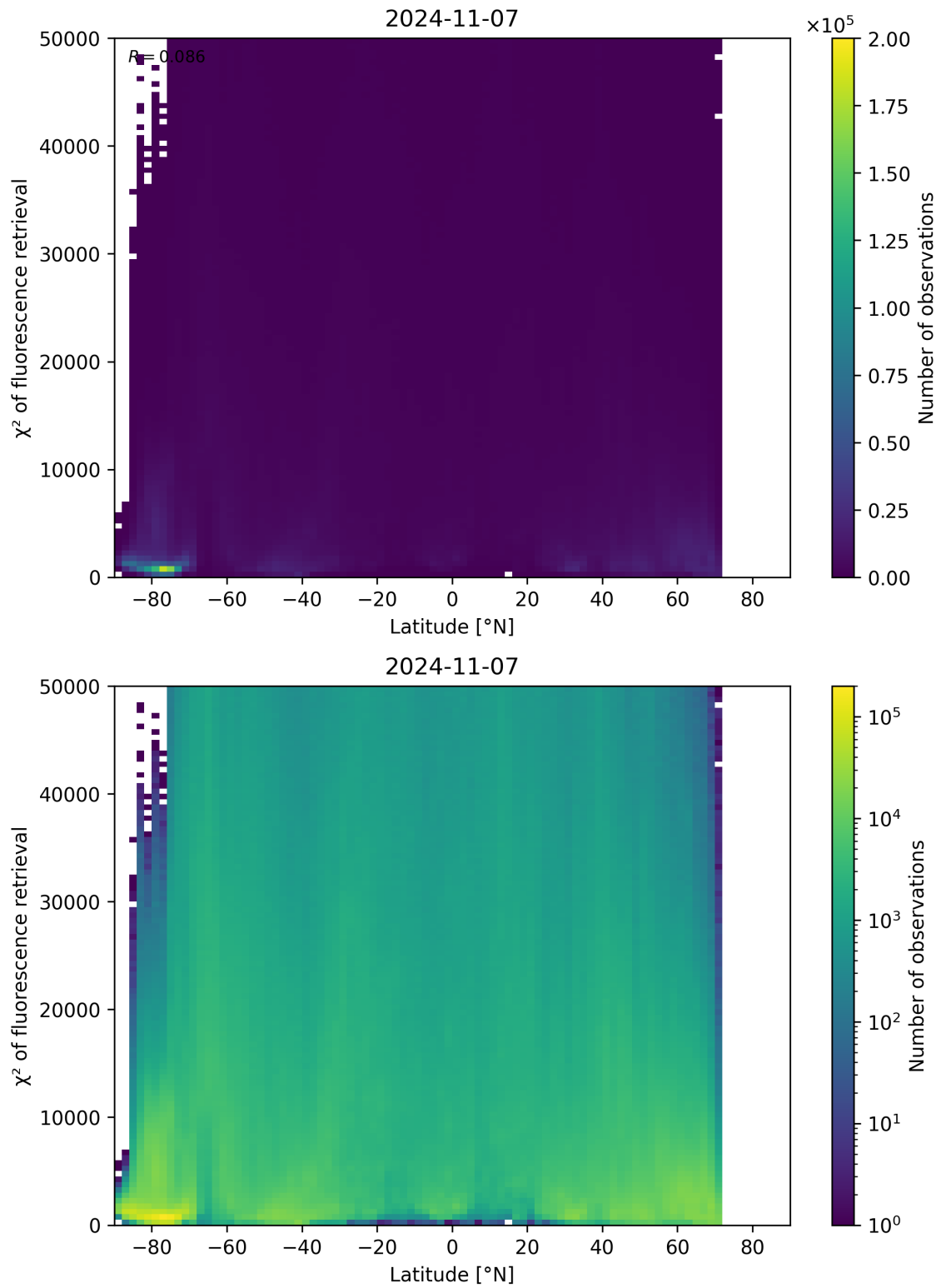
Figure 98: Scatter density plot of “Latitude” against “ \chi^2 of fluorescence retrieval” for 2024-11-06 to 2024-11-08.
