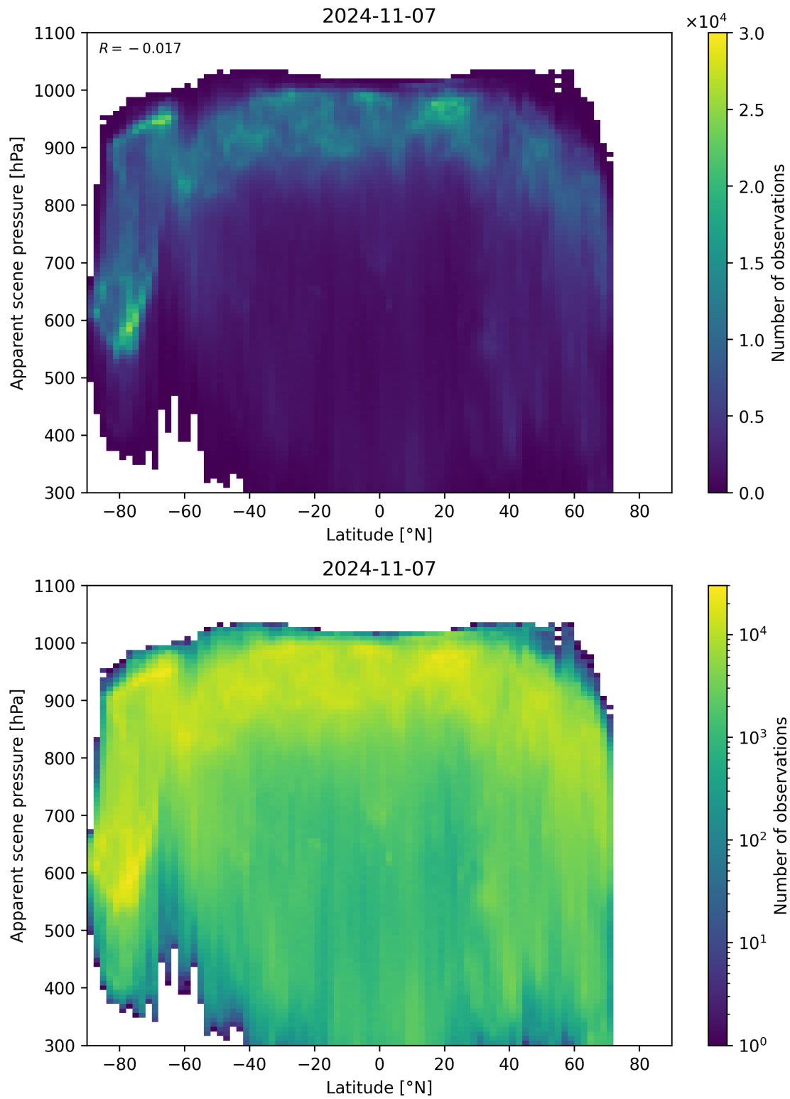
Figure 96: Scatter density plot of “Latitude” against “Apparent scene pressure” for 2024-11-06 to 2024-11-08.
