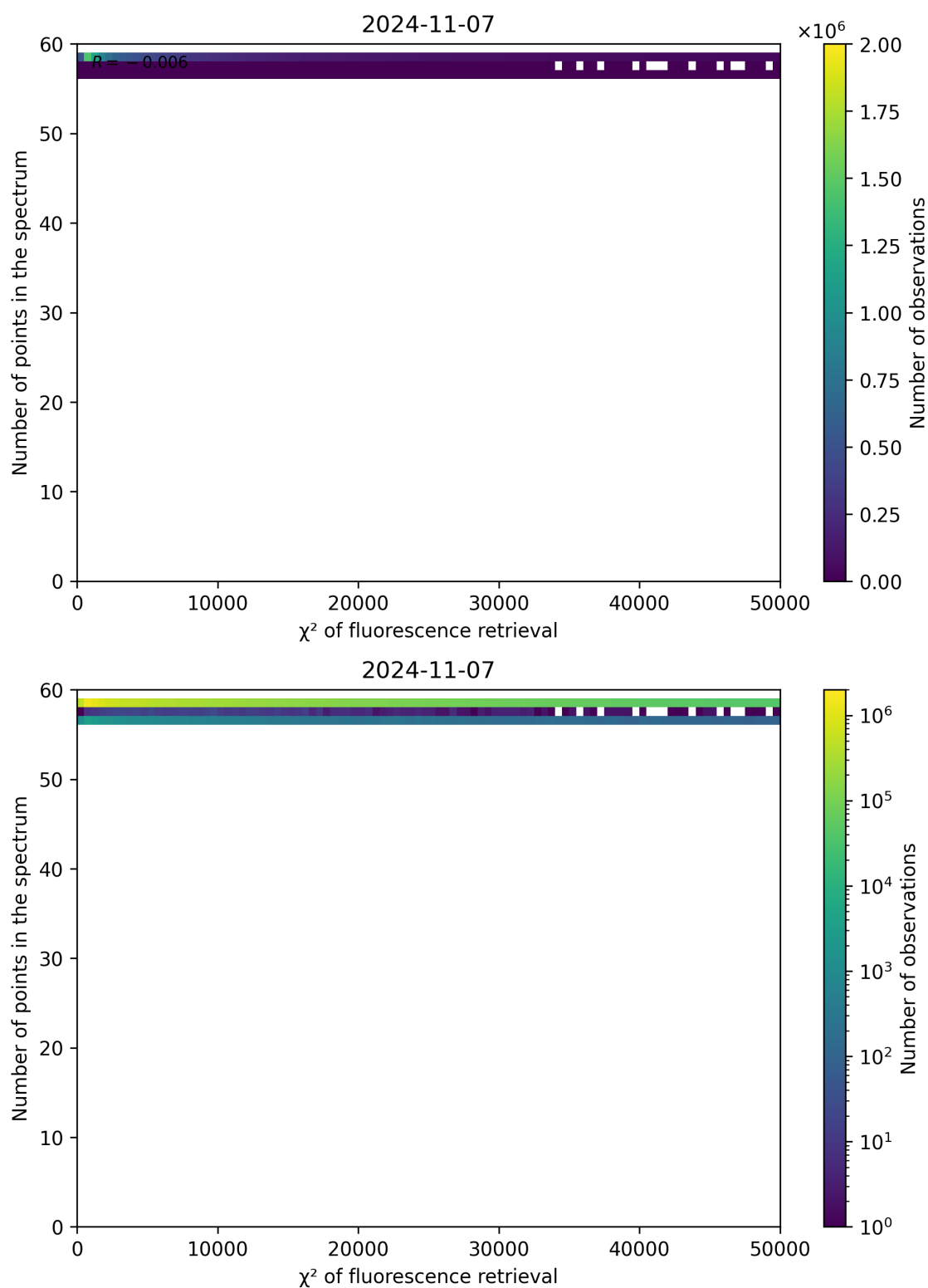
Figure 71: Scatter density plot of " \chi^2 of fluorescence retrieval" against "Number of points in the spectrum" for 2024-11-06 to 2024-11-08.
