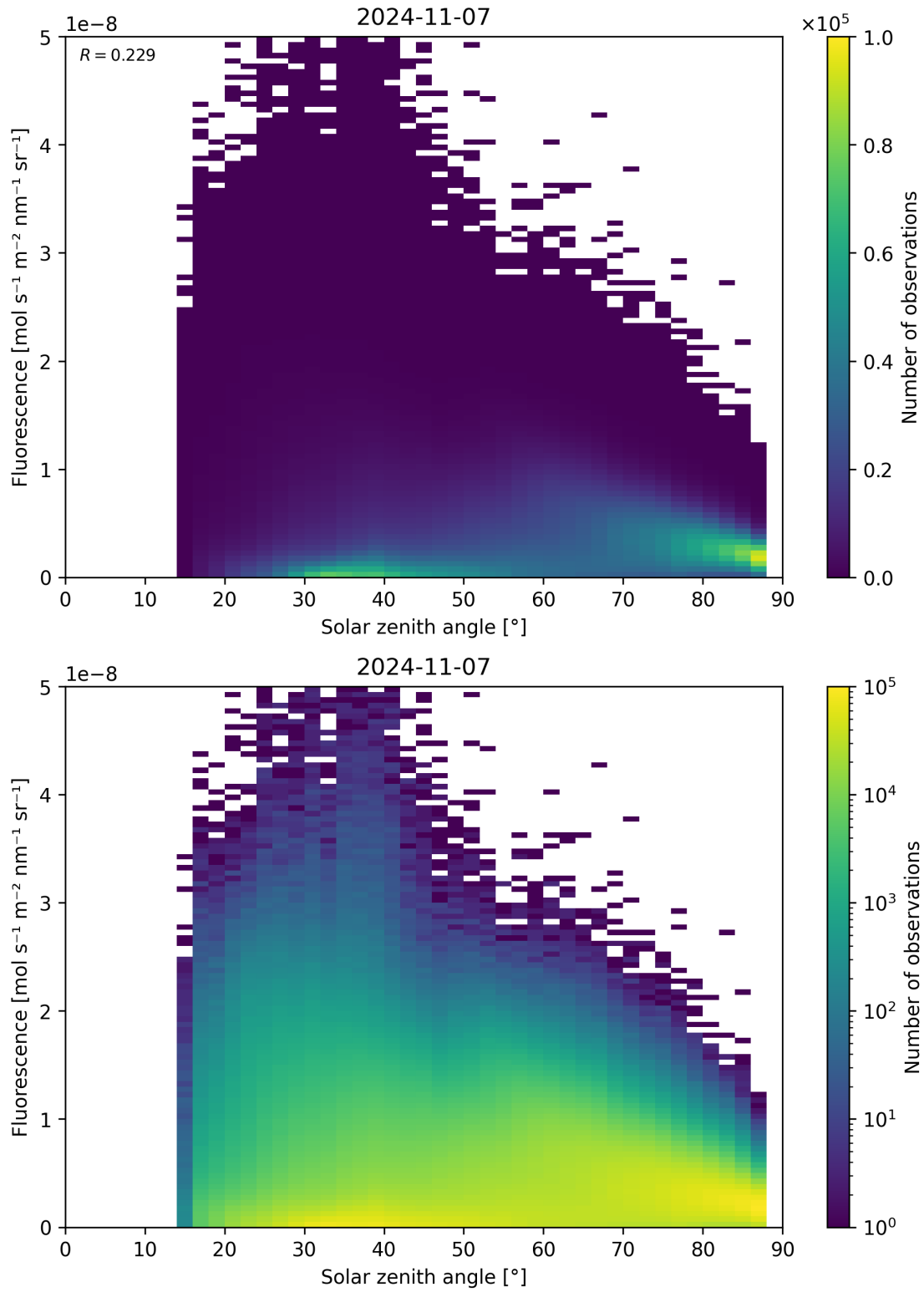
Figure 123: Scatter density plot of “Solar zenith angle” against “Fluorescence” for 2024-11-06 to 2024-11-08.
