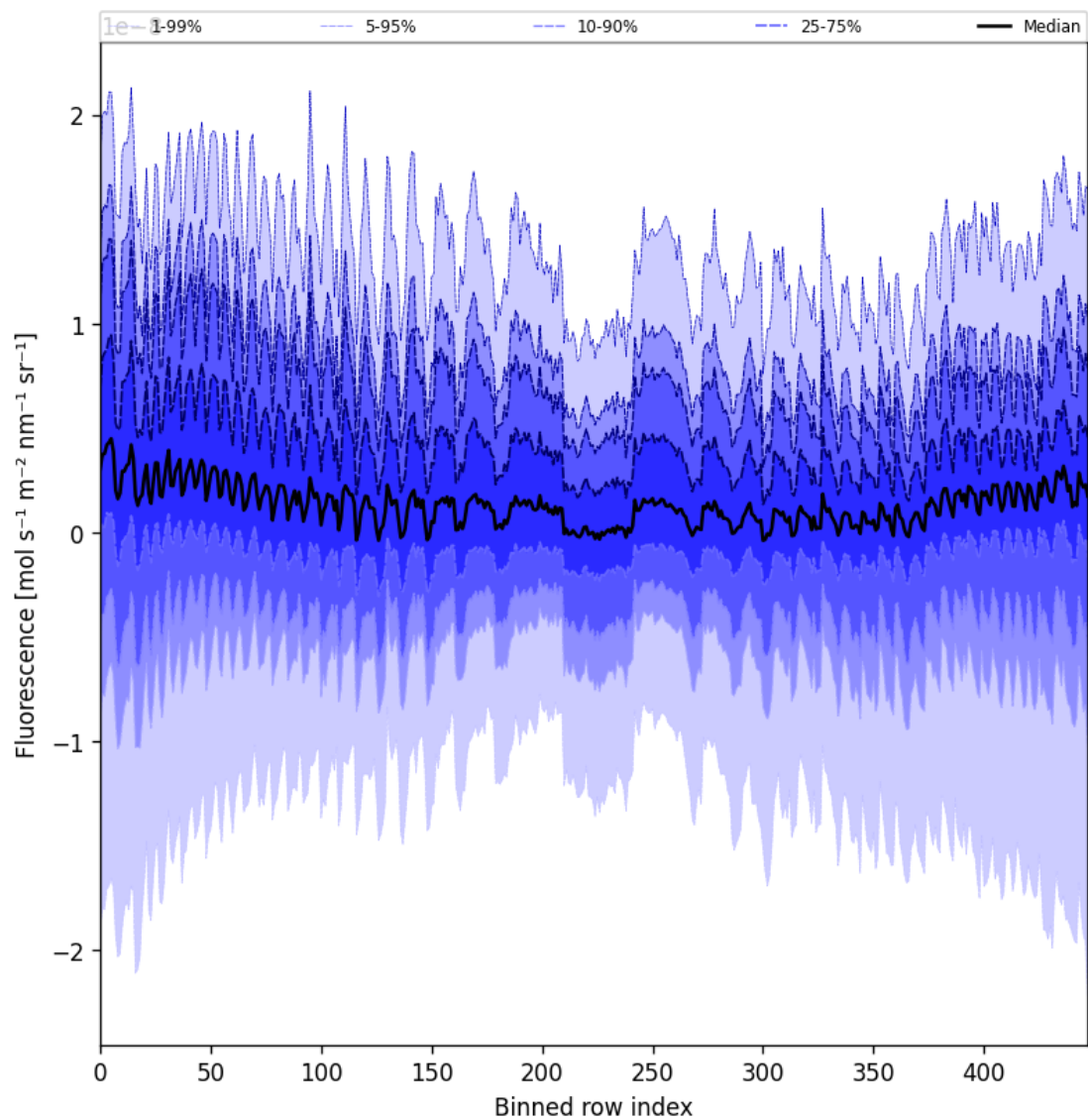
Figure 57: Along track statistics of “Fluorescence” for 2024-11-06 to 2024-11-08
