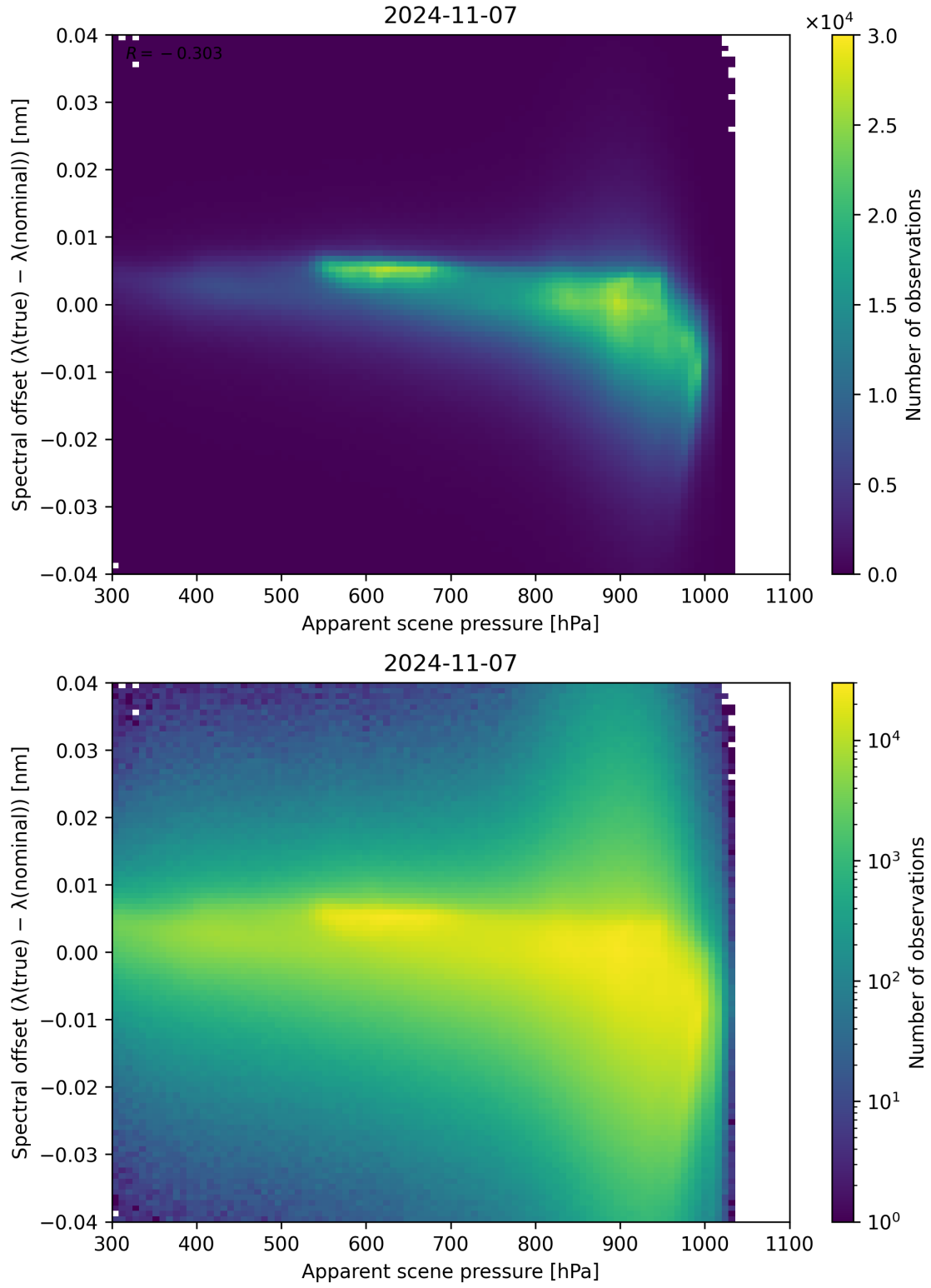
Figure 68: Scatter density plot of “Apparent scene pressure” against “Spectral offset ( \lambda_{\text{true}} - \lambda_{\text{nominal}} )” for 2024-11-06 to 2024-11-08.
