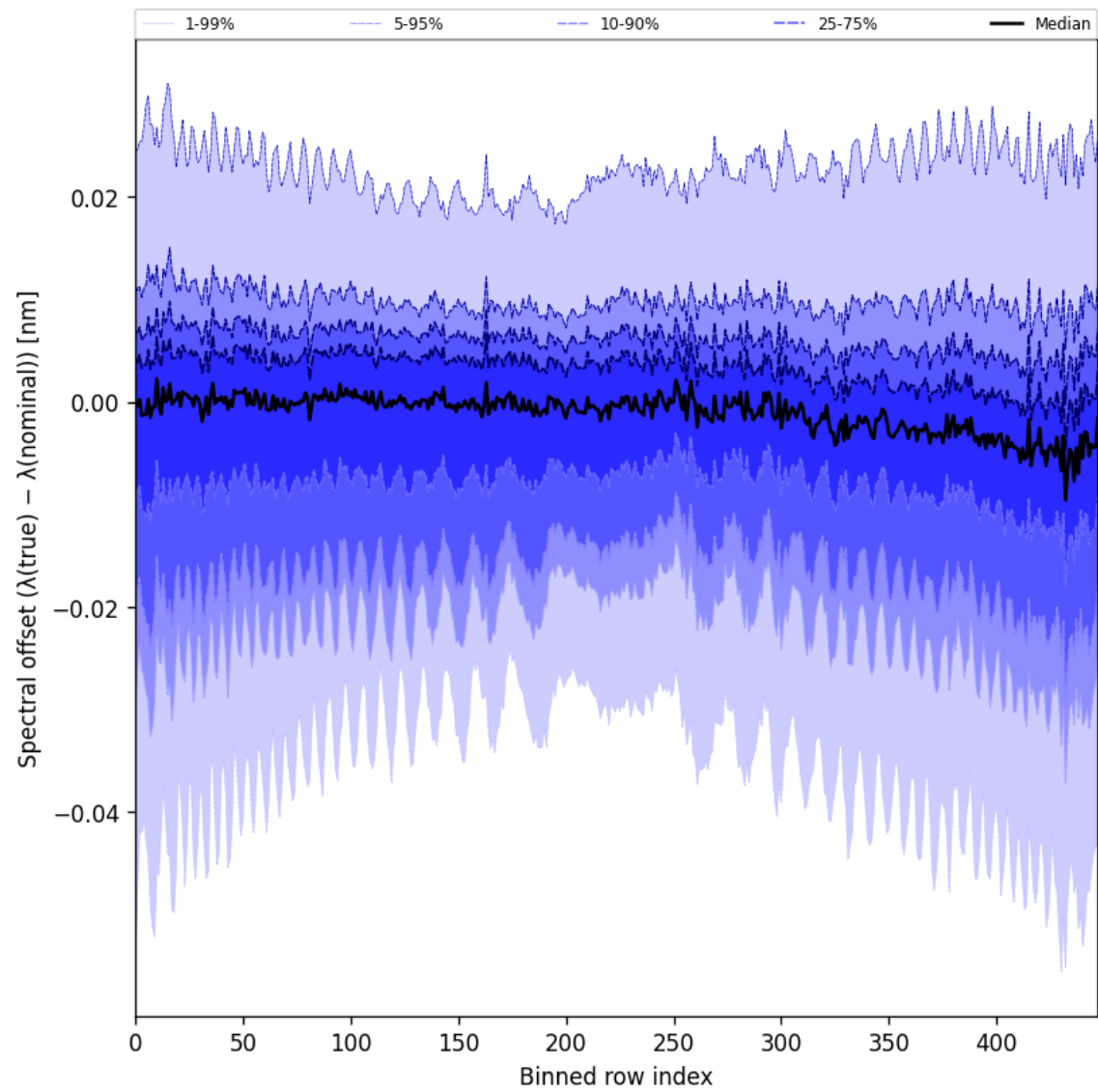
Figure 62: Along track statistics of “Spectral offset ( \lambda_{\text{true}} - \lambda_{\text{nominal}} )” for 2024-11-06 to 2024-11-08
