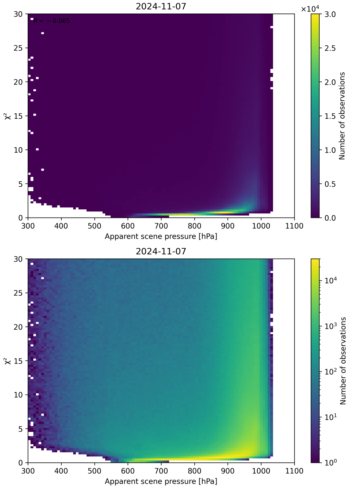
Figure 63: Scatter density plot of “Apparent scene pressure” against “ \chi^2 ” for 2024-11-06 to 2024-11-08.
