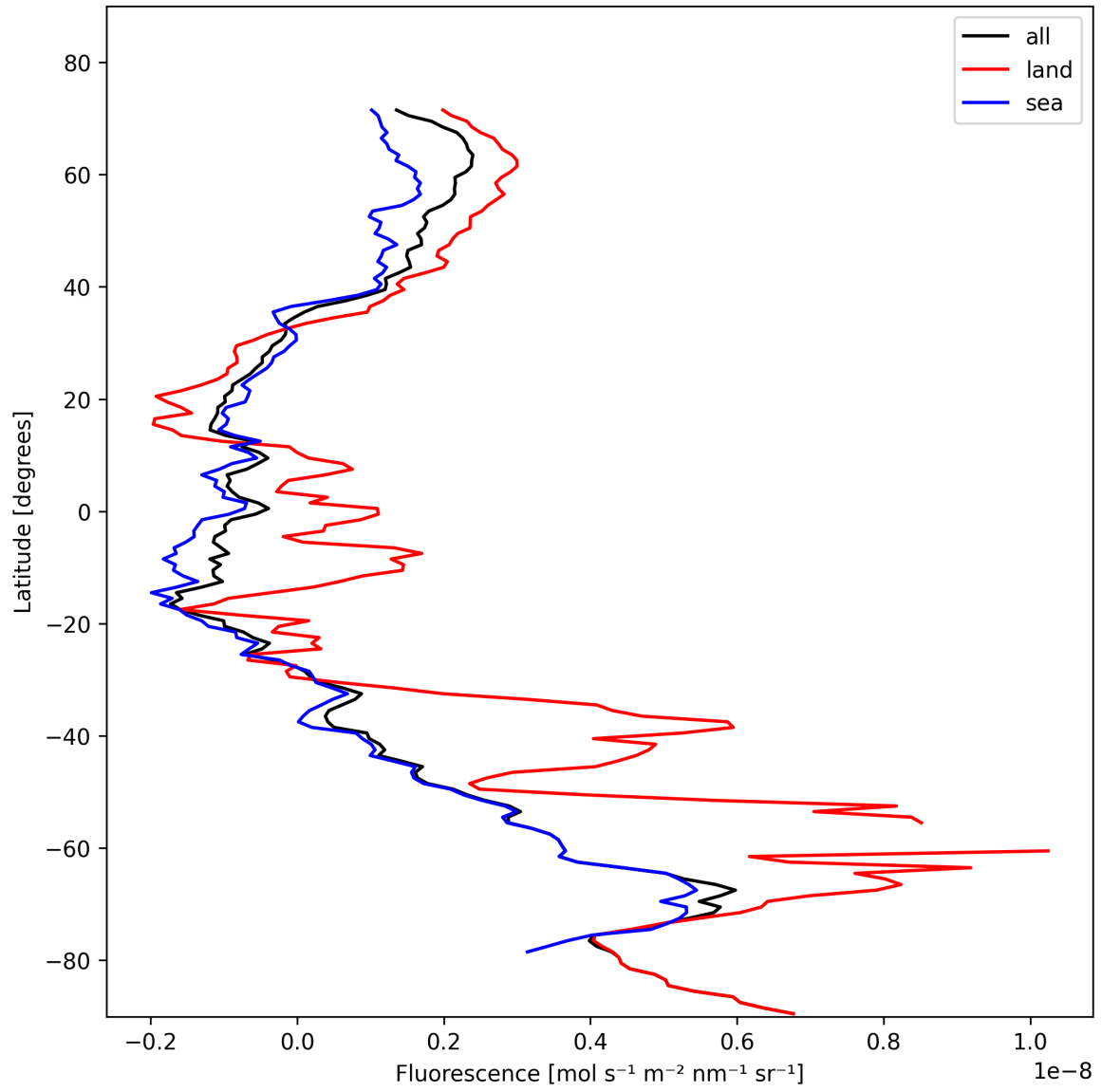
Figure 23: Zonal average of “Fluorescence” for 2024-11-06 to 2024-11-08.
