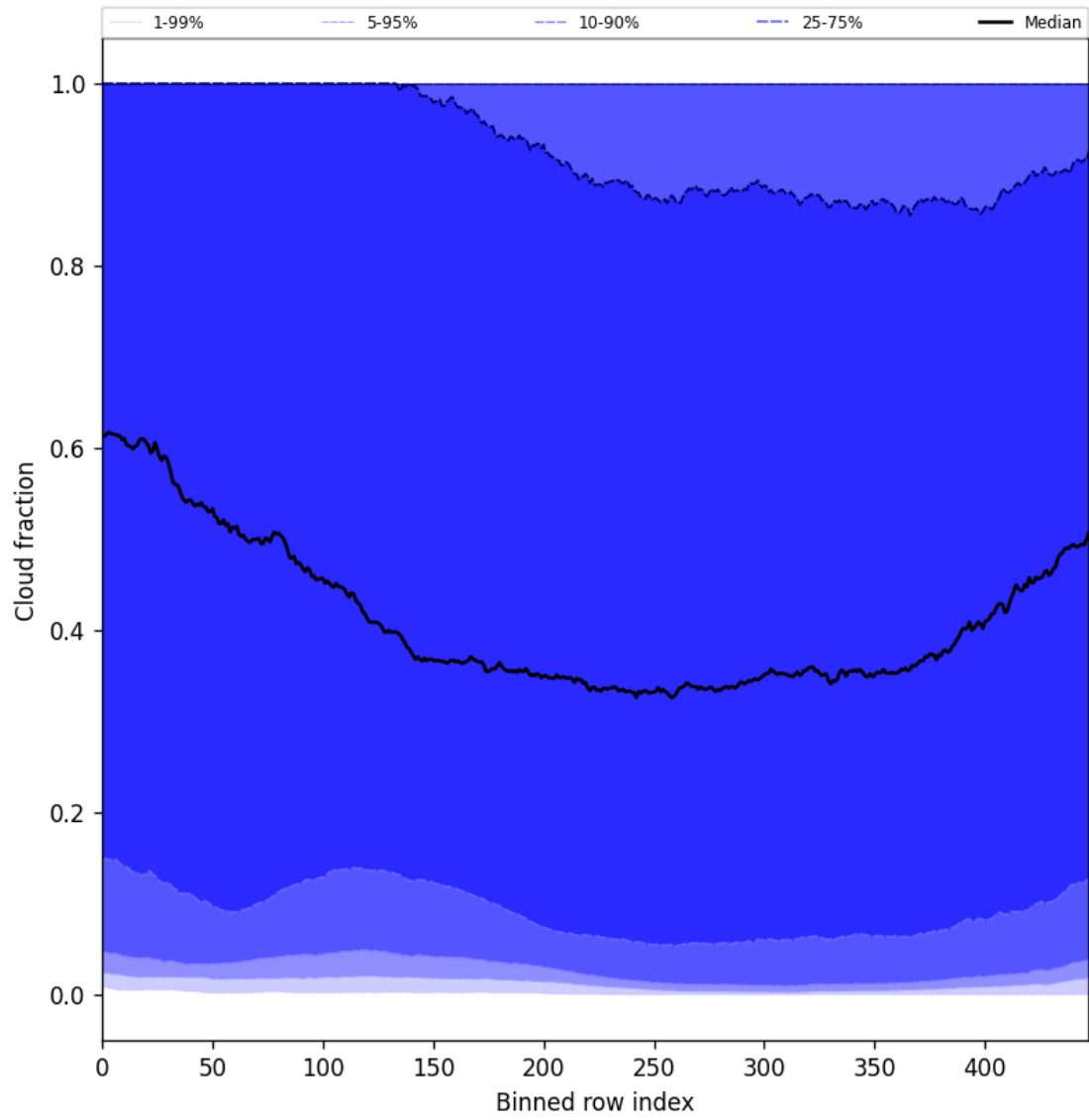
Figure 49: Along track statistics of “Cloud fraction” for 2024-11-06 to 2024-11-08
