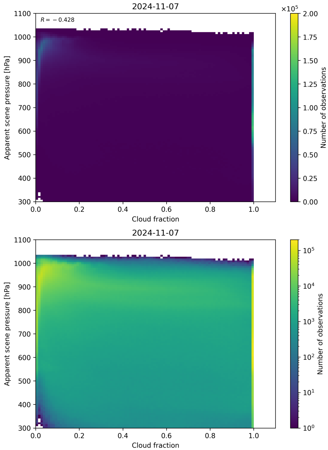
Figure 76: Scatter density plot of “Cloud fraction” against “Apparent scene pressure” for 2024-11-06 to 2024-11-08.
