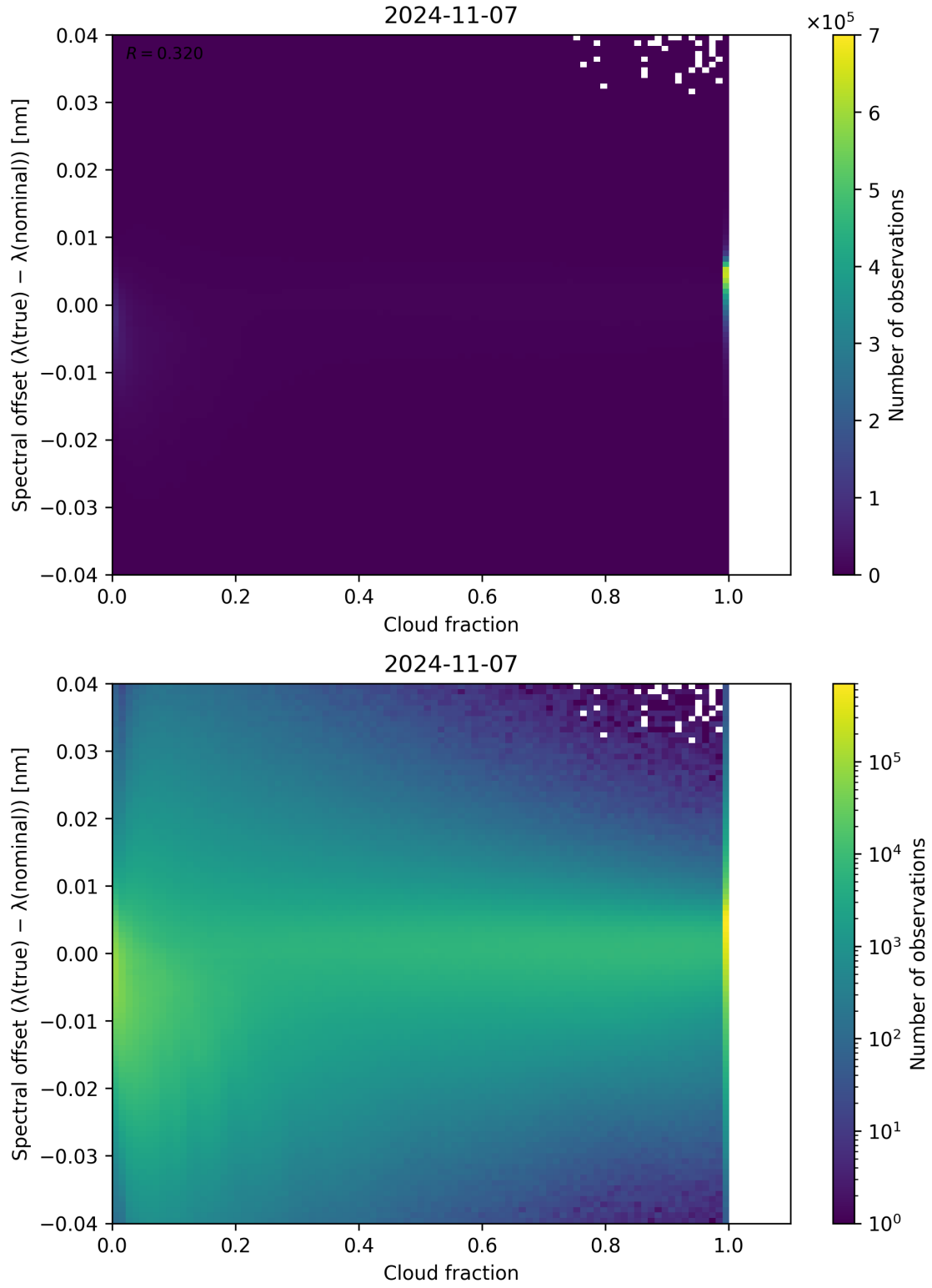
Figure 83: Scatter density plot of “Cloud fraction” against “Spectral offset ( \lambda_{\text{true}} - \lambda_{\text{nominal}} )” for 2024-11-06 to 2024-11-08.
