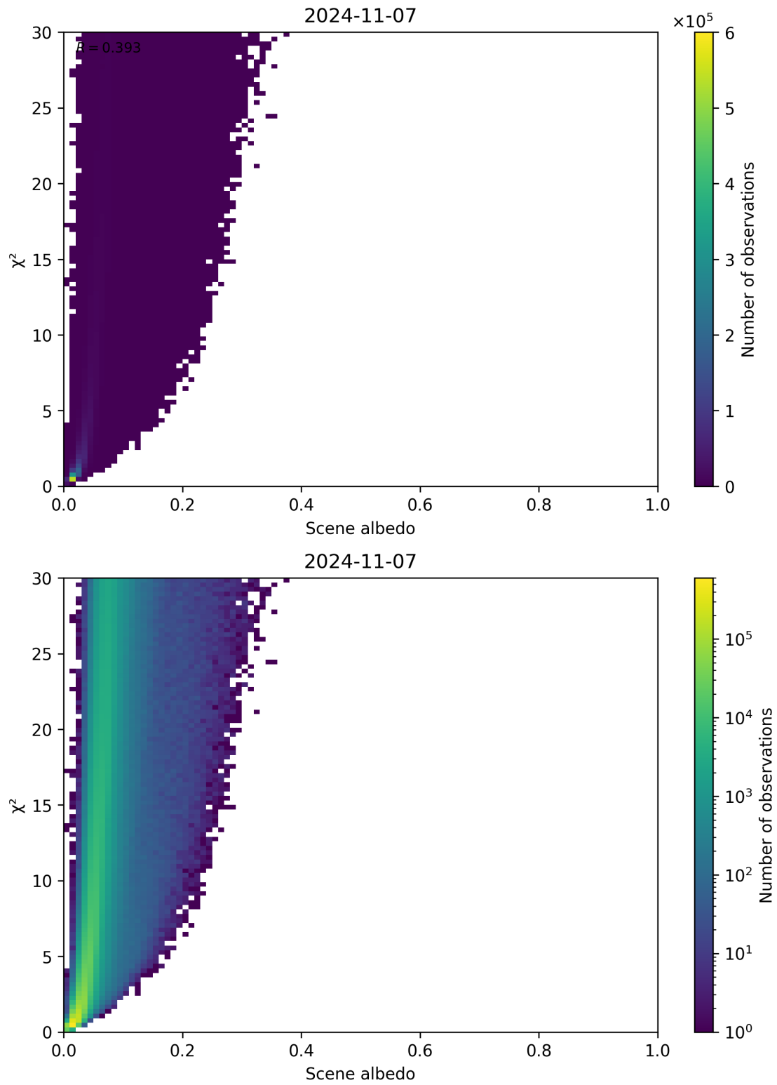
Figure 112: Scatter density plot of “Scene albedo” against “ \chi^2 ” for 2024-11-06 to 2024-11-08.
