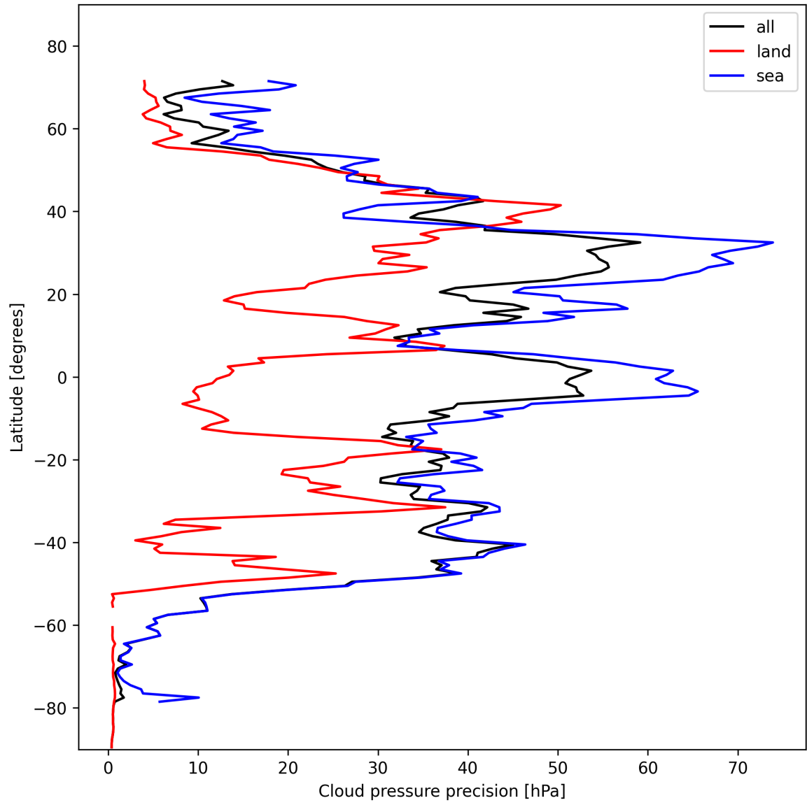
Figure 14: Zonal average of “Cloud pressure precision” for 2024-11-06 to 2024-11-08.
