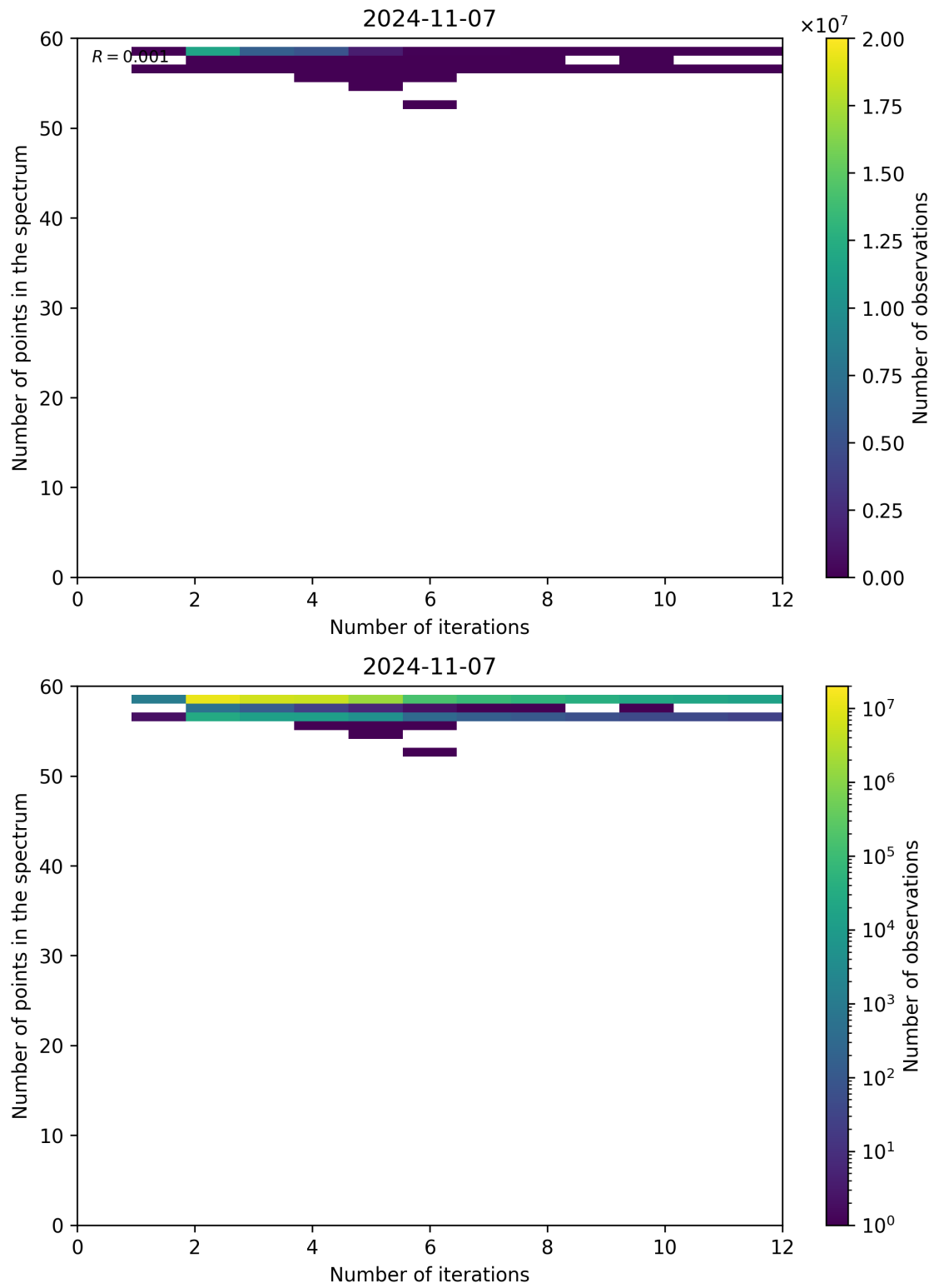
Figure 108: Scatter density plot of “Number of iterations” against “Number of points in the spectrum” for 2024-11-06 to 2024-11-08.
