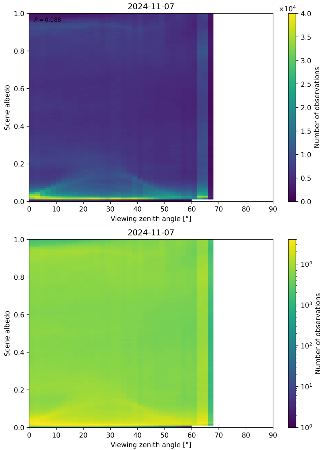
Figure 138: Scatter density plot of “Viewing zenith angle” against “Scene albedo” for 2024-11-06 to 2024-11-08.
