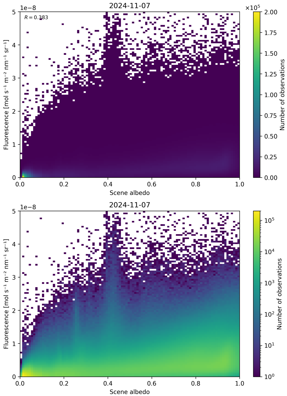
Figure 114: Scatter density plot of “Scene albedo” against “Fluorescence” for 2024-11-06 to 2024-11-08.
