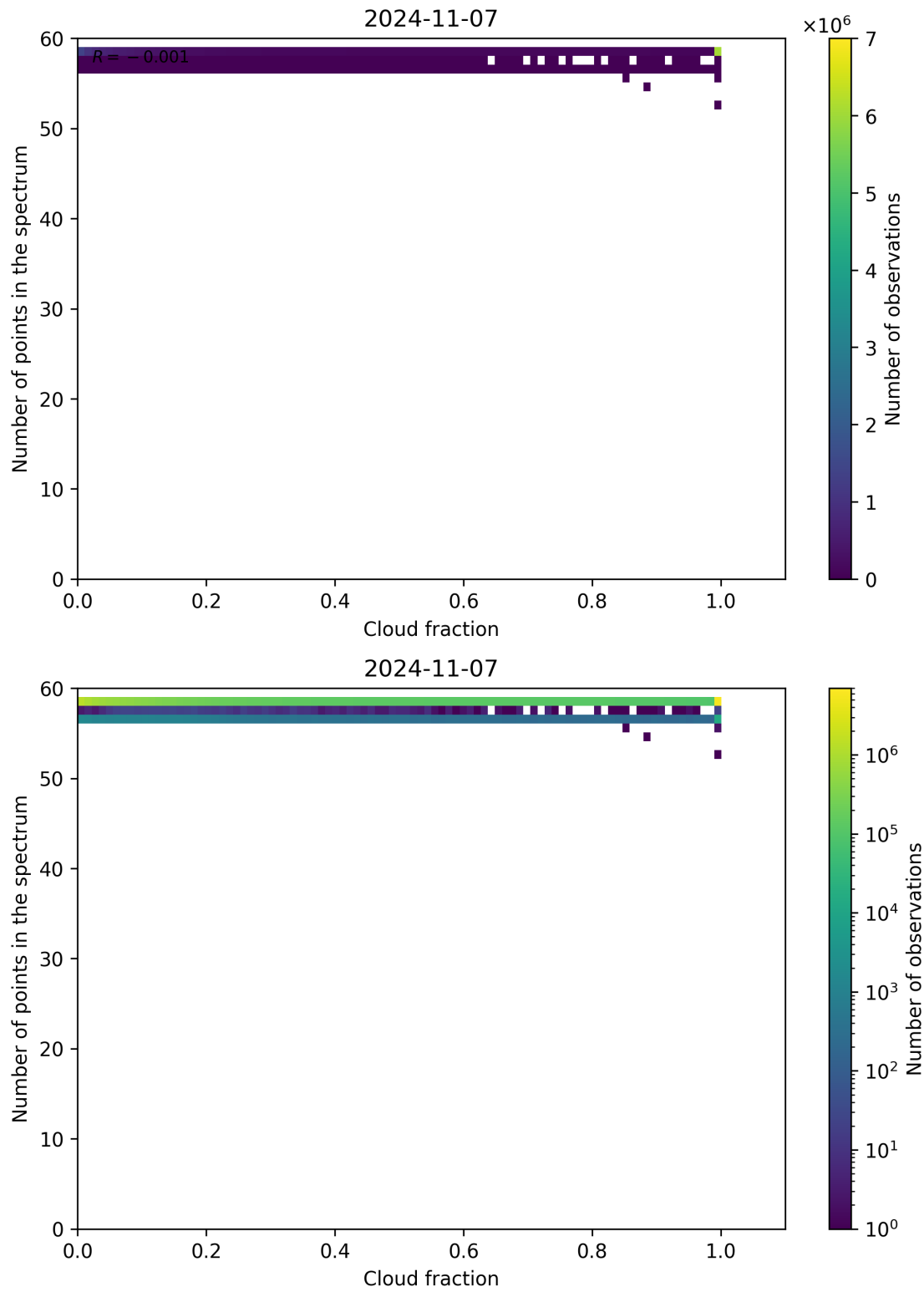
Figure 81: Scatter density plot of “Cloud fraction” against “Number of points in the spectrum” for 2024-11-06 to 2024-11-08.
