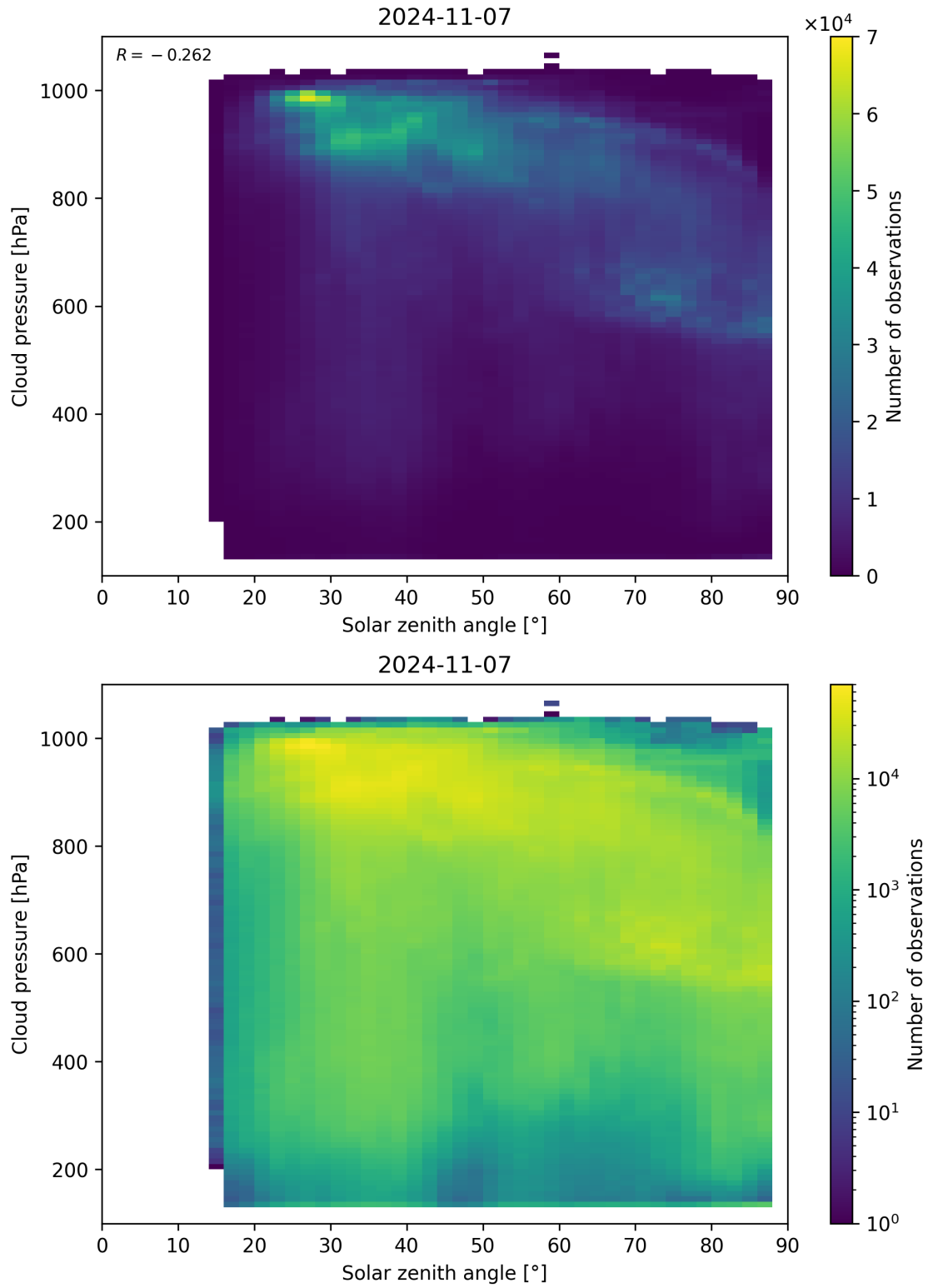
Figure 122: Scatter density plot of “Solar zenith angle” against “Cloud pressure” for 2024-11-06 to 2024-11-08.
