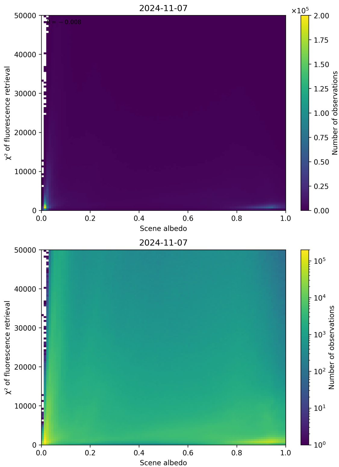
Figure 113: Scatter density plot of “Scene albedo” against “ \chi^2 of fluorescence retrieval” for 2024-11-06 to 2024-11-08.
