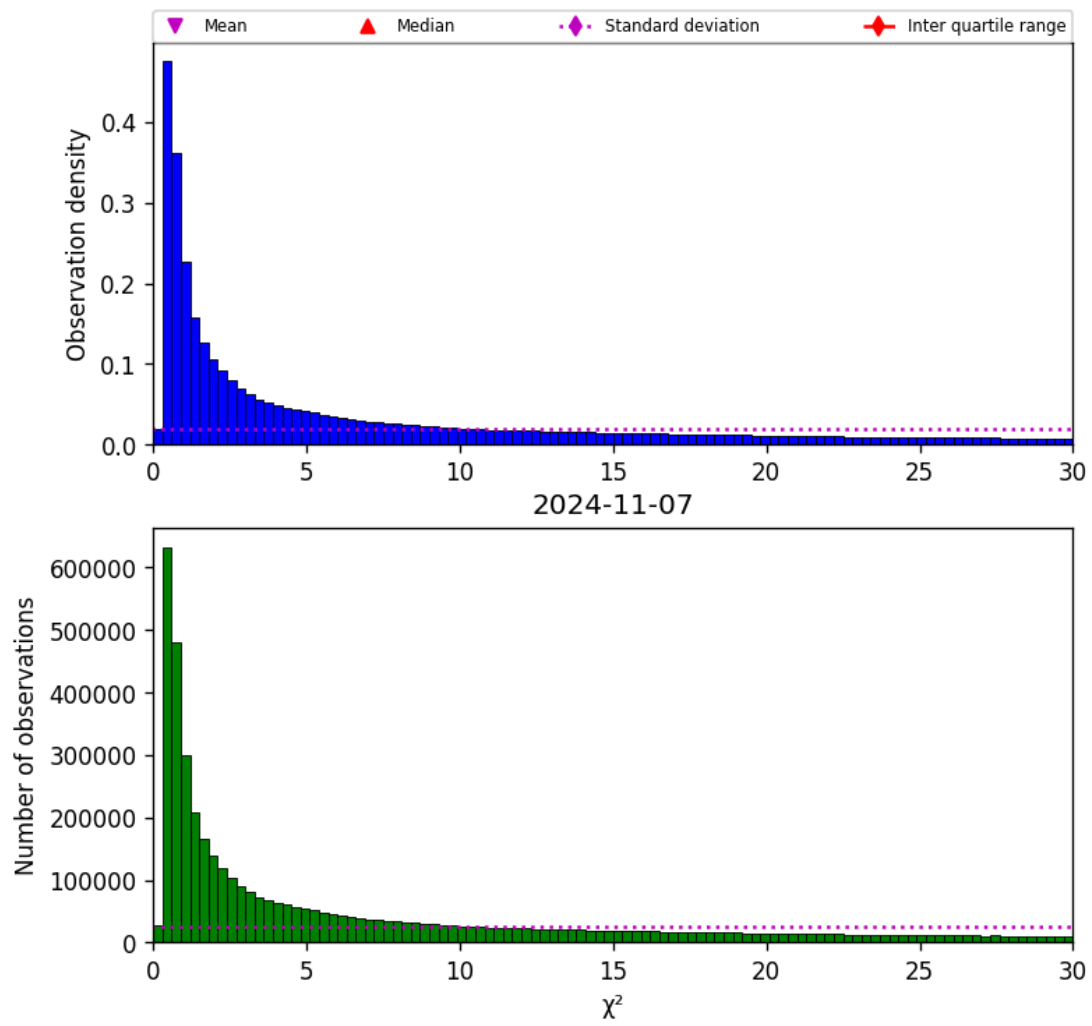
Figure 38: Histogram of " \chi^2 " for 2024-11-06 to 2024-11-08
