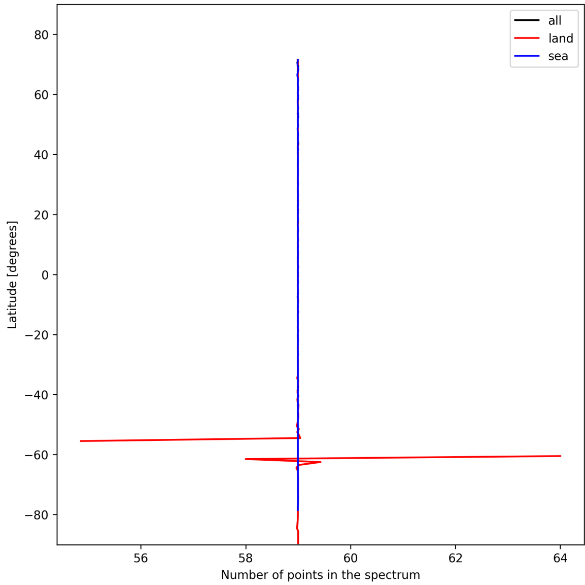
Figure 27: Zonal average of “Number of points in the spectrum” for 2024-11-06 to 2024-11-08.
