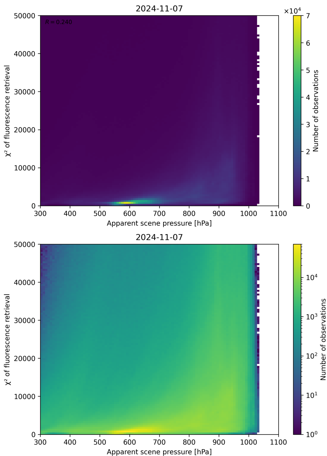
Figure 64: Scatter density plot of “Apparent scene pressure” against “ \chi^2 of fluorescence retrieval” for 2024-11-06 to 2024-11-08.
