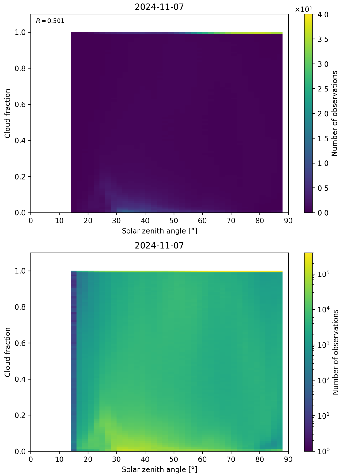
Figure 121: Scatter density plot of “Solar zenith angle” against “Cloud fraction” for 2024-11-06 to 2024-11-08.
