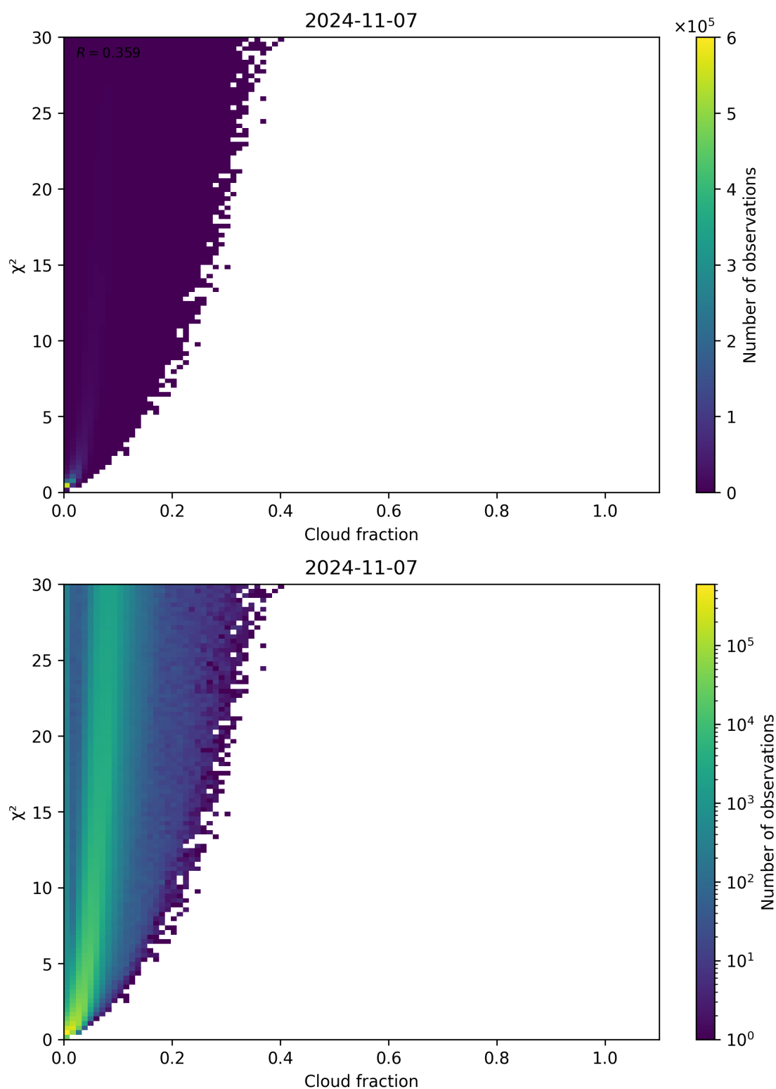
Figure 77: Scatter density plot of “Cloud fraction” against “ \chi^2 ” for 2024-11-06 to 2024-11-08.
