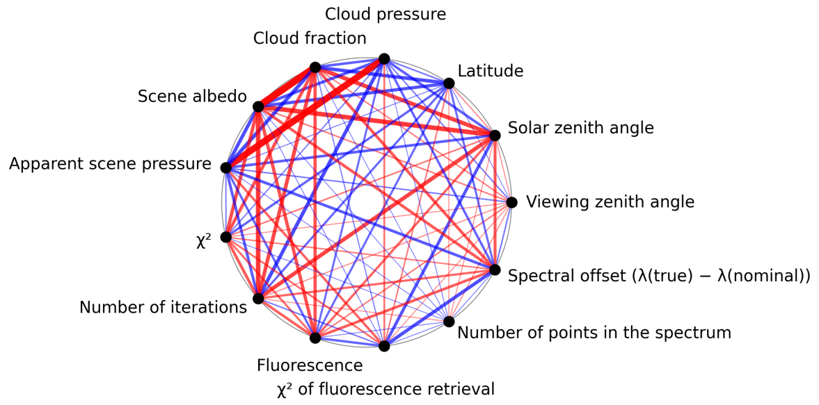
Figure 1: Map of correlation graph for 2024-11-06 to 2024-11-08.
