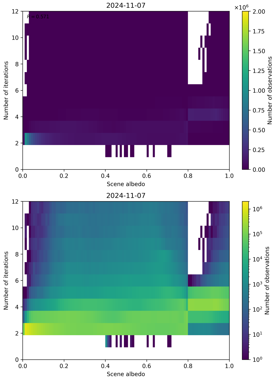
Figure 115: Scatter density plot of “Scene albedo” against “Number of iterations” for 2024-11-06 to 2024-11-08.
