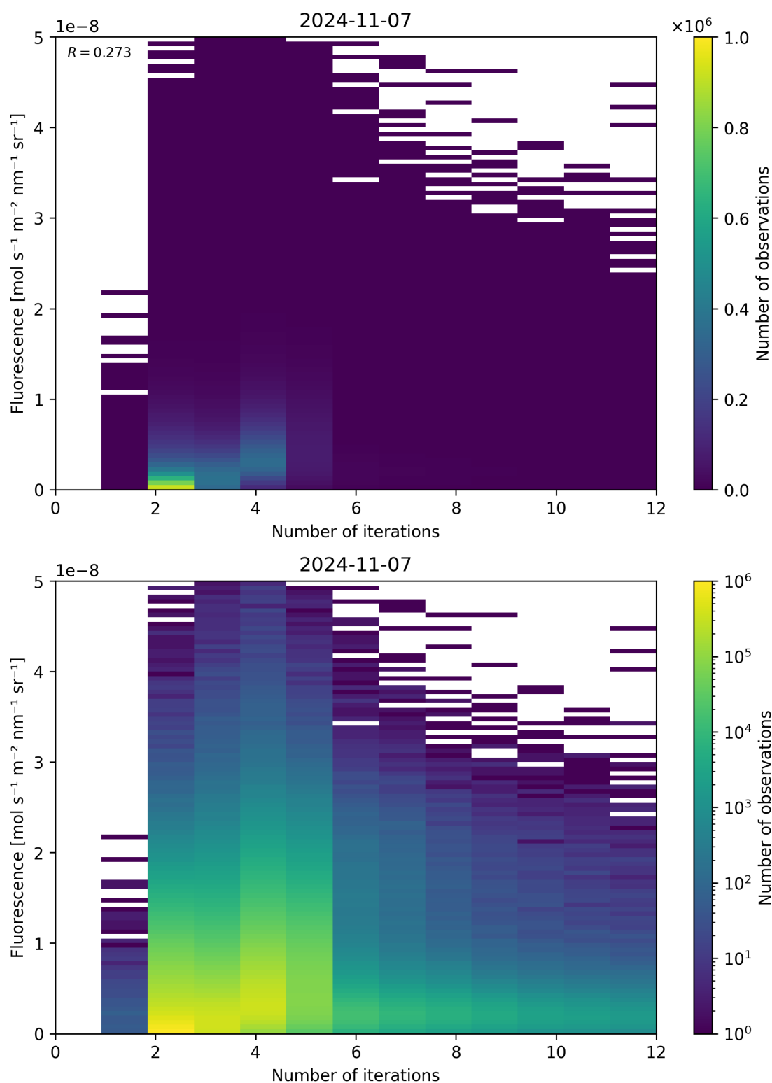
Figure 107: Scatter density plot of “Number of iterations” against “Fluorescence” for 2024-11-06 to 2024-11-08.
