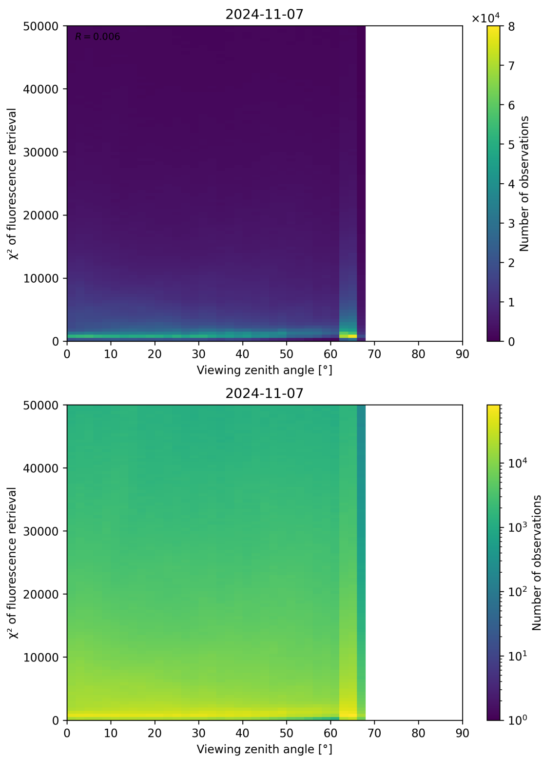
Figure 131: Scatter density plot of “Viewing zenith angle” against “ \chi^2 of fluorescence retrieval” for 2024-11-06 to 2024-11-08.
