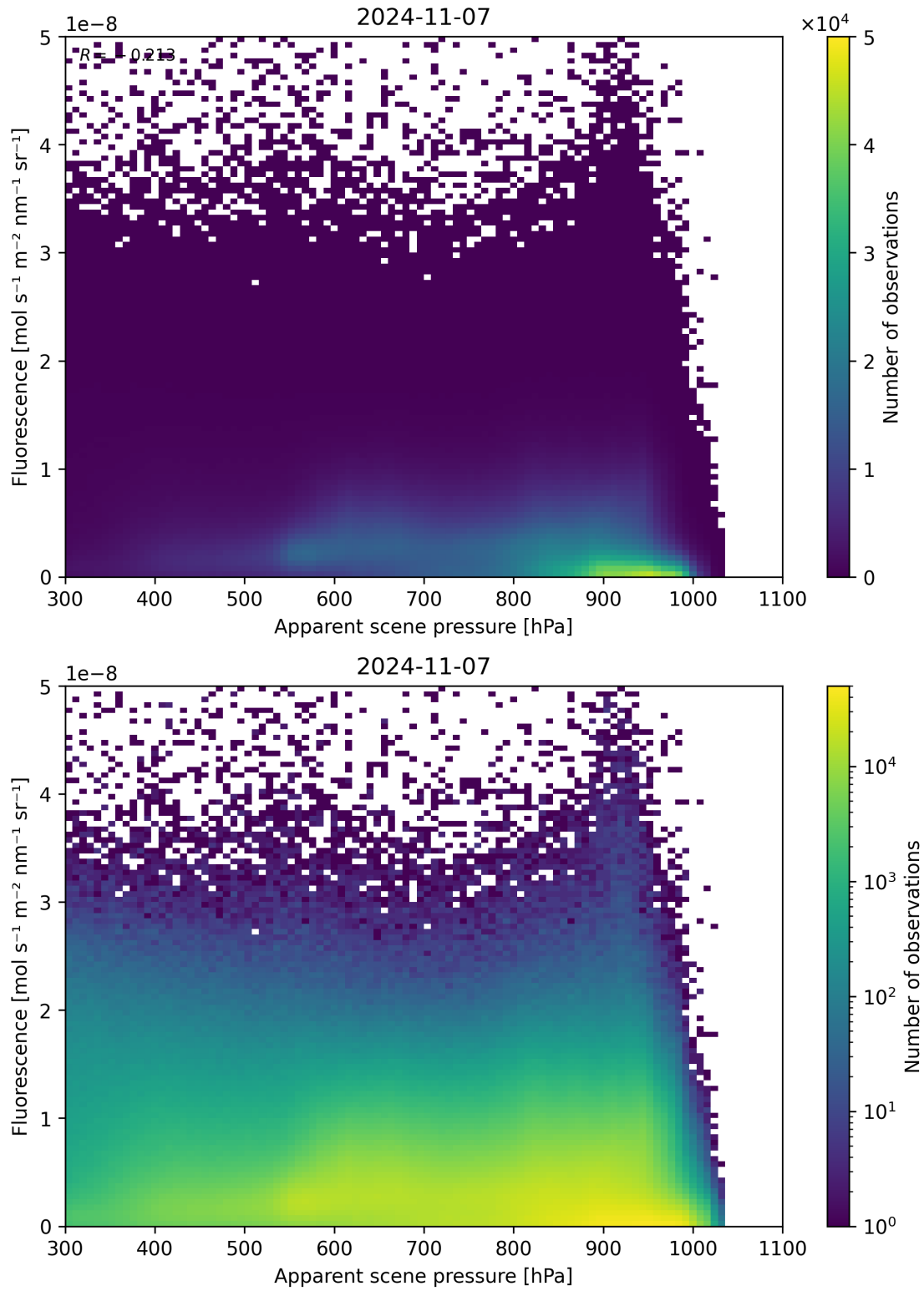
Figure 65: Scatter density plot of “Apparent scene pressure” against “Fluorescence” for 2024-11-06 to 2024-11-08.
