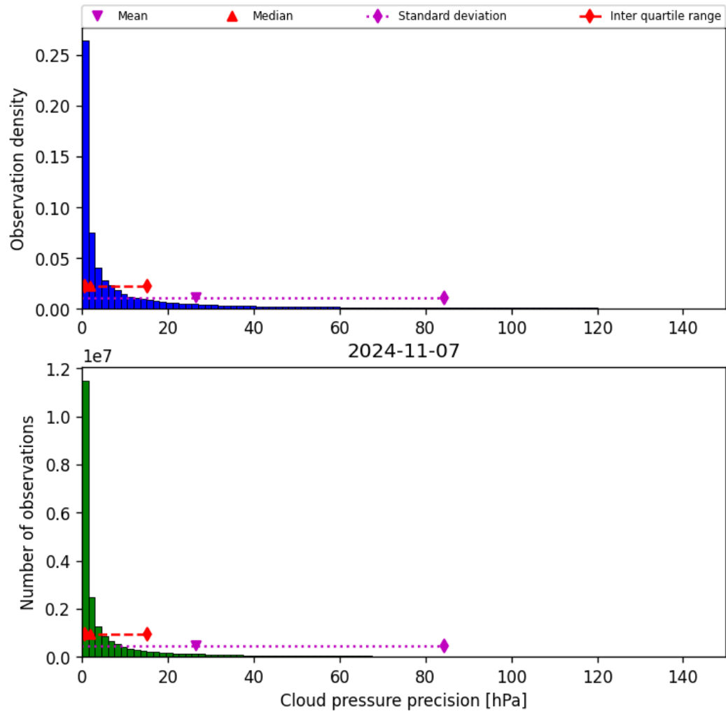
Figure 31: Histogram of “Cloud pressure precision” for 2024-11-06 to 2024-11-08
