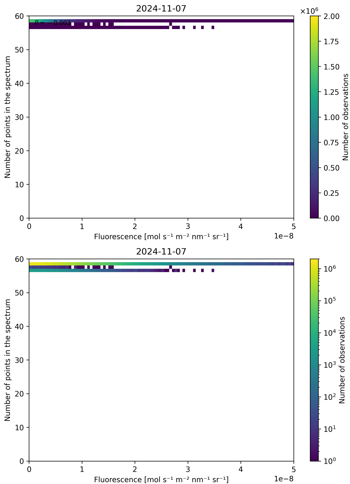
Figure 94: Scatter density plot of “Fluorescence” against “Number of points in the spectrum” for 2024-11-06 to 2024-11-08.
