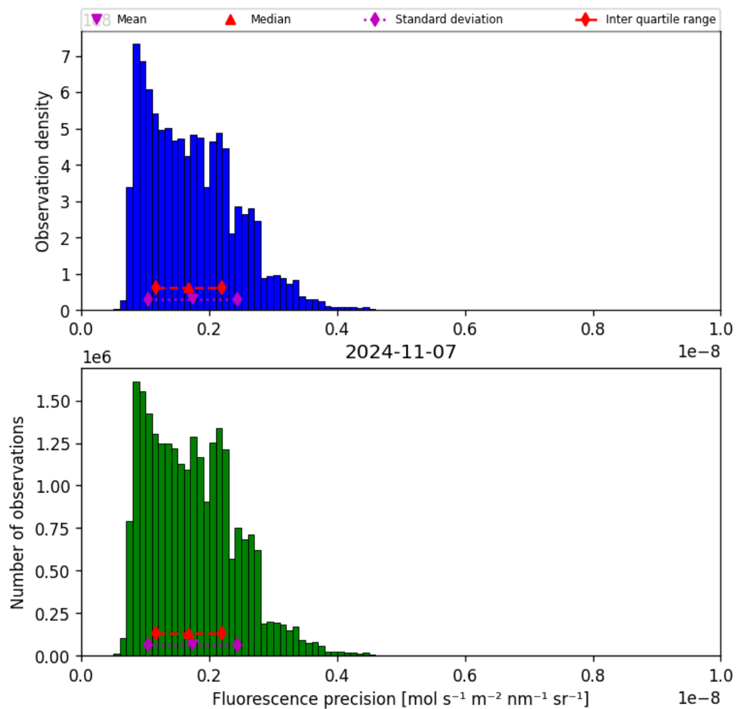
Figure 41: Histogram of “Fluorescence precision” for 2024-11-06 to 2024-11-08
