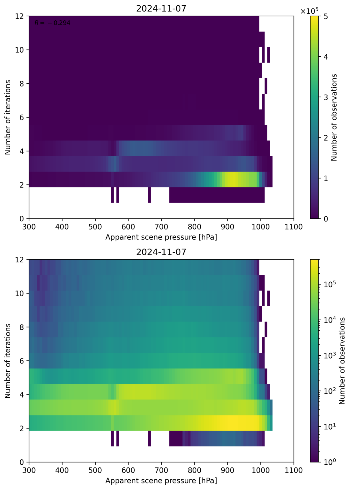
Figure 66: Scatter density plot of “Apparent scene pressure” against “Number of iterations” for 2024-11-06 to 2024-11-08.
