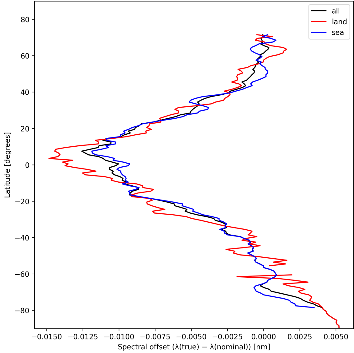
Figure 28: Zonal average of “Spectral offset ( \lambda_{\text{true}} - \lambda_{\text{nominal}} )” for 2024-11-06 to 2024-11-08.
