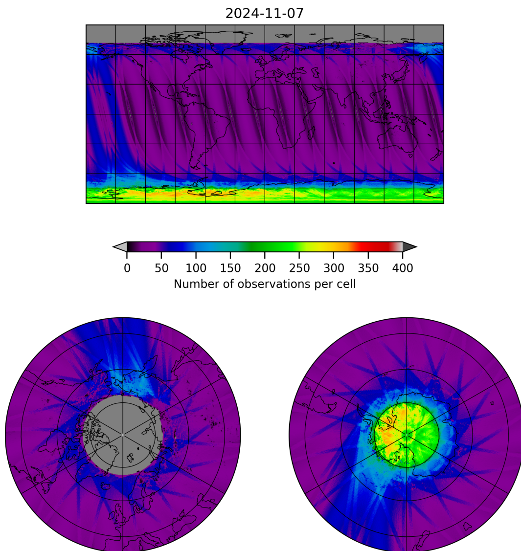
Figure 11: Map of the number of observations for 2024-11-06 to 2024-11-08
