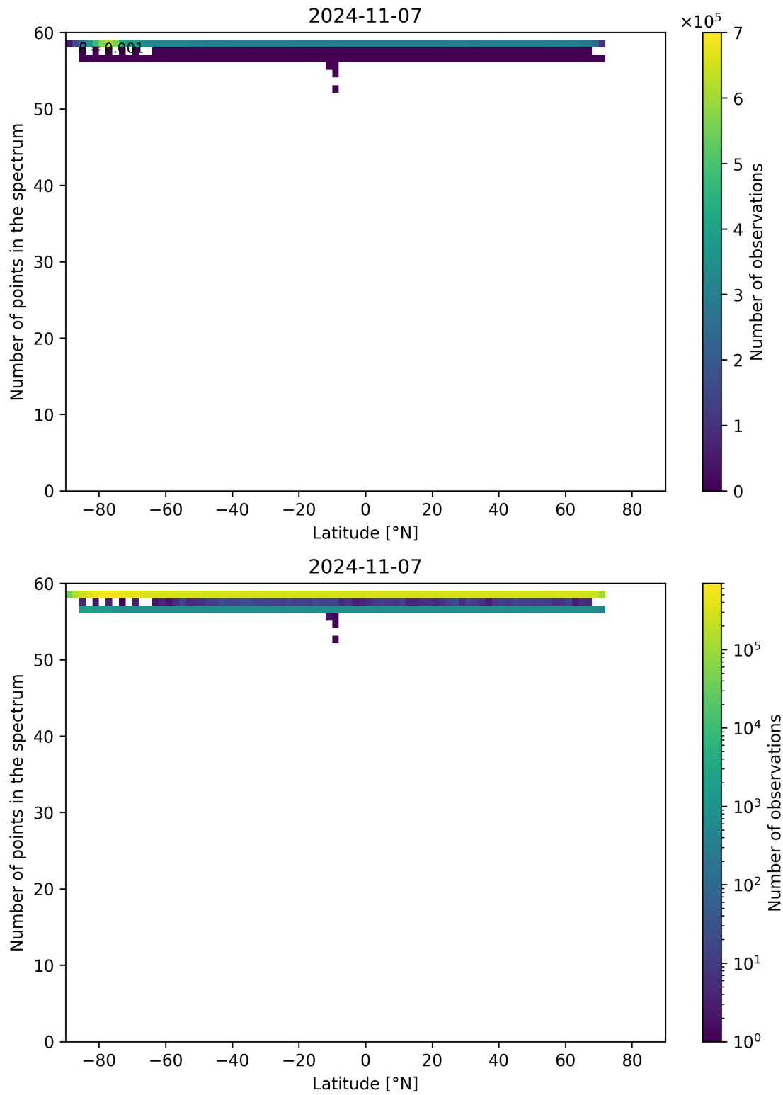
Figure 103: Scatter density plot of “Latitude” against “Number of points in the spectrum” for 2024-11-06 to 2024-11-08.
