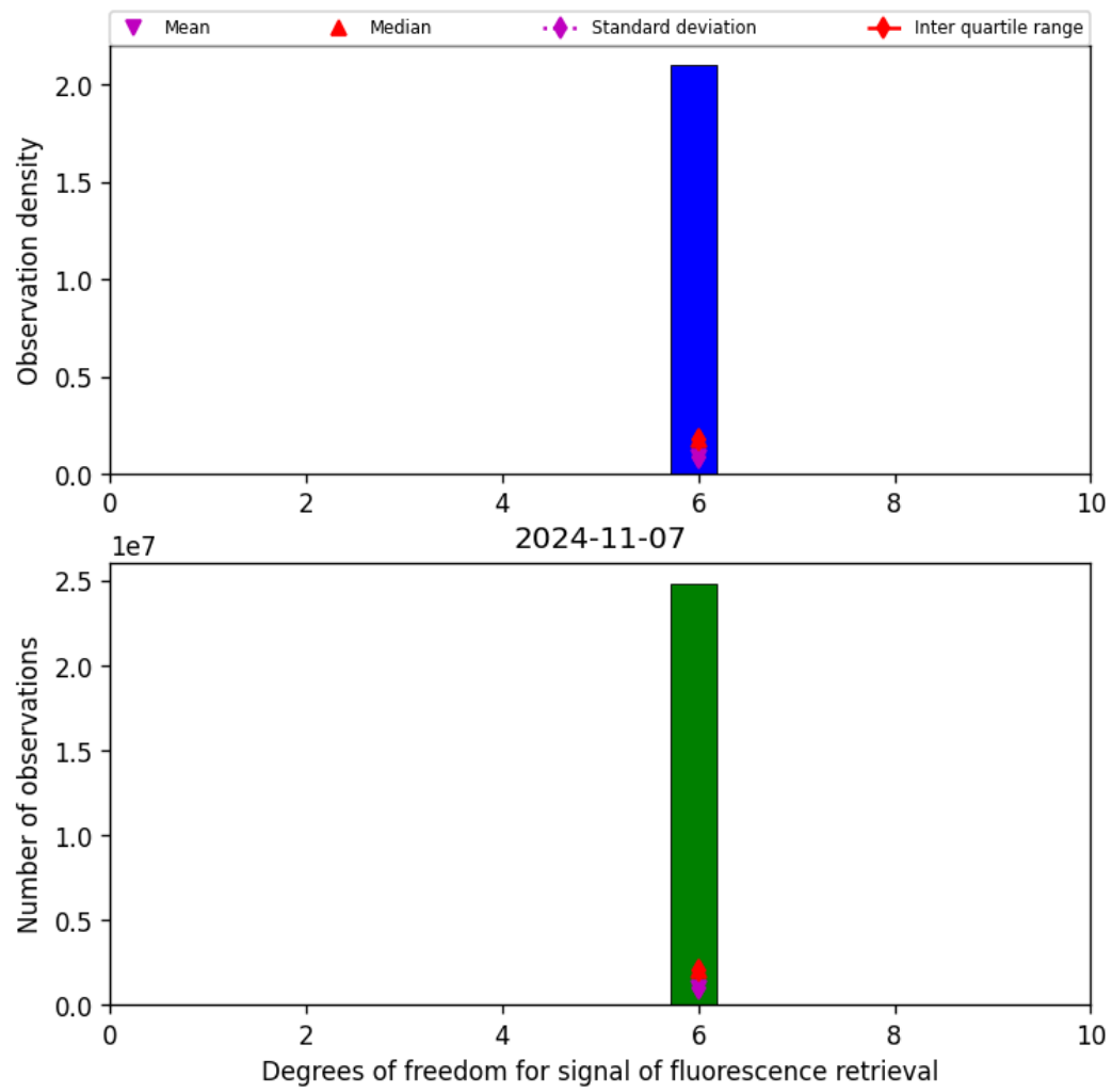
Figure 43: Histogram of “Degrees of freedom for signal of fluorescence retrieval” for 2024-11-06 to 2024-11-08
