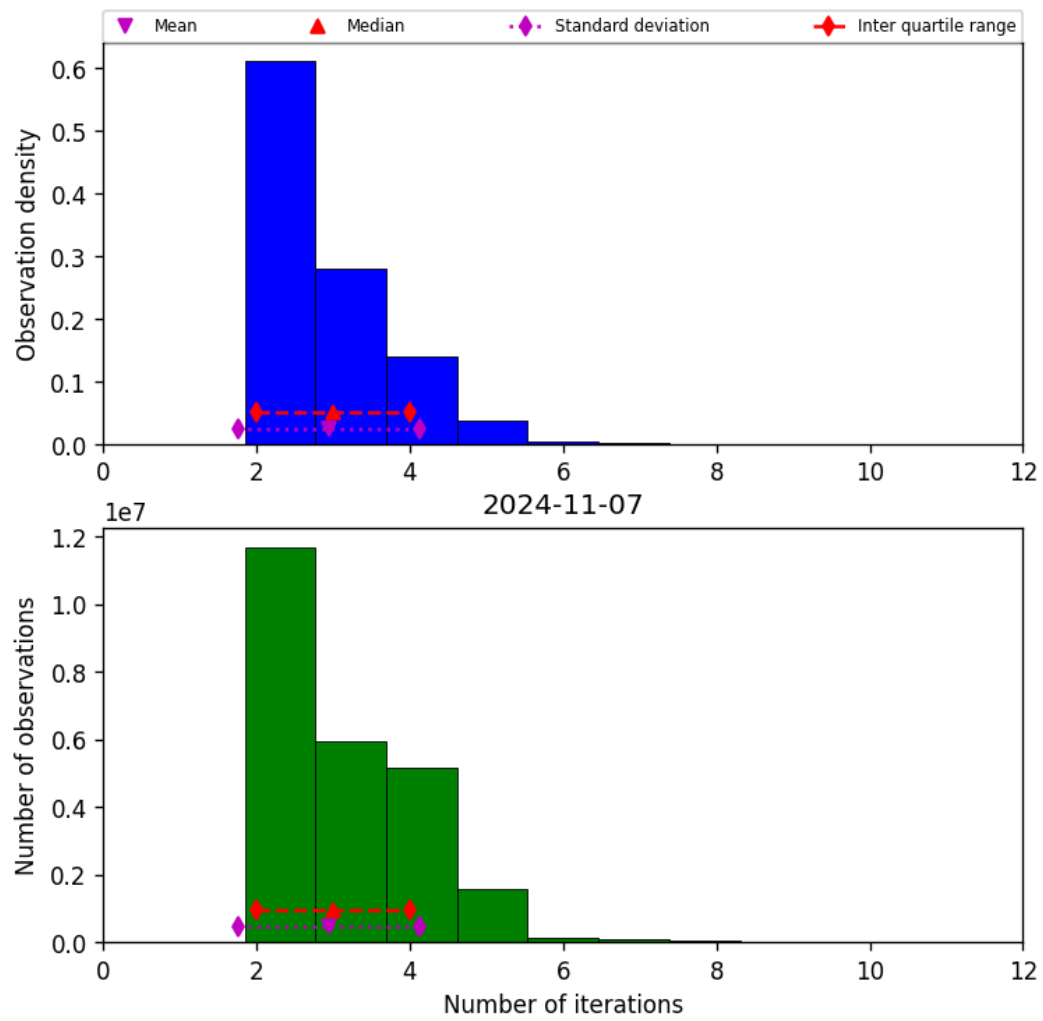
Figure 39: Histogram of “Number of iterations” for 2024-11-06 to 2024-11-08
