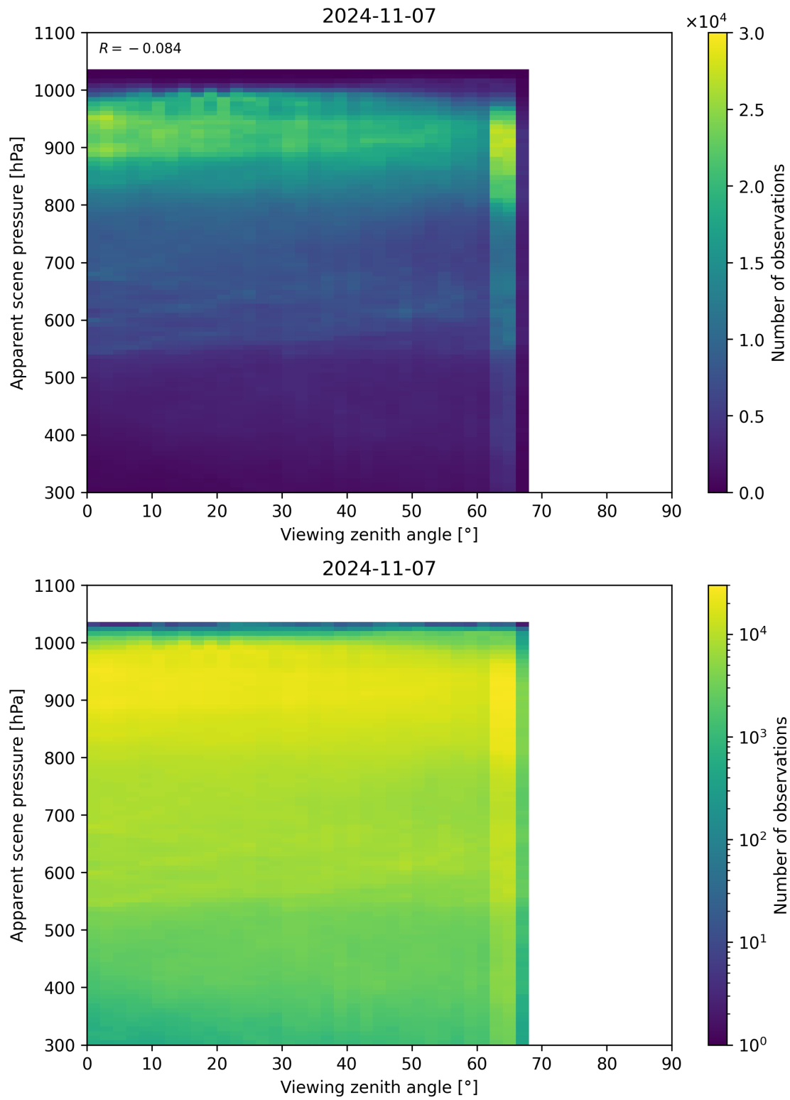
Figure 129: Scatter density plot of “Viewing zenith angle” against “Apparent scene pressure” for 2024-11-06 to 2024-11-08.
