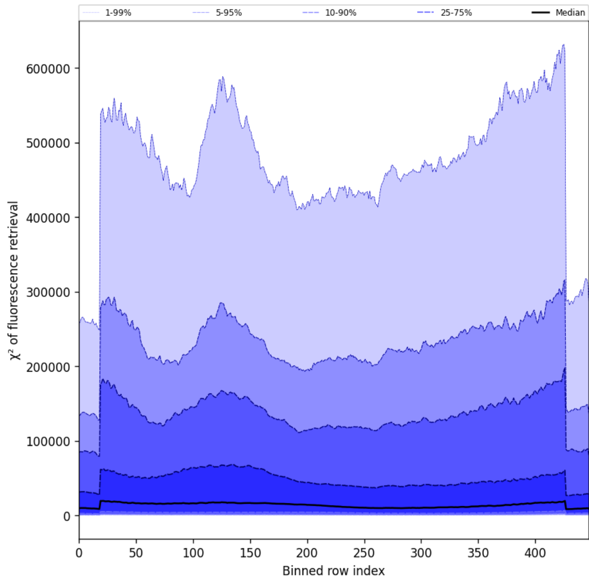
Figure 59: Along track statistics of " \chi^2 of fluorescence retrieval" for 2024-11-06 to 2024-11-08
