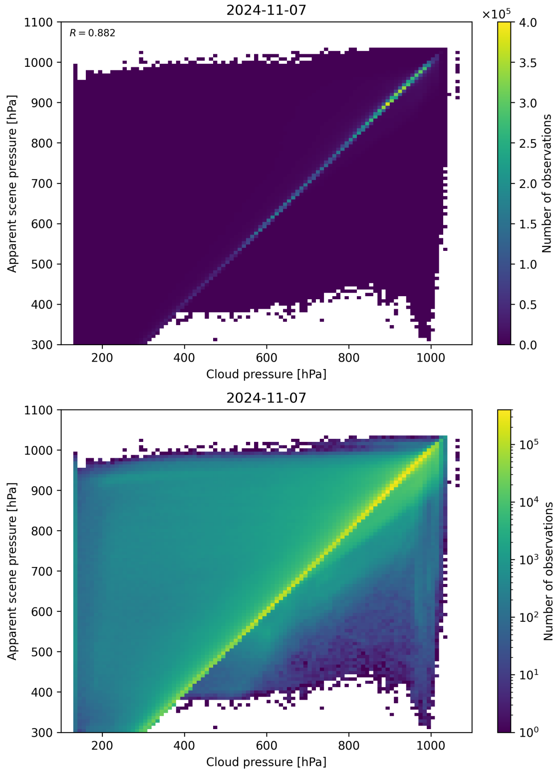
Figure 84: Scatter density plot of “Cloud pressure” against “Apparent scene pressure” for 2024-11-06 to 2024-11-08.
