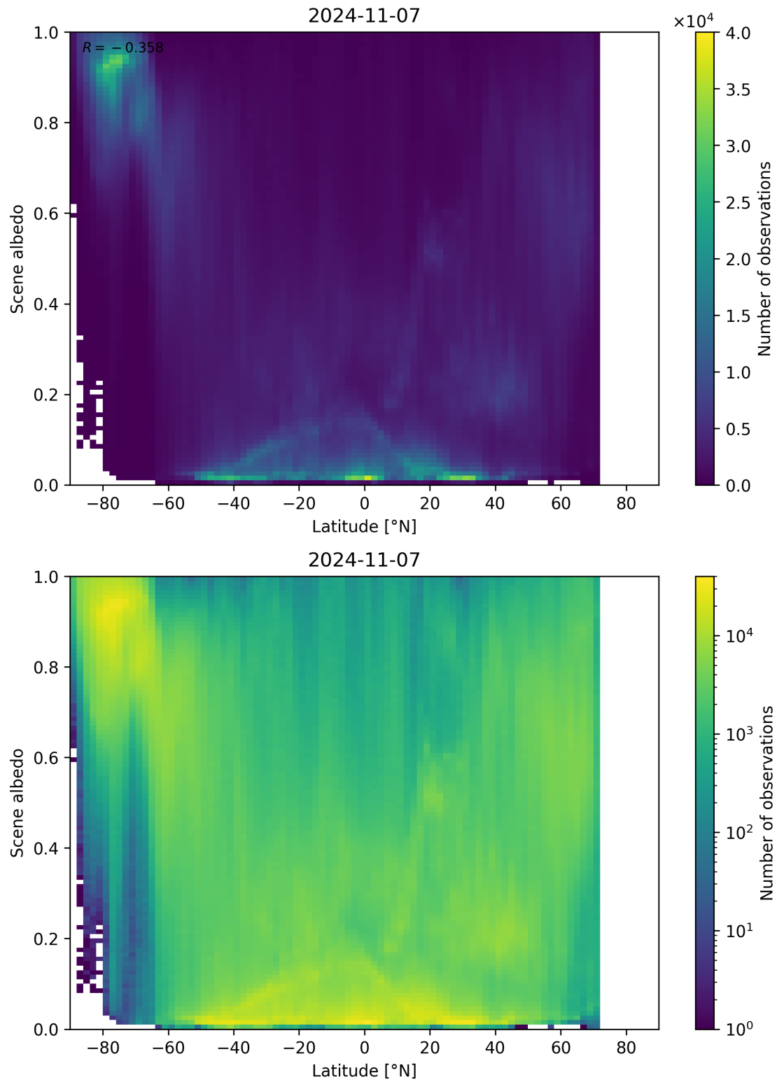
Figure 104: Scatter density plot of “Latitude” against “Scene albedo” for 2024-11-06 to 2024-11-08.
