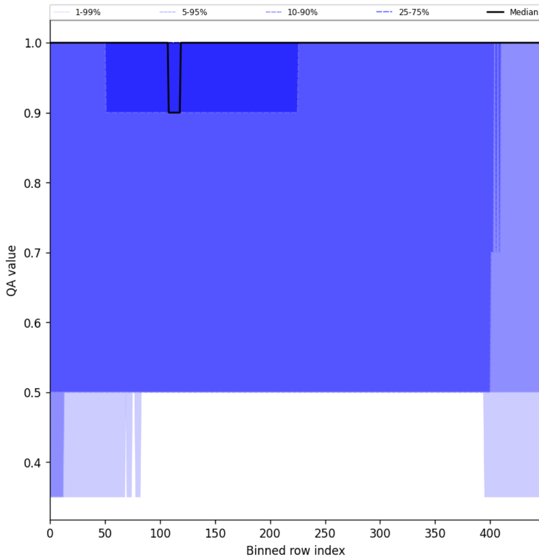
Figure 46: Along track statistics of “QA value” for 2024-11-06 to 2024-11-08
