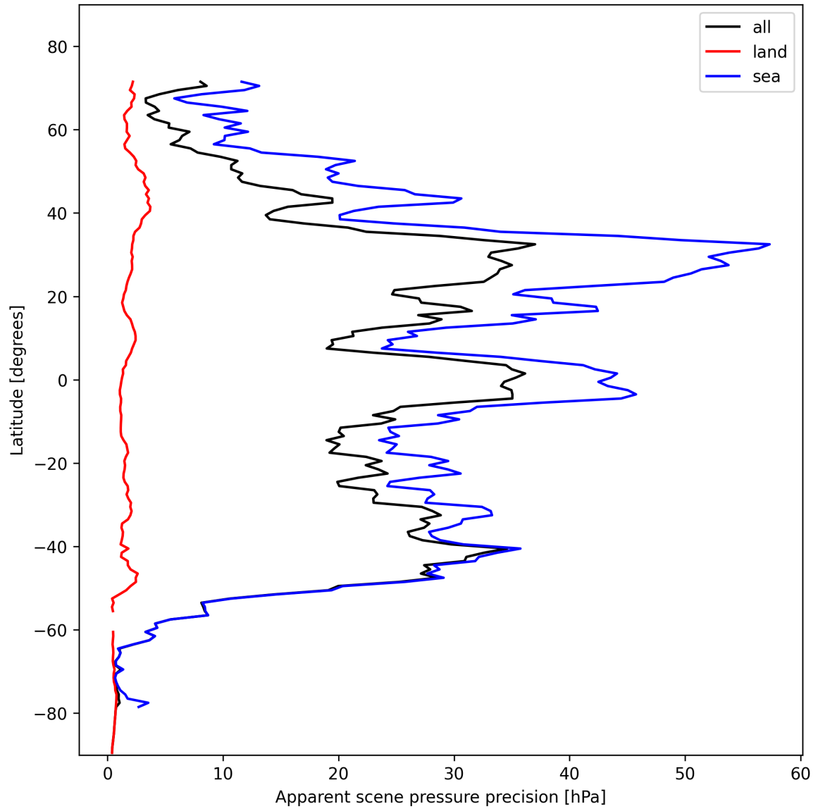
Figure 20: Zonal average of “Apparent scene pressure precision” for 2024-11-06 to 2024-11-08.
