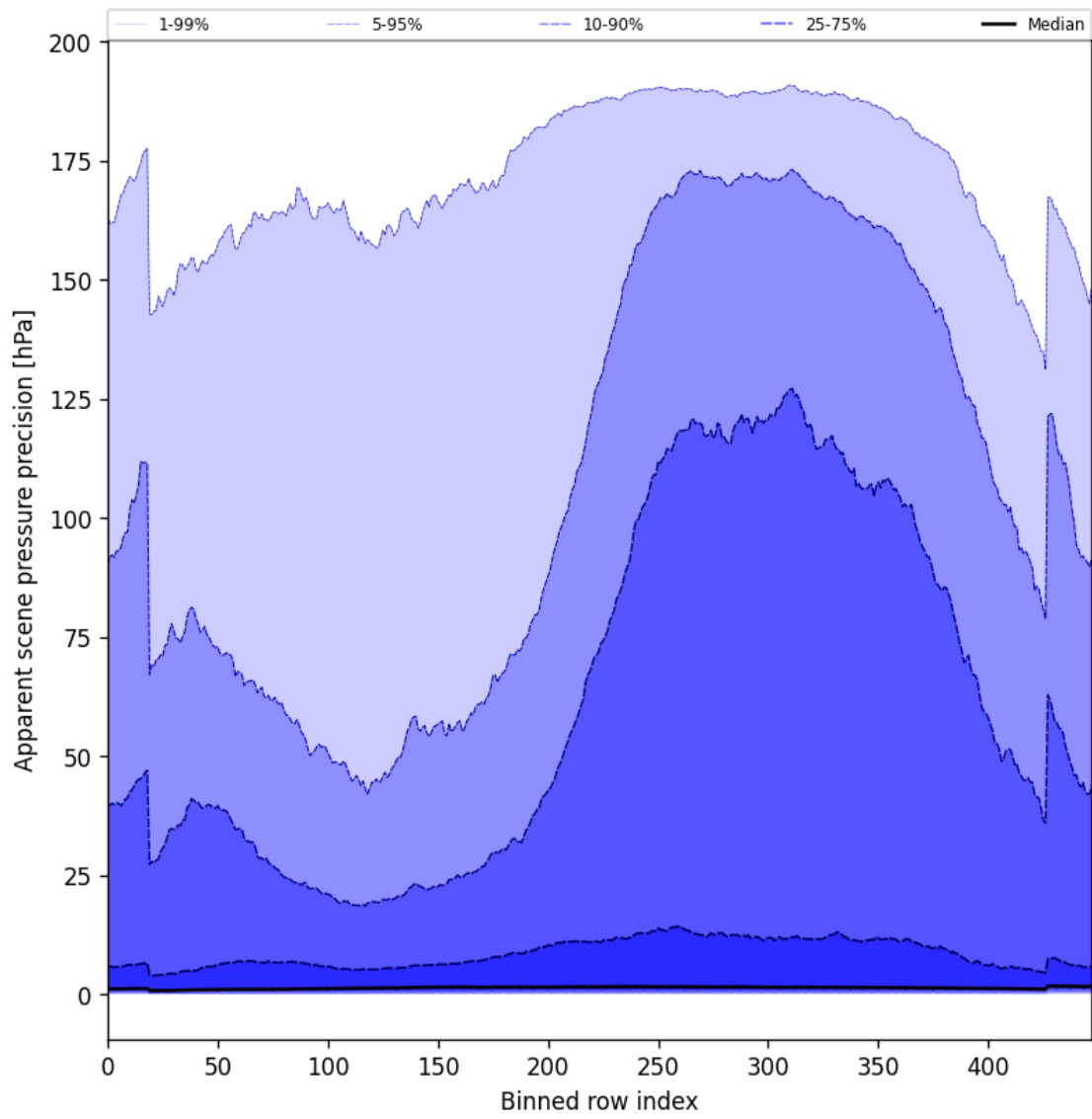
Figure 54: Along track statistics of “Apparent scene pressure precision” for 2024-11-06 to 2024-11-08
