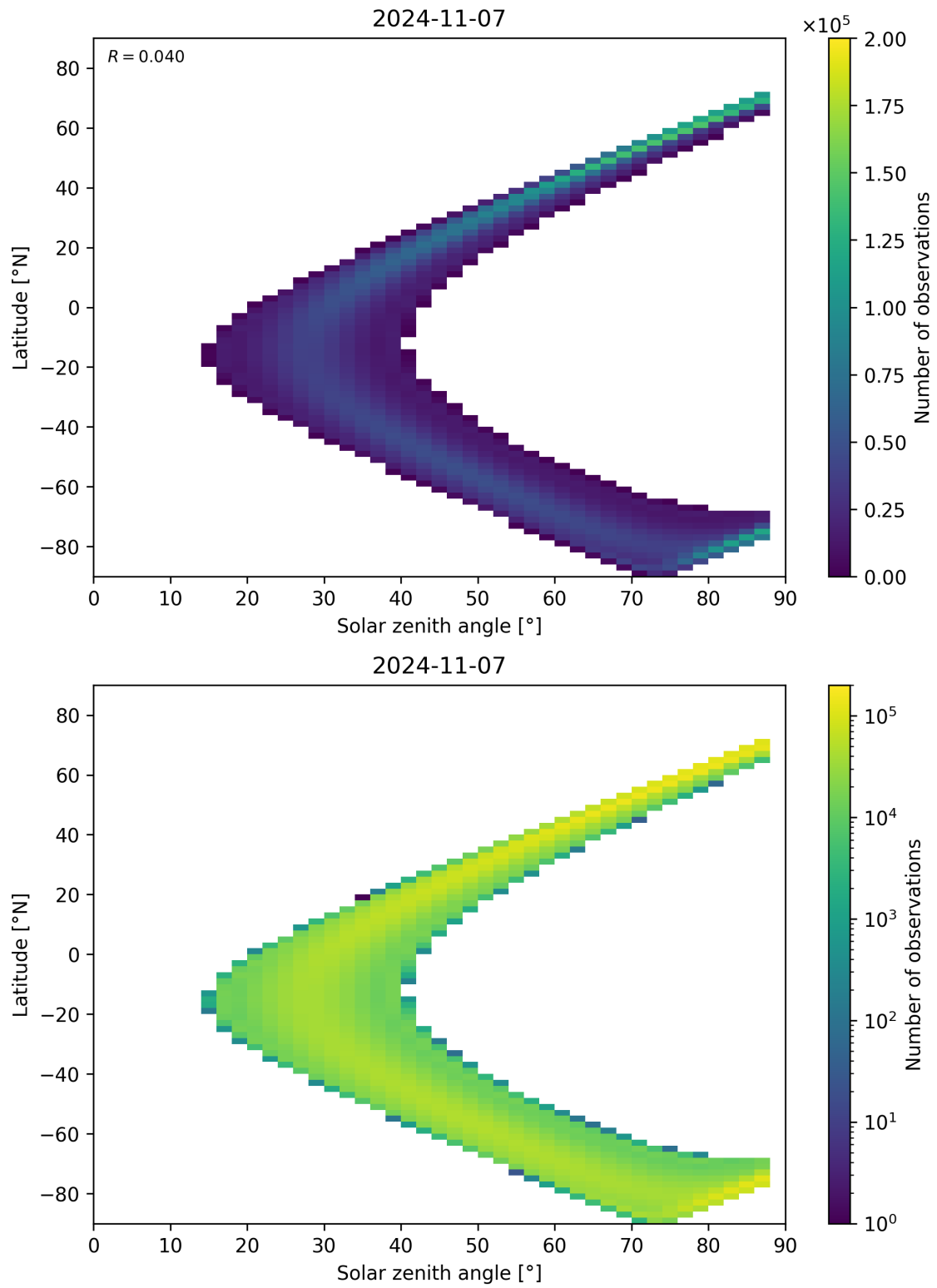
Figure 124: Scatter density plot of “Solar zenith angle” against “Latitude” for 2024-11-06 to 2024-11-08.
