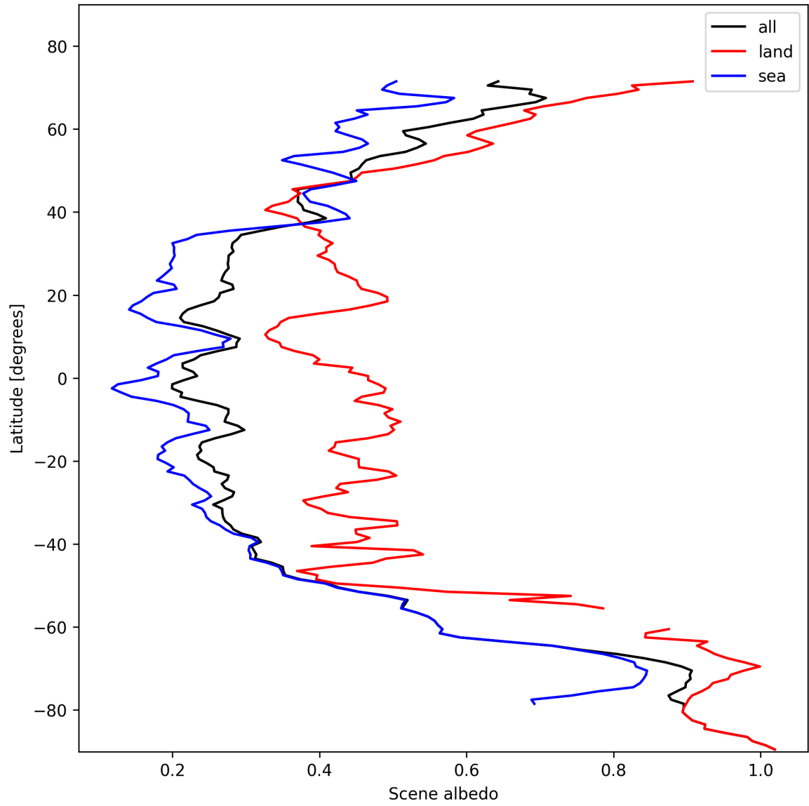
Figure 17: Zonal average of “Scene albedo” for 2024-11-06 to 2024-11-08.
