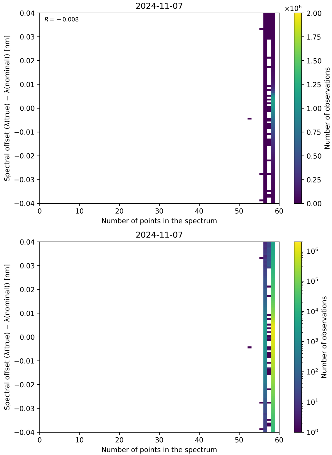
Figure 110: Scatter density plot of “Number of points in the spectrum” against “Spectral offset ( \lambda_{\text{true}} - \lambda_{\text{nominal}} )” for 2024-11-06 to 2024-11-08.
