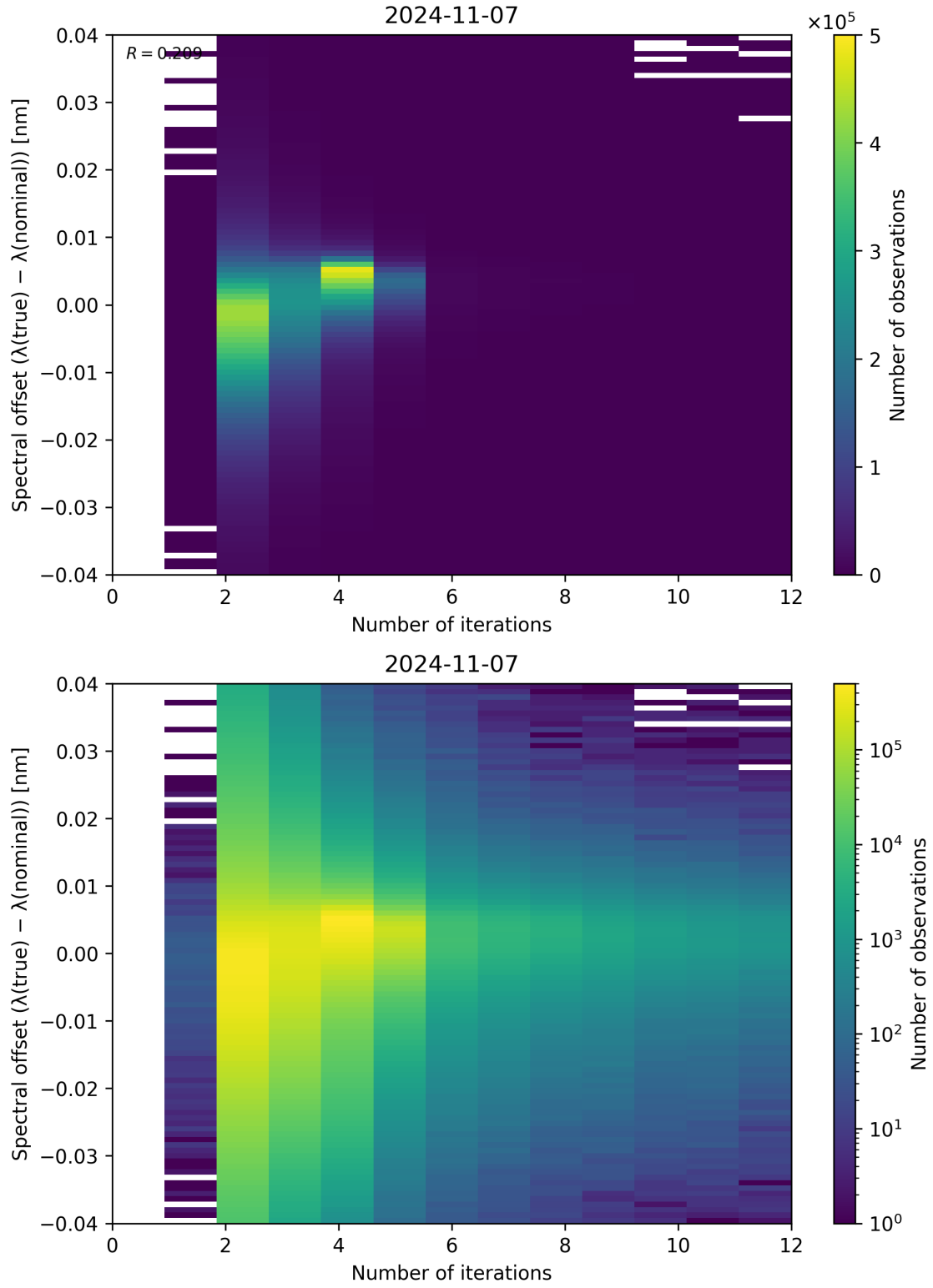
Figure 109: Scatter density plot of “Number of iterations” against “Spectral offset ( \lambda_{\text{true}} - \lambda_{\text{nominal}} )” for 2024-11-06 to 2024-11-08.
