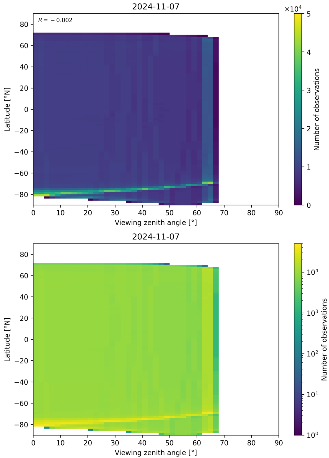
Figure 135: Scatter density plot of “Viewing zenith angle” against “Latitude” for 2024-11-06 to 2024-11-08.
