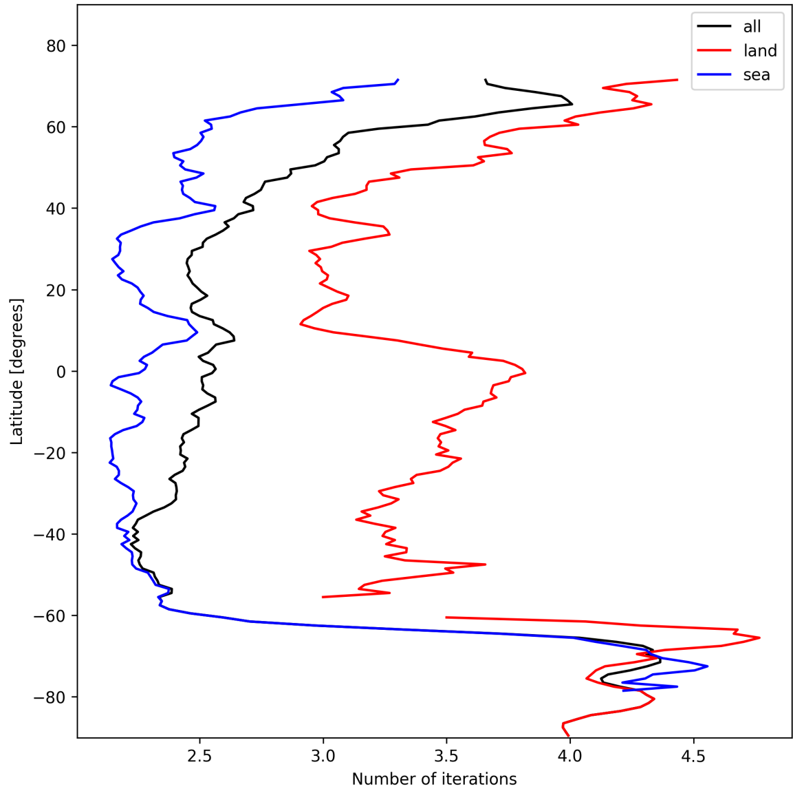
Figure 22: Zonal average of “Number of iterations” for 2024-11-06 to 2024-11-08.
