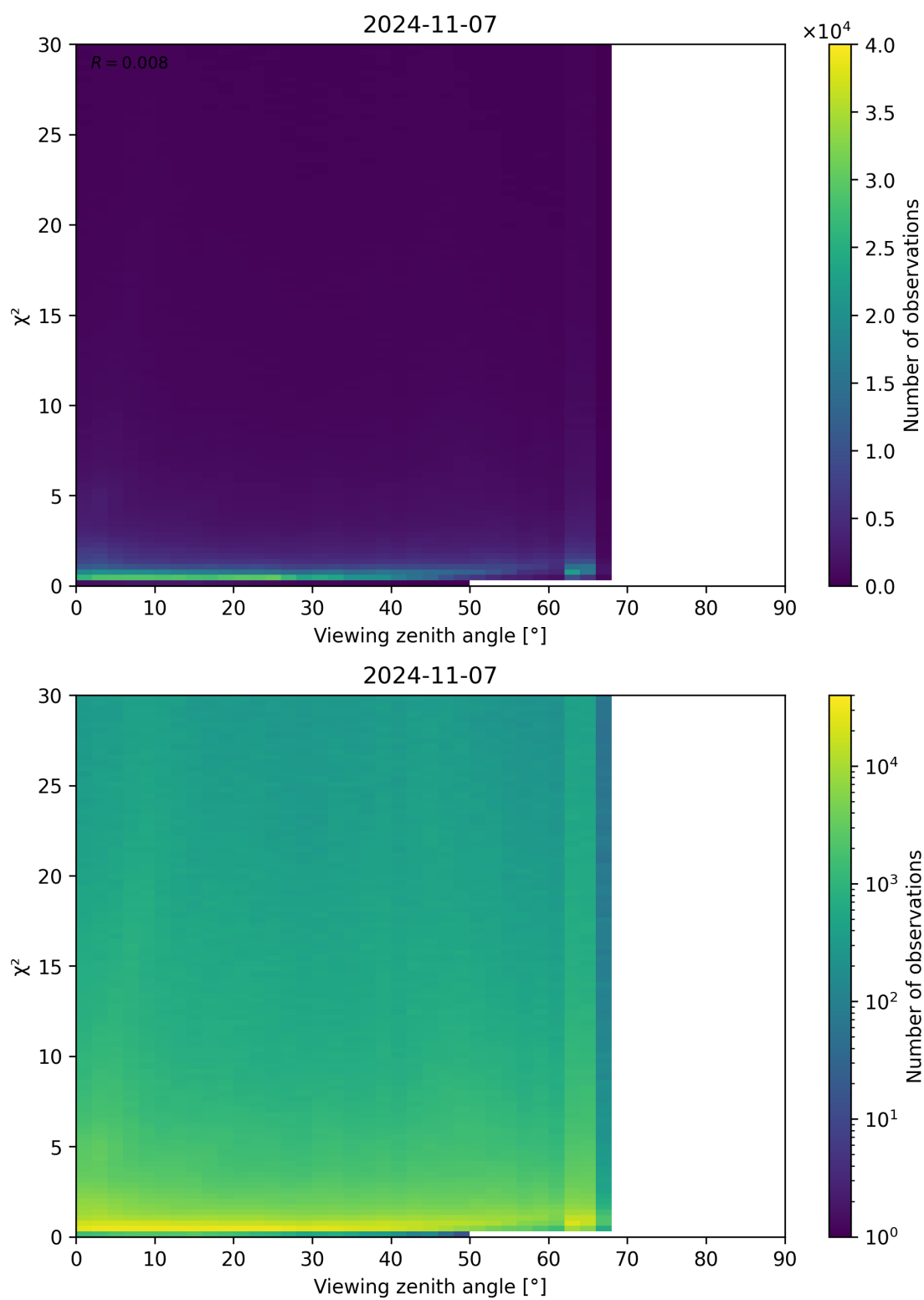
Figure 130: Scatter density plot of “Viewing zenith angle” against “ \chi^2 ” for 2024-11-06 to 2024-11-08.
