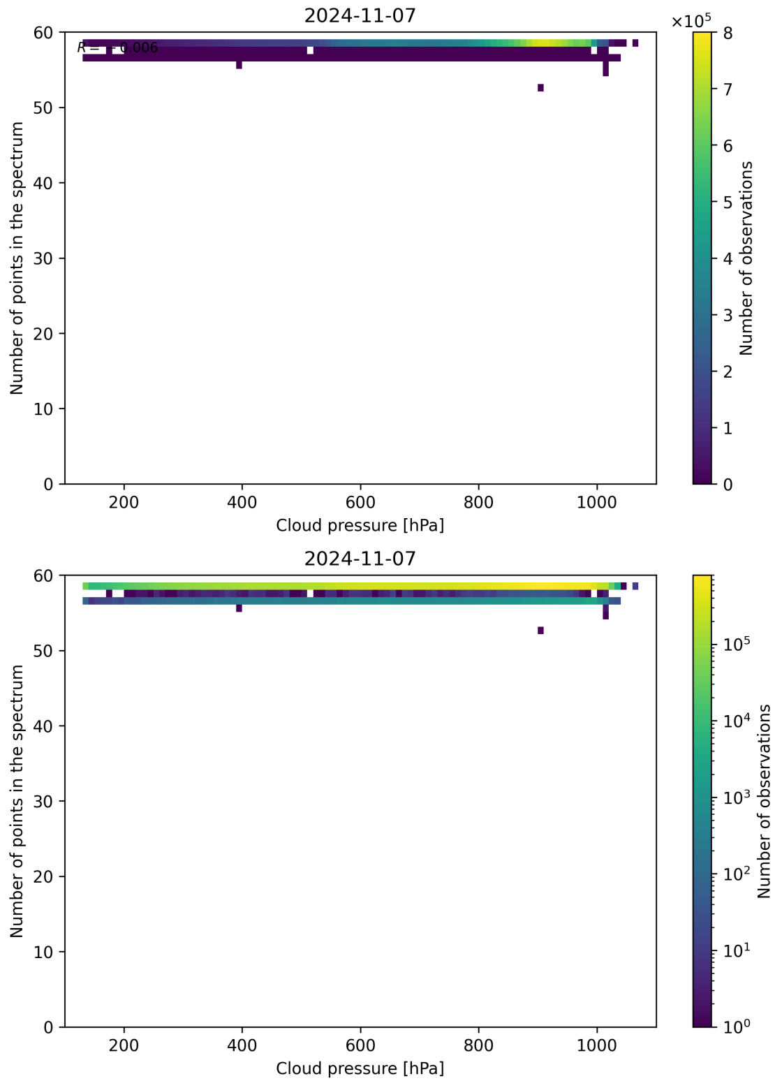
Figure 90: Scatter density plot of “Cloud pressure” against “Number of points in the spectrum” for 2024-11-06 to 2024-11-08.
