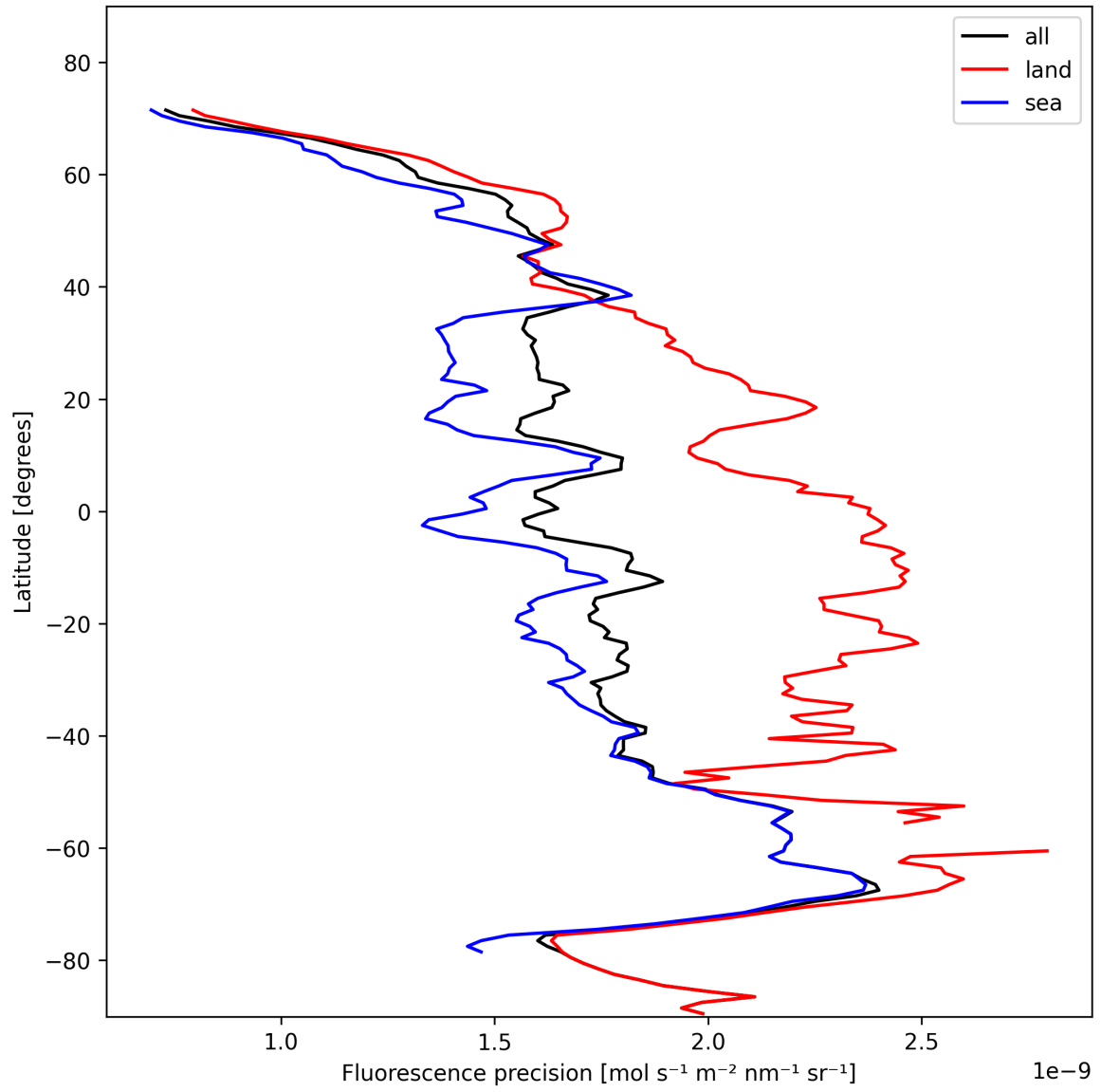
Figure 24: Zonal average of “Fluorescence precision” for 2024-11-06 to 2024-11-08.
