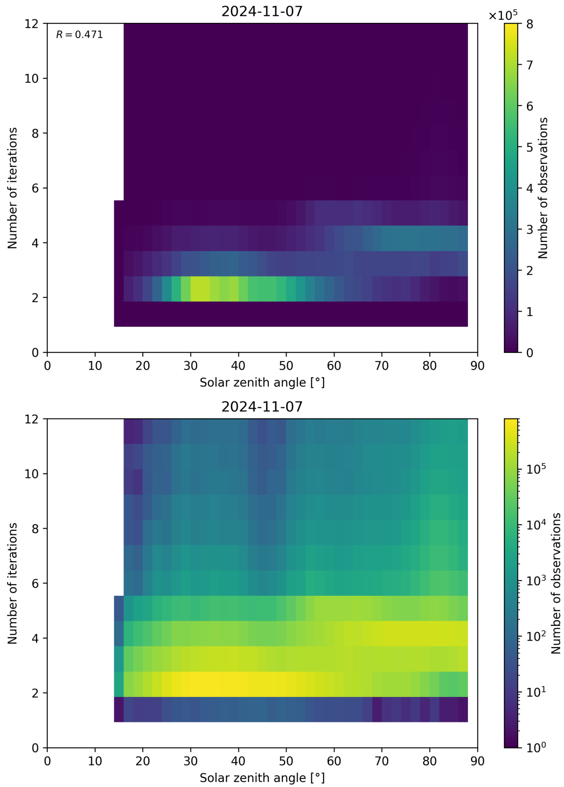
Figure 125: Scatter density plot of “Solar zenith angle” against “Number of iterations” for 2024-11-06 to 2024-11-08.
