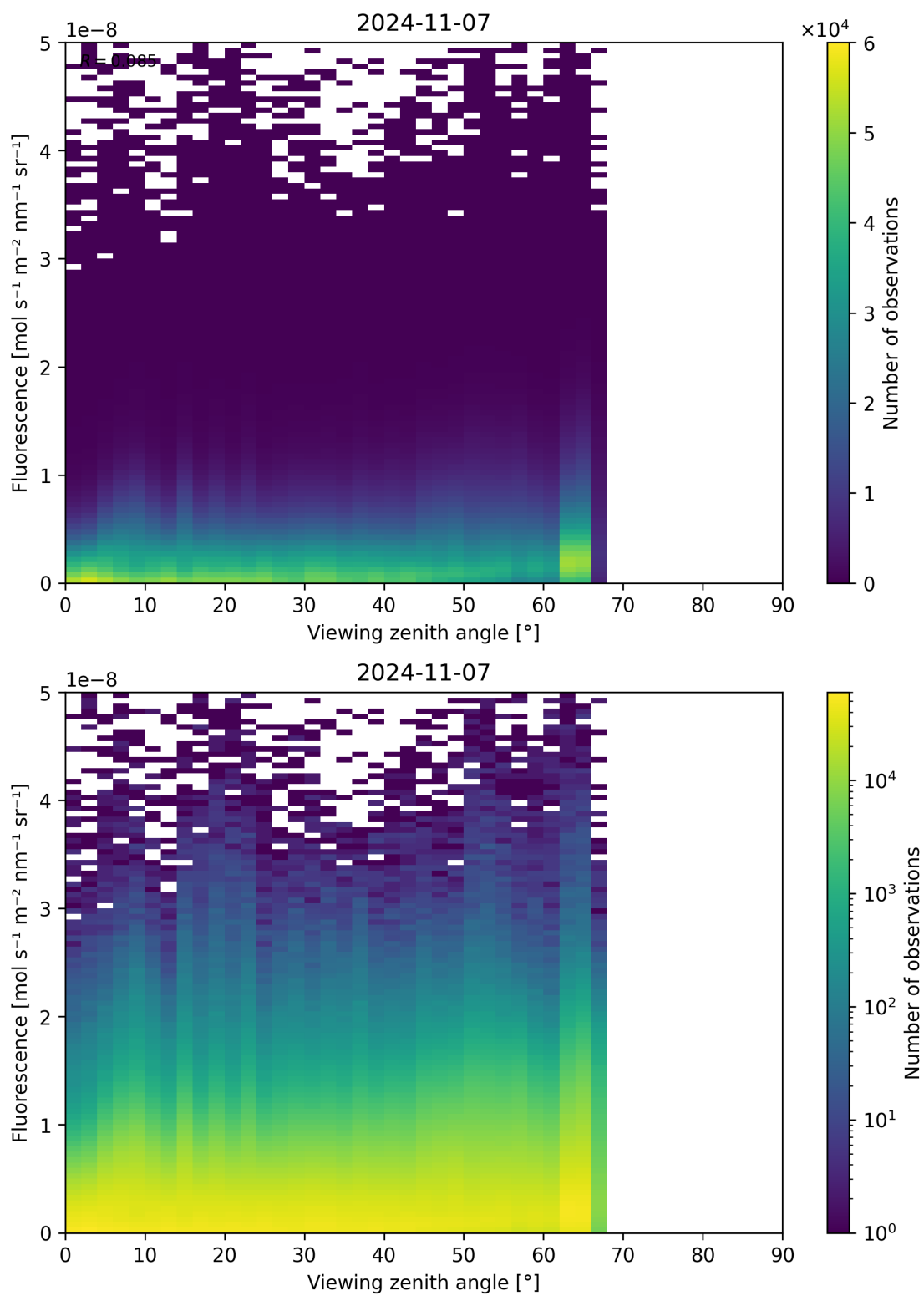
Figure 134: Scatter density plot of “Viewing zenith angle” against “Fluorescence” for 2024-11-06 to 2024-11-08.
