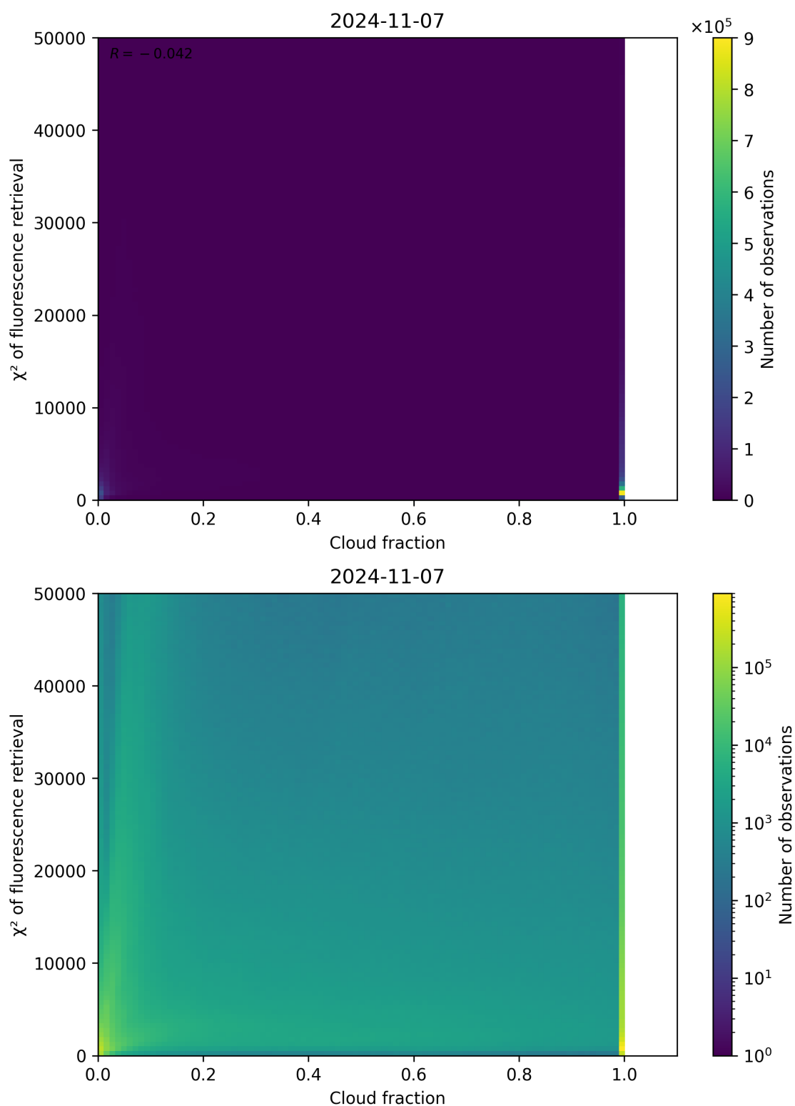
Figure 78: Scatter density plot of “Cloud fraction” against “ \chi^2 of fluorescence retrieval” for 2024-11-06 to 2024-11-08.
