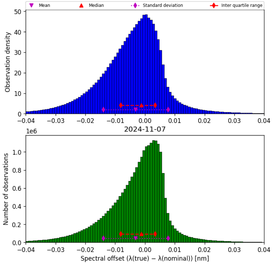
Figure 45: Histogram of “Spectral offset ( \lambda_{\text{true}} - \lambda_{\text{nominal}} )” for 2024-11-06 to 2024-11-08
