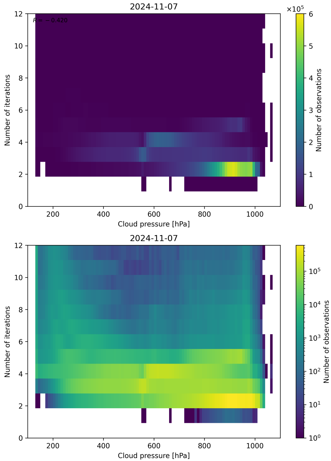
Figure 89: Scatter density plot of “Cloud pressure” against “Number of iterations” for 2024-11-06 to 2024-11-08.
