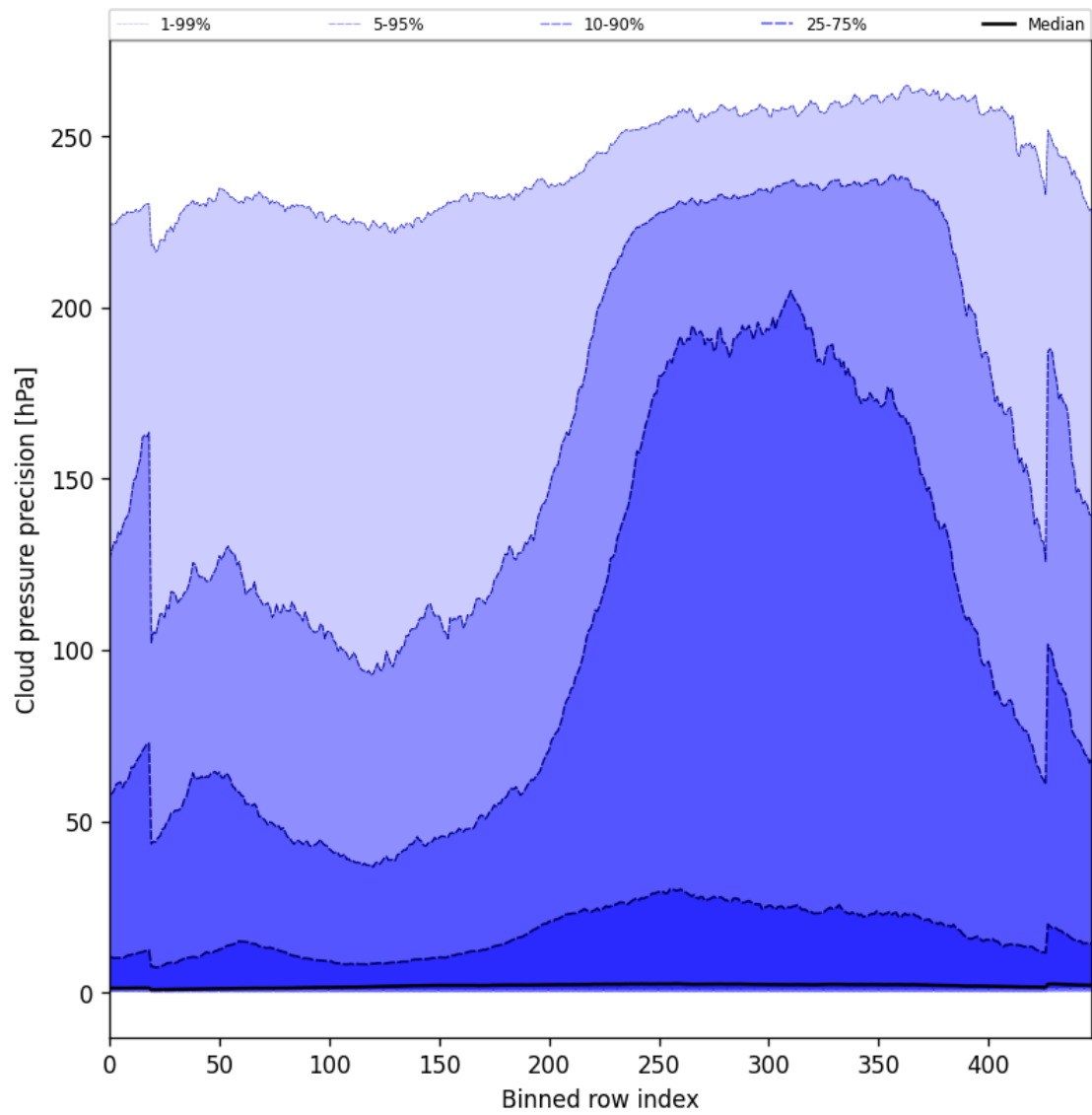
Figure 48: Along track statistics of “Cloud pressure precision” for 2024-11-06 to 2024-11-08
