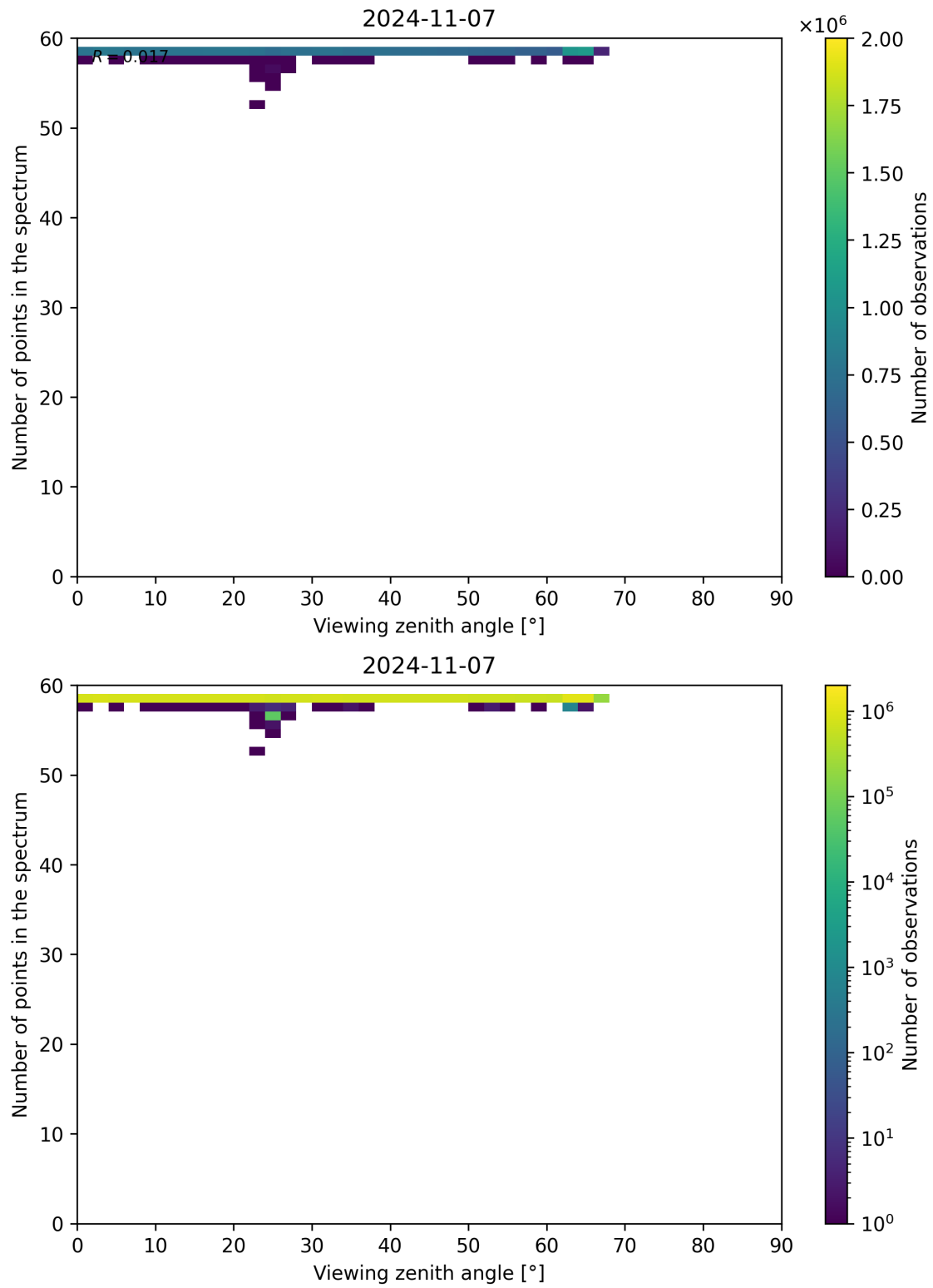
Figure 137: Scatter density plot of “Viewing zenith angle” against “Number of points in the spectrum” for 2024-11-06 to 2024-11-08.
