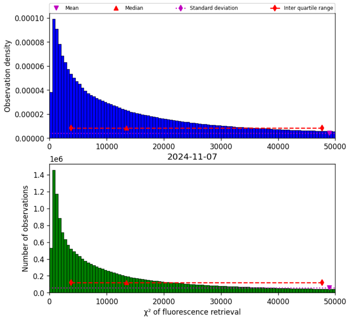
Figure 42: Histogram of “ \chi^2 of fluorescence retrieval” for 2024-11-06 to 2024-11-08
