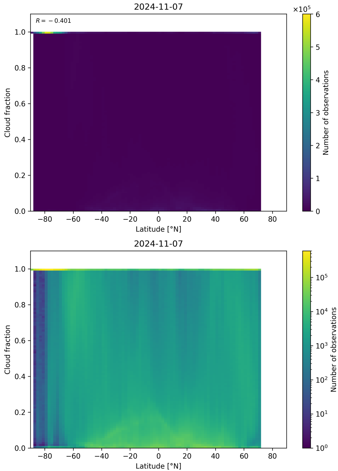
Figure 99: Scatter density plot of “Latitude” against “Cloud fraction” for 2024-11-06 to 2024-11-08.
