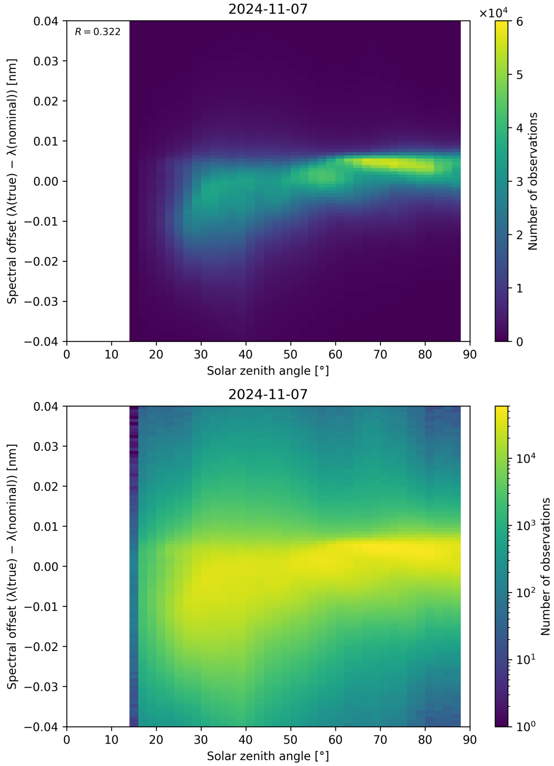
Figure 128: Scatter density plot of “Solar zenith angle” against “Spectral offset ( \lambda_{\text{true}} - \lambda_{\text{nominal}} )” for 2024-11-06 to 2024-11-08.
