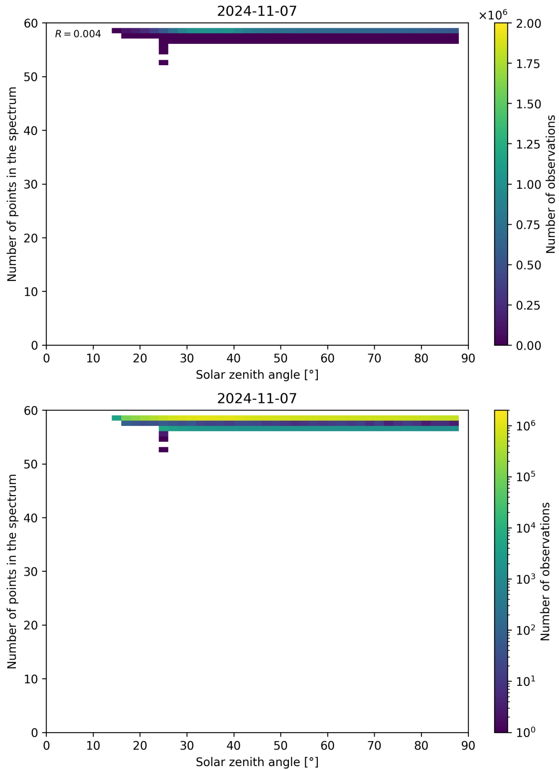
Figure 126: Scatter density plot of “Solar zenith angle” against “Number of points in the spectrum” for 2024-11-06 to 2024-11-08.
