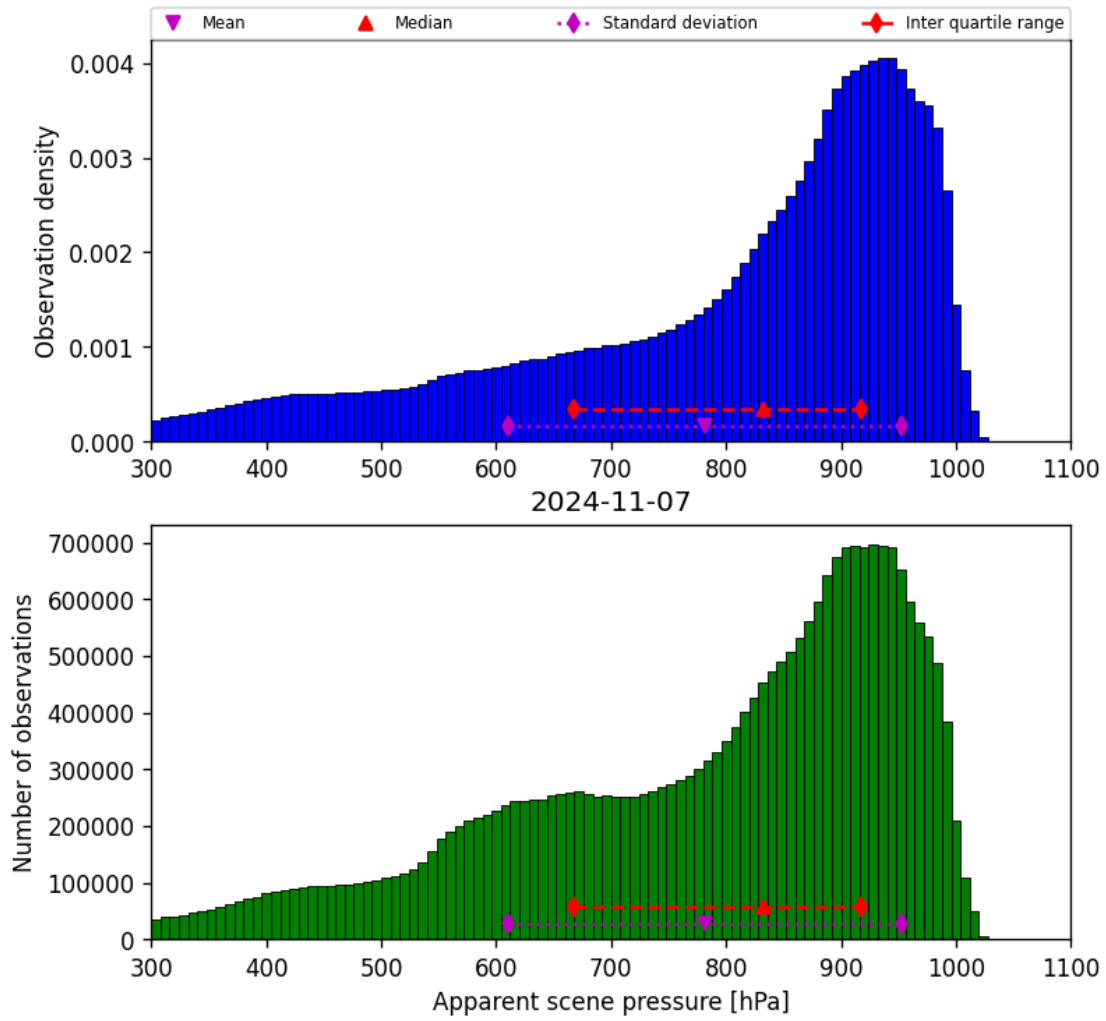
Figure 36: Histogram of “Apparent scene pressure” for 2024-11-06 to 2024-11-08
