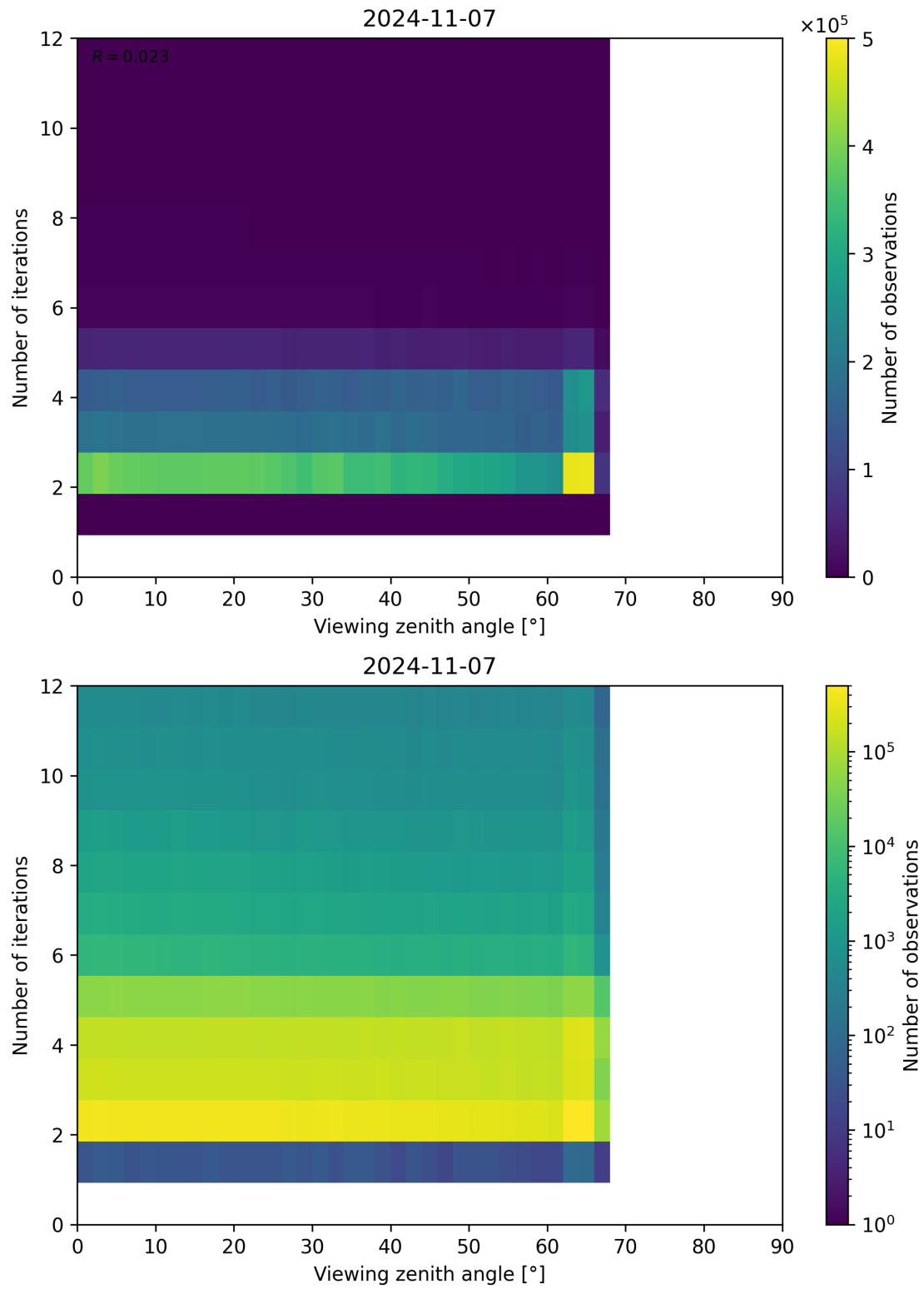
Figure 136: Scatter density plot of “Viewing zenith angle” against “Number of iterations” for 2024-11-06 to 2024-11-08.
