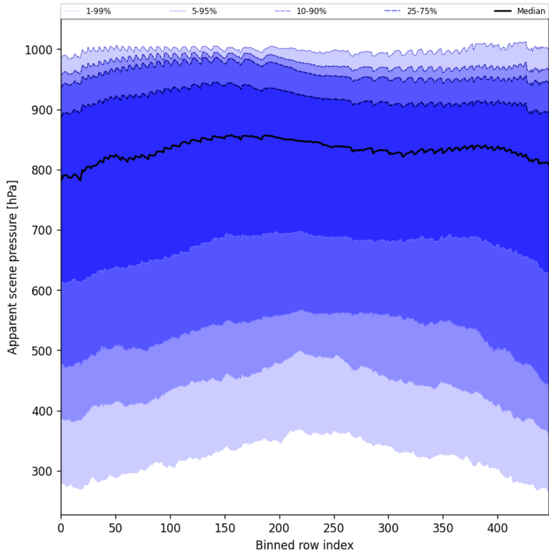
Figure 53: Along track statistics of “Apparent scene pressure” for 2024-11-06 to 2024-11-08
