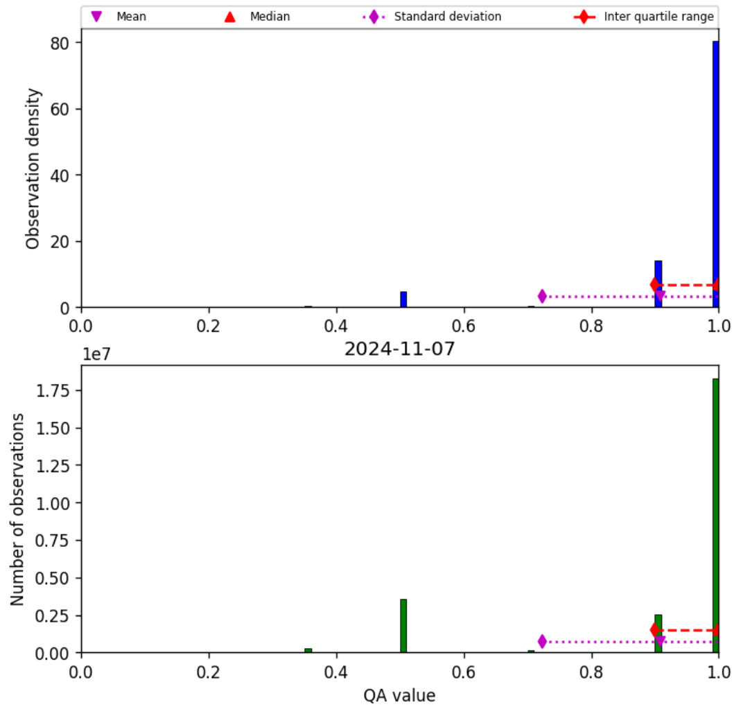
Figure 29: Histogram of “QA value” for 2024-11-06 to 2024-11-08
