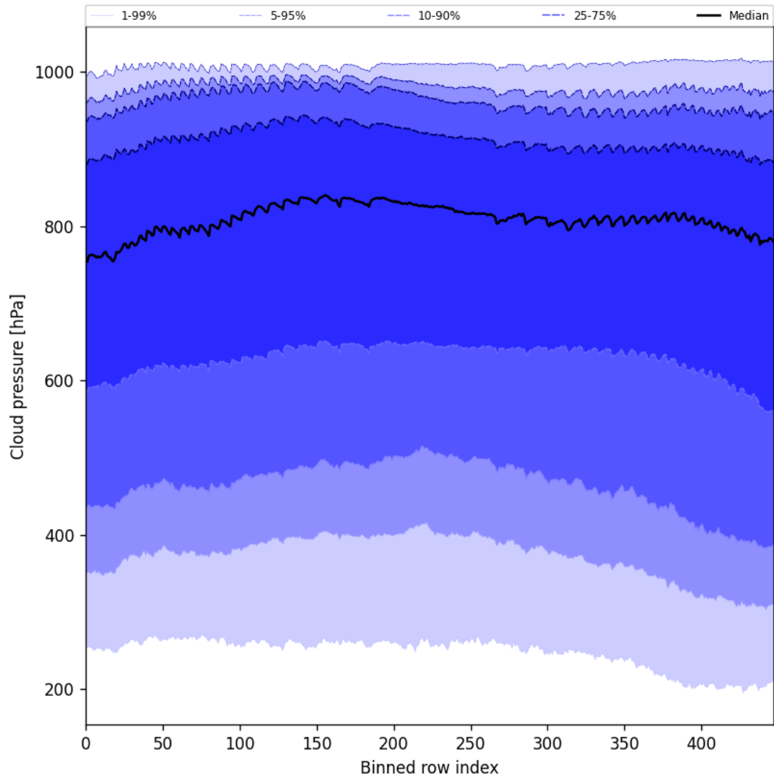
Figure 47: Along track statistics of “Cloud pressure” for 2024-11-06 to 2024-11-08
