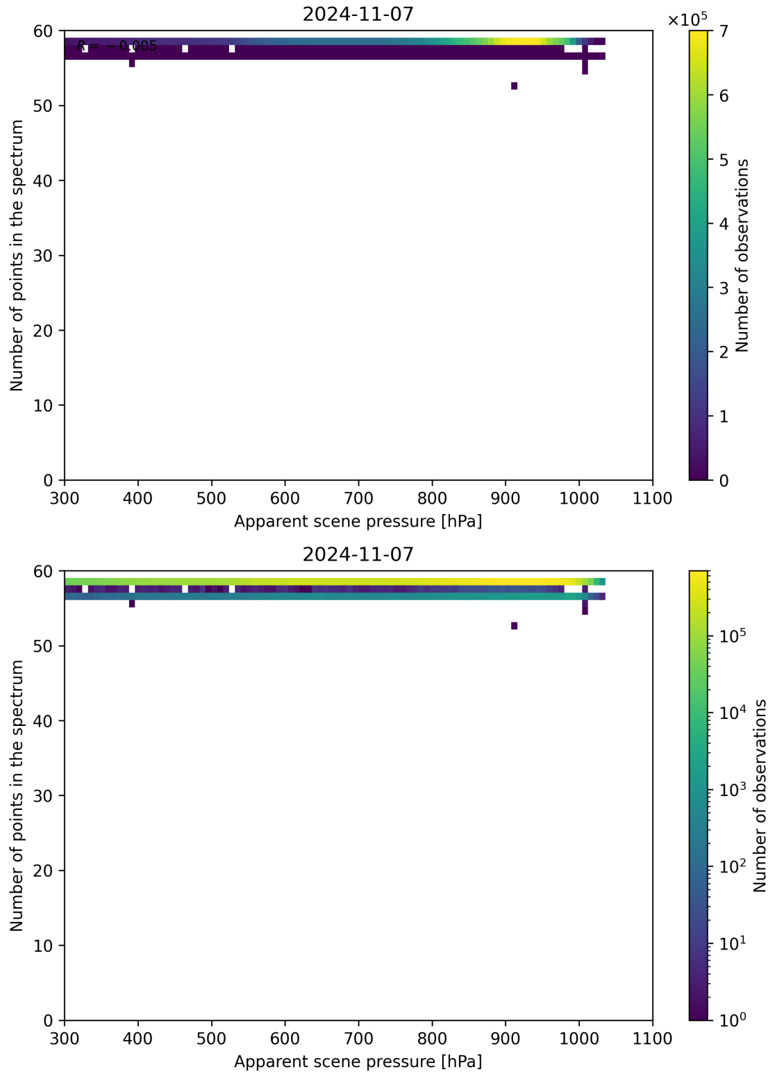
Figure 67: Scatter density plot of “Apparent scene pressure” against “Number of points in the spectrum” for 2024-11-06 to 2024-11-08.
