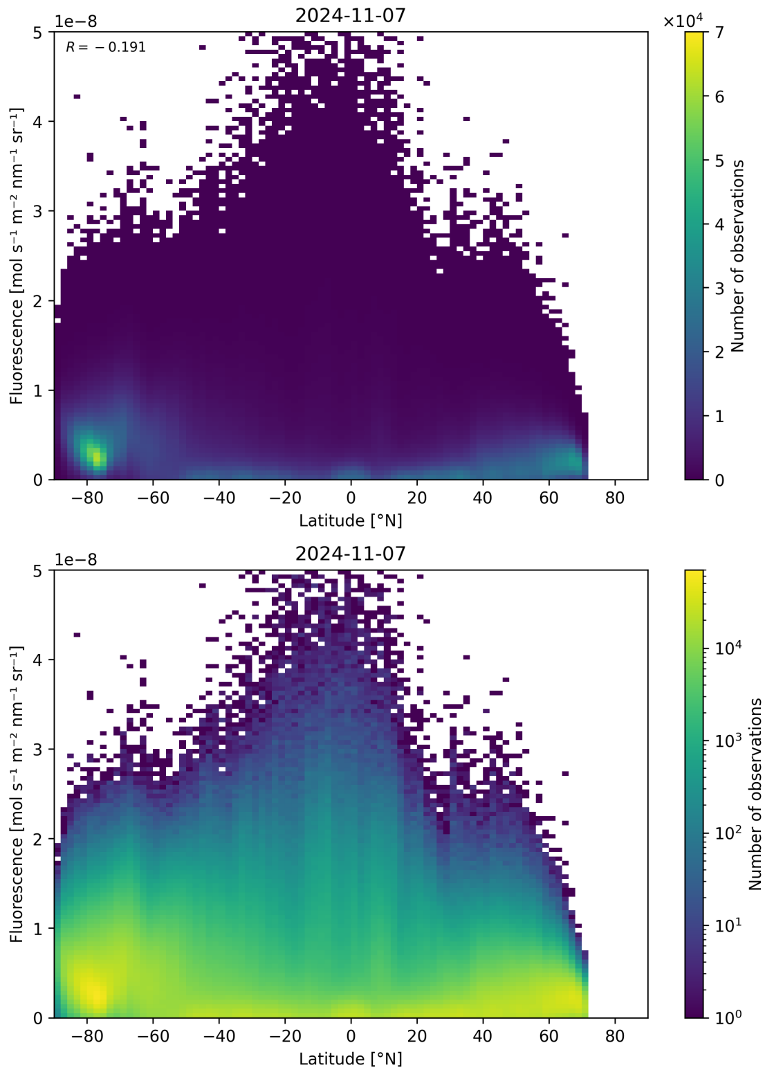
Figure 101: Scatter density plot of “Latitude” against “Fluorescence” for 2024-11-06 to 2024-11-08.
