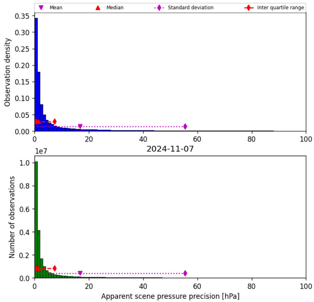
Figure 37: Histogram of “Apparent scene pressure precision” for 2024-11-06 to 2024-11-08
