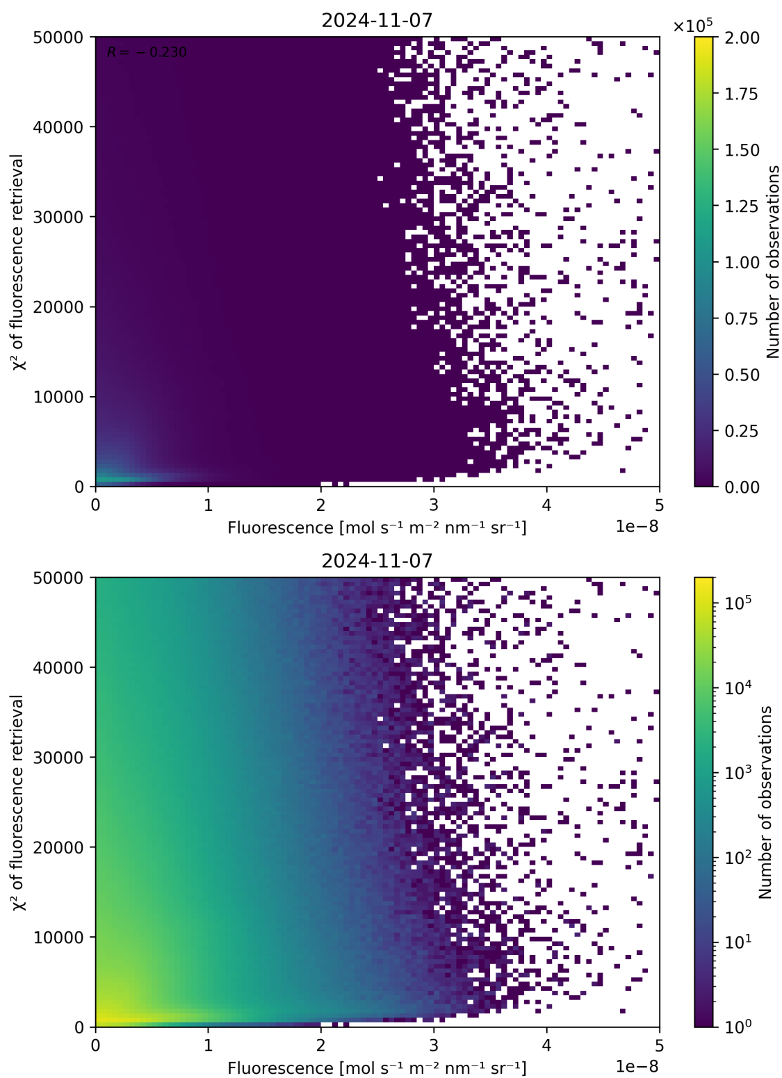
Figure 93: Scatter density plot of “Fluorescence” against “ \chi^2 of fluorescence retrieval” for 2024-11-06 to 2024-11-08.
