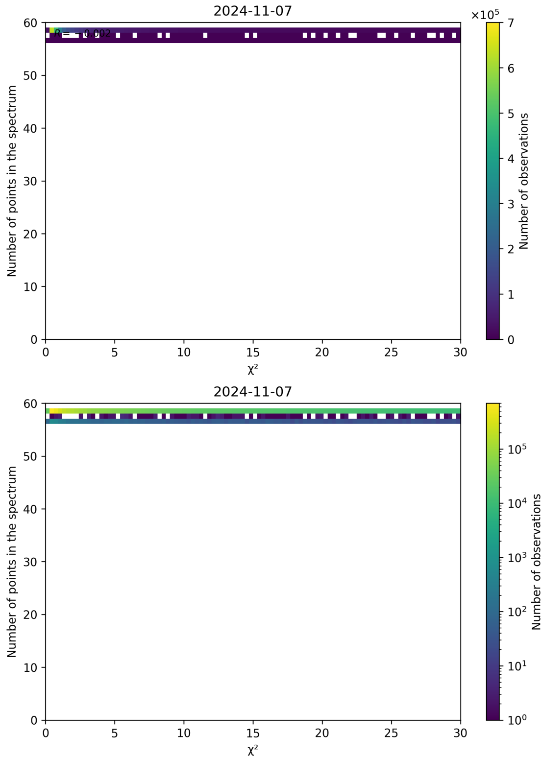
Figure 74: Scatter density plot of " \chi^2 " against "Number of points in the spectrum" for 2024-11-06 to 2024-11-08.
