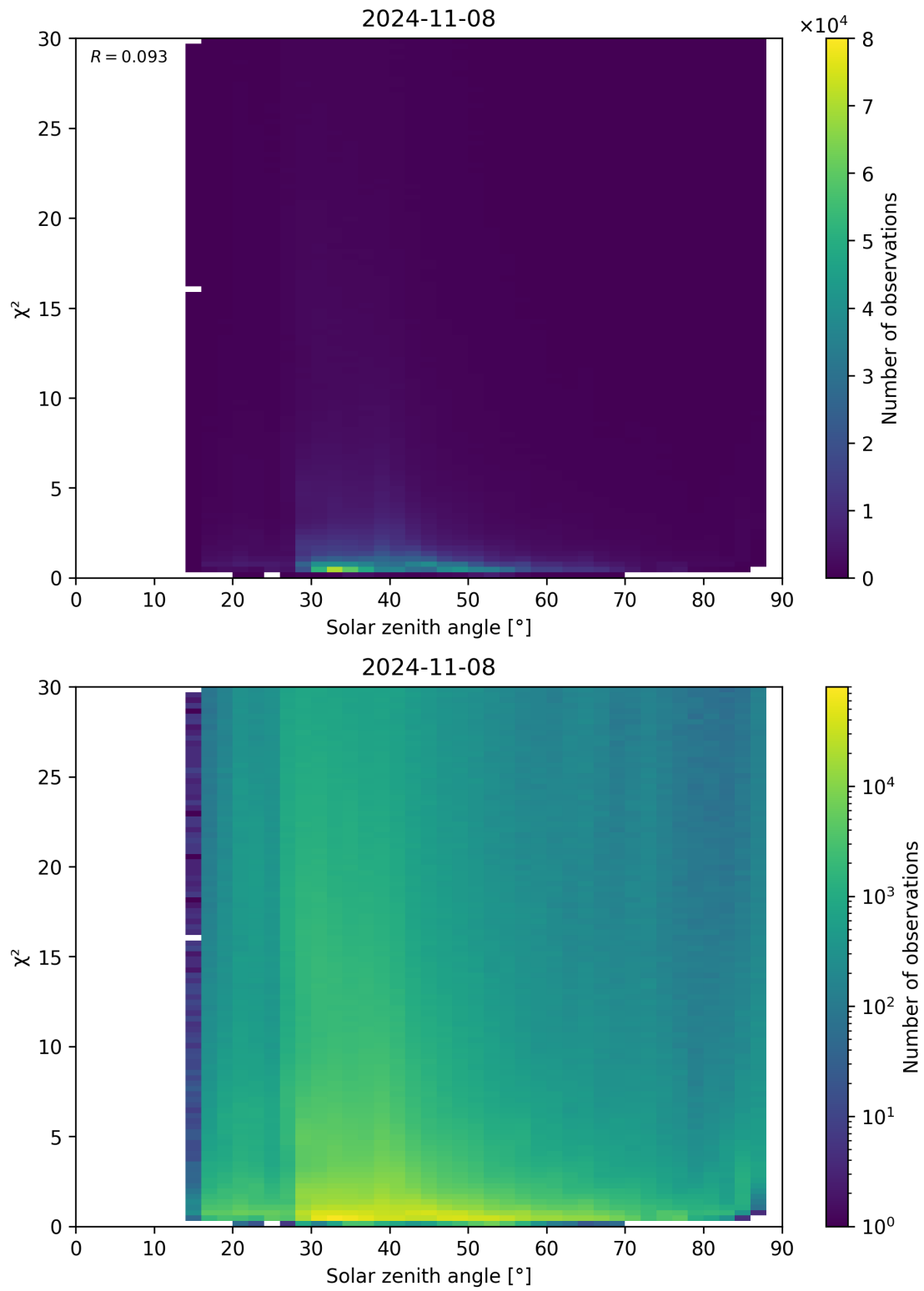
Figure 119: Scatter density plot of “Solar zenith angle” against “ \chi^2 ” for 2024-11-07 to 2024-11-09.
