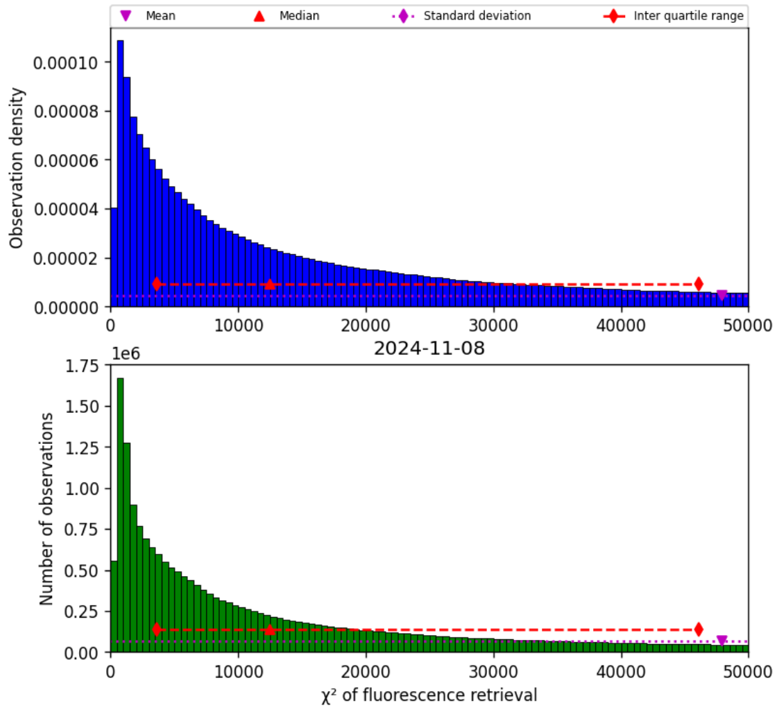
Figure 42: Histogram of “ \chi^2 of fluorescence retrieval” for 2024-11-07 to 2024-11-09
