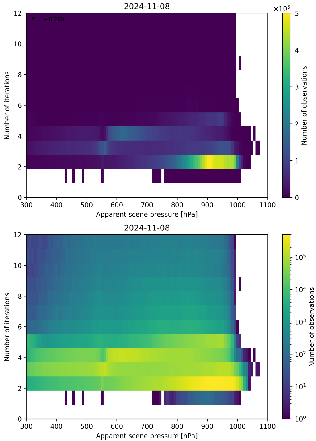
Figure 66: Scatter density plot of “Apparent scene pressure” against “Number of iterations” for 2024-11-07 to 2024-11-09.
