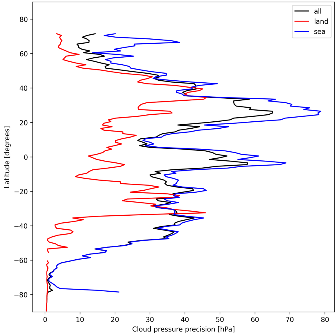
Figure 14: Zonal average of “Cloud pressure precision” for 2024-11-07 to 2024-11-09.
