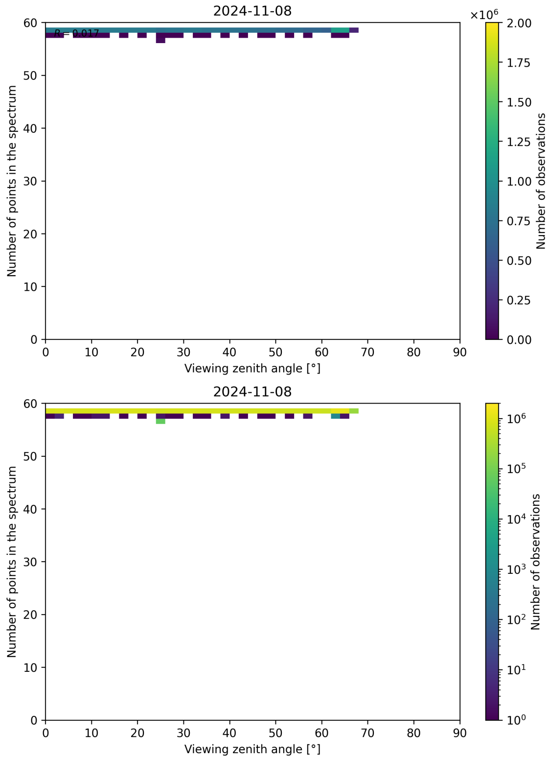
Figure 137: Scatter density plot of “Viewing zenith angle” against “Number of points in the spectrum” for 2024-11-07 to 2024-11-09.
