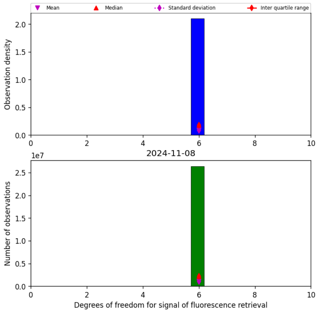
Figure 43: Histogram of "Degrees of freedom for signal of fluorescence retrieval" for 2024-11-07 to 2024-11-09
