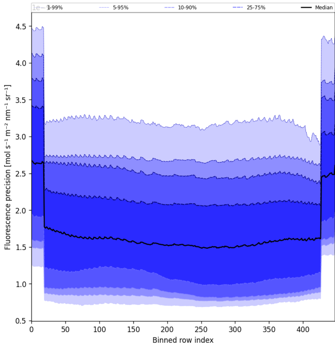
Figure 58: Along track statistics of “Fluorescence precision” for 2024-11-07 to 2024-11-09
