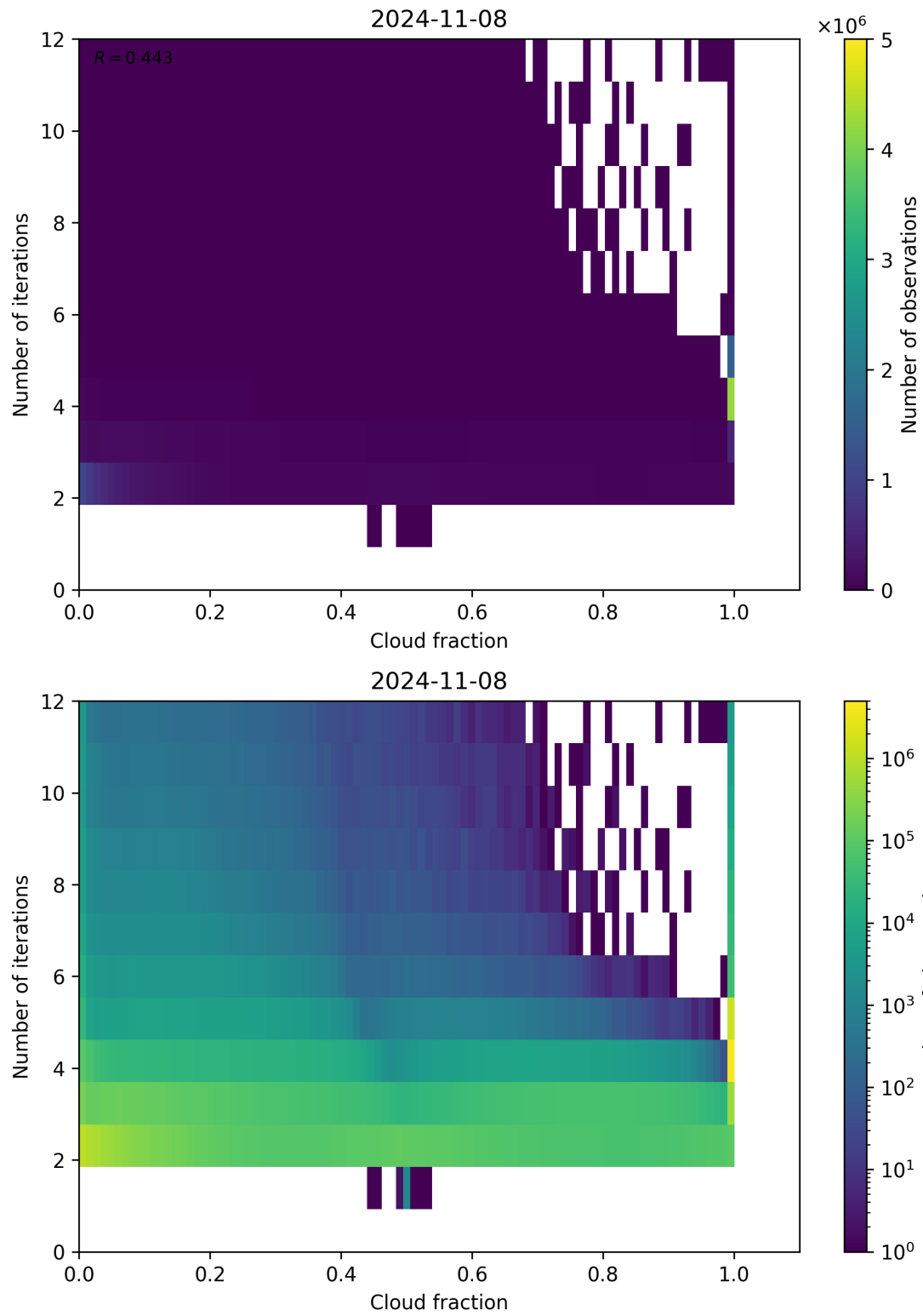
Figure 80: Scatter density plot of “Cloud fraction” against “Number of iterations” for 2024-11-07 to 2024-11-09.
