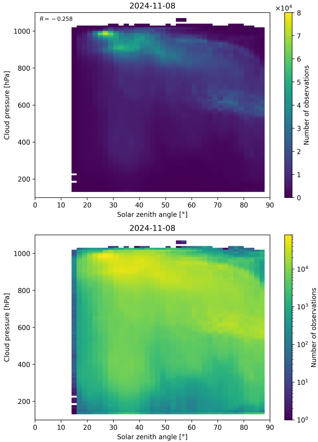
Figure 122: Scatter density plot of “Solar zenith angle” against “Cloud pressure” for 2024-11-07 to 2024-11-09.
