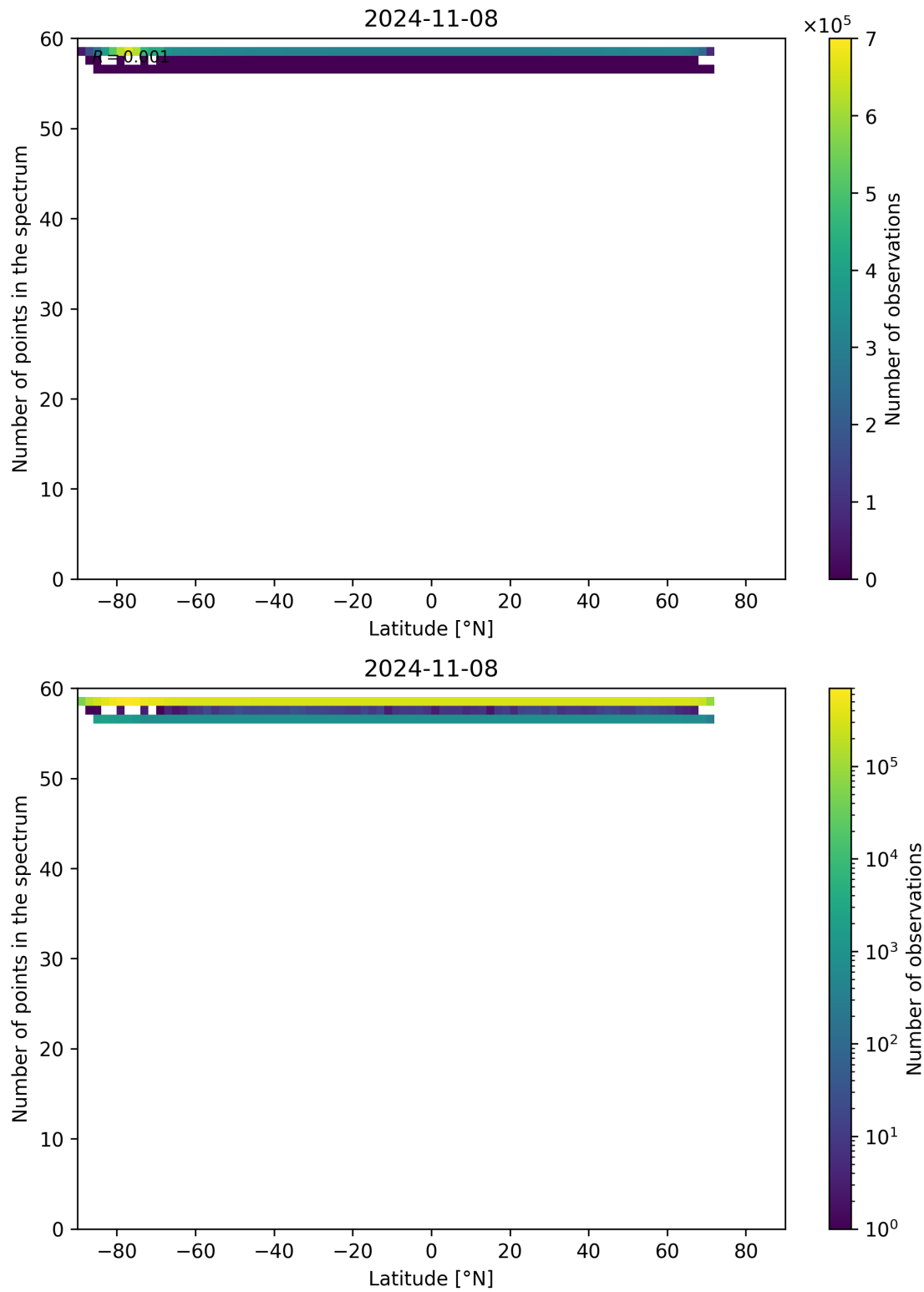
Figure 103: Scatter density plot of “Latitude” against “Number of points in the spectrum” for 2024-11-07 to 2024-11-09.
