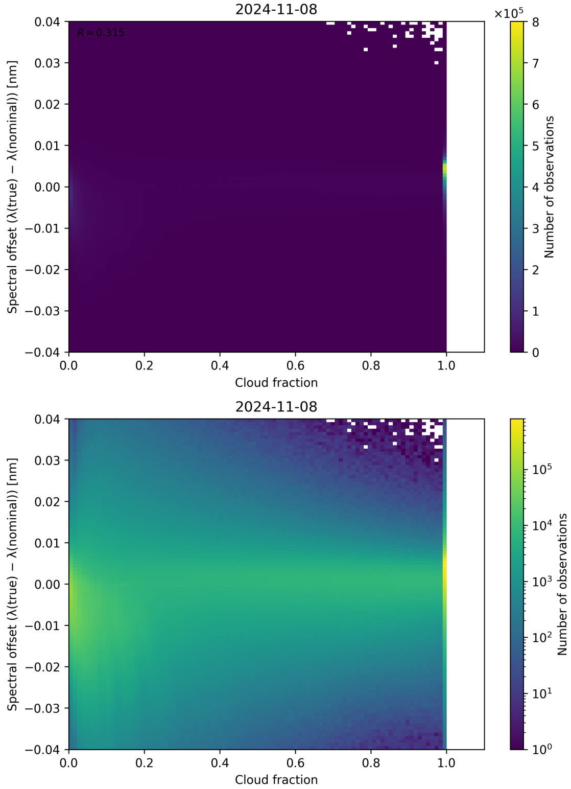
Figure 83: Scatter density plot of “Cloud fraction” against “Spectral offset ( \lambda_{\text{true}} - \lambda_{\text{nominal}} )” for 2024-11-07 to 2024-11-09.
