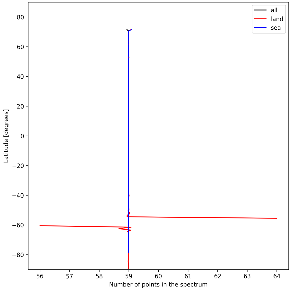
Figure 27: Zonal average of “Number of points in the spectrum” for 2024-11-07 to 2024-11-09.
