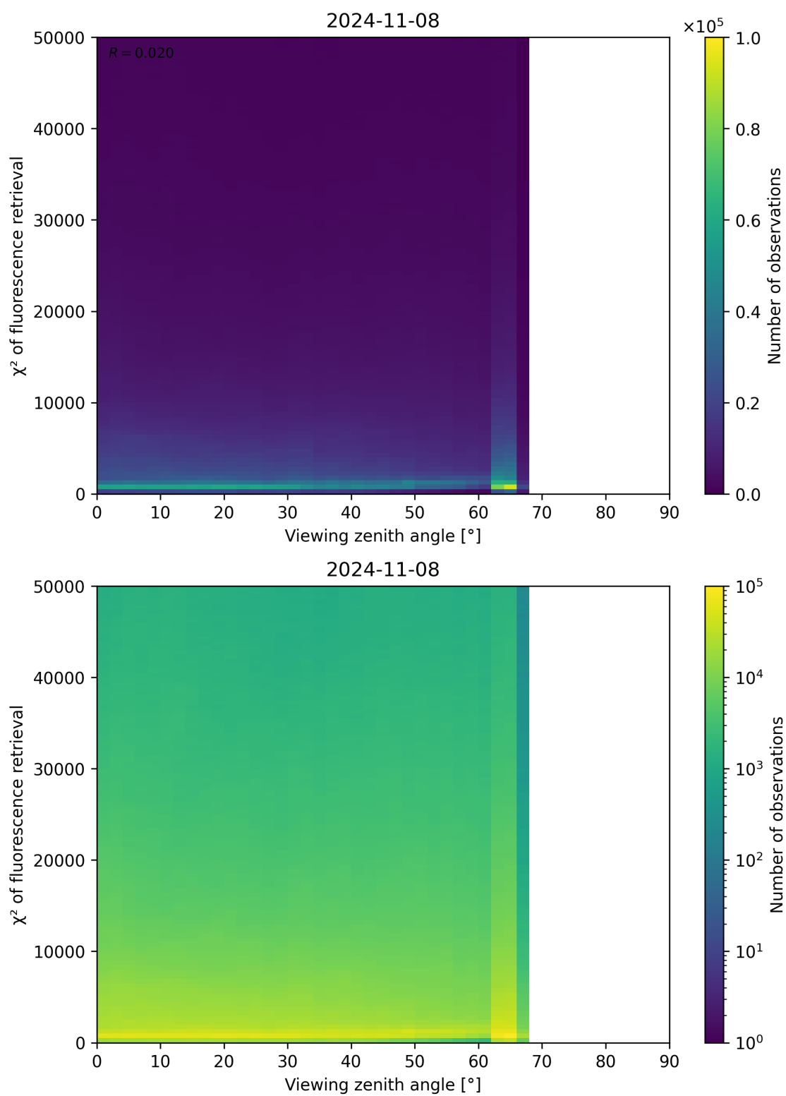
Figure 131: Scatter density plot of “Viewing zenith angle” against “ \chi^2 of fluorescence retrieval” for 2024-11-07 to 2024-11-09.
