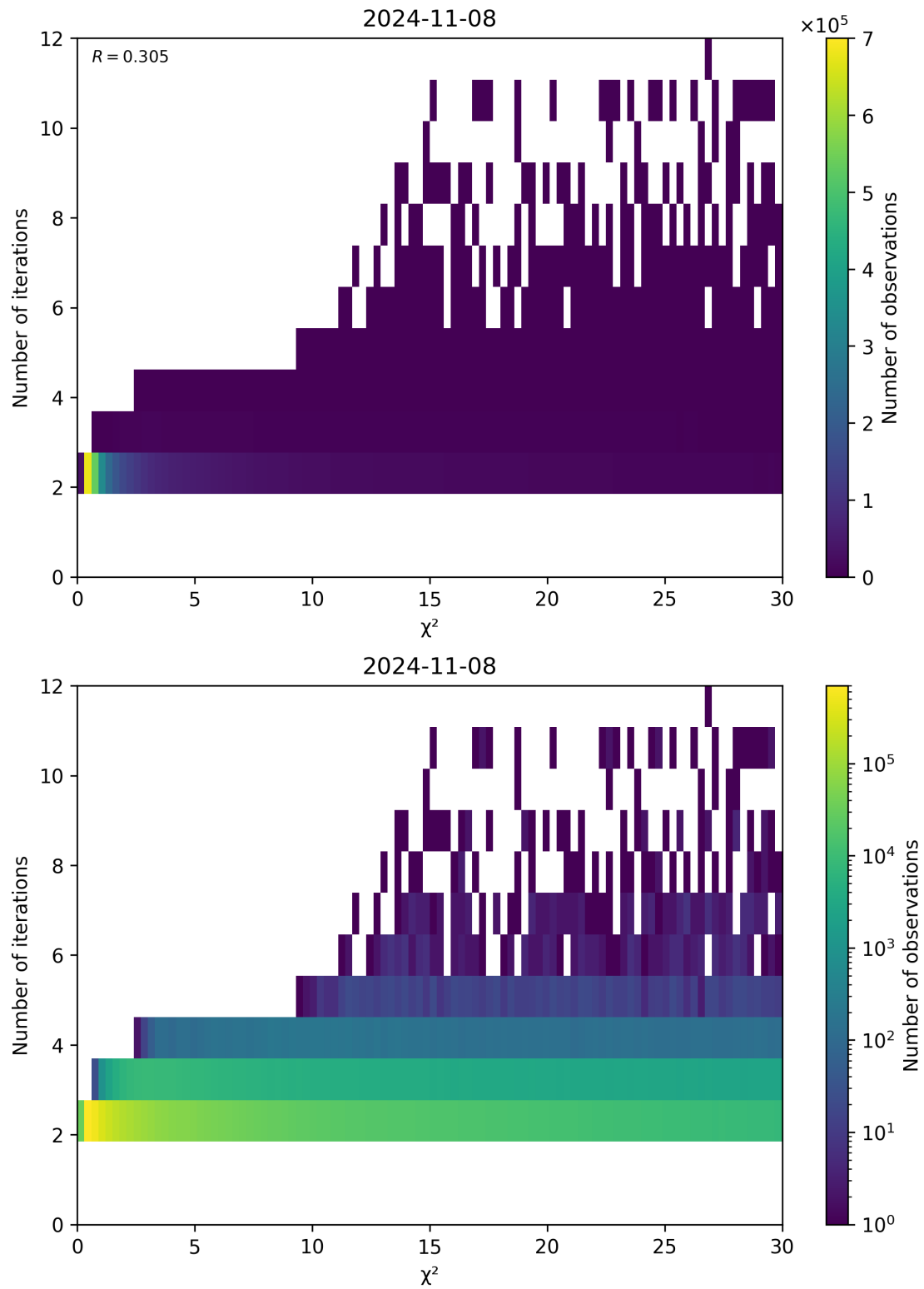
Figure 73: Scatter density plot of “ \chi^2 ” against “Number of iterations” for 2024-11-07 to 2024-11-09.
