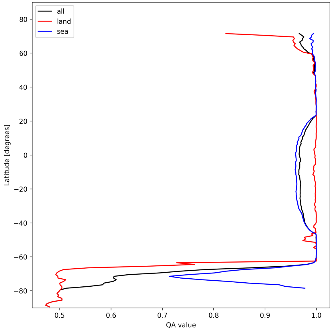
Figure 12: Zonal average of “QA value” for 2024-11-07 to 2024-11-09.
