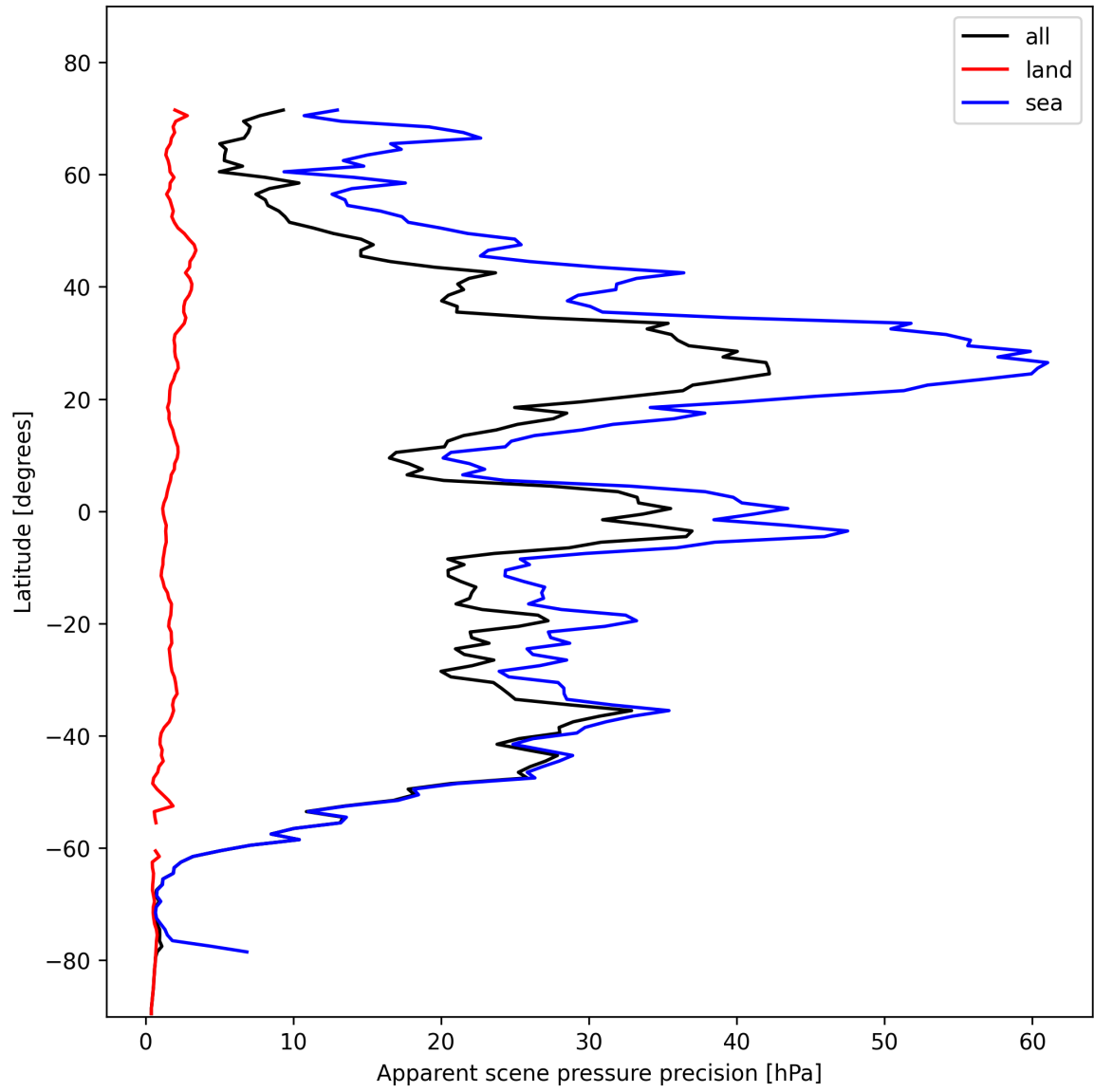
Figure 20: Zonal average of “Apparent scene pressure precision” for 2024-11-07 to 2024-11-09.
