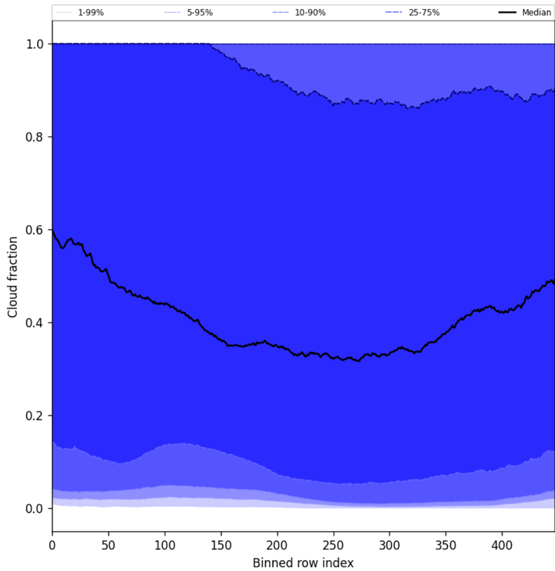
Figure 49: Along track statistics of “Cloud fraction” for 2024-11-07 to 2024-11-09
