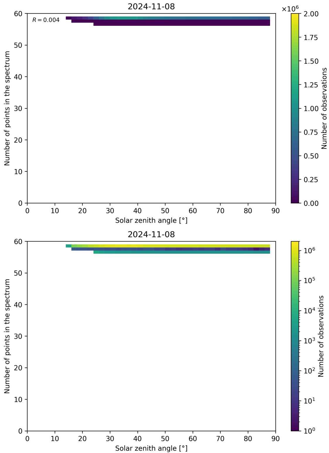
Figure 126: Scatter density plot of “Solar zenith angle” against “Number of points in the spectrum” for 2024-11-07 to 2024-11-09.
