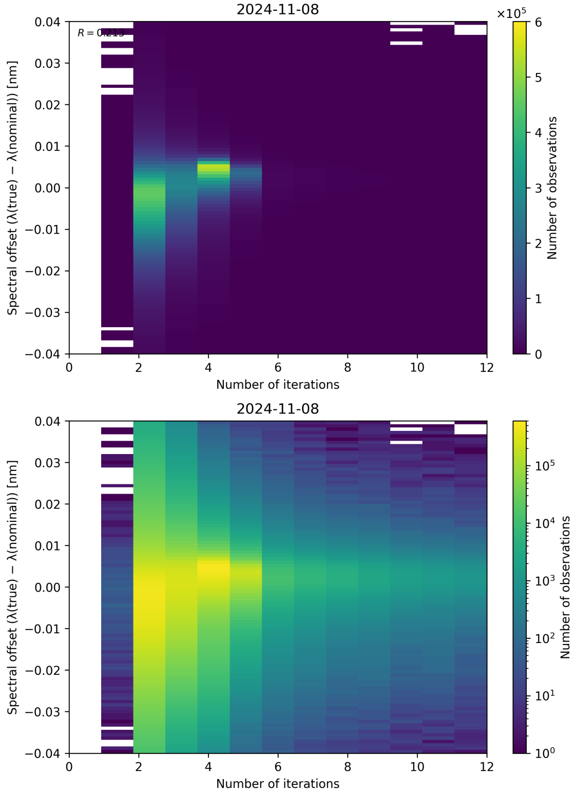
Figure 109: Scatter density plot of “Number of iterations” against “Spectral offset ( \lambda_{\text{true}} - \lambda_{\text{nominal}} )” for 2024-11-07 to 2024-11-09.
