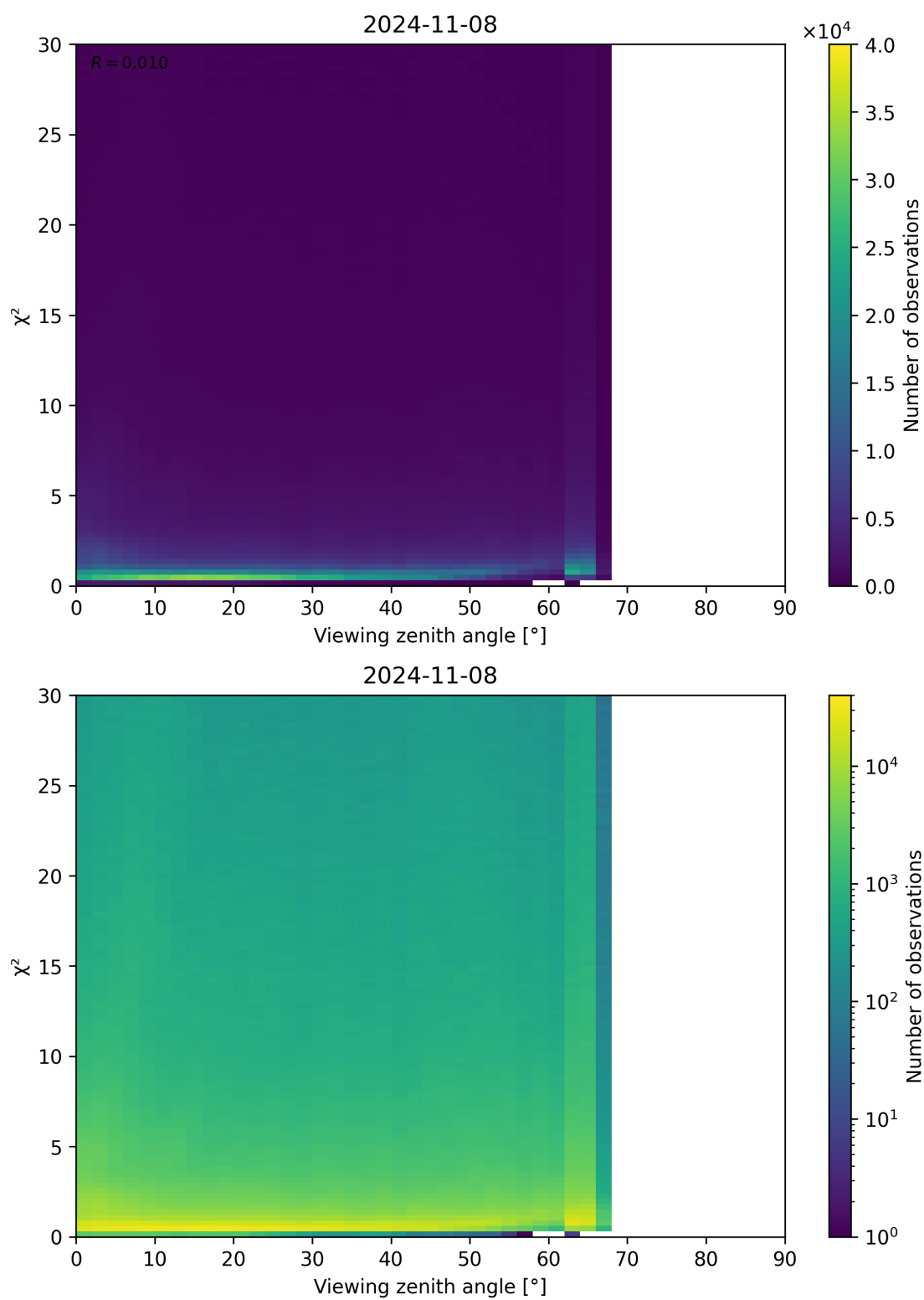
Figure 130: Scatter density plot of “Viewing zenith angle” against “ \chi^2 ” for 2024-11-07 to 2024-11-09.
