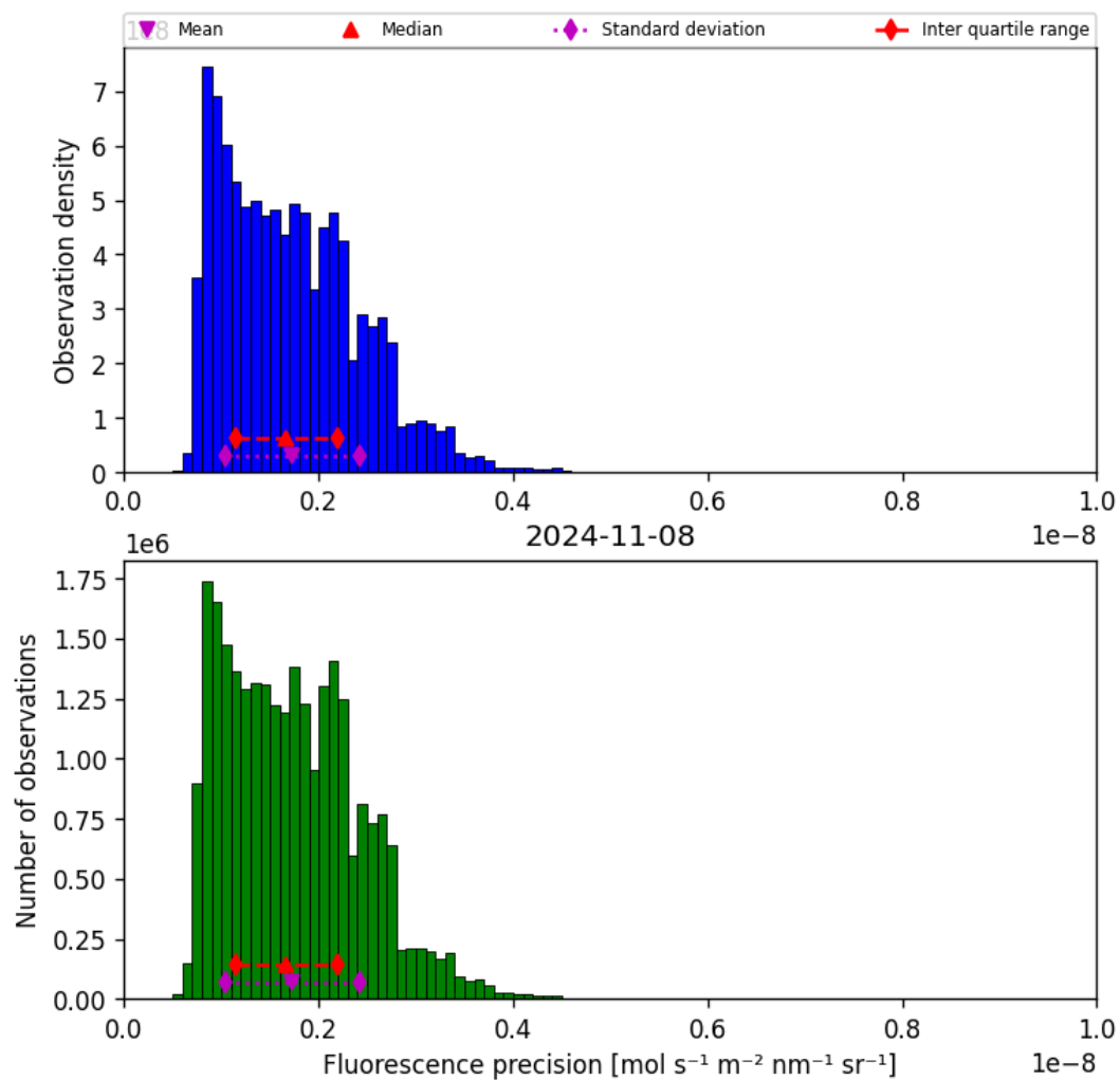
Figure 41: Histogram of “Fluorescence precision” for 2024-11-07 to 2024-11-09
