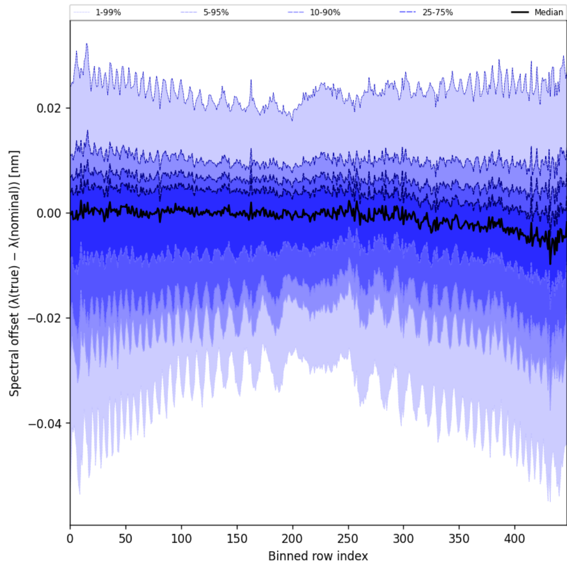
Figure 62: Along track statistics of “Spectral offset ( \lambda_{\text{true}} - \lambda_{\text{nominal}} )” for 2024-11-07 to 2024-11-09
