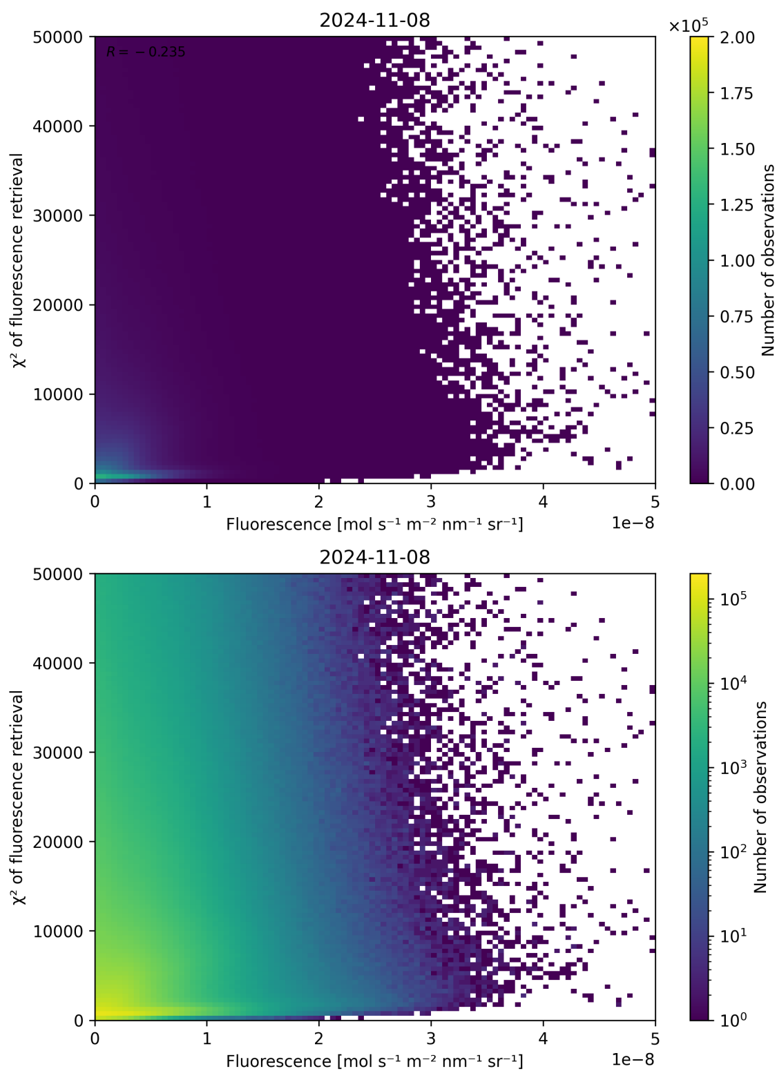
Figure 93: Scatter density plot of “Fluorescence” against “ \chi^2 of fluorescence retrieval” for 2024-11-07 to 2024-11-09.
