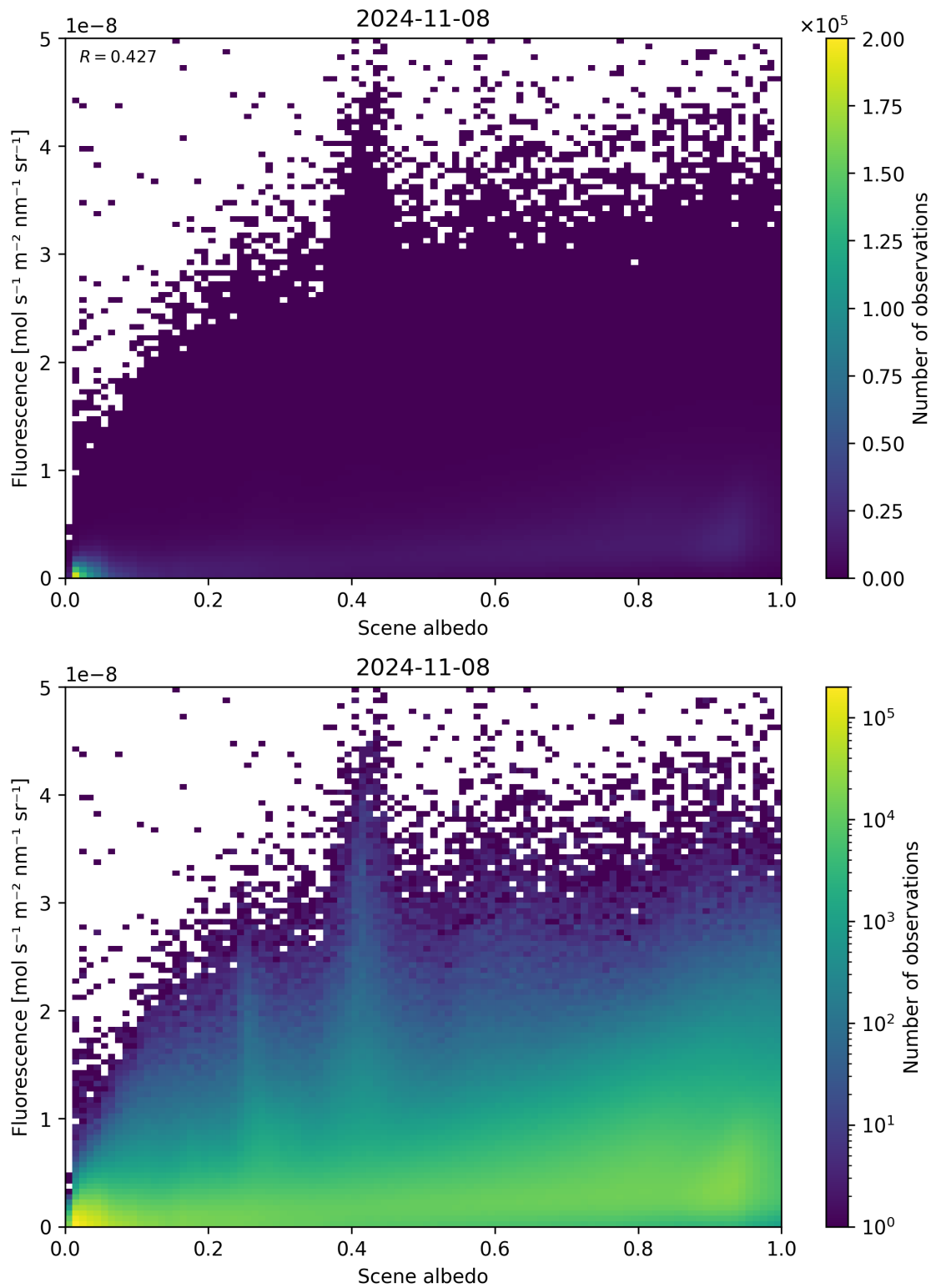
Figure 114: Scatter density plot of “Scene albedo” against “Fluorescence” for 2024-11-07 to 2024-11-09.
