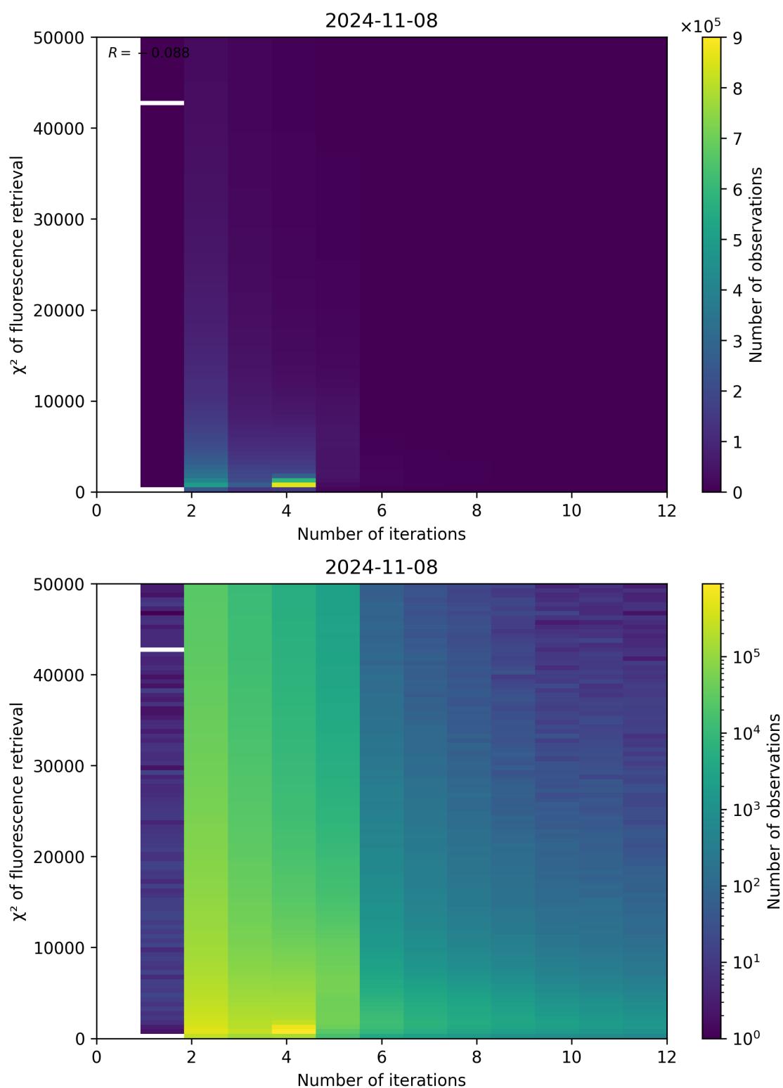
Figure 106: Scatter density plot of “Number of iterations” against “ \chi^2 of fluorescence retrieval” for 2024-11-07 to 2024-11-09.
