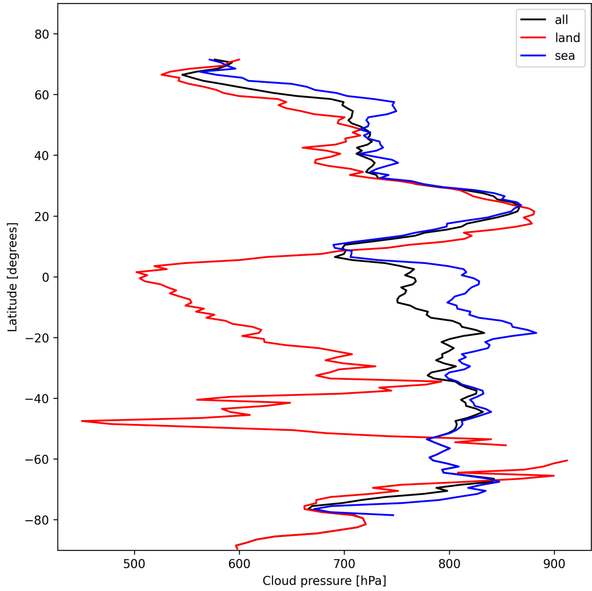
Figure 13: Zonal average of “Cloud pressure” for 2024-11-07 to 2024-11-09.
