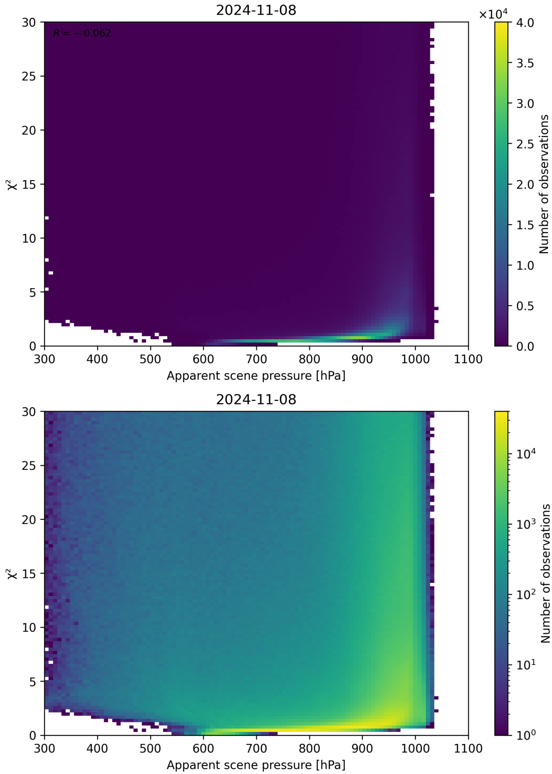
Figure 63: Scatter density plot of “Apparent scene pressure” against “ \chi^2 ” for 2024-11-07 to 2024-11-09.
