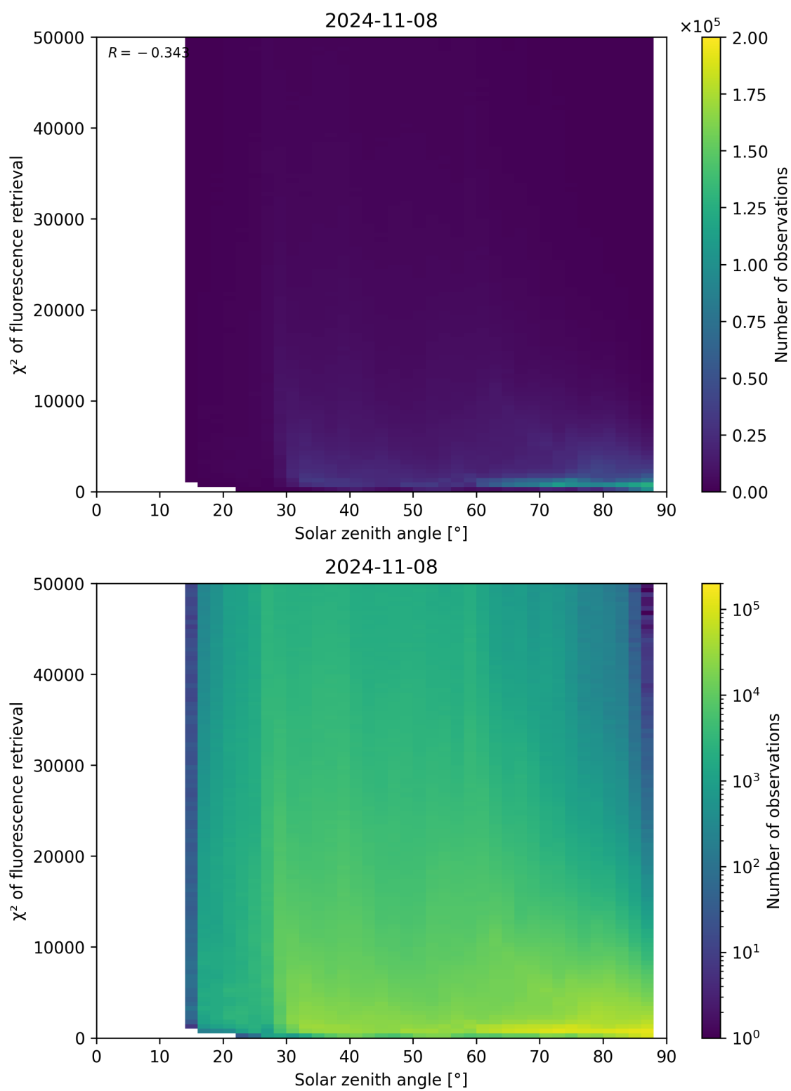
Figure 120: Scatter density plot of “Solar zenith angle” against “ \chi^2 of fluorescence retrieval” for 2024-11-07 to 2024-11-09.
