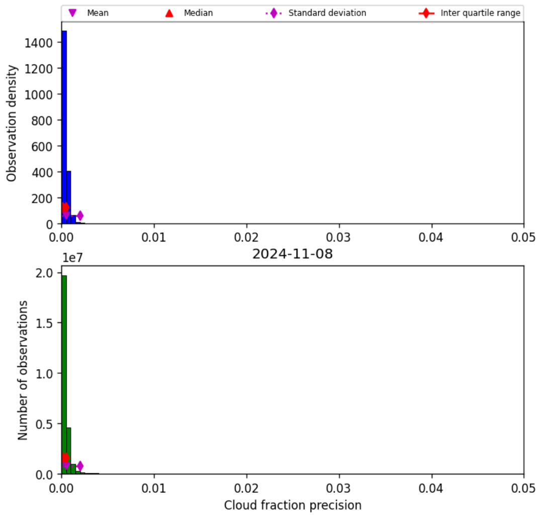
Figure 33: Histogram of “Cloud fraction precision” for 2024-11-07 to 2024-11-09
