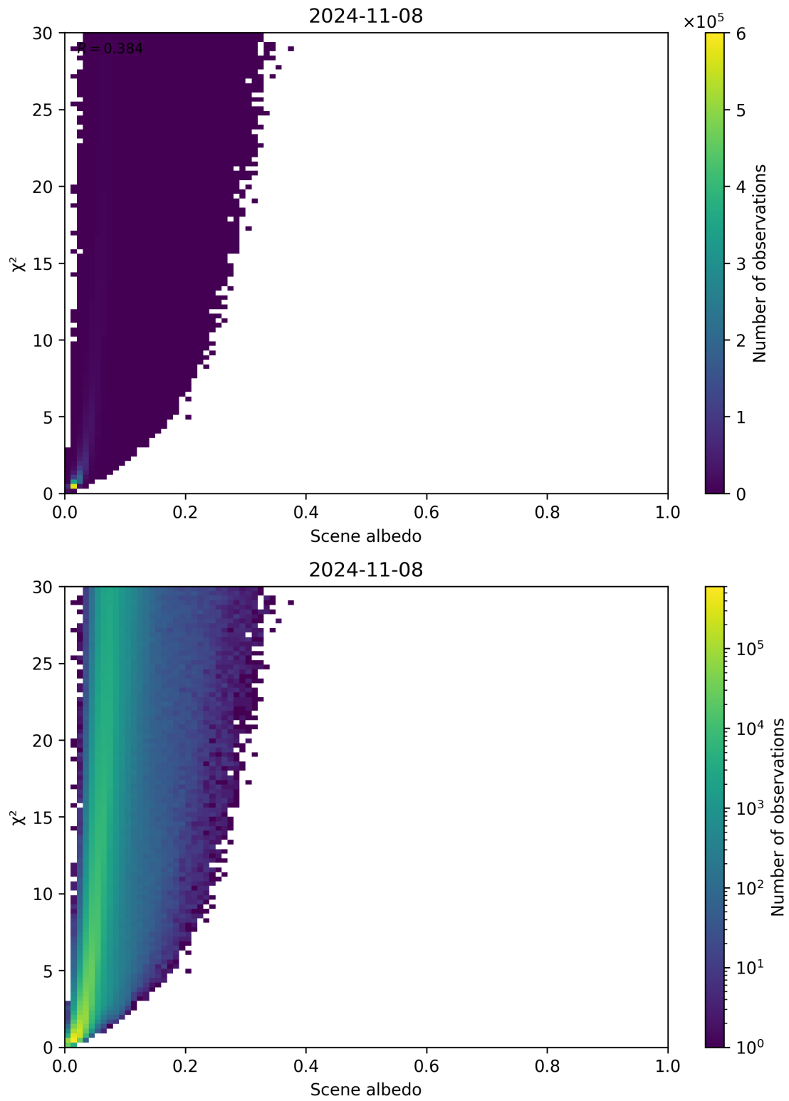
Figure 112: Scatter density plot of “Scene albedo” against “ \chi^2 ” for 2024-11-07 to 2024-11-09.
