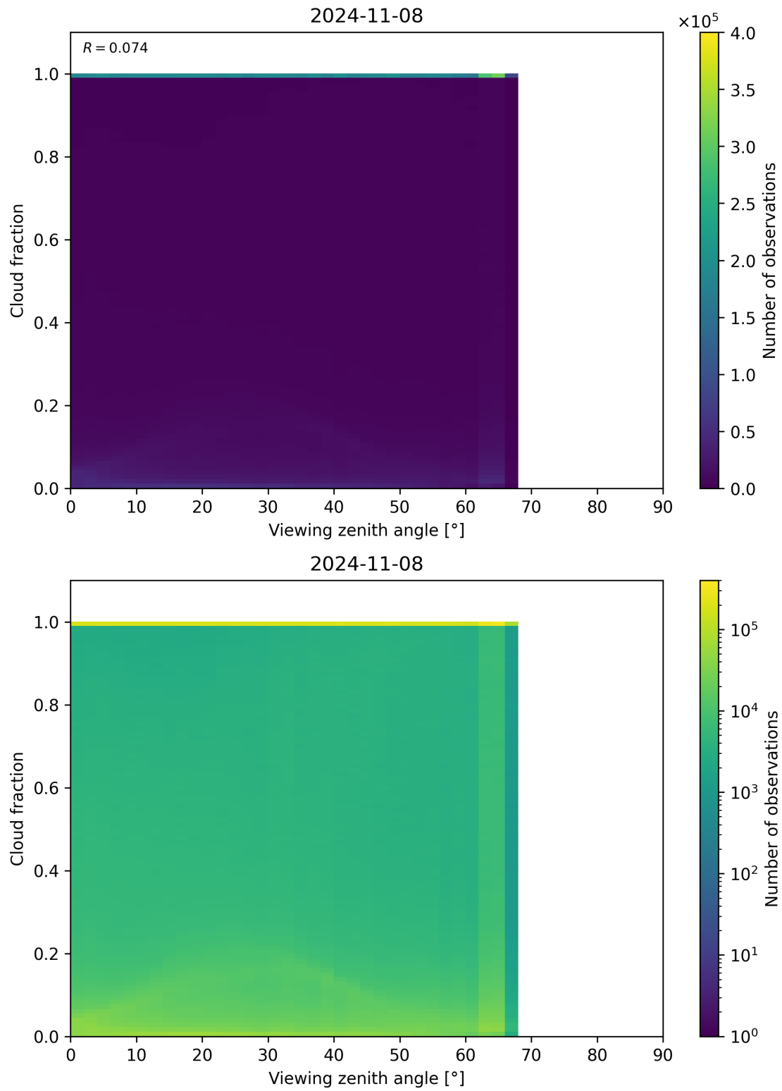
Figure 132: Scatter density plot of “Viewing zenith angle” against “Cloud fraction” for 2024-11-07 to 2024-11-09.
