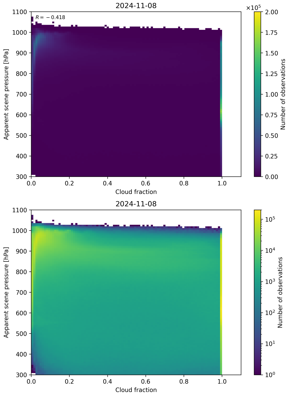
Figure 76: Scatter density plot of “Cloud fraction” against “Apparent scene pressure” for 2024-11-07 to 2024-11-09.
