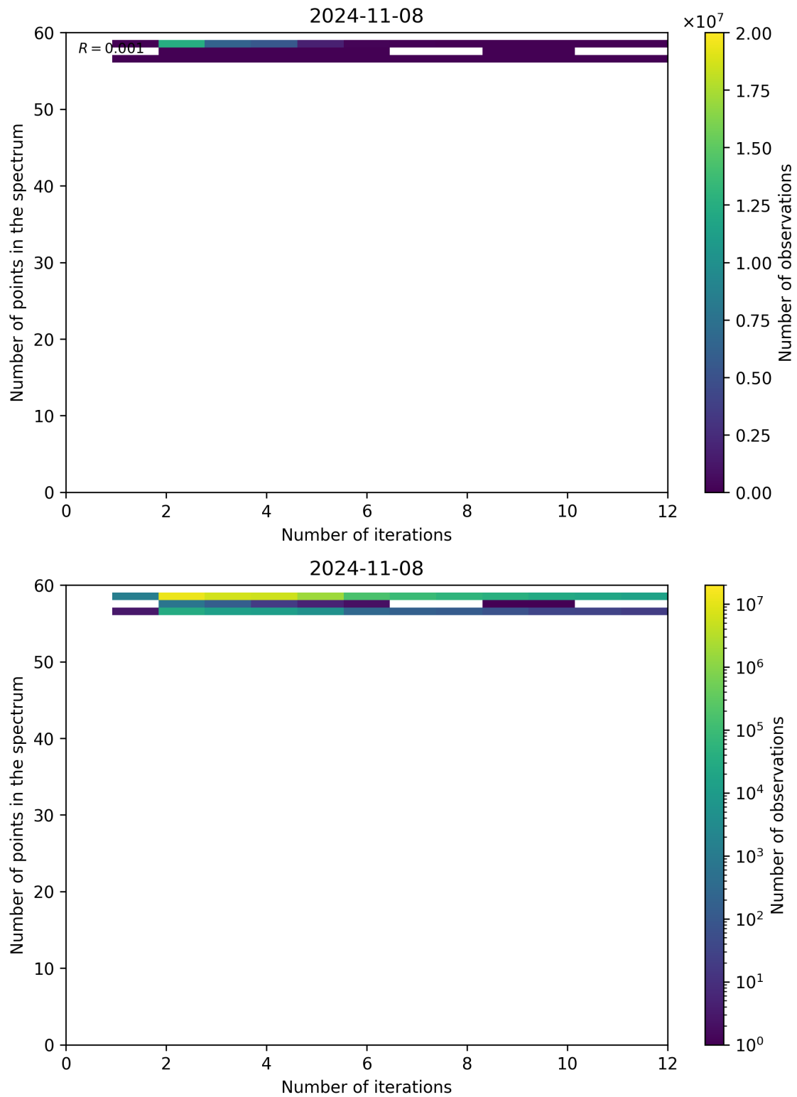
Figure 108: Scatter density plot of “Number of iterations” against “Number of points in the spectrum” for 2024-11-07 to 2024-11-09.
