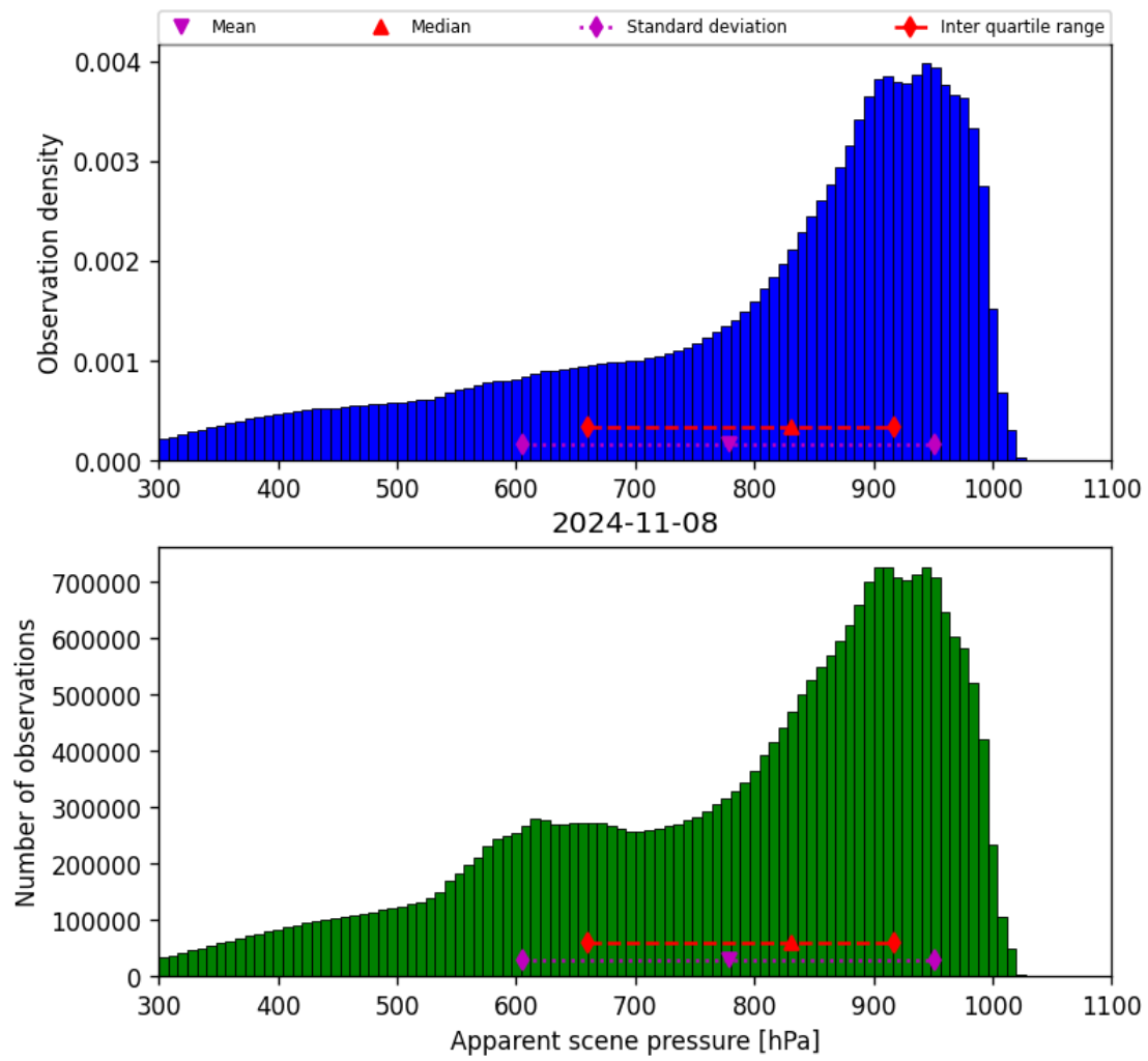
Figure 36: Histogram of “Apparent scene pressure” for 2024-11-07 to 2024-11-09
