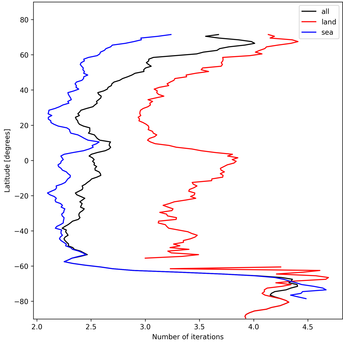
Figure 22: Zonal average of “Number of iterations” for 2024-11-07 to 2024-11-09.
