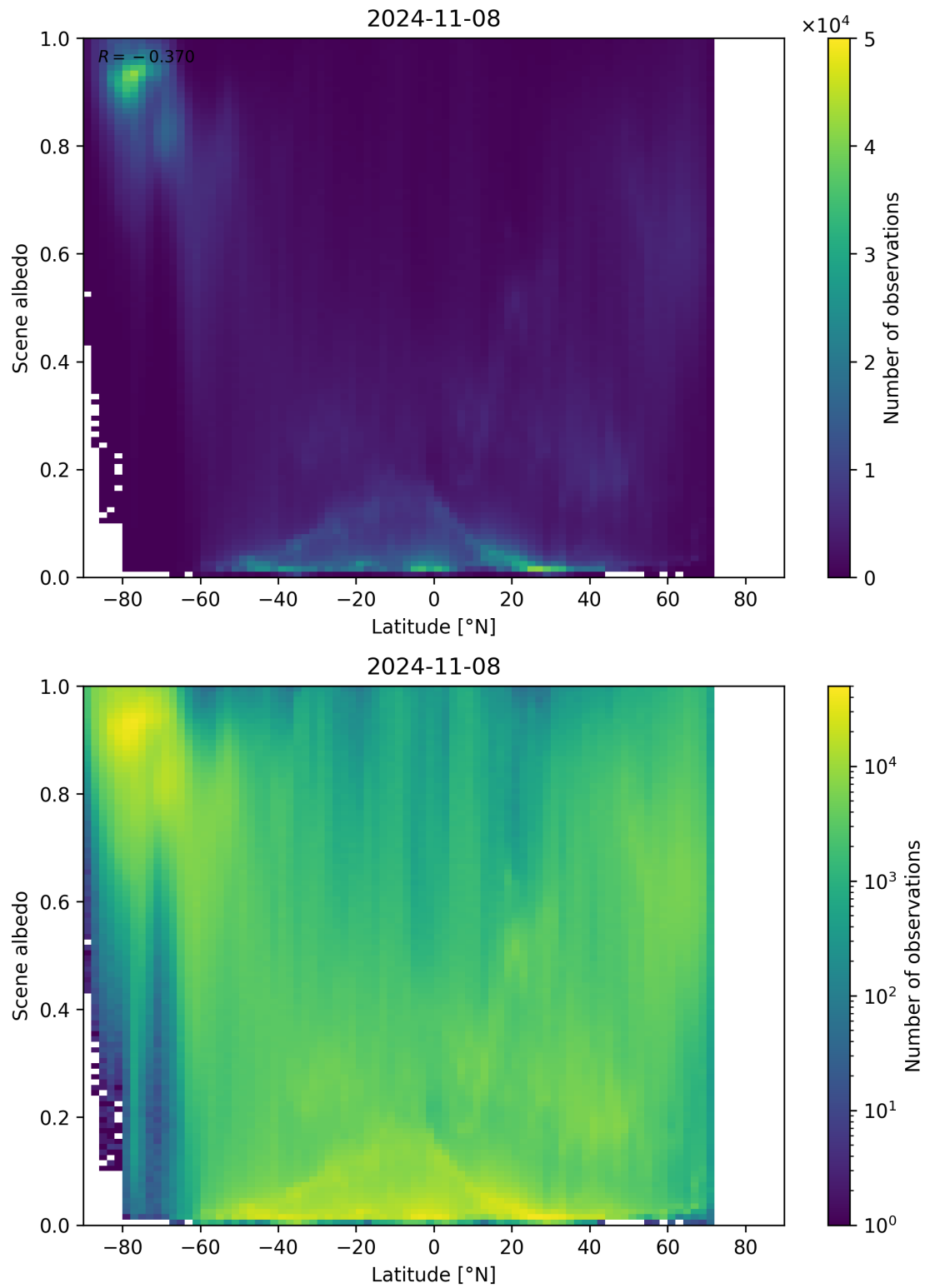
Figure 104: Scatter density plot of “Latitude” against “Scene albedo” for 2024-11-07 to 2024-11-09.
