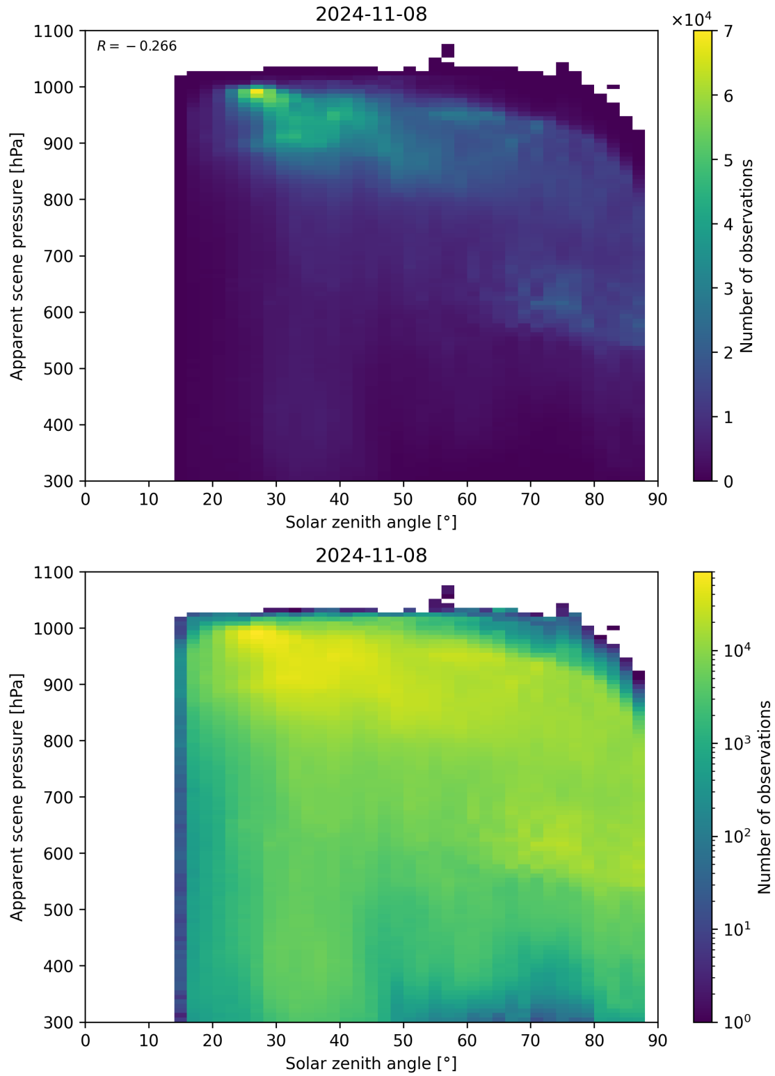
Figure 118: Scatter density plot of “Solar zenith angle” against “Apparent scene pressure” for 2024-11-07 to 2024-11-09.
