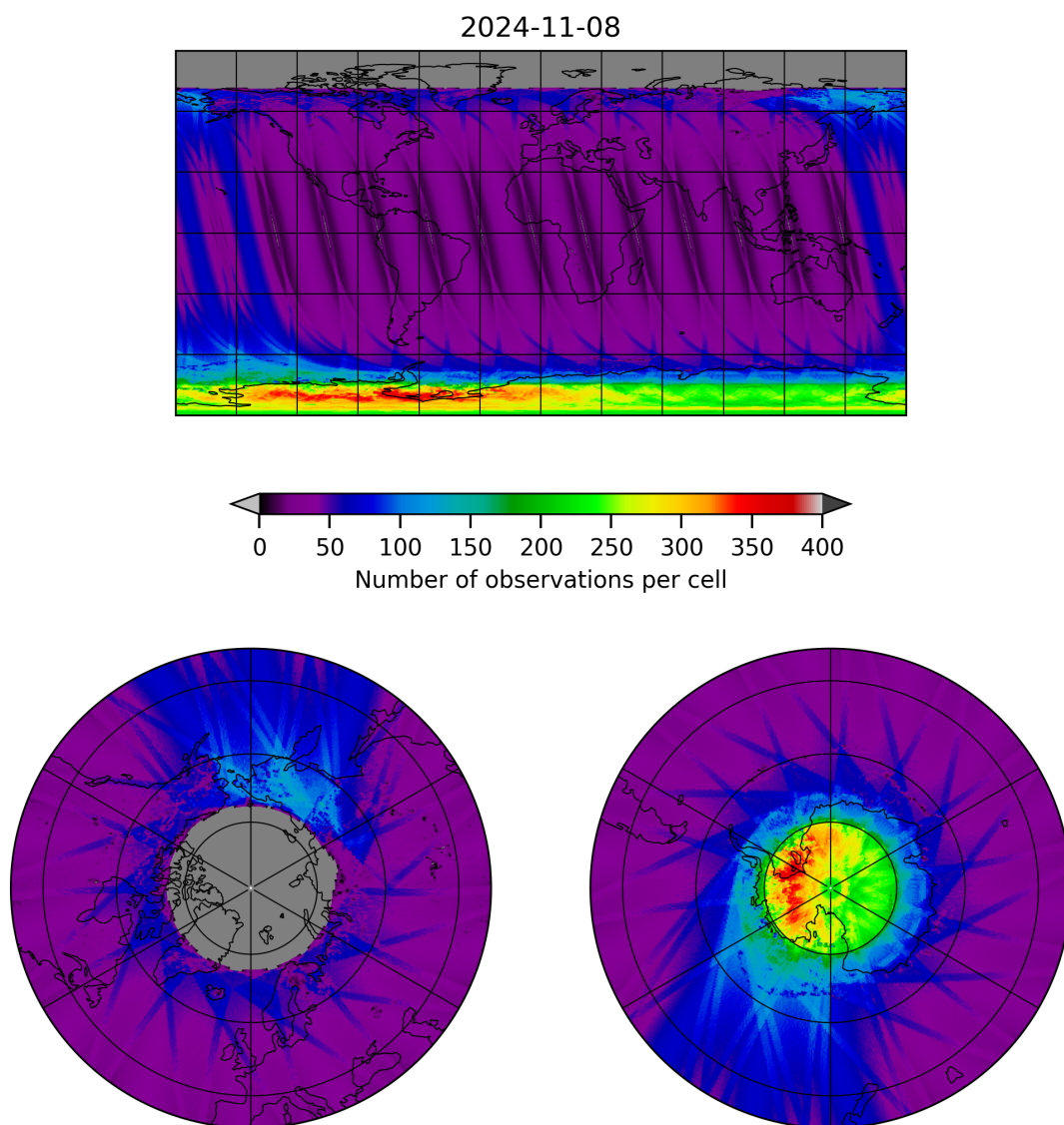
Figure 11: Map of the number of observations for 2024-11-07 to 2024-11-09
