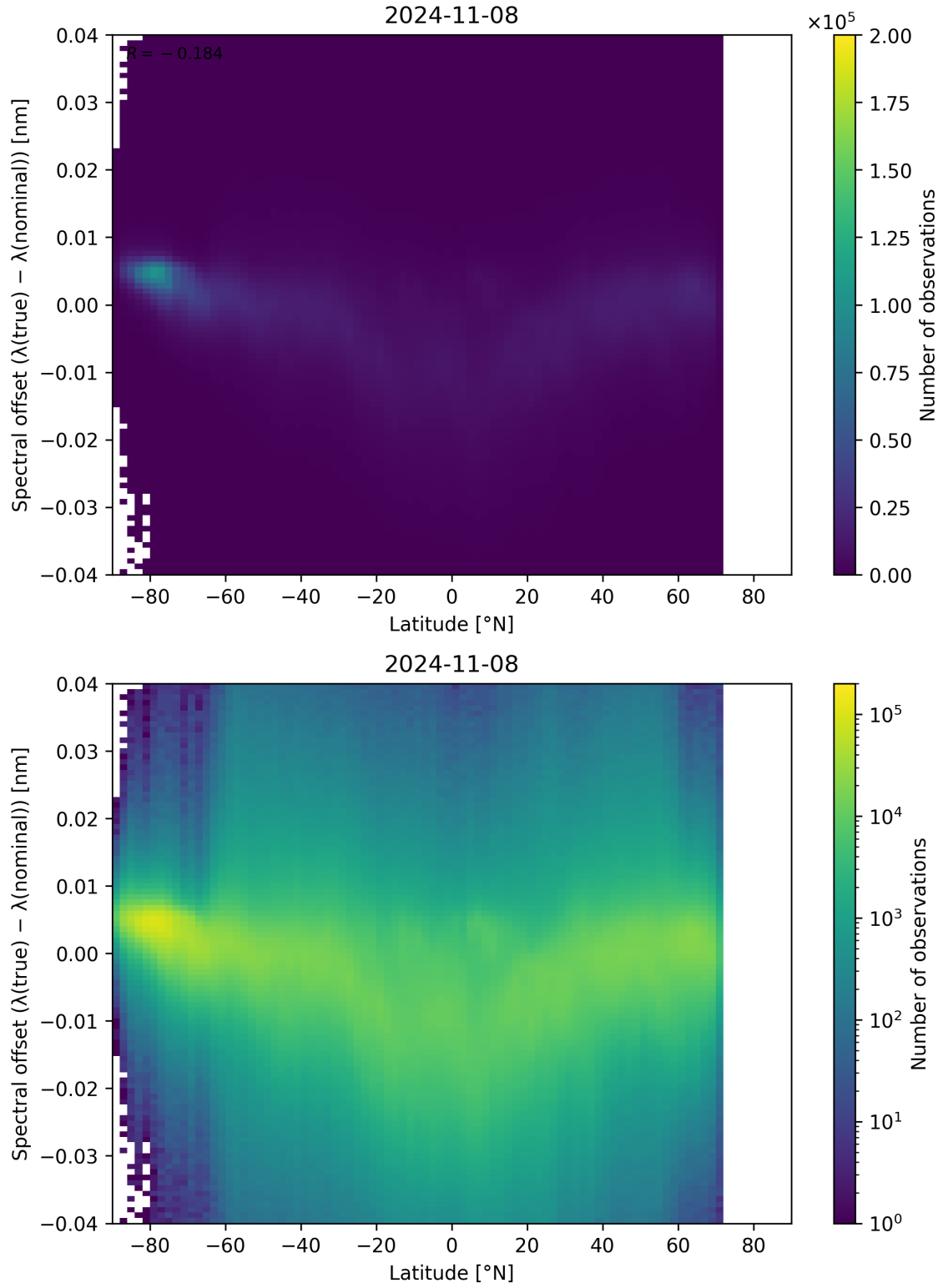
Figure 105: Scatter density plot of “Latitude” against “Spectral offset ( \lambda_{\text{true}} - \lambda_{\text{nominal}} )” for 2024-11-07 to 2024-11-09.
