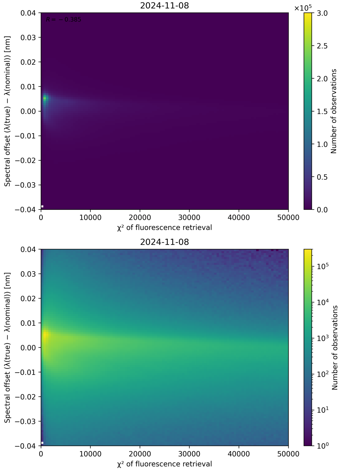
Figure 72: Scatter density plot of “ \chi^2 of fluorescence retrieval” against “Spectral offset ( \lambda_{\text{true}} - \lambda_{\text{nominal}} )” for 2024-11-07 to 2024-11-09.
