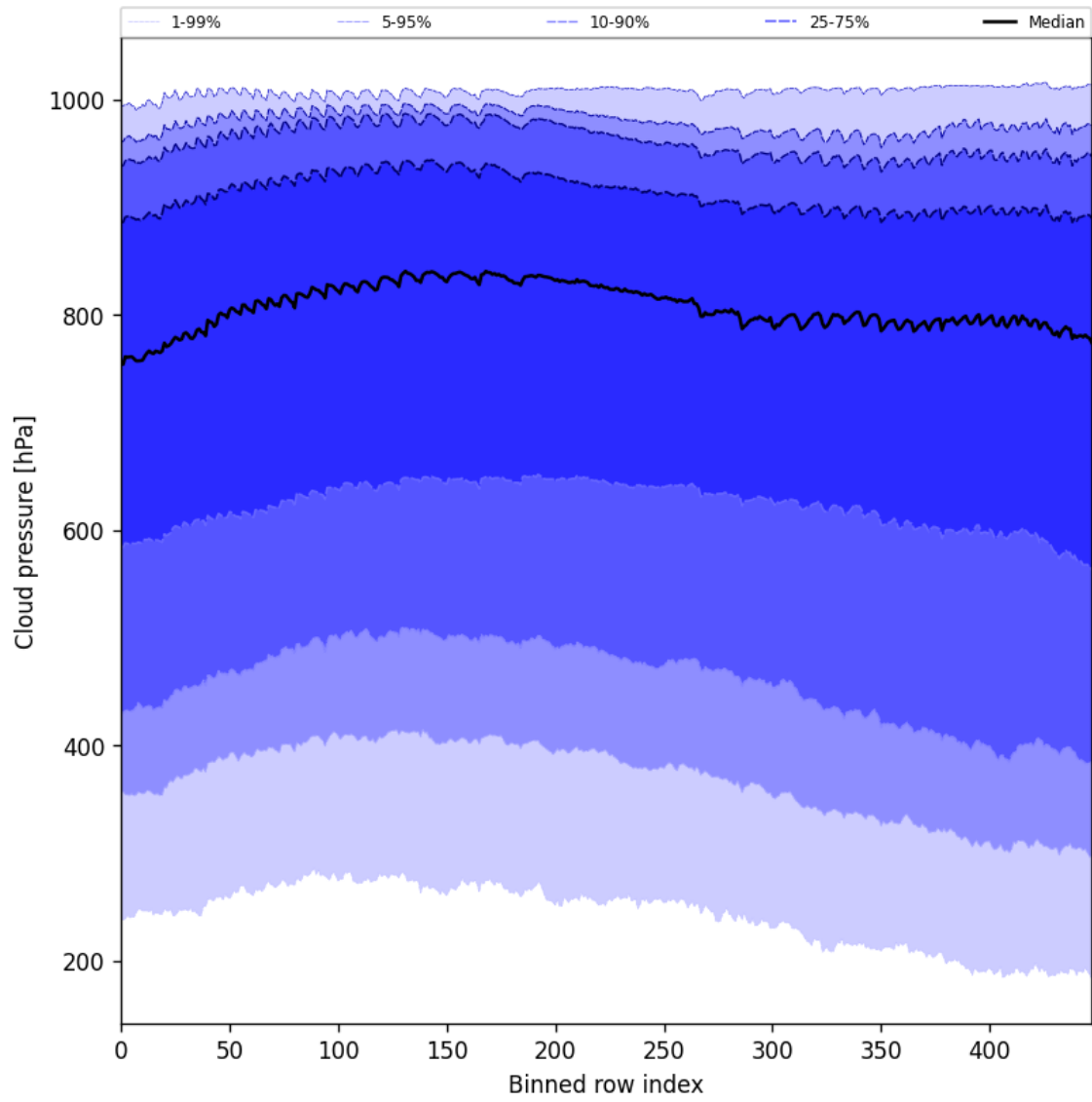
Figure 47: Along track statistics of “Cloud pressure” for 2024-11-07 to 2024-11-09
