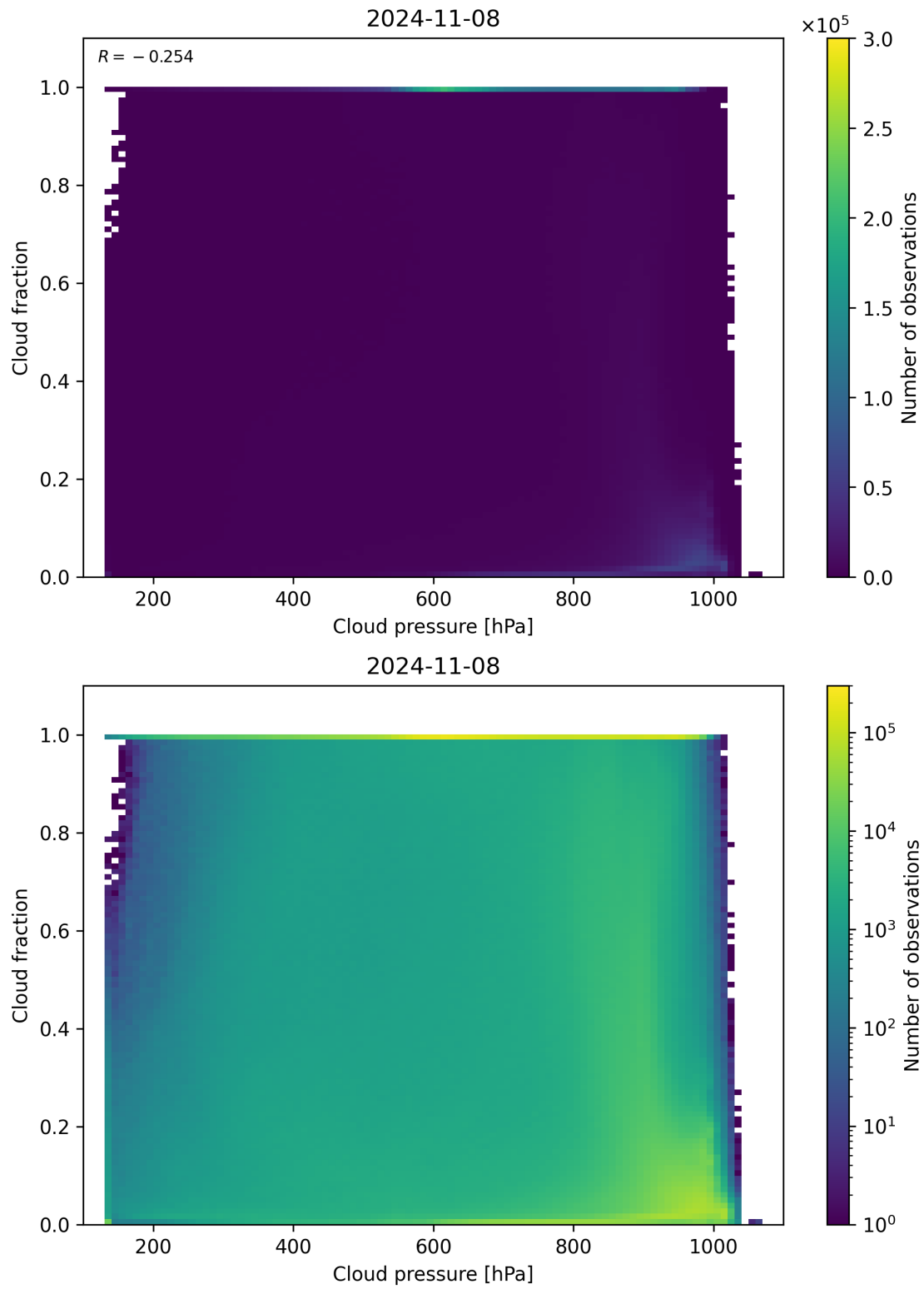
Figure 87: Scatter density plot of “Cloud pressure” against “Cloud fraction” for 2024-11-07 to 2024-11-09.
