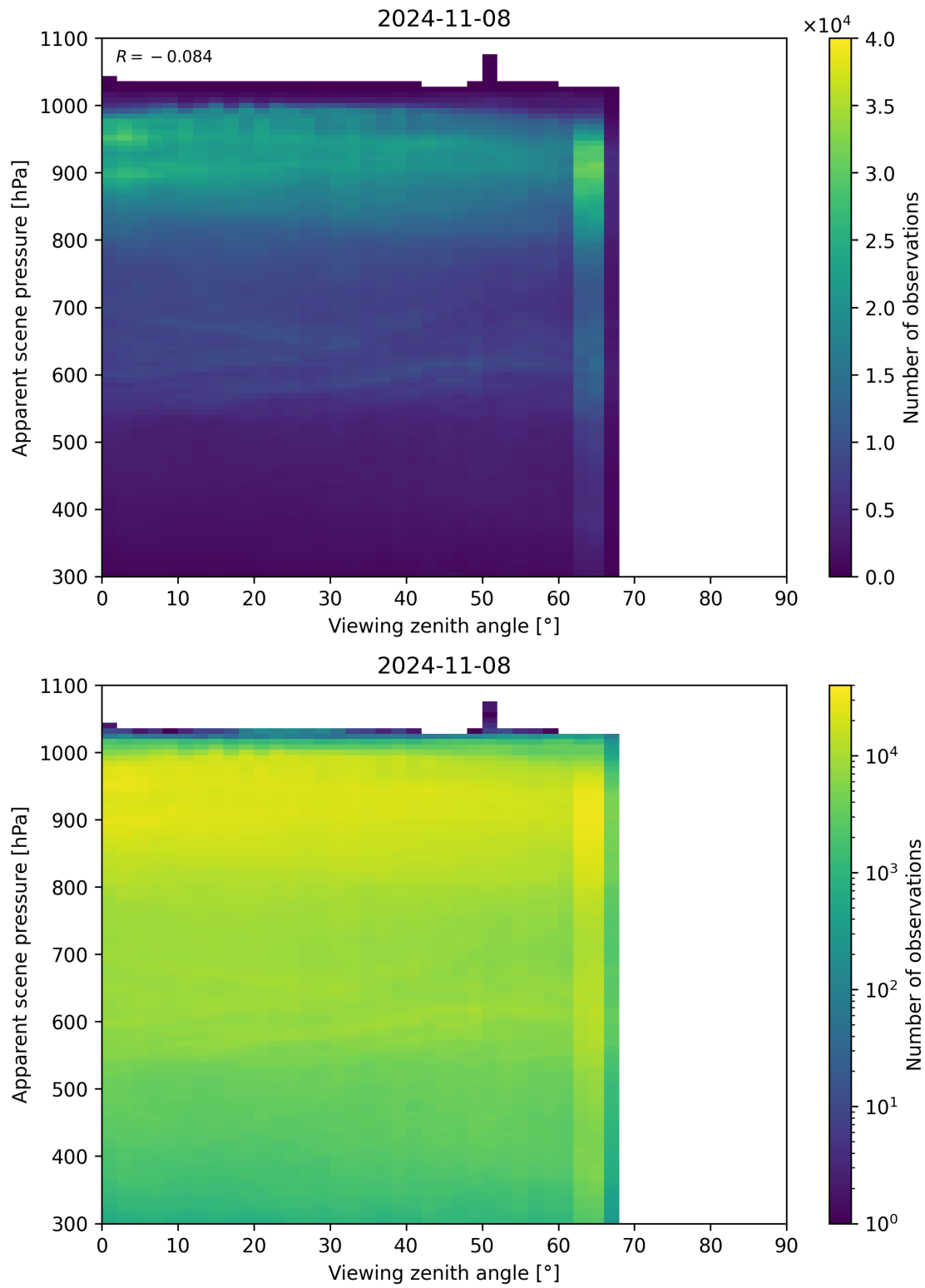
Figure 129: Scatter density plot of “Viewing zenith angle” against “Apparent scene pressure” for 2024-11-07 to 2024-11-09.
