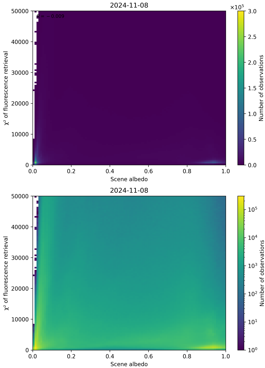
Figure 113: Scatter density plot of “Scene albedo” against “ \chi^2 of fluorescence retrieval” for 2024-11-07 to 2024-11-09.
