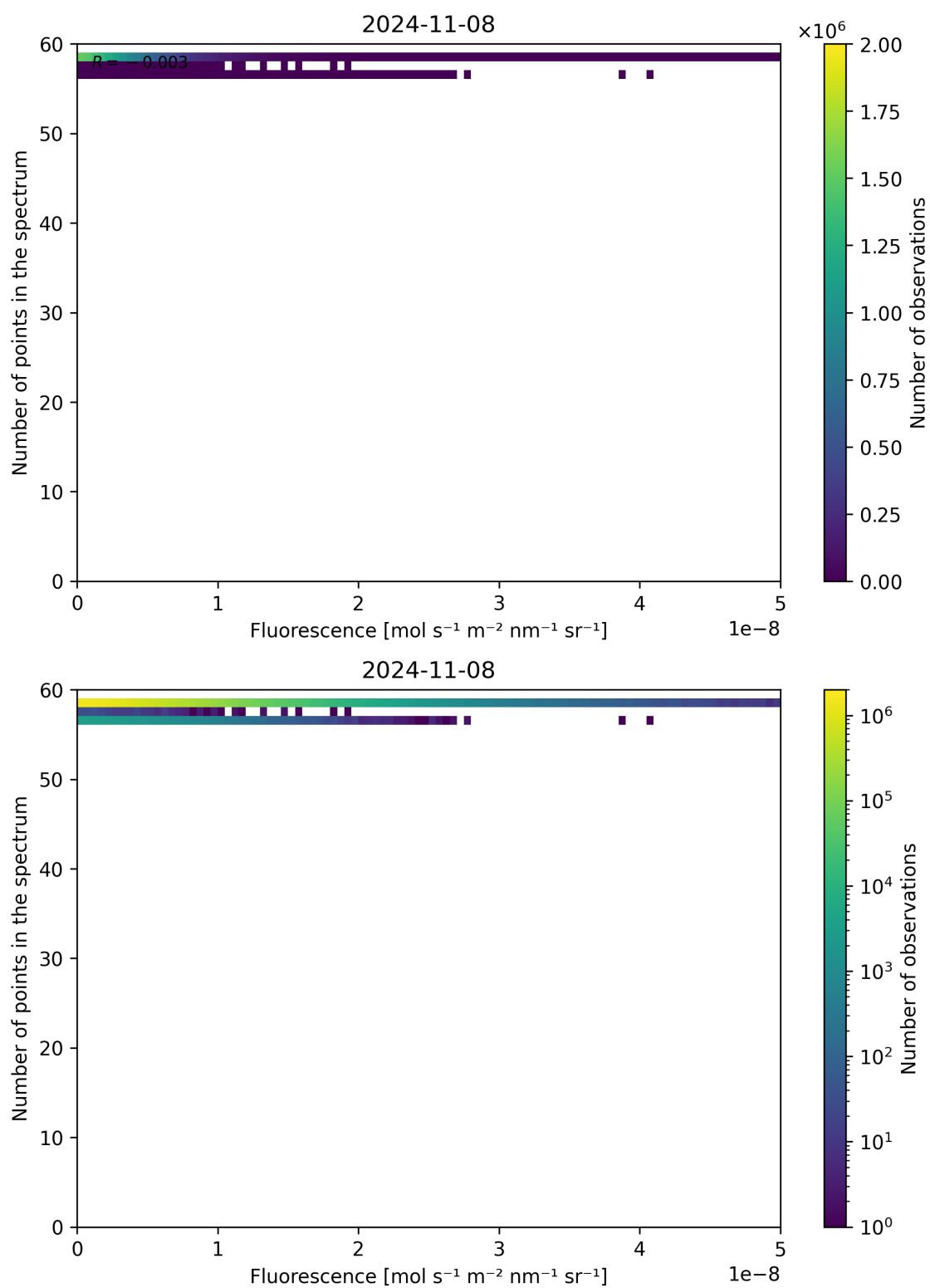
Figure 94: Scatter density plot of “Fluorescence” against “Number of points in the spectrum” for 2024-11-07 to 2024-11-09.
