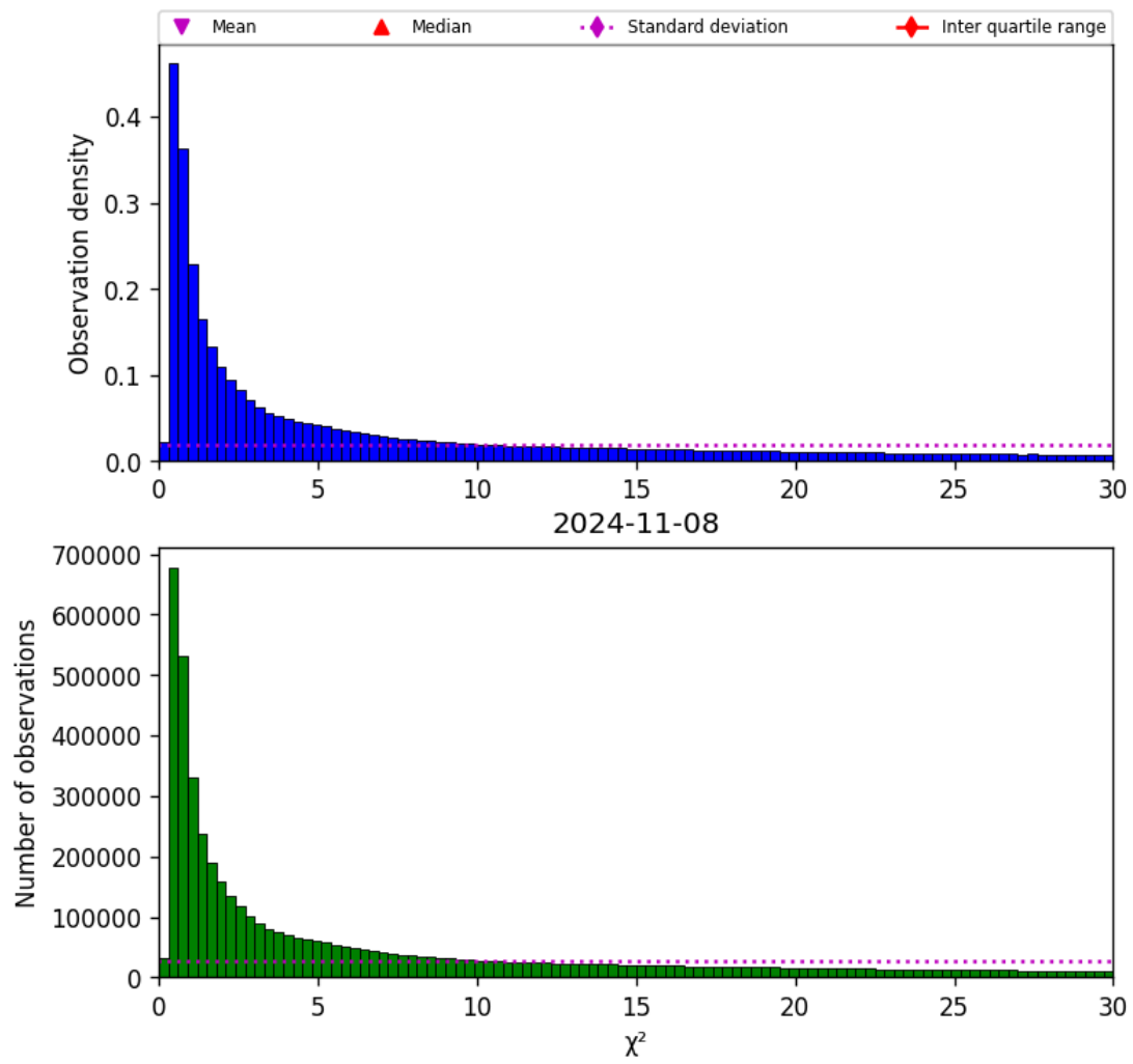
Figure 38: Histogram of “ \chi^2 ” for 2024-11-07 to 2024-11-09
