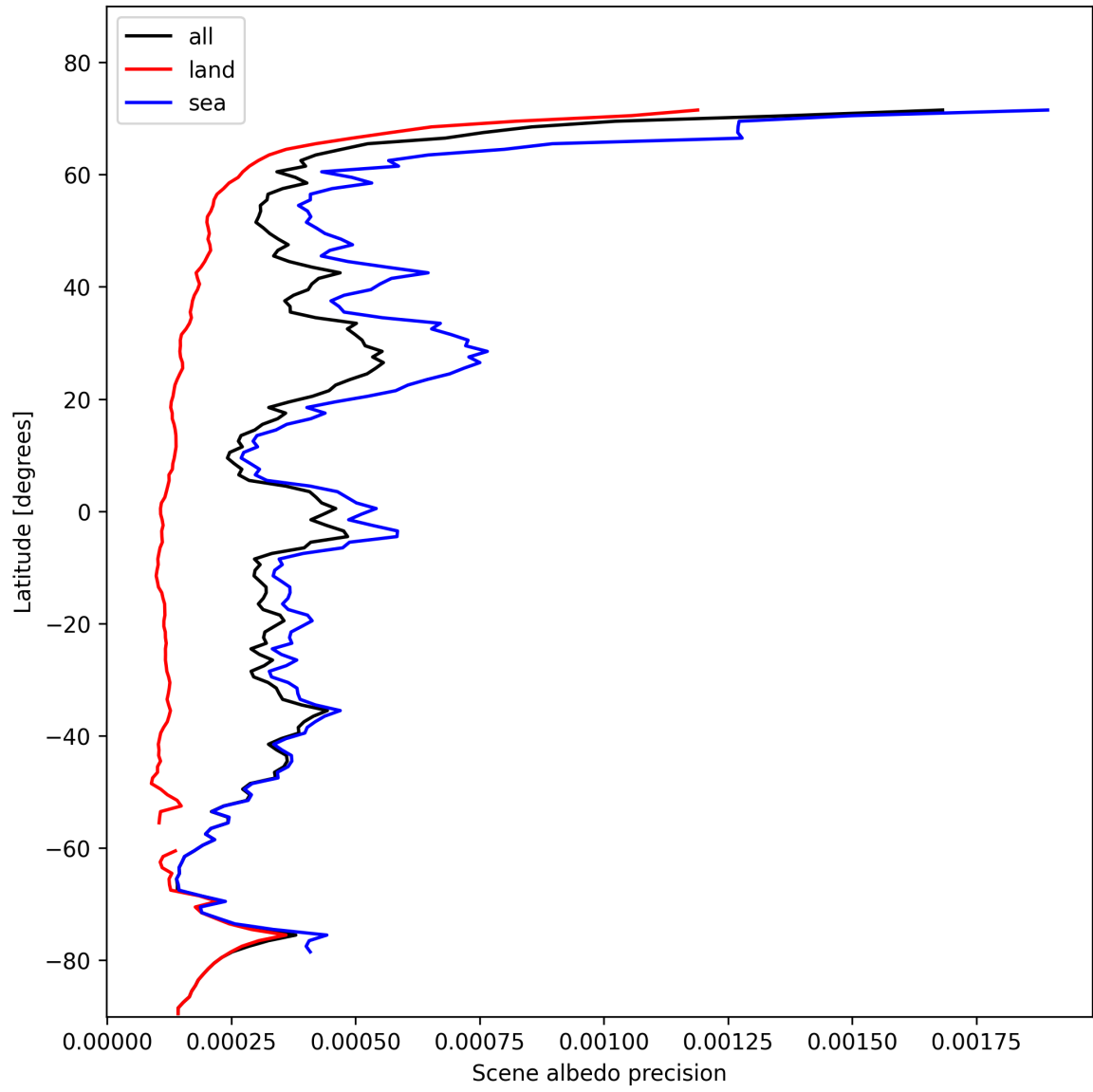
Figure 18: Zonal average of “Scene albedo precision” for 2024-11-07 to 2024-11-09.
