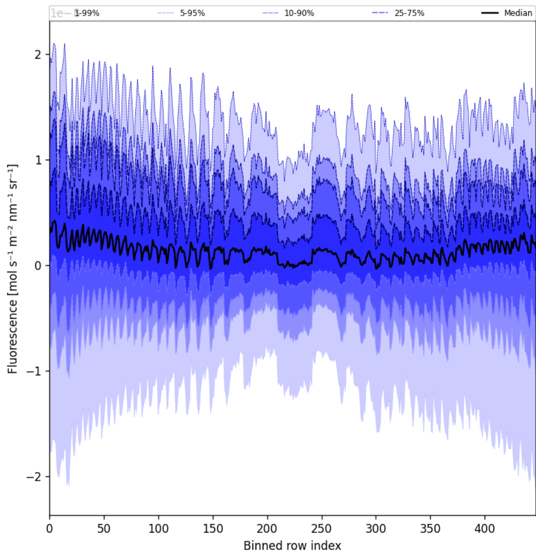
Figure 57: Along track statistics of “Fluorescence” for 2024-11-07 to 2024-11-09
