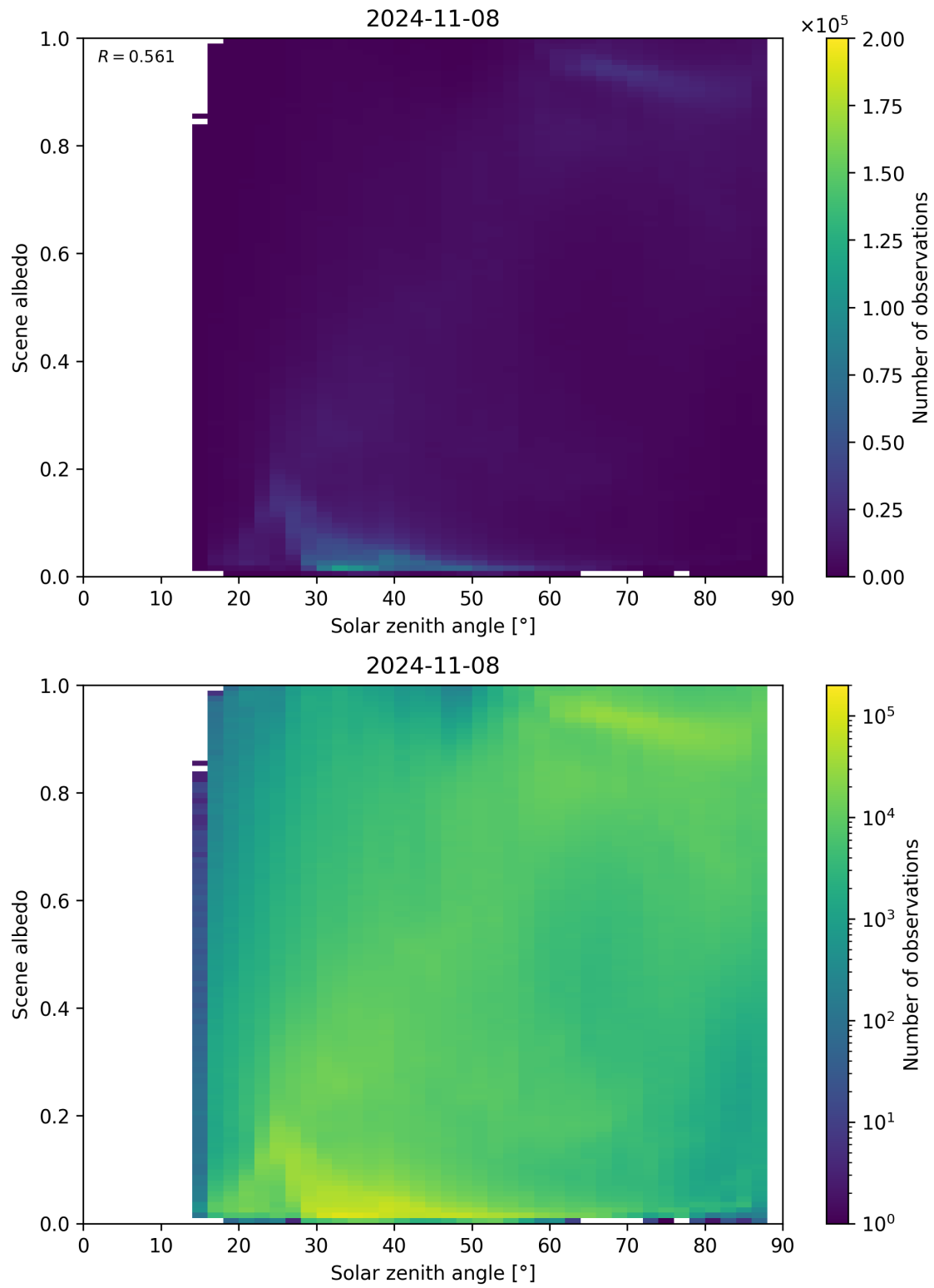
Figure 127: Scatter density plot of “Solar zenith angle” against “Scene albedo” for 2024-11-07 to 2024-11-09.
