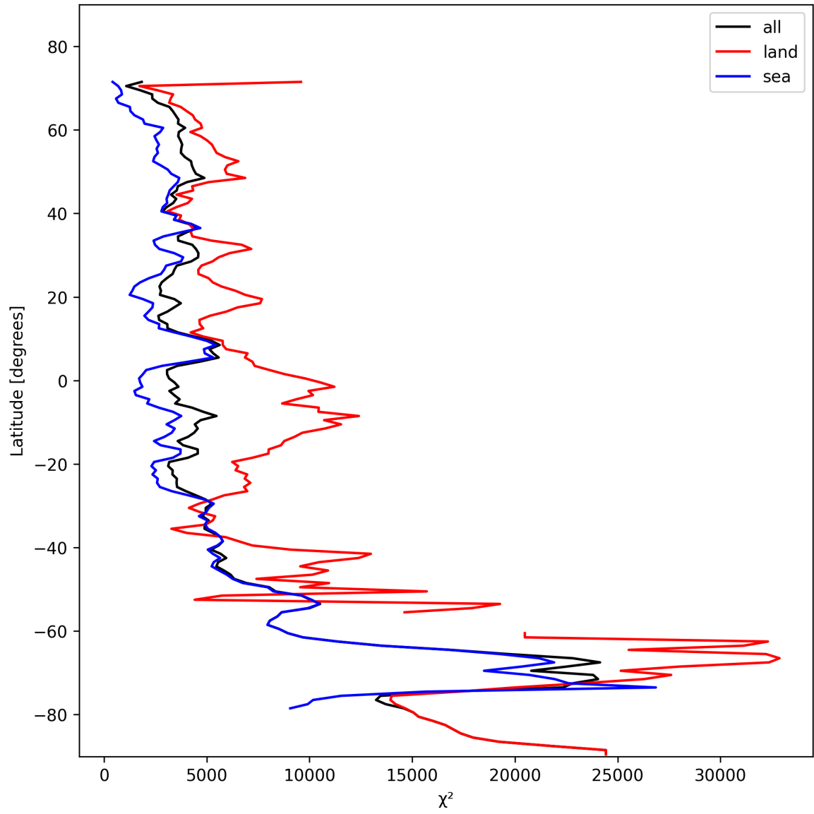
Figure 21: Zonal average of “ \chi^2 ” for 2024-11-07 to 2024-11-09.
