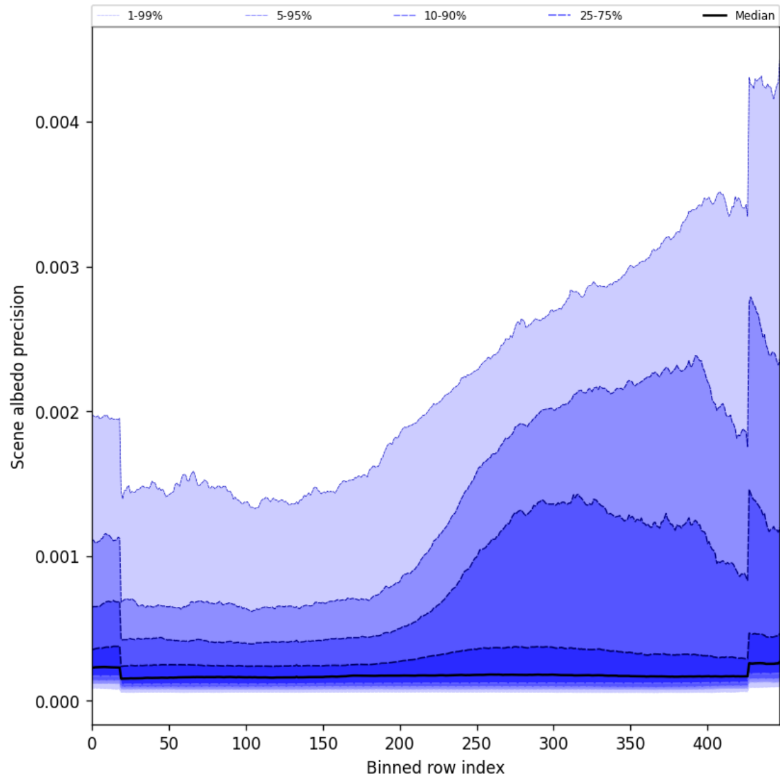
Figure 52: Along track statistics of “Scene albedo precision” for 2024-11-07 to 2024-11-09
