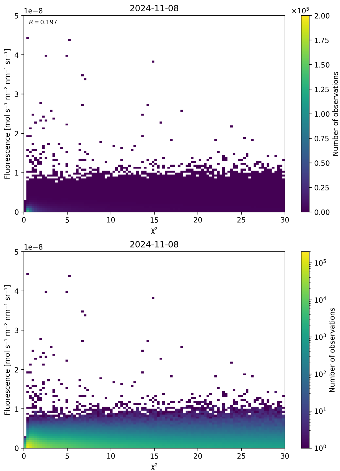
Figure 70: Scatter density plot of “ \chi^2 ” against “Fluorescence” for 2024-11-07 to 2024-11-09.
