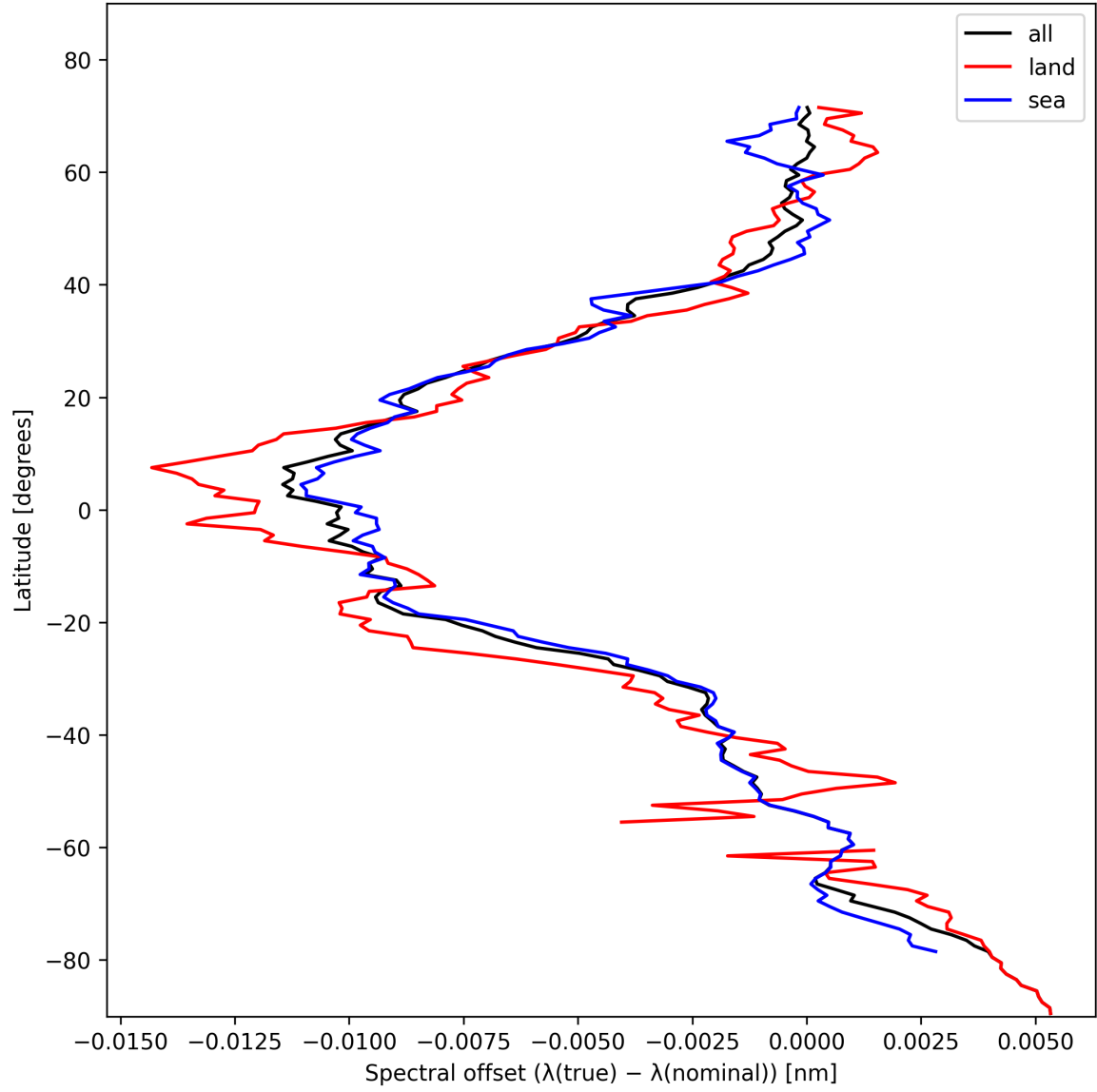
Figure 28: Zonal average of “Spectral offset ( \lambda_{\text{true}} - \lambda_{\text{nominal}} )” for 2024-11-07 to 2024-11-09.
