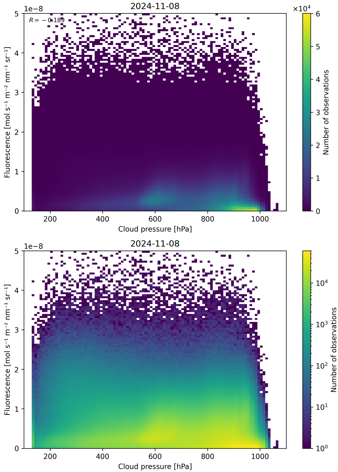
Figure 88: Scatter density plot of “Cloud pressure” against “Fluorescence” for 2024-11-07 to 2024-11-09.
