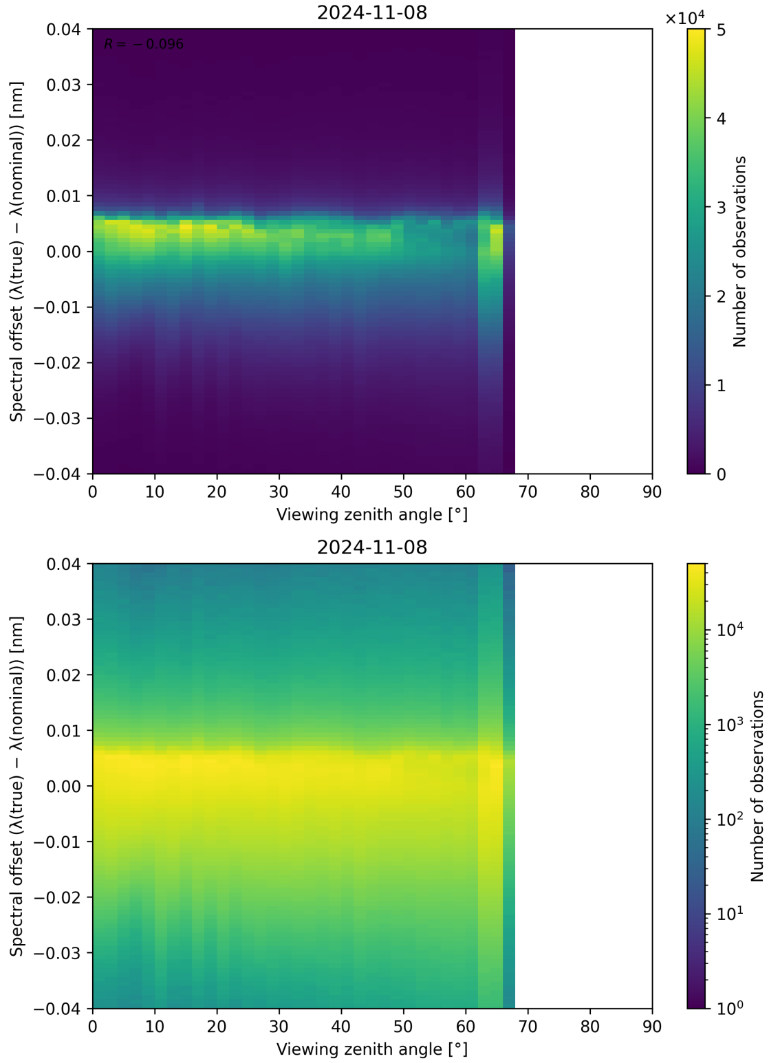
Figure 140: Scatter density plot of “Viewing zenith angle” against “Spectral offset ( \lambda_{\text{true}} - \lambda_{\text{nominal}} )” for 2024-11-07 to 2024-11-09.
