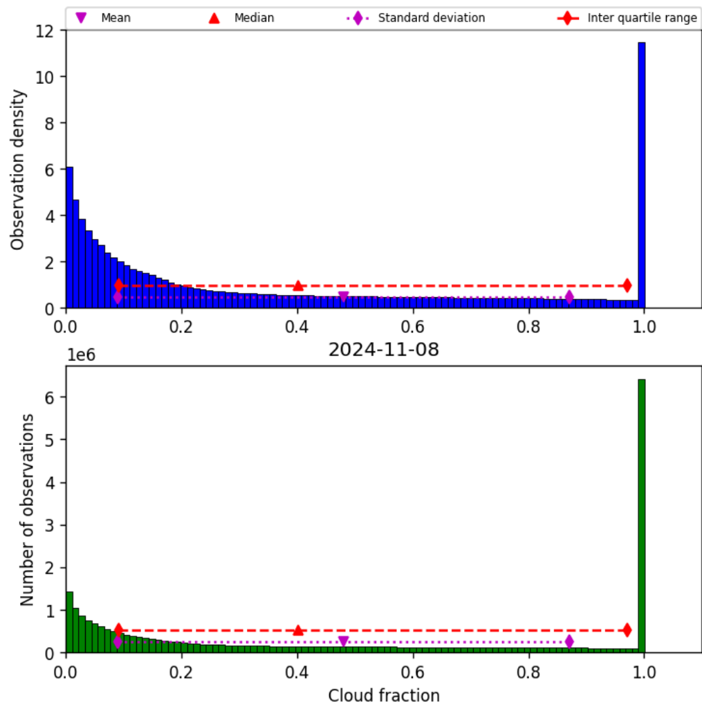
Figure 32: Histogram of “Cloud fraction” for 2024-11-07 to 2024-11-09
