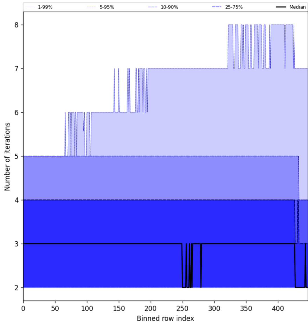
Figure 56: Along track statistics of “Number of iterations” for 2024-11-07 to 2024-11-09
