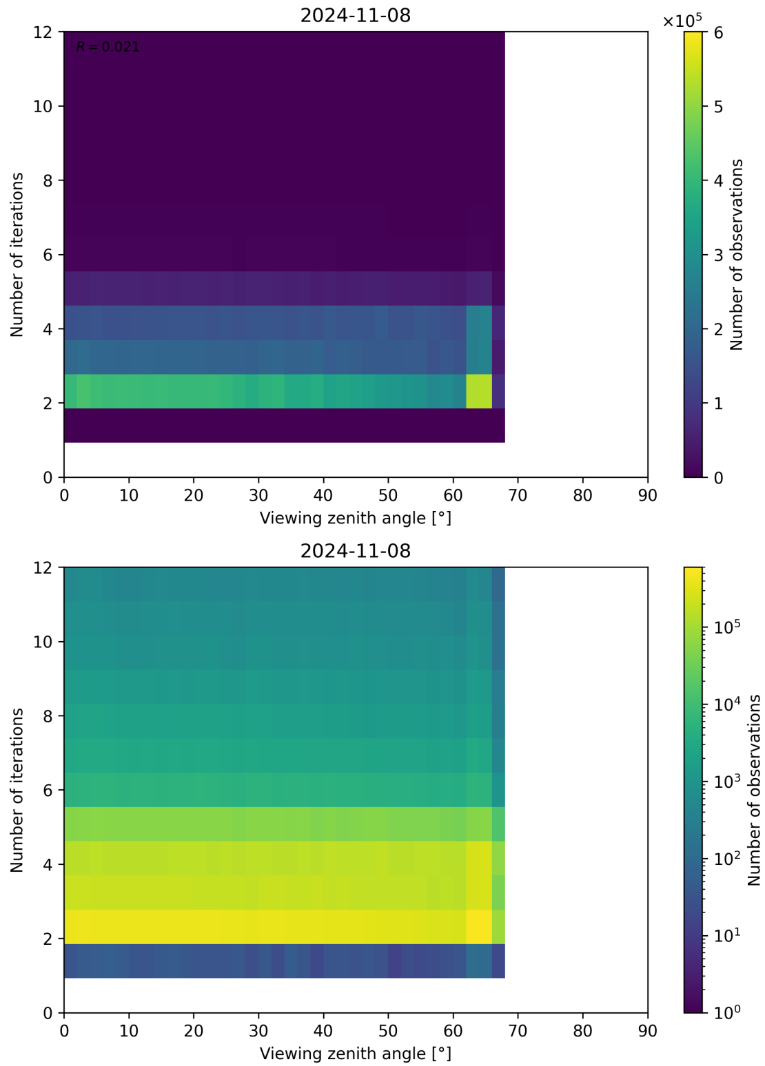
Figure 136: Scatter density plot of “Viewing zenith angle” against “Number of iterations” for 2024-11-07 to 2024-11-09.
