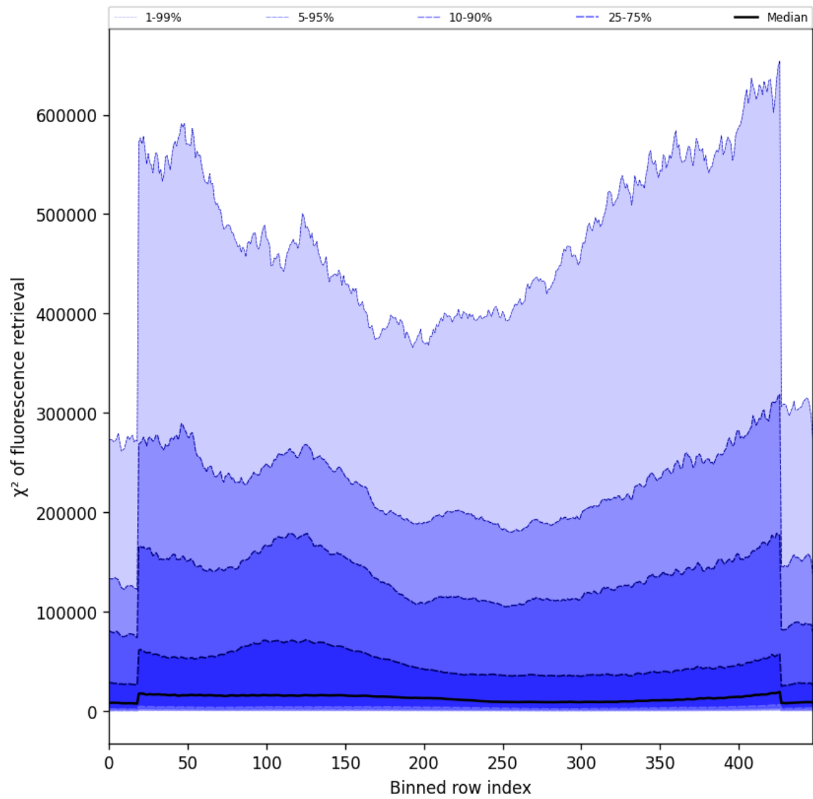
Figure 59: Along track statistics of “ \chi^2 of fluorescence retrieval” for 2024-11-07 to 2024-11-09
