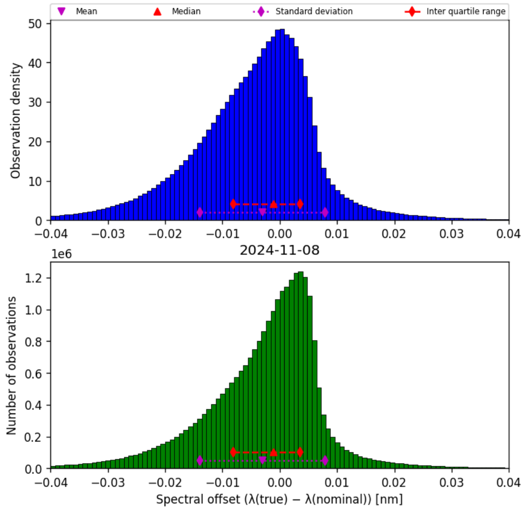
Figure 45: Histogram of “Spectral offset ( \lambda_{\text{true}} - \lambda_{\text{nominal}} )” for 2024-11-07 to 2024-11-09
