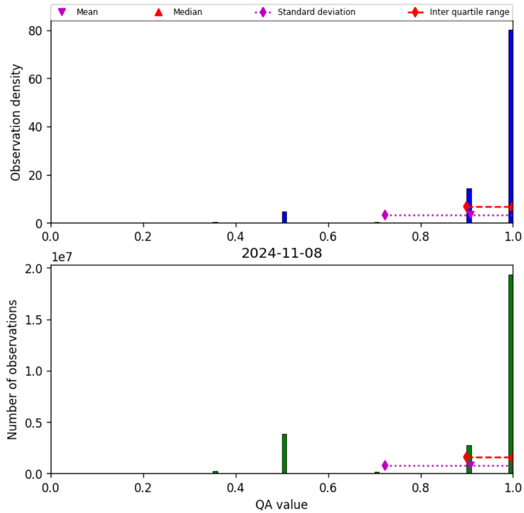
Figure 29: Histogram of “QA value” for 2024-11-07 to 2024-11-09
