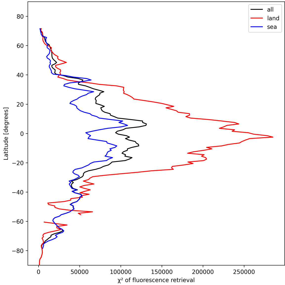
Figure 25: Zonal average of “ \chi^2 of fluorescence retrieval” for 2024-11-07 to 2024-11-09.
