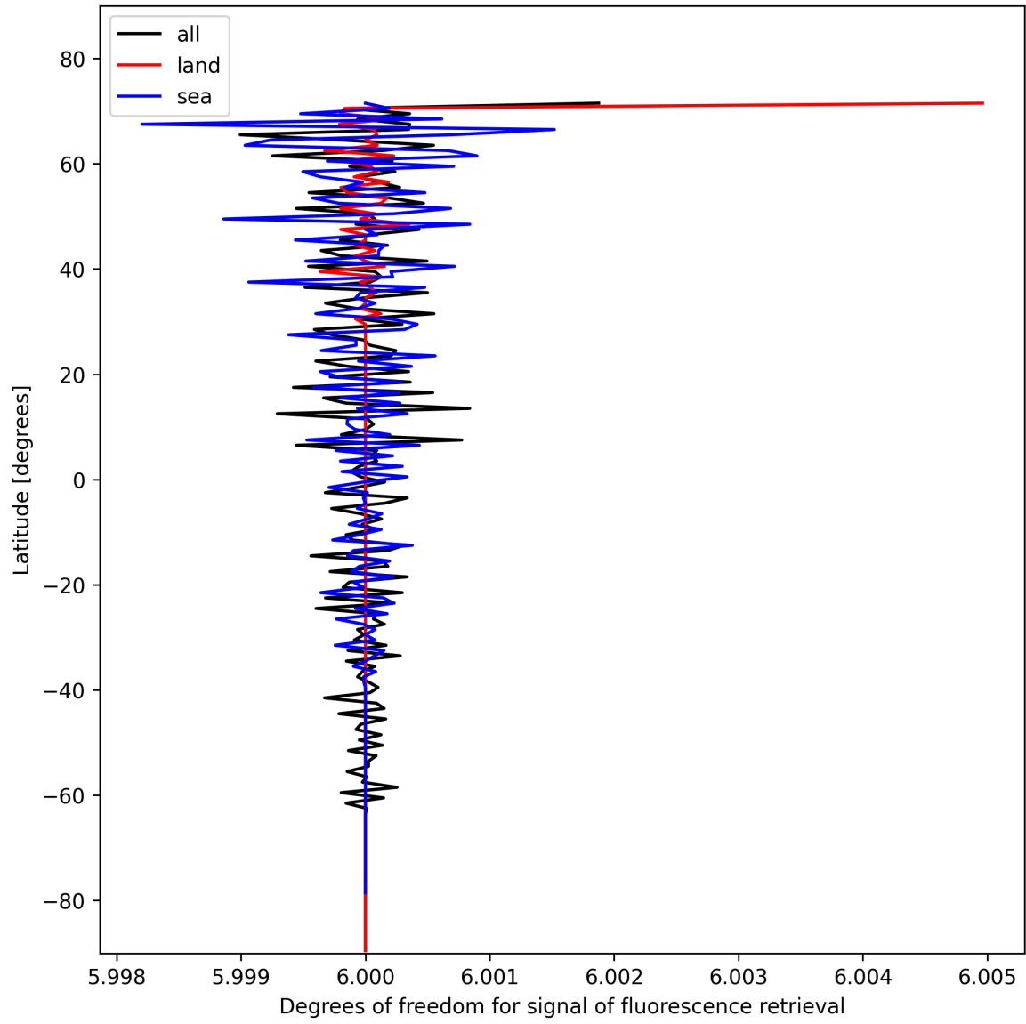
Figure 26: Zonal average of “Degrees of freedom for signal of fluorescence retrieval” for 2024-11-07 to 2024-11-09.
