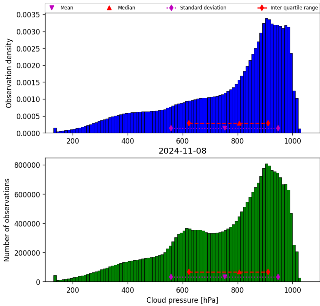
Figure 30: Histogram of “Cloud pressure” for 2024-11-07 to 2024-11-09
