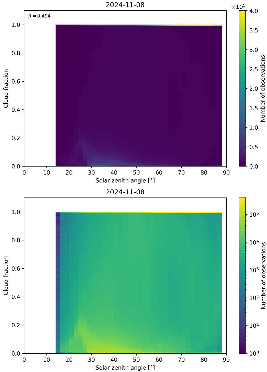
Figure 121: Scatter density plot of “Solar zenith angle” against “Cloud fraction” for 2024-11-07 to 2024-11-09.
