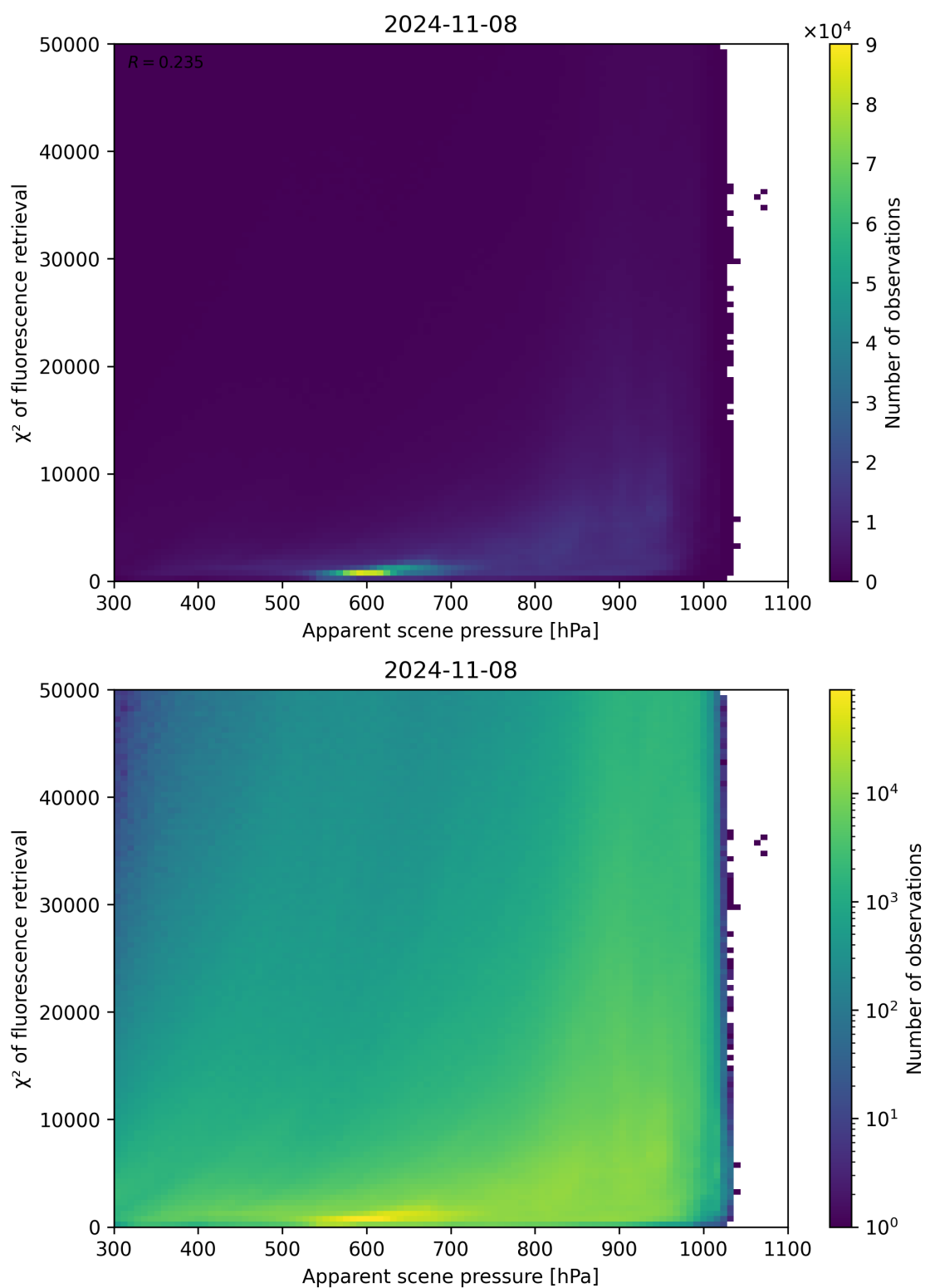
Figure 64: Scatter density plot of “Apparent scene pressure” against “ \chi^2 of fluorescence retrieval” for 2024-11-07 to 2024-11-09.
