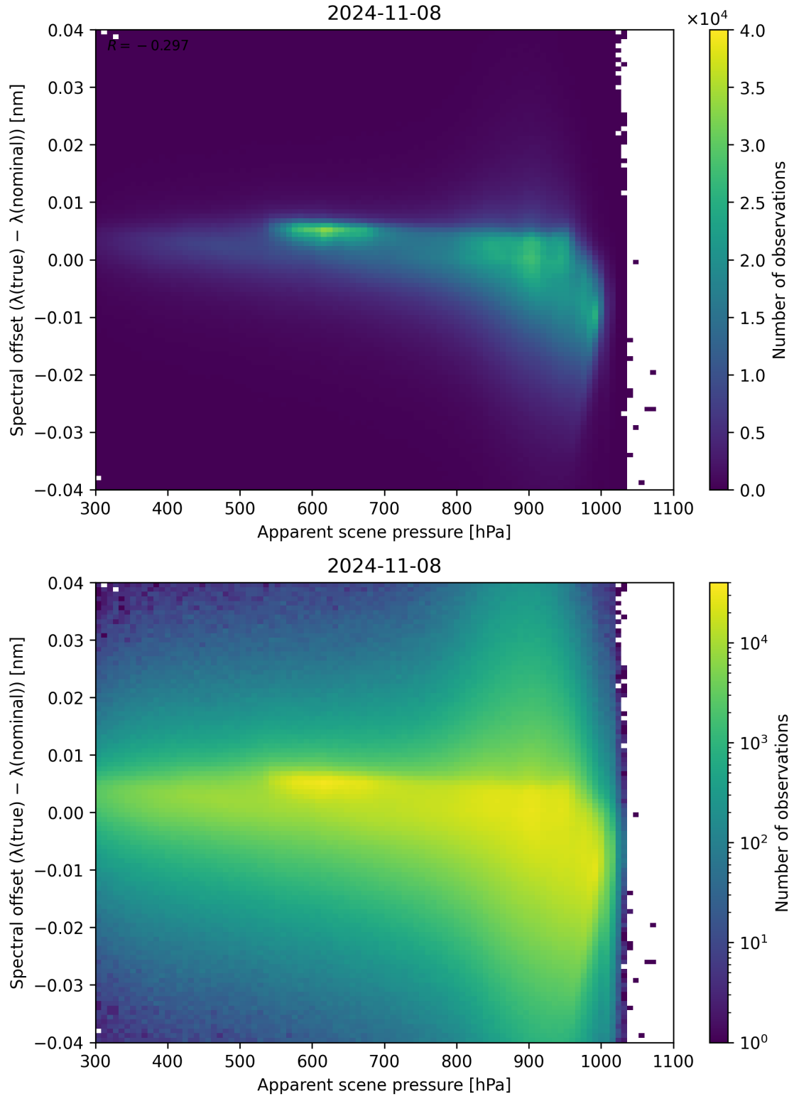
Figure 68: Scatter density plot of “Apparent scene pressure” against “Spectral offset ( \lambda_{\text{true}} - \lambda_{\text{nominal}} )” for 2024-11-07 to 2024-11-09.
