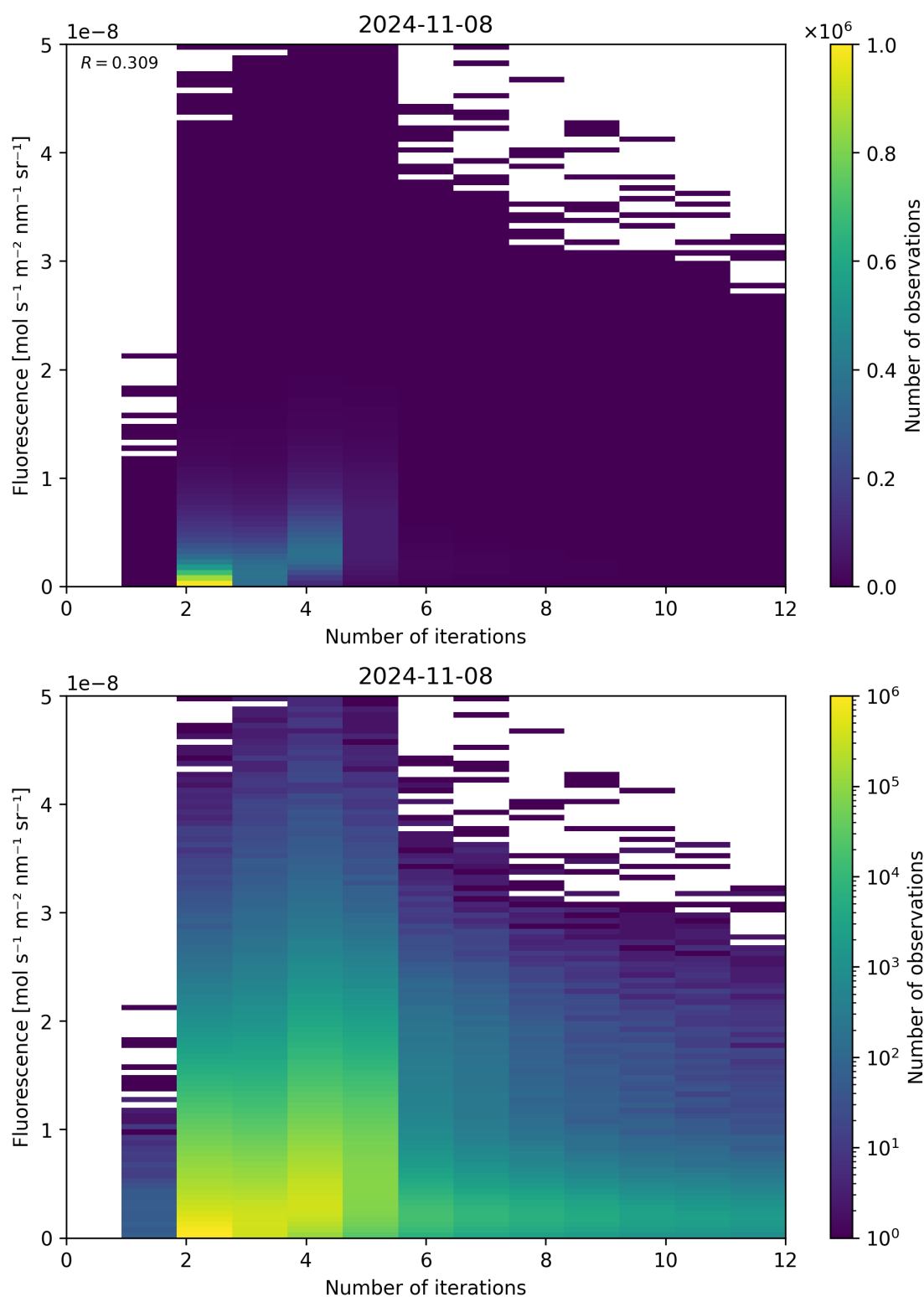
Figure 107: Scatter density plot of “Number of iterations” against “Fluorescence” for 2024-11-07 to 2024-11-09.
