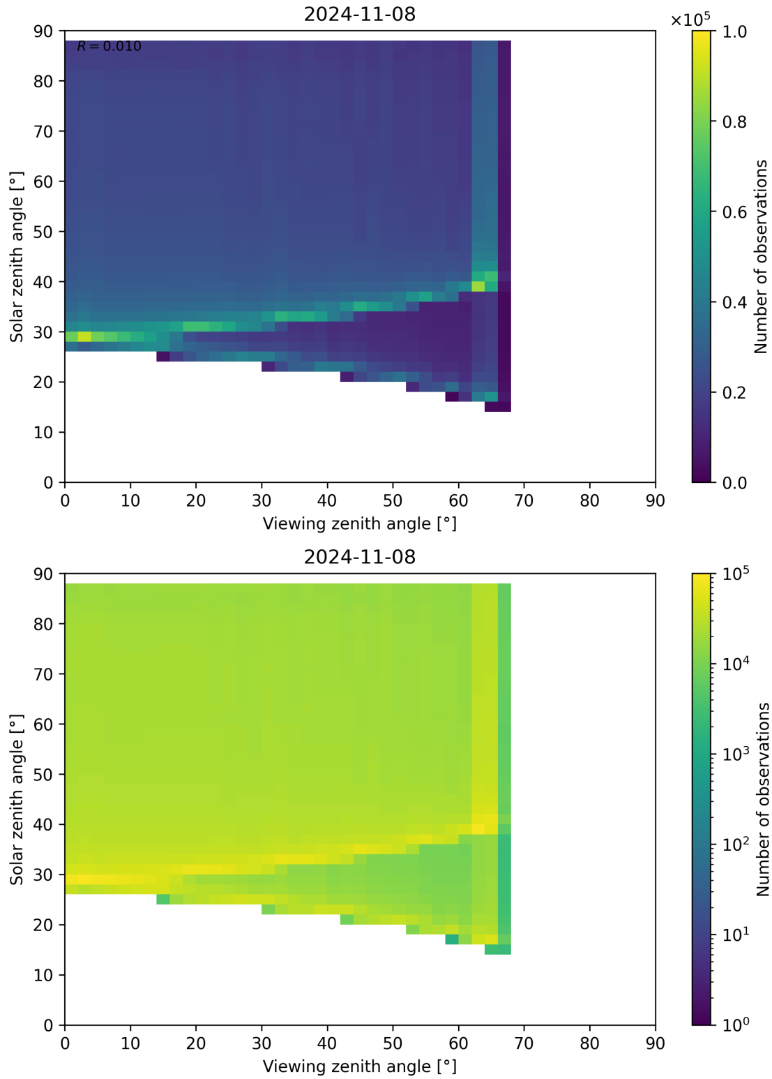
Figure 139: Scatter density plot of “Viewing zenith angle” against “Solar zenith angle” for 2024-11-07 to 2024-11-09.
