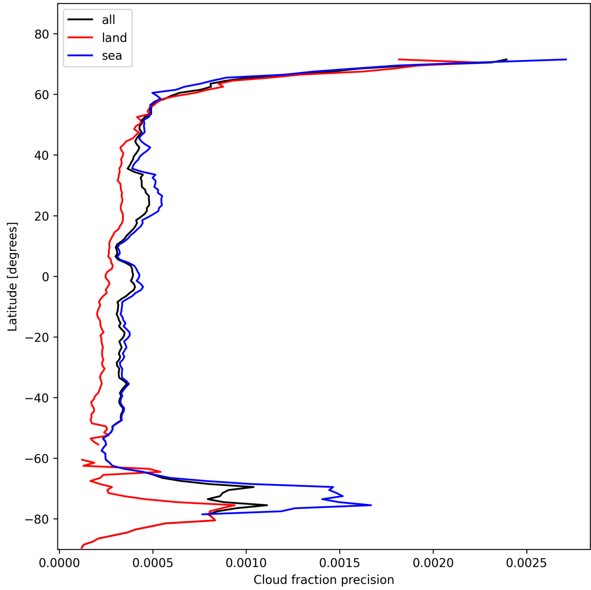
Figure 16: Zonal average of “Cloud fraction precision” for 2024-11-07 to 2024-11-09.
