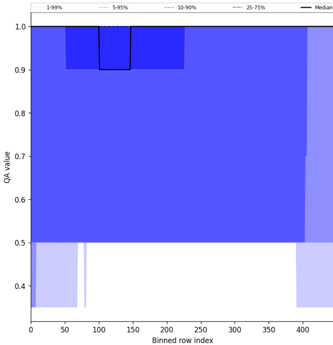
Figure 46: Along track statistics of “QA value” for 2024-11-07 to 2024-11-09
