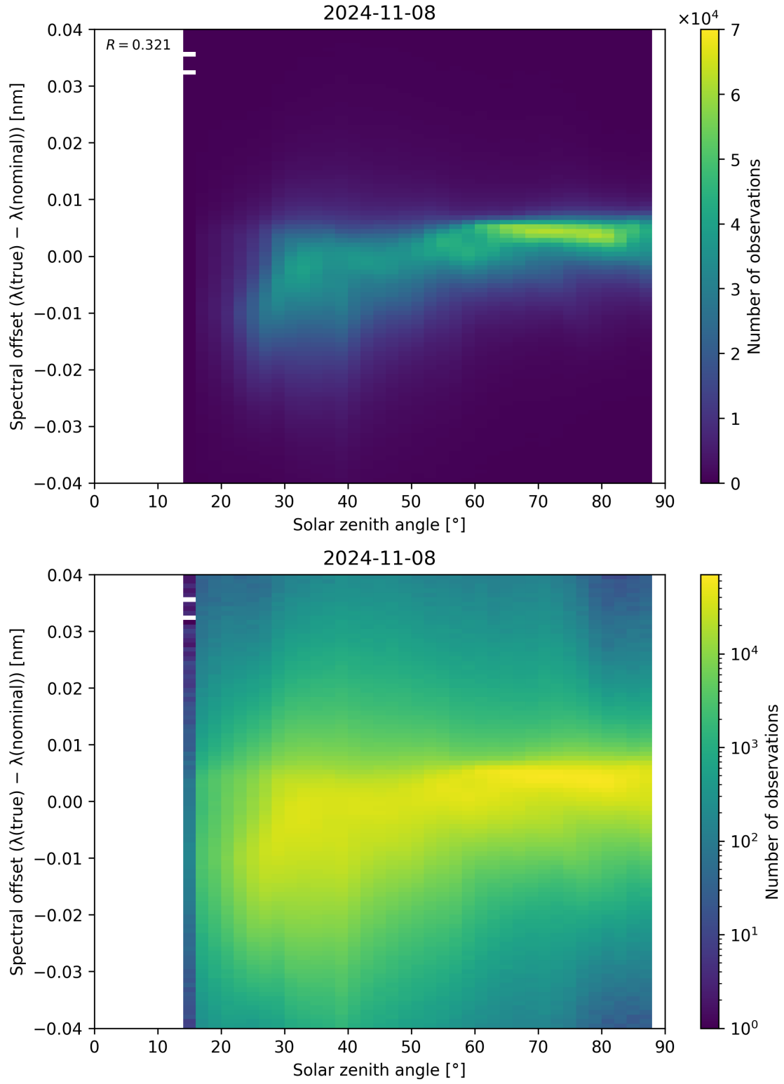
Figure 128: Scatter density plot of “Solar zenith angle” against “Spectral offset ( \lambda_{\text{true}} - \lambda_{\text{nominal}} )” for 2024-11-07 to 2024-11-09.
