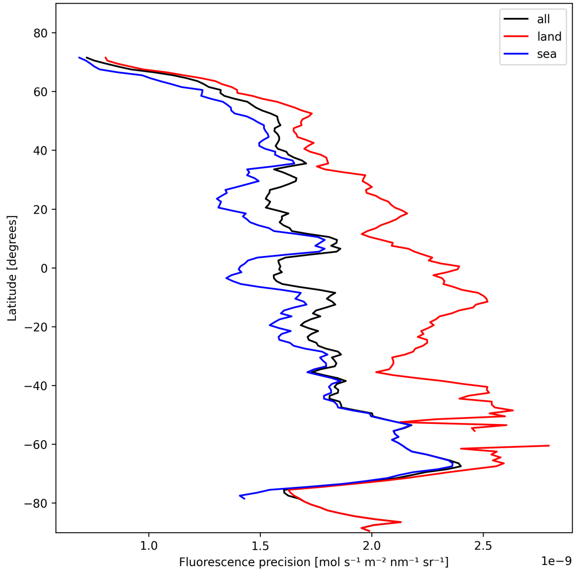
Figure 24: Zonal average of “Fluorescence precision” for 2024-11-07 to 2024-11-09.
