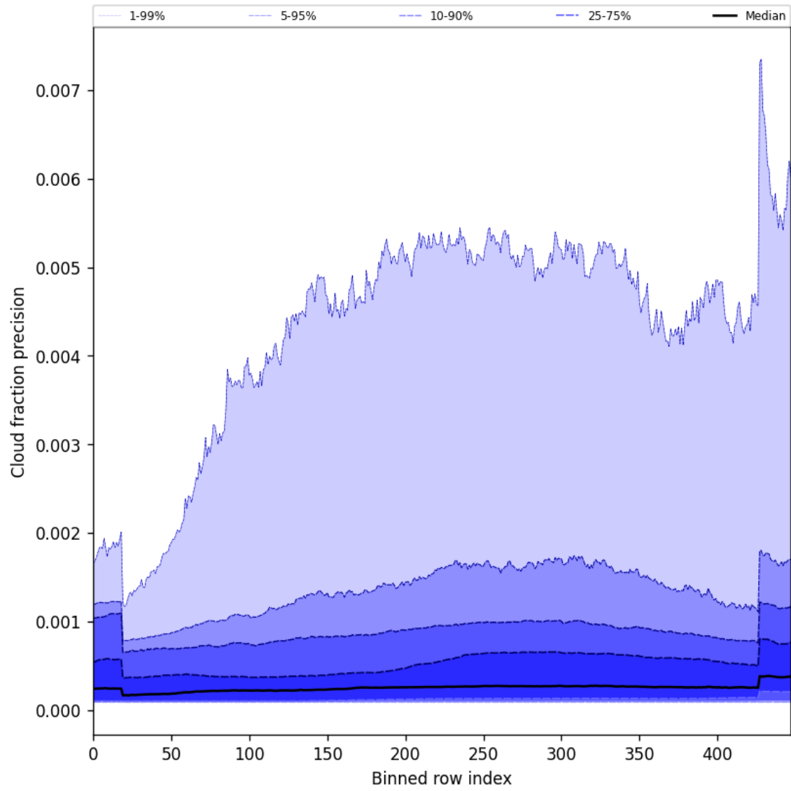
Figure 50: Along track statistics of “Cloud fraction precision” for 2024-11-07 to 2024-11-09
