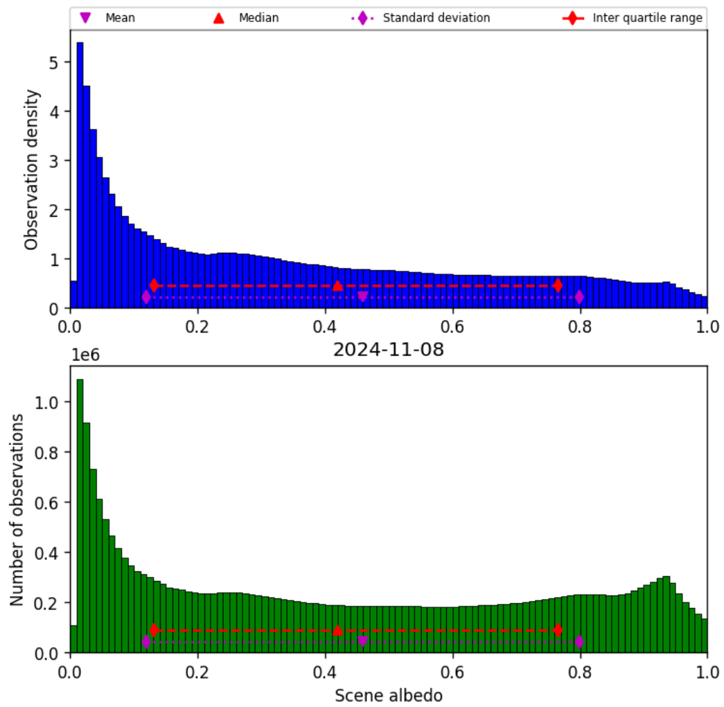
Figure 34: Histogram of “Scene albedo” for 2024-11-07 to 2024-11-09
