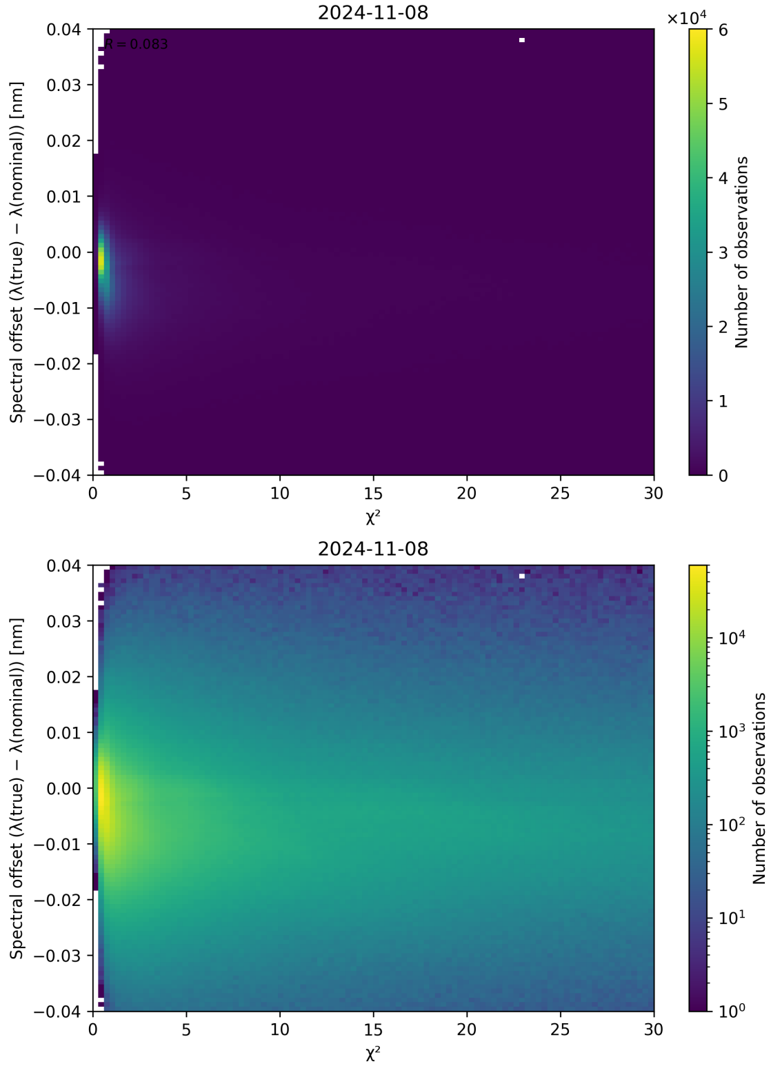
Figure 75: Scatter density plot of “ \chi^2 ” against “Spectral offset ( \lambda_{\text{true}} - \lambda_{\text{nominal}} )” for 2024-11-07 to 2024-11-09.
