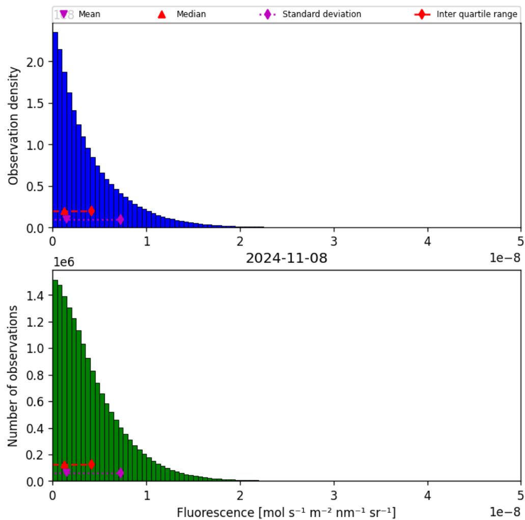
Figure 40: Histogram of “Fluorescence” for 2024-11-07 to 2024-11-09
