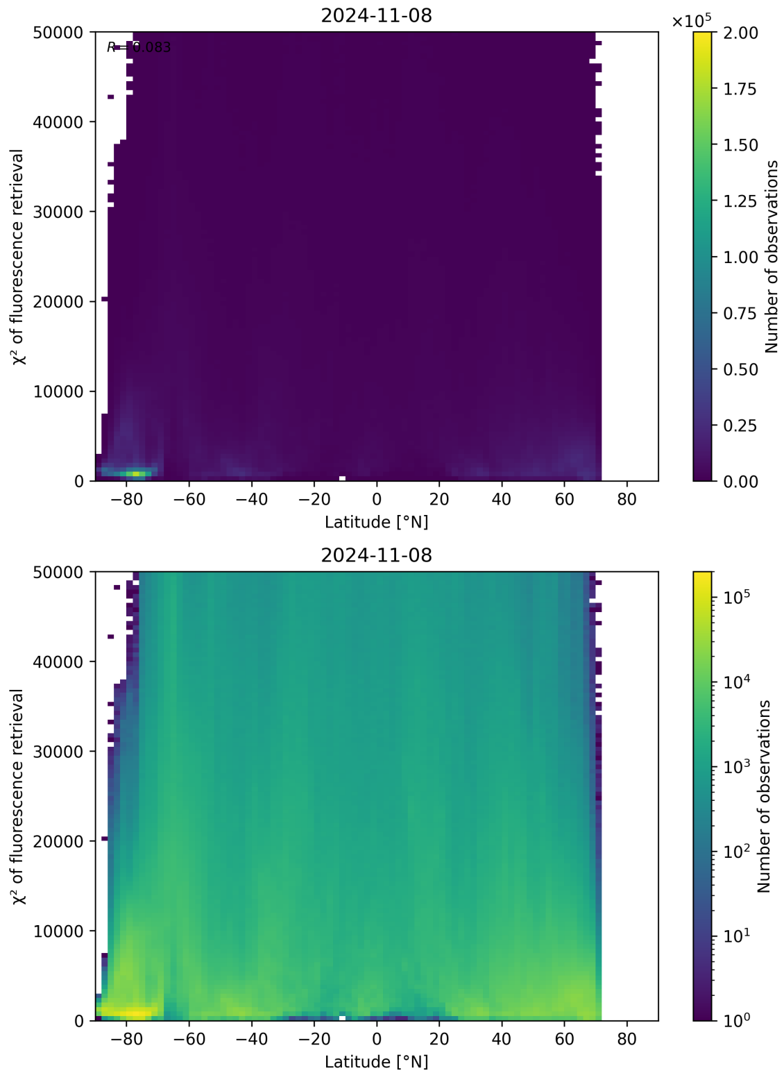
Figure 98: Scatter density plot of “Latitude” against “ \chi^2 of fluorescence retrieval” for 2024-11-07 to 2024-11-09.
