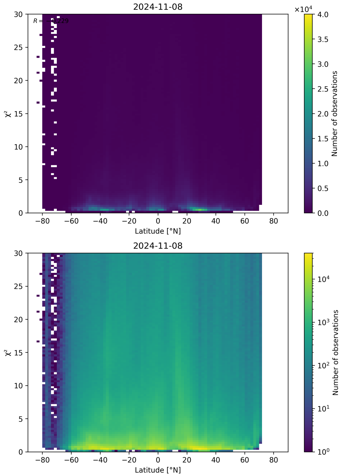
Figure 97: Scatter density plot of “Latitude” against “ \chi^2 ” for 2024-11-07 to 2024-11-09.
