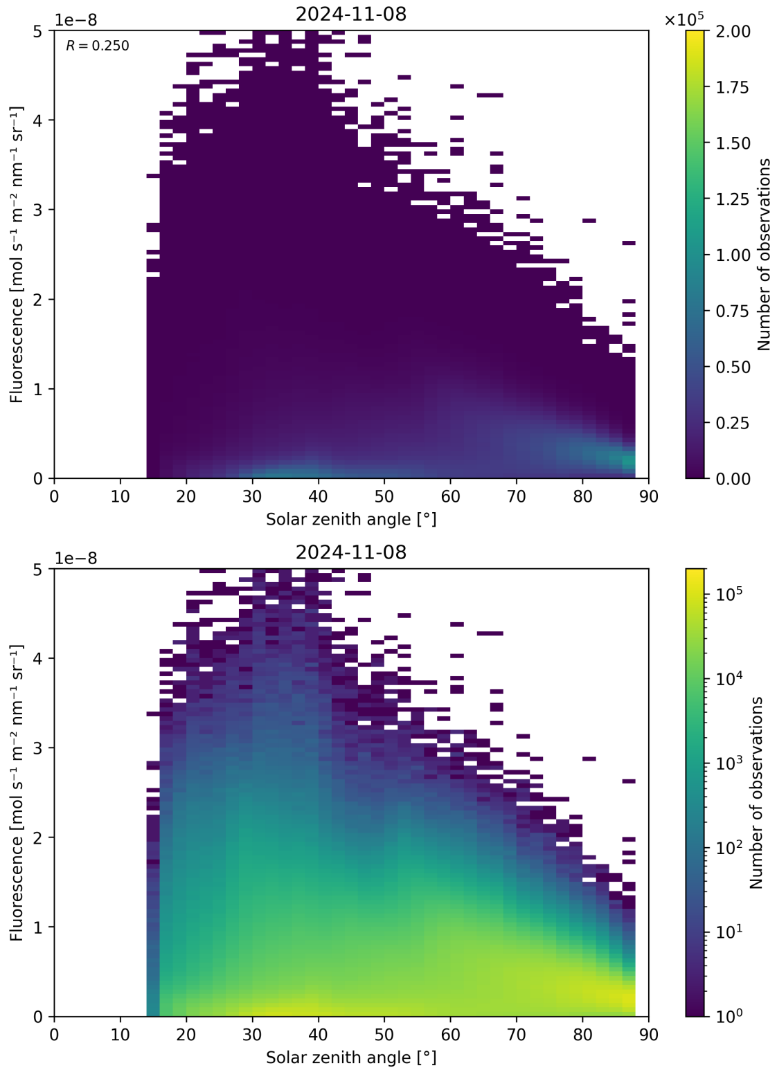
Figure 123: Scatter density plot of “Solar zenith angle” against “Fluorescence” for 2024-11-07 to 2024-11-09.
