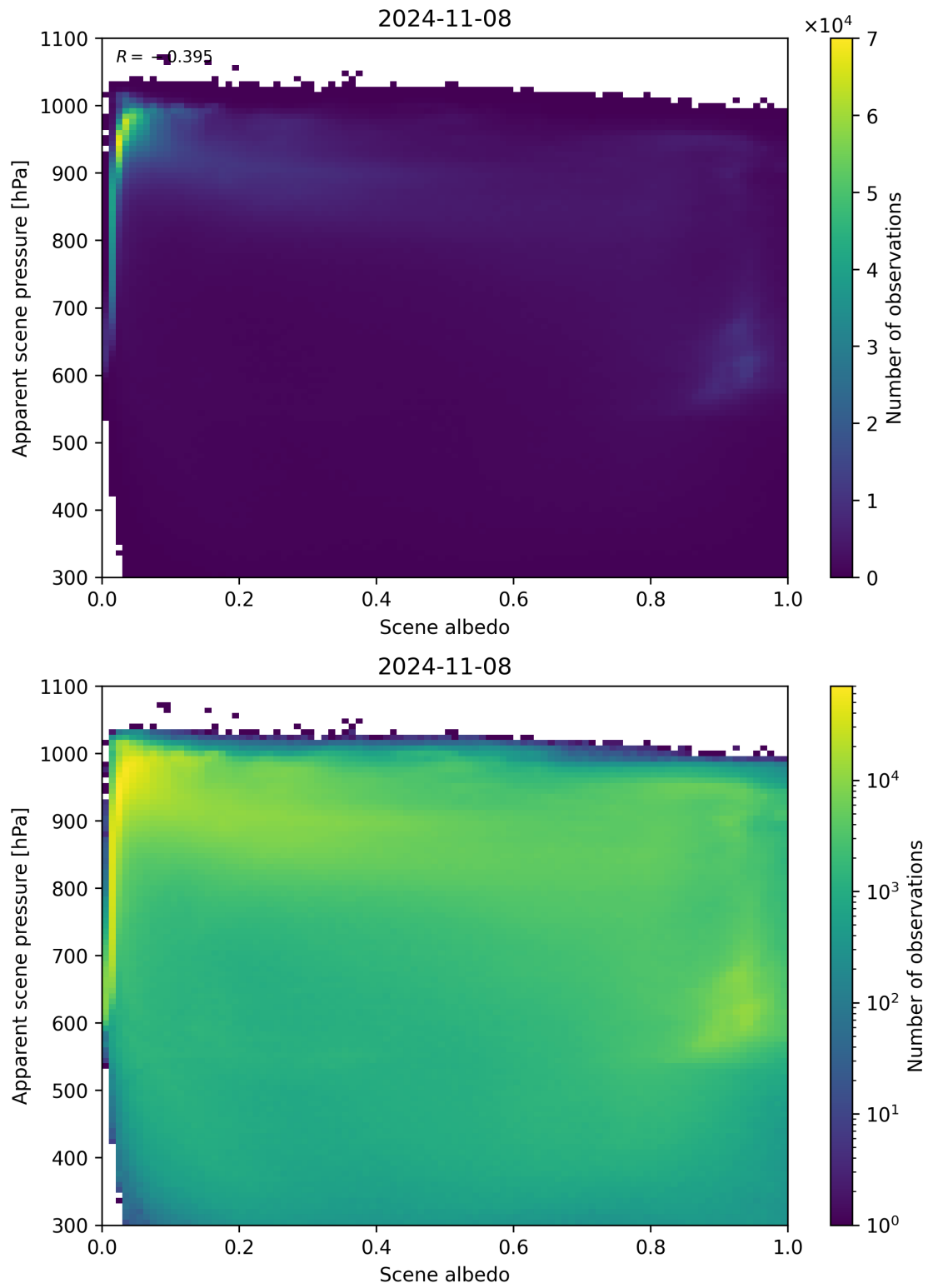
Figure 111: Scatter density plot of “Scene albedo” against “Apparent scene pressure” for 2024-11-07 to 2024-11-09.
