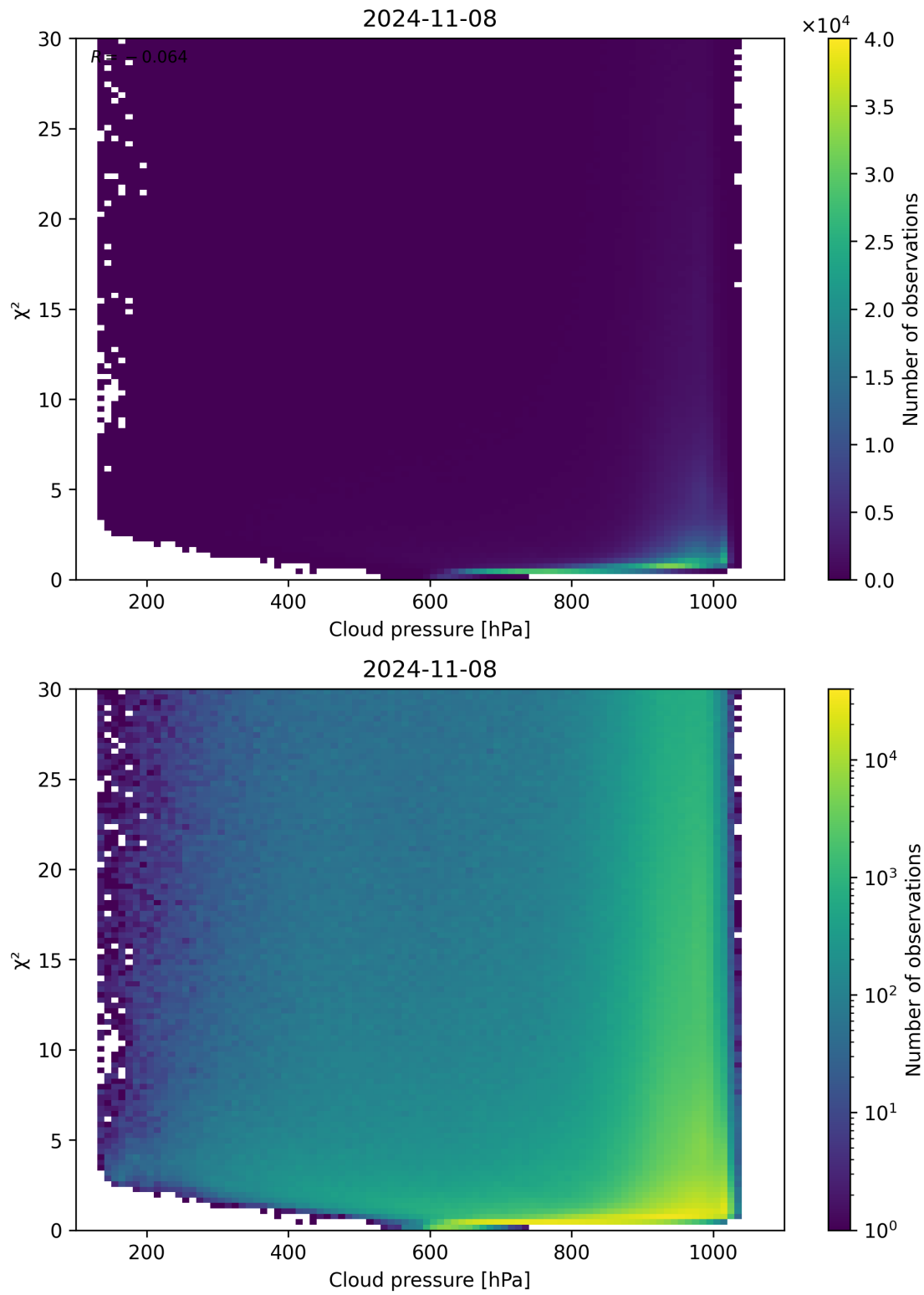
Figure 85: Scatter density plot of “Cloud pressure” against “ \chi^2 ” for 2024-11-07 to 2024-11-09.
