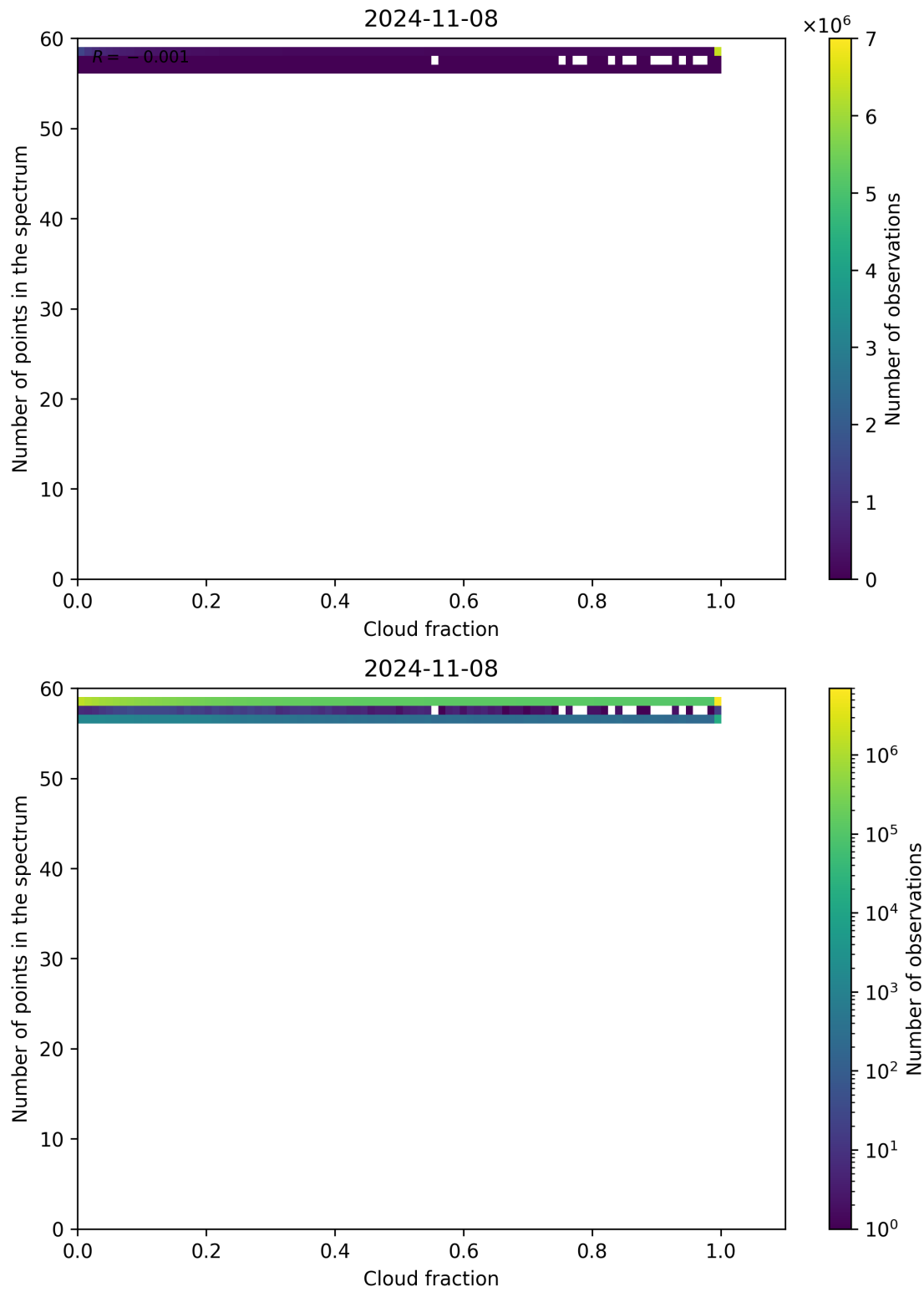
Figure 81: Scatter density plot of “Cloud fraction” against “Number of points in the spectrum” for 2024-11-07 to 2024-11-09.
