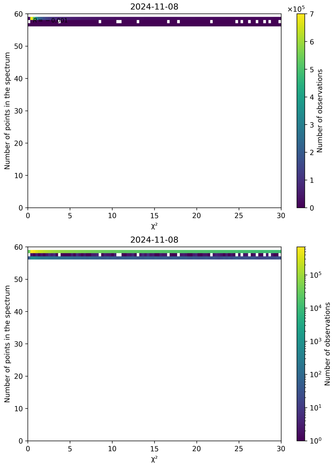
Figure 74: Scatter density plot of “ \chi^2 ” against “Number of points in the spectrum” for 2024-11-07 to 2024-11-09.
