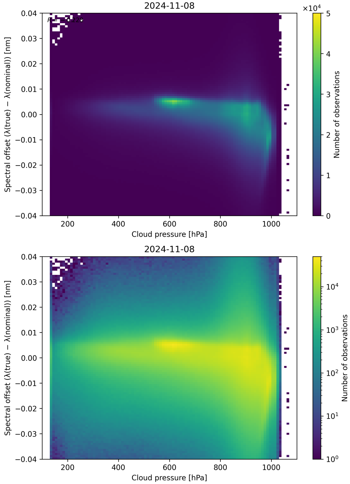
Figure 92: Scatter density plot of “Cloud pressure” against “Spectral offset ( \lambda_{\text{true}} - \lambda_{\text{nominal}} )” for 2024-11-07 to 2024-11-09.
