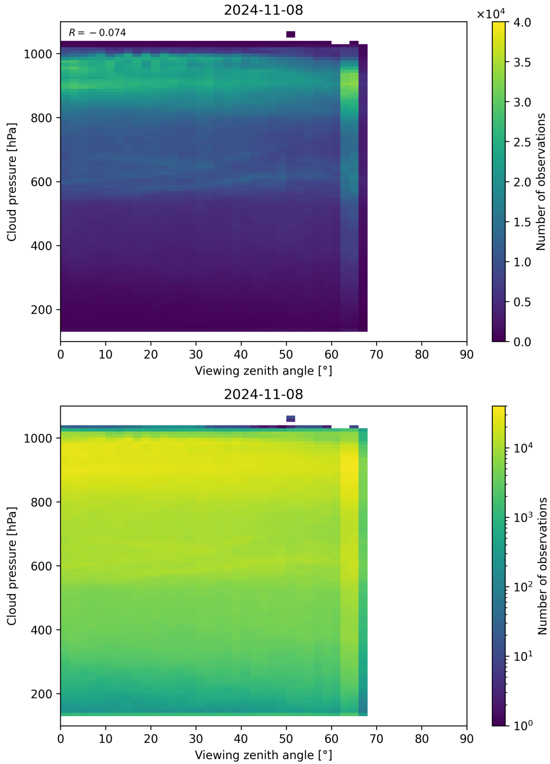
Figure 133: Scatter density plot of “Viewing zenith angle” against “Cloud pressure” for 2024-11-07 to 2024-11-09.
