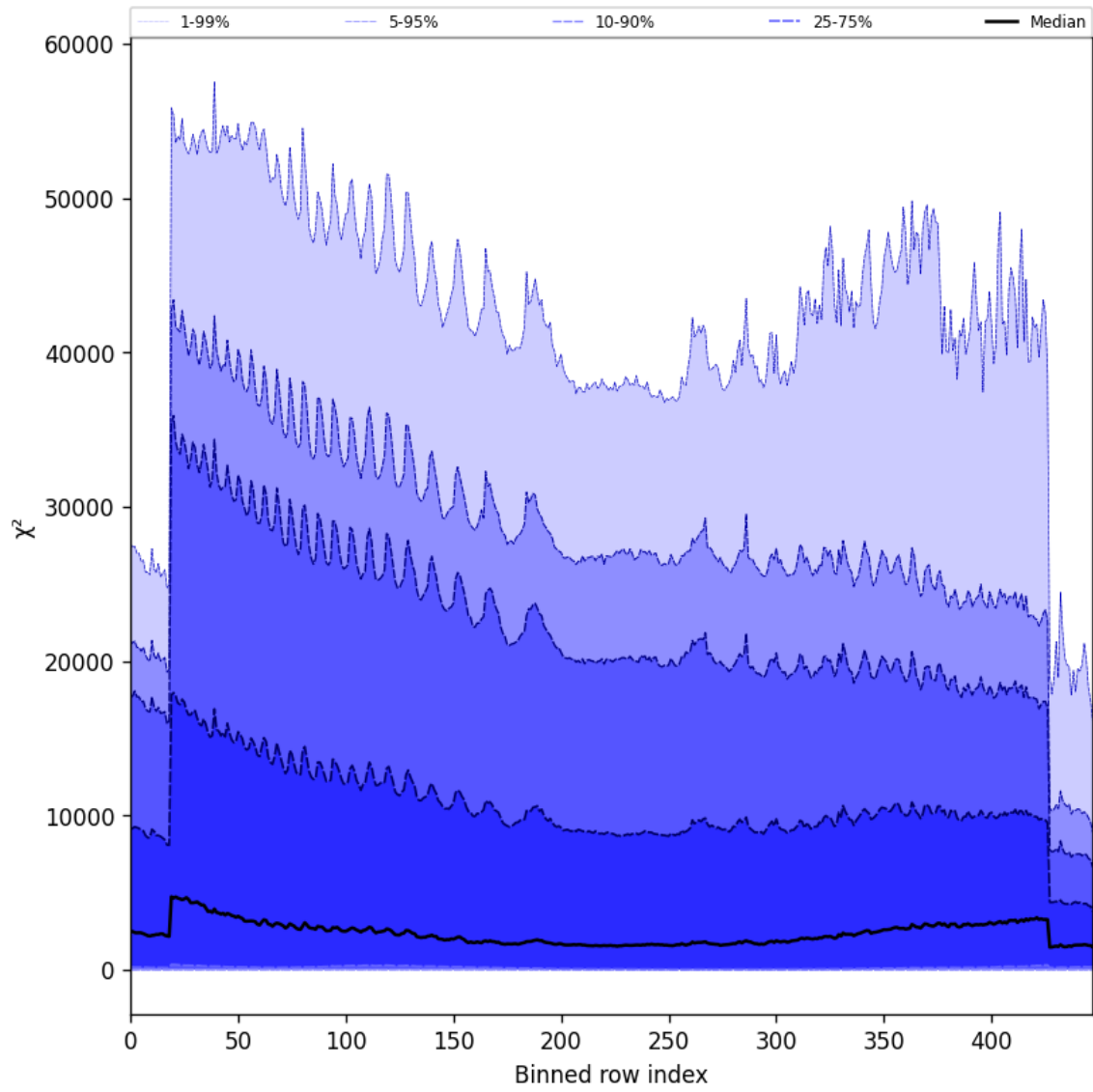
Figure 55: Along track statistics of “ \chi^2 ” for 2024-11-07 to 2024-11-09
