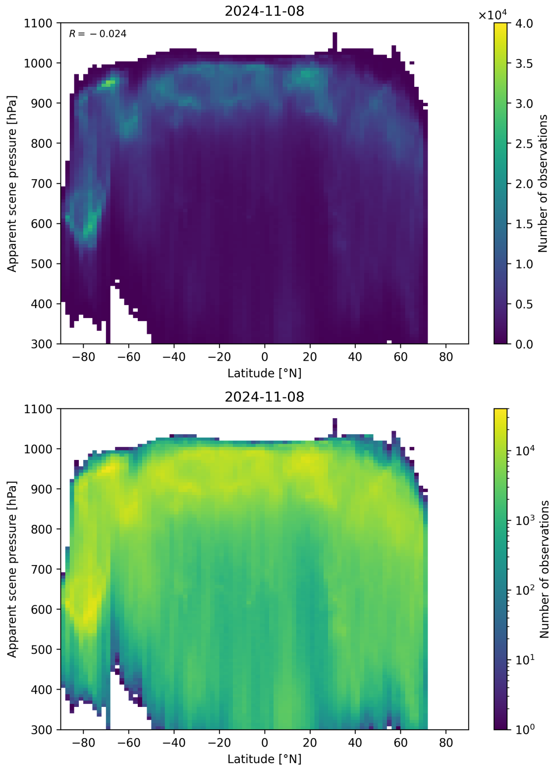
Figure 96: Scatter density plot of “Latitude” against “Apparent scene pressure” for 2024-11-07 to 2024-11-09.
