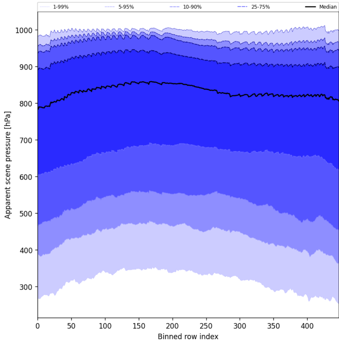
Figure 53: Along track statistics of “Apparent scene pressure” for 2024-11-07 to 2024-11-09
