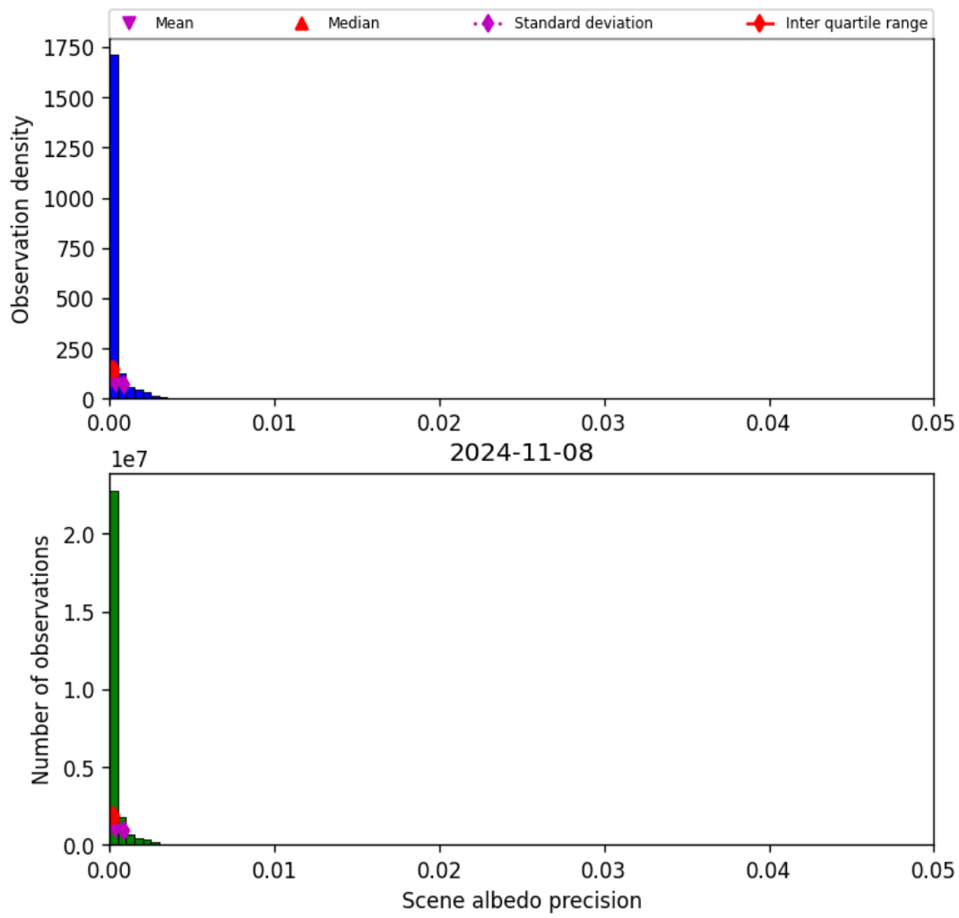
Figure 35: Histogram of “Scene albedo precision” for 2024-11-07 to 2024-11-09
