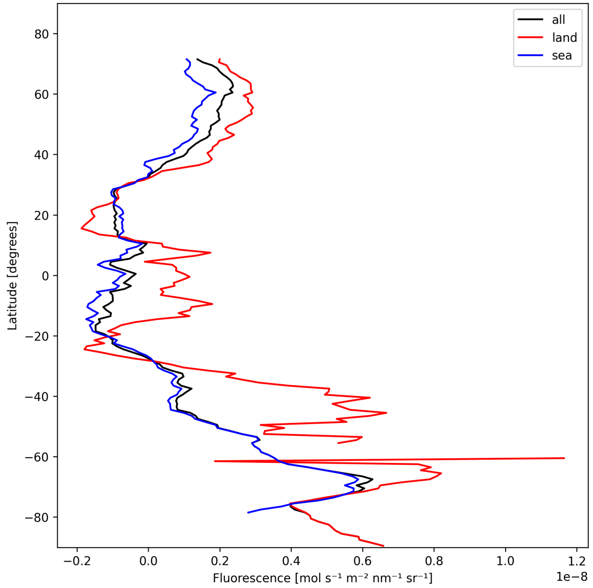
Figure 23: Zonal average of “Fluorescence” for 2024-11-07 to 2024-11-09.
