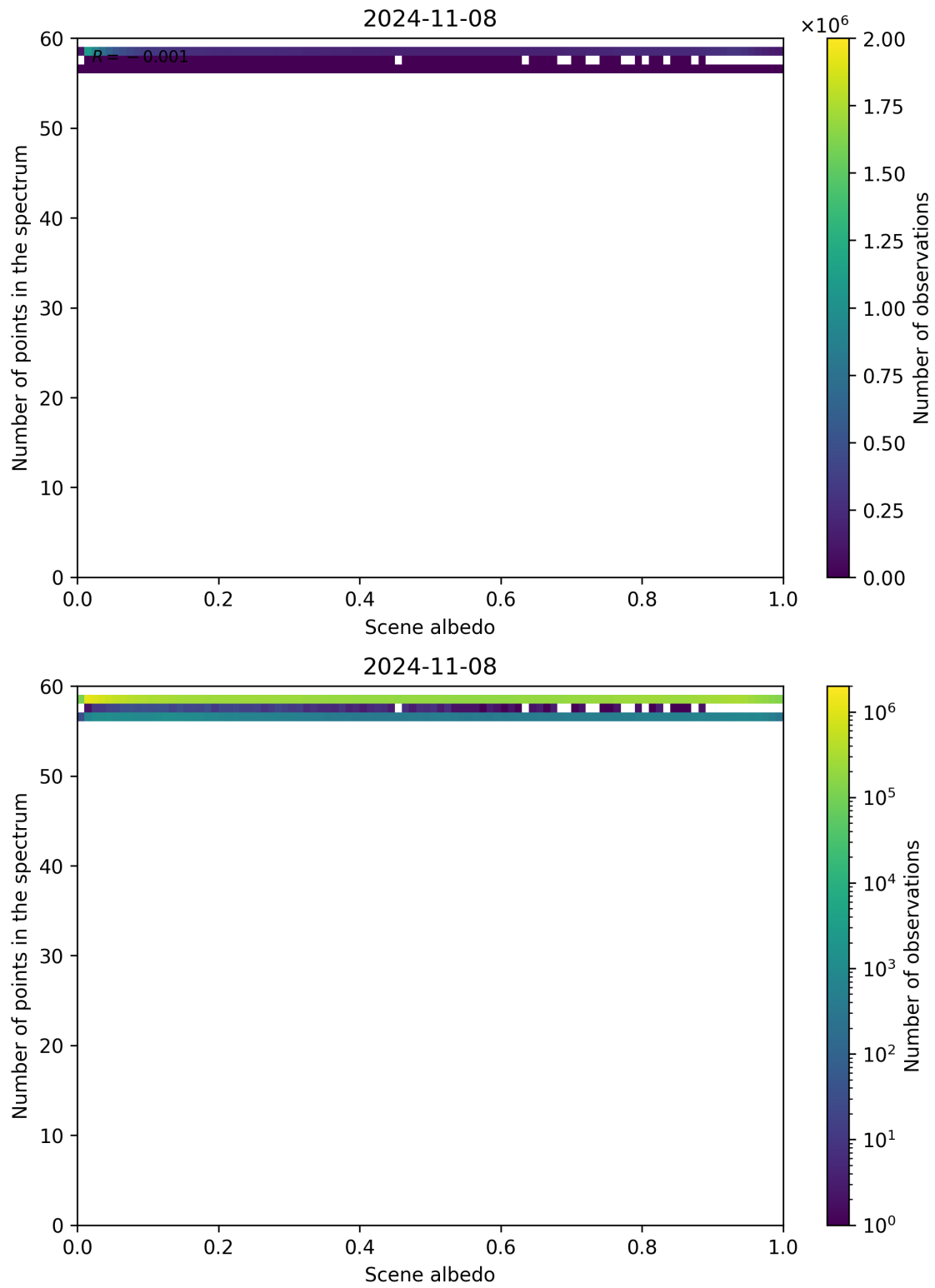
Figure 116: Scatter density plot of “Scene albedo” against “Number of points in the spectrum” for 2024-11-07 to 2024-11-09.
