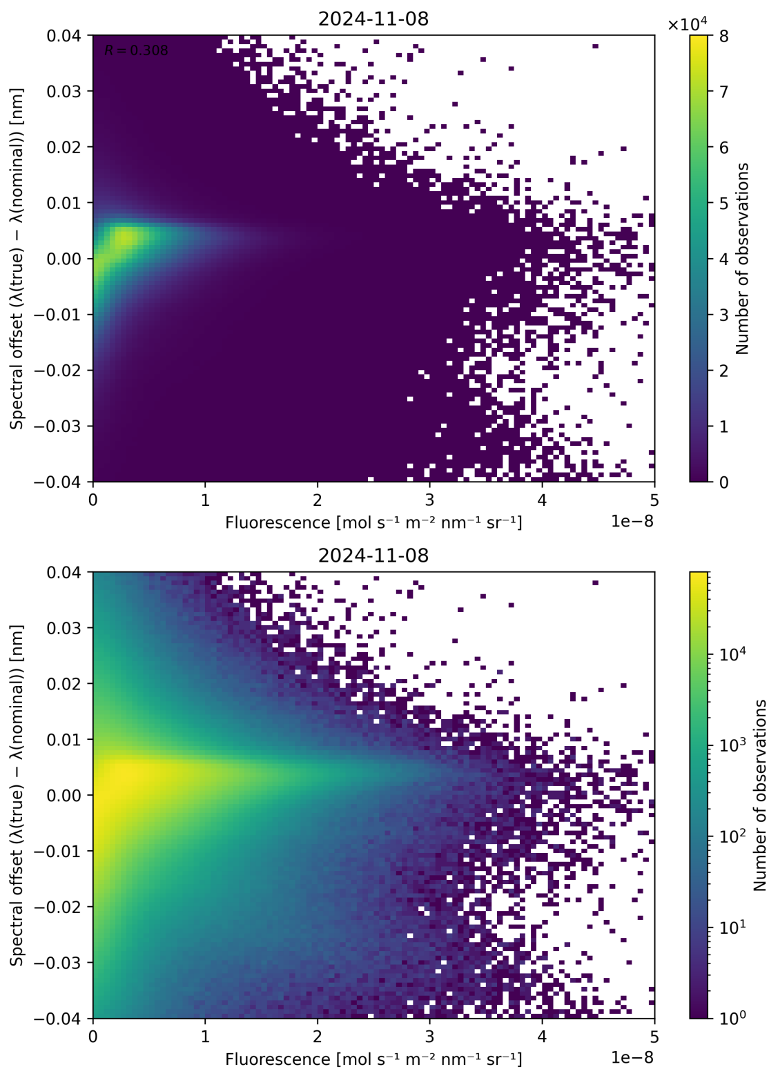
Figure 95: Scatter density plot of “Fluorescence” against “Spectral offset ( \lambda_{\text{true}} - \lambda_{\text{nominal}} )” for 2024-11-07 to 2024-11-09.
