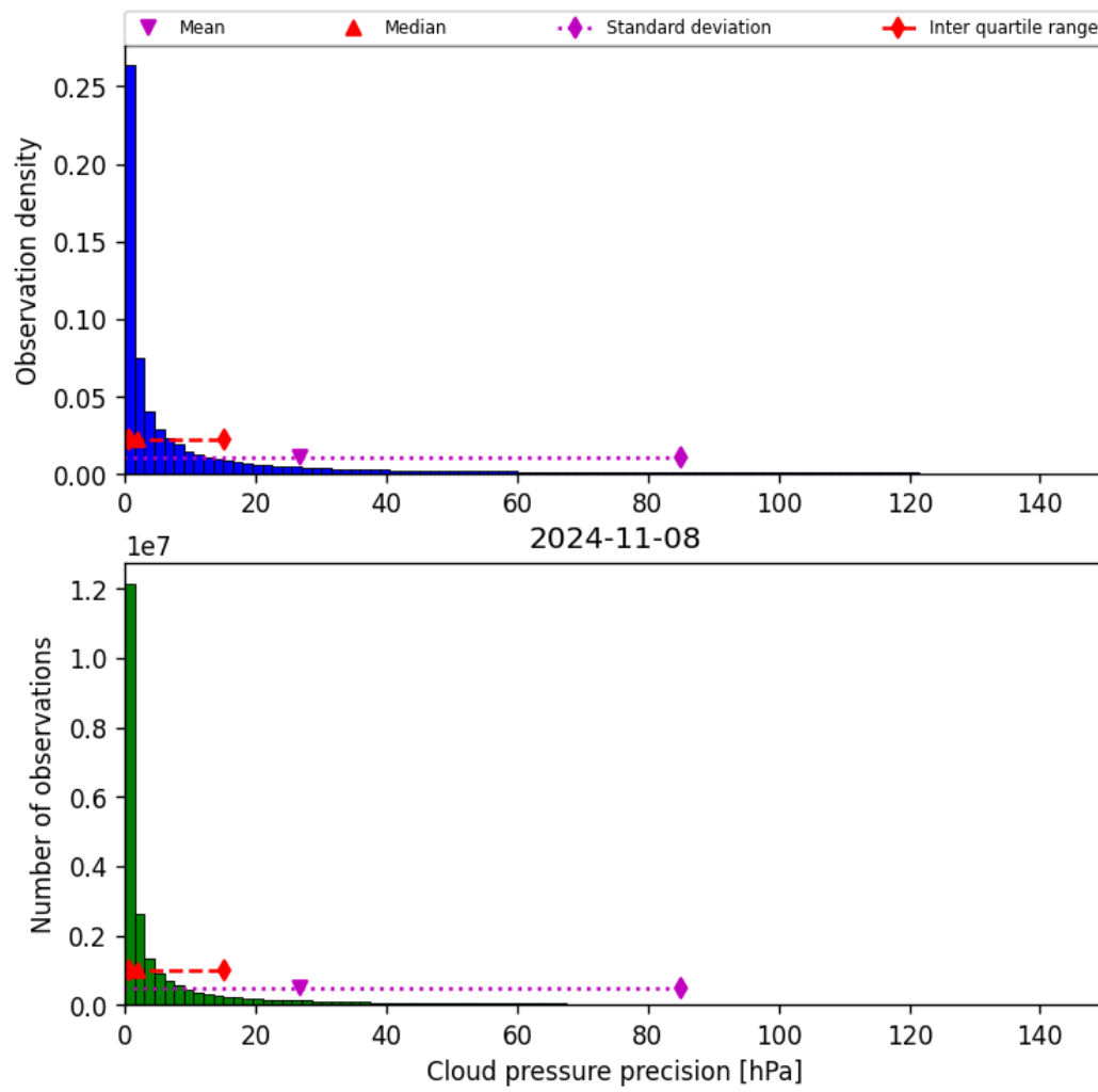
Figure 31: Histogram of “Cloud pressure precision” for 2024-11-07 to 2024-11-09
