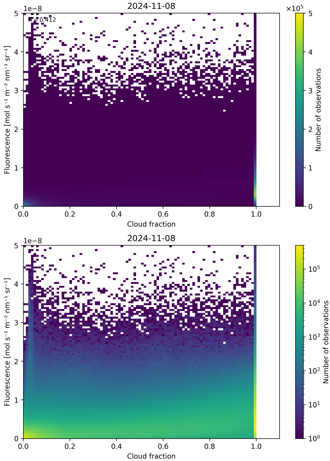
Figure 79: Scatter density plot of “Cloud fraction” against “Fluorescence” for 2024-11-07 to 2024-11-09.
