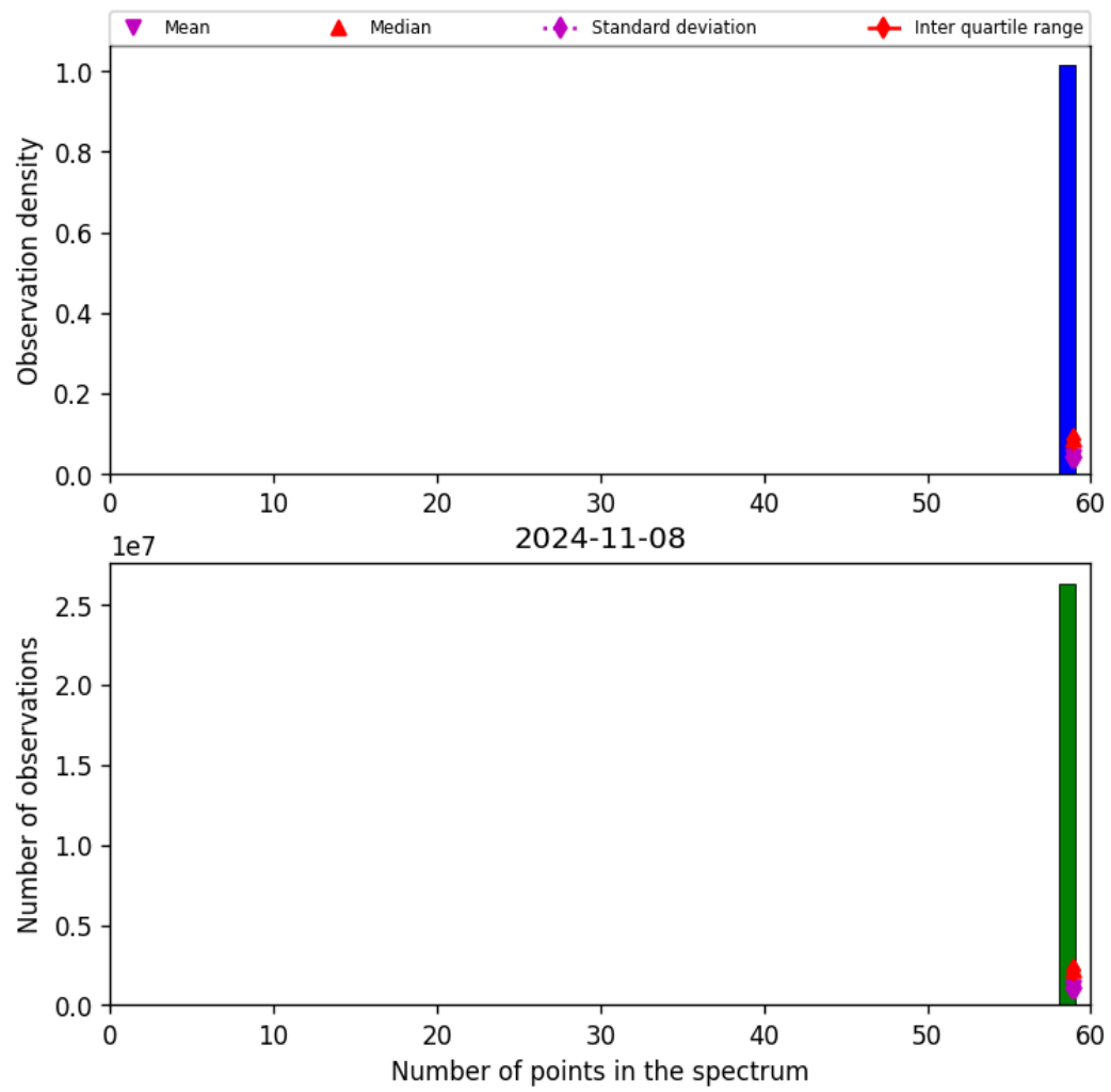
Figure 44: Histogram of “Number of points in the spectrum” for 2024-11-07 to 2024-11-09
