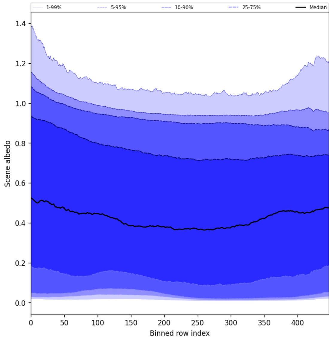
Figure 51: Along track statistics of “Scene albedo” for 2024-11-07 to 2024-11-09
