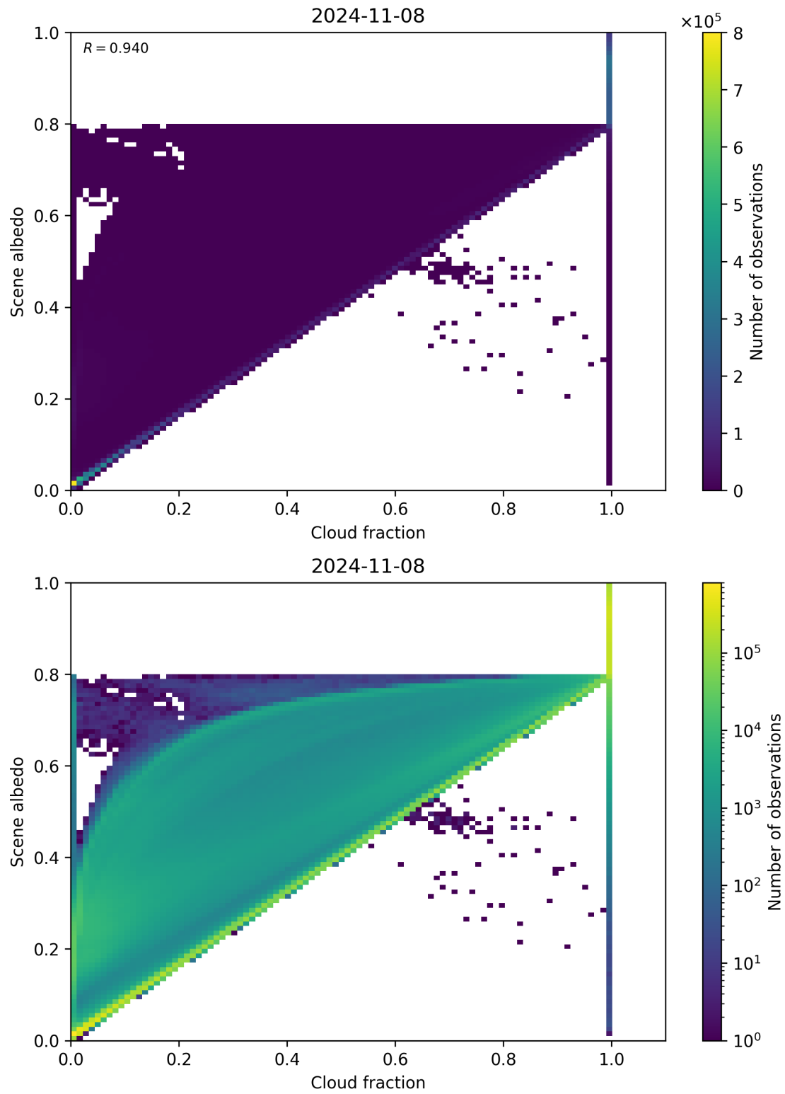
Figure 82: Scatter density plot of “Cloud fraction” against “Scene albedo” for 2024-11-07 to 2024-11-09.
