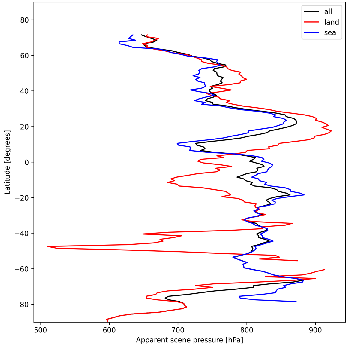
Figure 19: Zonal average of “Apparent scene pressure” for 2024-11-07 to 2024-11-09.
