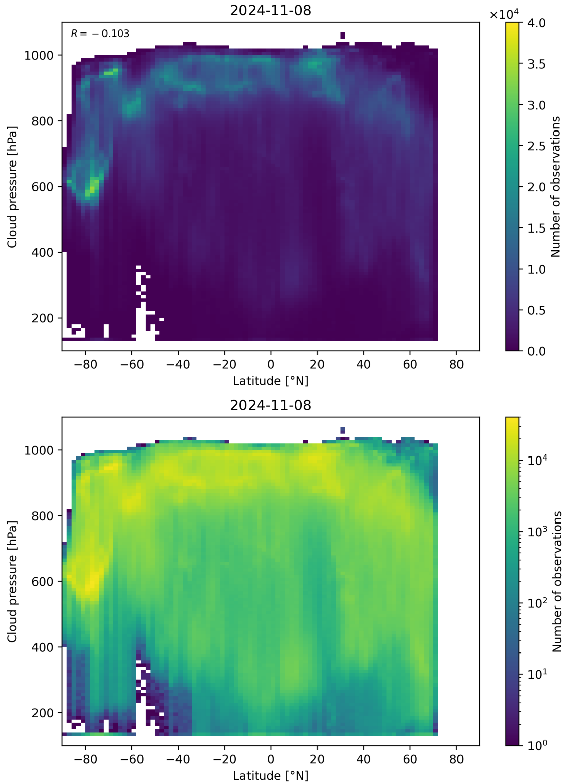
Figure 100: Scatter density plot of “Latitude” against “Cloud pressure” for 2024-11-07 to 2024-11-09.
