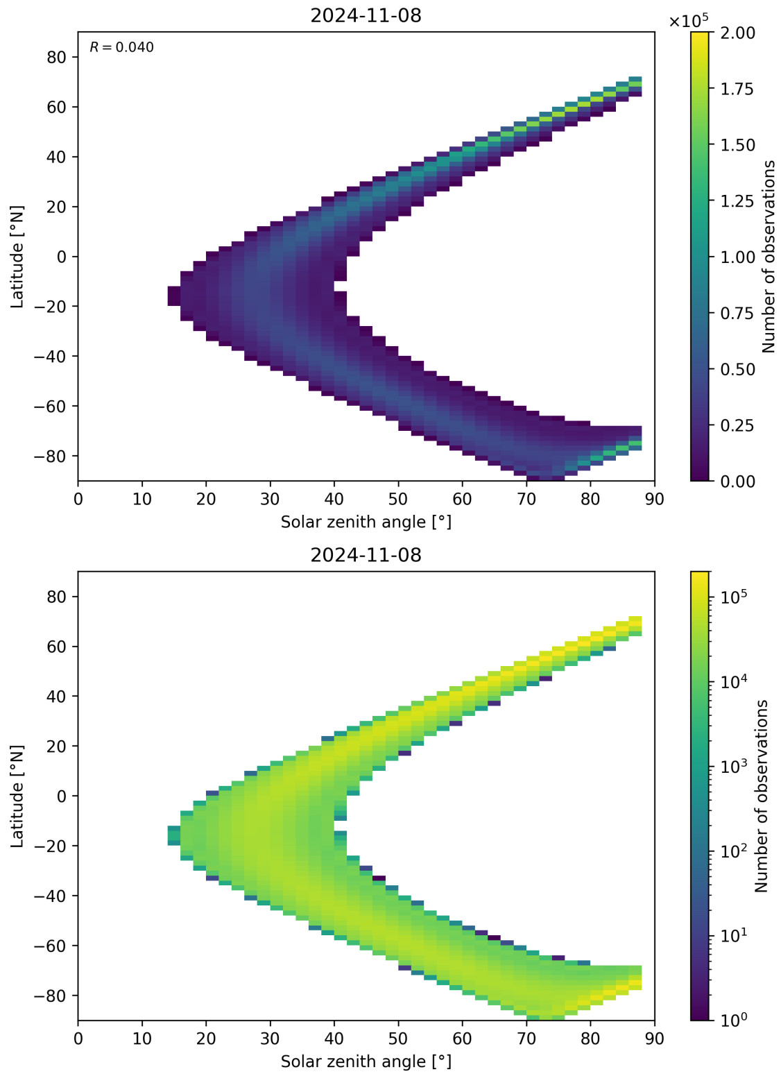
Figure 124: Scatter density plot of “Solar zenith angle” against “Latitude” for 2024-11-07 to 2024-11-09.
