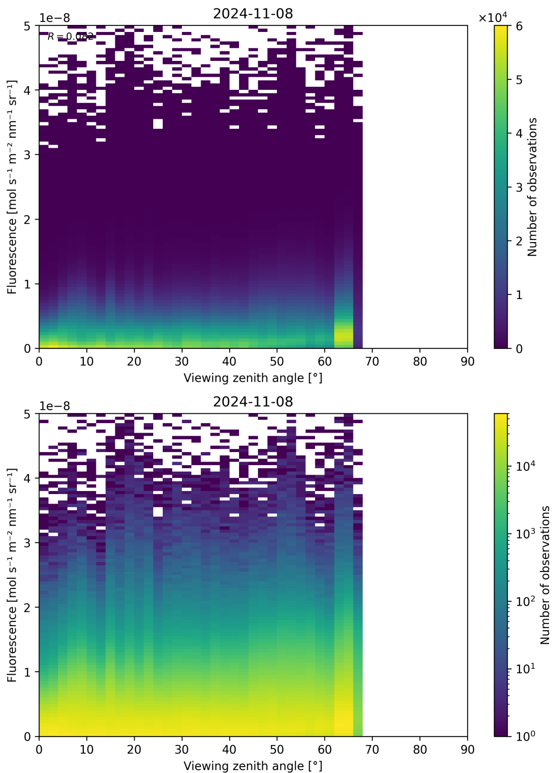
Figure 134: Scatter density plot of “Viewing zenith angle” against “Fluorescence” for 2024-11-07 to 2024-11-09.
