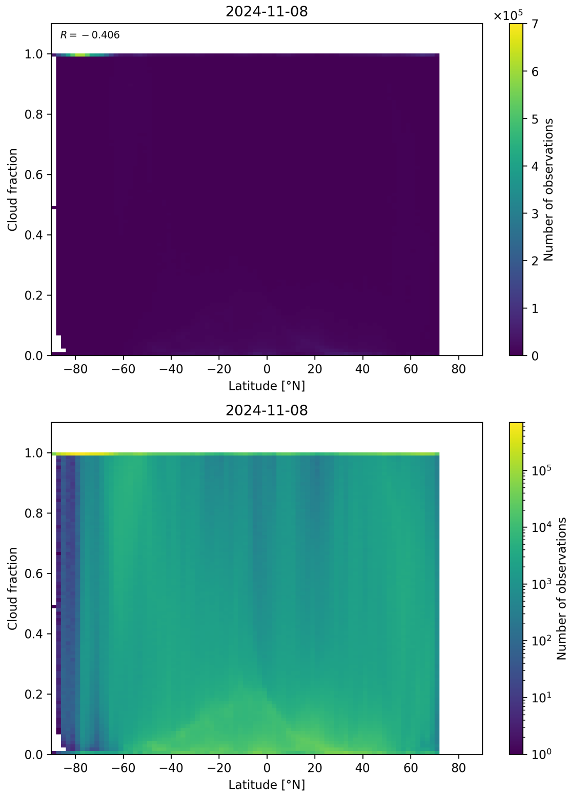
Figure 99: Scatter density plot of “Latitude” against “Cloud fraction” for 2024-11-07 to 2024-11-09.
