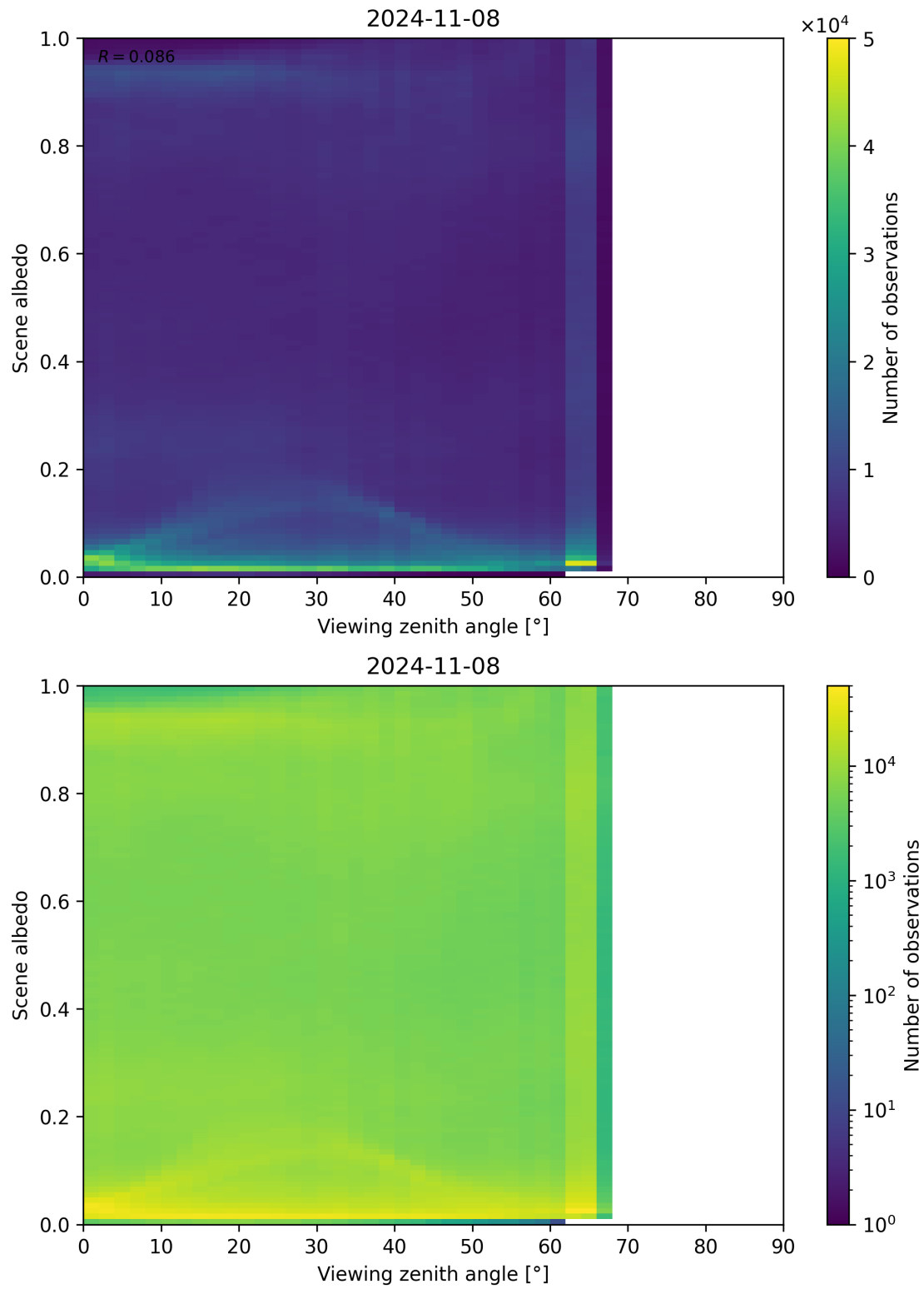
Figure 138: Scatter density plot of “Viewing zenith angle” against “Scene albedo” for 2024-11-07 to 2024-11-09.
