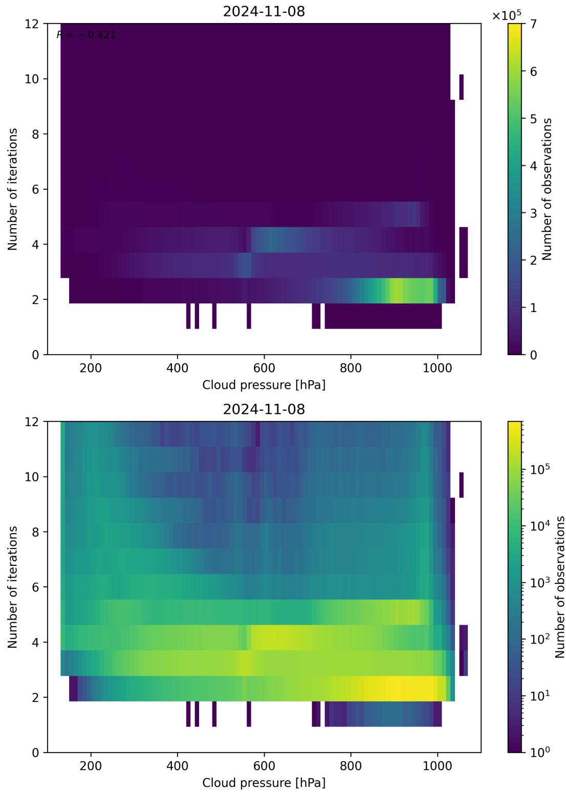
Figure 89: Scatter density plot of “Cloud pressure” against “Number of iterations” for 2024-11-07 to 2024-11-09.
