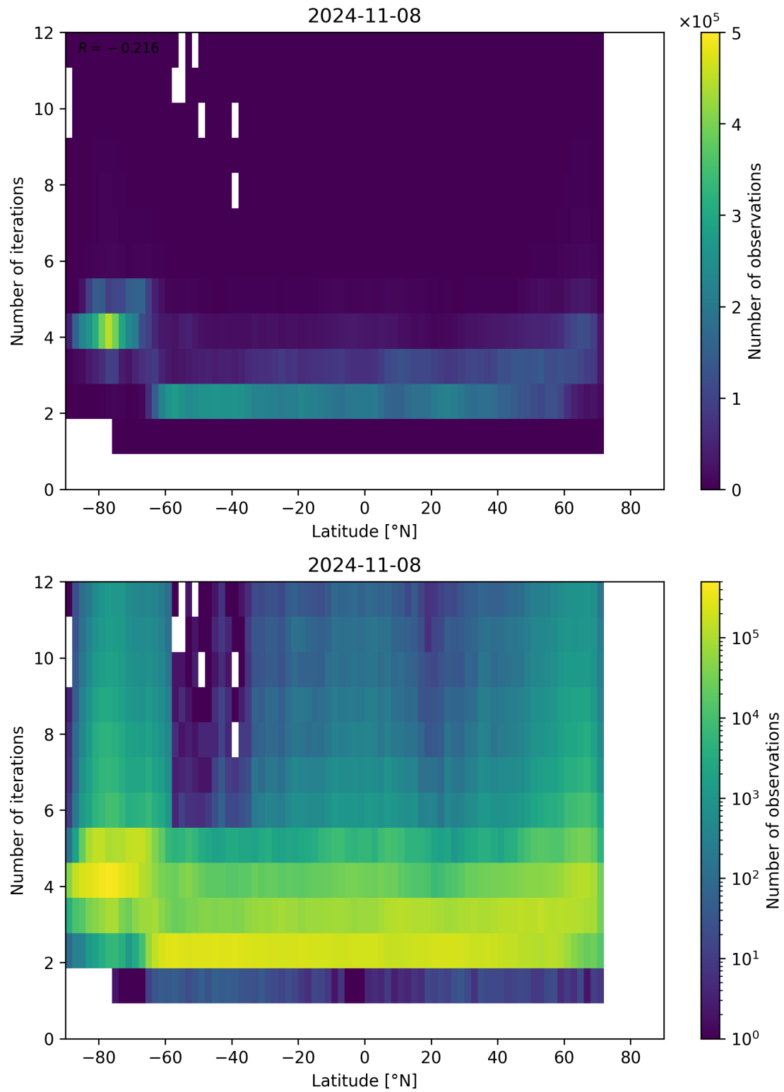
Figure 102: Scatter density plot of “Latitude” against “Number of iterations” for 2024-11-07 to 2024-11-09.
