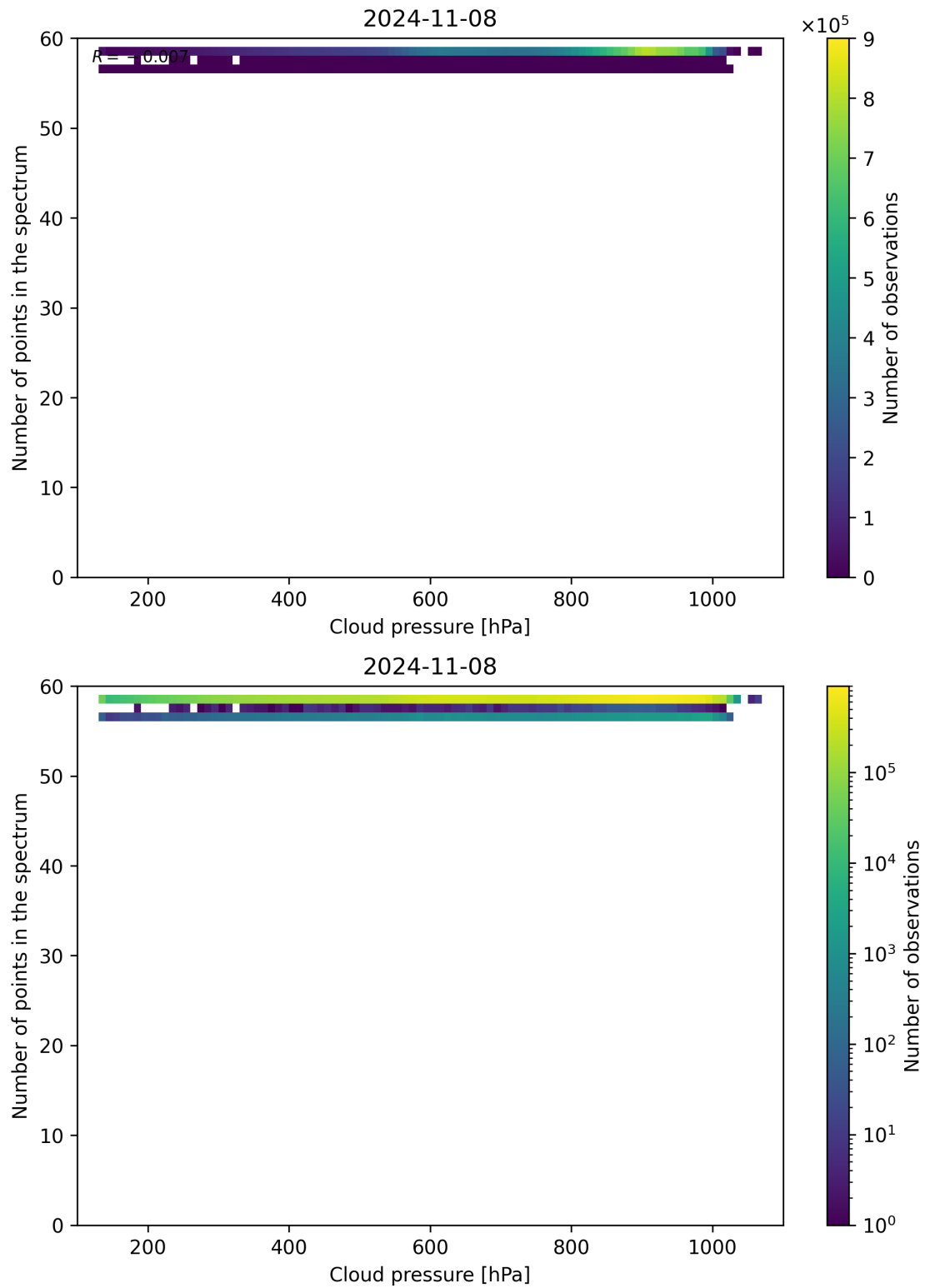
Figure 90: Scatter density plot of “Cloud pressure” against “Number of points in the spectrum” for 2024-11-07 to 2024-11-09.
