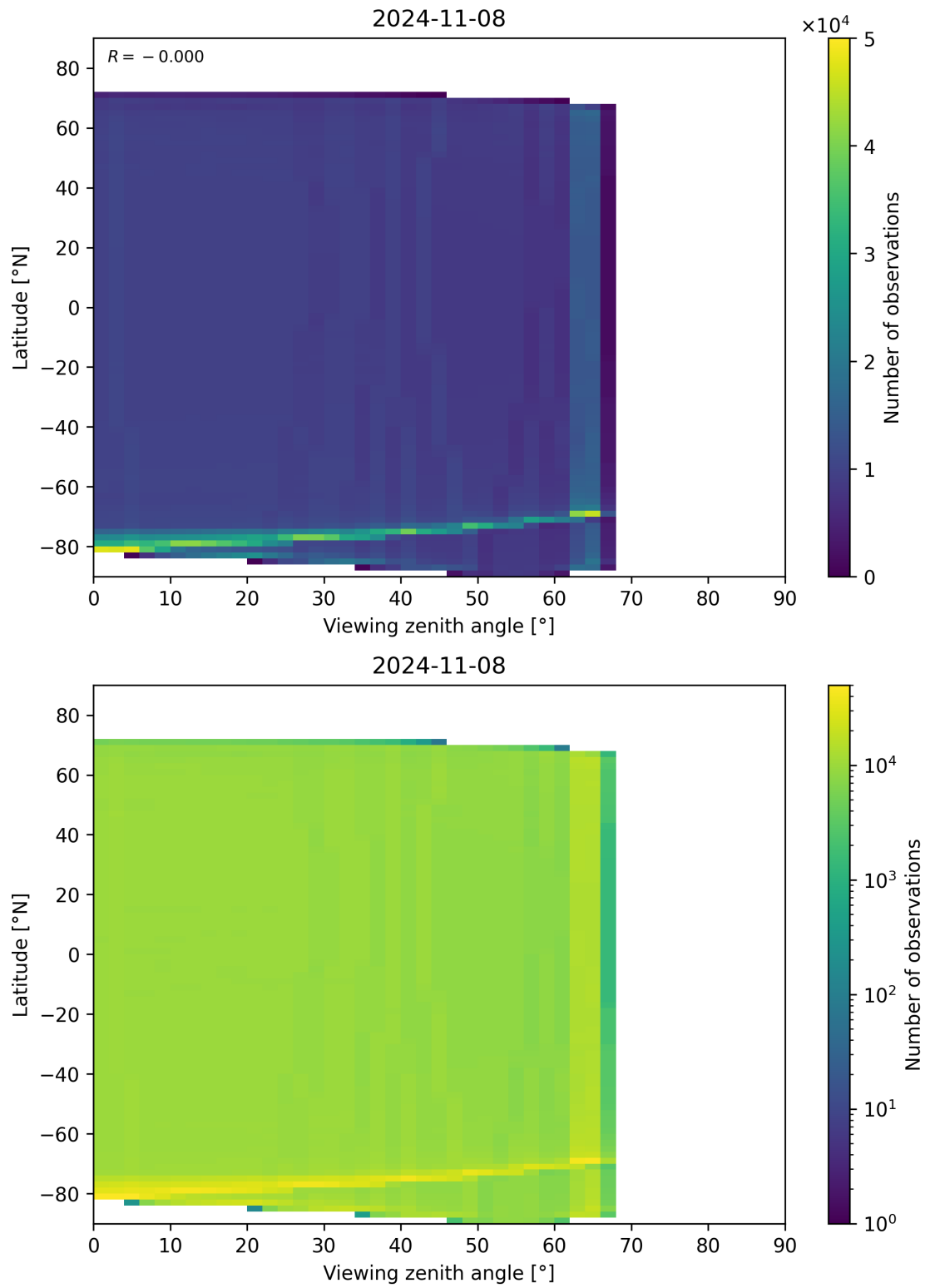
Figure 135: Scatter density plot of “Viewing zenith angle” against “Latitude” for 2024-11-07 to 2024-11-09.
