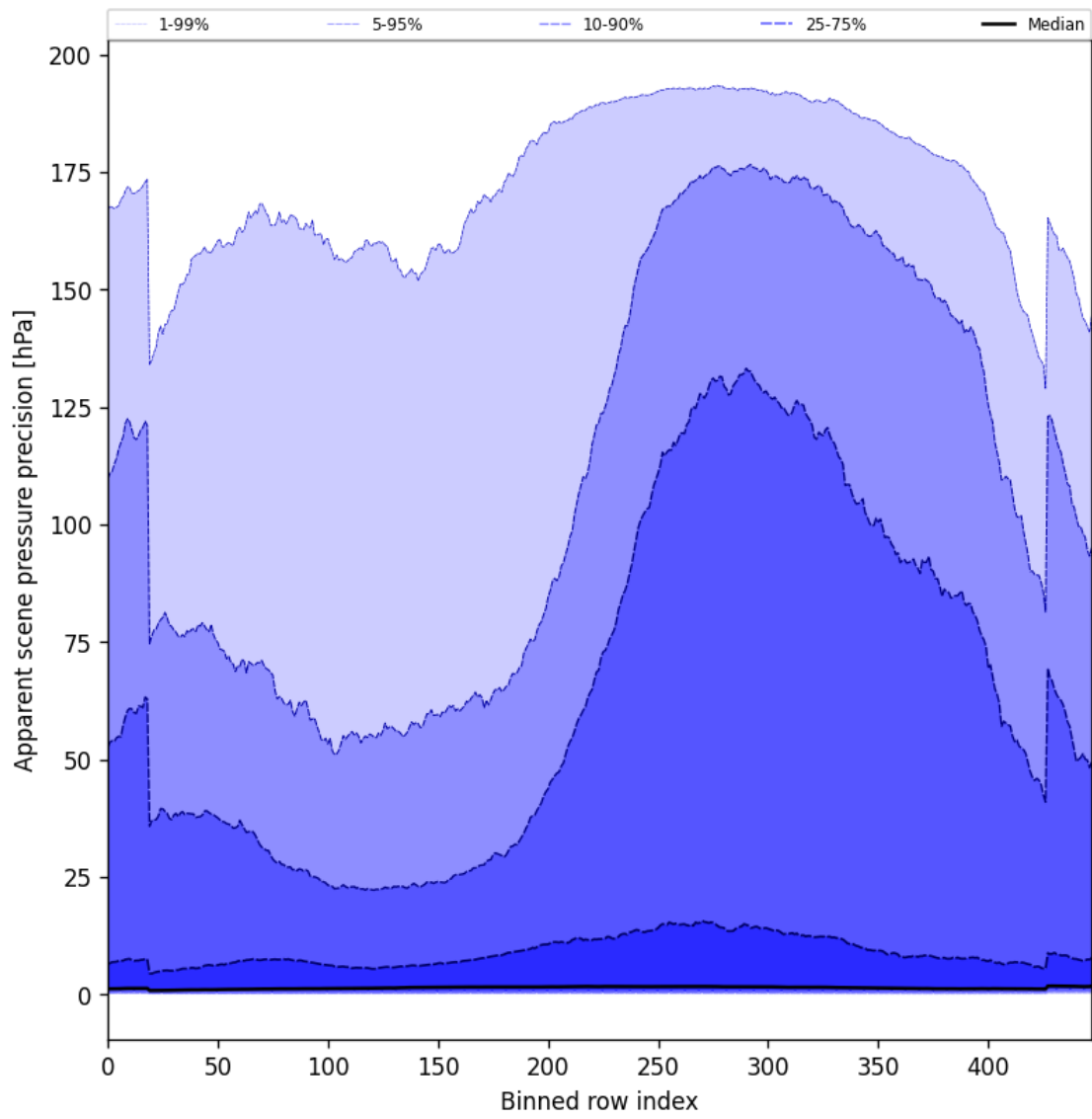
Figure 54: Along track statistics of “Apparent scene pressure precision” for 2024-11-07 to 2024-11-09
