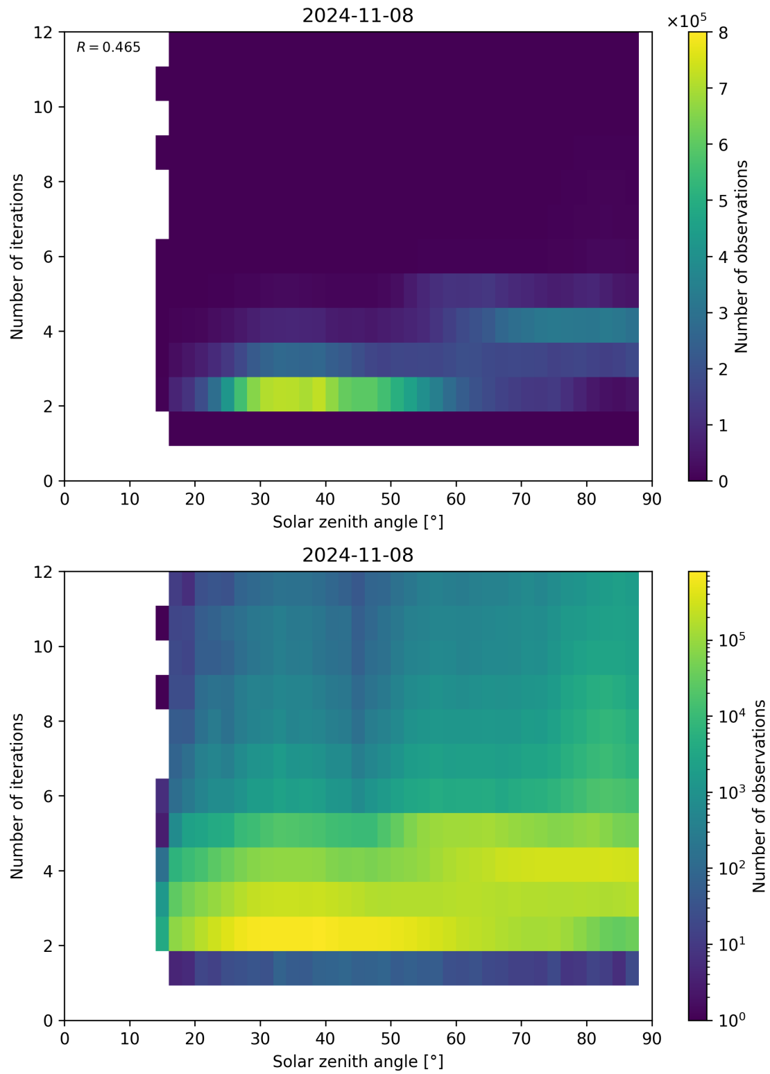
Figure 125: Scatter density plot of “Solar zenith angle” against “Number of iterations” for 2024-11-07 to 2024-11-09.
