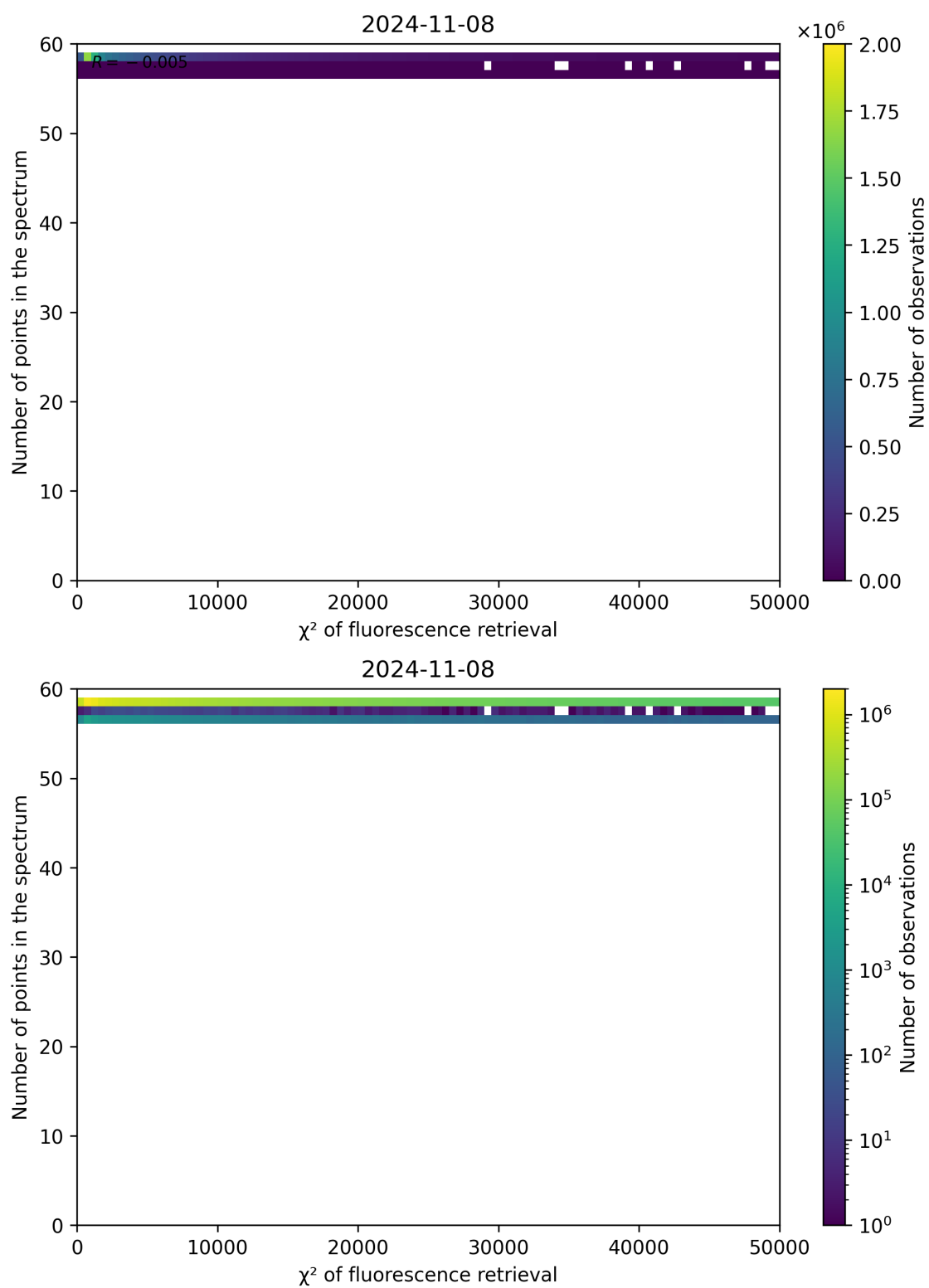
Figure 71: Scatter density plot of " \chi^2 of fluorescence retrieval" against "Number of points in the spectrum" for 2024-11-07 to 2024-11-09.
