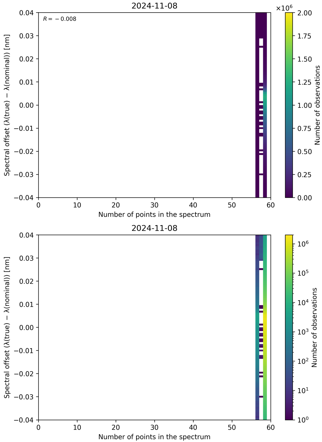
Figure 110: Scatter density plot of “Number of points in the spectrum” against “Spectral offset ( \lambda_{\text{true}} - \lambda_{\text{nominal}} )” for 2024-11-07 to 2024-11-09.
