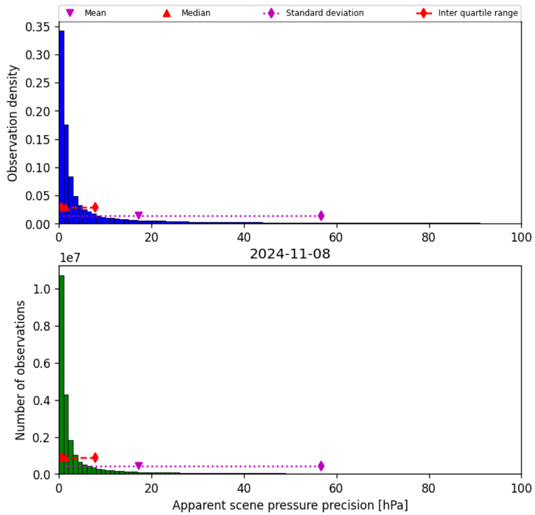
Figure 37: Histogram of “Apparent scene pressure precision” for 2024-11-07 to 2024-11-09
