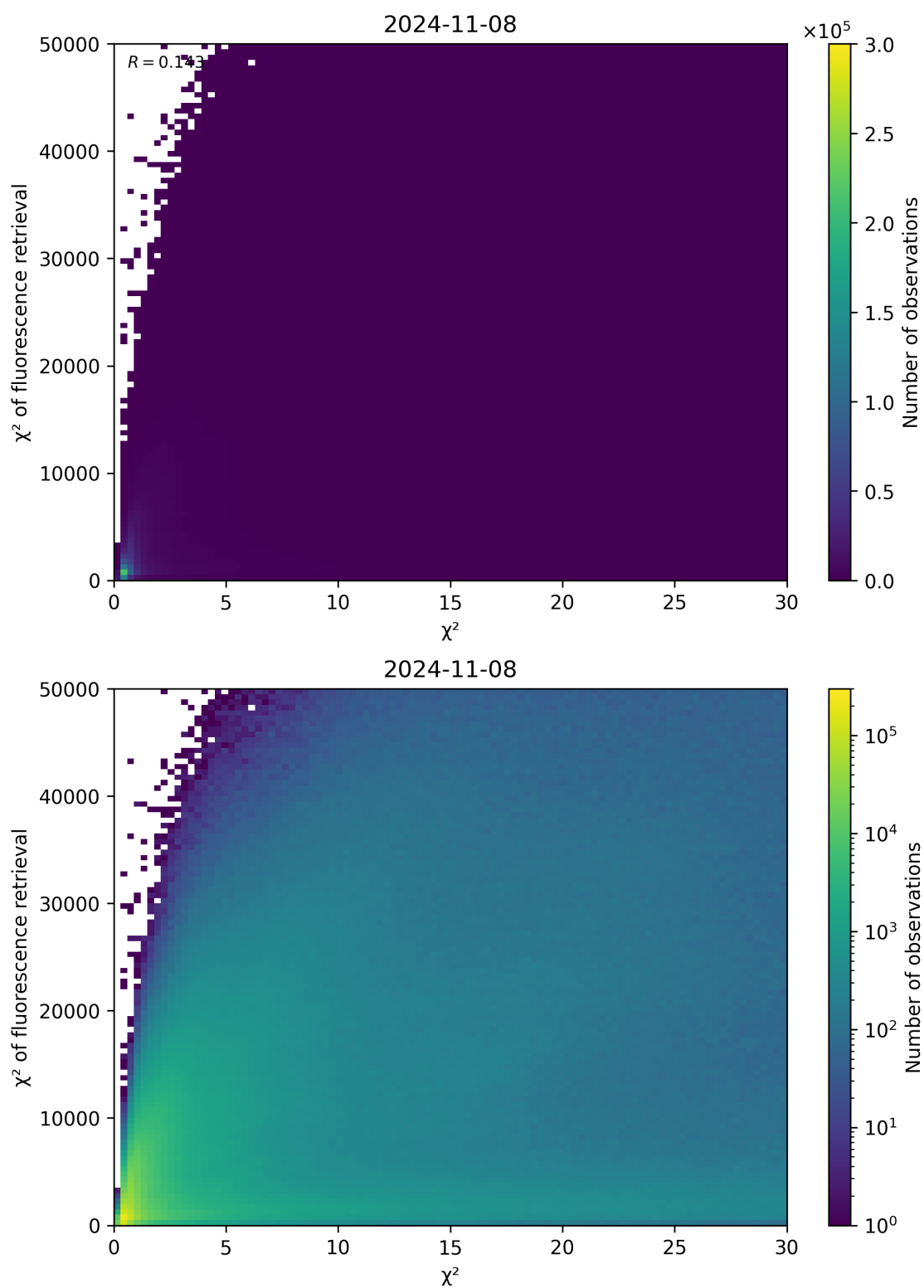
Figure 69: Scatter density plot of “ \chi^2 ” against “ \chi^2 of fluorescence retrieval” for 2024-11-07 to 2024-11-09.
