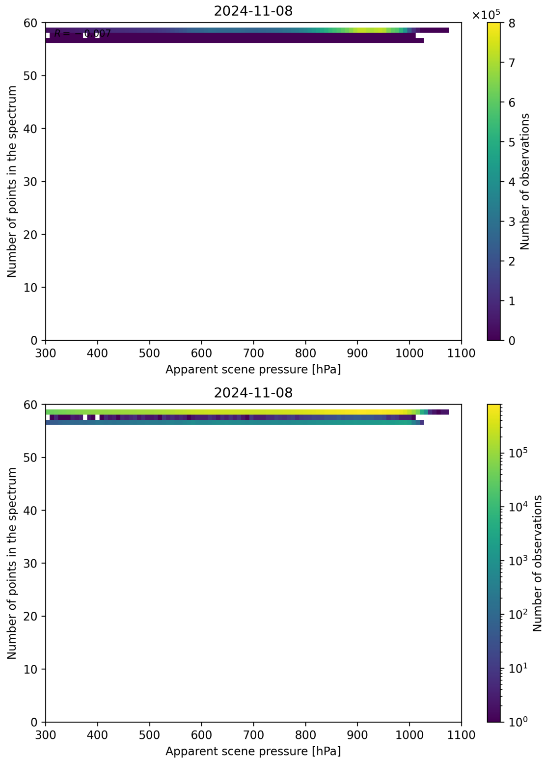
Figure 67: Scatter density plot of “Apparent scene pressure” against “Number of points in the spectrum” for 2024-11-07 to 2024-11-09.
