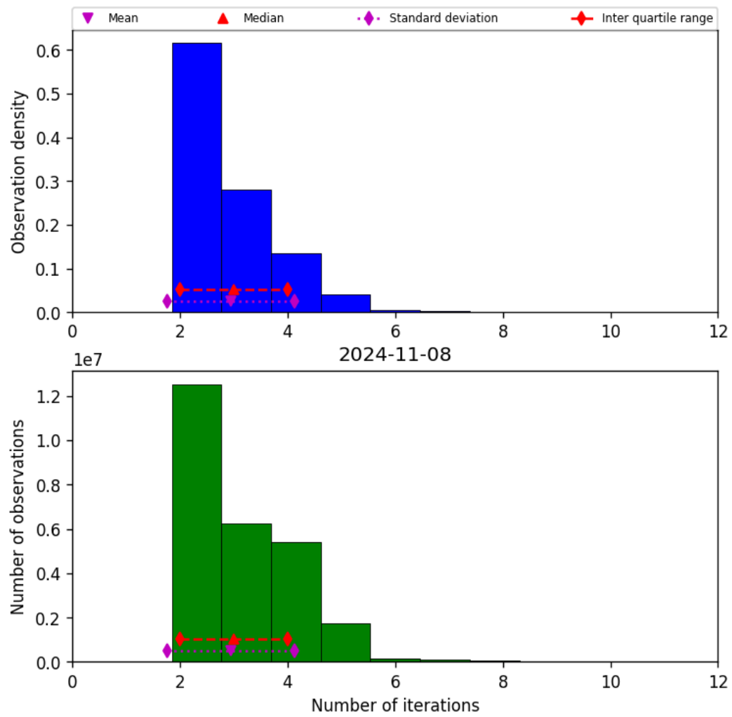
Figure 39: Histogram of “Number of iterations” for 2024-11-07 to 2024-11-09
