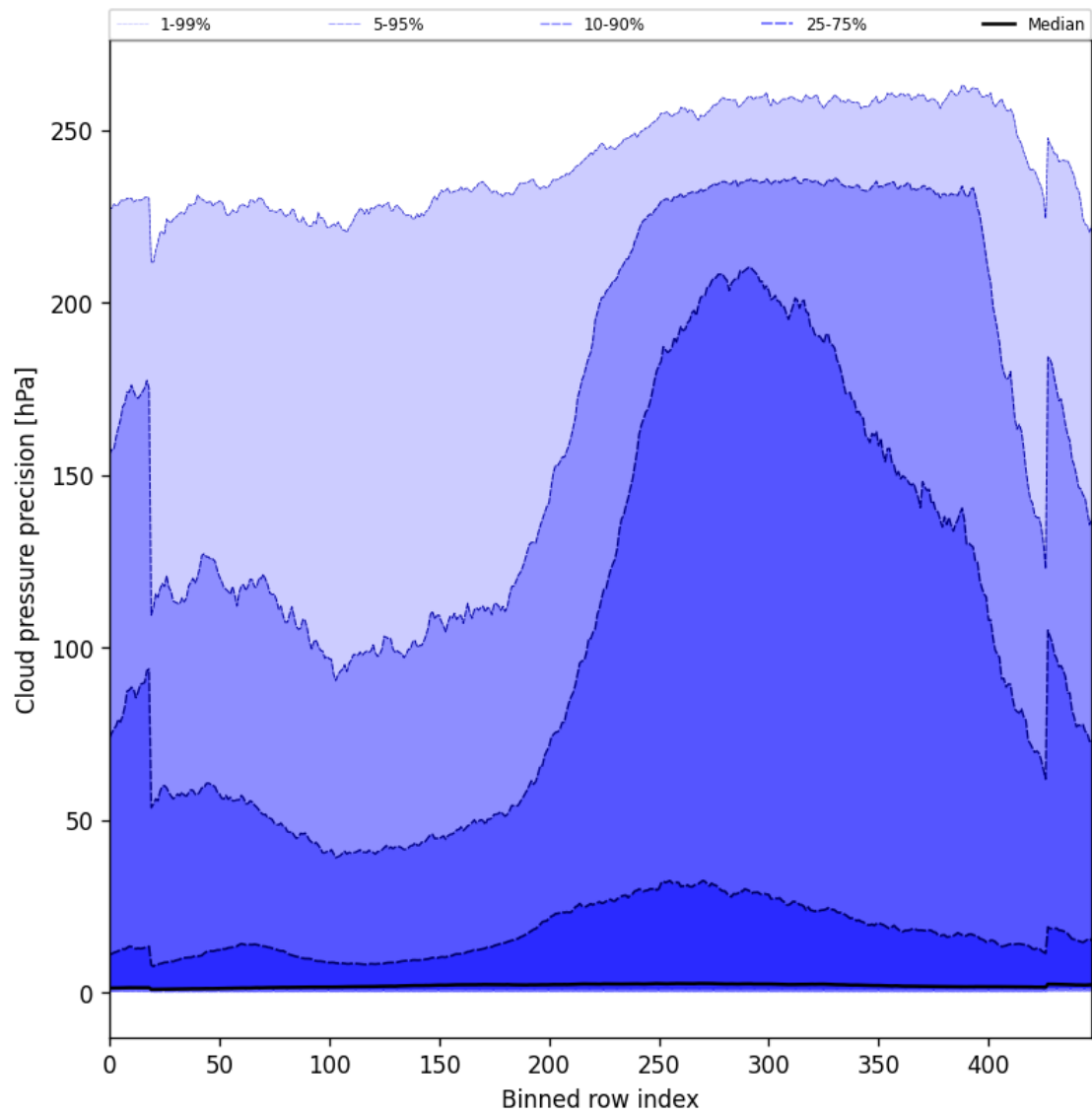
Figure 48: Along track statistics of “Cloud pressure precision” for 2024-11-07 to 2024-11-09
