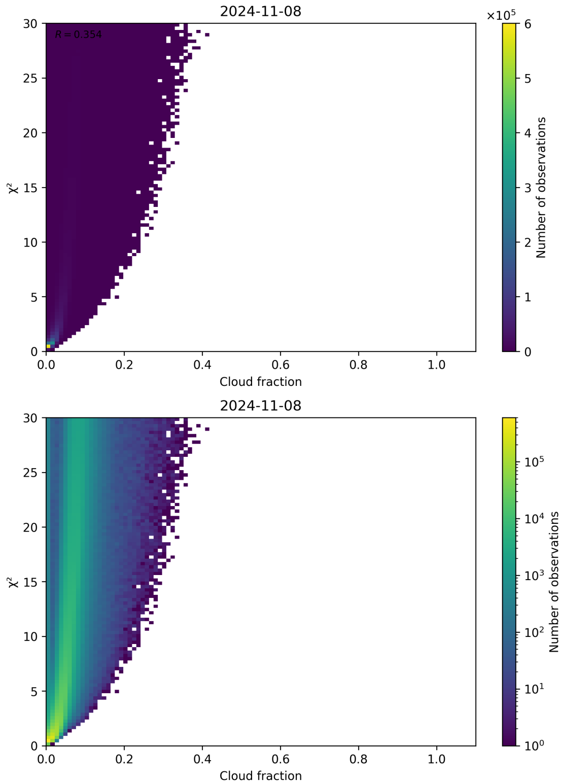
Figure 77: Scatter density plot of “Cloud fraction” against “ \chi^2 ” for 2024-11-07 to 2024-11-09.
