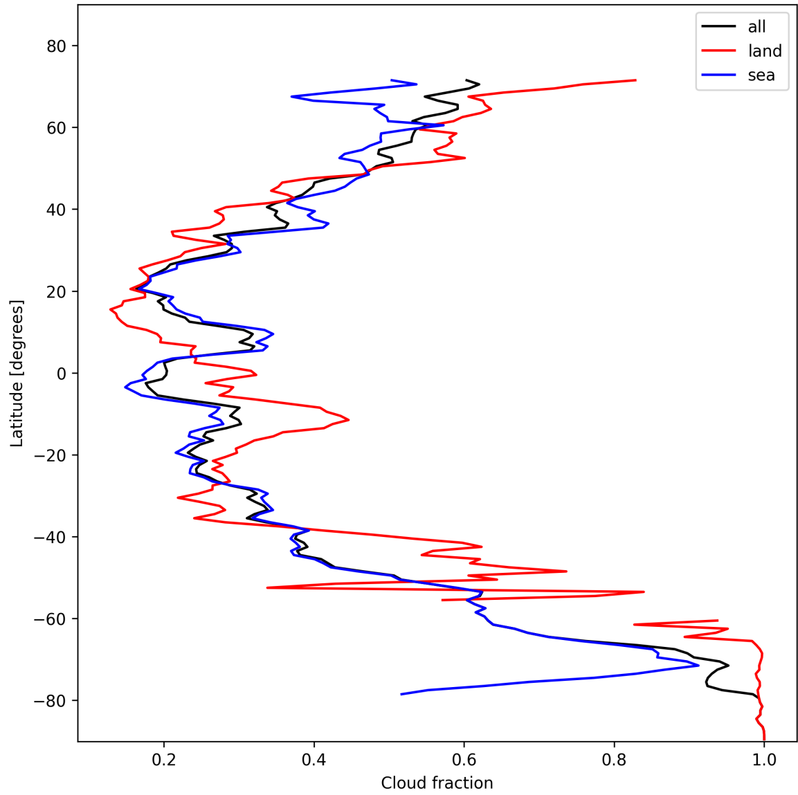
Figure 15: Zonal average of “Cloud fraction” for 2024-11-07 to 2024-11-09.
