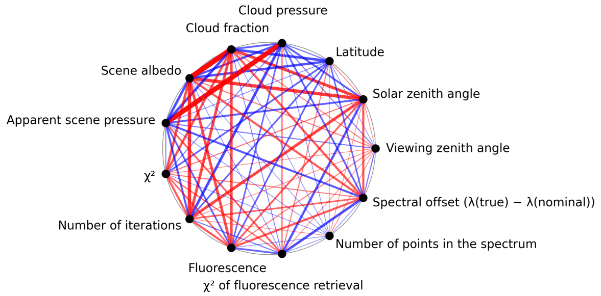
Figure 1: Map of correlation graph for 2024-11-07 to 2024-11-09.
