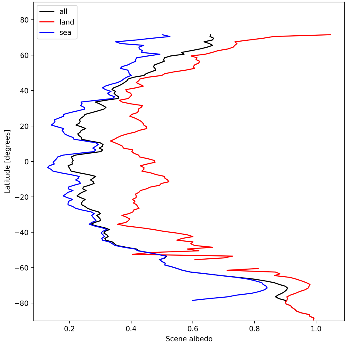
Figure 17: Zonal average of “Scene albedo” for 2024-11-07 to 2024-11-09.
