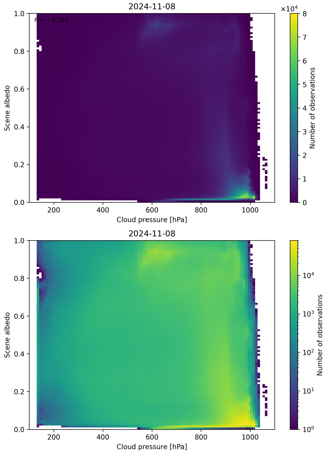
Figure 91: Scatter density plot of “Cloud pressure” against “Scene albedo” for 2024-11-07 to 2024-11-09.
