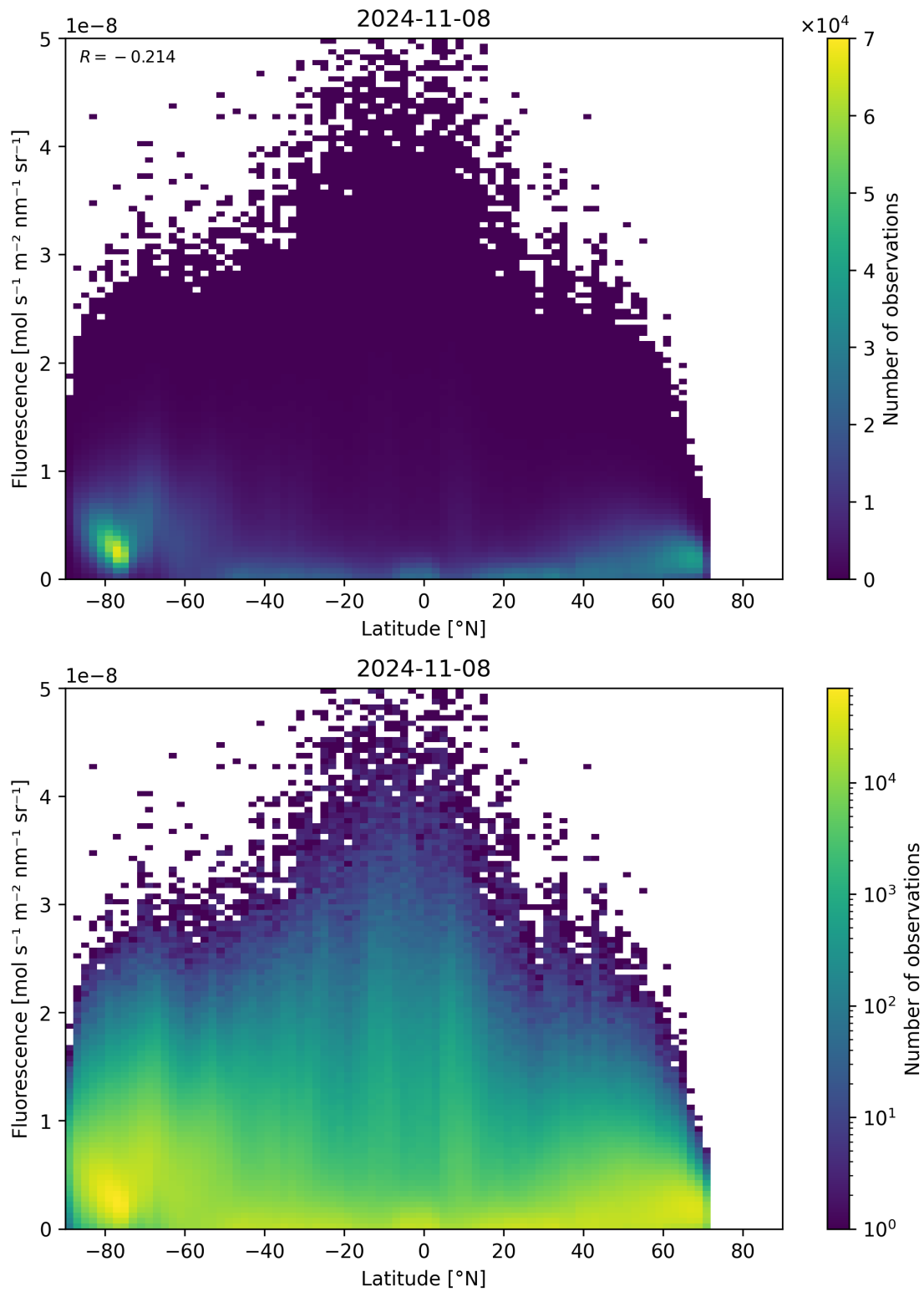
Figure 101: Scatter density plot of “Latitude” against “Fluorescence” for 2024-11-07 to 2024-11-09.
