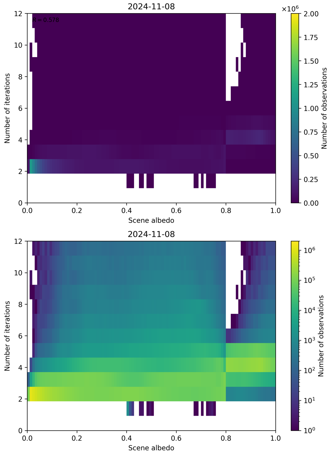
Figure 115: Scatter density plot of “Scene albedo” against “Number of iterations” for 2024-11-07 to 2024-11-09.
