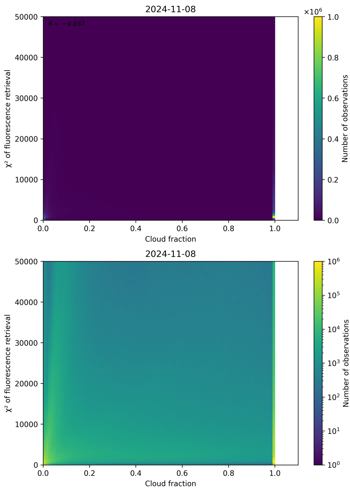
Figure 78: Scatter density plot of “Cloud fraction” against “ \chi^2 of fluorescence retrieval” for 2024-11-07 to 2024-11-09.
