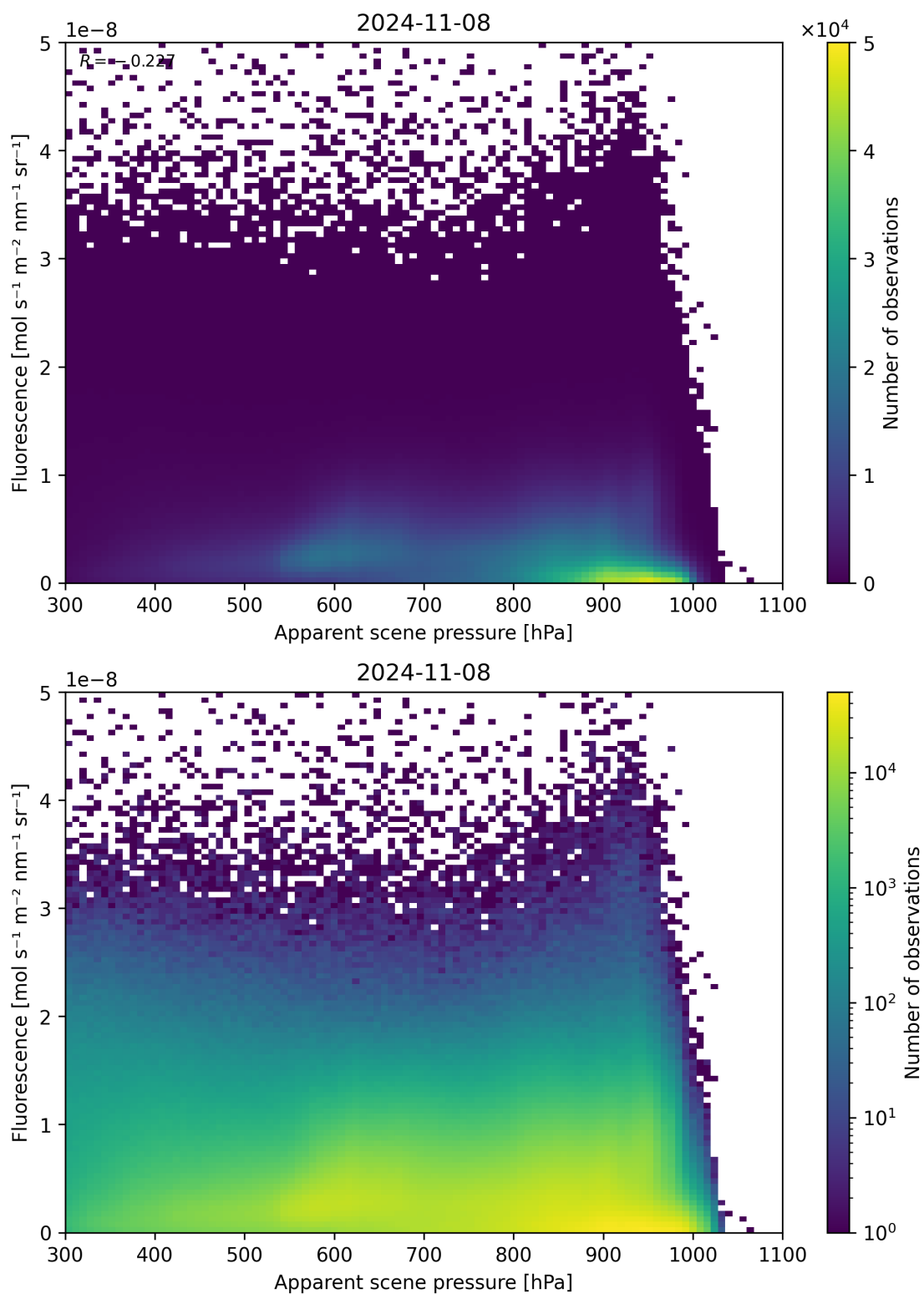
Figure 65: Scatter density plot of “Apparent scene pressure” against “Fluorescence” for 2024-11-07 to 2024-11-09.
