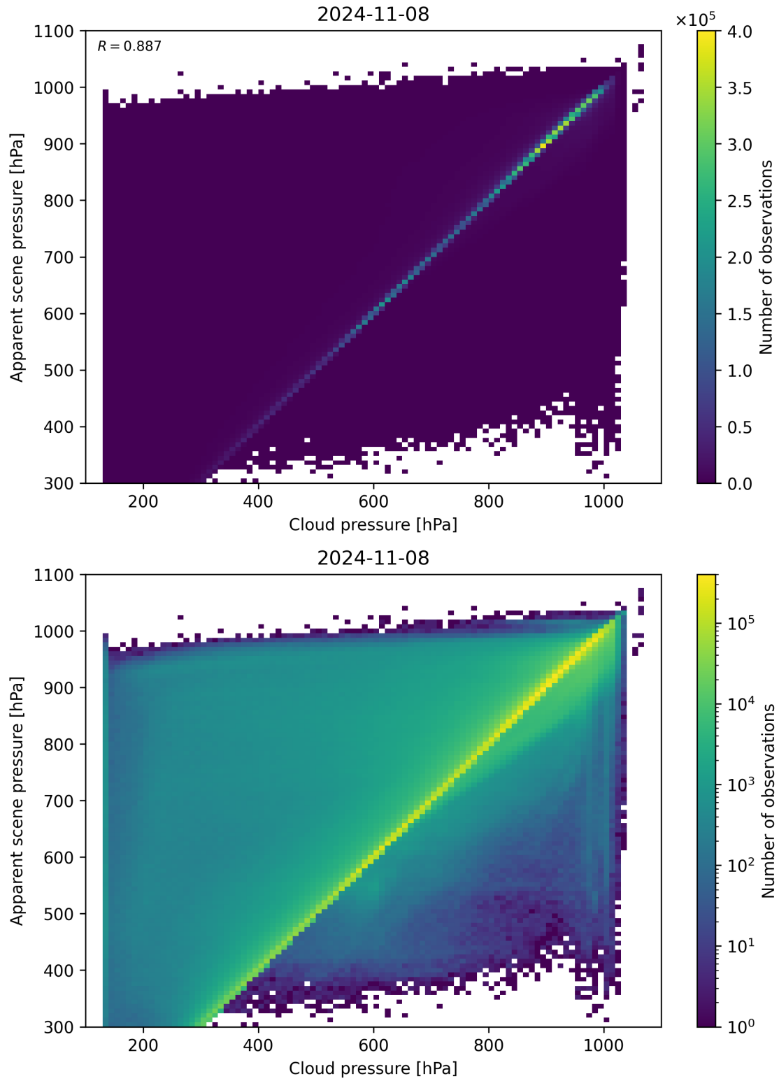
Figure 84: Scatter density plot of “Cloud pressure” against “Apparent scene pressure” for 2024-11-07 to 2024-11-09.
