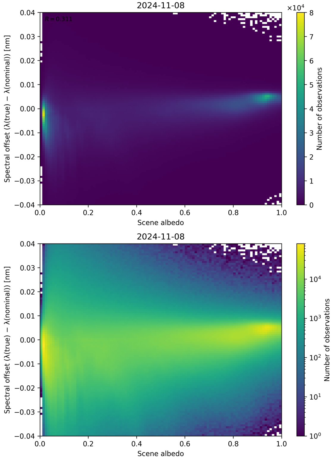
Figure 117: Scatter density plot of “Scene albedo” against “Spectral offset ( \lambda_{\text{true}} - \lambda_{\text{nominal}} )” for 2024-11-07 to 2024-11-09.
