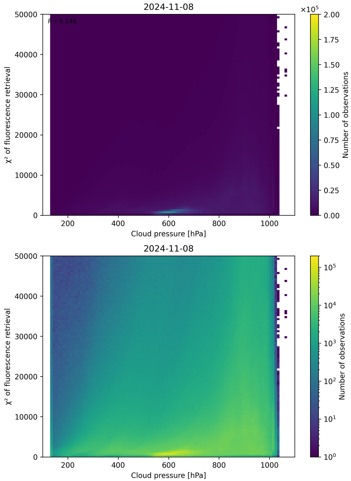
Figure 86: Scatter density plot of “Cloud pressure” against “ \chi^2 of fluorescence retrieval” for 2024-11-07 to 2024-11-09.
