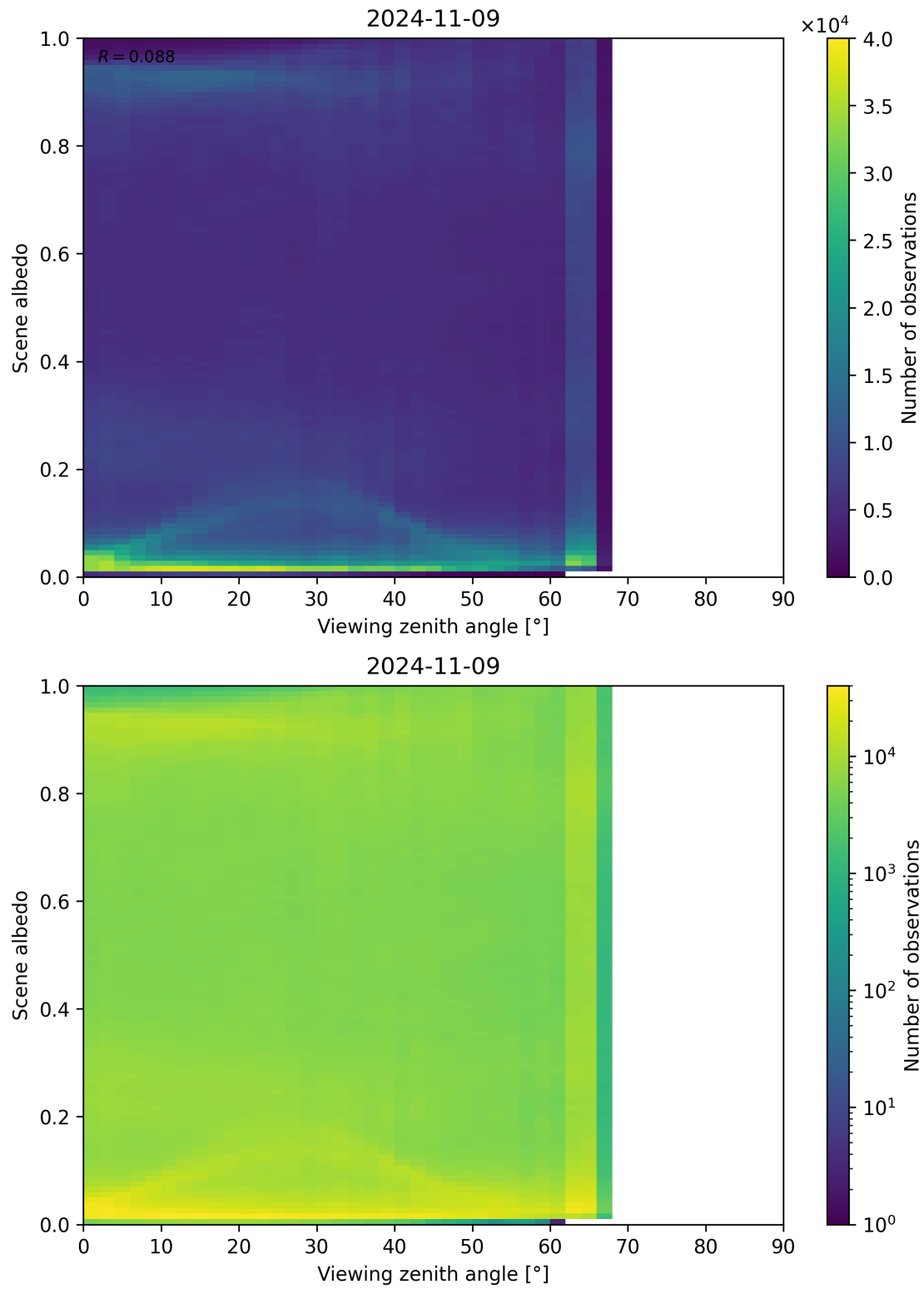
Figure 138: Scatter density plot of “Viewing zenith angle” against “Scene albedo” for 2024-11-09 to 2024-11-10.
