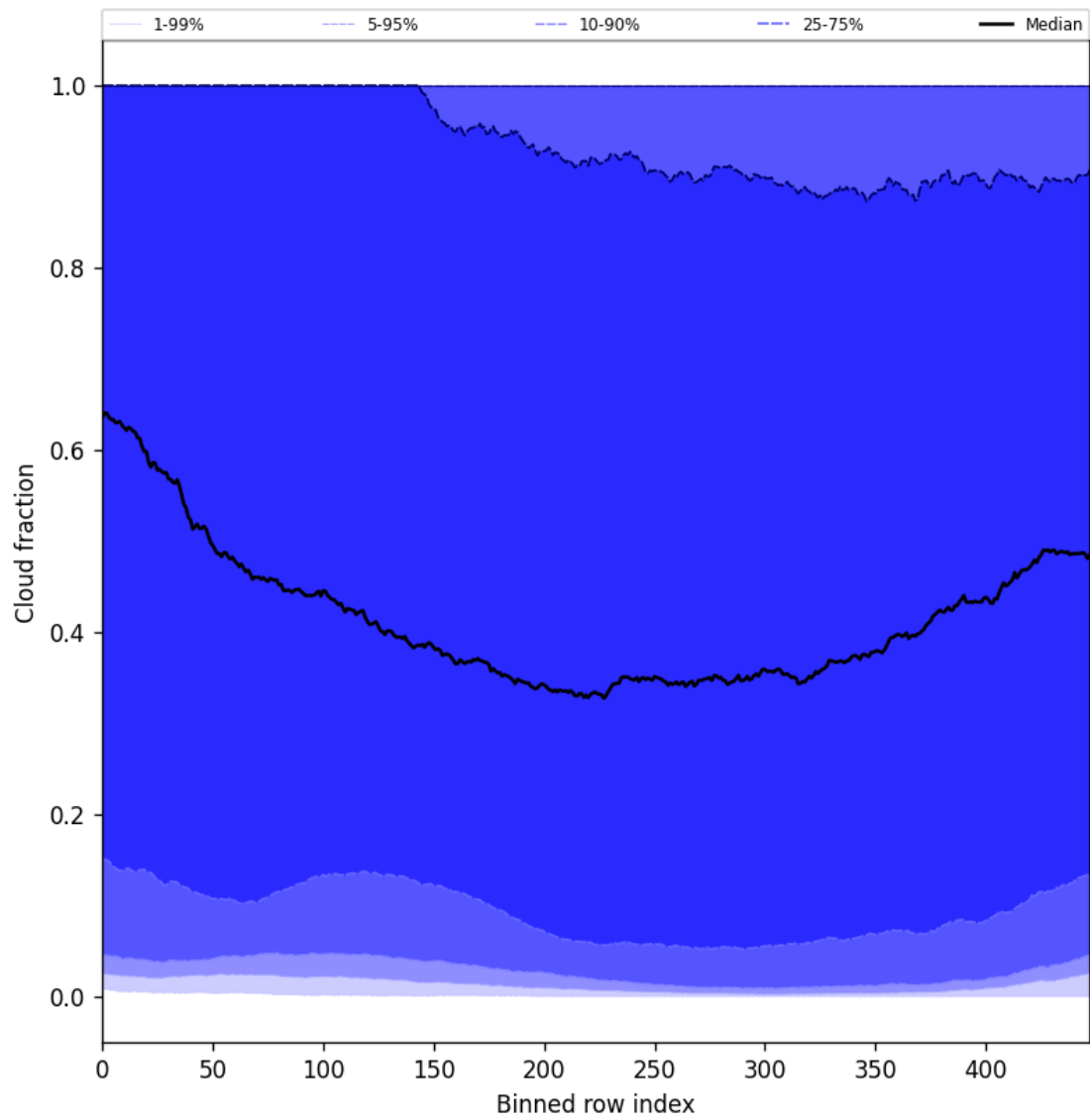
Figure 49: Along track statistics of “Cloud fraction” for 2024-11-09 to 2024-11-10
