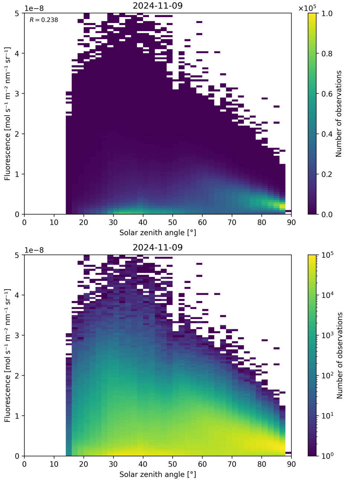
Figure 123: Scatter density plot of “Solar zenith angle” against “Fluorescence” for 2024-11-09 to 2024-11-10.
