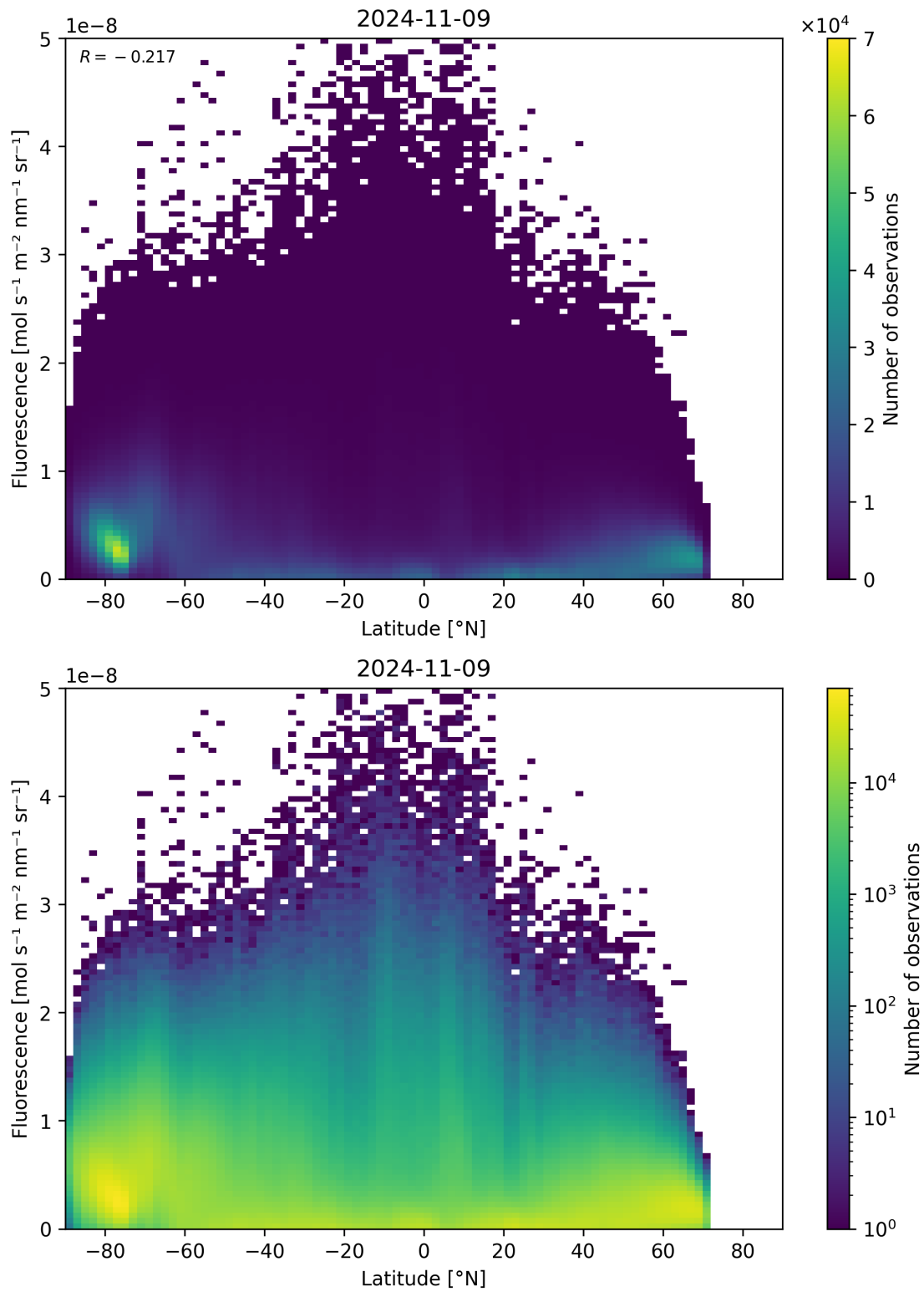
Figure 101: Scatter density plot of “Latitude” against “Fluorescence” for 2024-11-09 to 2024-11-10.
