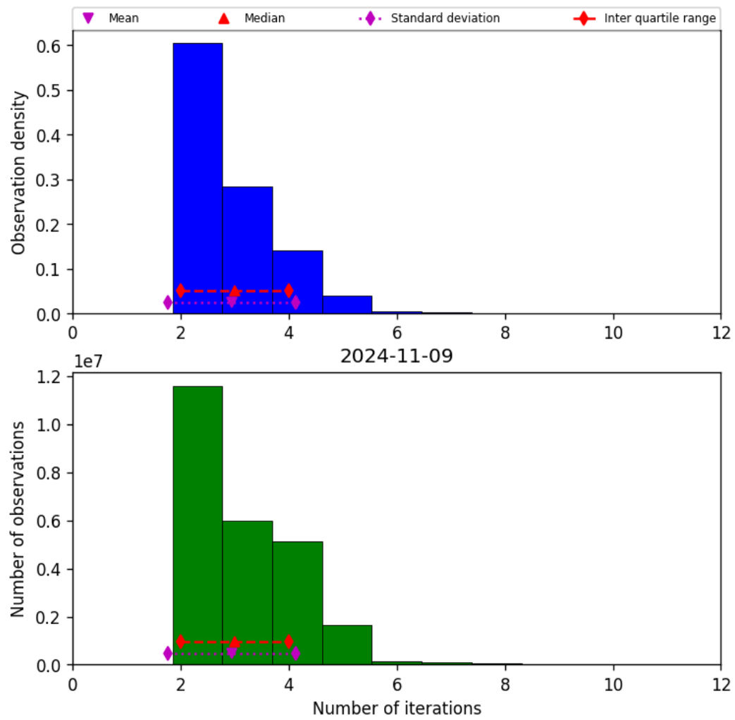
Figure 39: Histogram of “Number of iterations” for 2024-11-09 to 2024-11-10
