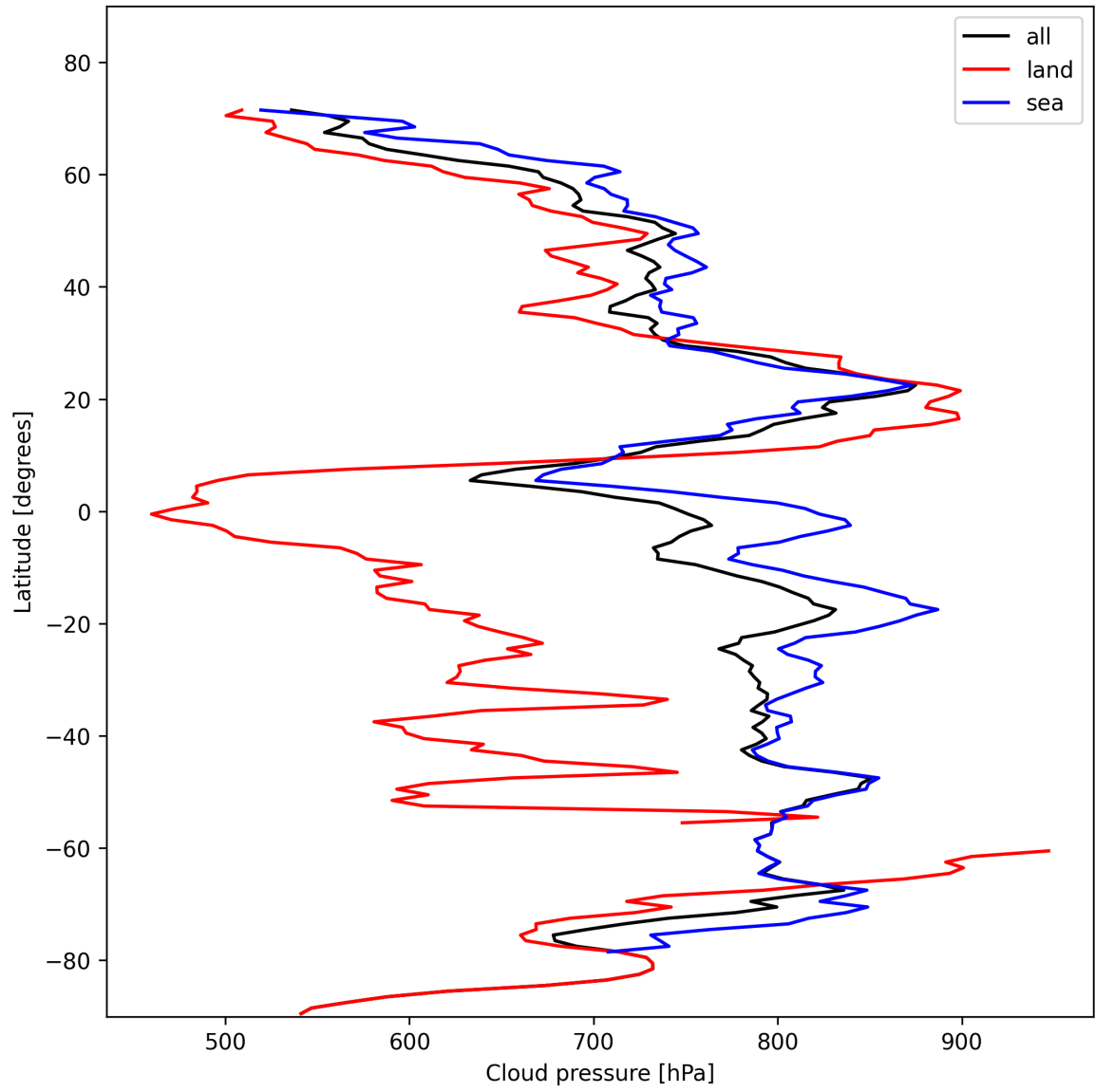
Figure 13: Zonal average of “Cloud pressure” for 2024-11-09 to 2024-11-10.
