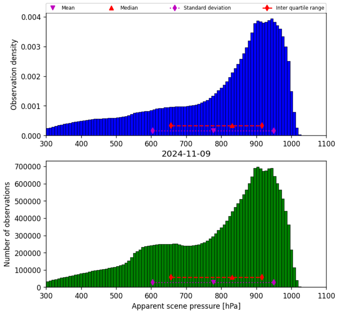
Figure 36: Histogram of “Apparent scene pressure” for 2024-11-09 to 2024-11-10
