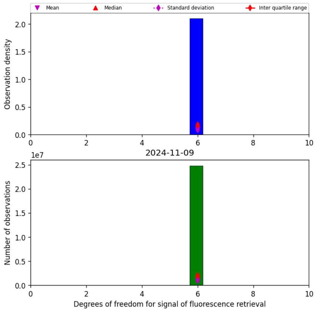
Figure 43: Histogram of “Degrees of freedom for signal of fluorescence retrieval” for 2024-11-09 to 2024-11-10
