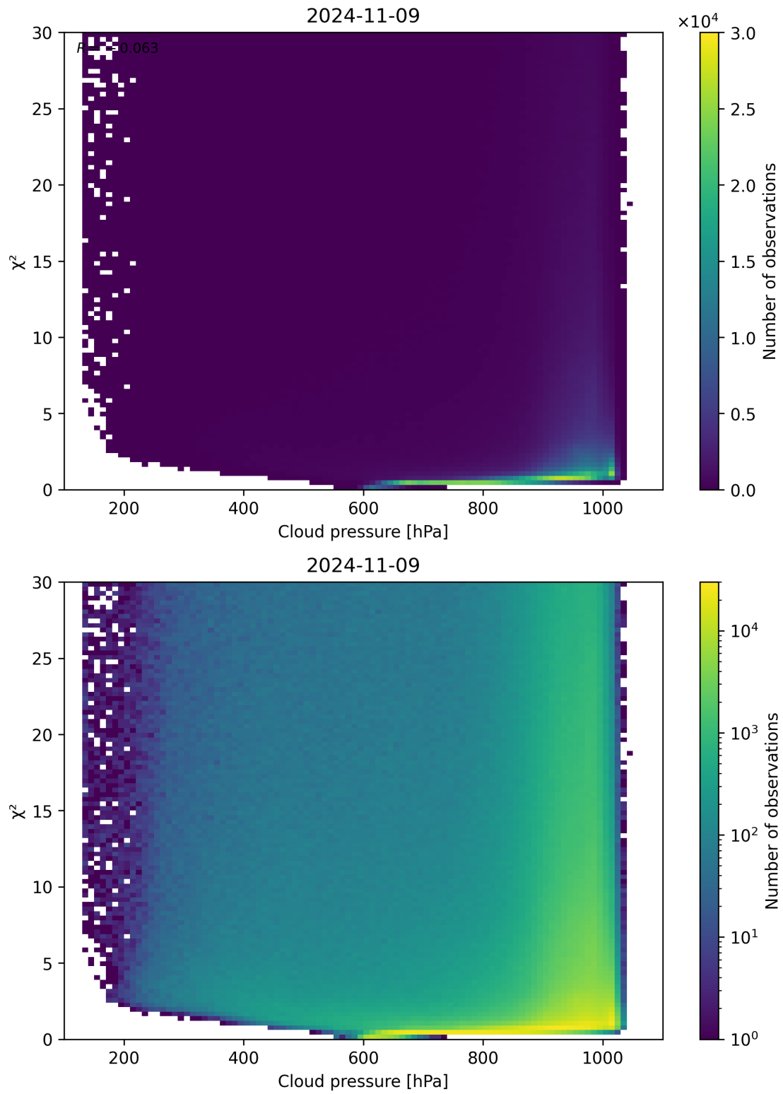
Figure 85: Scatter density plot of “Cloud pressure” against “ \chi^2 ” for 2024-11-09 to 2024-11-10.
