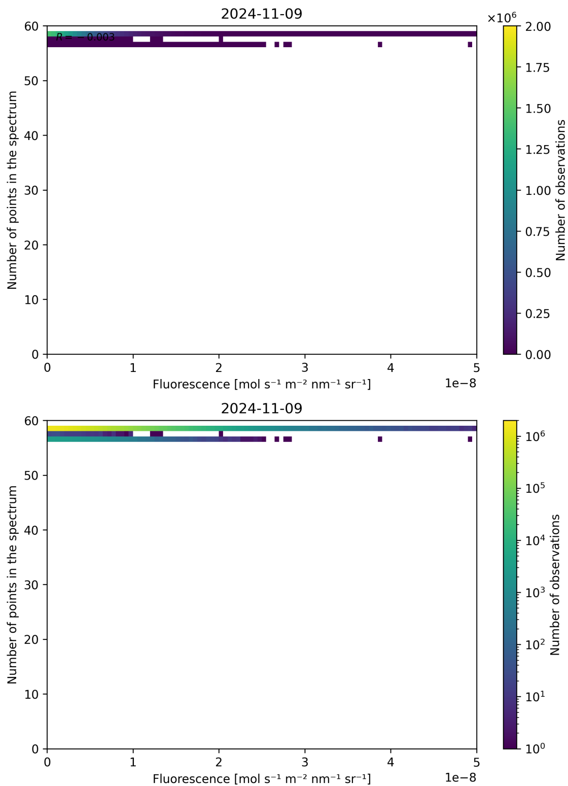
Figure 94: Scatter density plot of “Fluorescence” against “Number of points in the spectrum” for 2024-11-09 to 2024-11-10.
