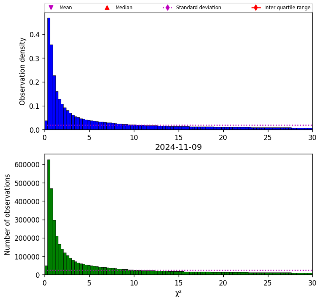
Figure 38: Histogram of “ \chi^2 ” for 2024-11-09 to 2024-11-10
