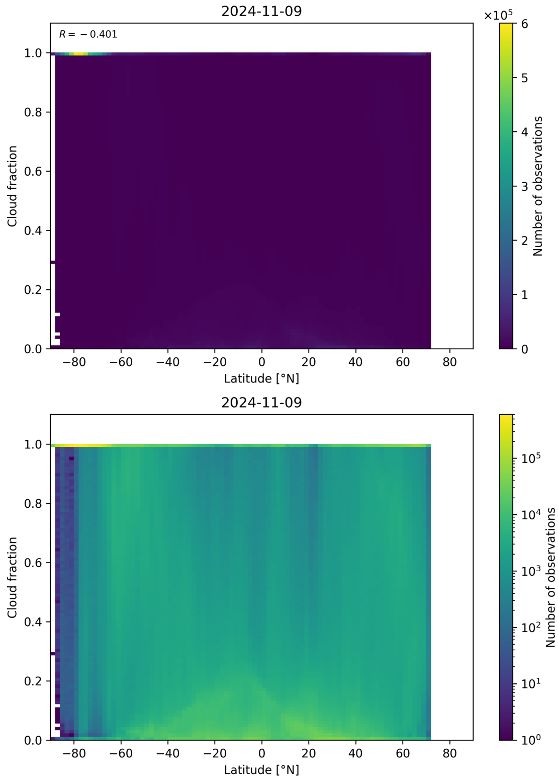
Figure 99: Scatter density plot of “Latitude” against “Cloud fraction” for 2024-11-09 to 2024-11-10.
