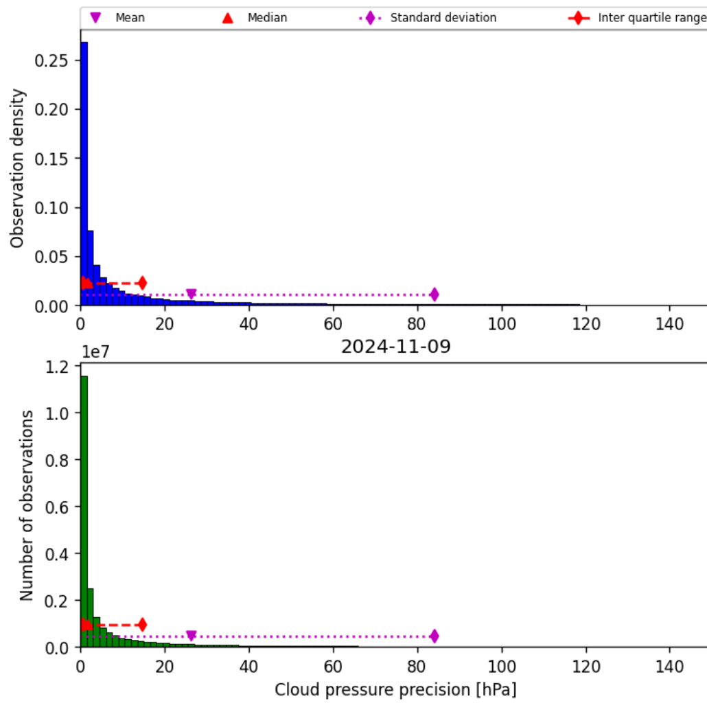
Figure 31: Histogram of “Cloud pressure precision” for 2024-11-09 to 2024-11-10
