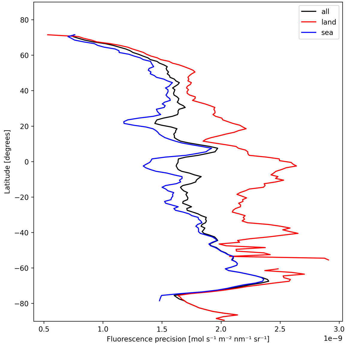
Figure 24: Zonal average of “Fluorescence precision” for 2024-11-09 to 2024-11-10.
