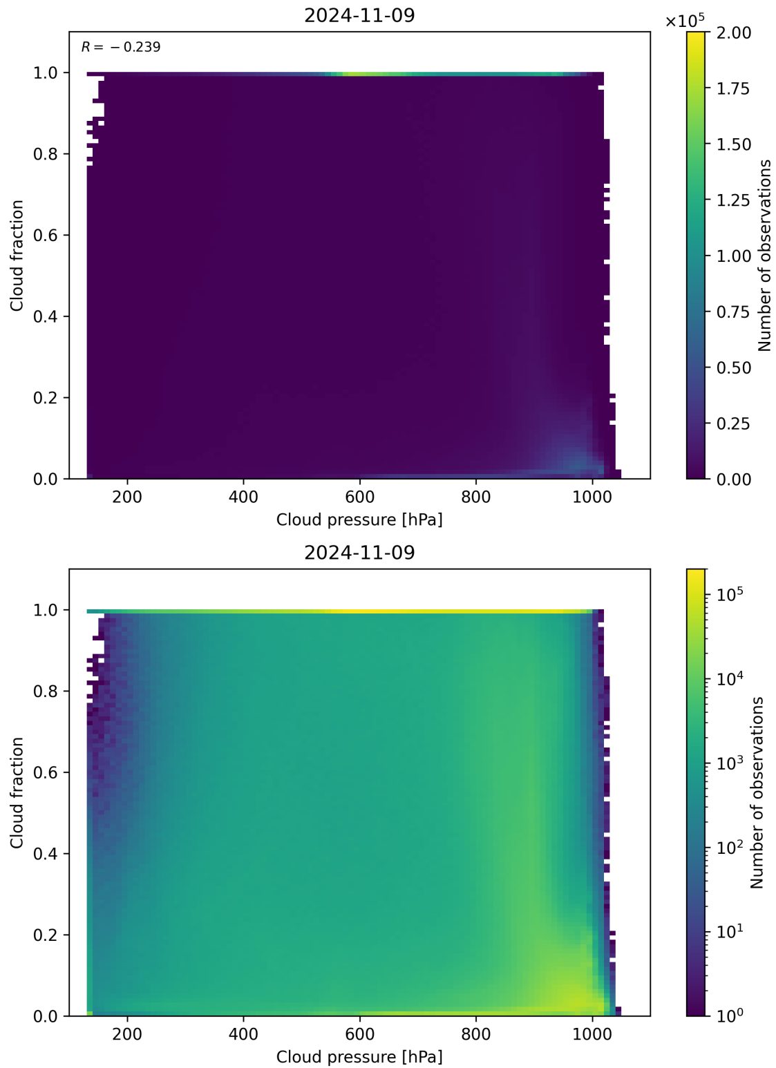
Figure 87: Scatter density plot of “Cloud pressure” against “Cloud fraction” for 2024-11-09 to 2024-11-10.
