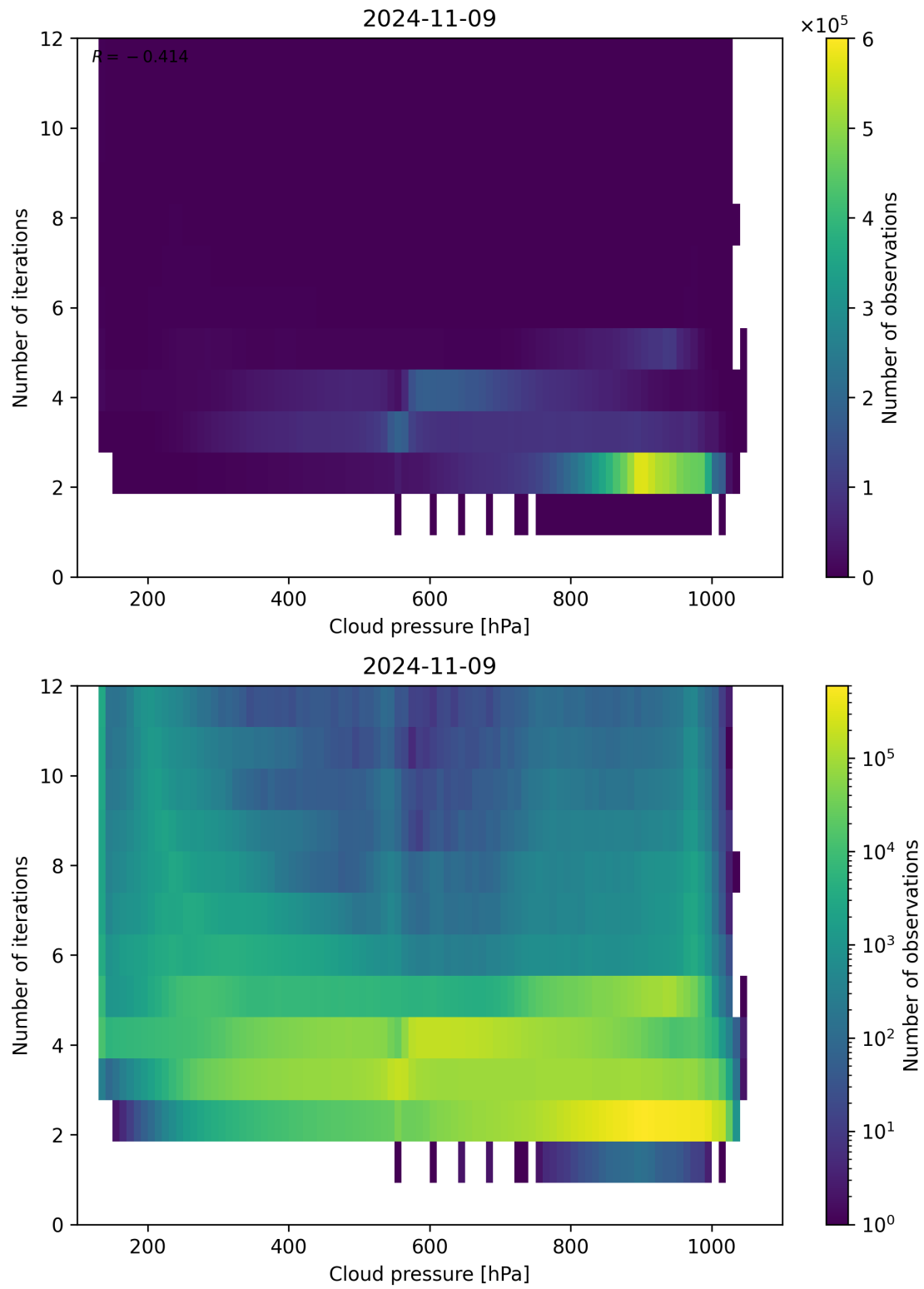
Figure 89: Scatter density plot of “Cloud pressure” against “Number of iterations” for 2024-11-09 to 2024-11-10.
