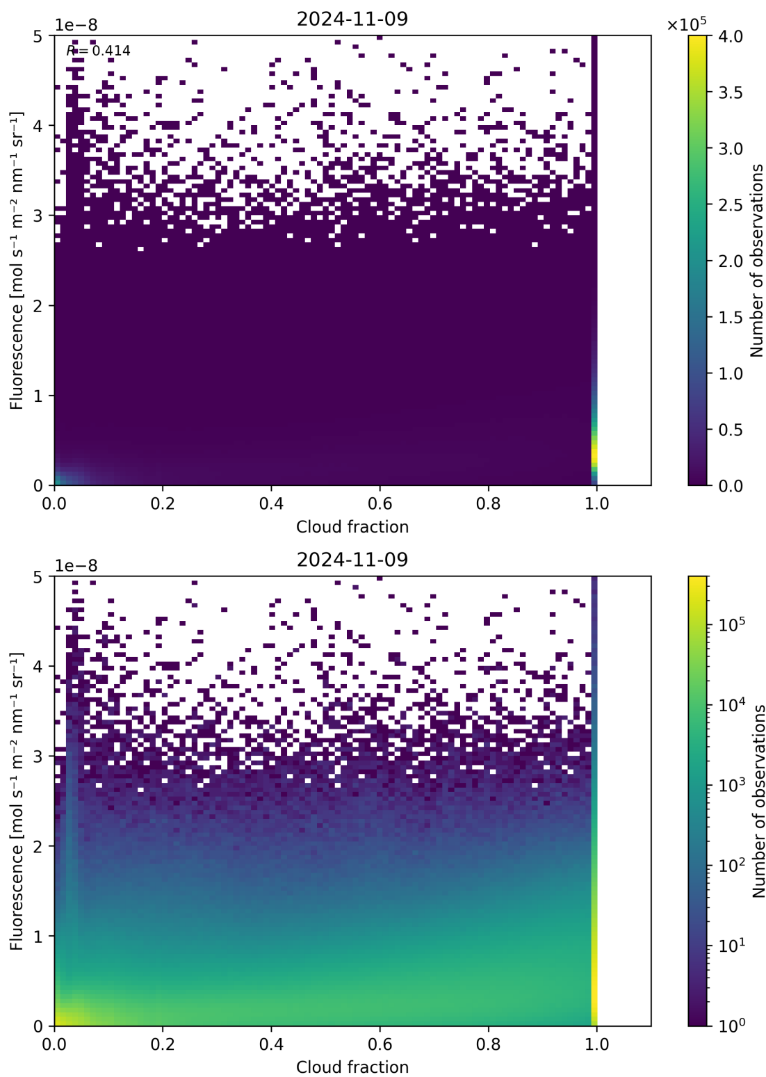
Figure 79: Scatter density plot of “Cloud fraction” against “Fluorescence” for 2024-11-09 to 2024-11-10.
