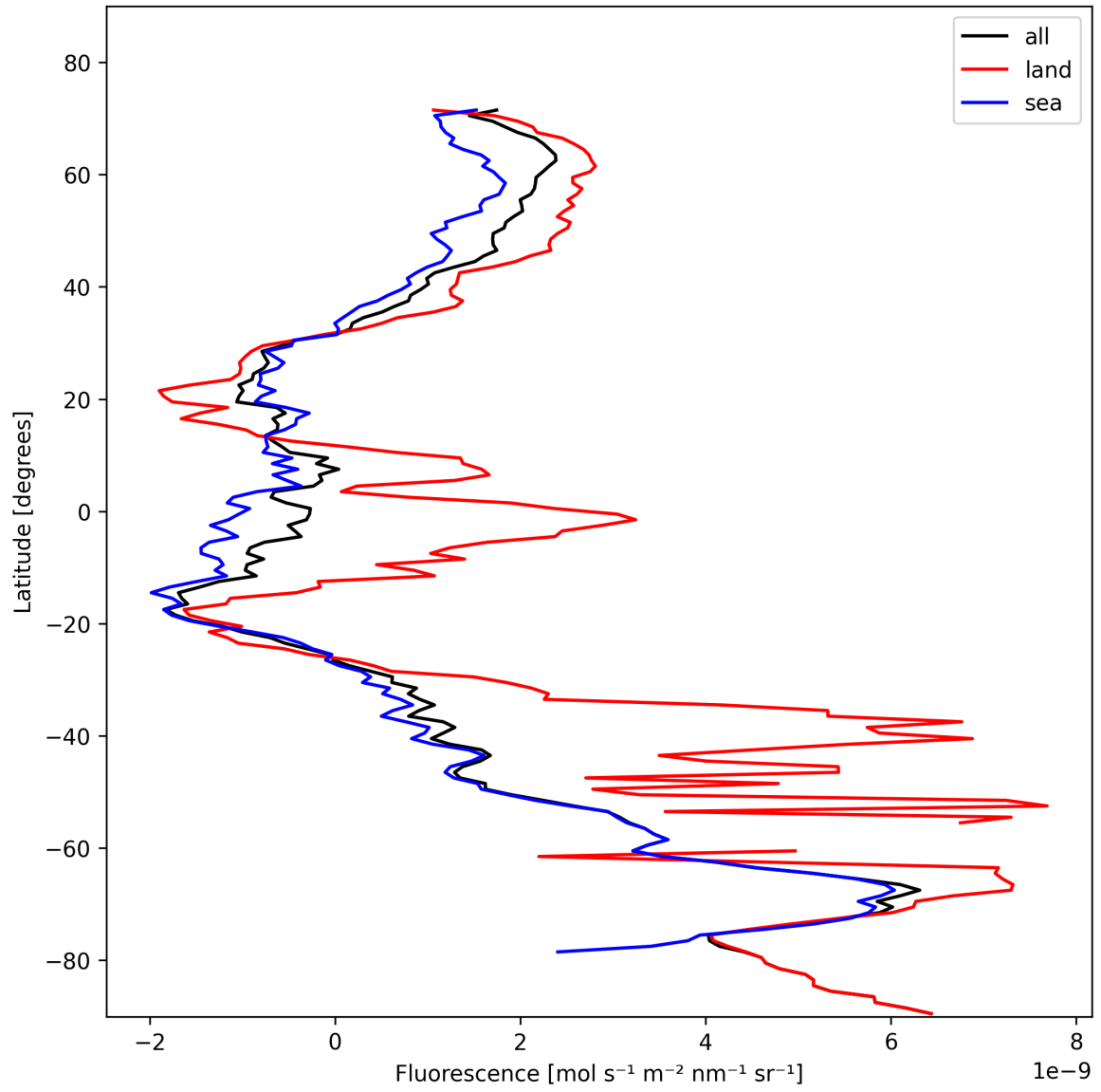
Figure 23: Zonal average of “Fluorescence” for 2024-11-09 to 2024-11-10.
