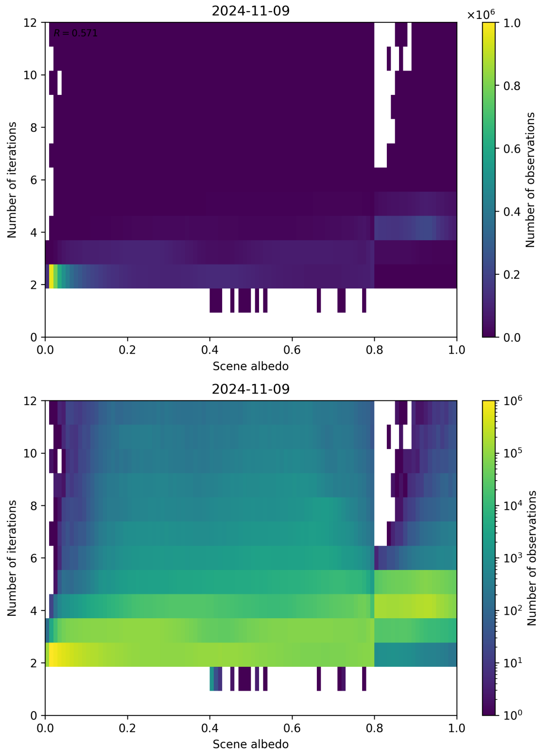
Figure 115: Scatter density plot of “Scene albedo” against “Number of iterations” for 2024-11-09 to 2024-11-10.
