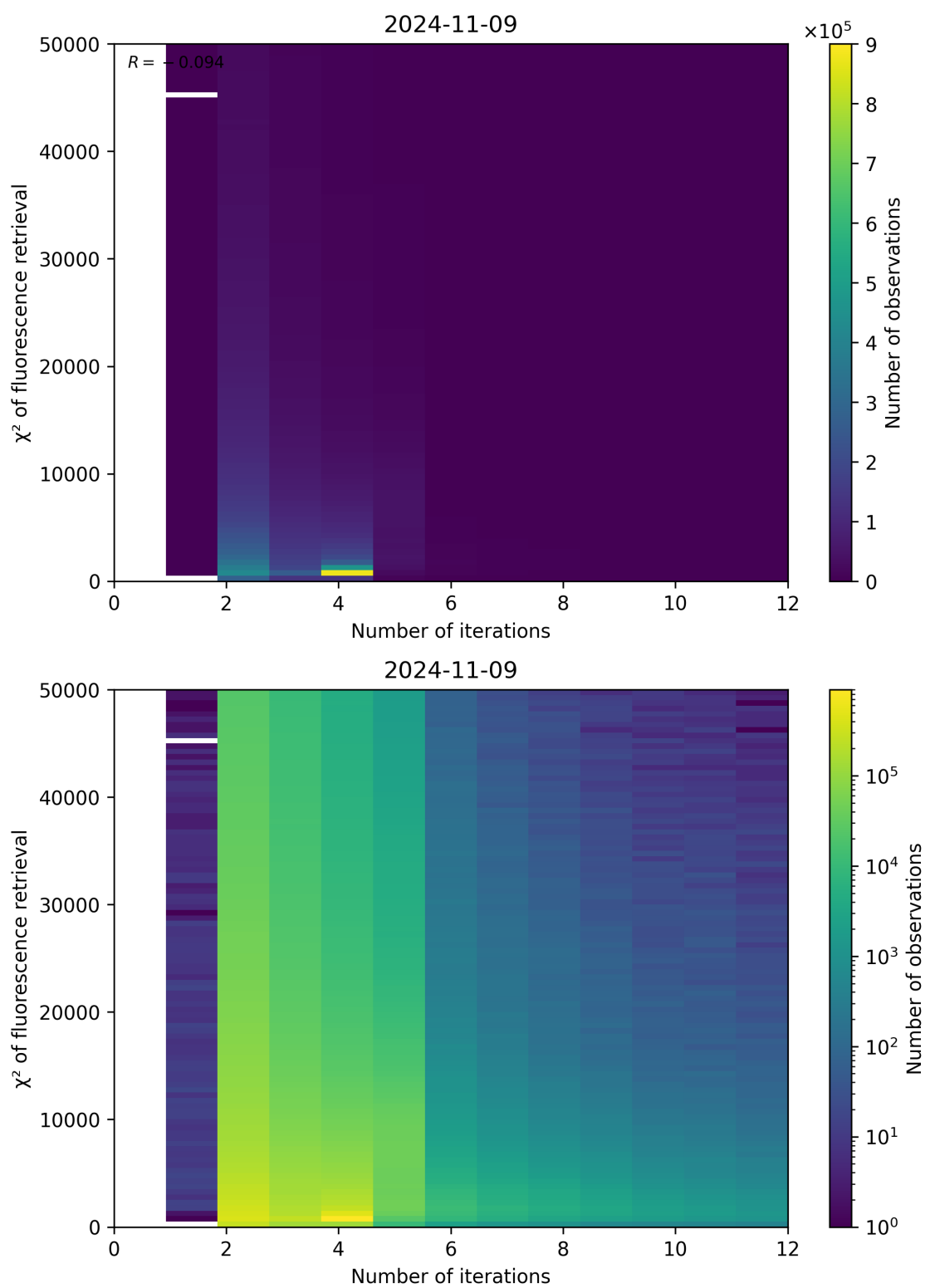
Figure 106: Scatter density plot of “Number of iterations” against “ \chi^2 of fluorescence retrieval” for 2024-11-09 to 2024-11-10.
