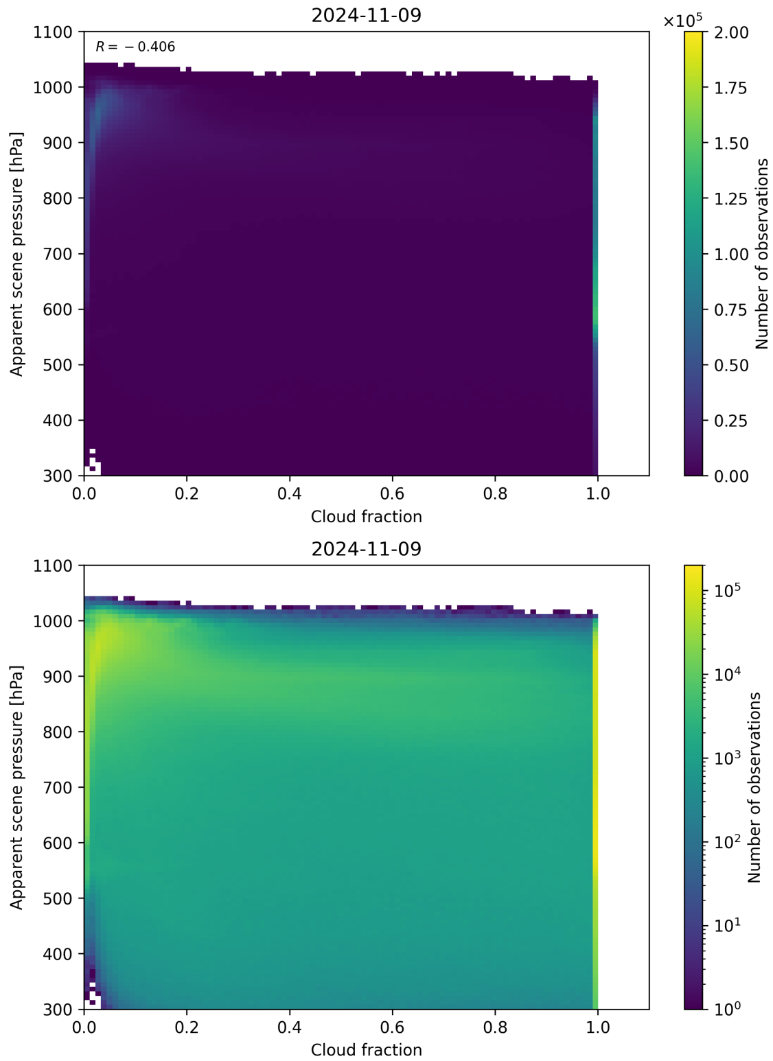
Figure 76: Scatter density plot of “Cloud fraction” against “Apparent scene pressure” for 2024-11-09 to 2024-11-10.
