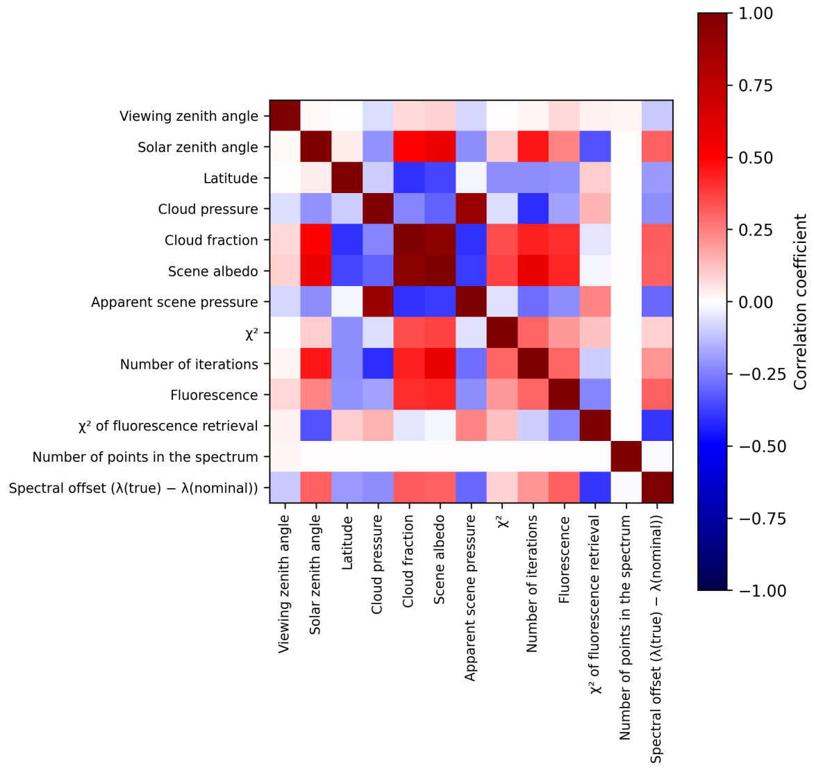
Figure 2: Map of correlation matrix for 2024-11-09 to 2024-11-10.
