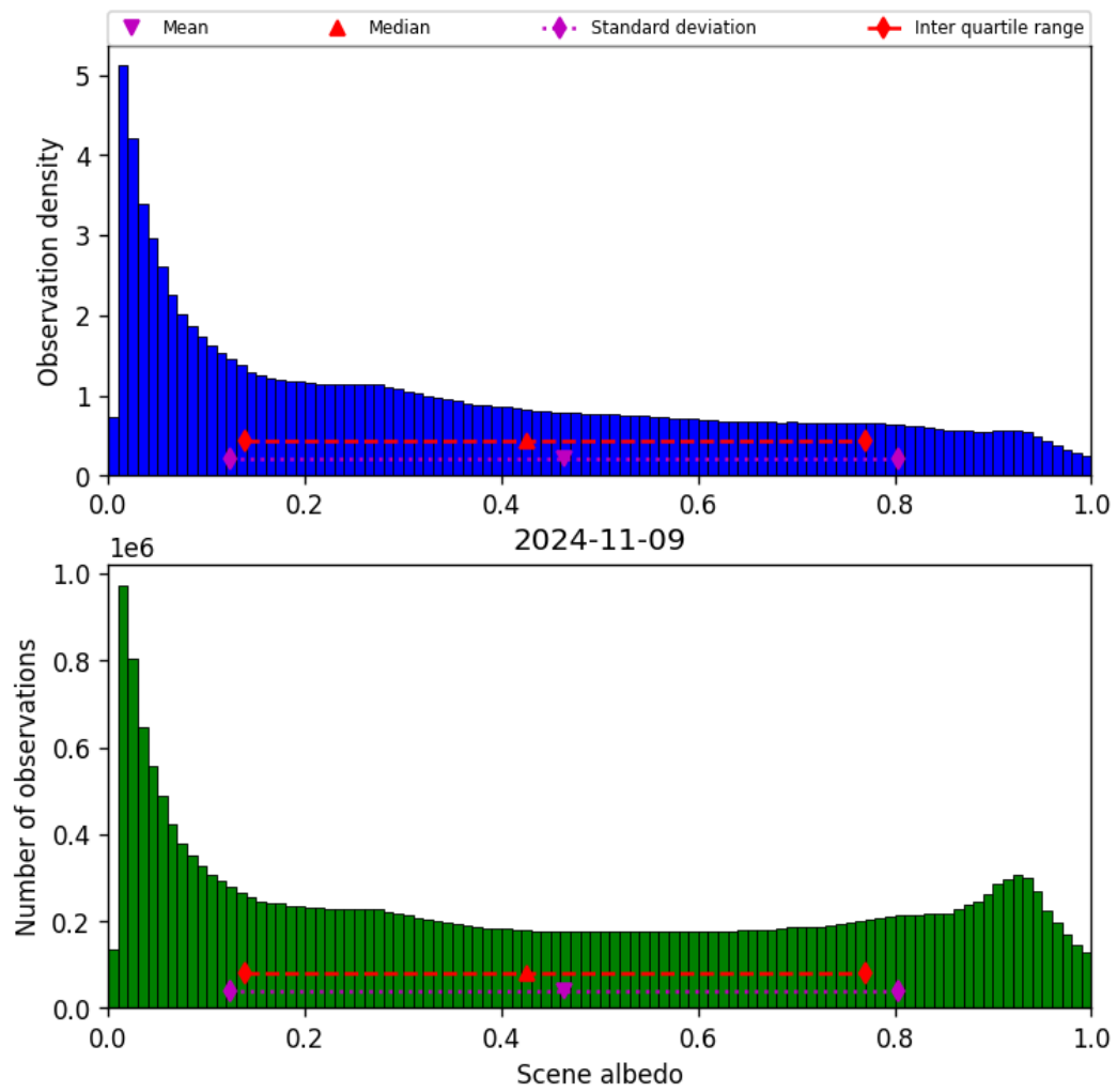
Figure 34: Histogram of “Scene albedo” for 2024-11-09 to 2024-11-10
