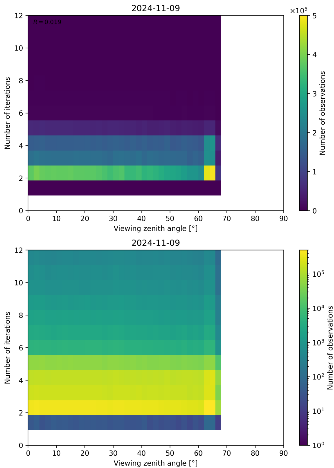
Figure 136: Scatter density plot of “Viewing zenith angle” against “Number of iterations” for 2024-11-09 to 2024-11-10.
