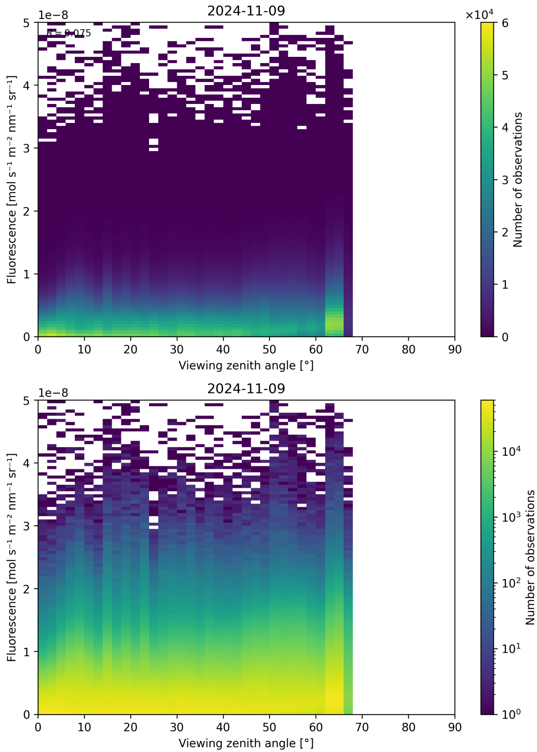
Figure 134: Scatter density plot of “Viewing zenith angle” against “Fluorescence” for 2024-11-09 to 2024-11-10.
