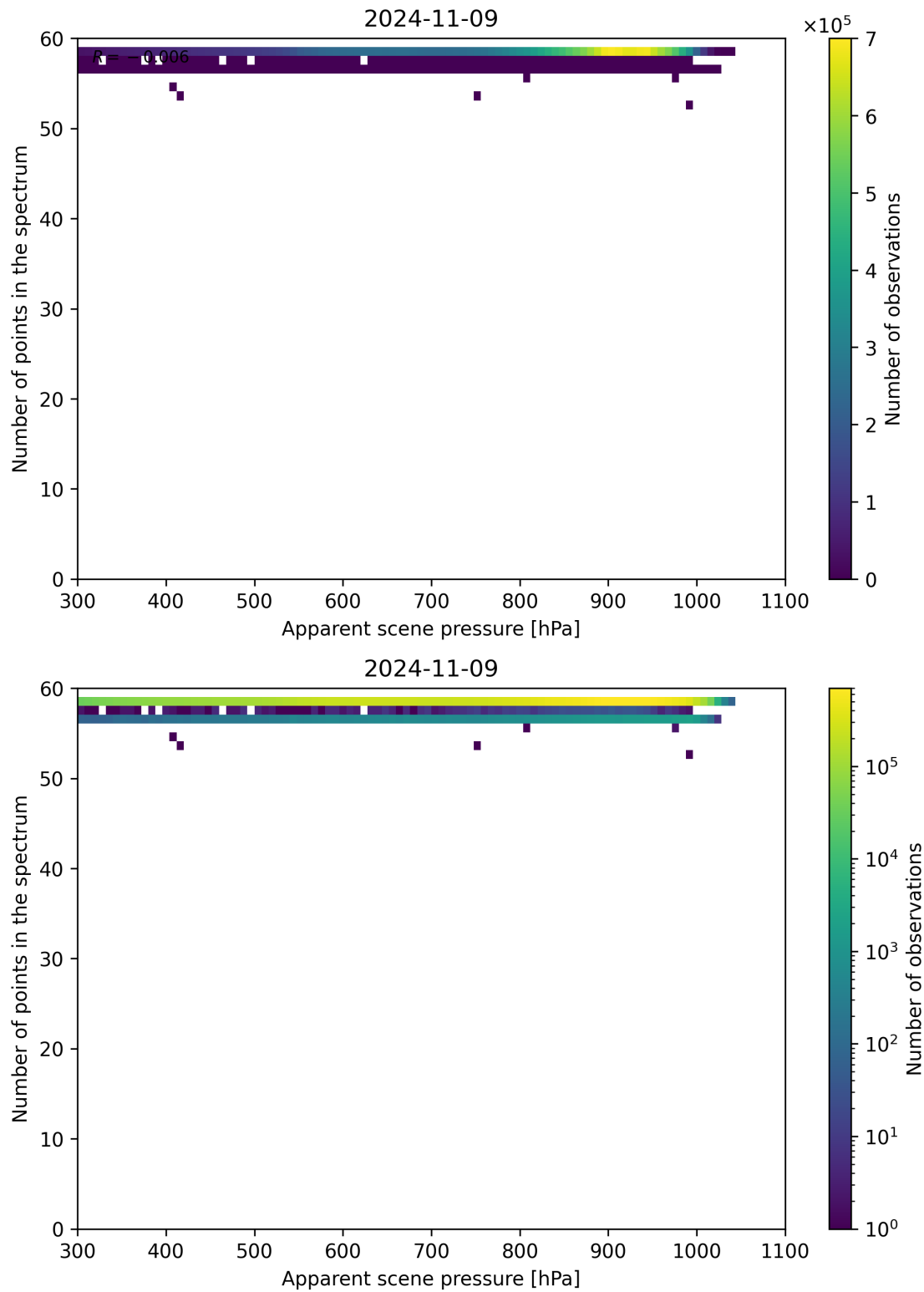
Figure 67: Scatter density plot of “Apparent scene pressure” against “Number of points in the spectrum” for 2024-11-09 to 2024-11-10.
