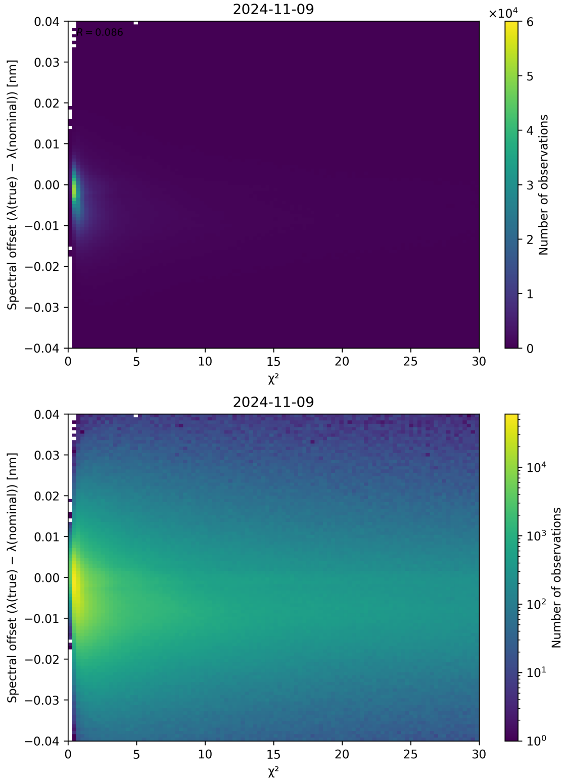
Figure 75: Scatter density plot of “ \chi^2 ” against “Spectral offset ( \lambda_{\text{true}} - \lambda_{\text{nominal}} )” for 2024-11-09 to 2024-11-10.
