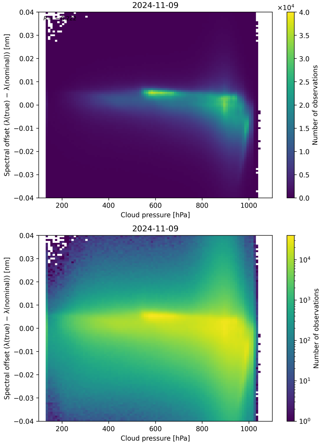
Figure 92: Scatter density plot of “Cloud pressure” against “Spectral offset ( \lambda_{\text{true}} - \lambda_{\text{nominal}} )” for 2024-11-09 to 2024-11-10.
