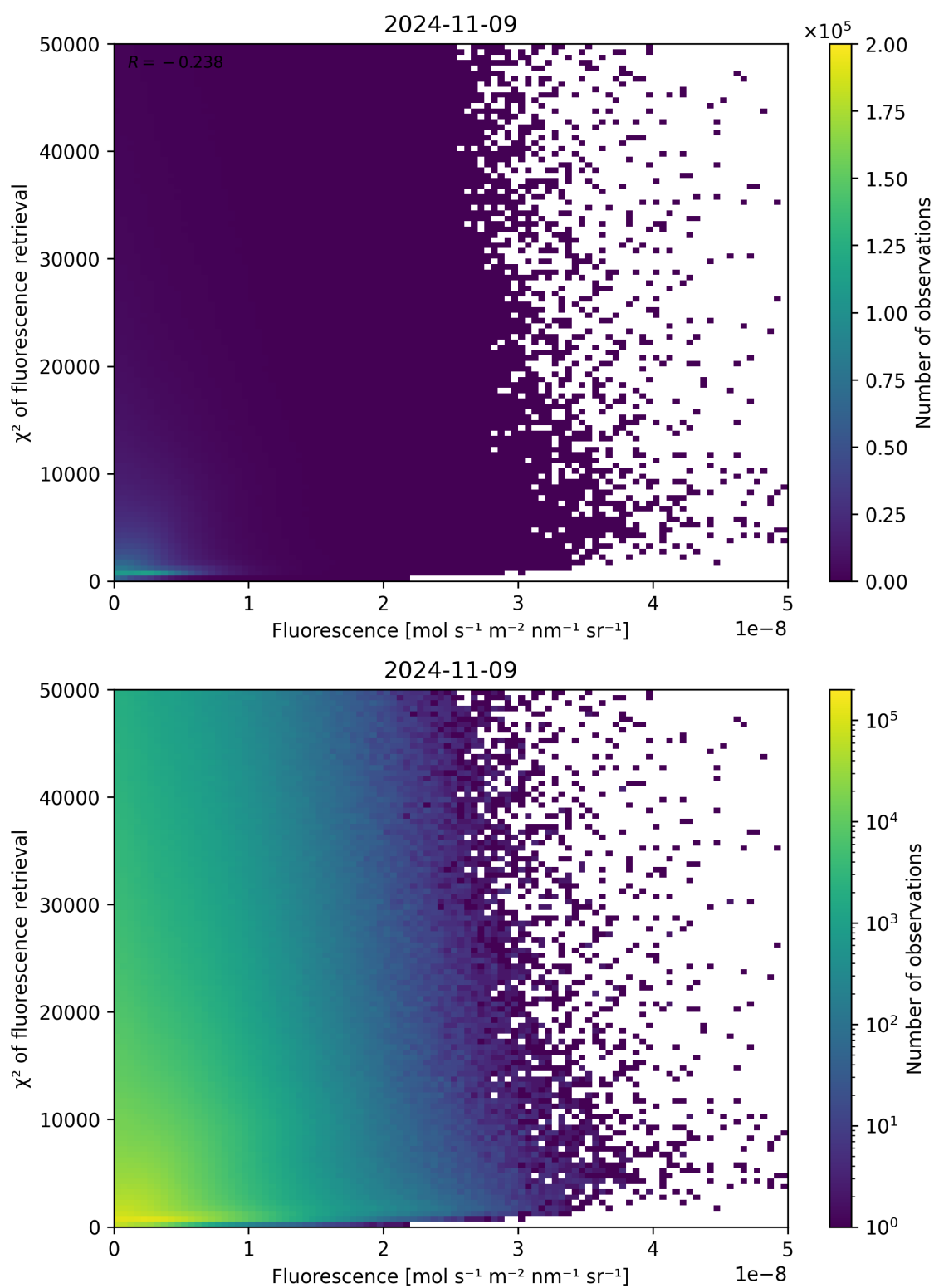
Figure 93: Scatter density plot of “Fluorescence” against “ \chi^2 of fluorescence retrieval” for 2024-11-09 to 2024-11-10.
