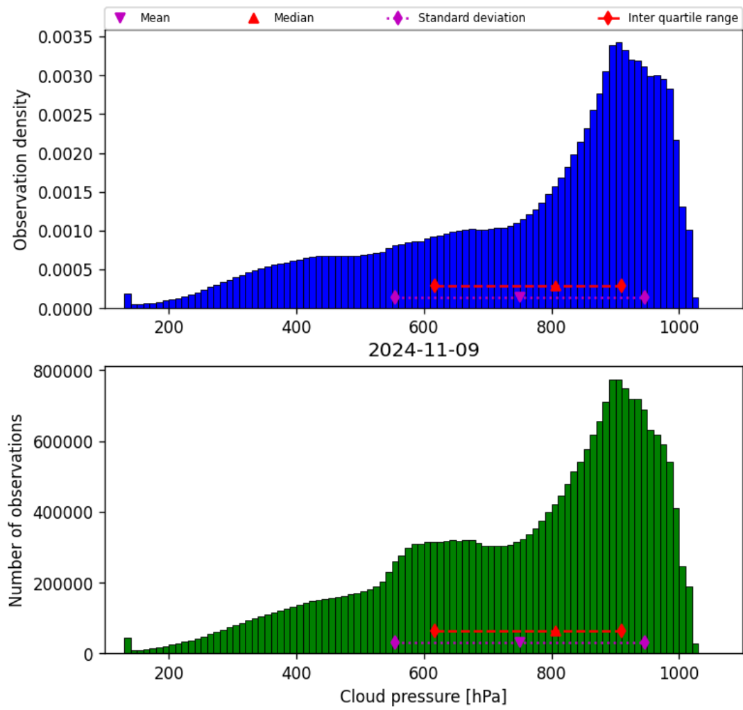
Figure 30: Histogram of “Cloud pressure” for 2024-11-09 to 2024-11-10
