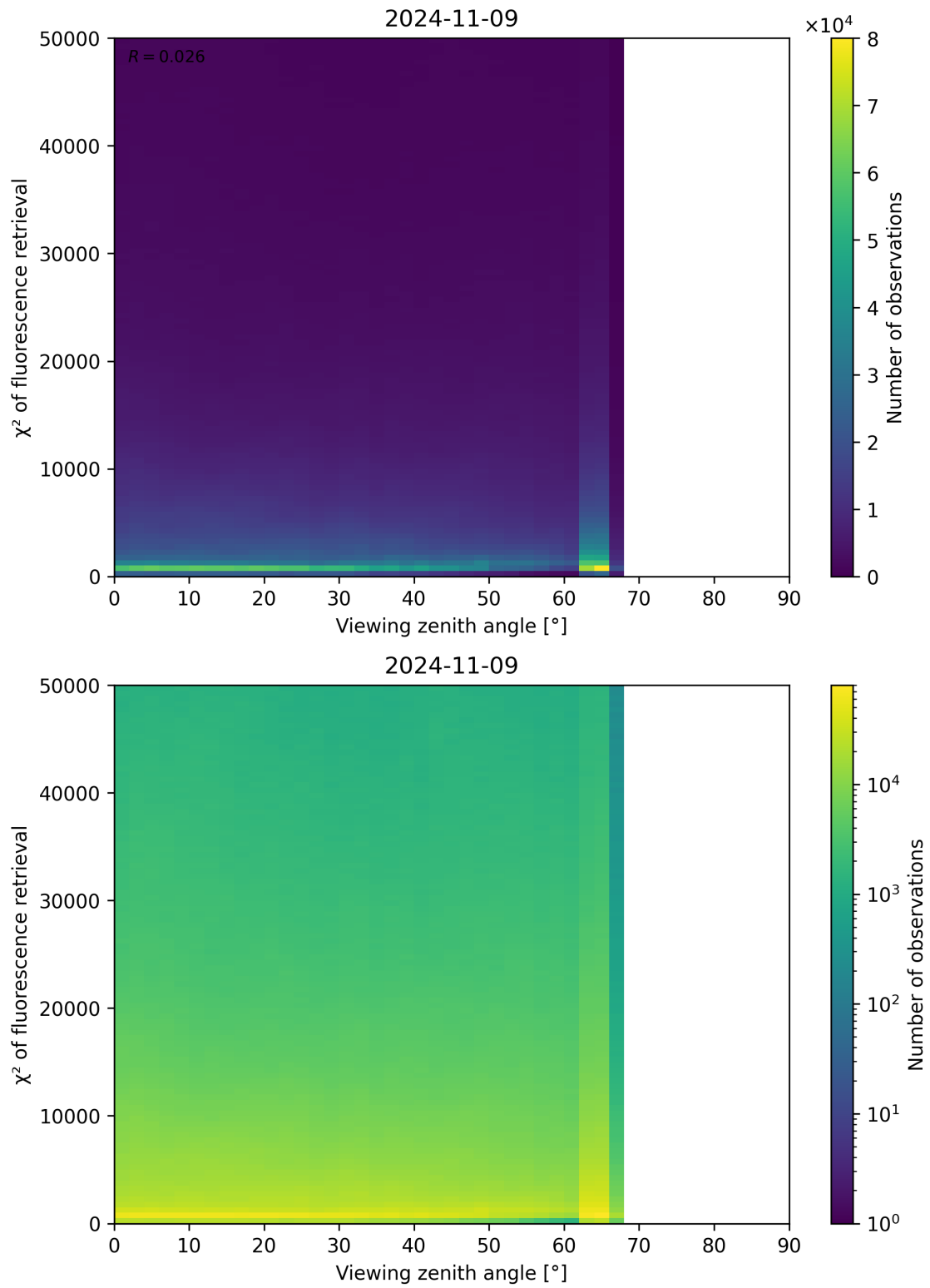
Figure 131: Scatter density plot of “Viewing zenith angle” against “ \chi^2 of fluorescence retrieval” for 2024-11-09 to 2024-11-10.
