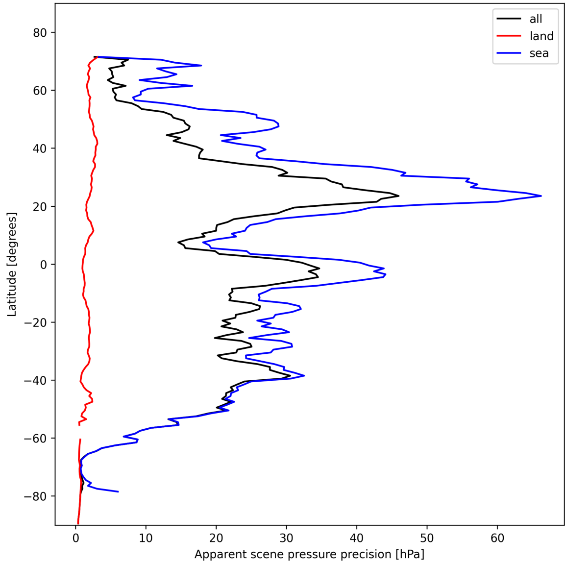
Figure 20: Zonal average of “Apparent scene pressure precision” for 2024-11-09 to 2024-11-10.
