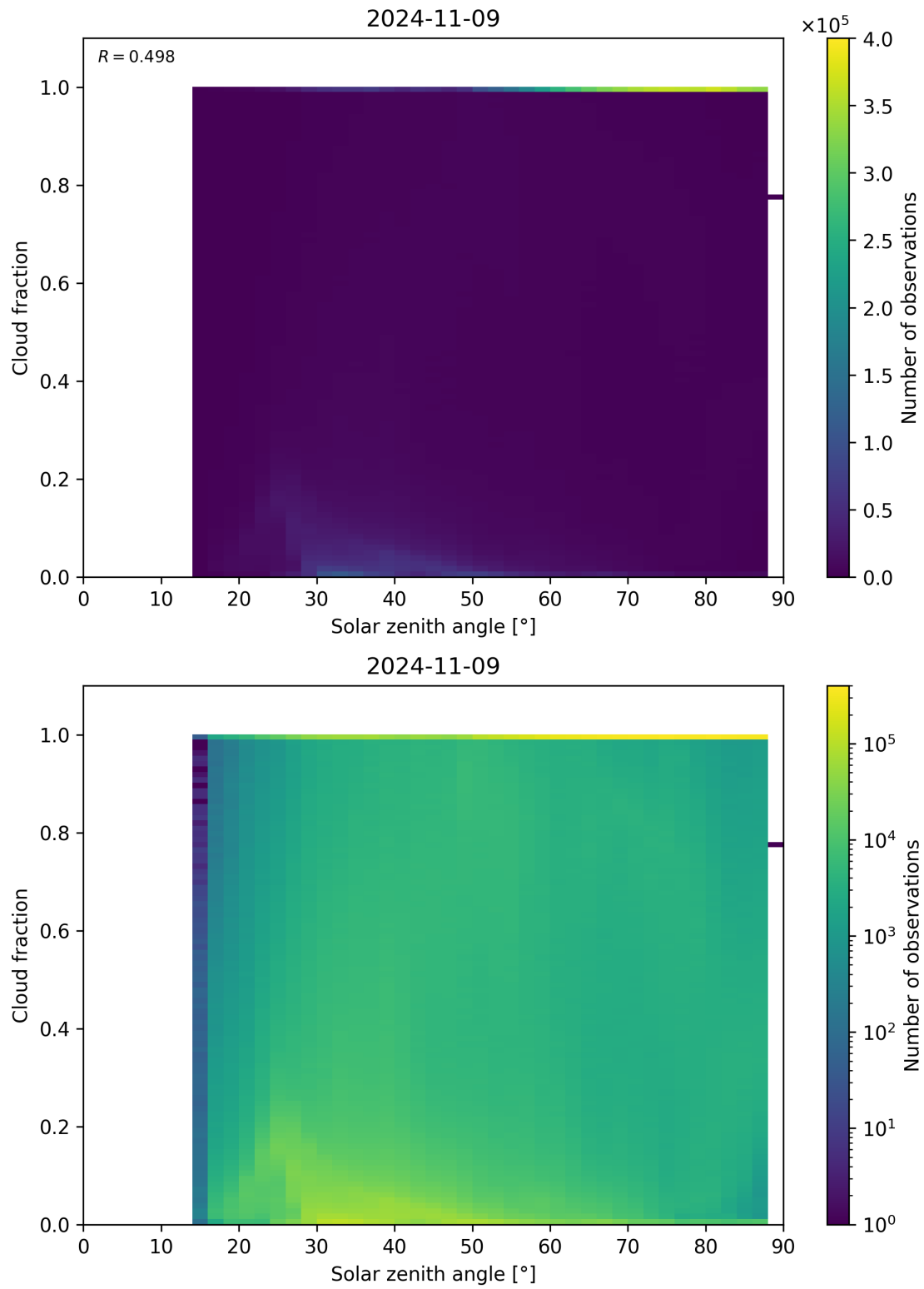
Figure 121: Scatter density plot of “Solar zenith angle” against “Cloud fraction” for 2024-11-09 to 2024-11-10.
