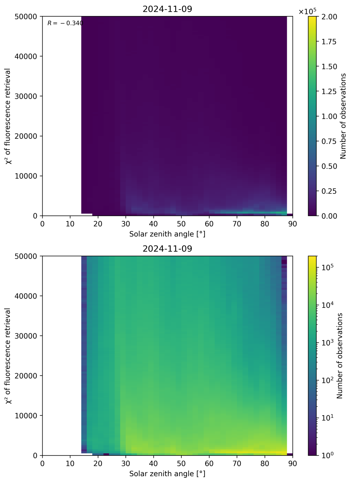
Figure 120: Scatter density plot of “Solar zenith angle” against “ \chi^2 of fluorescence retrieval” for 2024-11-09 to 2024-11-10.
