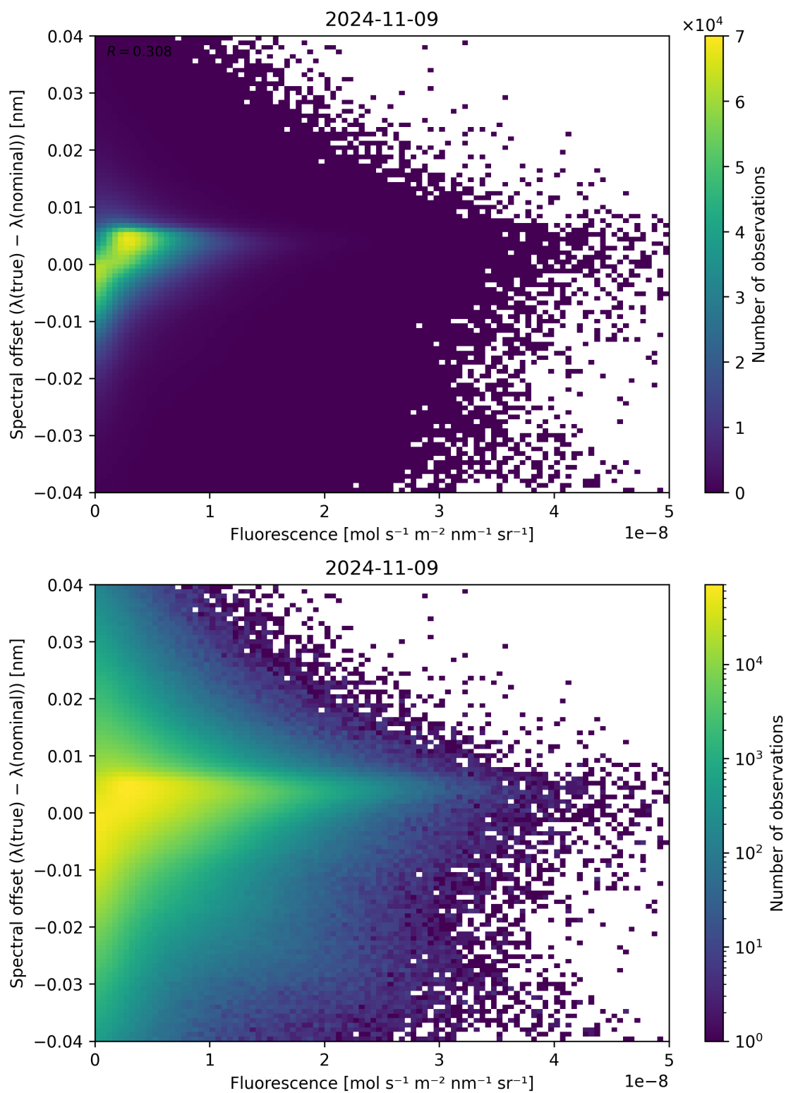
Figure 95: Scatter density plot of “Fluorescence” against “Spectral offset ( \lambda_{\text{true}} - \lambda_{\text{nominal}} )” for 2024-11-09 to 2024-11-10.
