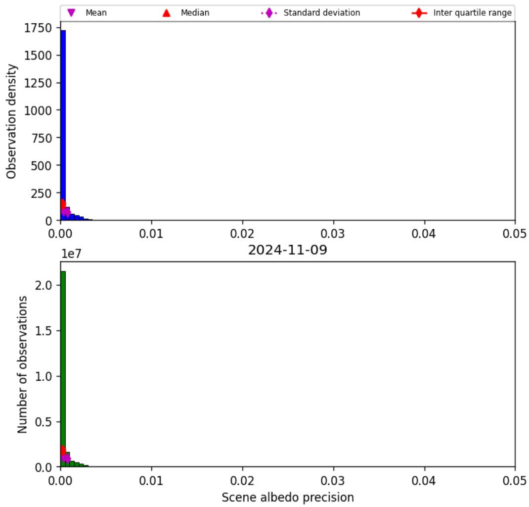
Figure 35: Histogram of “Scene albedo precision” for 2024-11-09 to 2024-11-10
