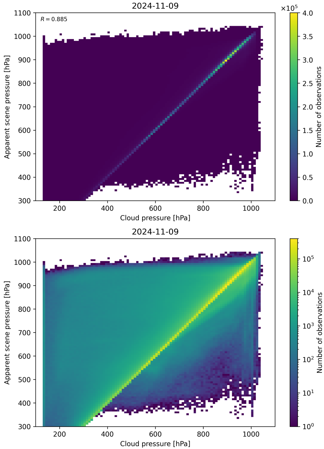
Figure 84: Scatter density plot of “Cloud pressure” against “Apparent scene pressure” for 2024-11-09 to 2024-11-10.
