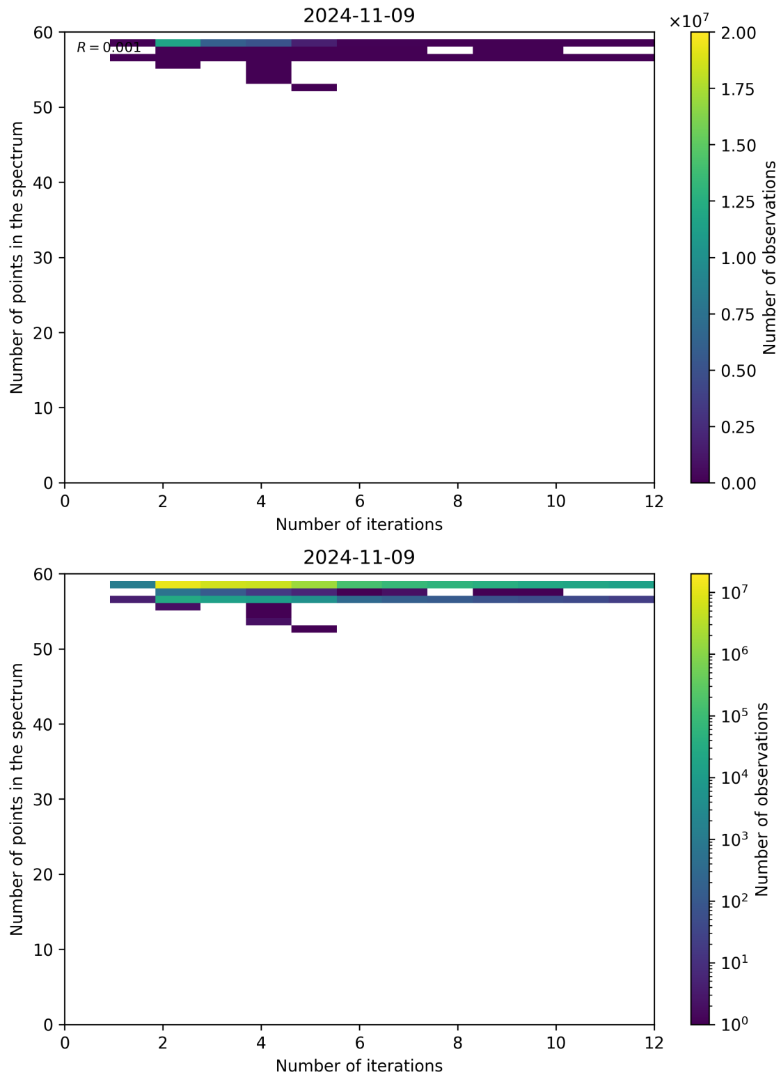
Figure 108: Scatter density plot of “Number of iterations” against “Number of points in the spectrum” for 2024-11-09 to 2024-11-10.
