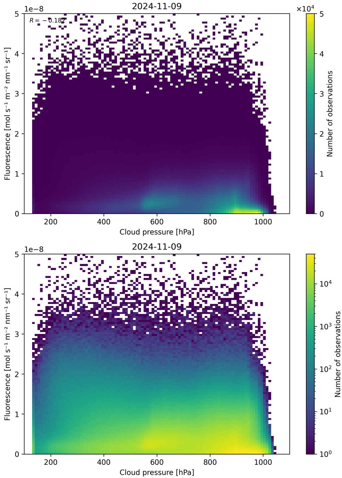
Figure 88: Scatter density plot of “Cloud pressure” against “Fluorescence” for 2024-11-09 to 2024-11-10.
