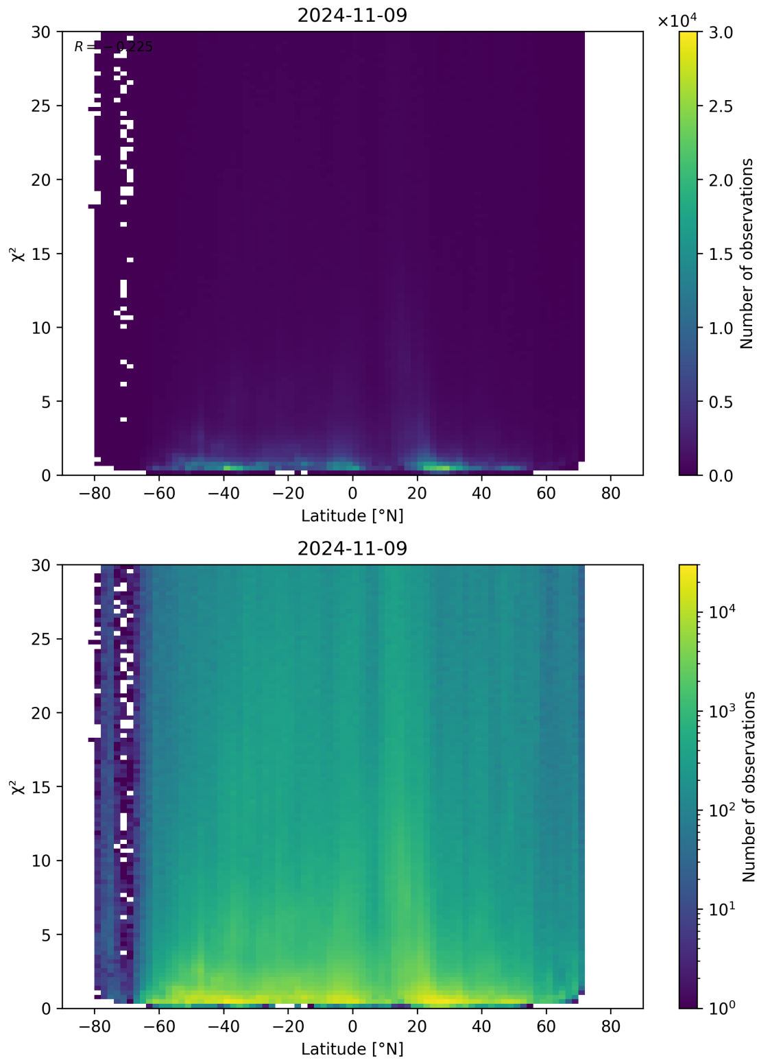
Figure 97: Scatter density plot of “Latitude” against “ \chi^2 ” for 2024-11-09 to 2024-11-10.
