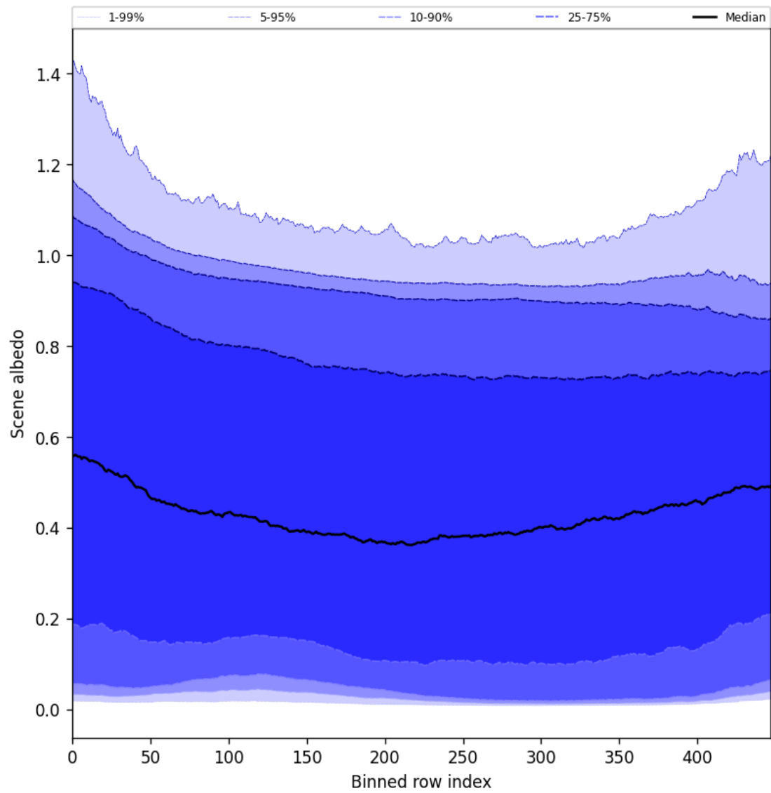
Figure 51: Along track statistics of “Scene albedo” for 2024-11-09 to 2024-11-10
