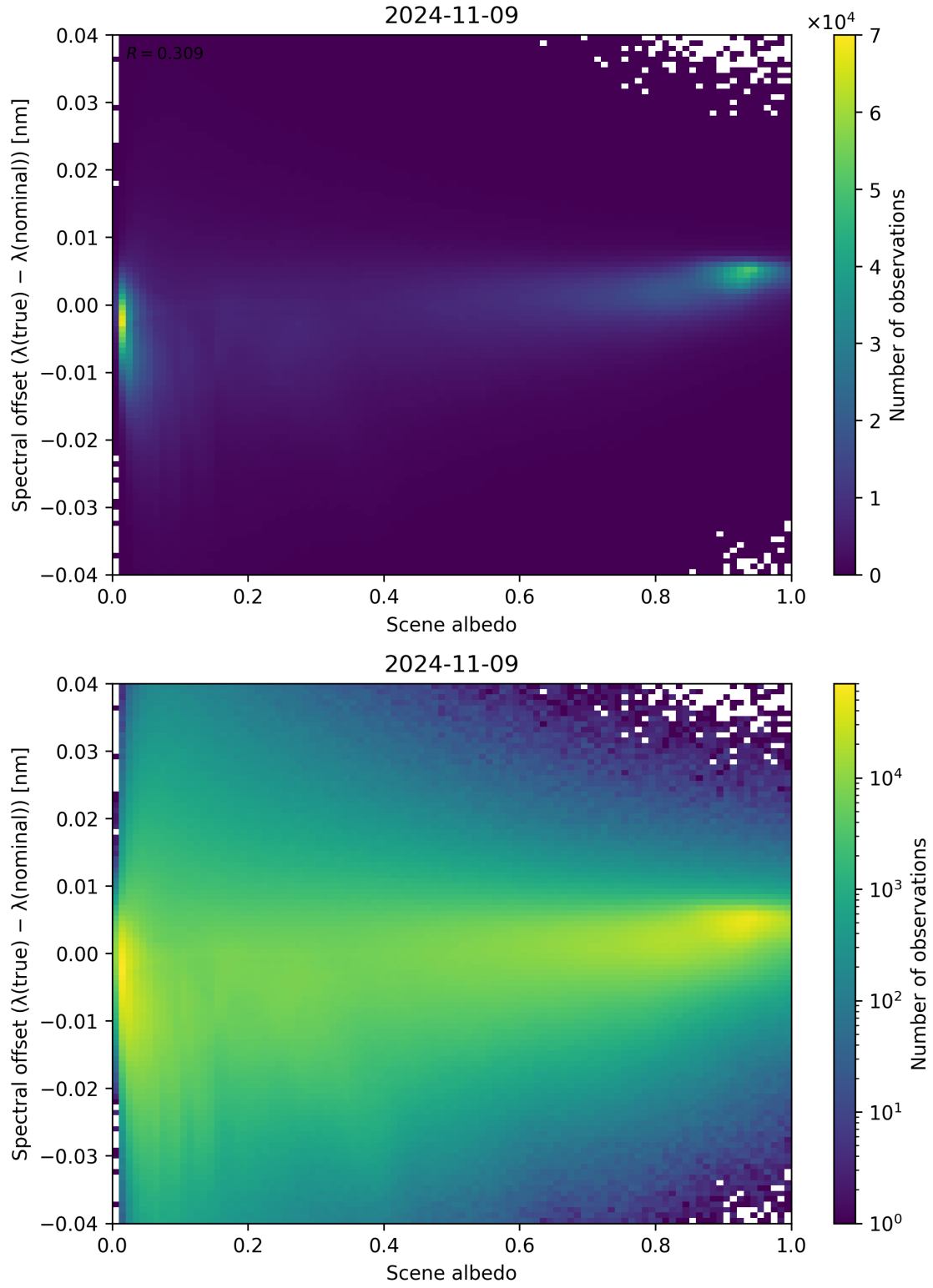
Figure 117: Scatter density plot of “Scene albedo” against “Spectral offset ( \lambda_{\text{true}} - \lambda_{\text{nominal}} )” for 2024-11-09 to 2024-11-10.
