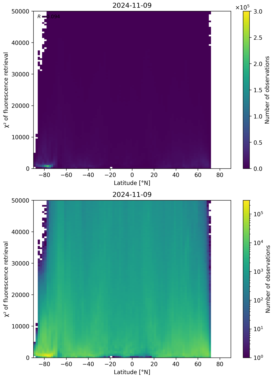
Figure 98: Scatter density plot of “Latitude” against “ \chi^2 of fluorescence retrieval” for 2024-11-09 to 2024-11-10.
