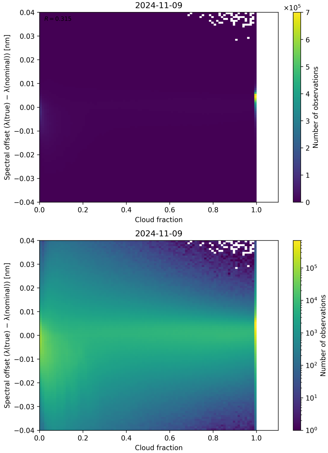
Figure 83: Scatter density plot of “Cloud fraction” against “Spectral offset ( \lambda_{\text{true}} - \lambda_{\text{nominal}} )” for 2024-11-09 to 2024-11-10.
