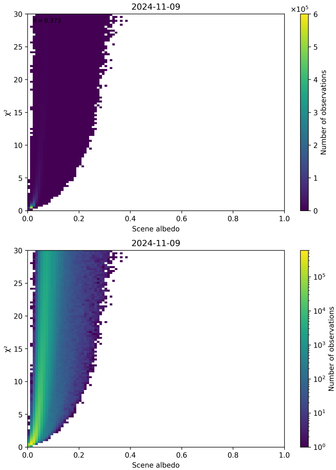
Figure 112: Scatter density plot of “Scene albedo” against “ \chi^2 ” for 2024-11-09 to 2024-11-10.
