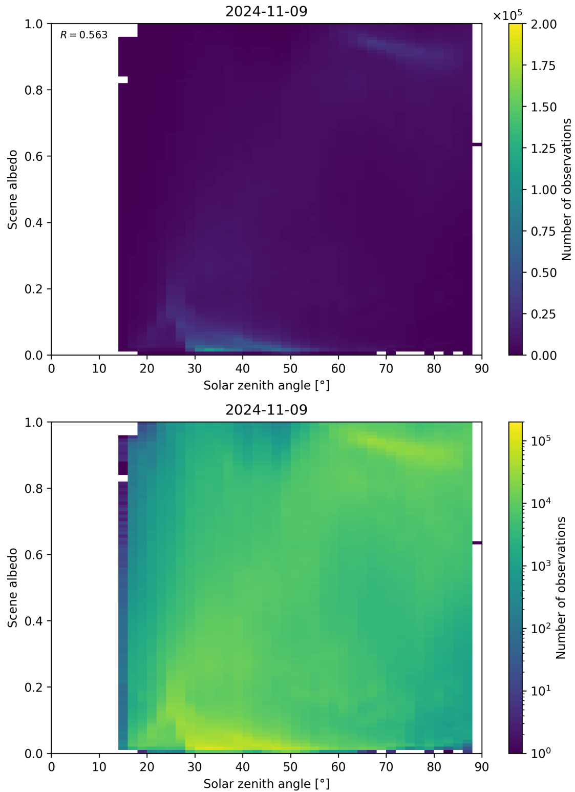
Figure 127: Scatter density plot of “Solar zenith angle” against “Scene albedo” for 2024-11-09 to 2024-11-10.
