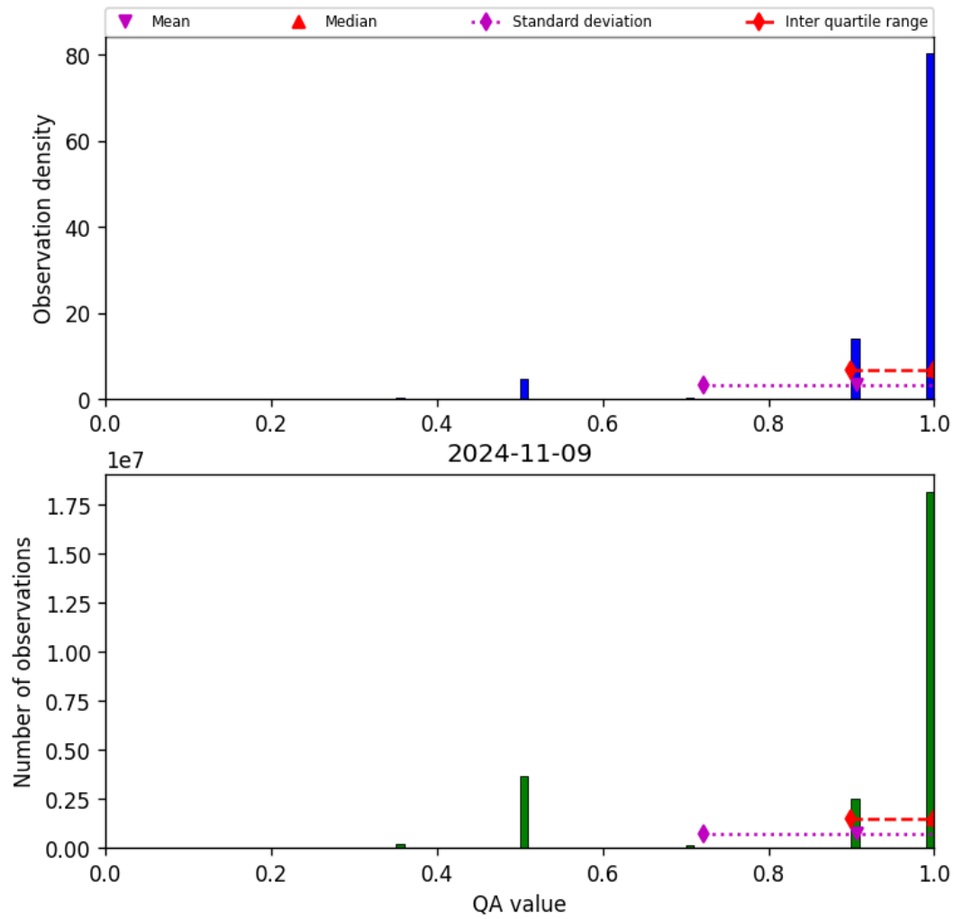
Figure 29: Histogram of “QA value” for 2024-11-09 to 2024-11-10
