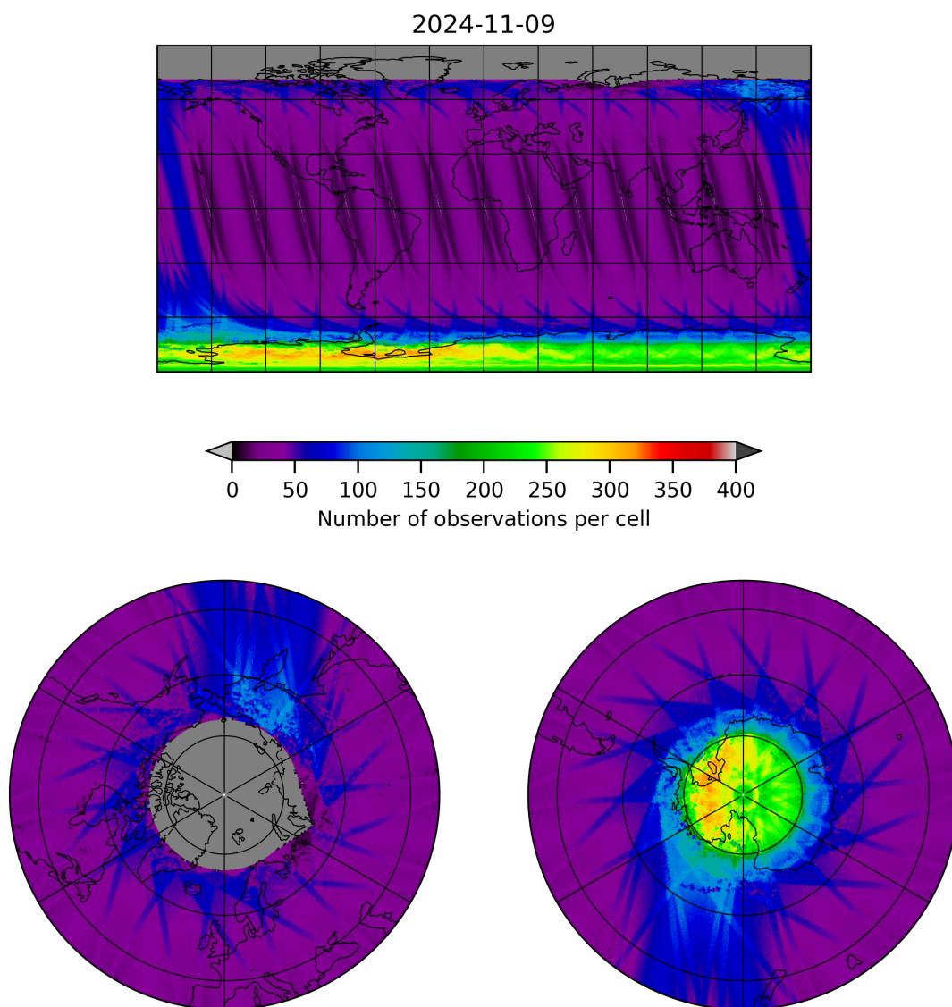
Figure 11: Map of the number of observations for 2024-11-09 to 2024-11-10
