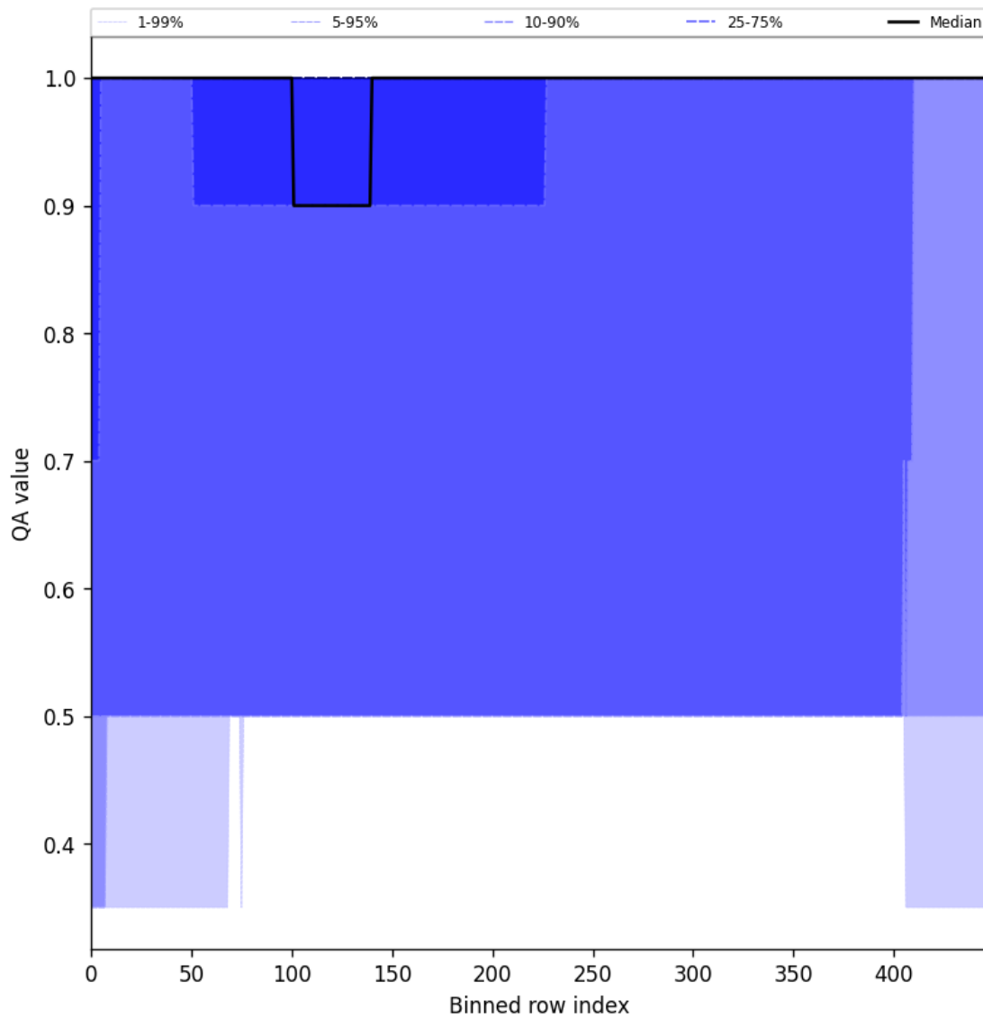
Figure 46: Along track statistics of “QA value” for 2024-11-09 to 2024-11-10
