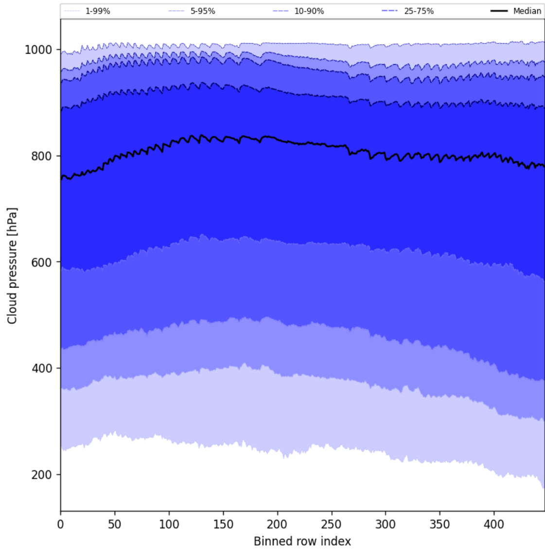
Figure 47: Along track statistics of “Cloud pressure” for 2024-11-09 to 2024-11-10
