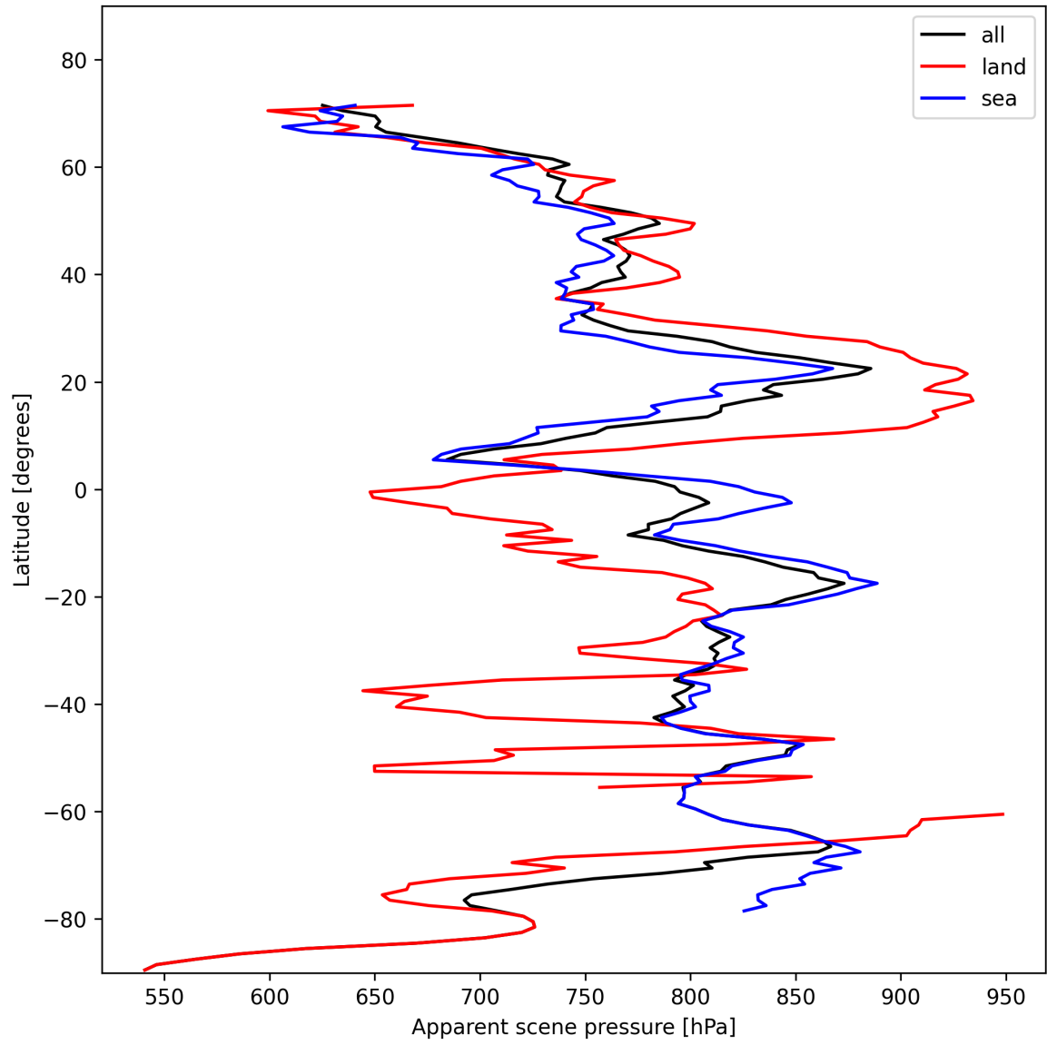
Figure 19: Zonal average of “Apparent scene pressure” for 2024-11-09 to 2024-11-10.
