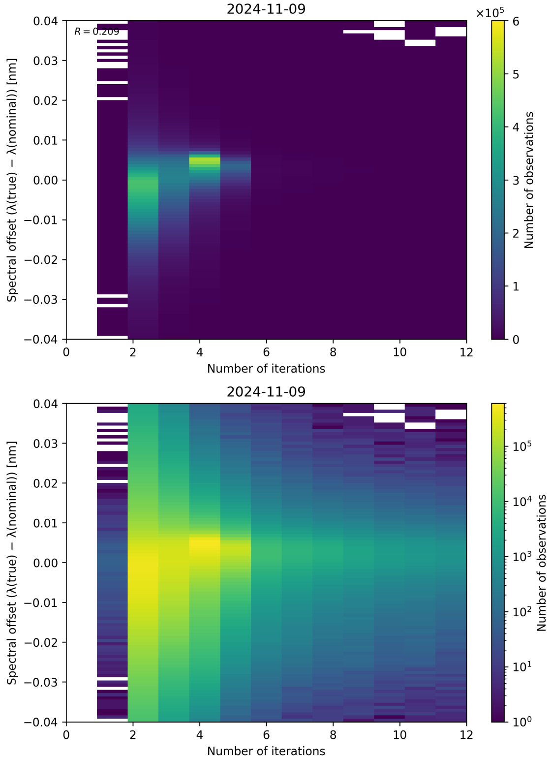
Figure 109: Scatter density plot of “Number of iterations” against “Spectral offset ( \lambda_{\text{true}} - \lambda_{\text{nominal}} )” for 2024-11-09 to 2024-11-10.
