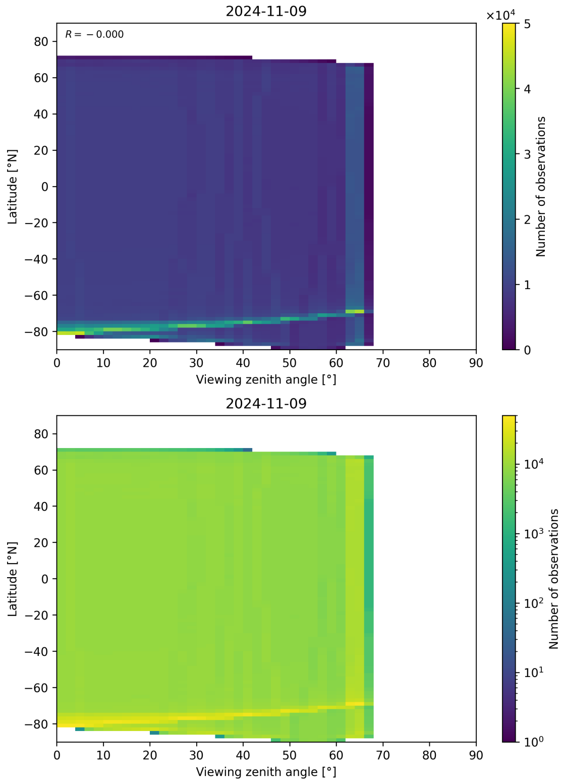
Figure 135: Scatter density plot of “Viewing zenith angle” against “Latitude” for 2024-11-09 to 2024-11-10.
