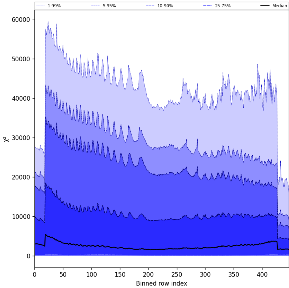
Figure 55: Along track statistics of “ \chi^2 ” for 2024-11-09 to 2024-11-10
