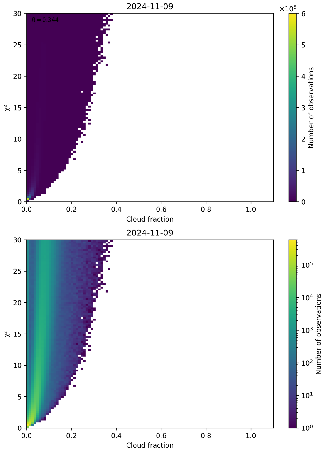
Figure 77: Scatter density plot of “Cloud fraction” against “ \chi^2 ” for 2024-11-09 to 2024-11-10.
