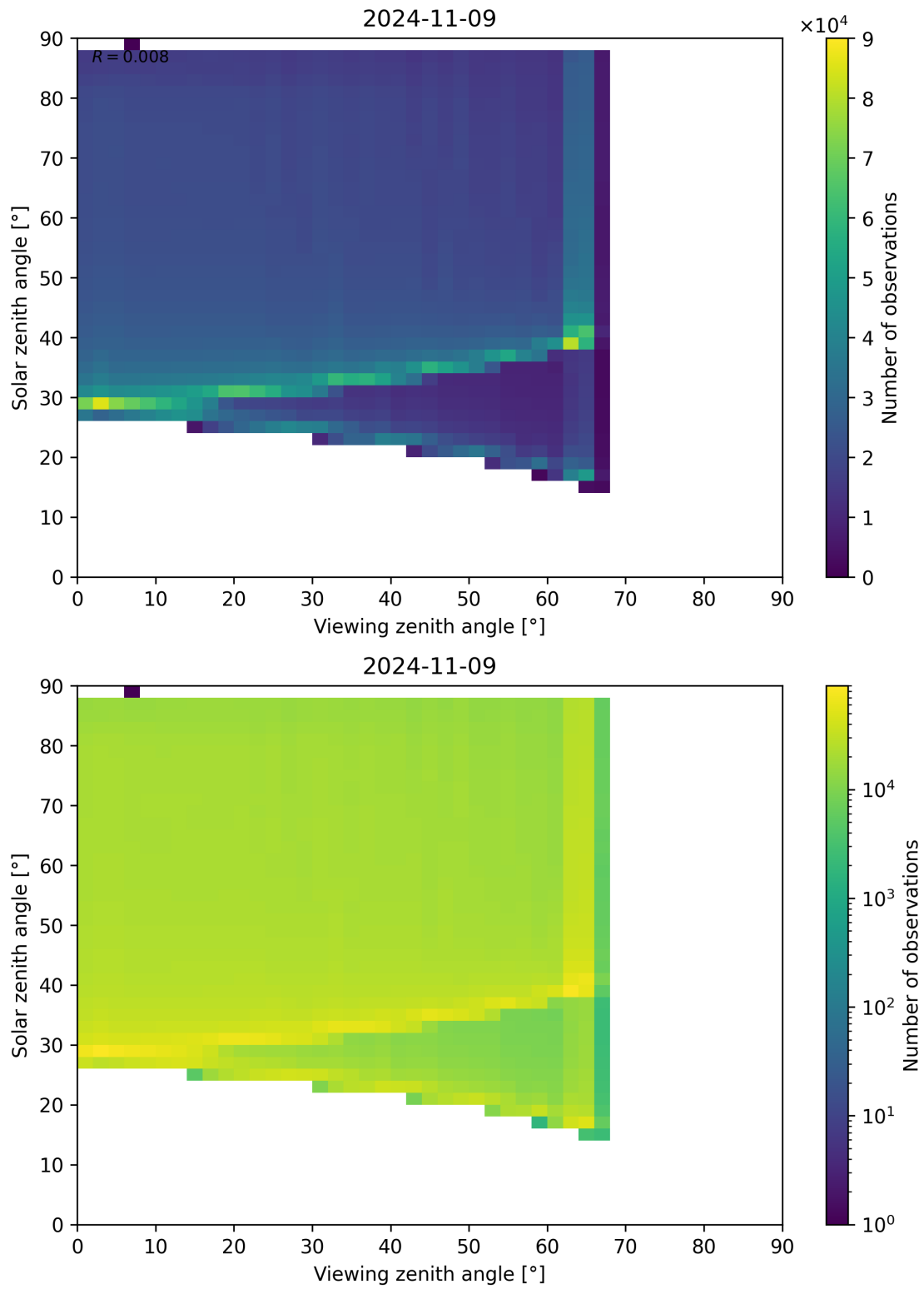
Figure 139: Scatter density plot of “Viewing zenith angle” against “Solar zenith angle” for 2024-11-09 to 2024-11-10.
