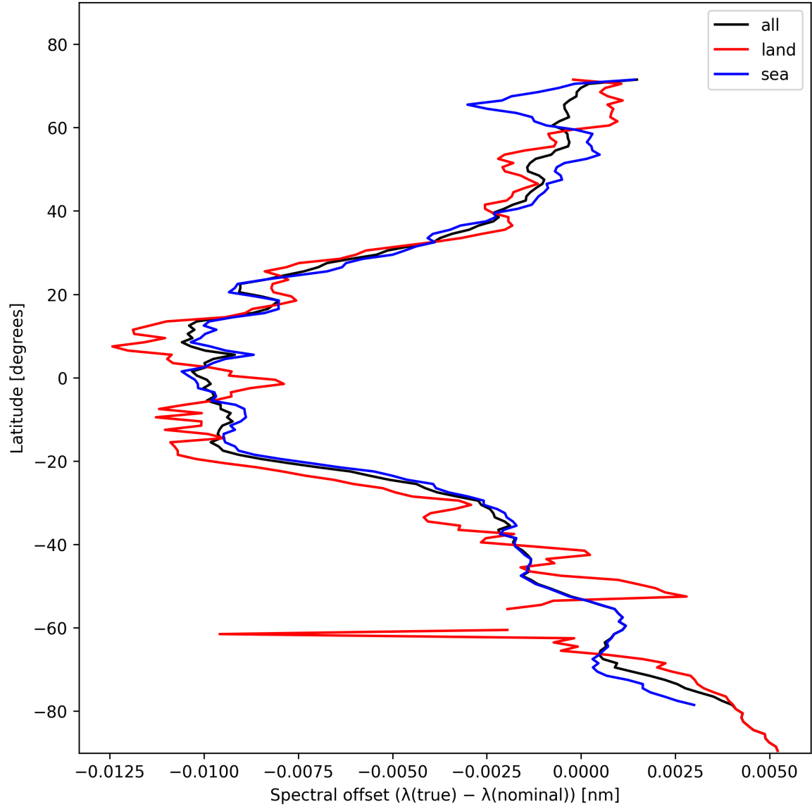
Figure 28: Zonal average of “Spectral offset ( \lambda_{\text{true}} - \lambda_{\text{nominal}} )” for 2024-11-09 to 2024-11-10.
