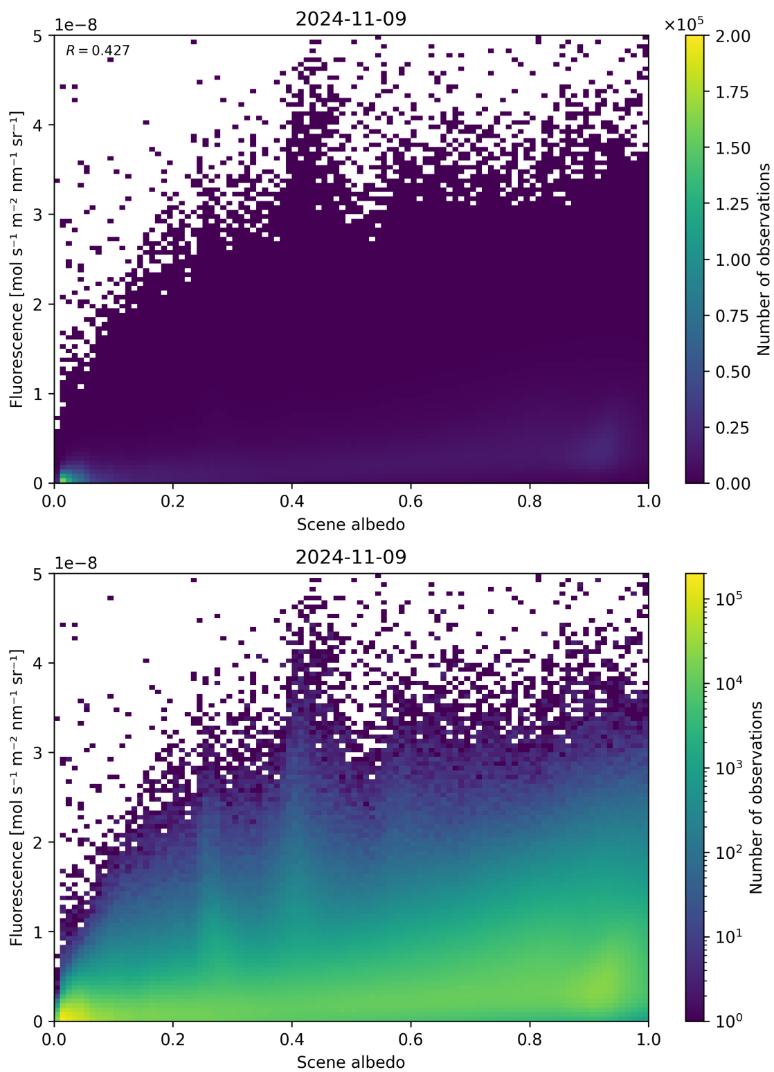
Figure 114: Scatter density plot of “Scene albedo” against “Fluorescence” for 2024-11-09 to 2024-11-10.
