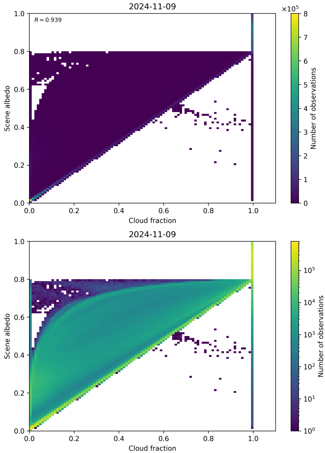
Figure 82: Scatter density plot of “Cloud fraction” against “Scene albedo” for 2024-11-09 to 2024-11-10.
