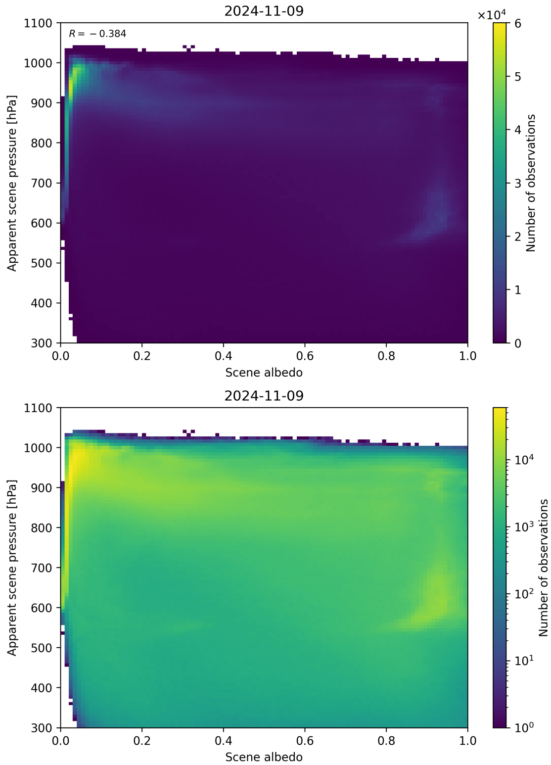
Figure 111: Scatter density plot of “Scene albedo” against “Apparent scene pressure” for 2024-11-09 to 2024-11-10.
