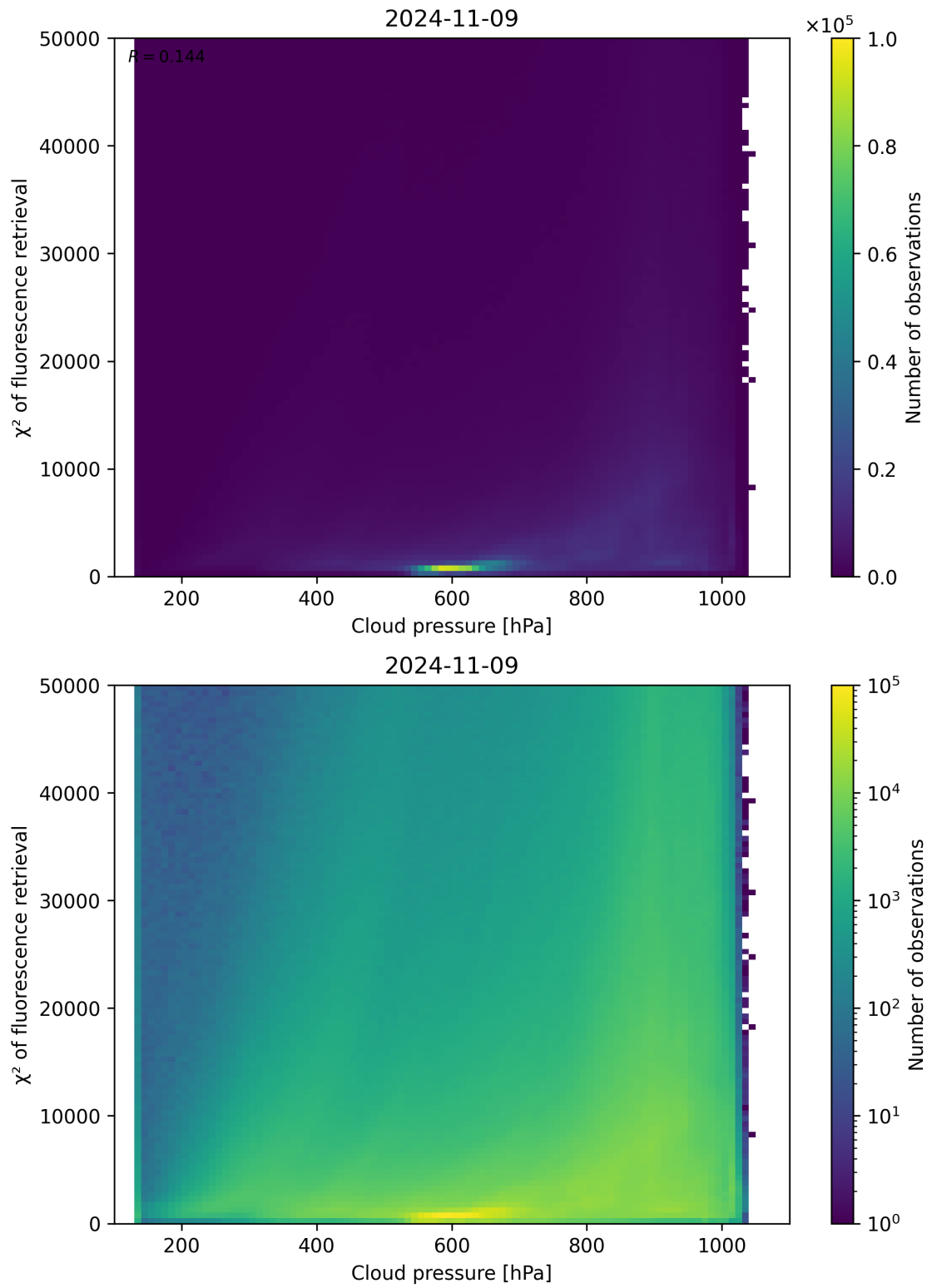
Figure 86: Scatter density plot of “Cloud pressure” against “ \chi^2 of fluorescence retrieval” for 2024-11-09 to 2024-11-10.
