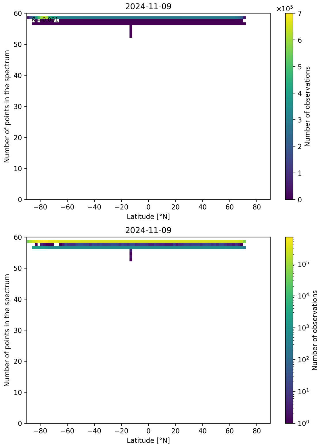
Figure 103: Scatter density plot of “Latitude” against “Number of points in the spectrum” for 2024-11-09 to 2024-11-10.
