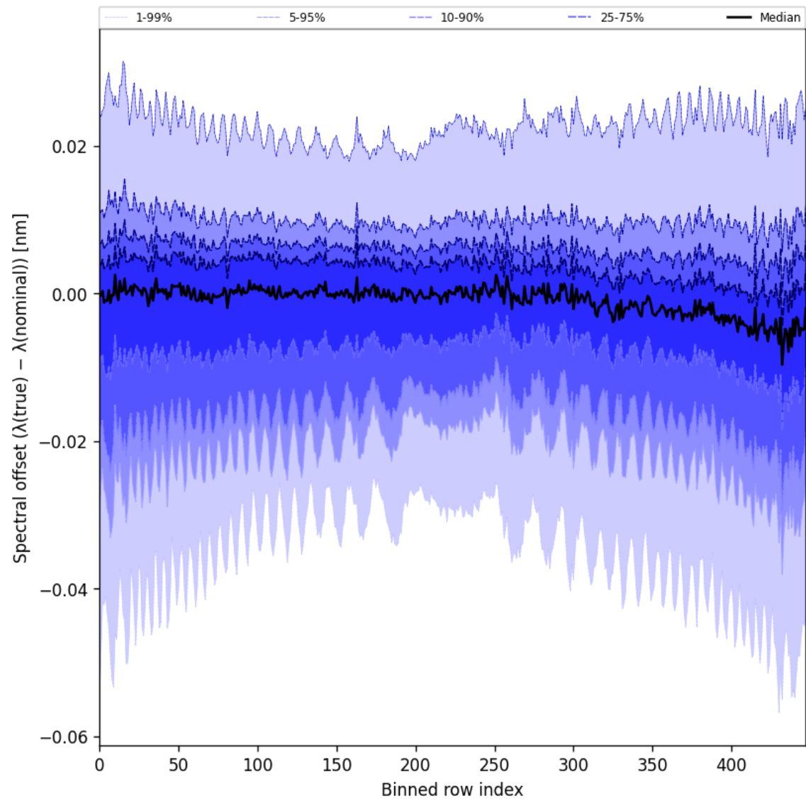
Figure 62: Along track statistics of “Spectral offset ( \lambda_{\text{true}} - \lambda_{\text{nominal}} )” for 2024-11-09 to 2024-11-10
