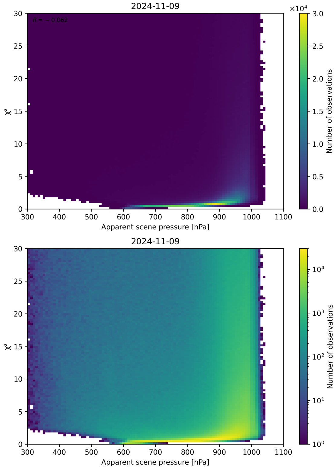
Figure 63: Scatter density plot of “Apparent scene pressure” against “ \chi^2 ” for 2024-11-09 to 2024-11-10.
