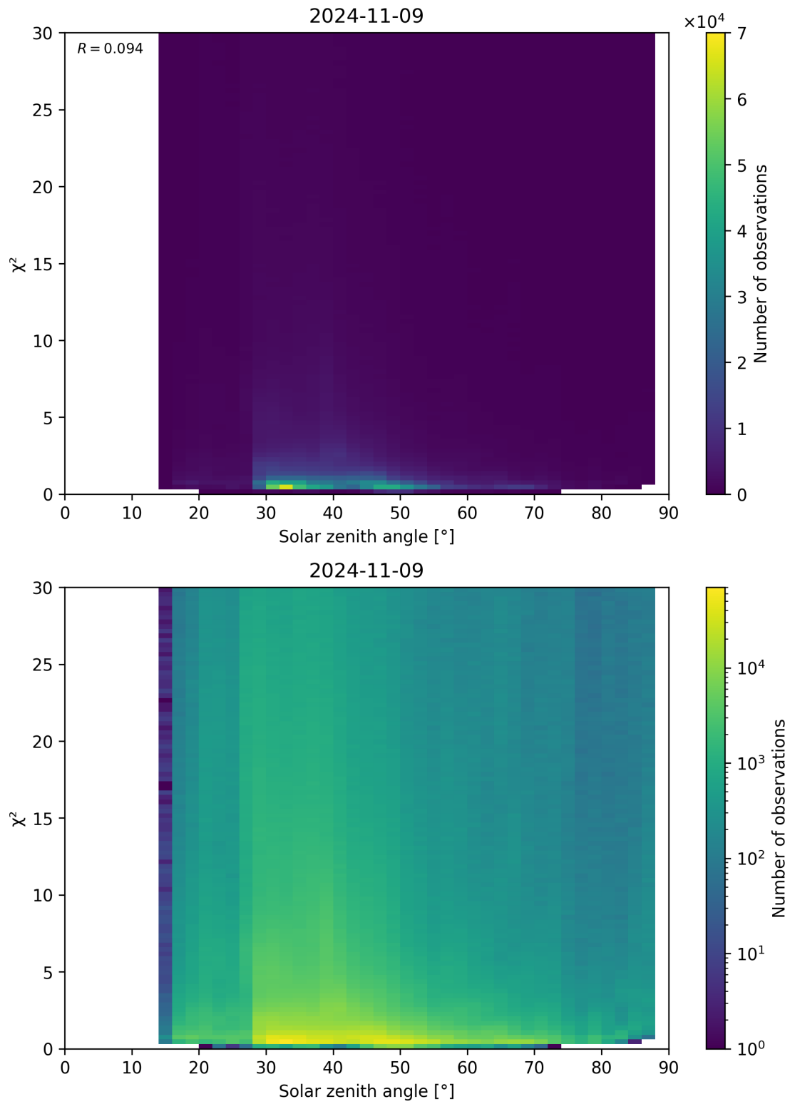
Figure 119: Scatter density plot of “Solar zenith angle” against “ \chi^2 ” for 2024-11-09 to 2024-11-10.
