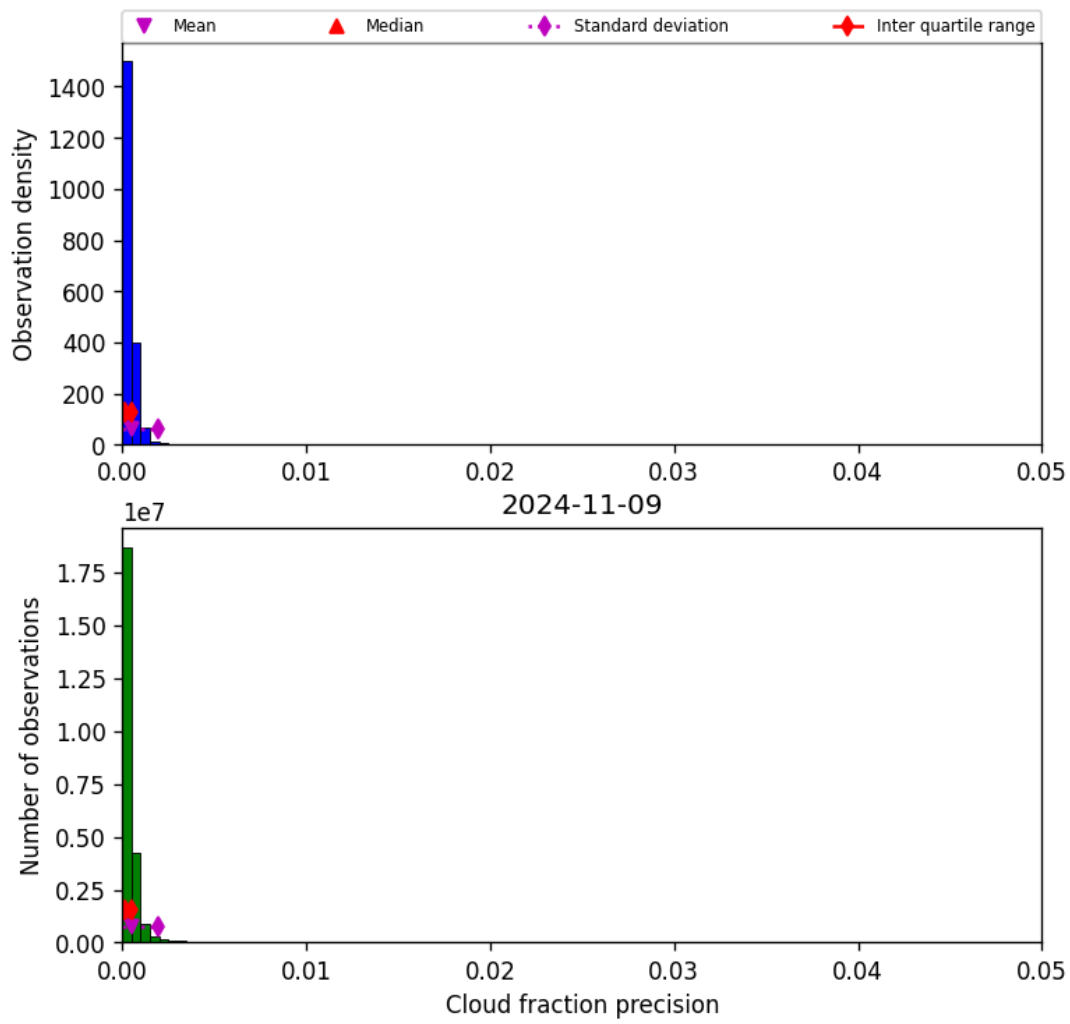
Figure 33: Histogram of “Cloud fraction precision” for 2024-11-09 to 2024-11-10
