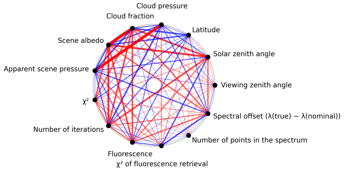
Figure 1: Map of correlation graph for 2024-11-09 to 2024-11-10.
