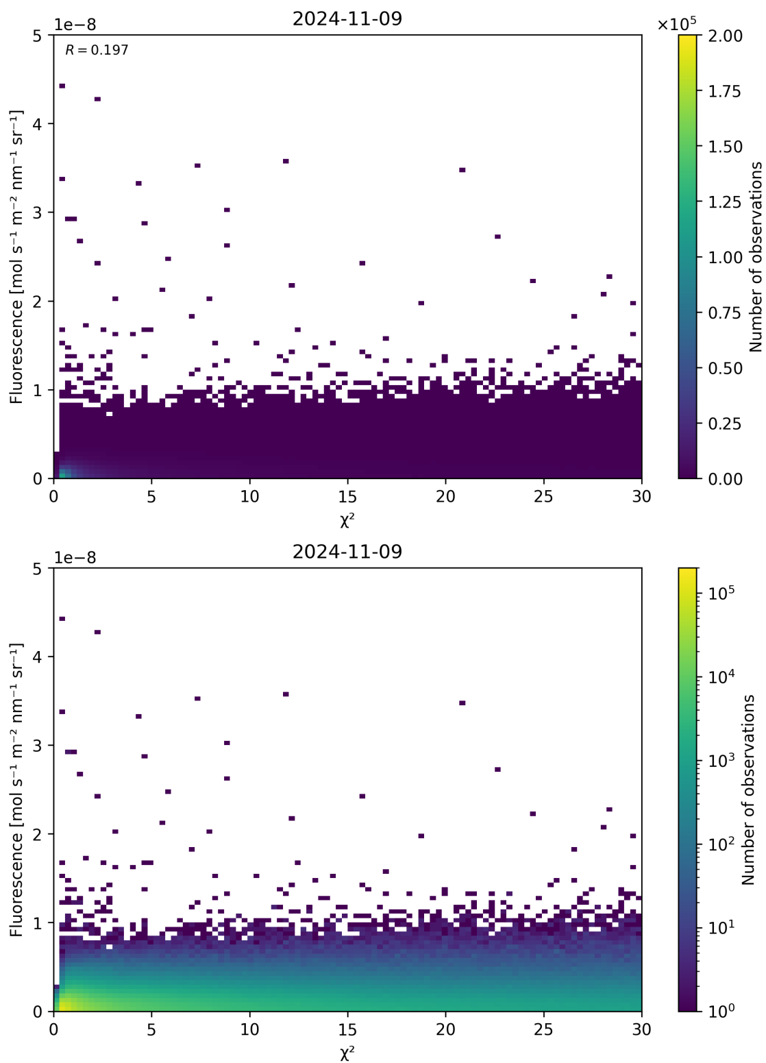
Figure 70: Scatter density plot of “ \chi^2 ” against “Fluorescence” for 2024-11-09 to 2024-11-10.
