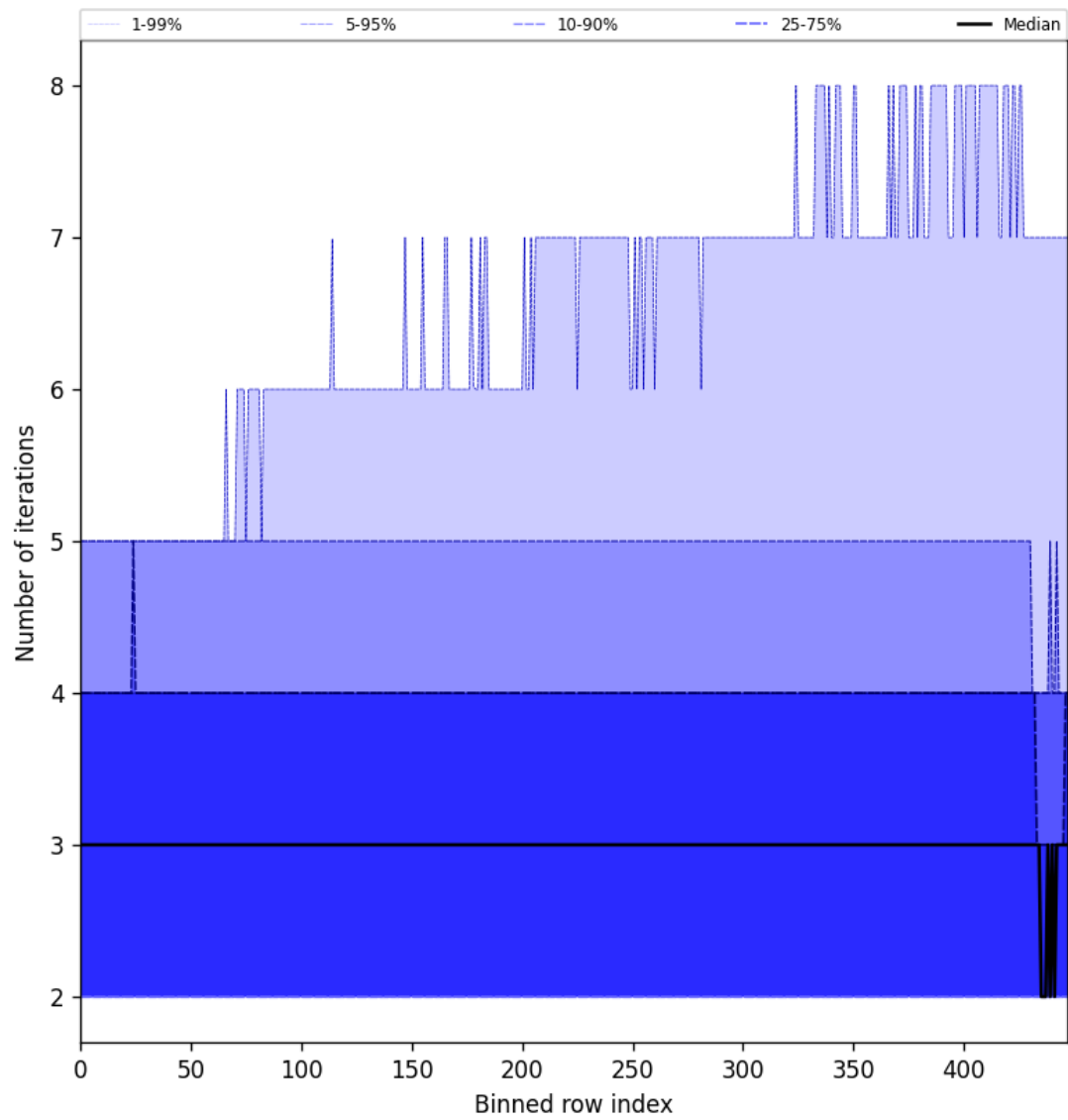
Figure 56: Along track statistics of “Number of iterations” for 2024-11-09 to 2024-11-10
