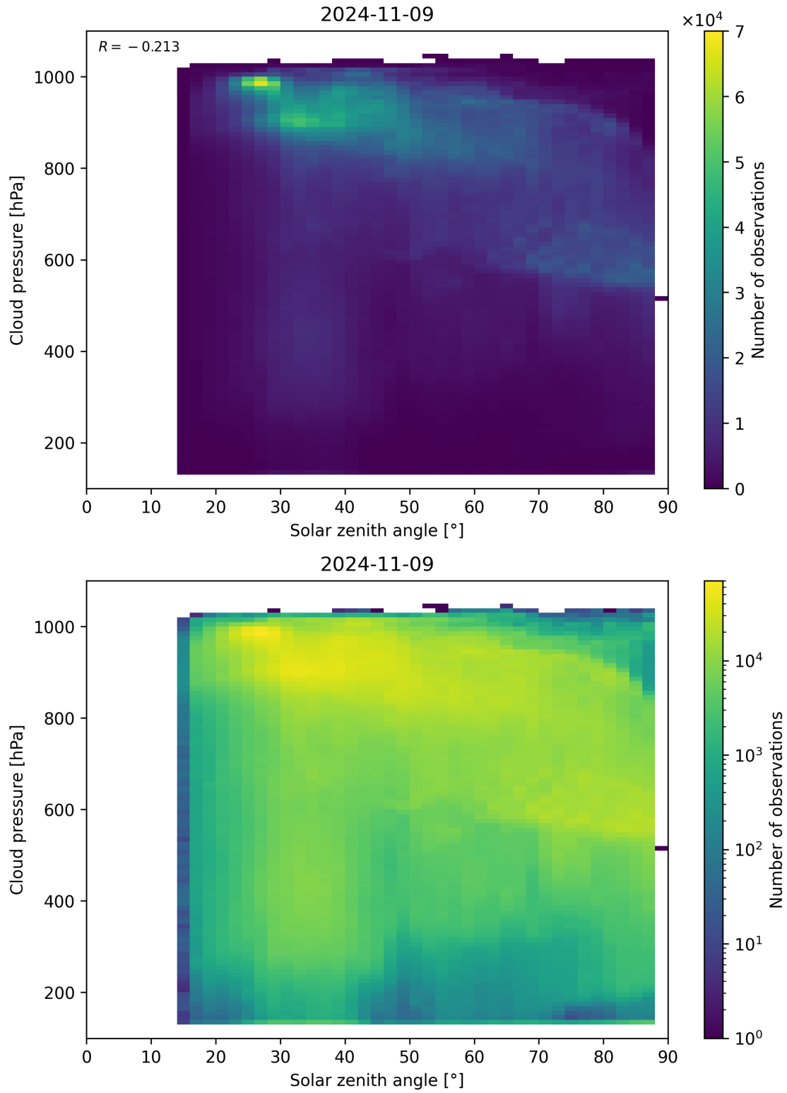
Figure 122: Scatter density plot of “Solar zenith angle” against “Cloud pressure” for 2024-11-09 to 2024-11-10.
