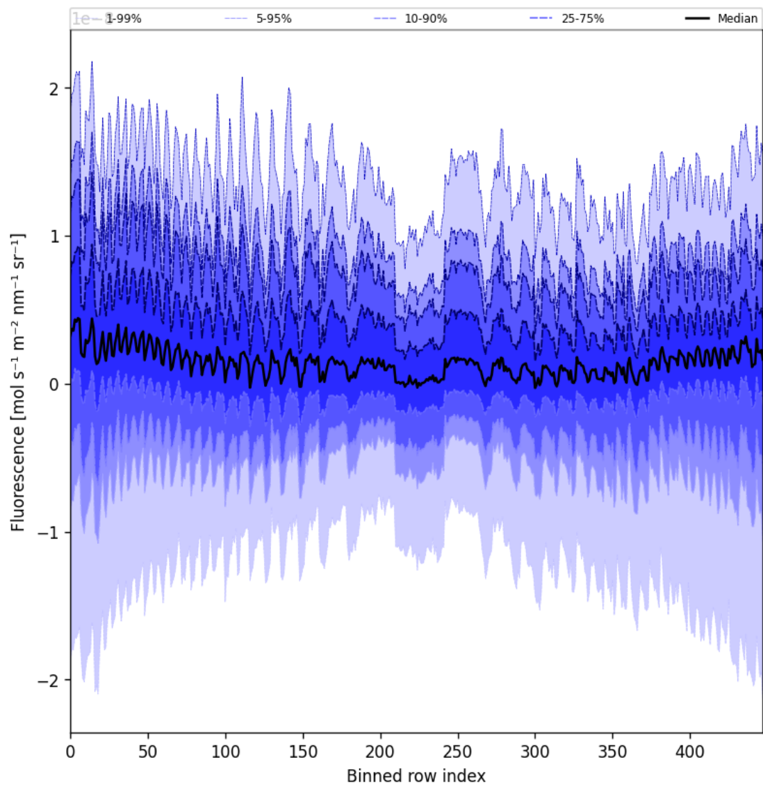
Figure 57: Along track statistics of "Fluorescence" for 2024-11-09 to 2024-11-10
