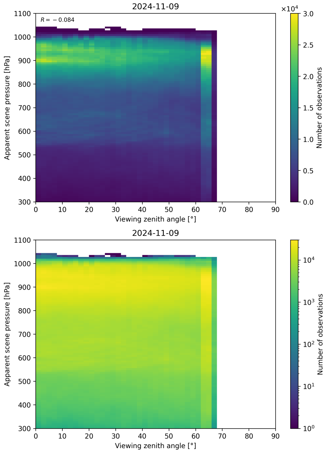
Figure 129: Scatter density plot of “Viewing zenith angle” against “Apparent scene pressure” for 2024-11-09 to 2024-11-10.
