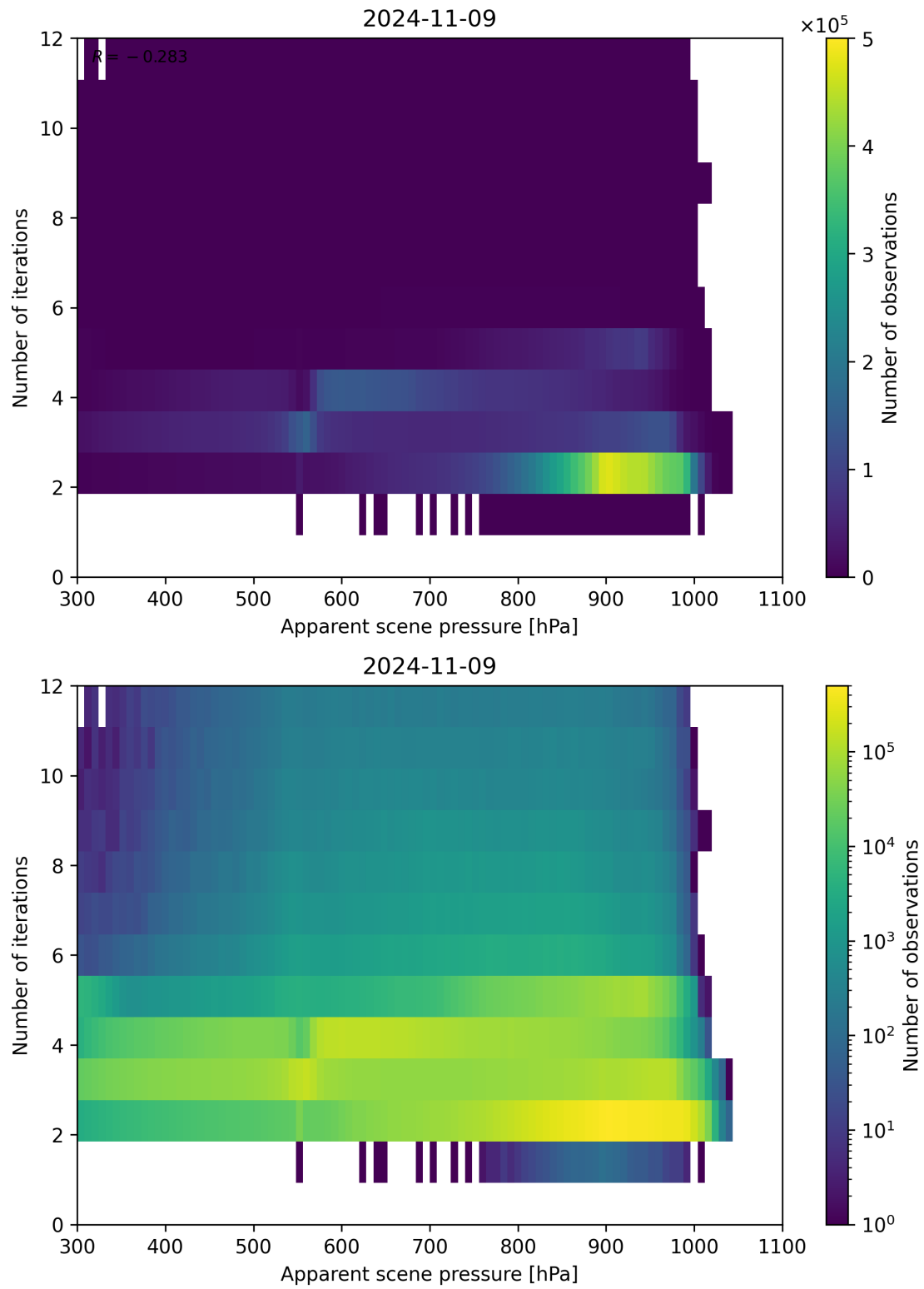
Figure 66: Scatter density plot of “Apparent scene pressure” against “Number of iterations” for 2024-11-09 to 2024-11-10.
