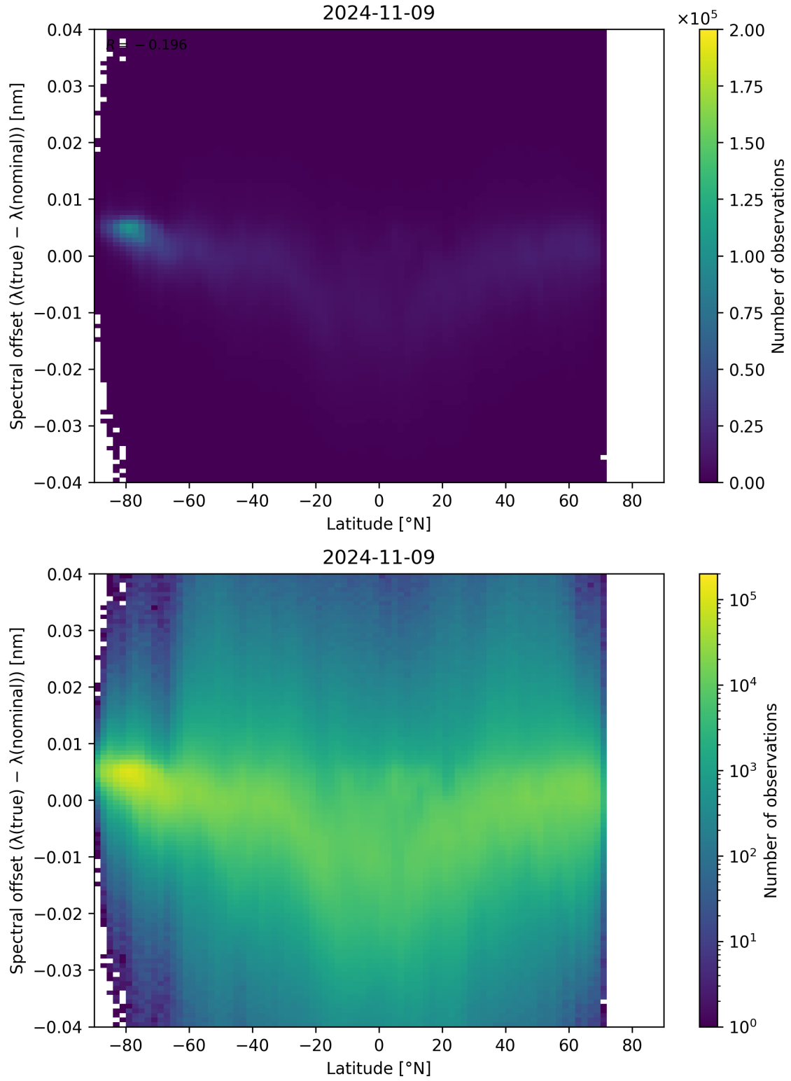
Figure 105: Scatter density plot of “Latitude” against “Spectral offset ( \lambda_{\text{true}} - \lambda_{\text{nominal}} )” for 2024-11-09 to 2024-11-10.
