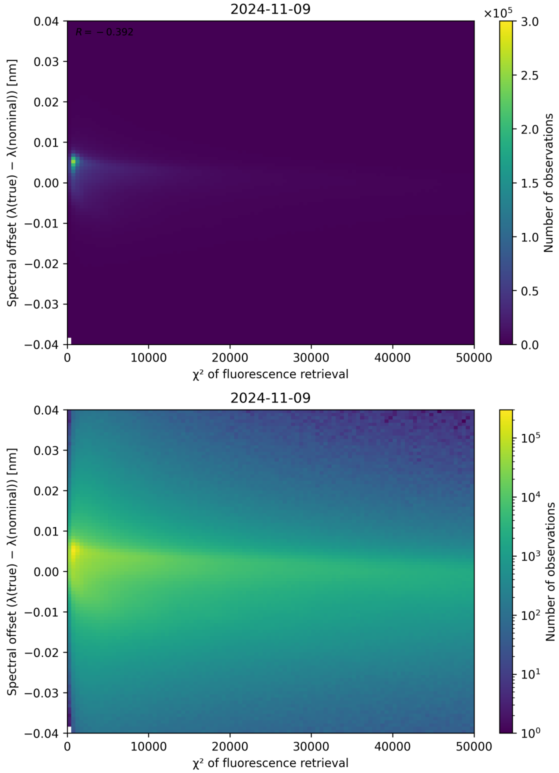
Figure 72: Scatter density plot of “ \chi^2 of fluorescence retrieval” against “Spectral offset ( \lambda_{\text{true}} - \lambda_{\text{nominal}} )” for 2024-11-09 to 2024-11-10.
