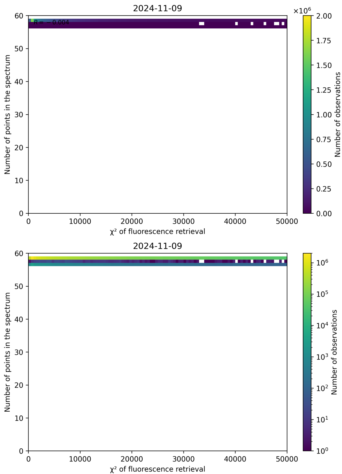
Figure 71: Scatter density plot of " \chi^2 of fluorescence retrieval" against "Number of points in the spectrum" for 2024-11-09 to 2024-11-10.
