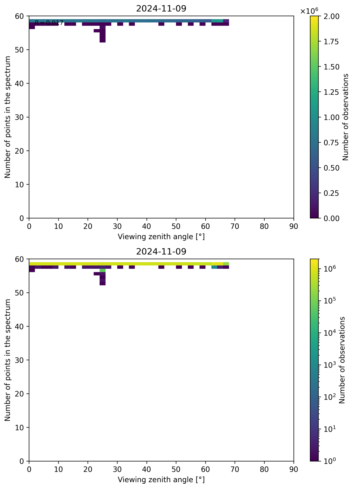
Figure 137: Scatter density plot of “Viewing zenith angle” against “Number of points in the spectrum” for 2024-11-09 to 2024-11-10.
