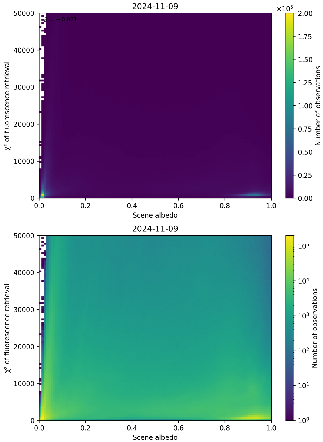
Figure 113: Scatter density plot of “Scene albedo” against “ \chi^2 of fluorescence retrieval” for 2024-11-09 to 2024-11-10.
