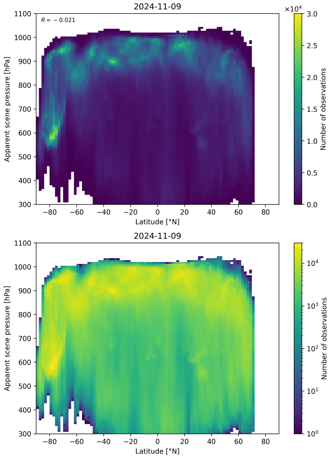
Figure 96: Scatter density plot of “Latitude” against “Apparent scene pressure” for 2024-11-09 to 2024-11-10.
