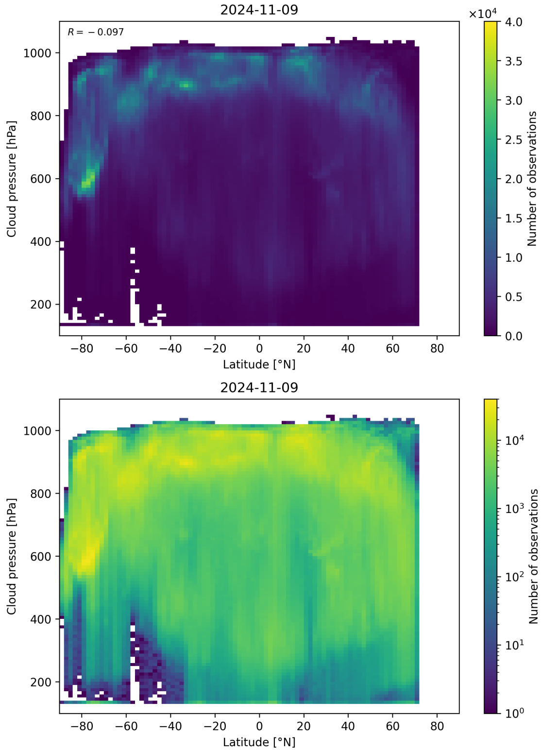
Figure 100: Scatter density plot of “Latitude” against “Cloud pressure” for 2024-11-09 to 2024-11-10.
