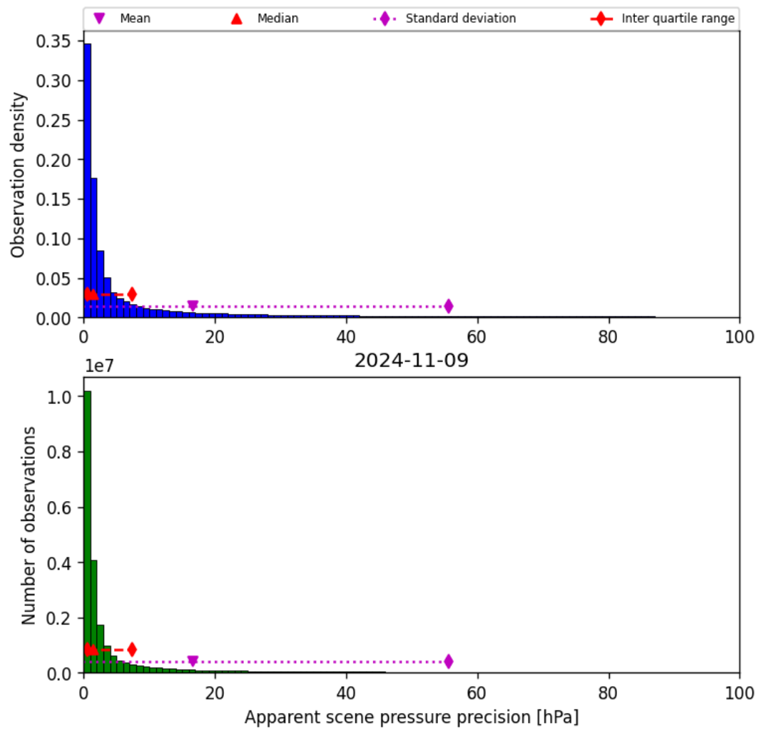
Figure 37: Histogram of “Apparent scene pressure precision” for 2024-11-09 to 2024-11-10
