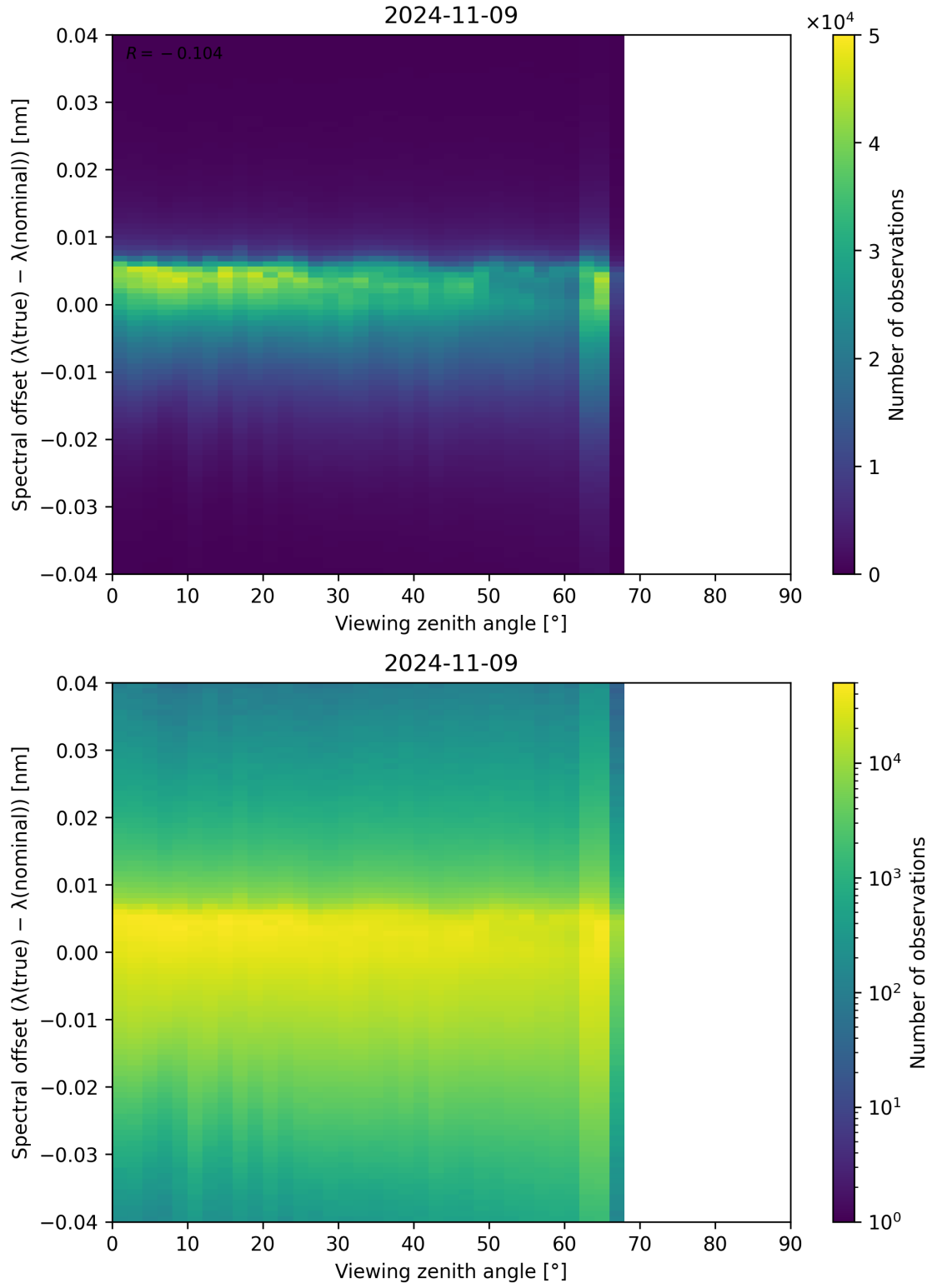
Figure 140: Scatter density plot of “Viewing zenith angle” against “Spectral offset ( \lambda_{\text{true}} - \lambda_{\text{nominal}} )” for 2024-11-09 to 2024-11-10.
