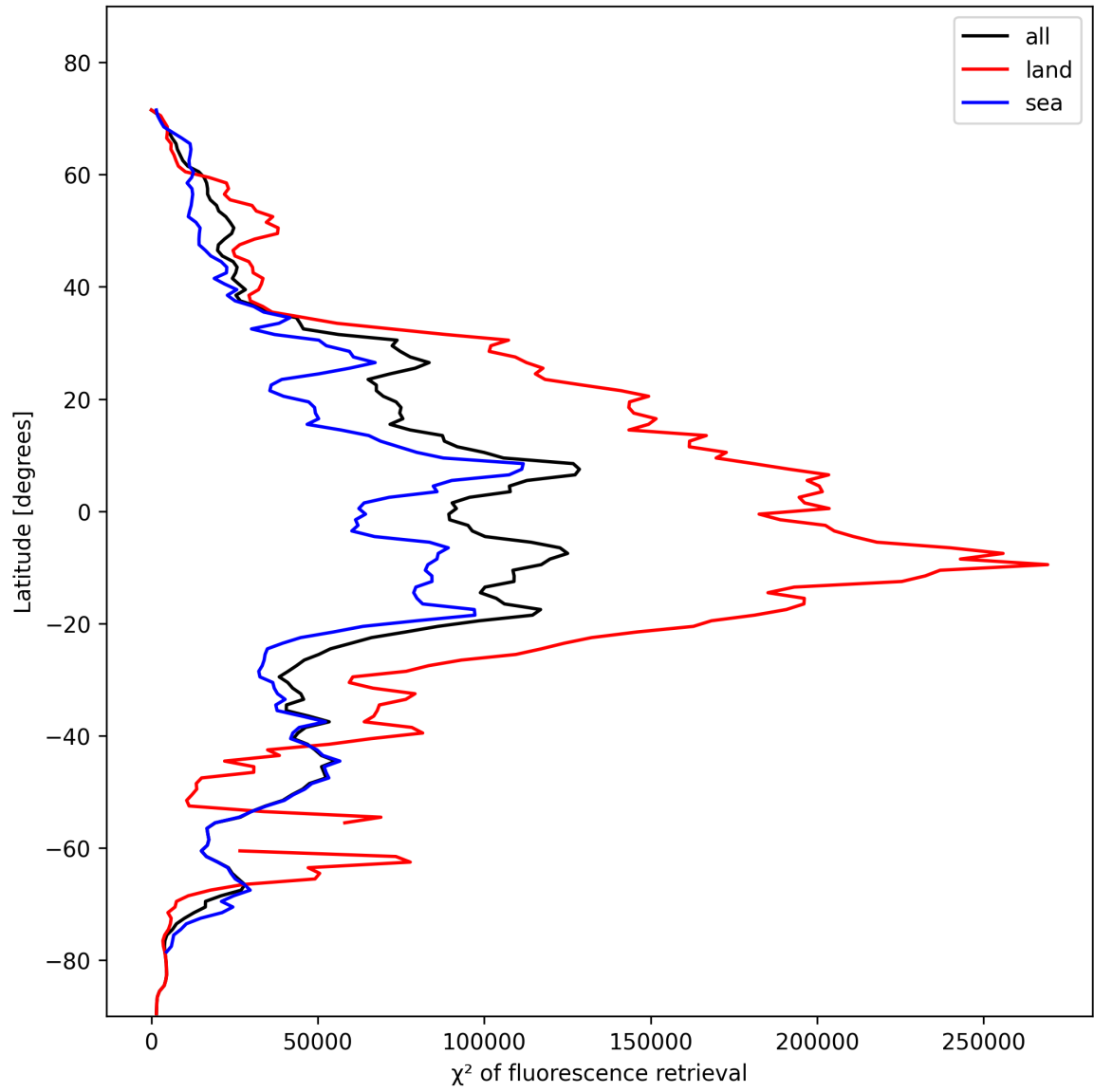
Figure 25: Zonal average of “ \chi^2 of fluorescence retrieval” for 2024-11-09 to 2024-11-10.
