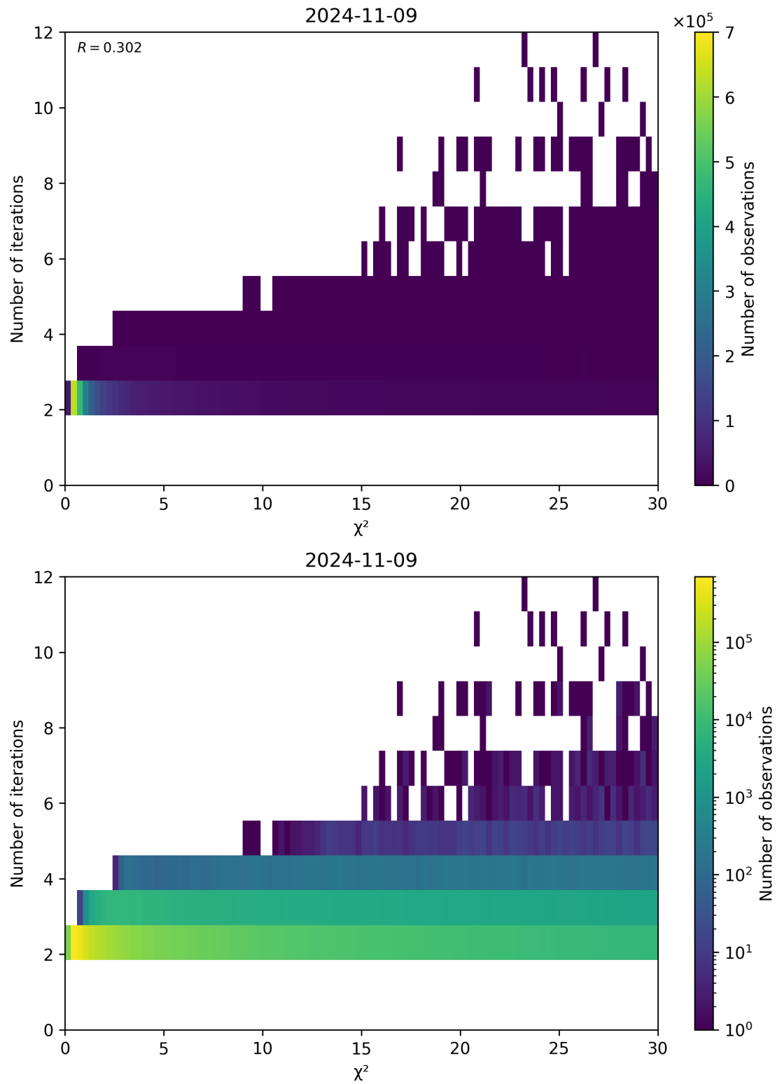
Figure 73: Scatter density plot of " \chi^2 " against "Number of iterations" for 2024-11-09 to 2024-11-10.
