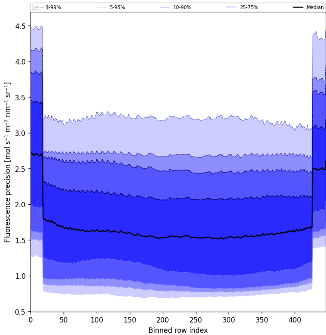
Figure 58: Along track statistics of “Fluorescence precision” for 2024-11-09 to 2024-11-10
