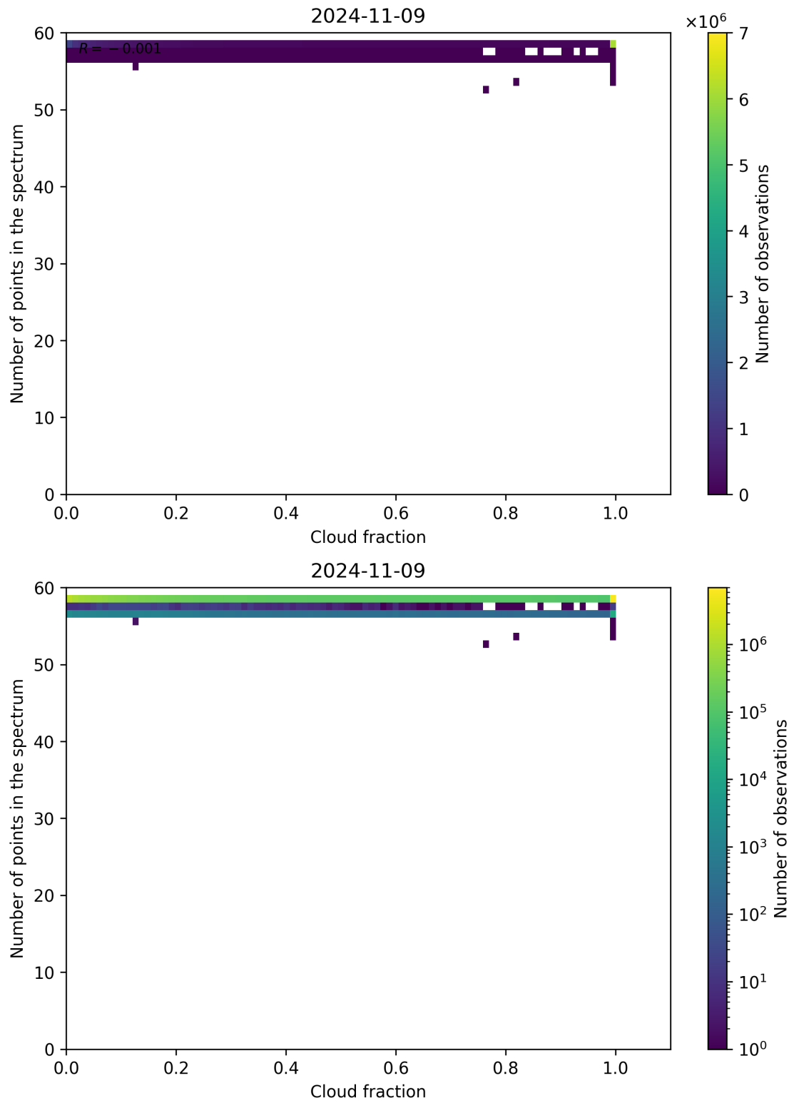
Figure 81: Scatter density plot of “Cloud fraction” against “Number of points in the spectrum” for 2024-11-09 to 2024-11-10.
