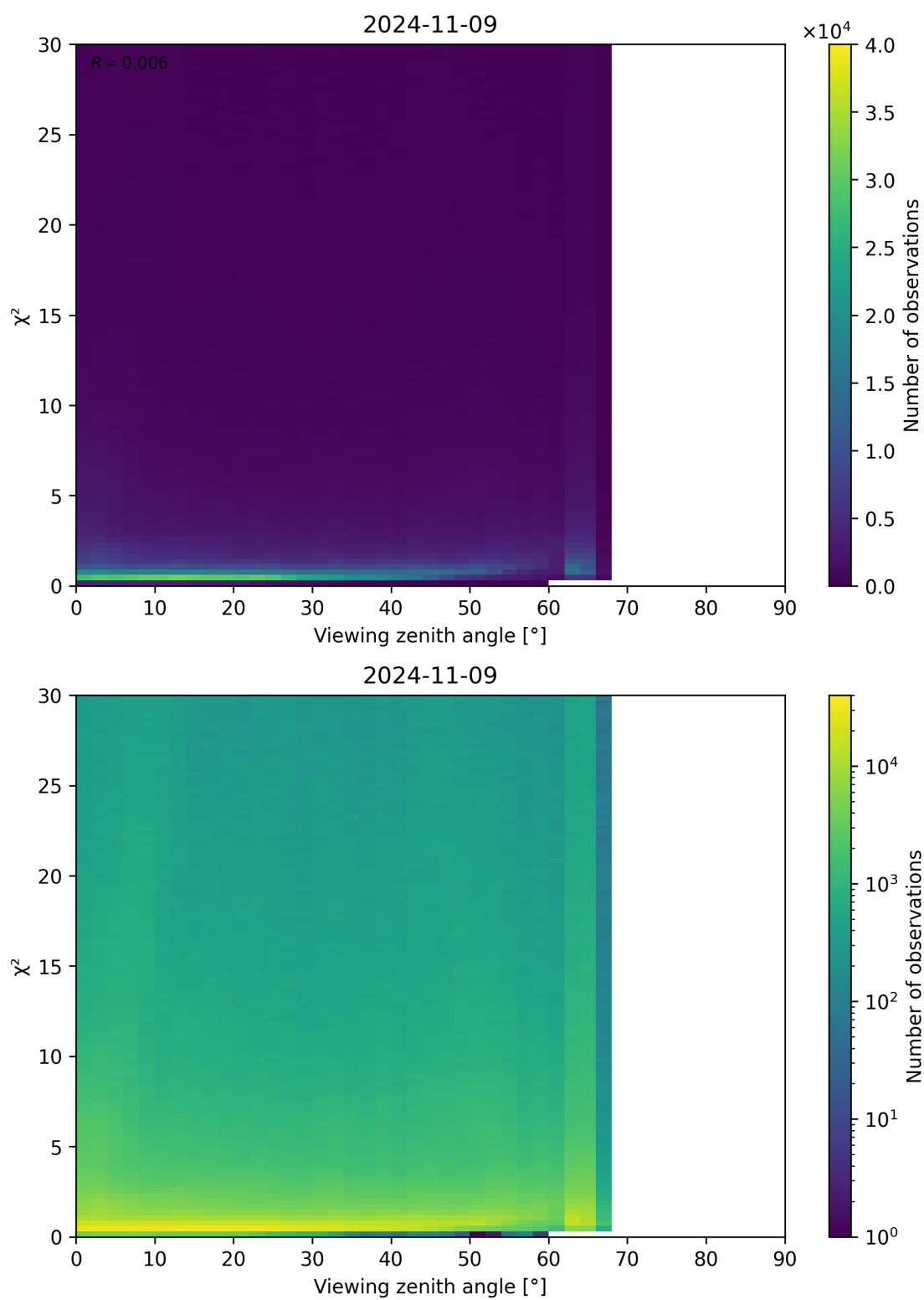
Figure 130: Scatter density plot of “Viewing zenith angle” against “ \chi^2 ” for 2024-11-09 to 2024-11-10.
