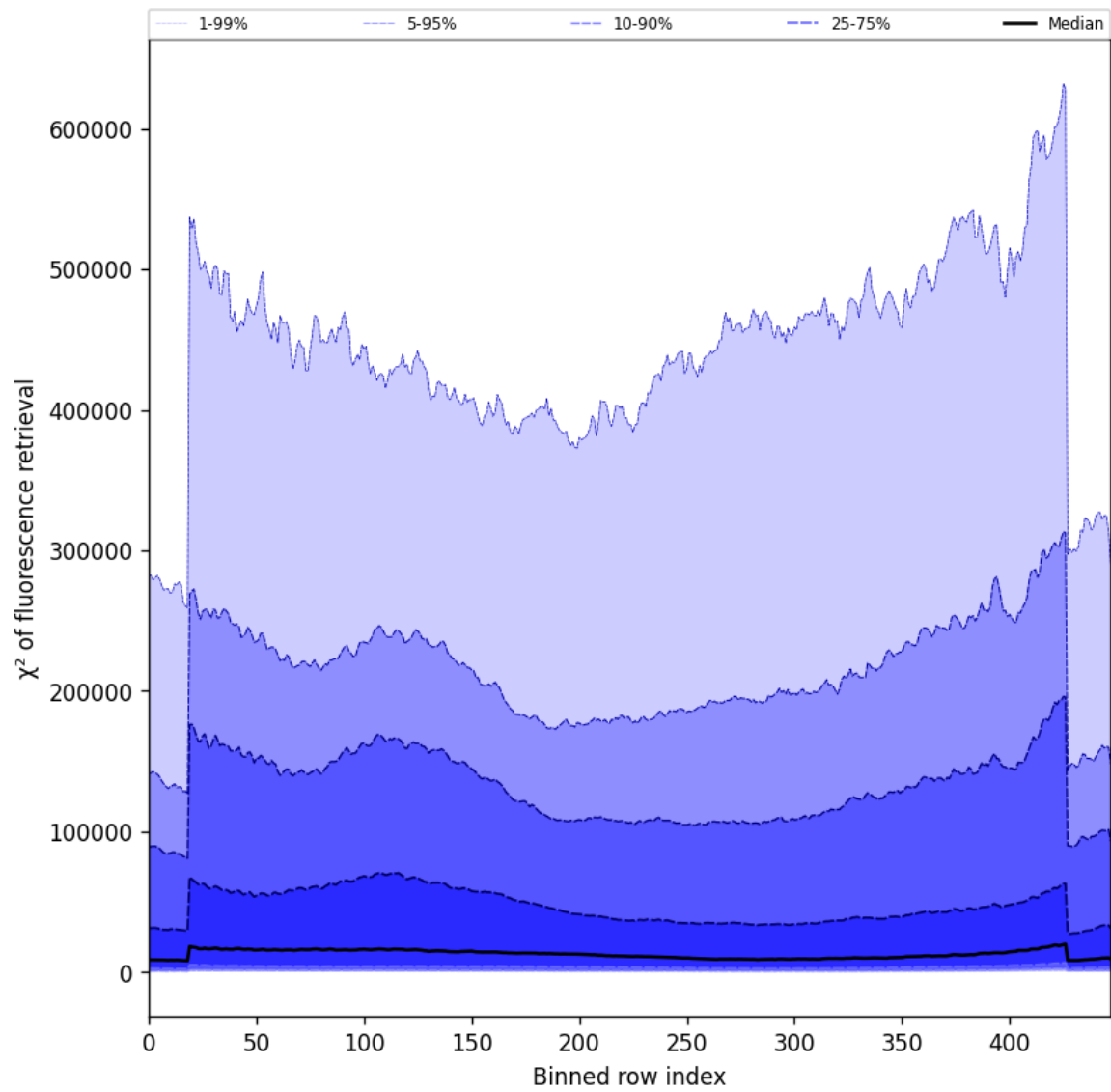
Figure 59: Along track statistics of “ \chi^2 of fluorescence retrieval” for 2024-11-09 to 2024-11-10
