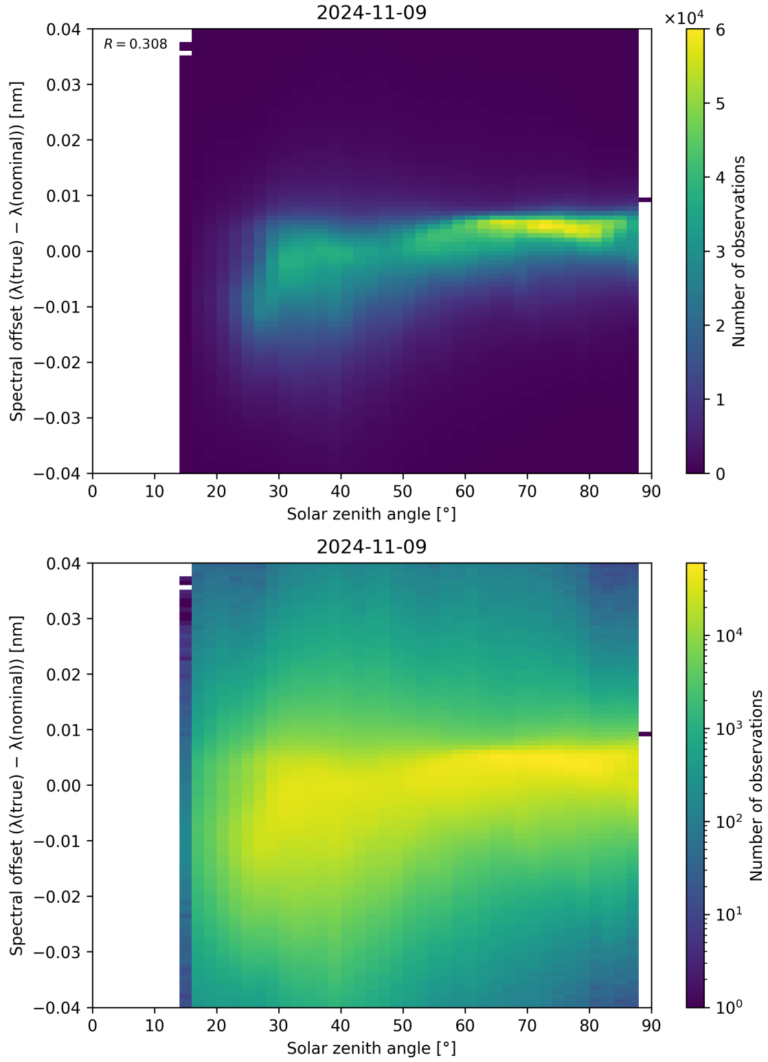
Figure 128: Scatter density plot of “Solar zenith angle” against “Spectral offset ( \lambda_{\text{true}} - \lambda_{\text{nominal}} )” for 2024-11-09 to 2024-11-10.
