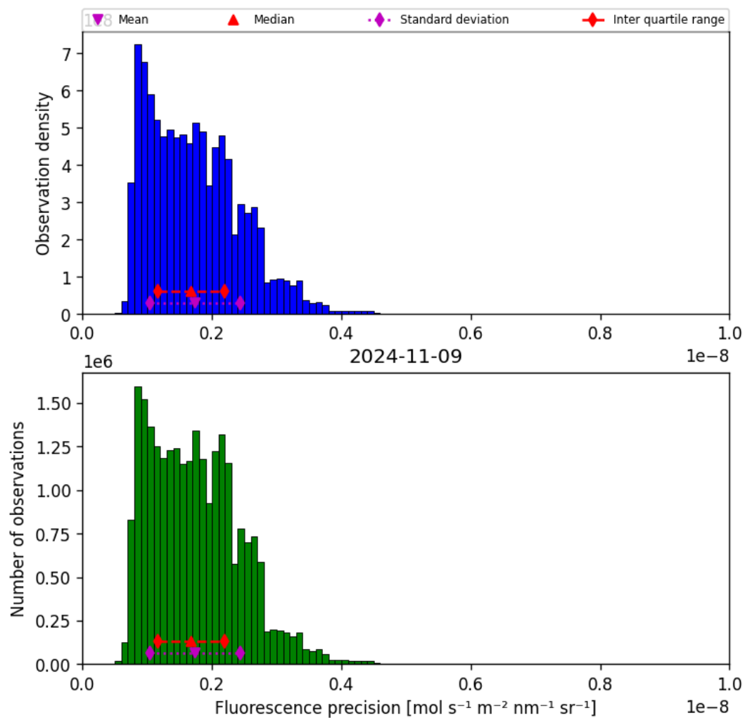
Figure 41: Histogram of “Fluorescence precision” for 2024-11-09 to 2024-11-10
