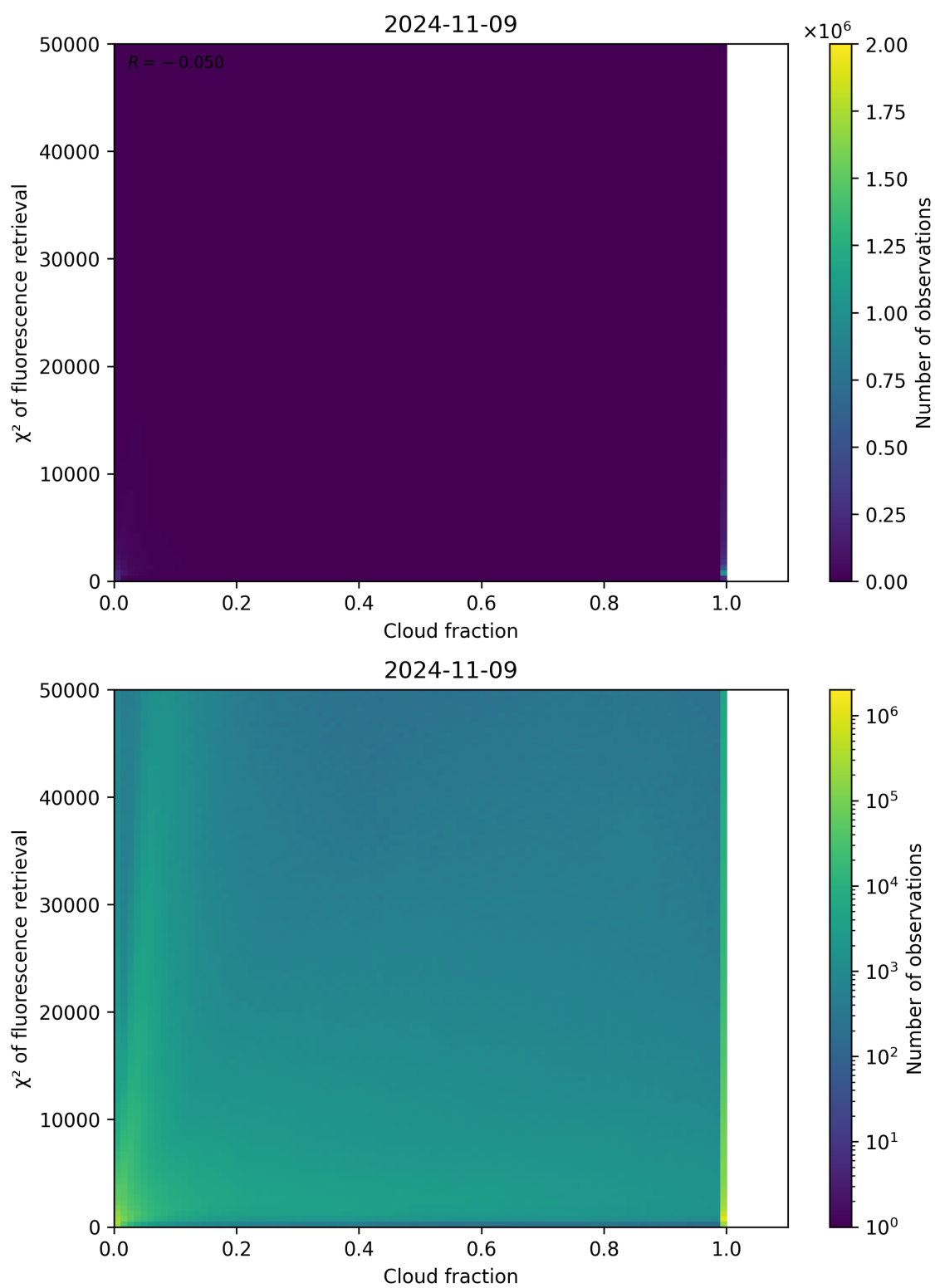
Figure 78: Scatter density plot of “Cloud fraction” against “ \chi^2 of fluorescence retrieval” for 2024-11-09 to 2024-11-10.
