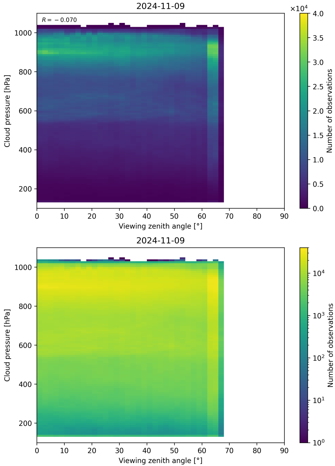
Figure 133: Scatter density plot of “Viewing zenith angle” against “Cloud pressure” for 2024-11-09 to 2024-11-10.
