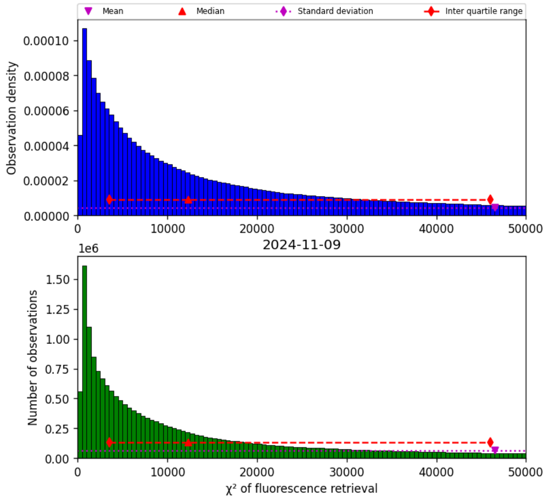
Figure 42: Histogram of “ \chi^2 of fluorescence retrieval” for 2024-11-09 to 2024-11-10
