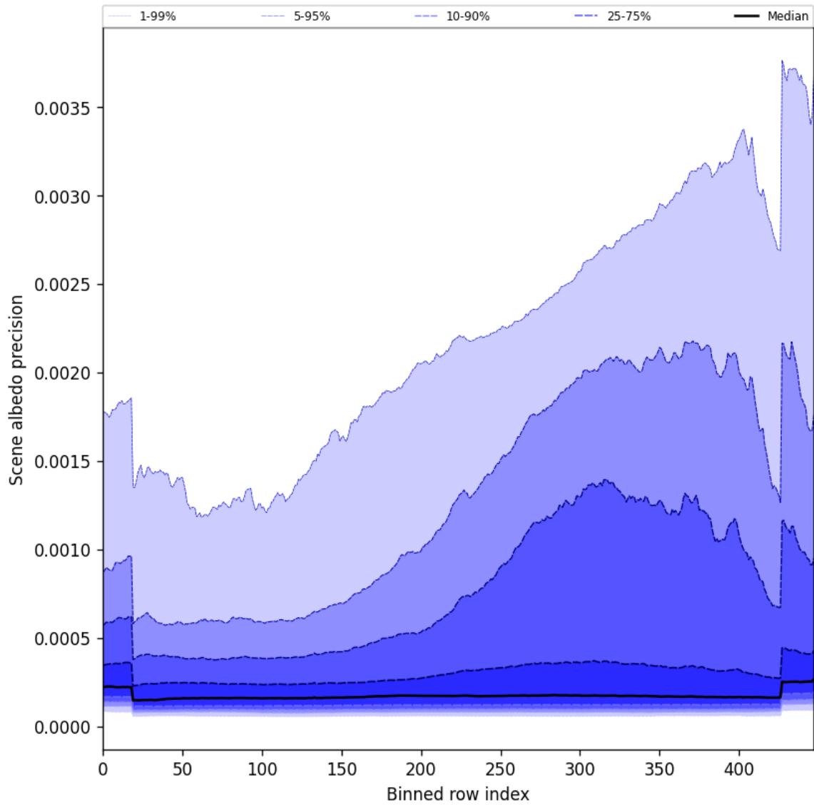
Figure 52: Along track statistics of “Scene albedo precision” for 2024-11-09 to 2024-11-10
