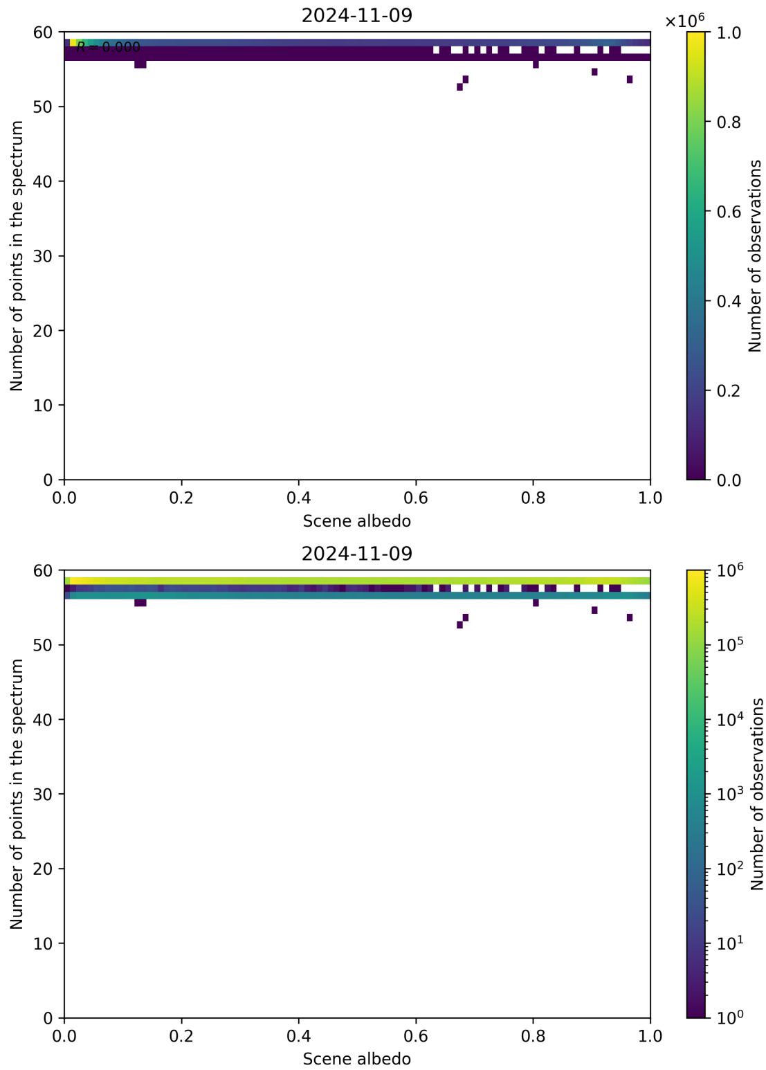
Figure 116: Scatter density plot of “Scene albedo” against “Number of points in the spectrum” for 2024-11-09 to 2024-11-10.
