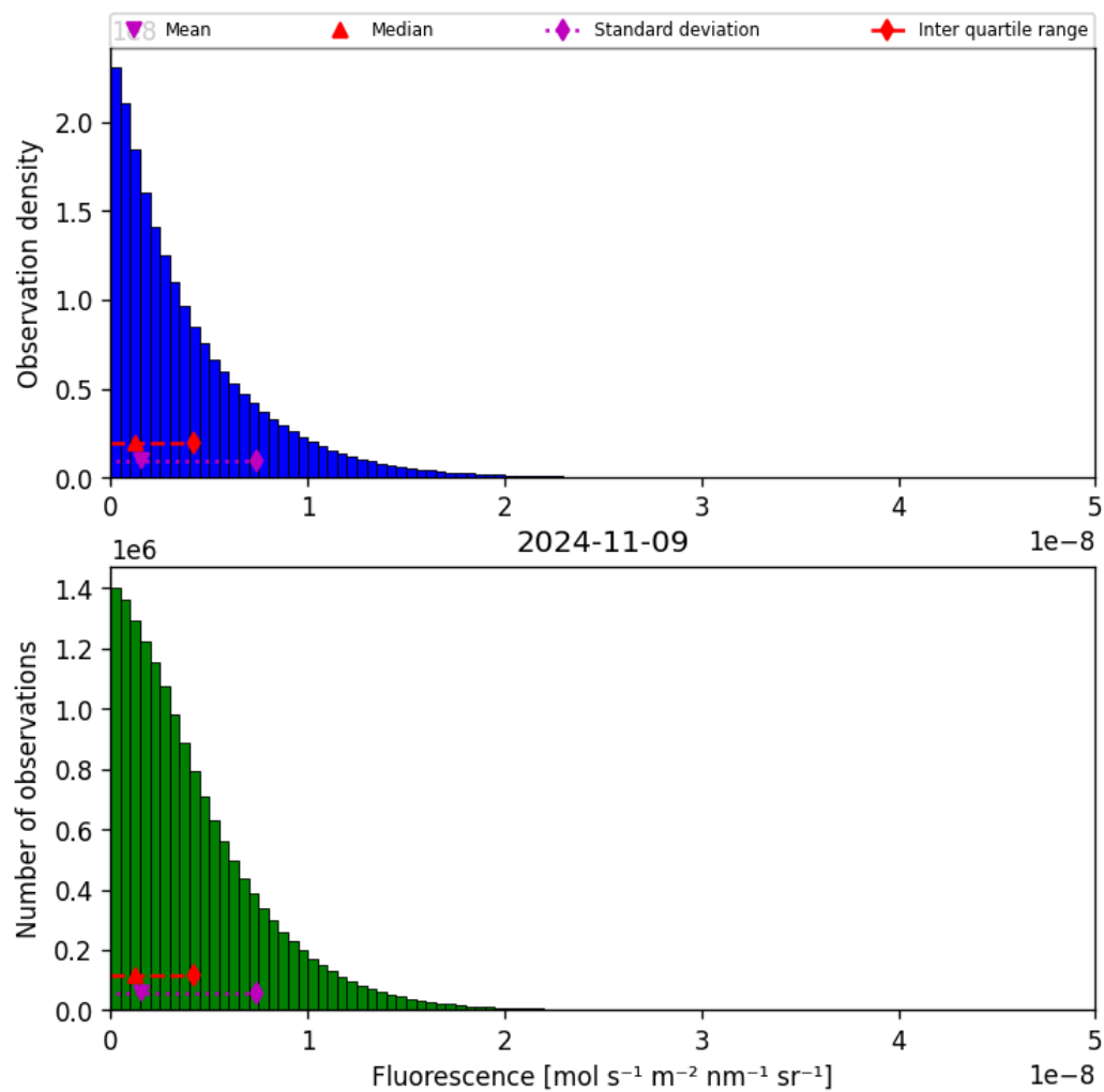
Figure 40: Histogram of “Fluorescence” for 2024-11-09 to 2024-11-10
