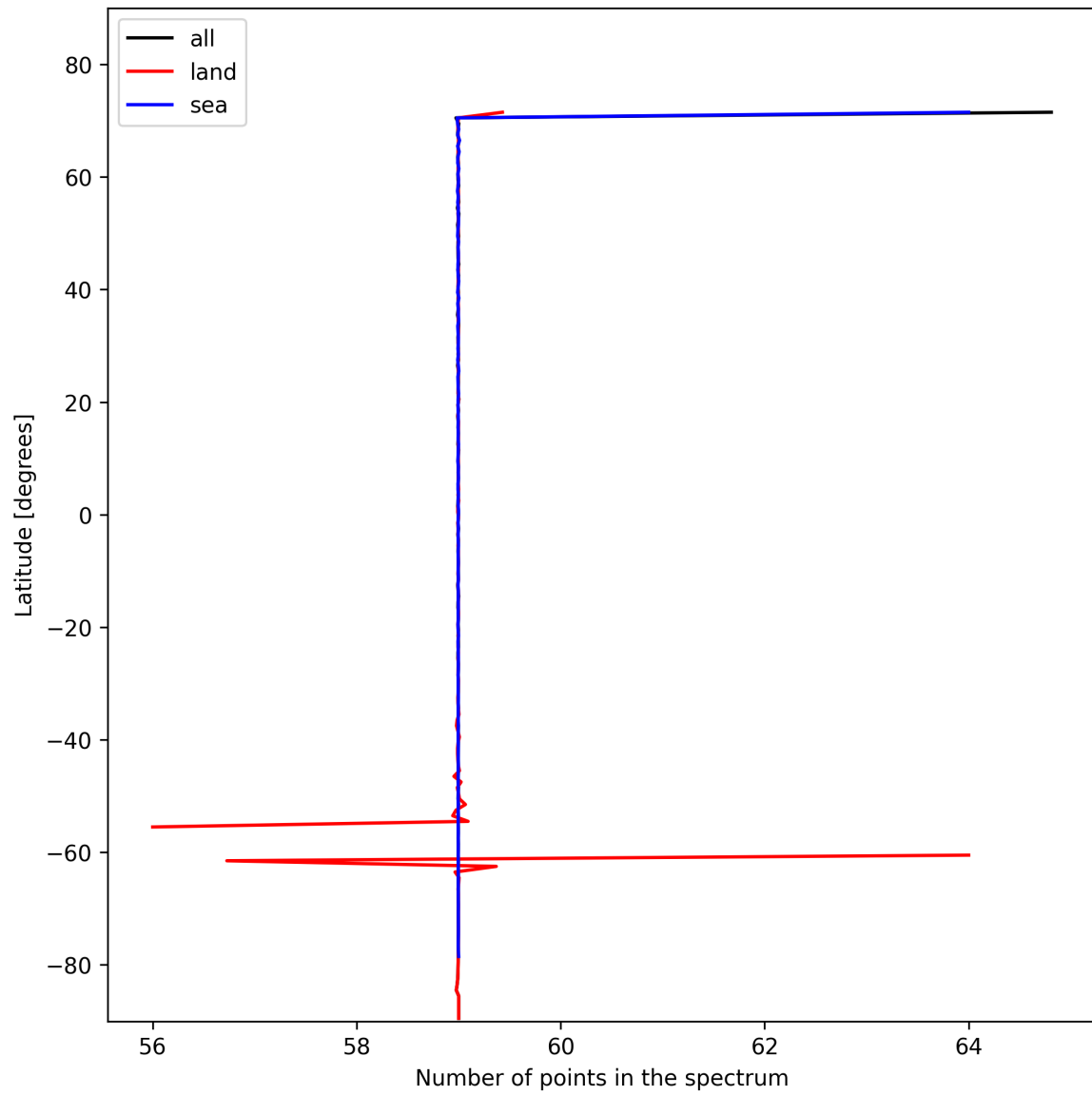
Figure 27: Zonal average of “Number of points in the spectrum” for 2024-11-09 to 2024-11-10.
