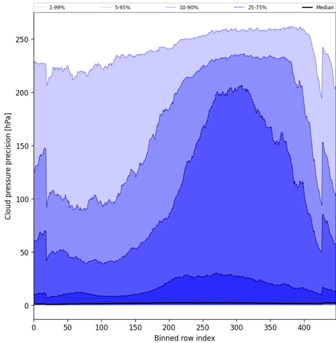
Figure 48: Along track statistics of “Cloud pressure precision” for 2024-11-09 to 2024-11-10
