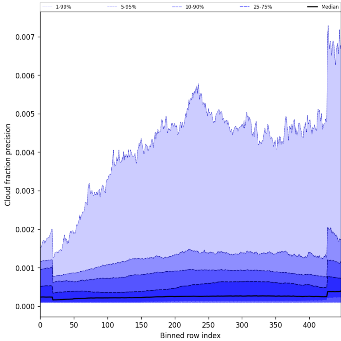
Figure 50: Along track statistics of “Cloud fraction precision” for 2024-11-09 to 2024-11-10
