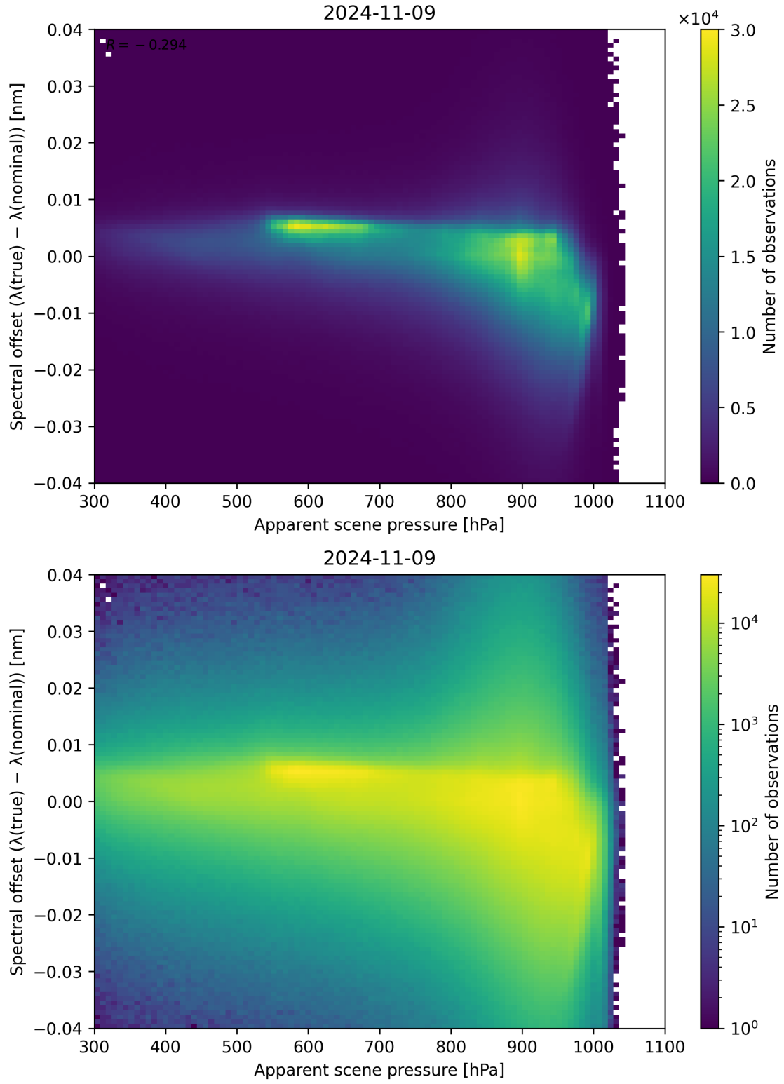
Figure 68: Scatter density plot of “Apparent scene pressure” against “Spectral offset ( \lambda_{\text{true}} - \lambda_{\text{nominal}} )” for 2024-11-09 to 2024-11-10.
