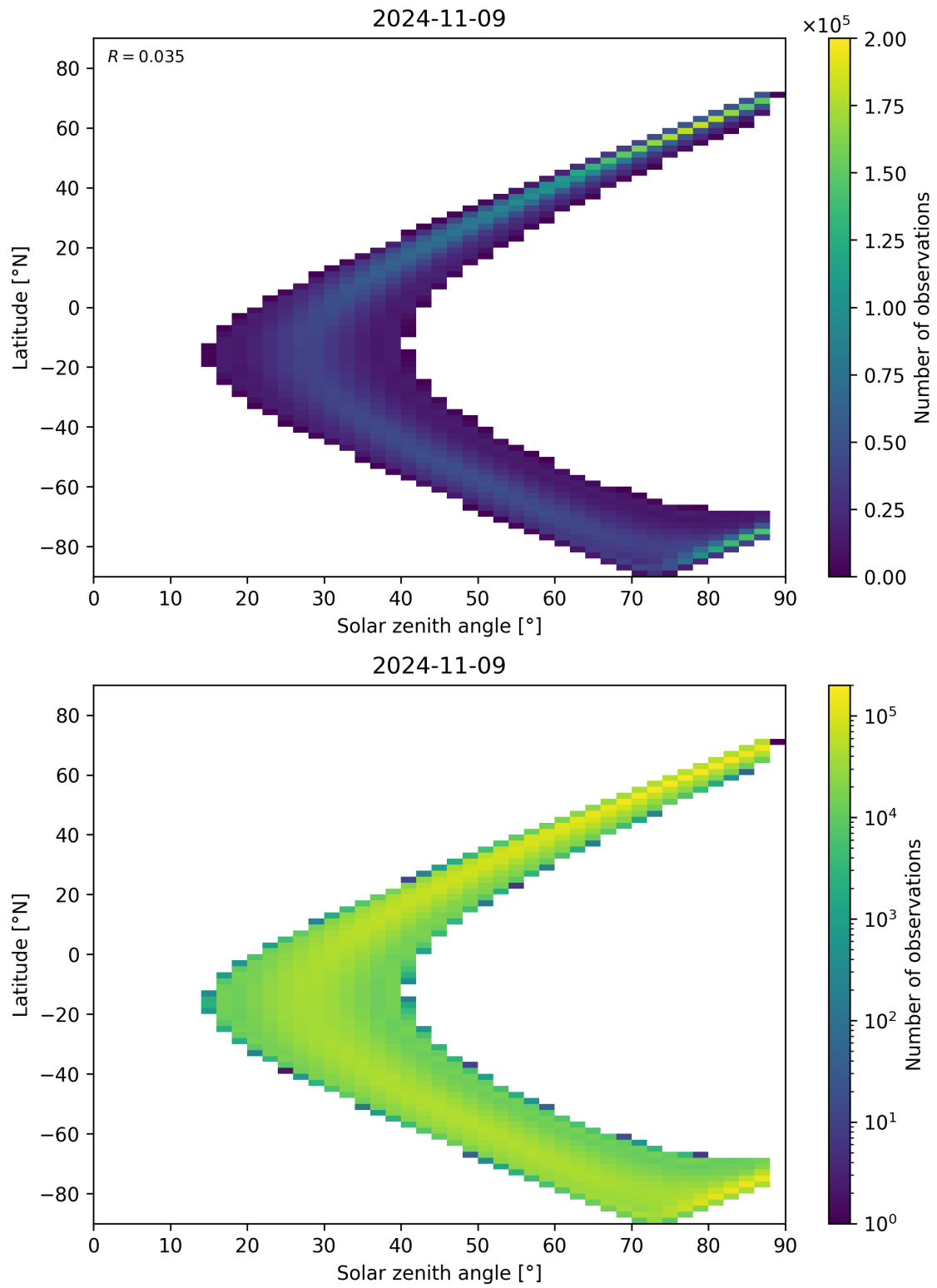
Figure 124: Scatter density plot of “Solar zenith angle” against “Latitude” for 2024-11-09 to 2024-11-10.
