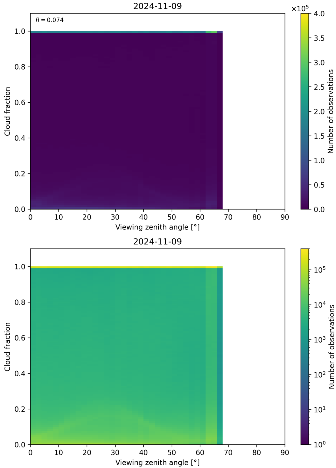
Figure 132: Scatter density plot of “Viewing zenith angle” against “Cloud fraction” for 2024-11-09 to 2024-11-10.
