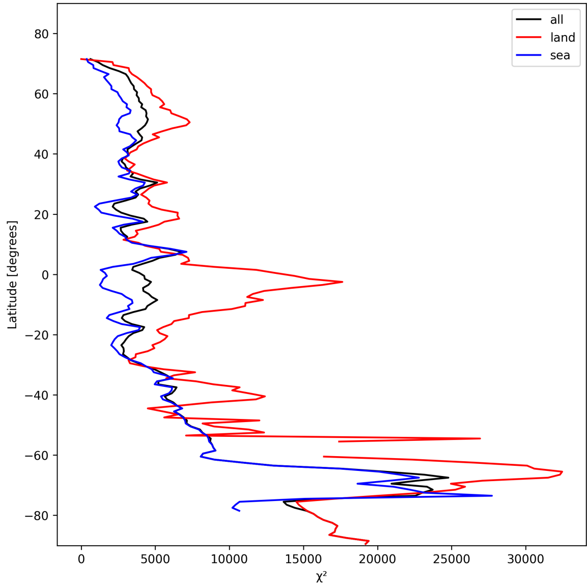
Figure 21: Zonal average of “ \chi^2 ” for 2024-11-09 to 2024-11-10.
