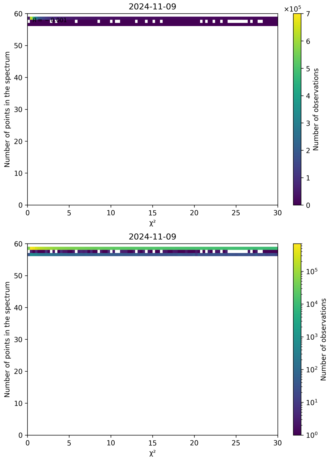
Figure 74: Scatter density plot of “ \chi^2 ” against “Number of points in the spectrum” for 2024-11-09 to 2024-11-10.
