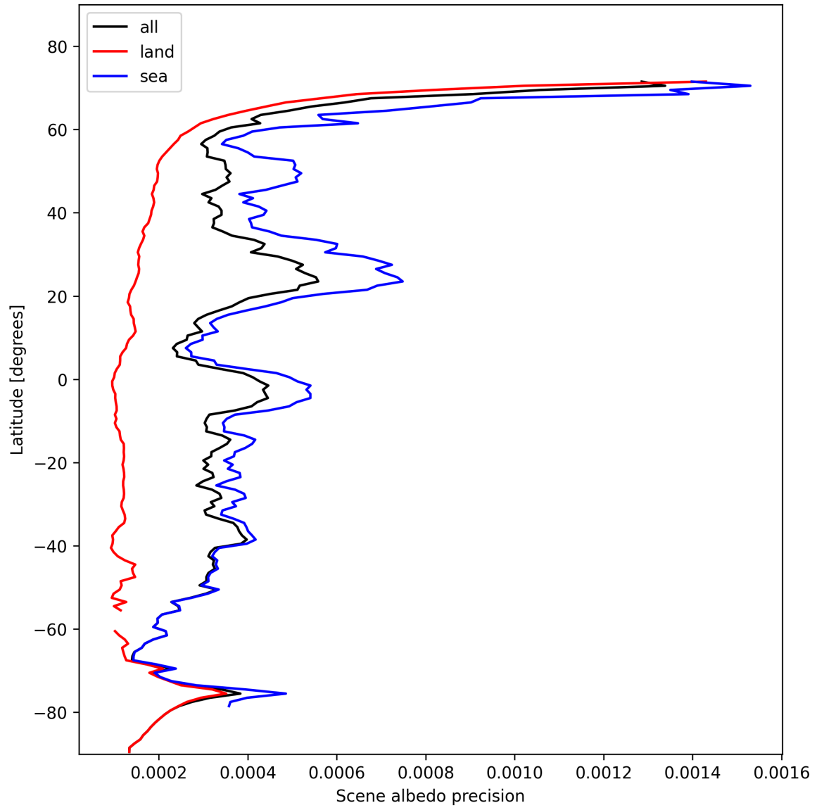
Figure 18: Zonal average of “Scene albedo precision” for 2024-11-09 to 2024-11-10.
