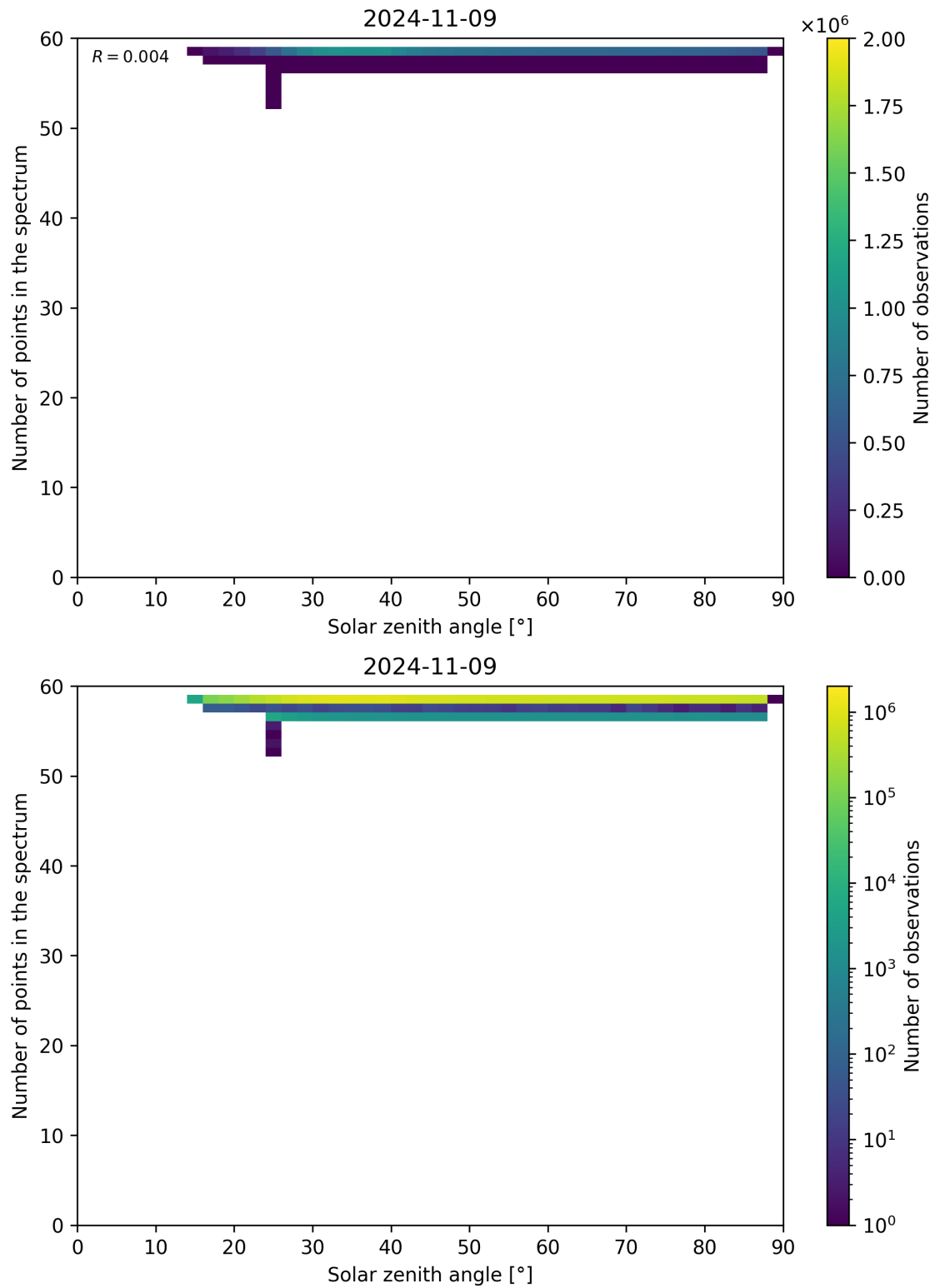
Figure 126: Scatter density plot of “Solar zenith angle” against “Number of points in the spectrum” for 2024-11-09 to 2024-11-10.
