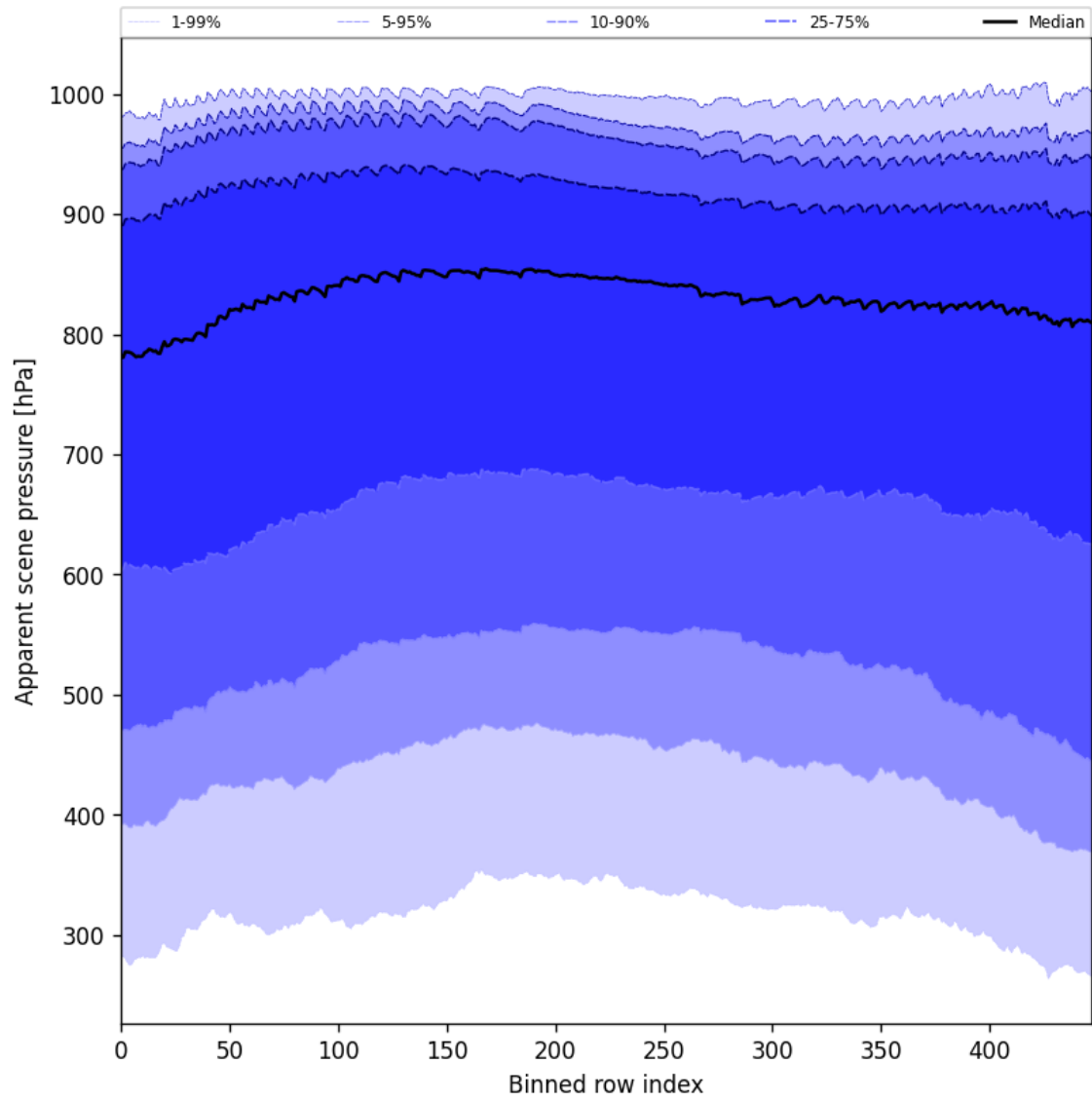
Figure 53: Along track statistics of “Apparent scene pressure” for 2024-11-09 to 2024-11-10
