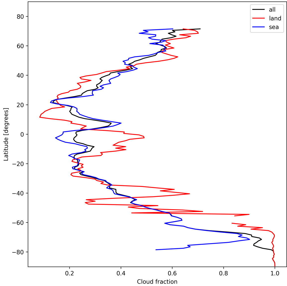
Figure 15: Zonal average of “Cloud fraction” for 2024-11-09 to 2024-11-10.
