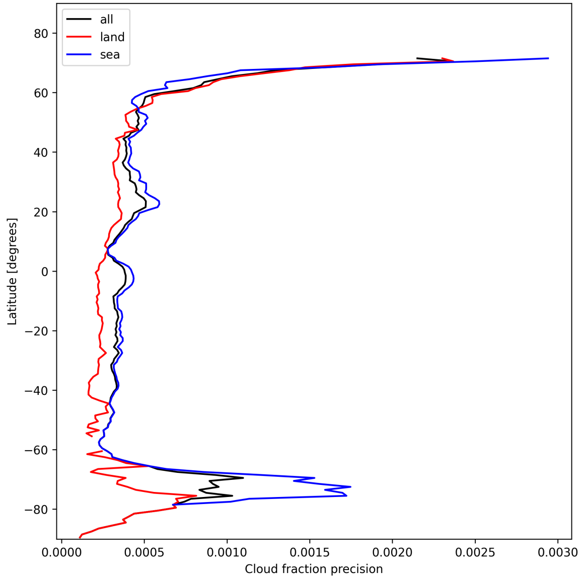
Figure 16: Zonal average of “Cloud fraction precision” for 2024-11-09 to 2024-11-10.
