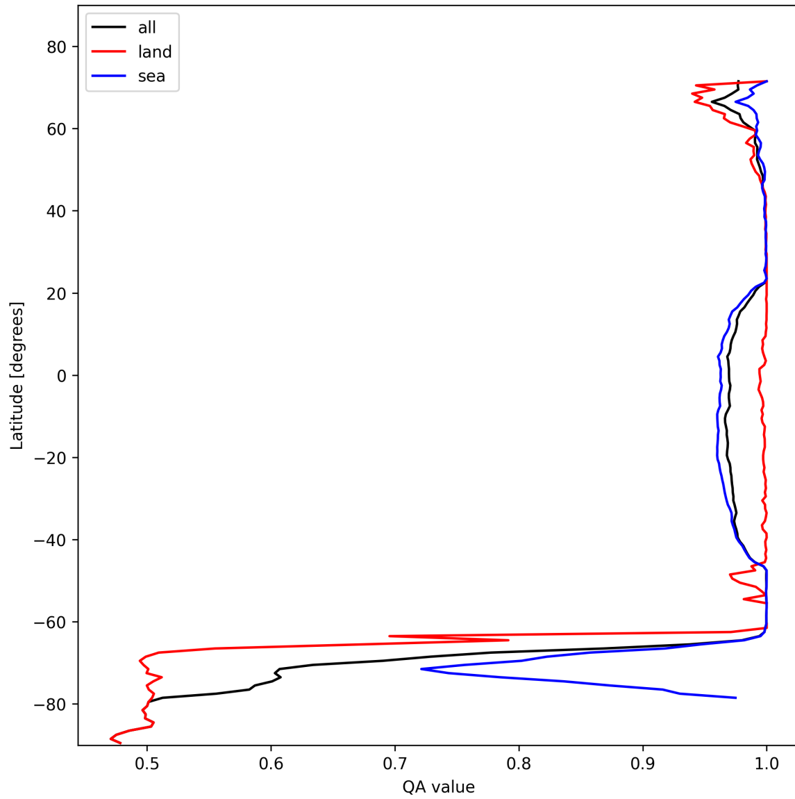
Figure 12: Zonal average of “QA value” for 2024-11-09 to 2024-11-10.
