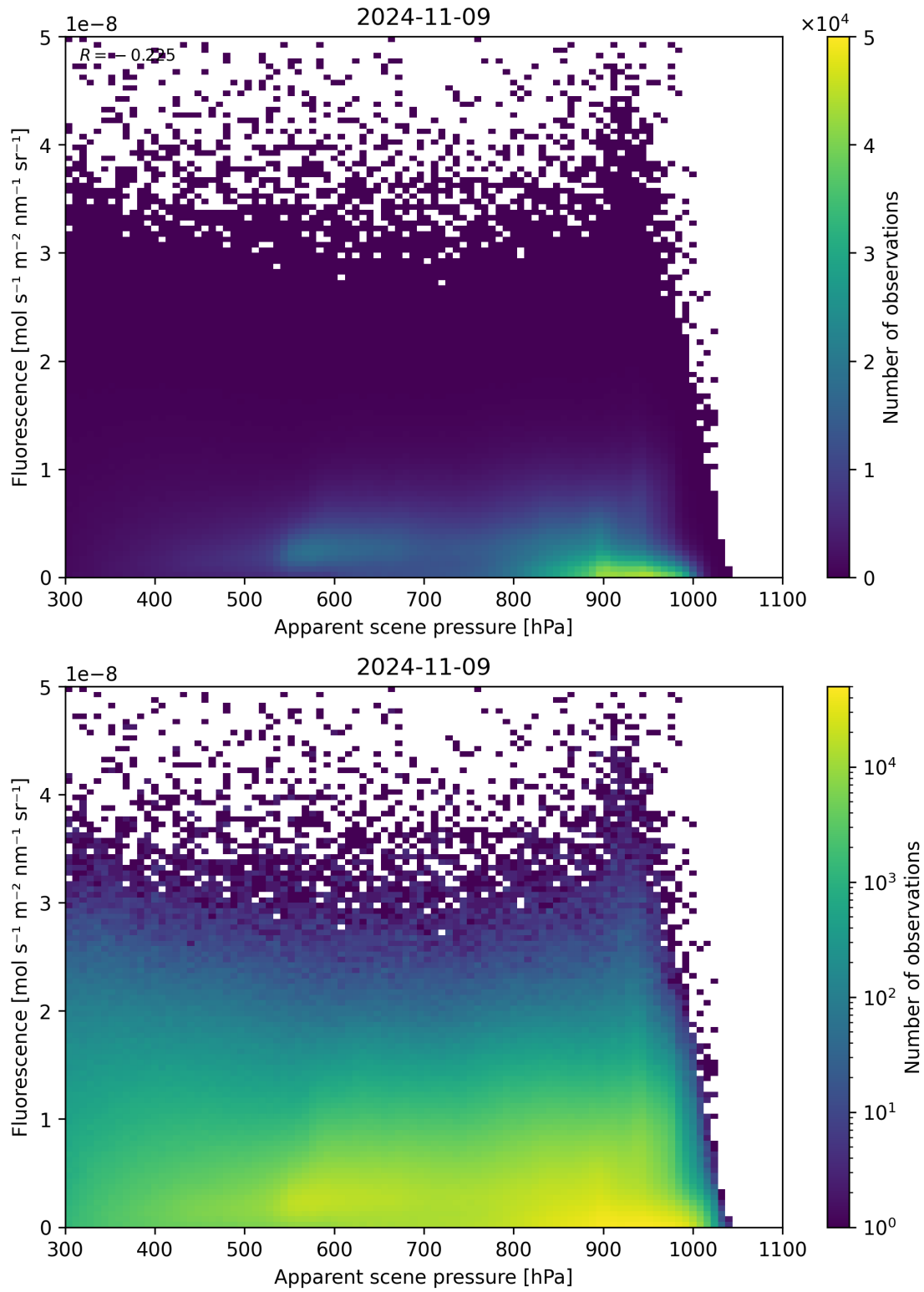
Figure 65: Scatter density plot of “Apparent scene pressure” against “Fluorescence” for 2024-11-09 to 2024-11-10.
