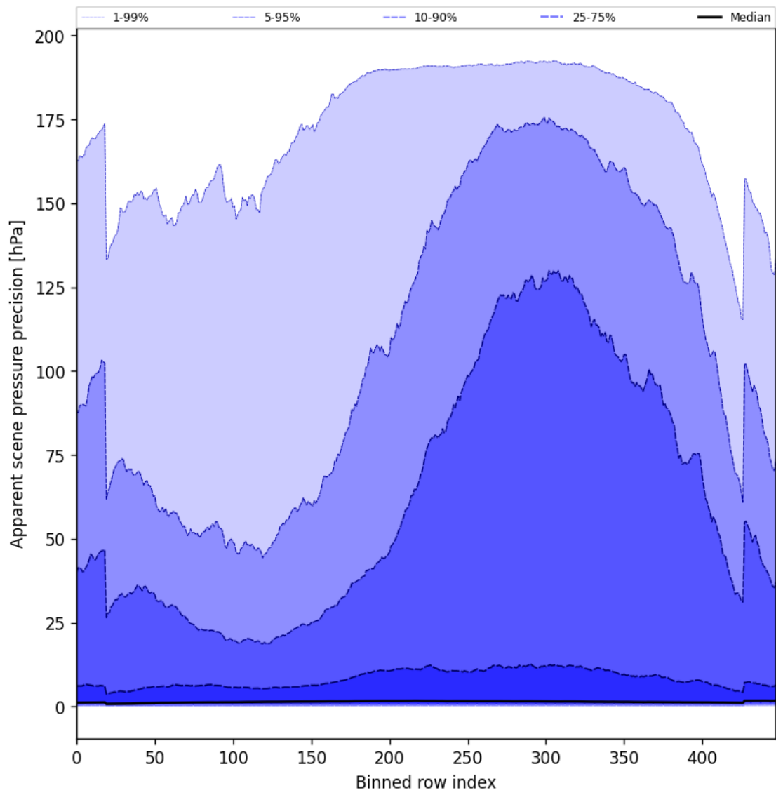
Figure 54: Along track statistics of “Apparent scene pressure precision” for 2024-11-09 to 2024-11-10
