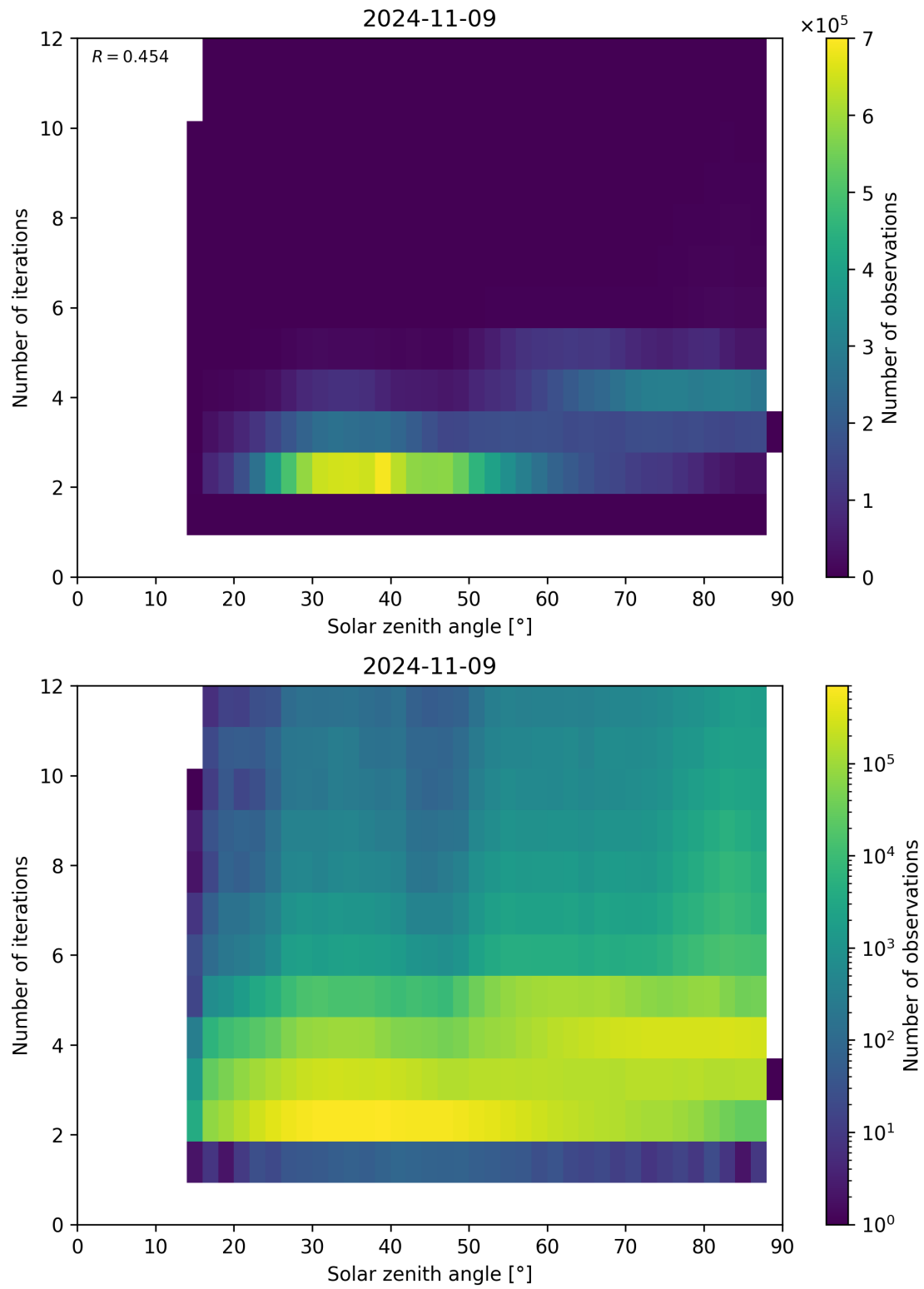
Figure 125: Scatter density plot of “Solar zenith angle” against “Number of iterations” for 2024-11-09 to 2024-11-10.
