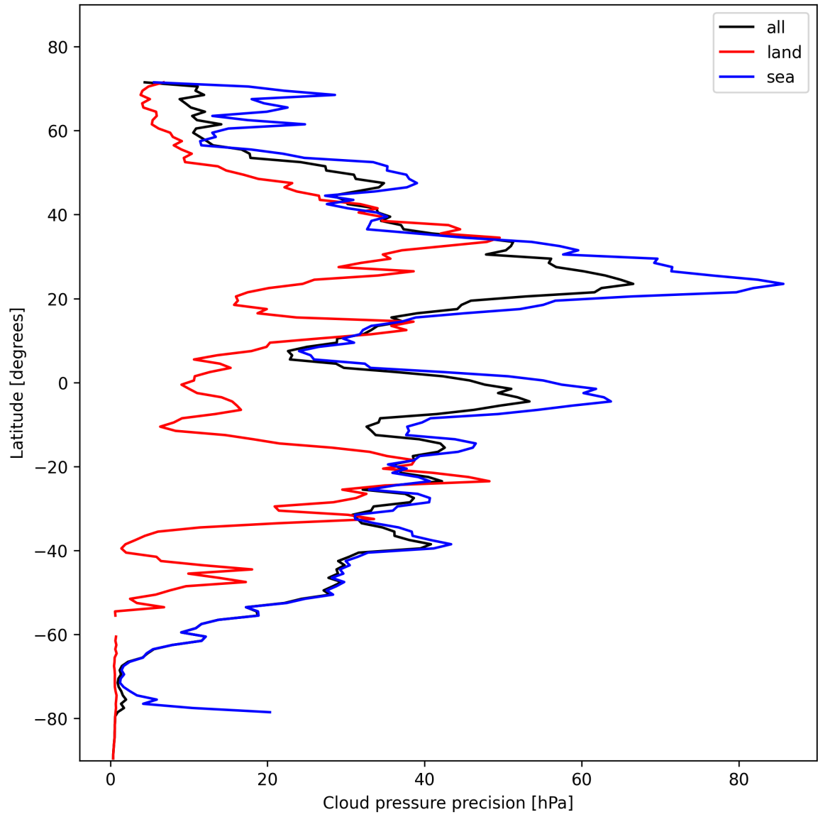
Figure 14: Zonal average of "Cloud pressure precision" for 2024-11-09 to 2024-11-10.
