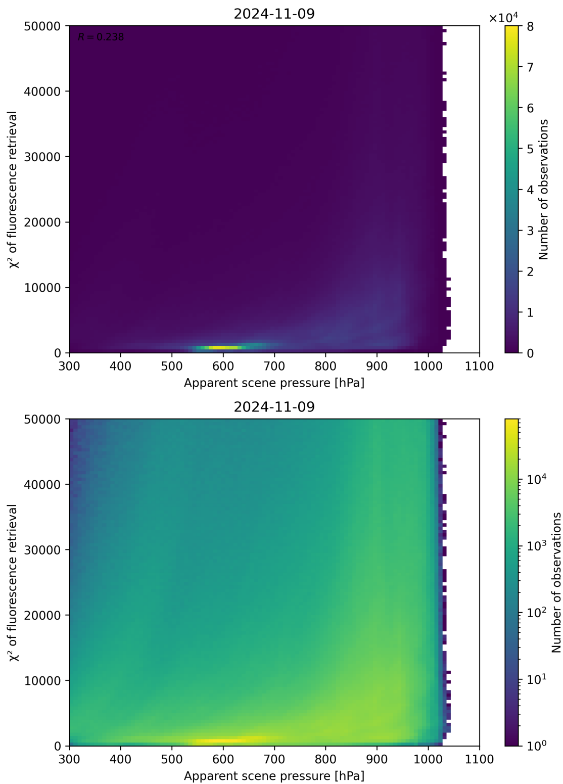
Figure 64: Scatter density plot of “Apparent scene pressure” against “ \chi^2 of fluorescence retrieval” for 2024-11-09 to 2024-11-10.
