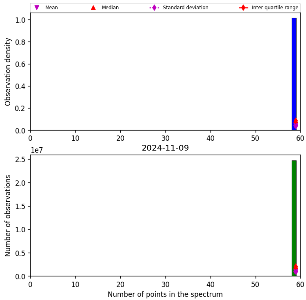
Figure 44: Histogram of “Number of points in the spectrum” for 2024-11-09 to 2024-11-10
