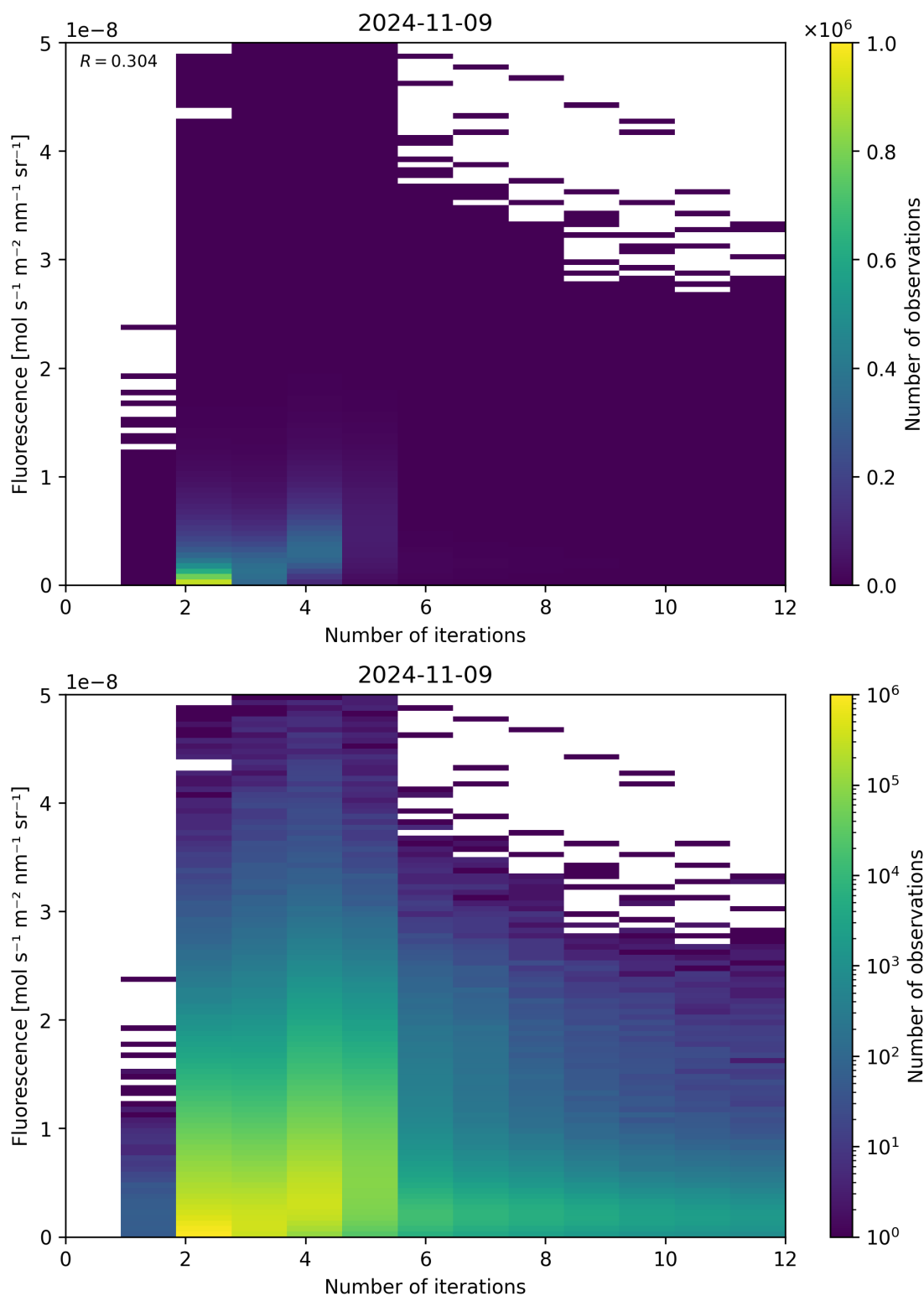
Figure 107: Scatter density plot of “Number of iterations” against “Fluorescence” for 2024-11-09 to 2024-11-10.
