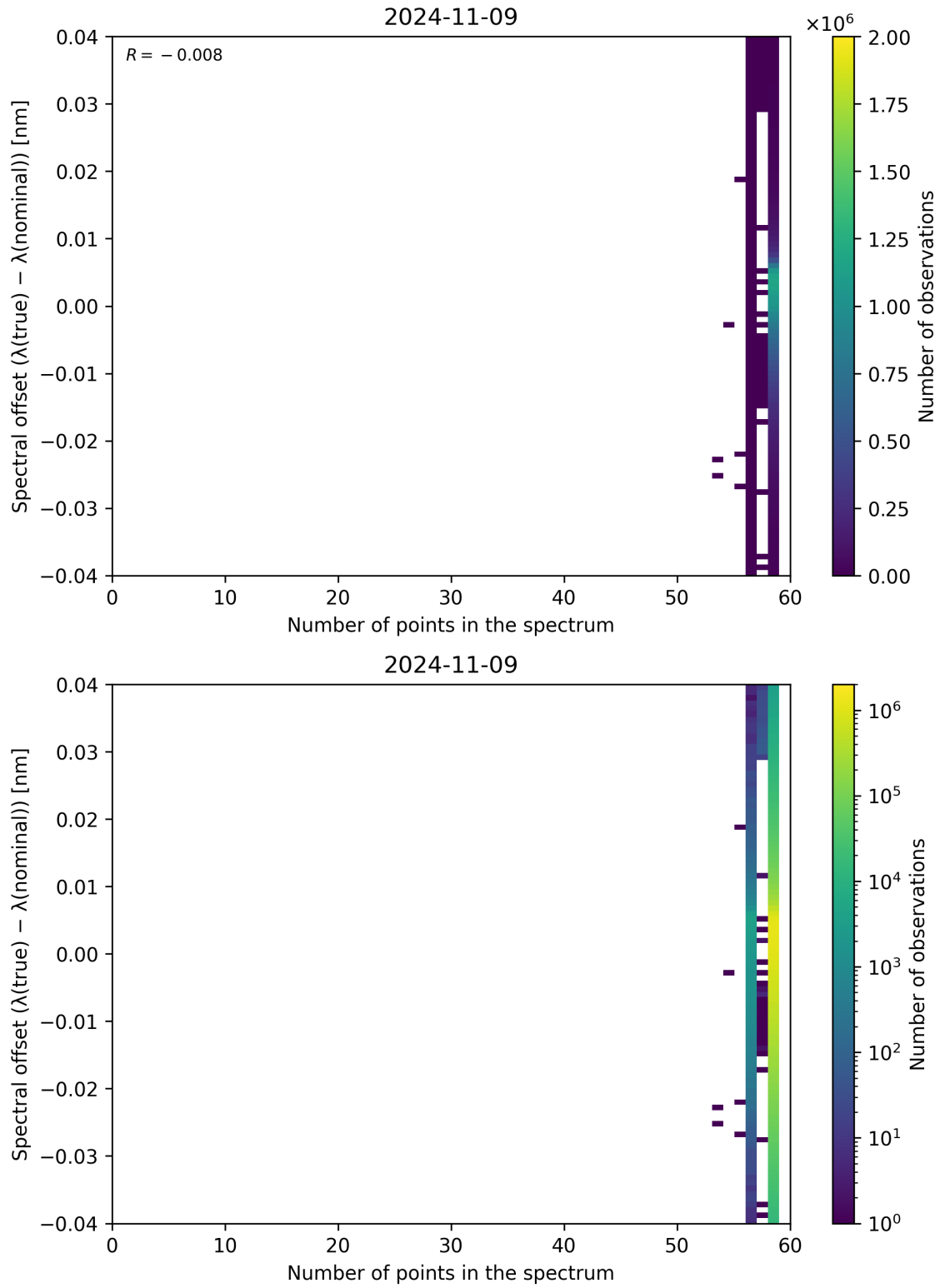
Figure 110: Scatter density plot of “Number of points in the spectrum” against “Spectral offset ( \lambda_{\text{true}} - \lambda_{\text{nominal}} )” for 2024-11-09 to 2024-11-10.
