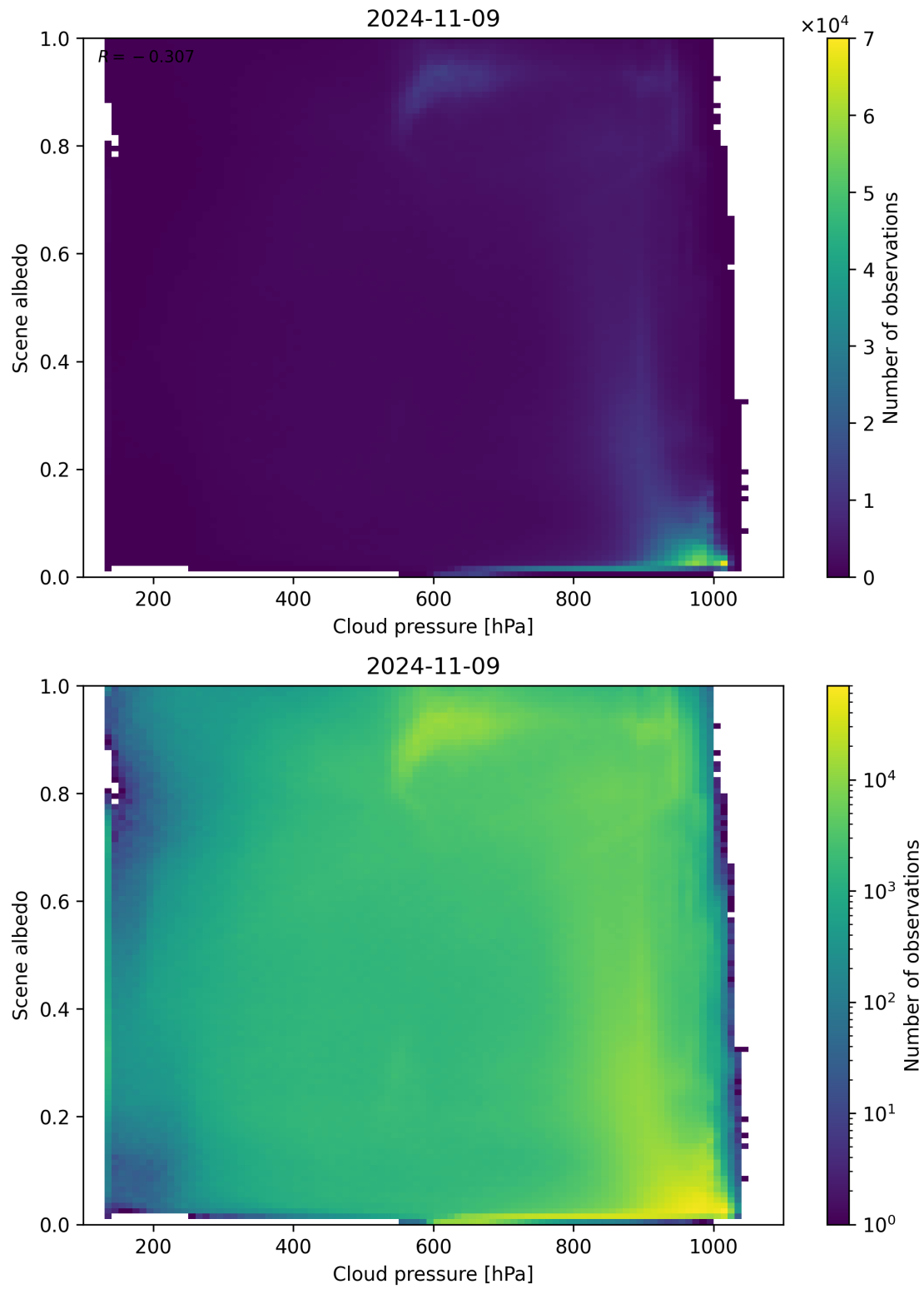
Figure 91: Scatter density plot of “Cloud pressure” against “Scene albedo” for 2024-11-09 to 2024-11-10.
