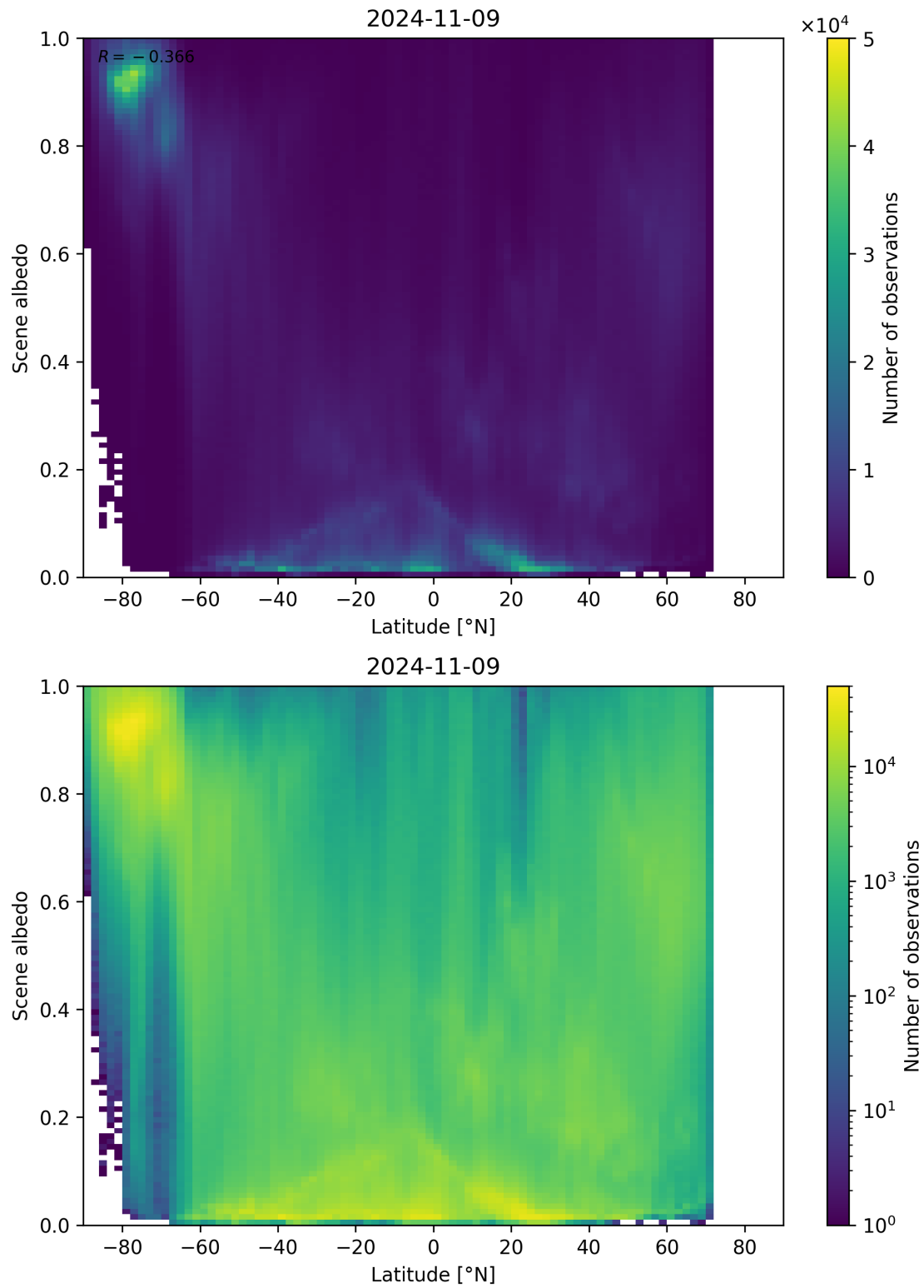
Figure 104: Scatter density plot of “Latitude” against “Scene albedo” for 2024-11-09 to 2024-11-10.
