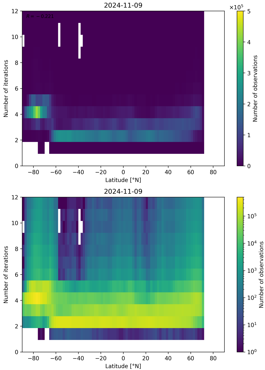
Figure 102: Scatter density plot of “Latitude” against “Number of iterations” for 2024-11-09 to 2024-11-10.
