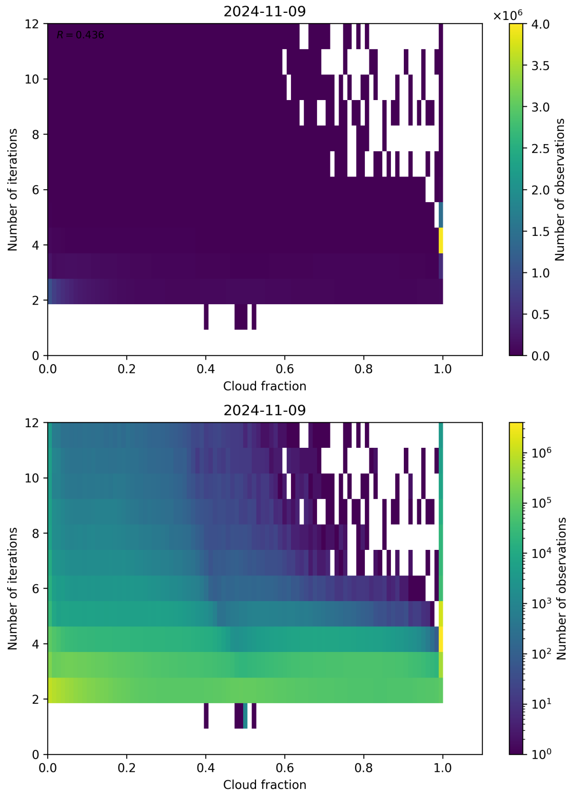
Figure 80: Scatter density plot of “Cloud fraction” against “Number of iterations” for 2024-11-09 to 2024-11-10.
