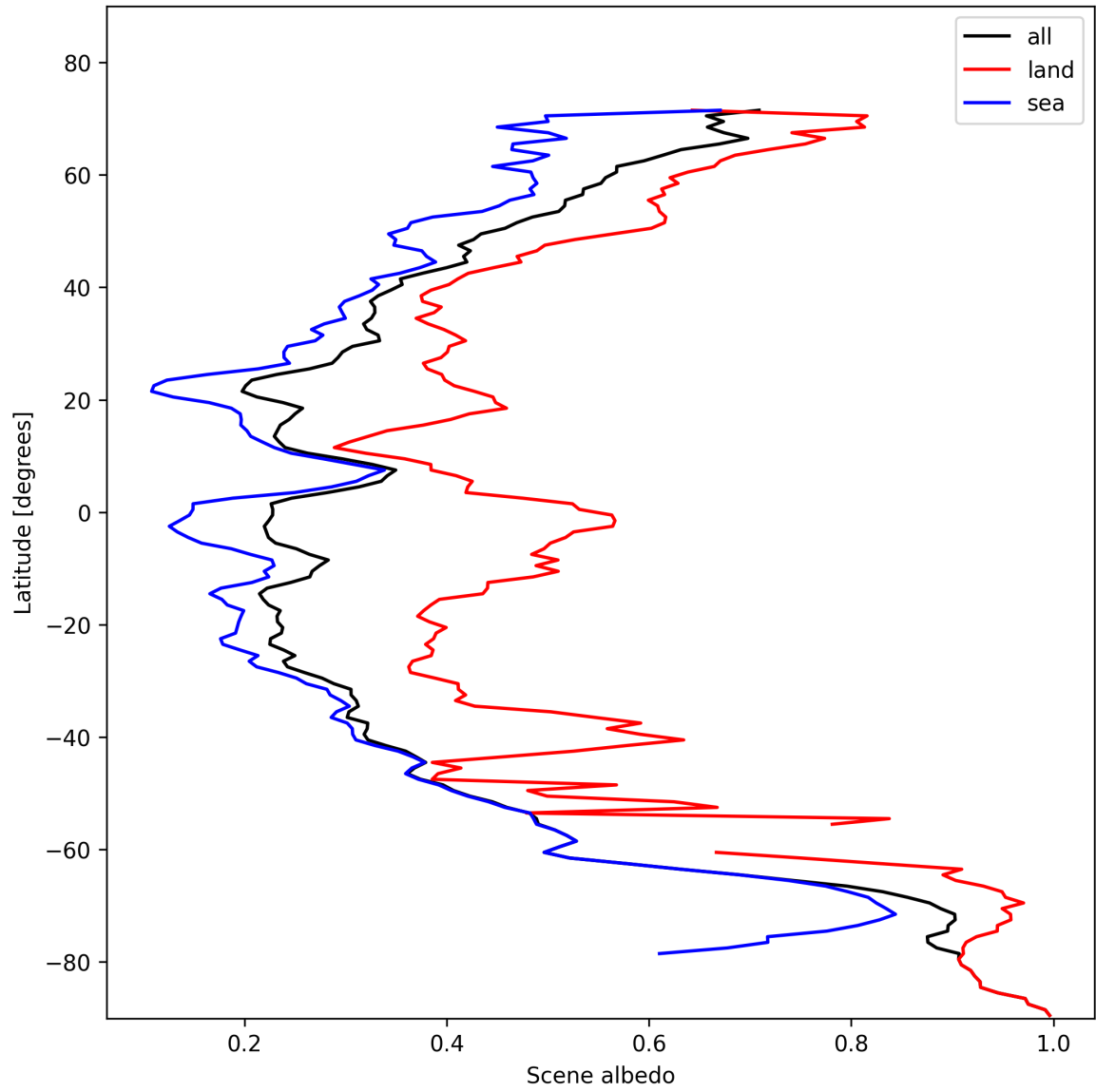
Figure 17: Zonal average of “Scene albedo” for 2024-11-09 to 2024-11-10.
