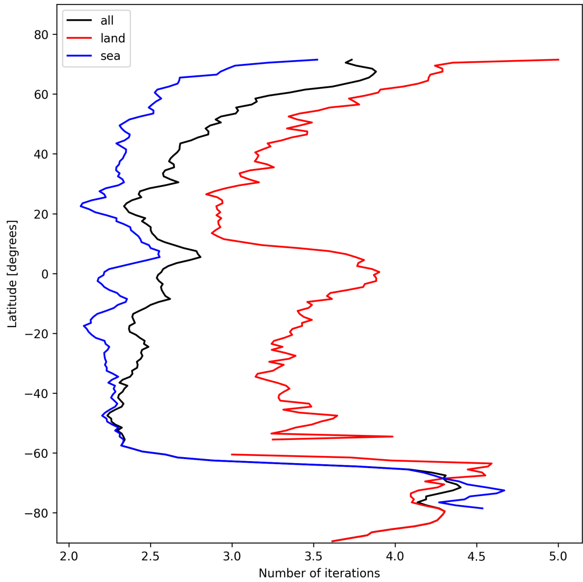
Figure 22: Zonal average of “Number of iterations” for 2024-11-09 to 2024-11-10.
