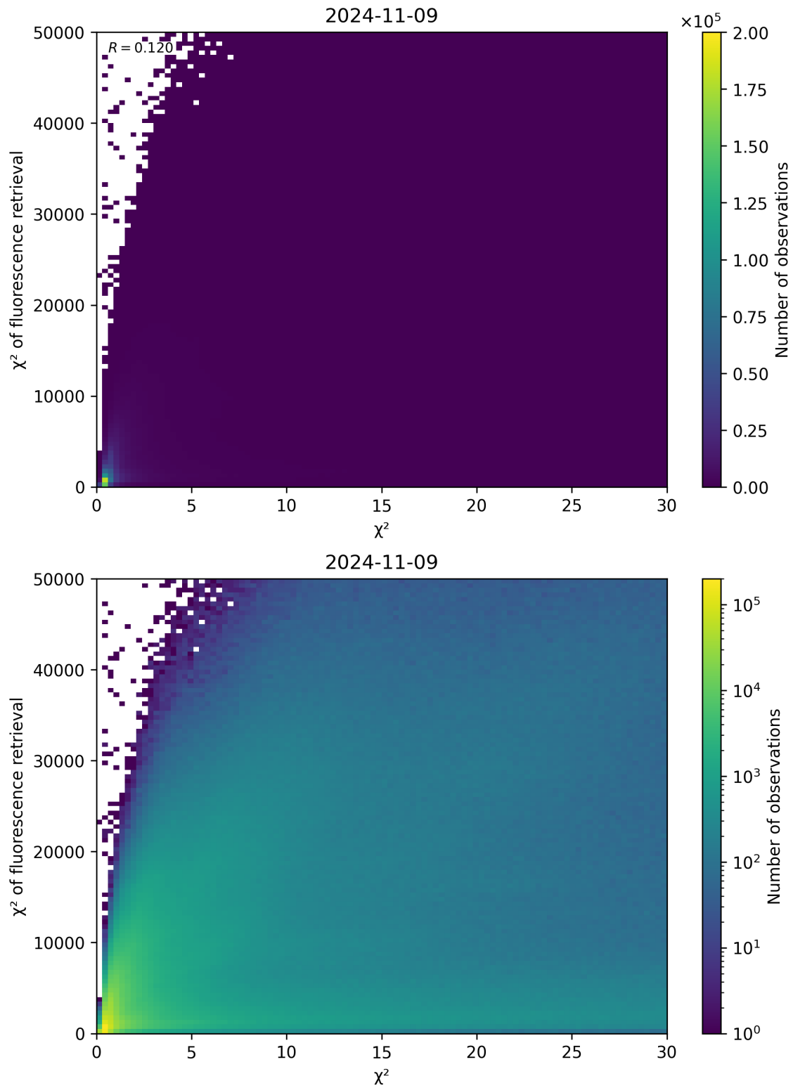
Figure 69: Scatter density plot of “ \chi^2 ” against “ \chi^2 of fluorescence retrieval” for 2024-11-09 to 2024-11-10.
