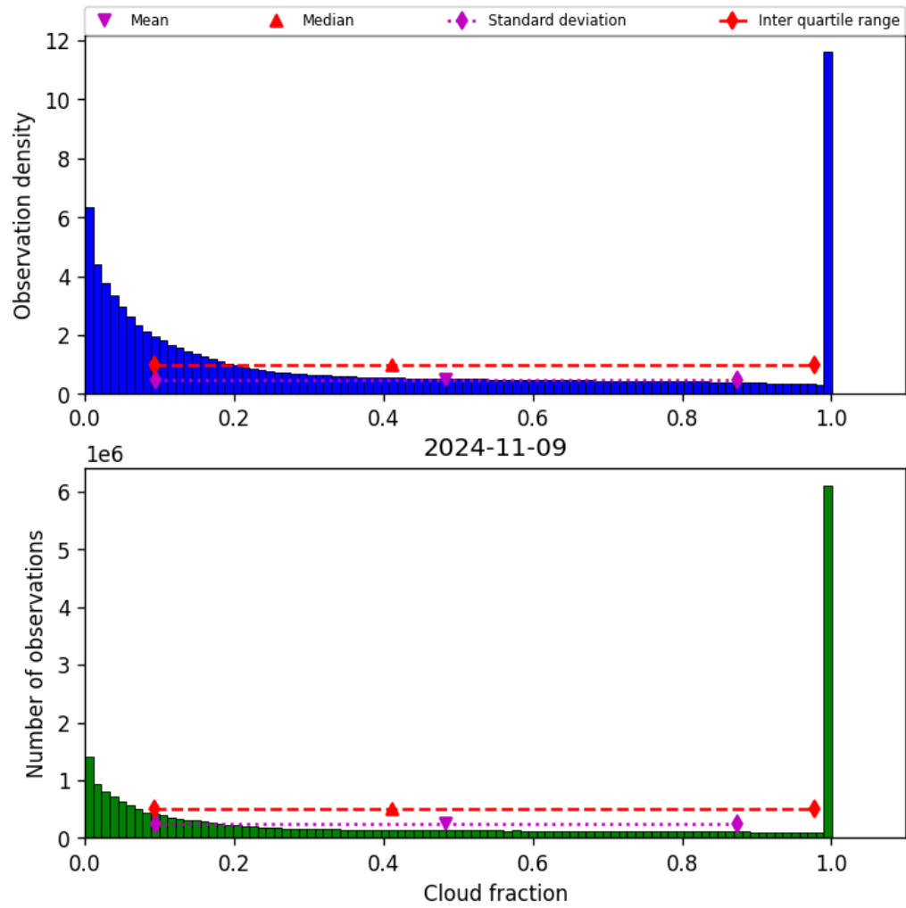
Figure 32: Histogram of “Cloud fraction” for 2024-11-09 to 2024-11-10
