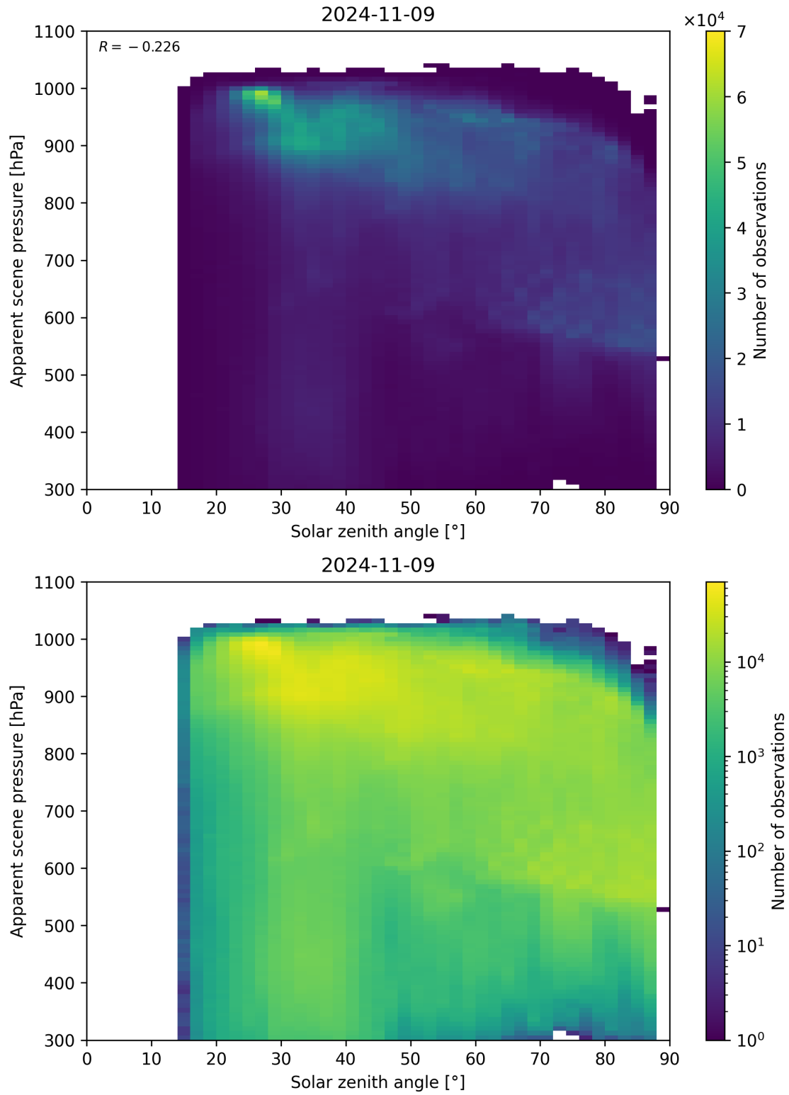
Figure 118: Scatter density plot of “Solar zenith angle” against “Apparent scene pressure” for 2024-11-09 to 2024-11-10.
