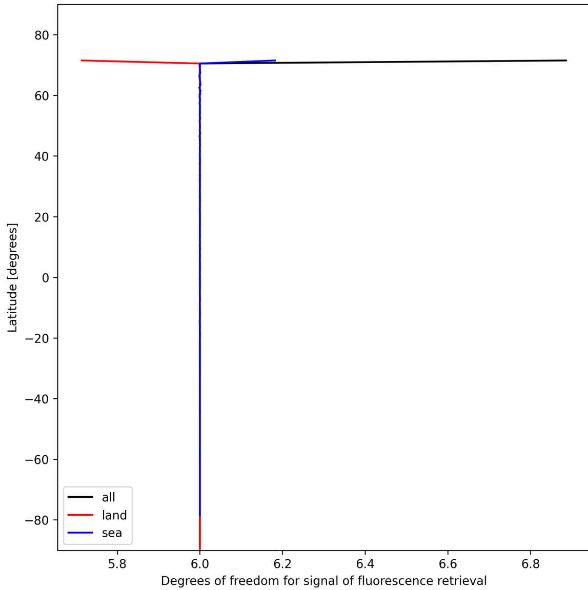
Figure 26: Zonal average of “Degrees of freedom for signal of fluorescence retrieval” for 2024-11-09 to 2024-11-10.
