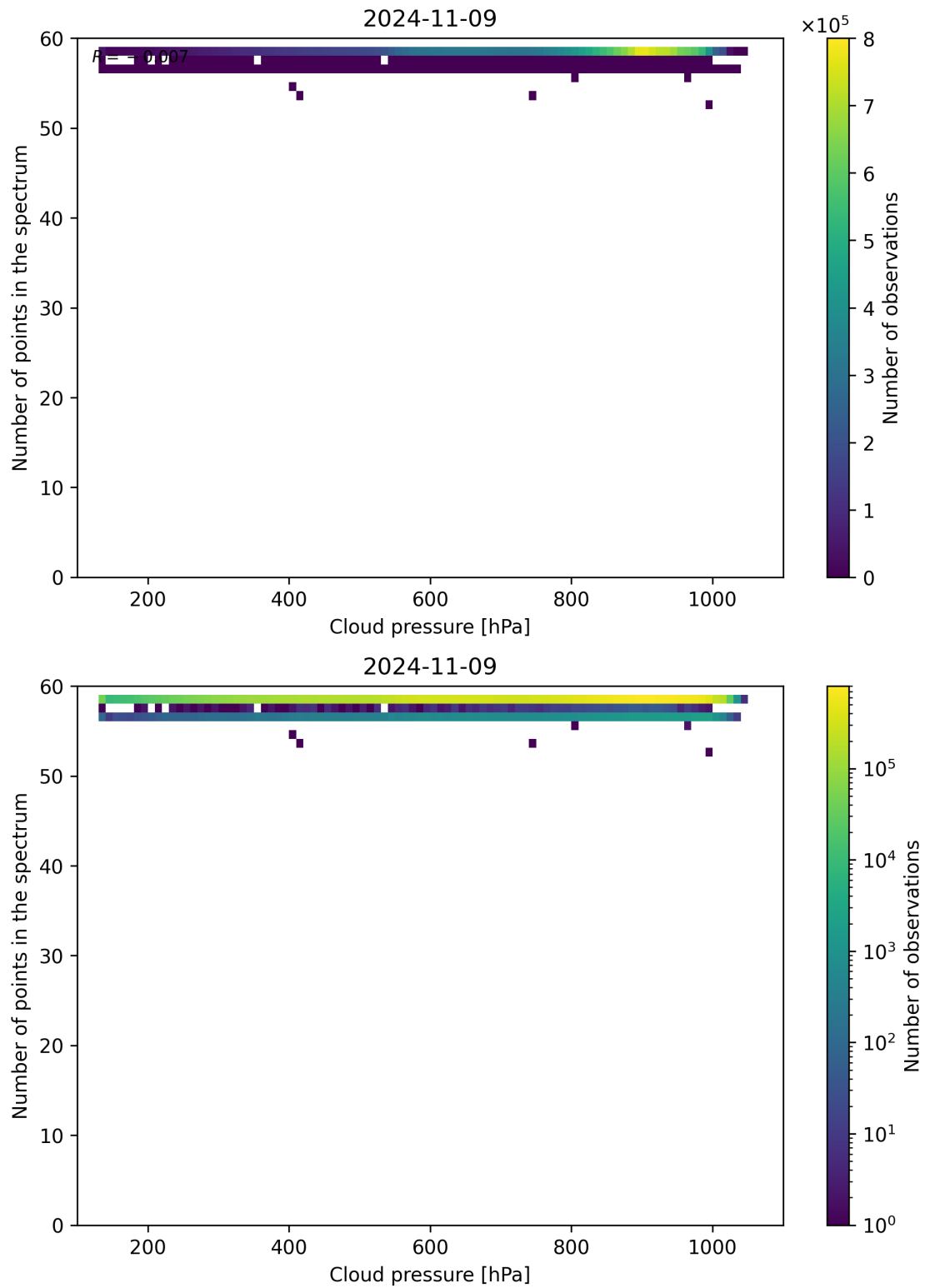
Figure 90: Scatter density plot of “Cloud pressure” against “Number of points in the spectrum” for 2024-11-09 to 2024-11-10.
