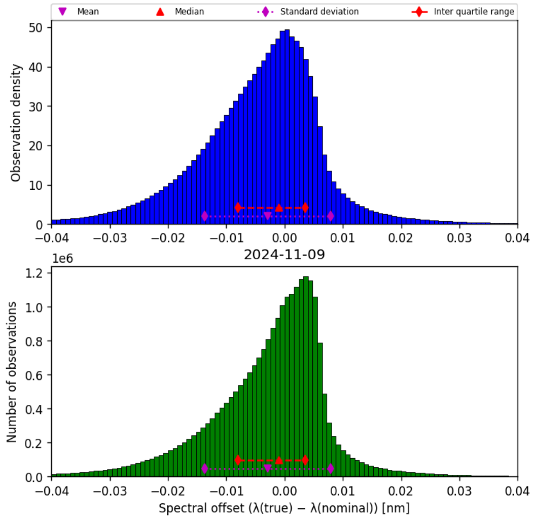
Figure 45: Histogram of “Spectral offset ( \lambda_{\text{true}} - \lambda_{\text{nominal}} )” for 2024-11-09 to 2024-11-10
