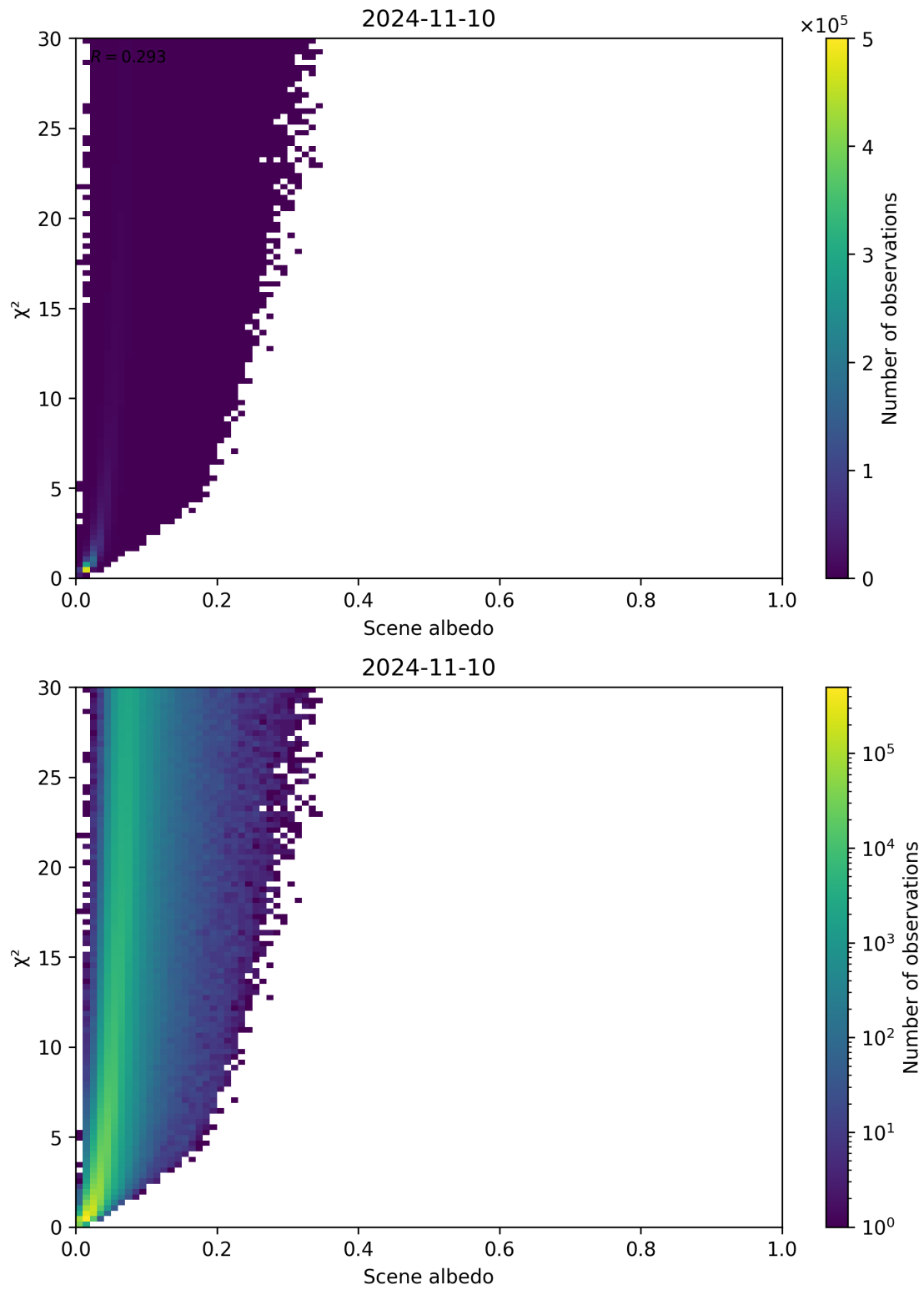
Figure 112: Scatter density plot of “Scene albedo” against “ \chi^2 ” for 2024-11-09 to 2024-11-11.
