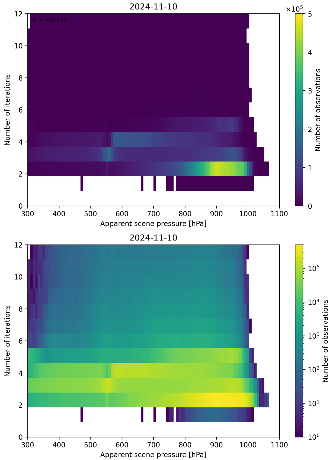
Figure 66: Scatter density plot of “Apparent scene pressure” against “Number of iterations” for 2024-11-09 to 2024-11-11.
