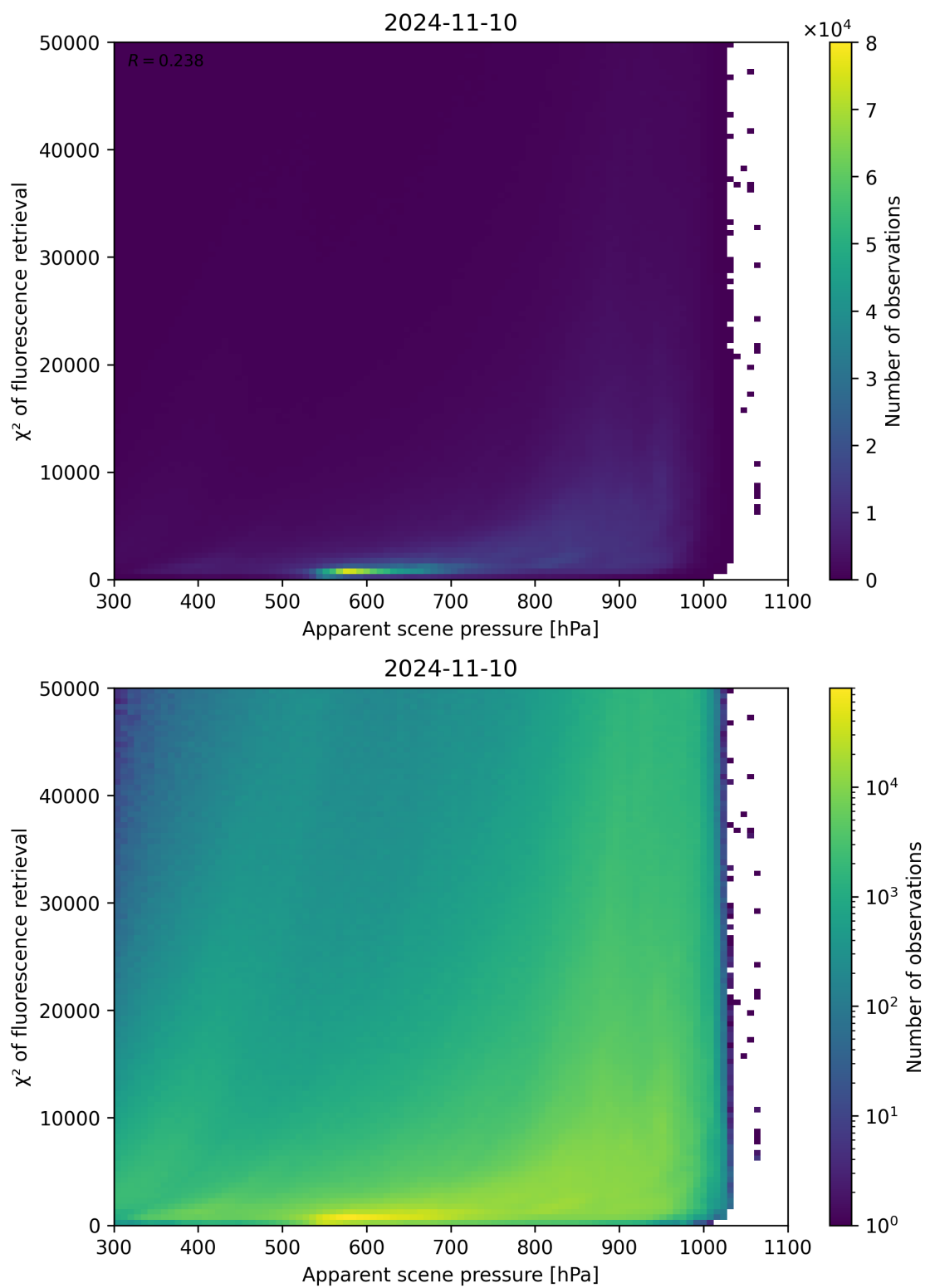
Figure 64: Scatter density plot of “Apparent scene pressure” against “ \chi^2 of fluorescence retrieval” for 2024-11-09 to 2024-11-11.
