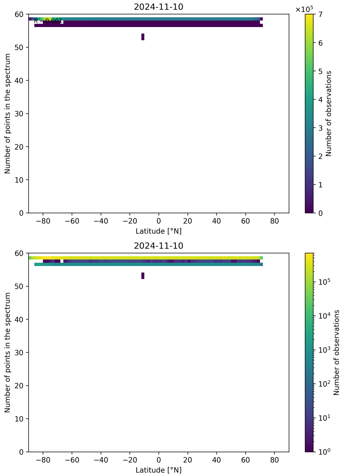
Figure 103: Scatter density plot of “Latitude” against “Number of points in the spectrum” for 2024-11-09 to 2024-11-11.
