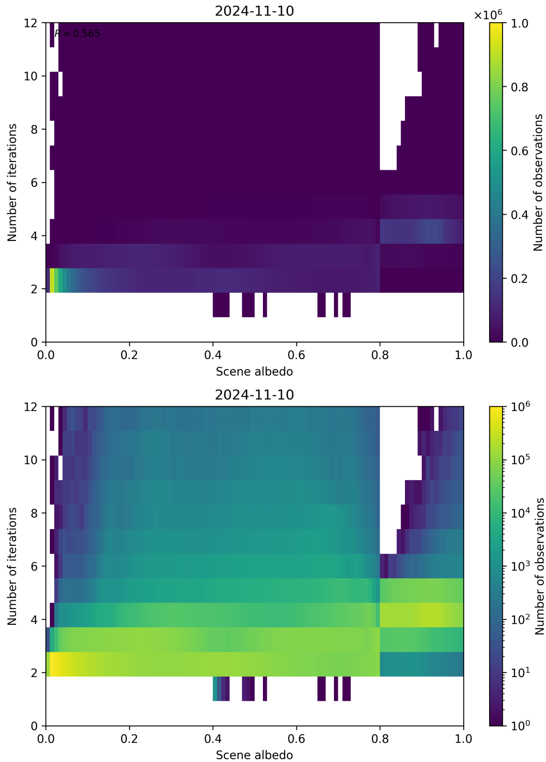
Figure 115: Scatter density plot of “Scene albedo” against “Number of iterations” for 2024-11-09 to 2024-11-11.
