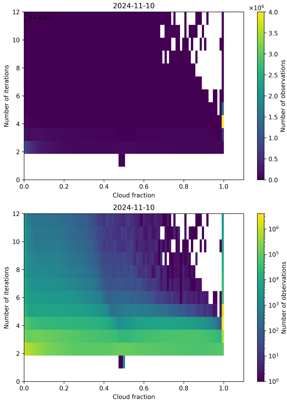
Figure 80: Scatter density plot of “Cloud fraction” against “Number of iterations” for 2024-11-09 to 2024-11-11.
