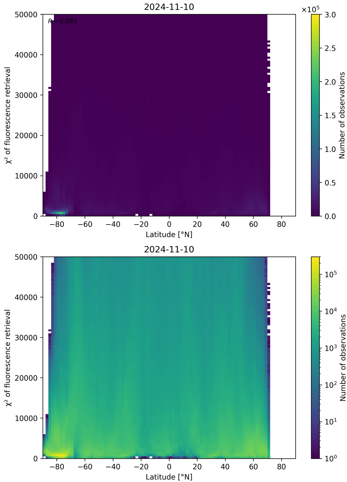
Figure 98: Scatter density plot of “Latitude” against “ \chi^2 of fluorescence retrieval” for 2024-11-09 to 2024-11-11.
