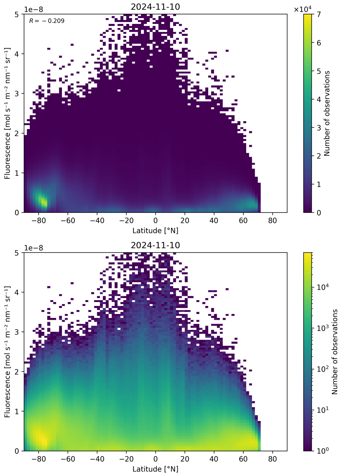
Figure 101: Scatter density plot of “Latitude” against “Fluorescence” for 2024-11-09 to 2024-11-11.
