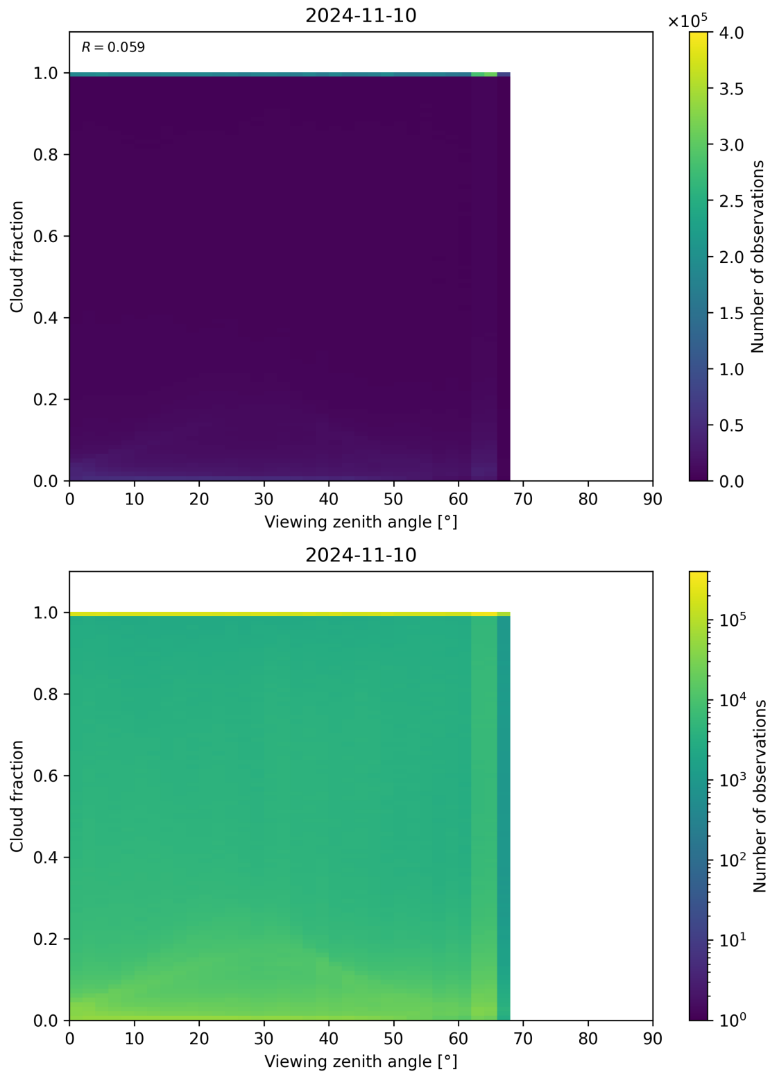
Figure 132: Scatter density plot of “Viewing zenith angle” against “Cloud fraction” for 2024-11-09 to 2024-11-11.
