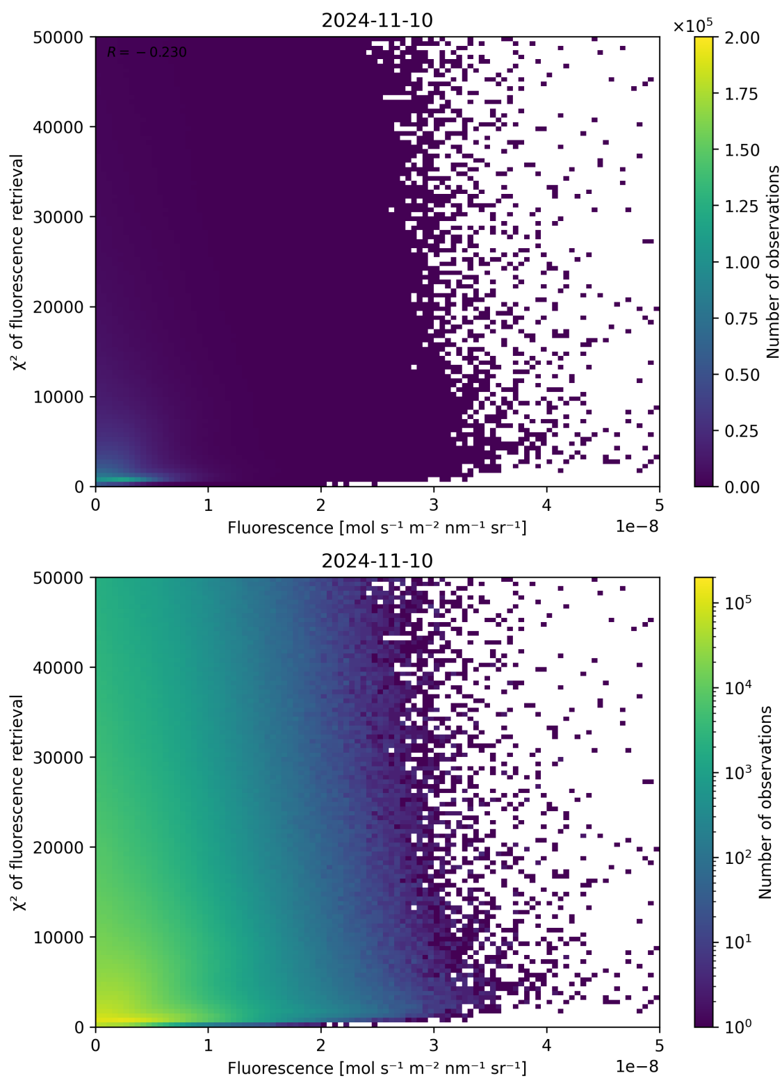
Figure 93: Scatter density plot of “Fluorescence” against “ \chi^2 of fluorescence retrieval” for 2024-11-09 to 2024-11-11.
