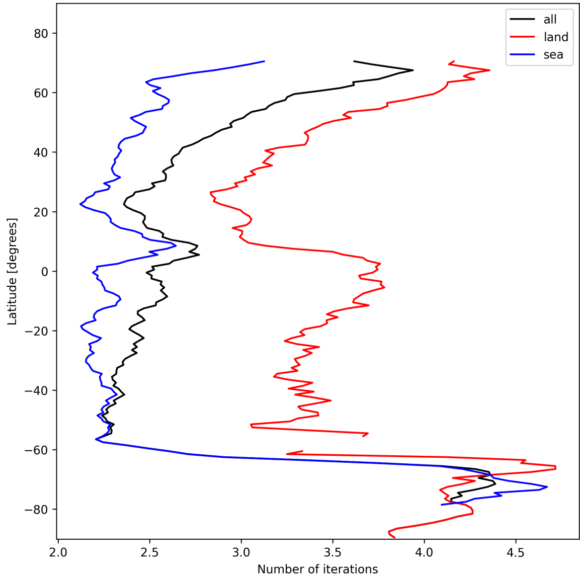
Figure 22: Zonal average of “Number of iterations” for 2024-11-09 to 2024-11-11.
