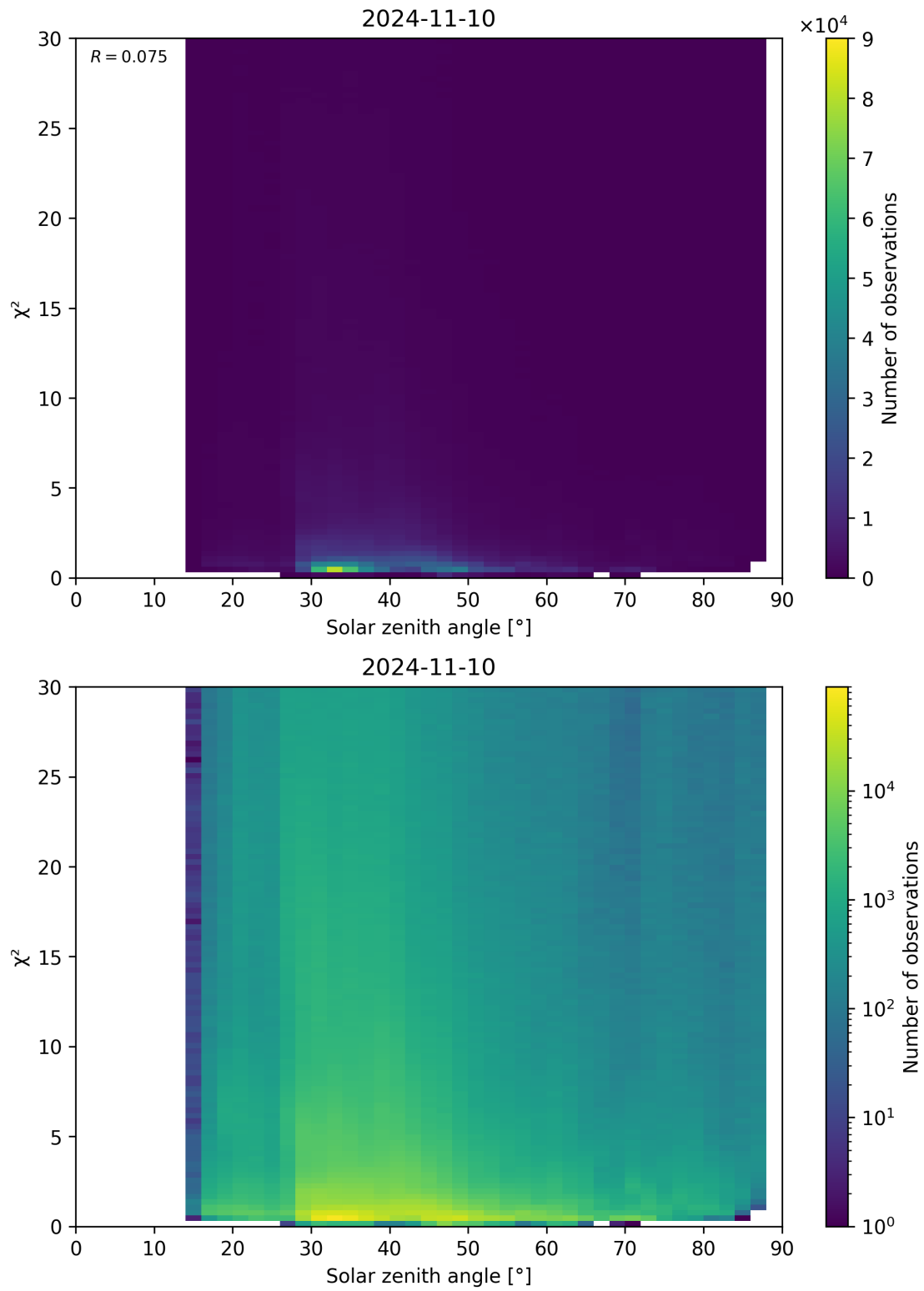
Figure 119: Scatter density plot of “Solar zenith angle” against “ \chi^2 ” for 2024-11-09 to 2024-11-11.
