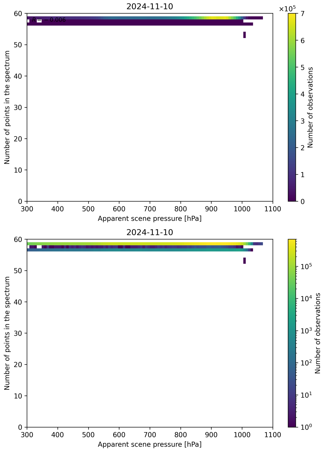
Figure 67: Scatter density plot of “Apparent scene pressure” against “Number of points in the spectrum” for 2024-11-09 to 2024-11-11.
