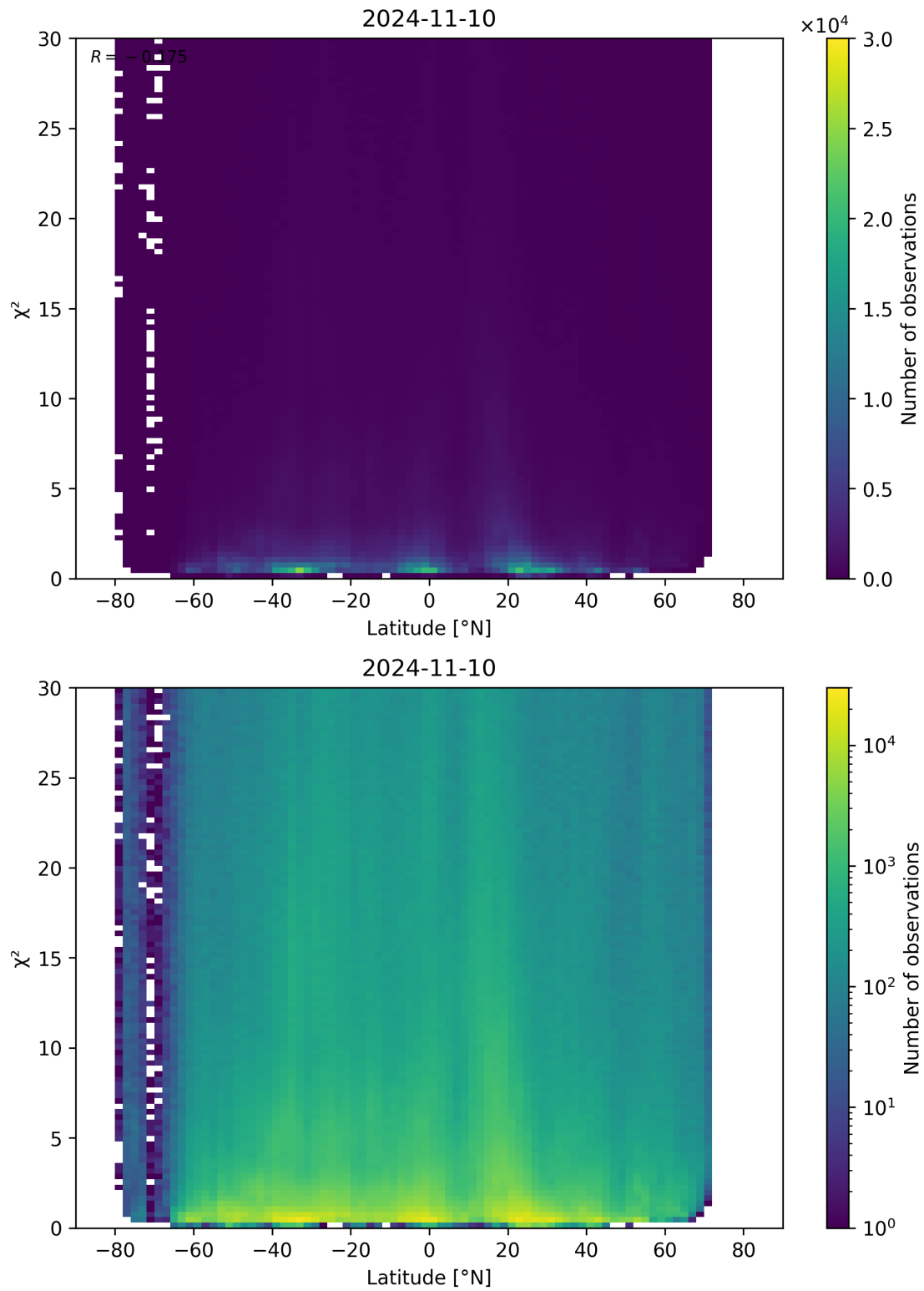
Figure 97: Scatter density plot of “Latitude” against “ \chi^2 ” for 2024-11-09 to 2024-11-11.
