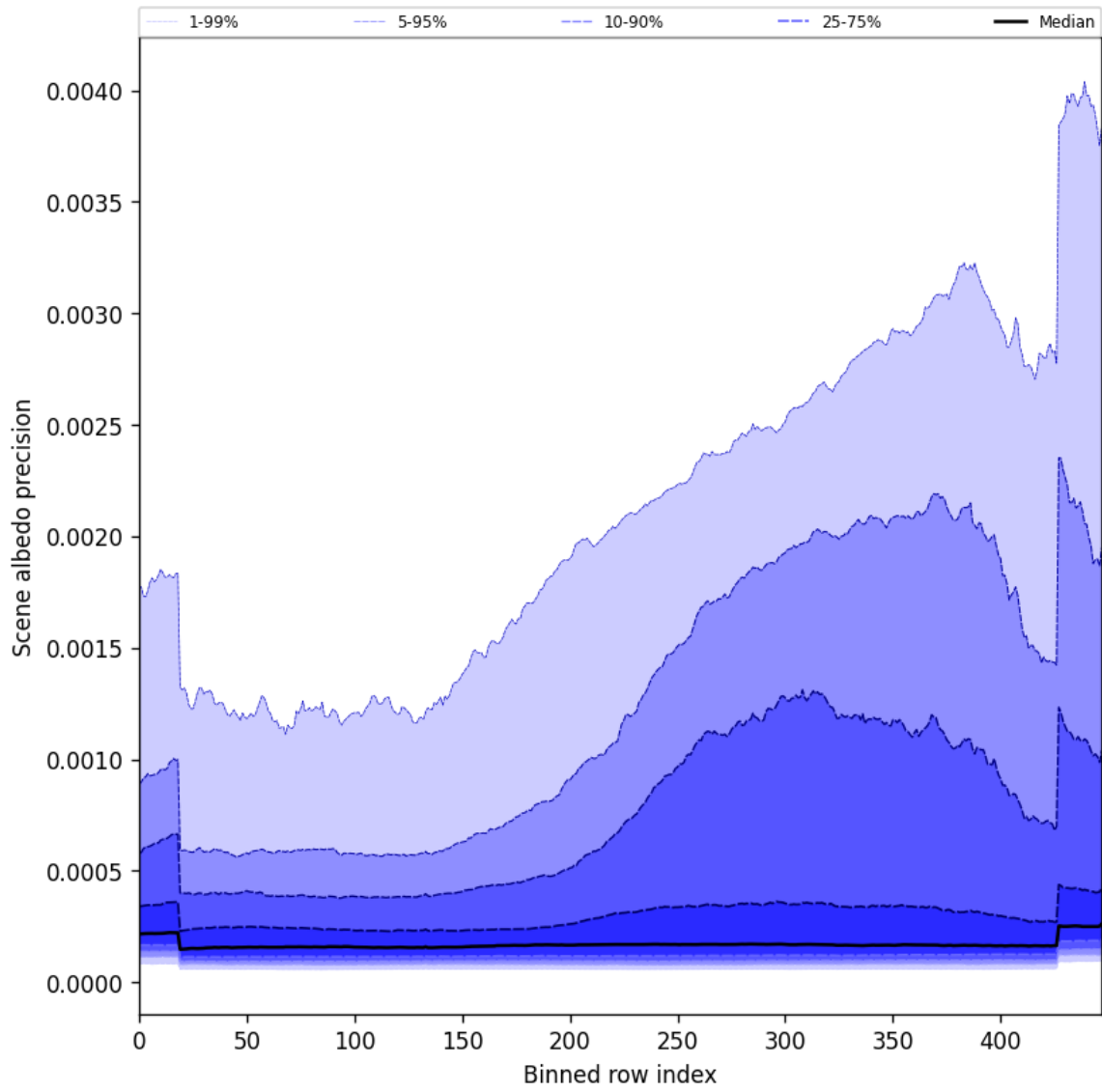
Figure 52: Along track statistics of “Scene albedo precision” for 2024-11-09 to 2024-11-11
