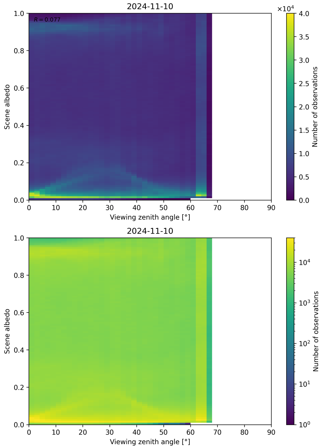
Figure 138: Scatter density plot of “Viewing zenith angle” against “Scene albedo” for 2024-11-09 to 2024-11-11.
