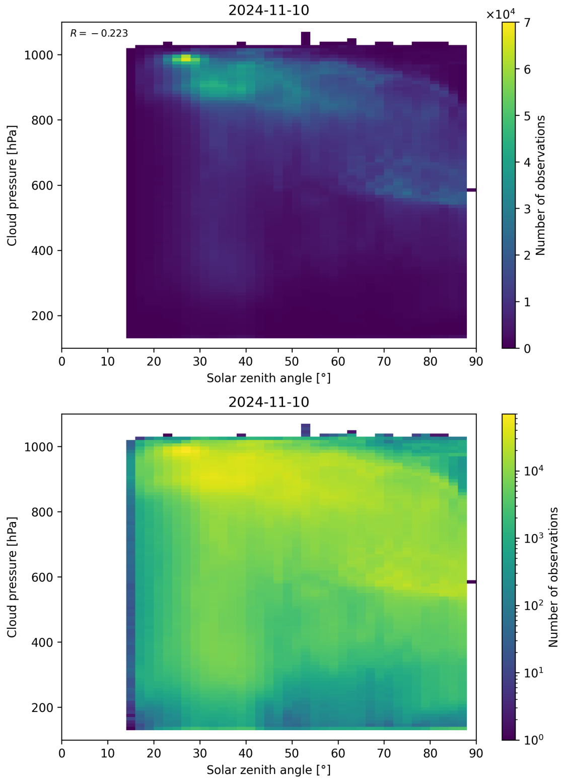
Figure 122: Scatter density plot of “Solar zenith angle” against “Cloud pressure” for 2024-11-09 to 2024-11-11.
