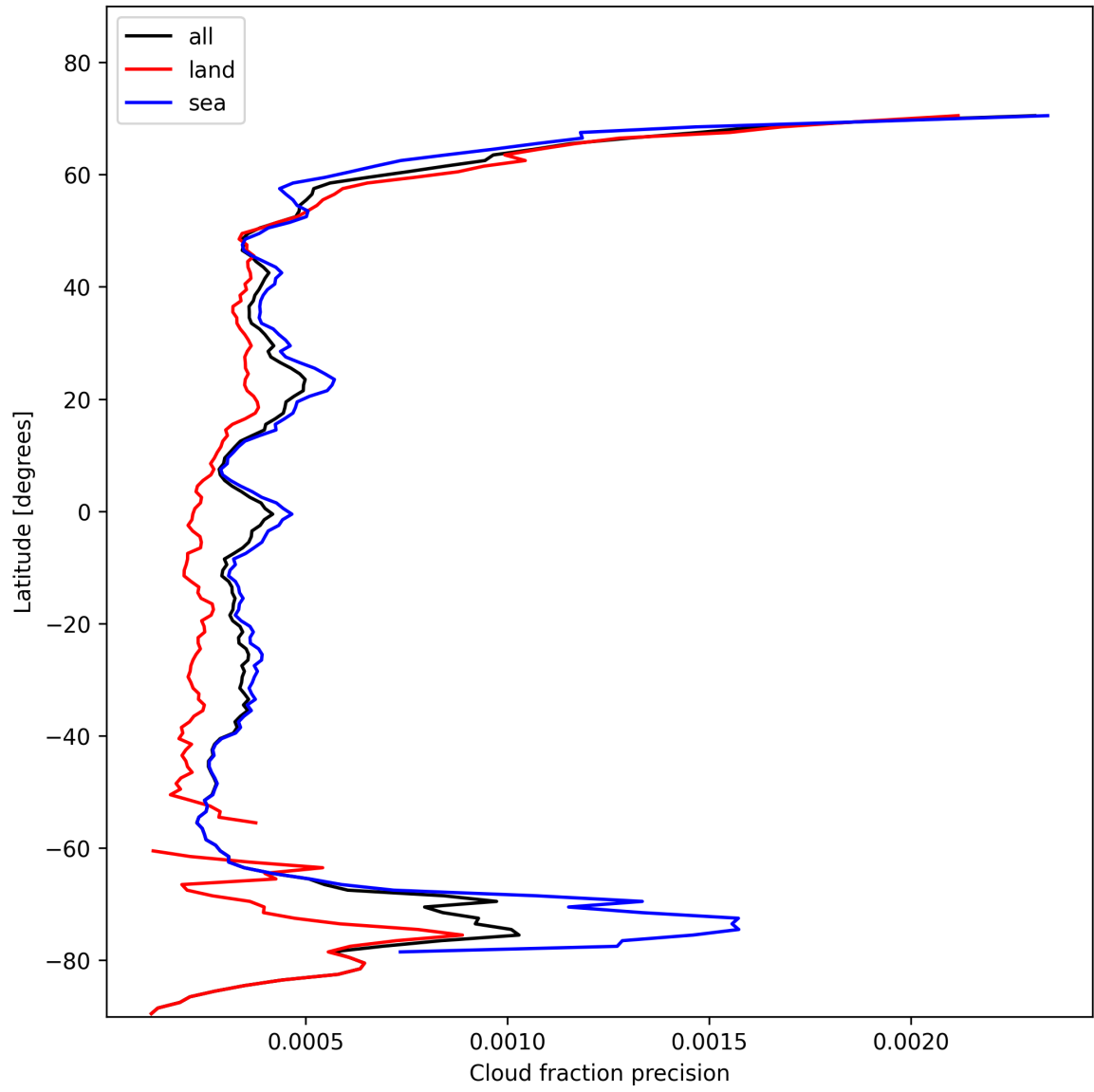
Figure 16: Zonal average of “Cloud fraction precision” for 2024-11-09 to 2024-11-11.
