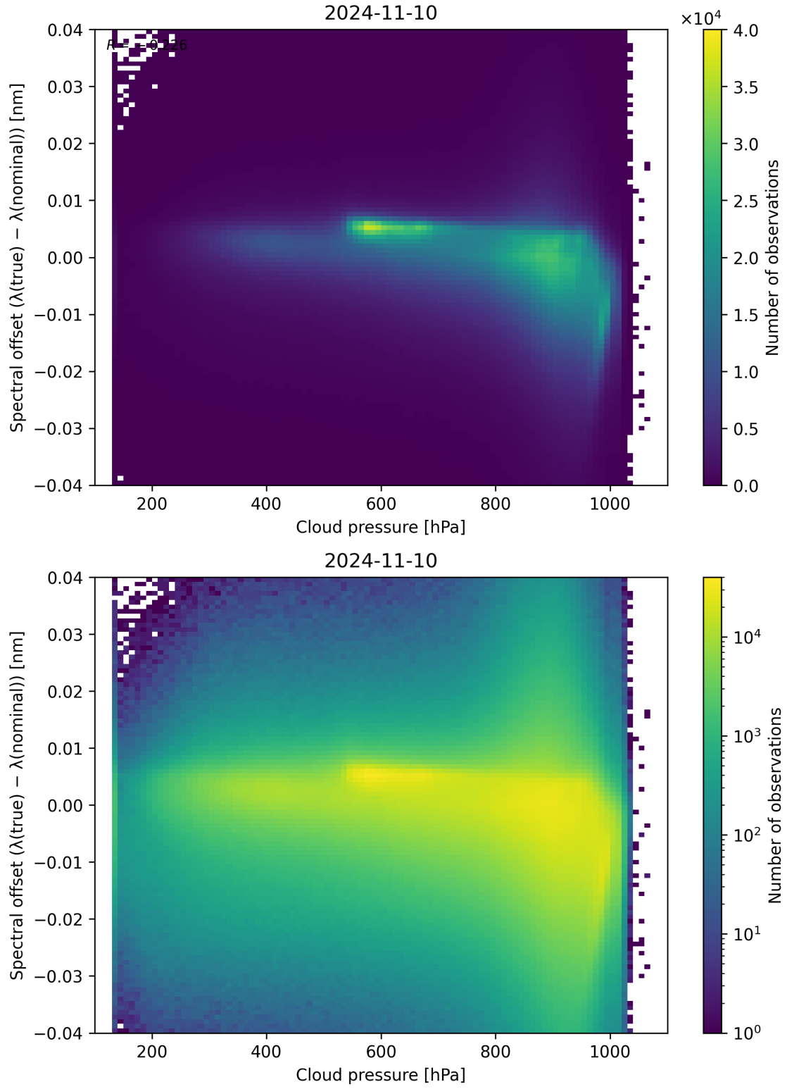
Figure 92: Scatter density plot of “Cloud pressure” against “Spectral offset ( \lambda_{\text{true}} - \lambda_{\text{nominal}} )” for 2024-11-09 to 2024-11-11.
