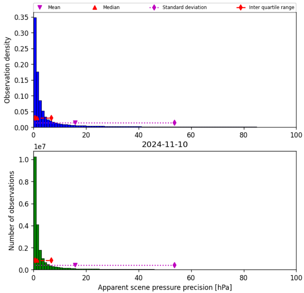
Figure 37: Histogram of “Apparent scene pressure precision” for 2024-11-09 to 2024-11-11
