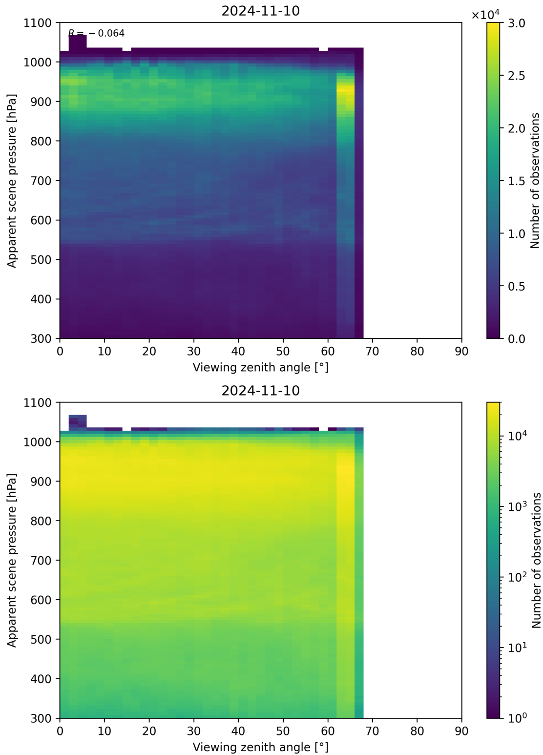
Figure 129: Scatter density plot of “Viewing zenith angle” against “Apparent scene pressure” for 2024-11-09 to 2024-11-11.
