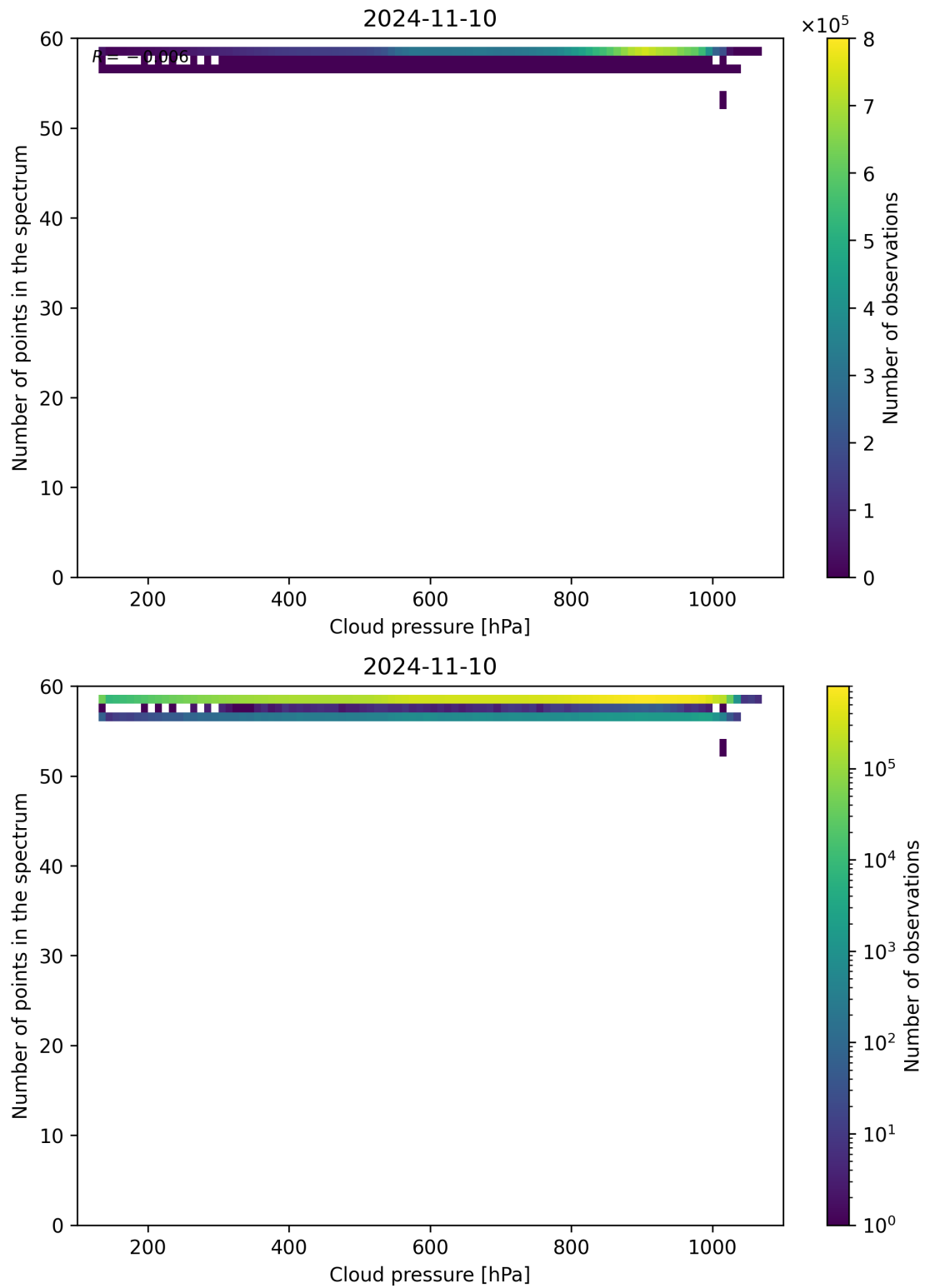
Figure 90: Scatter density plot of “Cloud pressure” against “Number of points in the spectrum” for 2024-11-09 to 2024-11-11.
