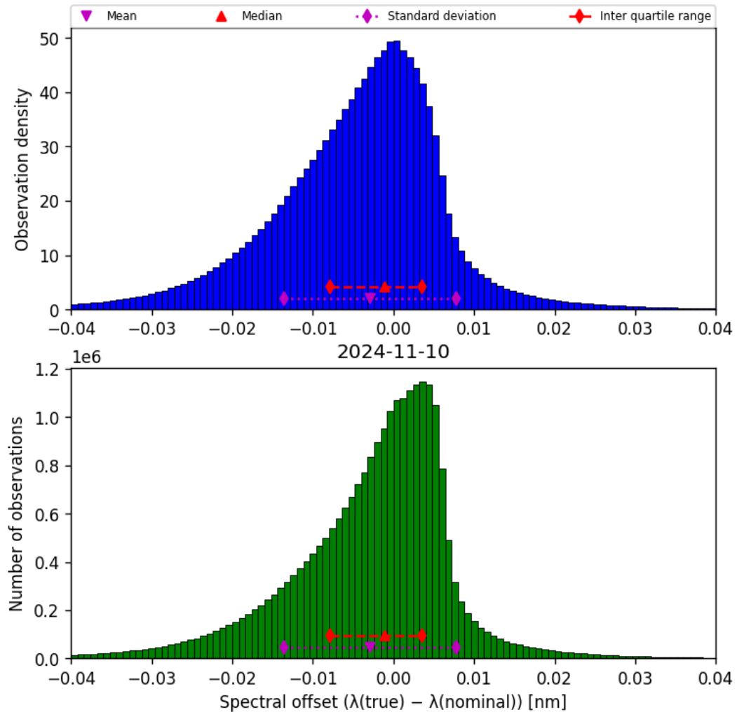
Figure 45: Histogram of “Spectral offset ( \lambda_{\text{true}} - \lambda_{\text{nominal}} )” for 2024-11-09 to 2024-11-11
