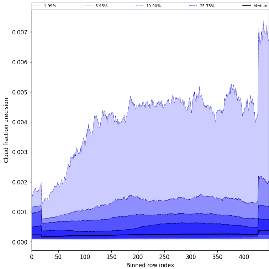
Figure 50: Along track statistics of “Cloud fraction precision” for 2024-11-09 to 2024-11-11
