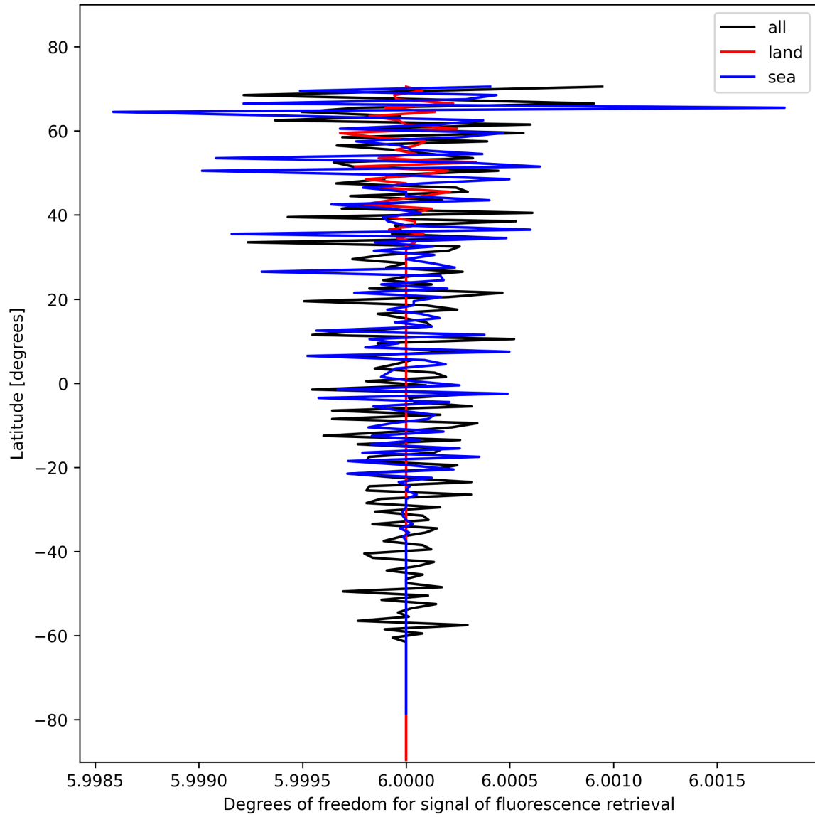
Figure 26: Zonal average of “Degrees of freedom for signal of fluorescence retrieval” for 2024-11-09 to 2024-11-11.
