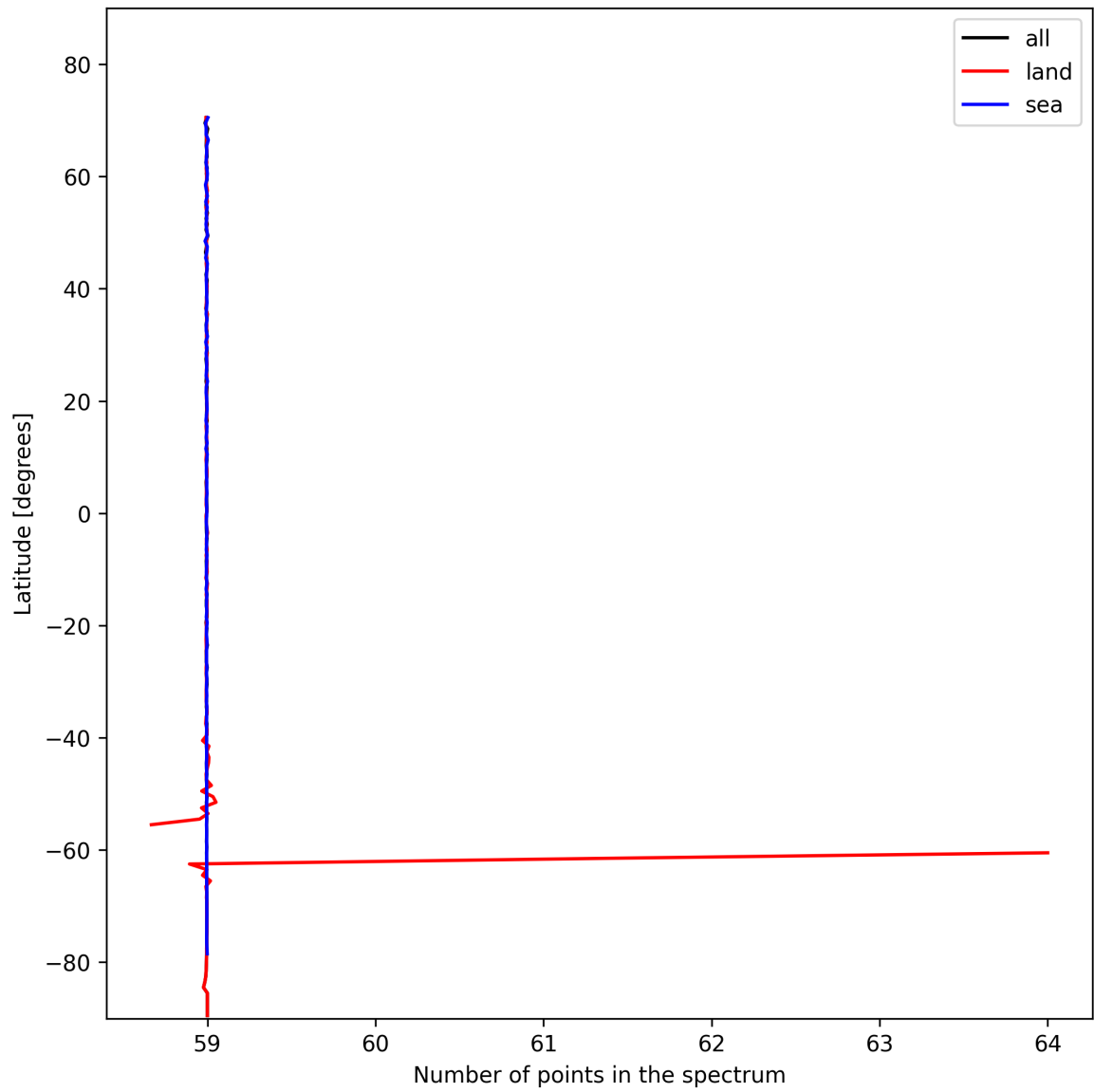
Figure 27: Zonal average of “Number of points in the spectrum” for 2024-11-09 to 2024-11-11.
