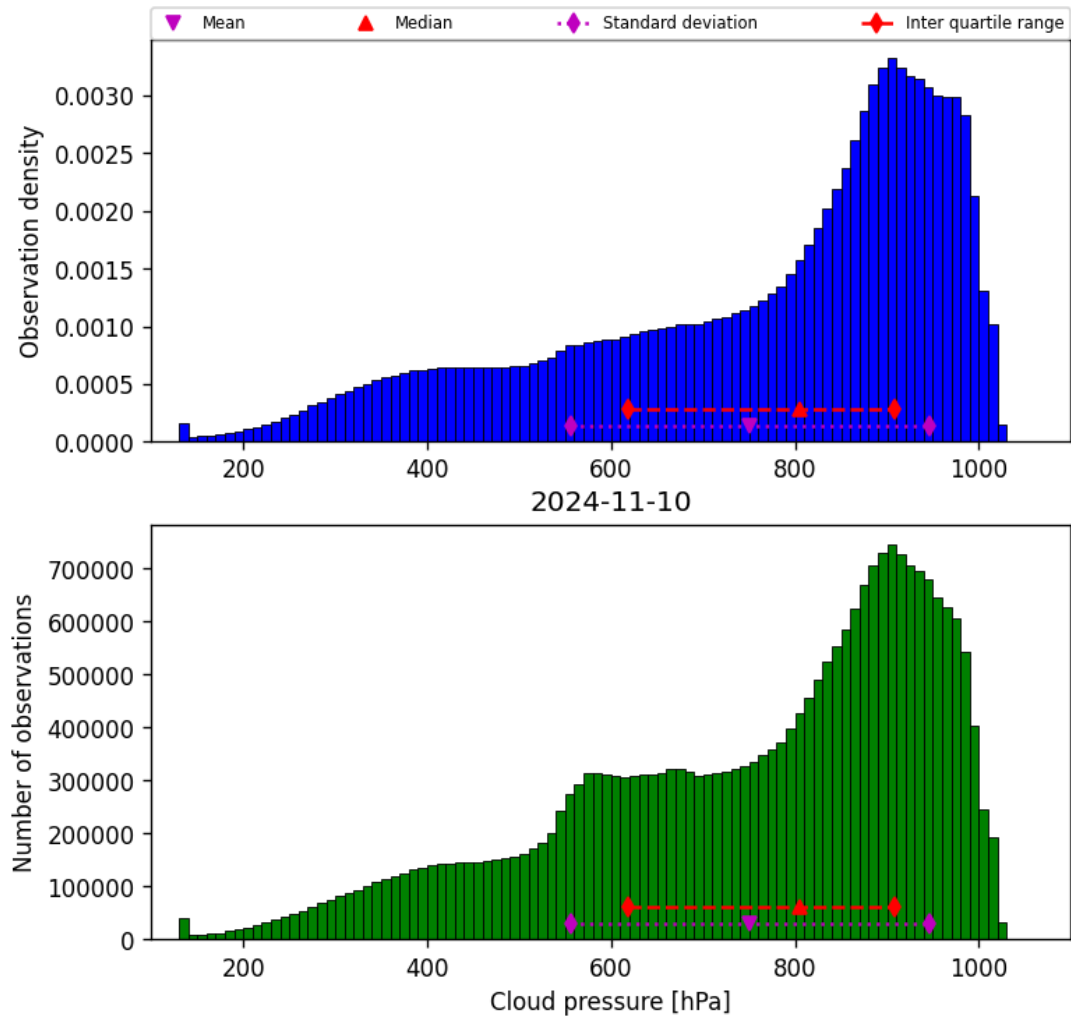
Figure 30: Histogram of “Cloud pressure” for 2024-11-09 to 2024-11-11
