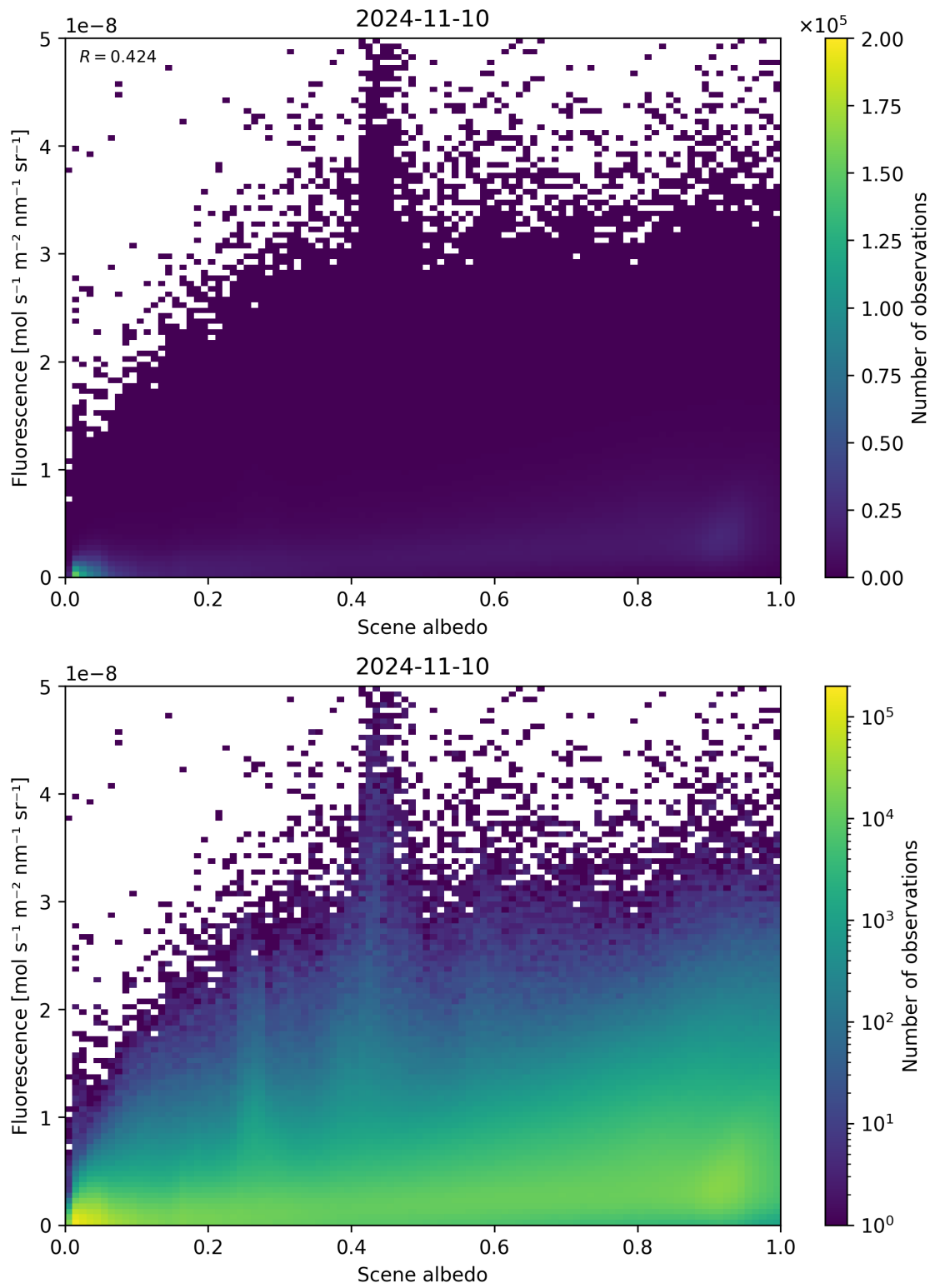
Figure 114: Scatter density plot of “Scene albedo” against “Fluorescence” for 2024-11-09 to 2024-11-11.
