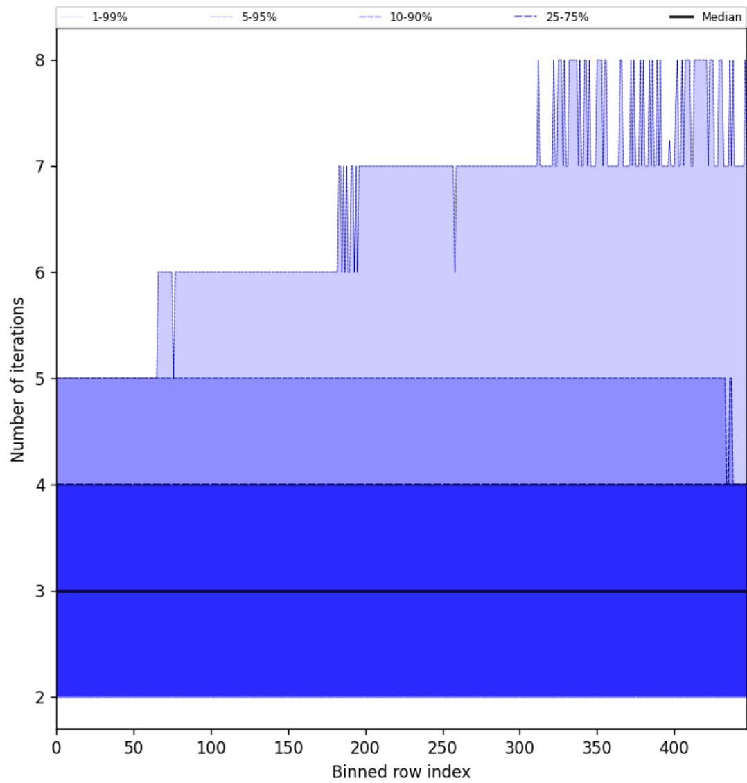
Figure 56: Along track statistics of “Number of iterations” for 2024-11-09 to 2024-11-11
