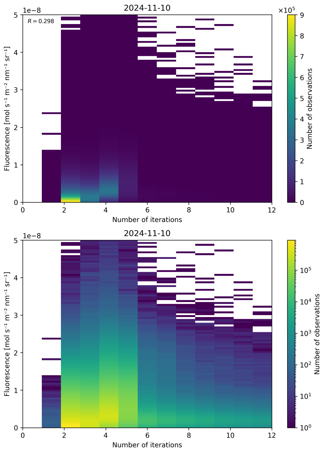
Figure 107: Scatter density plot of “Number of iterations” against “Fluorescence” for 2024-11-09 to 2024-11-11.
