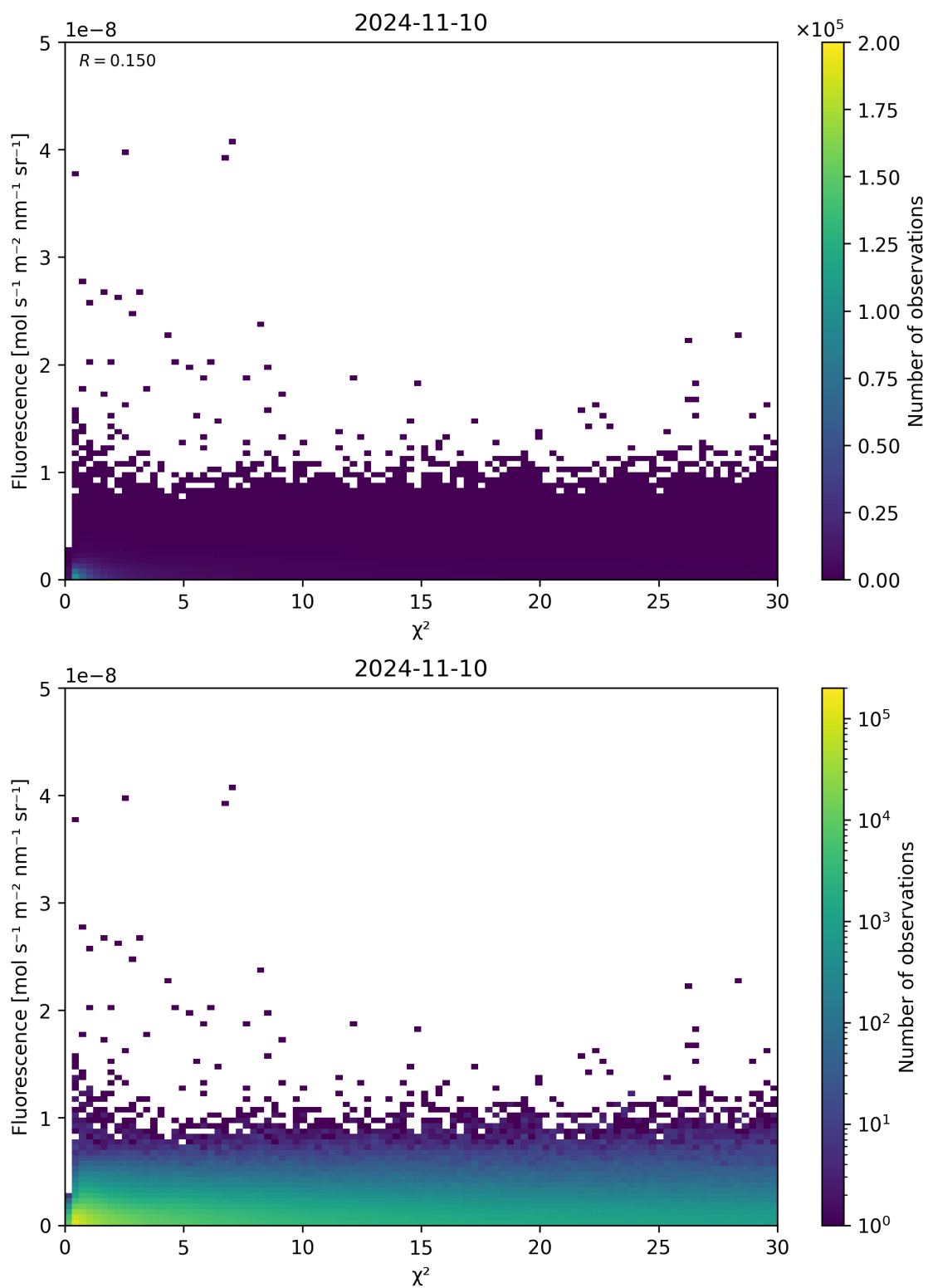
Figure 70: Scatter density plot of “ \chi^2 ” against “Fluorescence” for 2024-11-09 to 2024-11-11.
