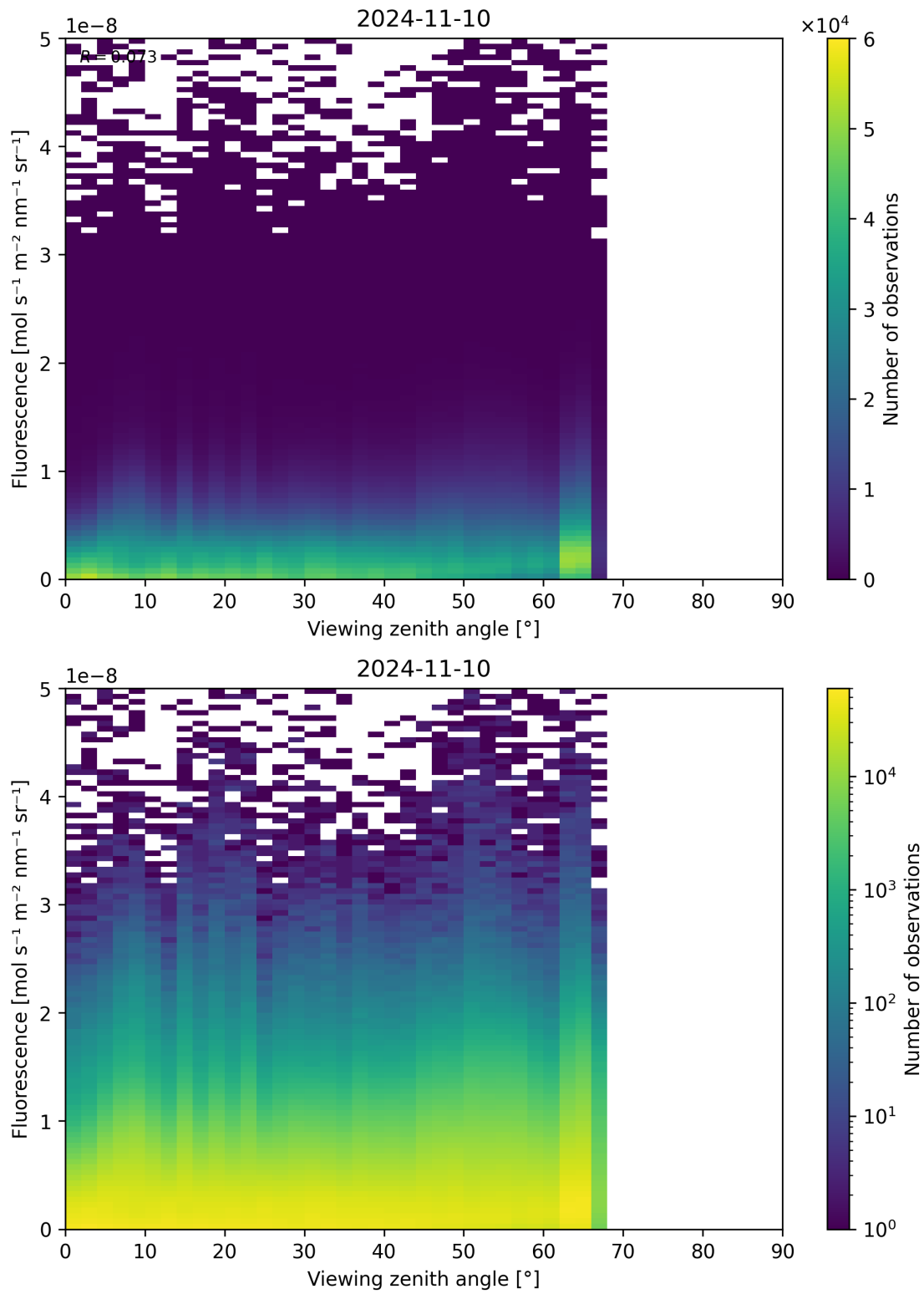
Figure 134: Scatter density plot of “Viewing zenith angle” against “Fluorescence” for 2024-11-09 to 2024-11-11.
