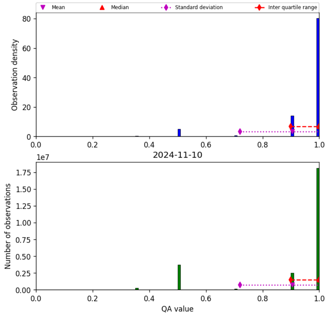
Figure 29: Histogram of “QA value” for 2024-11-09 to 2024-11-11
