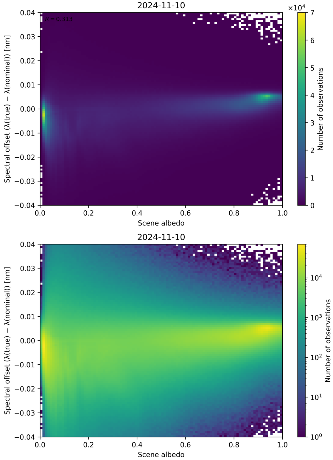
Figure 117: Scatter density plot of “Scene albedo” against “Spectral offset ( \lambda_{\text{true}} - \lambda_{\text{nominal}} )” for 2024-11-09 to 2024-11-11.
