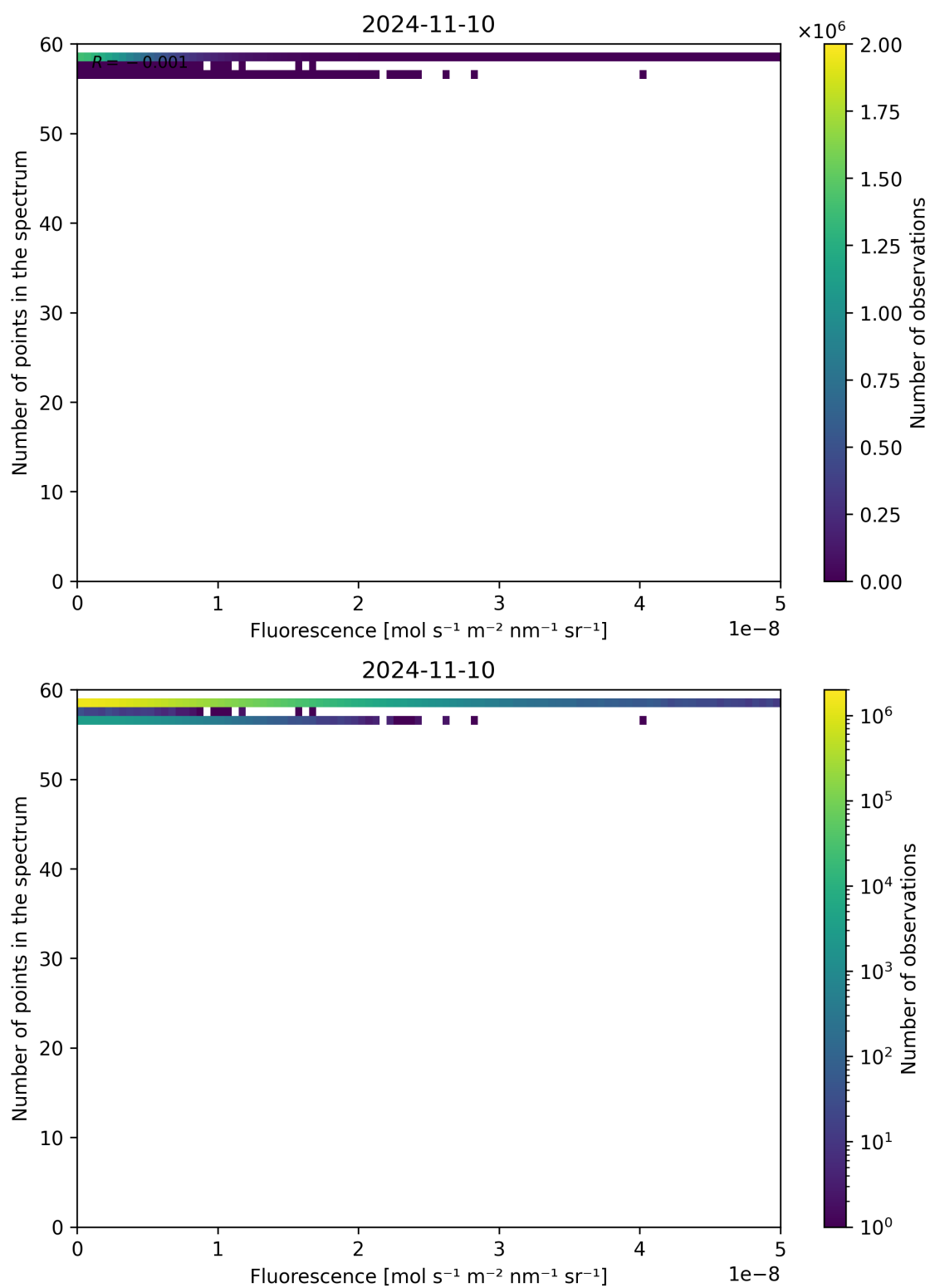
Figure 94: Scatter density plot of “Fluorescence” against “Number of points in the spectrum” for 2024-11-09 to 2024-11-11.
