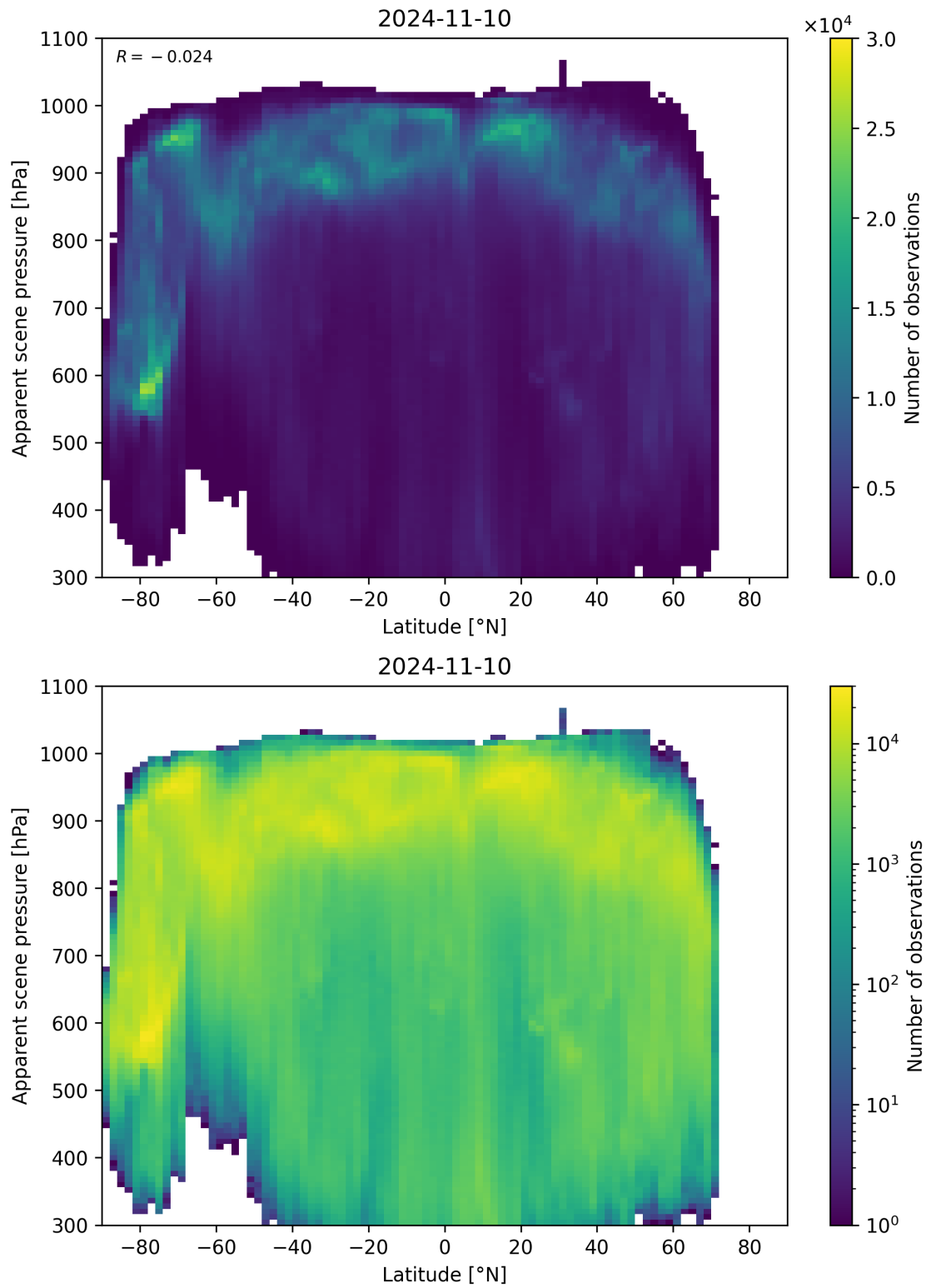
Figure 96: Scatter density plot of “Latitude” against “Apparent scene pressure” for 2024-11-09 to 2024-11-11.
