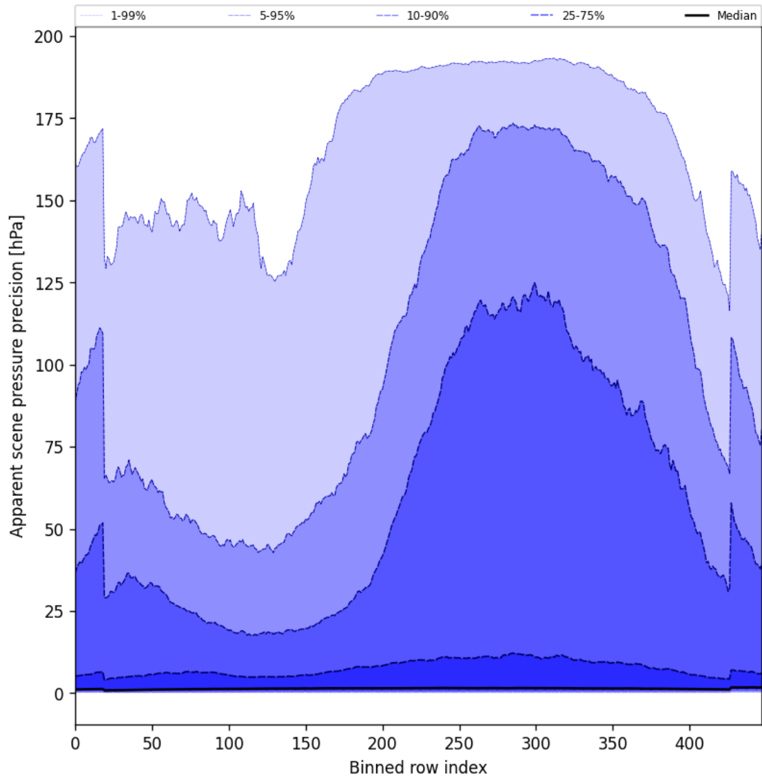
Figure 54: Along track statistics of “Apparent scene pressure precision” for 2024-11-09 to 2024-11-11
