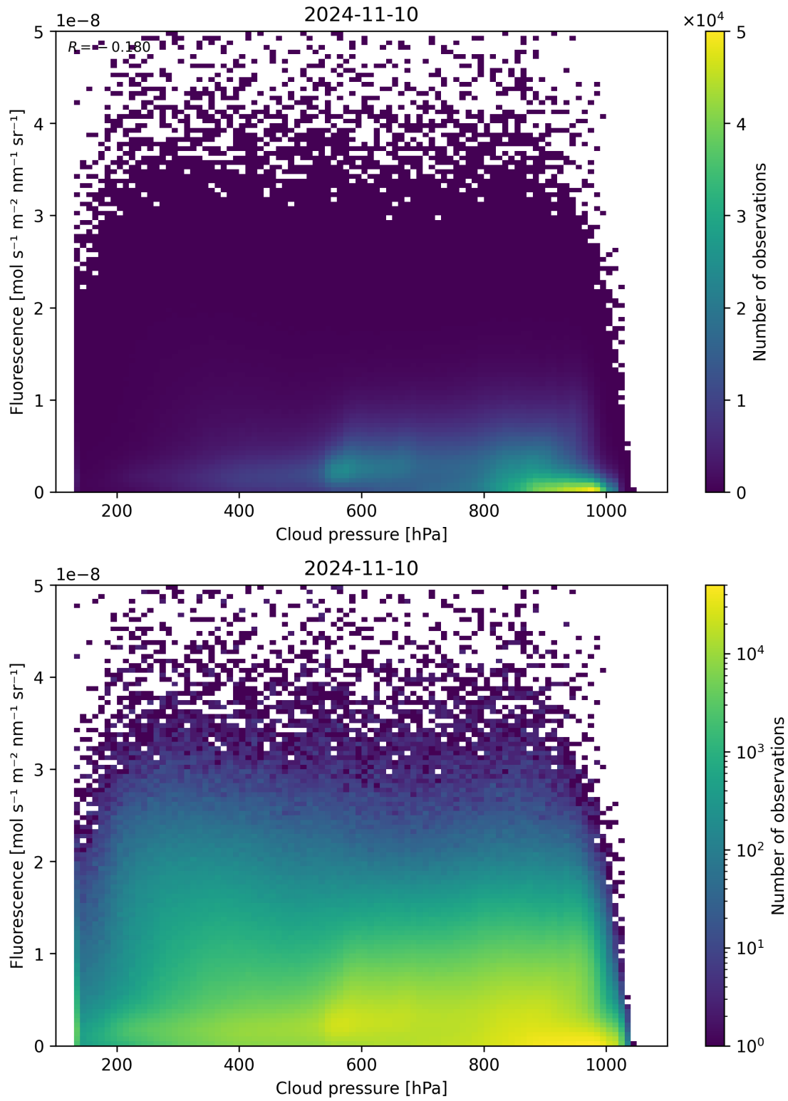
Figure 88: Scatter density plot of “Cloud pressure” against “Fluorescence” for 2024-11-09 to 2024-11-11.
