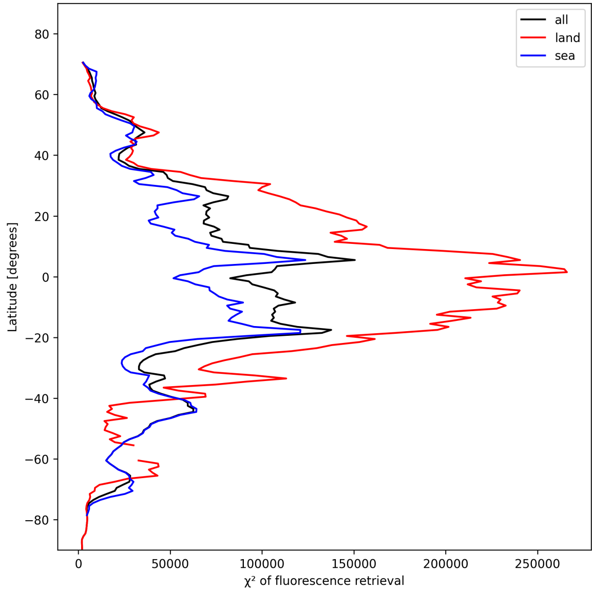
Figure 25: Zonal average of “ \chi^2 of fluorescence retrieval” for 2024-11-09 to 2024-11-11.
