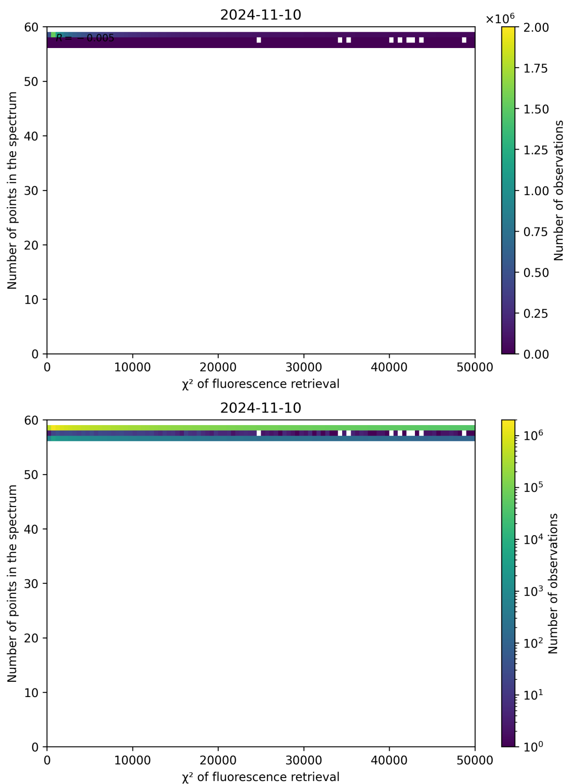
Figure 71: Scatter density plot of " \chi^2 of fluorescence retrieval" against "Number of points in the spectrum" for 2024-11-09 to 2024-11-11.
