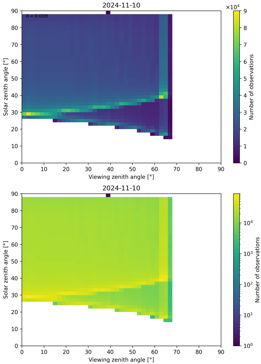
Figure 139: Scatter density plot of “Viewing zenith angle” against “Solar zenith angle” for 2024-11-09 to 2024-11-11.
