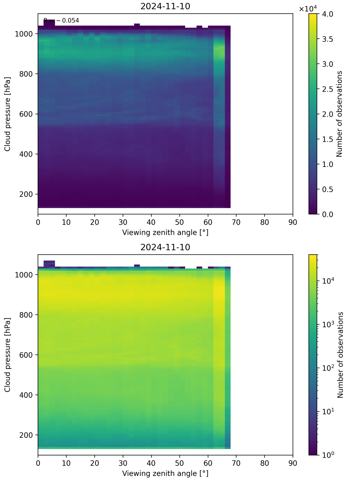
Figure 133: Scatter density plot of “Viewing zenith angle” against “Cloud pressure” for 2024-11-09 to 2024-11-11.
