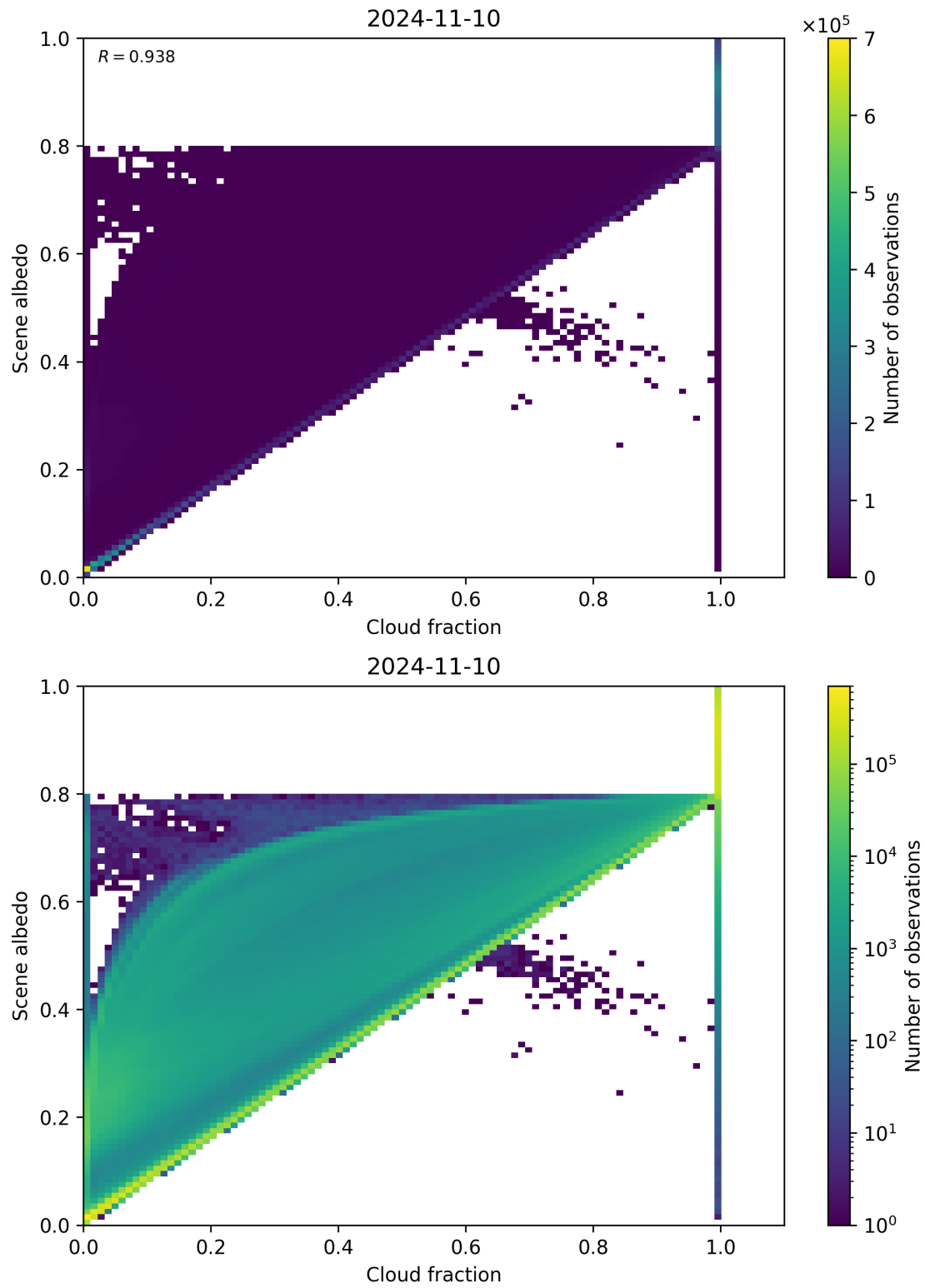
Figure 82: Scatter density plot of “Cloud fraction” against “Scene albedo” for 2024-11-09 to 2024-11-11.
