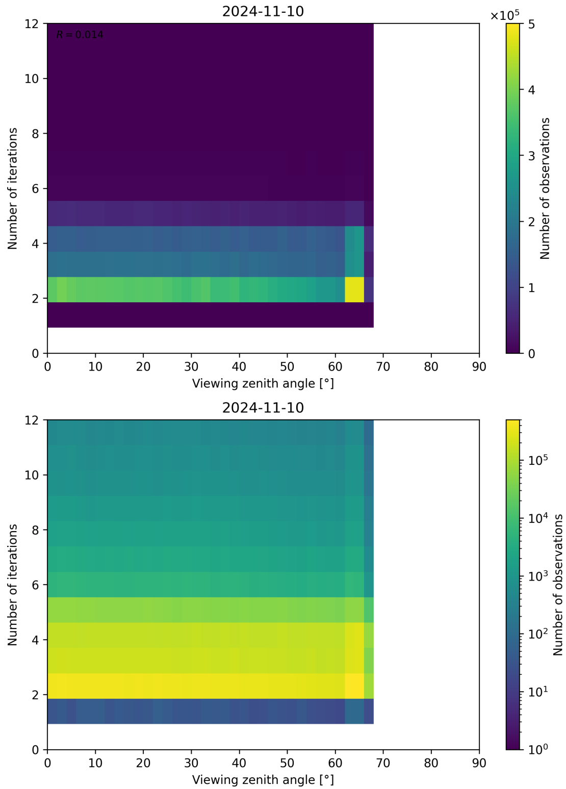
Figure 136: Scatter density plot of “Viewing zenith angle” against “Number of iterations” for 2024-11-09 to 2024-11-11.
