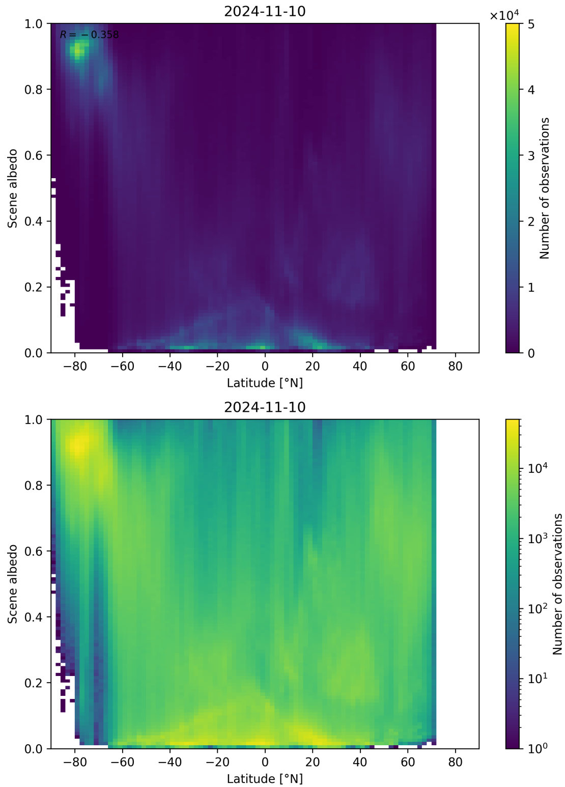
Figure 104: Scatter density plot of “Latitude” against “Scene albedo” for 2024-11-09 to 2024-11-11.
