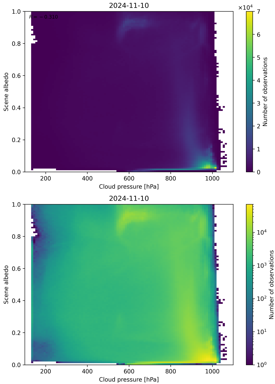
Figure 91: Scatter density plot of “Cloud pressure” against “Scene albedo” for 2024-11-09 to 2024-11-11.
