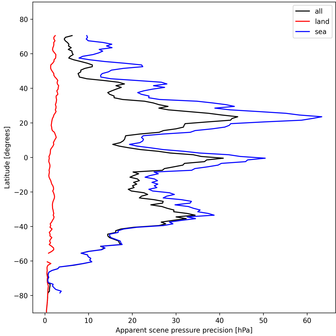
Figure 20: Zonal average of “Apparent scene pressure precision” for 2024-11-09 to 2024-11-11.
