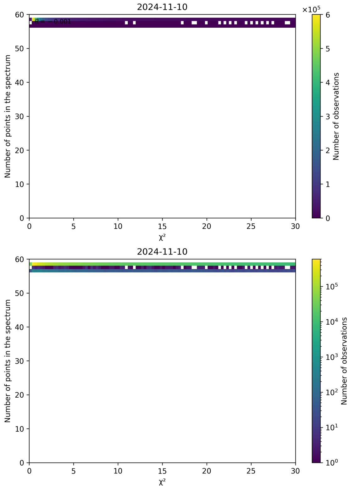
Figure 74: Scatter density plot of " \chi^2 " against "Number of points in the spectrum" for 2024-11-09 to 2024-11-11.
