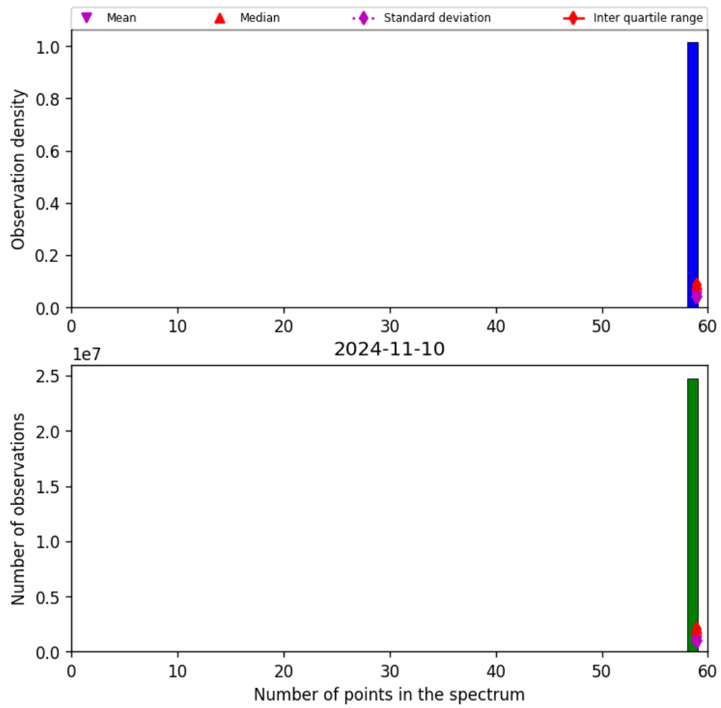
Figure 44: Histogram of “Number of points in the spectrum” for 2024-11-09 to 2024-11-11
