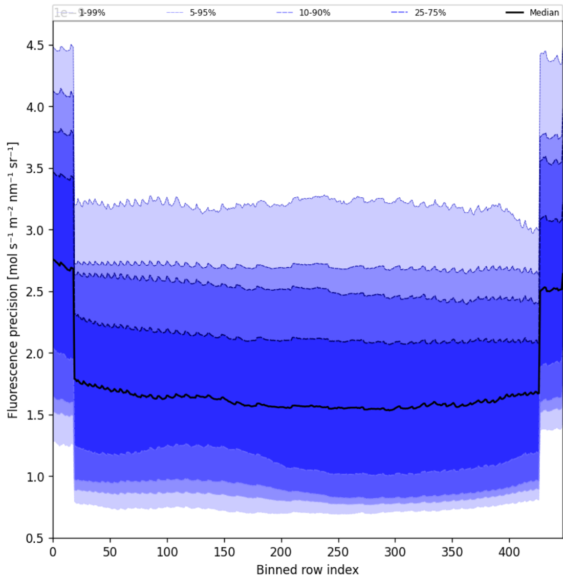
Figure 58: Along track statistics of “Fluorescence precision” for 2024-11-09 to 2024-11-11
