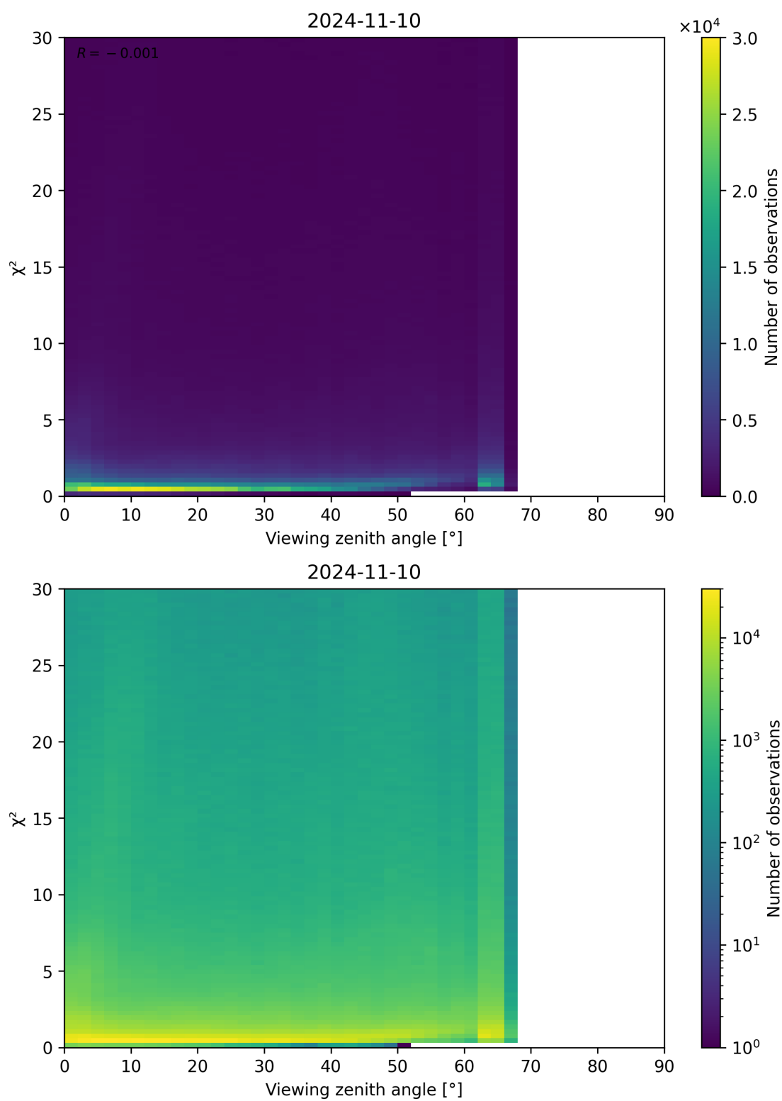
Figure 130: Scatter density plot of “Viewing zenith angle” against “ \chi^2 ” for 2024-11-09 to 2024-11-11.
