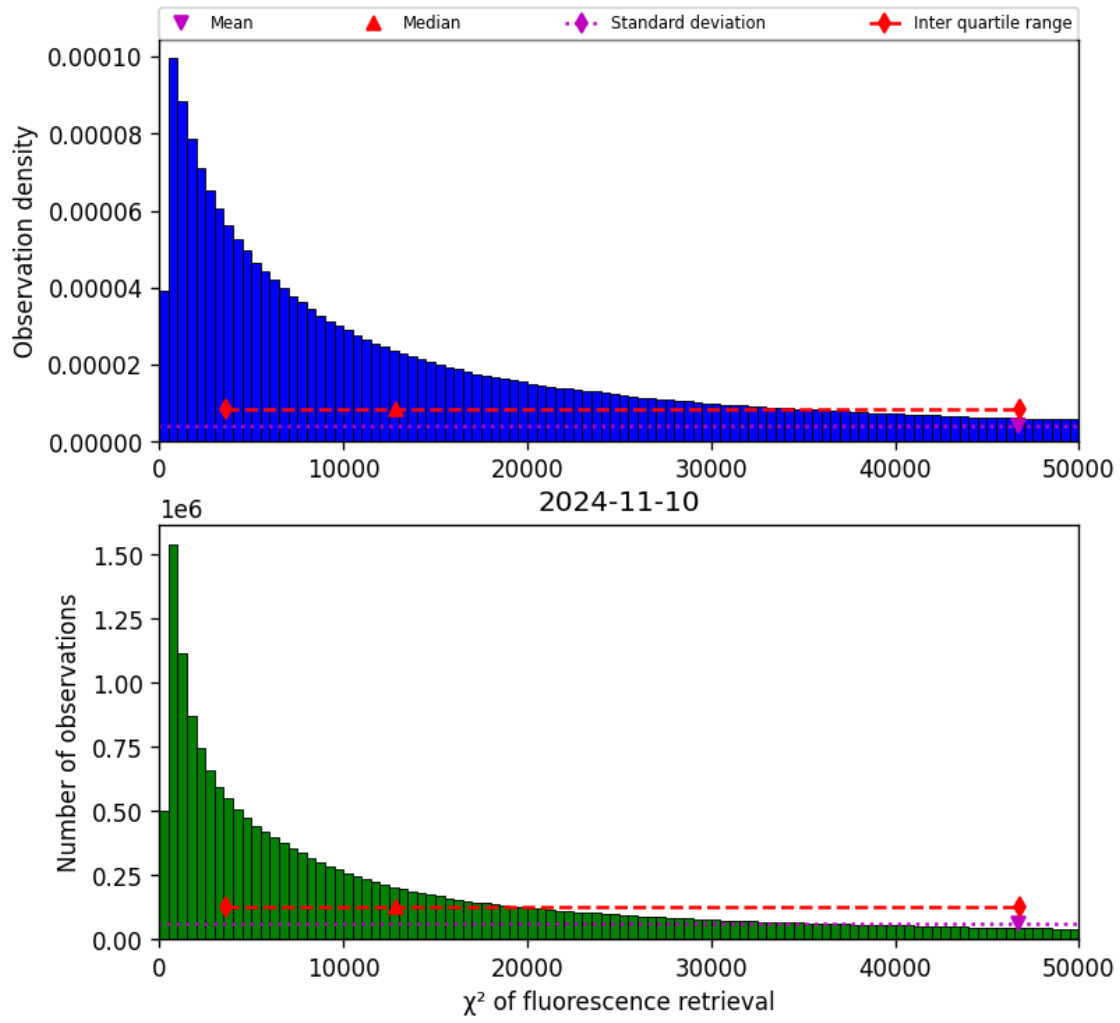
Figure 42: Histogram of “ \chi^2 of fluorescence retrieval” for 2024-11-09 to 2024-11-11
