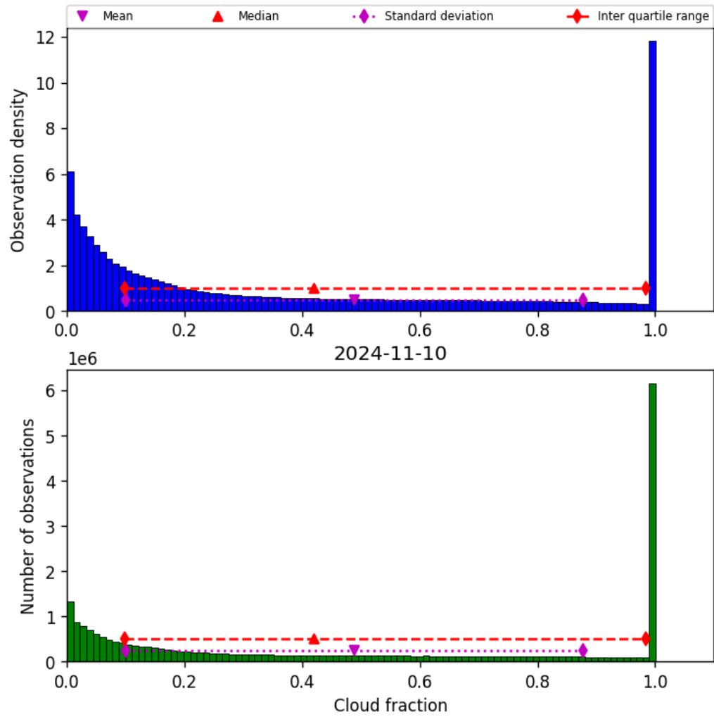
Figure 32: Histogram of “Cloud fraction” for 2024-11-09 to 2024-11-11
