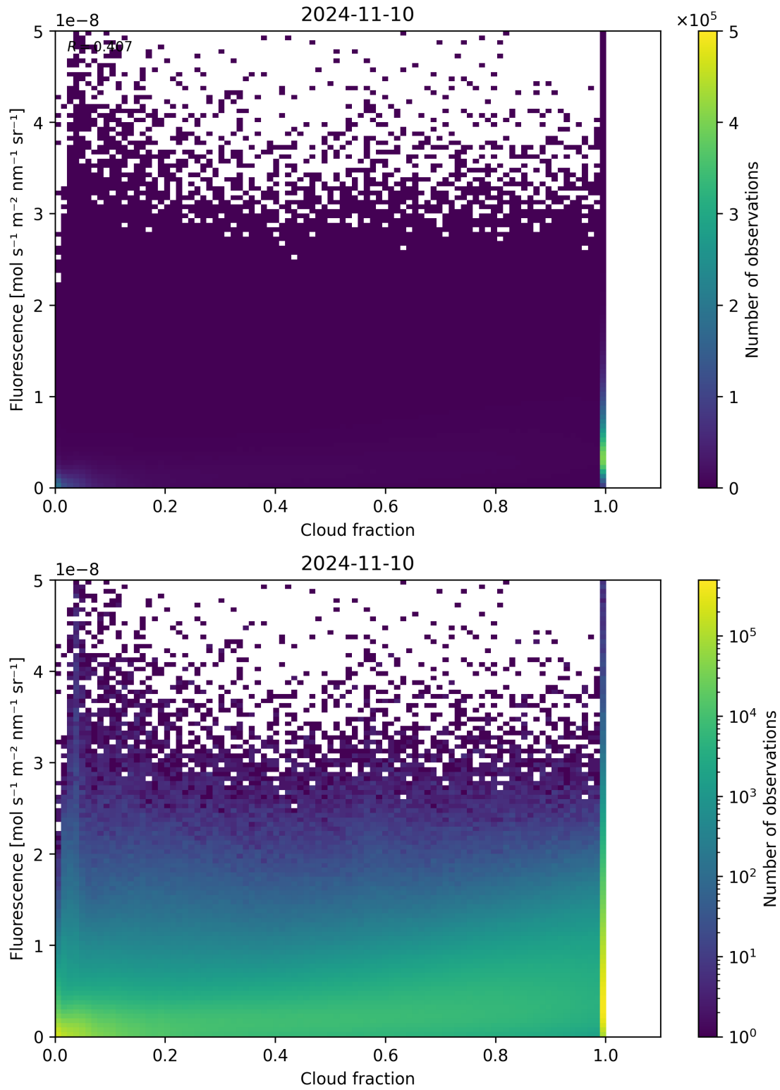
Figure 79: Scatter density plot of “Cloud fraction” against “Fluorescence” for 2024-11-09 to 2024-11-11.
