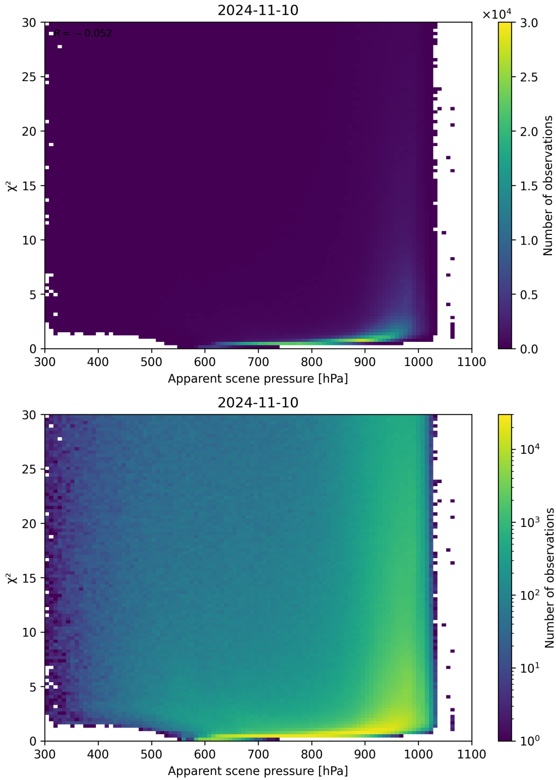
Figure 63: Scatter density plot of “Apparent scene pressure” against “ \chi^2 ” for 2024-11-09 to 2024-11-11.
