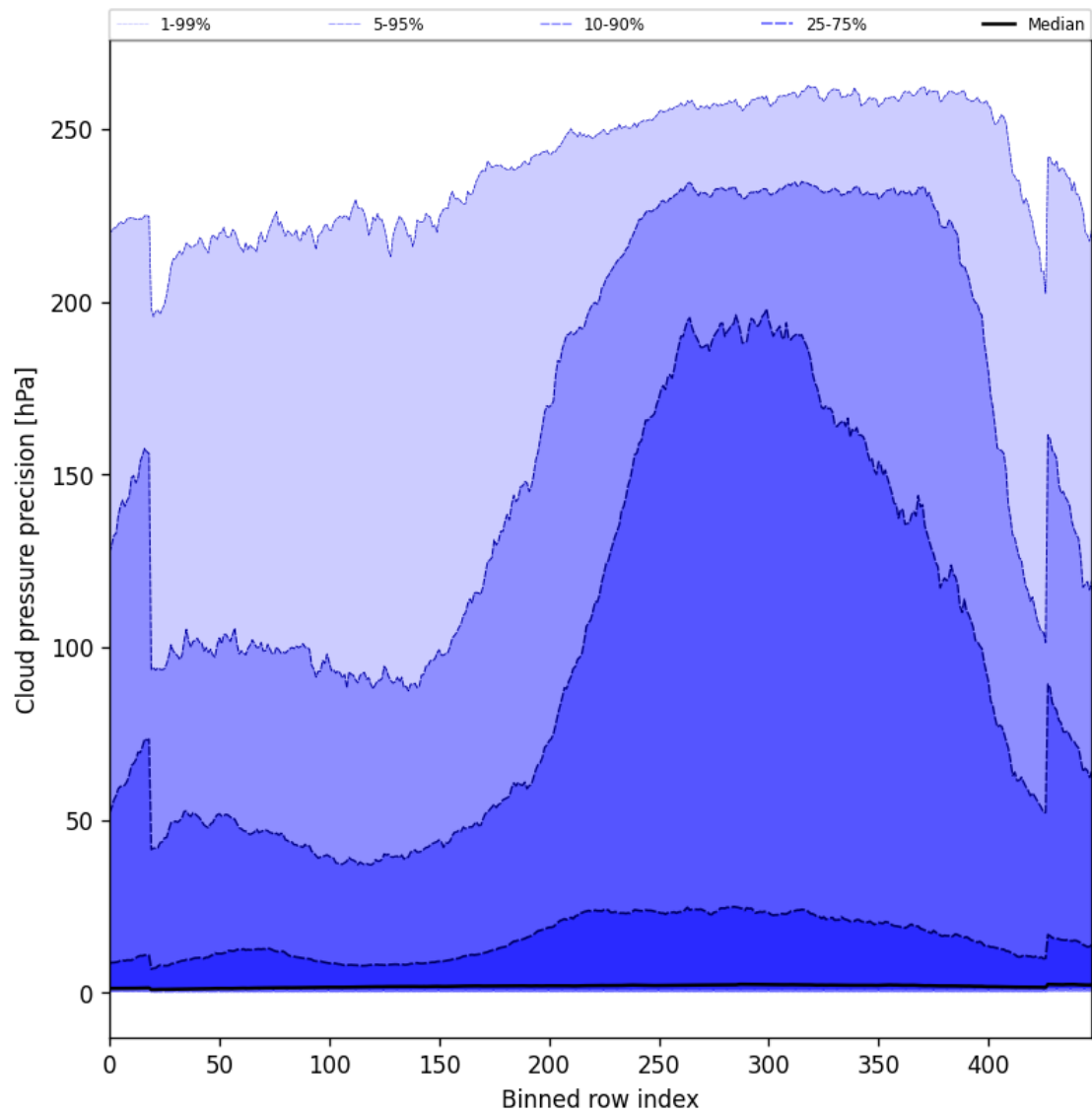
Figure 48: Along track statistics of “Cloud pressure precision” for 2024-11-09 to 2024-11-11
