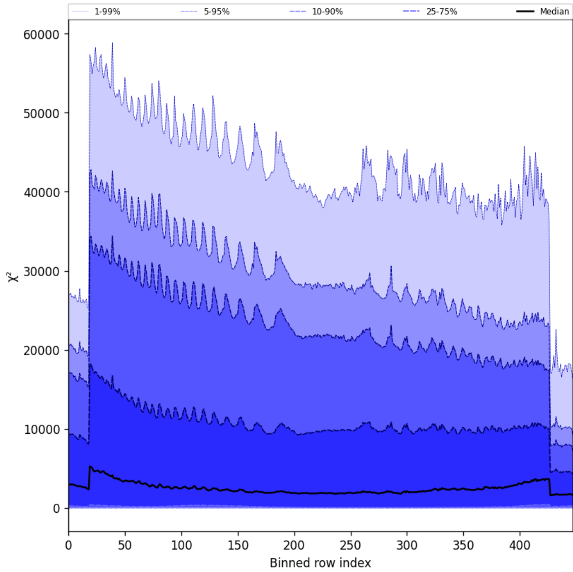
Figure 55: Along track statistics of “ \chi^2 ” for 2024-11-09 to 2024-11-11
