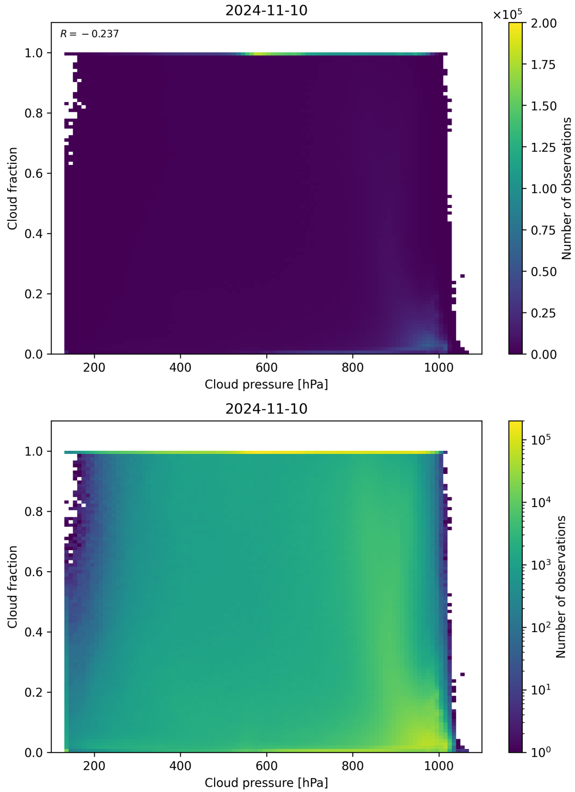
Figure 87: Scatter density plot of “Cloud pressure” against “Cloud fraction” for 2024-11-09 to 2024-11-11.
