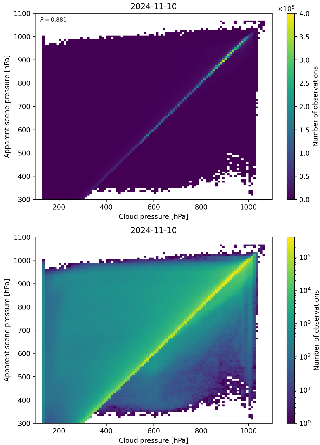
Figure 84: Scatter density plot of “Cloud pressure” against “Apparent scene pressure” for 2024-11-09 to 2024-11-11.
