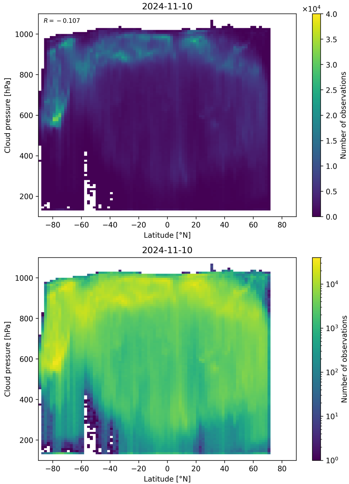
Figure 100: Scatter density plot of “Latitude” against “Cloud pressure” for 2024-11-09 to 2024-11-11.
