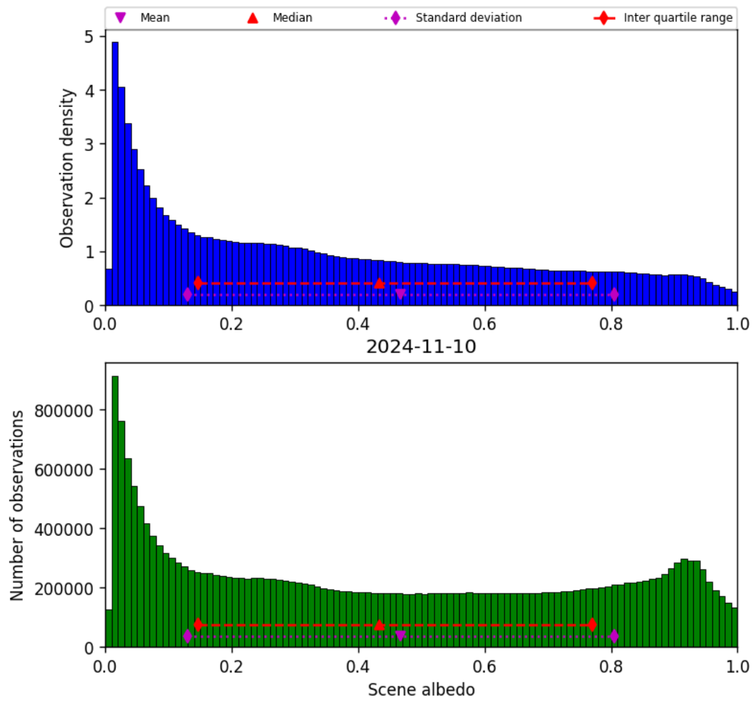
Figure 34: Histogram of “Scene albedo” for 2024-11-09 to 2024-11-11
