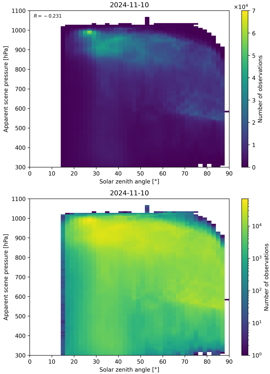
Figure 118: Scatter density plot of “Solar zenith angle” against “Apparent scene pressure” for 2024-11-09 to 2024-11-11.
