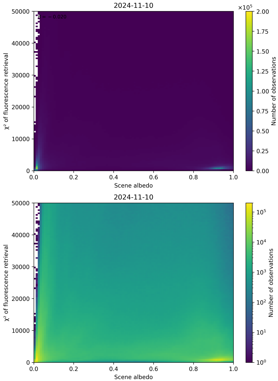
Figure 113: Scatter density plot of “Scene albedo” against “ \chi^2 of fluorescence retrieval” for 2024-11-09 to 2024-11-11.
