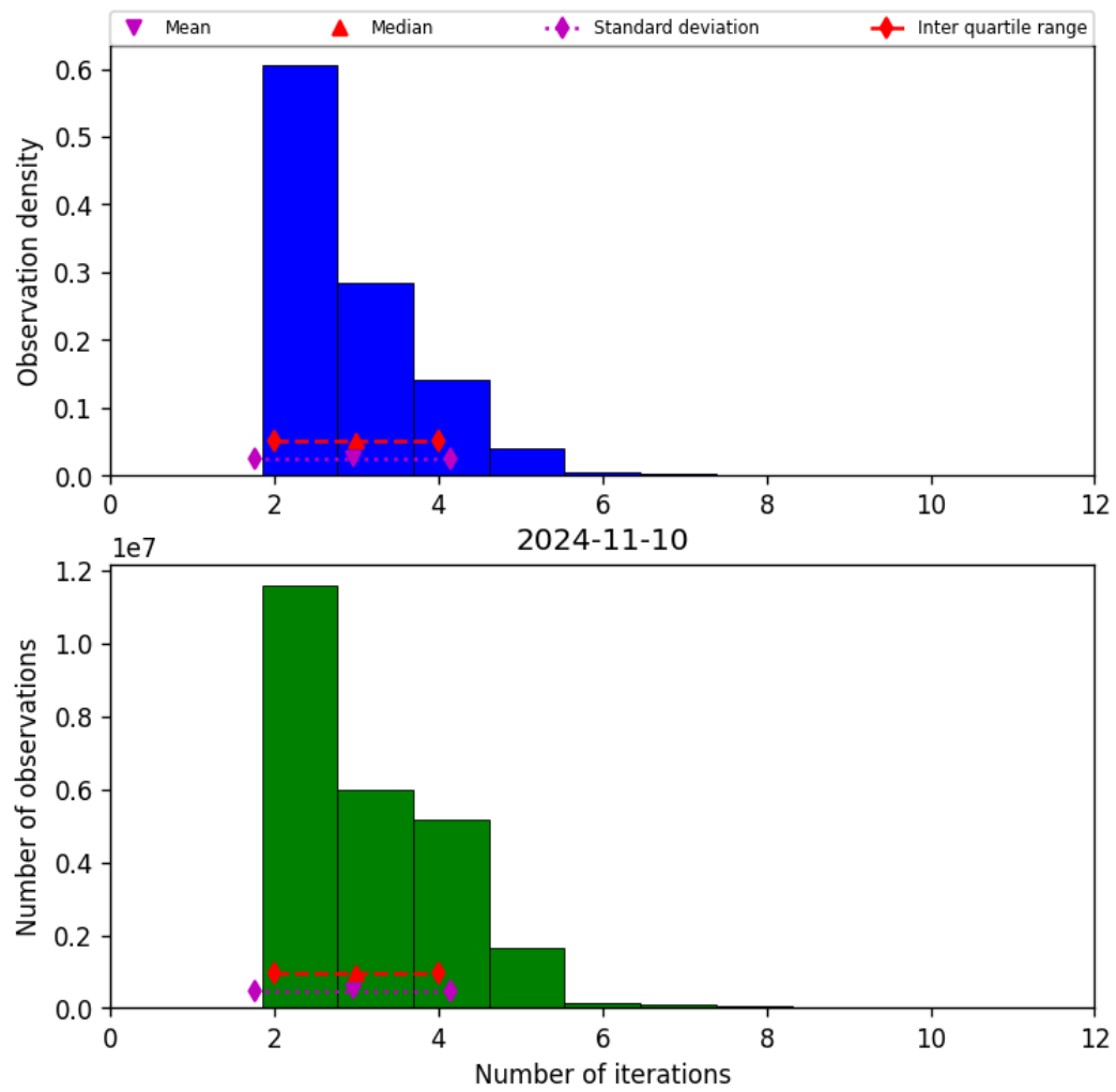
Figure 39: Histogram of “Number of iterations” for 2024-11-09 to 2024-11-11
