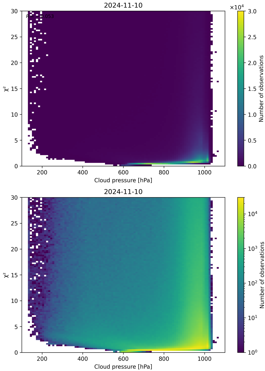
Figure 85: Scatter density plot of “Cloud pressure” against “ \chi^2 ” for 2024-11-09 to 2024-11-11.
