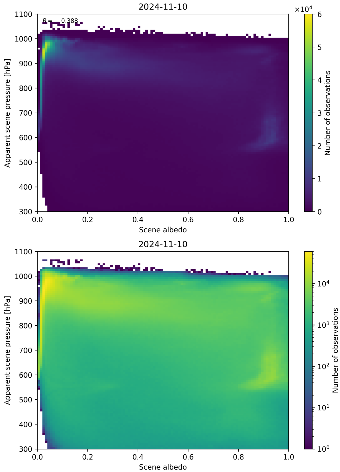
Figure 111: Scatter density plot of “Scene albedo” against “Apparent scene pressure” for 2024-11-09 to 2024-11-11.
