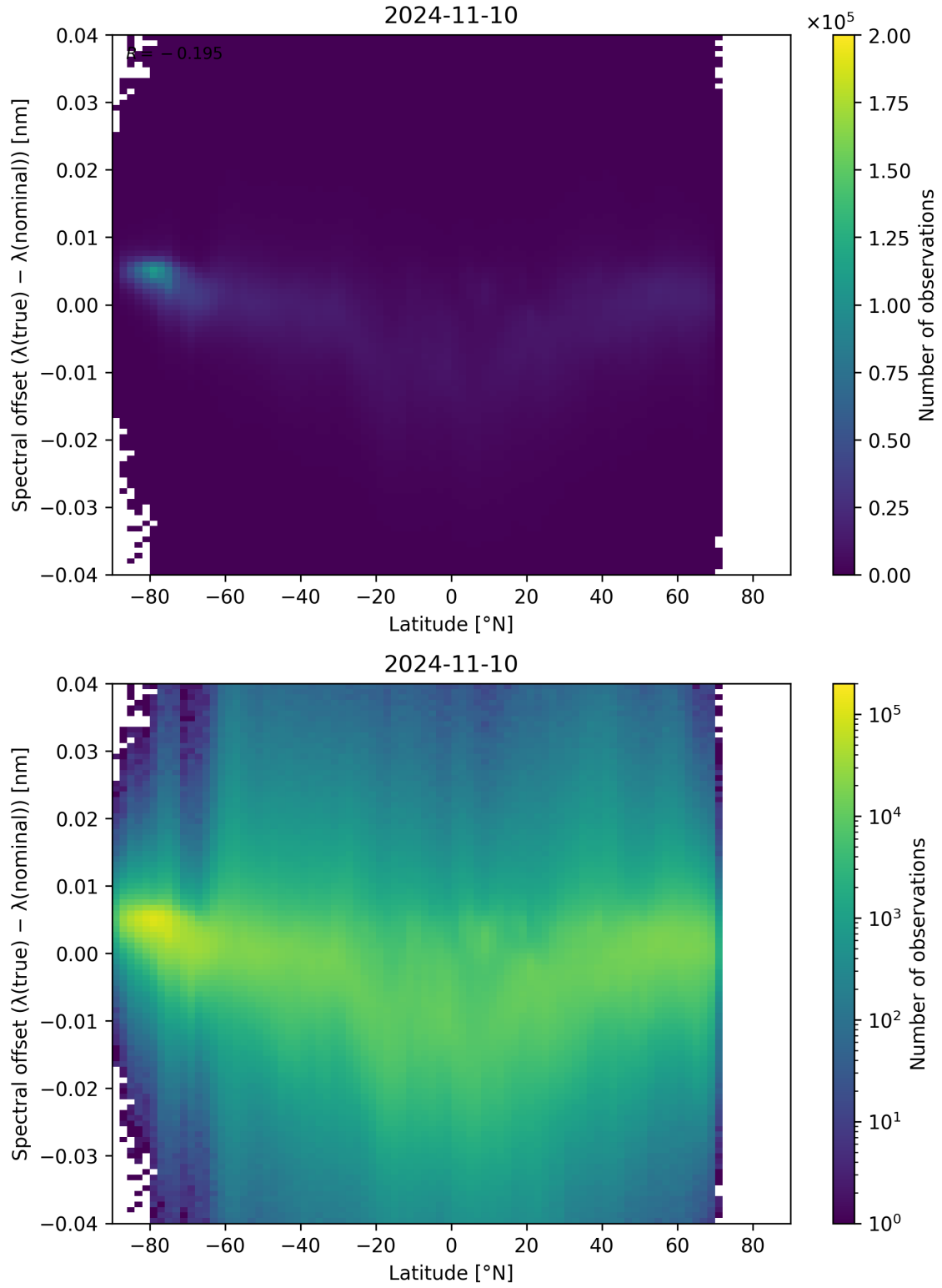
Figure 105: Scatter density plot of “Latitude” against “Spectral offset ( \lambda_{\text{true}} - \lambda_{\text{nominal}} )” for 2024-11-09 to 2024-11-11.
