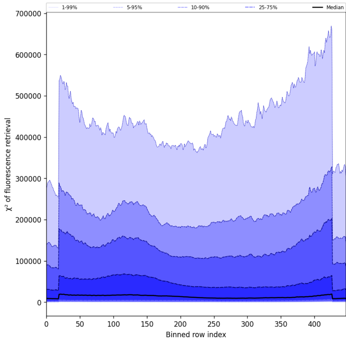
Figure 59: Along track statistics of “ \chi^2 of fluorescence retrieval” for 2024-11-09 to 2024-11-11
