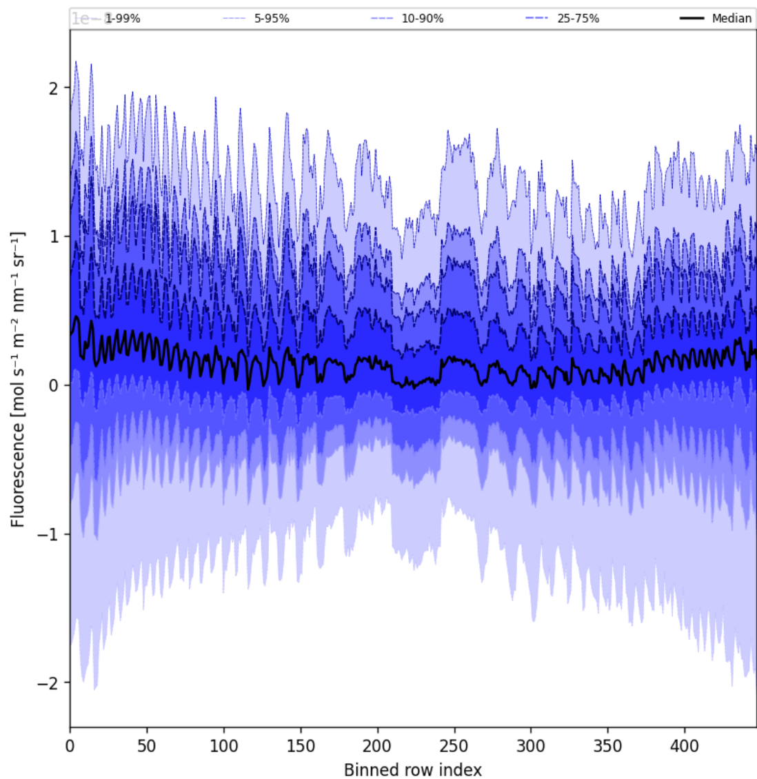
Figure 57: Along track statistics of "Fluorescence" for 2024-11-09 to 2024-11-11
