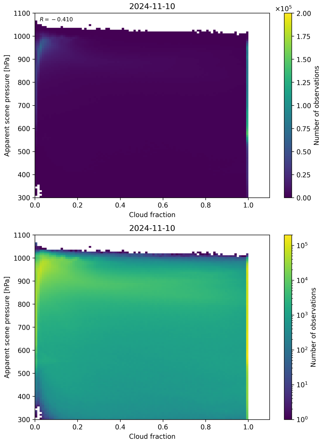
Figure 76: Scatter density plot of “Cloud fraction” against “Apparent scene pressure” for 2024-11-09 to 2024-11-11.
