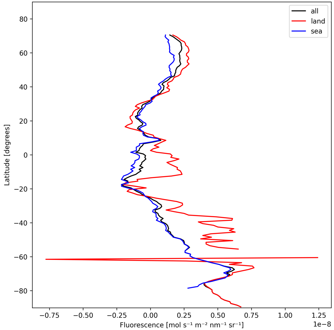
Figure 23: Zonal average of “Fluorescence” for 2024-11-09 to 2024-11-11.
