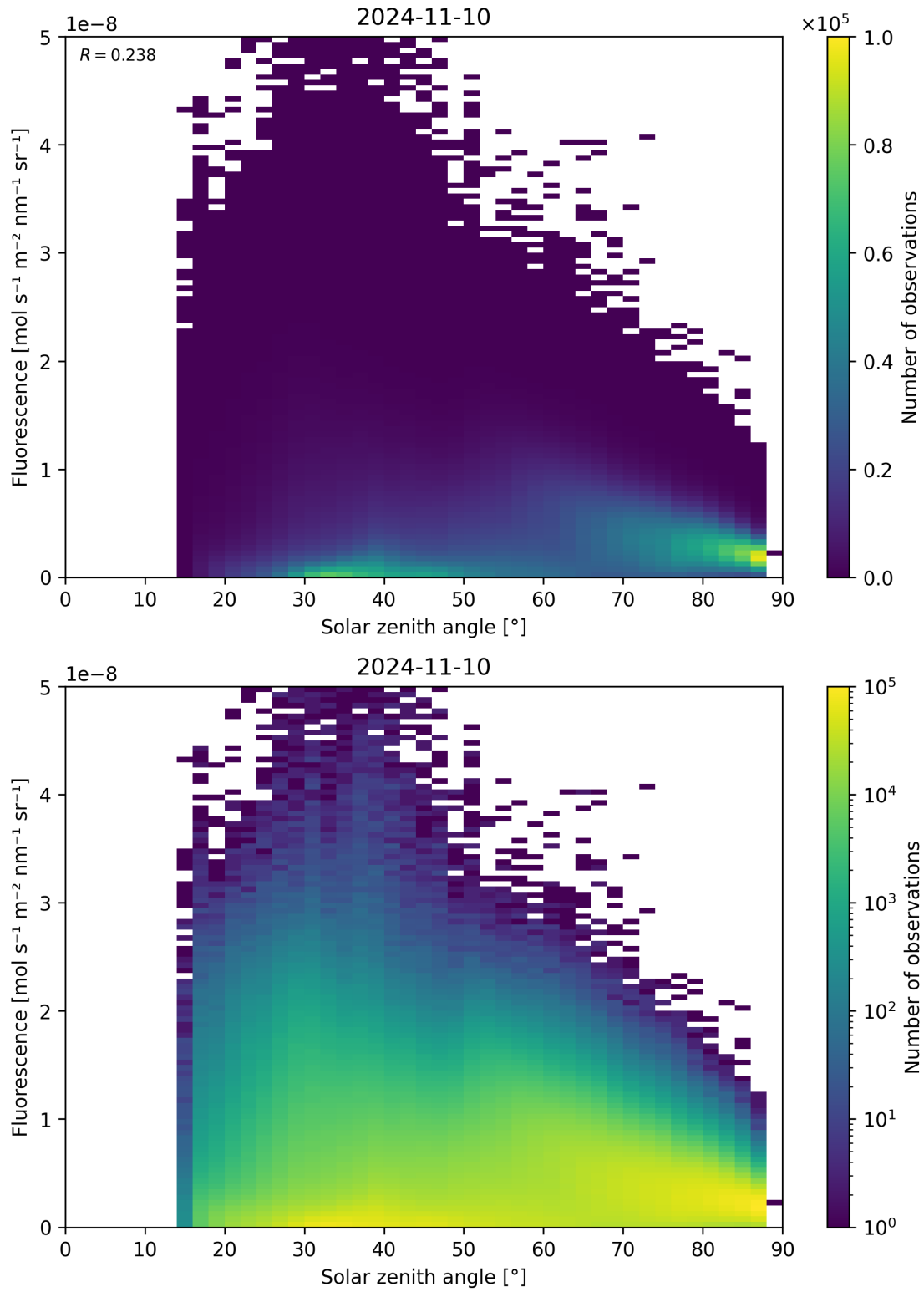
Figure 123: Scatter density plot of “Solar zenith angle” against “Fluorescence” for 2024-11-09 to 2024-11-11.
