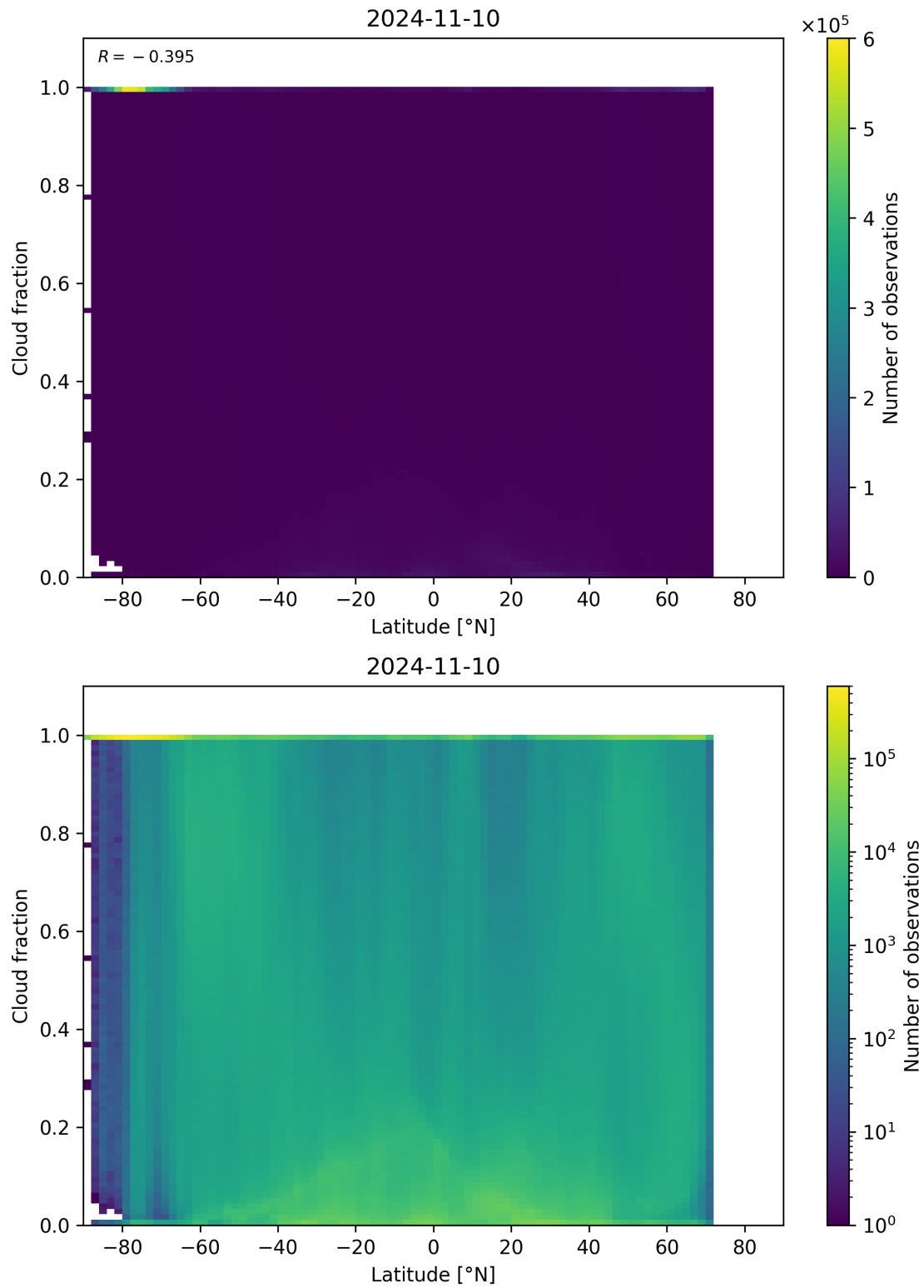
Figure 99: Scatter density plot of “Latitude” against “Cloud fraction” for 2024-11-09 to 2024-11-11.
