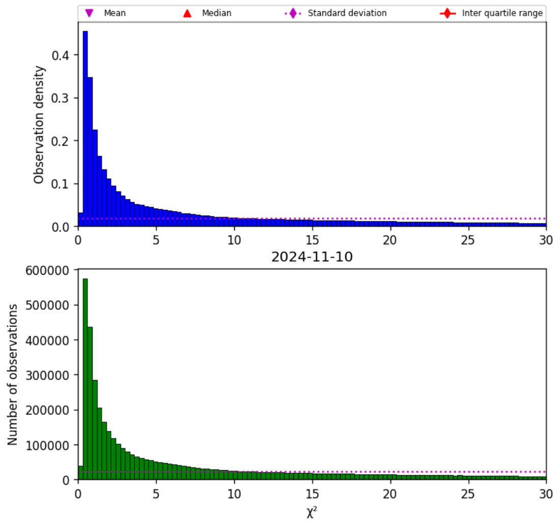
Figure 38: Histogram of “ \chi^2 ” for 2024-11-09 to 2024-11-11
