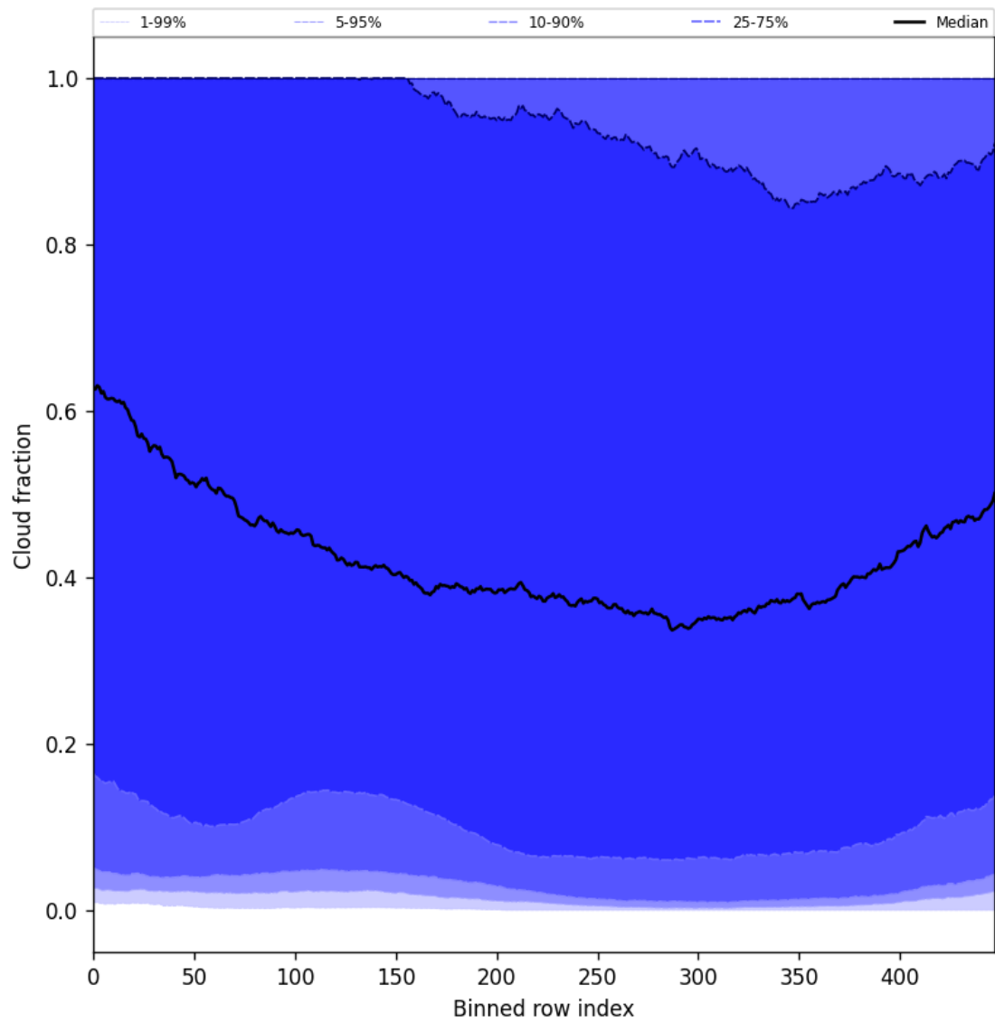
Figure 49: Along track statistics of “Cloud fraction” for 2024-11-09 to 2024-11-11
