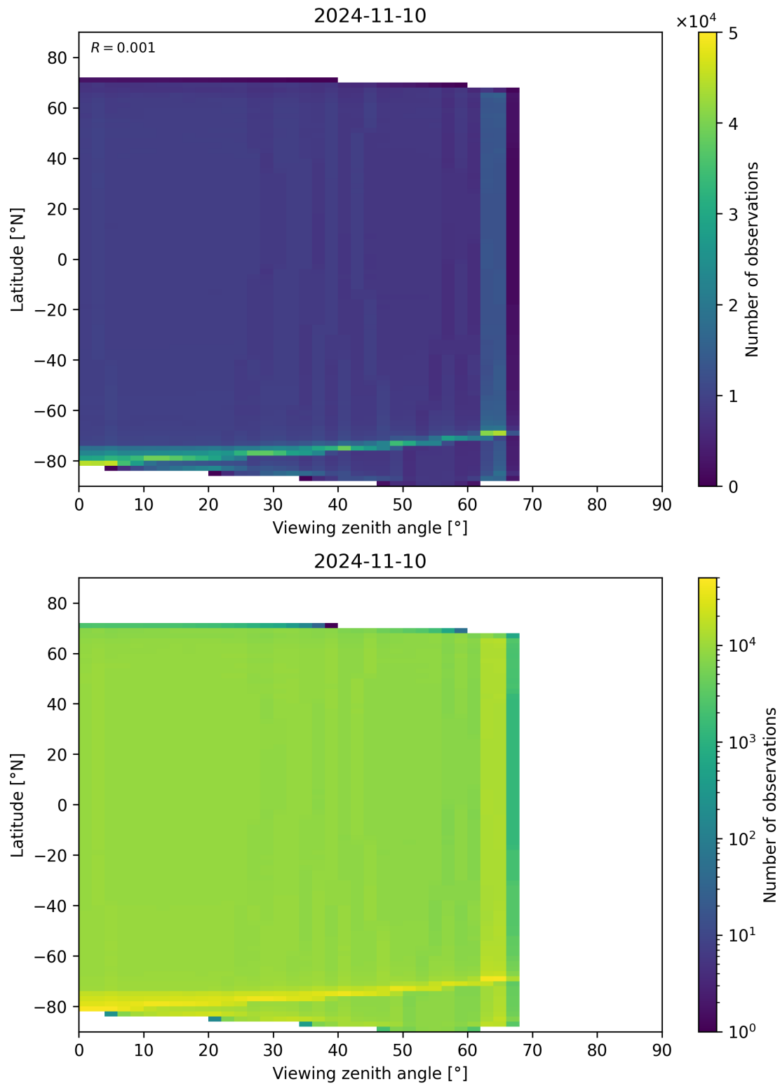
Figure 135: Scatter density plot of “Viewing zenith angle” against “Latitude” for 2024-11-09 to 2024-11-11.
