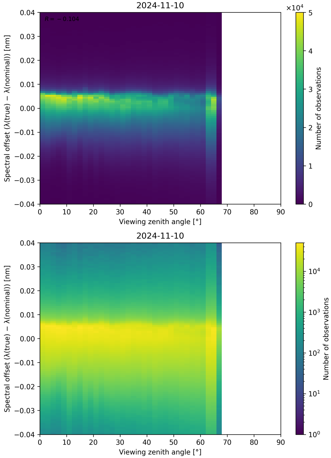
Figure 140: Scatter density plot of “Viewing zenith angle” against “Spectral offset ( \lambda_{\text{true}} - \lambda_{\text{nominal}} )” for 2024-11-09 to 2024-11-11.
