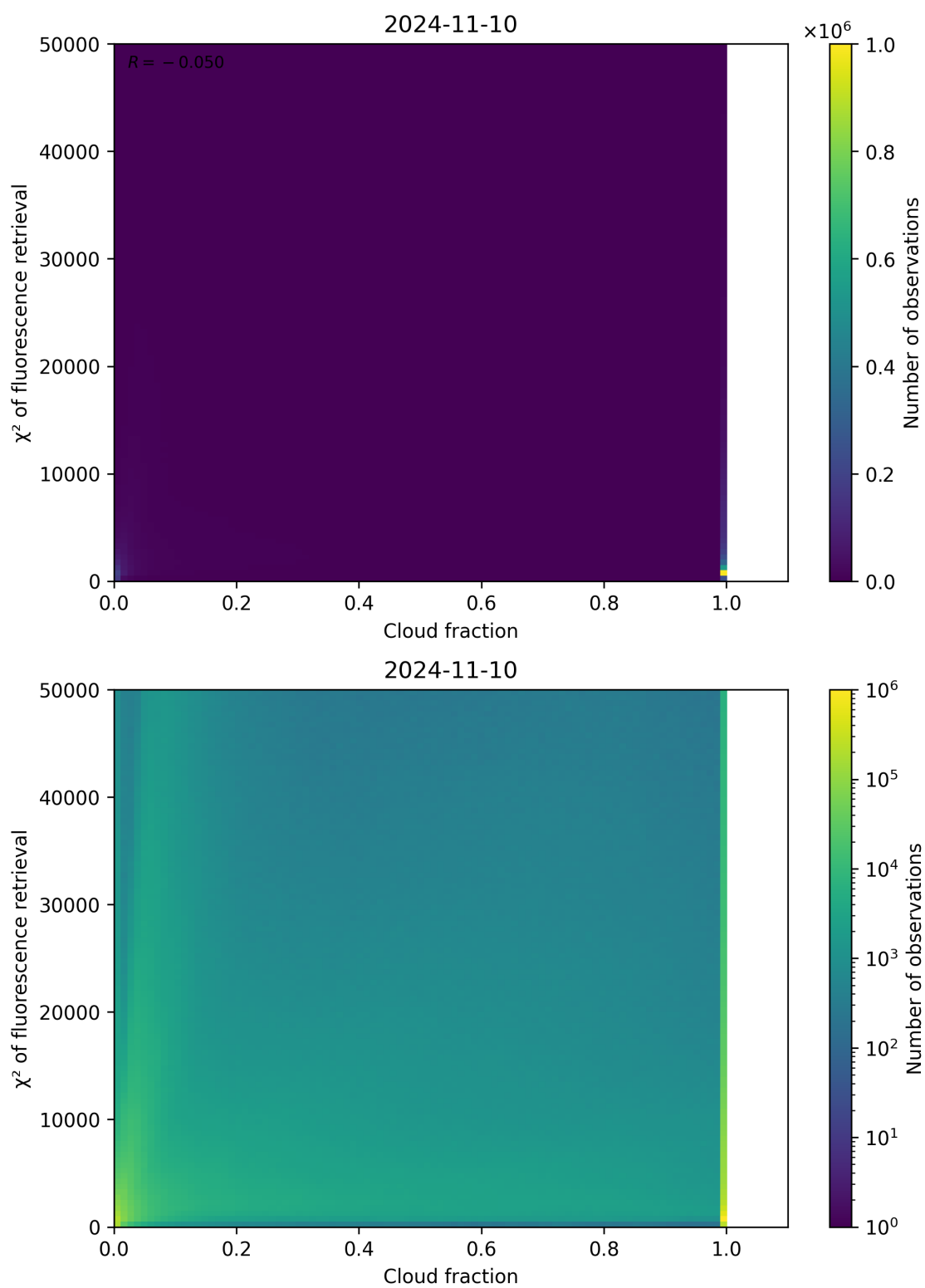
Figure 78: Scatter density plot of “Cloud fraction” against “ \chi^2 of fluorescence retrieval” for 2024-11-09 to 2024-11-11.
