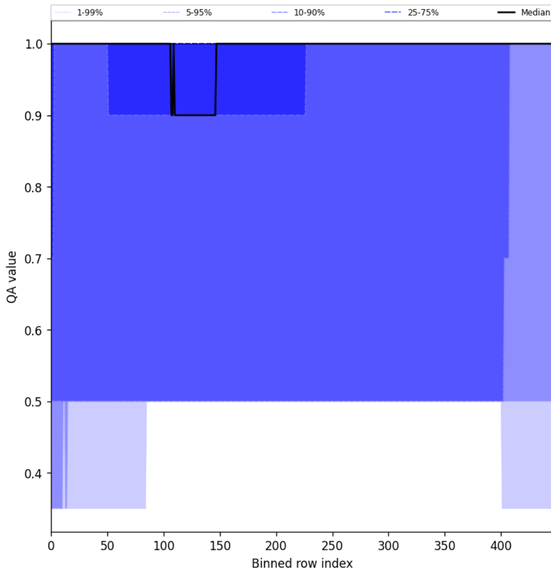
Figure 46: Along track statistics of “QA value” for 2024-11-09 to 2024-11-11
