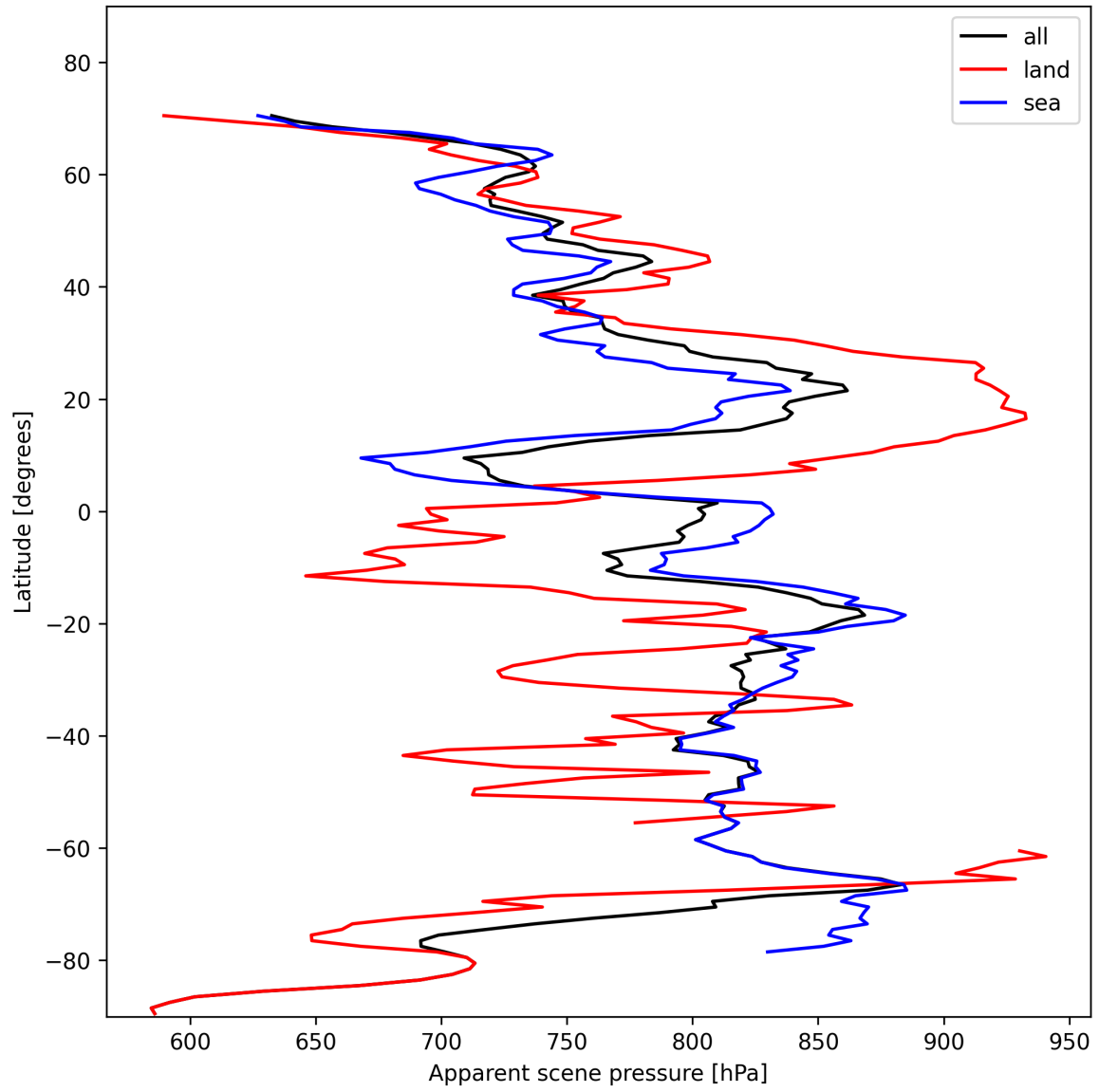
Figure 19: Zonal average of “Apparent scene pressure” for 2024-11-09 to 2024-11-11.
