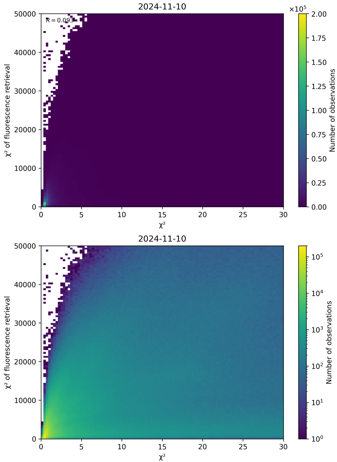
Figure 69: Scatter density plot of “ \chi^2 ” against “ \chi^2 of fluorescence retrieval” for 2024-11-09 to 2024-11-11.
