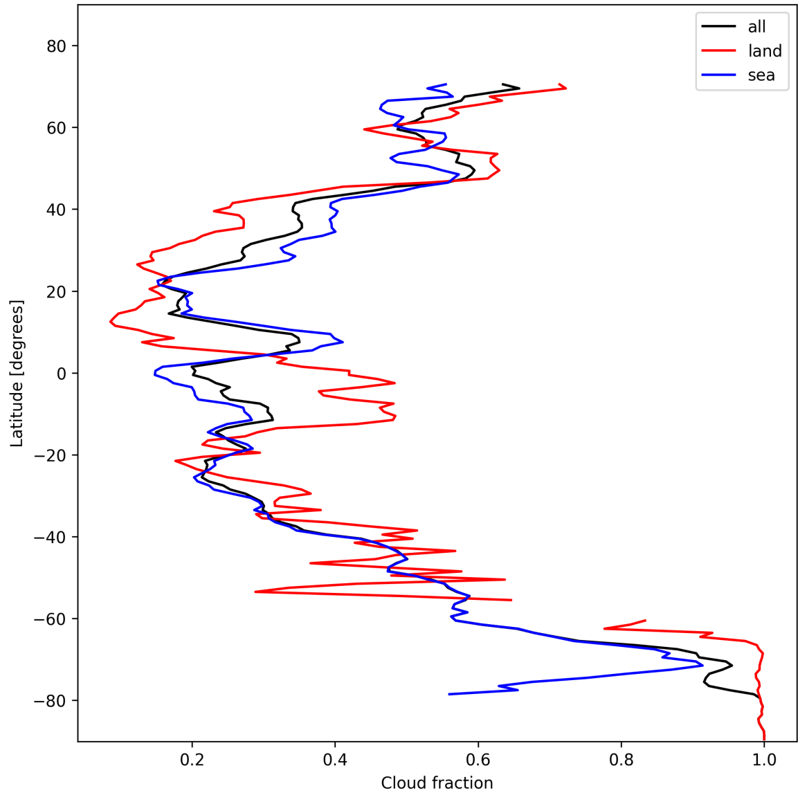
Figure 15: Zonal average of “Cloud fraction” for 2024-11-09 to 2024-11-11.
