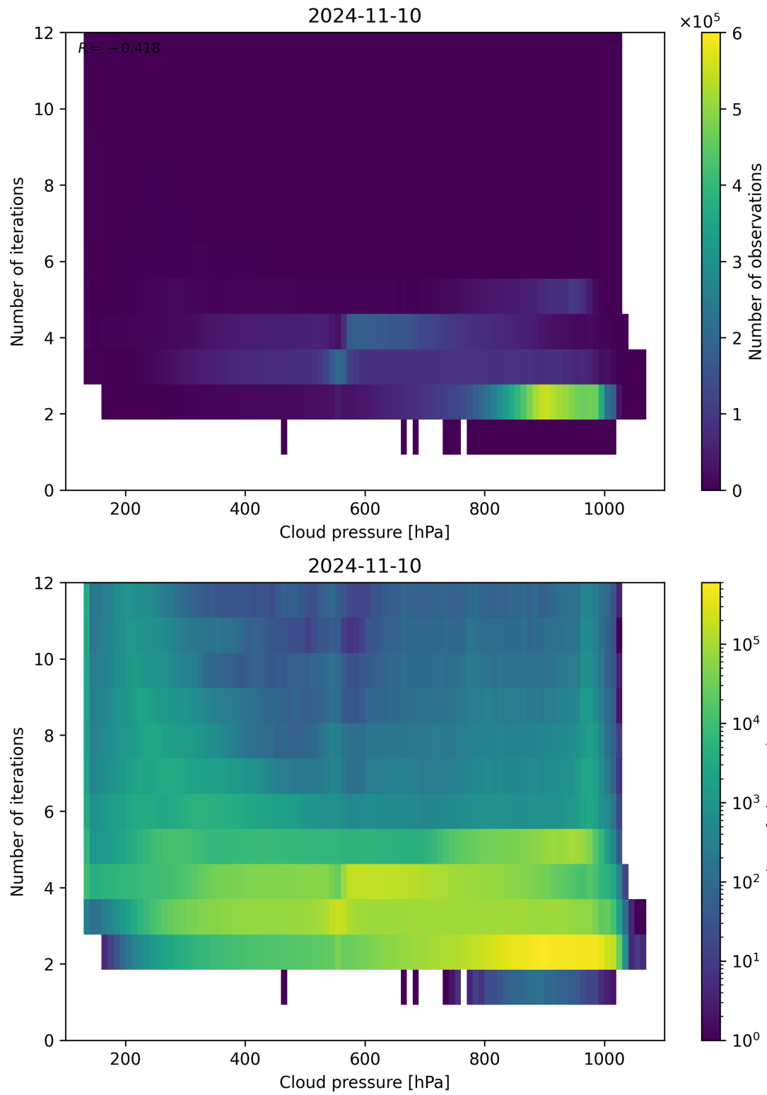
Figure 89: Scatter density plot of “Cloud pressure” against “Number of iterations” for 2024-11-09 to 2024-11-11.
