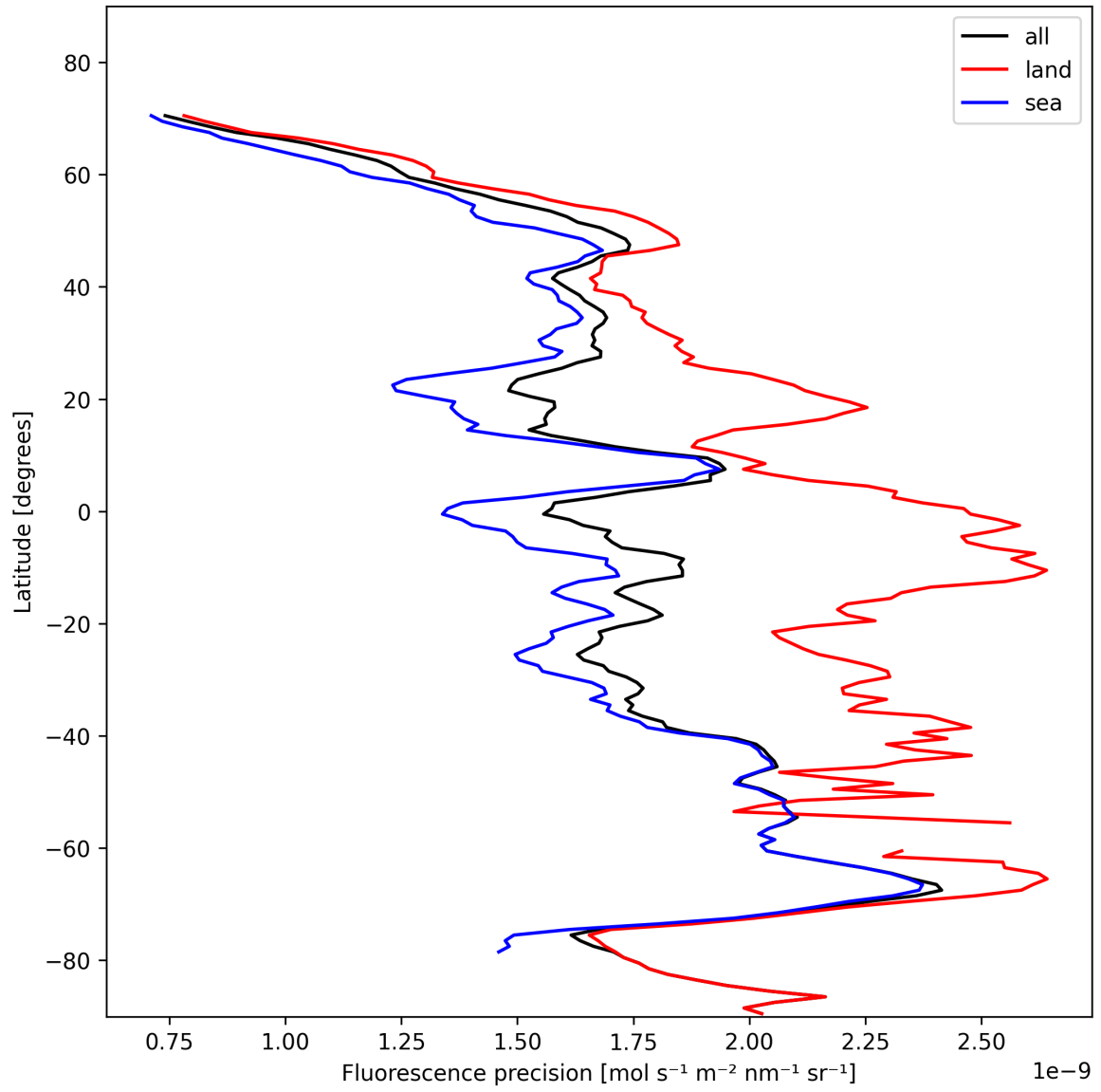
Figure 24: Zonal average of “Fluorescence precision” for 2024-11-09 to 2024-11-11.
