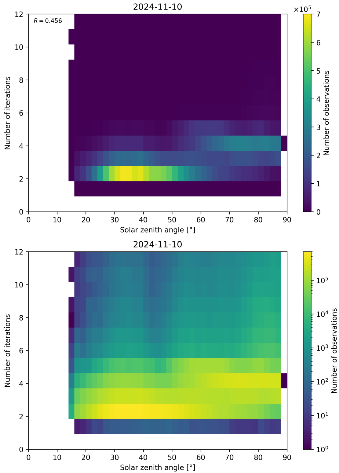
Figure 125: Scatter density plot of “Solar zenith angle” against “Number of iterations” for 2024-11-09 to 2024-11-11.
