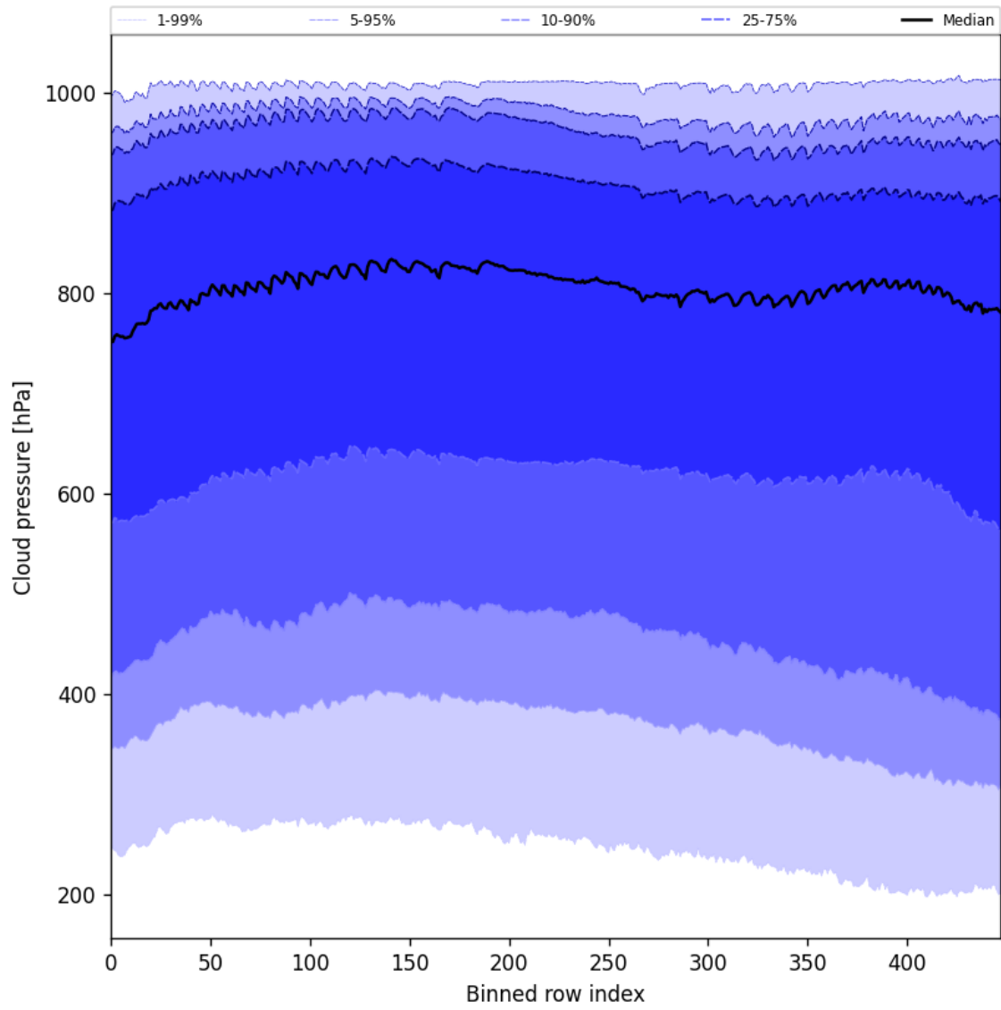
Figure 47: Along track statistics of “Cloud pressure” for 2024-11-09 to 2024-11-11
