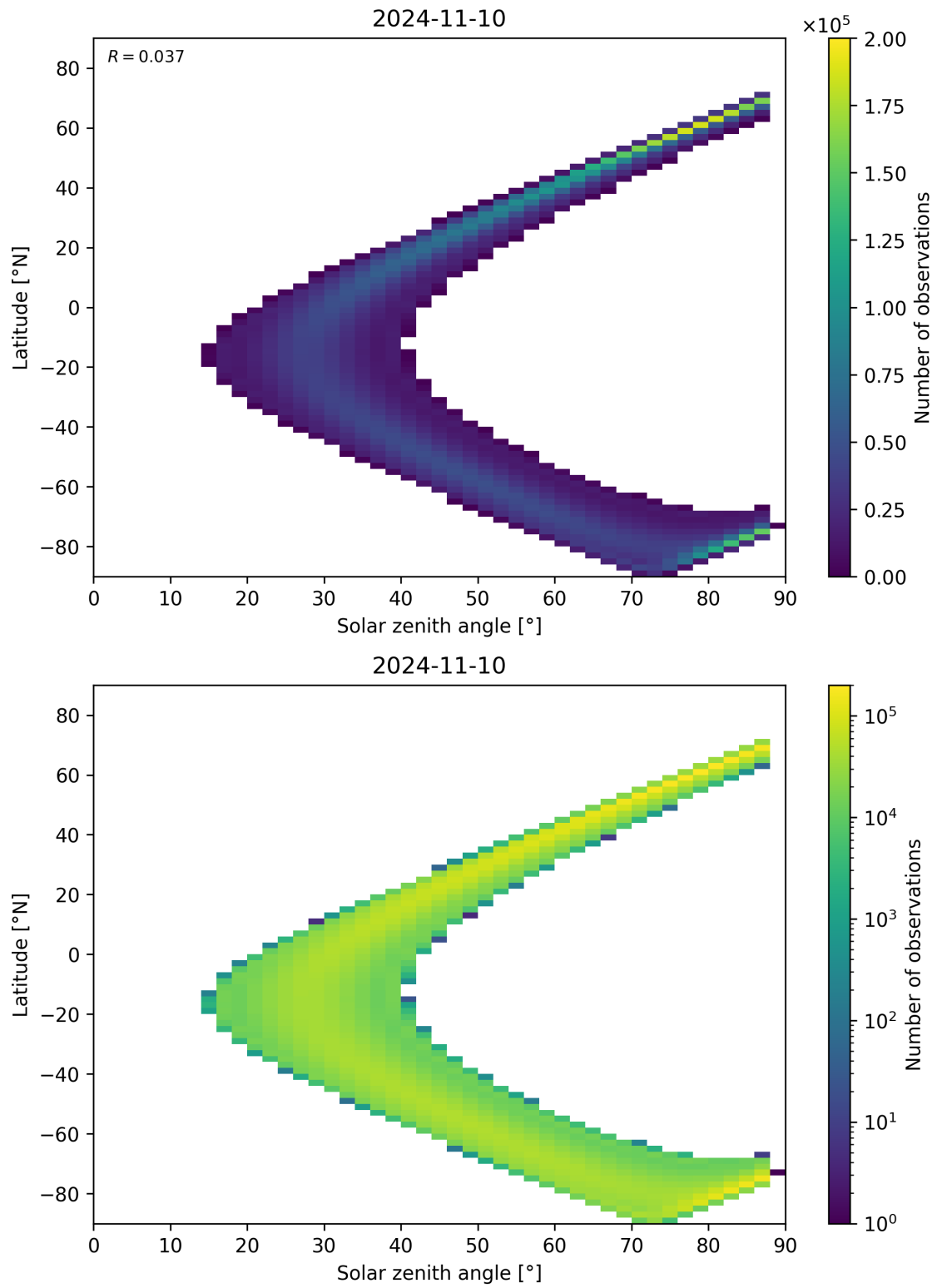
Figure 124: Scatter density plot of “Solar zenith angle” against “Latitude” for 2024-11-09 to 2024-11-11.
