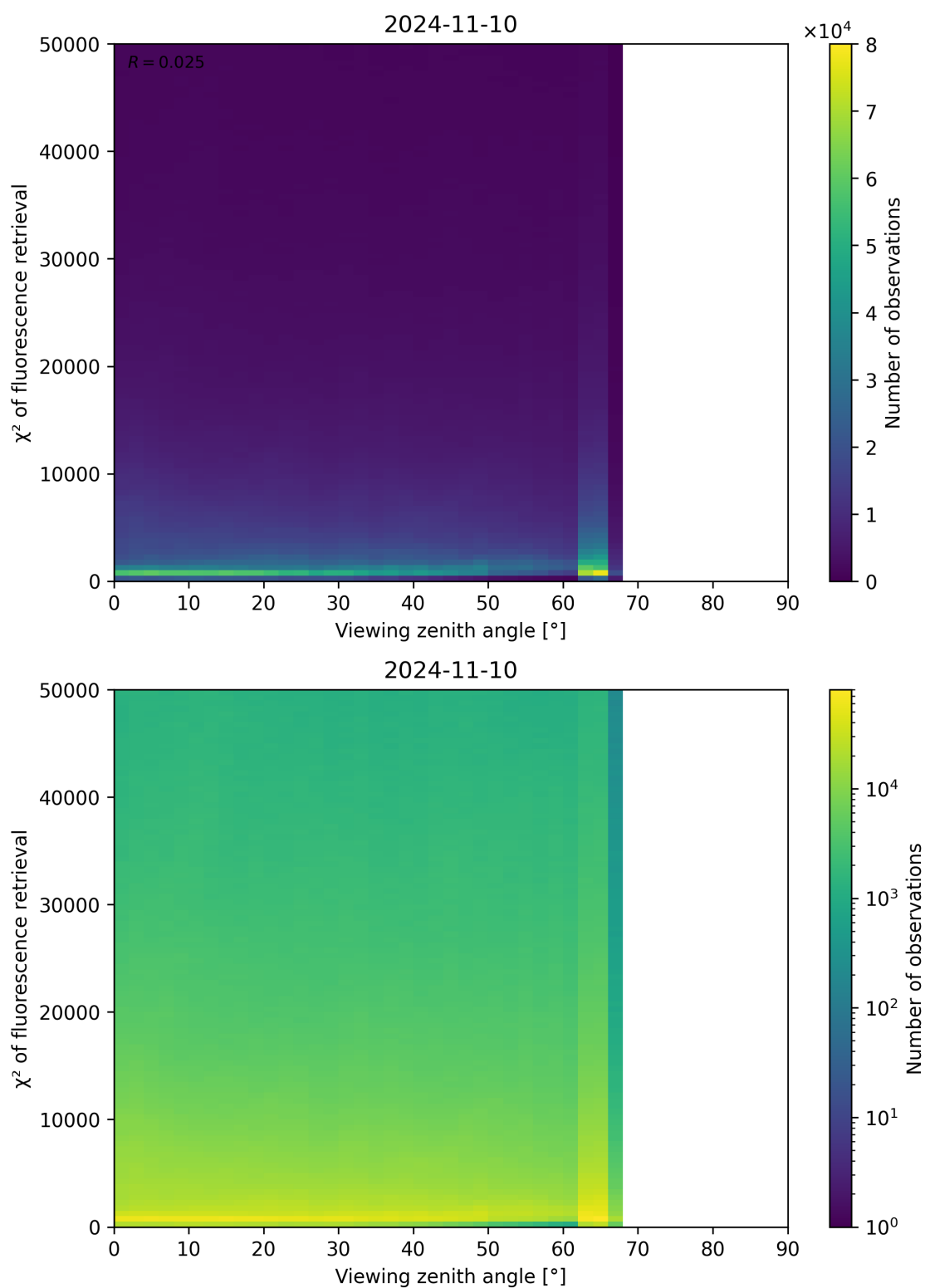
Figure 131: Scatter density plot of “Viewing zenith angle” against “ \chi^2 of fluorescence retrieval” for 2024-11-09 to 2024-11-11.
