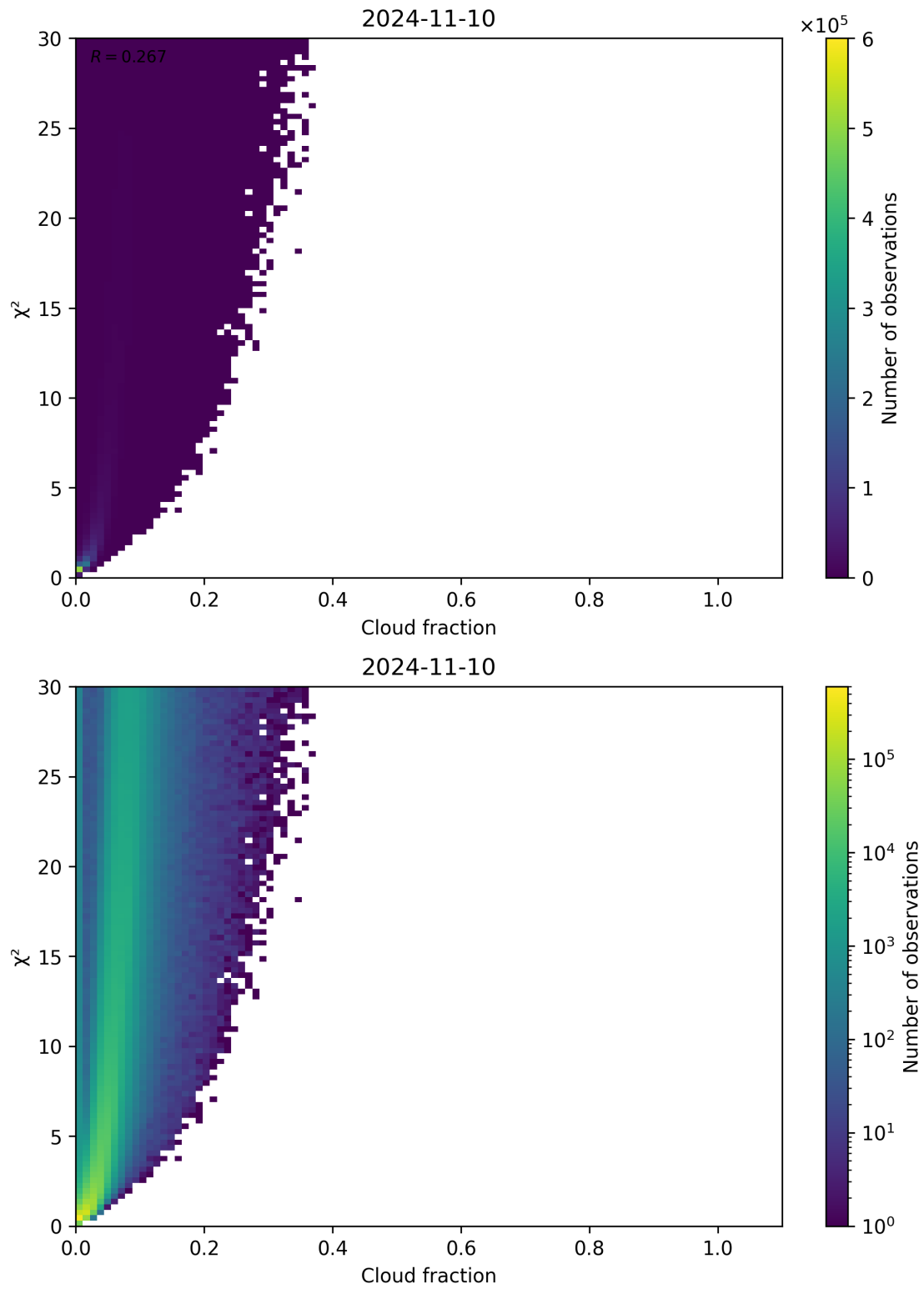
Figure 77: Scatter density plot of “Cloud fraction” against “ \chi^2 ” for 2024-11-09 to 2024-11-11.
