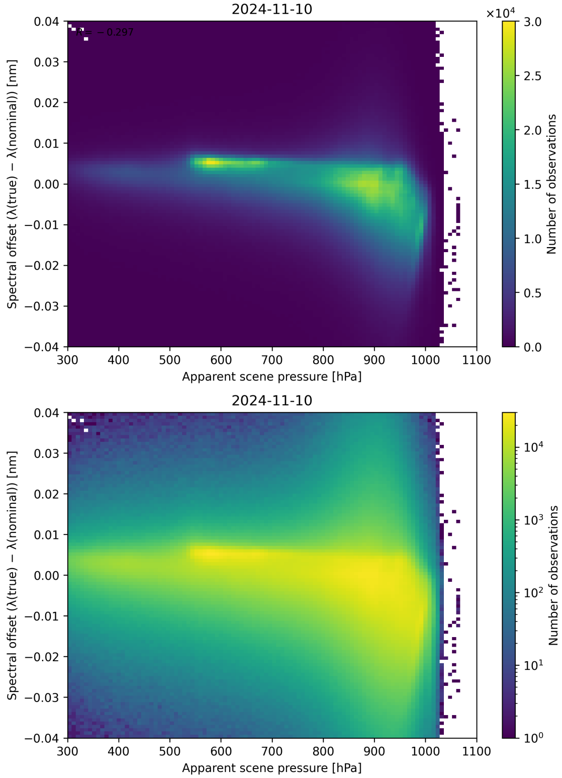
Figure 68: Scatter density plot of “Apparent scene pressure” against “Spectral offset ( \lambda_{\text{true}} - \lambda_{\text{nominal}} )” for 2024-11-09 to 2024-11-11.
