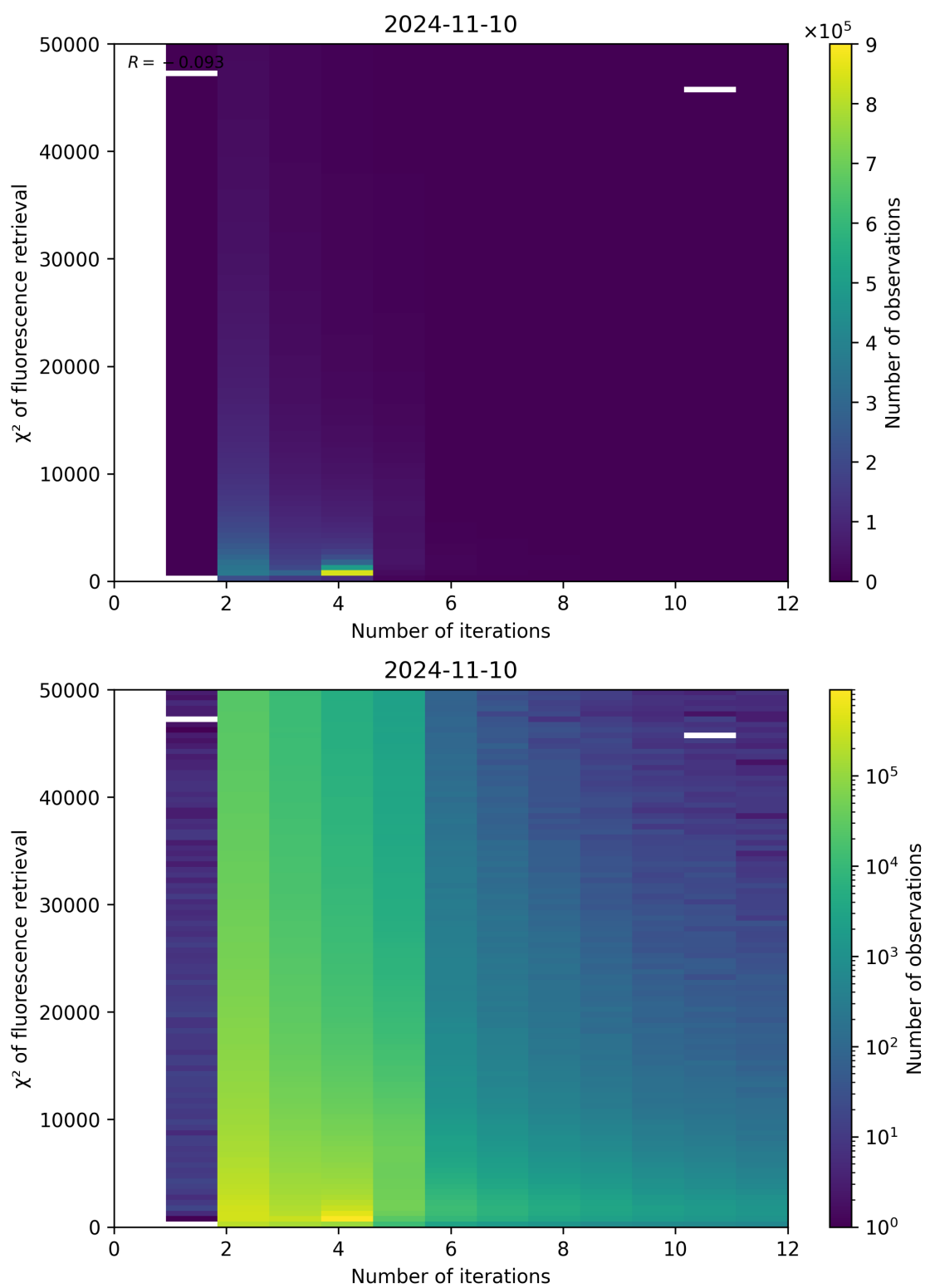
Figure 106: Scatter density plot of “Number of iterations” against “ \chi^2 of fluorescence retrieval” for 2024-11-09 to 2024-11-11.
