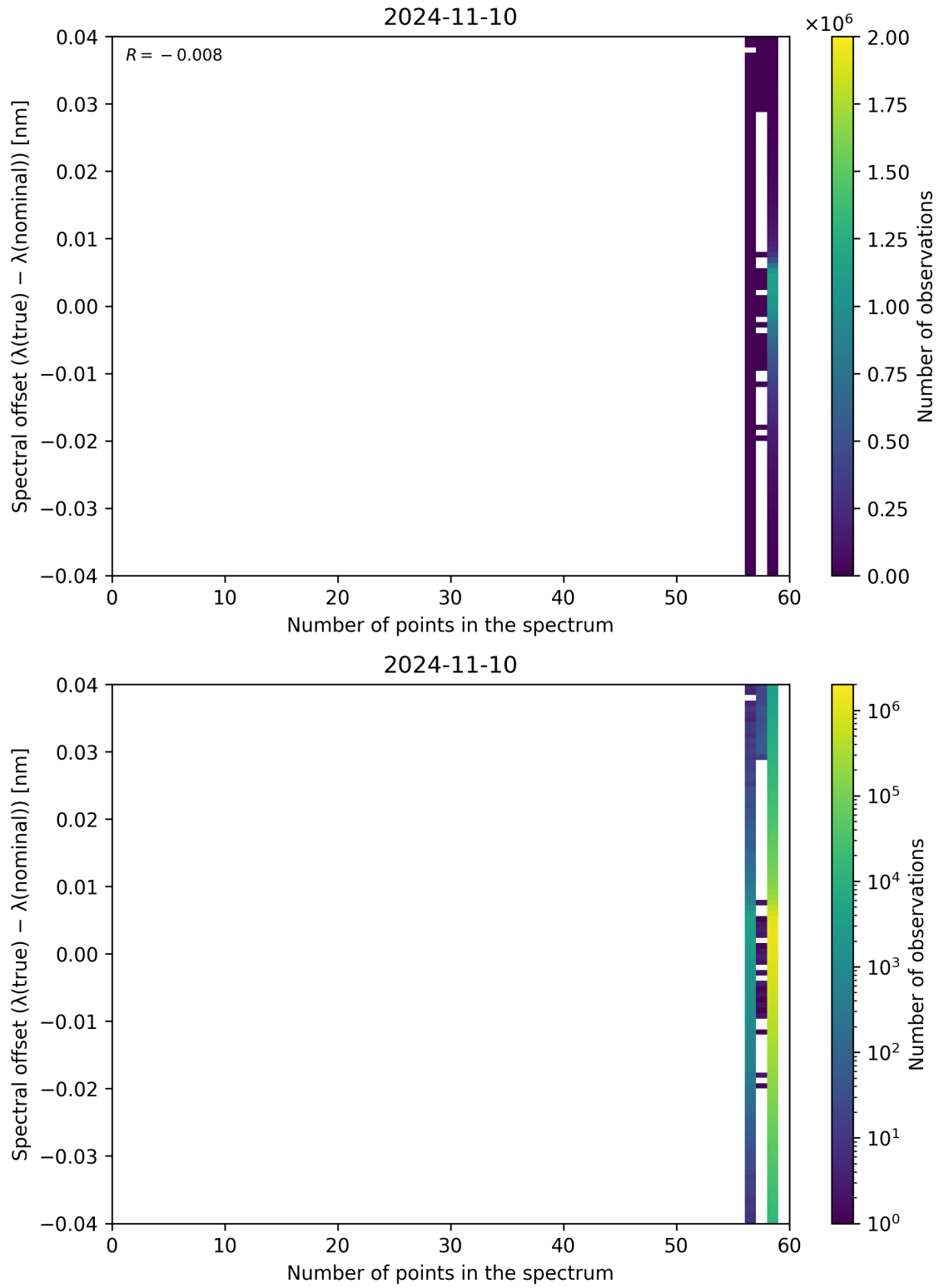
Figure 110: Scatter density plot of “Number of points in the spectrum” against “Spectral offset ( \lambda_{\text{true}} - \lambda_{\text{nominal}} )” for 2024-11-09 to 2024-11-11.
