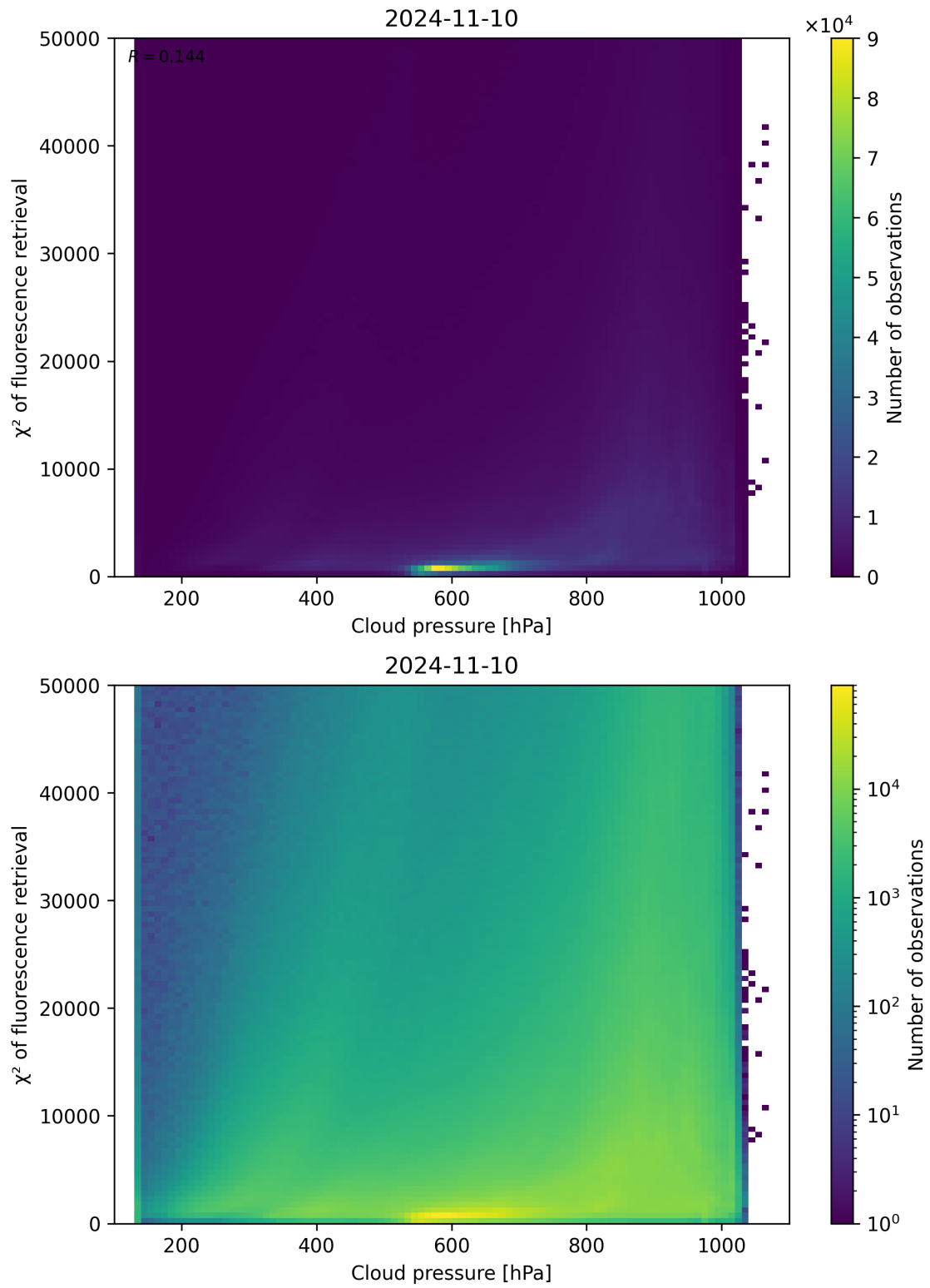
Figure 86: Scatter density plot of “Cloud pressure” against “ \chi^2 of fluorescence retrieval” for 2024-11-09 to 2024-11-11.
