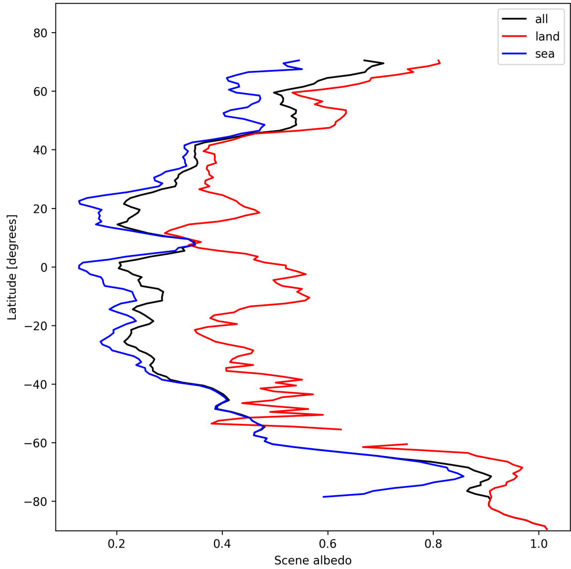
Figure 17: Zonal average of “Scene albedo” for 2024-11-09 to 2024-11-11.
