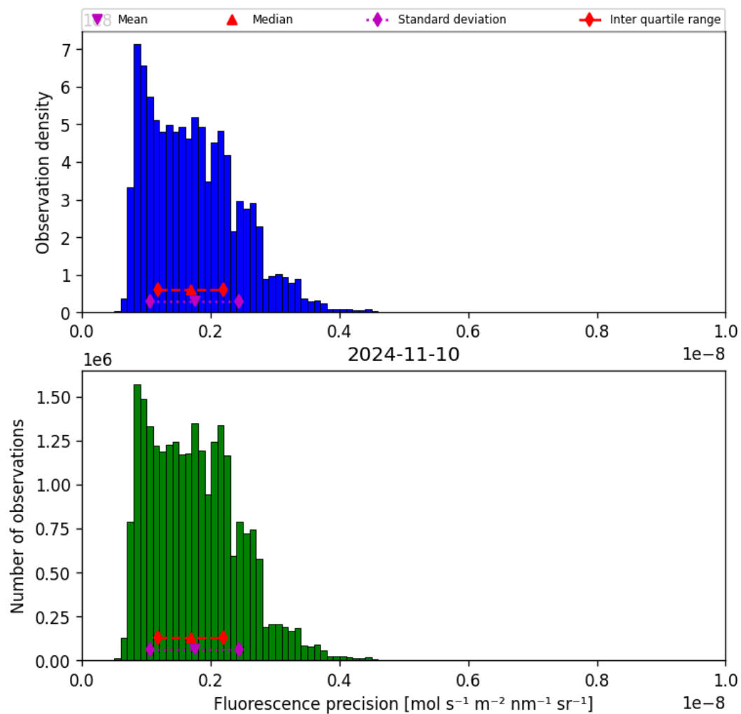
Figure 41: Histogram of “Fluorescence precision” for 2024-11-09 to 2024-11-11
