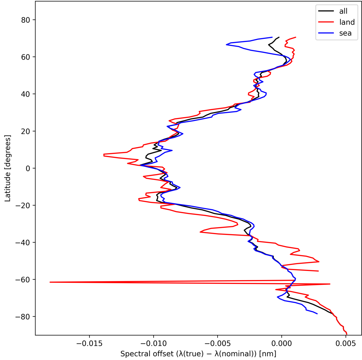
Figure 28: Zonal average of “Spectral offset ( \lambda_{\text{true}} - \lambda_{\text{nominal}} )” for 2024-11-09 to 2024-11-11.
