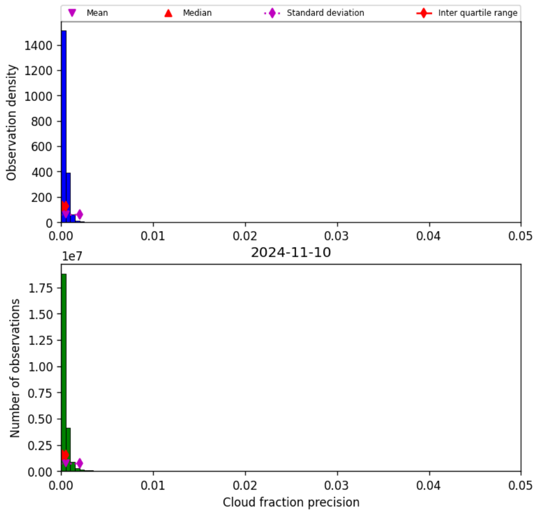
Figure 33: Histogram of “Cloud fraction precision” for 2024-11-09 to 2024-11-11
