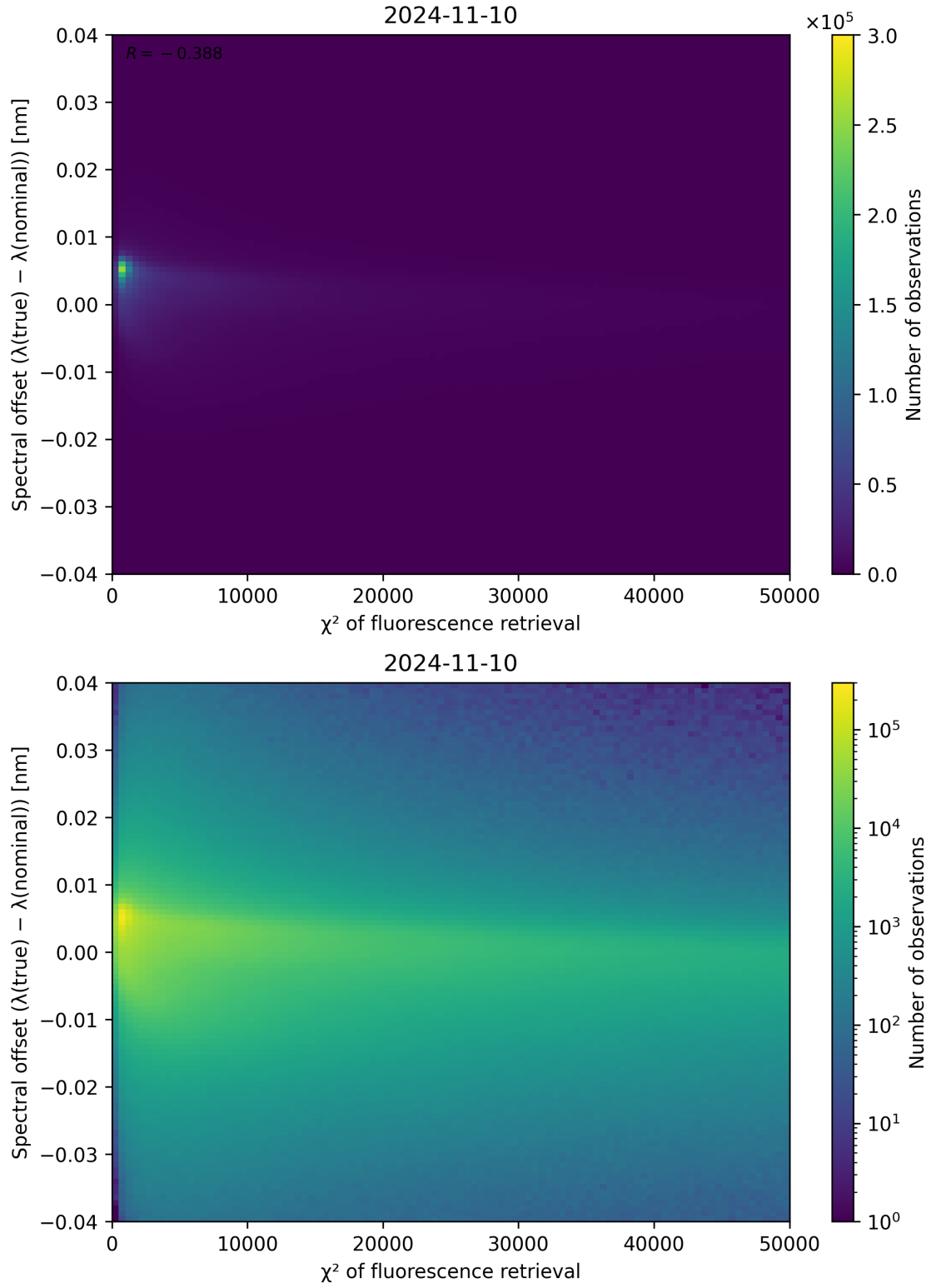
Figure 72: Scatter density plot of “ \chi^2 of fluorescence retrieval” against “Spectral offset ( \lambda_{\text{true}} - \lambda_{\text{nominal}} )” for 2024-11-09 to 2024-11-11.
