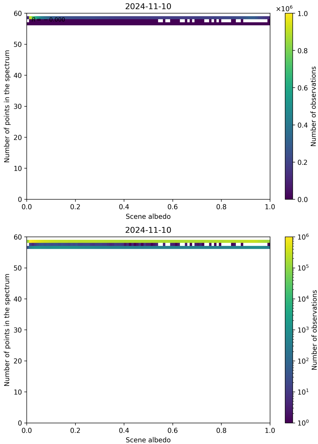
Figure 116: Scatter density plot of “Scene albedo” against “Number of points in the spectrum” for 2024-11-09 to 2024-11-11.
