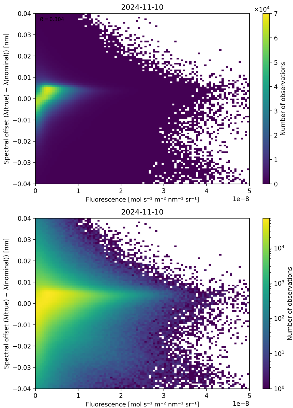
Figure 95: Scatter density plot of “Fluorescence” against “Spectral offset ( \lambda_{\text{true}} - \lambda_{\text{nominal}} )” for 2024-11-09 to 2024-11-11.
