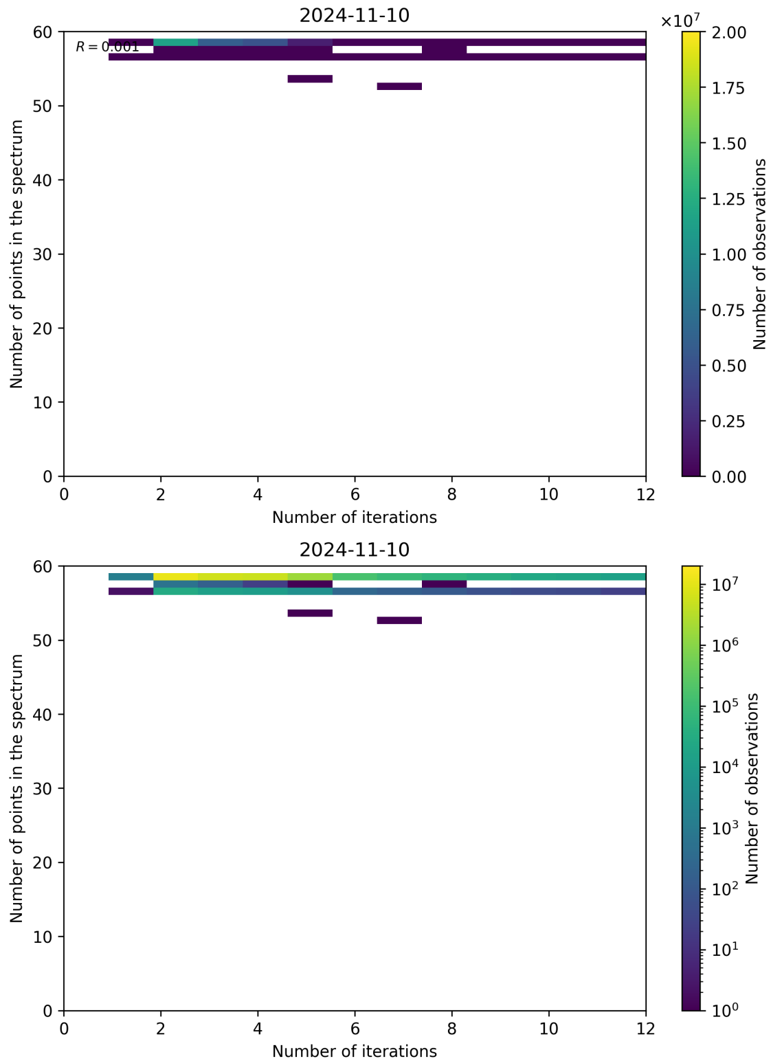
Figure 108: Scatter density plot of “Number of iterations” against “Number of points in the spectrum” for 2024-11-09 to 2024-11-11.
