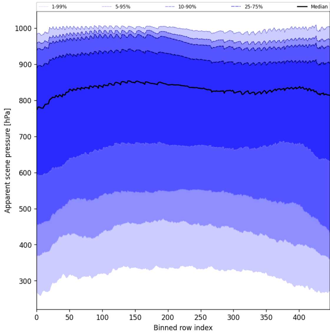
Figure 53: Along track statistics of “Apparent scene pressure” for 2024-11-09 to 2024-11-11
