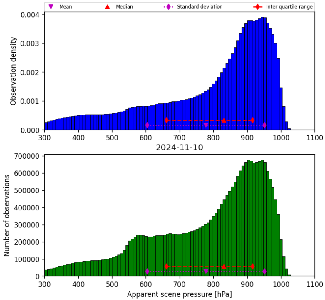
Figure 36: Histogram of “Apparent scene pressure” for 2024-11-09 to 2024-11-11
