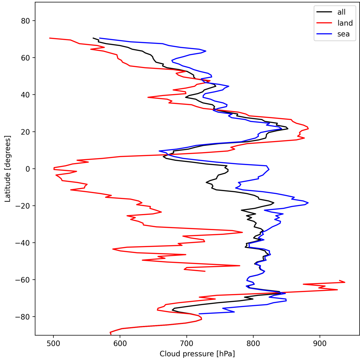
Figure 13: Zonal average of “Cloud pressure” for 2024-11-09 to 2024-11-11.
