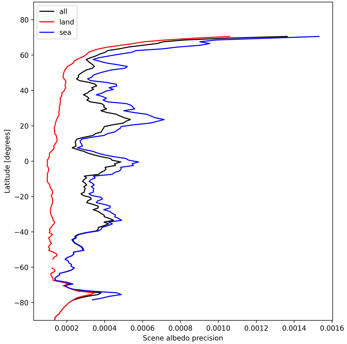
Figure 18: Zonal average of "Scene albedo precision" for 2024-11-09 to 2024-11-11.
