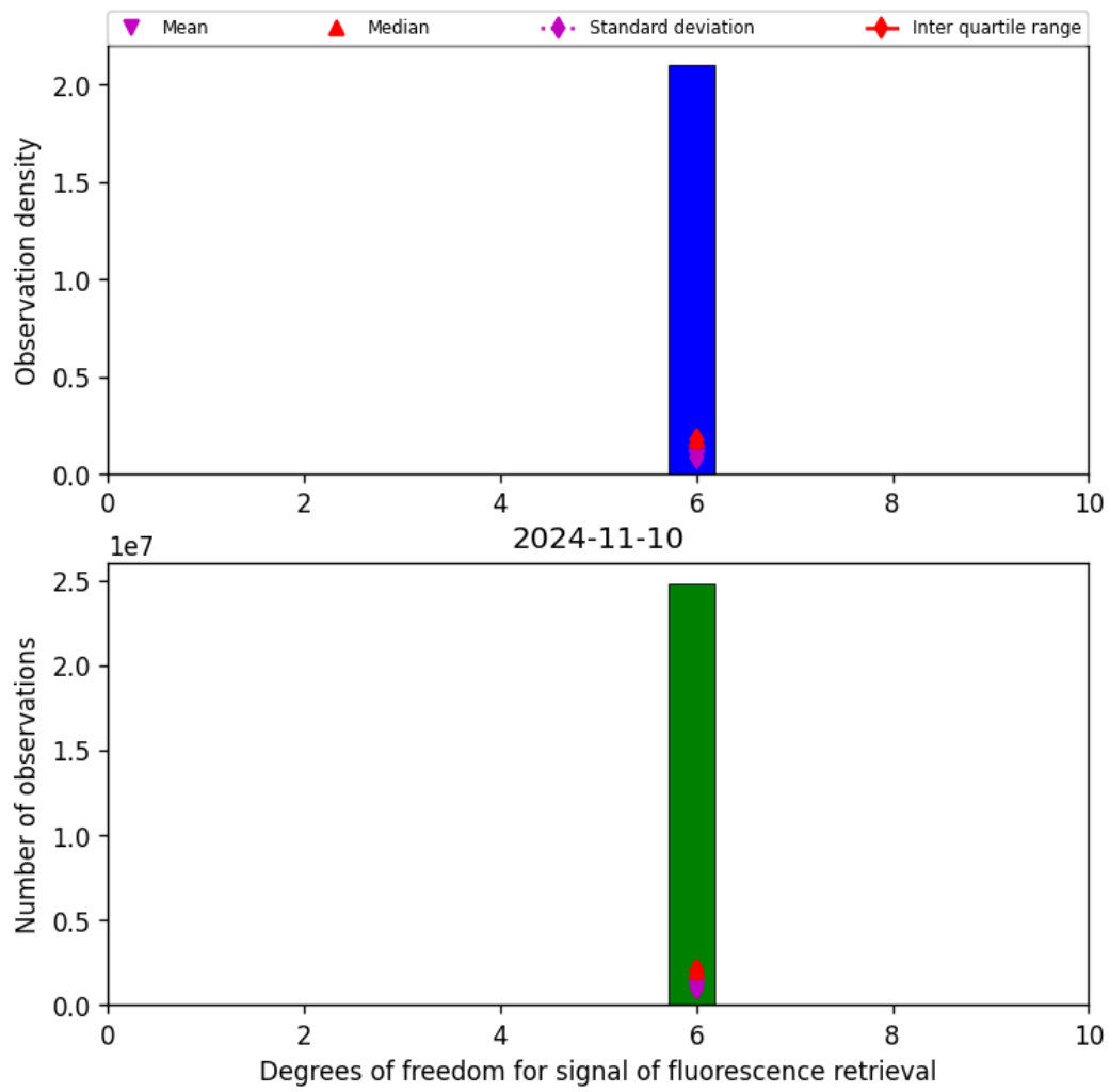
Figure 43: Histogram of "Degrees of freedom for signal of fluorescence retrieval" for 2024-11-09 to 2024-11-11
