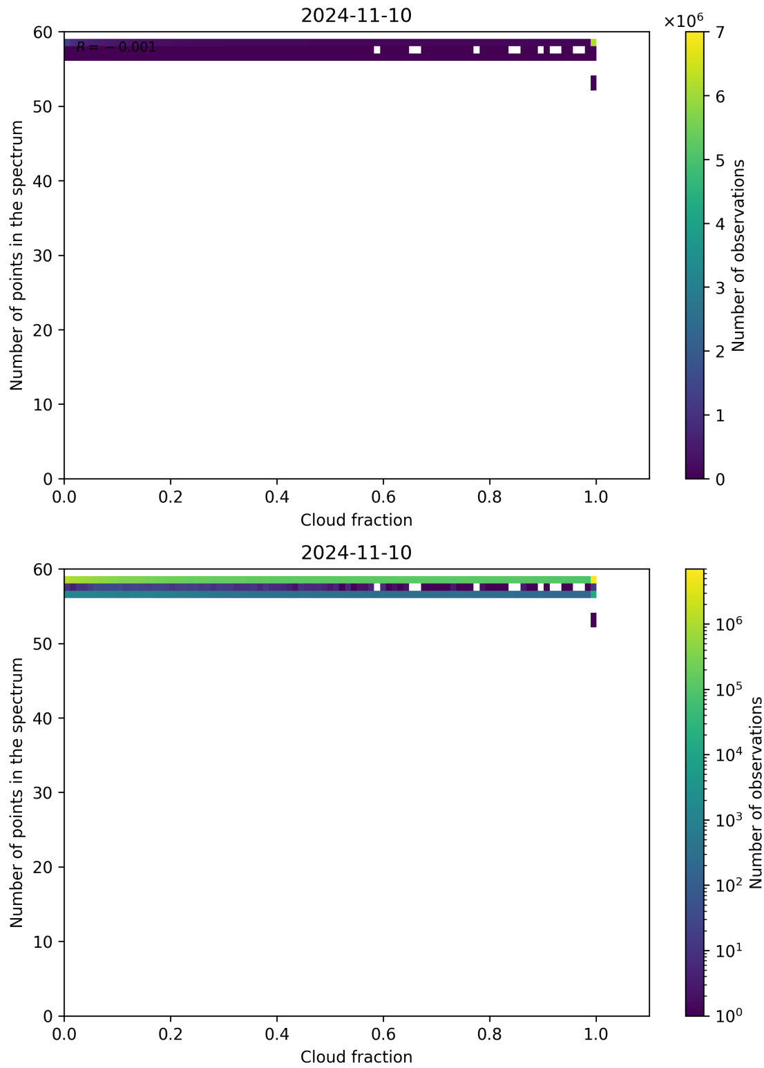
Figure 81: Scatter density plot of “Cloud fraction” against “Number of points in the spectrum” for 2024-11-09 to 2024-11-11.
