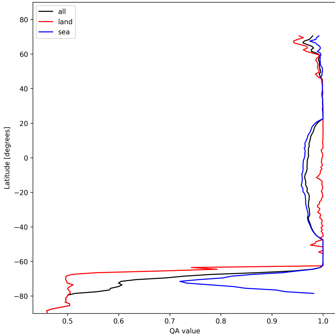
Figure 12: Zonal average of “QA value” for 2024-11-09 to 2024-11-11.
