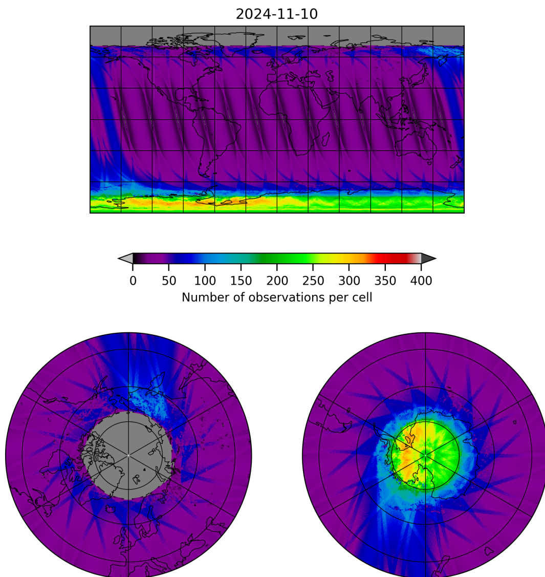
Figure 11: Map of the number of observations for 2024-11-09 to 2024-11-11
