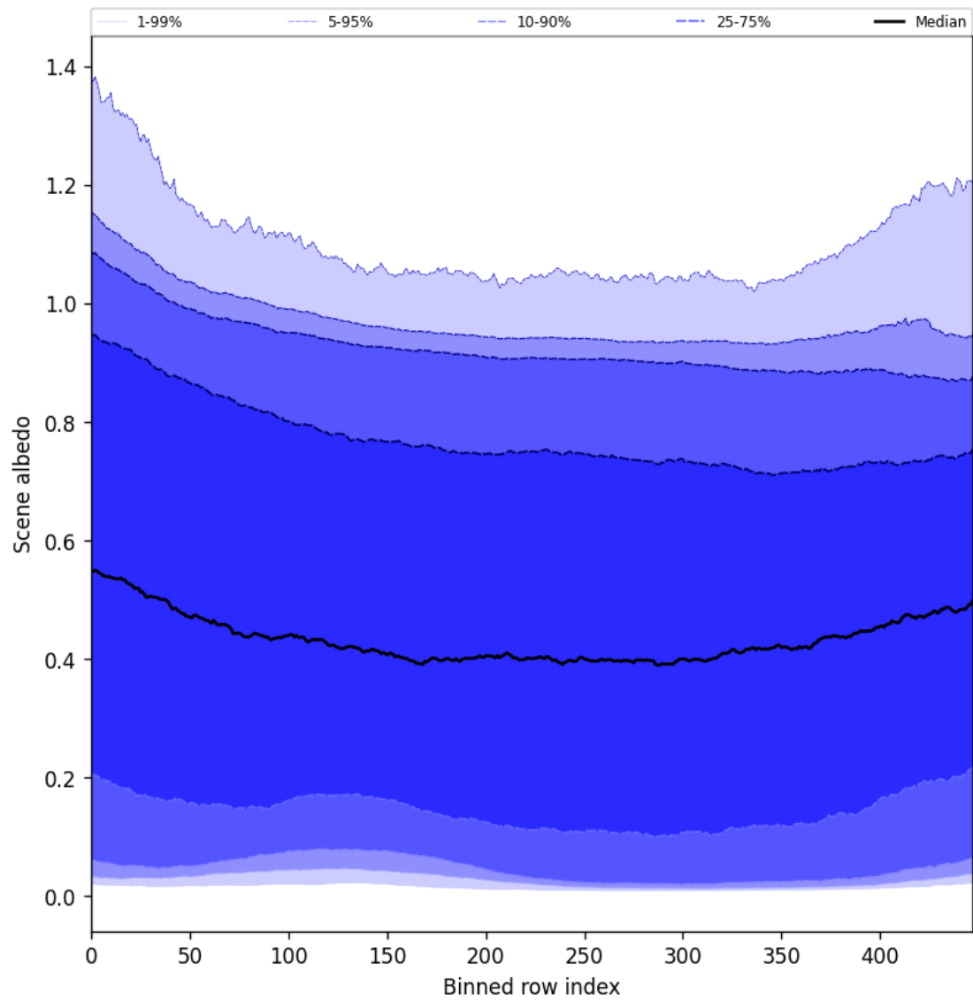
Figure 51: Along track statistics of “Scene albedo” for 2024-11-09 to 2024-11-11
