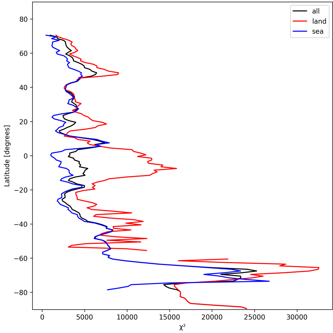
Figure 21: Zonal average of “ \chi^2 ” for 2024-11-09 to 2024-11-11.
