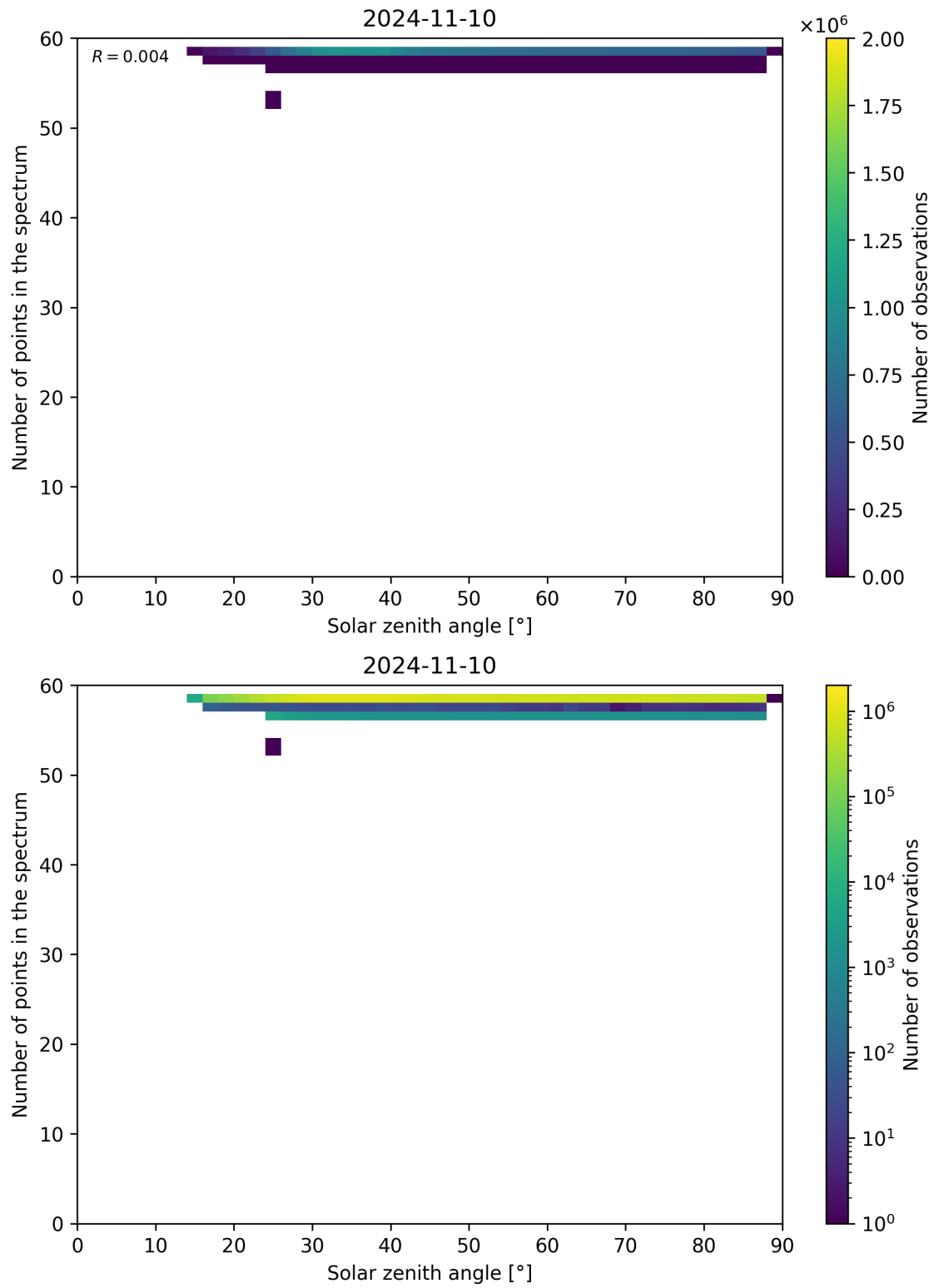
Figure 126: Scatter density plot of “Solar zenith angle” against “Number of points in the spectrum” for 2024-11-09 to 2024-11-11.
