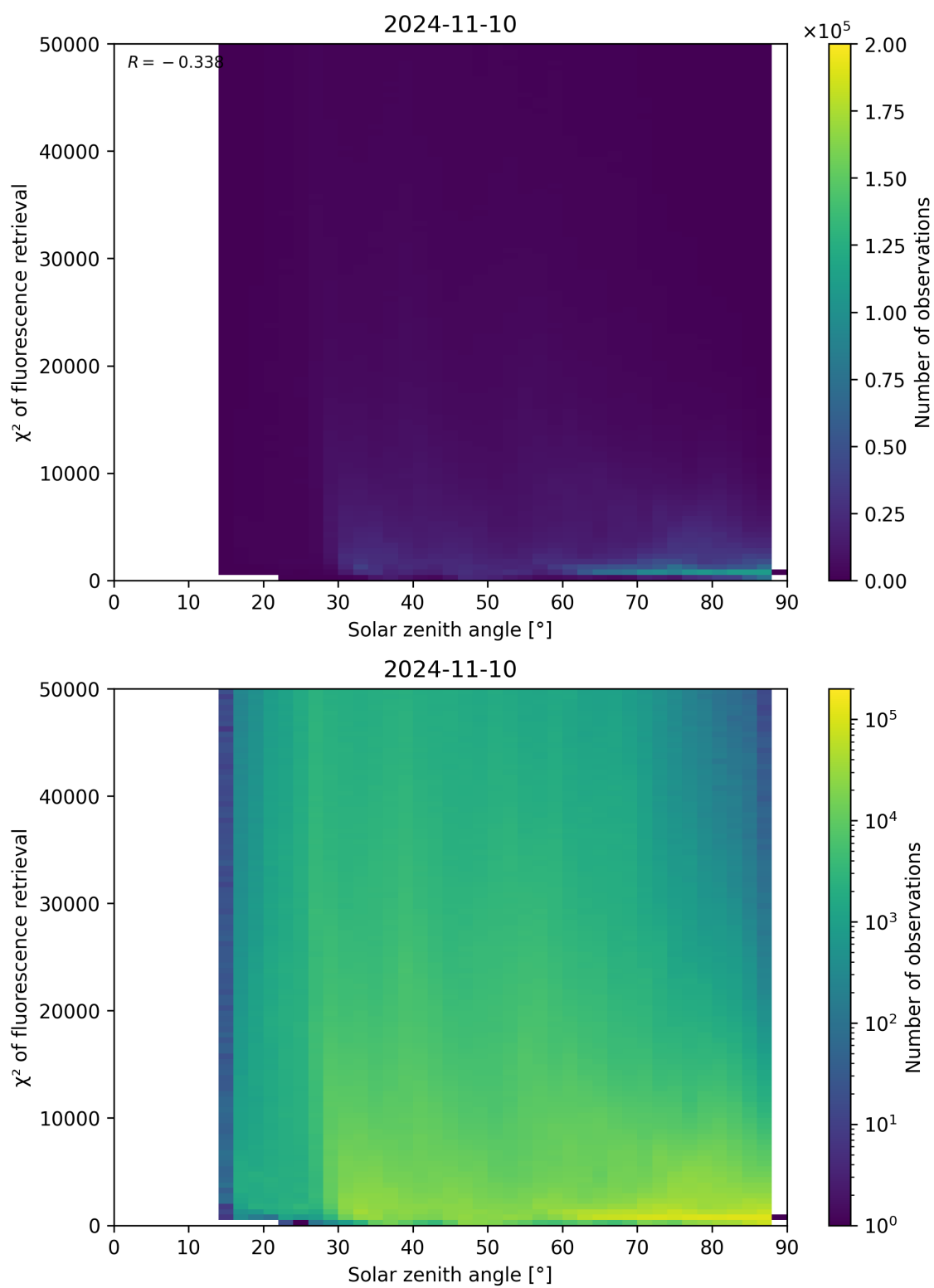
Figure 120: Scatter density plot of “Solar zenith angle” against “ \chi^2 of fluorescence retrieval” for 2024-11-09 to 2024-11-11.
