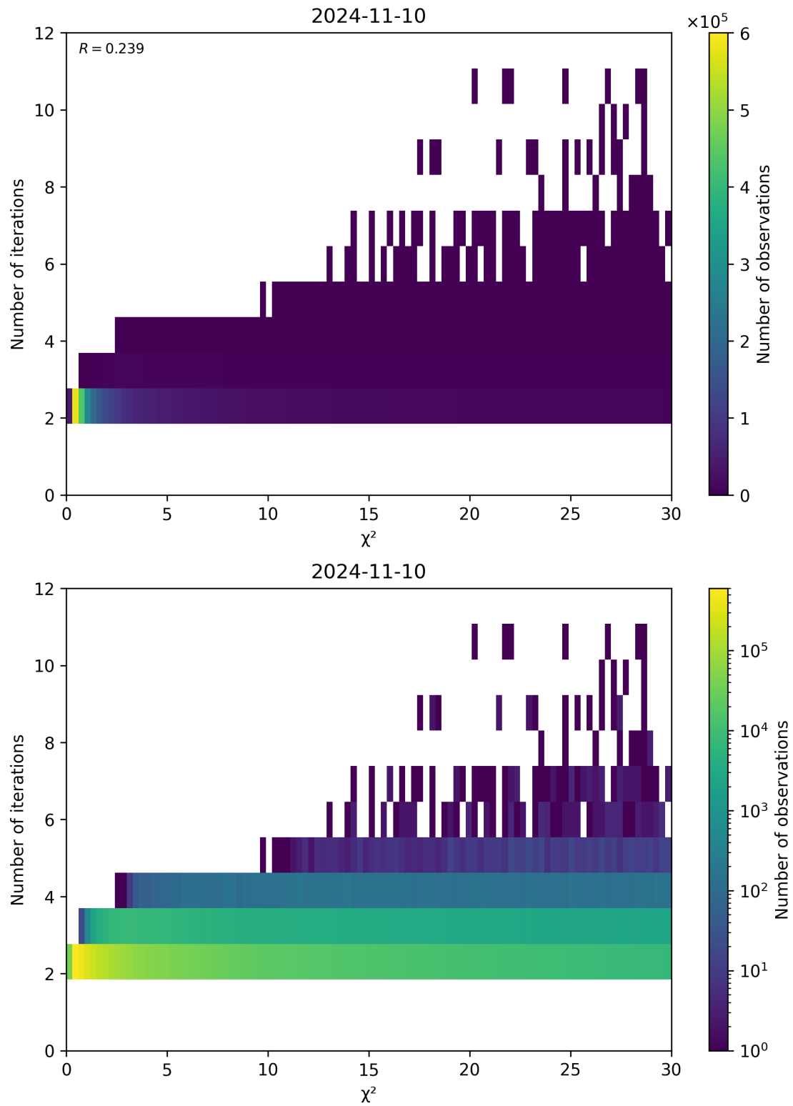
Figure 73: Scatter density plot of “ \chi^2 ” against “Number of iterations” for 2024-11-09 to 2024-11-11.
