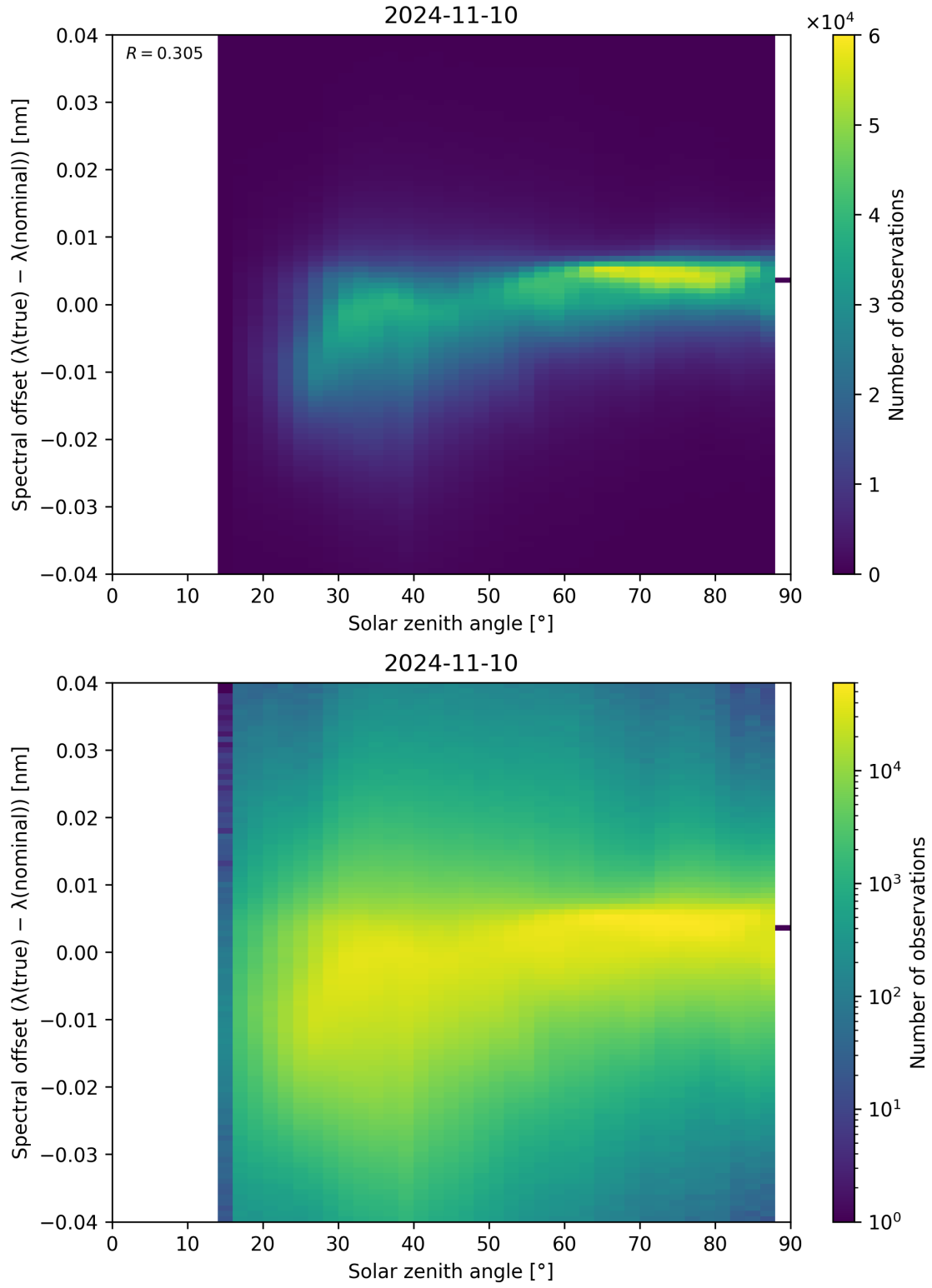
Figure 128: Scatter density plot of “Solar zenith angle” against “Spectral offset ( \lambda_{\text{true}} - \lambda_{\text{nominal}} )” for 2024-11-09 to 2024-11-11.
