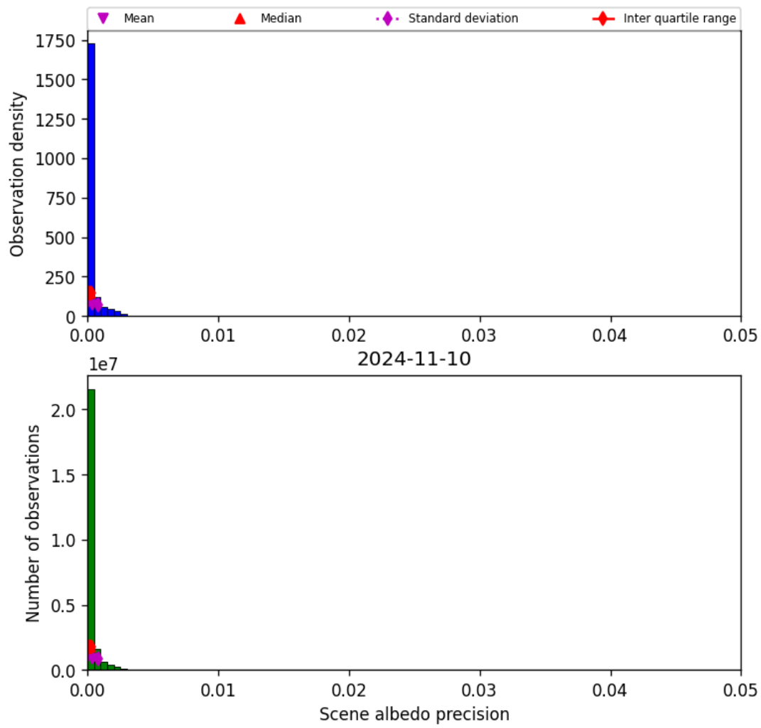
Figure 35: Histogram of “Scene albedo precision” for 2024-11-09 to 2024-11-11
