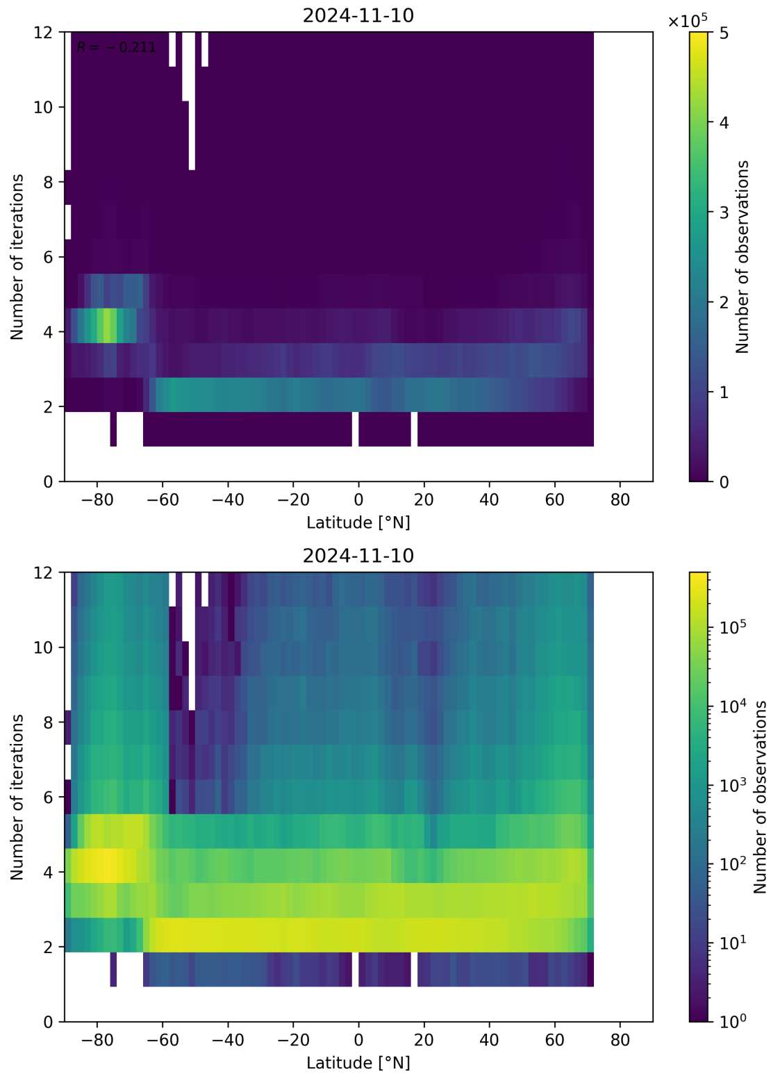
Figure 102: Scatter density plot of “Latitude” against “Number of iterations” for 2024-11-09 to 2024-11-11.
