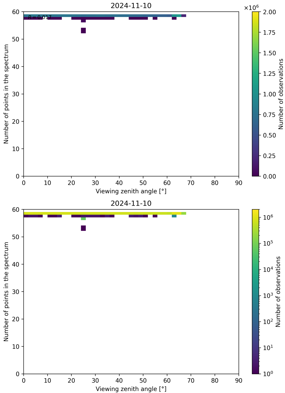
Figure 137: Scatter density plot of “Viewing zenith angle” against “Number of points in the spectrum” for 2024-11-09 to 2024-11-11.
