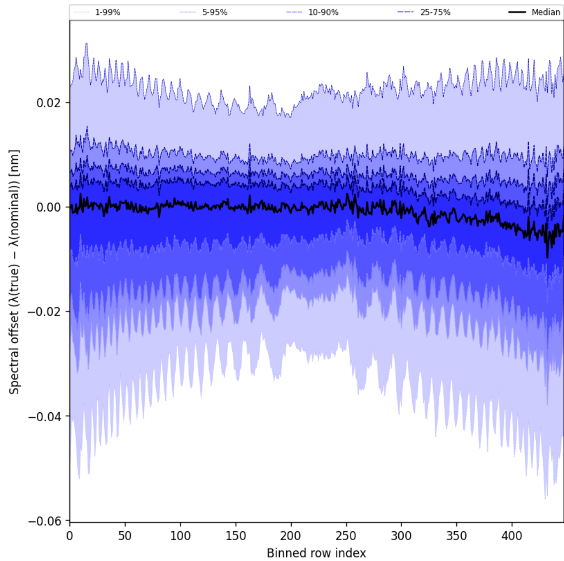
Figure 62: Along track statistics of “Spectral offset ( \lambda_{\text{true}} - \lambda_{\text{nominal}} )” for 2024-11-09 to 2024-11-11
