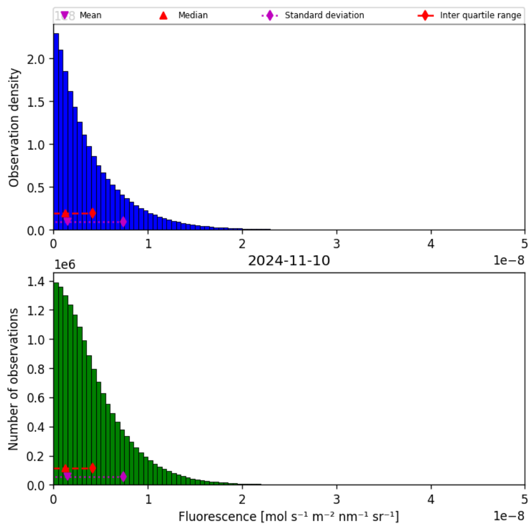
Figure 40: Histogram of “Fluorescence” for 2024-11-09 to 2024-11-11
