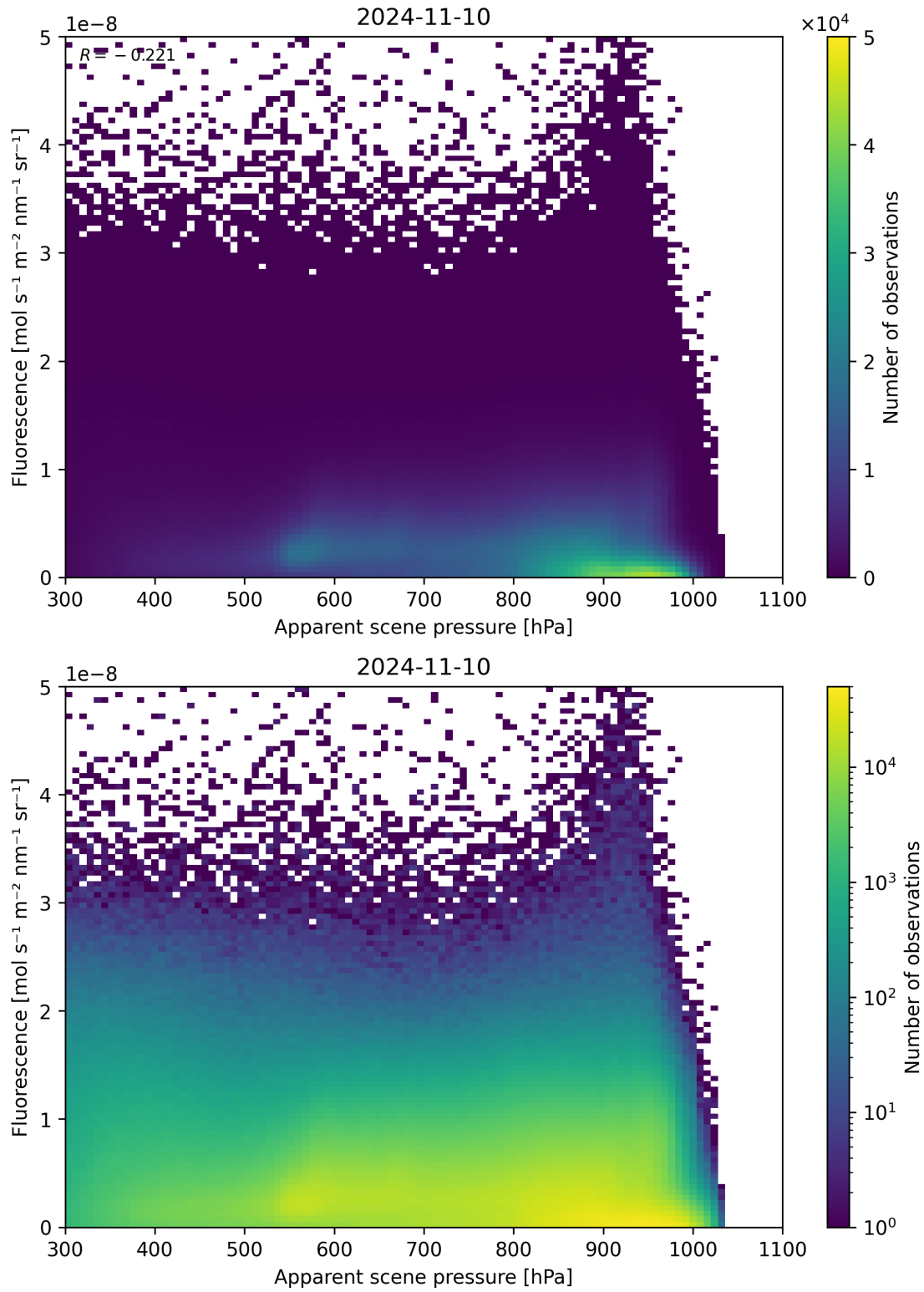
Figure 65: Scatter density plot of “Apparent scene pressure” against “Fluorescence” for 2024-11-09 to 2024-11-11.
