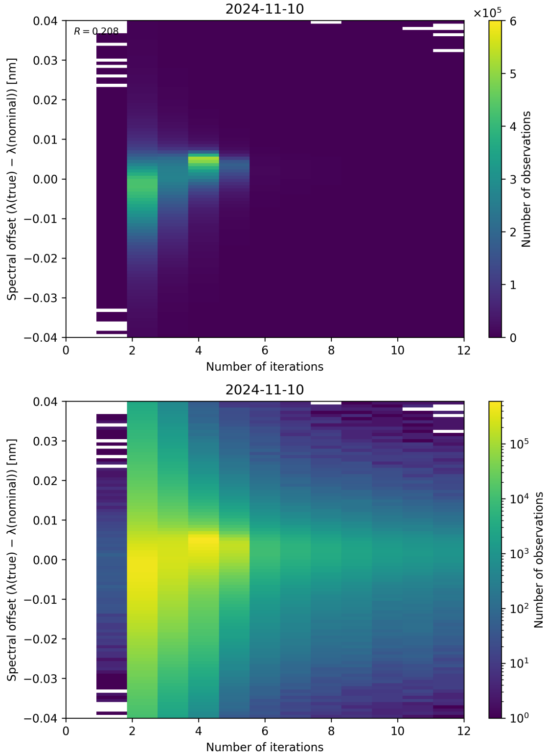
Figure 109: Scatter density plot of “Number of iterations” against “Spectral offset ( \lambda_{\text{true}} - \lambda_{\text{nominal}} )” for 2024-11-09 to 2024-11-11.
