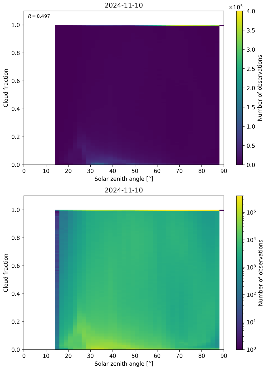
Figure 121: Scatter density plot of “Solar zenith angle” against “Cloud fraction” for 2024-11-09 to 2024-11-11.
