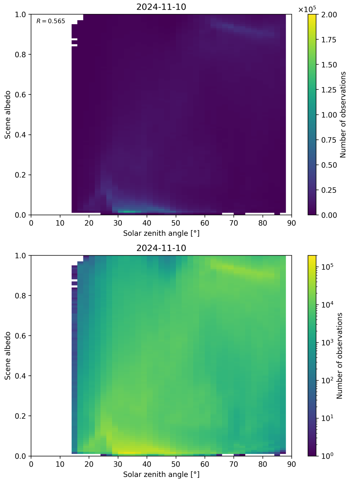
Figure 127: Scatter density plot of “Solar zenith angle” against “Scene albedo” for 2024-11-09 to 2024-11-11.
