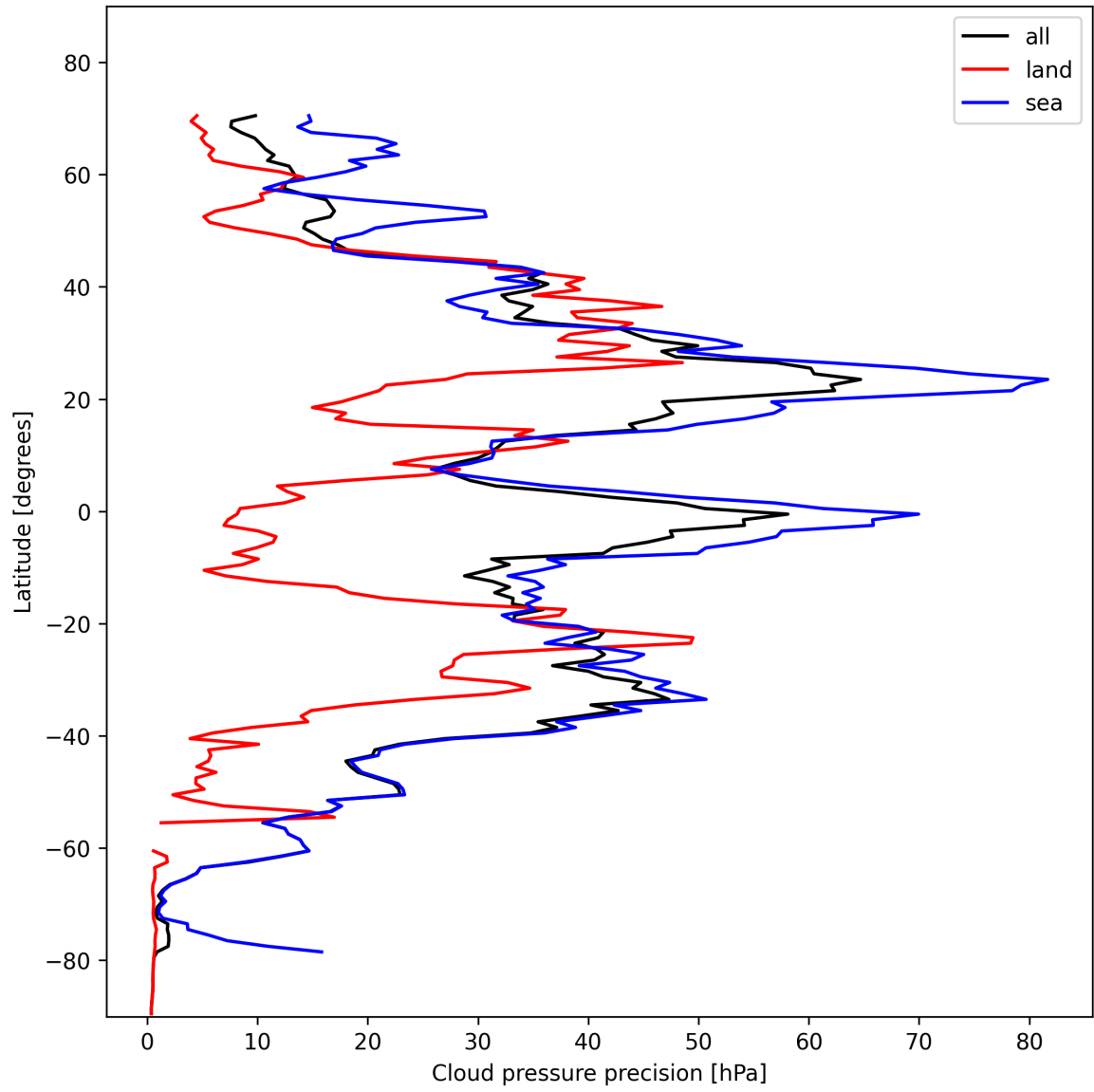
Figure 14: Zonal average of “Cloud pressure precision” for 2024-11-09 to 2024-11-11.
