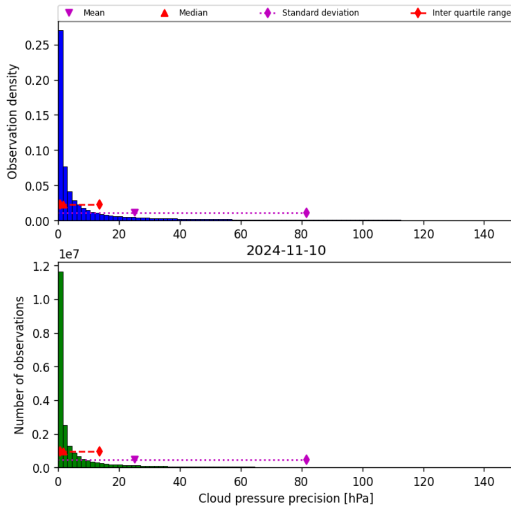
Figure 31: Histogram of “Cloud pressure precision” for 2024-11-09 to 2024-11-11
