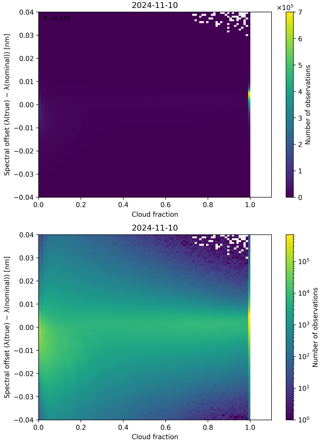
Figure 83: Scatter density plot of “Cloud fraction” against “Spectral offset ( \lambda_{\text{true}} - \lambda_{\text{nominal}} )” for 2024-11-09 to 2024-11-11.
