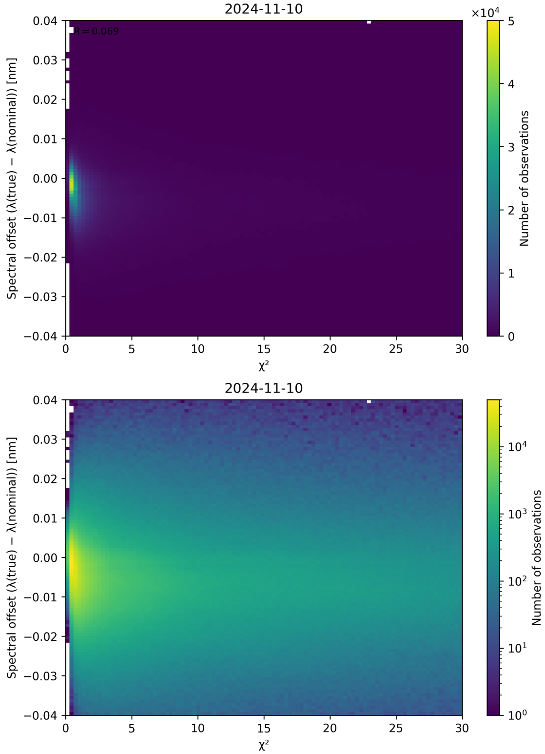
Figure 75: Scatter density plot of " \chi^2 " against "Spectral offset ( \lambda_{\text{true}} - \lambda_{\text{nominal}} )" for 2024-11-09 to 2024-11-11.
