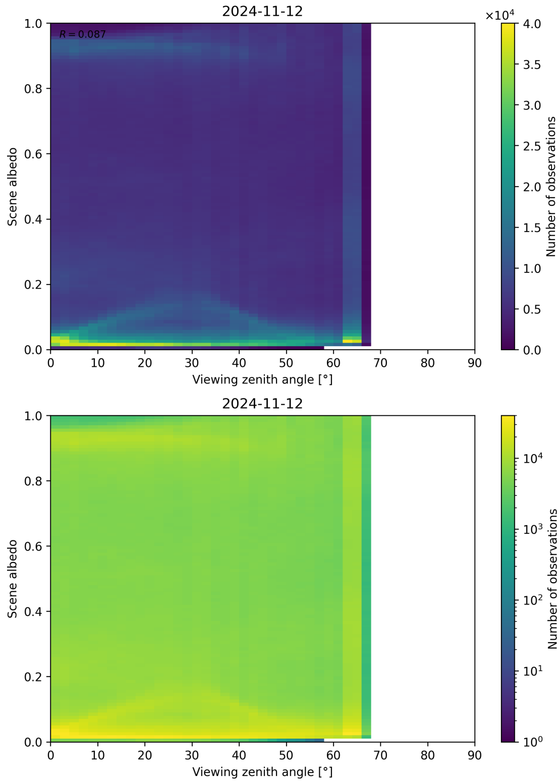
Figure 138: Scatter density plot of “Viewing zenith angle” against “Scene albedo” for 2024-11-11 to 2024-11-13.
