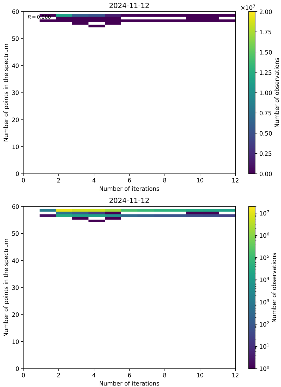
Figure 108: Scatter density plot of “Number of iterations” against “Number of points in the spectrum” for 2024-11-11 to 2024-11-13.
