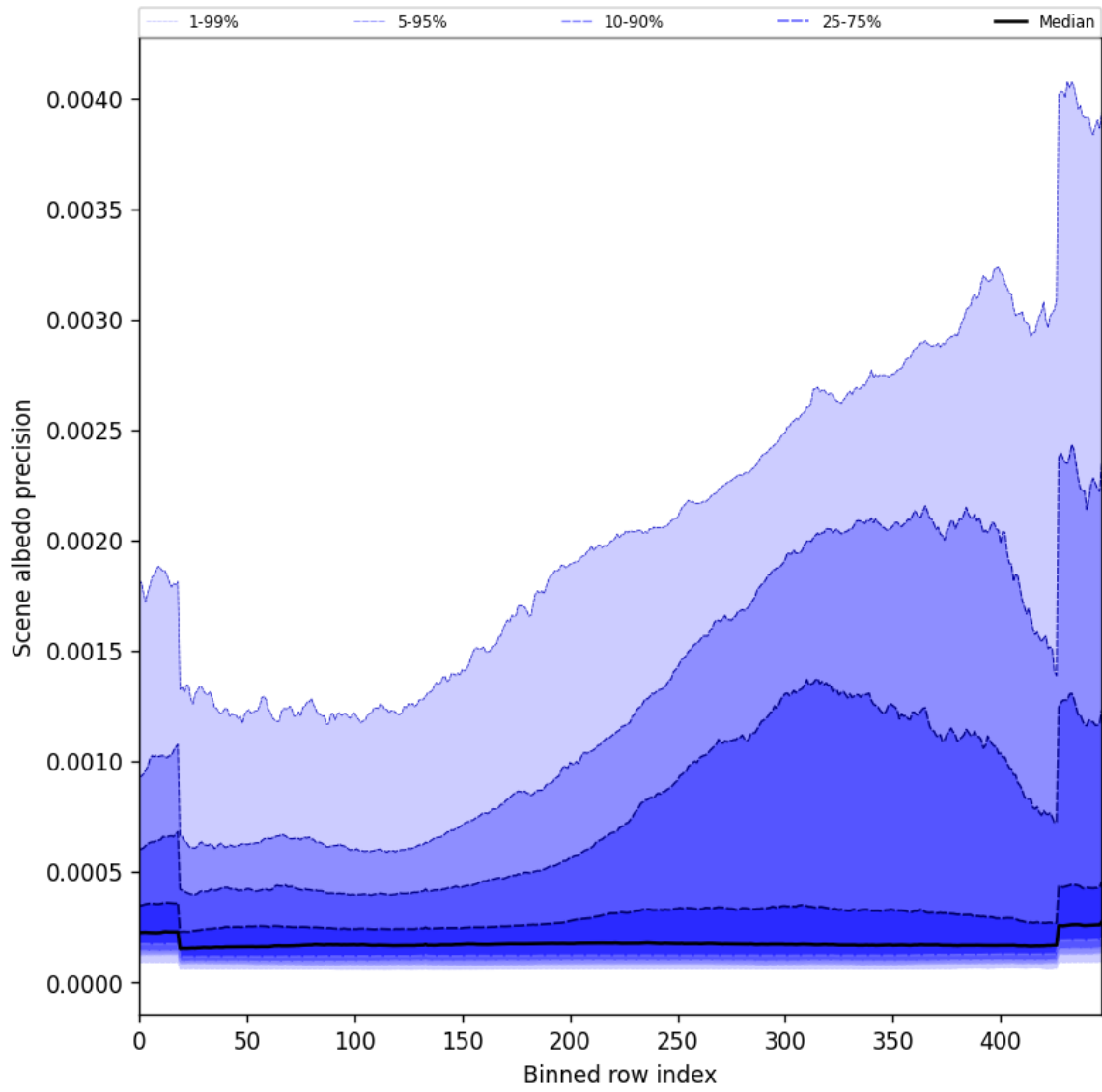
Figure 52: Along track statistics of “Scene albedo precision” for 2024-11-11 to 2024-11-13
