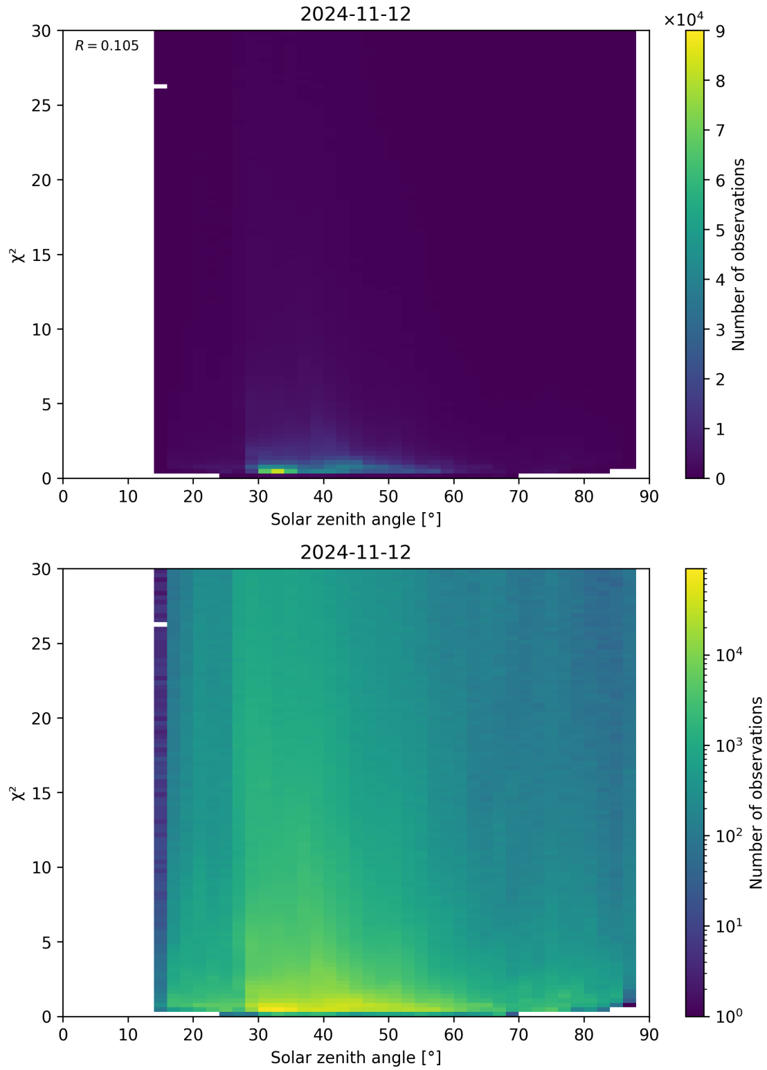
Figure 119: Scatter density plot of “Solar zenith angle” against “ \chi^2 ” for 2024-11-11 to 2024-11-13.
