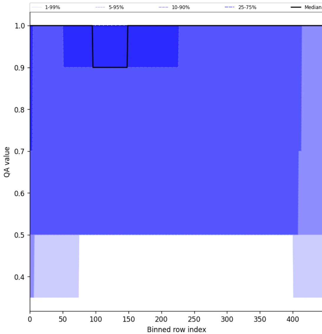
Figure 46: Along track statistics of “QA value” for 2024-11-11 to 2024-11-13
