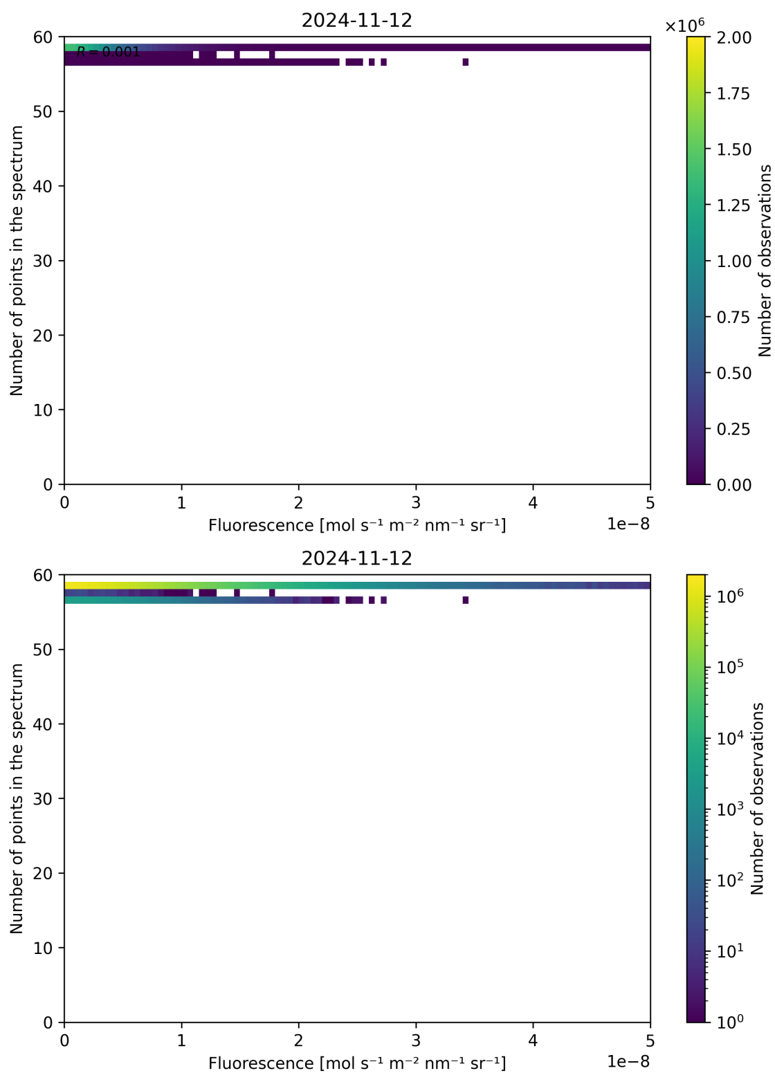
Figure 94: Scatter density plot of “Fluorescence” against “Number of points in the spectrum” for 2024-11-11 to 2024-11-13.
