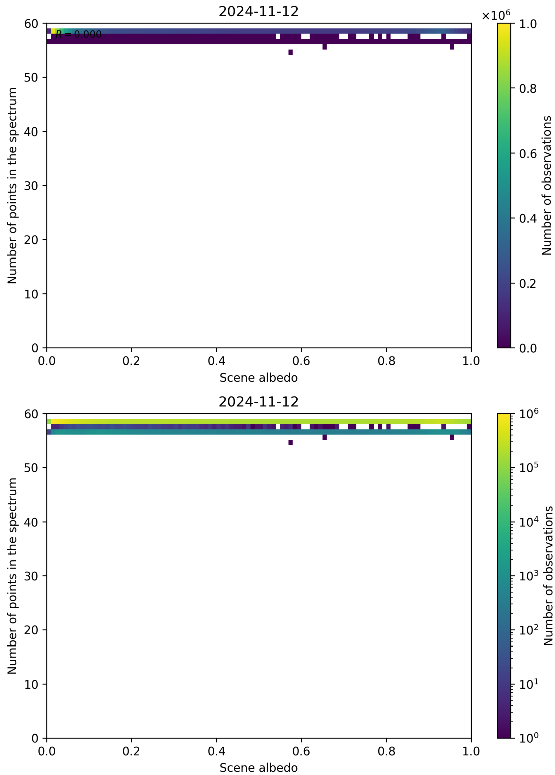
Figure 116: Scatter density plot of “Scene albedo” against “Number of points in the spectrum” for 2024-11-11 to 2024-11-13.
