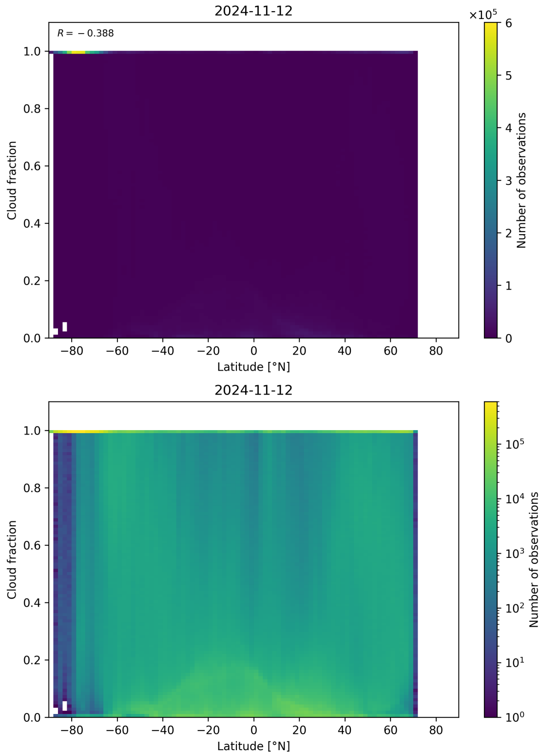
Figure 99: Scatter density plot of “Latitude” against “Cloud fraction” for 2024-11-11 to 2024-11-13.
