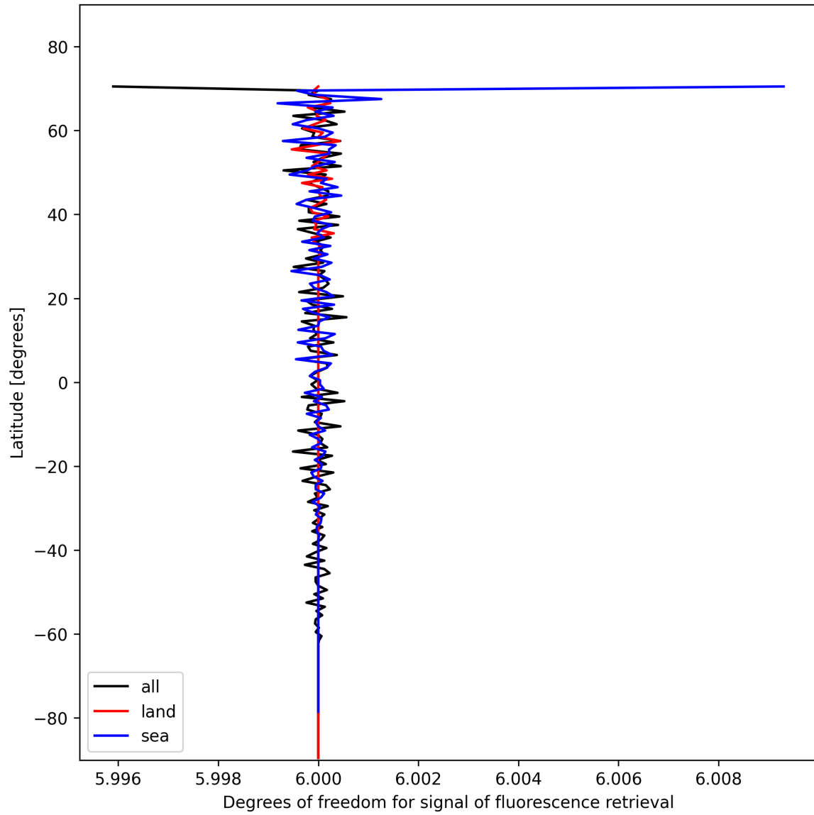
Figure 26: Zonal average of “Degrees of freedom for signal of fluorescence retrieval” for 2024-11-11 to 2024-11-13.
