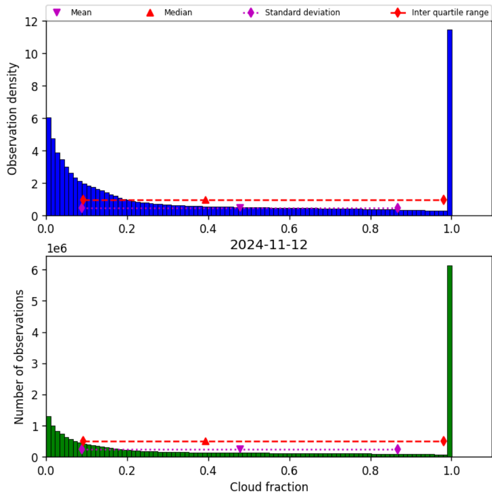
Figure 32: Histogram of “Cloud fraction” for 2024-11-11 to 2024-11-13
