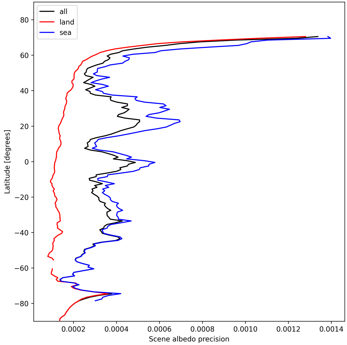
Figure 18: Zonal average of “Scene albedo precision” for 2024-11-11 to 2024-11-13.
