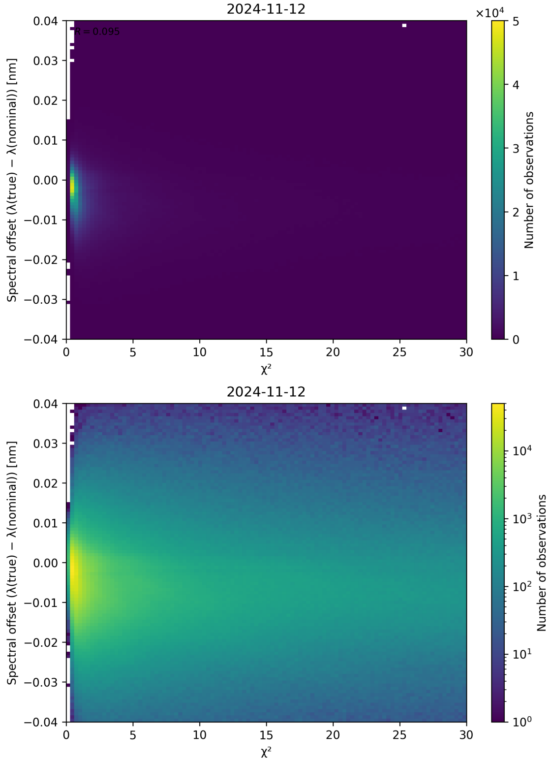
Figure 75: Scatter density plot of “ \chi^2 ” against “Spectral offset ( \lambda_{\text{true}} - \lambda_{\text{nominal}} )” for 2024-11-11 to 2024-11-13.
