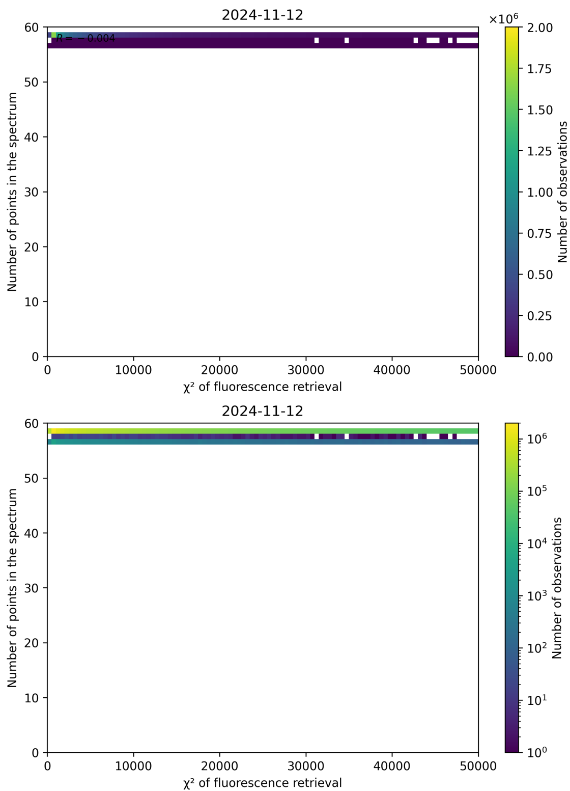
Figure 71: Scatter density plot of " \chi^2 of fluorescence retrieval" against "Number of points in the spectrum" for 2024-11-11 to 2024-11-13.
