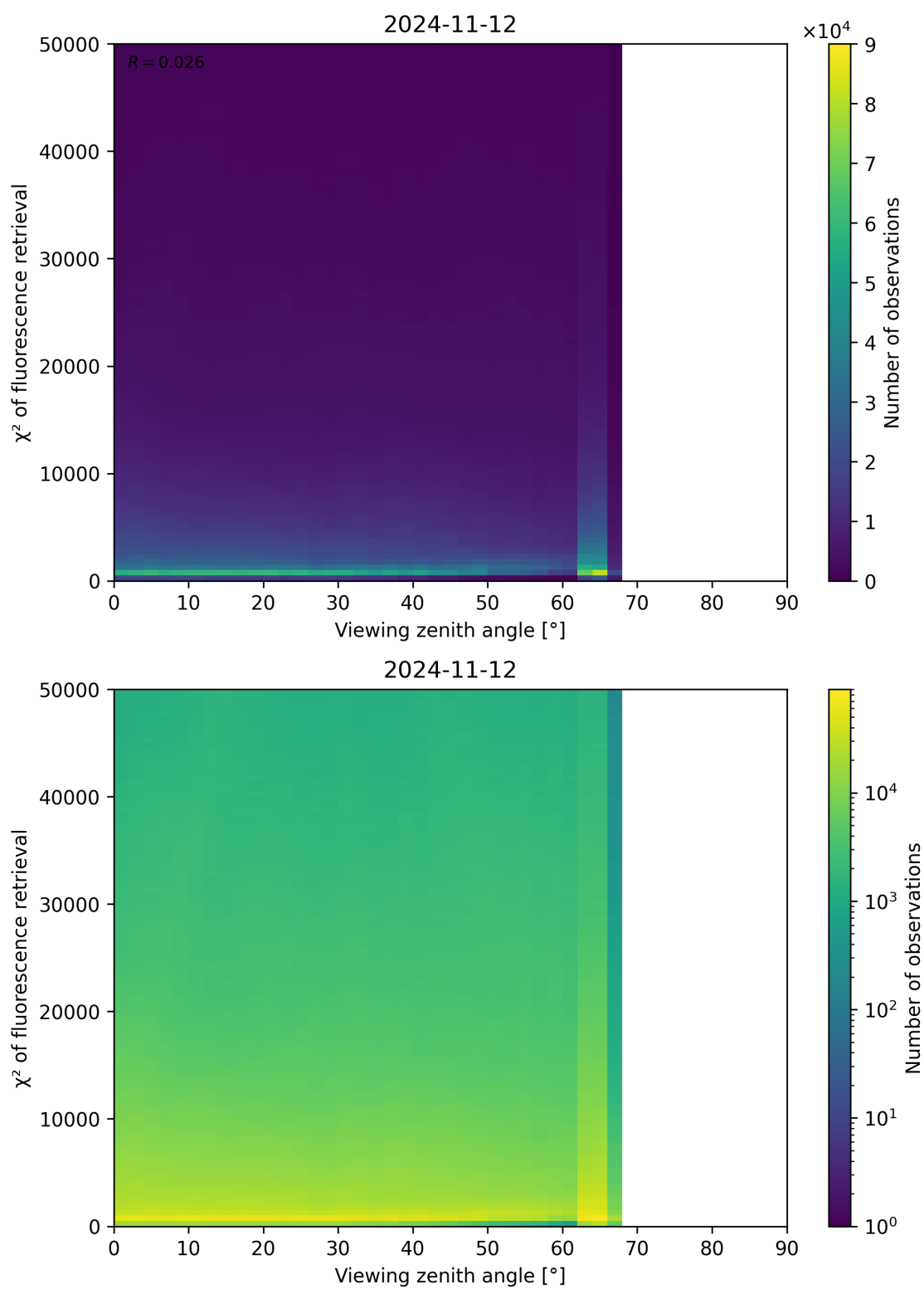
Figure 131: Scatter density plot of “Viewing zenith angle” against “ \chi^2 of fluorescence retrieval” for 2024-11-11 to 2024-11-13.
