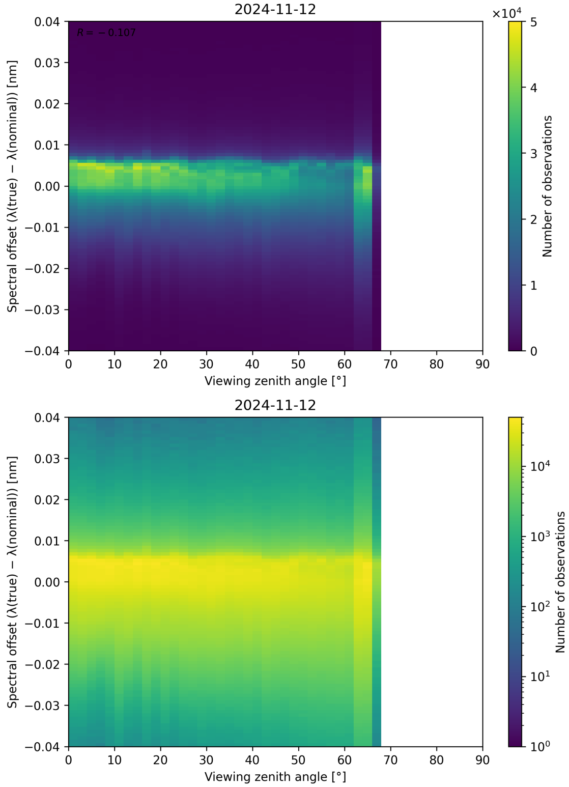
Figure 140: Scatter density plot of “Viewing zenith angle” against “Spectral offset ( \lambda_{\text{true}} - \lambda_{\text{nominal}} )” for 2024-11-11 to 2024-11-13.
