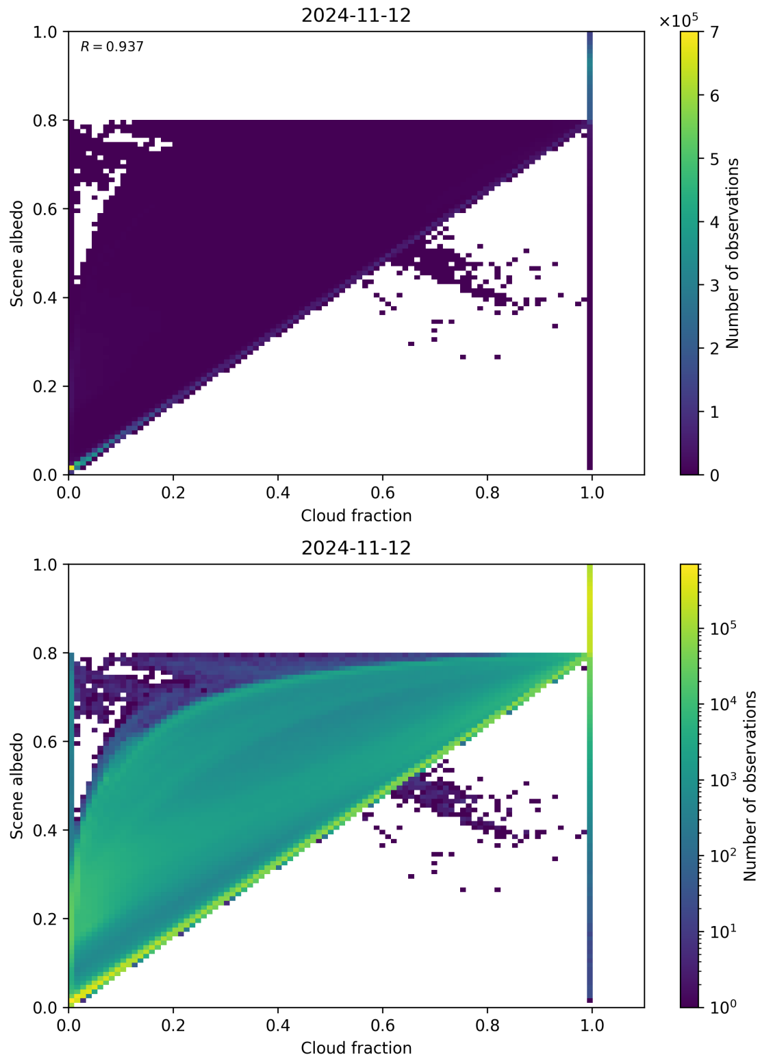
Figure 82: Scatter density plot of “Cloud fraction” against “Scene albedo” for 2024-11-11 to 2024-11-13.
