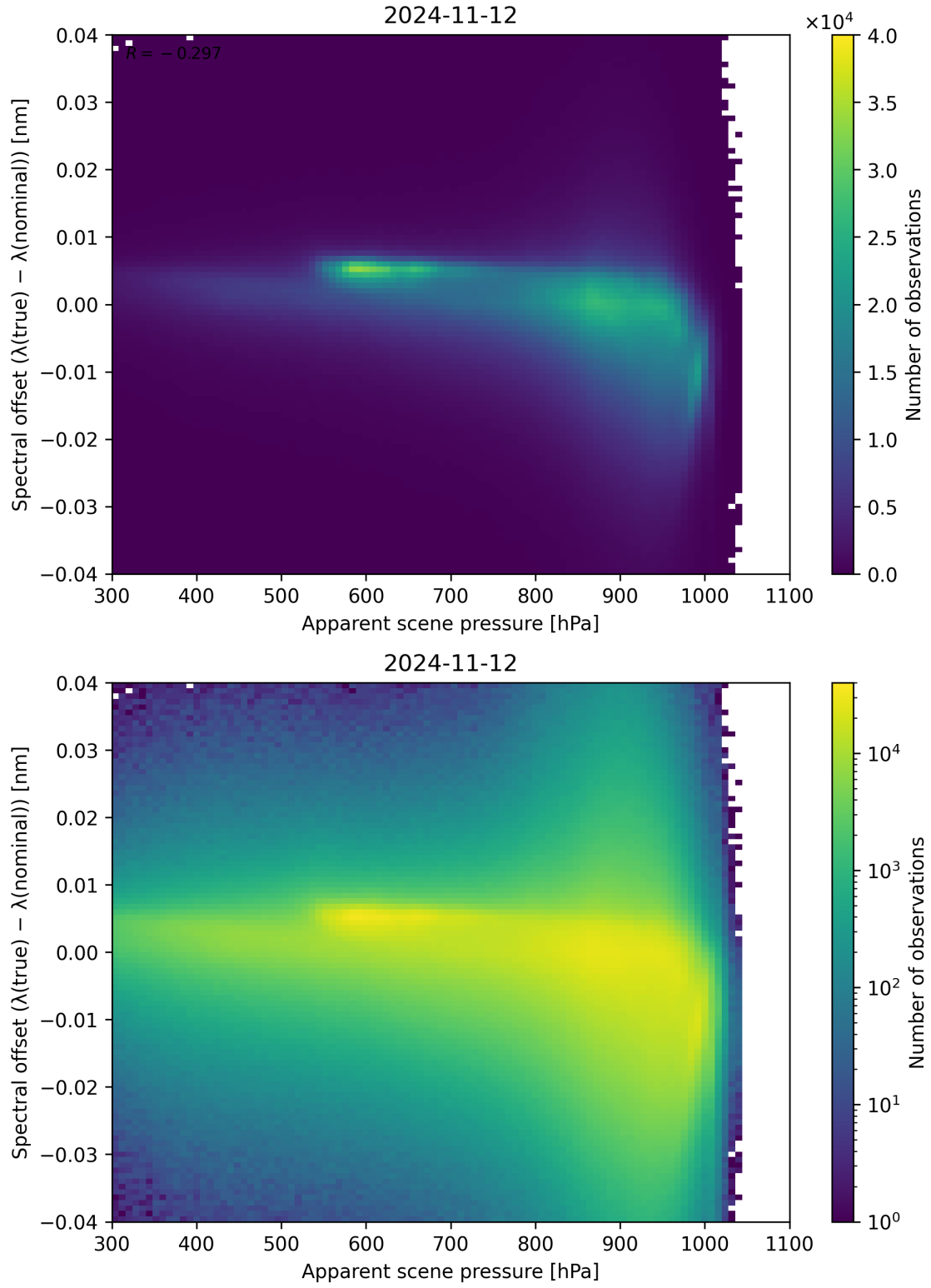
Figure 68: Scatter density plot of “Apparent scene pressure” against “Spectral offset ( \lambda_{\text{true}} - \lambda_{\text{nominal}} )” for 2024-11-11 to 2024-11-13.
