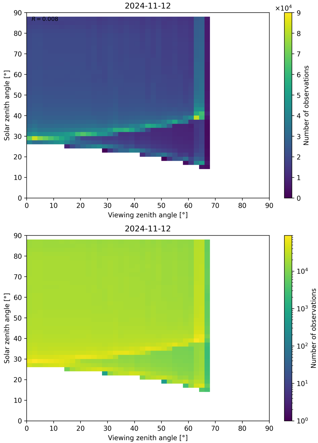
Figure 139: Scatter density plot of “Viewing zenith angle” against “Solar zenith angle” for 2024-11-11 to 2024-11-13.
