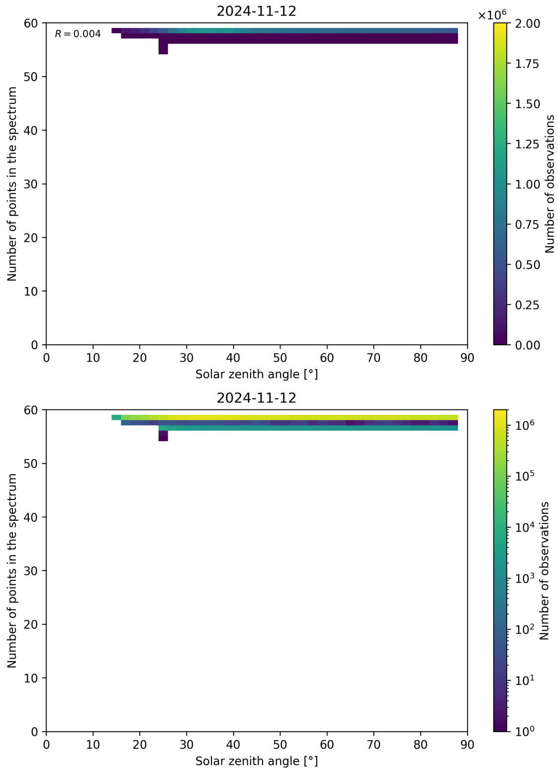
Figure 126: Scatter density plot of “Solar zenith angle” against “Number of points in the spectrum” for 2024-11-11 to 2024-11-13.
