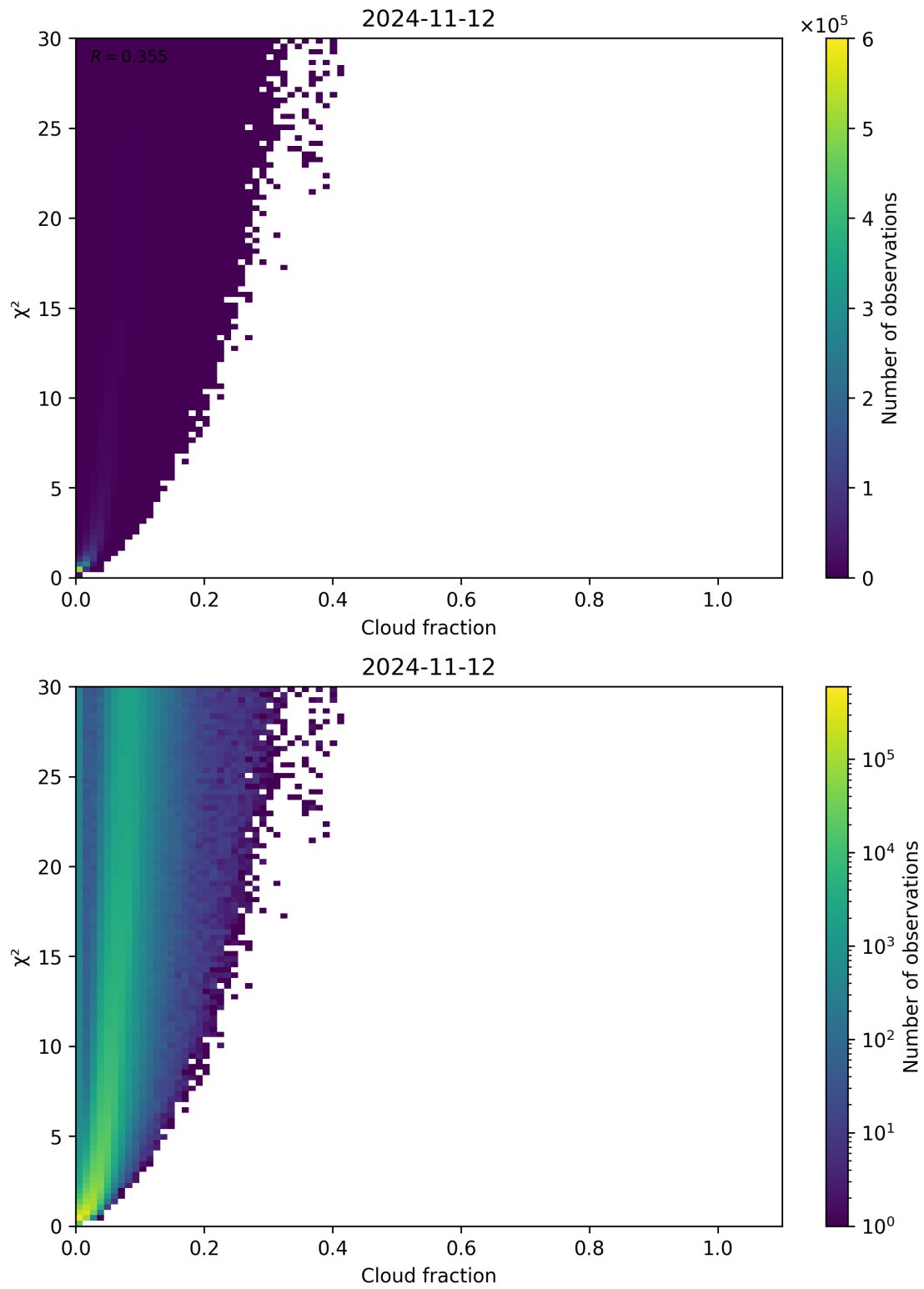
Figure 77: Scatter density plot of “Cloud fraction” against “ \chi^2 ” for 2024-11-11 to 2024-11-13.
