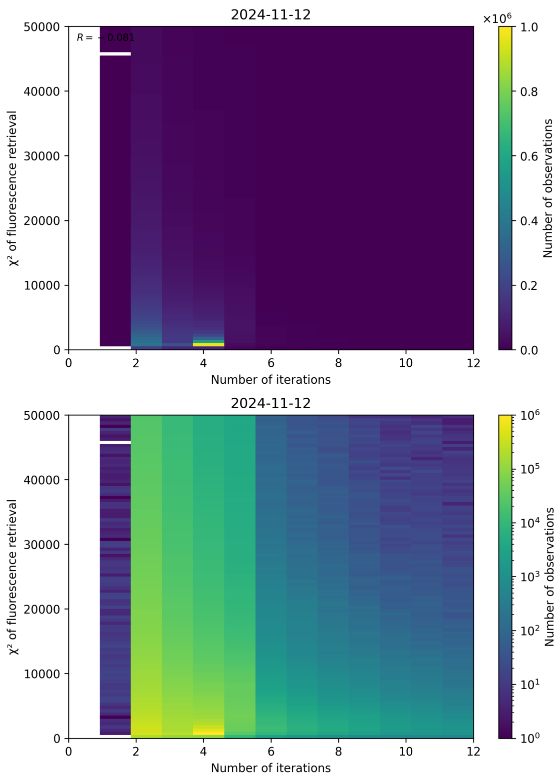
Figure 106: Scatter density plot of “Number of iterations” against “ \chi^2 of fluorescence retrieval” for 2024-11-11 to 2024-11-13.
