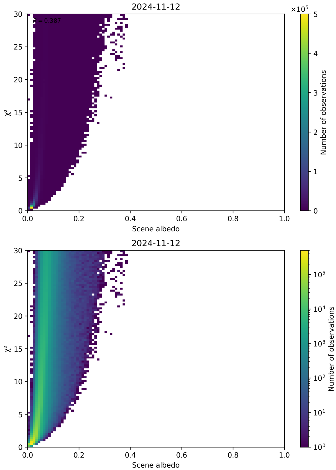
Figure 112: Scatter density plot of “Scene albedo” against “ \chi^2 ” for 2024-11-11 to 2024-11-13.
