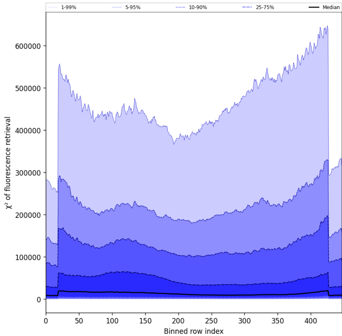
Figure 59: Along track statistics of “ \chi^2 of fluorescence retrieval” for 2024-11-11 to 2024-11-13
