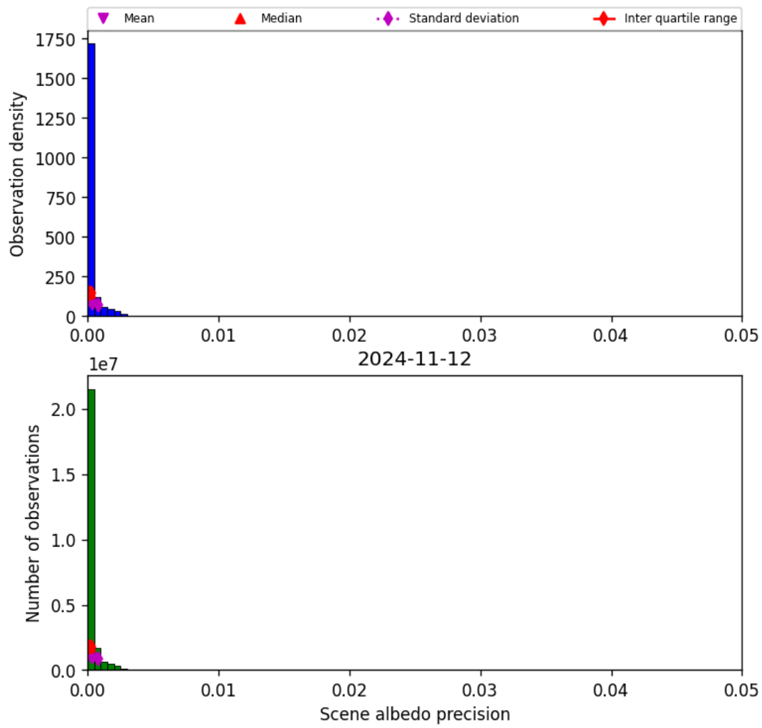
Figure 35: Histogram of “Scene albedo precision” for 2024-11-11 to 2024-11-13
