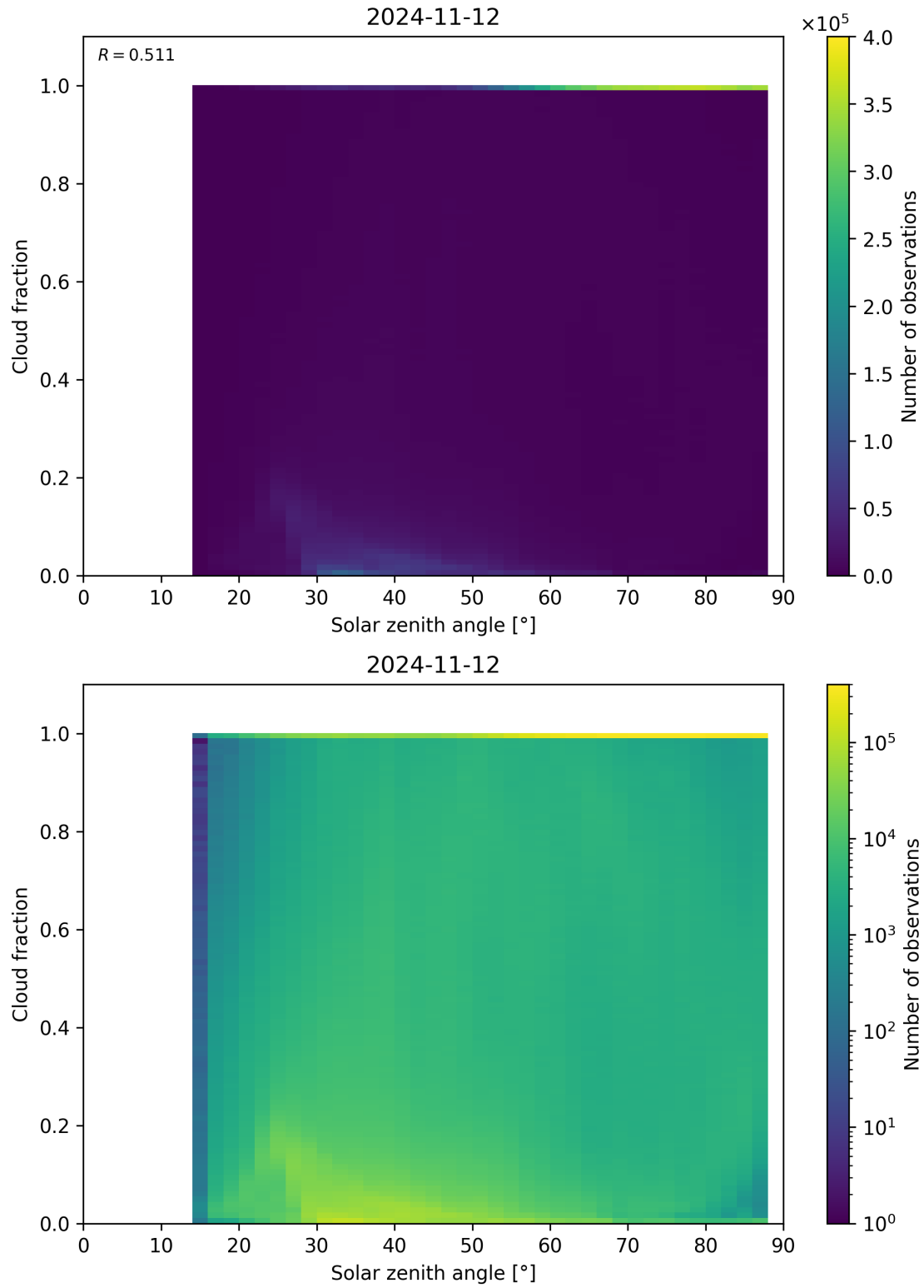
Figure 121: Scatter density plot of “Solar zenith angle” against “Cloud fraction” for 2024-11-11 to 2024-11-13.
