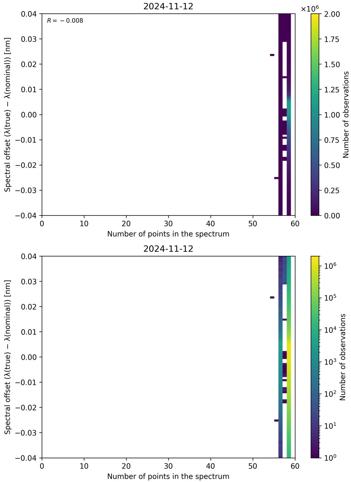
Figure 110: Scatter density plot of “Number of points in the spectrum” against “Spectral offset ( \lambda_{\text{true}} - \lambda_{\text{nominal}} )” for 2024-11-11 to 2024-11-13.
