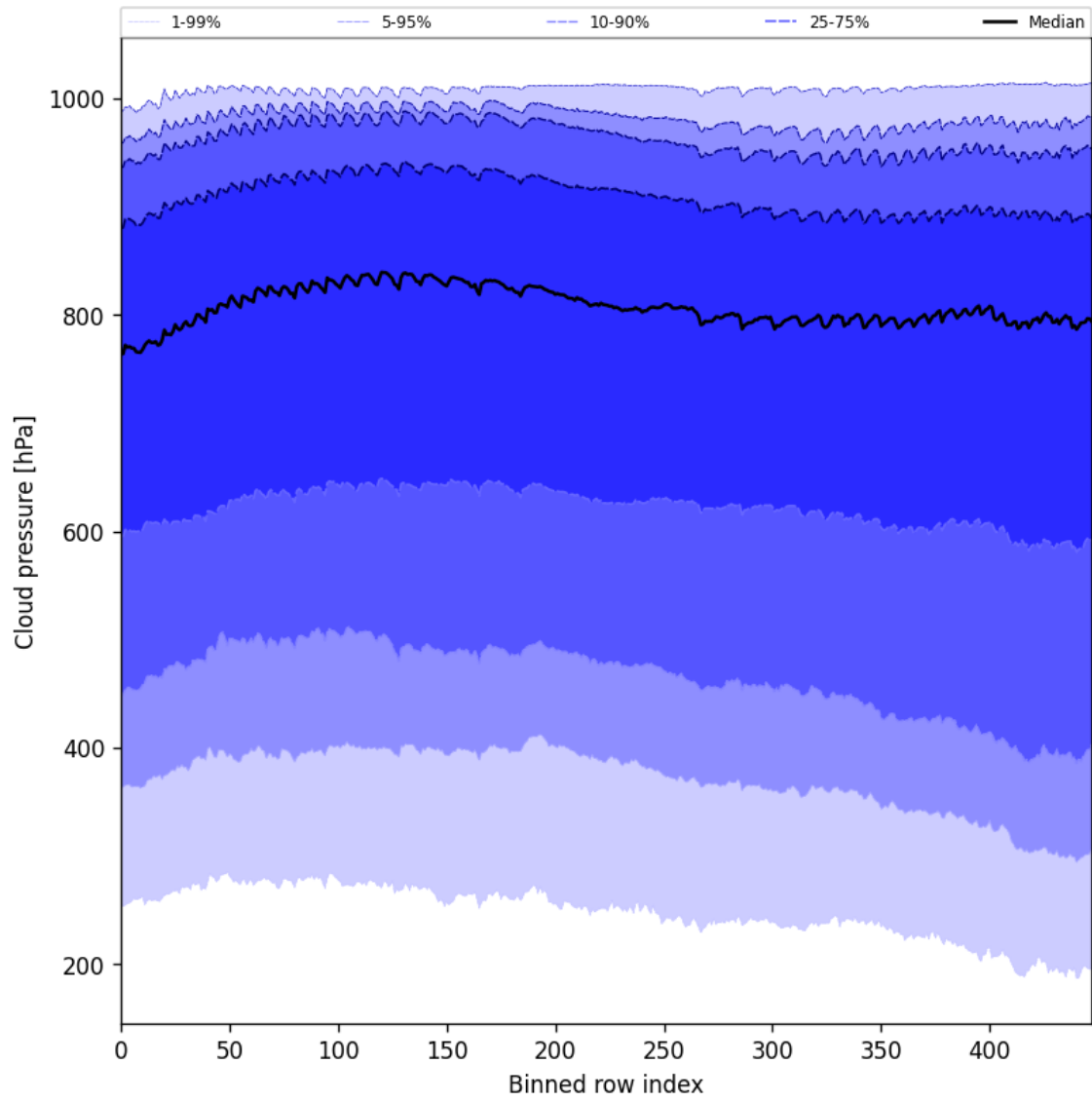
Figure 47: Along track statistics of “Cloud pressure” for 2024-11-11 to 2024-11-13
