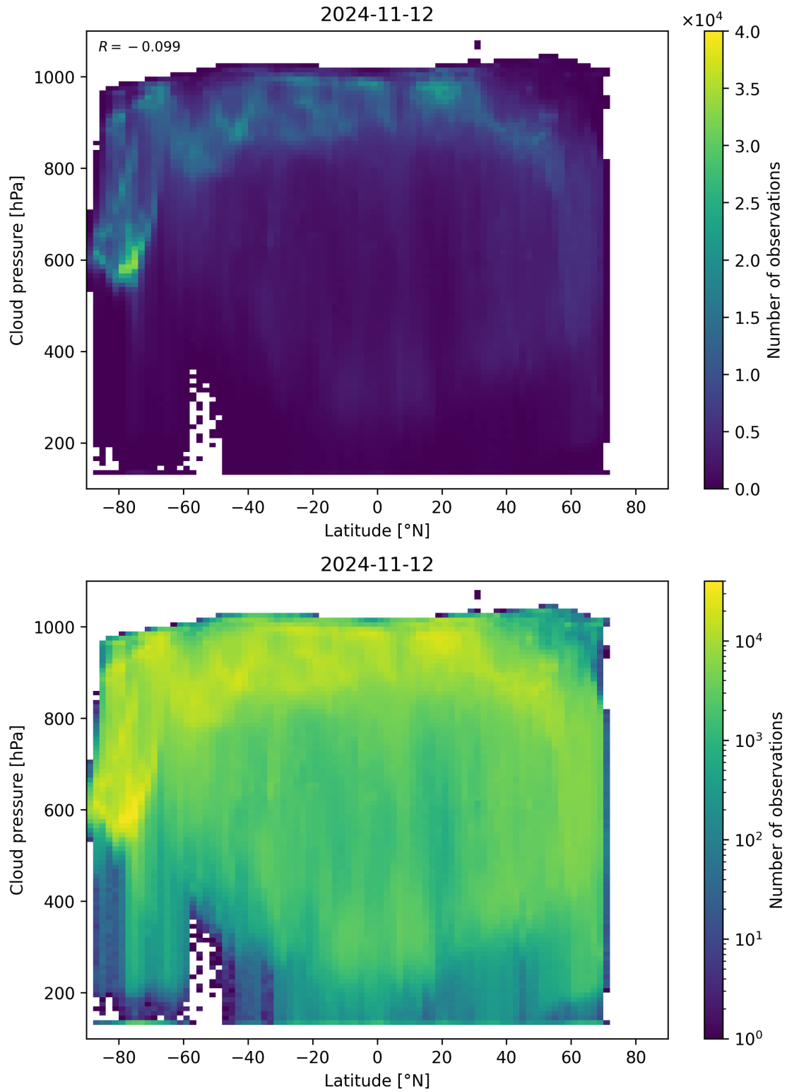
Figure 100: Scatter density plot of “Latitude” against “Cloud pressure” for 2024-11-11 to 2024-11-13.
