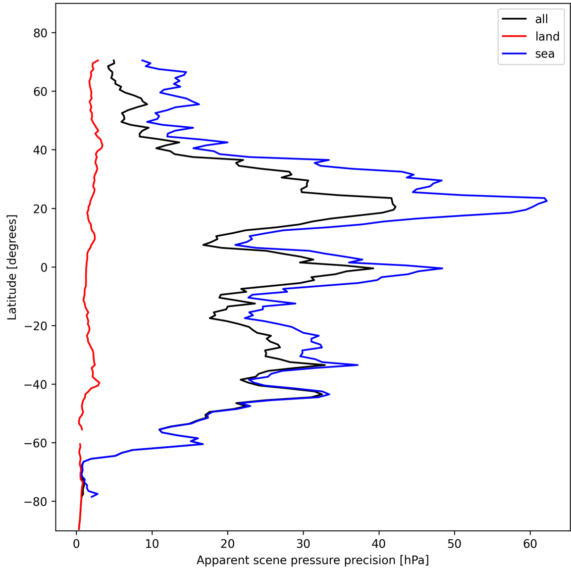
Figure 20: Zonal average of “Apparent scene pressure precision” for 2024-11-11 to 2024-11-13.
