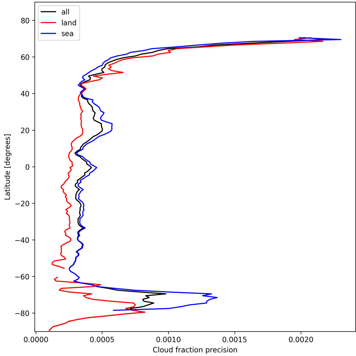
Figure 16: Zonal average of “Cloud fraction precision” for 2024-11-11 to 2024-11-13.
