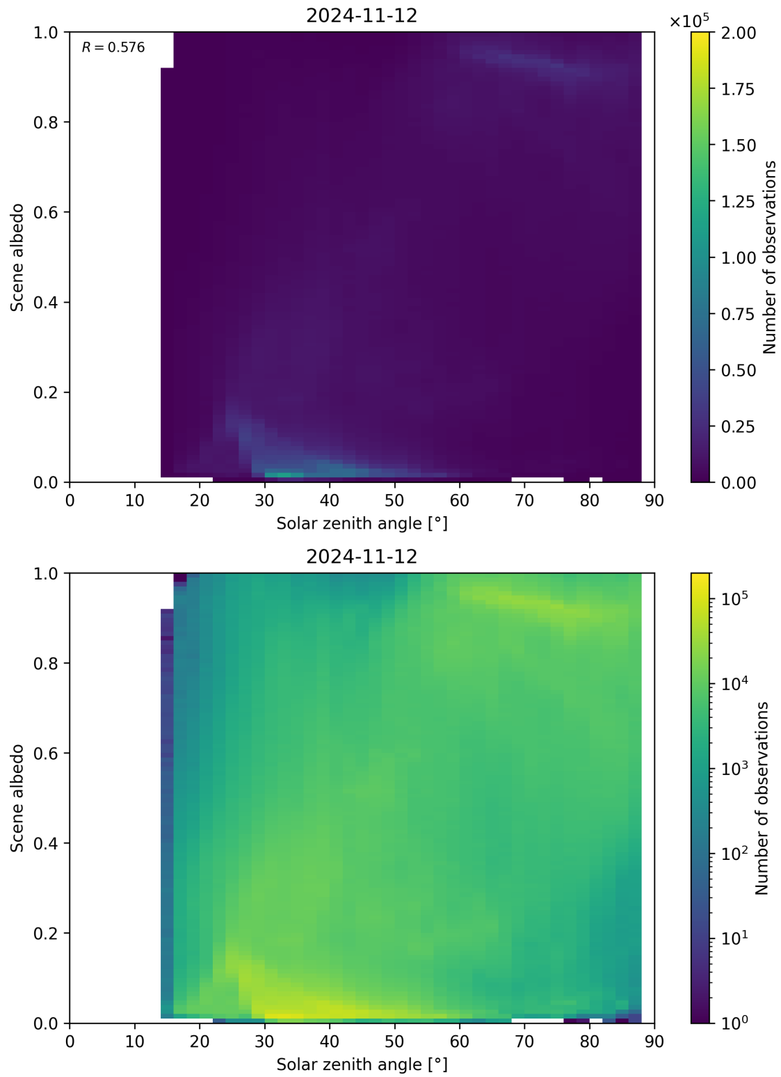
Figure 127: Scatter density plot of “Solar zenith angle” against “Scene albedo” for 2024-11-11 to 2024-11-13.
