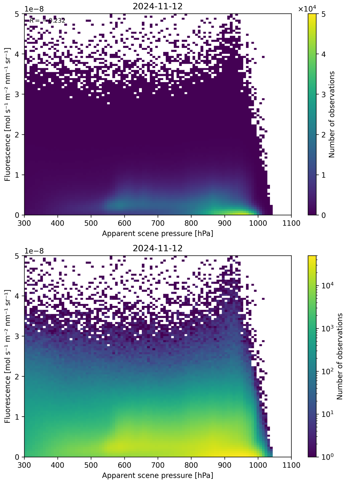
Figure 65: Scatter density plot of “Apparent scene pressure” against “Fluorescence” for 2024-11-11 to 2024-11-13.
