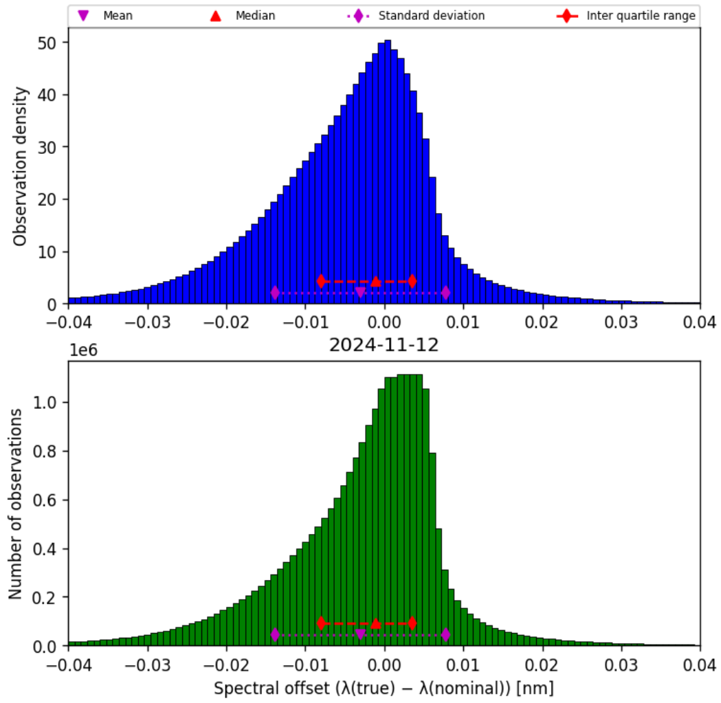
Figure 45: Histogram of “Spectral offset ( \lambda_{\text{true}} - \lambda_{\text{nominal}} )” for 2024-11-11 to 2024-11-13
