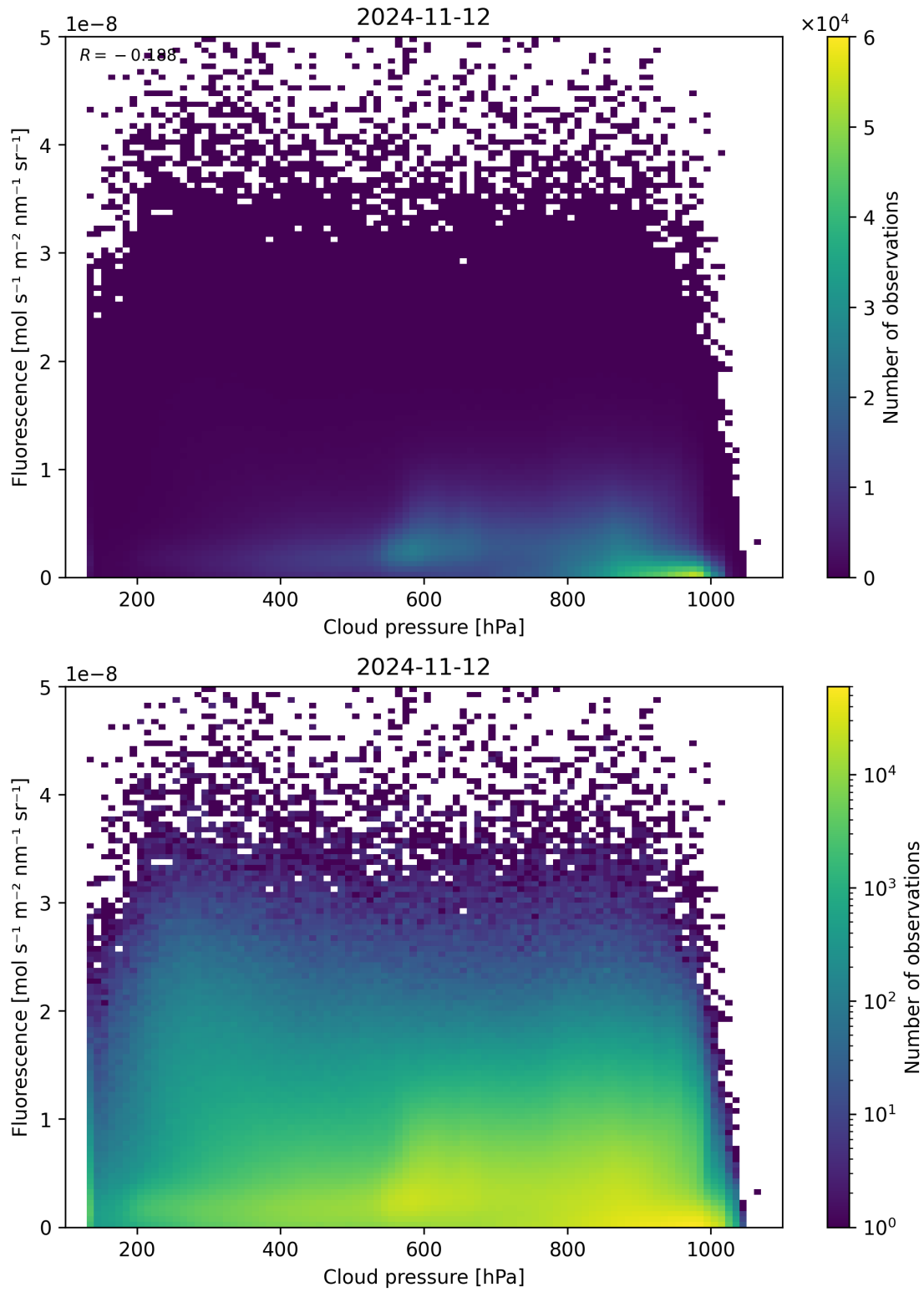
Figure 88: Scatter density plot of “Cloud pressure” against “Fluorescence” for 2024-11-11 to 2024-11-13.
