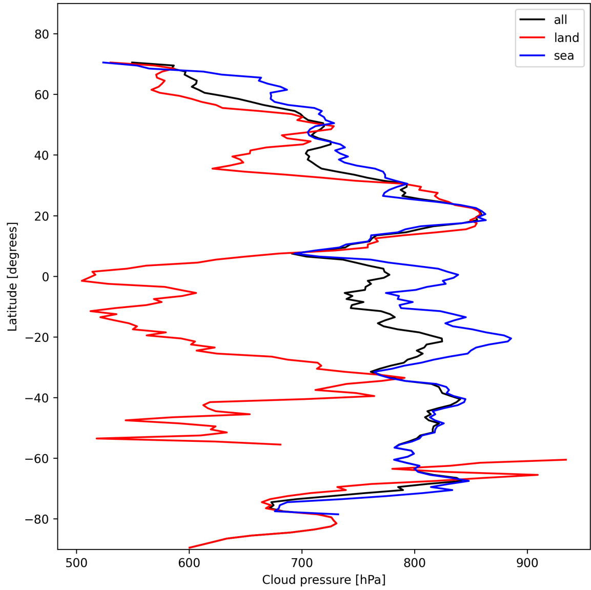
Figure 13: Zonal average of “Cloud pressure” for 2024-11-11 to 2024-11-13.
