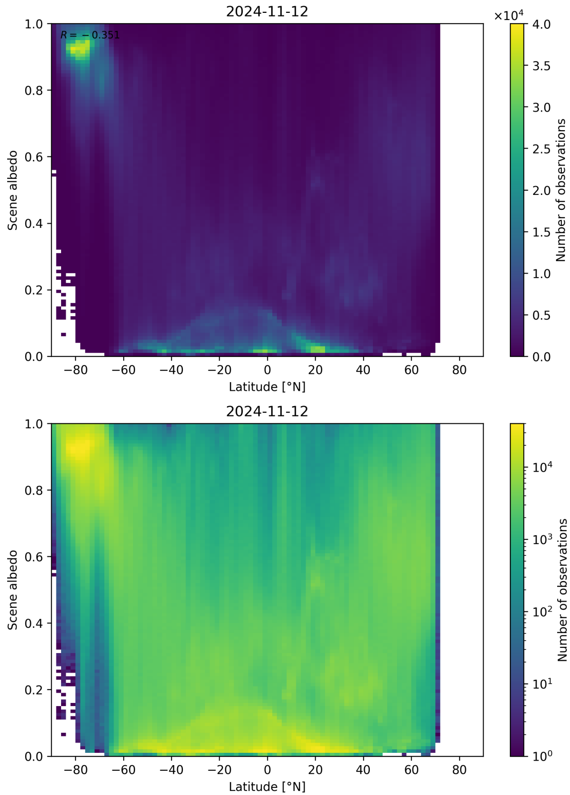
Figure 104: Scatter density plot of “Latitude” against “Scene albedo” for 2024-11-11 to 2024-11-13.
