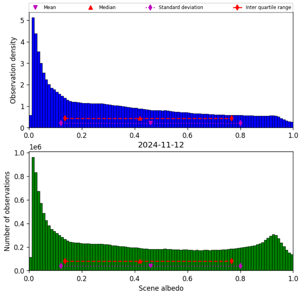
Figure 34: Histogram of “Scene albedo” for 2024-11-11 to 2024-11-13
