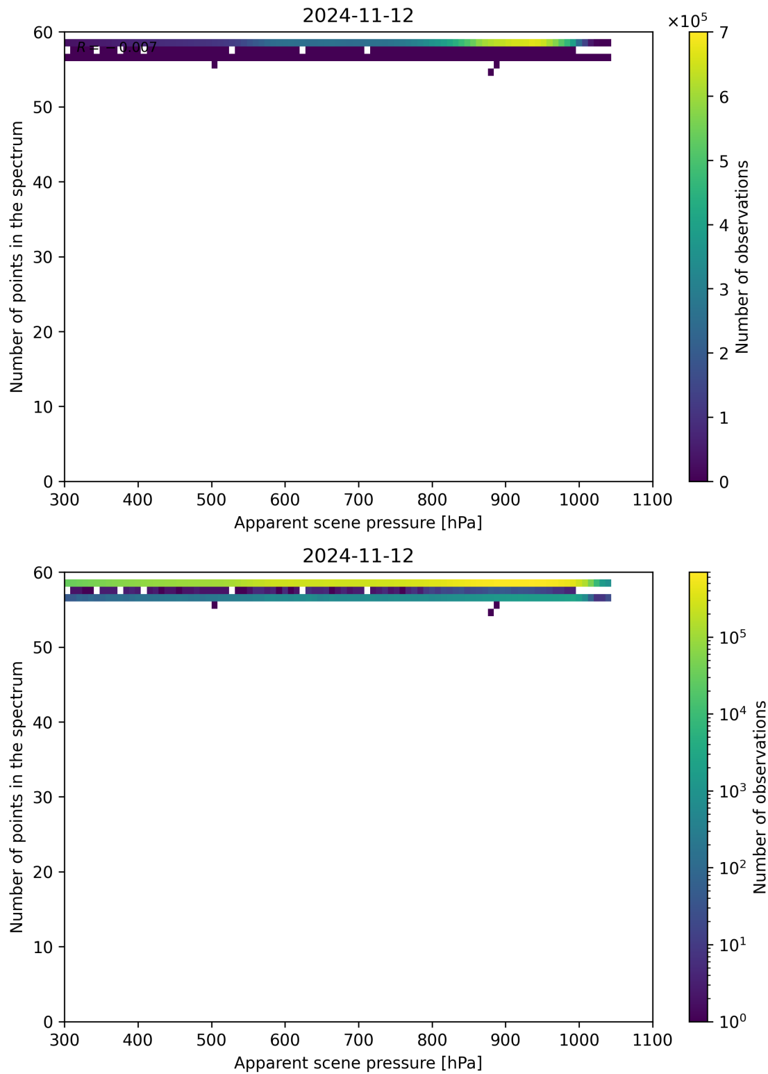
Figure 67: Scatter density plot of “Apparent scene pressure” against “Number of points in the spectrum” for 2024-11-11 to 2024-11-13.
