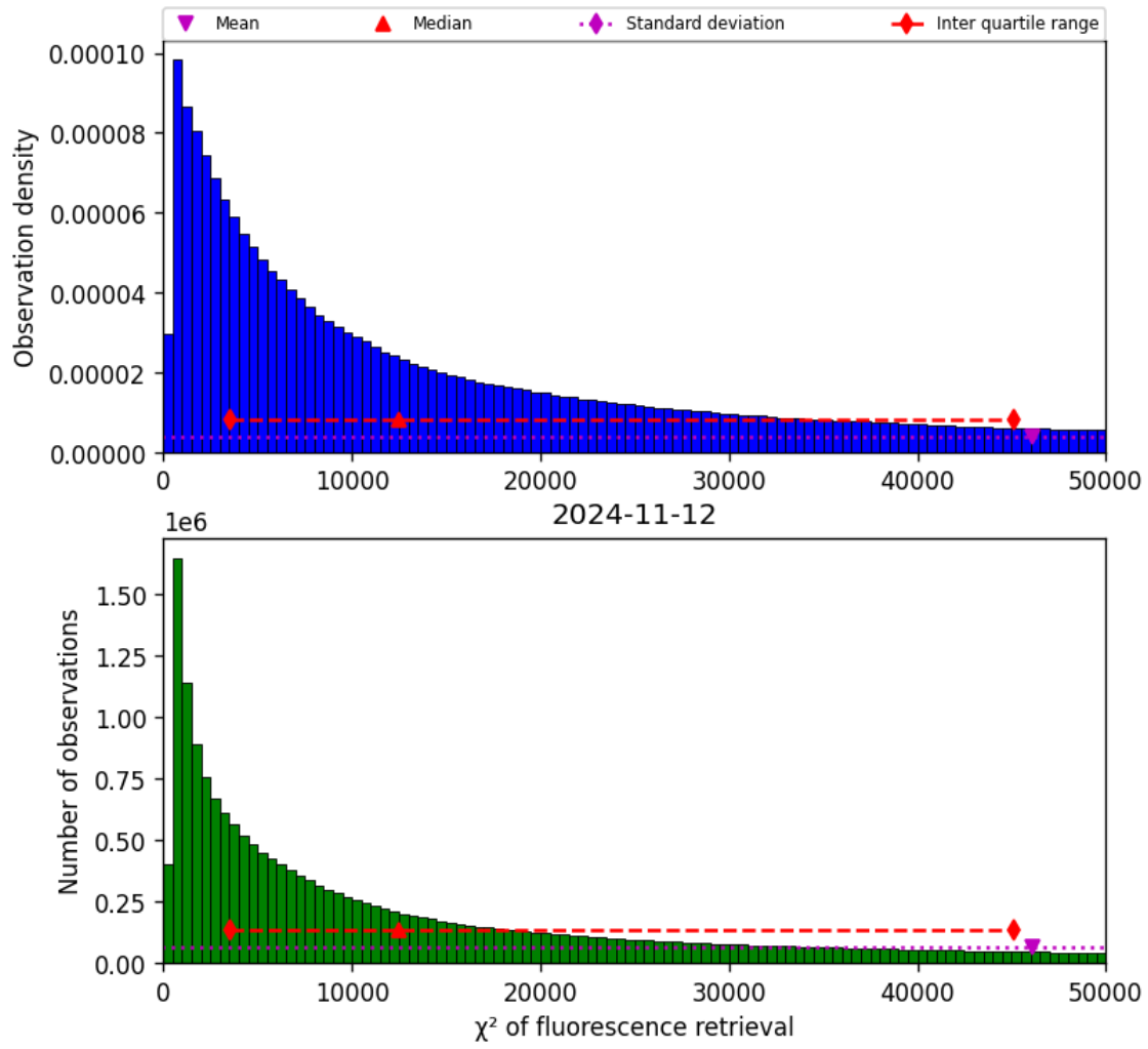
Figure 42: Histogram of “ \chi^2 of fluorescence retrieval” for 2024-11-11 to 2024-11-13
