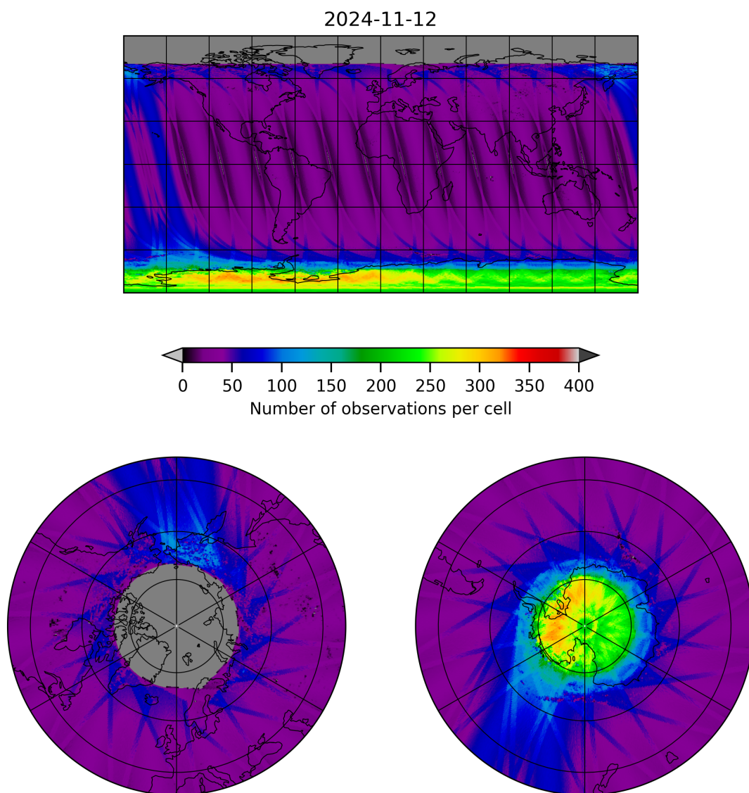
Figure 11: Map of the number of observations for 2024-11-11 to 2024-11-13
