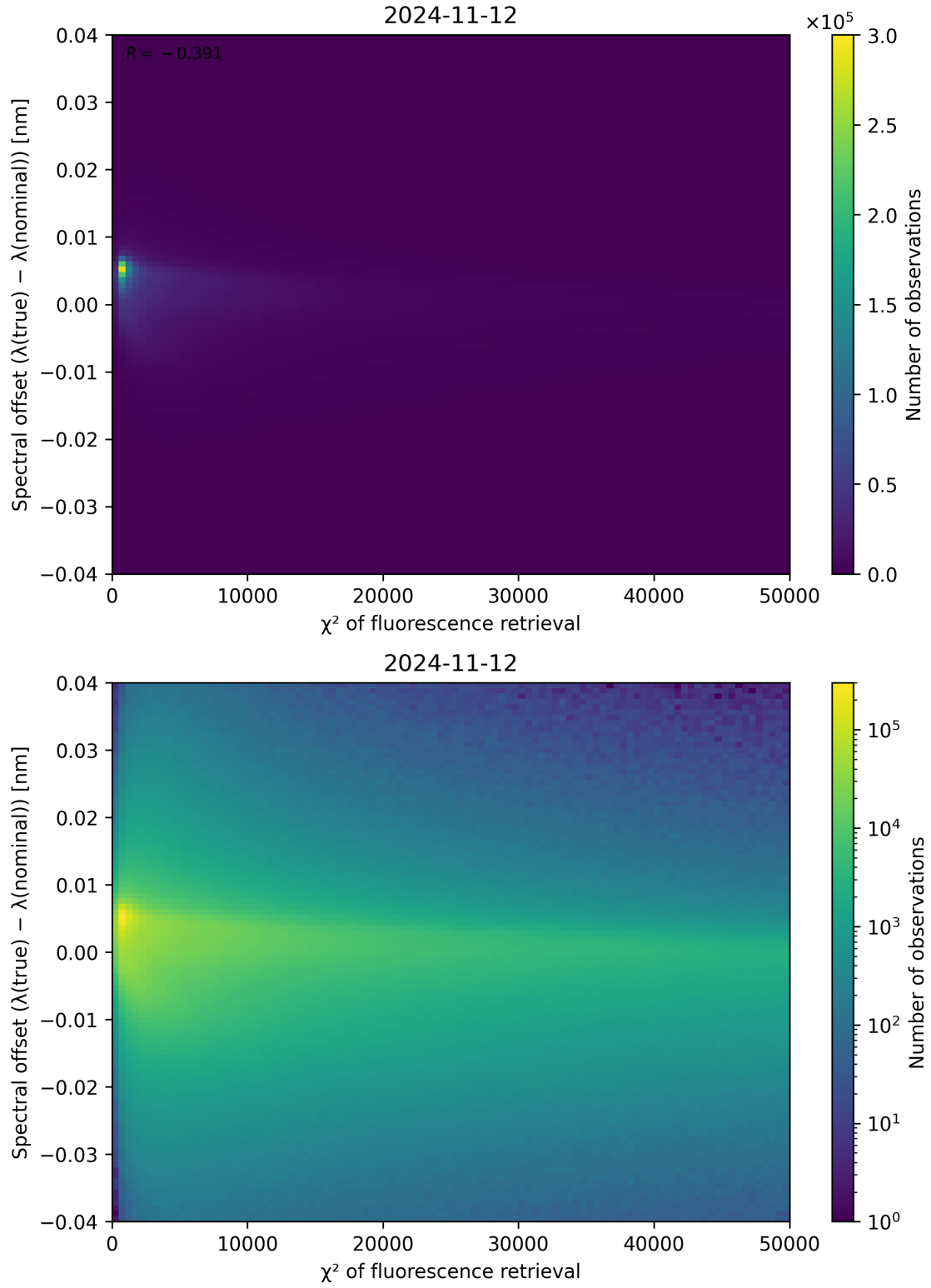
Figure 72: Scatter density plot of “ \chi^2 of fluorescence retrieval” against “Spectral offset ( \lambda_{\text{true}} - \lambda_{\text{nominal}} )” for 2024-11-11 to 2024-11-13.
