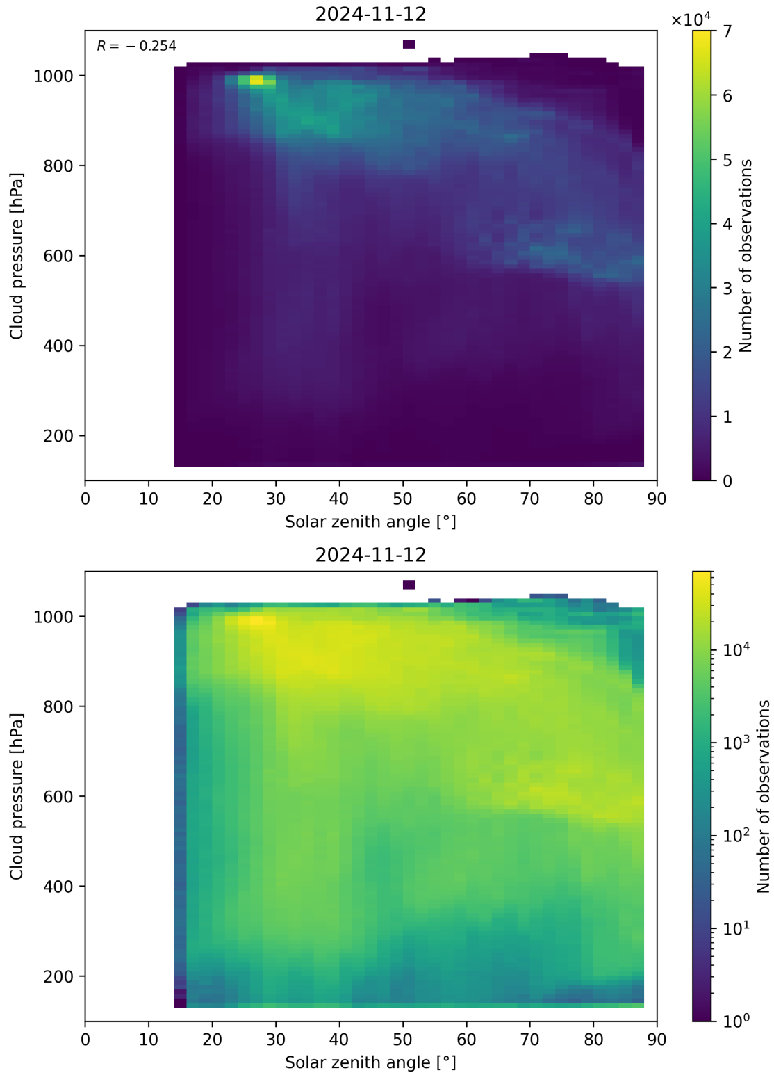
Figure 122: Scatter density plot of “Solar zenith angle” against “Cloud pressure” for 2024-11-11 to 2024-11-13.
