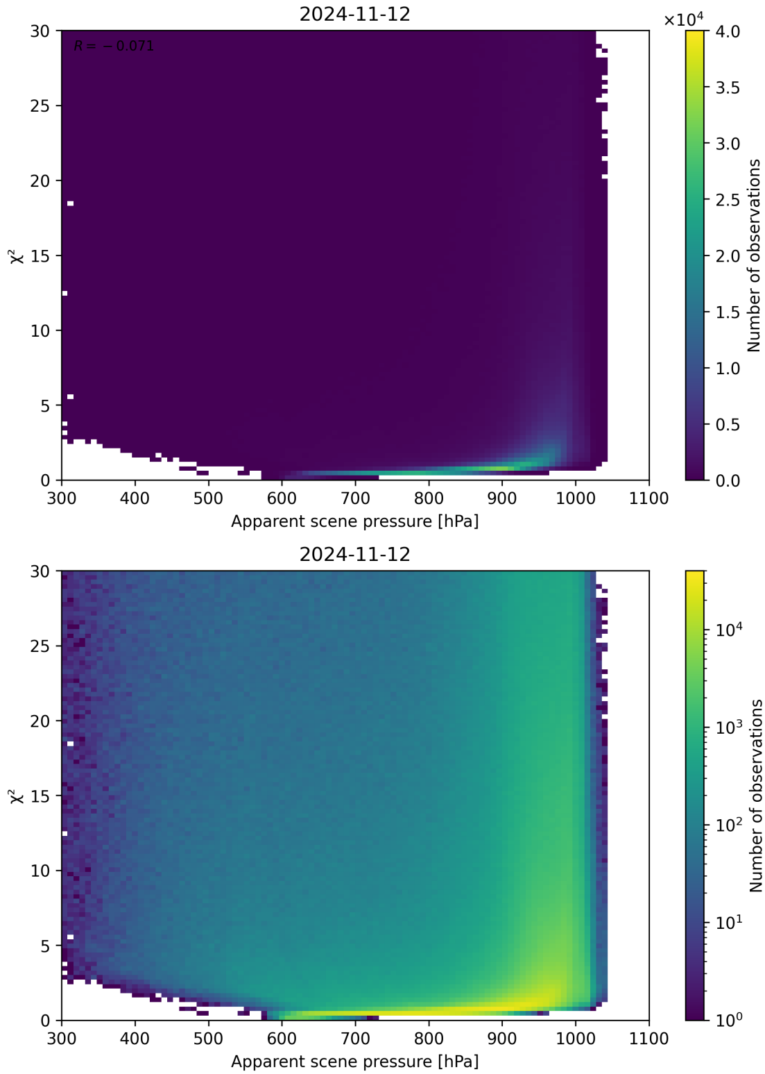
Figure 63: Scatter density plot of “Apparent scene pressure” against “ \chi^2 ” for 2024-11-11 to 2024-11-13.
