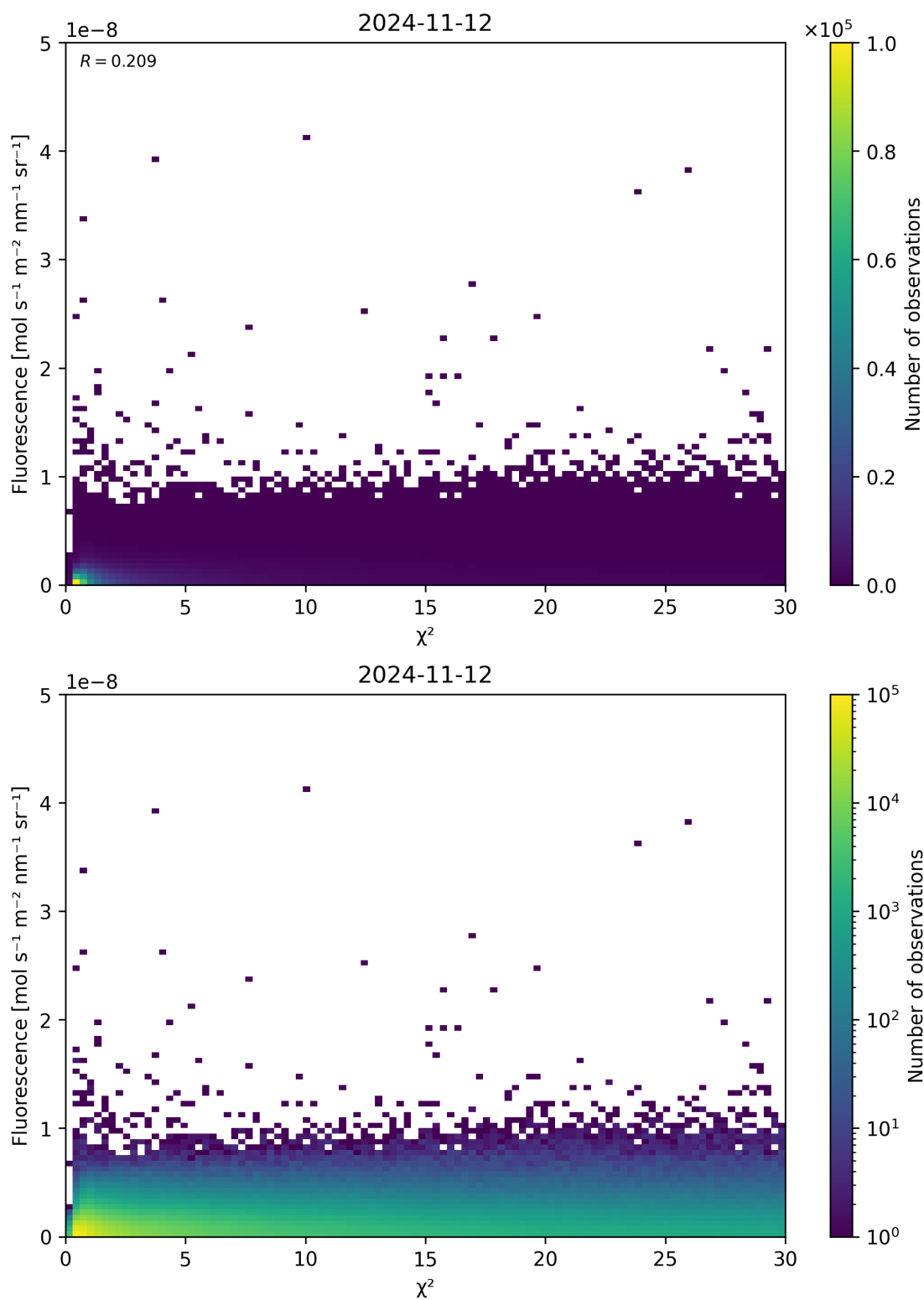
Figure 70: Scatter density plot of “ \chi^2 ” against “Fluorescence” for 2024-11-11 to 2024-11-13.
