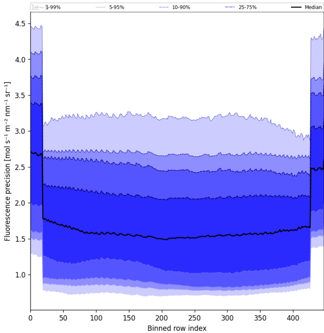
Figure 58: Along track statistics of “Fluorescence precision” for 2024-11-11 to 2024-11-13
