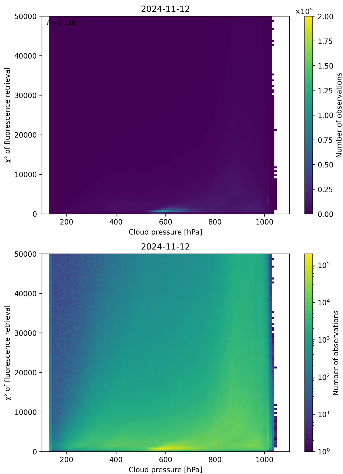
Figure 86: Scatter density plot of “Cloud pressure” against “ \chi^2 of fluorescence retrieval” for 2024-11-11 to 2024-11-13.
