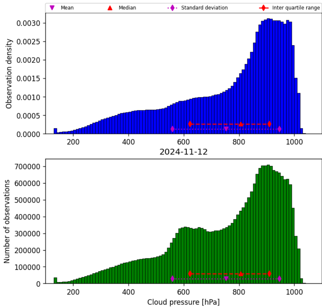
Figure 30: Histogram of “Cloud pressure” for 2024-11-11 to 2024-11-13
