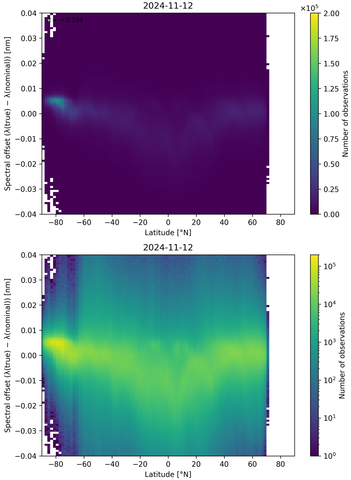
Figure 105: Scatter density plot of “Latitude” against “Spectral offset ( \lambda_{\text{true}} - \lambda_{\text{nominal}} )” for 2024-11-11 to 2024-11-13.
