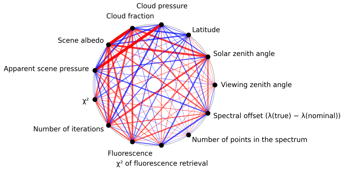
Figure 1: Map of correlation graph for 2024-11-11 to 2024-11-13.
