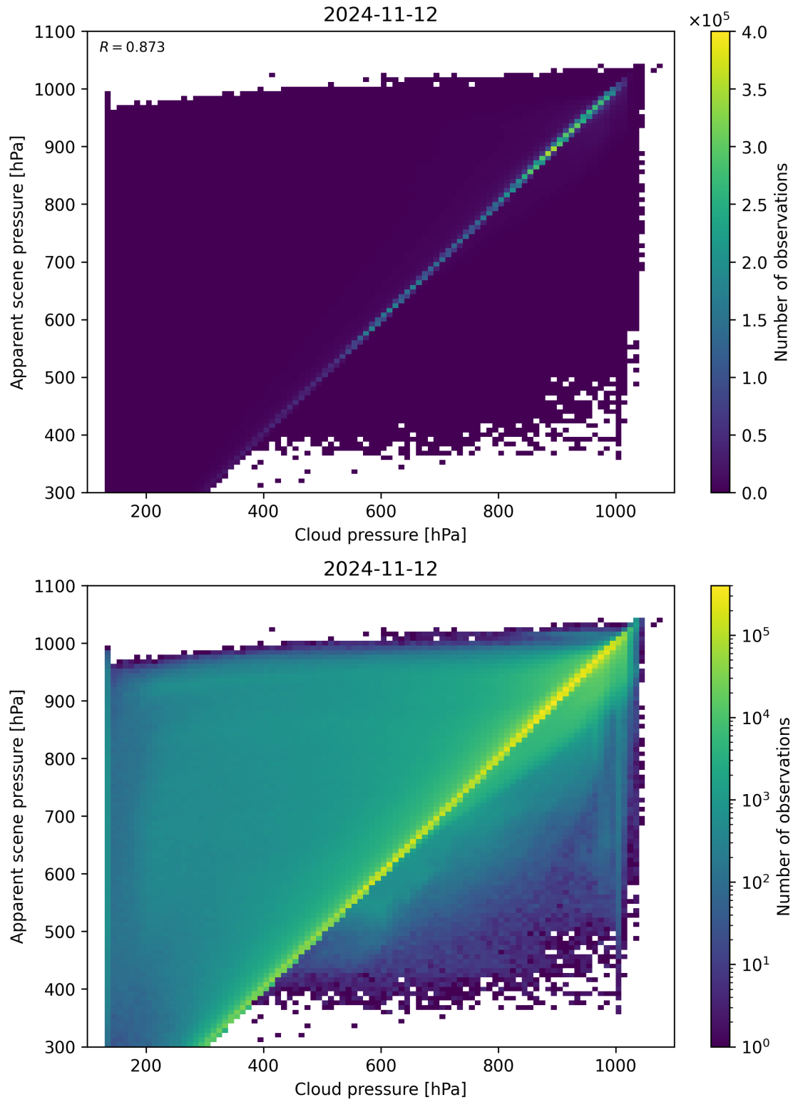
Figure 84: Scatter density plot of “Cloud pressure” against “Apparent scene pressure” for 2024-11-11 to 2024-11-13.
