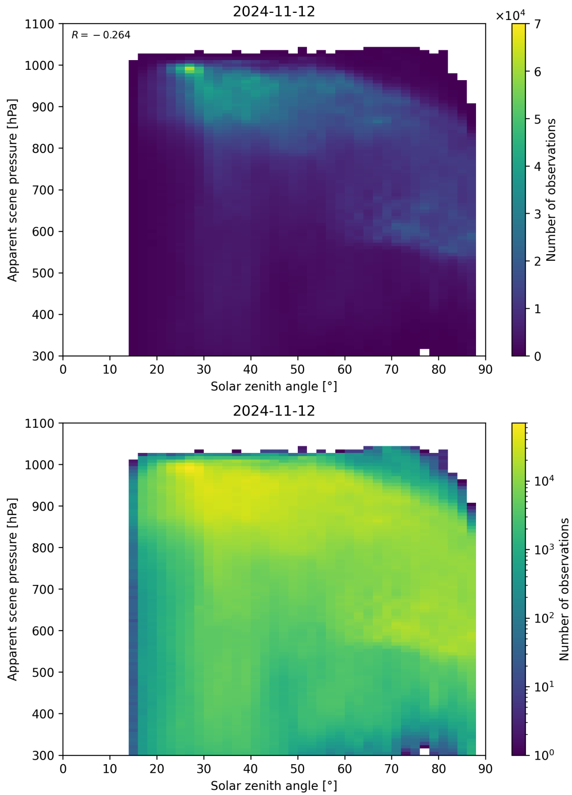
Figure 118: Scatter density plot of “Solar zenith angle” against “Apparent scene pressure” for 2024-11-11 to 2024-11-13.
