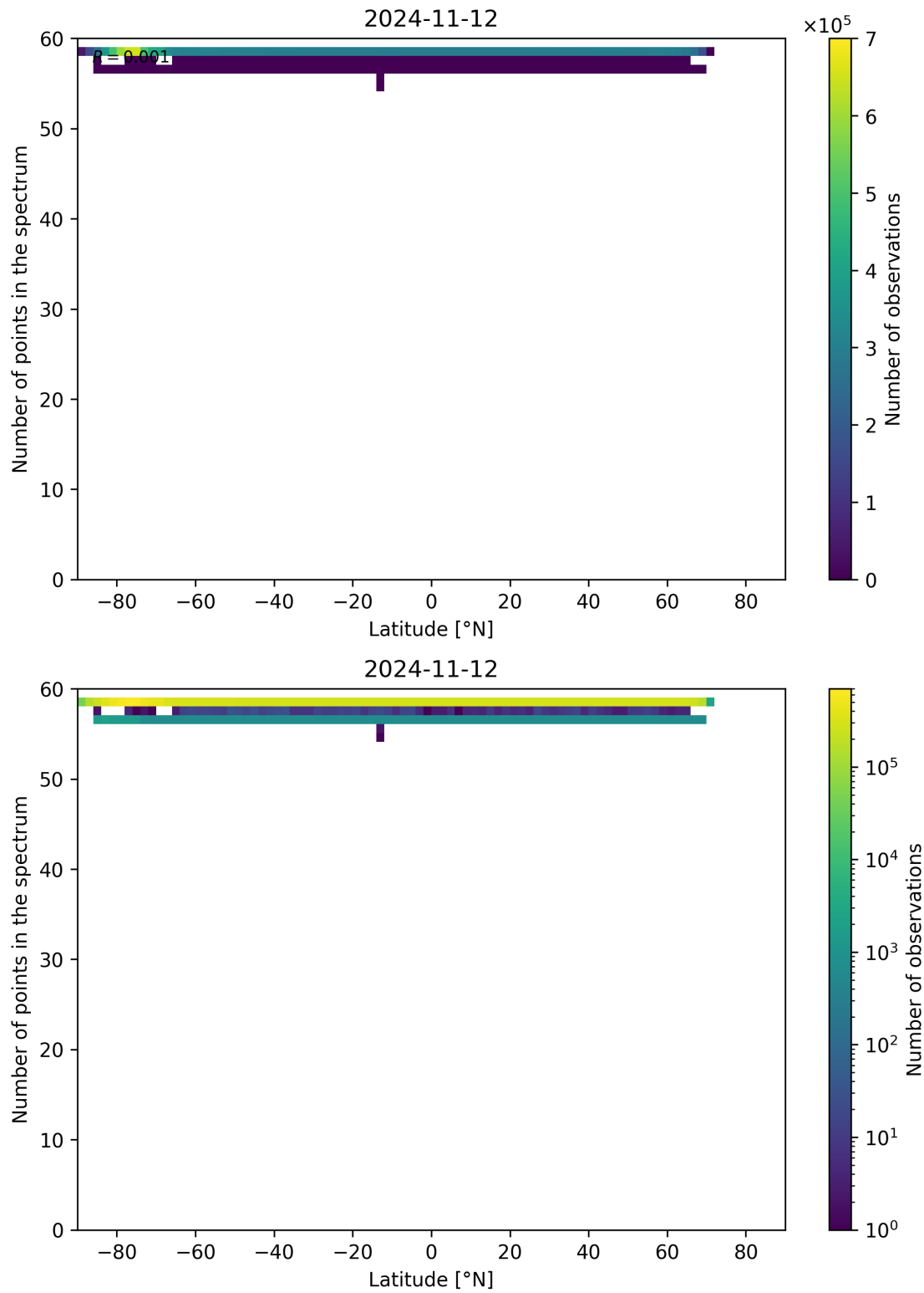
Figure 103: Scatter density plot of “Latitude” against “Number of points in the spectrum” for 2024-11-11 to 2024-11-13.
