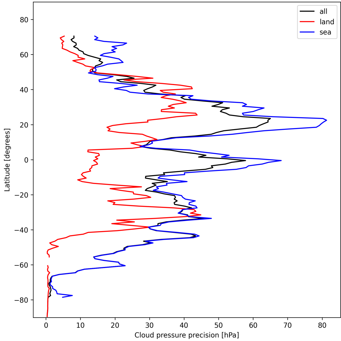
Figure 14: Zonal average of “Cloud pressure precision” for 2024-11-11 to 2024-11-13.
