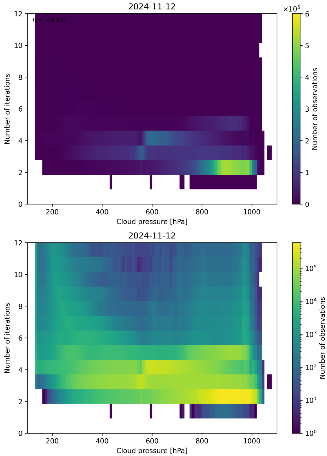
Figure 89: Scatter density plot of “Cloud pressure” against “Number of iterations” for 2024-11-11 to 2024-11-13.
