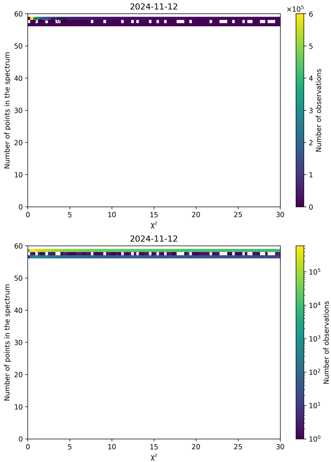
Figure 74: Scatter density plot of “ \chi^2 ” against “Number of points in the spectrum” for 2024-11-11 to 2024-11-13.
