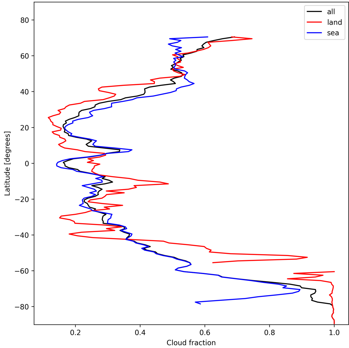
Figure 15: Zonal average of “Cloud fraction” for 2024-11-11 to 2024-11-13.
