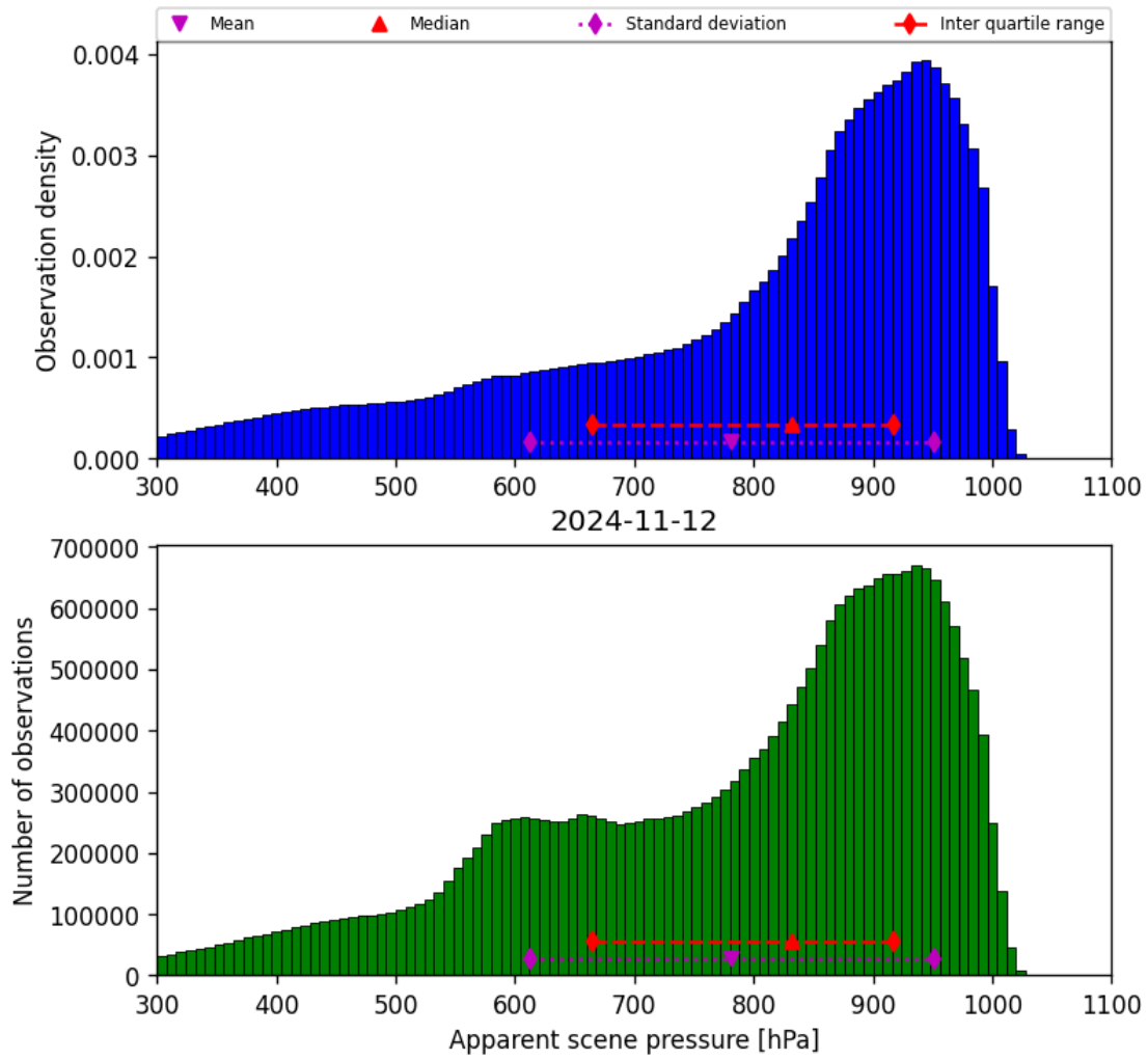
Figure 36: Histogram of “Apparent scene pressure” for 2024-11-11 to 2024-11-13
