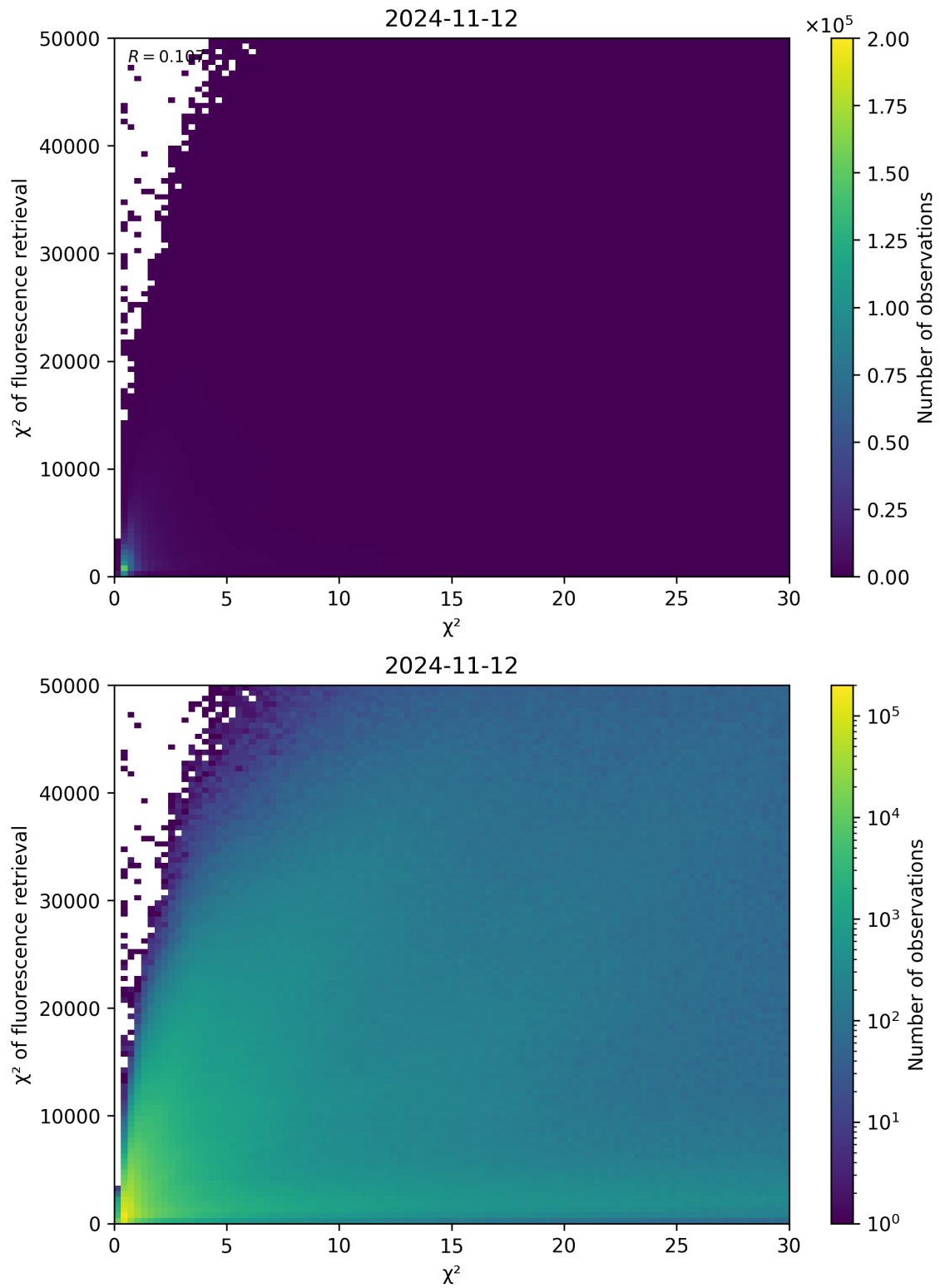
Figure 69: Scatter density plot of “ \chi^2 ” against “ \chi^2 of fluorescence retrieval” for 2024-11-11 to 2024-11-13.
