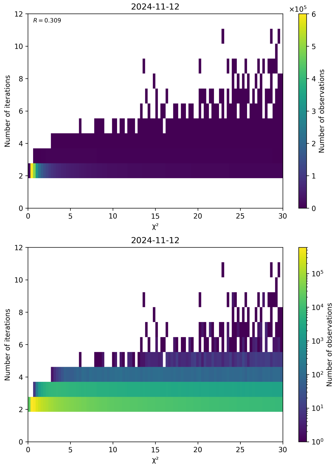
Figure 73: Scatter density plot of “ \chi^2 ” against “Number of iterations” for 2024-11-11 to 2024-11-13.
