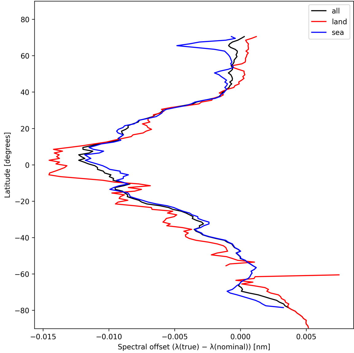
Figure 28: Zonal average of “Spectral offset ( \lambda_{\text{true}} - \lambda_{\text{nominal}} )” for 2024-11-11 to 2024-11-13.
