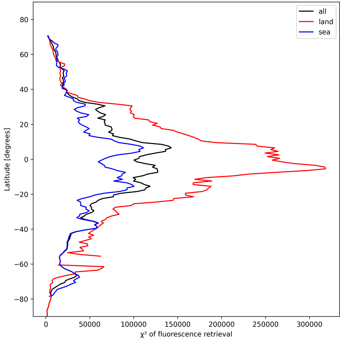
Figure 25: Zonal average of “ \chi^2 of fluorescence retrieval” for 2024-11-11 to 2024-11-13.
