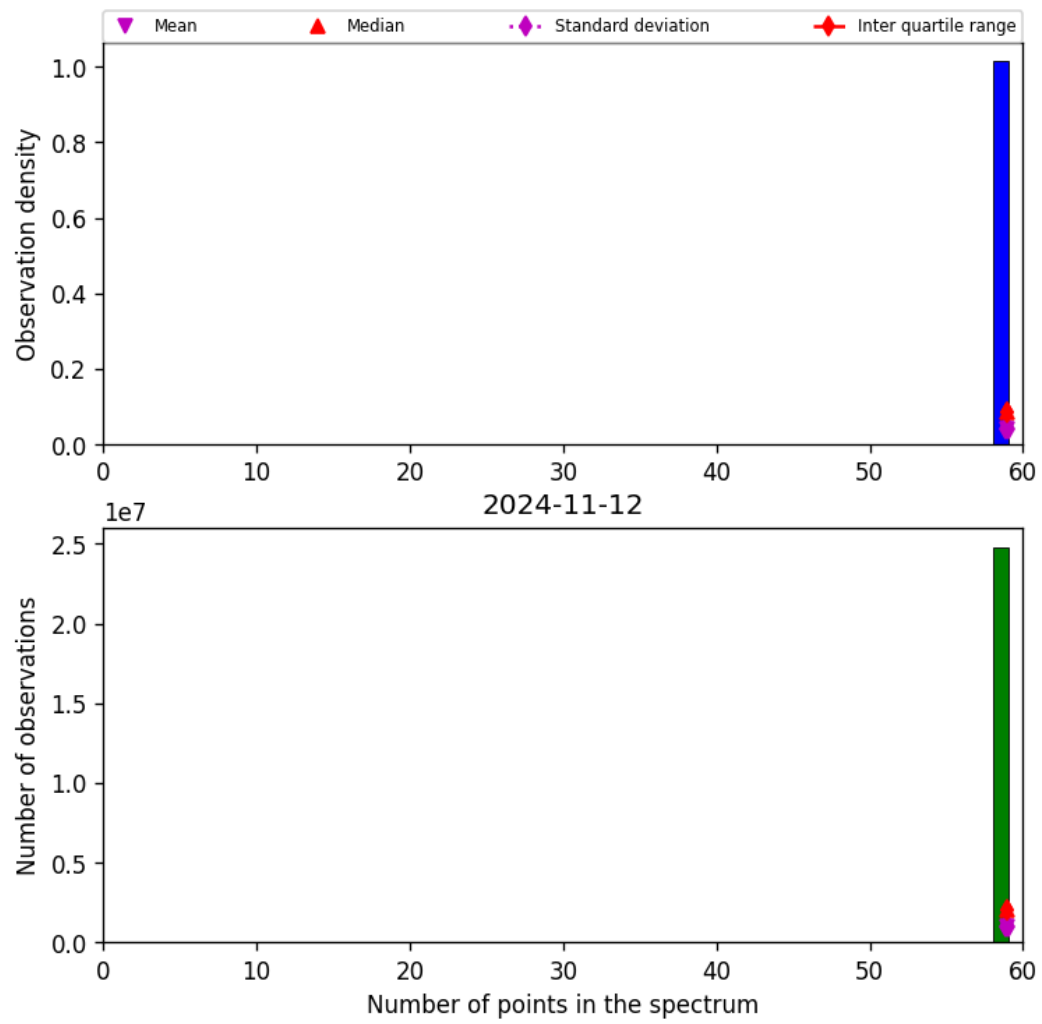
Figure 44: Histogram of “Number of points in the spectrum” for 2024-11-11 to 2024-11-13
