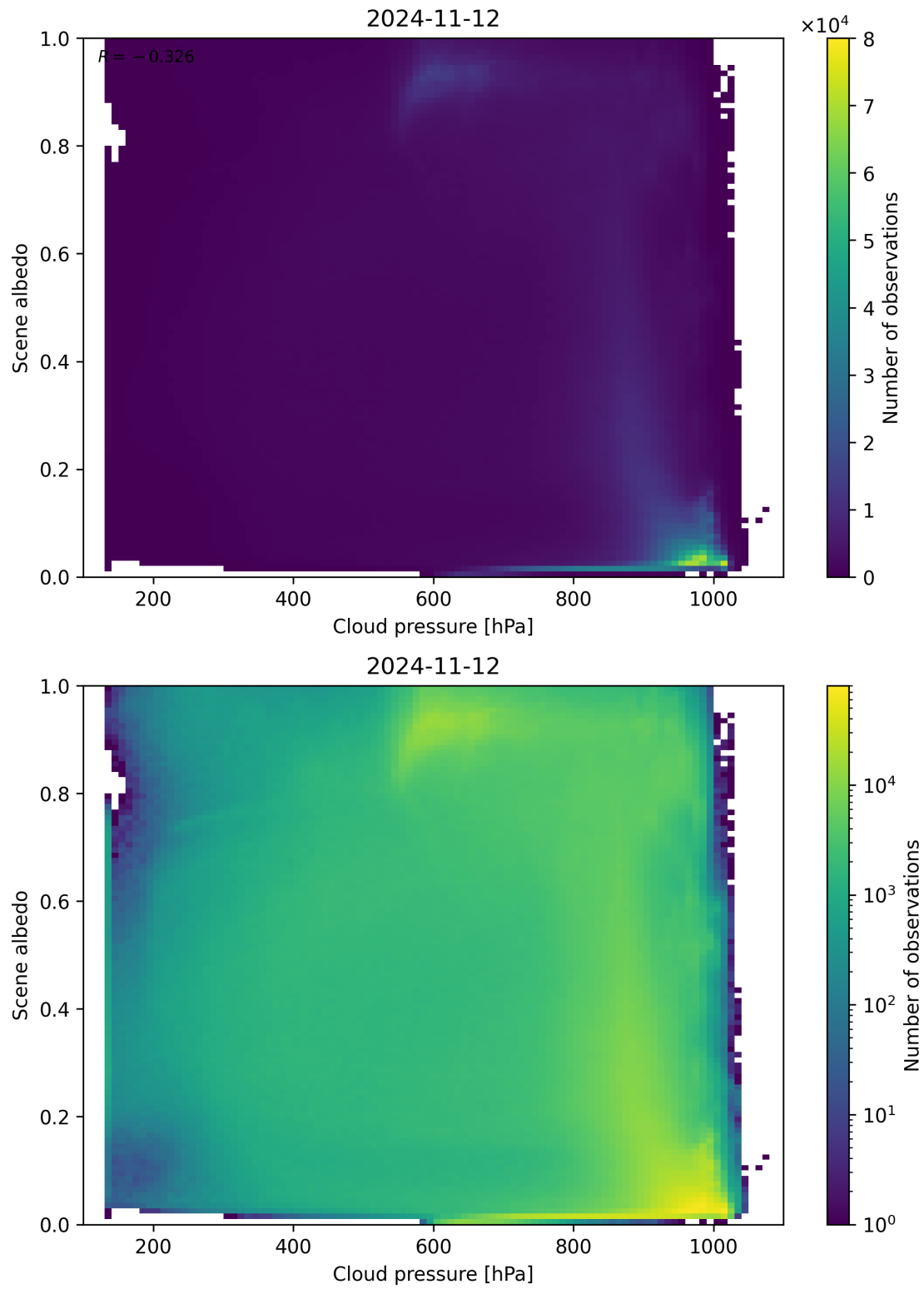
Figure 91: Scatter density plot of “Cloud pressure” against “Scene albedo” for 2024-11-11 to 2024-11-13.
