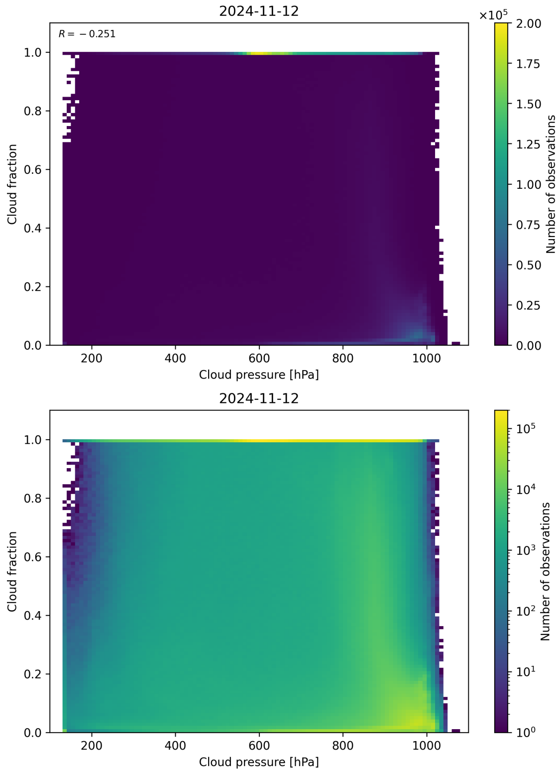
Figure 87: Scatter density plot of “Cloud pressure” against “Cloud fraction” for 2024-11-11 to 2024-11-13.
