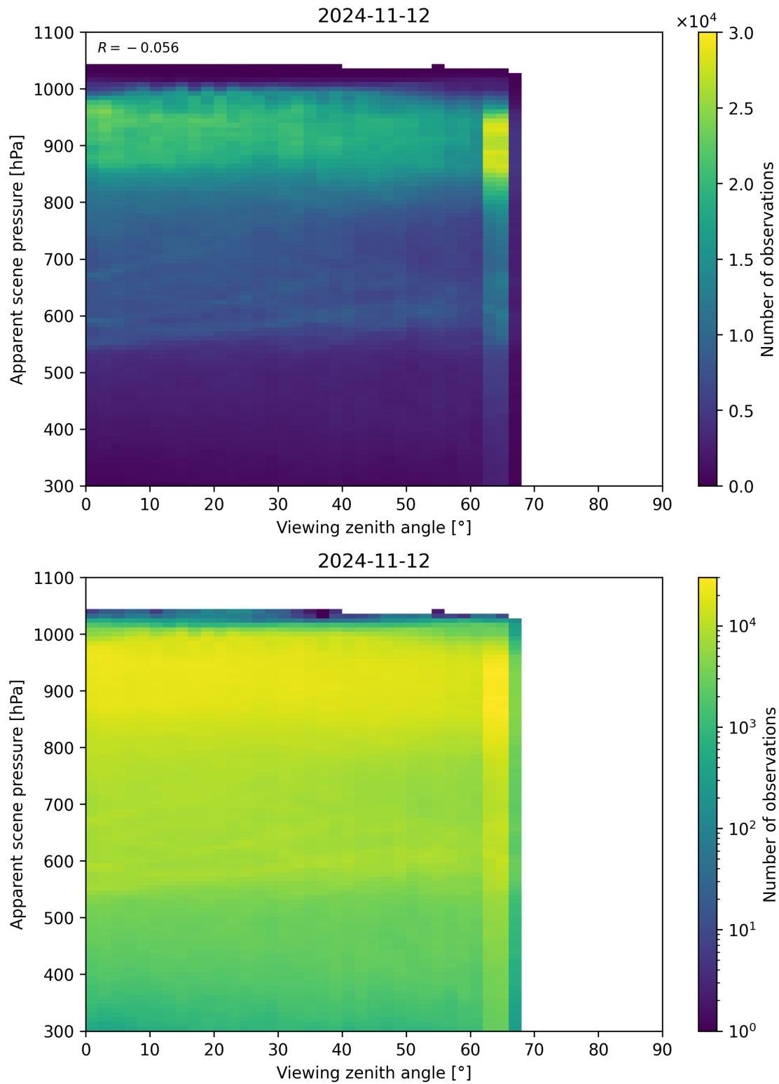
Figure 129: Scatter density plot of “Viewing zenith angle” against “Apparent scene pressure” for 2024-11-11 to 2024-11-13.
