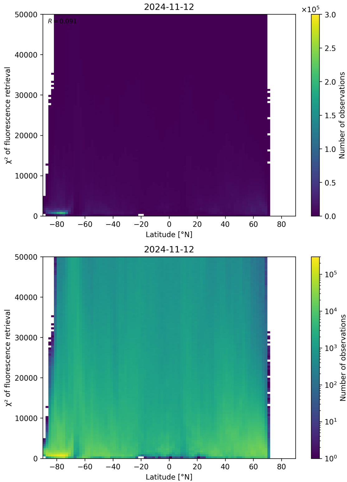
Figure 98: Scatter density plot of “Latitude” against “ \chi^2 of fluorescence retrieval” for 2024-11-11 to 2024-11-13.
