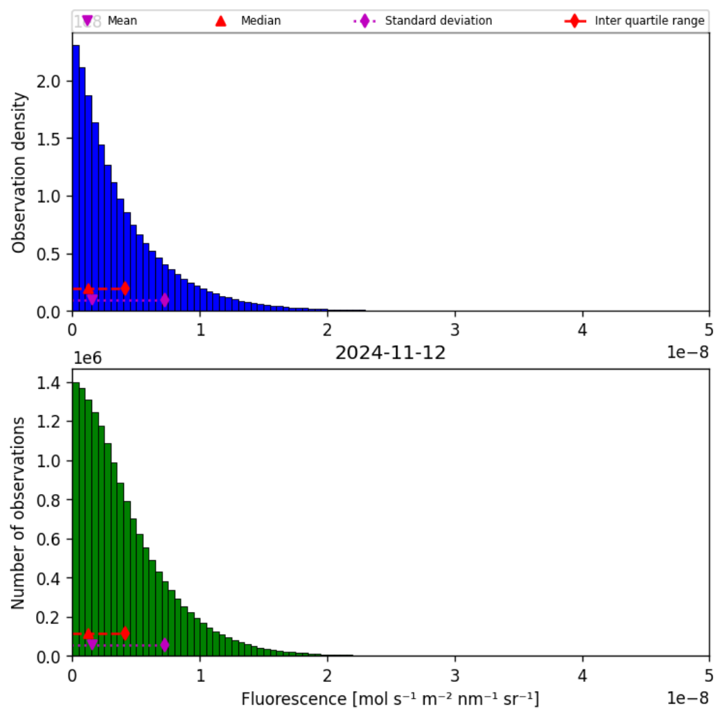
Figure 40: Histogram of “Fluorescence” for 2024-11-11 to 2024-11-13
