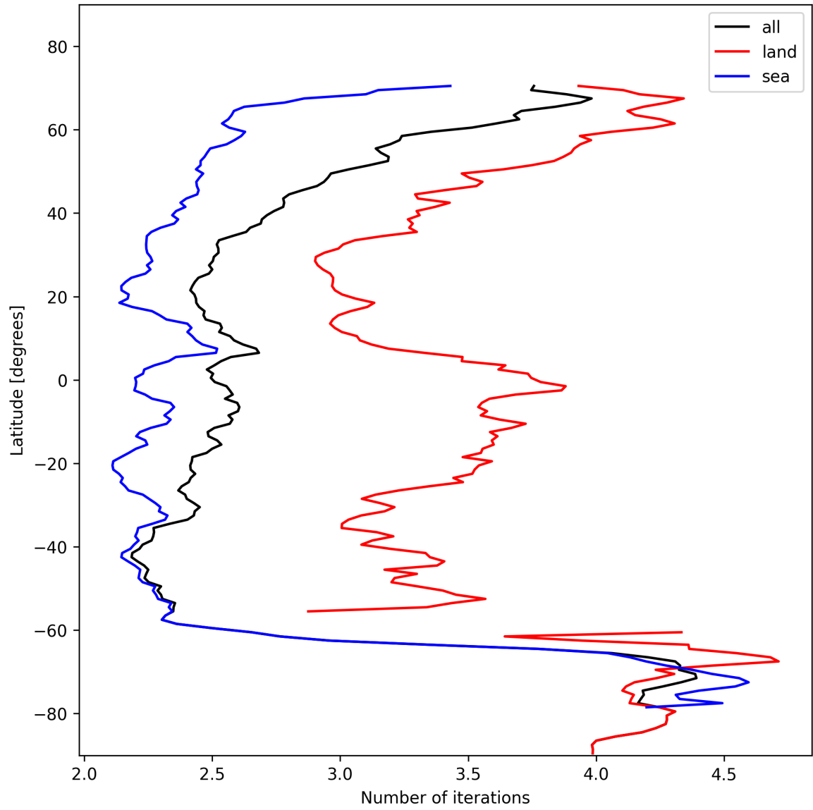
Figure 22: Zonal average of “Number of iterations” for 2024-11-11 to 2024-11-13.
