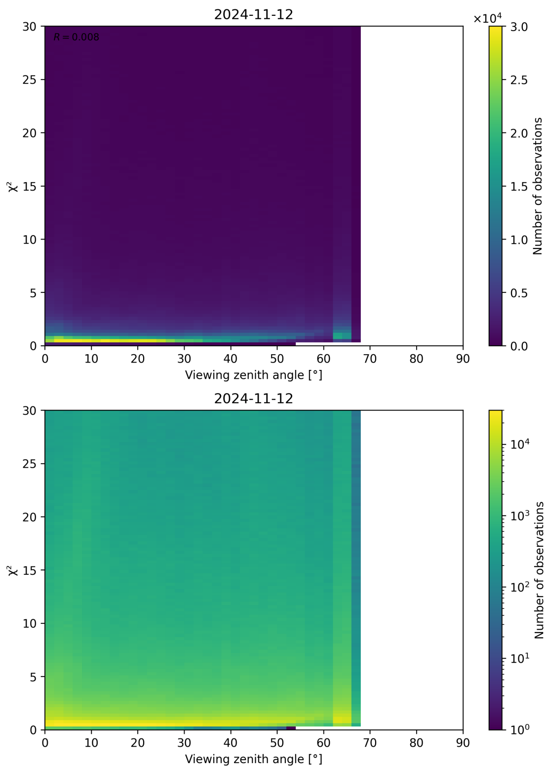
Figure 130: Scatter density plot of “Viewing zenith angle” against “ \chi^2 ” for 2024-11-11 to 2024-11-13.
