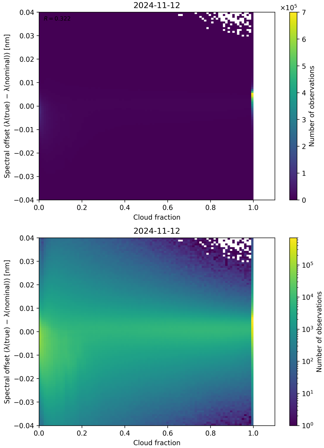
Figure 83: Scatter density plot of “Cloud fraction” against “Spectral offset ( \lambda_{\text{true}} - \lambda_{\text{nominal}} )” for 2024-11-11 to 2024-11-13.
