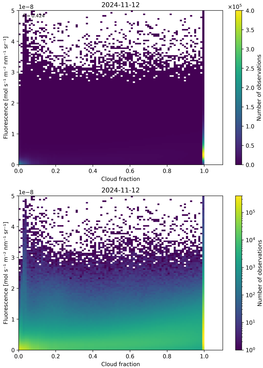
Figure 79: Scatter density plot of “Cloud fraction” against “Fluorescence” for 2024-11-11 to 2024-11-13.
