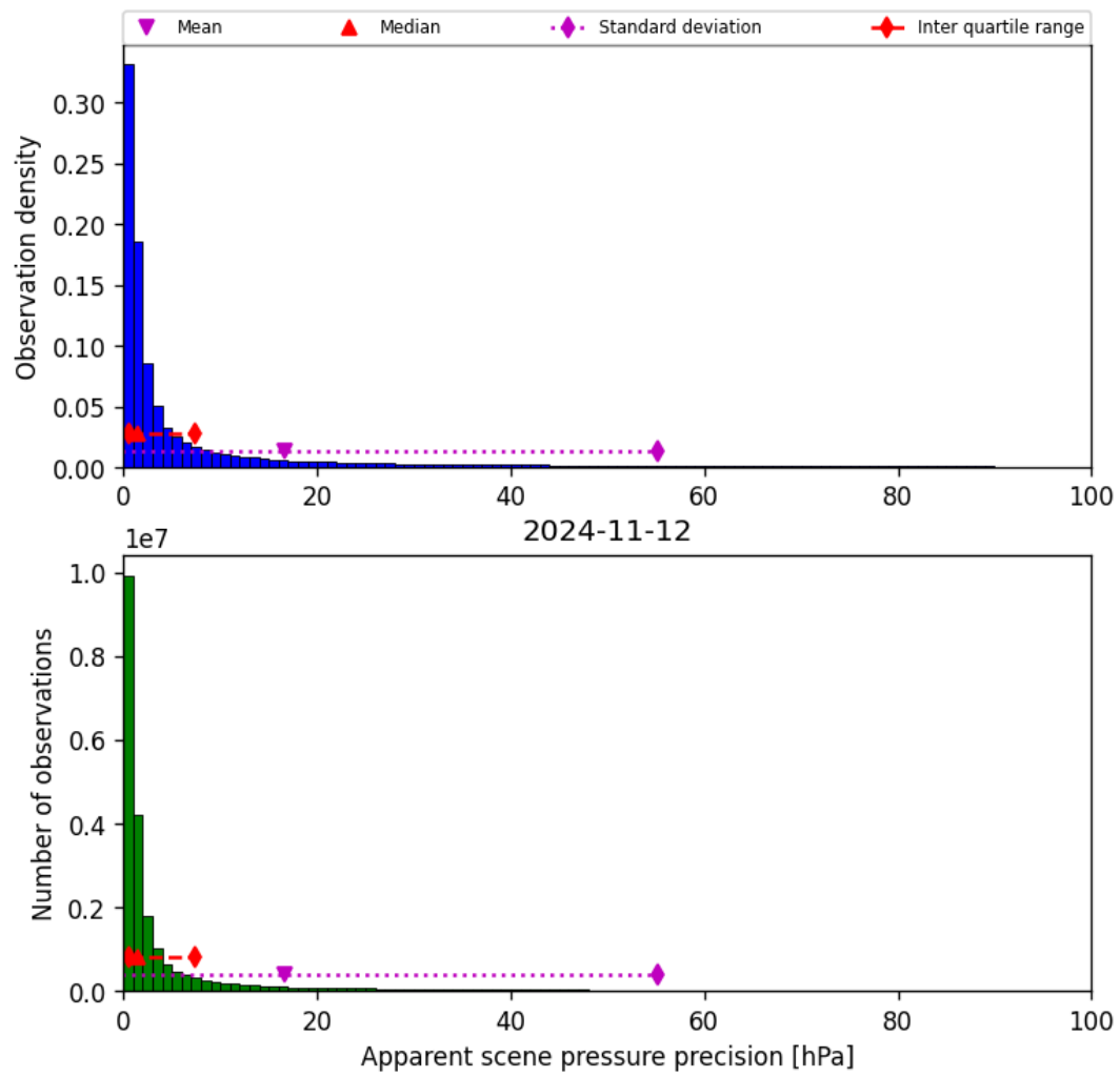
Figure 37: Histogram of “Apparent scene pressure precision” for 2024-11-11 to 2024-11-13
