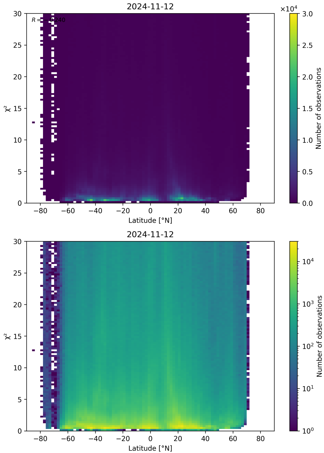
Figure 97: Scatter density plot of “Latitude” against “ \chi^2 ” for 2024-11-11 to 2024-11-13.
