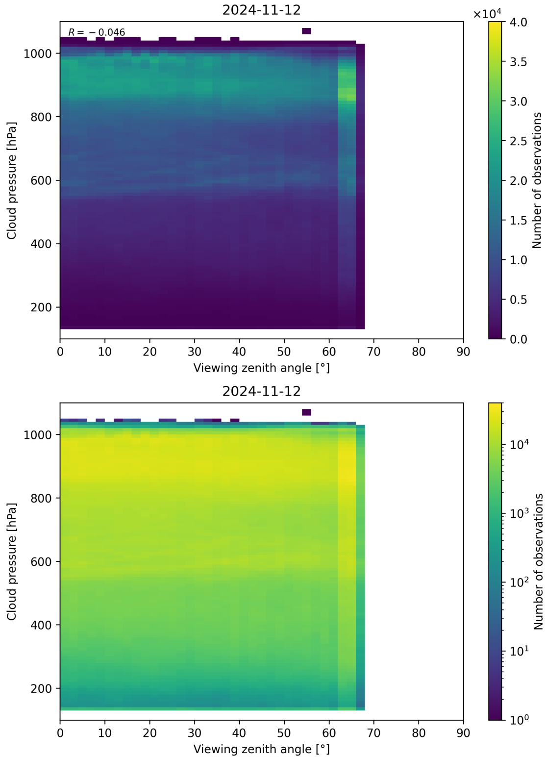
Figure 133: Scatter density plot of “Viewing zenith angle” against “Cloud pressure” for 2024-11-11 to 2024-11-13.
