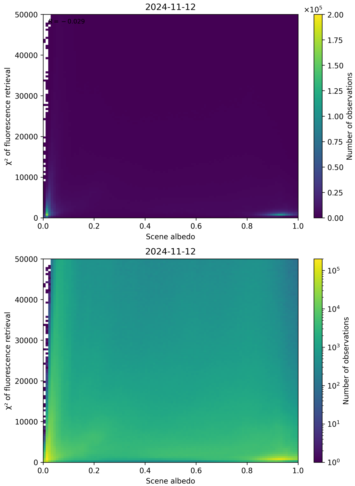
Figure 113: Scatter density plot of “Scene albedo” against “ \chi^2 of fluorescence retrieval” for 2024-11-11 to 2024-11-13.
