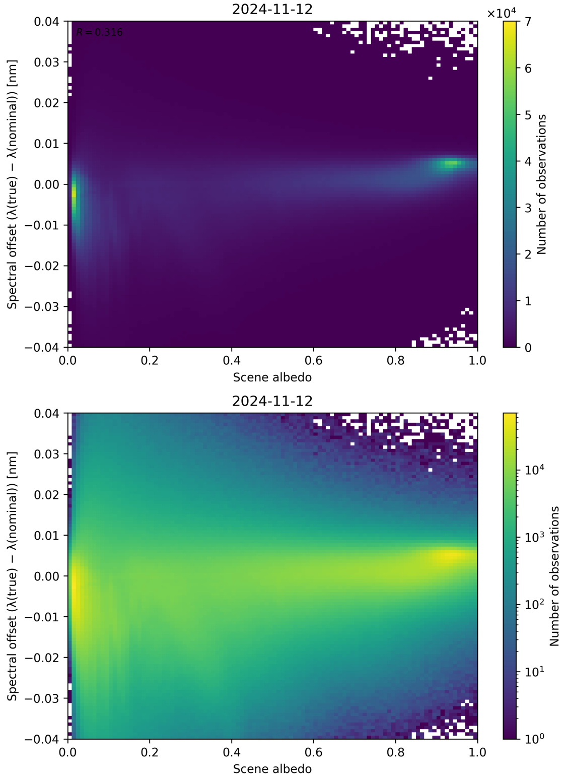
Figure 117: Scatter density plot of “Scene albedo” against “Spectral offset ( \lambda_{\text{true}} - \lambda_{\text{nominal}} )” for 2024-11-11 to 2024-11-13.
