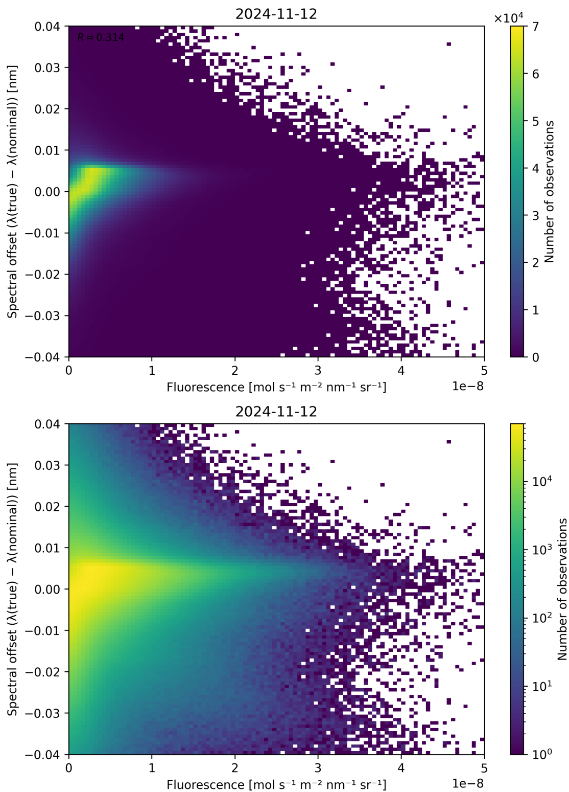
Figure 95: Scatter density plot of “Fluorescence” against “Spectral offset ( \lambda_{\text{true}} - \lambda_{\text{nominal}} )” for 2024-11-11 to 2024-11-13.
