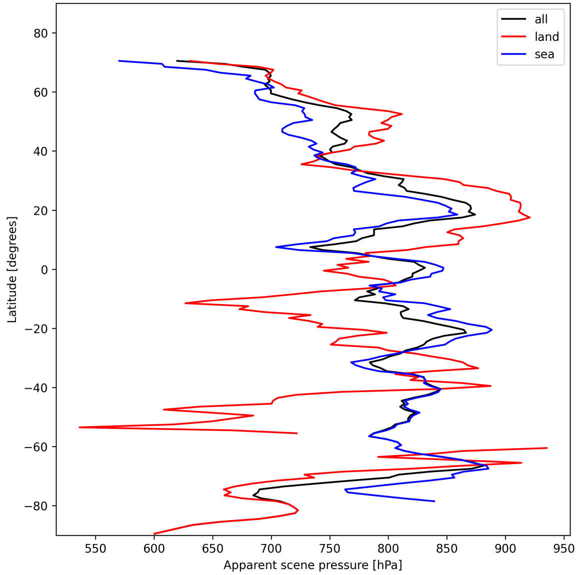
Figure 19: Zonal average of “Apparent scene pressure” for 2024-11-11 to 2024-11-13.
