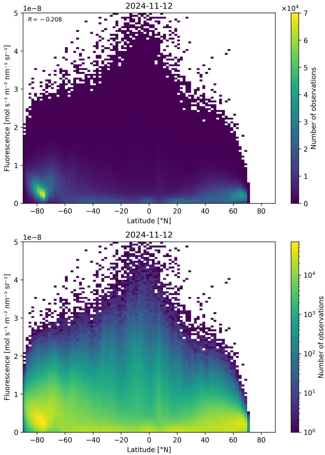
Figure 101: Scatter density plot of “Latitude” against “Fluorescence” for 2024-11-11 to 2024-11-13.
