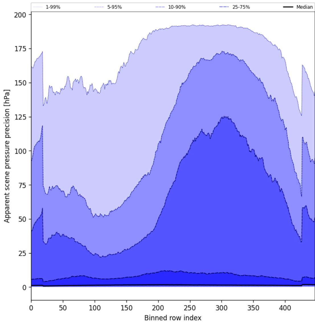
Figure 54: Along track statistics of “Apparent scene pressure precision” for 2024-11-11 to 2024-11-13
