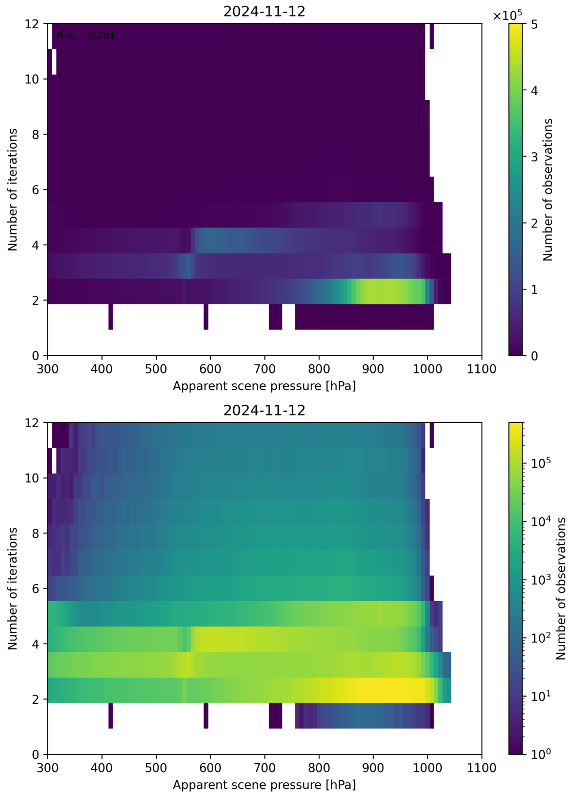
Figure 66: Scatter density plot of “Apparent scene pressure” against “Number of iterations” for 2024-11-11 to 2024-11-13.
