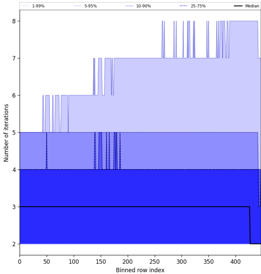
Figure 56: Along track statistics of “Number of iterations” for 2024-11-11 to 2024-11-13
