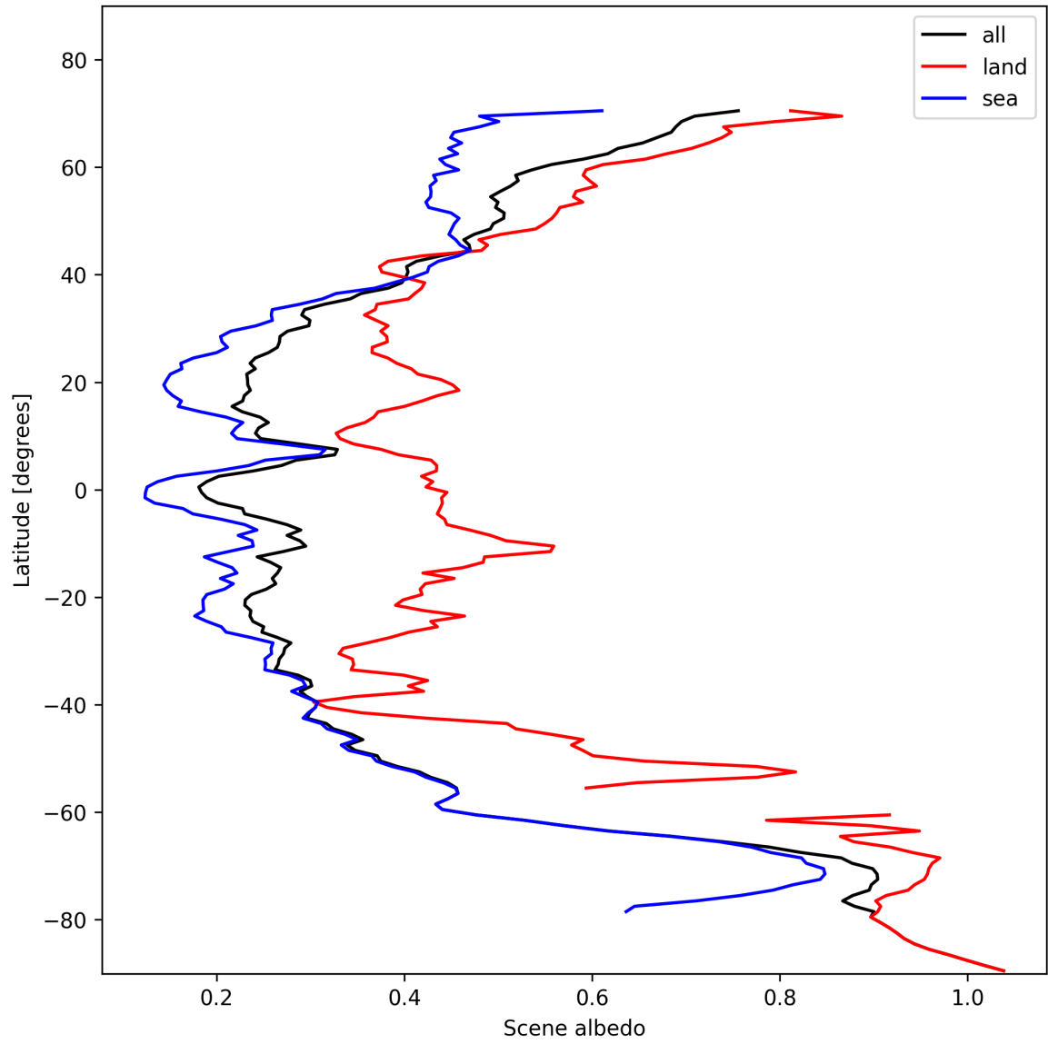
Figure 17: Zonal average of “Scene albedo” for 2024-11-11 to 2024-11-13.
