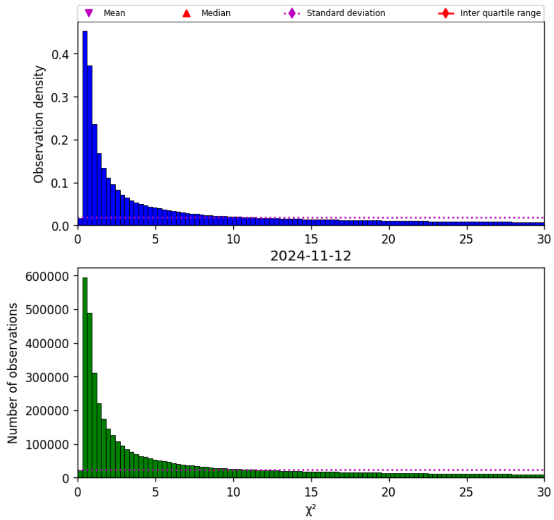
Figure 38: Histogram of " \chi^2 " for 2024-11-11 to 2024-11-13
