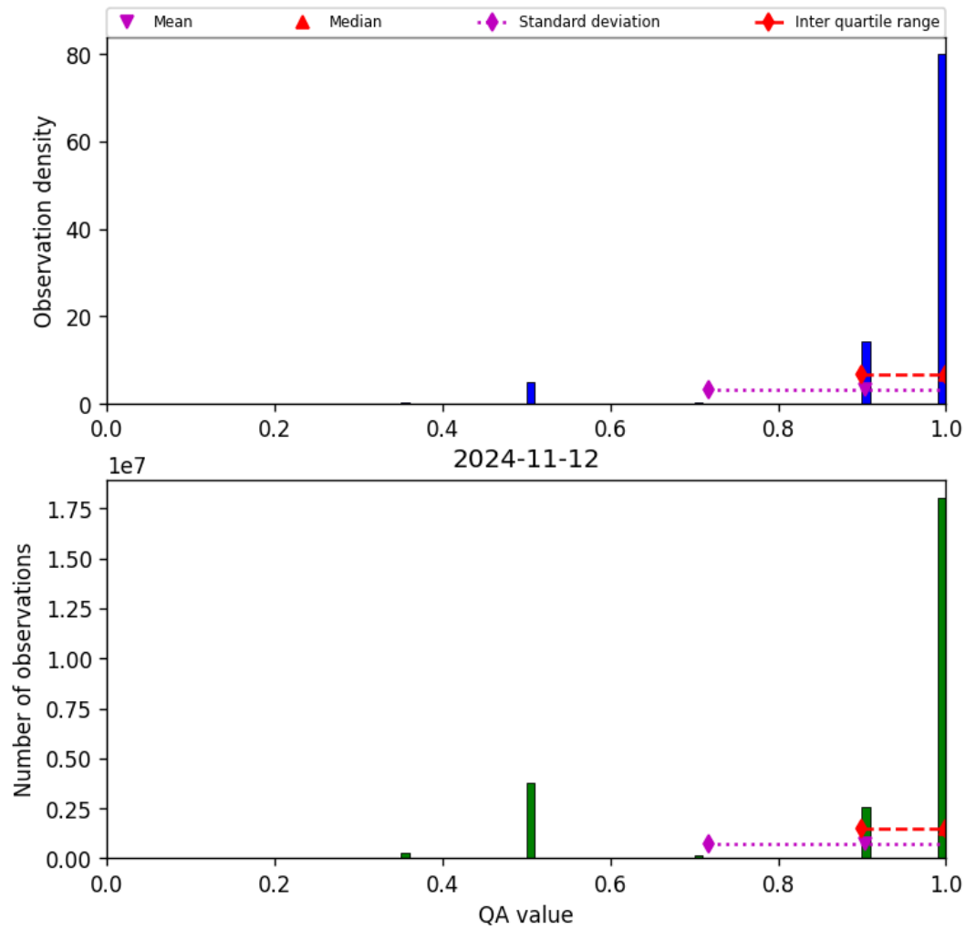
Figure 29: Histogram of “QA value” for 2024-11-11 to 2024-11-13
