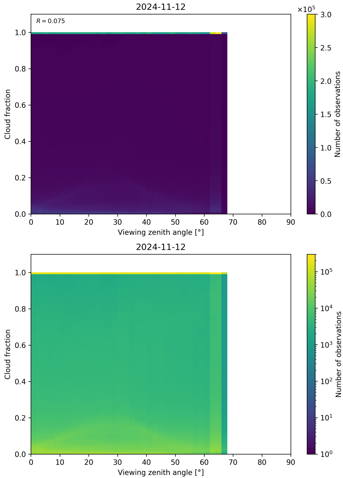
Figure 132: Scatter density plot of “Viewing zenith angle” against “Cloud fraction” for 2024-11-11 to 2024-11-13.
