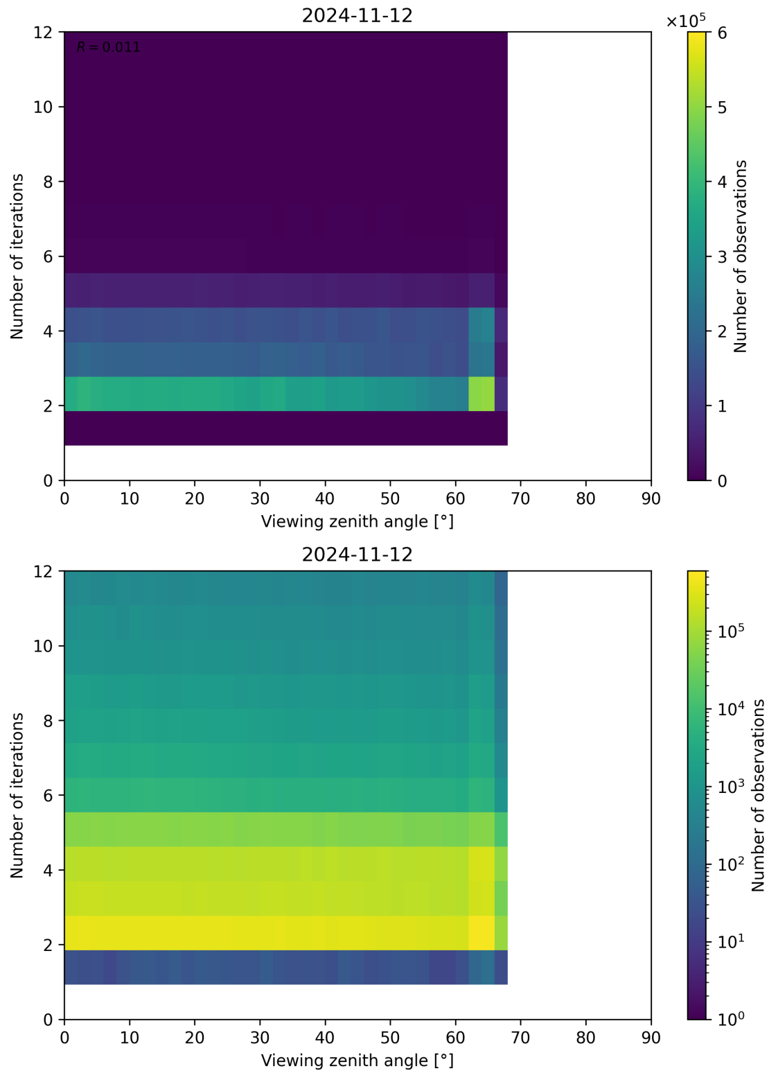
Figure 136: Scatter density plot of “Viewing zenith angle” against “Number of iterations” for 2024-11-11 to 2024-11-13.
