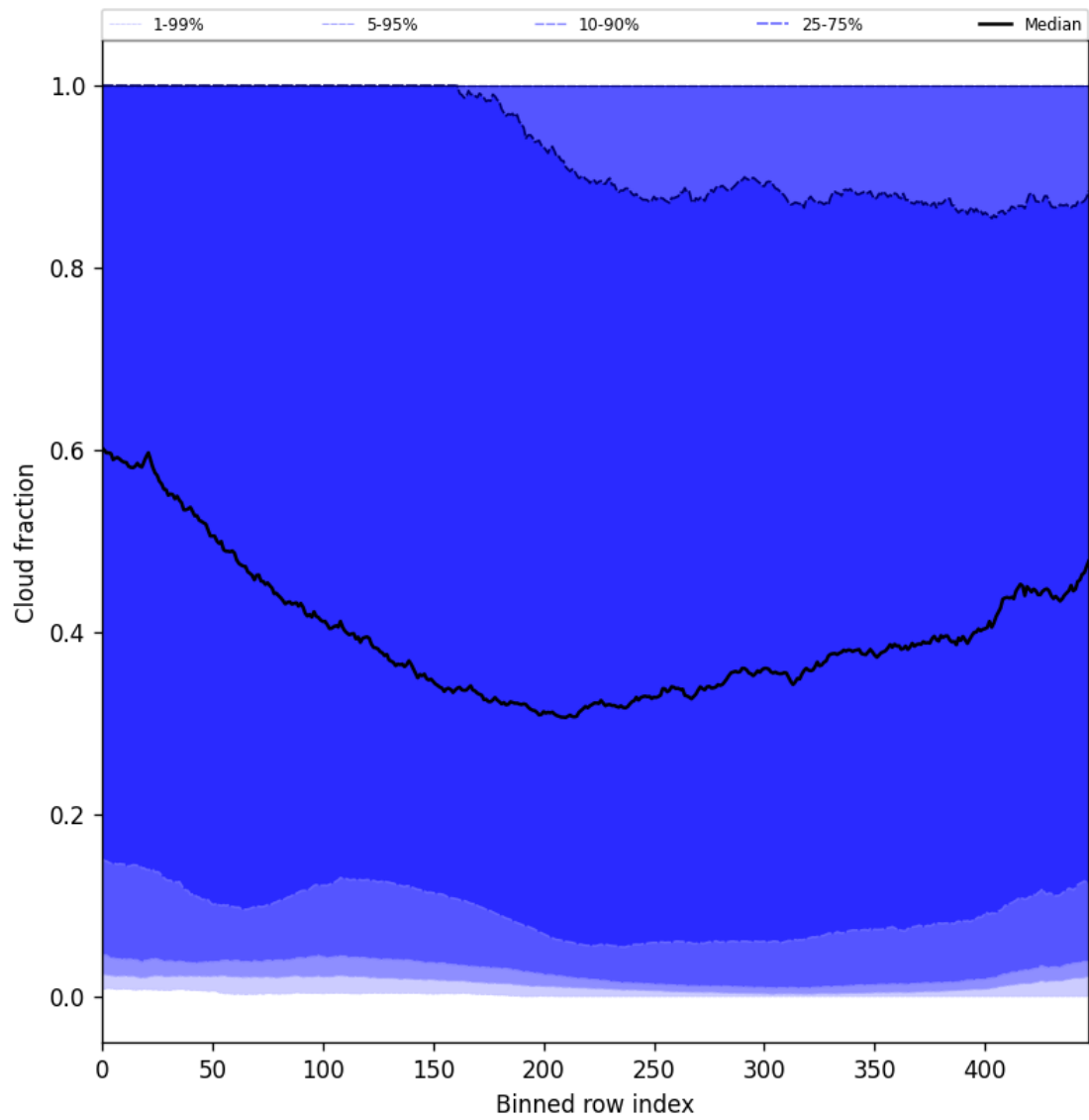
Figure 49: Along track statistics of “Cloud fraction” for 2024-11-11 to 2024-11-13
