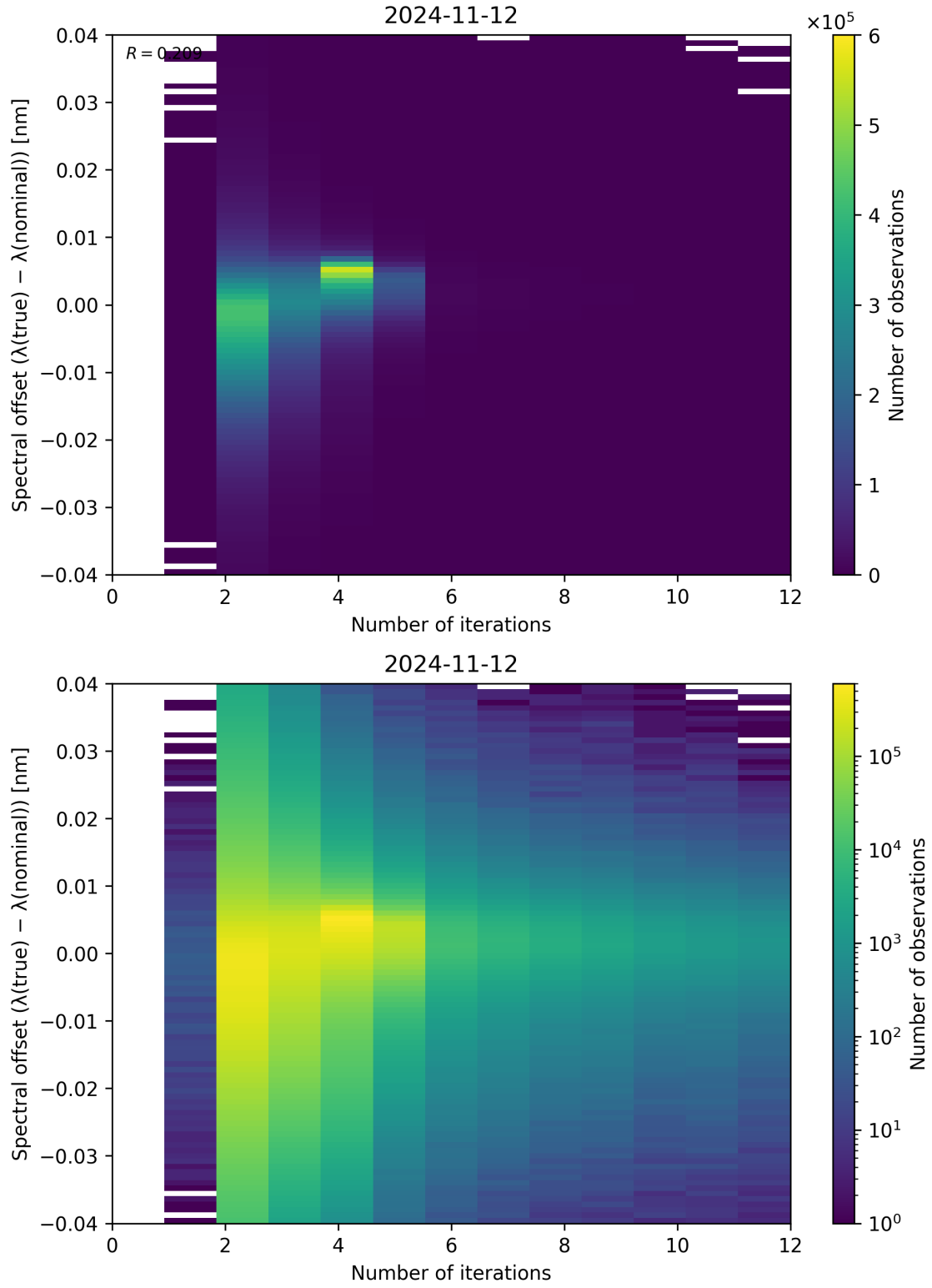
Figure 109: Scatter density plot of “Number of iterations” against “Spectral offset ( \lambda_{\text{true}} - \lambda_{\text{nominal}} )” for 2024-11-11 to 2024-11-13.
