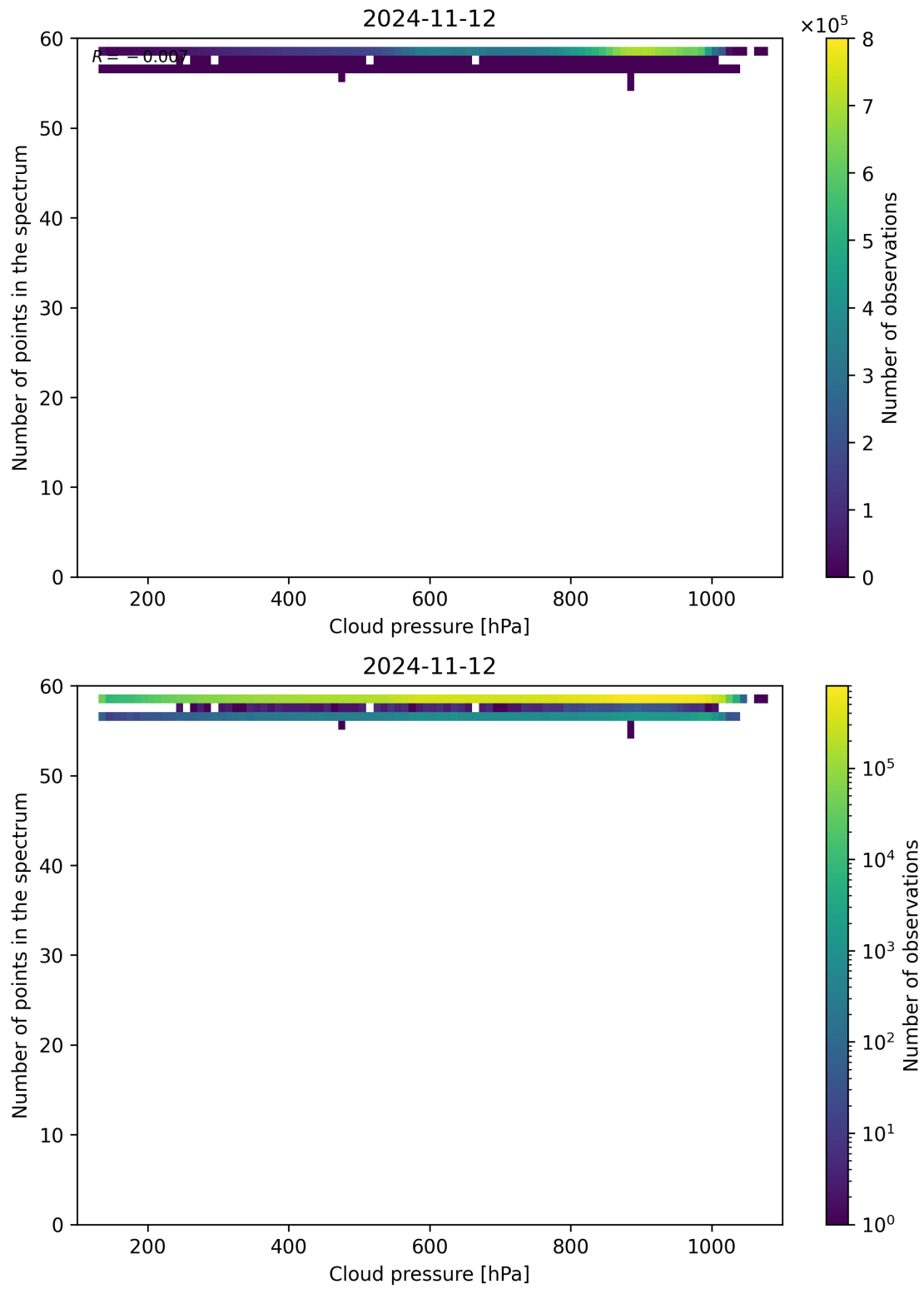
Figure 90: Scatter density plot of “Cloud pressure” against “Number of points in the spectrum” for 2024-11-11 to 2024-11-13.
