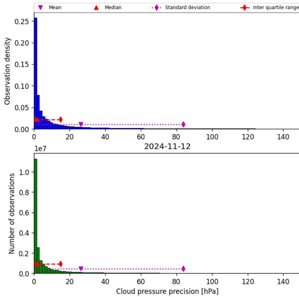
Figure 31: Histogram of “Cloud pressure precision” for 2024-11-11 to 2024-11-13
