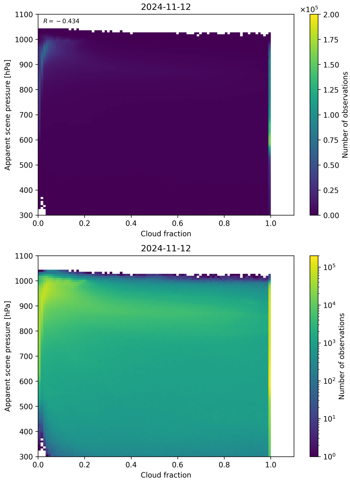
Figure 76: Scatter density plot of “Cloud fraction” against “Apparent scene pressure” for 2024-11-11 to 2024-11-13.
