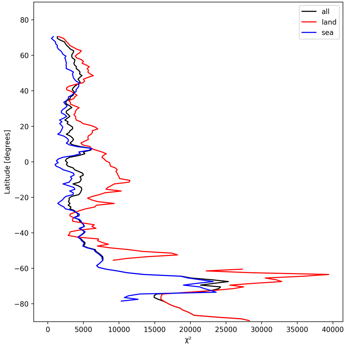
Figure 21: Zonal average of “ \chi^2 ” for 2024-11-11 to 2024-11-13.
