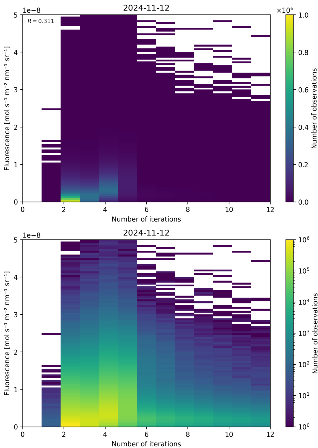
Figure 107: Scatter density plot of “Number of iterations” against “Fluorescence” for 2024-11-11 to 2024-11-13.
