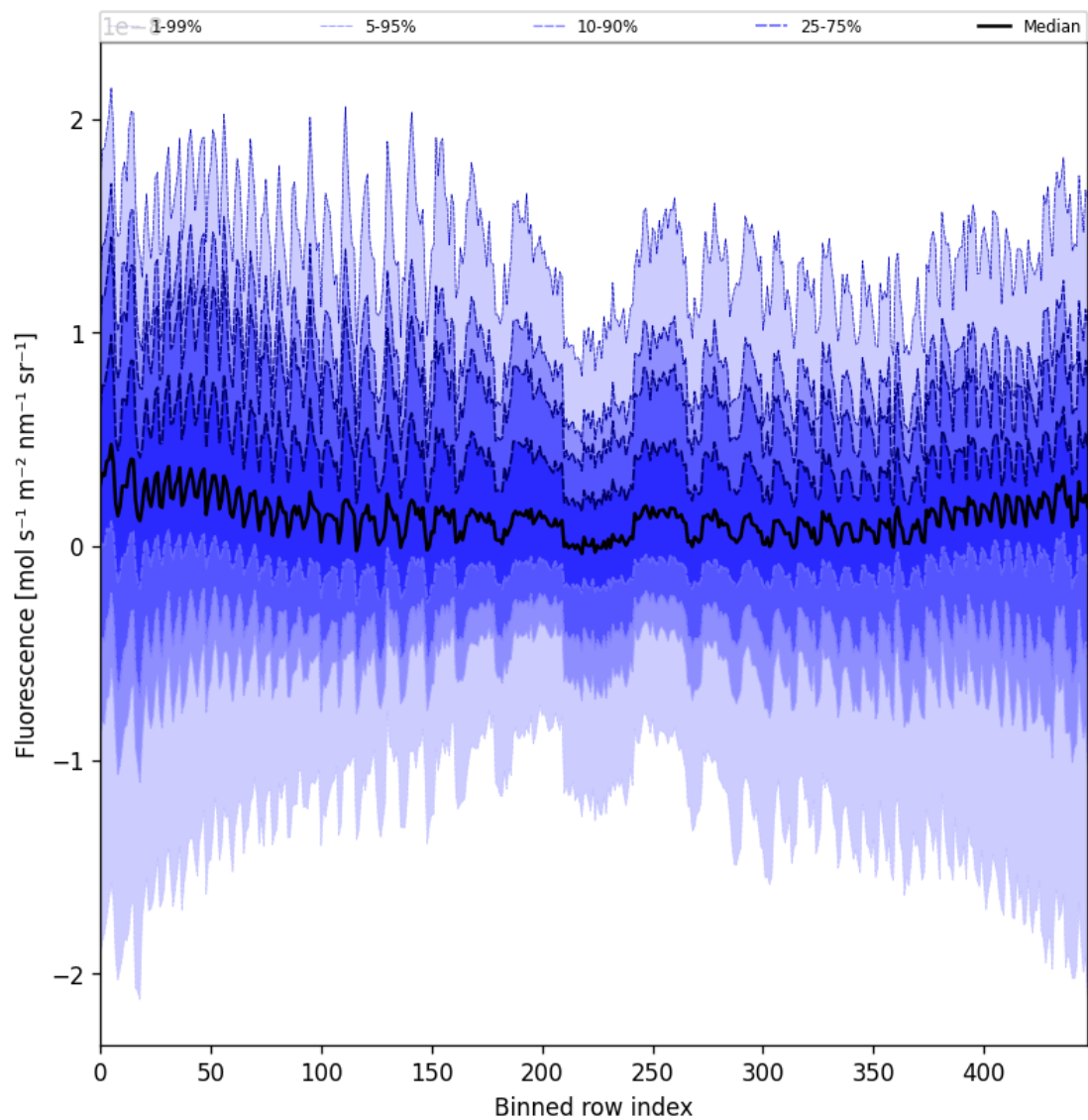
Figure 57: Along track statistics of “Fluorescence” for 2024-11-11 to 2024-11-13
