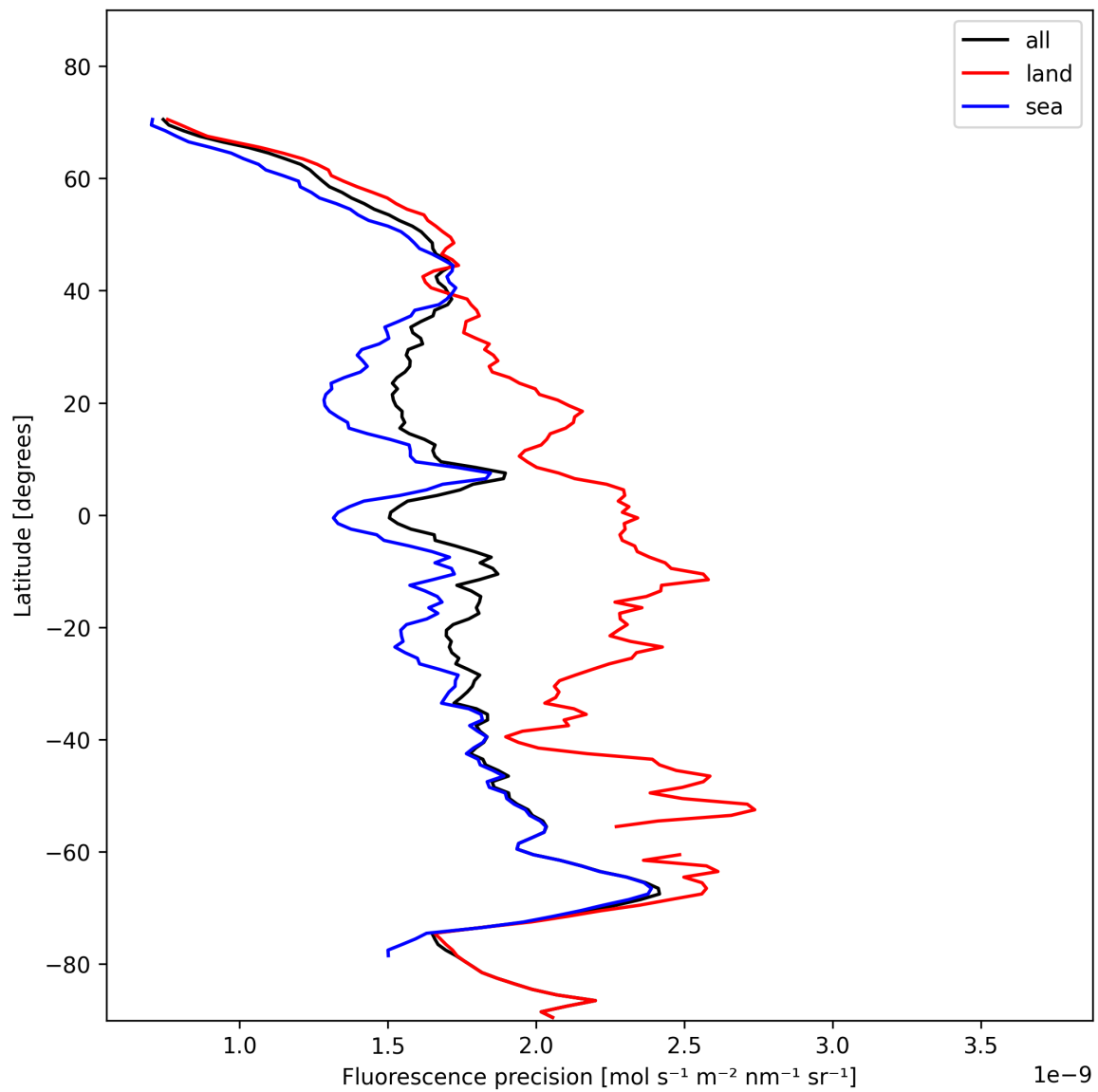
Figure 24: Zonal average of “Fluorescence precision” for 2024-11-11 to 2024-11-13.
