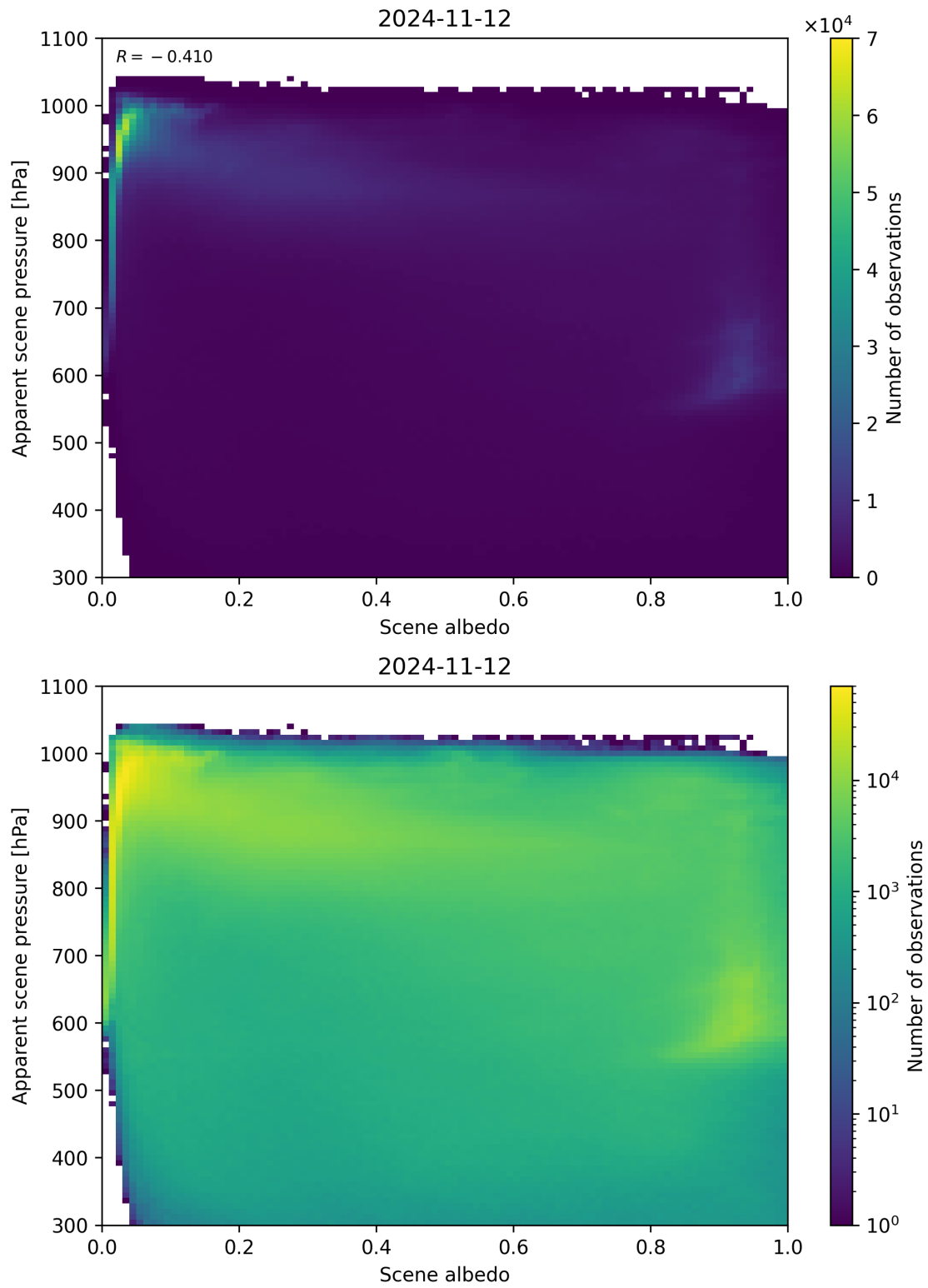
Figure 111: Scatter density plot of “Scene albedo” against “Apparent scene pressure” for 2024-11-11 to 2024-11-13.
