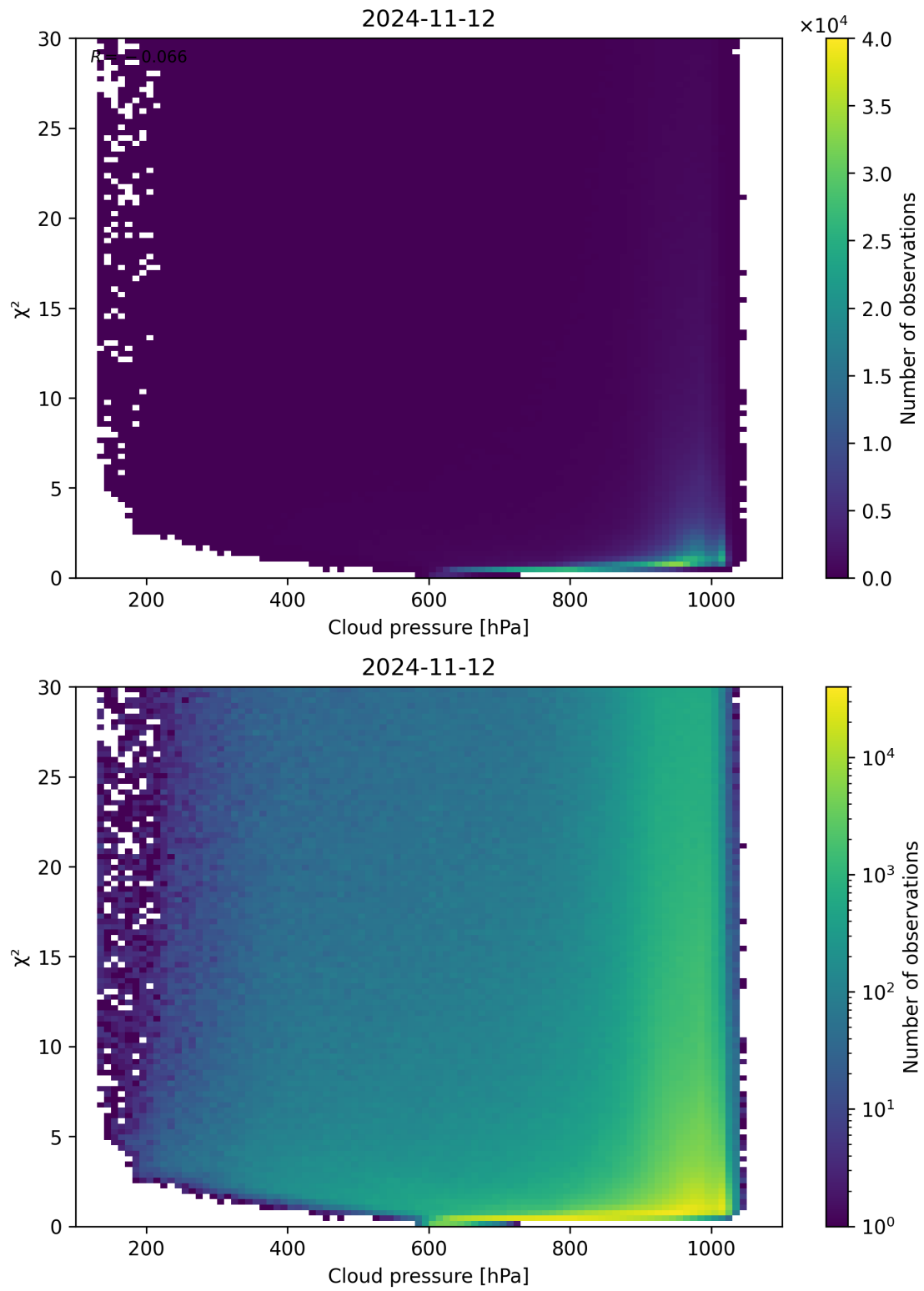
Figure 85: Scatter density plot of “Cloud pressure” against “ \chi^2 ” for 2024-11-11 to 2024-11-13.
