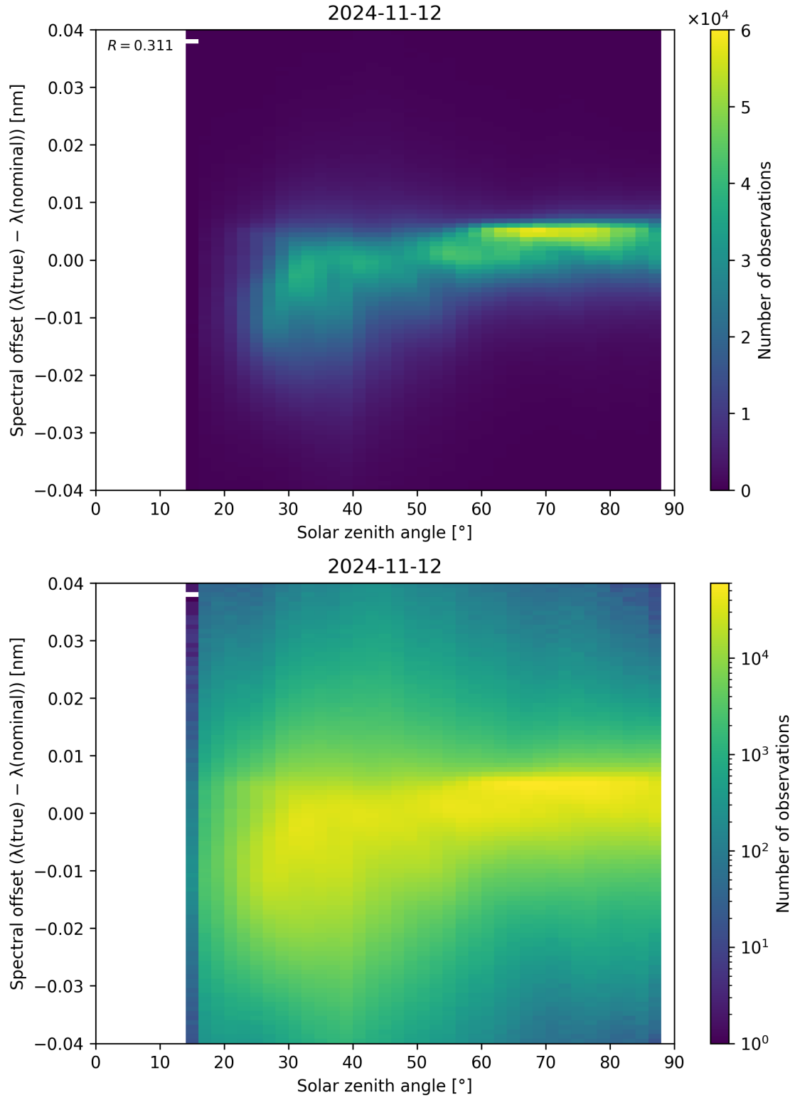
Figure 128: Scatter density plot of “Solar zenith angle” against “Spectral offset ( \lambda_{\text{true}} - \lambda_{\text{nominal}} )” for 2024-11-11 to 2024-11-13.
