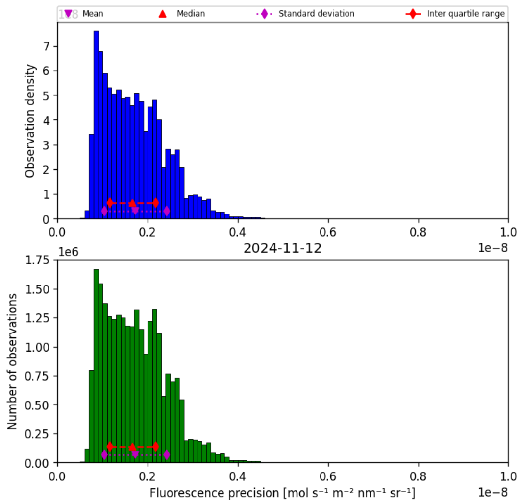
Figure 41: Histogram of “Fluorescence precision” for 2024-11-11 to 2024-11-13
