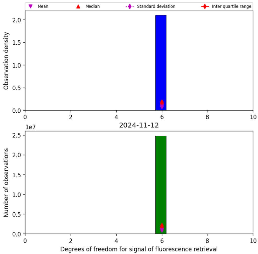
Figure 43: Histogram of "Degrees of freedom for signal of fluorescence retrieval" for 2024-11-11 to 2024-11-13
