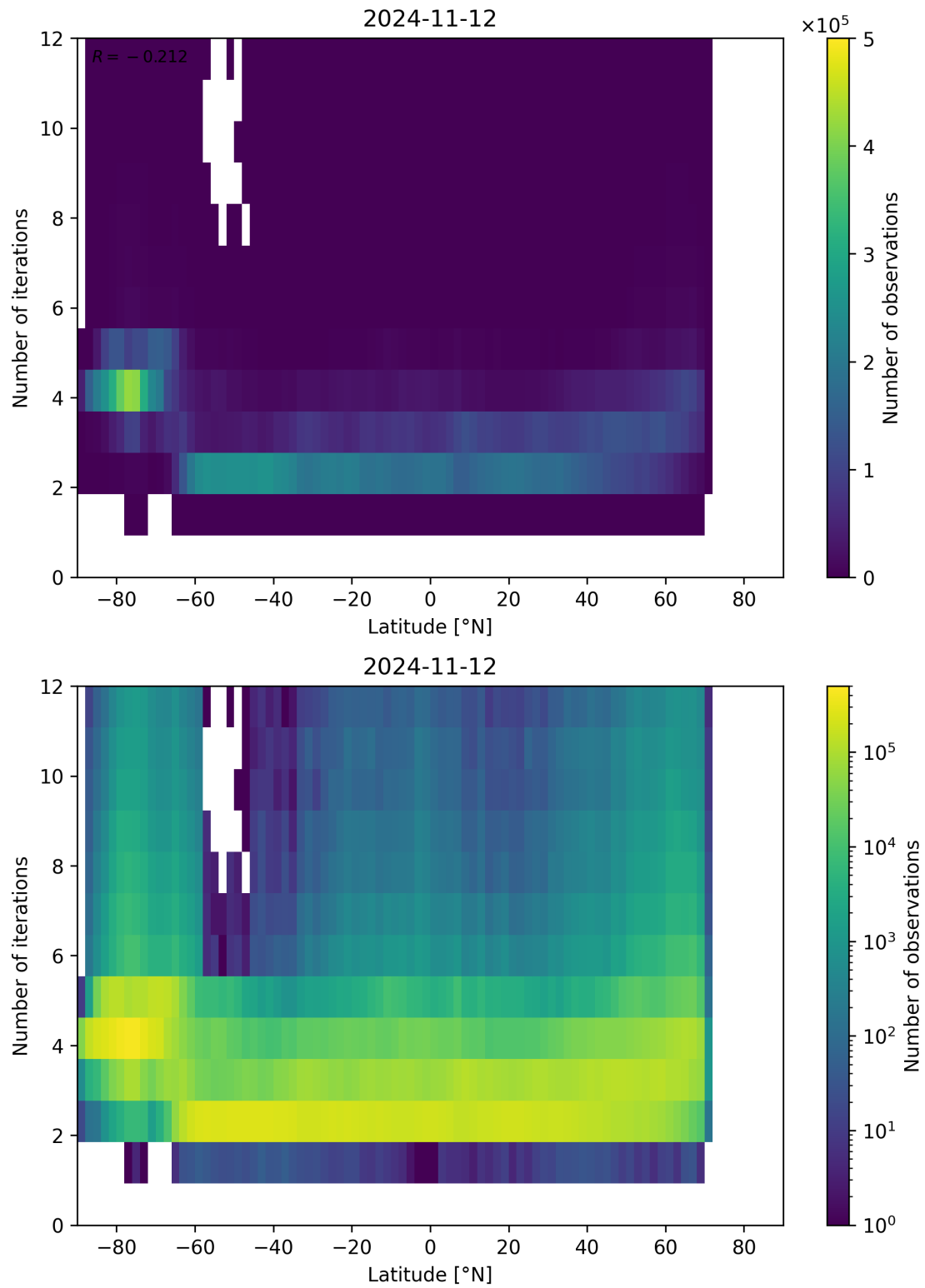
Figure 102: Scatter density plot of “Latitude” against “Number of iterations” for 2024-11-11 to 2024-11-13.
