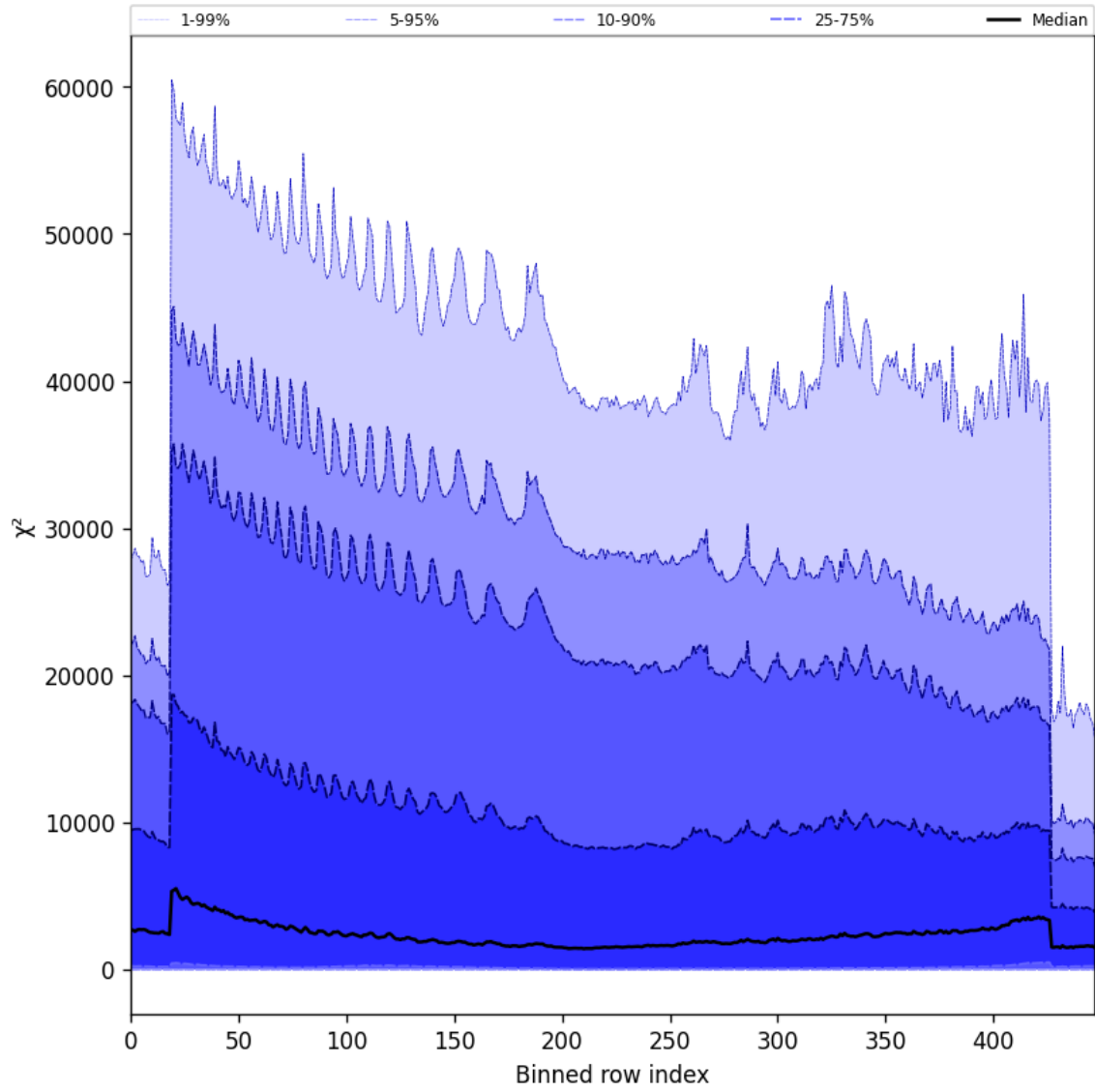
Figure 55: Along track statistics of “ \chi^2 ” for 2024-11-11 to 2024-11-13
