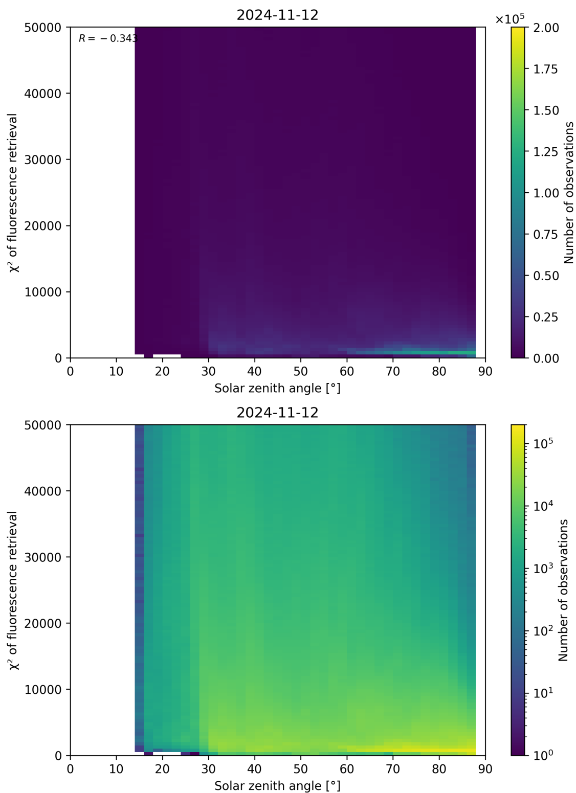
Figure 120: Scatter density plot of “Solar zenith angle” against “ \chi^2 of fluorescence retrieval” for 2024-11-11 to 2024-11-13.
