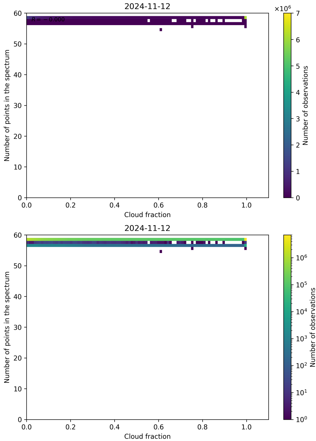
Figure 81: Scatter density plot of “Cloud fraction” against “Number of points in the spectrum” for 2024-11-11 to 2024-11-13.
