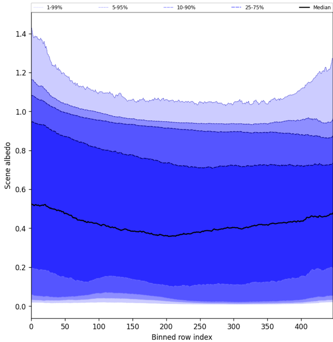
Figure 51: Along track statistics of “Scene albedo” for 2024-11-11 to 2024-11-13
