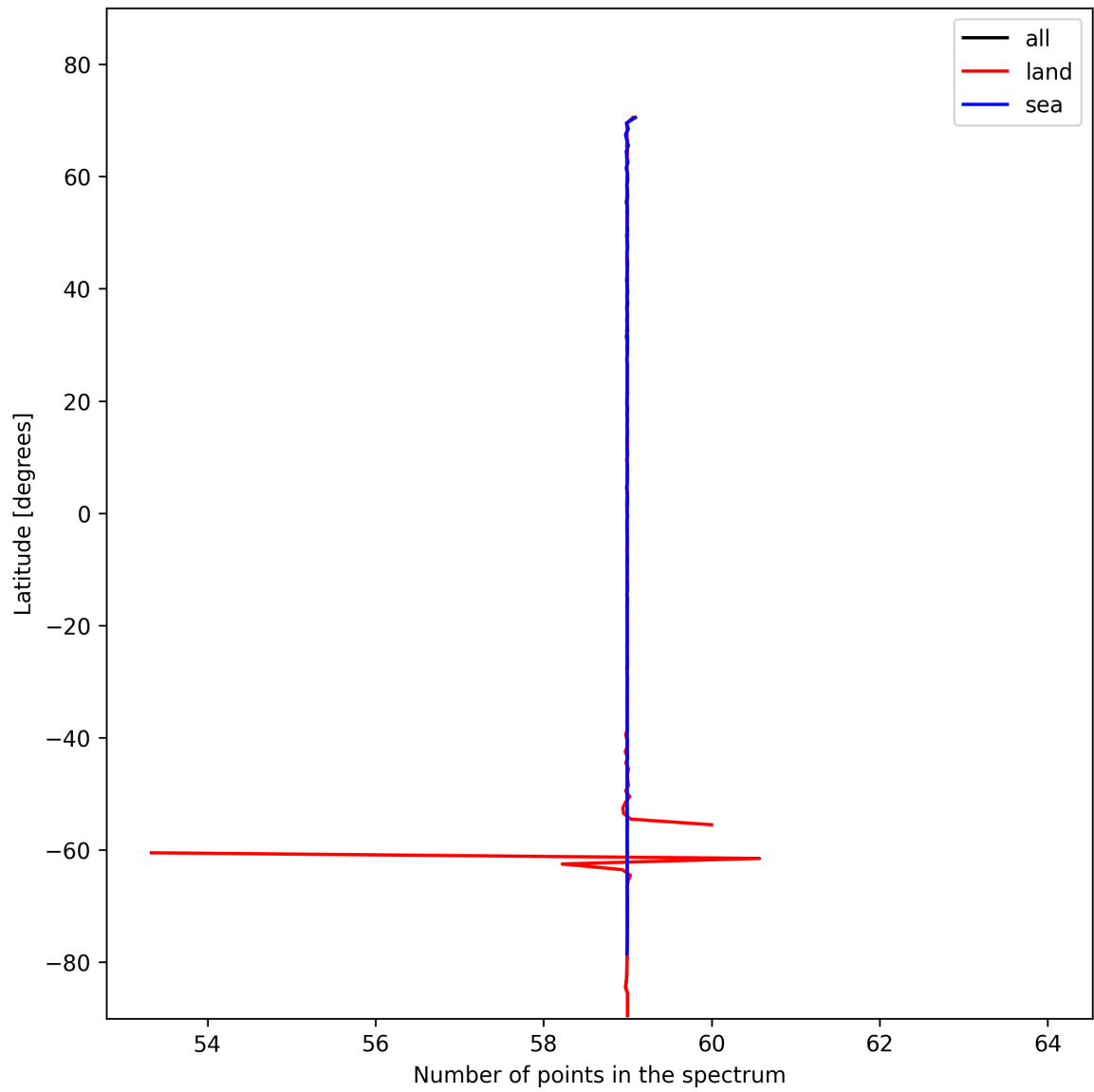
Figure 27: Zonal average of “Number of points in the spectrum” for 2024-11-11 to 2024-11-13.
