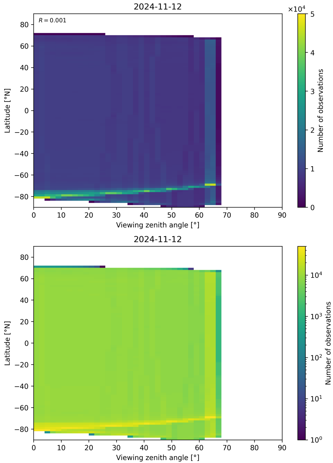
Figure 135: Scatter density plot of “Viewing zenith angle” against “Latitude” for 2024-11-11 to 2024-11-13.
