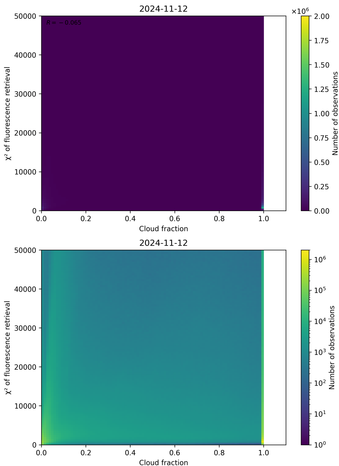
Figure 78: Scatter density plot of “Cloud fraction” against “ \chi^2 of fluorescence retrieval” for 2024-11-11 to 2024-11-13.
