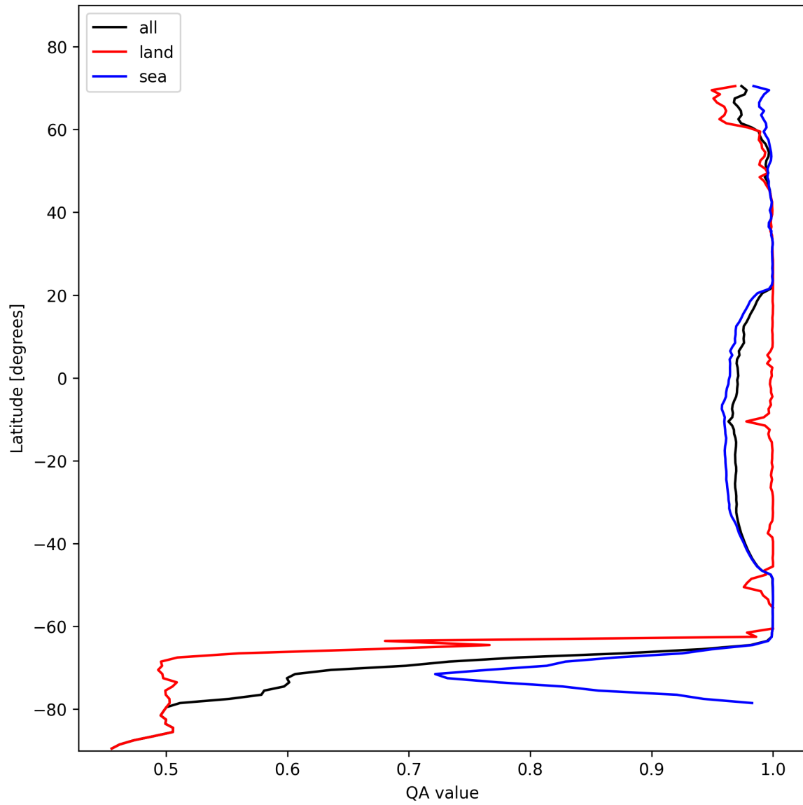
Figure 12: Zonal average of “QA value” for 2024-11-11 to 2024-11-13.
