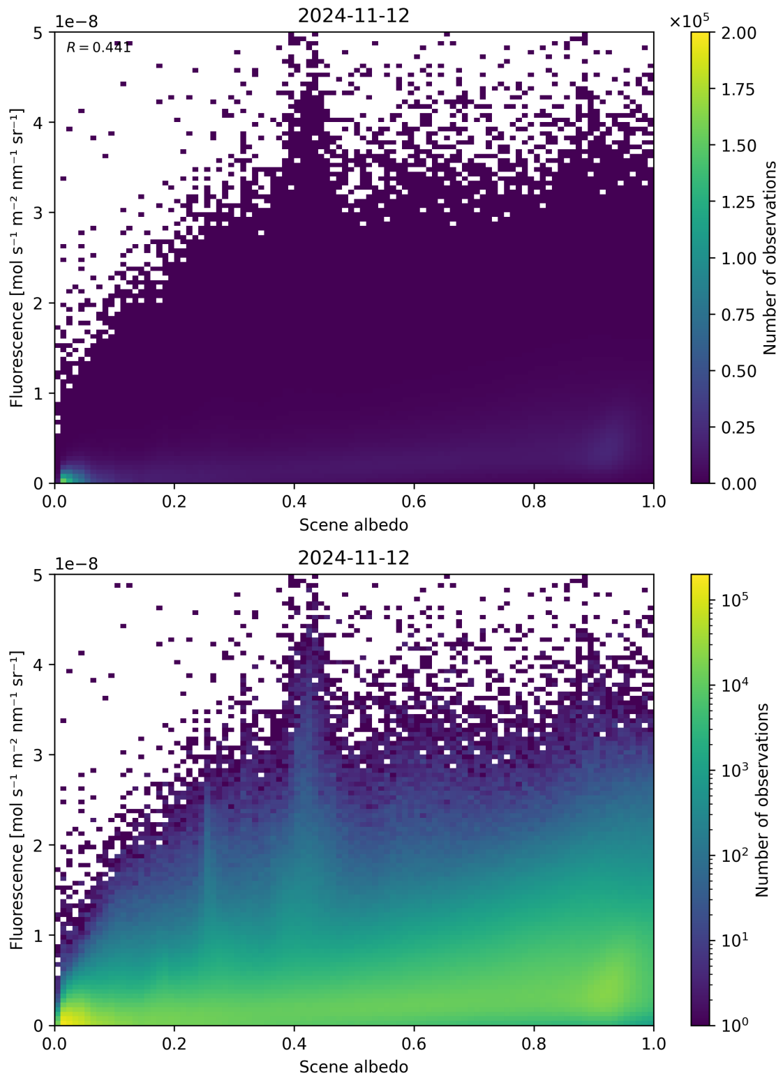
Figure 114: Scatter density plot of “Scene albedo” against “Fluorescence” for 2024-11-11 to 2024-11-13.
