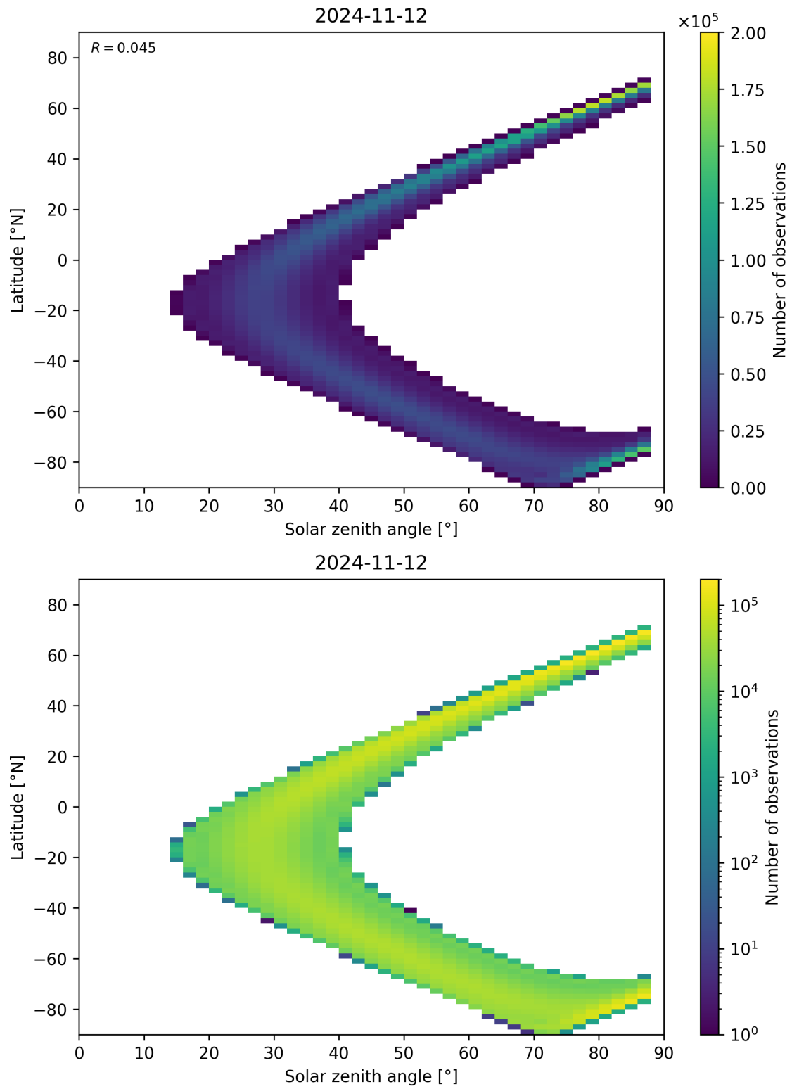
Figure 124: Scatter density plot of “Solar zenith angle” against “Latitude” for 2024-11-11 to 2024-11-13.
