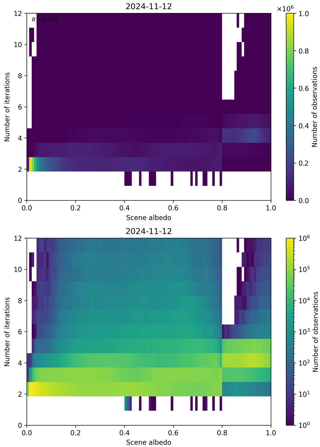
Figure 115: Scatter density plot of “Scene albedo” against “Number of iterations” for 2024-11-11 to 2024-11-13.
