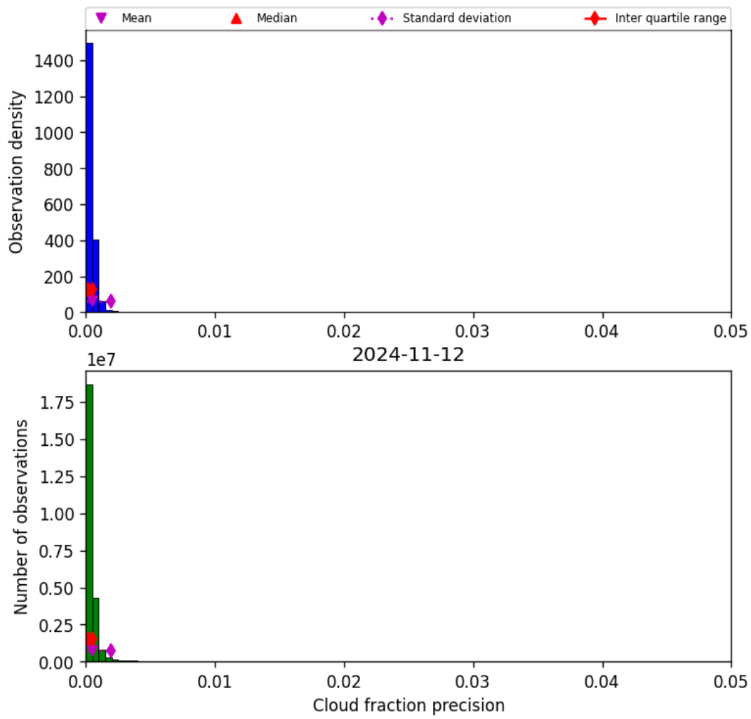
Figure 33: Histogram of “Cloud fraction precision” for 2024-11-11 to 2024-11-13
