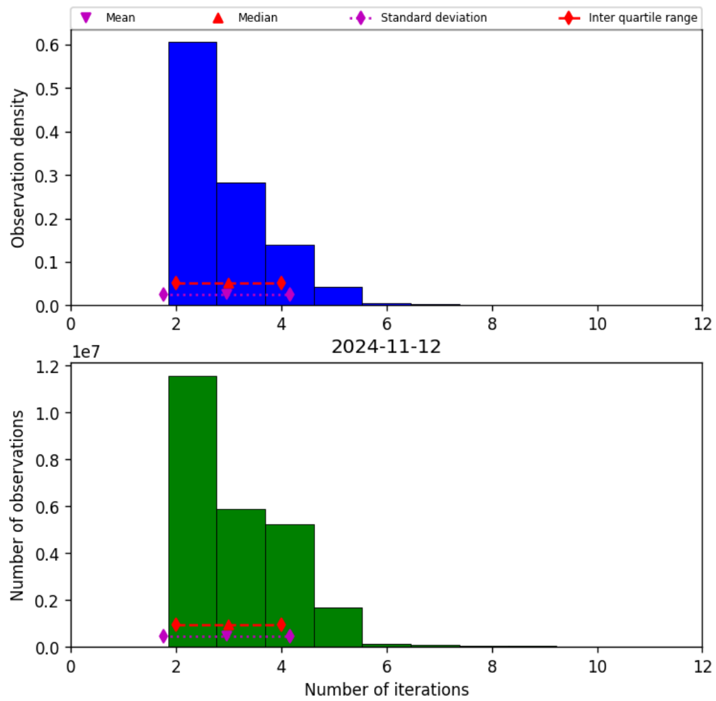
Figure 39: Histogram of “Number of iterations” for 2024-11-11 to 2024-11-13
