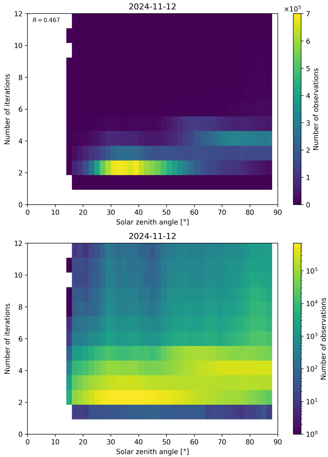
Figure 125: Scatter density plot of “Solar zenith angle” against “Number of iterations” for 2024-11-11 to 2024-11-13.
