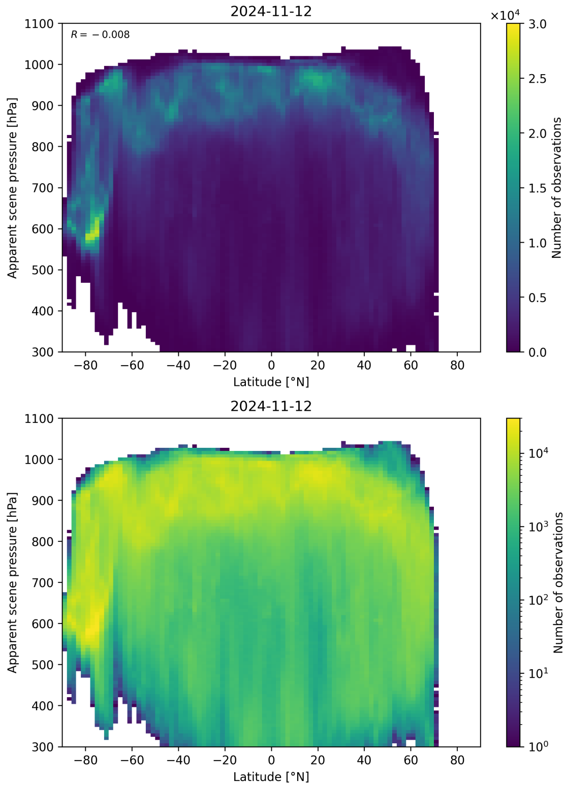
Figure 96: Scatter density plot of “Latitude” against “Apparent scene pressure” for 2024-11-11 to 2024-11-13.
