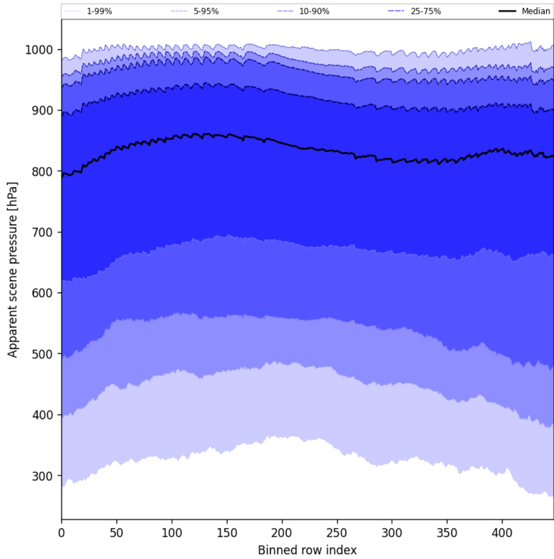
Figure 53: Along track statistics of “Apparent scene pressure” for 2024-11-11 to 2024-11-13
