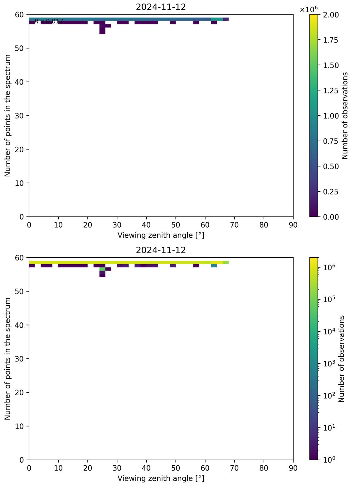
Figure 137: Scatter density plot of “Viewing zenith angle” against “Number of points in the spectrum” for 2024-11-11 to 2024-11-13.
