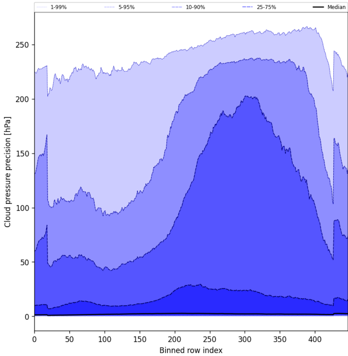
Figure 48: Along track statistics of “Cloud pressure precision” for 2024-11-11 to 2024-11-13
