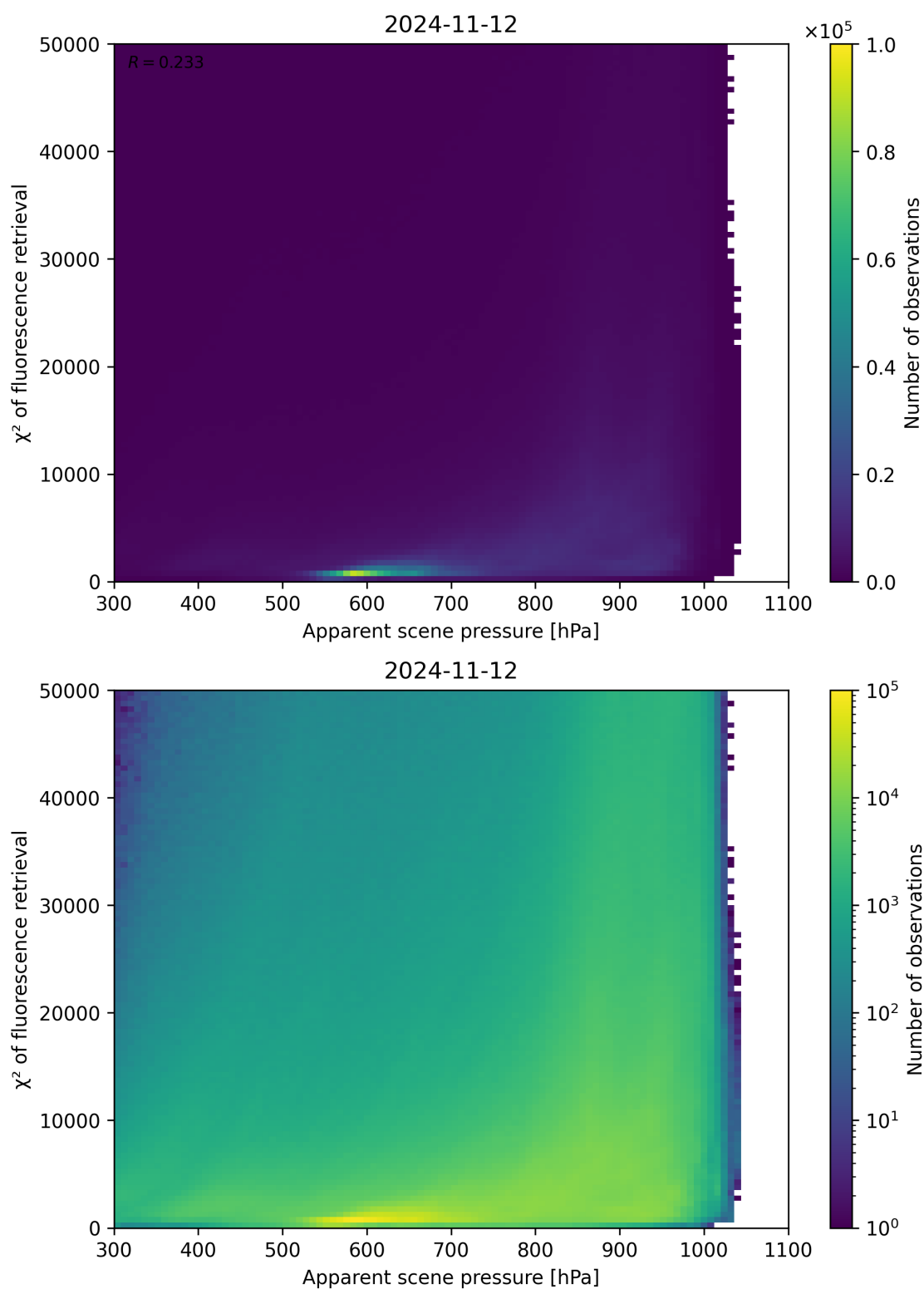
Figure 64: Scatter density plot of “Apparent scene pressure” against “ \chi^2 of fluorescence retrieval” for 2024-11-11 to 2024-11-13.
