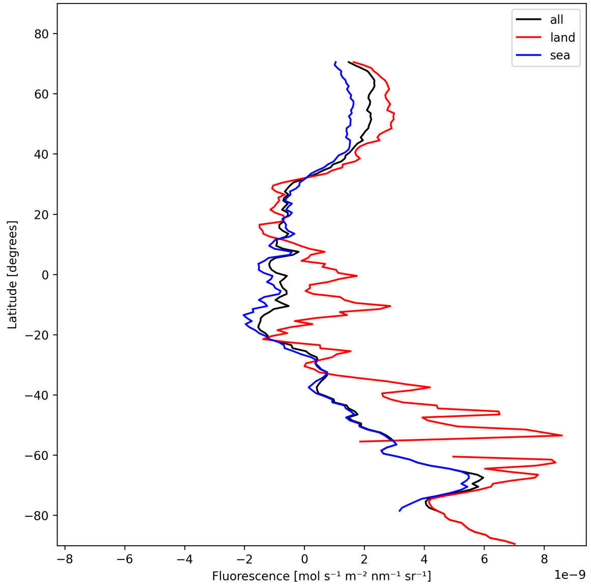
Figure 23: Zonal average of “Fluorescence” for 2024-11-11 to 2024-11-13.
