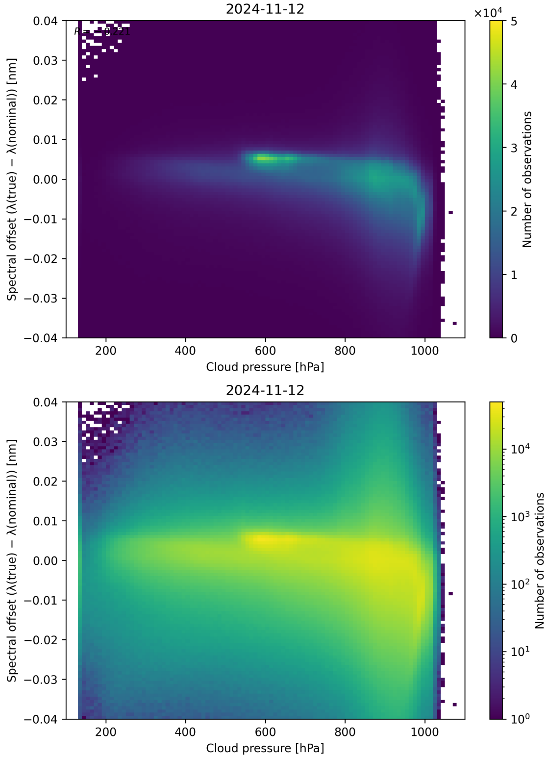
Figure 92: Scatter density plot of “Cloud pressure” against “Spectral offset ( \lambda_{\text{true}} - \lambda_{\text{nominal}} )” for 2024-11-11 to 2024-11-13.
