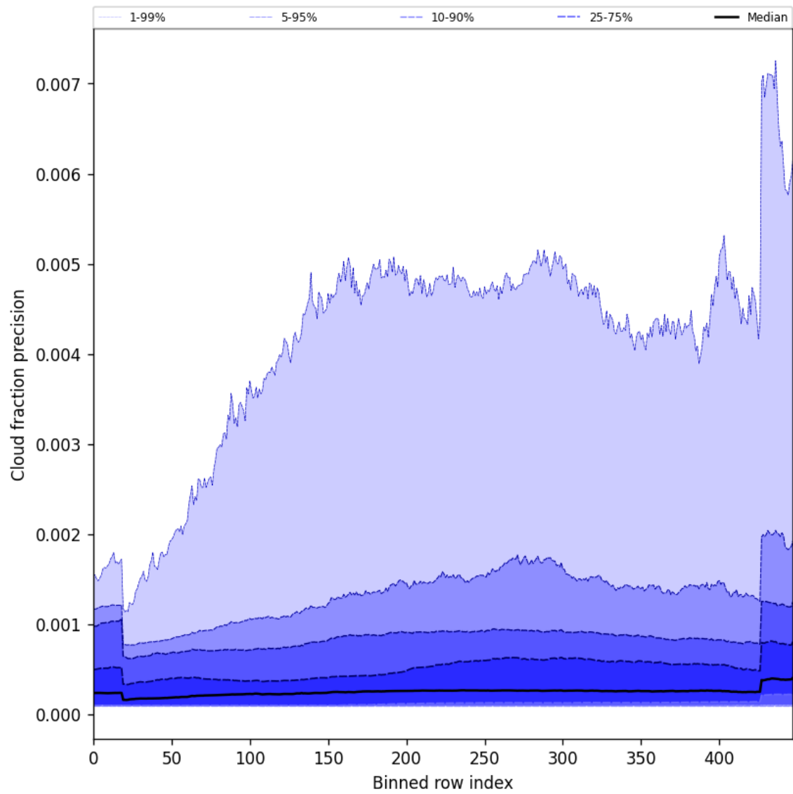
Figure 50: Along track statistics of “Cloud fraction precision” for 2024-11-11 to 2024-11-13
