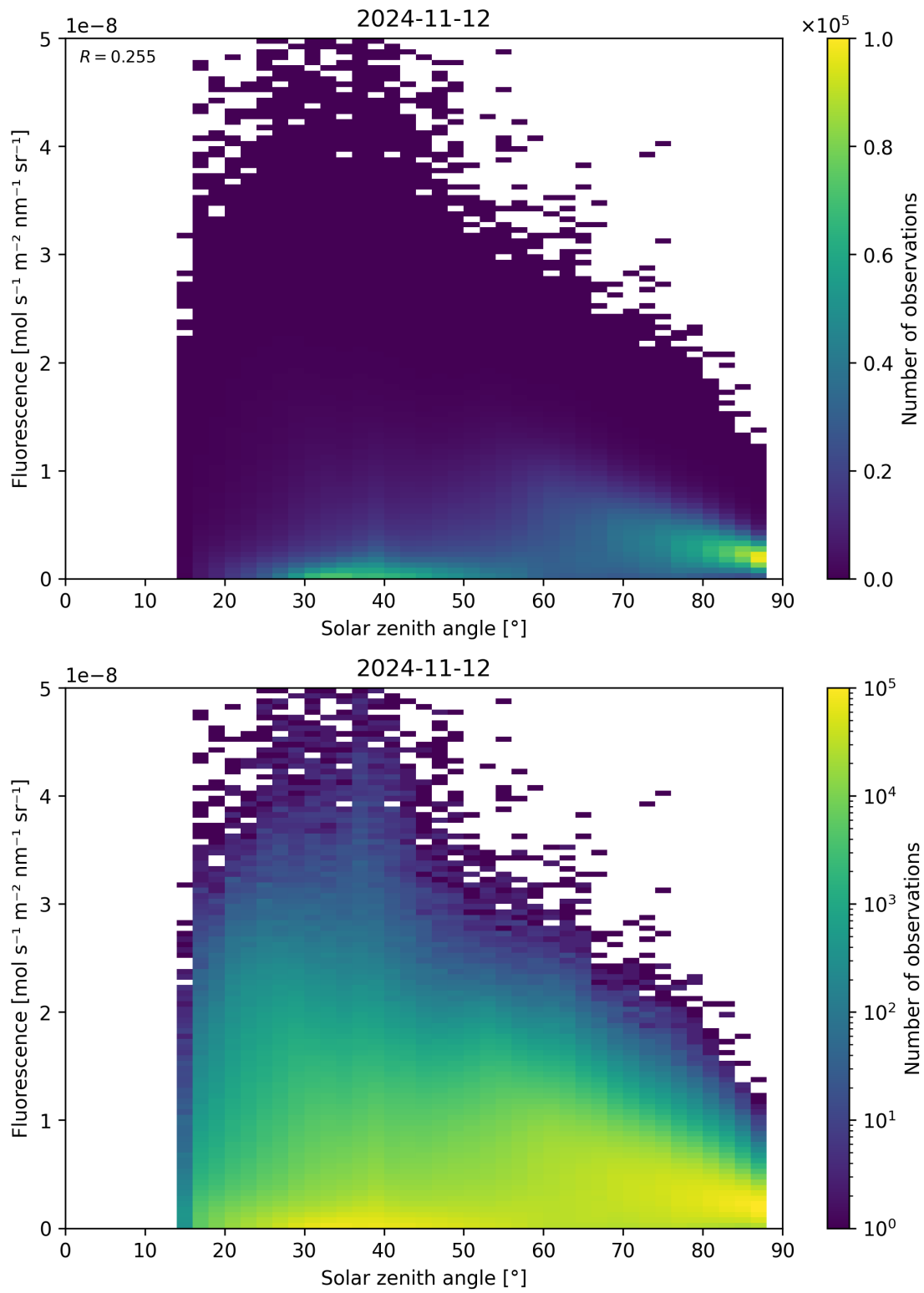
Figure 123: Scatter density plot of “Solar zenith angle” against “Fluorescence” for 2024-11-11 to 2024-11-13.
