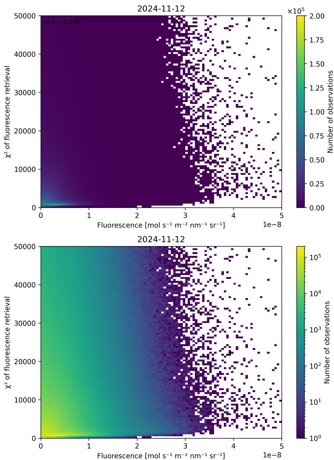
Figure 93: Scatter density plot of “Fluorescence” against “ \chi^2 of fluorescence retrieval” for 2024-11-11 to 2024-11-13.
