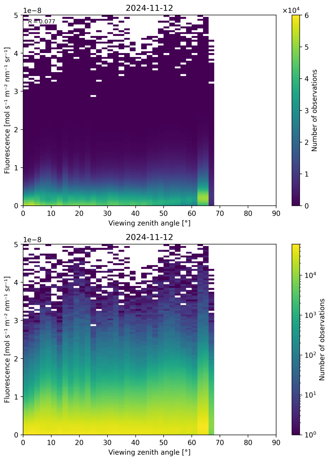
Figure 134: Scatter density plot of “Viewing zenith angle” against “Fluorescence” for 2024-11-11 to 2024-11-13.
