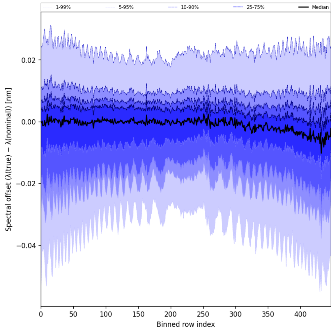
Figure 62: Along track statistics of “Spectral offset ( \lambda_{\text{true}} - \lambda_{\text{nominal}} )” for 2024-11-11 to 2024-11-13
