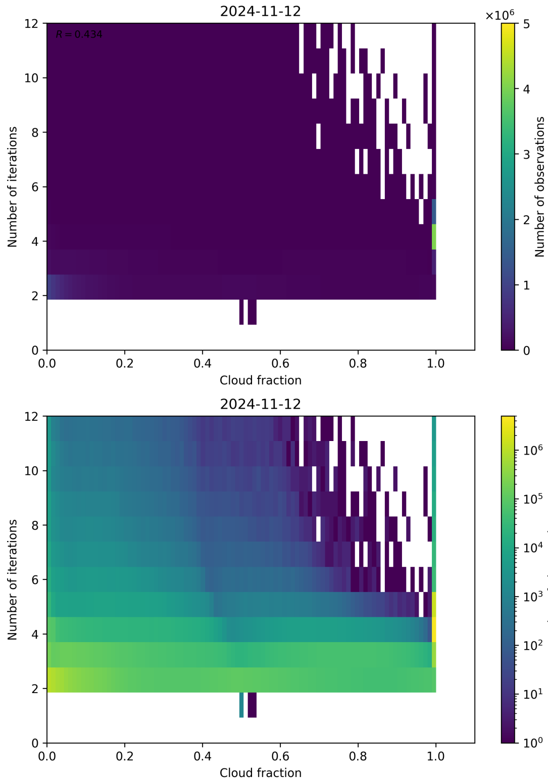
Figure 80: Scatter density plot of “Cloud fraction” against “Number of iterations” for 2024-11-11 to 2024-11-13.
