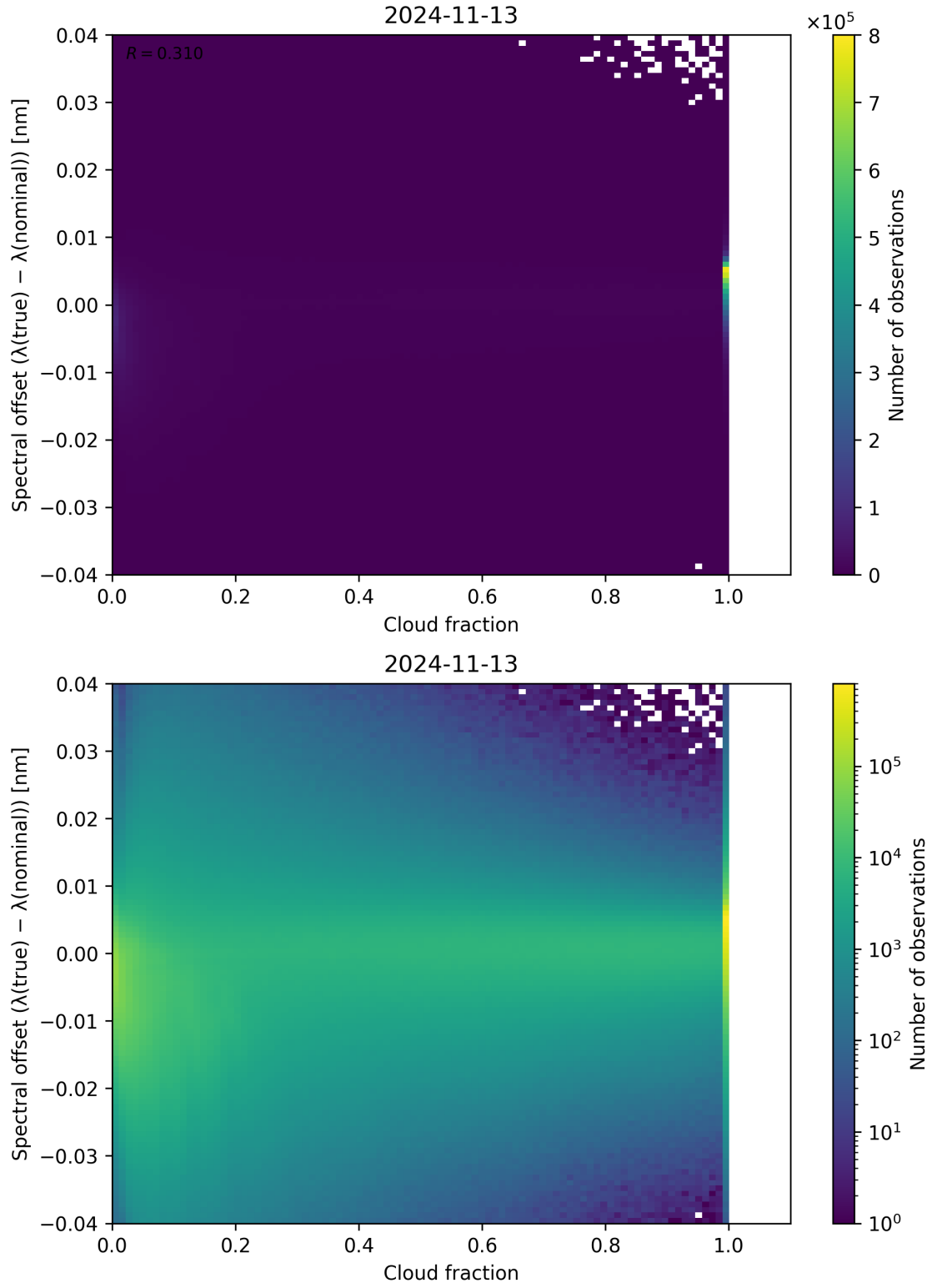
Figure 83: Scatter density plot of “Cloud fraction” against “Spectral offset ( \lambda_{\text{true}} - \lambda_{\text{nominal}} )” for 2024-11-12 to 2024-11-14.
