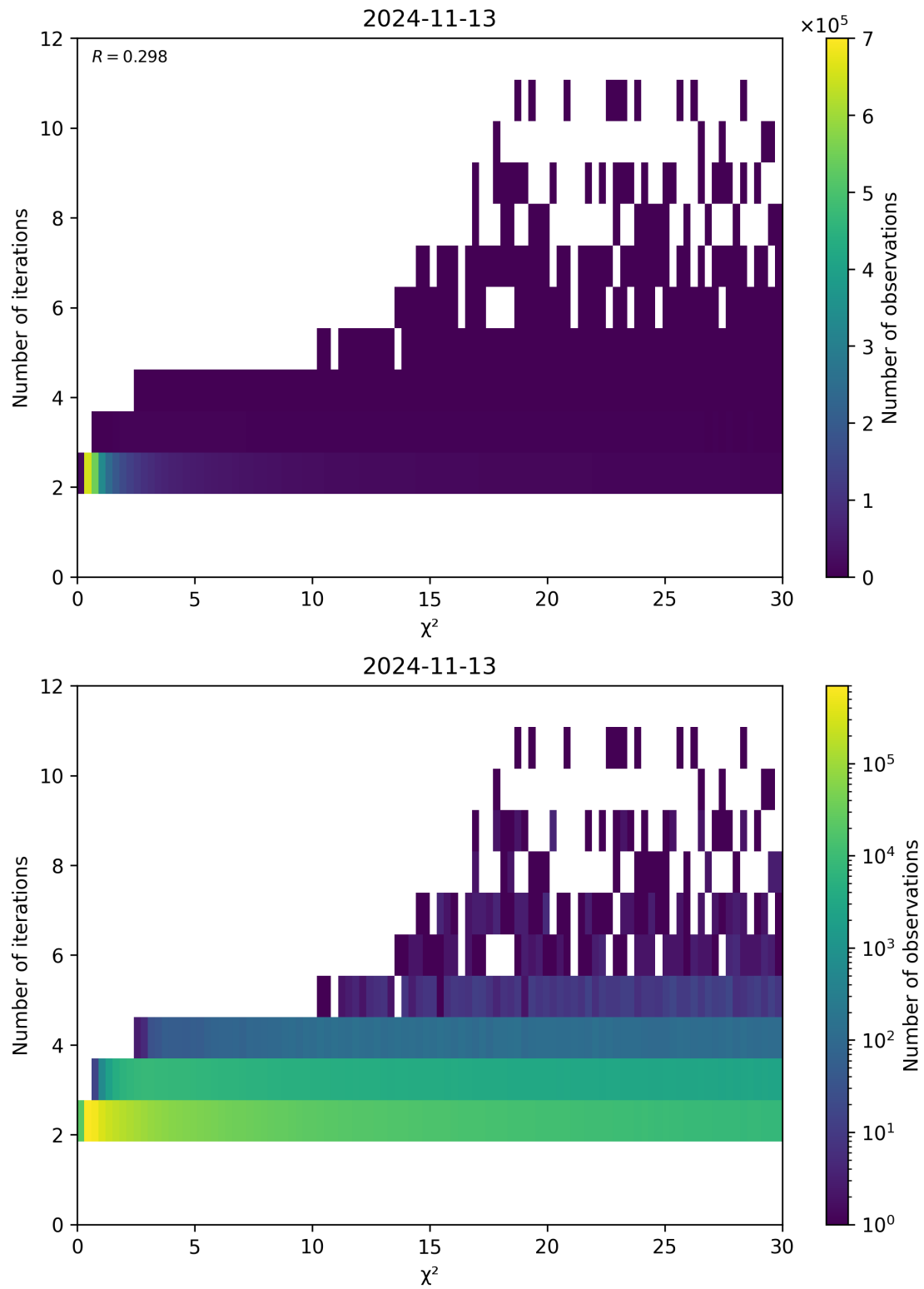
Figure 73: Scatter density plot of “ \chi^2 ” against “Number of iterations” for 2024-11-12 to 2024-11-14.
