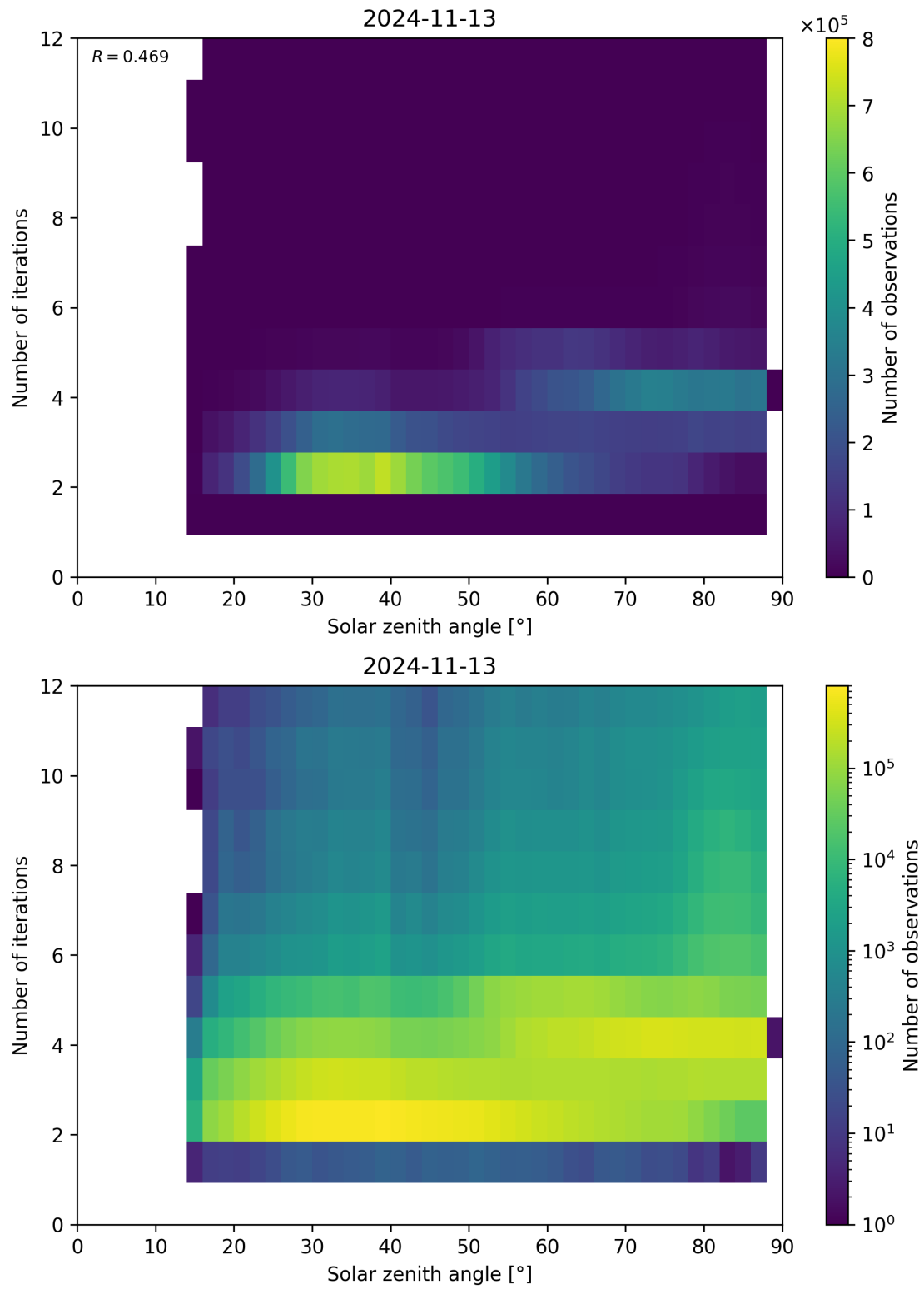
Figure 125: Scatter density plot of “Solar zenith angle” against “Number of iterations” for 2024-11-12 to 2024-11-14.
