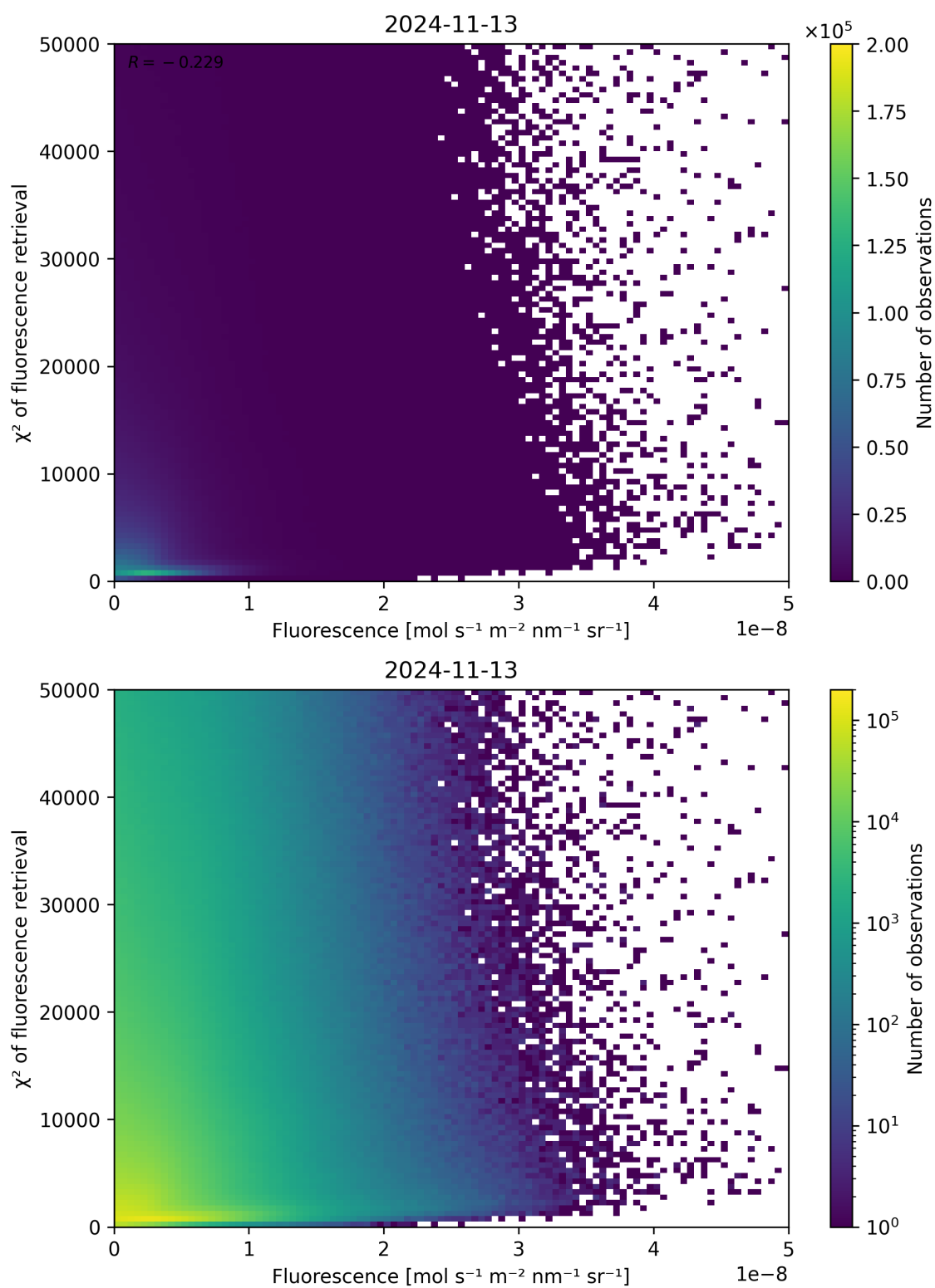
Figure 93: Scatter density plot of “Fluorescence” against “ \chi^2 of fluorescence retrieval” for 2024-11-12 to 2024-11-14.
