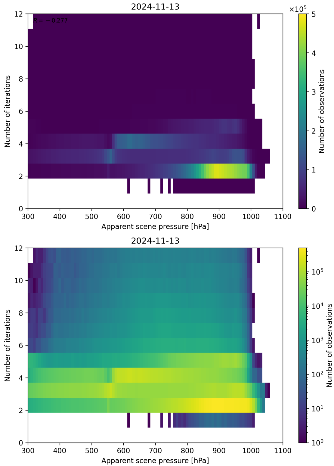
Figure 66: Scatter density plot of “Apparent scene pressure” against “Number of iterations” for 2024-11-12 to 2024-11-14.
