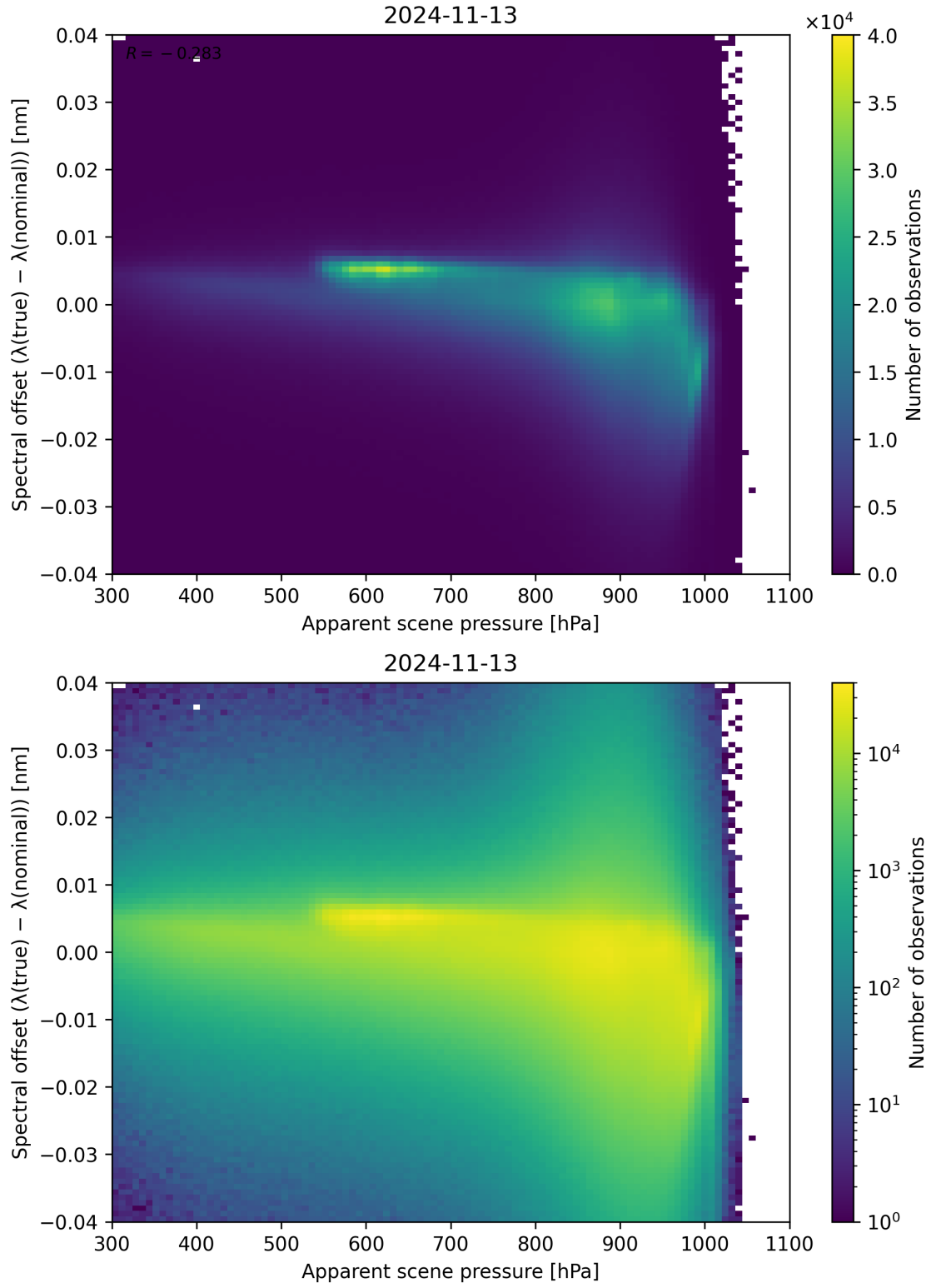
Figure 68: Scatter density plot of “Apparent scene pressure” against “Spectral offset ( \lambda_{\text{true}} - \lambda_{\text{nominal}} )” for 2024-11-12 to 2024-11-14.
