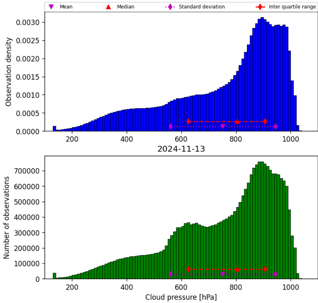
Figure 30: Histogram of “Cloud pressure” for 2024-11-12 to 2024-11-14
