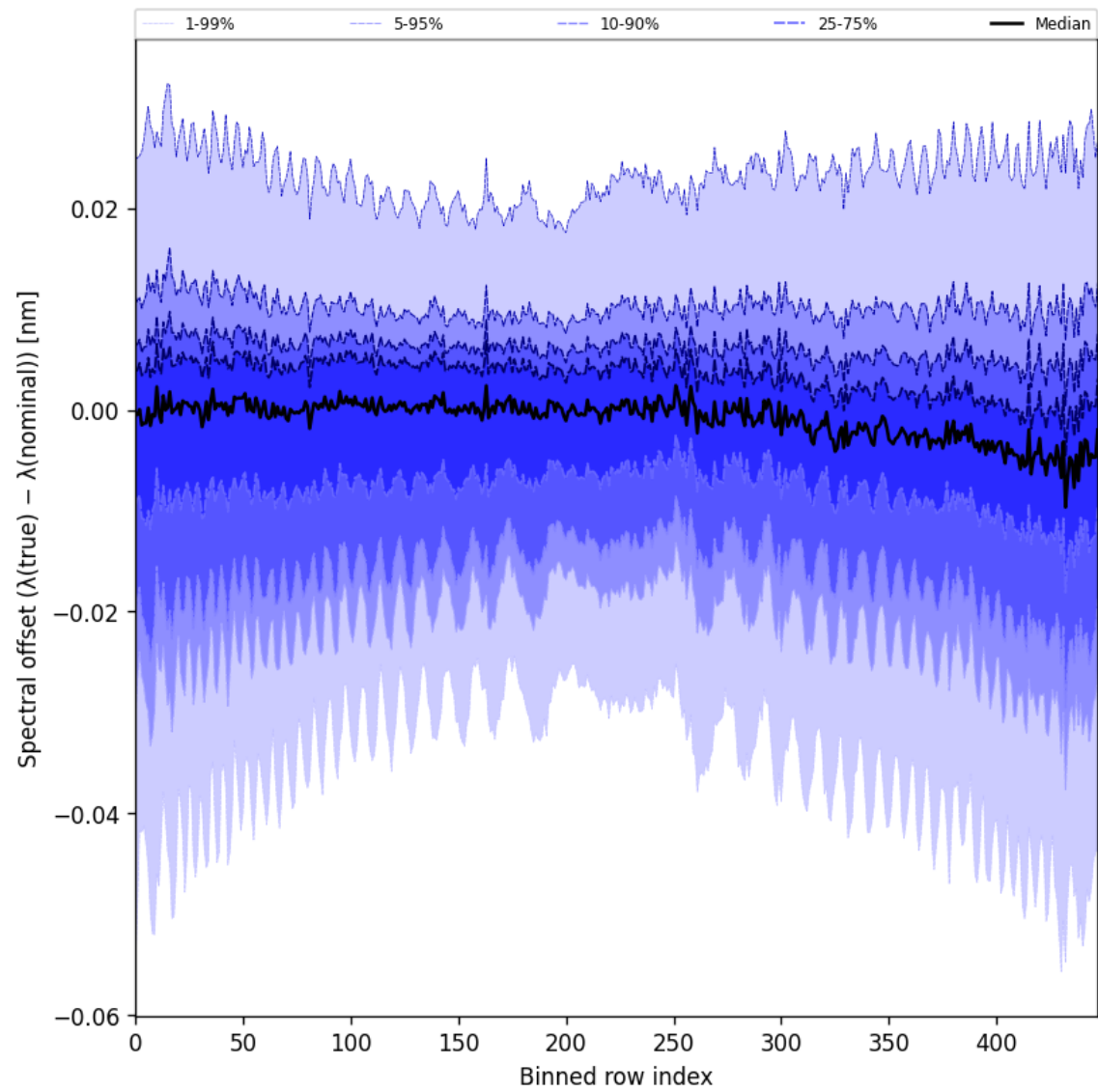
Figure 62: Along track statistics of “Spectral offset ( \lambda_{\text{true}} - \lambda_{\text{nominal}} )” for 2024-11-12 to 2024-11-14
