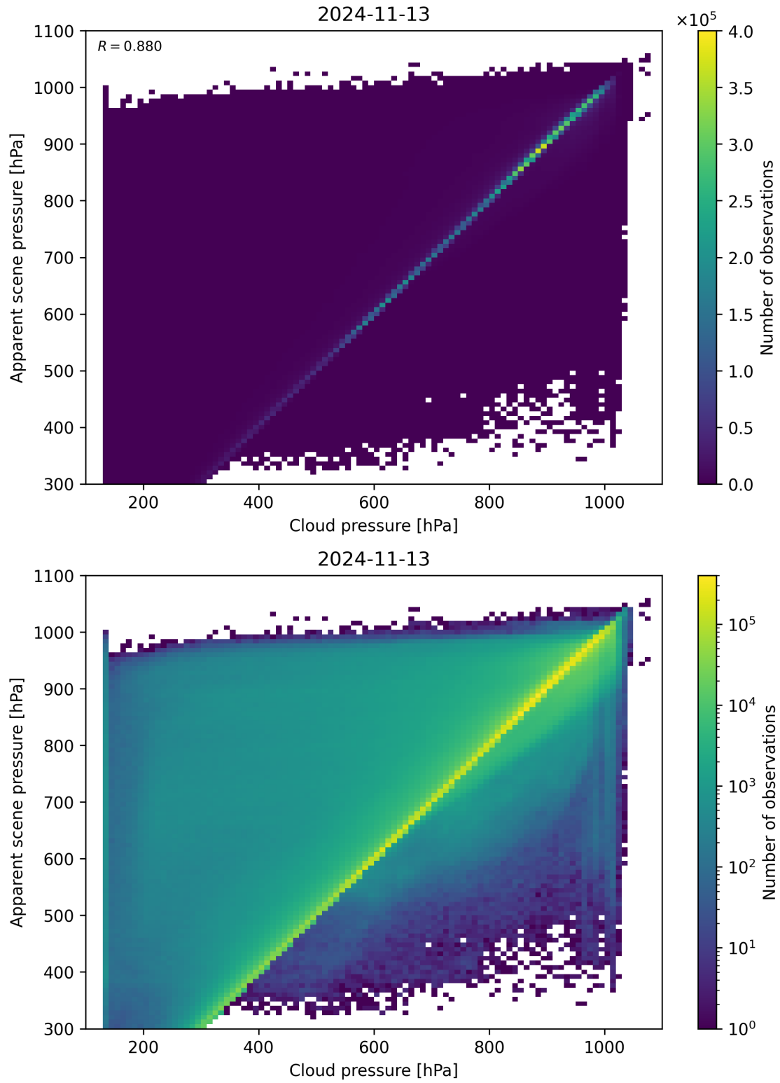
Figure 84: Scatter density plot of “Cloud pressure” against “Apparent scene pressure” for 2024-11-12 to 2024-11-14.
