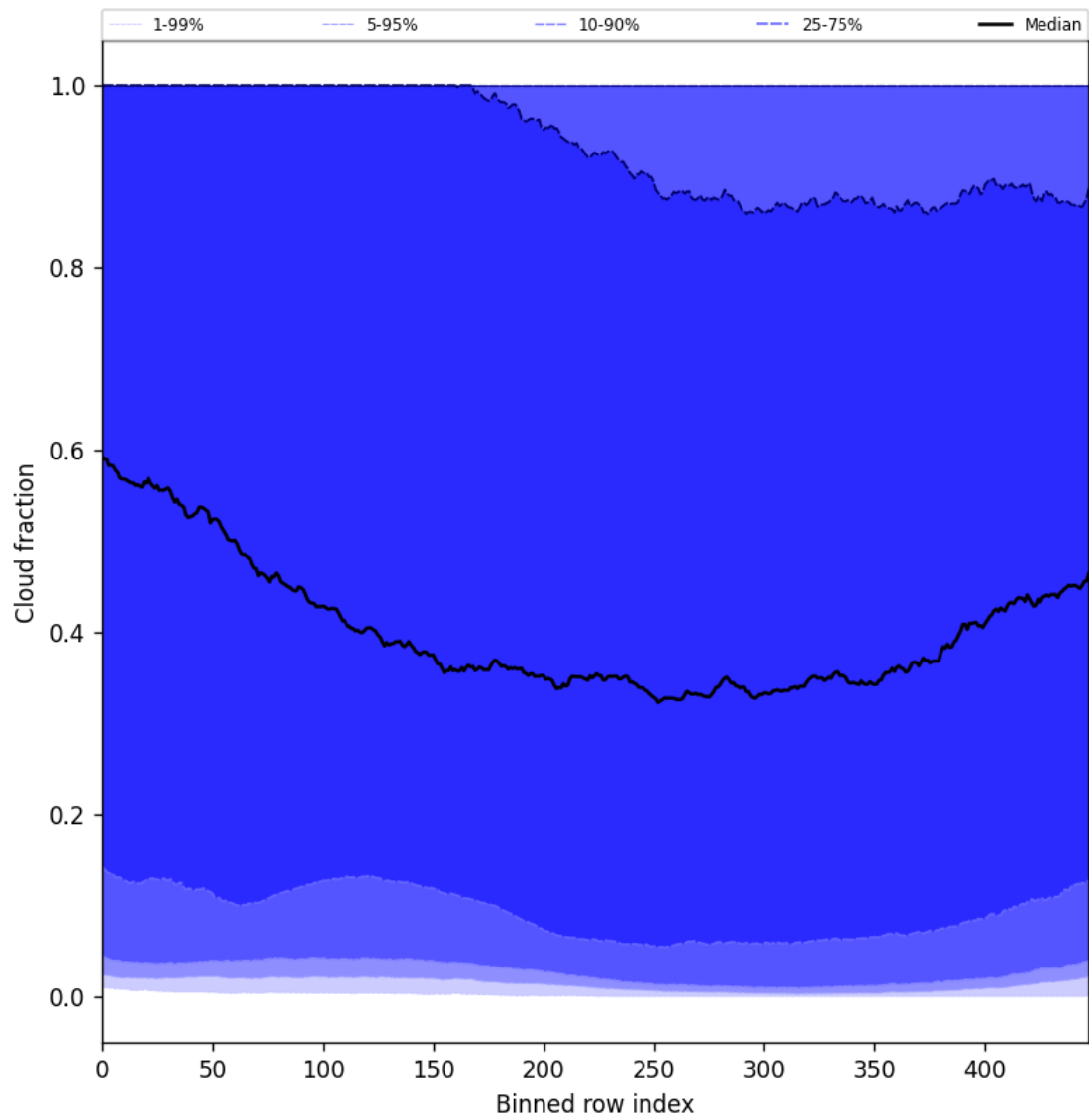
Figure 49: Along track statistics of “Cloud fraction” for 2024-11-12 to 2024-11-14
