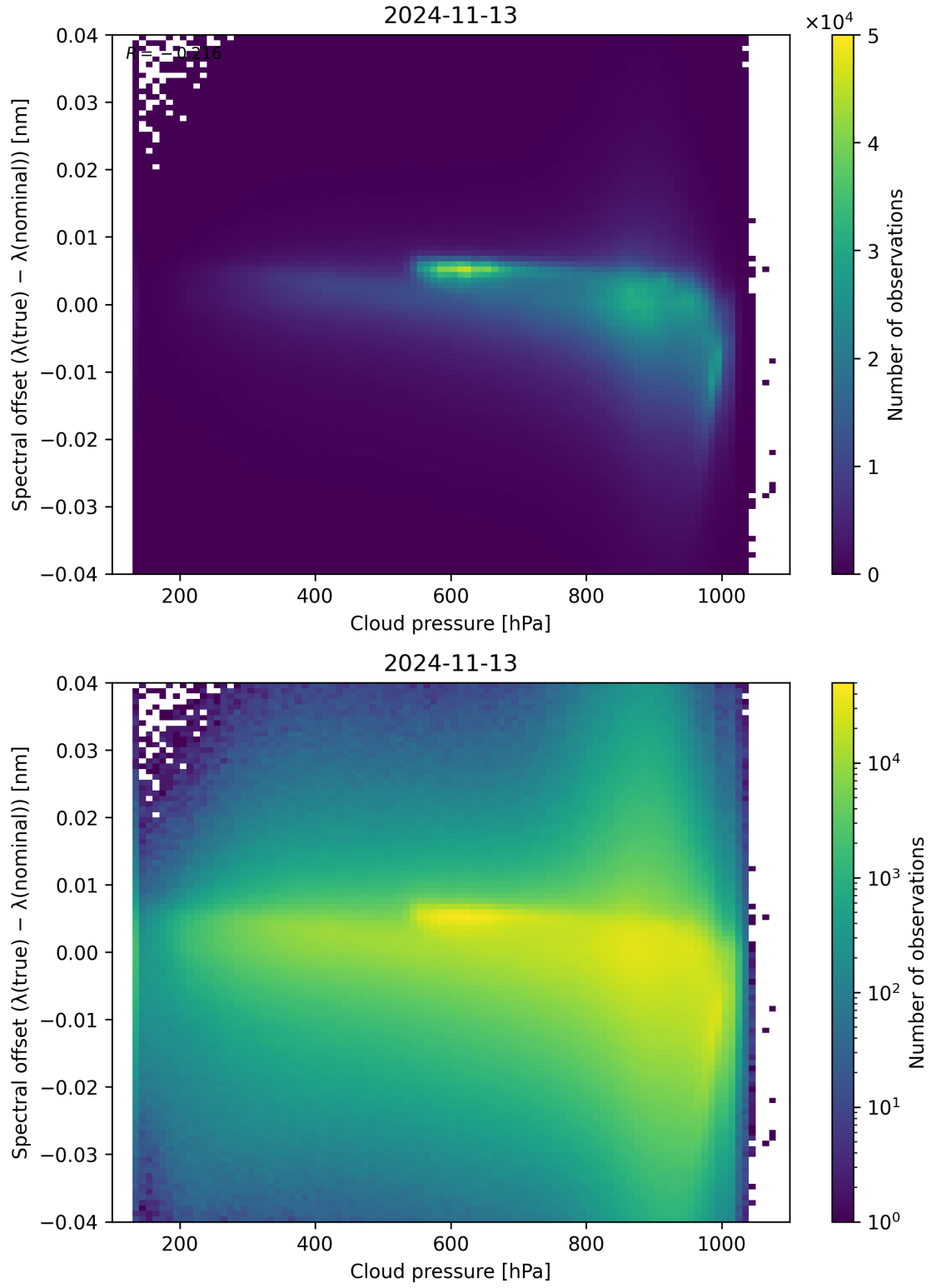
Figure 92: Scatter density plot of “Cloud pressure” against “Spectral offset ( \lambda_{\text{true}} - \lambda_{\text{nominal}} )” for 2024-11-12 to 2024-11-14.
