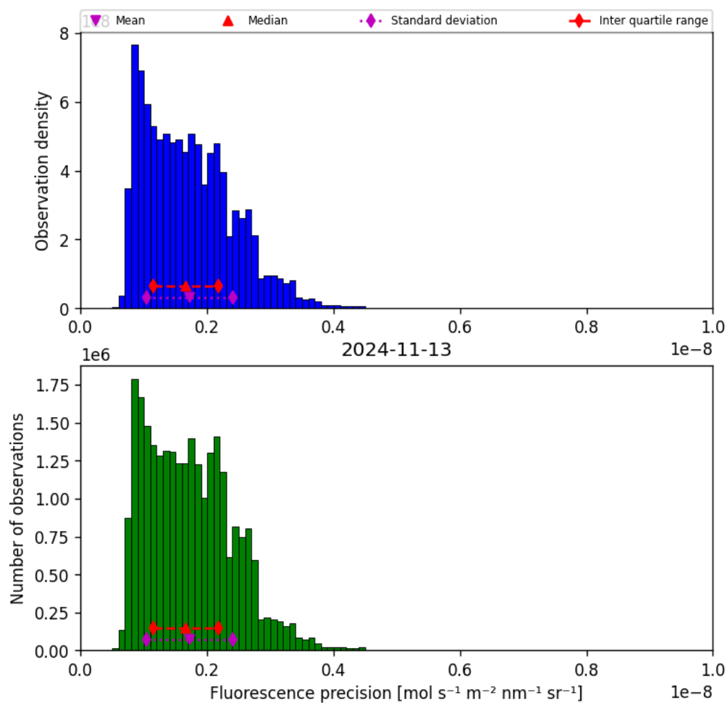
Figure 41: Histogram of “Fluorescence precision” for 2024-11-12 to 2024-11-14
