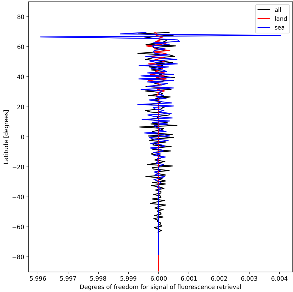
Figure 26: Zonal average of “Degrees of freedom for signal of fluorescence retrieval” for 2024-11-12 to 2024-11-14.
