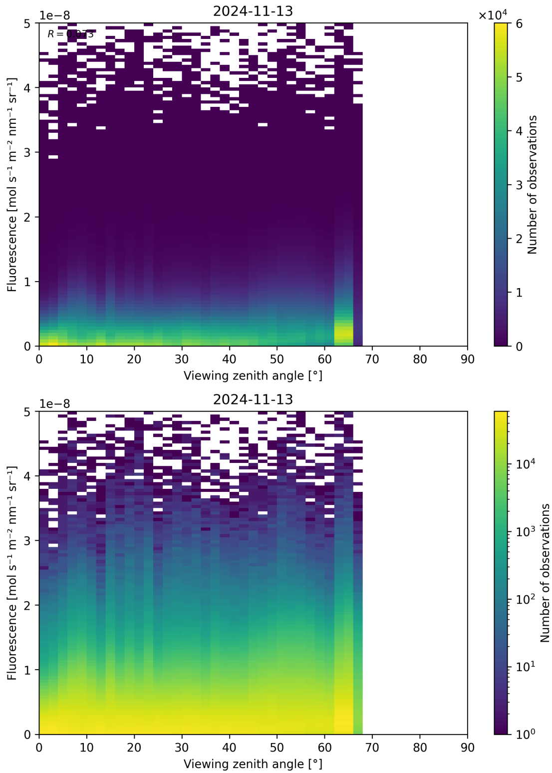
Figure 134: Scatter density plot of “Viewing zenith angle” against “Fluorescence” for 2024-11-12 to 2024-11-14.
