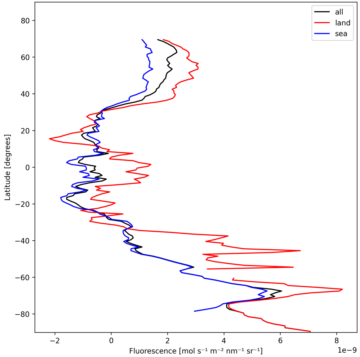
Figure 23: Zonal average of “Fluorescence” for 2024-11-12 to 2024-11-14.
