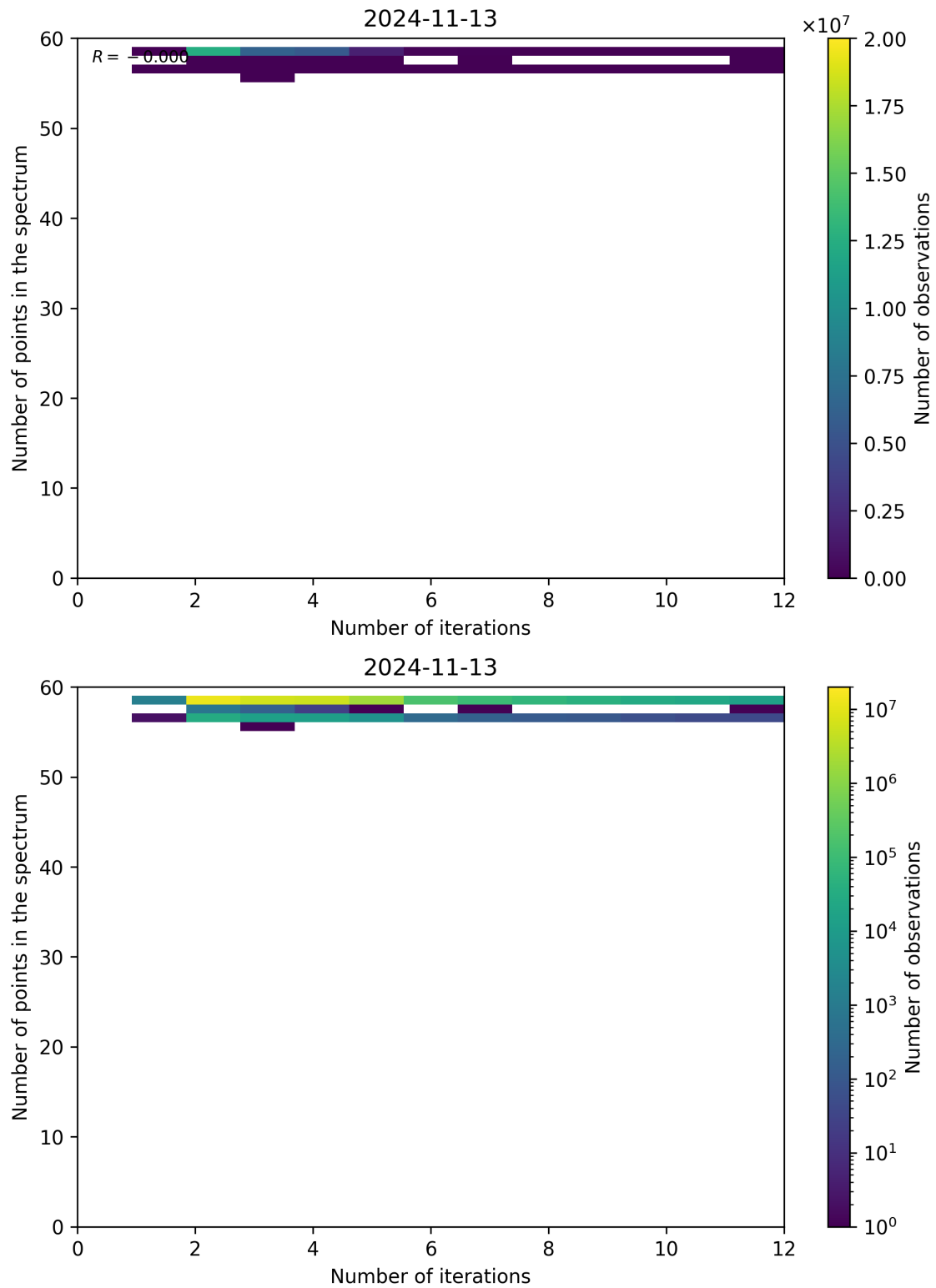
Figure 108: Scatter density plot of “Number of iterations” against “Number of points in the spectrum” for 2024-11-12 to 2024-11-14.
