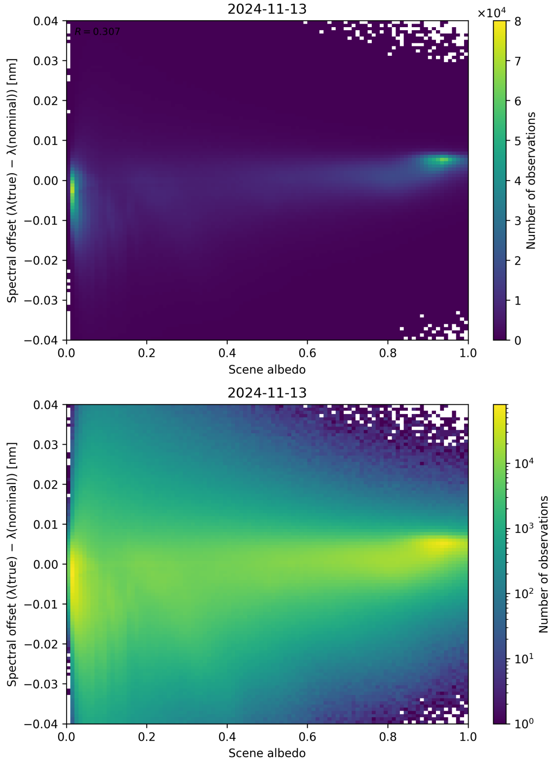
Figure 117: Scatter density plot of “Scene albedo” against “Spectral offset ( \lambda_{\text{true}} - \lambda_{\text{nominal}} )” for 2024-11-12 to 2024-11-14.
