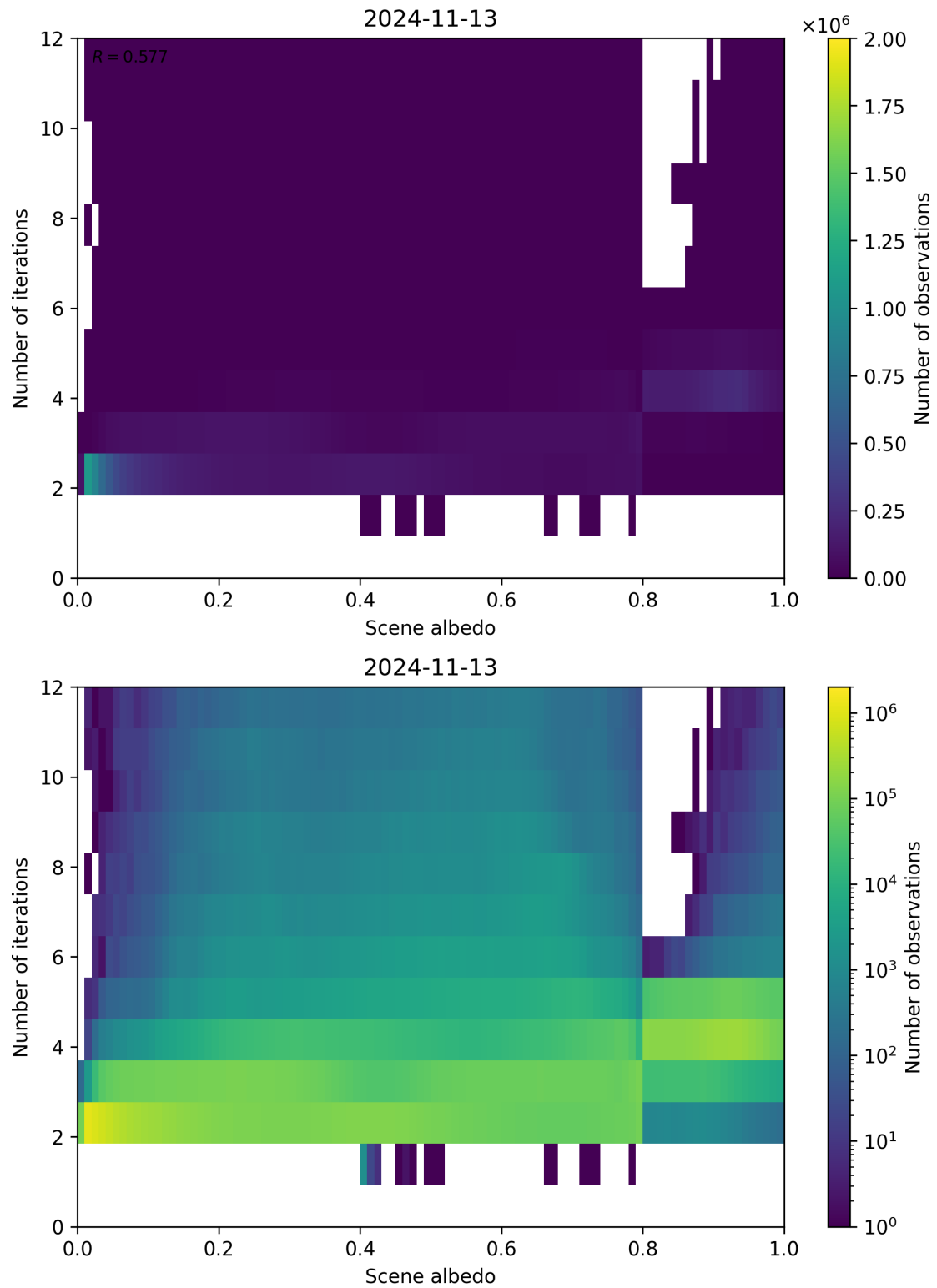
Figure 115: Scatter density plot of “Scene albedo” against “Number of iterations” for 2024-11-12 to 2024-11-14.
