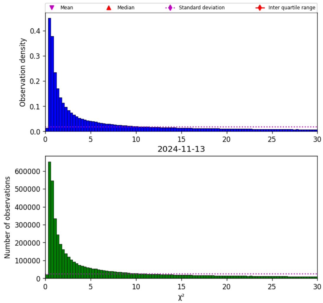
Figure 38: Histogram of “ \chi^2 ” for 2024-11-12 to 2024-11-14
