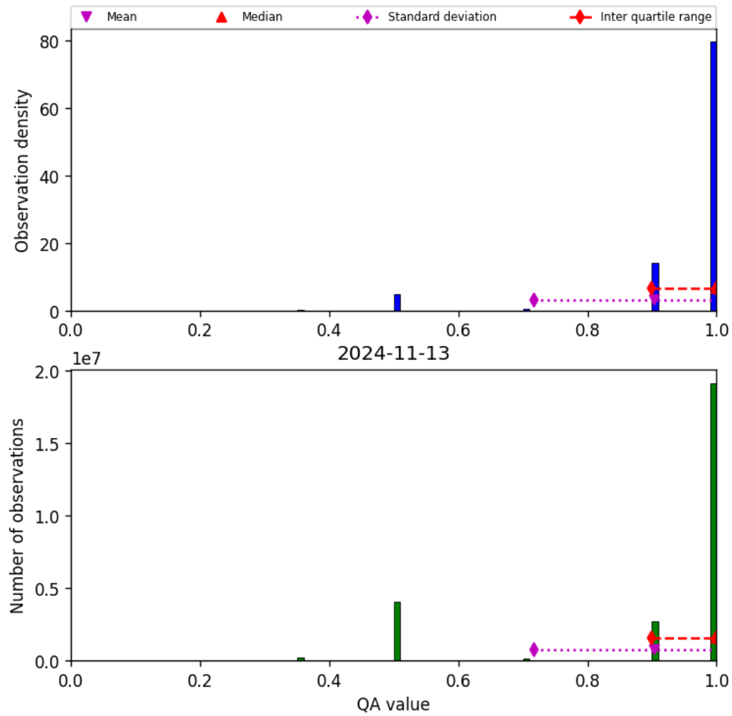
Figure 29: Histogram of “QA value” for 2024-11-12 to 2024-11-14
