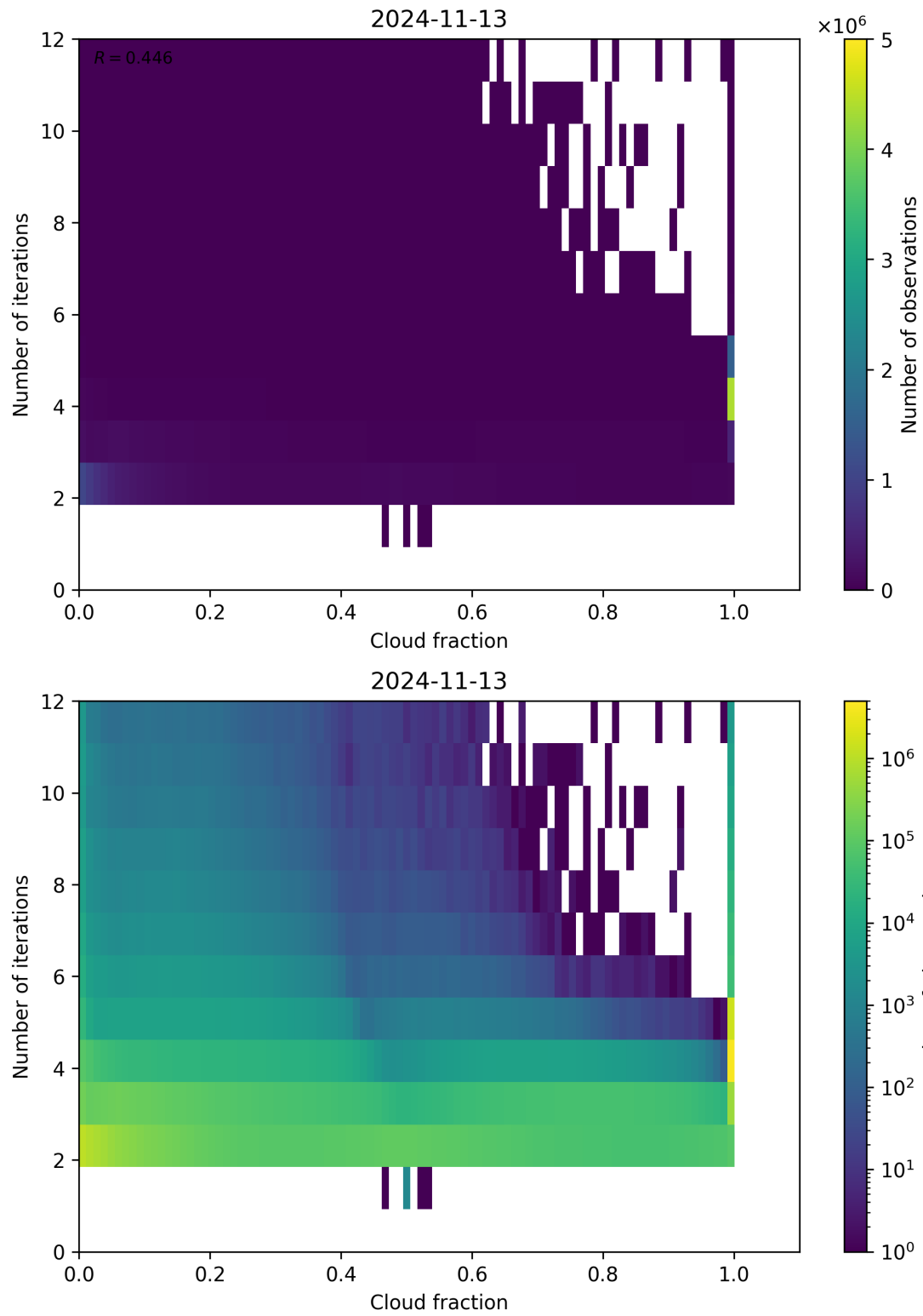
Figure 80: Scatter density plot of “Cloud fraction” against “Number of iterations” for 2024-11-12 to 2024-11-14.
