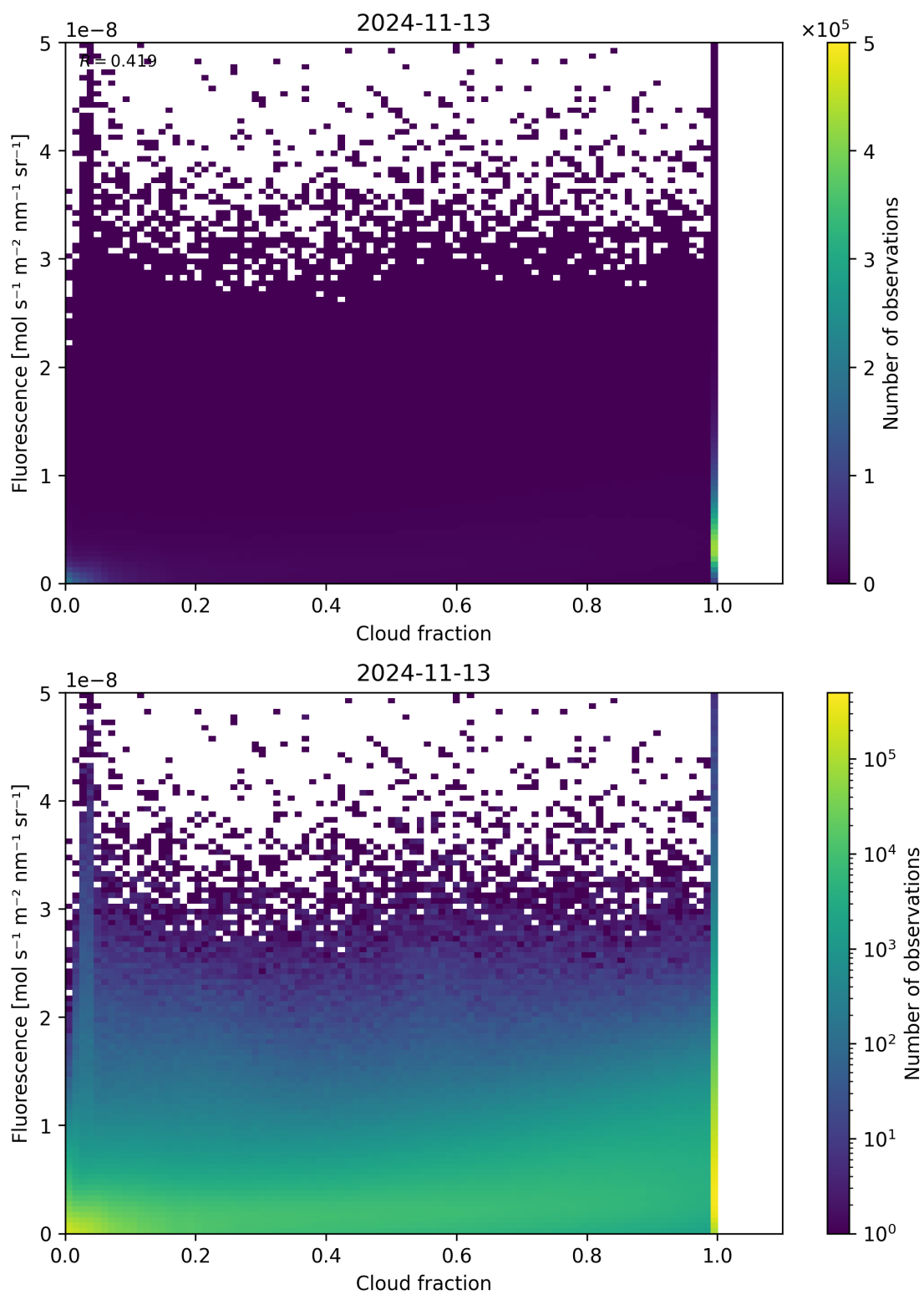
Figure 79: Scatter density plot of “Cloud fraction” against “Fluorescence” for 2024-11-12 to 2024-11-14.
