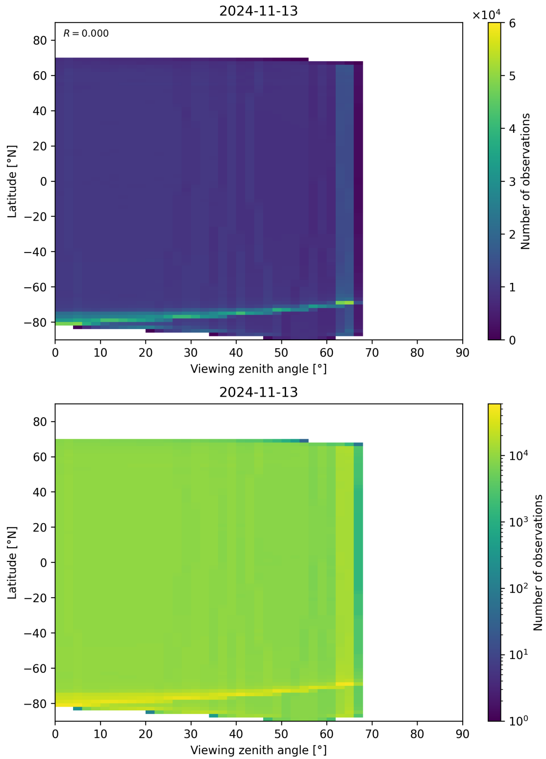
Figure 135: Scatter density plot of “Viewing zenith angle” against “Latitude” for 2024-11-12 to 2024-11-14.
