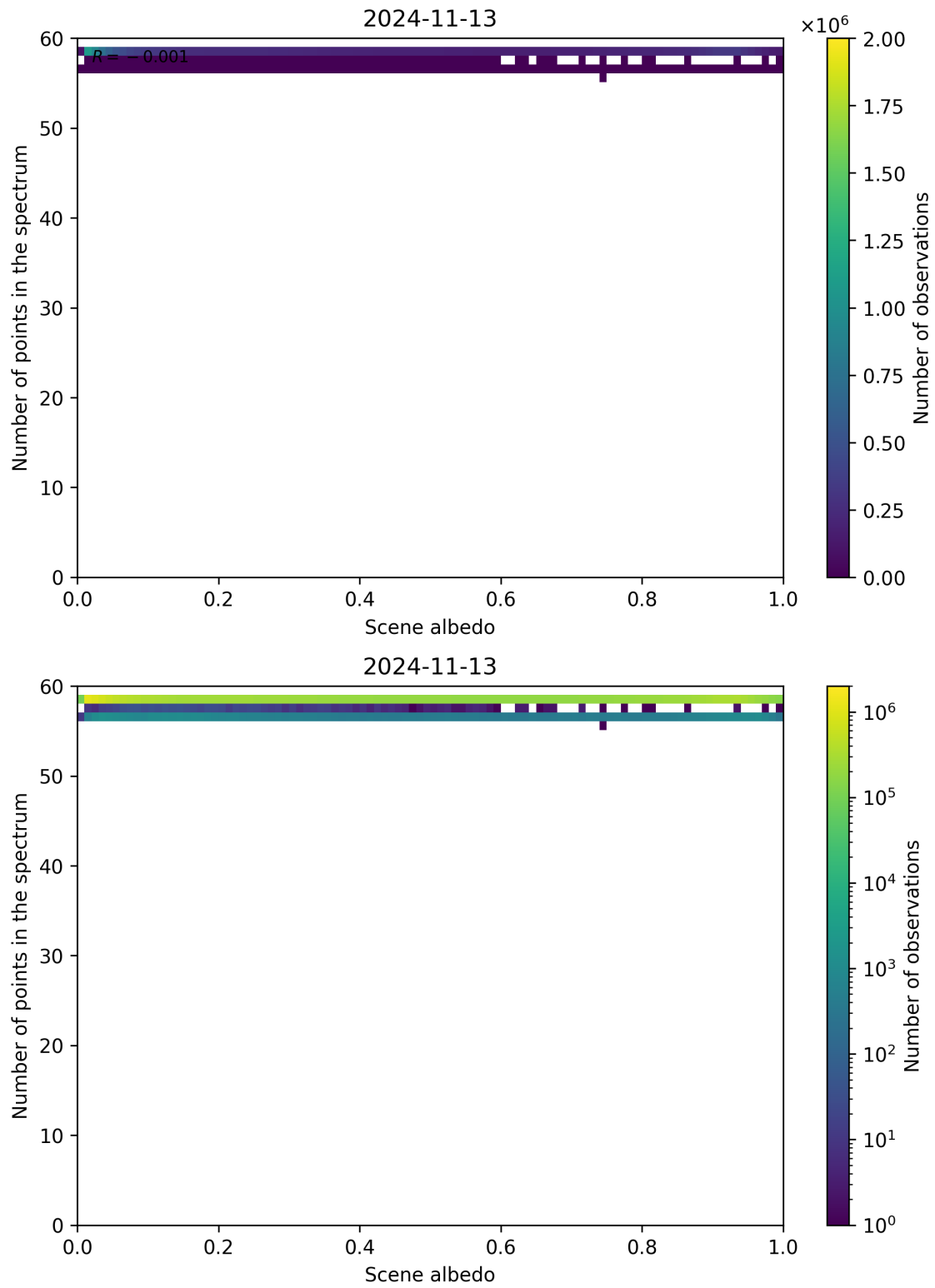
Figure 116: Scatter density plot of “Scene albedo” against “Number of points in the spectrum” for 2024-11-12 to 2024-11-14.
