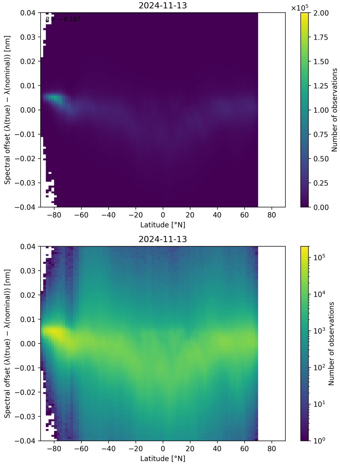
Figure 105: Scatter density plot of “Latitude” against “Spectral offset ( \lambda_{\text{true}} - \lambda_{\text{nominal}} )” for 2024-11-12 to 2024-11-14.
