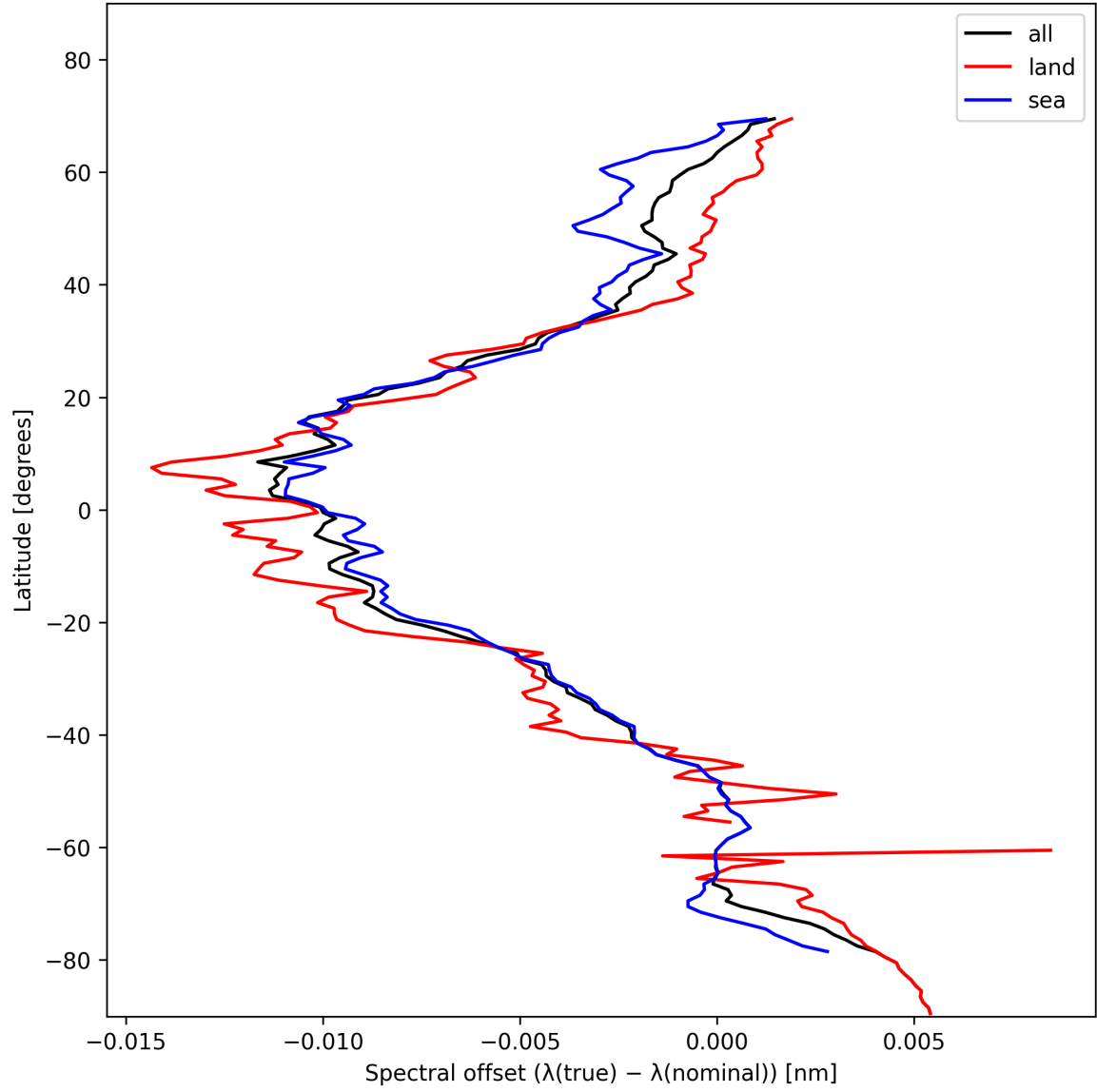
Figure 28: Zonal average of “Spectral offset ( \lambda_{\text{true}} - \lambda_{\text{nominal}} )” for 2024-11-14 to 2024-11-15.
