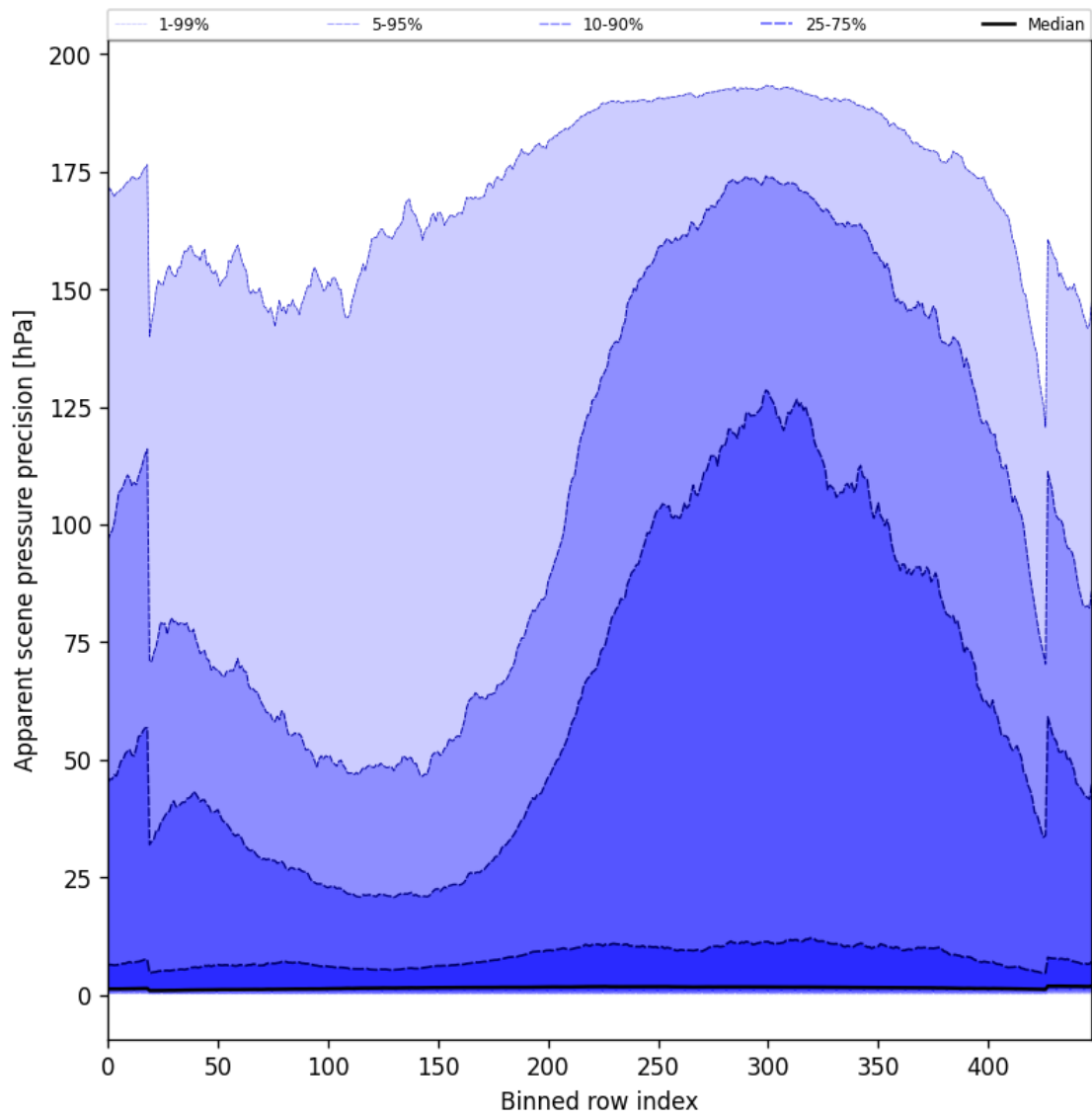
Figure 54: Along track statistics of “Apparent scene pressure precision” for 2024-11-14 to 2024-11-15
