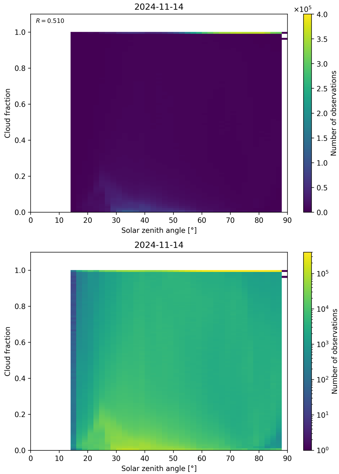
Figure 121: Scatter density plot of “Solar zenith angle” against “Cloud fraction” for 2024-11-14 to 2024-11-15.
