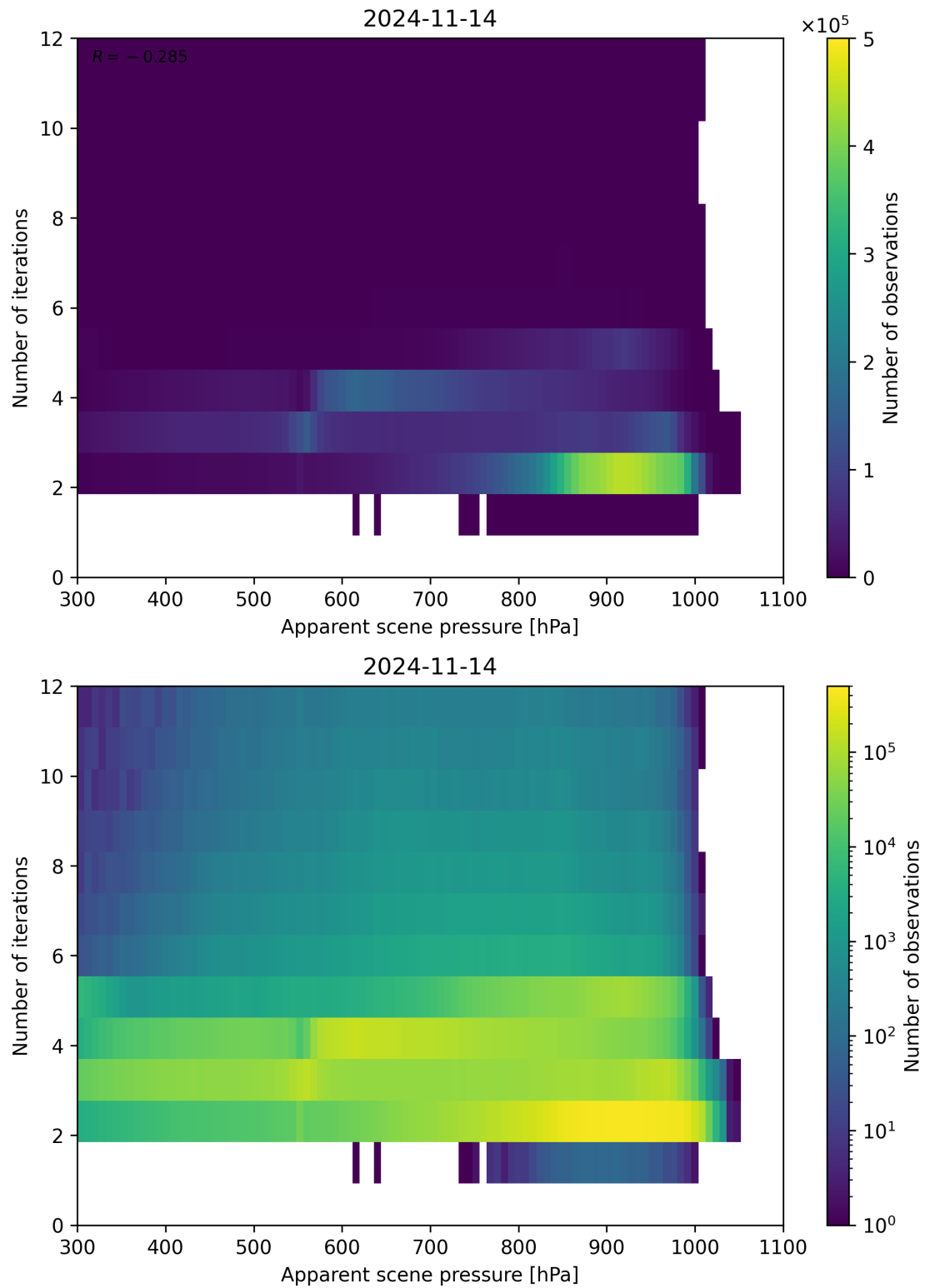
Figure 66: Scatter density plot of “Apparent scene pressure” against “Number of iterations” for 2024-11-14 to 2024-11-15.
