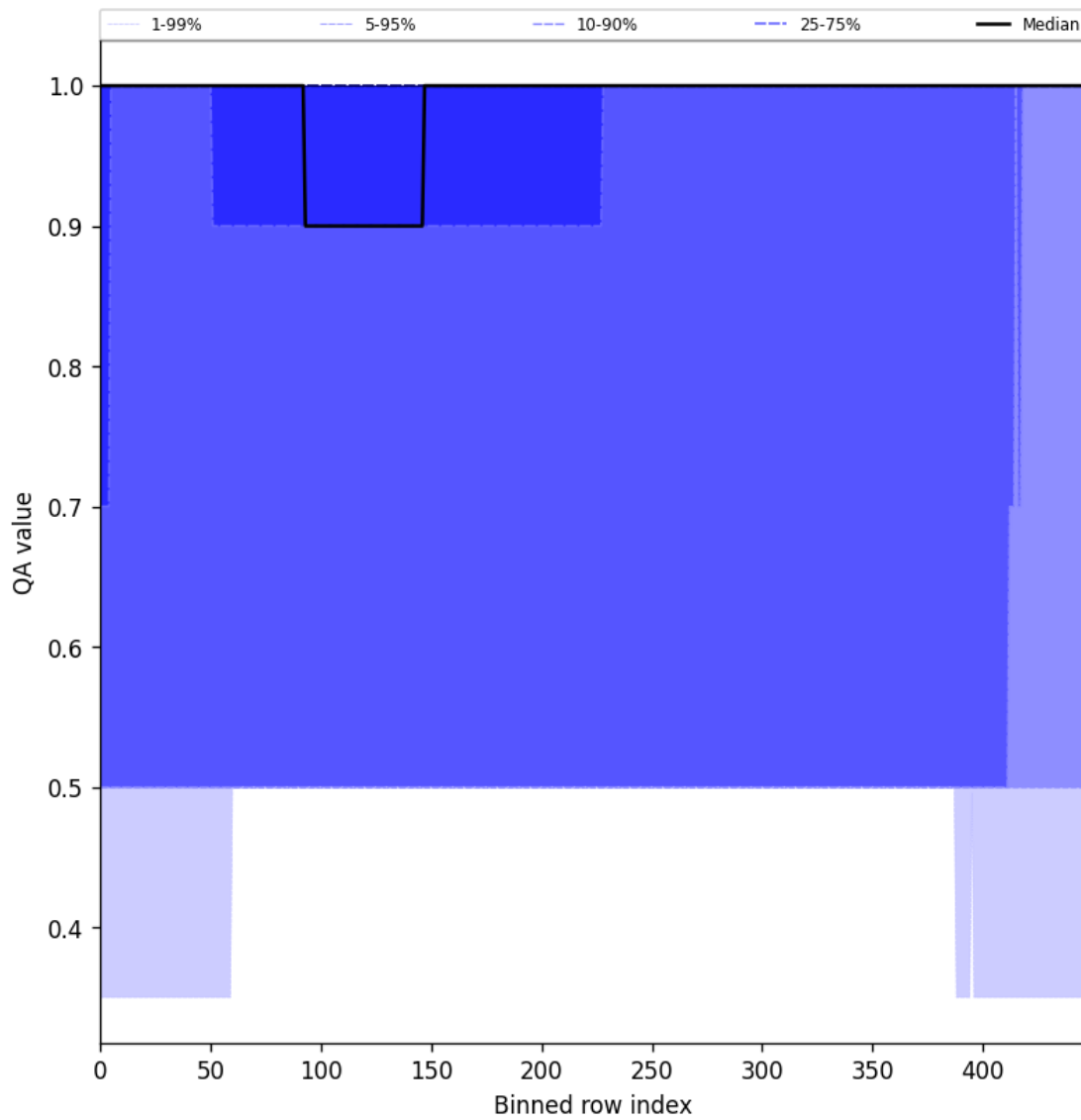
Figure 46: Along track statistics of “QA value” for 2024-11-14 to 2024-11-15
