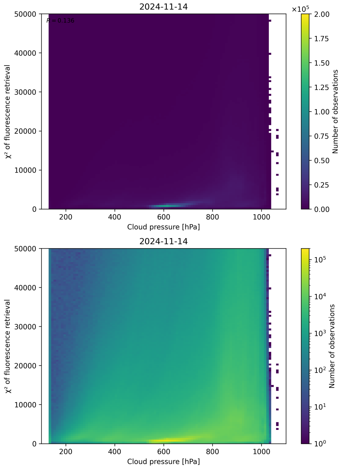
Figure 86: Scatter density plot of “Cloud pressure” against “ \chi^2 of fluorescence retrieval” for 2024-11-14 to 2024-11-15.
