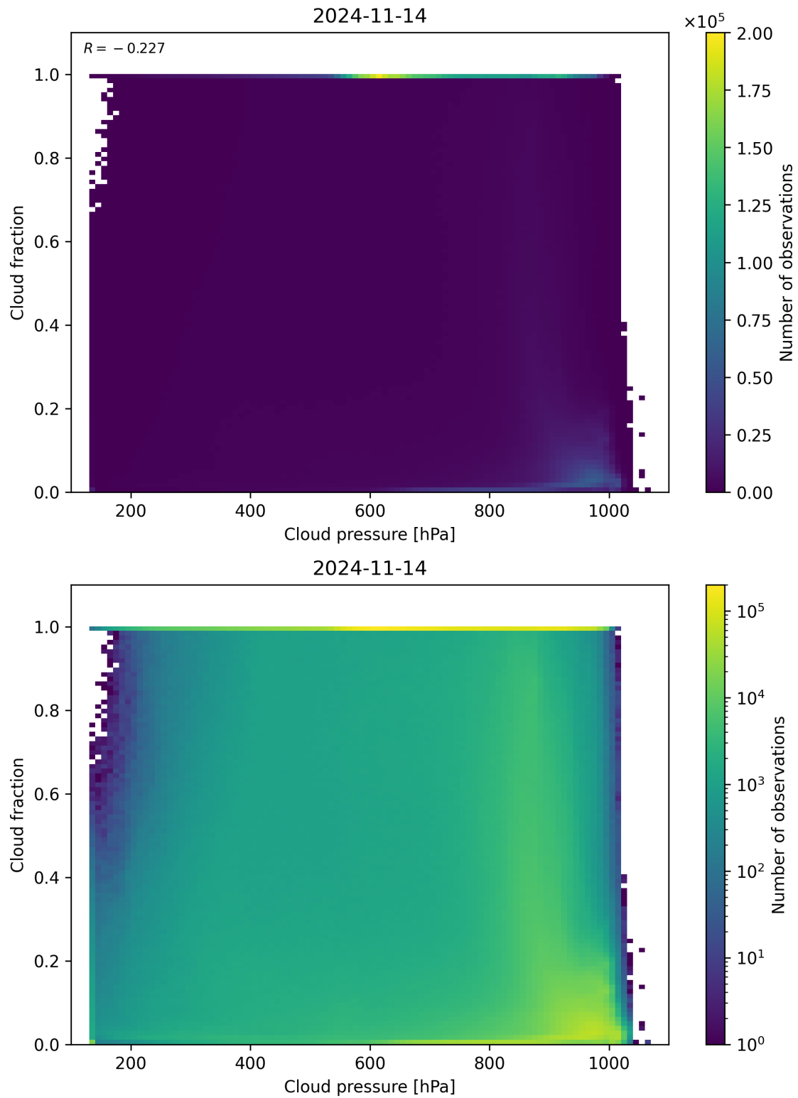
Figure 87: Scatter density plot of “Cloud pressure” against “Cloud fraction” for 2024-11-14 to 2024-11-15.
