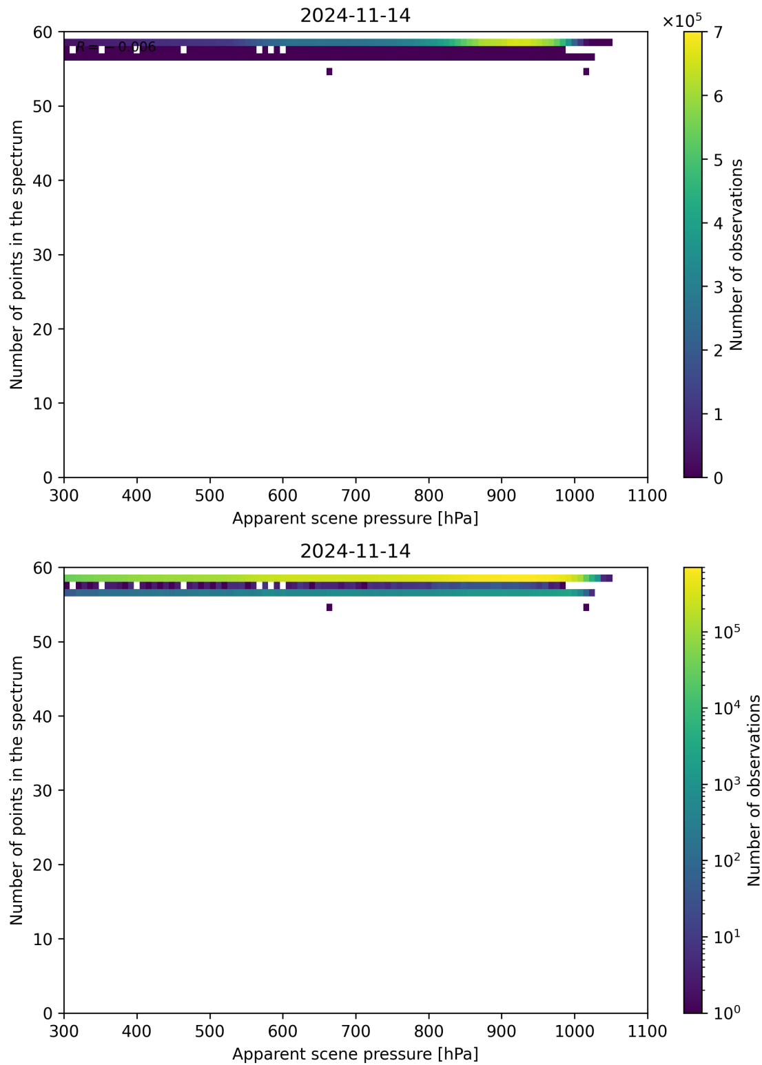
Figure 67: Scatter density plot of “Apparent scene pressure” against “Number of points in the spectrum” for 2024-11-14 to 2024-11-15.
