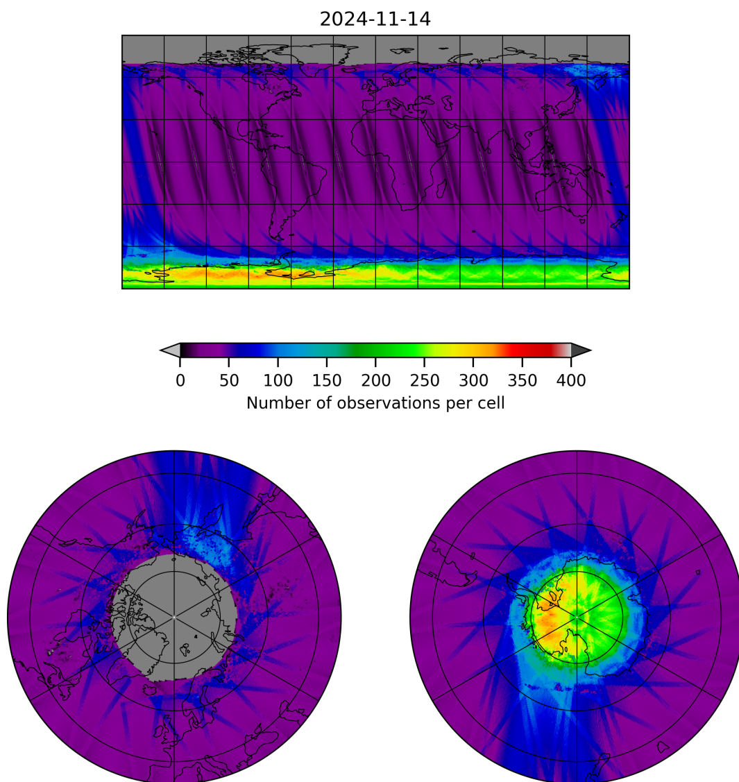
Figure 11: Map of the number of observations for 2024-11-14 to 2024-11-15
