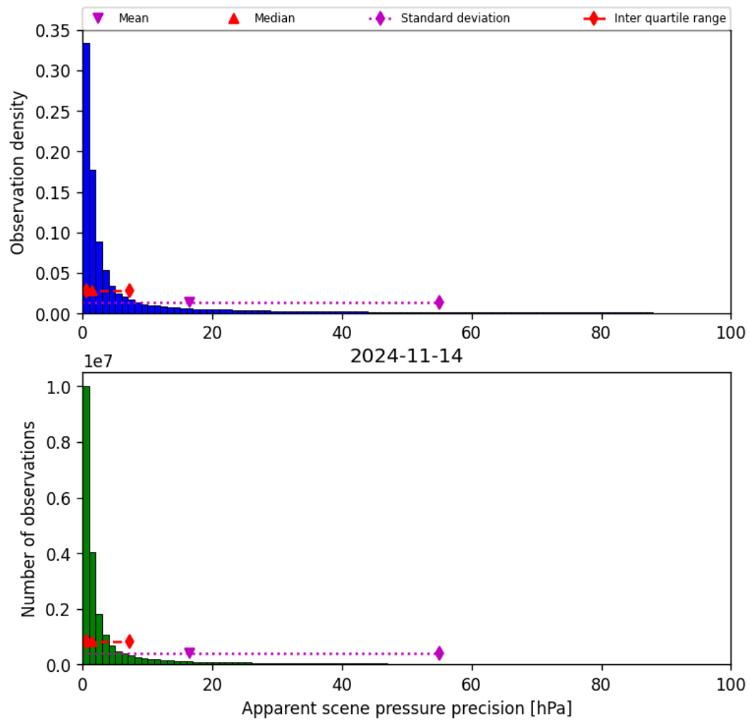
Figure 37: Histogram of “Apparent scene pressure precision” for 2024-11-14 to 2024-11-15
