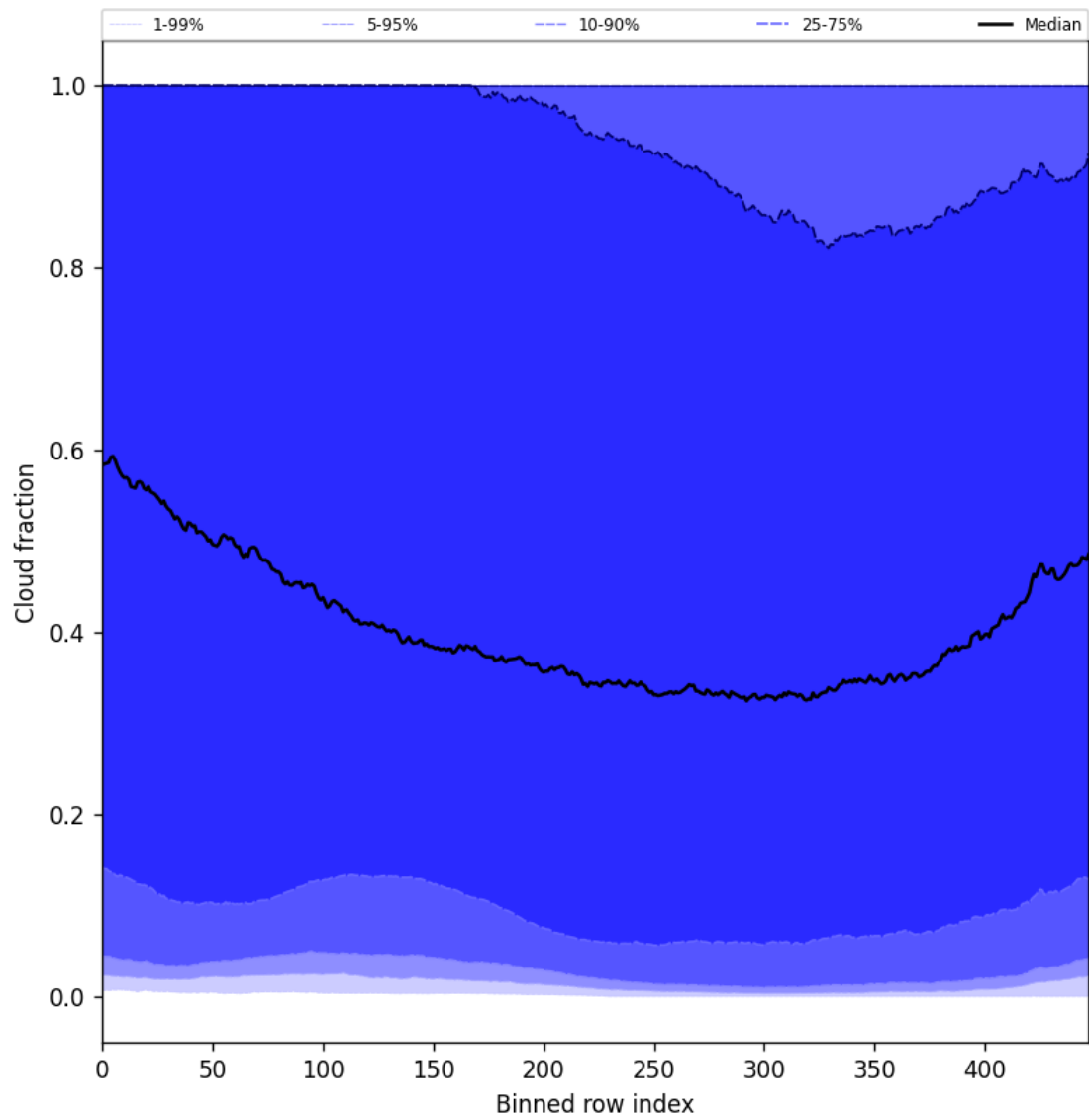
Figure 49: Along track statistics of “Cloud fraction” for 2024-11-14 to 2024-11-15
