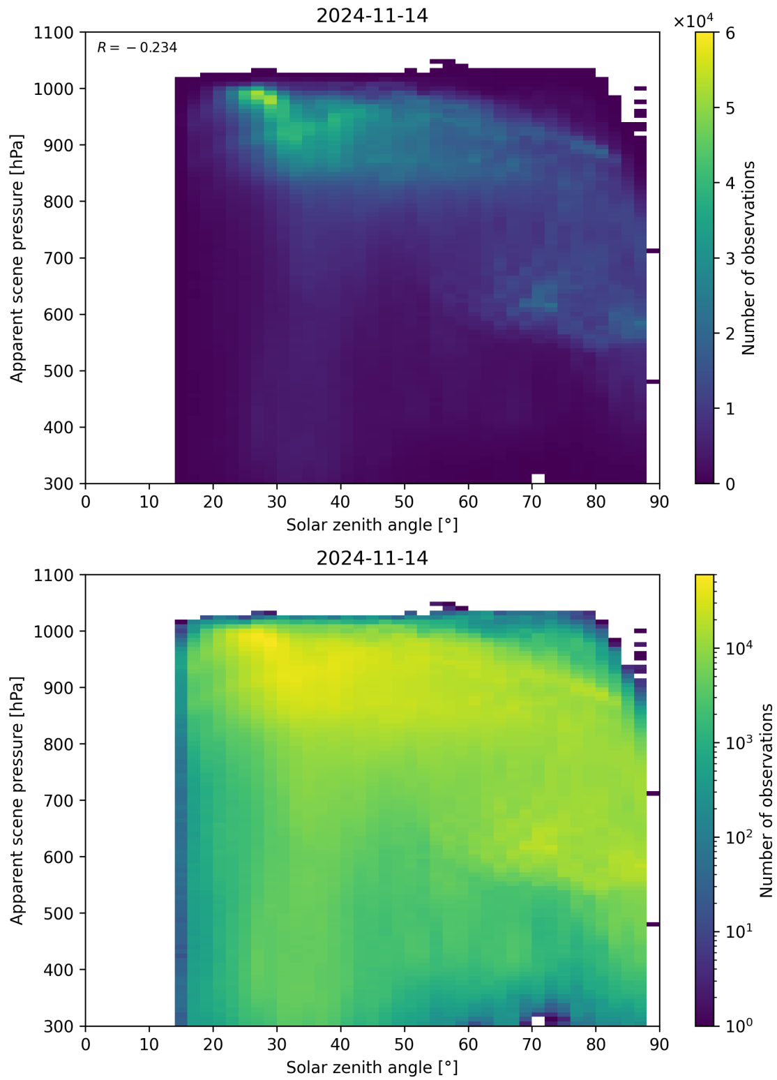
Figure 118: Scatter density plot of “Solar zenith angle” against “Apparent scene pressure” for 2024-11-14 to 2024-11-15.
