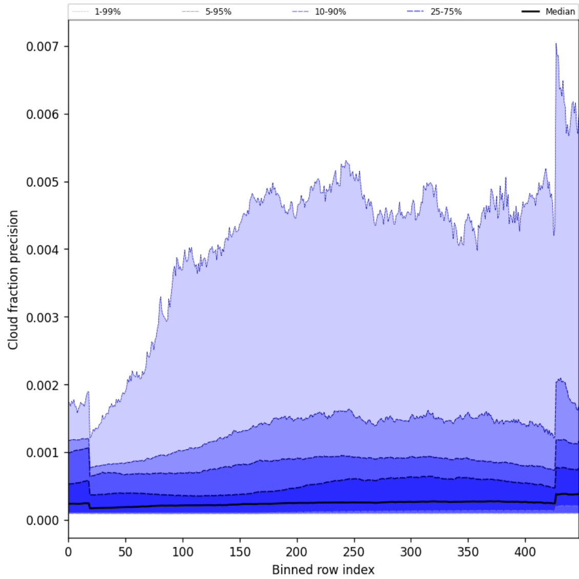
Figure 50: Along track statistics of “Cloud fraction precision” for 2024-11-14 to 2024-11-15
