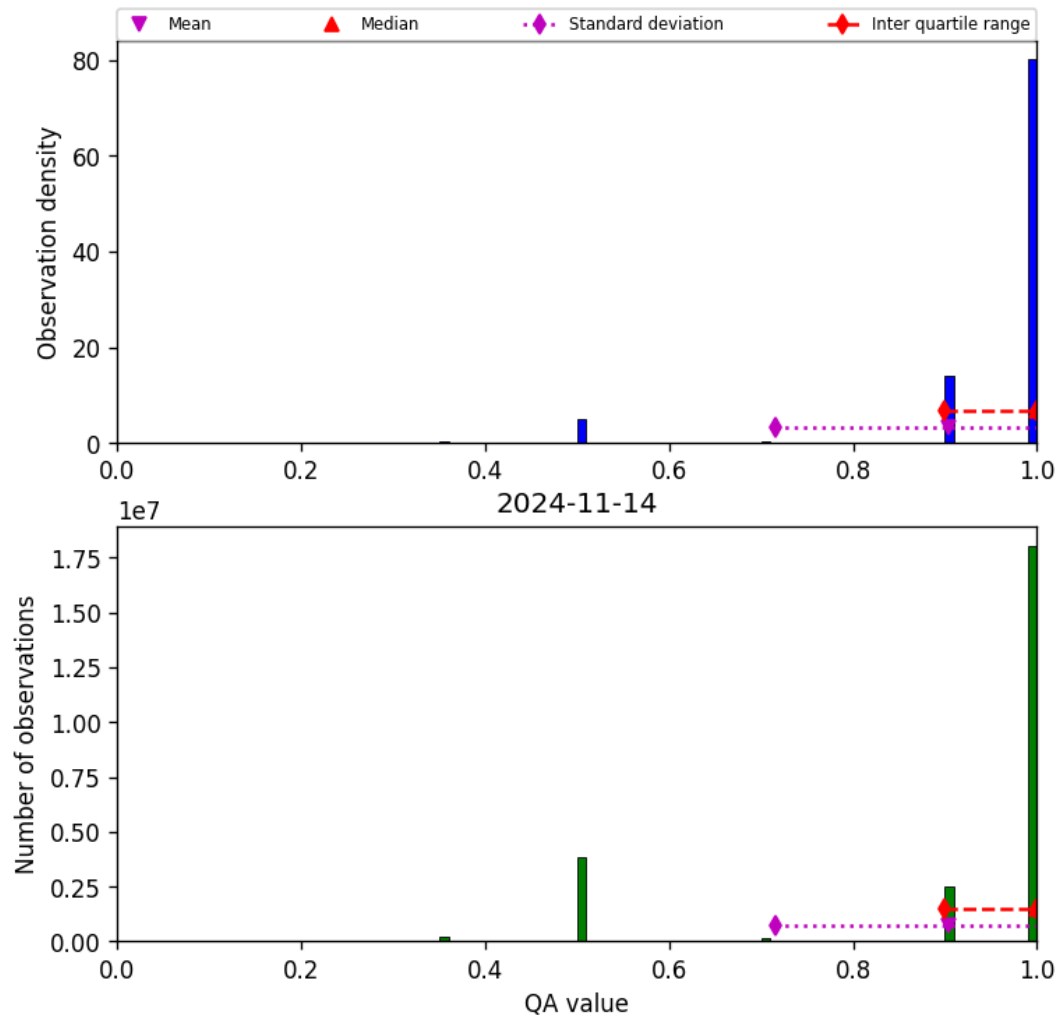
Figure 29: Histogram of “QA value” for 2024-11-14 to 2024-11-15
