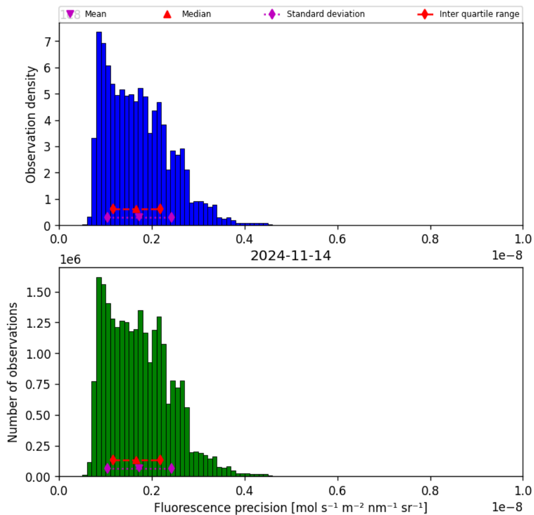
Figure 41: Histogram of “Fluorescence precision” for 2024-11-14 to 2024-11-15
