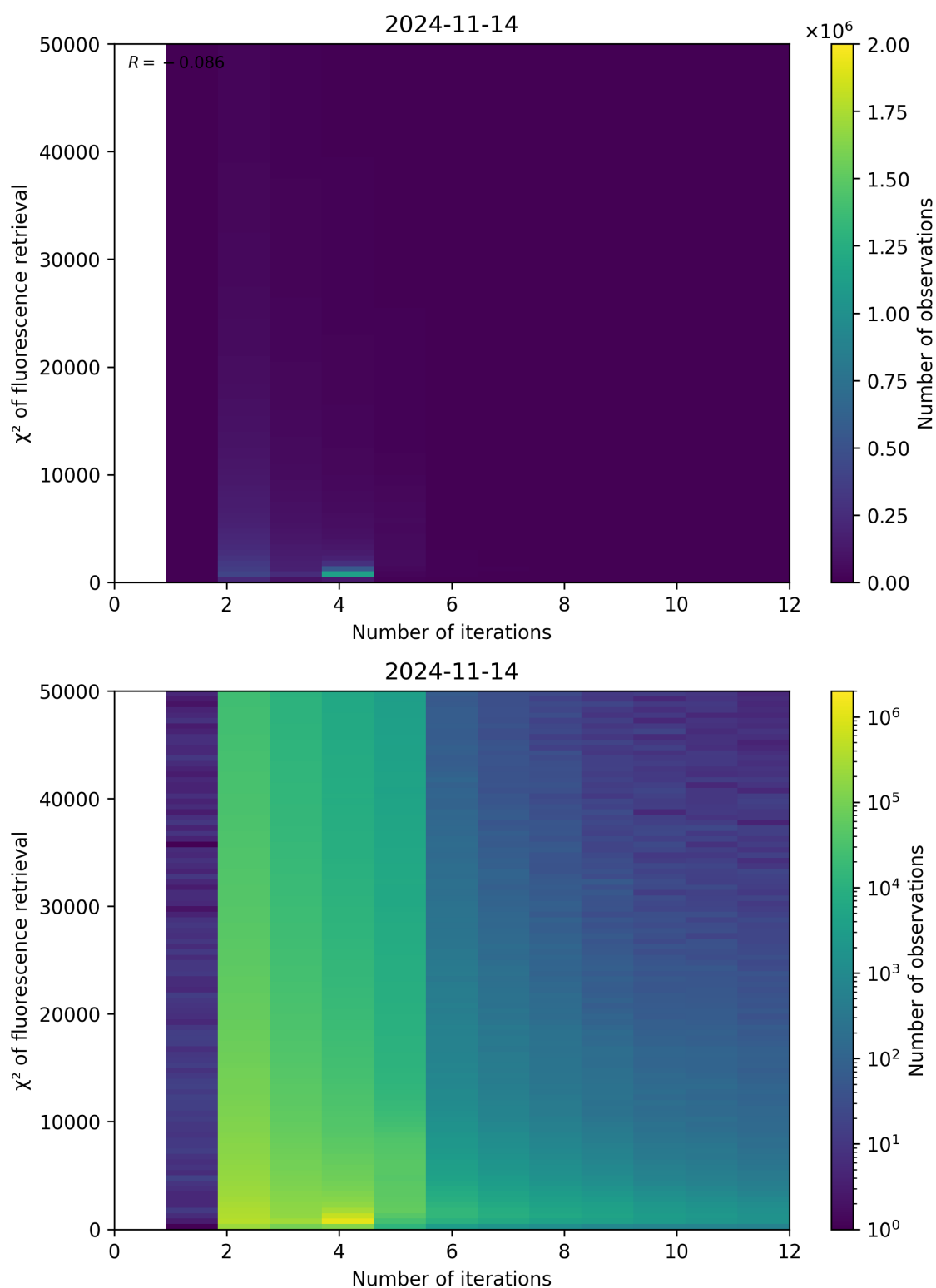
Figure 106: Scatter density plot of “Number of iterations” against “ \chi^2 of fluorescence retrieval” for 2024-11-14 to 2024-11-15.
