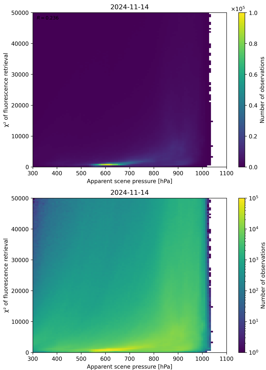
Figure 64: Scatter density plot of “Apparent scene pressure” against “ \chi^2 of fluorescence retrieval” for 2024-11-14 to 2024-11-15.
