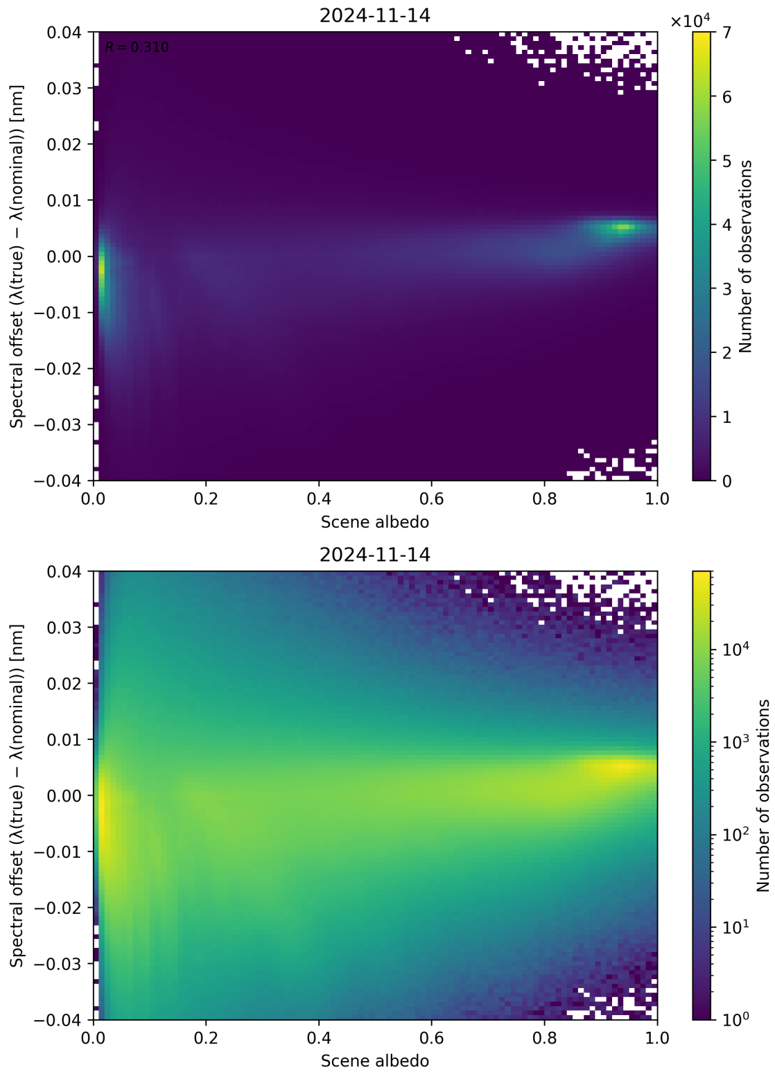
Figure 117: Scatter density plot of “Scene albedo” against “Spectral offset ( \lambda_{\text{true}} - \lambda_{\text{nominal}} )” for 2024-11-14 to 2024-11-15.
