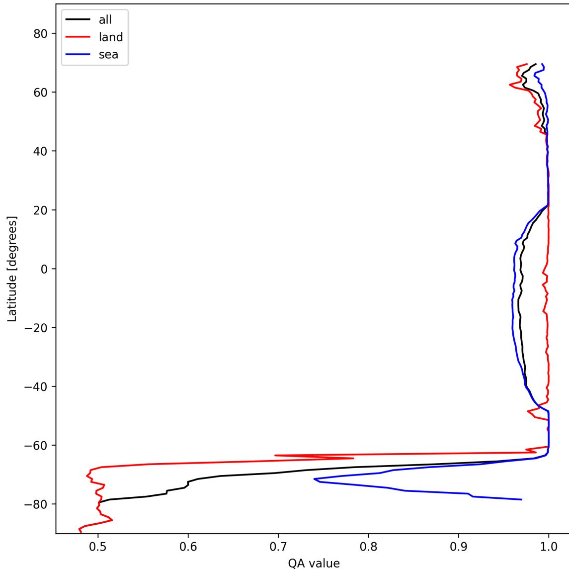
Figure 12: Zonal average of “QA value” for 2024-11-14 to 2024-11-15.
