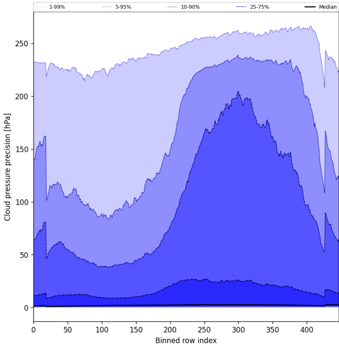
Figure 48: Along track statistics of “Cloud pressure precision” for 2024-11-14 to 2024-11-15
