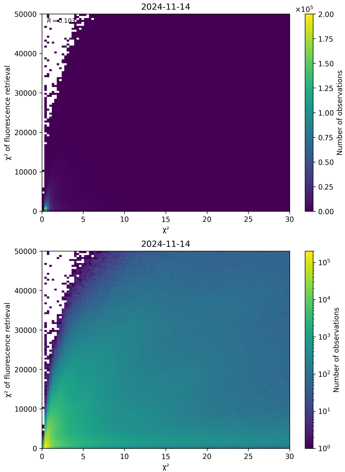
Figure 69: Scatter density plot of “ \chi^2 ” against “ \chi^2 of fluorescence retrieval” for 2024-11-14 to 2024-11-15.
