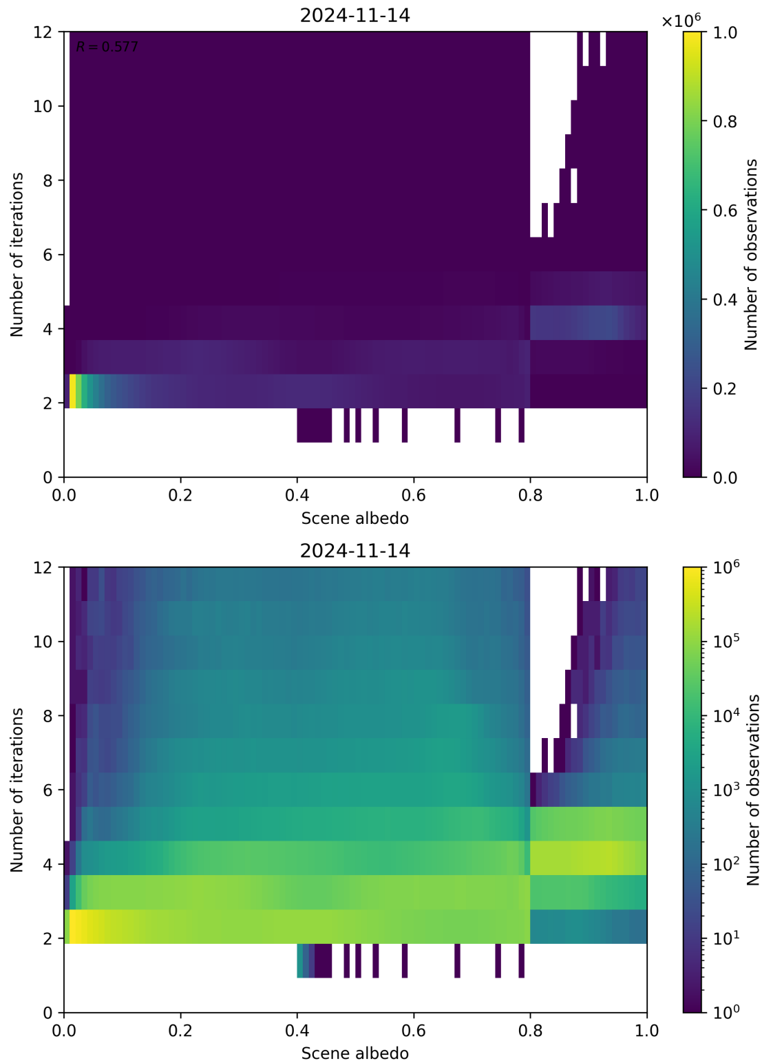
Figure 115: Scatter density plot of “Scene albedo” against “Number of iterations” for 2024-11-14 to 2024-11-15.
