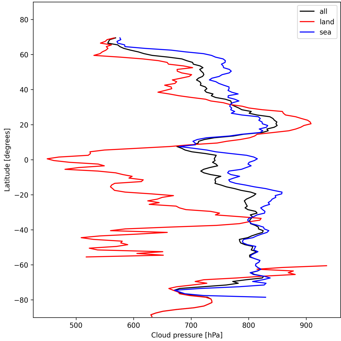
Figure 13: Zonal average of “Cloud pressure” for 2024-11-14 to 2024-11-15.
