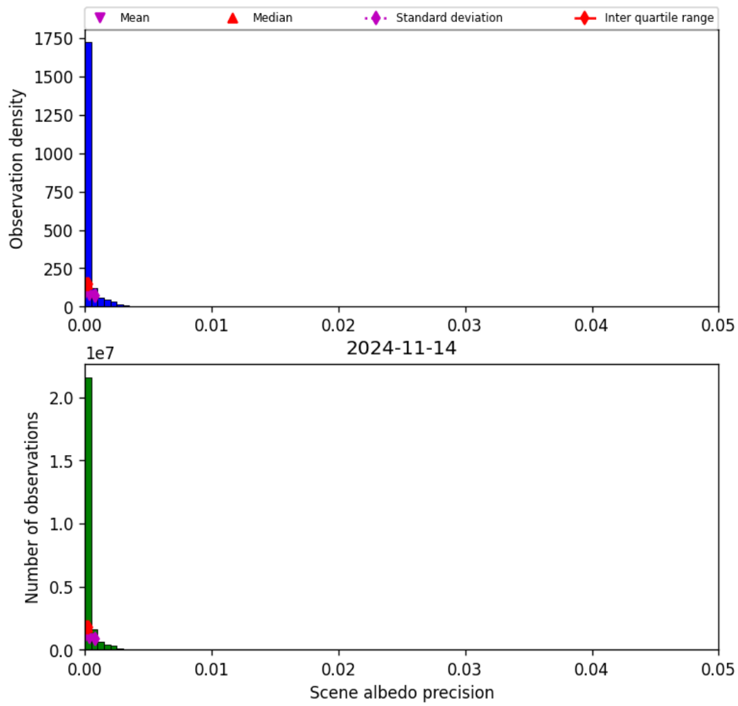
Figure 35: Histogram of “Scene albedo precision” for 2024-11-14 to 2024-11-15
