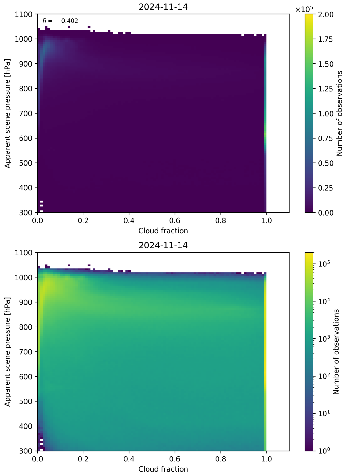
Figure 76: Scatter density plot of “Cloud fraction” against “Apparent scene pressure” for 2024-11-14 to 2024-11-15.
