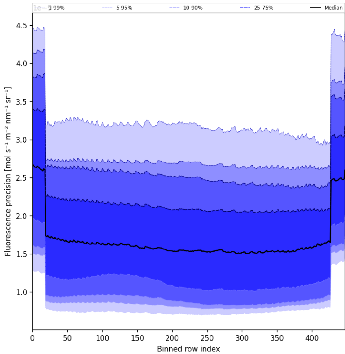
Figure 58: Along track statistics of “Fluorescence precision” for 2024-11-14 to 2024-11-15
