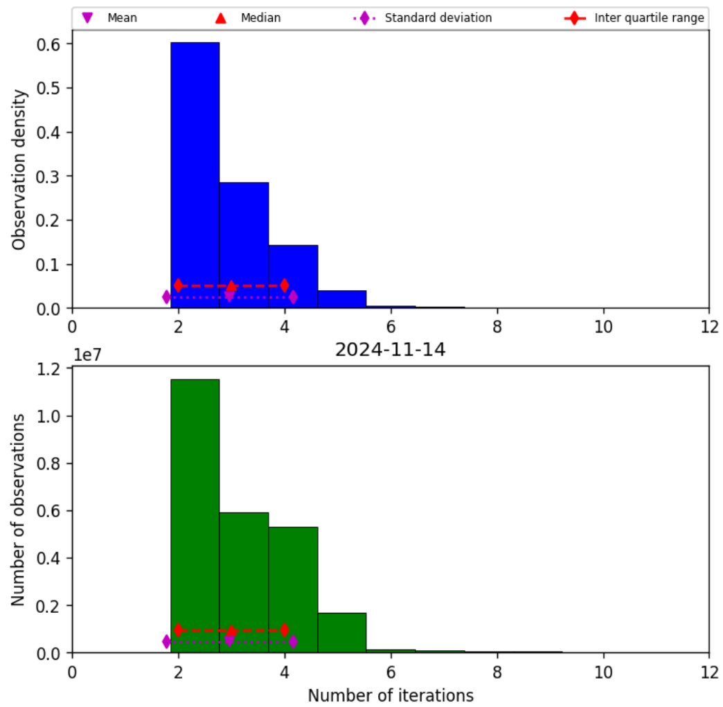
Figure 39: Histogram of “Number of iterations” for 2024-11-14 to 2024-11-15
