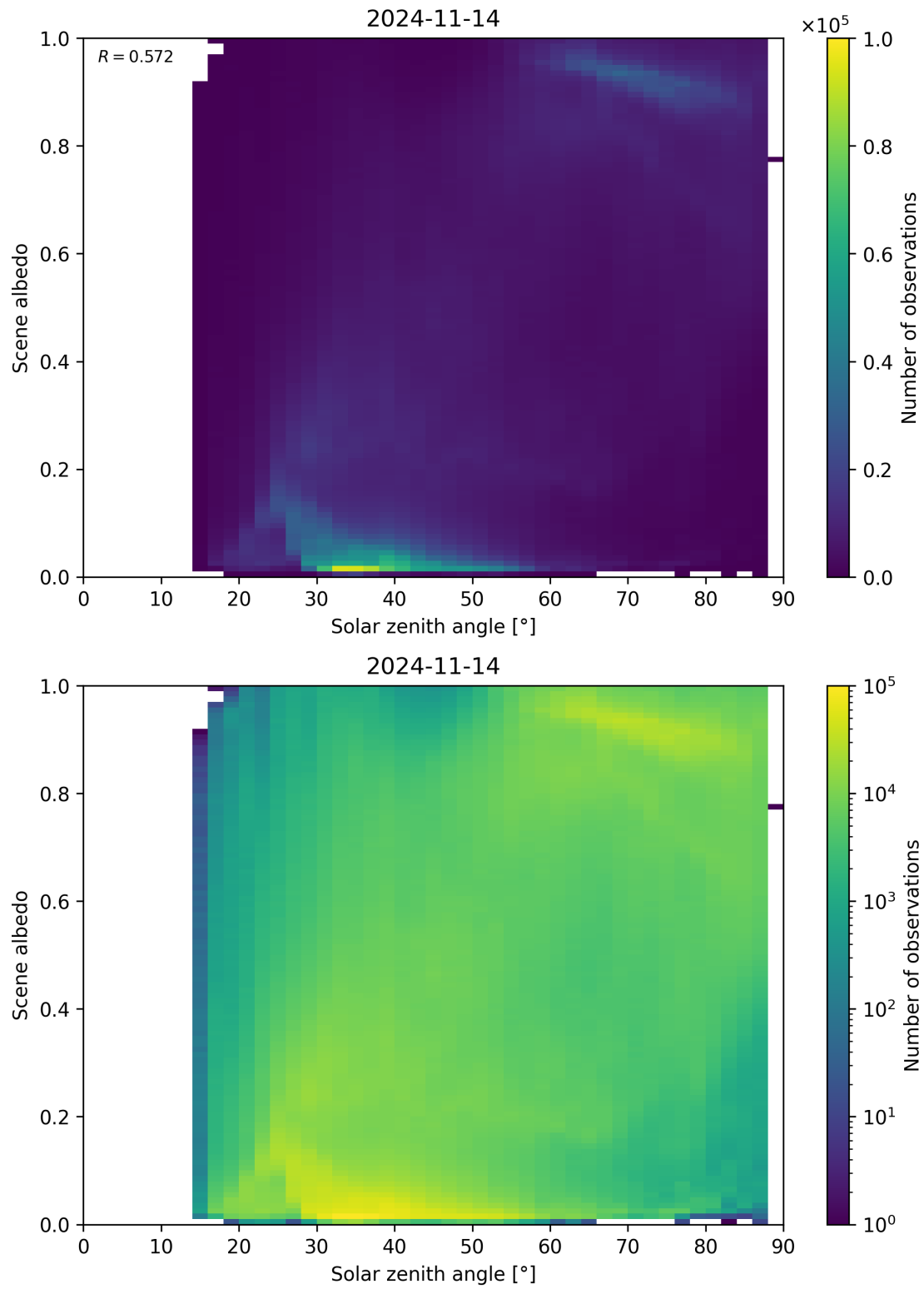
Figure 127: Scatter density plot of “Solar zenith angle” against “Scene albedo” for 2024-11-14 to 2024-11-15.
