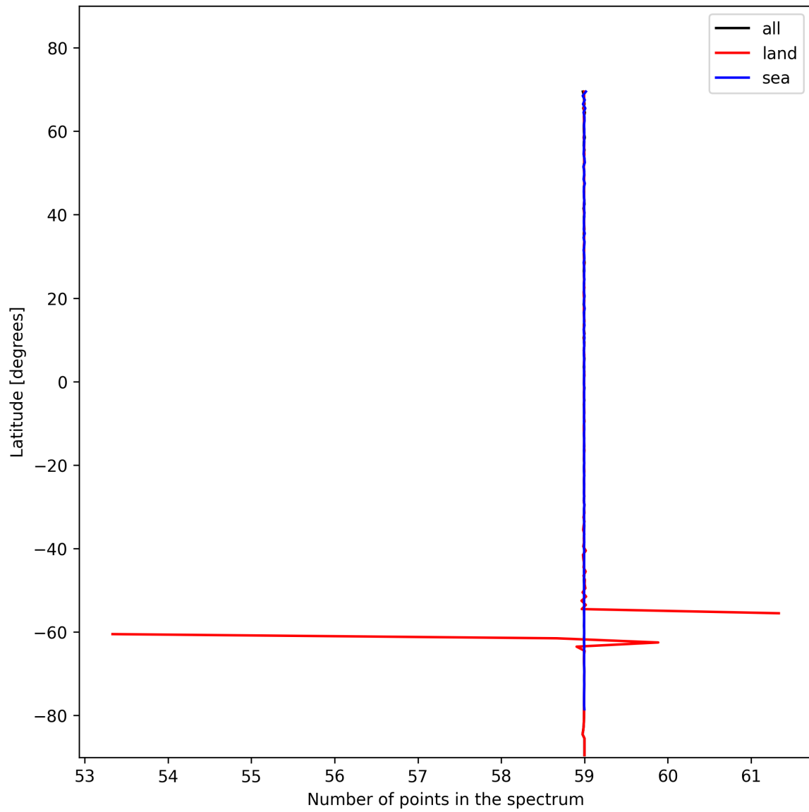
Figure 27: Zonal average of “Number of points in the spectrum” for 2024-11-14 to 2024-11-15.
