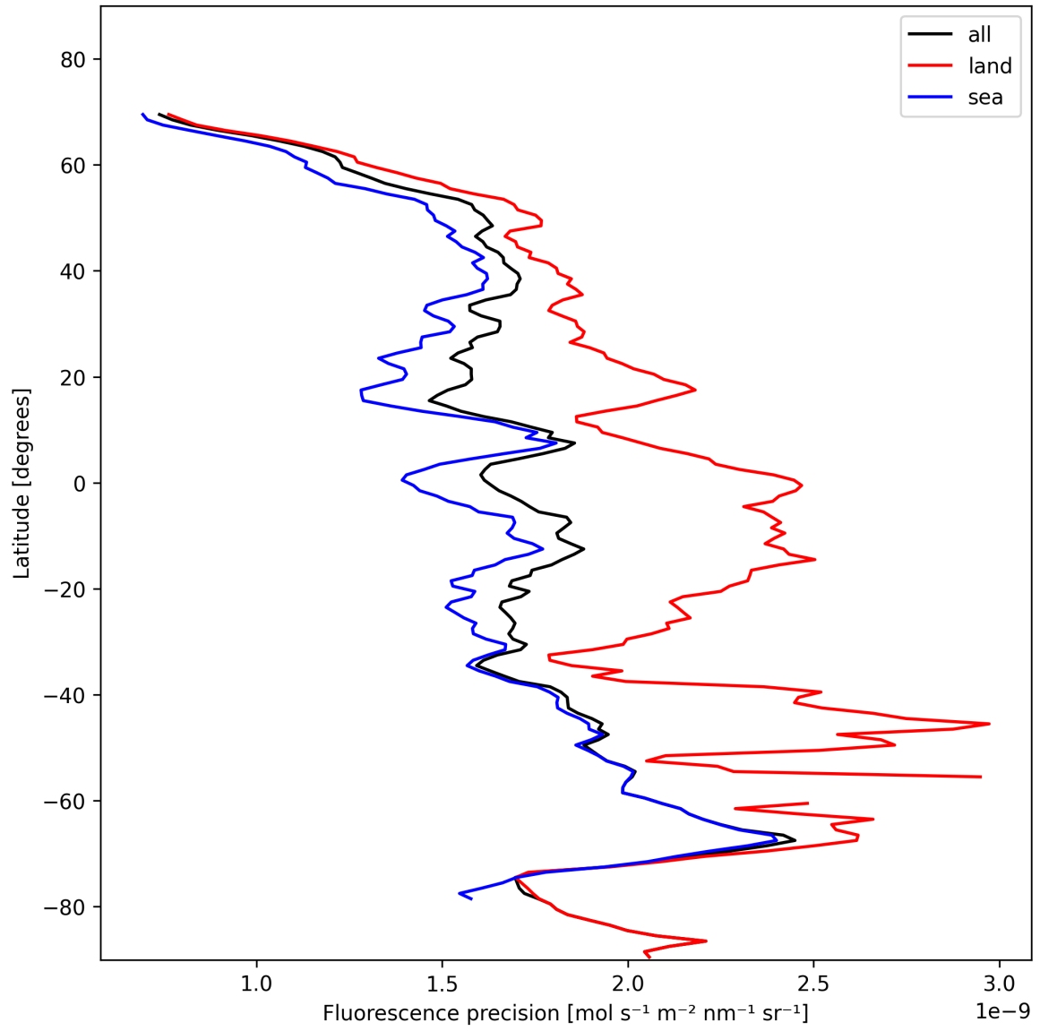
Figure 24: Zonal average of “Fluorescence precision” for 2024-11-14 to 2024-11-15.
