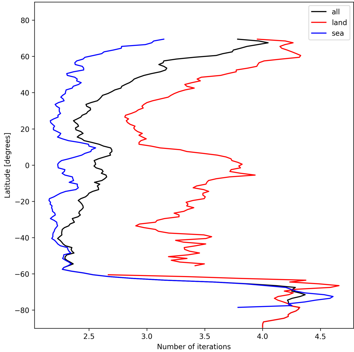
Figure 22: Zonal average of “Number of iterations” for 2024-11-14 to 2024-11-15.
