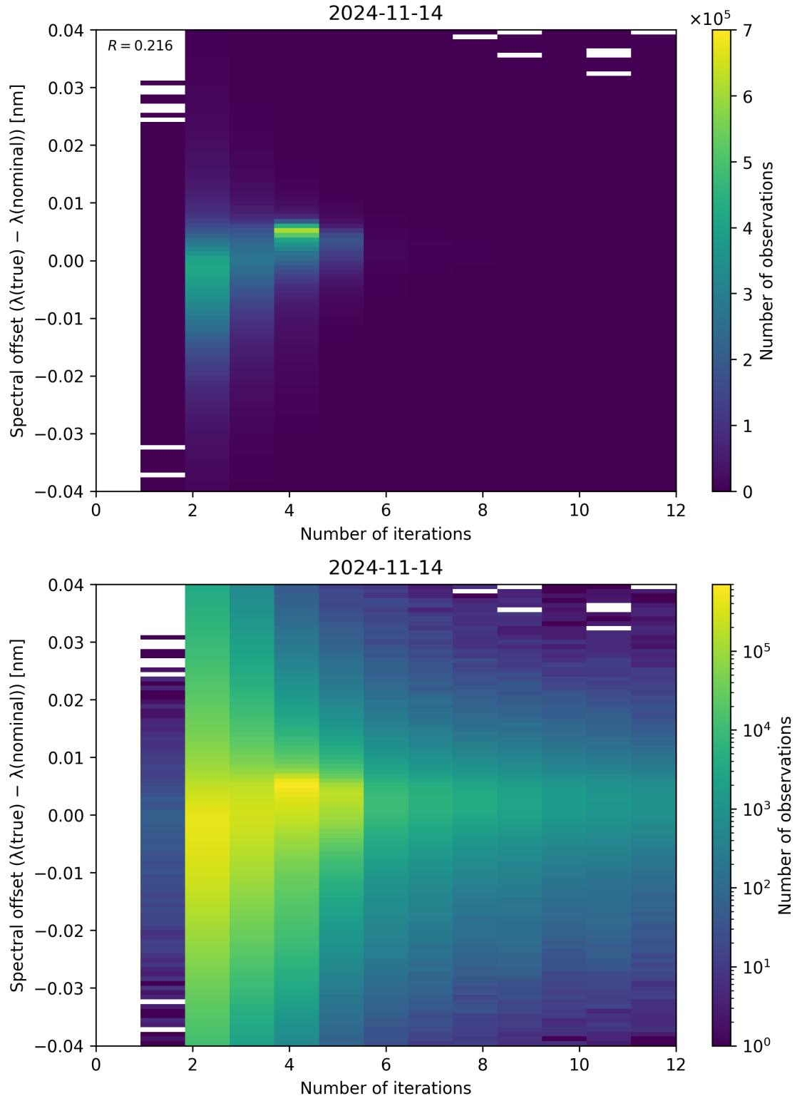
Figure 109: Scatter density plot of “Number of iterations” against “Spectral offset ( \lambda_{\text{true}} - \lambda_{\text{nominal}} )” for 2024-11-14 to 2024-11-15.
