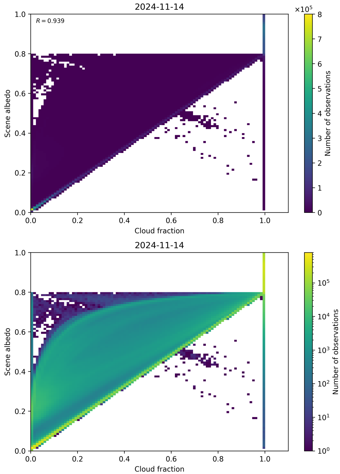
Figure 82: Scatter density plot of “Cloud fraction” against “Scene albedo” for 2024-11-14 to 2024-11-15.
