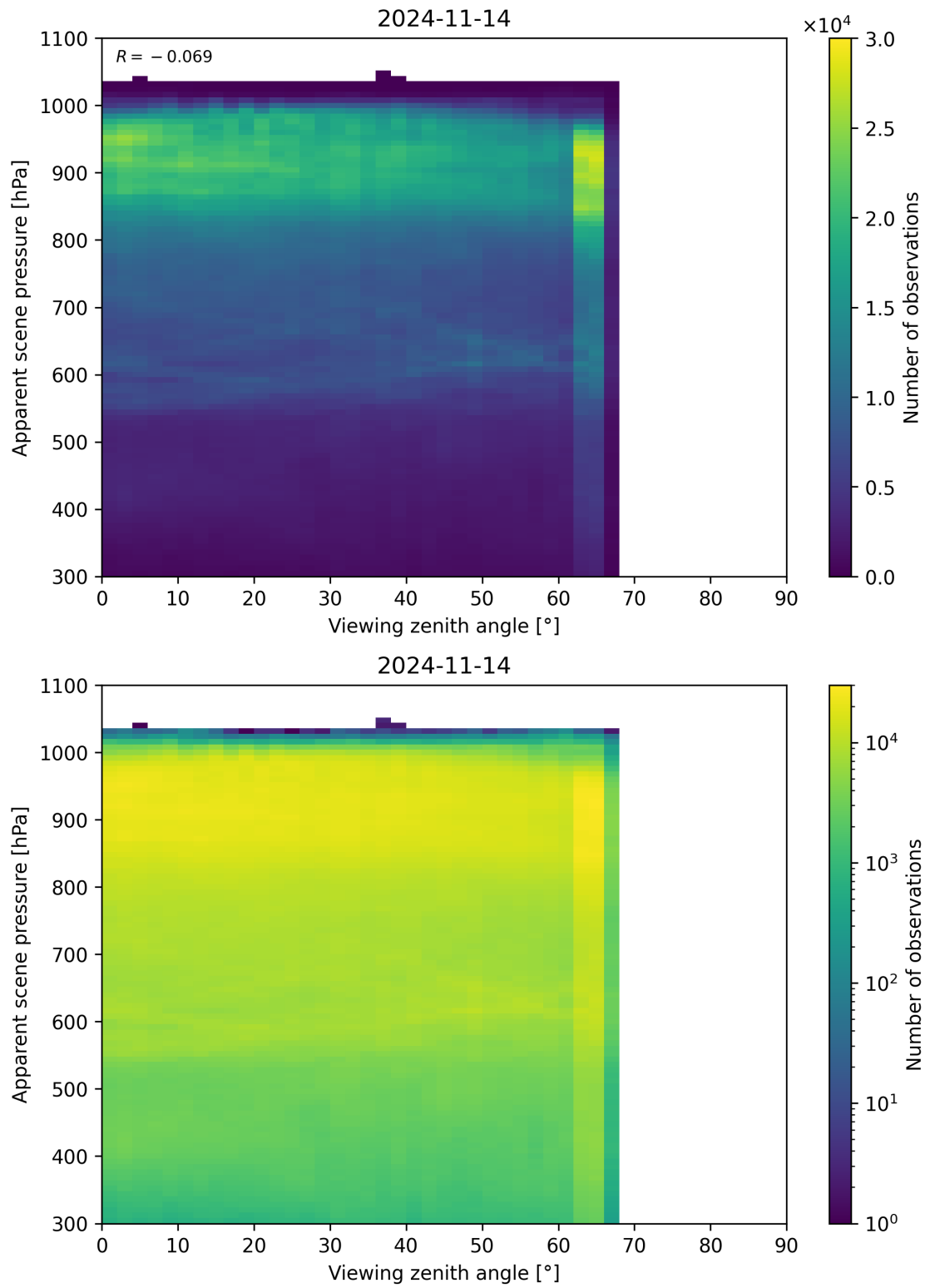
Figure 129: Scatter density plot of “Viewing zenith angle” against “Apparent scene pressure” for 2024-11-14 to 2024-11-15.
