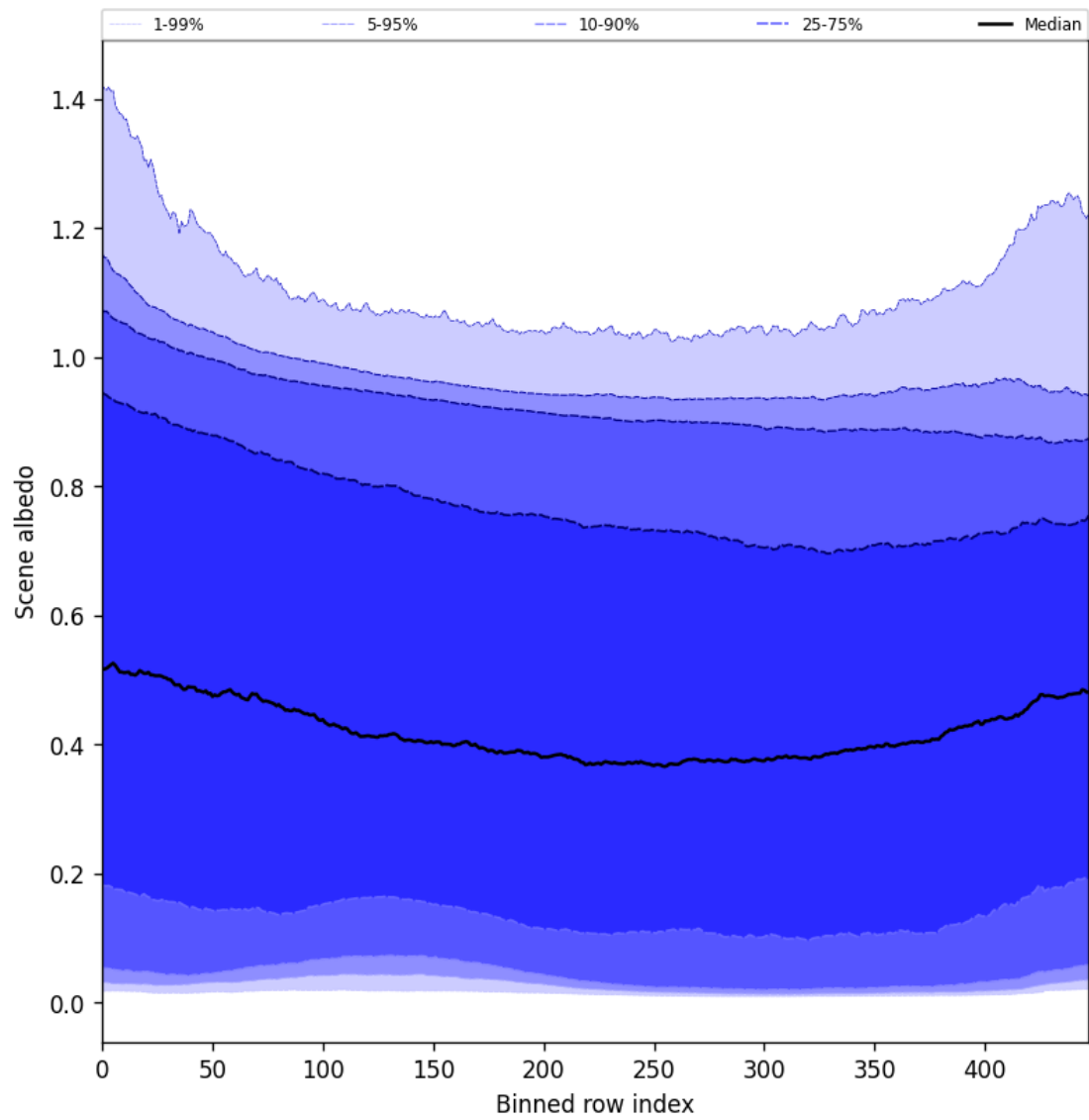
Figure 51: Along track statistics of “Scene albedo” for 2024-11-14 to 2024-11-15
