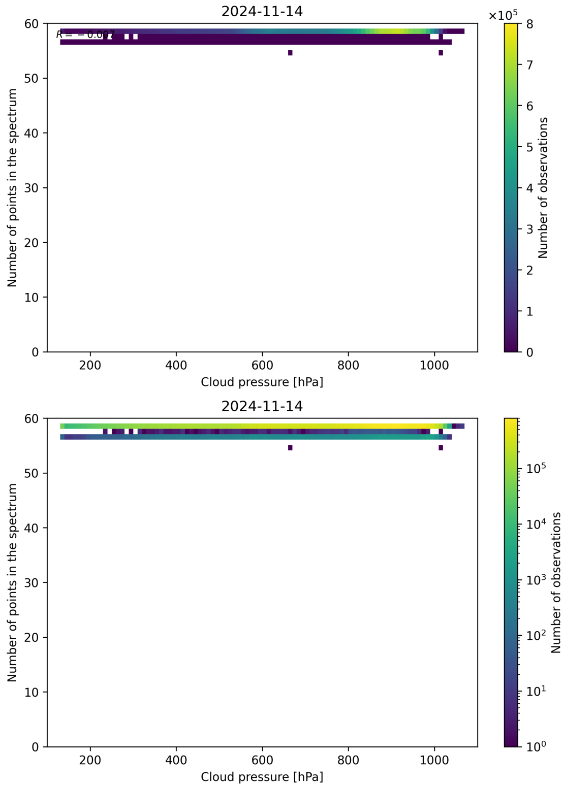
Figure 90: Scatter density plot of “Cloud pressure” against “Number of points in the spectrum” for 2024-11-14 to 2024-11-15.
