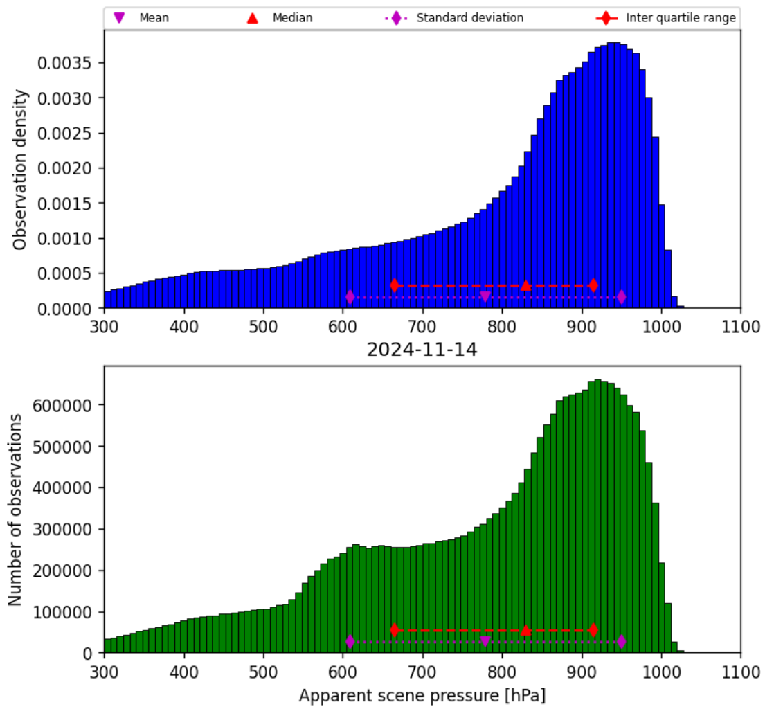
Figure 36: Histogram of “Apparent scene pressure” for 2024-11-14 to 2024-11-15
