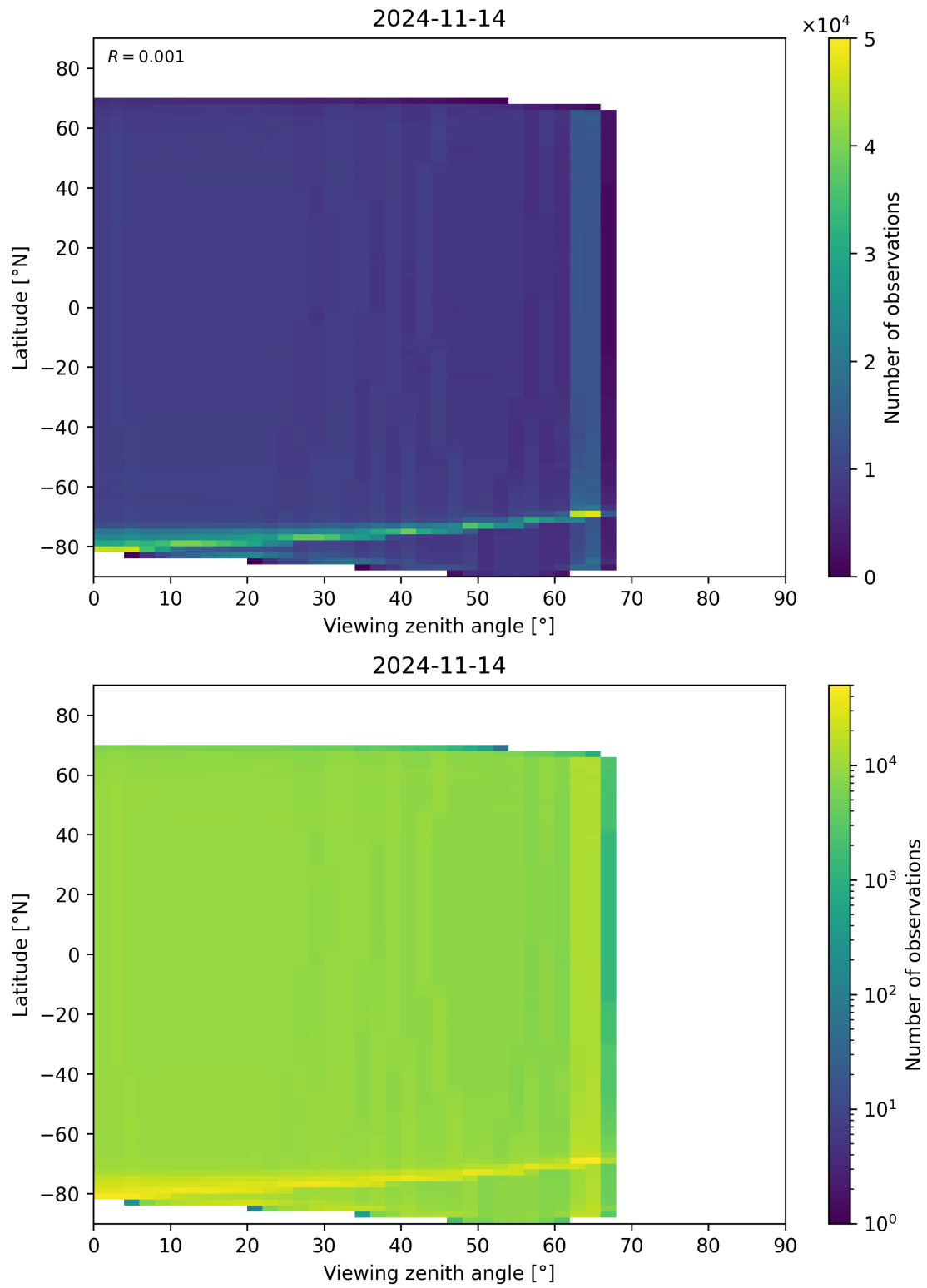
Figure 135: Scatter density plot of “Viewing zenith angle” against “Latitude” for 2024-11-14 to 2024-11-15.
