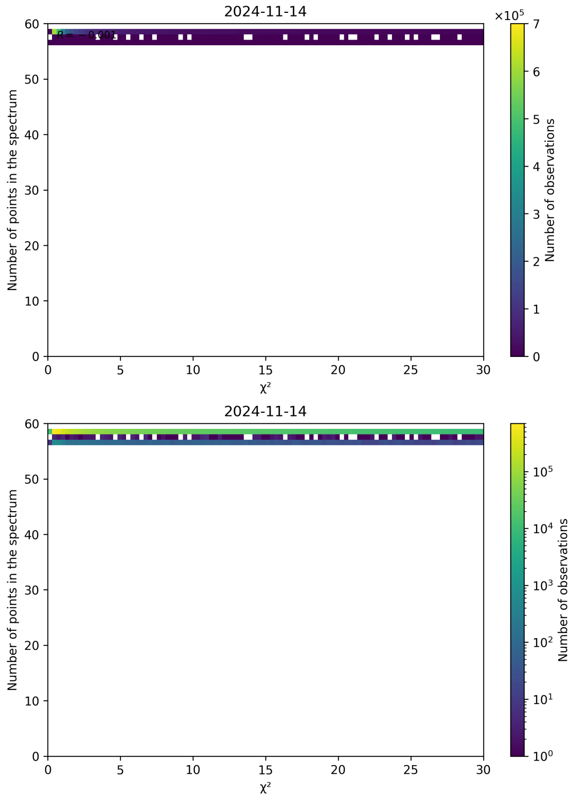
Figure 74: Scatter density plot of “ \chi^2 ” against “Number of points in the spectrum” for 2024-11-14 to 2024-11-15.
