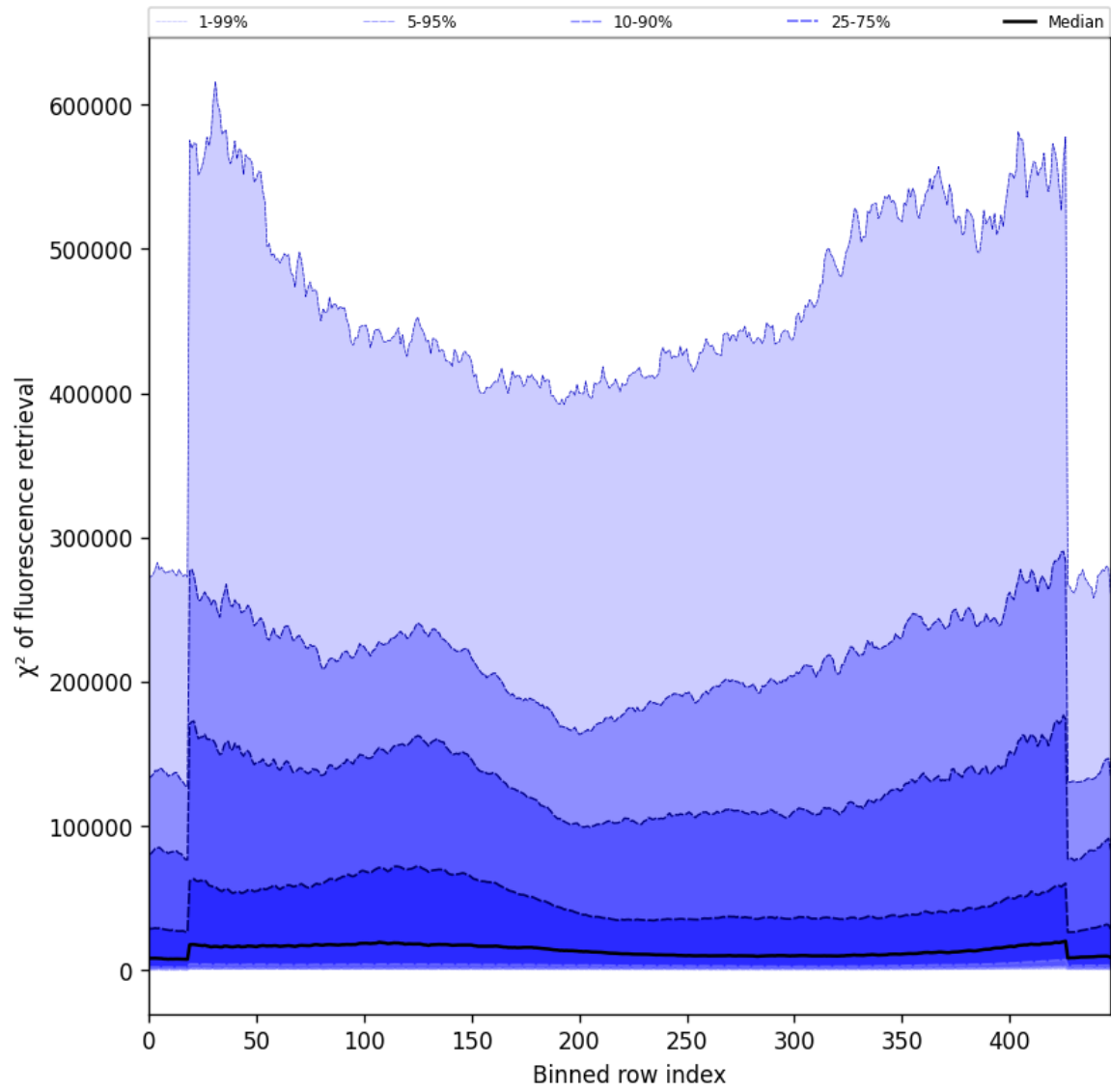
Figure 59: Along track statistics of “ \chi^2 of fluorescence retrieval” for 2024-11-14 to 2024-11-15
