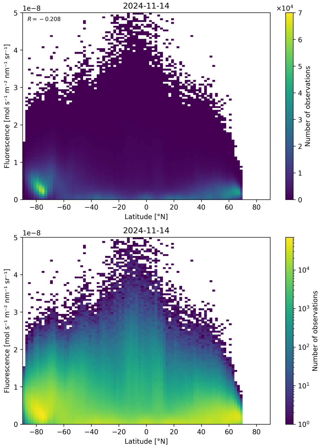
Figure 101: Scatter density plot of “Latitude” against “Fluorescence” for 2024-11-14 to 2024-11-15.
