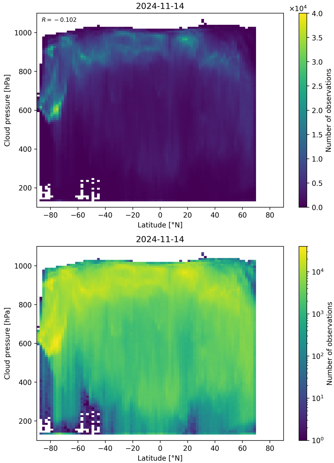
Figure 100: Scatter density plot of “Latitude” against “Cloud pressure” for 2024-11-14 to 2024-11-15.
