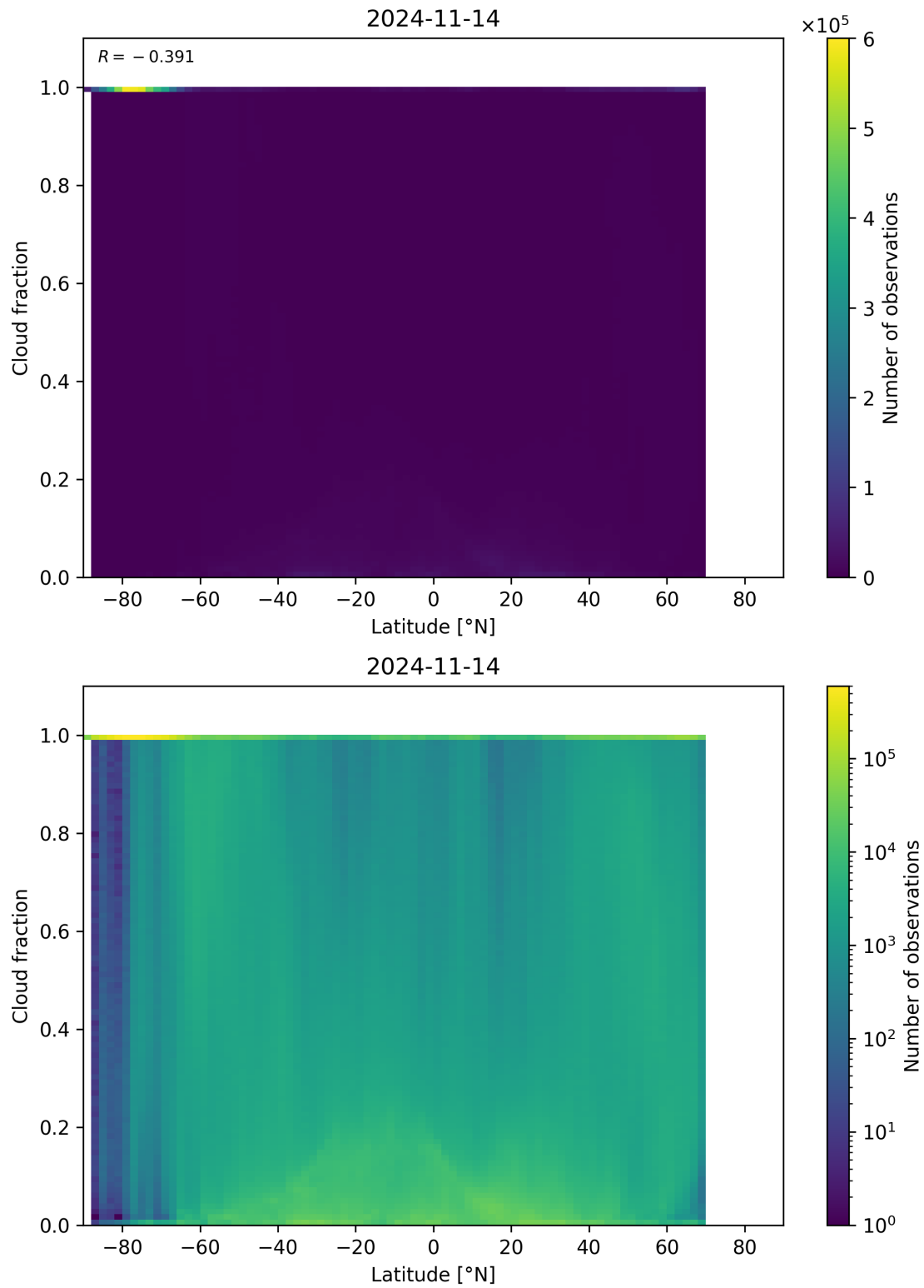
Figure 99: Scatter density plot of “Latitude” against “Cloud fraction” for 2024-11-14 to 2024-11-15.
