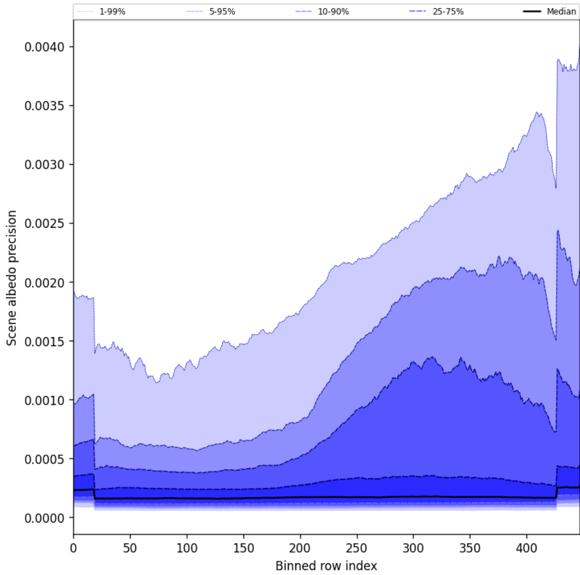
Figure 52: Along track statistics of “Scene albedo precision” for 2024-11-14 to 2024-11-15
