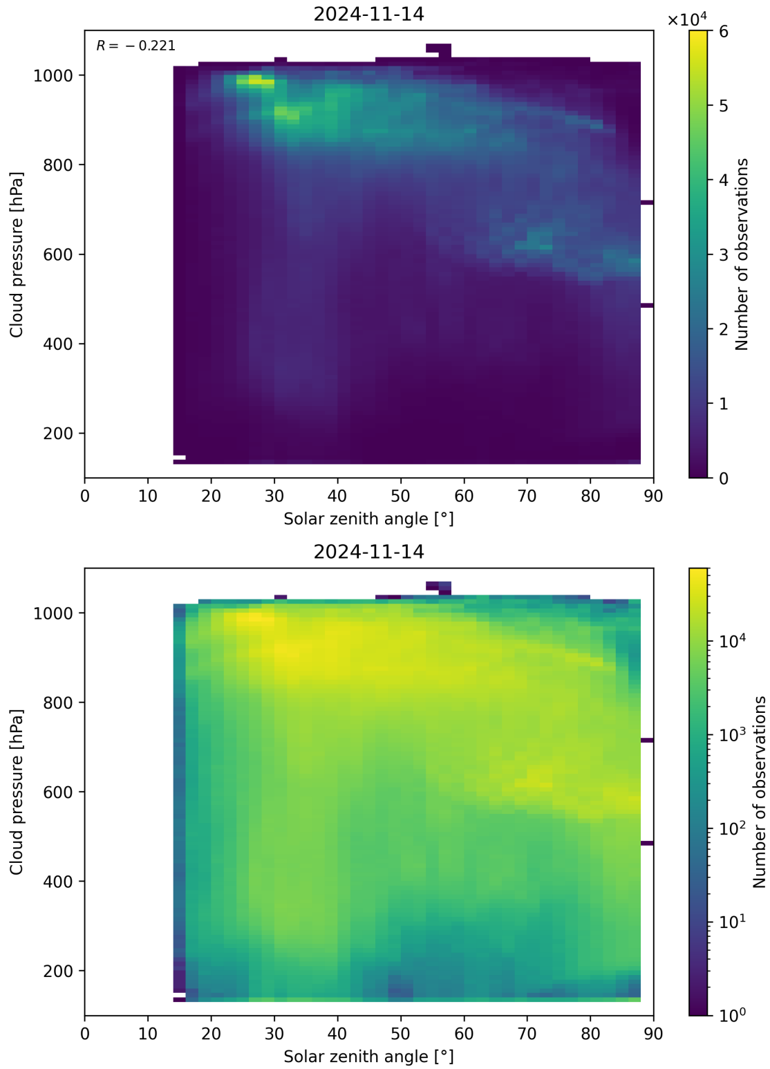
Figure 122: Scatter density plot of “Solar zenith angle” against “Cloud pressure” for 2024-11-14 to 2024-11-15.
