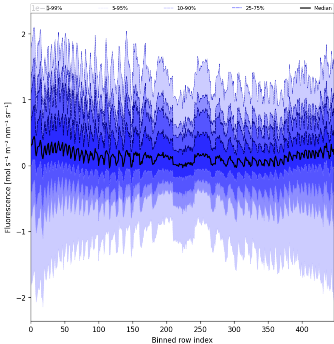
Figure 57: Along track statistics of “Fluorescence” for 2024-11-14 to 2024-11-15
