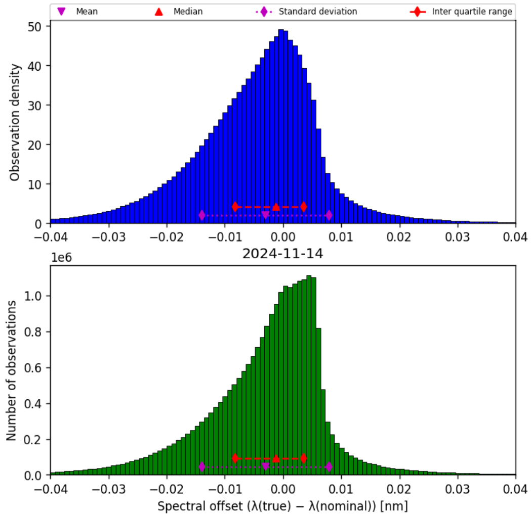
Figure 45: Histogram of “Spectral offset ( \lambda_{\text{true}} - \lambda_{\text{nominal}} )” for 2024-11-14 to 2024-11-15
