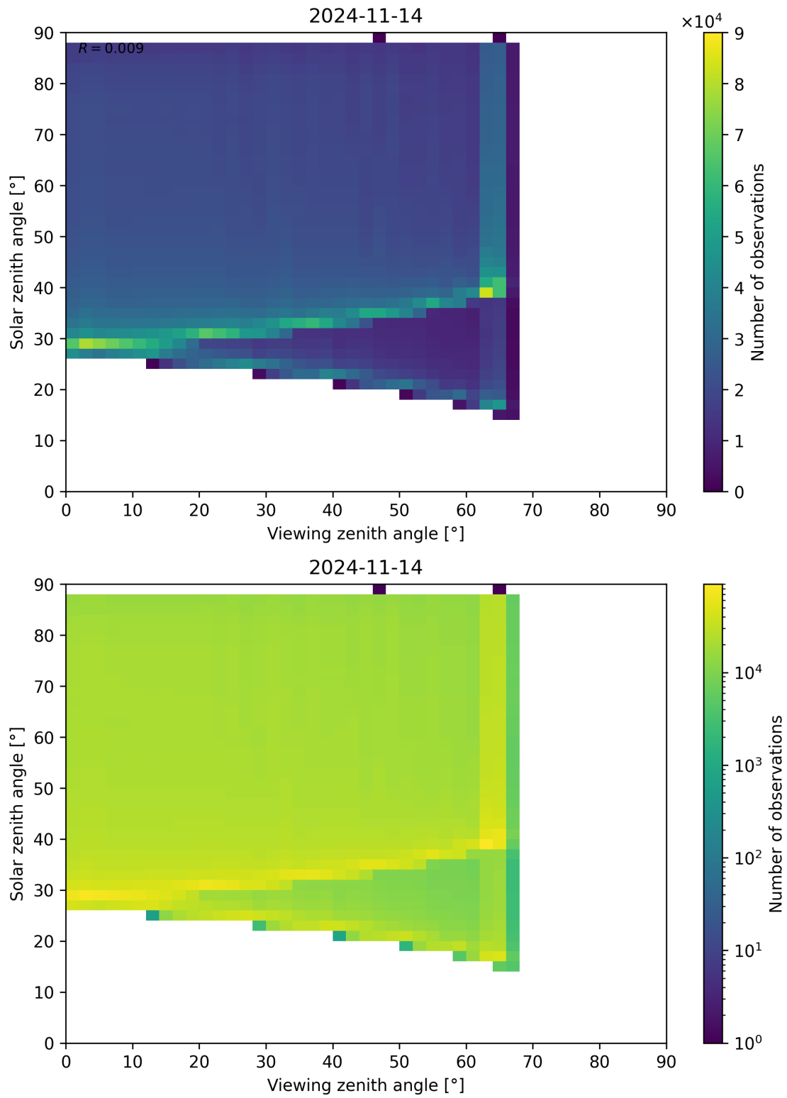
Figure 139: Scatter density plot of “Viewing zenith angle” against “Solar zenith angle” for 2024-11-14 to 2024-11-15.
