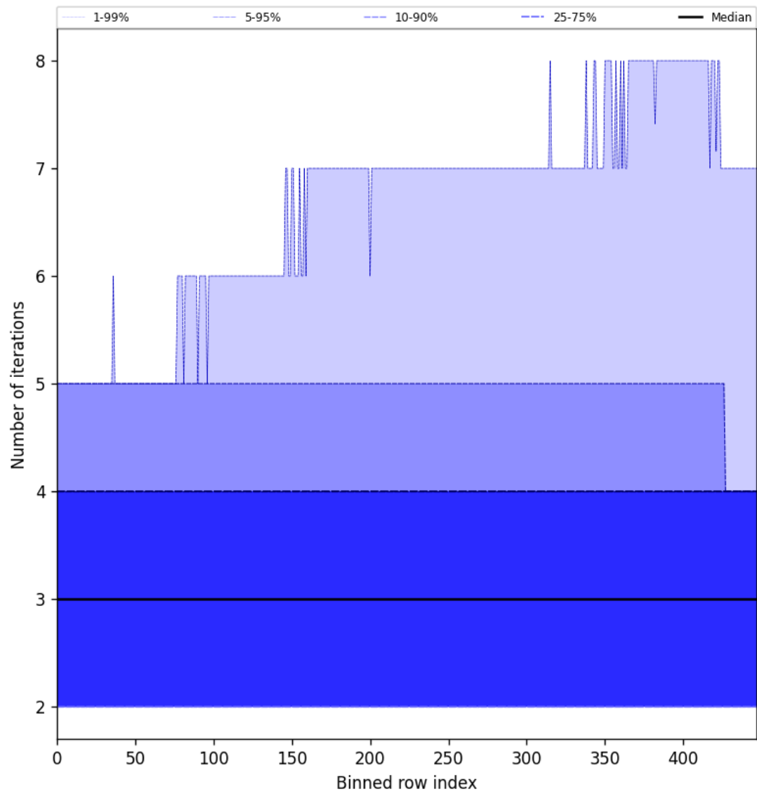
Figure 56: Along track statistics of “Number of iterations” for 2024-11-14 to 2024-11-15
