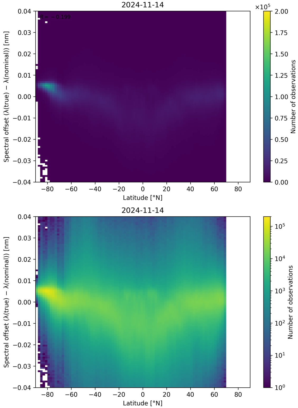
Figure 105: Scatter density plot of “Latitude” against “Spectral offset ( \lambda_{\text{true}} - \lambda_{\text{nominal}} )” for 2024-11-14 to 2024-11-15.
