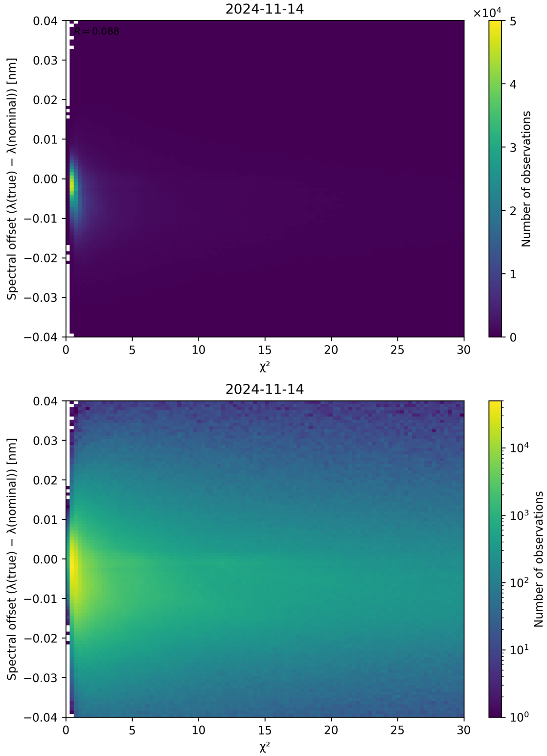
Figure 75: Scatter density plot of “ \chi^2 ” against “Spectral offset ( \lambda_{\text{true}} - \lambda_{\text{nominal}} )” for 2024-11-14 to 2024-11-15.
