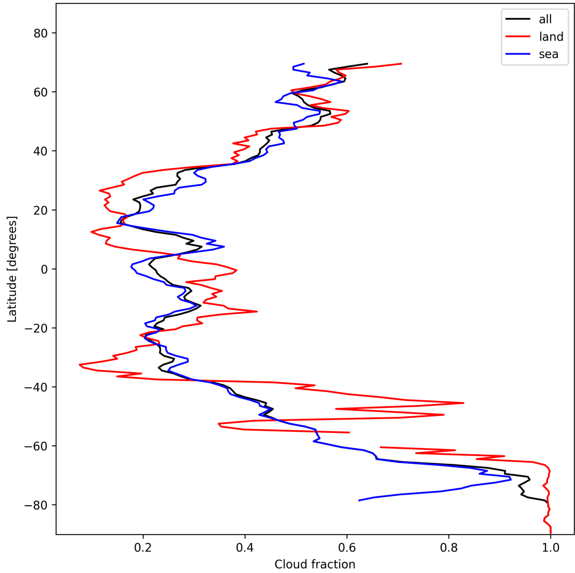
Figure 15: Zonal average of “Cloud fraction” for 2024-11-14 to 2024-11-15.
