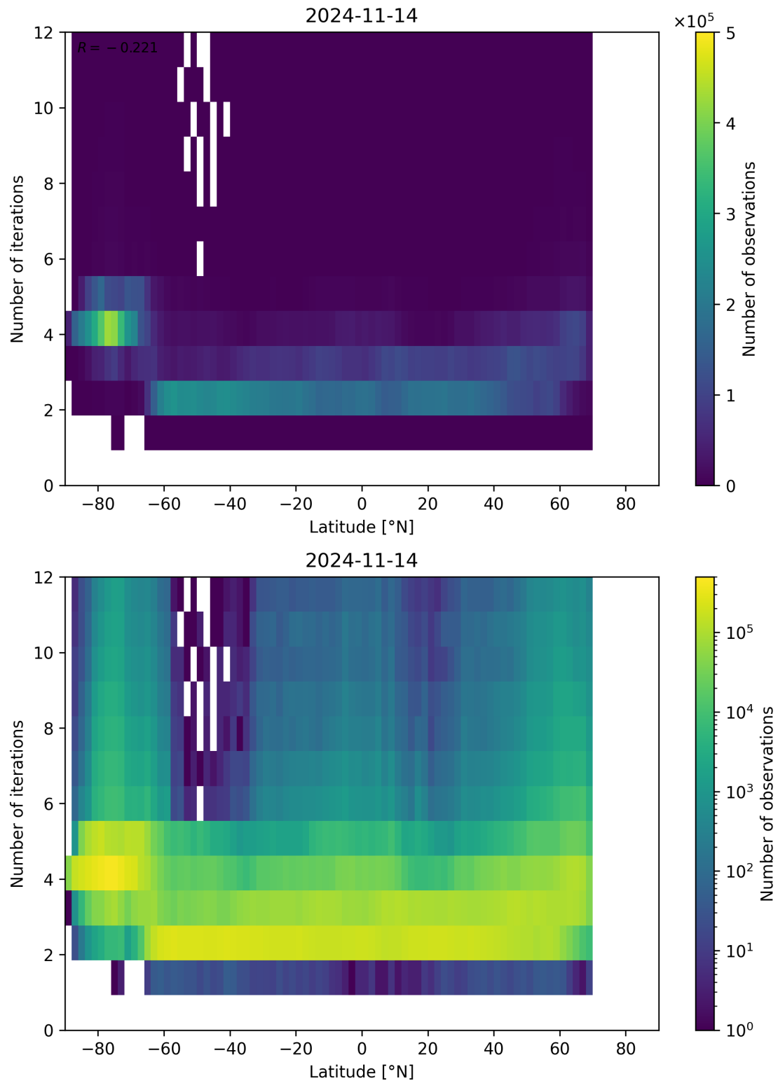
Figure 102: Scatter density plot of “Latitude” against “Number of iterations” for 2024-11-14 to 2024-11-15.
