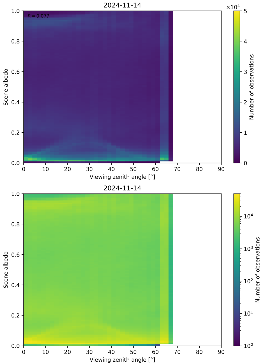
Figure 138: Scatter density plot of “Viewing zenith angle” against “Scene albedo” for 2024-11-14 to 2024-11-15.
