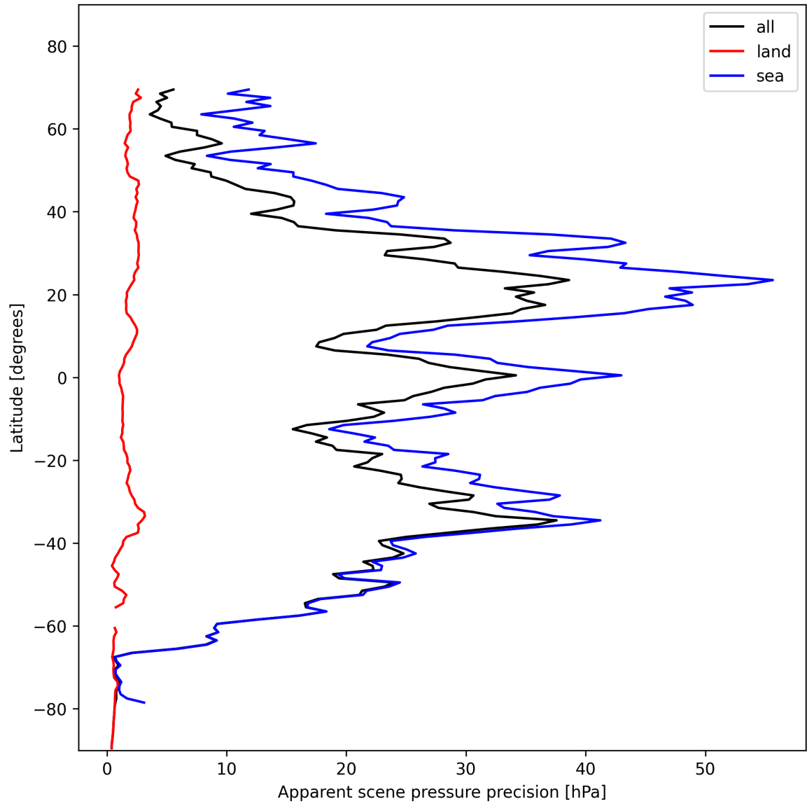
Figure 20: Zonal average of “Apparent scene pressure precision” for 2024-11-14 to 2024-11-15.
