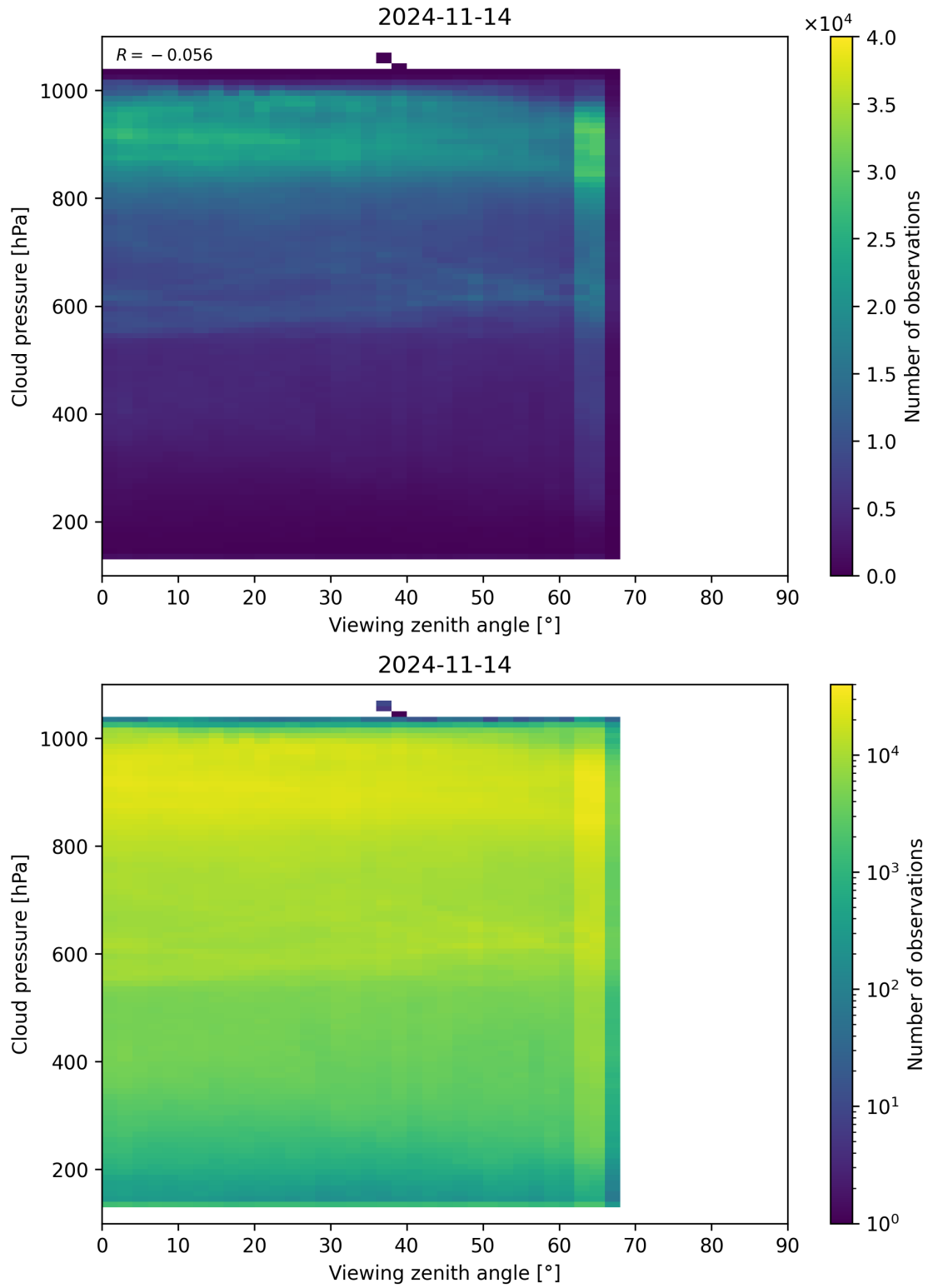
Figure 133: Scatter density plot of “Viewing zenith angle” against “Cloud pressure” for 2024-11-14 to 2024-11-15.
