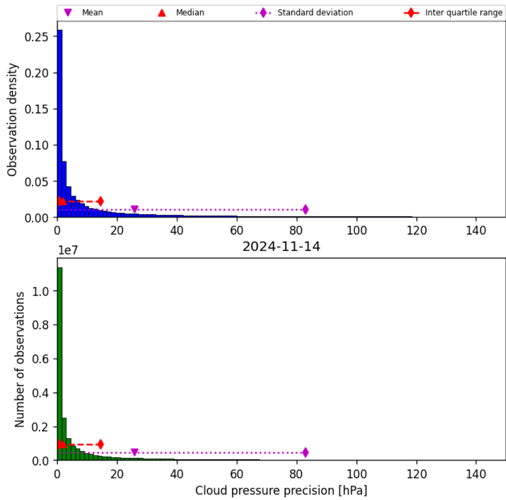
Figure 31: Histogram of “Cloud pressure precision” for 2024-11-14 to 2024-11-15
