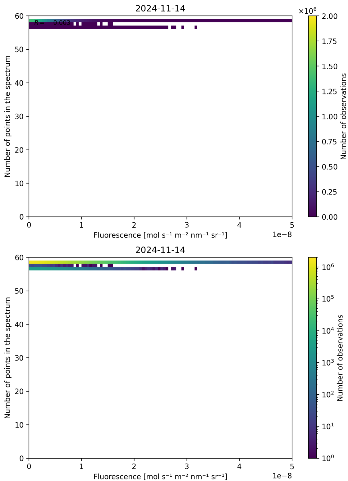
Figure 94: Scatter density plot of “Fluorescence” against “Number of points in the spectrum” for 2024-11-14 to 2024-11-15.
