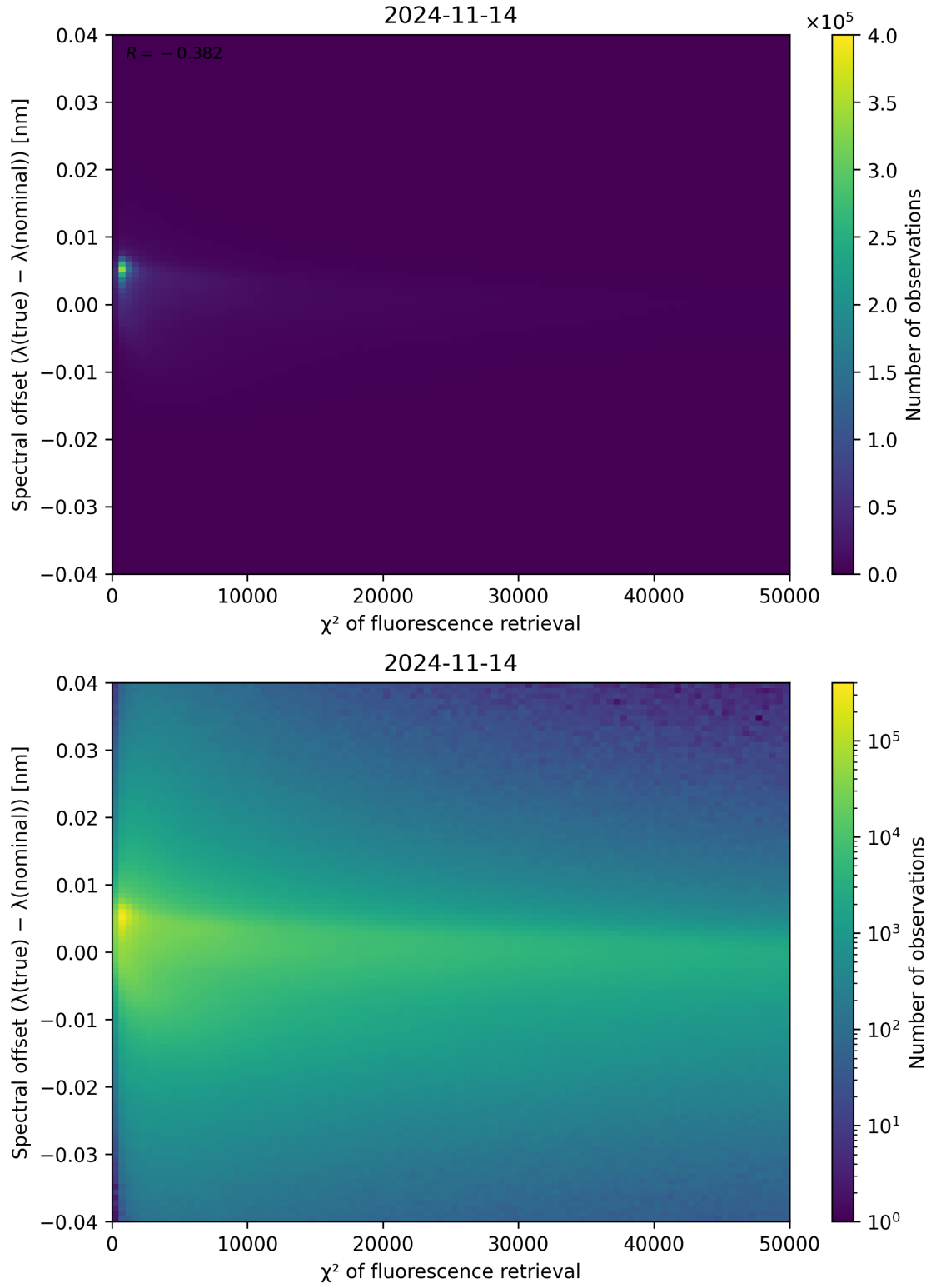
Figure 72: Scatter density plot of “ \chi^2 of fluorescence retrieval” against “Spectral offset ( \lambda_{\text{true}} - \lambda_{\text{nominal}} )” for 2024-11-14 to 2024-11-15.
