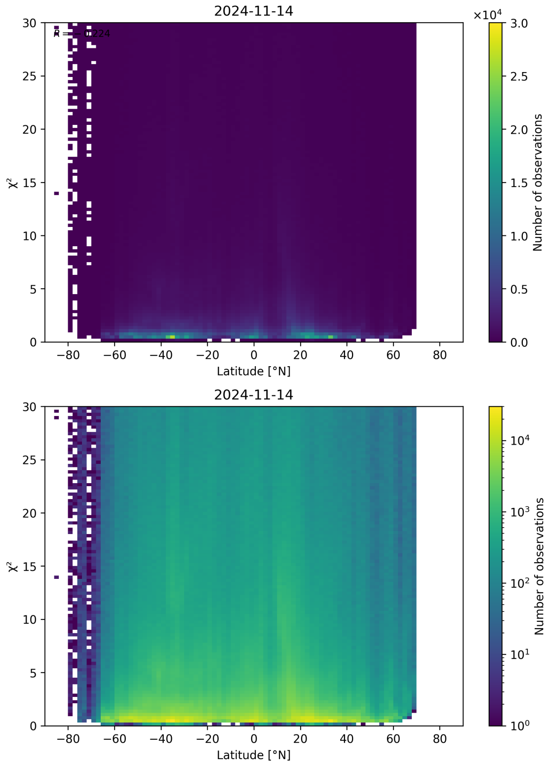
Figure 97: Scatter density plot of “Latitude” against “ \chi^2 ” for 2024-11-14 to 2024-11-15.
