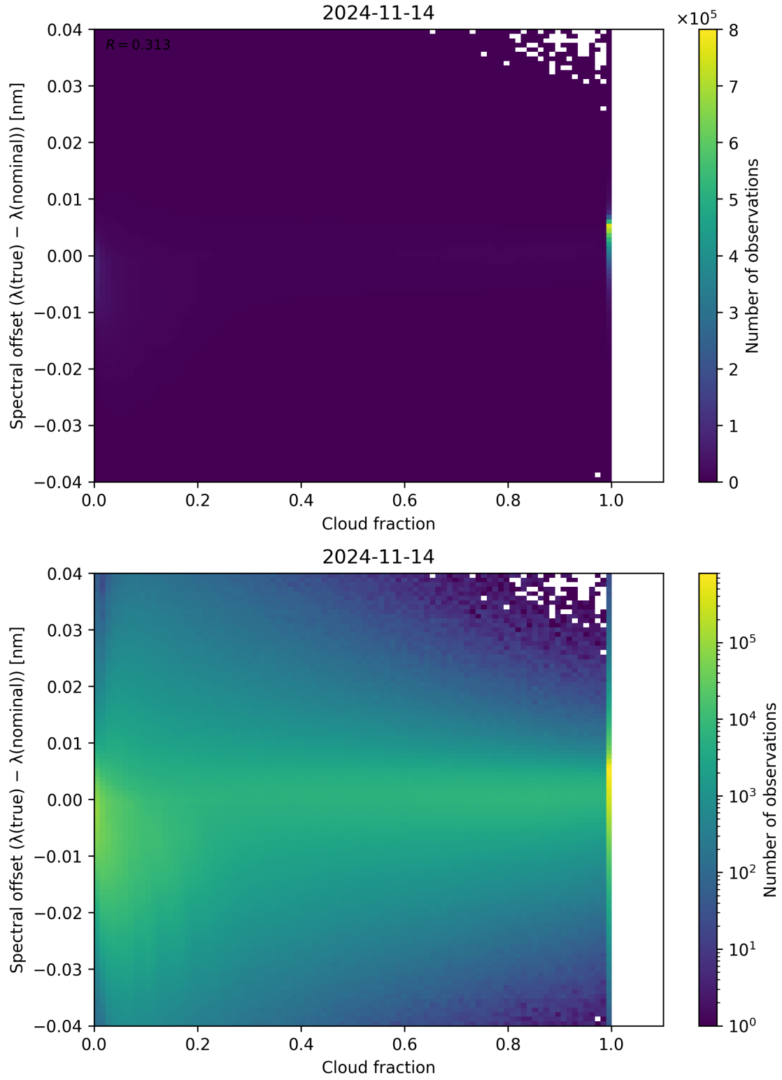
Figure 83: Scatter density plot of “Cloud fraction” against “Spectral offset ( \lambda_{\text{true}} - \lambda_{\text{nominal}} )” for 2024-11-14 to 2024-11-15.
