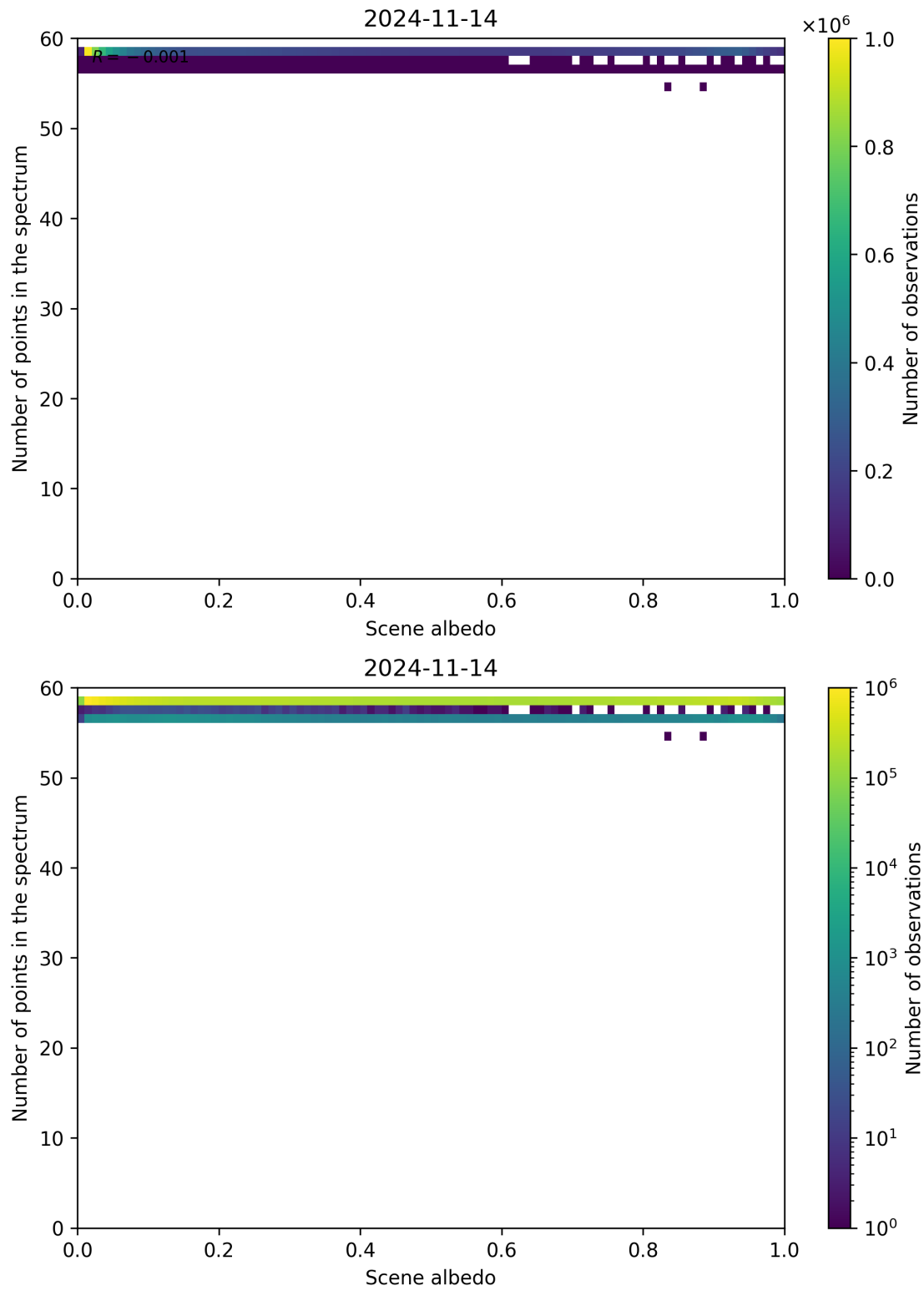
Figure 116: Scatter density plot of “Scene albedo” against “Number of points in the spectrum” for 2024-11-14 to 2024-11-15.
