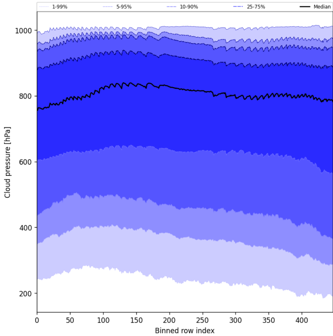
Figure 47: Along track statistics of “Cloud pressure” for 2024-11-14 to 2024-11-15
