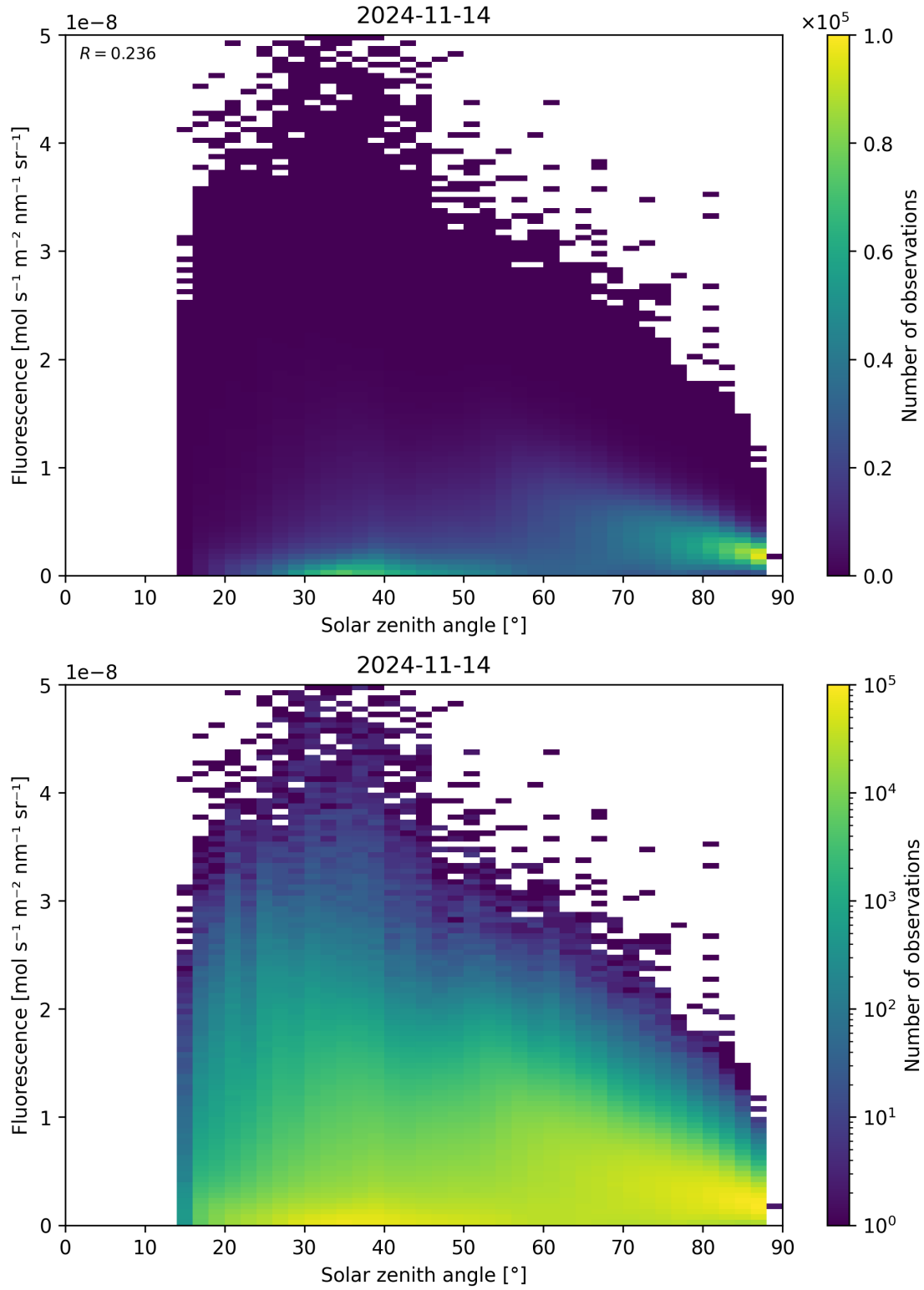
Figure 123: Scatter density plot of “Solar zenith angle” against “Fluorescence” for 2024-11-14 to 2024-11-15.
