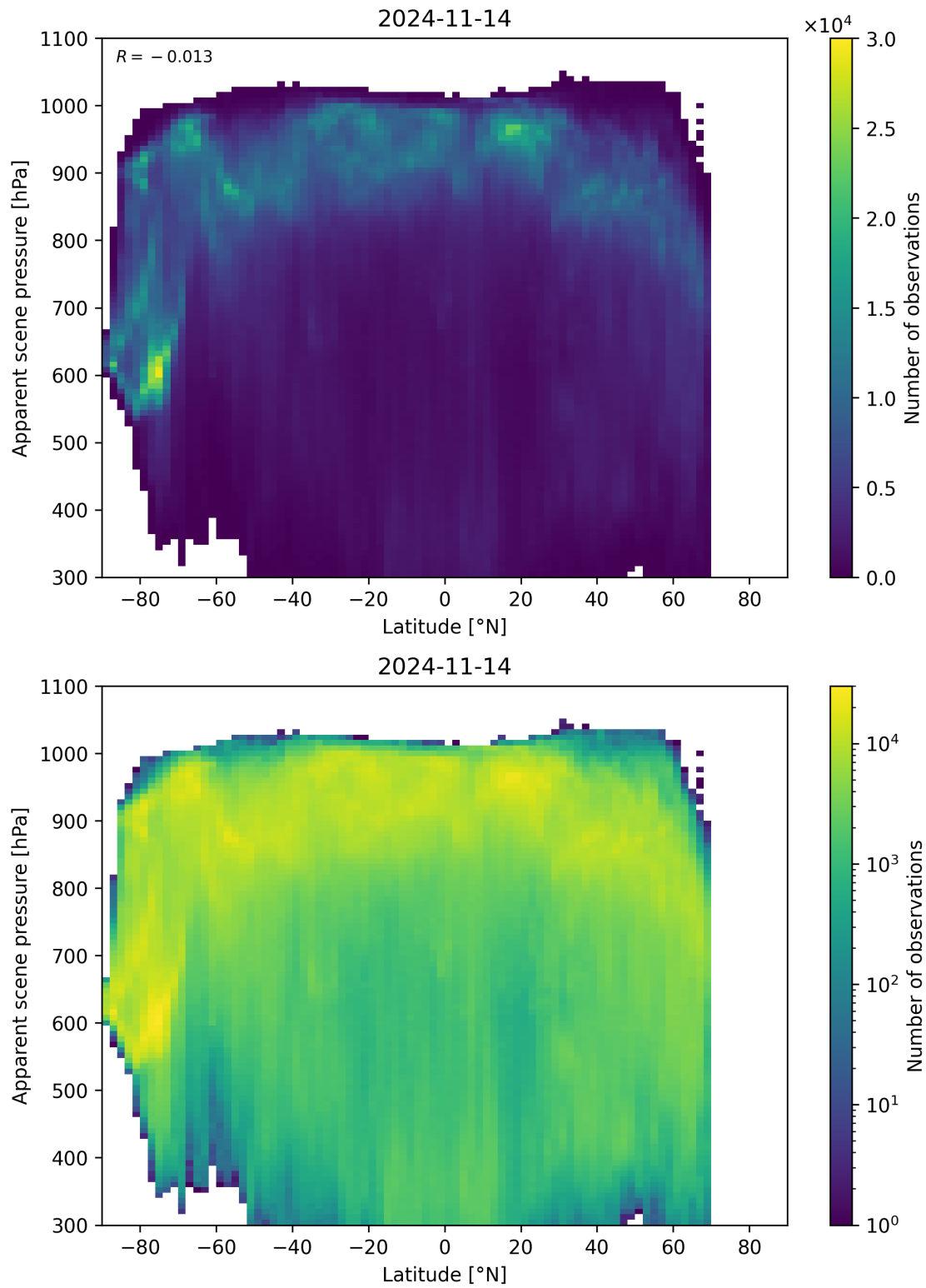
Figure 96: Scatter density plot of “Latitude” against “Apparent scene pressure” for 2024-11-14 to 2024-11-15.
