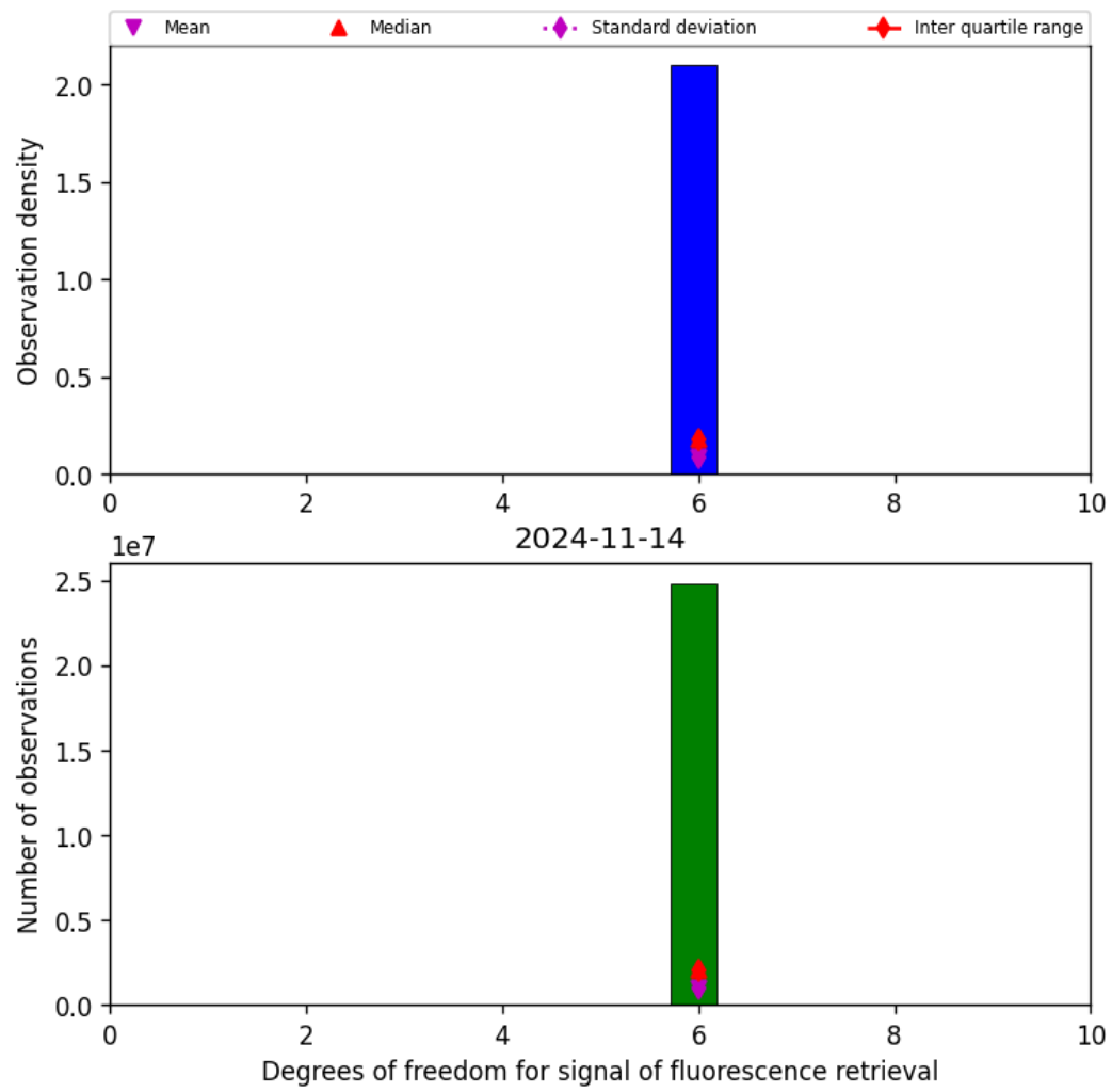
Figure 43: Histogram of “Degrees of freedom for signal of fluorescence retrieval” for 2024-11-14 to 2024-11-15
