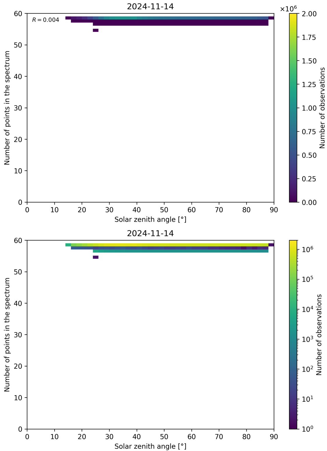
Figure 126: Scatter density plot of “Solar zenith angle” against “Number of points in the spectrum” for 2024-11-14 to 2024-11-15.
