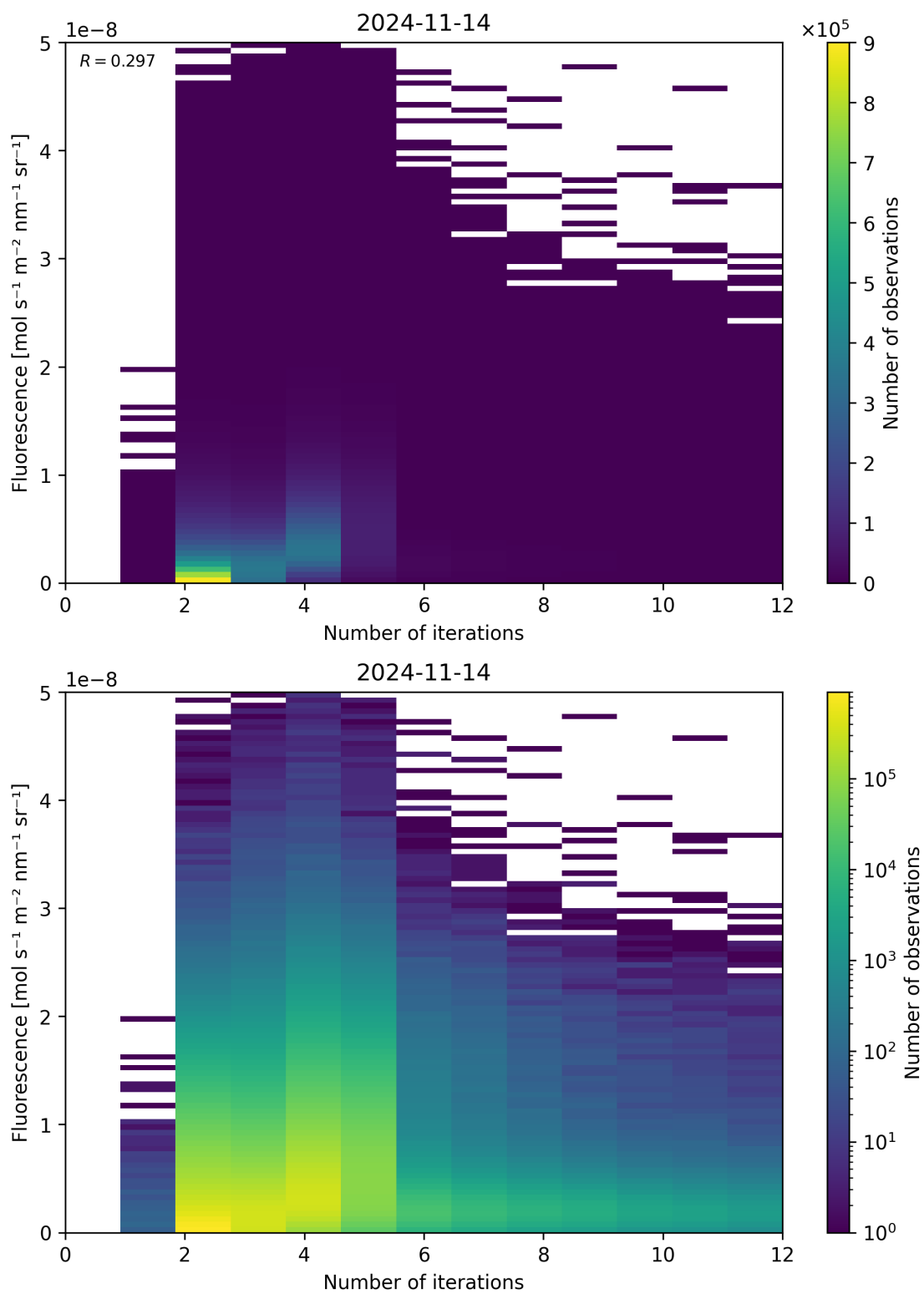
Figure 107: Scatter density plot of “Number of iterations” against “Fluorescence” for 2024-11-14 to 2024-11-15.
