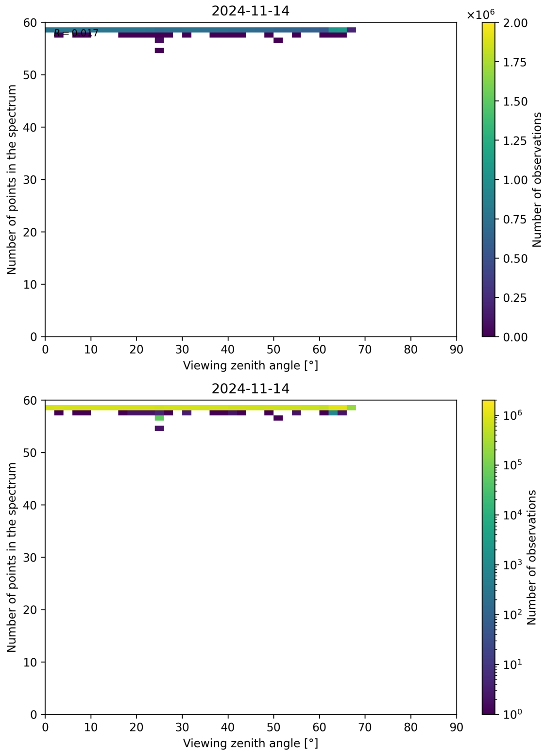
Figure 137: Scatter density plot of “Viewing zenith angle” against “Number of points in the spectrum” for 2024-11-14 to 2024-11-15.
