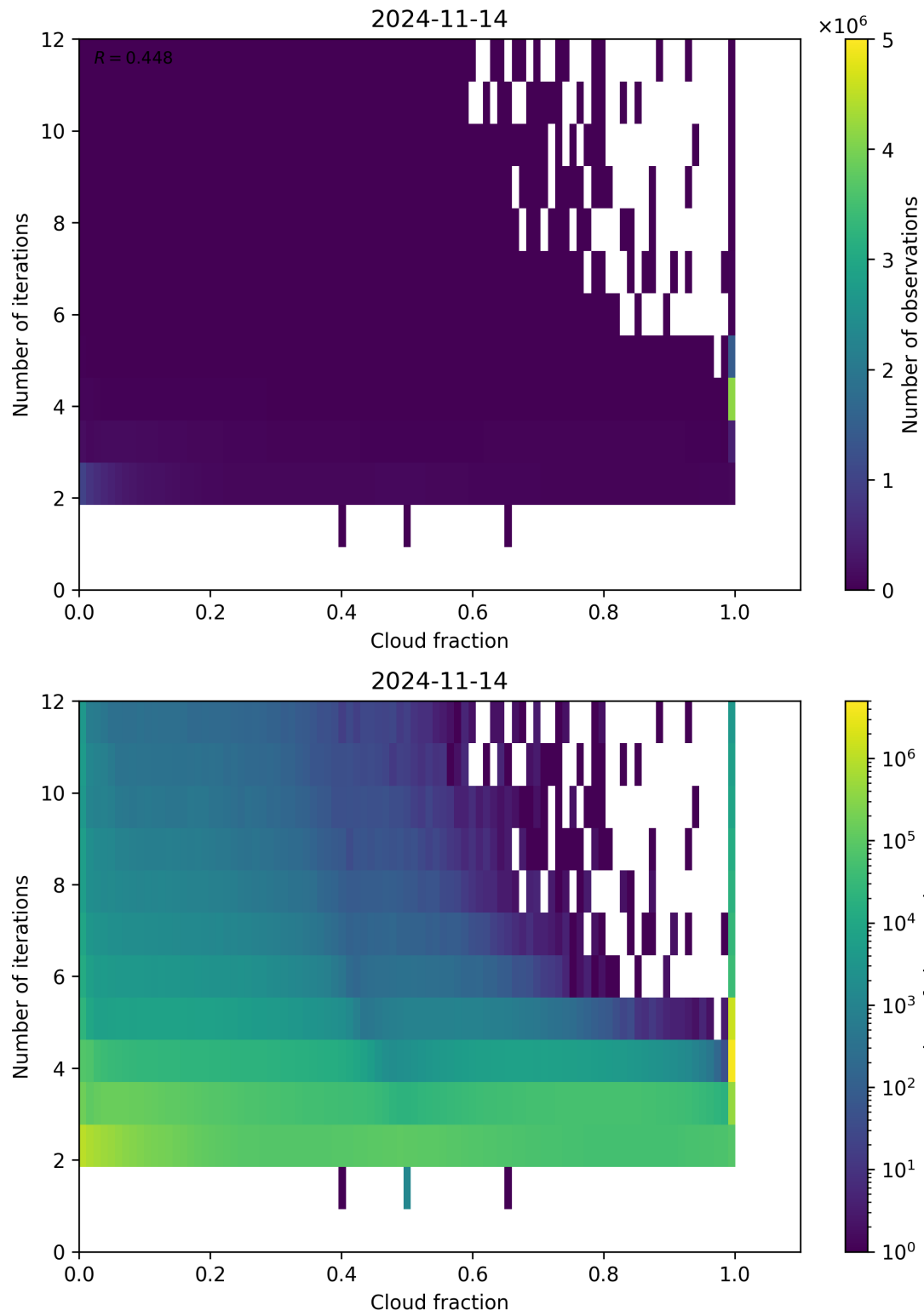
Figure 80: Scatter density plot of “Cloud fraction” against “Number of iterations” for 2024-11-14 to 2024-11-15.
