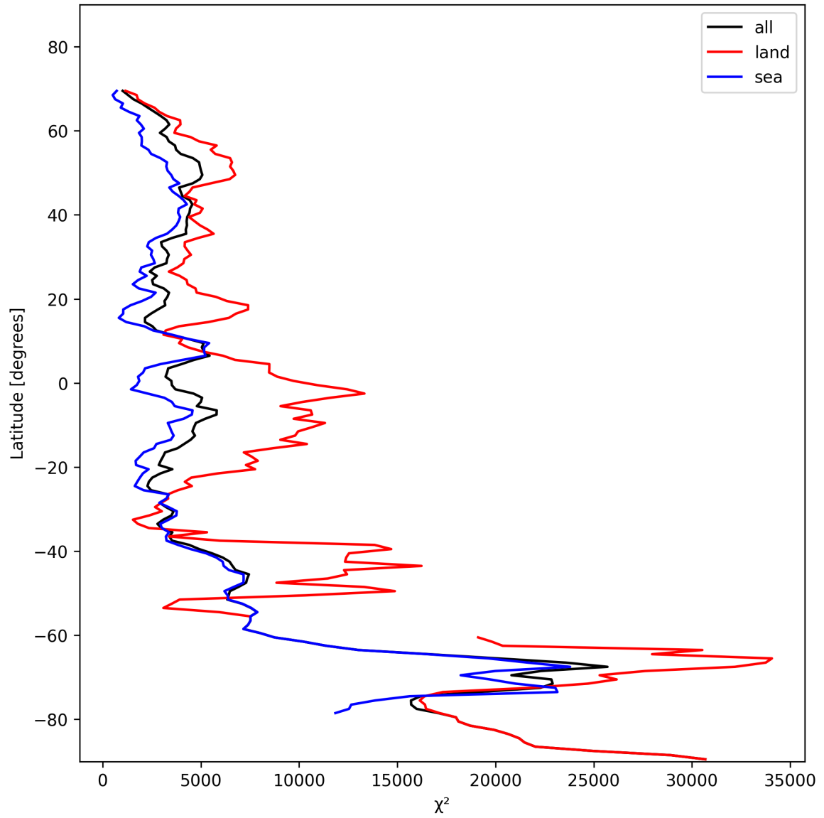
Figure 21: Zonal average of “ \chi^2 ” for 2024-11-14 to 2024-11-15.
