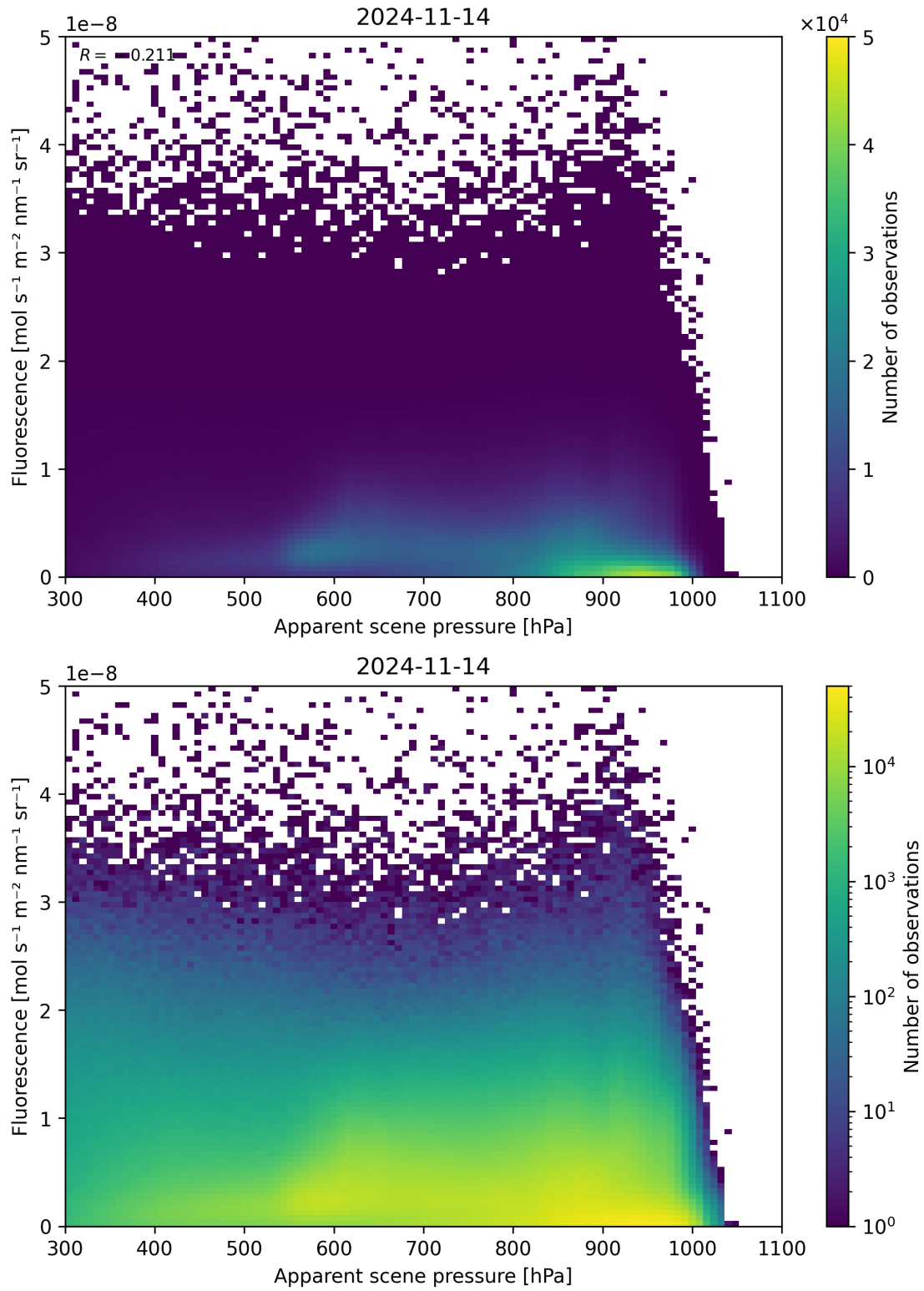
Figure 65: Scatter density plot of “Apparent scene pressure” against “Fluorescence” for 2024-11-14 to 2024-11-15.
