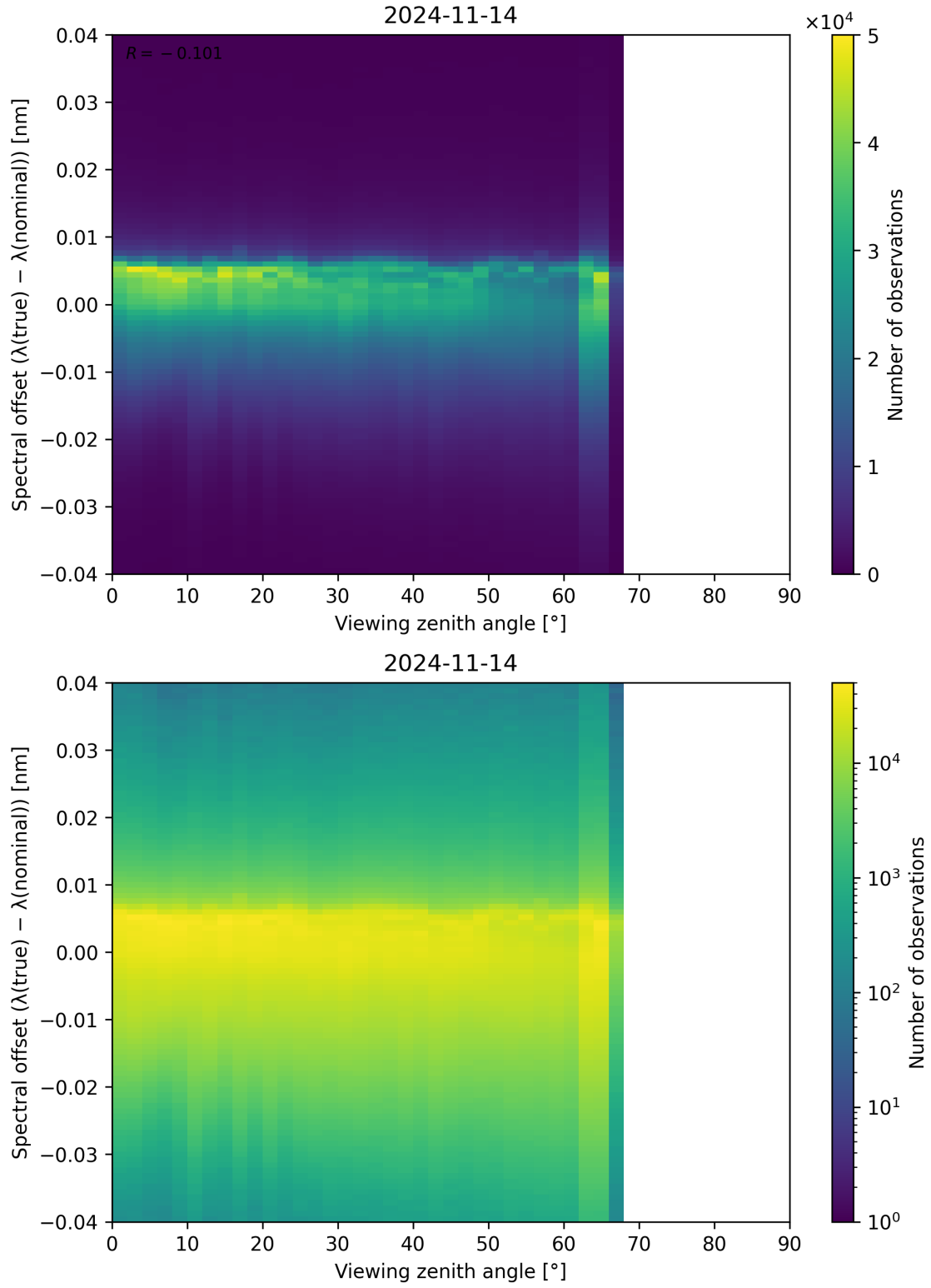
Figure 140: Scatter density plot of “Viewing zenith angle” against “Spectral offset ( \lambda_{\text{true}} - \lambda_{\text{nominal}} )” for 2024-11-14 to 2024-11-15.
