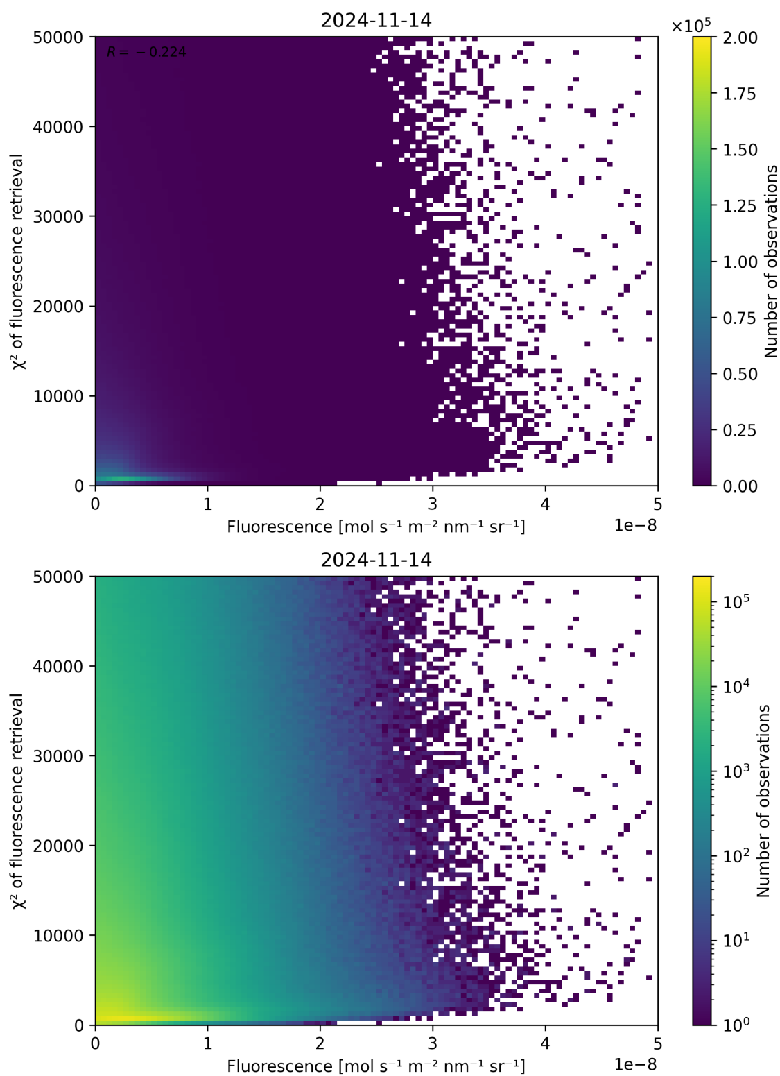
Figure 93: Scatter density plot of “Fluorescence” against “ \chi^2 of fluorescence retrieval” for 2024-11-14 to 2024-11-15.
