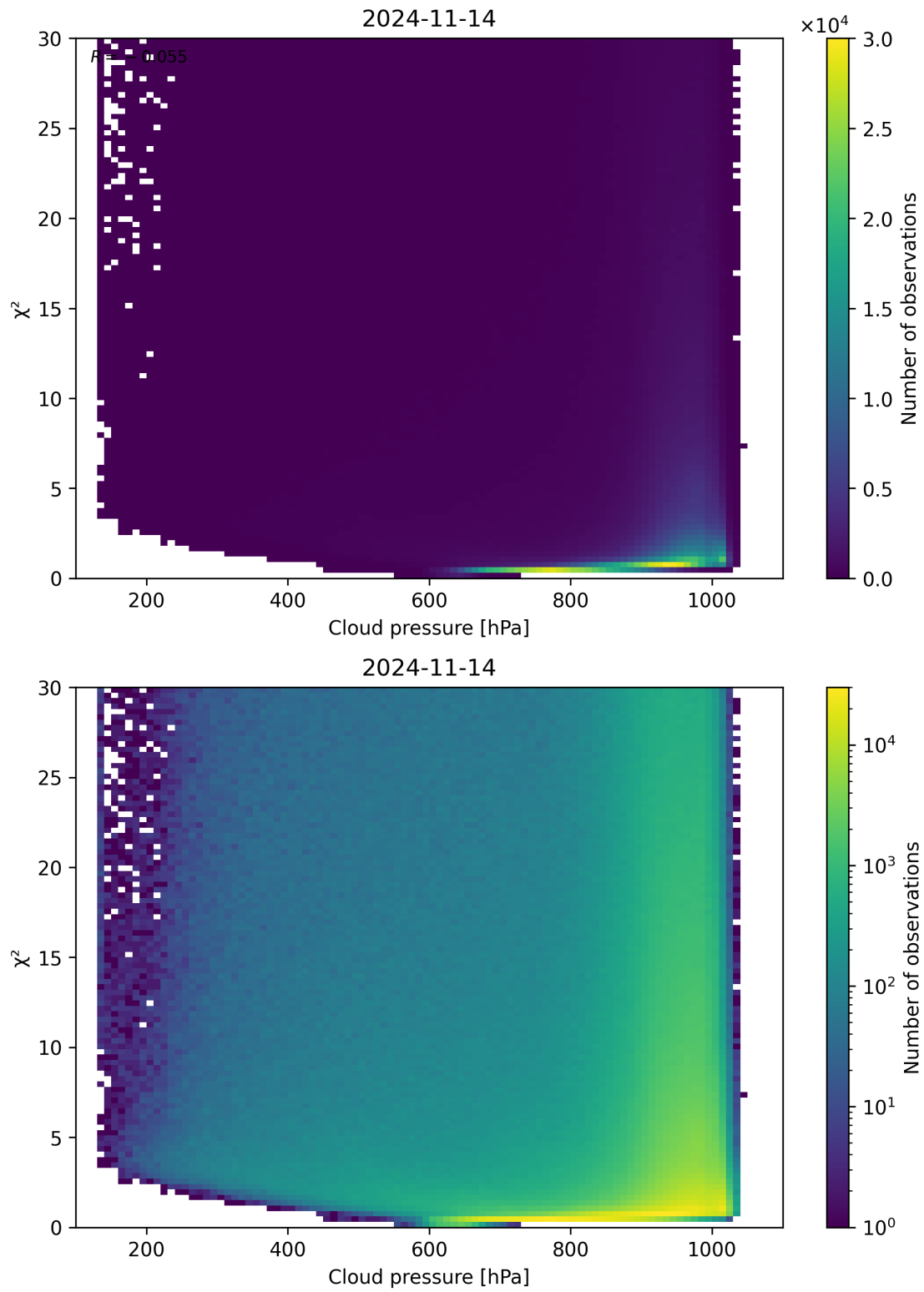
Figure 85: Scatter density plot of “Cloud pressure” against “ \chi^2 ” for 2024-11-14 to 2024-11-15.
