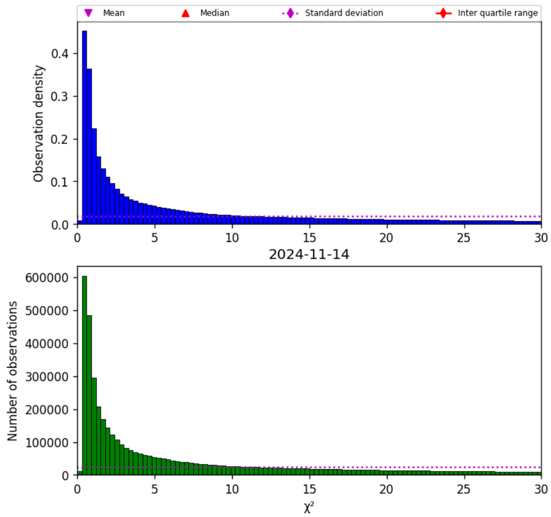
Figure 38: Histogram of " \chi^2 " for 2024-11-14 to 2024-11-15
