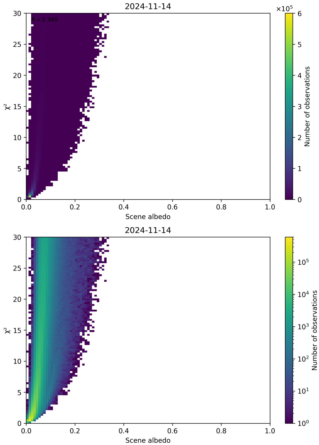
Figure 112: Scatter density plot of “Scene albedo” against “ \chi^2 ” for 2024-11-14 to 2024-11-15.
