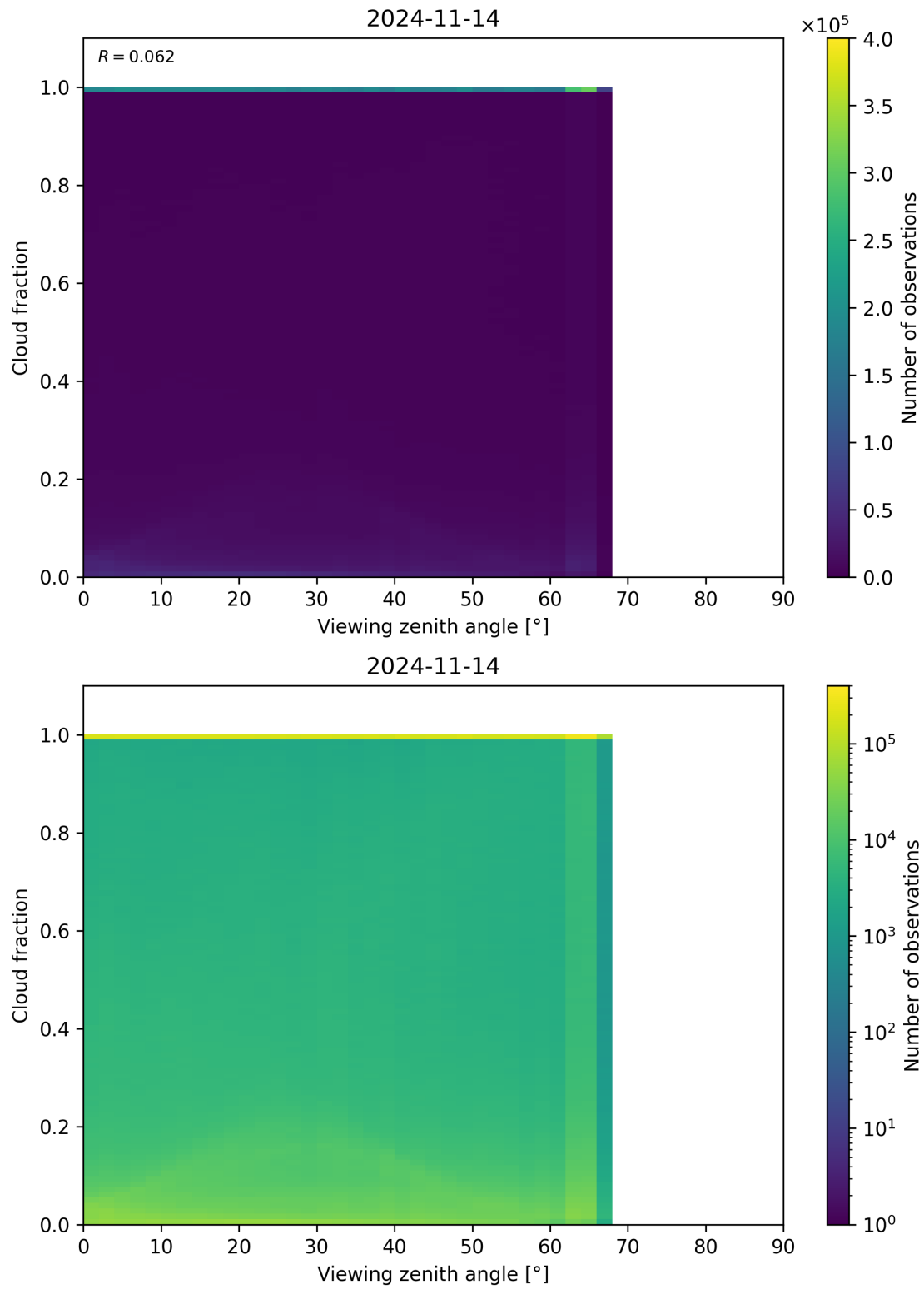
Figure 132: Scatter density plot of “Viewing zenith angle” against “Cloud fraction” for 2024-11-14 to 2024-11-15.
