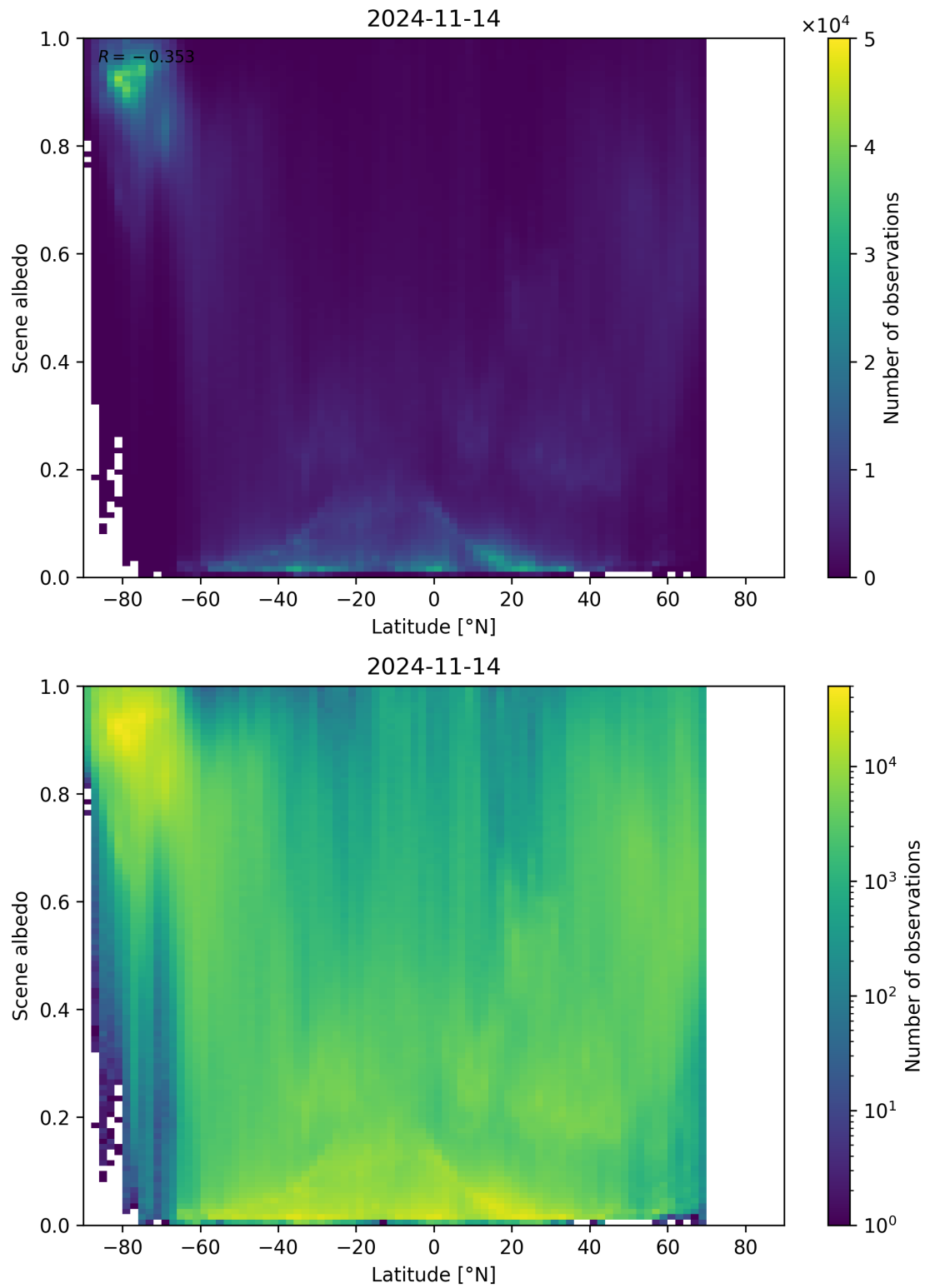
Figure 104: Scatter density plot of “Latitude” against “Scene albedo” for 2024-11-14 to 2024-11-15.
