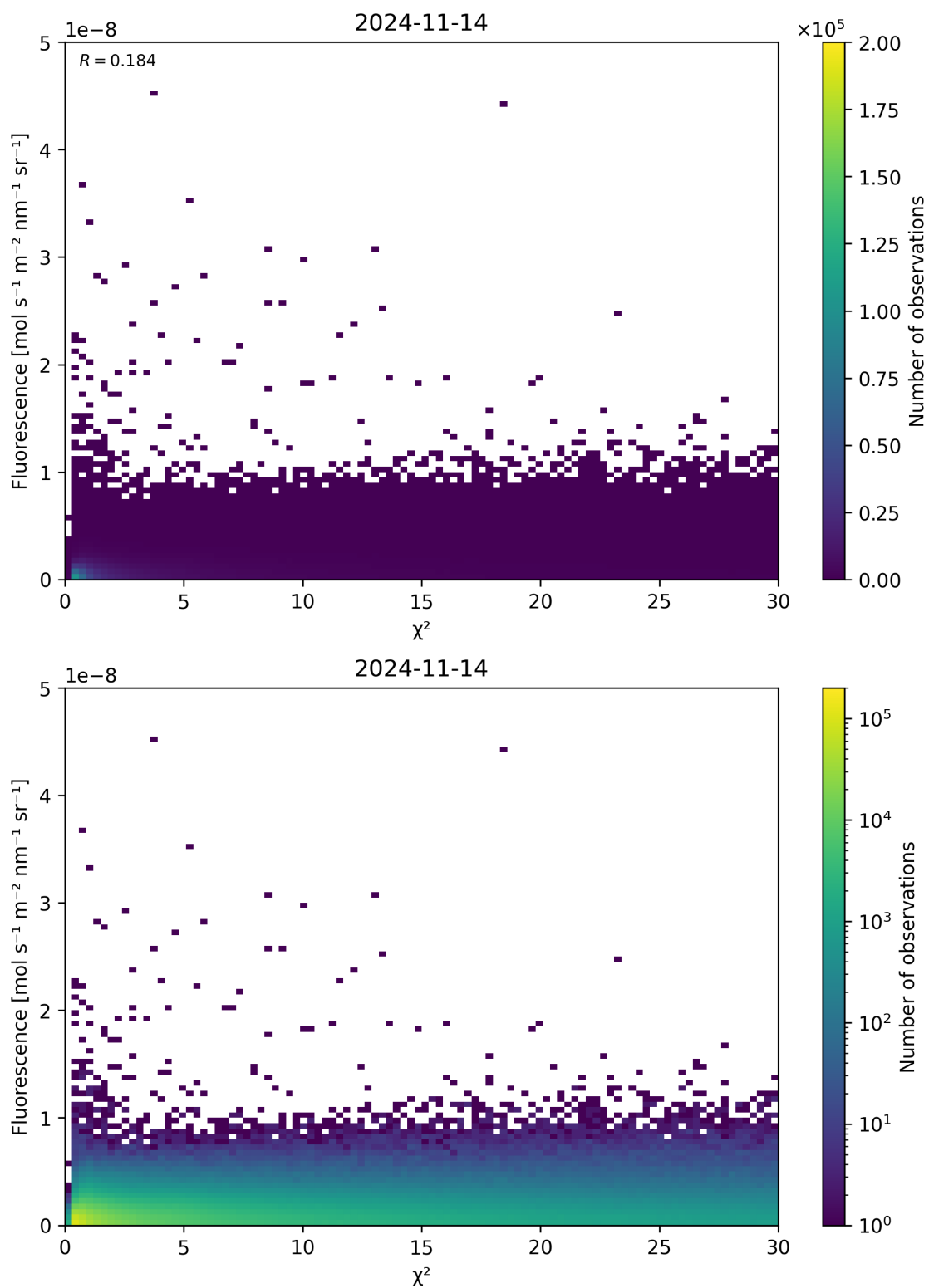
Figure 70: Scatter density plot of “ \chi^2 ” against “Fluorescence” for 2024-11-14 to 2024-11-15.
