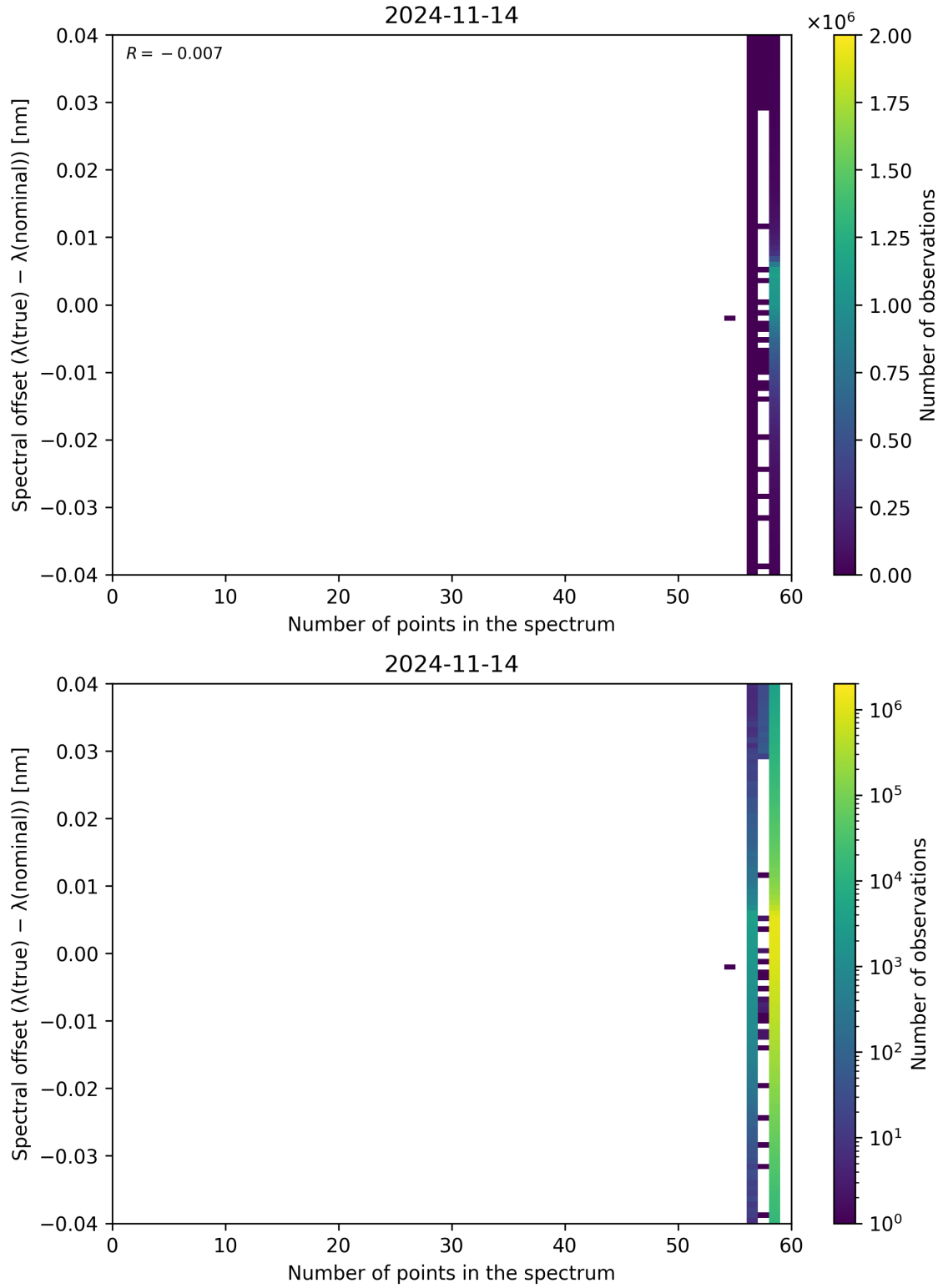
Figure 110: Scatter density plot of “Number of points in the spectrum” against “Spectral offset ( \lambda_{\text{true}} - \lambda_{\text{nominal}} )” for 2024-11-14 to 2024-11-15.
