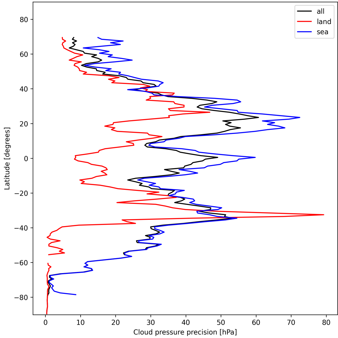
Figure 14: Zonal average of “Cloud pressure precision” for 2024-11-14 to 2024-11-15.
