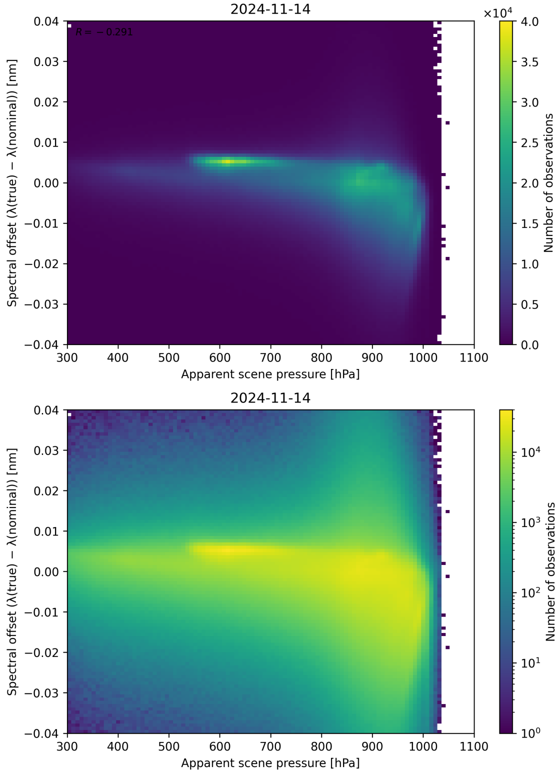
Figure 68: Scatter density plot of “Apparent scene pressure” against “Spectral offset ( \lambda_{\text{true}} - \lambda_{\text{nominal}} )” for 2024-11-14 to 2024-11-15.
