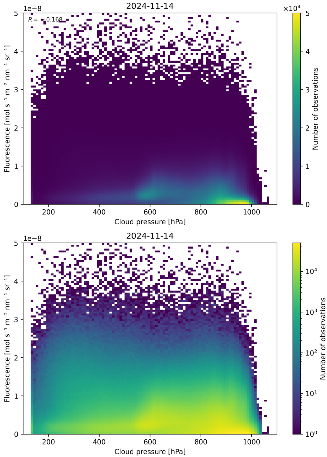
Figure 88: Scatter density plot of “Cloud pressure” against “Fluorescence” for 2024-11-14 to 2024-11-15.
