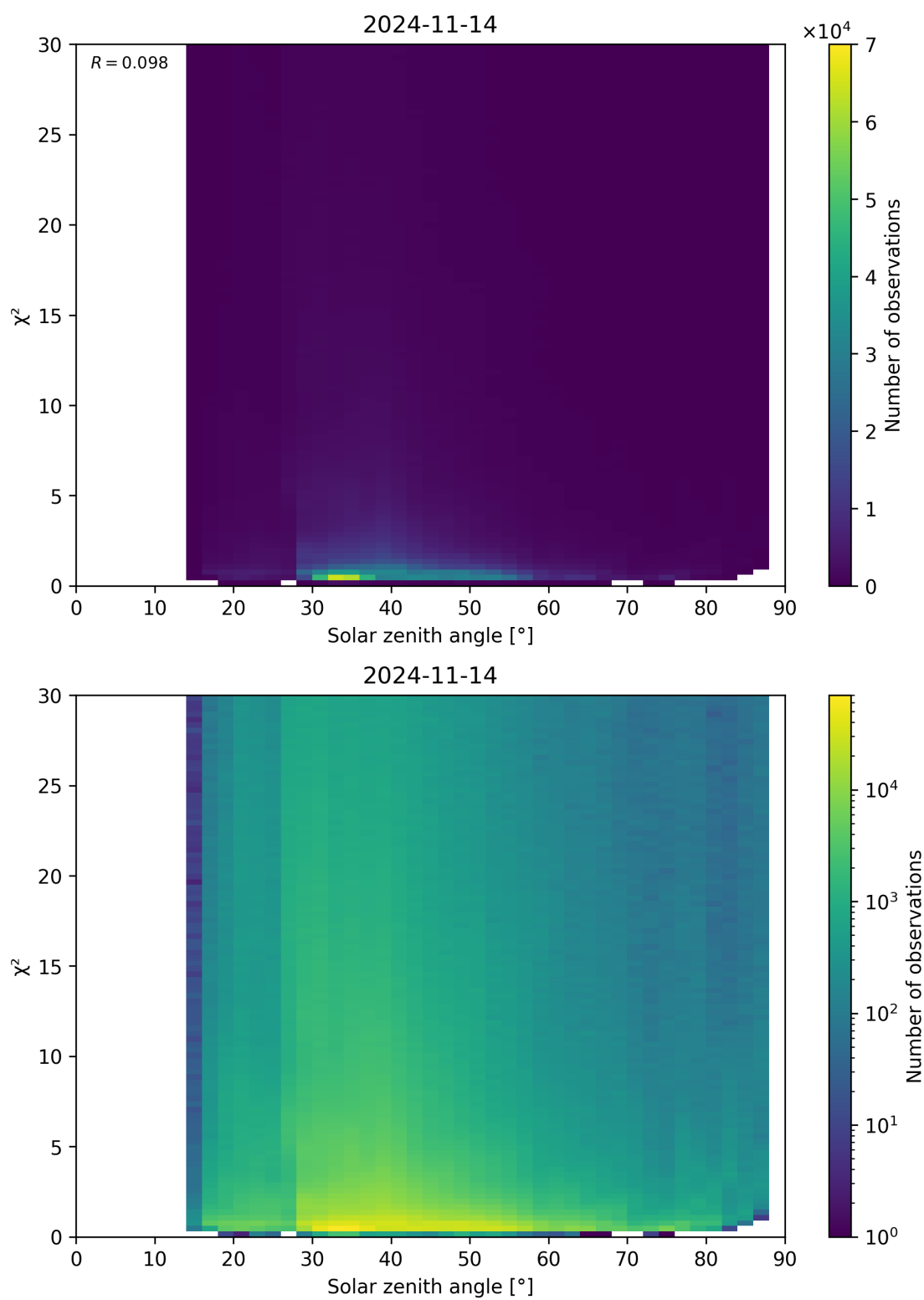
Figure 119: Scatter density plot of “Solar zenith angle” against “ \chi^2 ” for 2024-11-14 to 2024-11-15.
