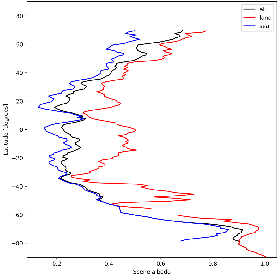
Figure 17: Zonal average of “Scene albedo” for 2024-11-14 to 2024-11-15.
