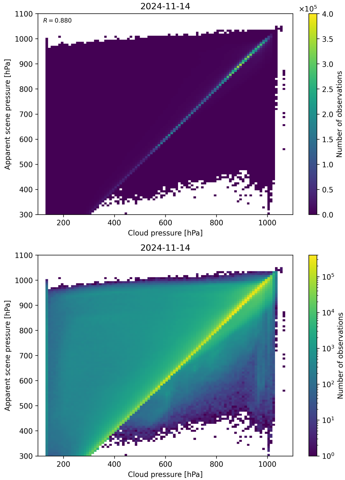
Figure 84: Scatter density plot of “Cloud pressure” against “Apparent scene pressure” for 2024-11-14 to 2024-11-15.
