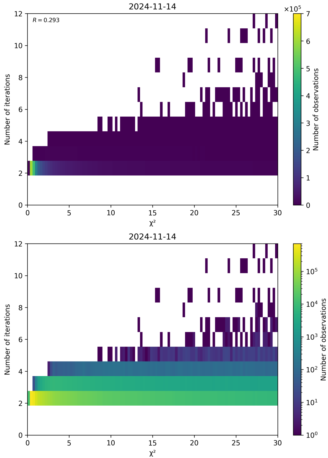
Figure 73: Scatter density plot of “ \chi^2 ” against “Number of iterations” for 2024-11-14 to 2024-11-15.
