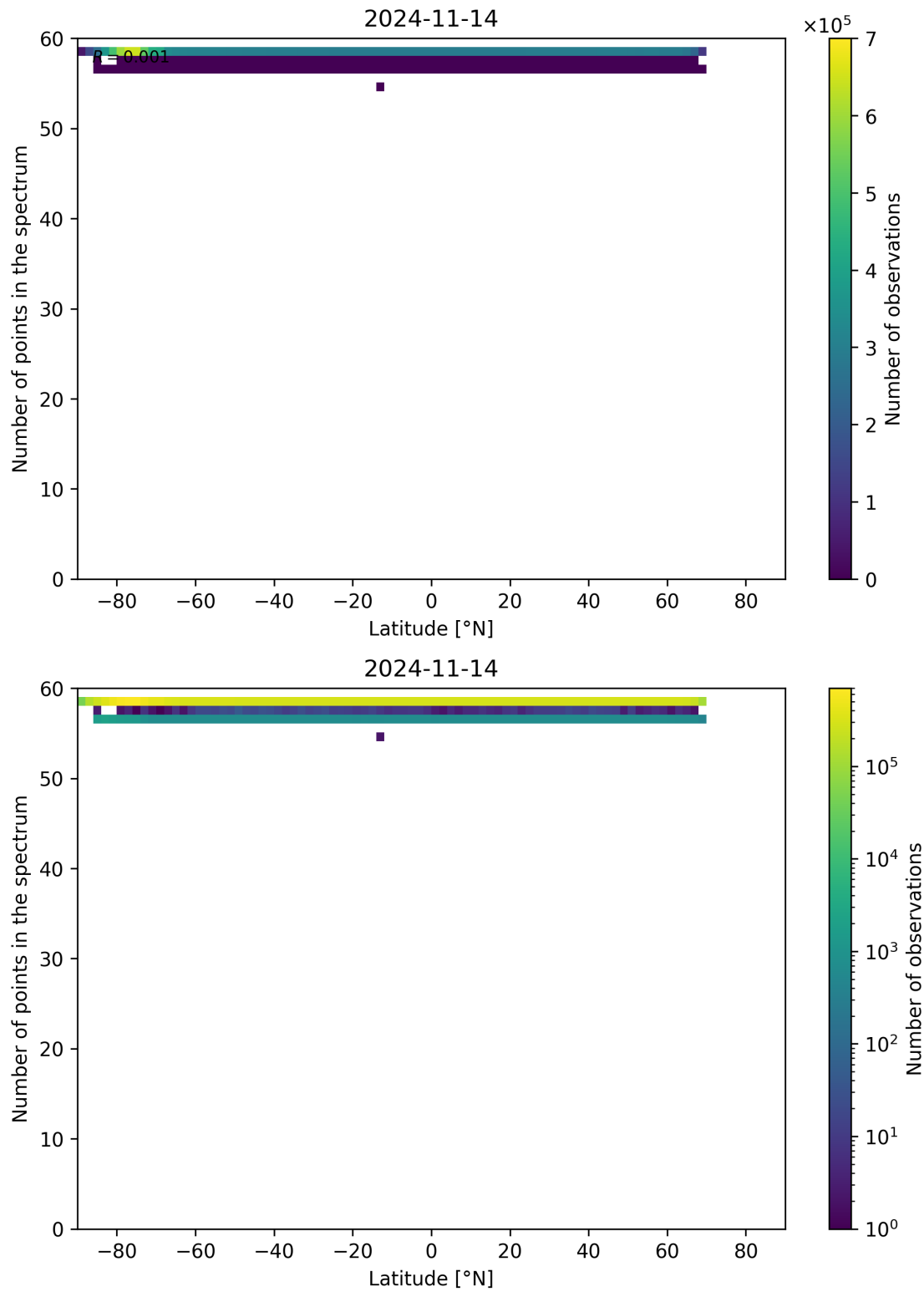
Figure 103: Scatter density plot of “Latitude” against “Number of points in the spectrum” for 2024-11-14 to 2024-11-15.
