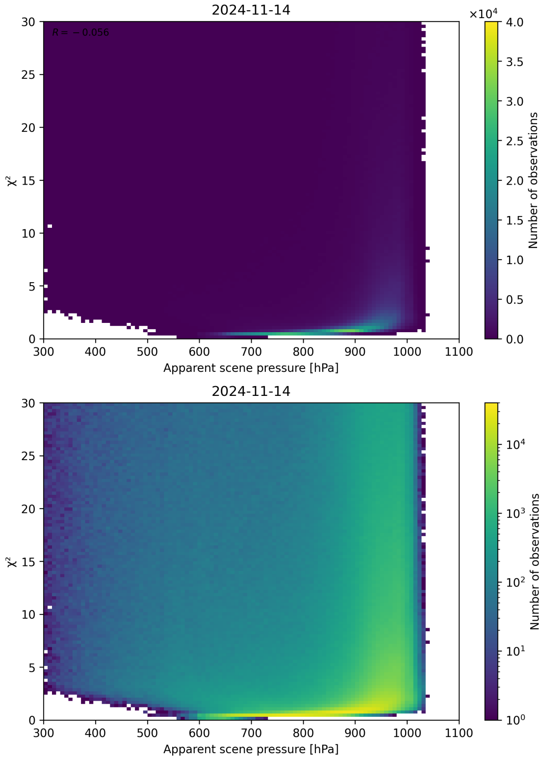
Figure 63: Scatter density plot of “Apparent scene pressure” against “ \chi^2 ” for 2024-11-14 to 2024-11-15.
