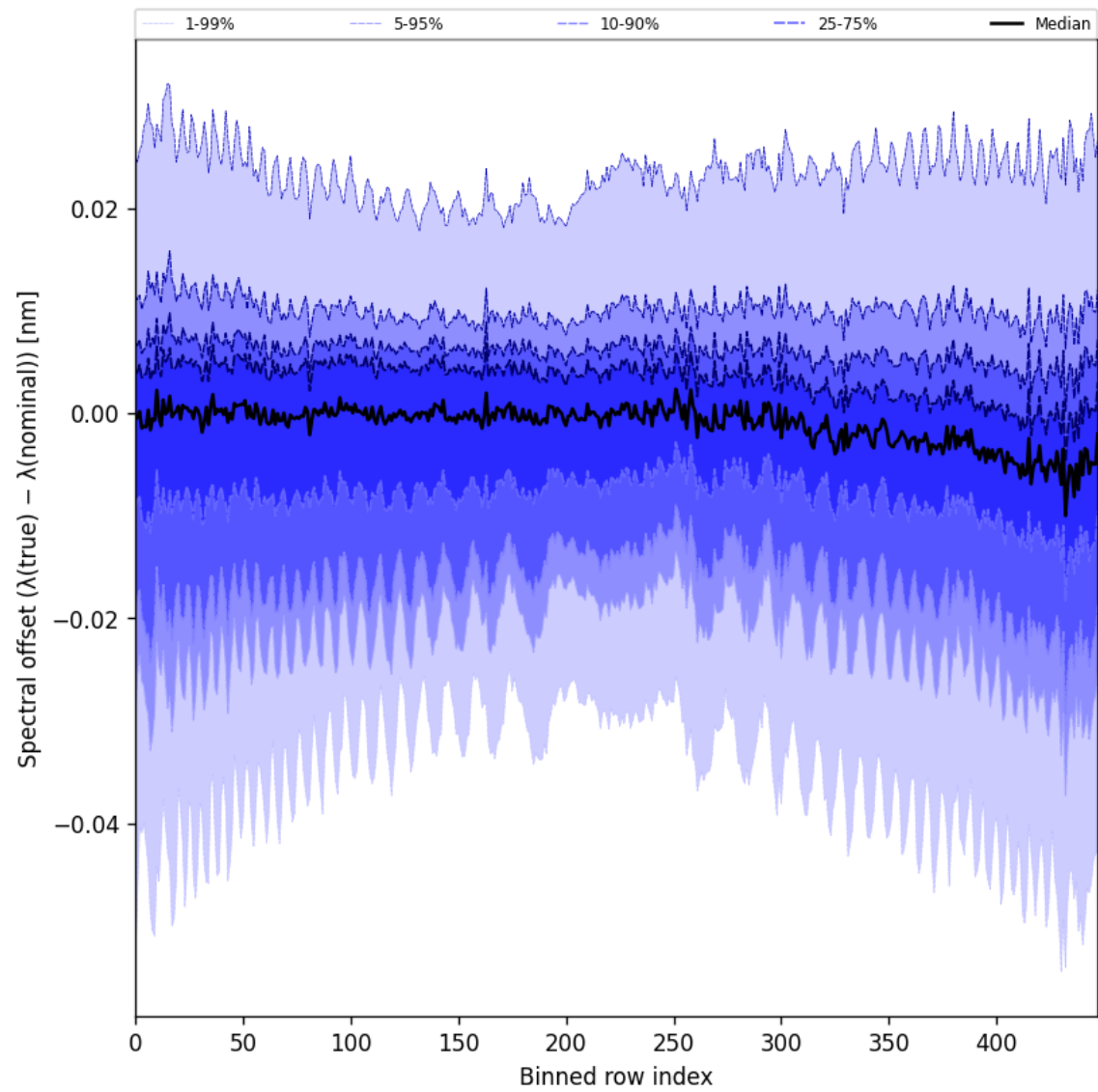
Figure 62: Along track statistics of “Spectral offset ( \lambda_{\text{true}} - \lambda_{\text{nominal}} )” for 2024-11-14 to 2024-11-15
