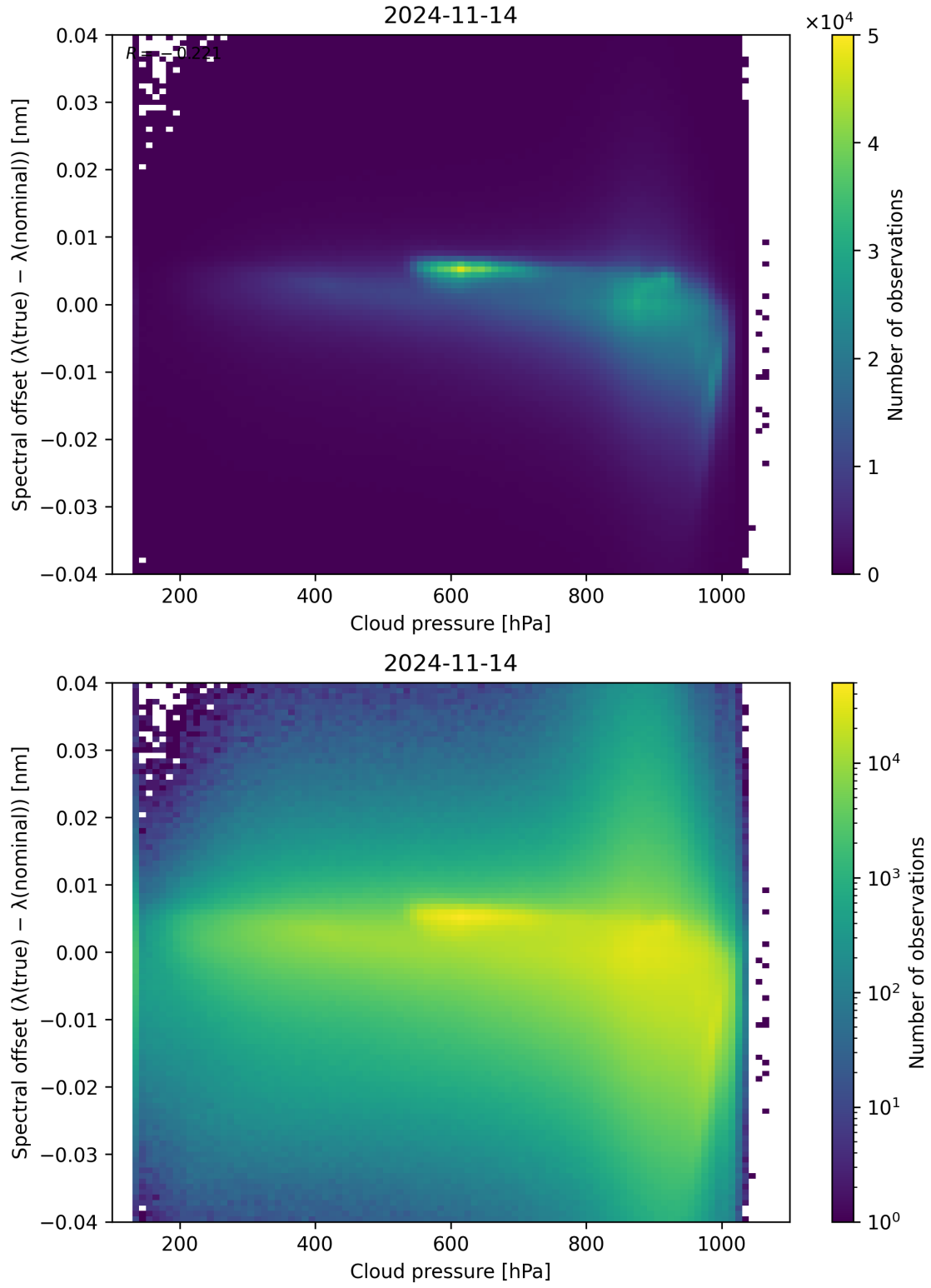
Figure 92: Scatter density plot of “Cloud pressure” against “Spectral offset ( \lambda_{\text{true}} - \lambda_{\text{nominal}} )” for 2024-11-14 to 2024-11-15.
