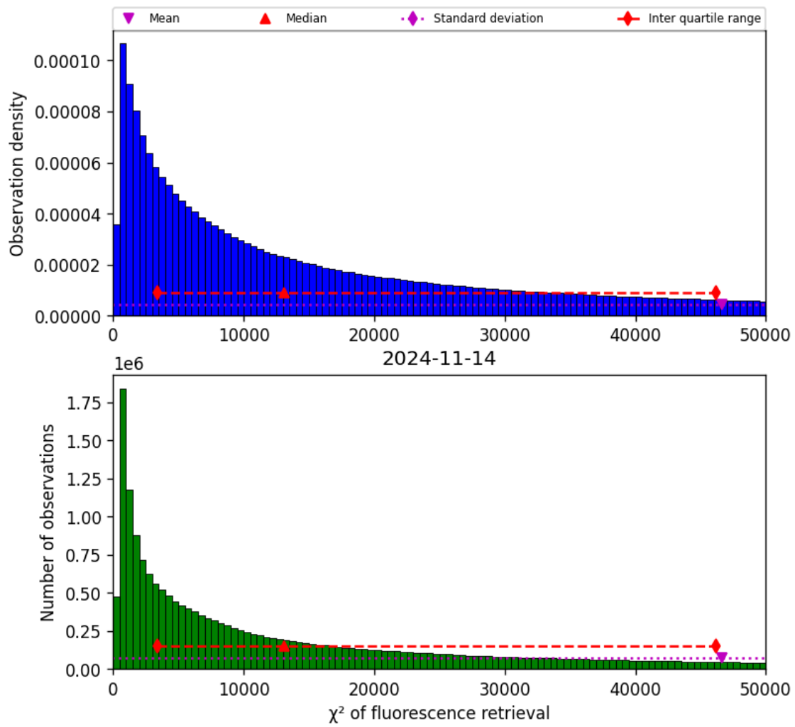
Figure 42: Histogram of “ \chi^2 of fluorescence retrieval” for 2024-11-14 to 2024-11-15
