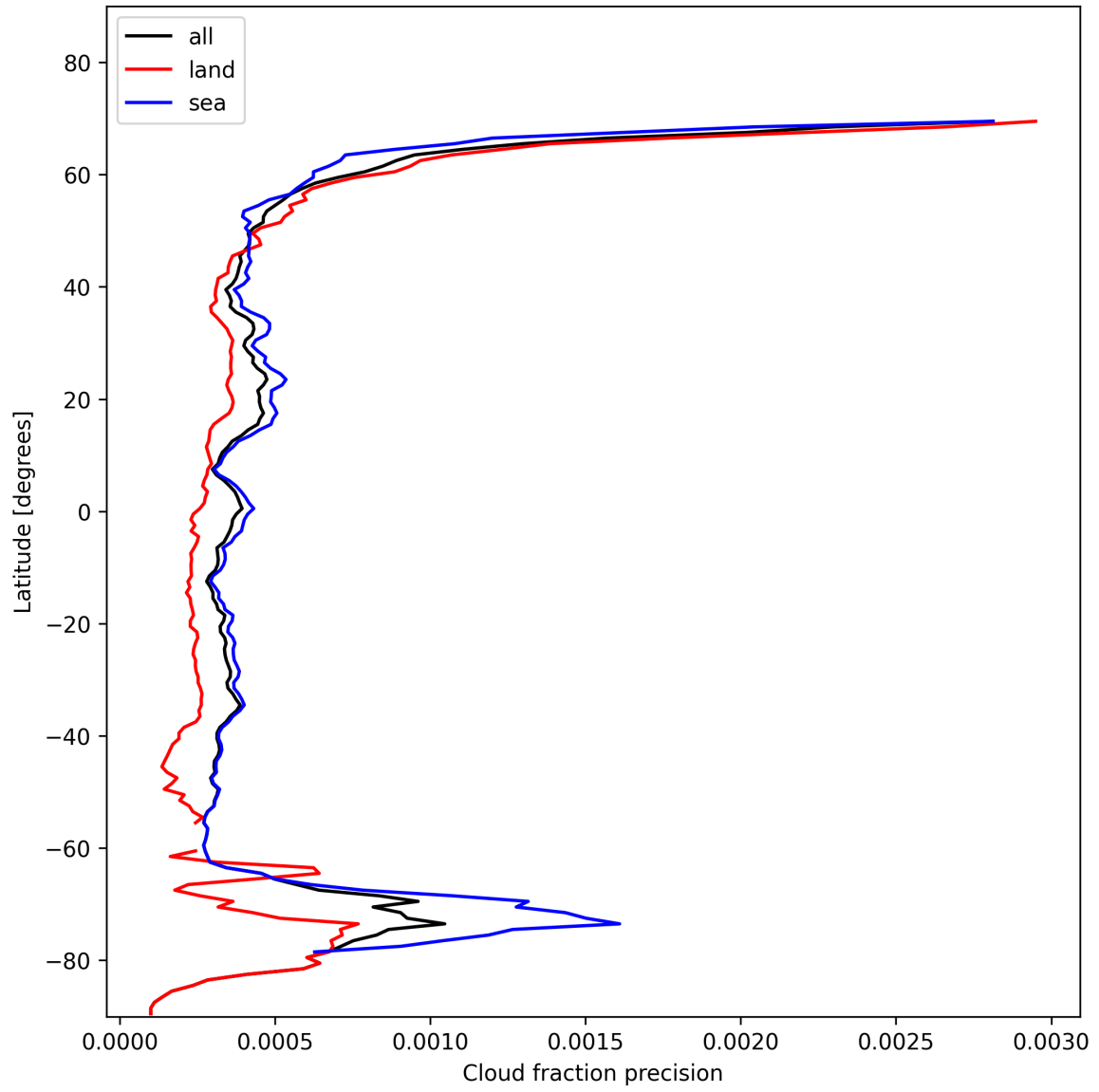
Figure 16: Zonal average of “Cloud fraction precision” for 2024-11-14 to 2024-11-15.
