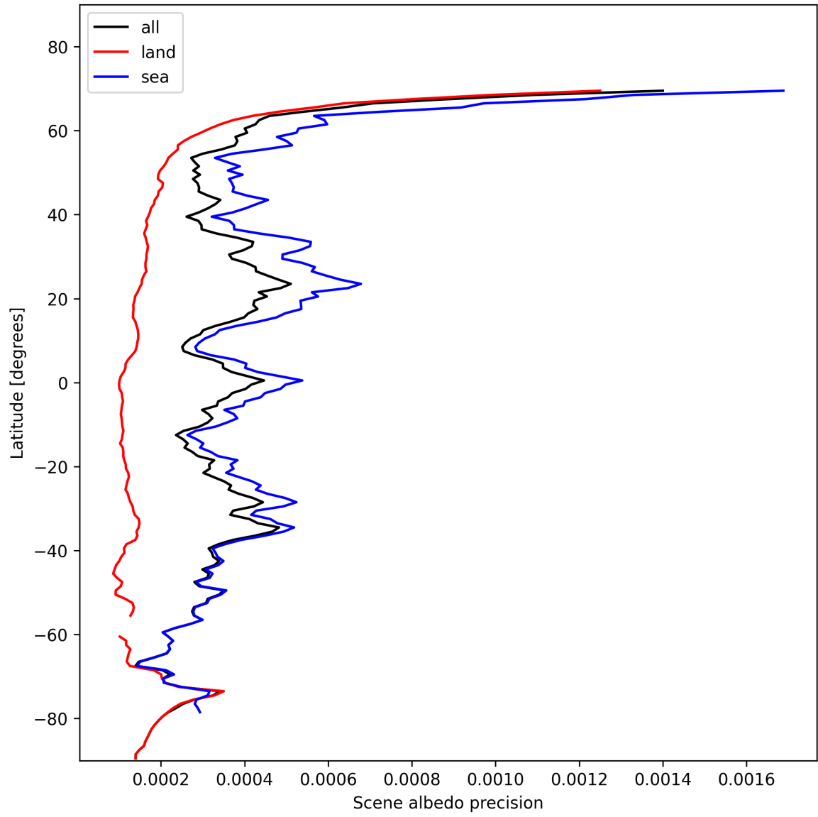
Figure 18: Zonal average of "Scene albedo precision" for 2024-11-14 to 2024-11-15.
