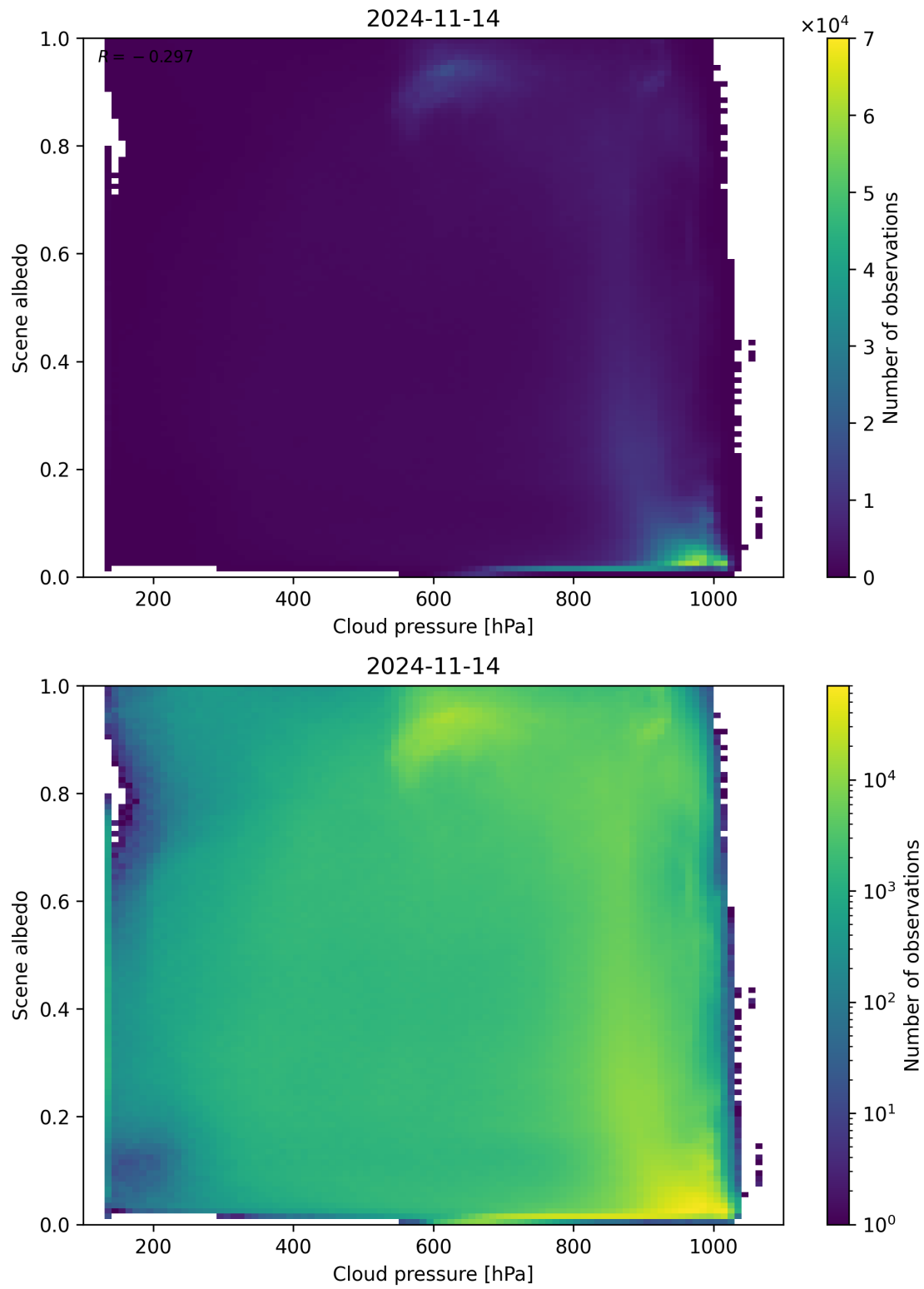
Figure 91: Scatter density plot of “Cloud pressure” against “Scene albedo” for 2024-11-14 to 2024-11-15.
