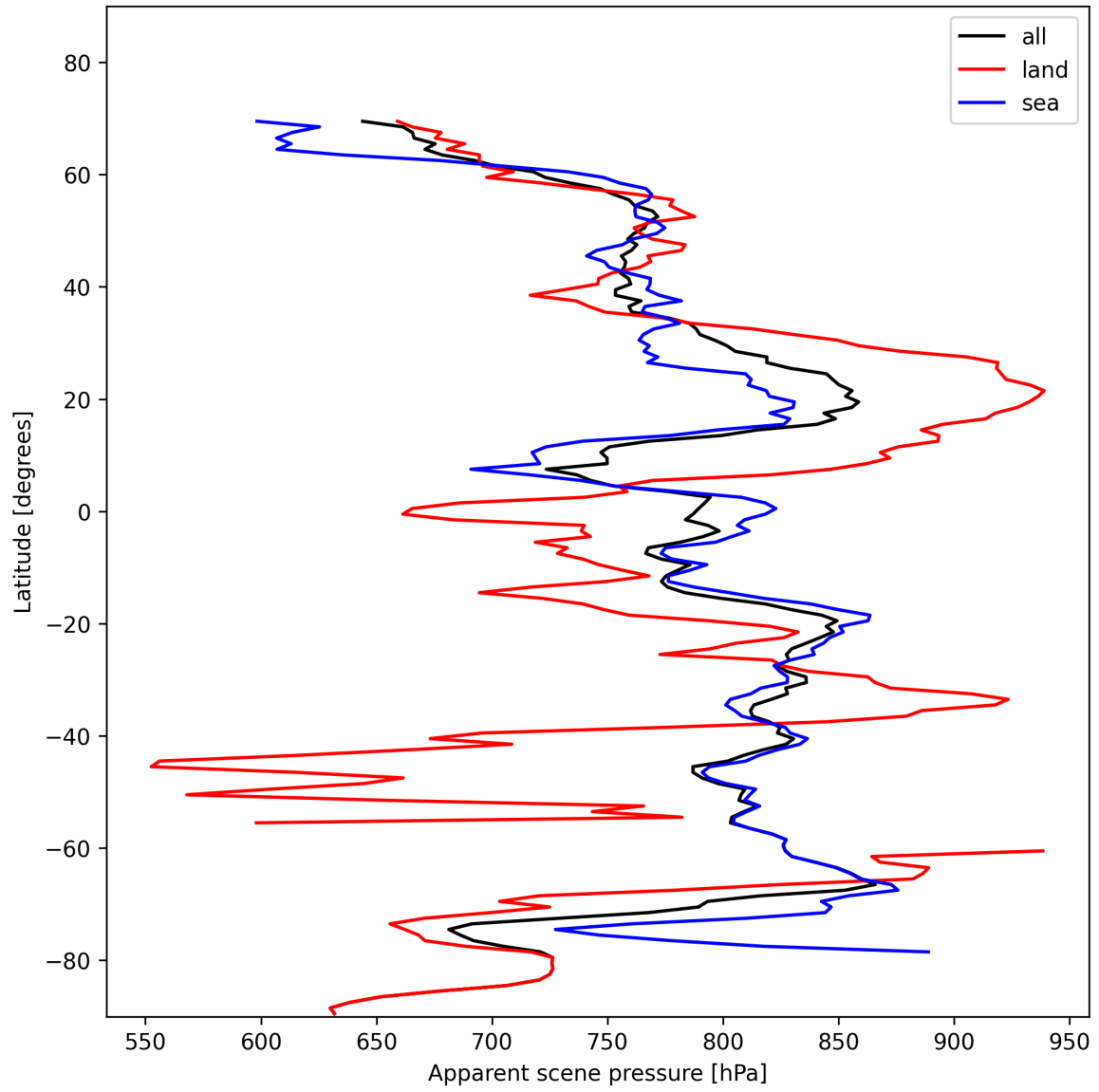
Figure 19: Zonal average of “Apparent scene pressure” for 2024-11-14 to 2024-11-15.
