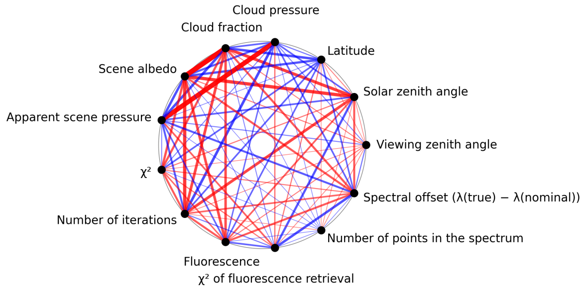
Figure 1: Map of correlation graph for 2024-11-14 to 2024-11-15.
