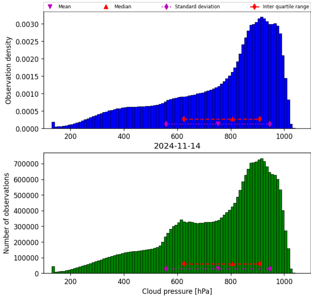
Figure 30: Histogram of “Cloud pressure” for 2024-11-14 to 2024-11-15
