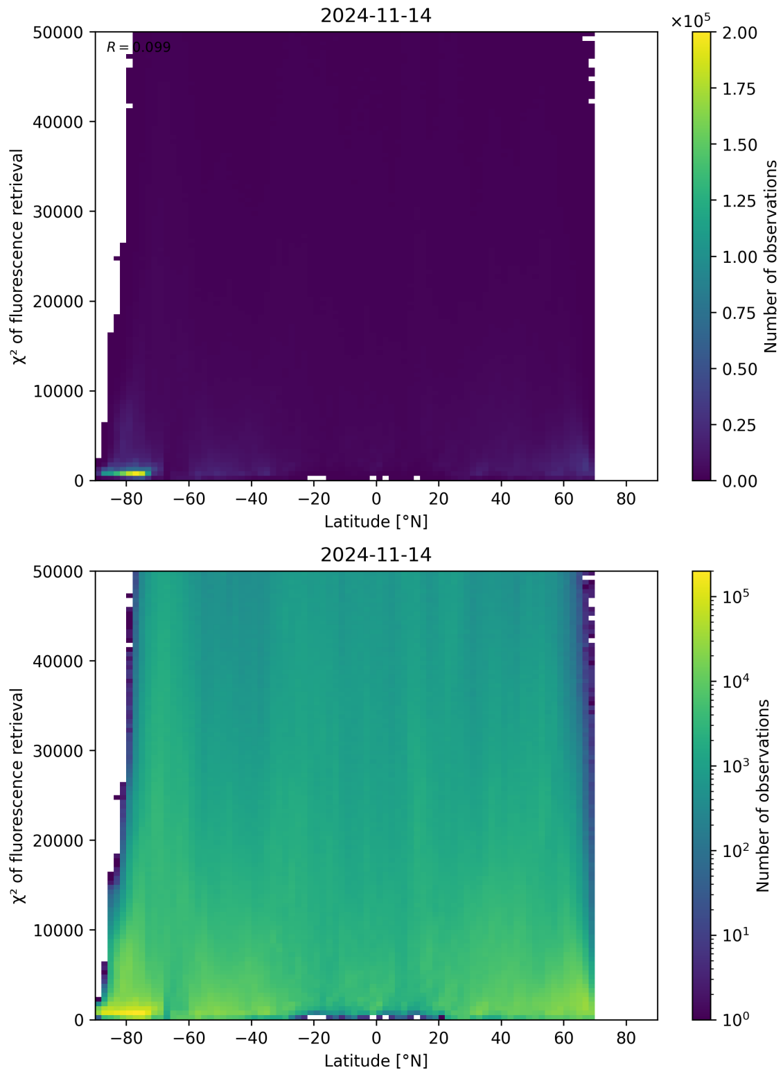
Figure 98: Scatter density plot of “Latitude” against “ \chi^2 of fluorescence retrieval” for 2024-11-14 to 2024-11-15.
