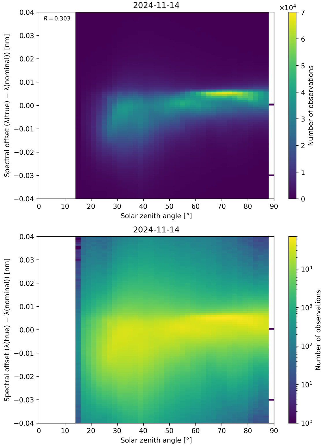
Figure 128: Scatter density plot of “Solar zenith angle” against “Spectral offset ( \lambda_{\text{true}} - \lambda_{\text{nominal}} )” for 2024-11-14 to 2024-11-15.
