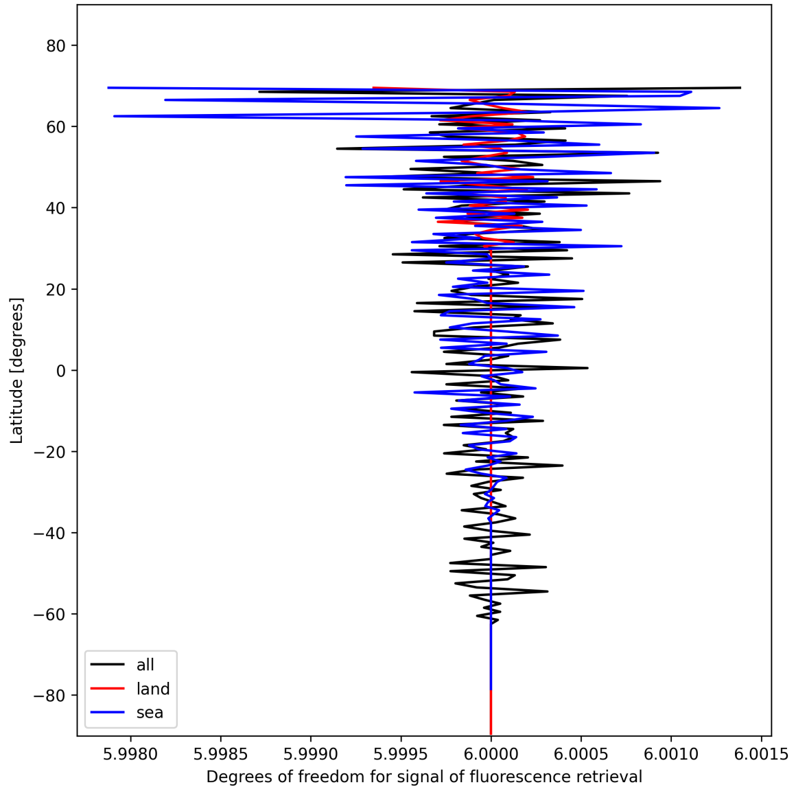
Figure 26: Zonal average of “Degrees of freedom for signal of fluorescence retrieval” for 2024-11-14 to 2024-11-15.
