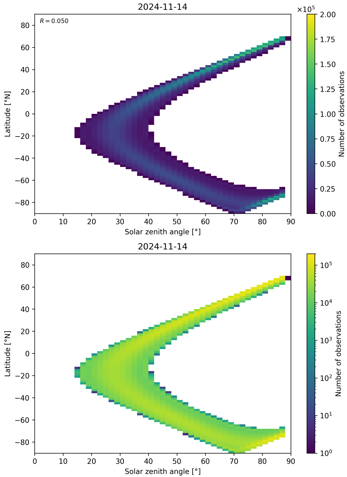
Figure 124: Scatter density plot of “Solar zenith angle” against “Latitude” for 2024-11-14 to 2024-11-15.
