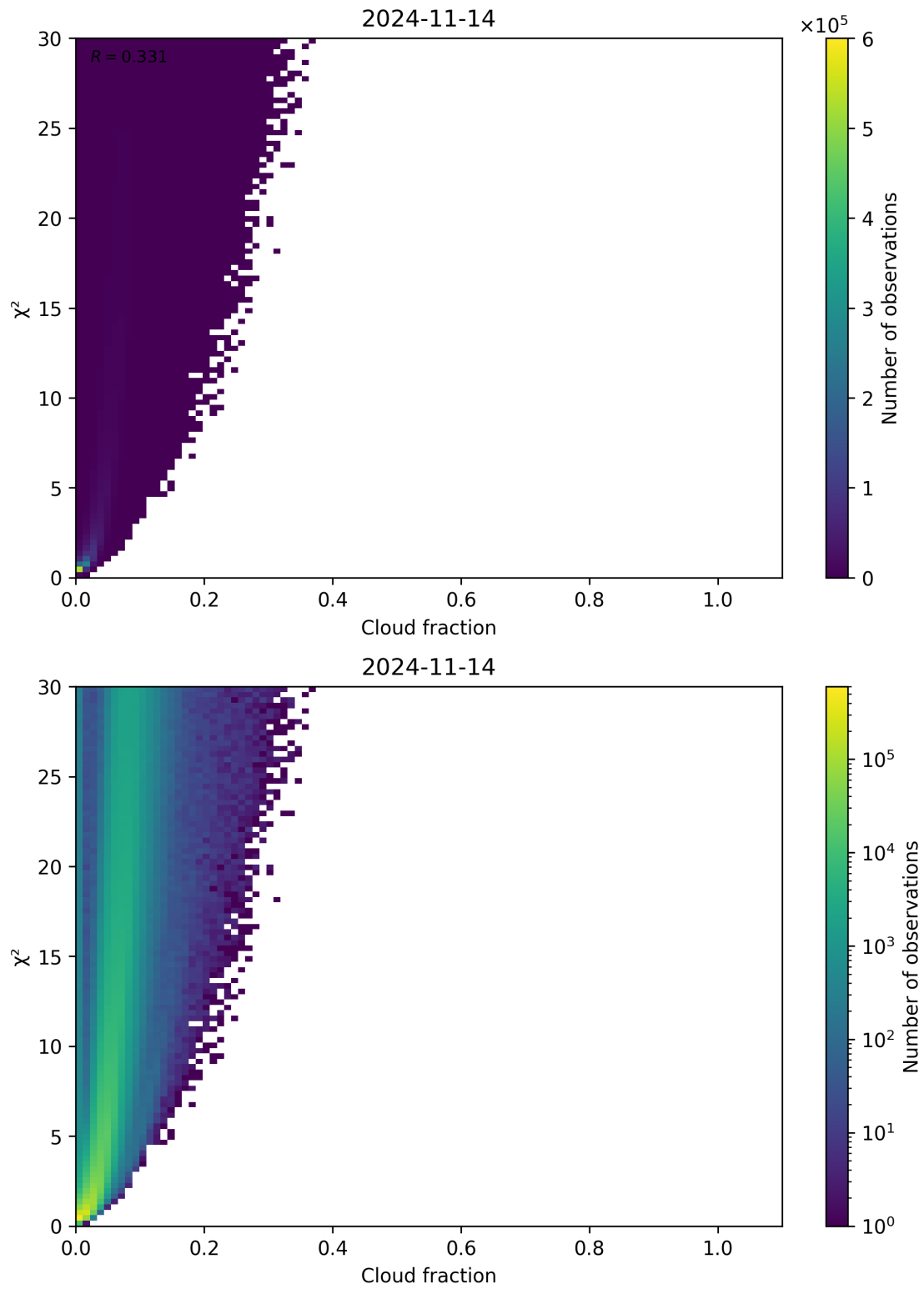
Figure 77: Scatter density plot of “Cloud fraction” against “ \chi^2 ” for 2024-11-14 to 2024-11-15.
