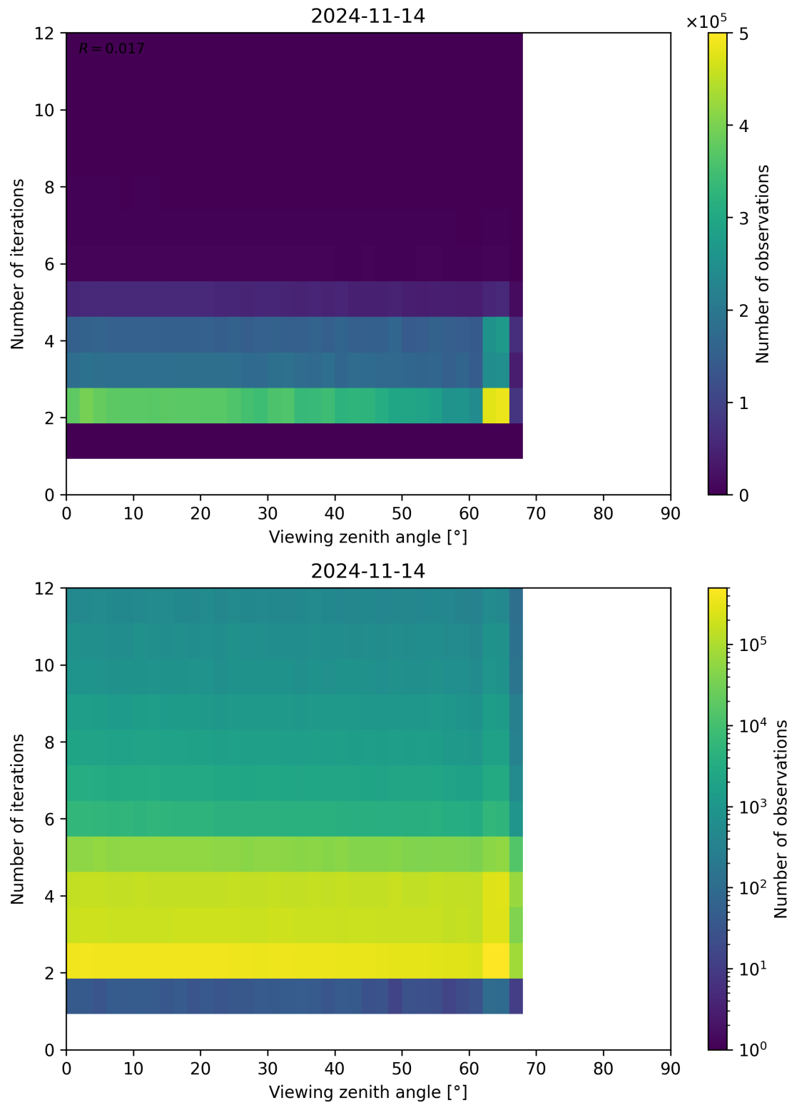
Figure 136: Scatter density plot of “Viewing zenith angle” against “Number of iterations” for 2024-11-14 to 2024-11-15.
