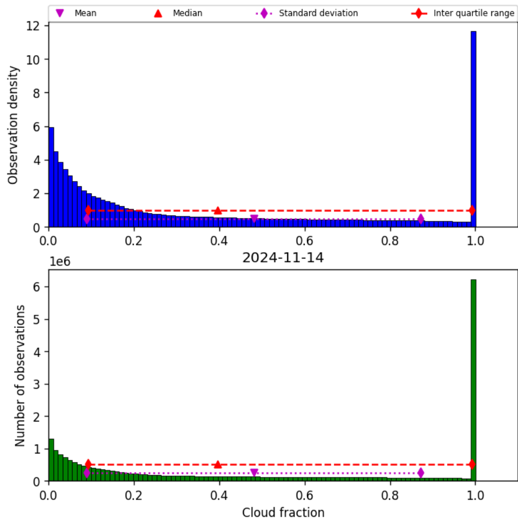
Figure 32: Histogram of “Cloud fraction” for 2024-11-14 to 2024-11-15
