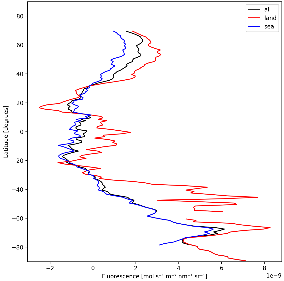
Figure 23: Zonal average of “Fluorescence” for 2024-11-14 to 2024-11-15.
