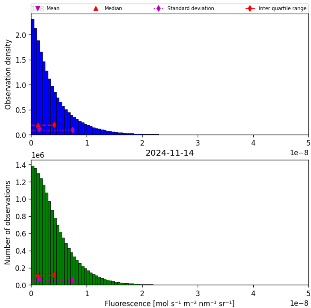
Figure 40: Histogram of “Fluorescence” for 2024-11-14 to 2024-11-15
