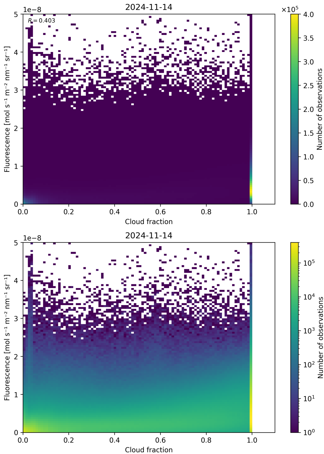
Figure 79: Scatter density plot of “Cloud fraction” against “Fluorescence” for 2024-11-14 to 2024-11-15.
