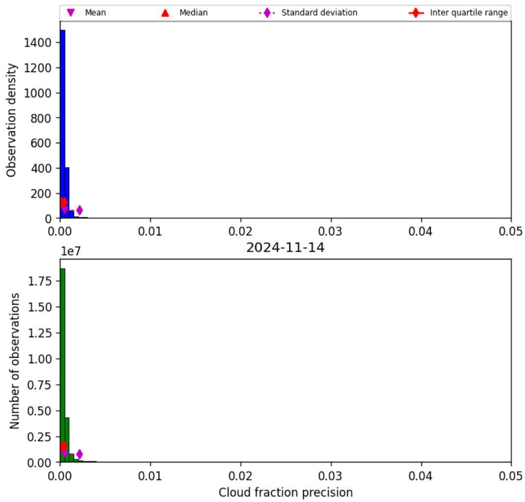
Figure 33: Histogram of “Cloud fraction precision” for 2024-11-14 to 2024-11-15
