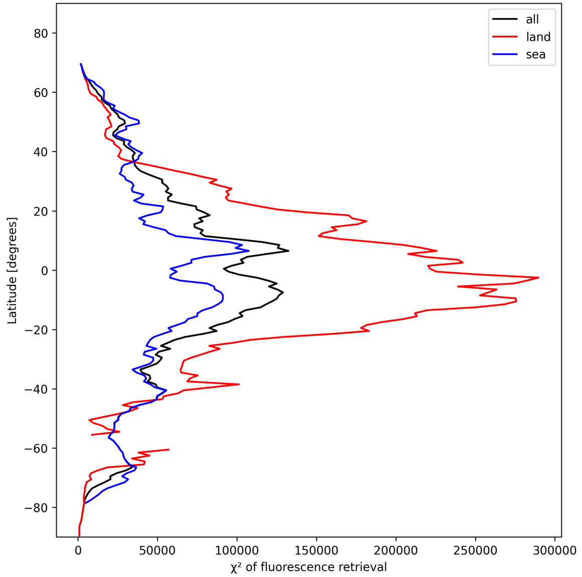
Figure 25: Zonal average of “ \chi^2 of fluorescence retrieval” for 2024-11-14 to 2024-11-15.
