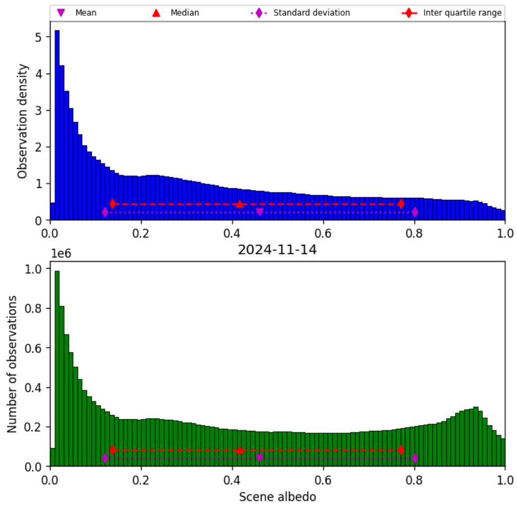
Figure 34: Histogram of “Scene albedo” for 2024-11-14 to 2024-11-15
