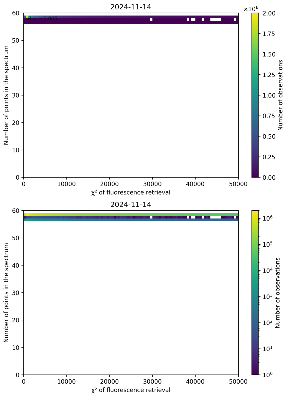
Figure 71: Scatter density plot of “ \chi^2 of fluorescence retrieval” against “Number of points in the spectrum” for 2024-11-14 to 2024-11-15.
