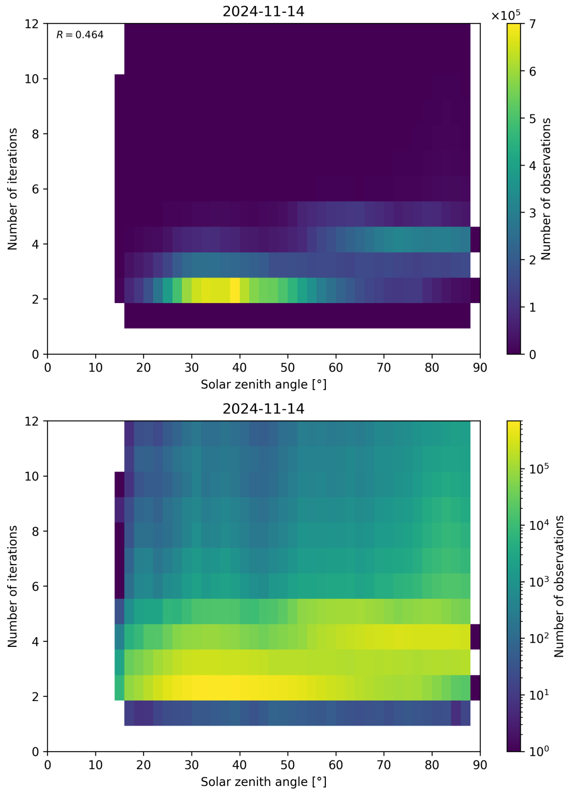
Figure 125: Scatter density plot of “Solar zenith angle” against “Number of iterations” for 2024-11-14 to 2024-11-15.
