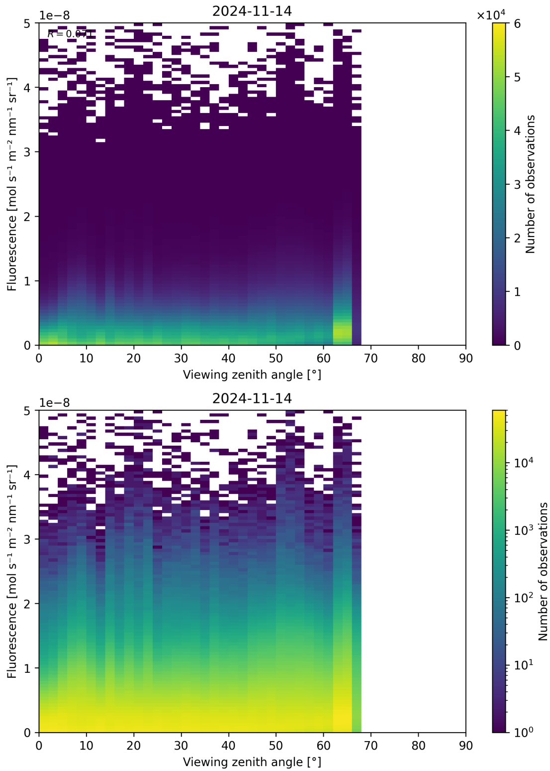
Figure 134: Scatter density plot of “Viewing zenith angle” against “Fluorescence” for 2024-11-14 to 2024-11-15.
