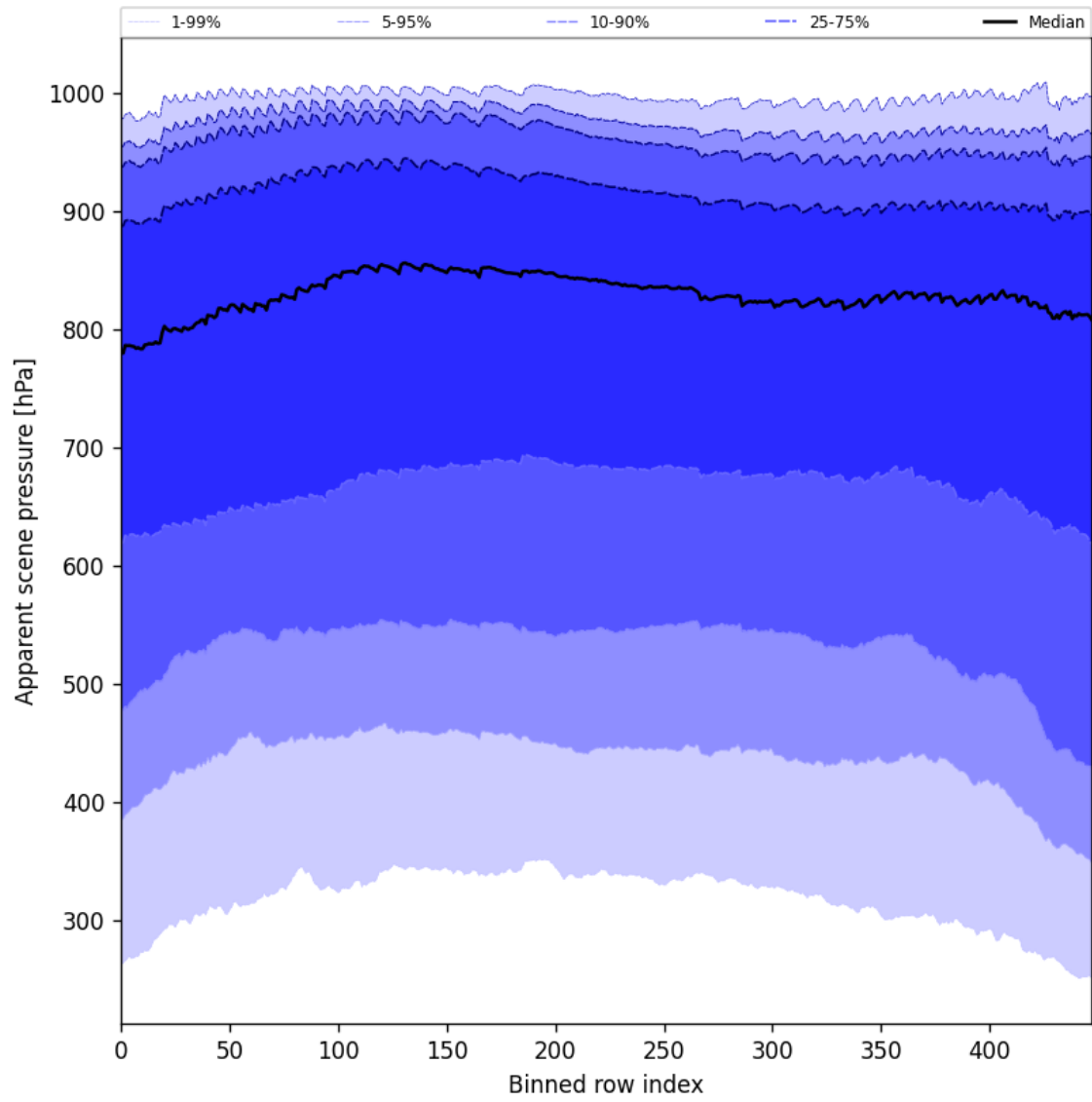
Figure 53: Along track statistics of “Apparent scene pressure” for 2024-11-14 to 2024-11-15
