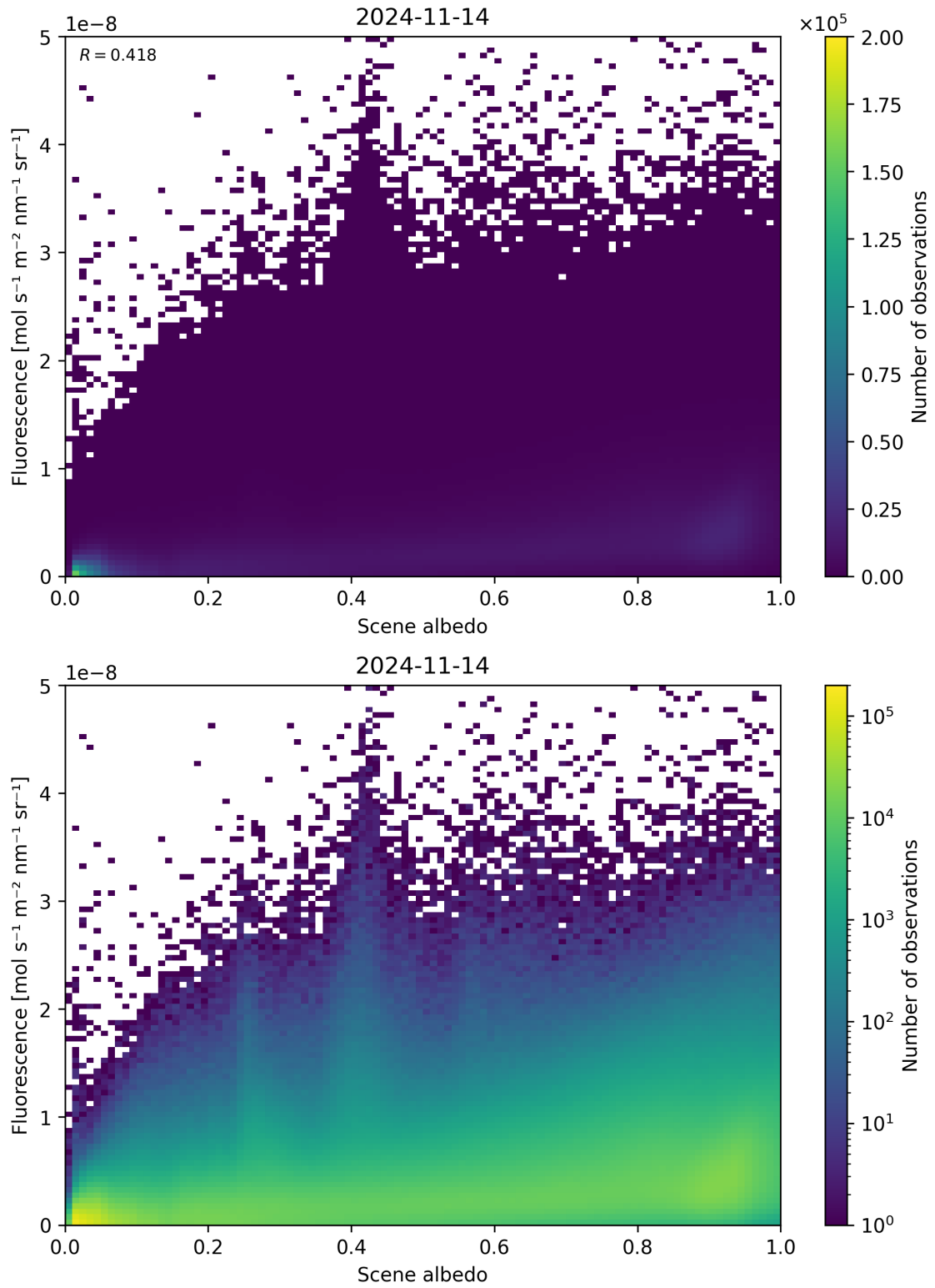
Figure 114: Scatter density plot of “Scene albedo” against “Fluorescence” for 2024-11-14 to 2024-11-15.
