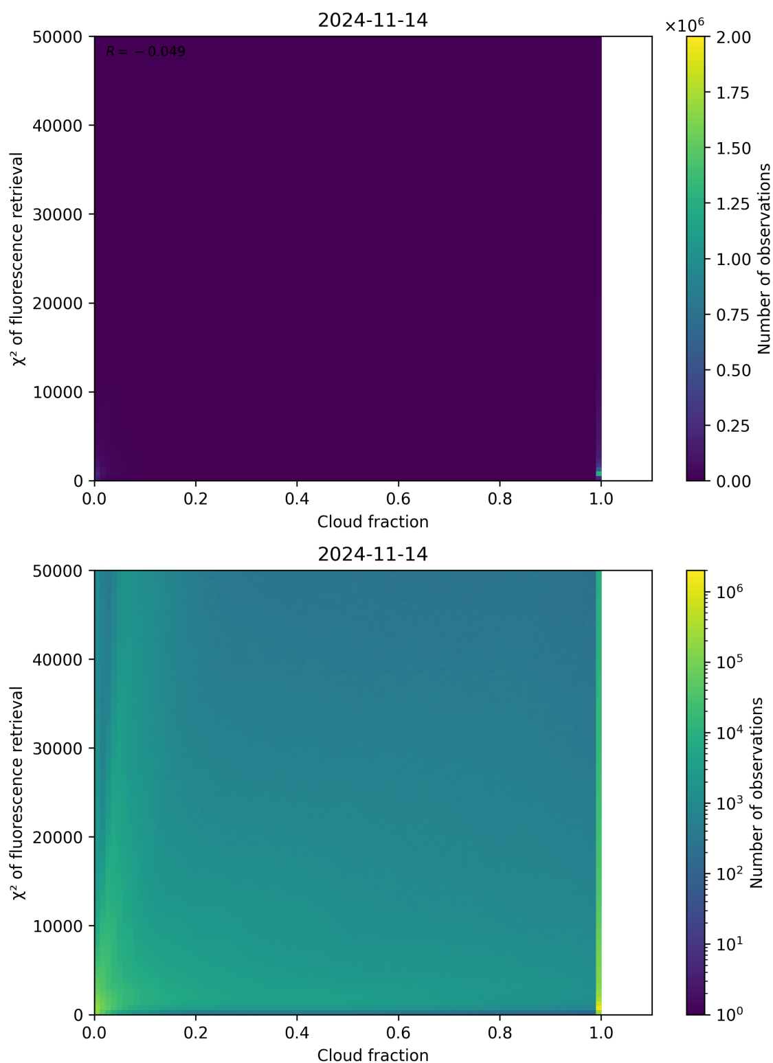
Figure 78: Scatter density plot of “Cloud fraction” against “ \chi^2 of fluorescence retrieval” for 2024-11-14 to 2024-11-15.
