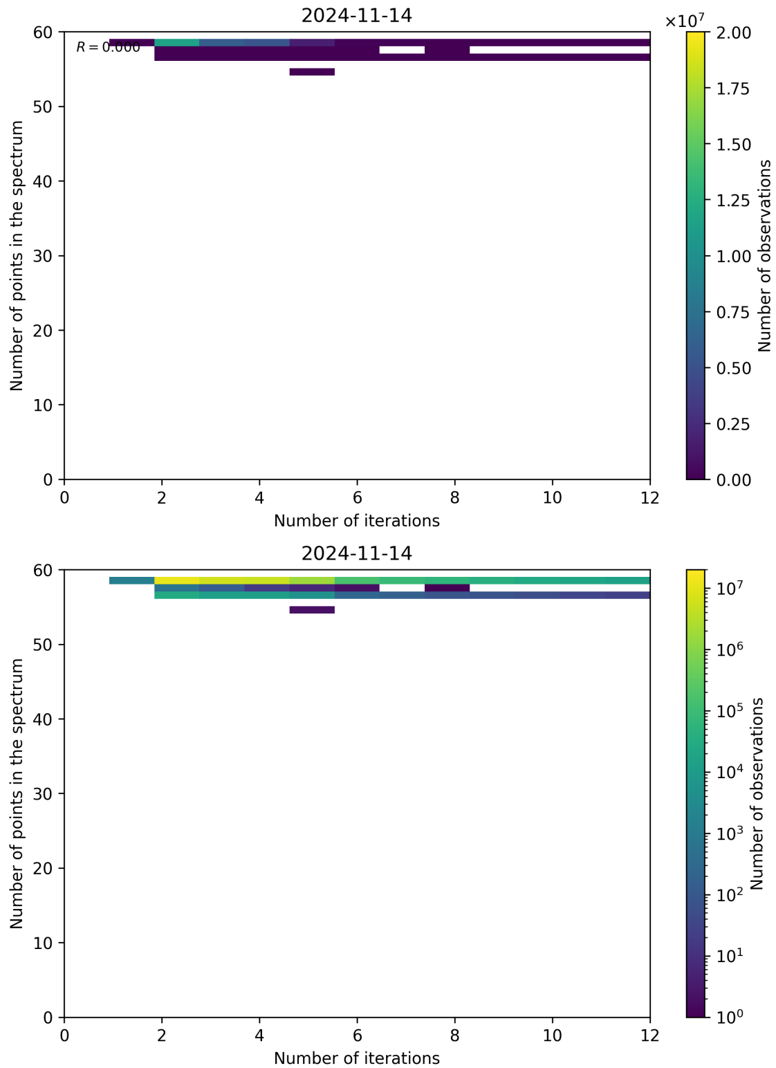
Figure 108: Scatter density plot of “Number of iterations” against “Number of points in the spectrum” for 2024-11-14 to 2024-11-15.
