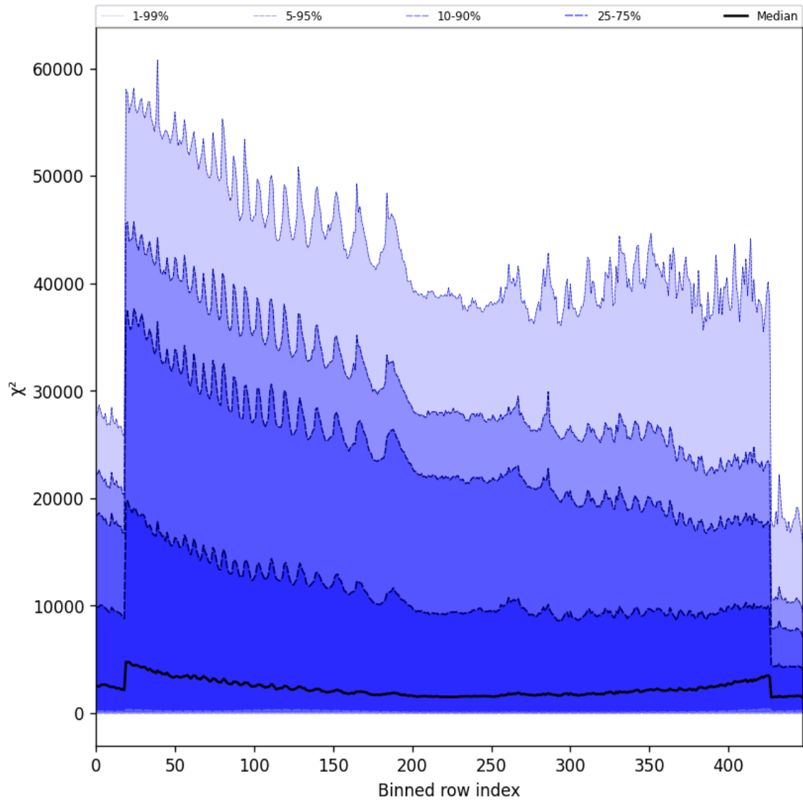
Figure 55: Along track statistics of “ \chi^2 ” for 2024-11-14 to 2024-11-15
