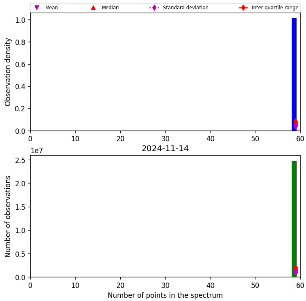
Figure 44: Histogram of “Number of points in the spectrum” for 2024-11-14 to 2024-11-15
