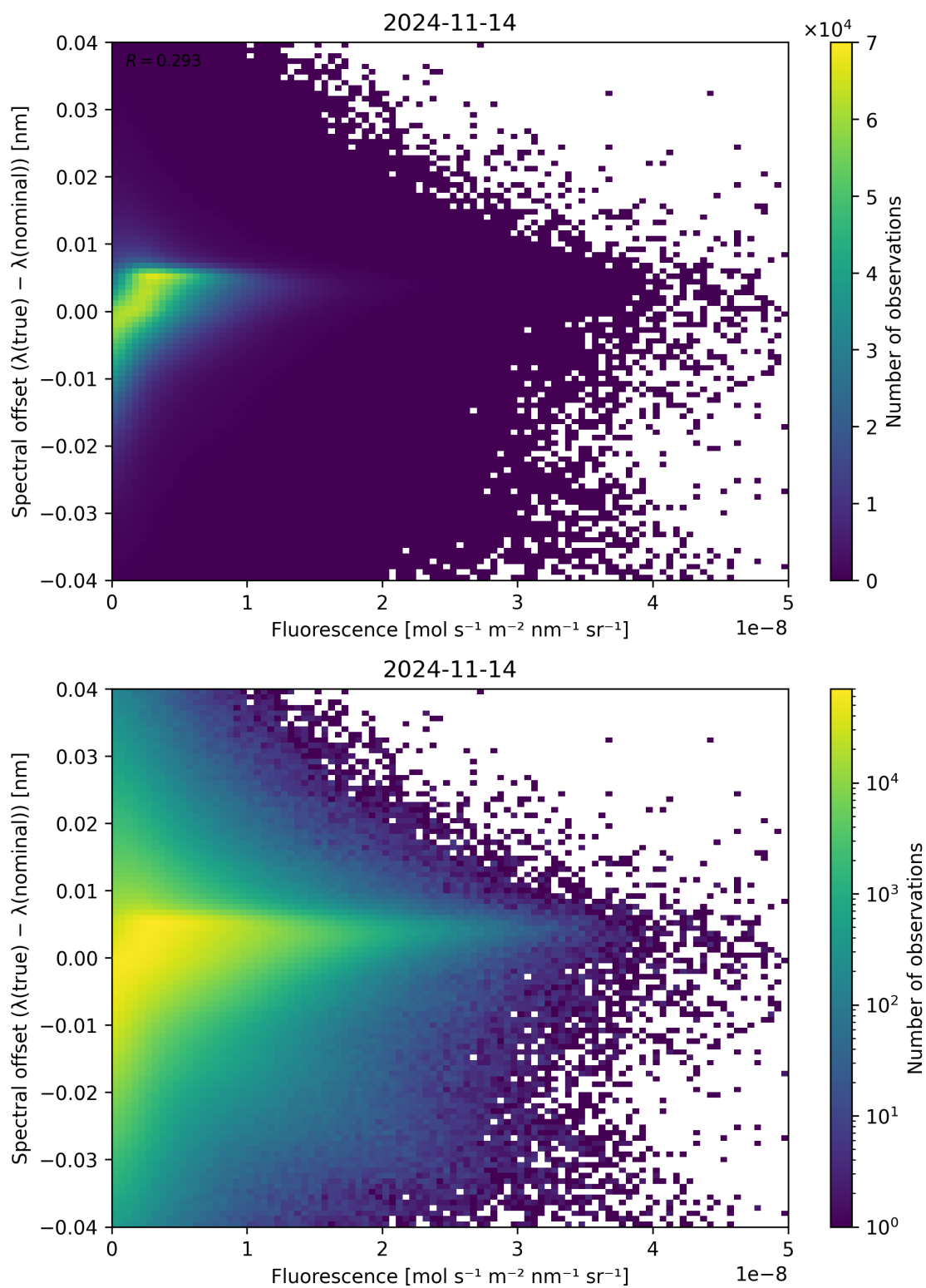
Figure 95: Scatter density plot of “Fluorescence” against “Spectral offset ( \lambda_{\text{true}} - \lambda_{\text{nominal}} )” for 2024-11-14 to 2024-11-15.
