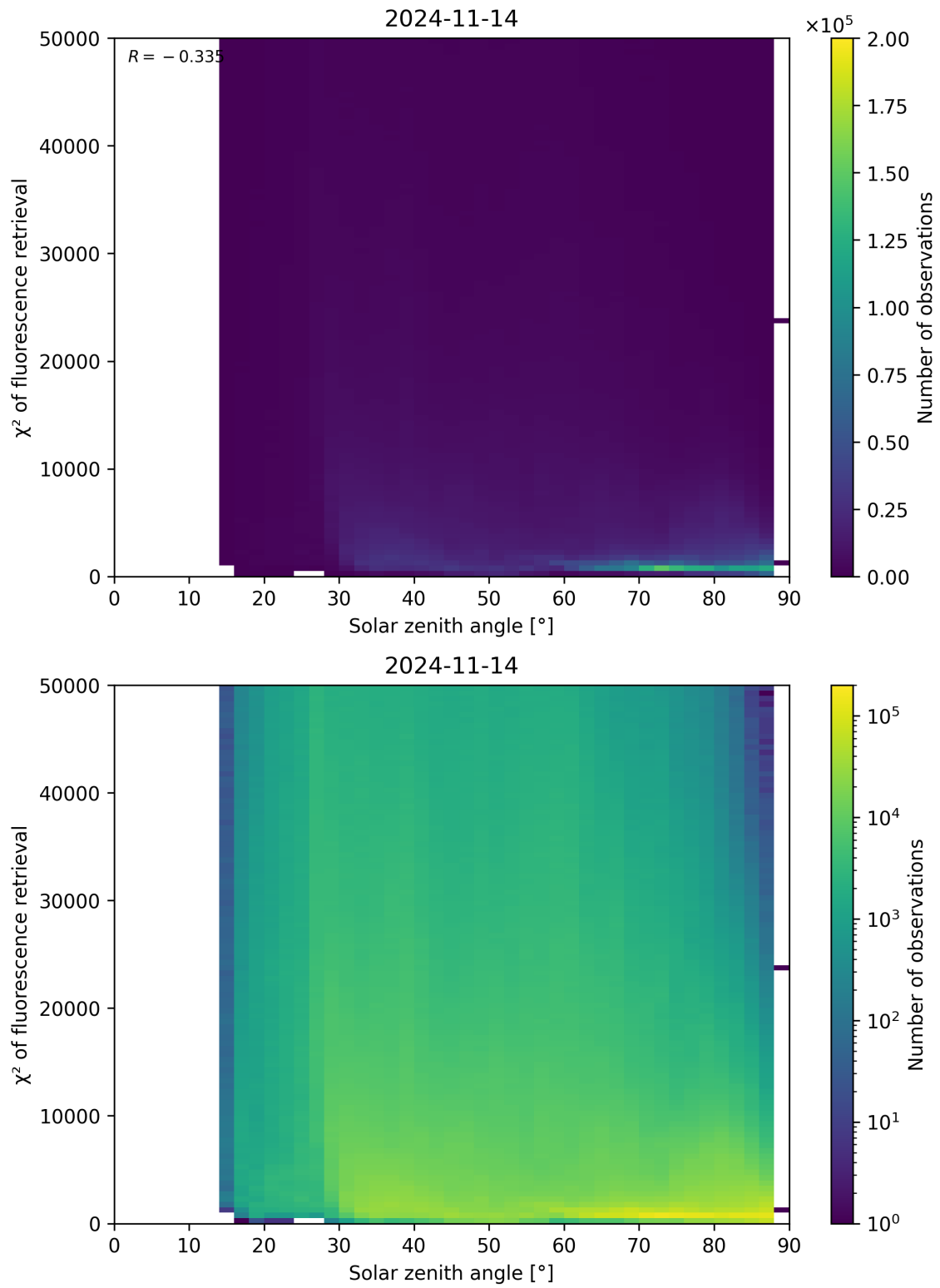
Figure 120: Scatter density plot of “Solar zenith angle” against “ \chi^2 of fluorescence retrieval” for 2024-11-14 to 2024-11-15.
