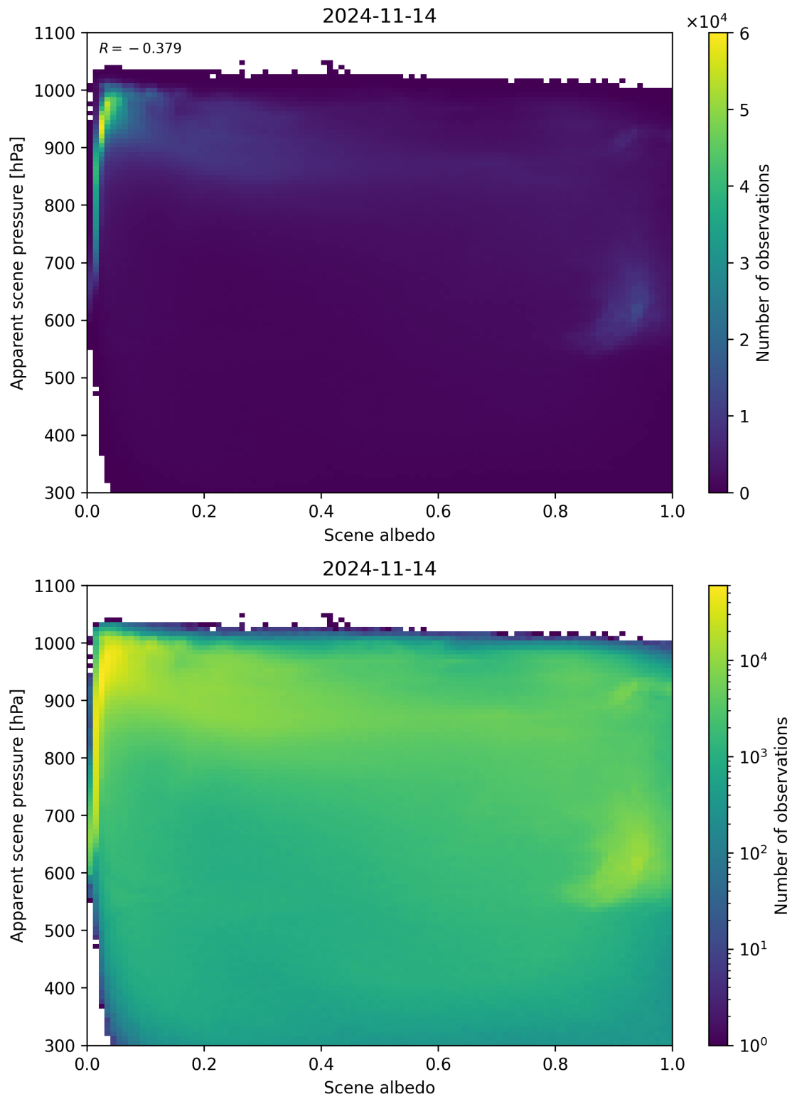
Figure 111: Scatter density plot of “Scene albedo” against “Apparent scene pressure” for 2024-11-14 to 2024-11-15.
