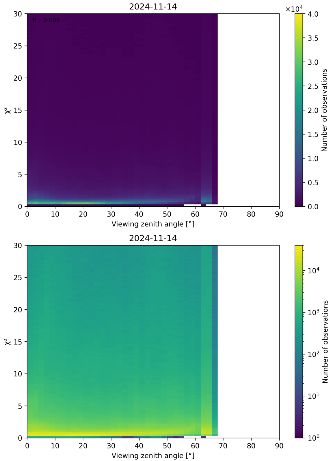
Figure 130: Scatter density plot of “Viewing zenith angle” against “ \chi^2 ” for 2024-11-14 to 2024-11-15.
