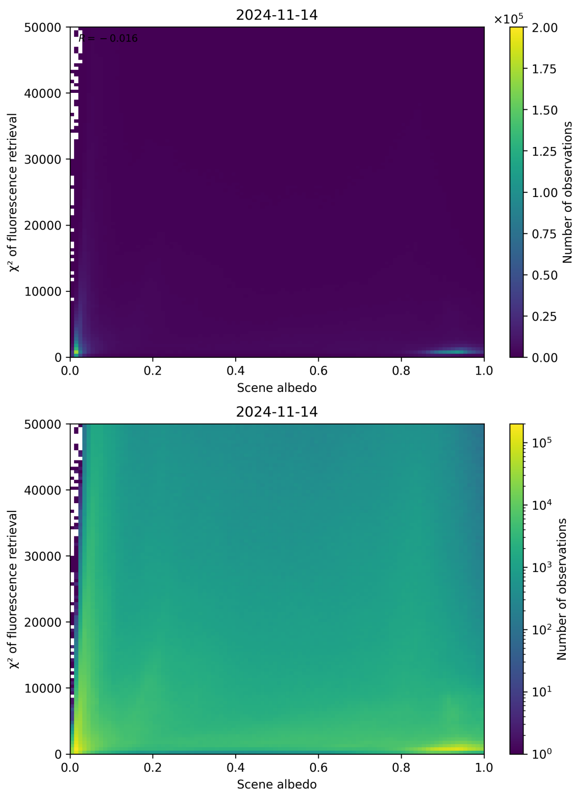
Figure 113: Scatter density plot of “Scene albedo” against “ \chi^2 of fluorescence retrieval” for 2024-11-14 to 2024-11-15.
