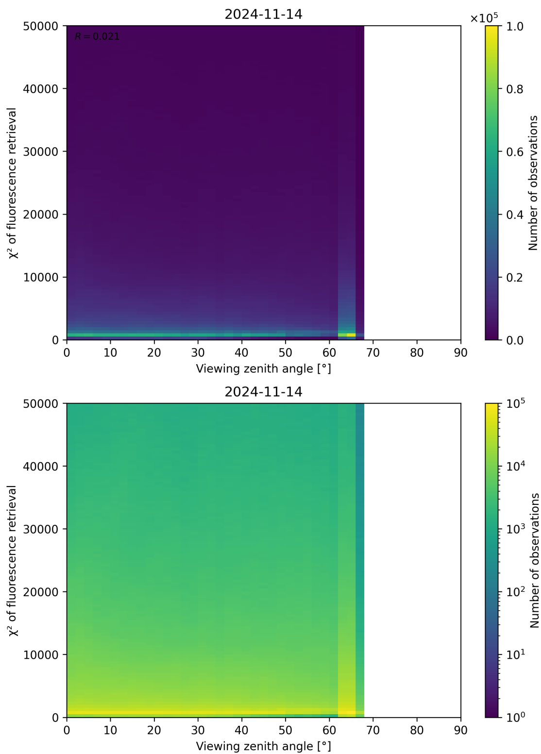
Figure 131: Scatter density plot of “Viewing zenith angle” against “ \chi^2 of fluorescence retrieval” for 2024-11-14 to 2024-11-15.
