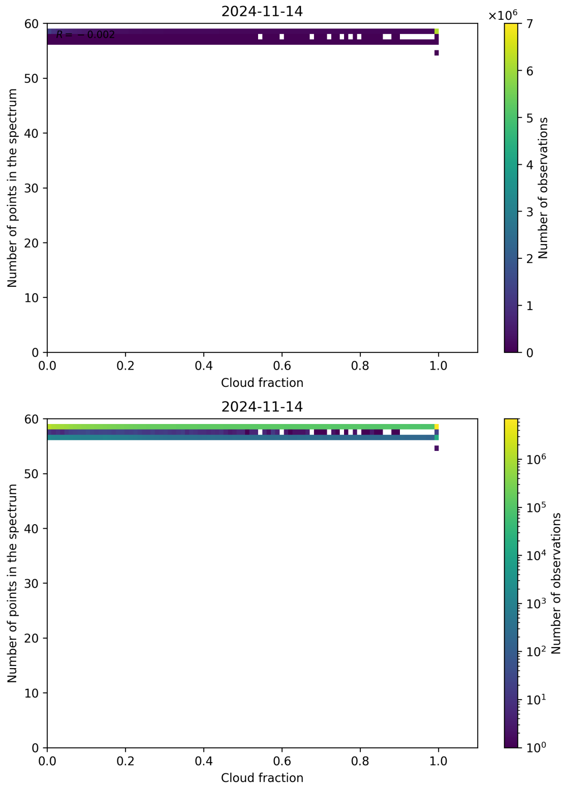
Figure 81: Scatter density plot of “Cloud fraction” against “Number of points in the spectrum” for 2024-11-14 to 2024-11-15.
