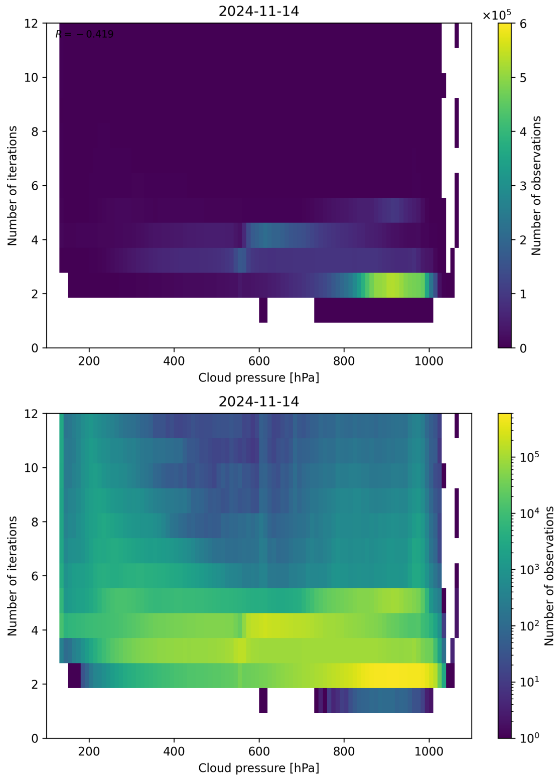
Figure 89: Scatter density plot of “Cloud pressure” against “Number of iterations” for 2024-11-14 to 2024-11-15.
