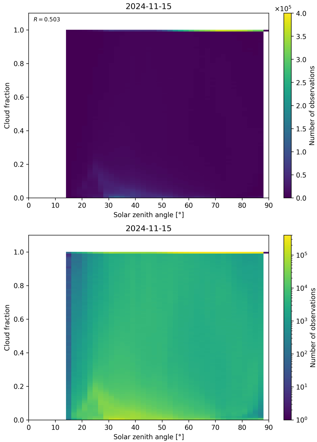
Figure 121: Scatter density plot of “Solar zenith angle” against “Cloud fraction” for 2024-11-14 to 2024-11-16.
