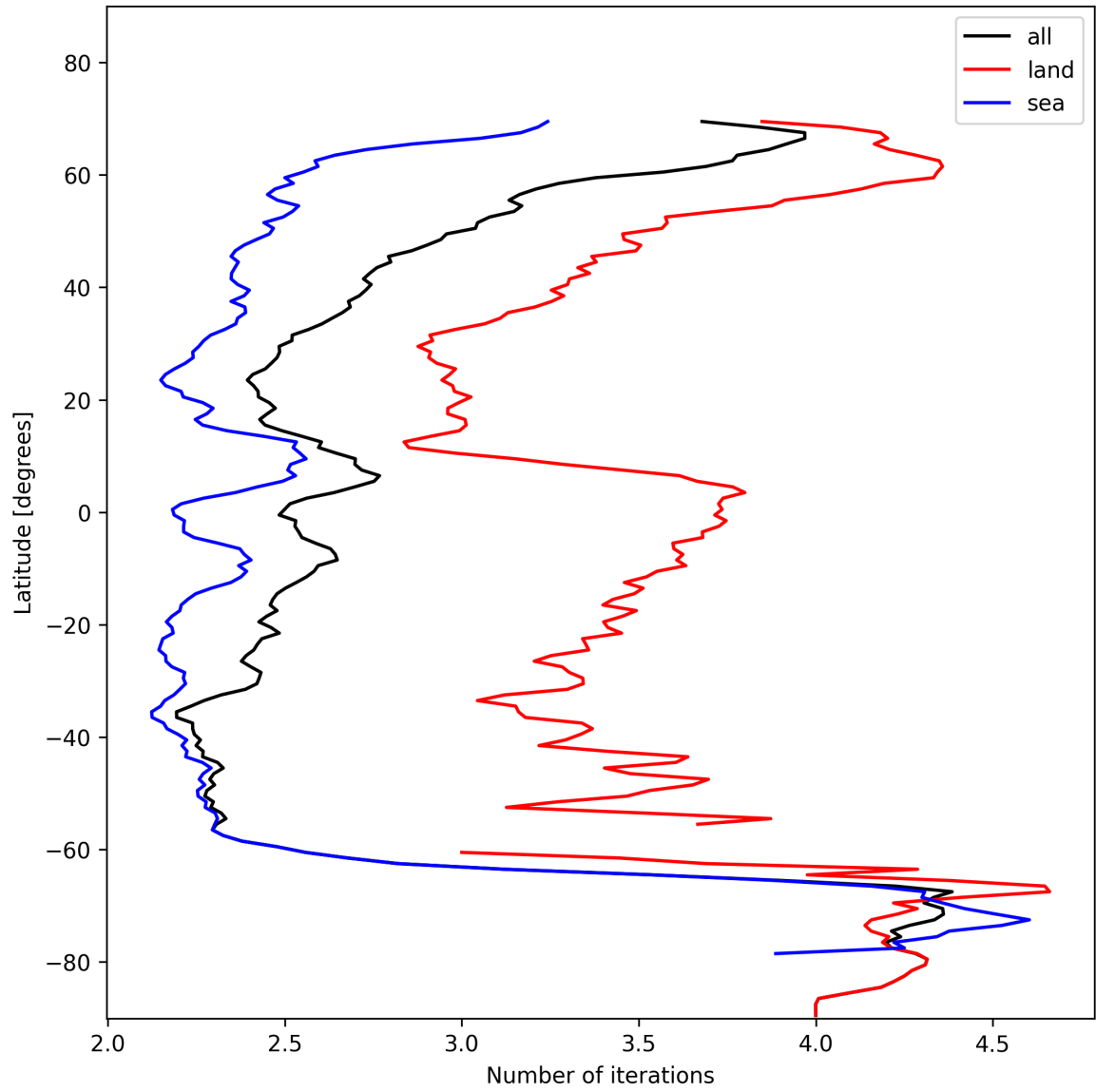
Figure 22: Zonal average of “Number of iterations” for 2024-11-14 to 2024-11-16.
