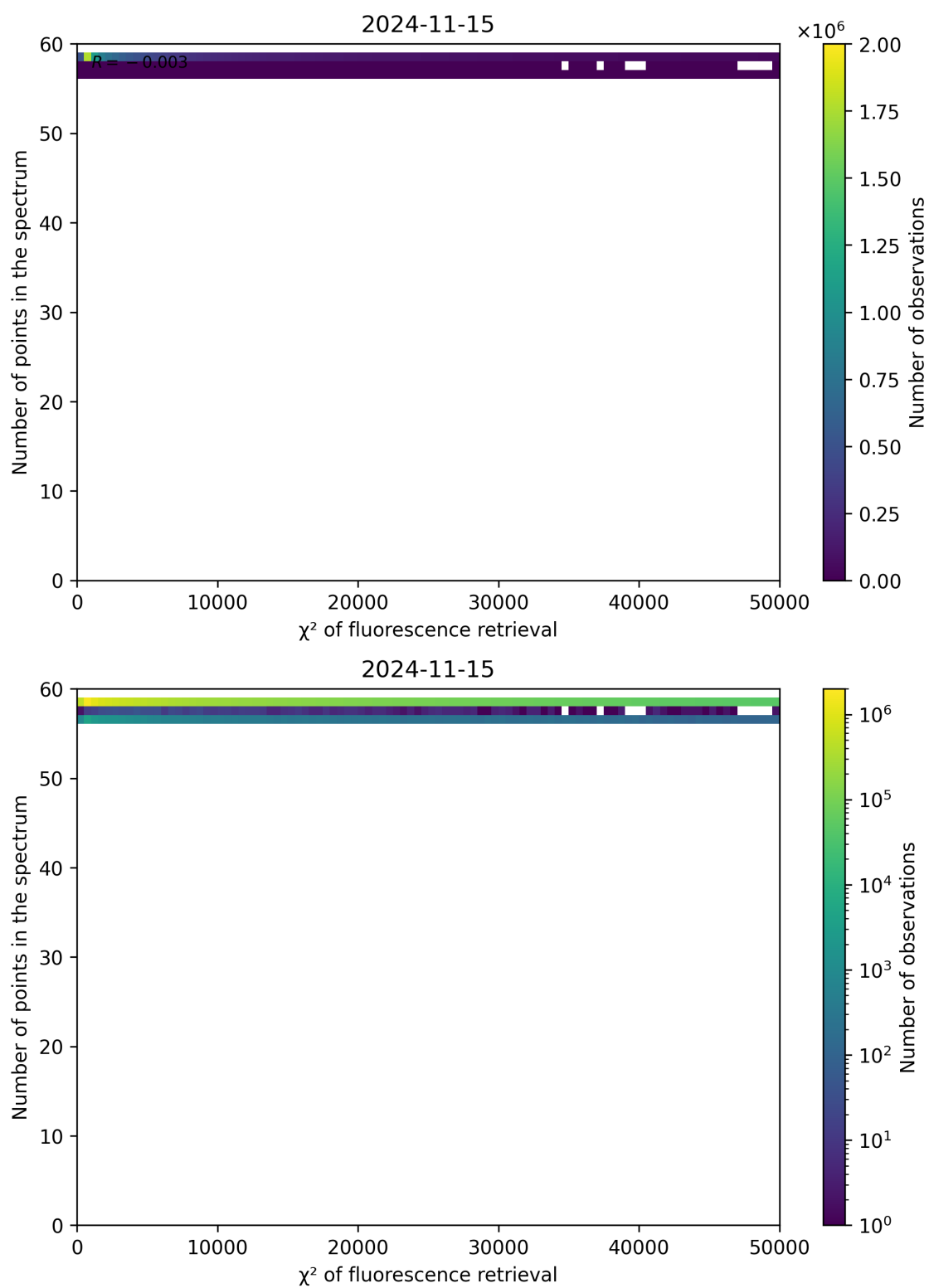
Figure 71: Scatter density plot of “ \chi^2 of fluorescence retrieval” against “Number of points in the spectrum” for 2024-11-14 to 2024-11-16.
