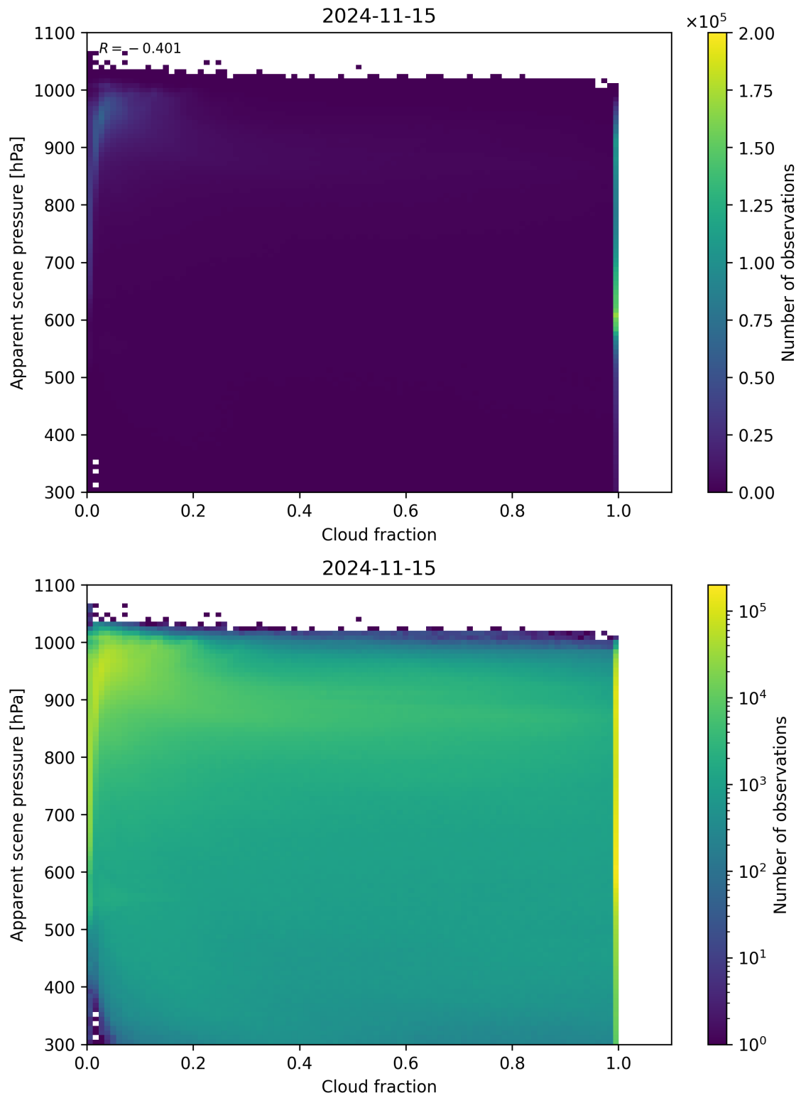
Figure 76: Scatter density plot of “Cloud fraction” against “Apparent scene pressure” for 2024-11-14 to 2024-11-16.
