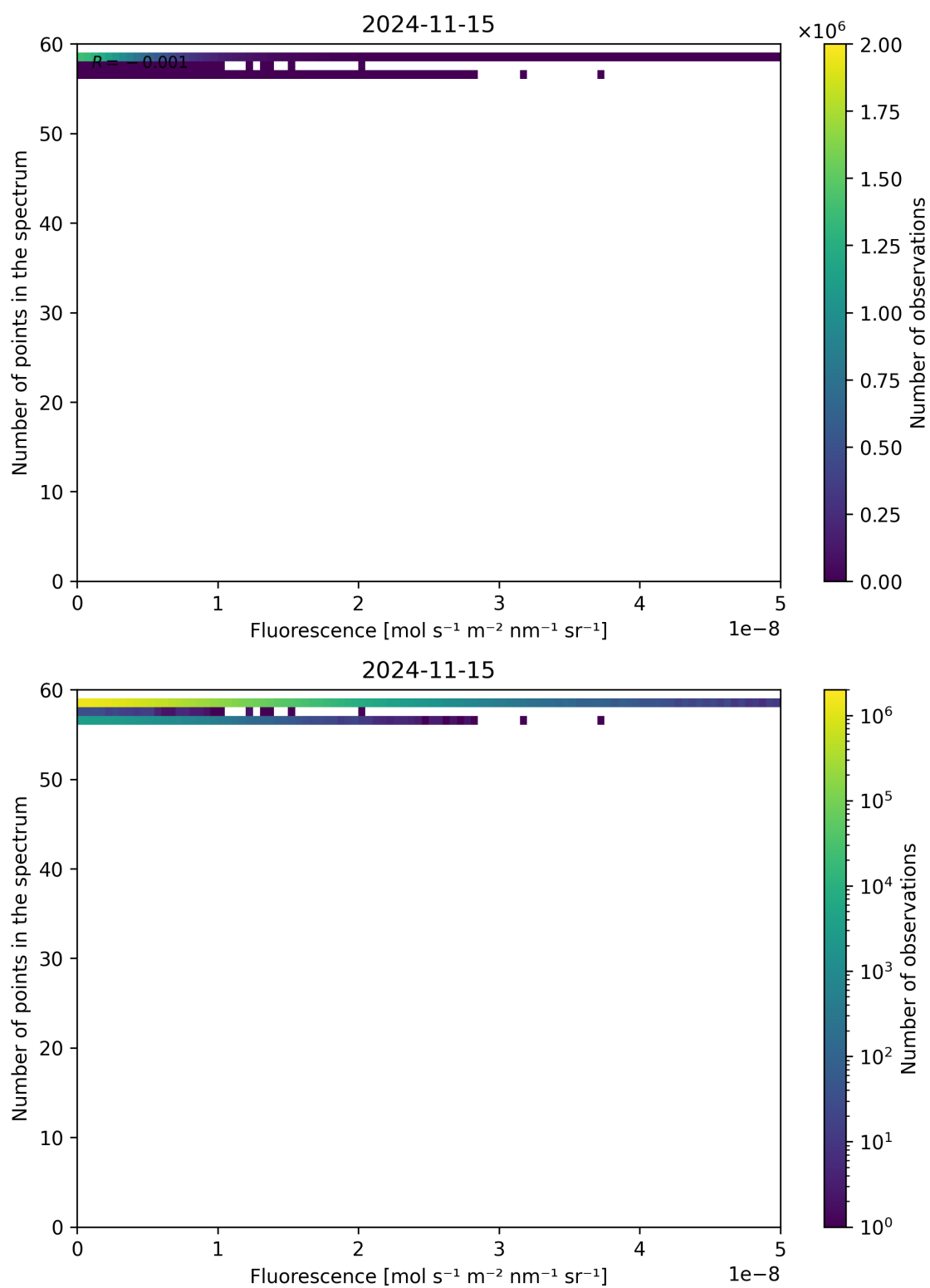
Figure 94: Scatter density plot of “Fluorescence” against “Number of points in the spectrum” for 2024-11-14 to 2024-11-16.
