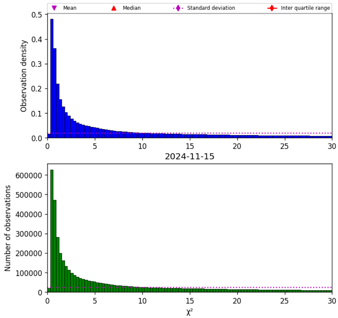
Figure 38: Histogram of " \chi^2 " for 2024-11-14 to 2024-11-16
