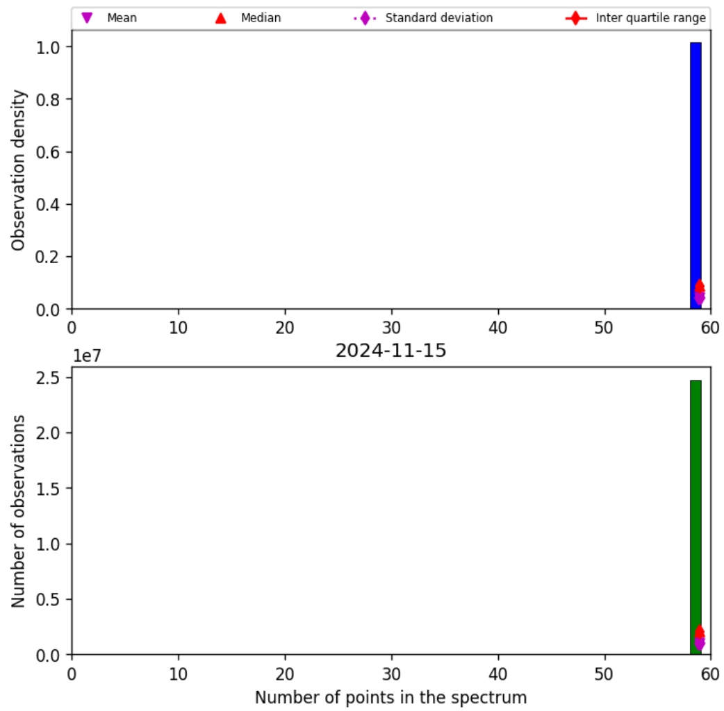
Figure 44: Histogram of “Number of points in the spectrum” for 2024-11-14 to 2024-11-16
