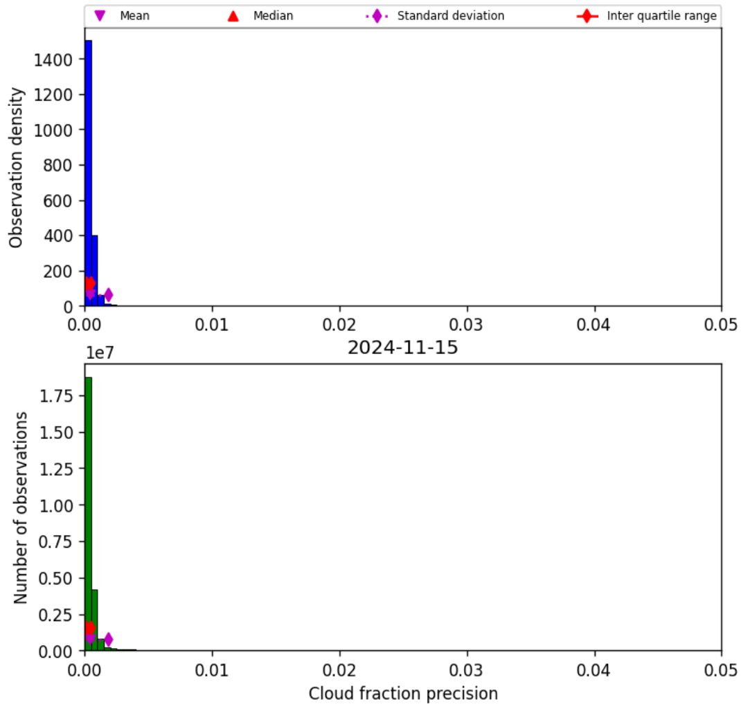
Figure 33: Histogram of “Cloud fraction precision” for 2024-11-14 to 2024-11-16
