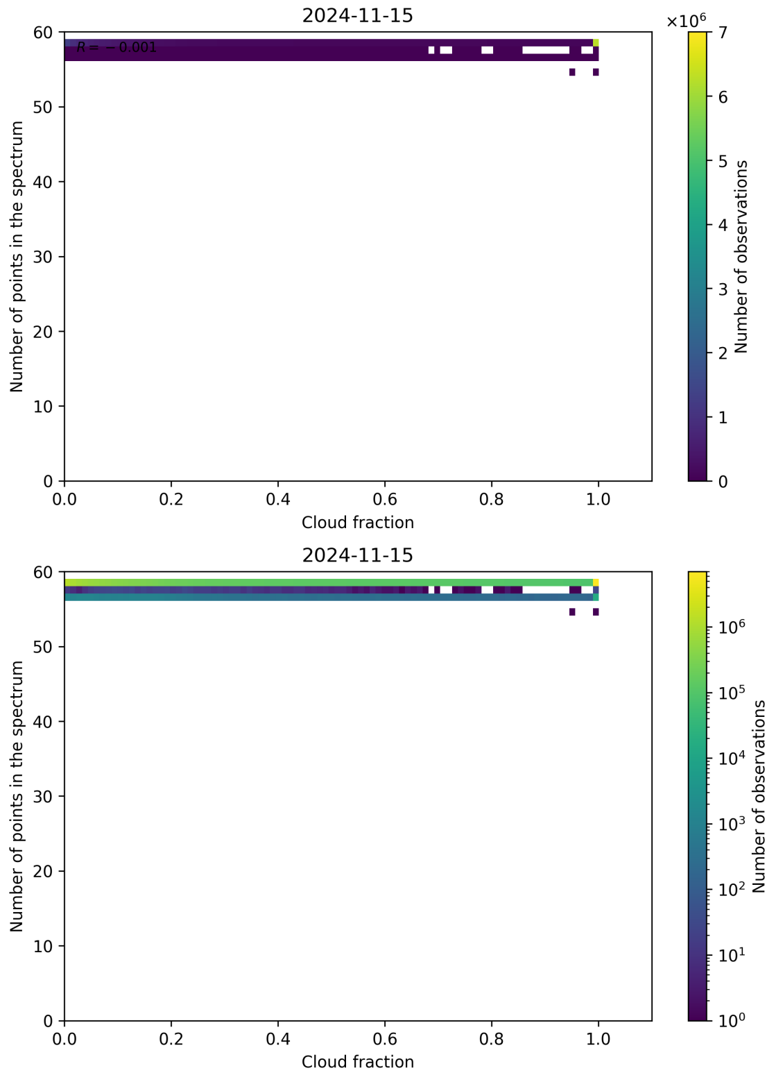
Figure 81: Scatter density plot of “Cloud fraction” against “Number of points in the spectrum” for 2024-11-14 to 2024-11-16.
