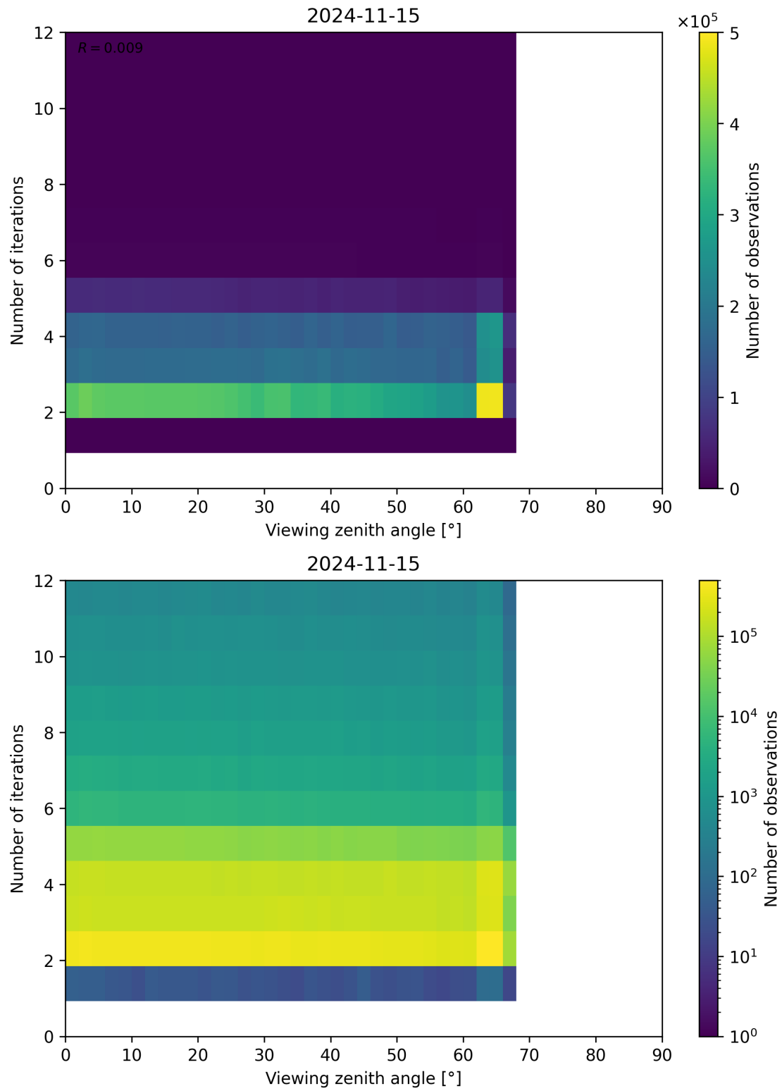
Figure 136: Scatter density plot of “Viewing zenith angle” against “Number of iterations” for 2024-11-14 to 2024-11-16.
