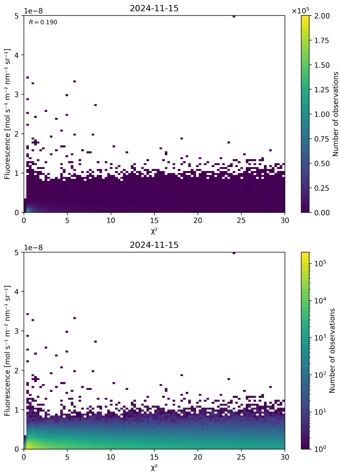
Figure 70: Scatter density plot of “ \chi^2 ” against “Fluorescence” for 2024-11-14 to 2024-11-16.
