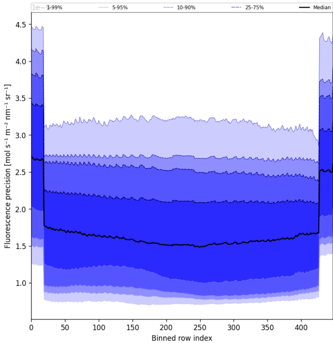
Figure 58: Along track statistics of “Fluorescence precision” for 2024-11-14 to 2024-11-16
