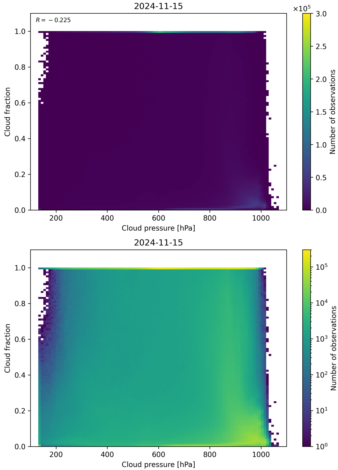
Figure 87: Scatter density plot of “Cloud pressure” against “Cloud fraction” for 2024-11-14 to 2024-11-16.
