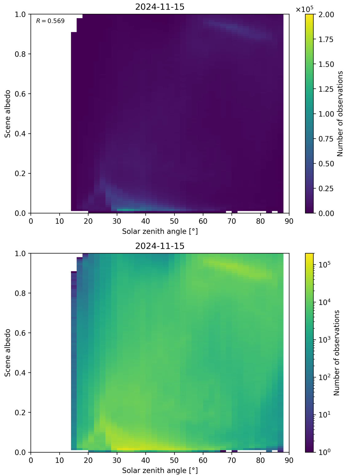
Figure 127: Scatter density plot of “Solar zenith angle” against “Scene albedo” for 2024-11-14 to 2024-11-16.
