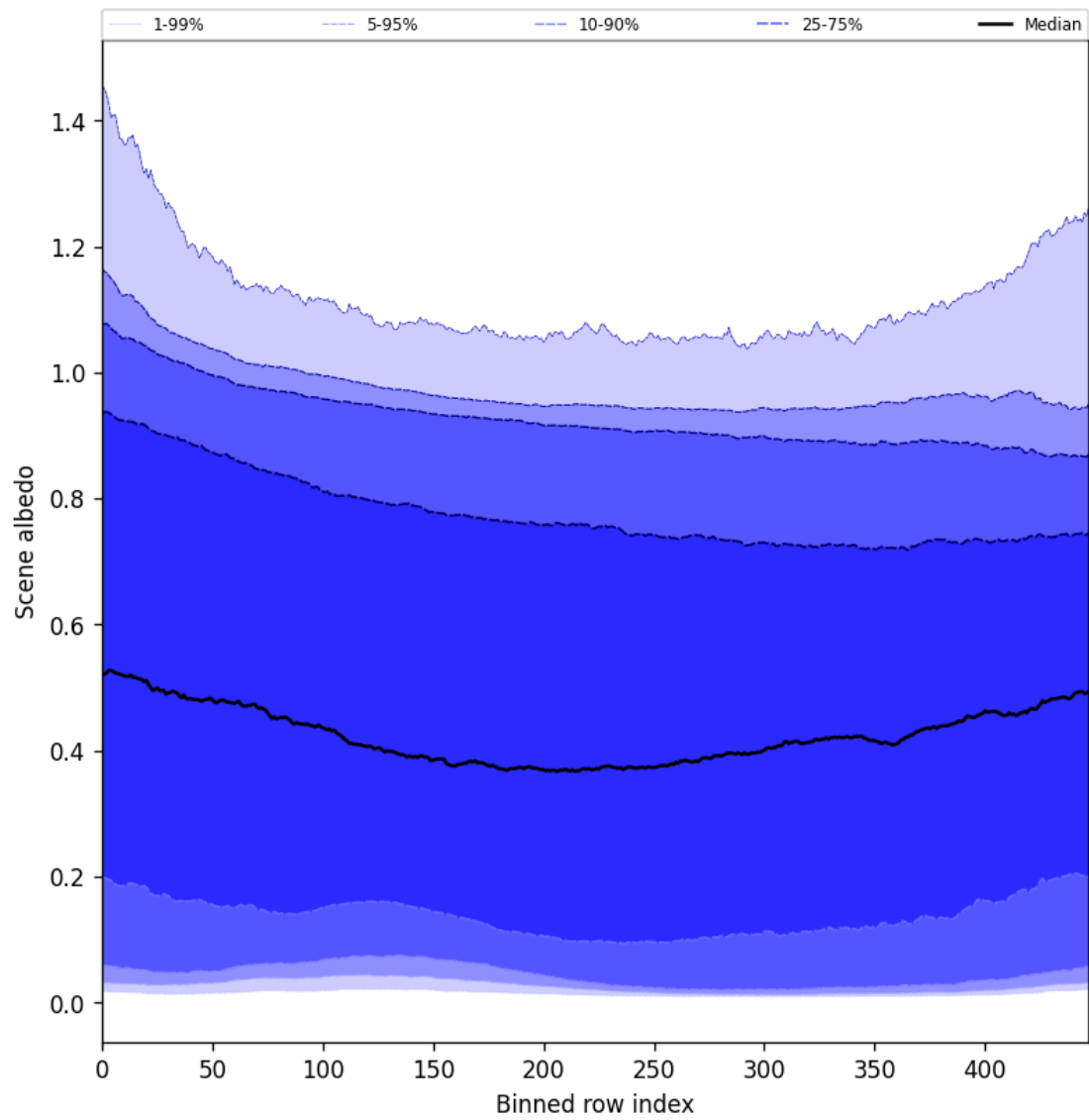
Figure 51: Along track statistics of “Scene albedo” for 2024-11-14 to 2024-11-16
