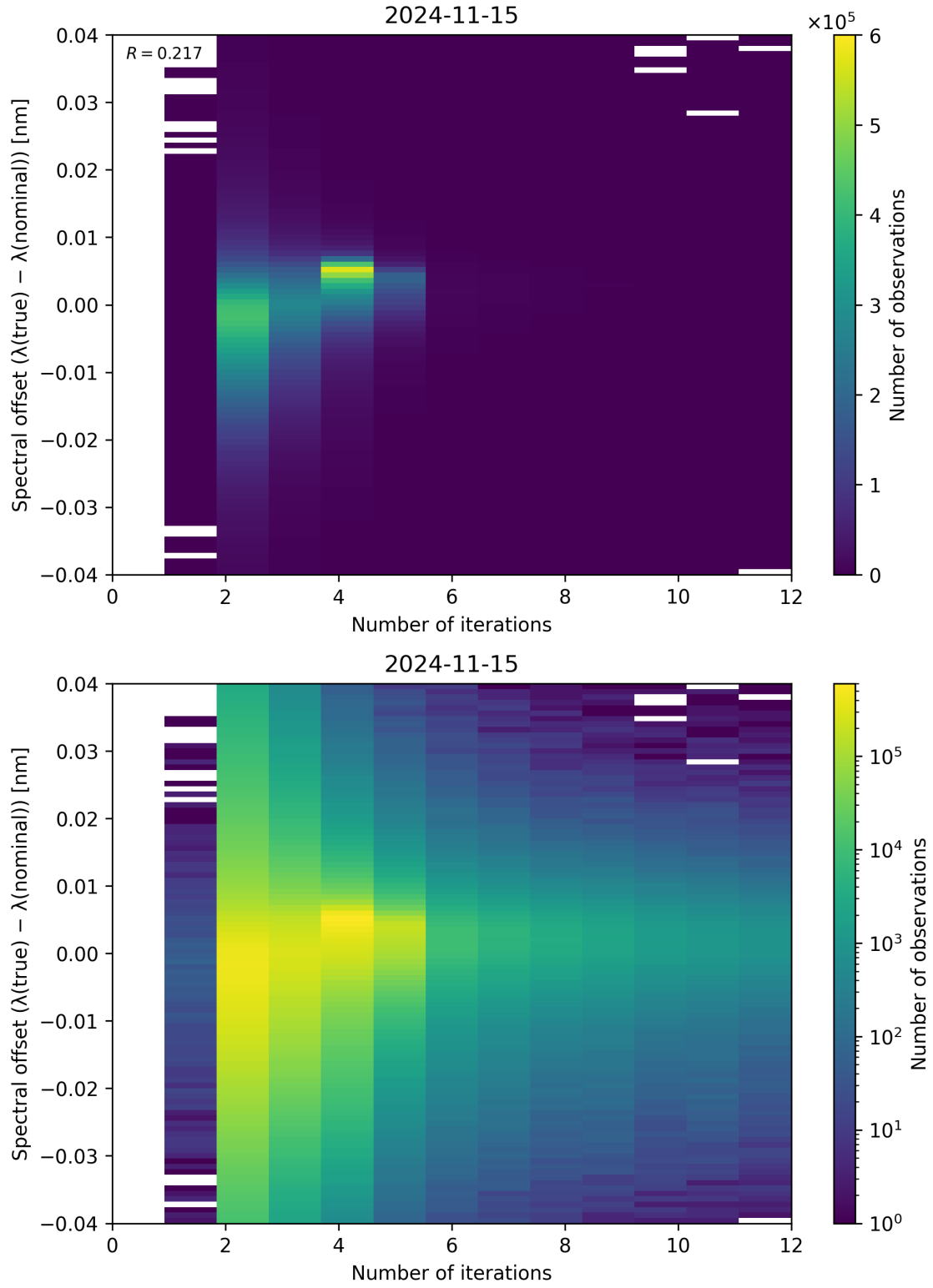
Figure 109: Scatter density plot of “Number of iterations” against “Spectral offset ( \lambda_{\text{true}} - \lambda_{\text{nominal}} )” for 2024-11-14 to 2024-11-16.
