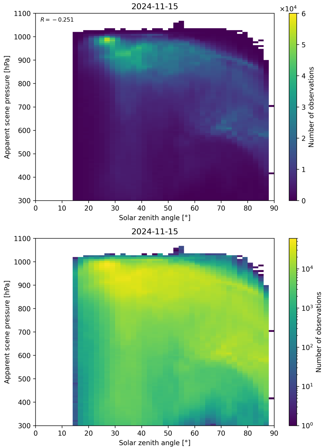
Figure 118: Scatter density plot of “Solar zenith angle” against “Apparent scene pressure” for 2024-11-14 to 2024-11-16.
