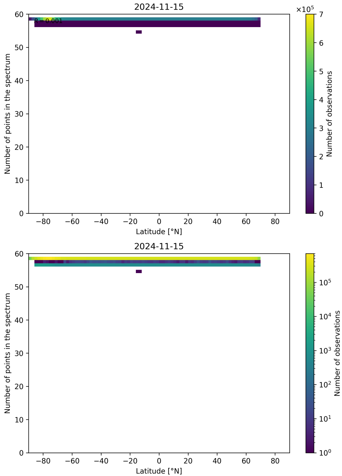
Figure 103: Scatter density plot of “Latitude” against “Number of points in the spectrum” for 2024-11-14 to 2024-11-16.
