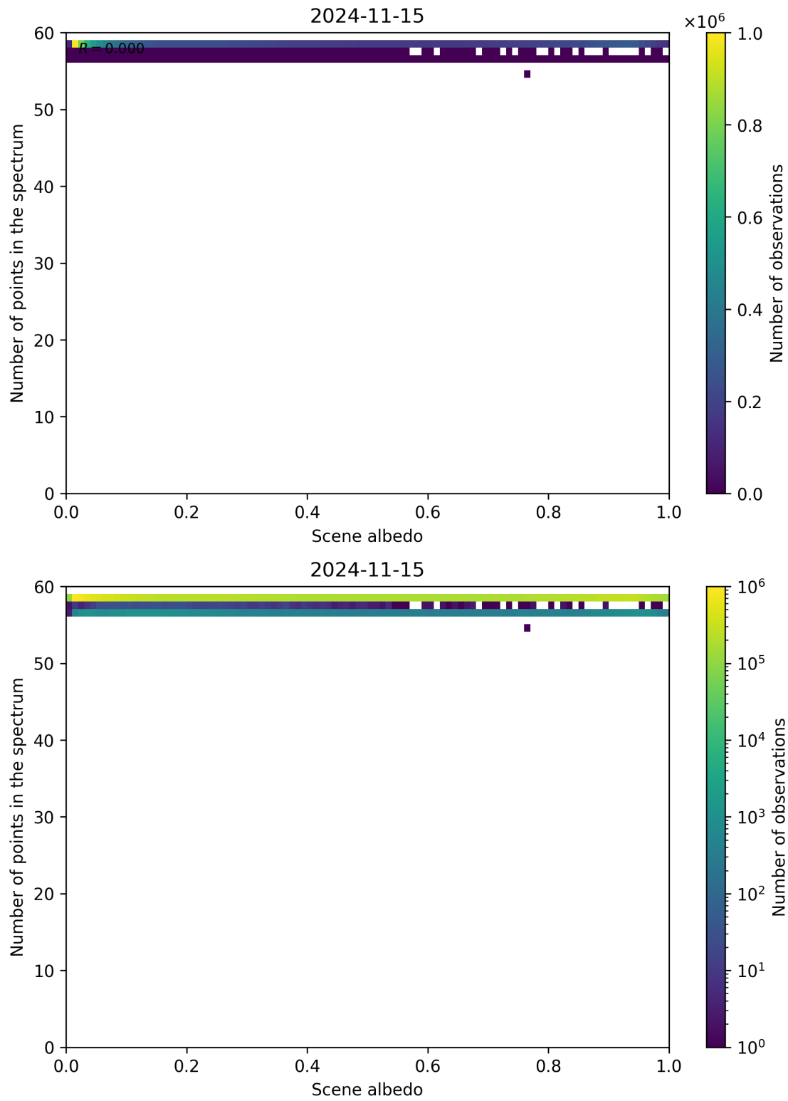
Figure 116: Scatter density plot of “Scene albedo” against “Number of points in the spectrum” for 2024-11-14 to 2024-11-16.
