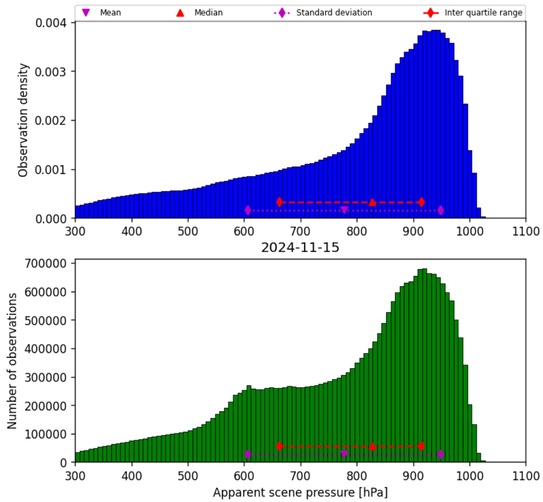
Figure 36: Histogram of “Apparent scene pressure” for 2024-11-14 to 2024-11-16
