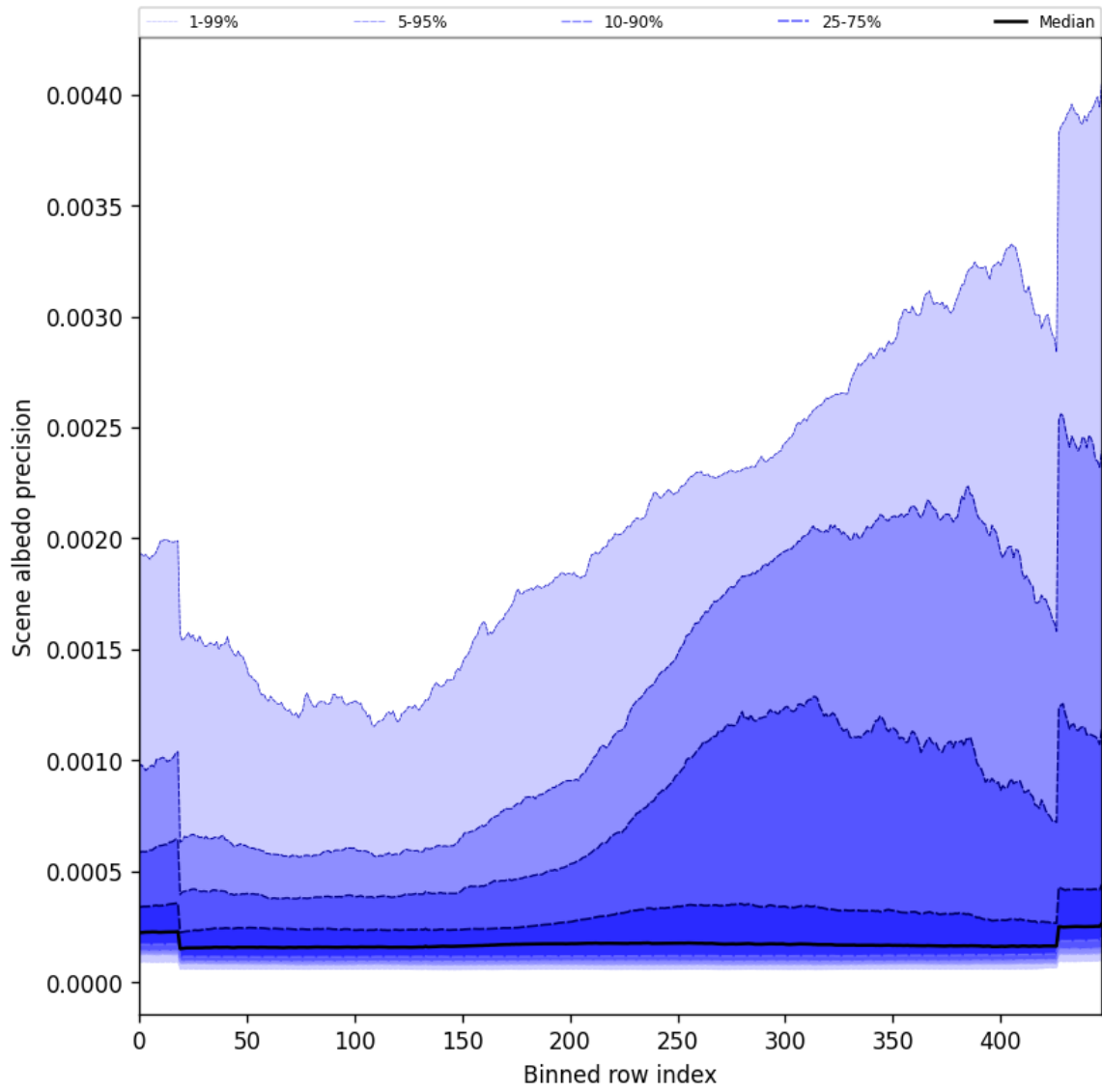
Figure 52: Along track statistics of “Scene albedo precision” for 2024-11-14 to 2024-11-16
