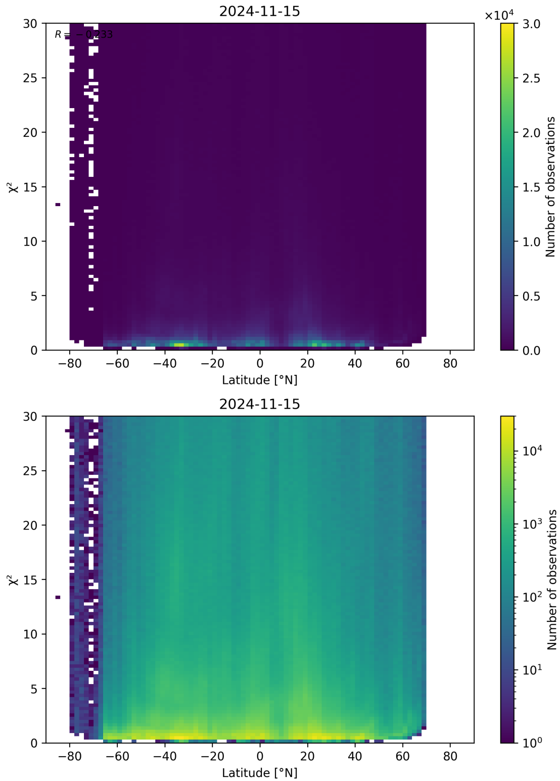
Figure 97: Scatter density plot of “Latitude” against “ \chi^2 ” for 2024-11-14 to 2024-11-16.
