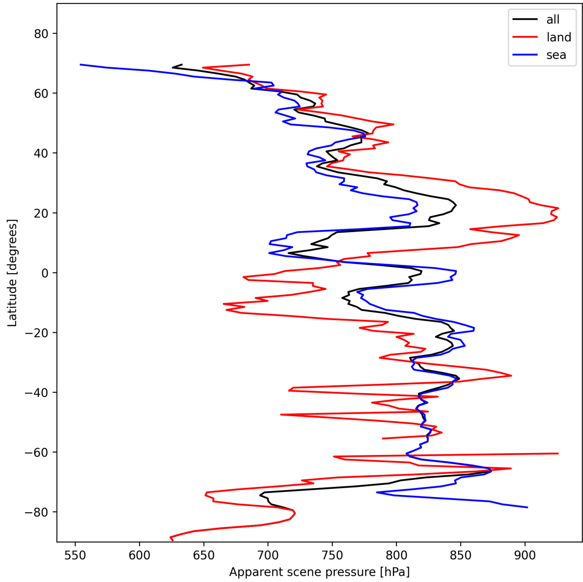
Figure 19: Zonal average of “Apparent scene pressure” for 2024-11-14 to 2024-11-16.
