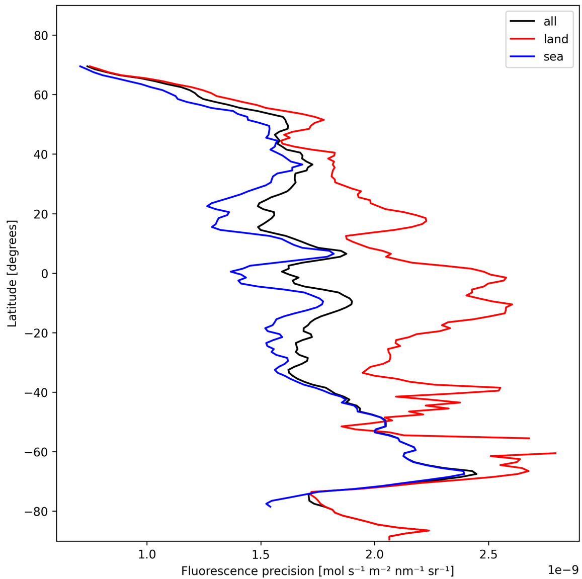
Figure 24: Zonal average of “Fluorescence precision” for 2024-11-14 to 2024-11-16.
