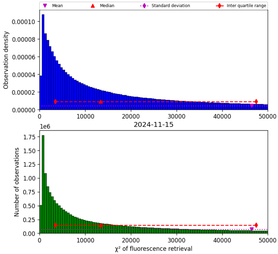
Figure 42: Histogram of “ \chi^2 of fluorescence retrieval” for 2024-11-14 to 2024-11-16
