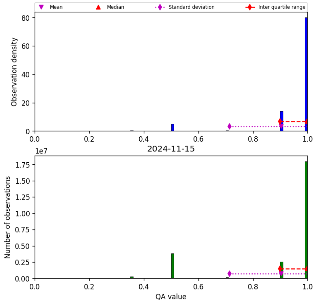
Figure 29: Histogram of “QA value” for 2024-11-14 to 2024-11-16
