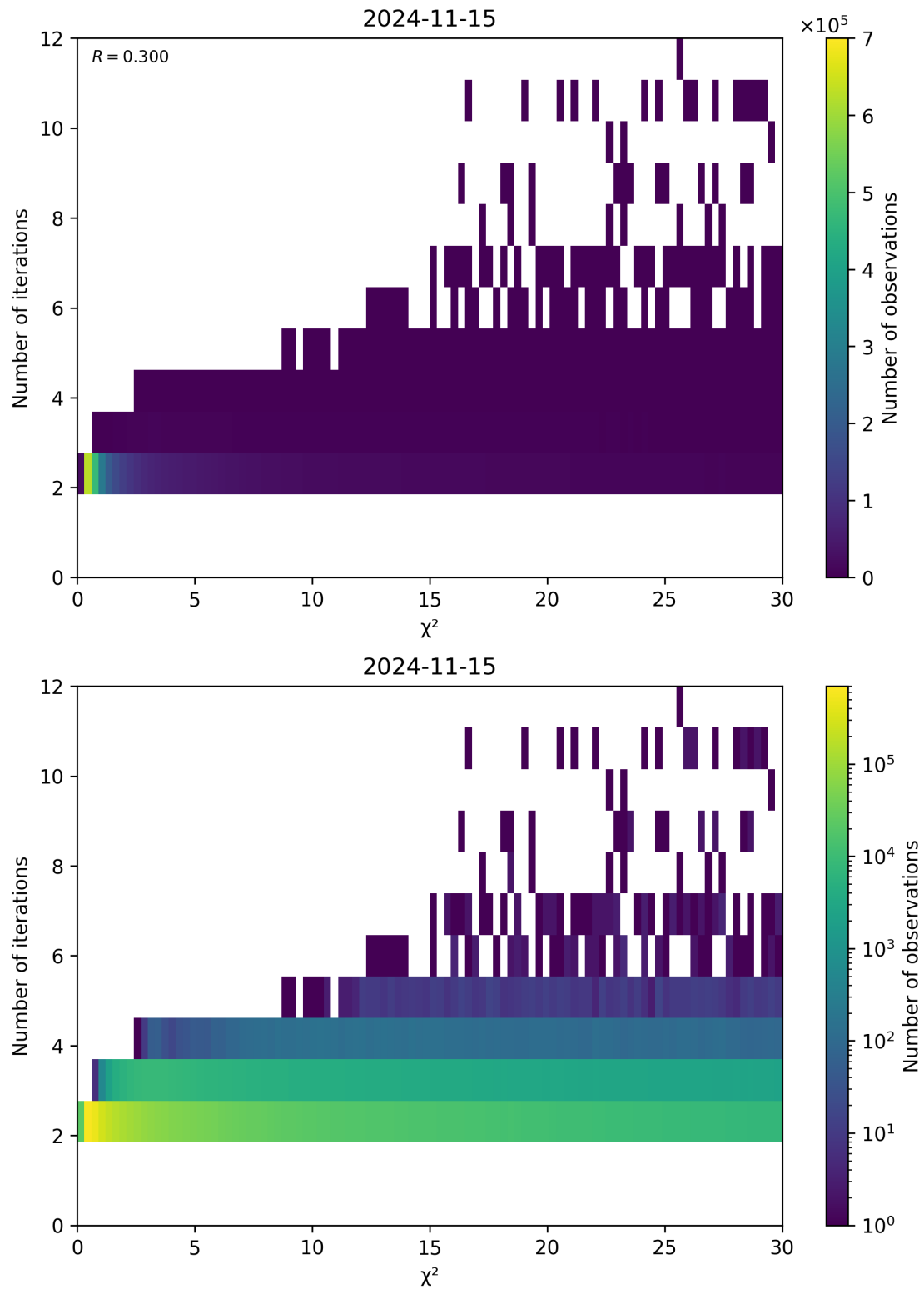
Figure 73: Scatter density plot of “ \chi^2 ” against “Number of iterations” for 2024-11-14 to 2024-11-16.
