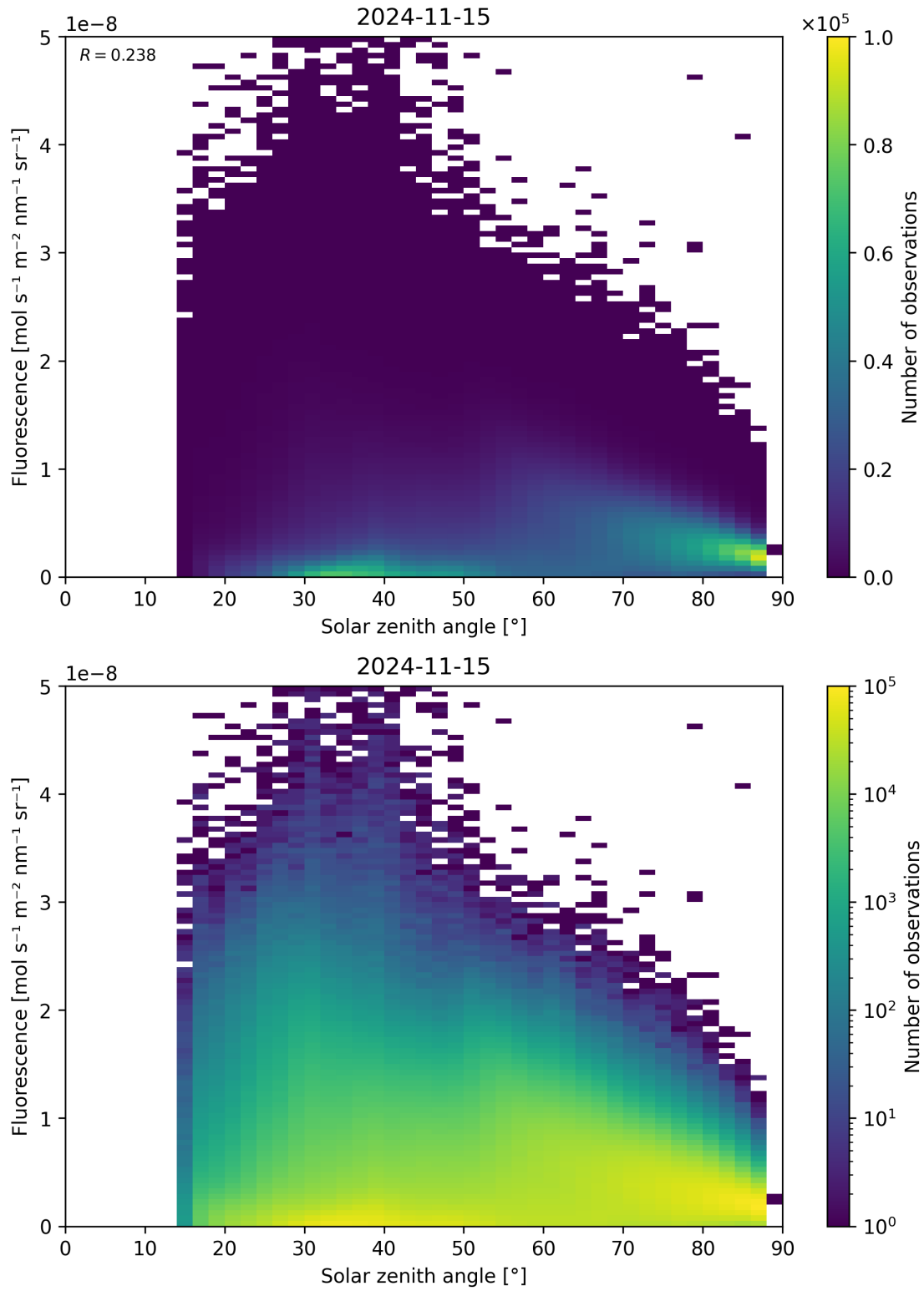
Figure 123: Scatter density plot of “Solar zenith angle” against “Fluorescence” for 2024-11-14 to 2024-11-16.
