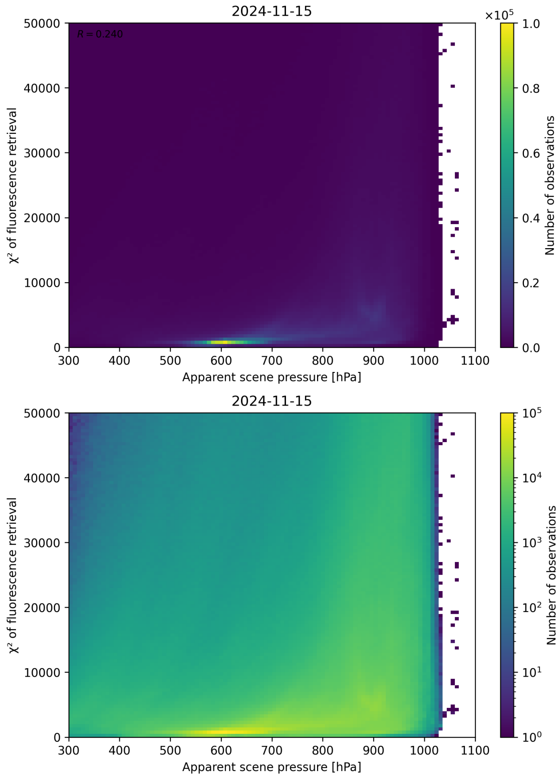
Figure 64: Scatter density plot of “Apparent scene pressure” against “ \chi^2 of fluorescence retrieval” for 2024-11-14 to 2024-11-16.
