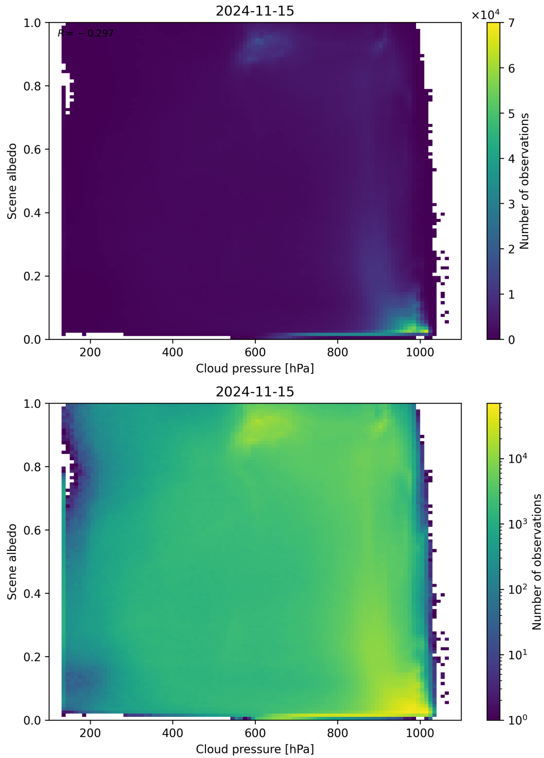
Figure 91: Scatter density plot of “Cloud pressure” against “Scene albedo” for 2024-11-14 to 2024-11-16.
