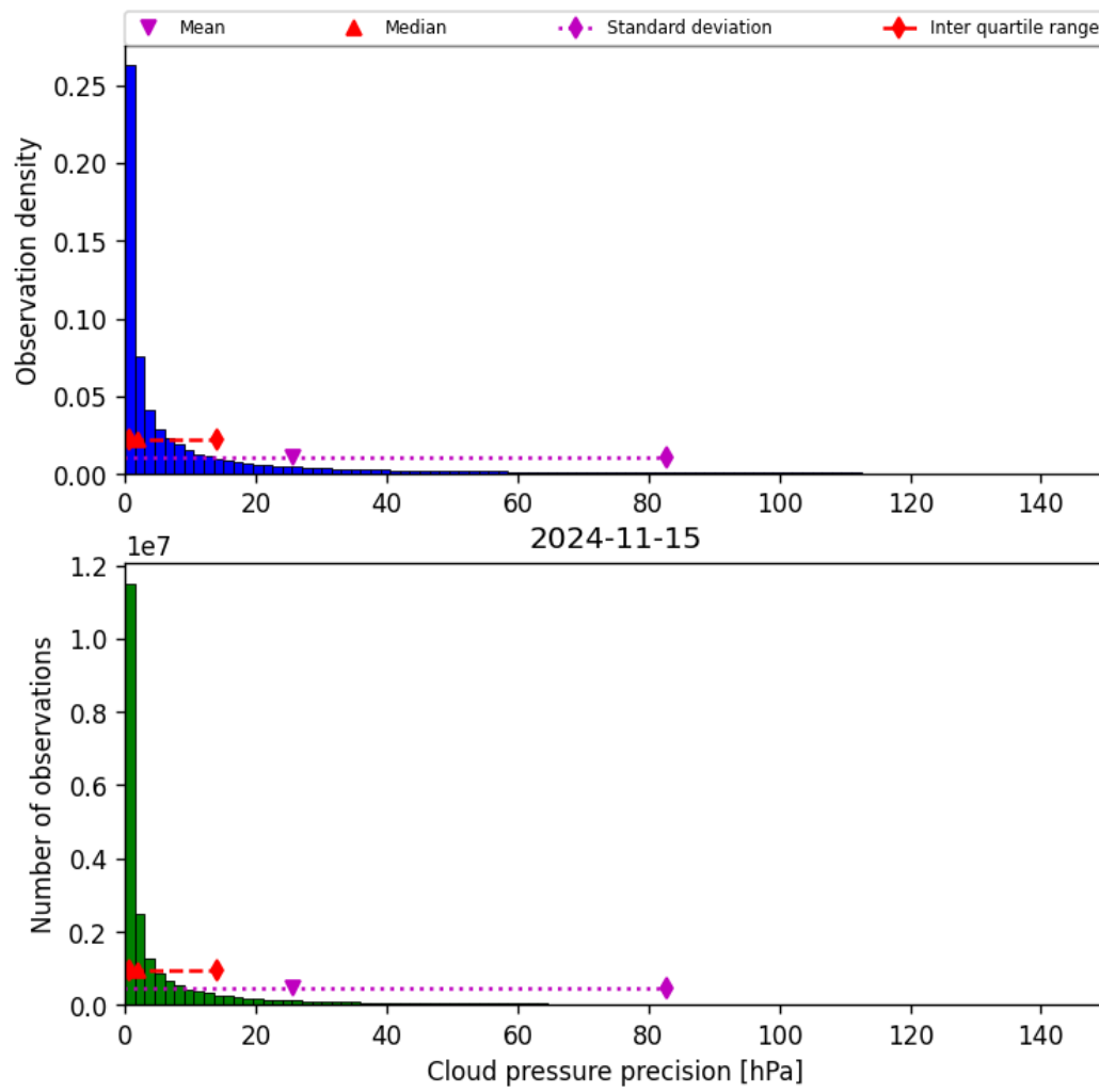
Figure 31: Histogram of “Cloud pressure precision” for 2024-11-14 to 2024-11-16
