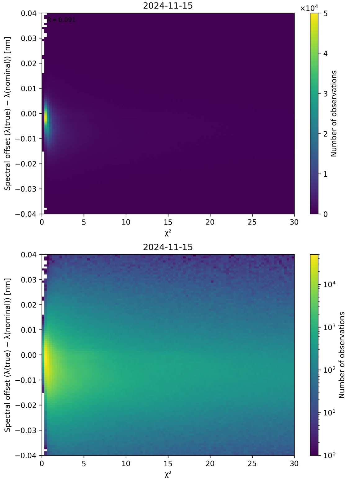
Figure 75: Scatter density plot of “ \chi^2 ” against “Spectral offset ( \lambda_{\text{true}} - \lambda_{\text{nominal}} )” for 2024-11-14 to 2024-11-16.
