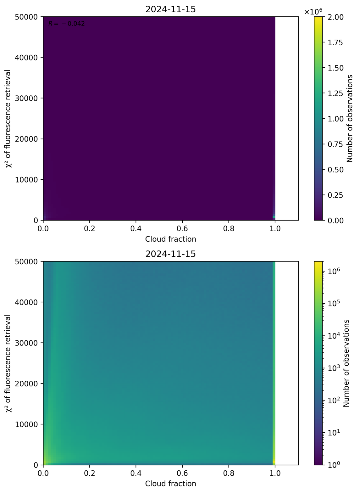
Figure 78: Scatter density plot of “Cloud fraction” against “ \chi^2 of fluorescence retrieval” for 2024-11-14 to 2024-11-16.
