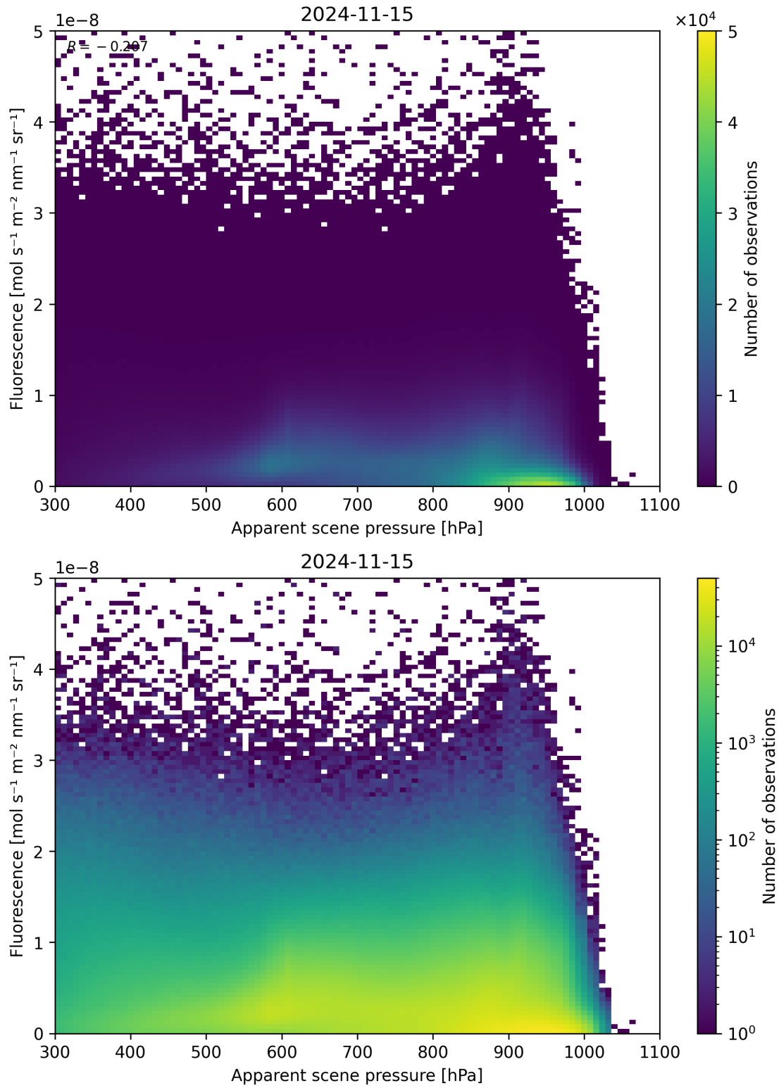
Figure 65: Scatter density plot of “Apparent scene pressure” against “Fluorescence” for 2024-11-14 to 2024-11-16.
