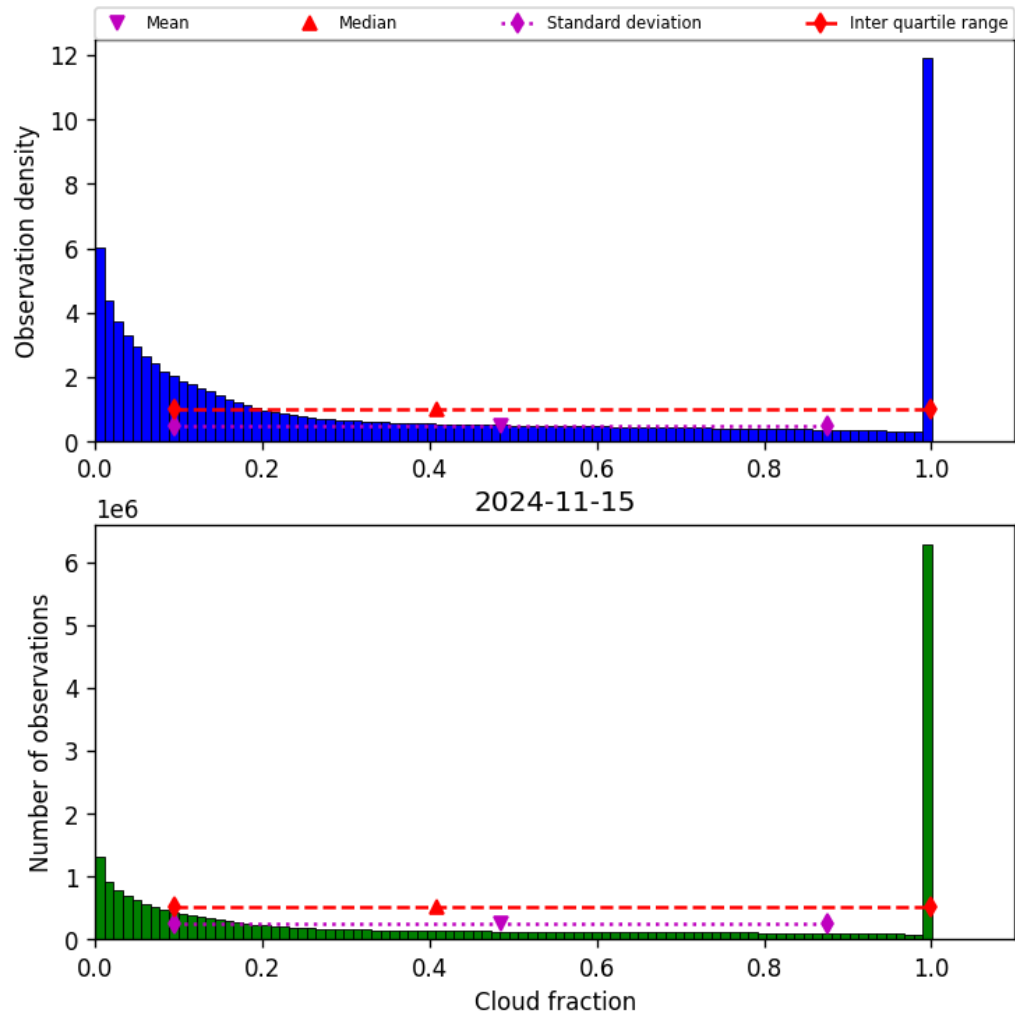
Figure 32: Histogram of “Cloud fraction” for 2024-11-14 to 2024-11-16
