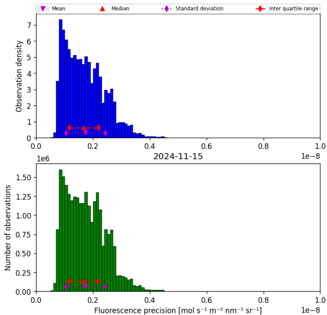
Figure 41: Histogram of “Fluorescence precision” for 2024-11-14 to 2024-11-16
