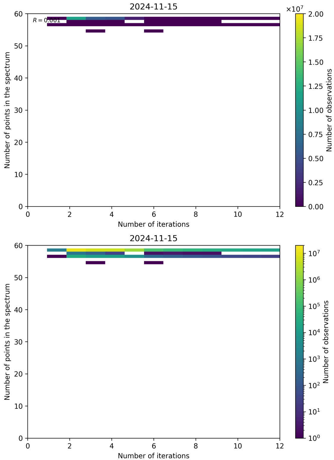
Figure 108: Scatter density plot of “Number of iterations” against “Number of points in the spectrum” for 2024-11-14 to 2024-11-16.
