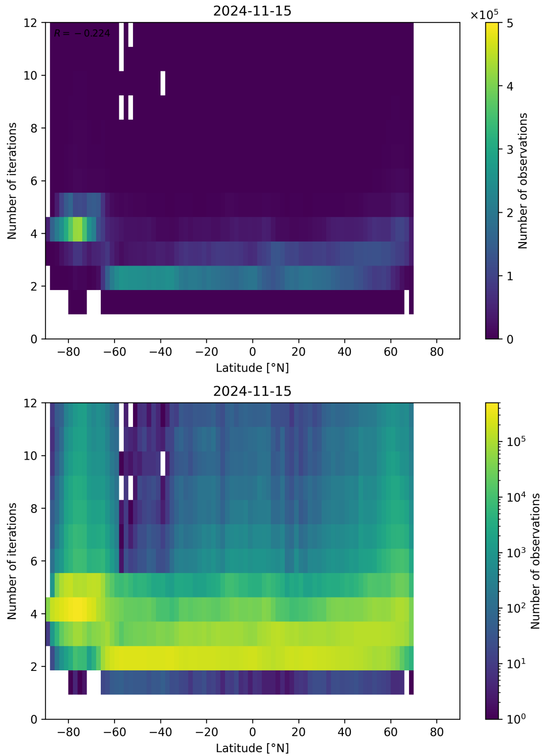
Figure 102: Scatter density plot of “Latitude” against “Number of iterations” for 2024-11-14 to 2024-11-16.
