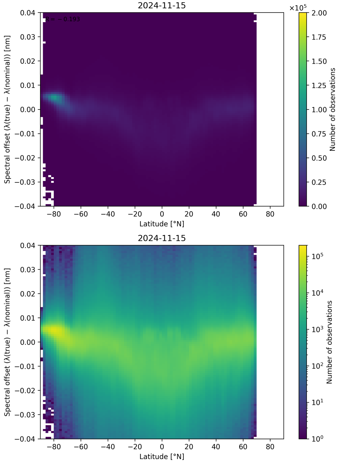
Figure 105: Scatter density plot of “Latitude” against “Spectral offset ( \lambda_{\text{true}} - \lambda_{\text{nominal}} )” for 2024-11-14 to 2024-11-16.
