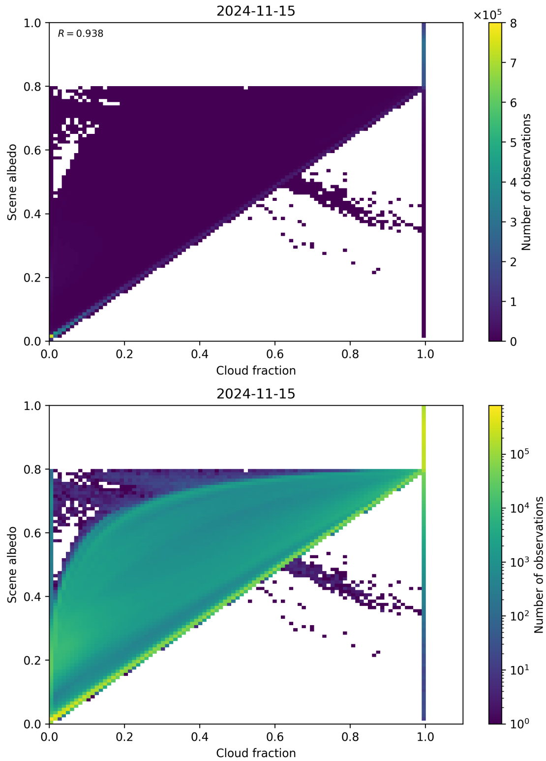
Figure 82: Scatter density plot of “Cloud fraction” against “Scene albedo” for 2024-11-14 to 2024-11-16.
