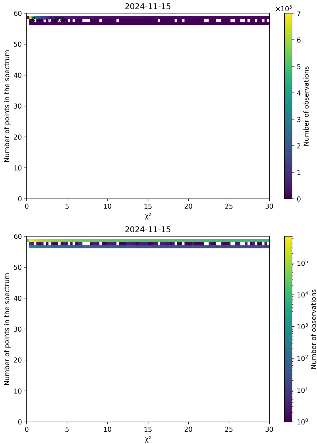
Figure 74: Scatter density plot of “ \chi^2 ” against “Number of points in the spectrum” for 2024-11-14 to 2024-11-16.
