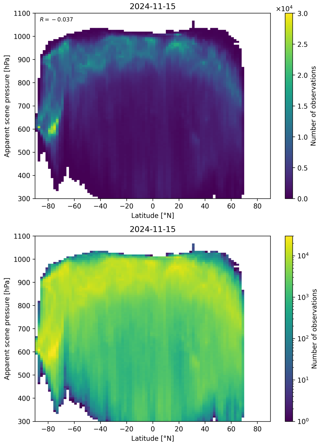
Figure 96: Scatter density plot of “Latitude” against “Apparent scene pressure” for 2024-11-14 to 2024-11-16.
