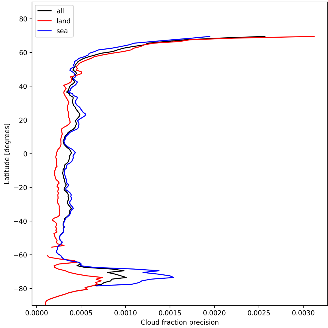
Figure 16: Zonal average of “Cloud fraction precision” for 2024-11-14 to 2024-11-16.
