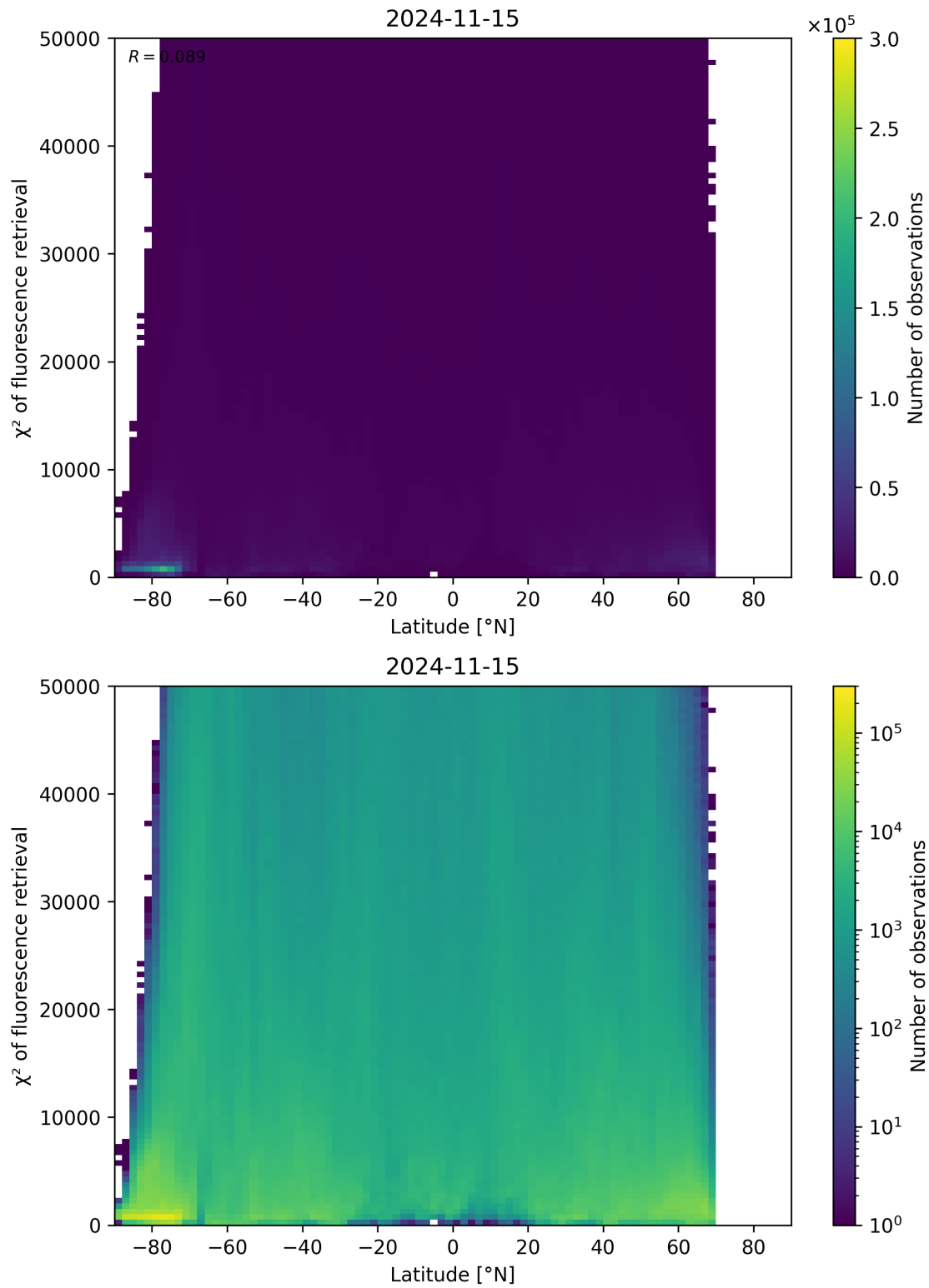
Figure 98: Scatter density plot of “Latitude” against “ \chi^2 of fluorescence retrieval” for 2024-11-14 to 2024-11-16.
