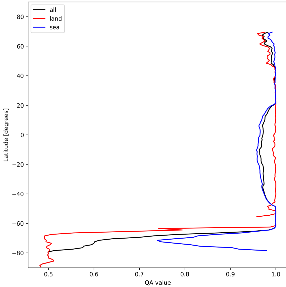
Figure 12: Zonal average of “QA value” for 2024-11-14 to 2024-11-16.
