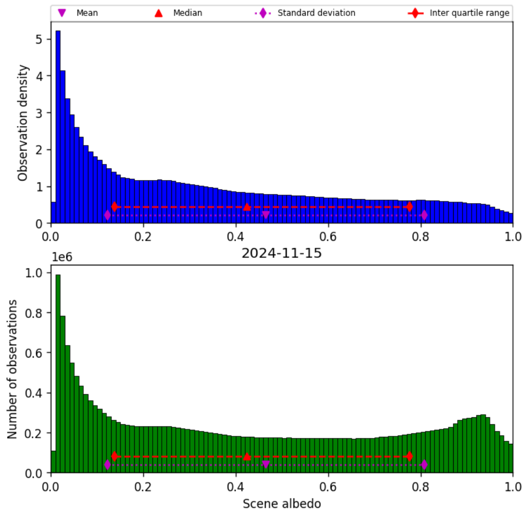
Figure 34: Histogram of “Scene albedo” for 2024-11-14 to 2024-11-16
