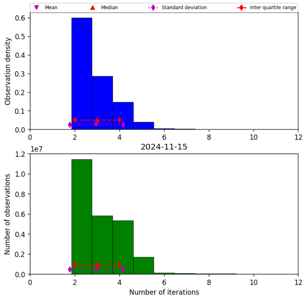
Figure 39: Histogram of “Number of iterations” for 2024-11-14 to 2024-11-16
