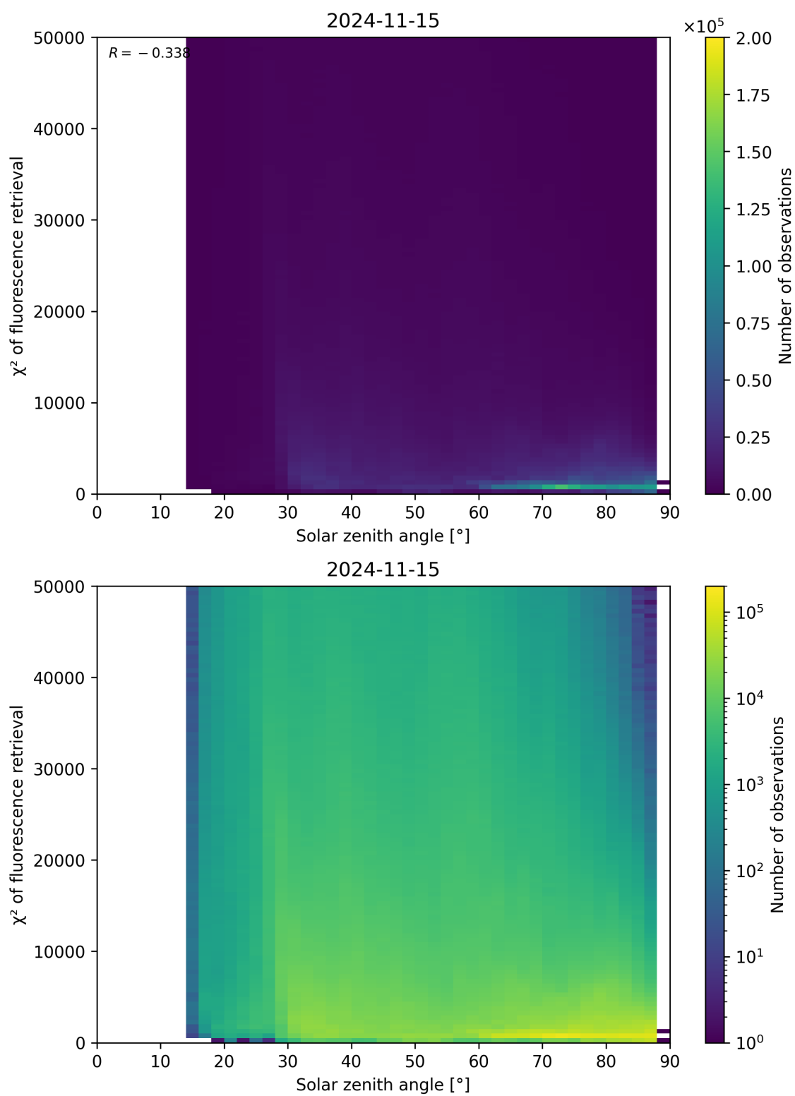
Figure 120: Scatter density plot of “Solar zenith angle” against “ \chi^2 of fluorescence retrieval” for 2024-11-14 to 2024-11-16.
