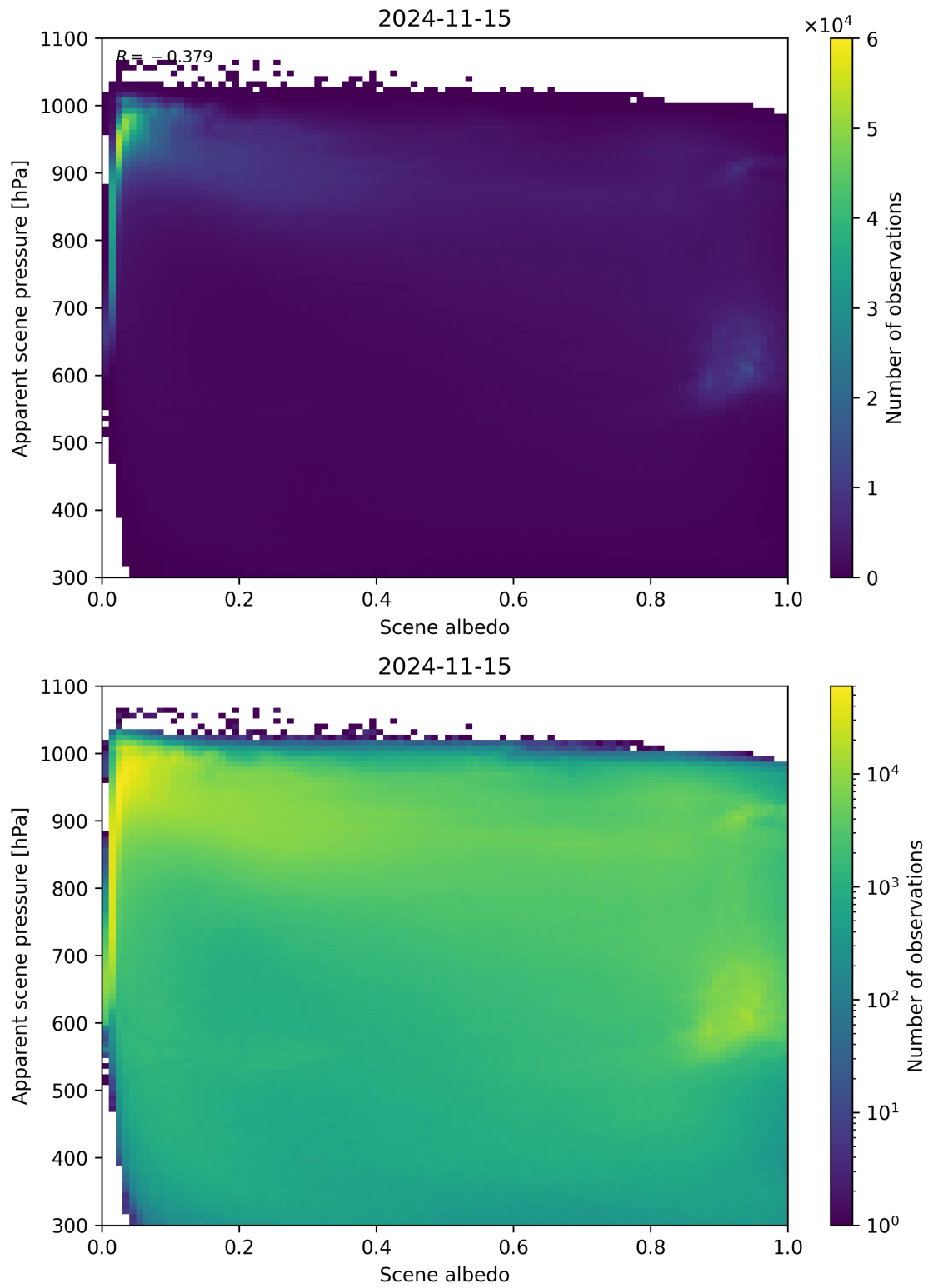
Figure 111: Scatter density plot of “Scene albedo” against “Apparent scene pressure” for 2024-11-14 to 2024-11-16.
