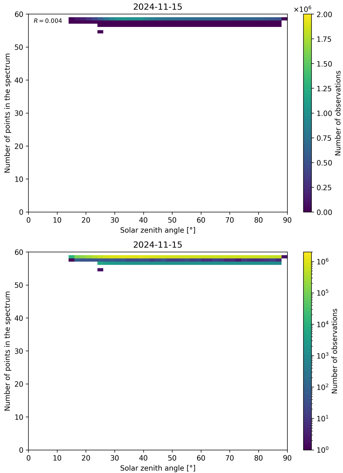
Figure 126: Scatter density plot of “Solar zenith angle” against “Number of points in the spectrum” for 2024-11-14 to 2024-11-16.
