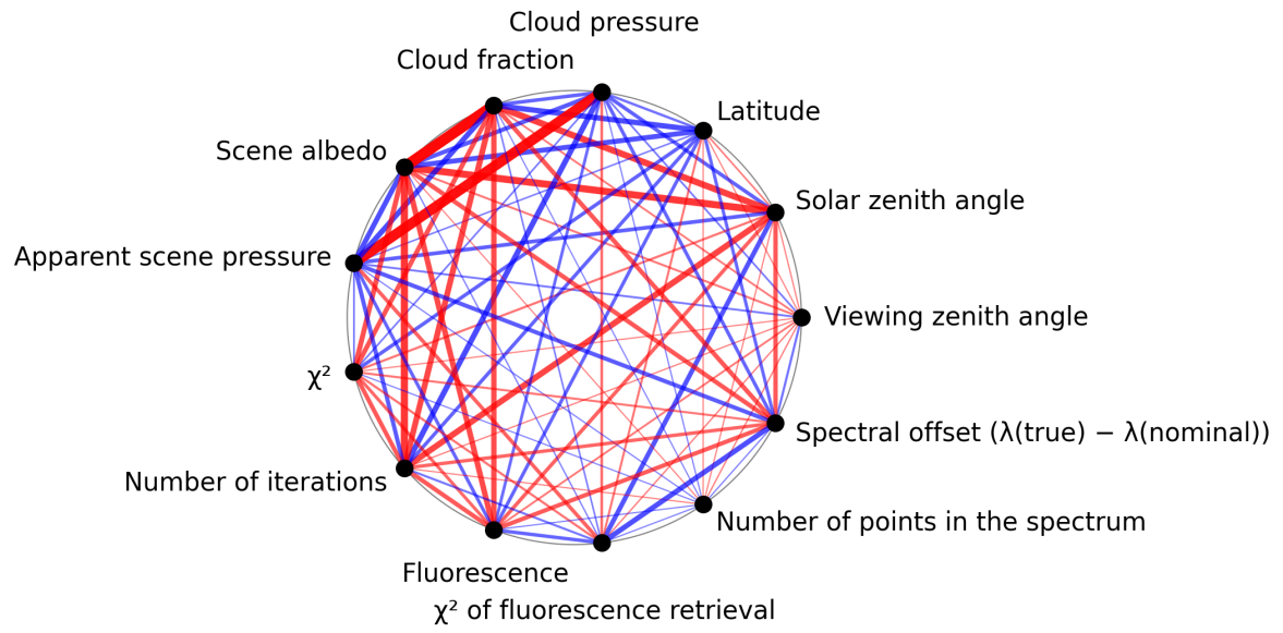
Figure 1: Map of correlation graph for 2024-11-14 to 2024-11-16.
