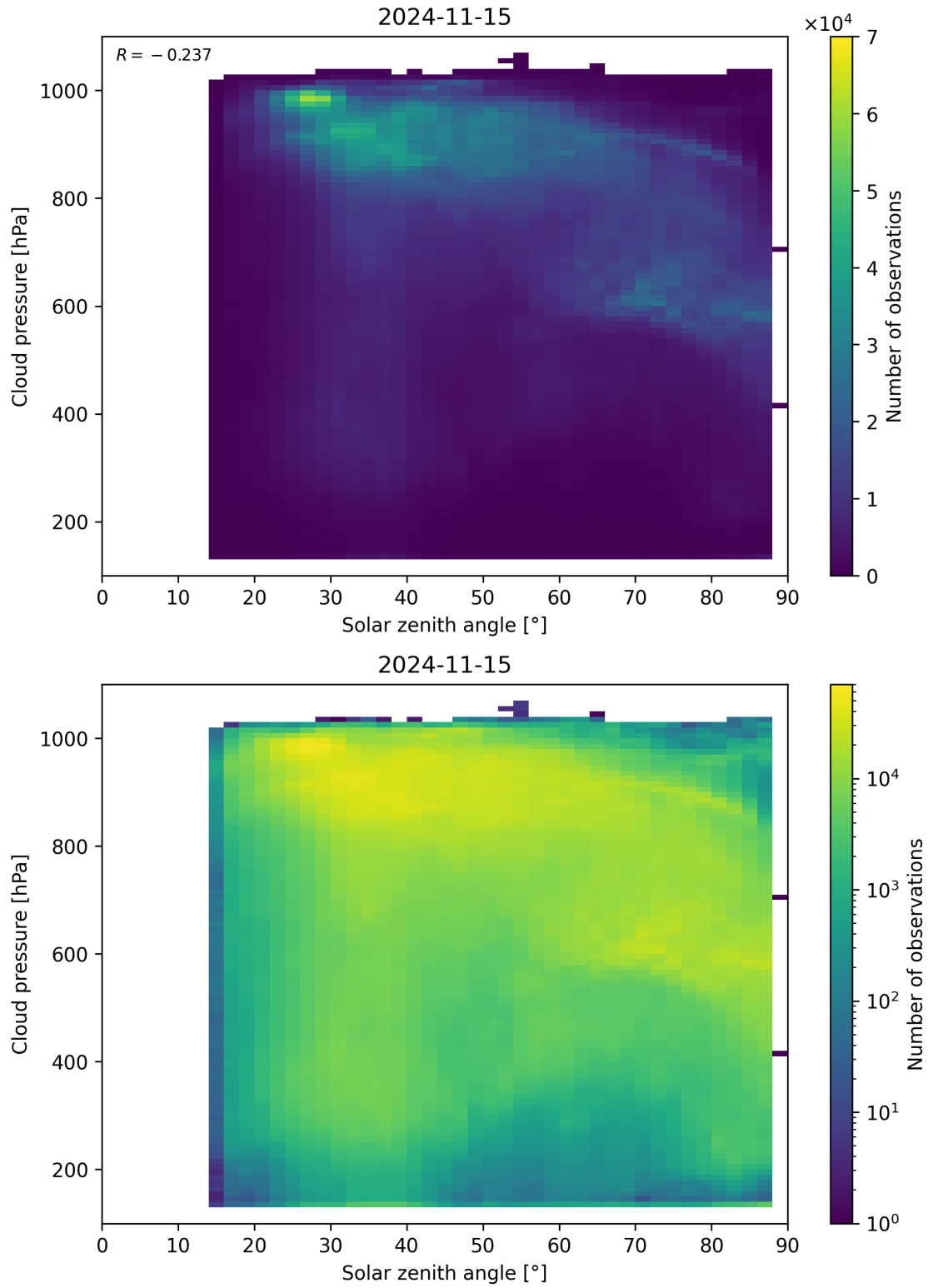
Figure 122: Scatter density plot of “Solar zenith angle” against “Cloud pressure” for 2024-11-14 to 2024-11-16.
