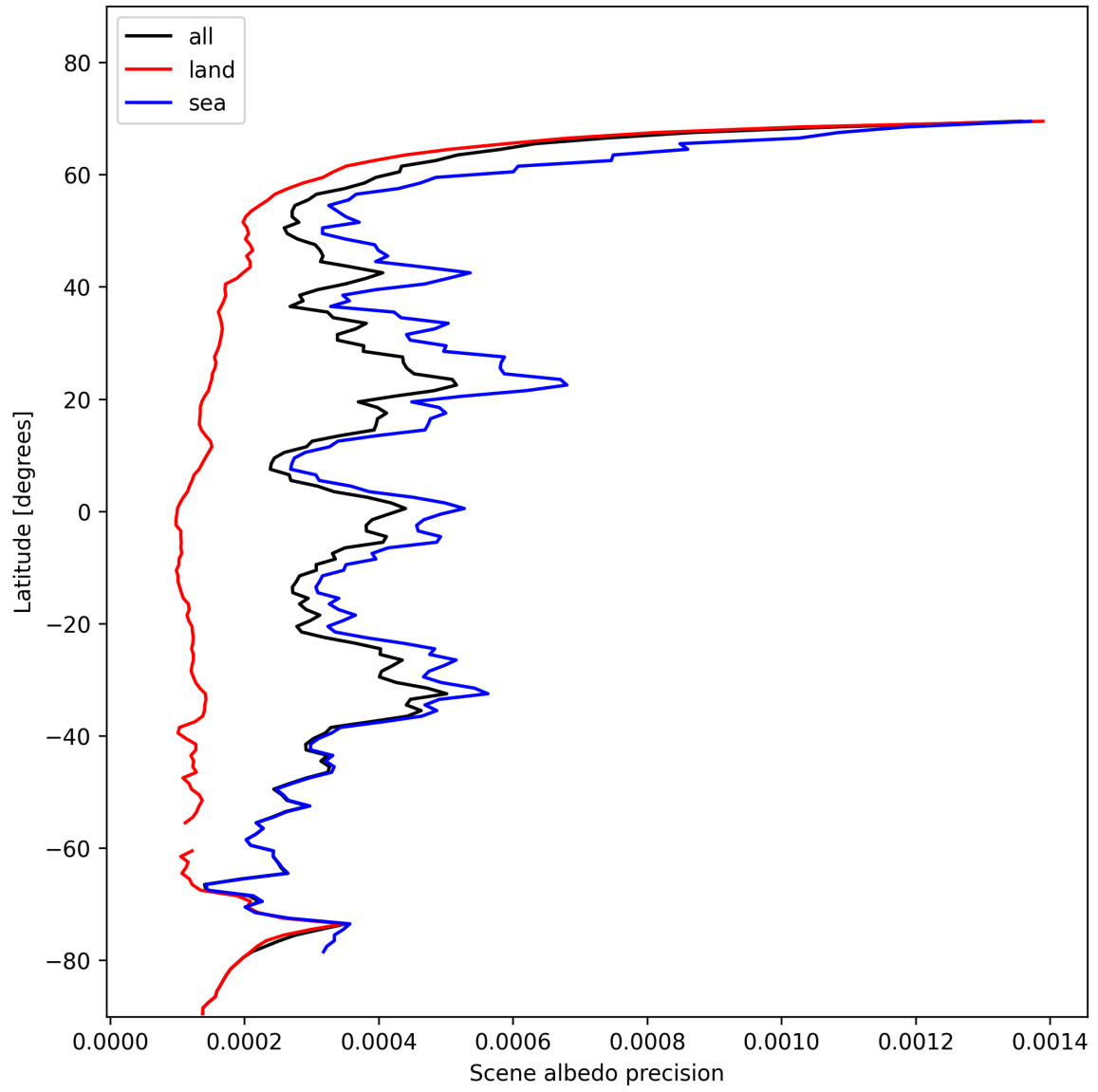
Figure 18: Zonal average of "Scene albedo precision" for 2024-11-14 to 2024-11-16.
