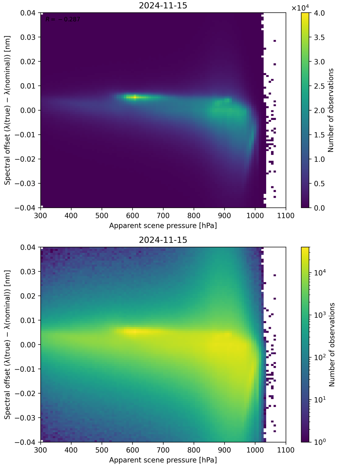
Figure 68: Scatter density plot of “Apparent scene pressure” against “Spectral offset ( \lambda_{\text{true}} - \lambda_{\text{nominal}} )” for 2024-11-14 to 2024-11-16.
