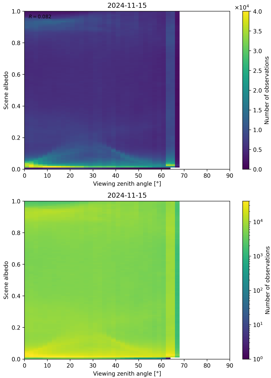
Figure 138: Scatter density plot of “Viewing zenith angle” against “Scene albedo” for 2024-11-14 to 2024-11-16.
