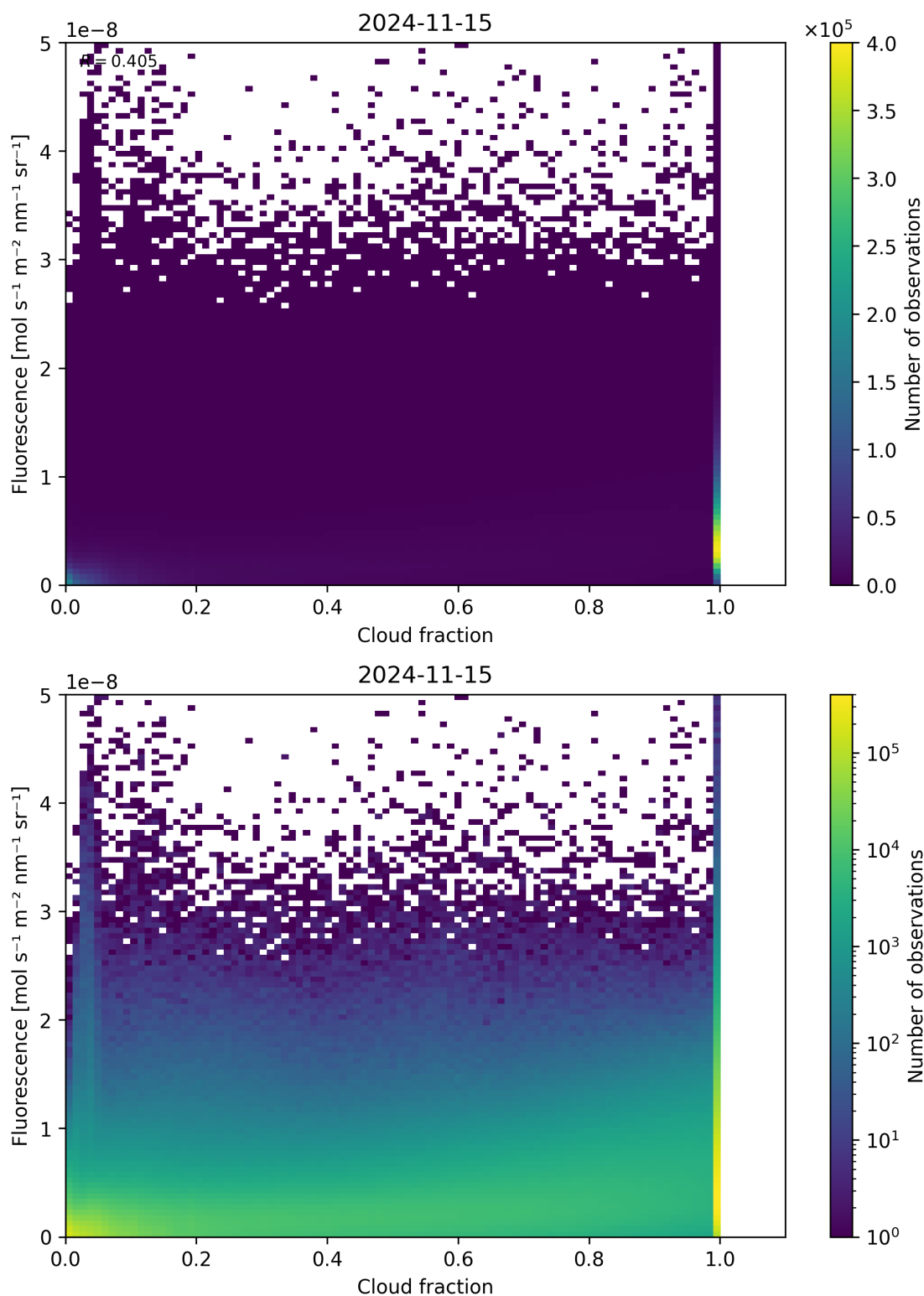
Figure 79: Scatter density plot of “Cloud fraction” against “Fluorescence” for 2024-11-14 to 2024-11-16.
