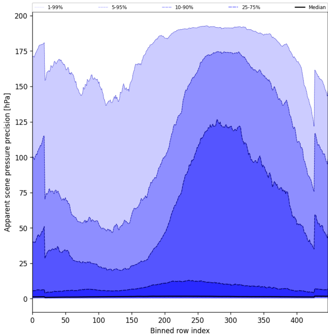
Figure 54: Along track statistics of “Apparent scene pressure precision” for 2024-11-14 to 2024-11-16
