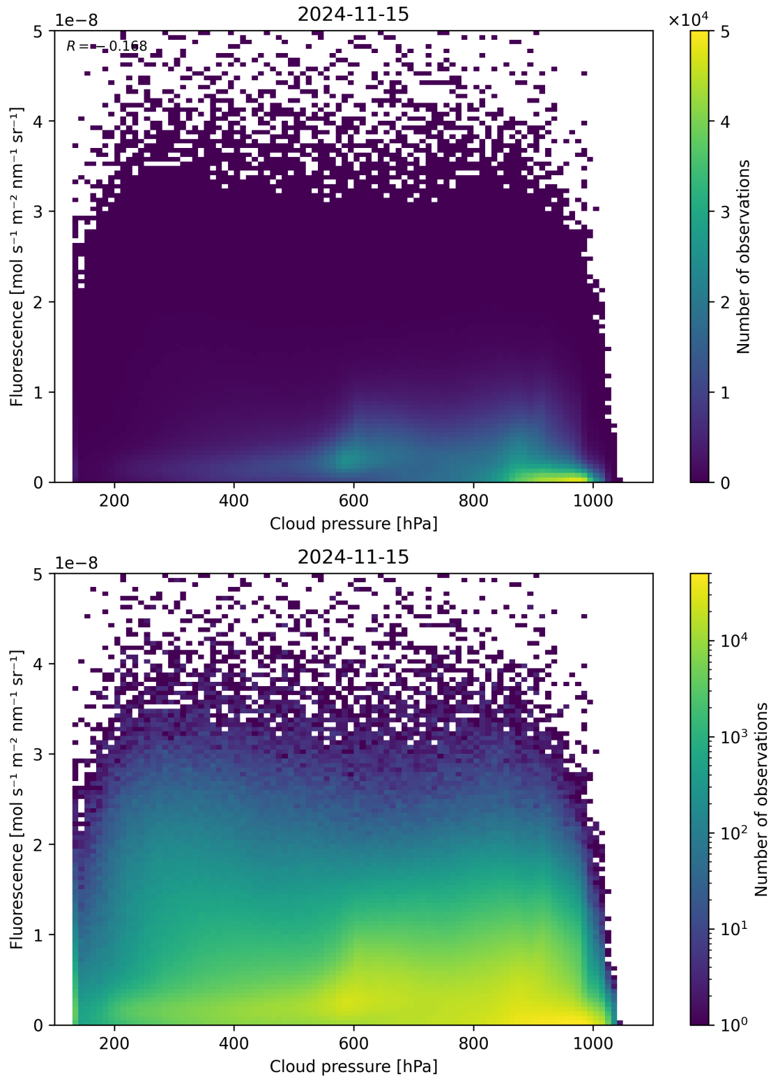
Figure 88: Scatter density plot of “Cloud pressure” against “Fluorescence” for 2024-11-14 to 2024-11-16.
