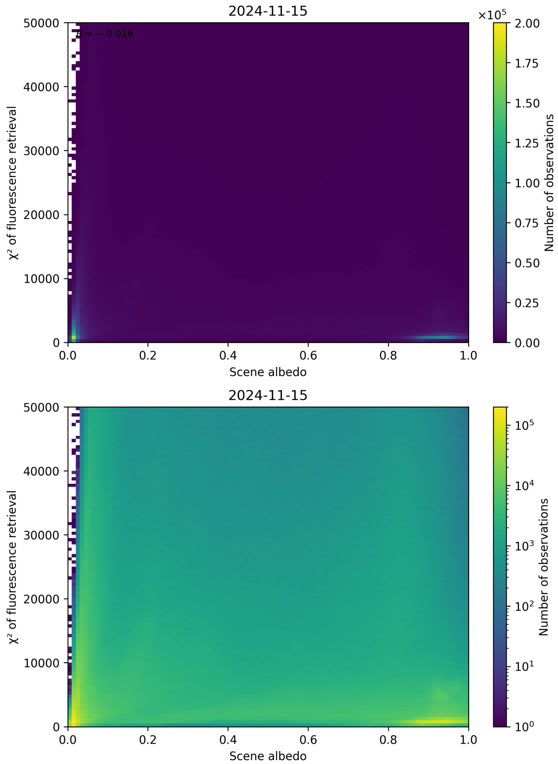
Figure 113: Scatter density plot of “Scene albedo” against “ \chi^2 of fluorescence retrieval” for 2024-11-14 to 2024-11-16.
