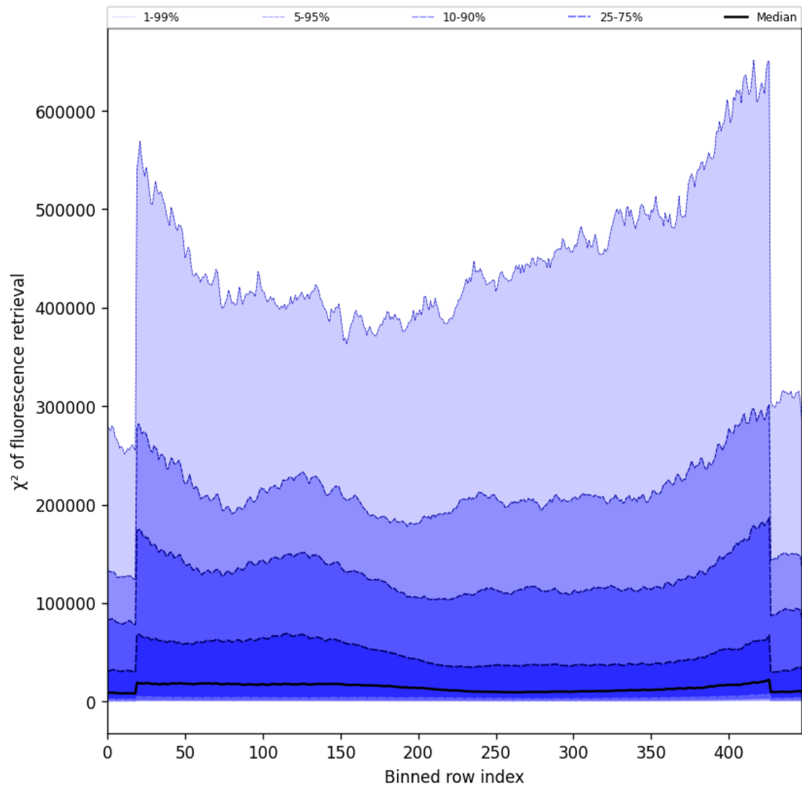
Figure 59: Along track statistics of “ \chi^2 of fluorescence retrieval” for 2024-11-14 to 2024-11-16
