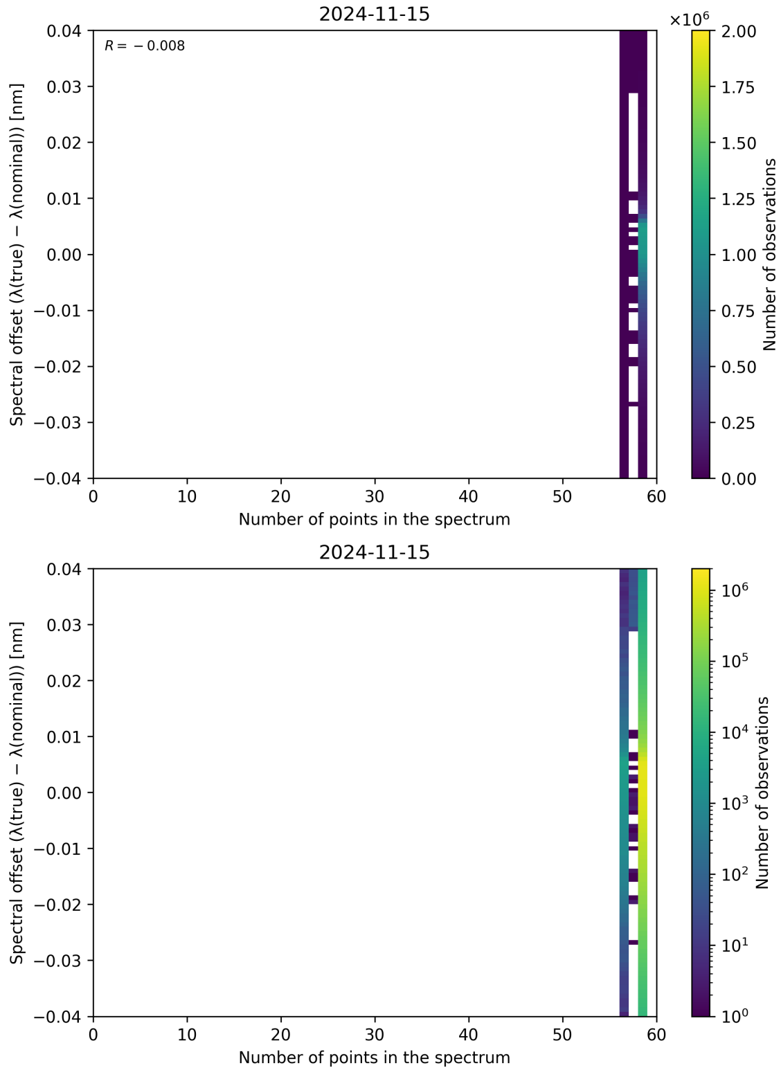
Figure 110: Scatter density plot of “Number of points in the spectrum” against “Spectral offset ( \lambda_{\text{true}} - \lambda_{\text{nominal}} )” for 2024-11-14 to 2024-11-16.
