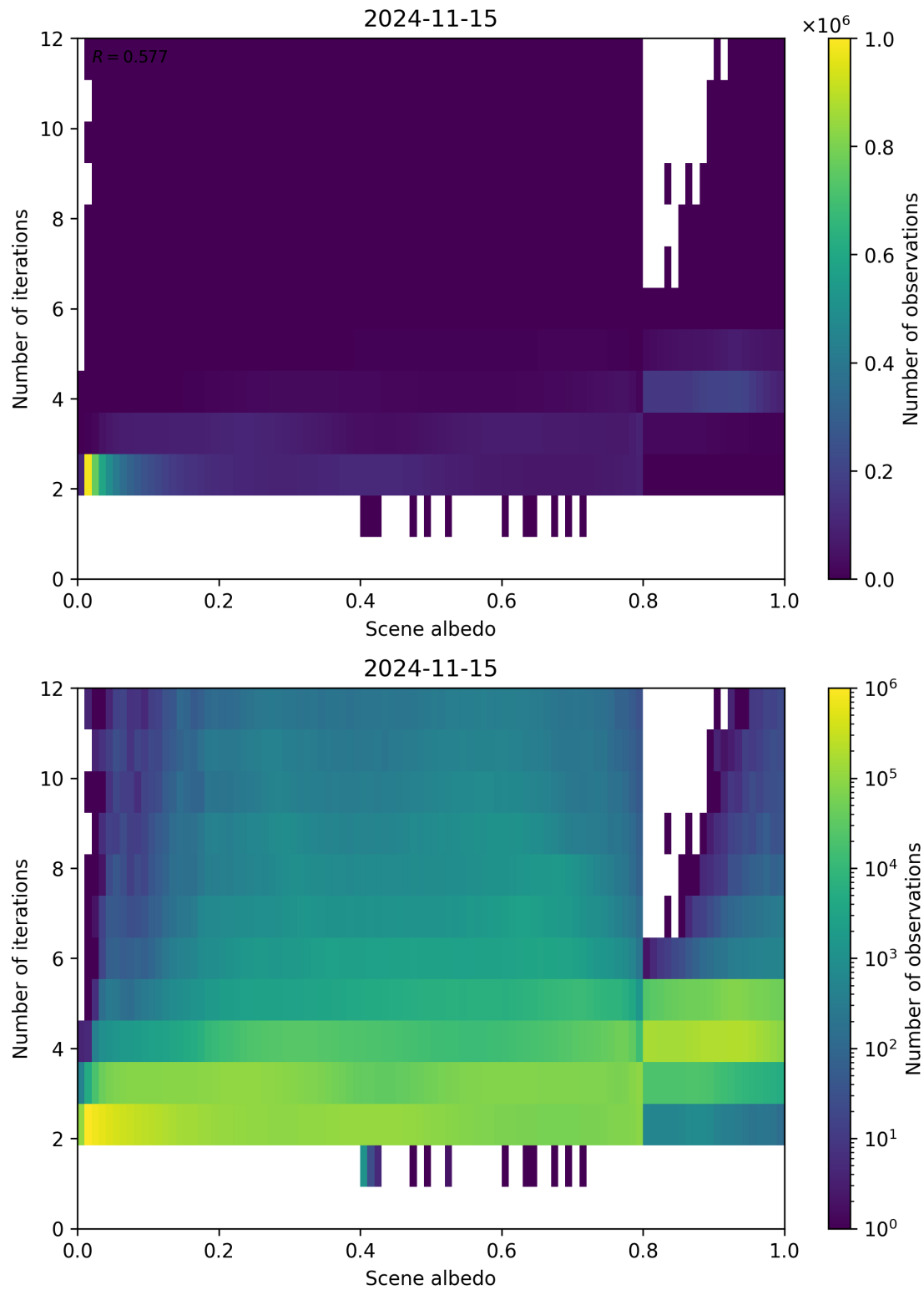
Figure 115: Scatter density plot of “Scene albedo” against “Number of iterations” for 2024-11-14 to 2024-11-16.
