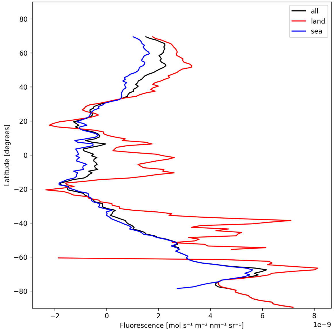
Figure 23: Zonal average of “Fluorescence” for 2024-11-14 to 2024-11-16.
