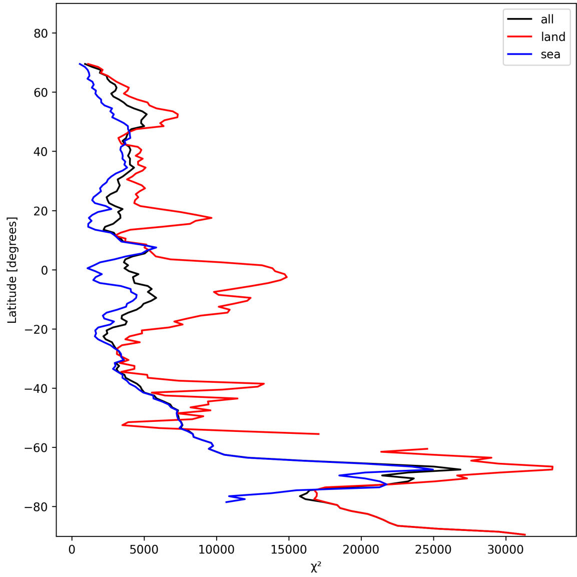
Figure 21: Zonal average of “ \chi^2 ” for 2024-11-14 to 2024-11-16.
