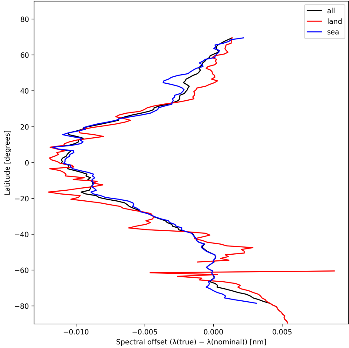
Figure 28: Zonal average of “Spectral offset ( \lambda_{\text{true}} - \lambda_{\text{nominal}} )” for 2024-11-14 to 2024-11-16.
