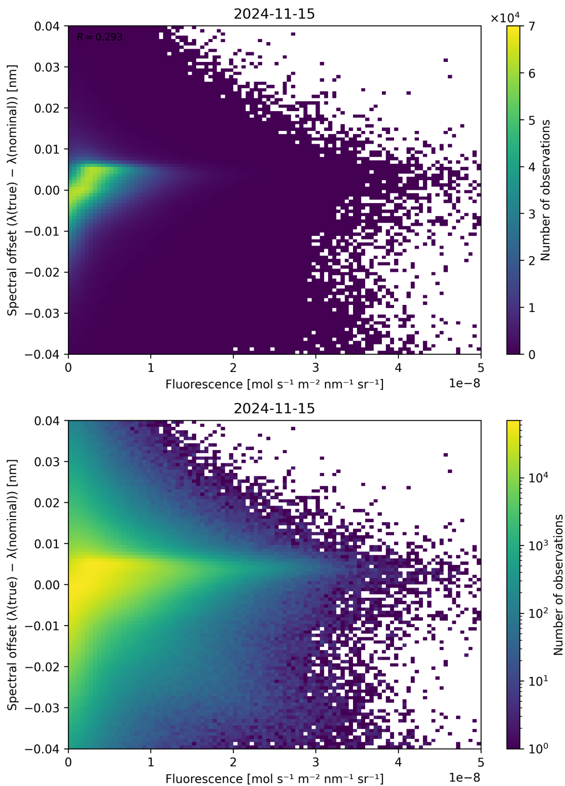
Figure 95: Scatter density plot of “Fluorescence” against “Spectral offset ( \lambda_{\text{true}} - \lambda_{\text{nominal}} )” for 2024-11-14 to 2024-11-16.
