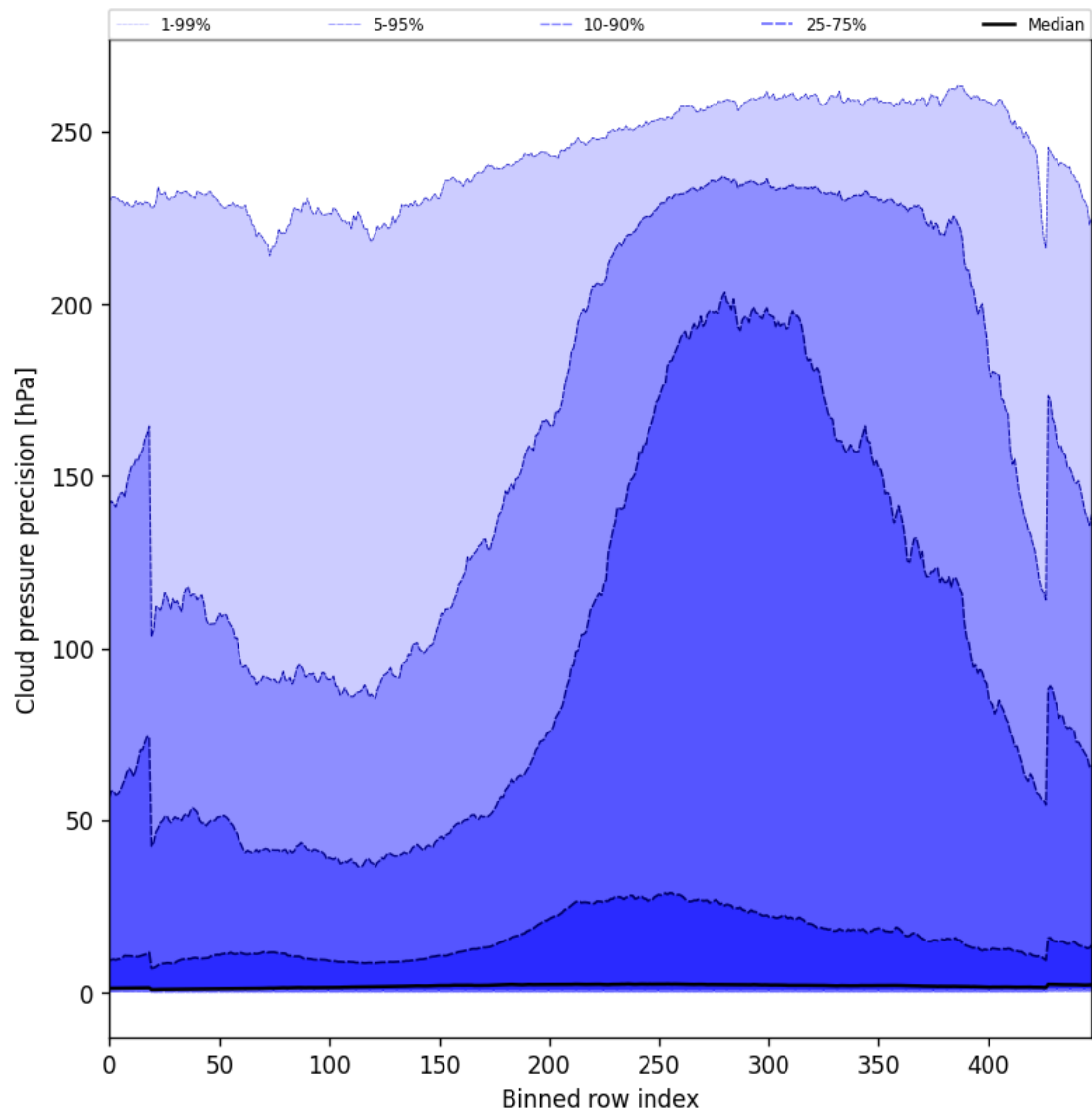
Figure 48: Along track statistics of “Cloud pressure precision” for 2024-11-14 to 2024-11-16
