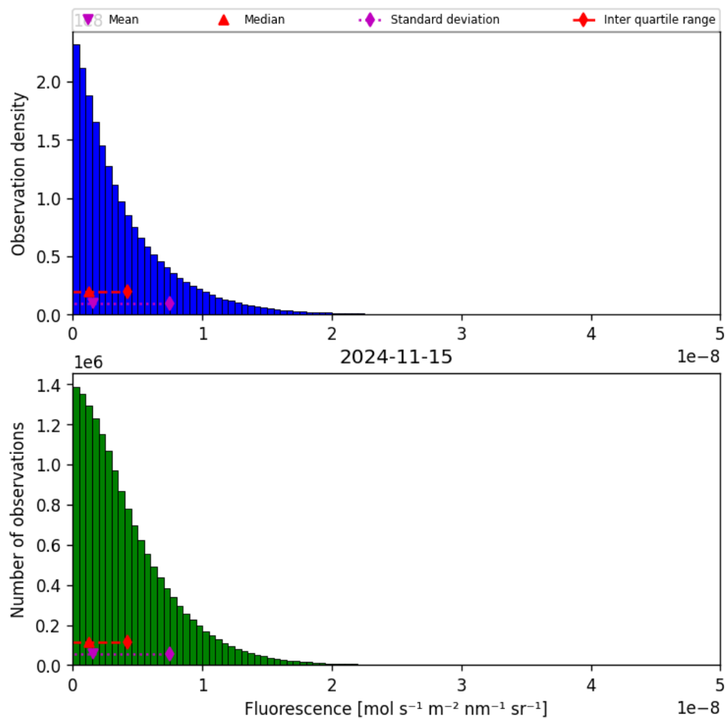
Figure 40: Histogram of “Fluorescence” for 2024-11-14 to 2024-11-16
