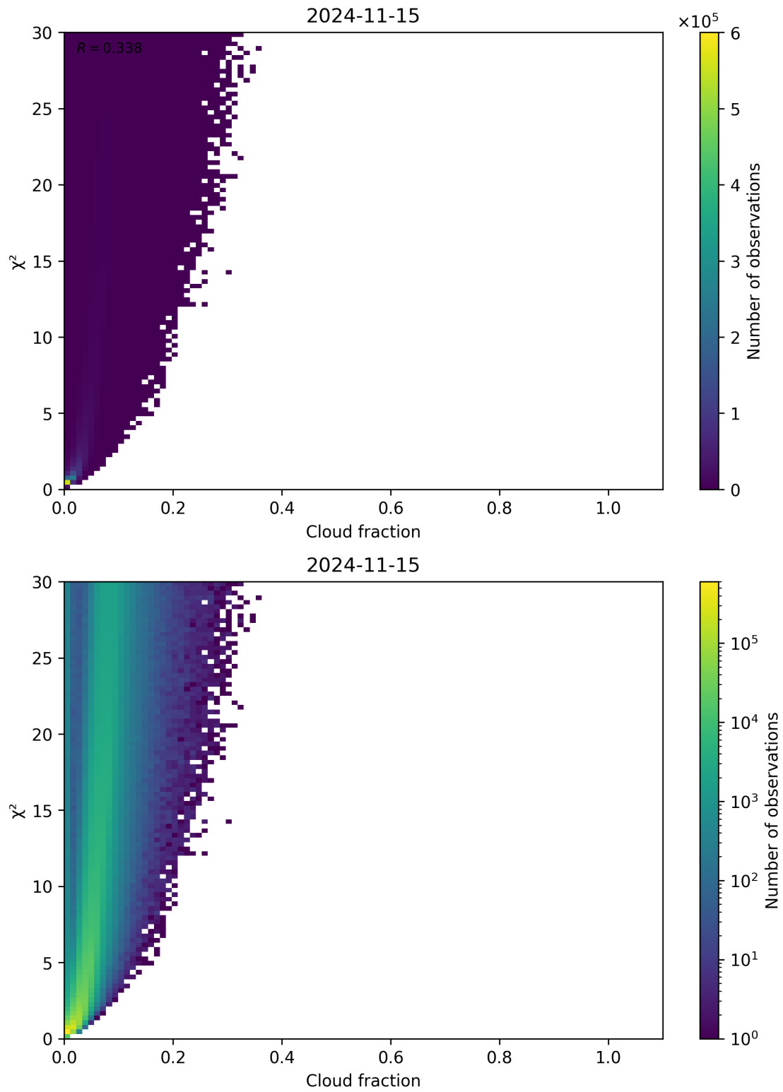
Figure 77: Scatter density plot of “Cloud fraction” against “ \chi^2 ” for 2024-11-14 to 2024-11-16.
