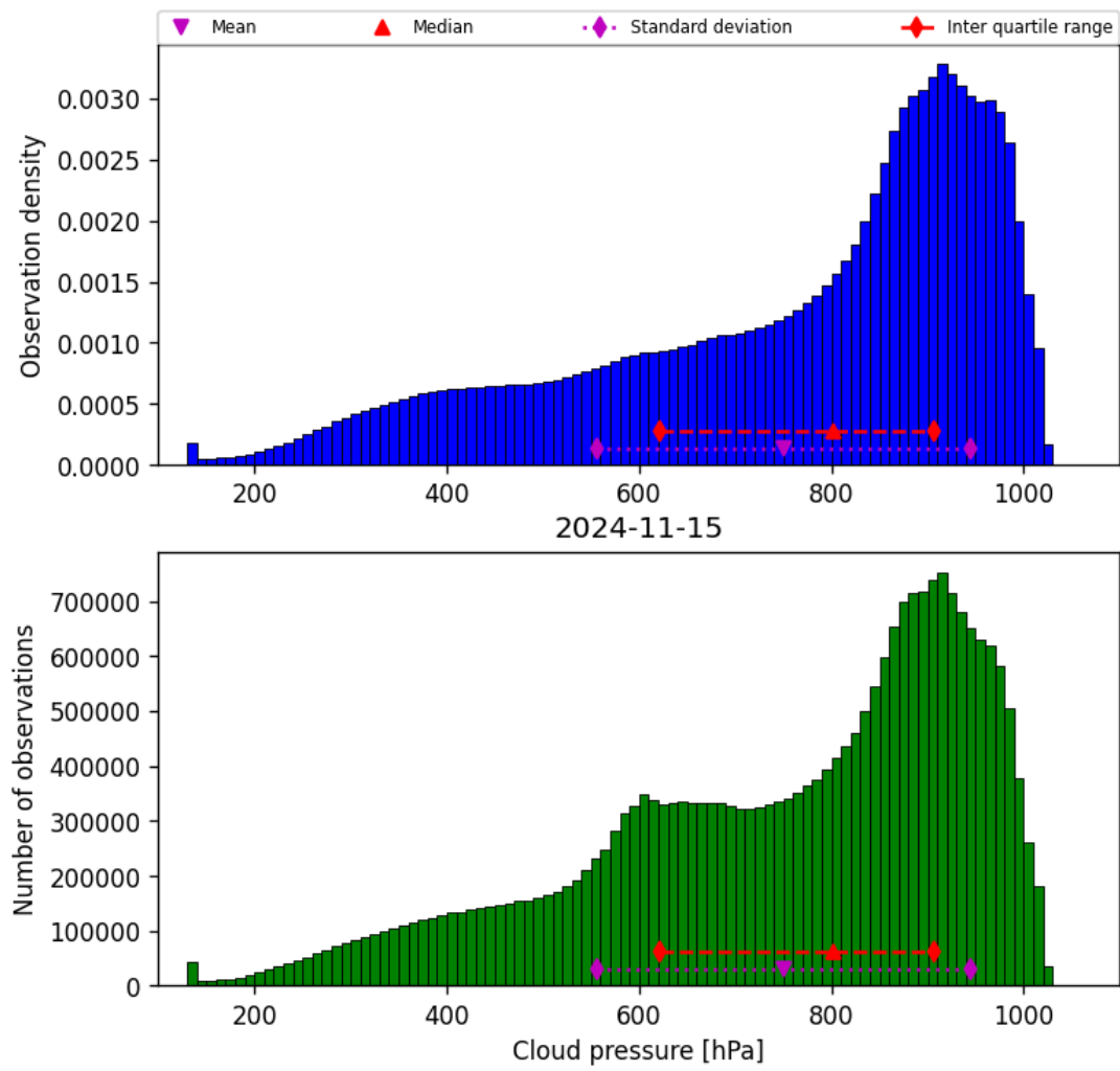
Figure 30: Histogram of “Cloud pressure” for 2024-11-14 to 2024-11-16
