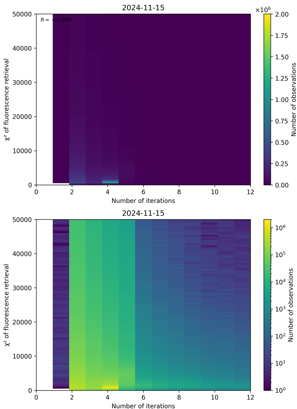
Figure 106: Scatter density plot of “Number of iterations” against “ \chi^2 of fluorescence retrieval” for 2024-11-14 to 2024-11-16.
