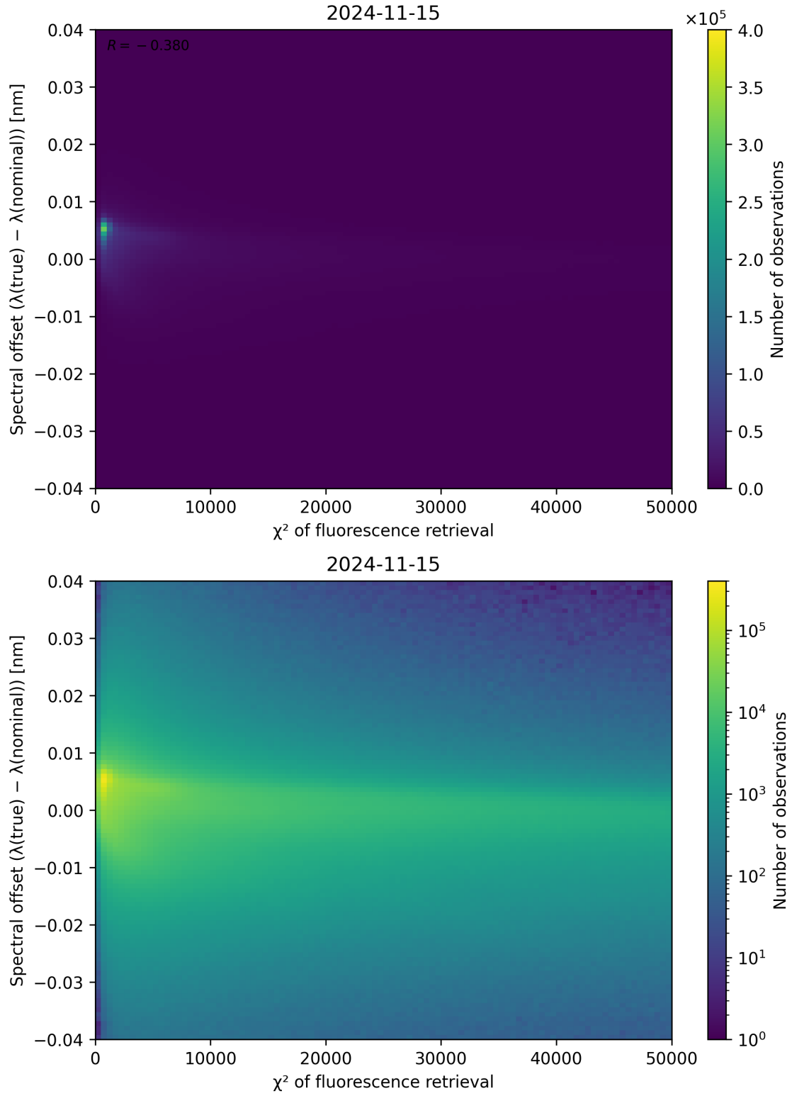
Figure 72: Scatter density plot of “ \chi^2 of fluorescence retrieval” against “Spectral offset ( \lambda_{\text{true}} - \lambda_{\text{nominal}} )” for 2024-11-14 to 2024-11-16.
