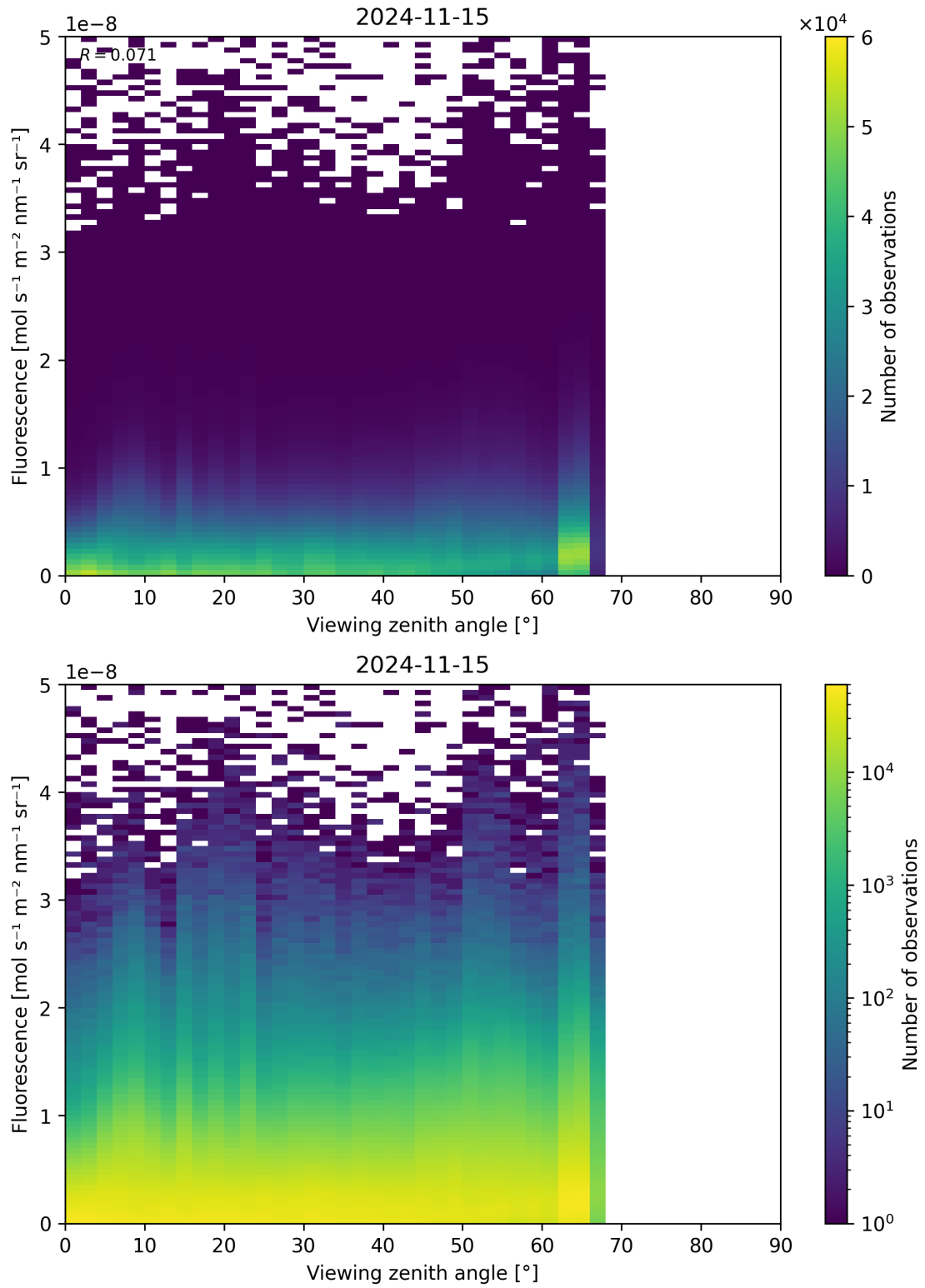
Figure 134: Scatter density plot of “Viewing zenith angle” against “Fluorescence” for 2024-11-14 to 2024-11-16.
