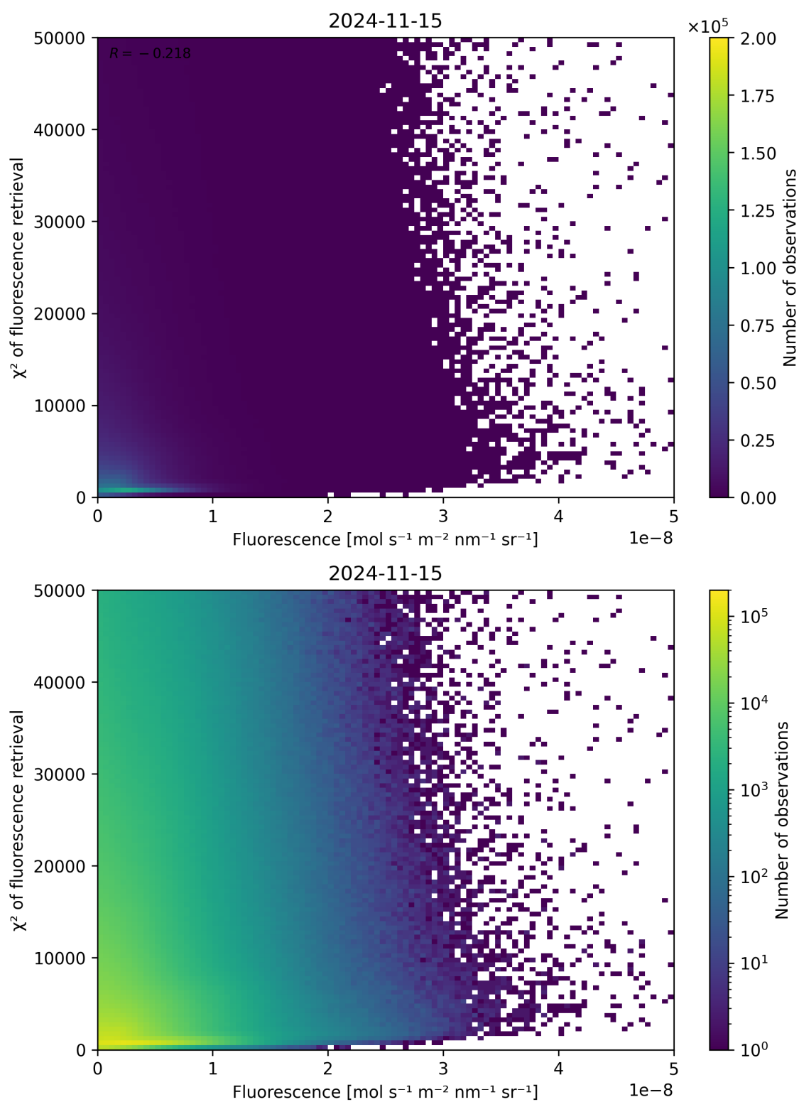
Figure 93: Scatter density plot of “Fluorescence” against “ \chi^2 of fluorescence retrieval” for 2024-11-14 to 2024-11-16.
