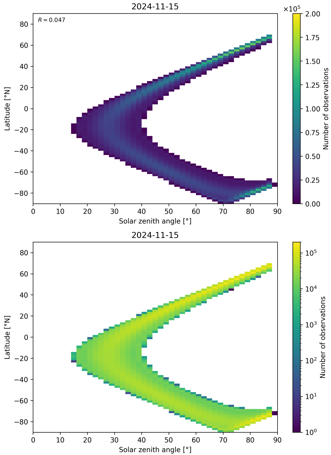
Figure 124: Scatter density plot of “Solar zenith angle” against “Latitude” for 2024-11-14 to 2024-11-16.
