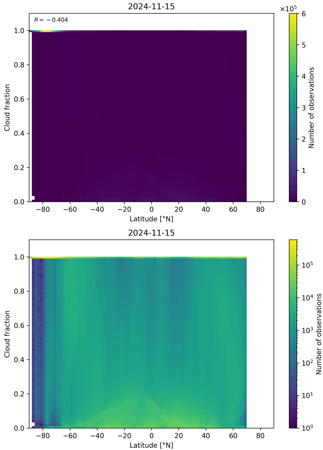
Figure 99: Scatter density plot of “Latitude” against “Cloud fraction” for 2024-11-14 to 2024-11-16.
