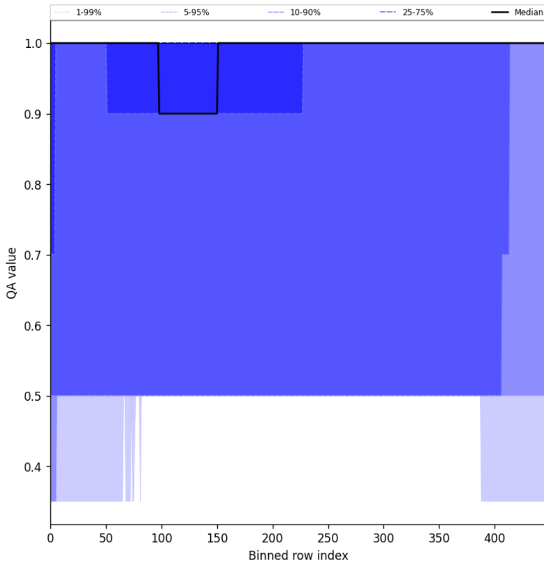
Figure 46: Along track statistics of “QA value” for 2024-11-14 to 2024-11-16
