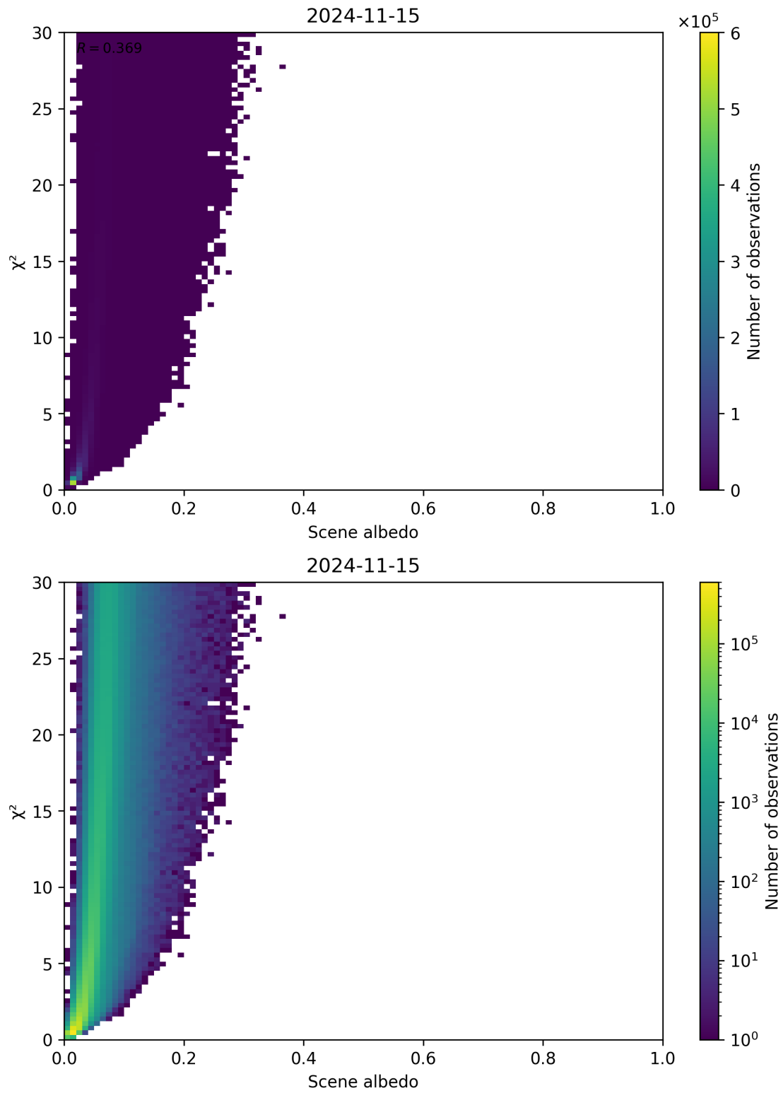
Figure 112: Scatter density plot of “Scene albedo” against “ \chi^2 ” for 2024-11-14 to 2024-11-16.
