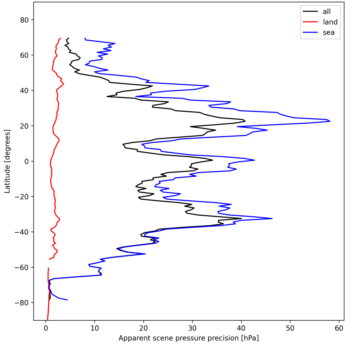
Figure 20: Zonal average of “Apparent scene pressure precision” for 2024-11-14 to 2024-11-16.
