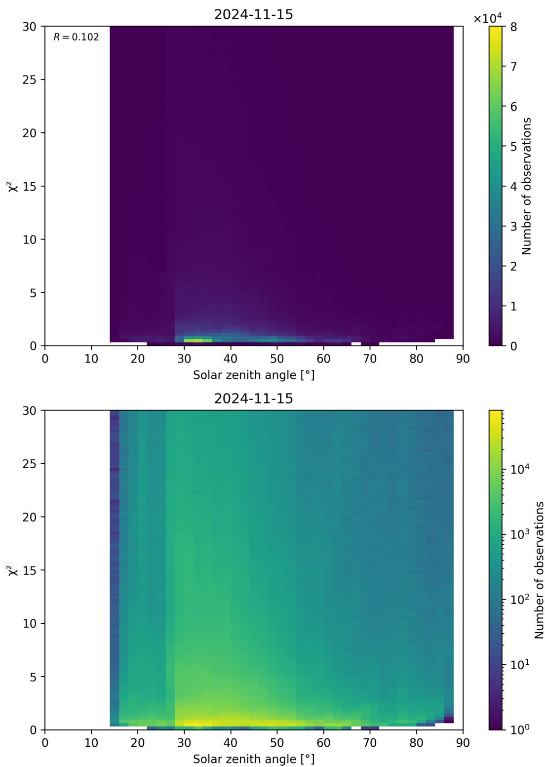
Figure 119: Scatter density plot of “Solar zenith angle” against “ \chi^2 ” for 2024-11-14 to 2024-11-16.
