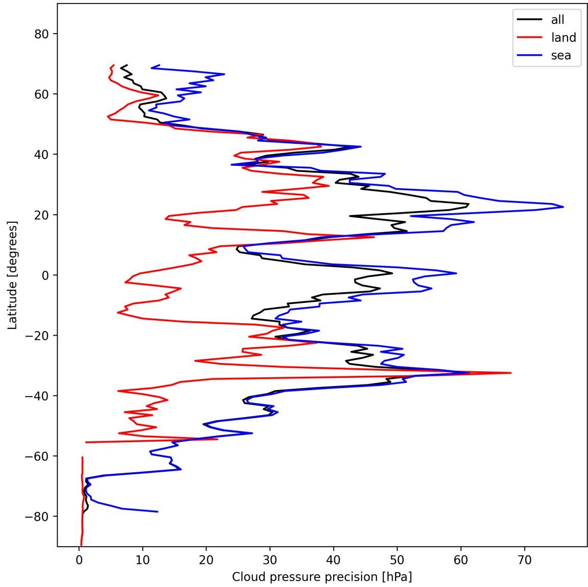
Figure 14: Zonal average of “Cloud pressure precision” for 2024-11-14 to 2024-11-16.
