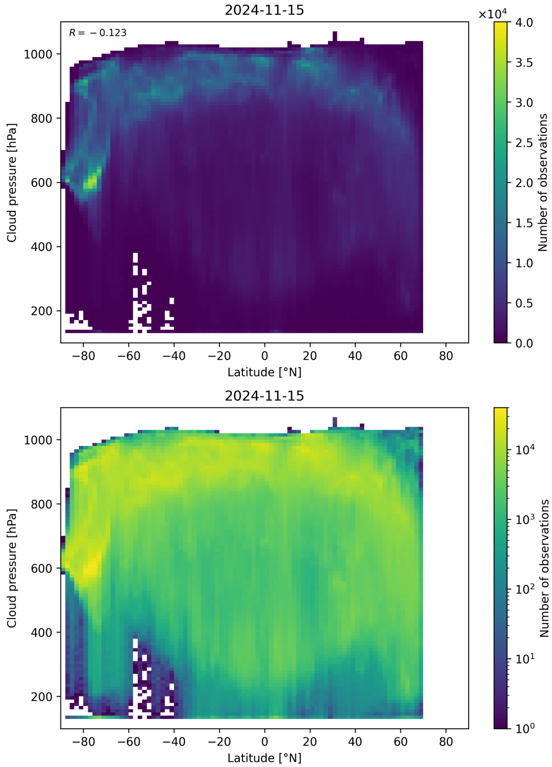
Figure 100: Scatter density plot of “Latitude” against “Cloud pressure” for 2024-11-14 to 2024-11-16.
