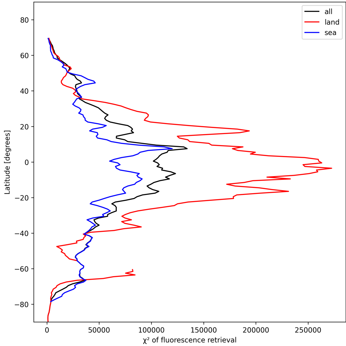
Figure 25: Zonal average of “ \chi^2 of fluorescence retrieval” for 2024-11-14 to 2024-11-16.
