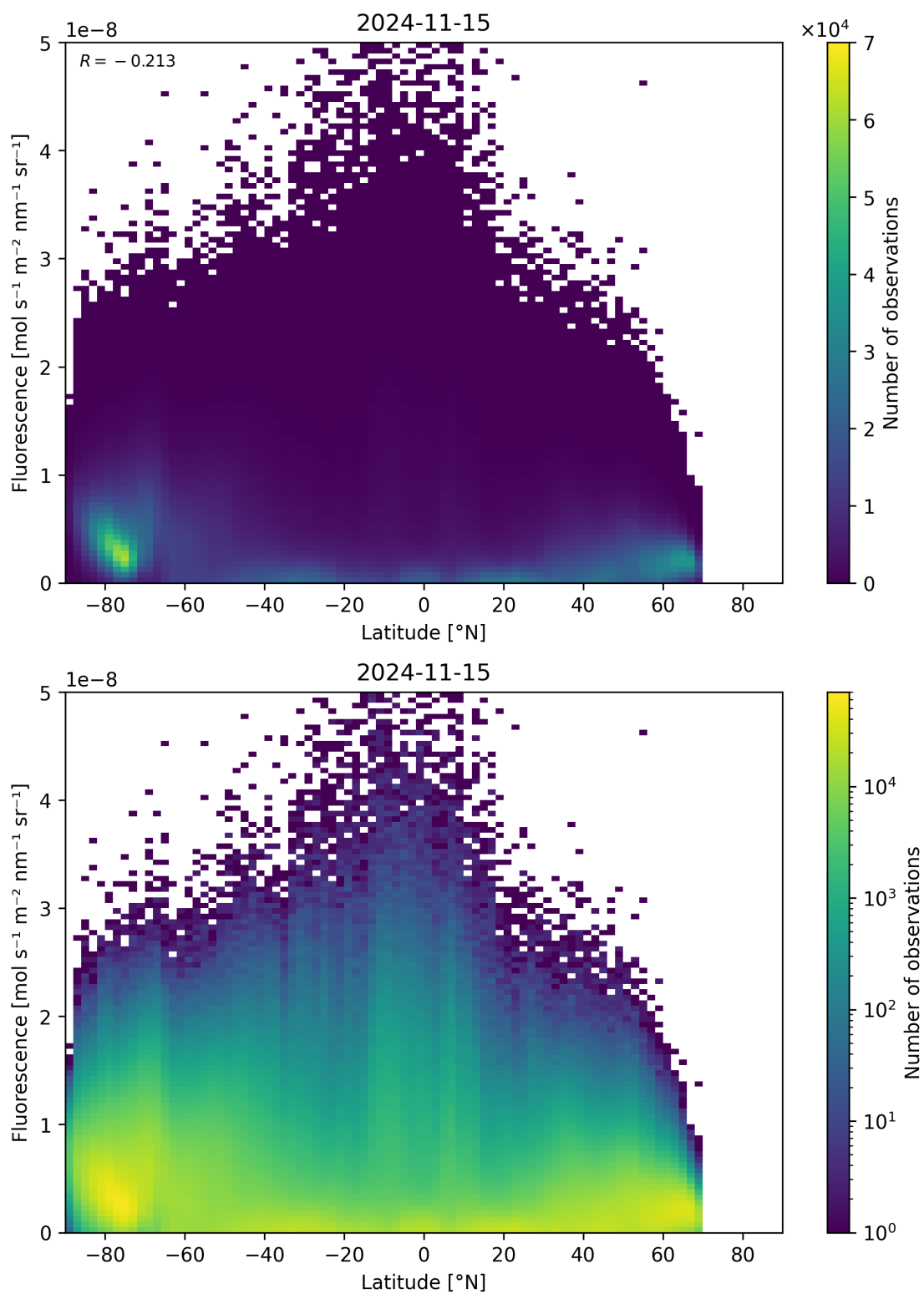
Figure 101: Scatter density plot of “Latitude” against “Fluorescence” for 2024-11-14 to 2024-11-16.
