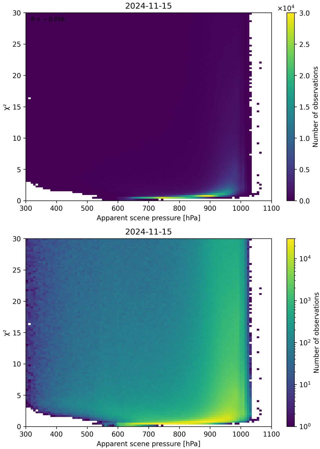
Figure 63: Scatter density plot of “Apparent scene pressure” against “ \chi^2 ” for 2024-11-14 to 2024-11-16.
