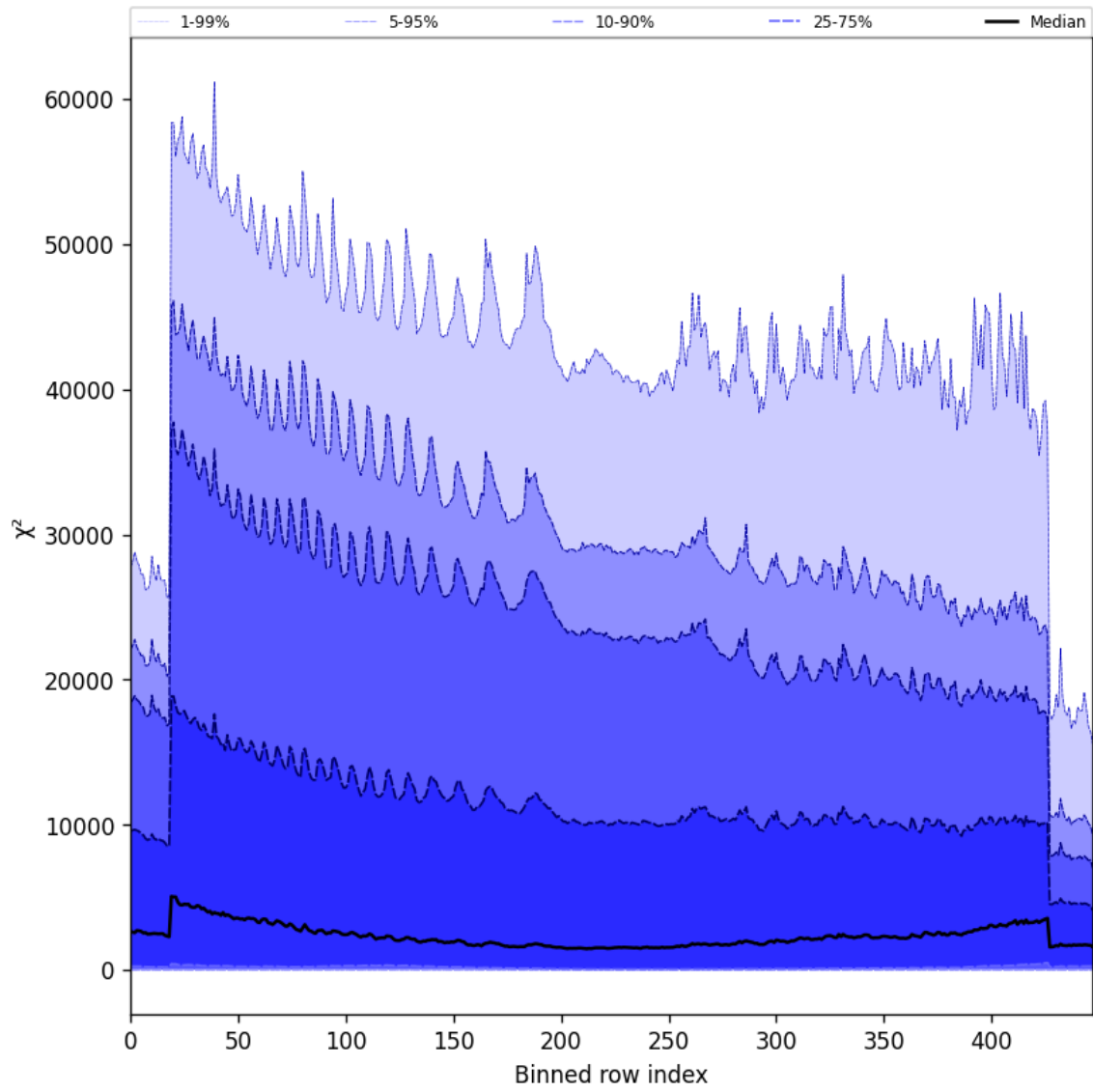
Figure 55: Along track statistics of “ \chi^2 ” for 2024-11-14 to 2024-11-16
