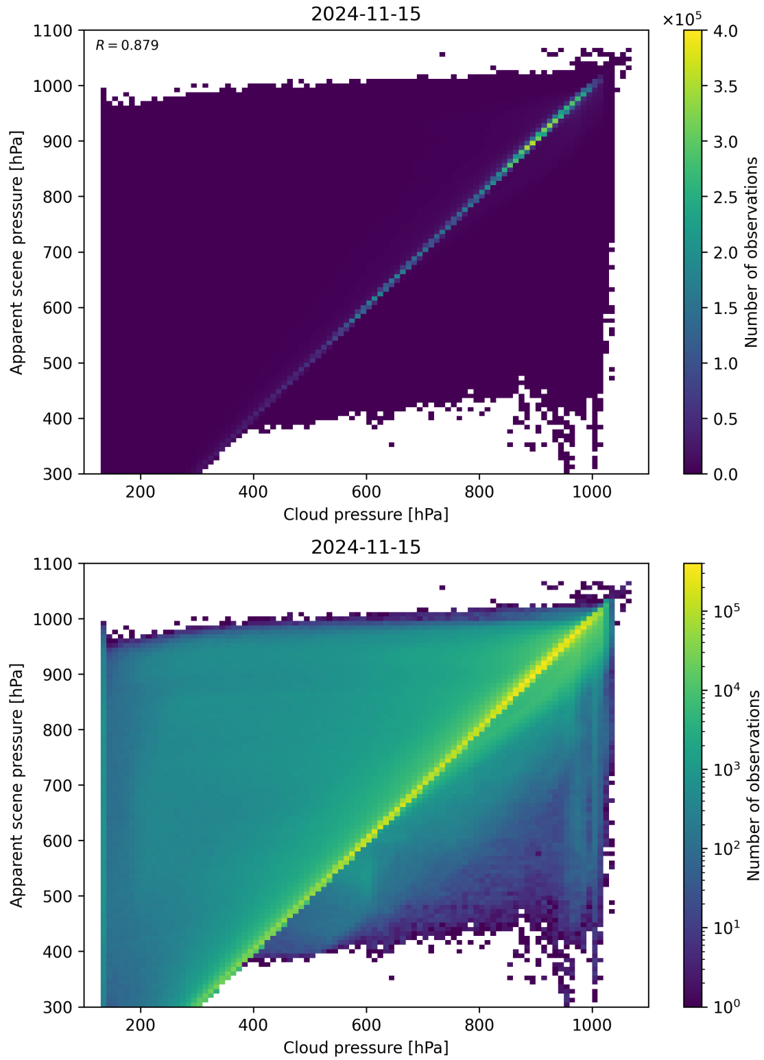
Figure 84: Scatter density plot of “Cloud pressure” against “Apparent scene pressure” for 2024-11-14 to 2024-11-16.
