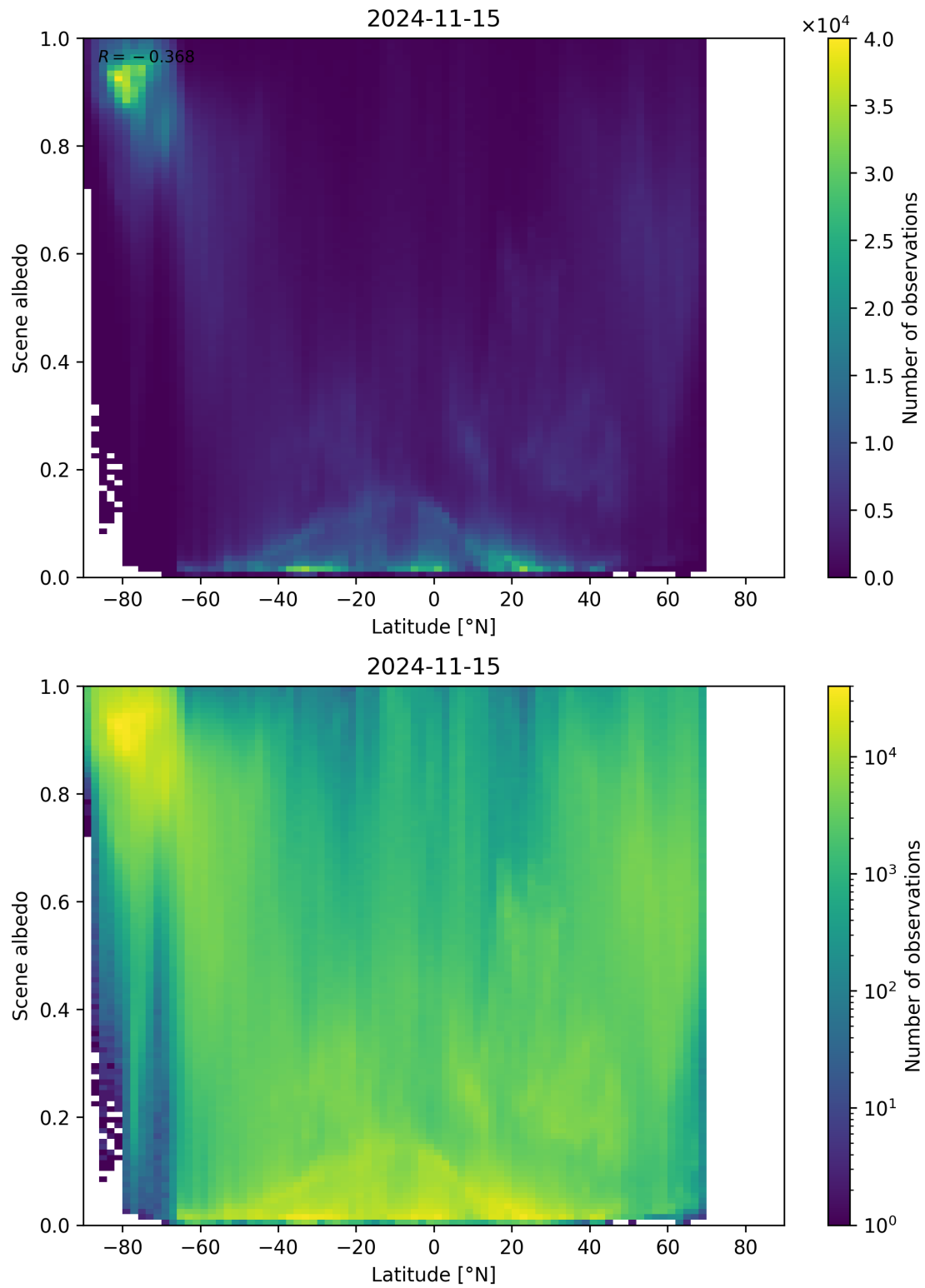
Figure 104: Scatter density plot of “Latitude” against “Scene albedo” for 2024-11-14 to 2024-11-16.
