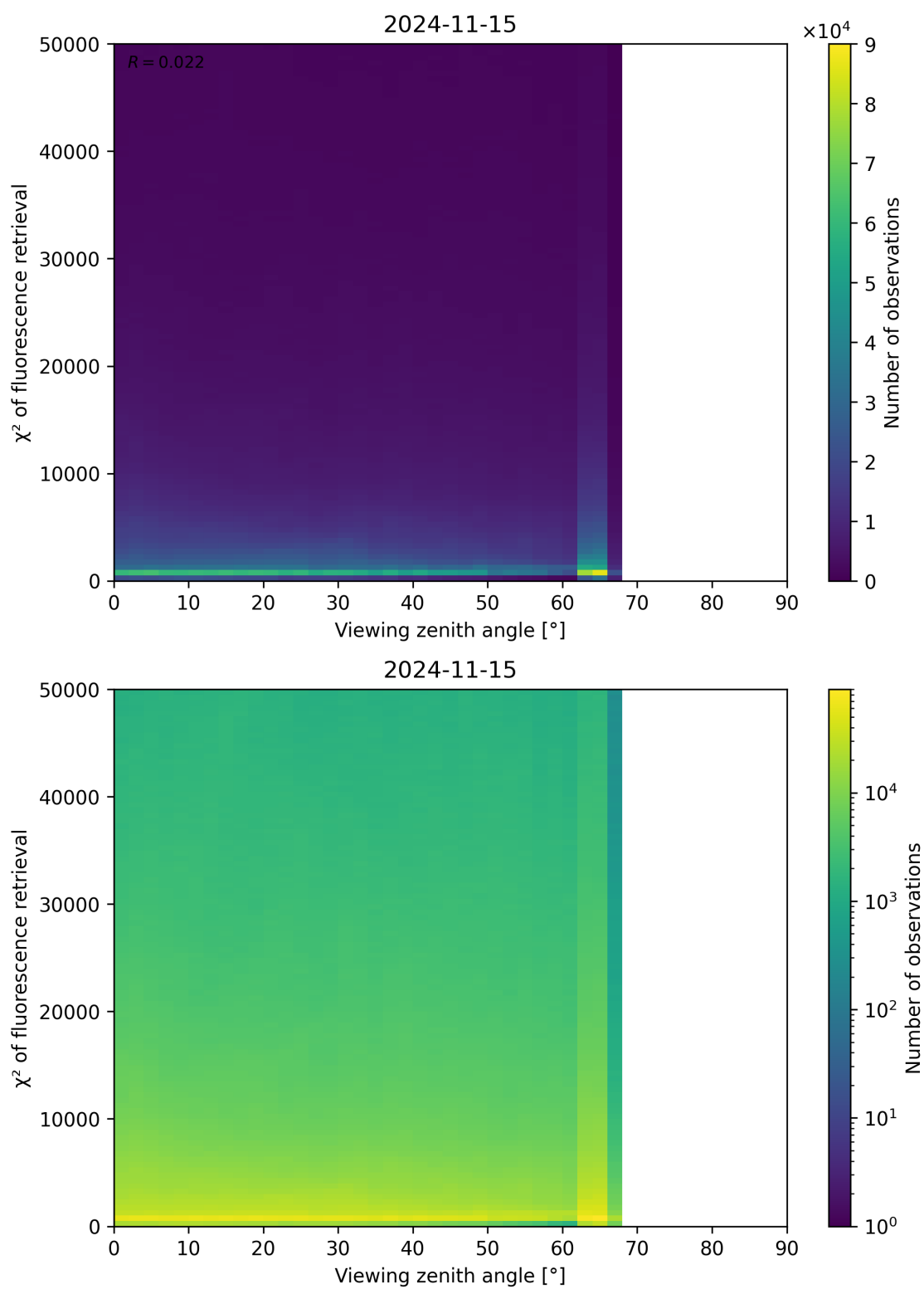
Figure 131: Scatter density plot of “Viewing zenith angle” against “ \chi^2 of fluorescence retrieval” for 2024-11-14 to 2024-11-16.
