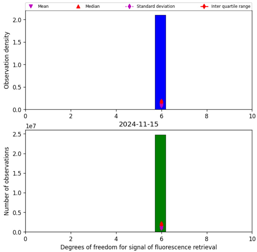
Figure 43: Histogram of “Degrees of freedom for signal of fluorescence retrieval” for 2024-11-14 to 2024-11-16
