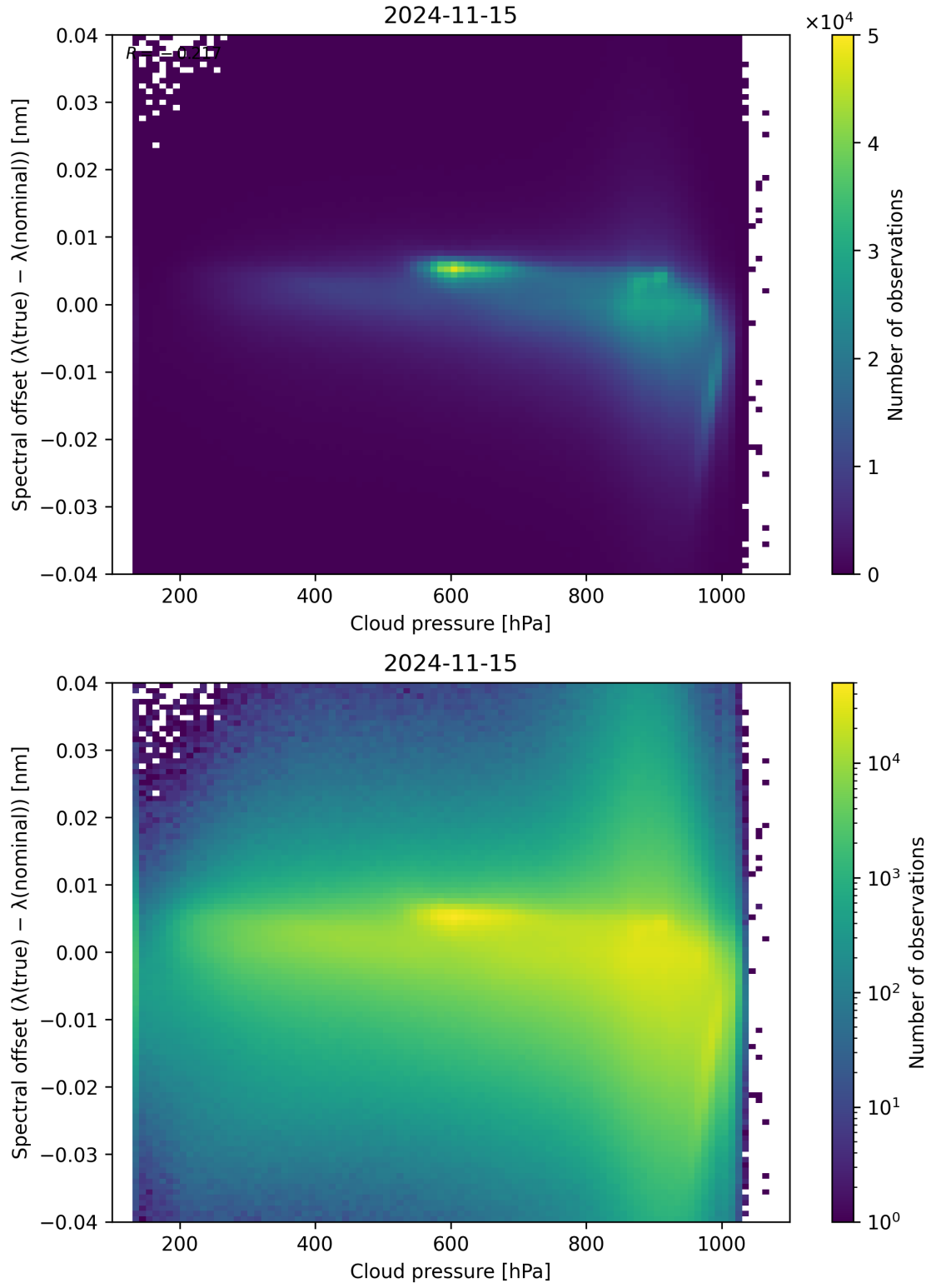
Figure 92: Scatter density plot of “Cloud pressure” against “Spectral offset ( \lambda_{\text{true}} - \lambda_{\text{nominal}} )” for 2024-11-14 to 2024-11-16.
