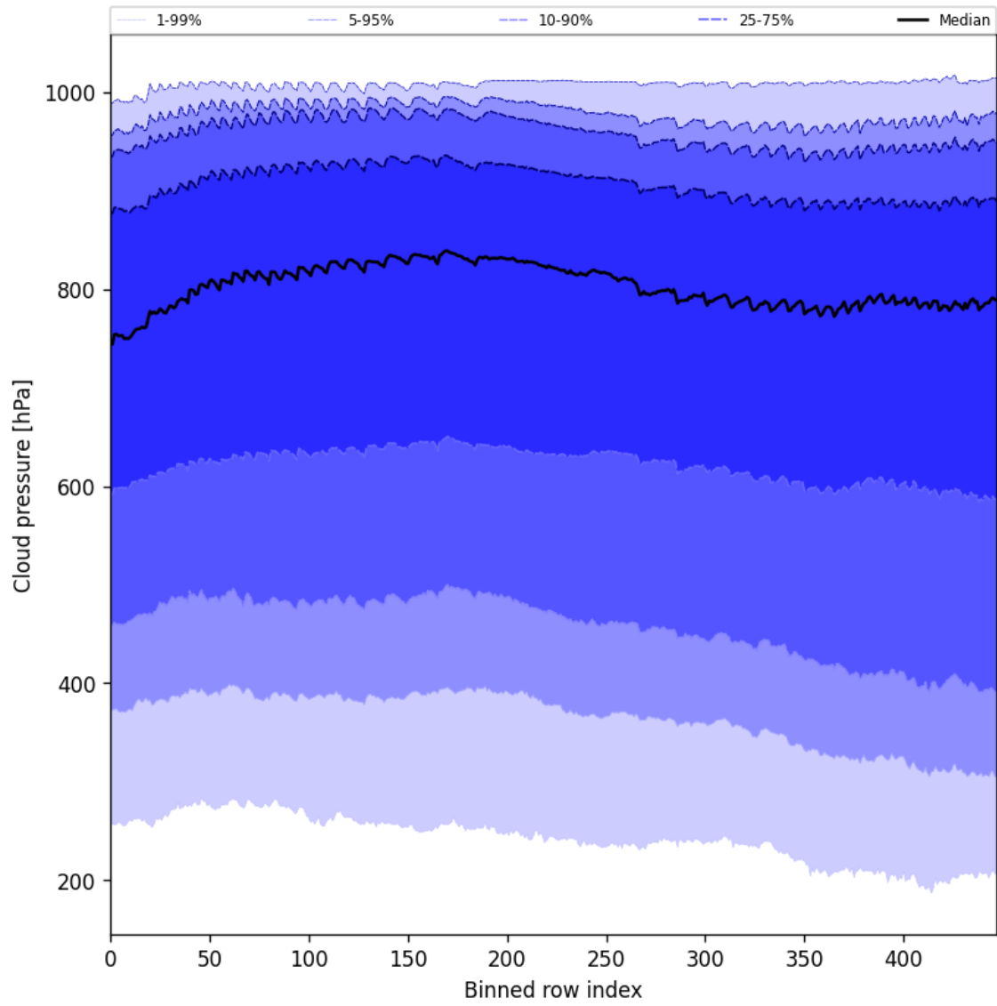
Figure 47: Along track statistics of “Cloud pressure” for 2024-11-14 to 2024-11-16
