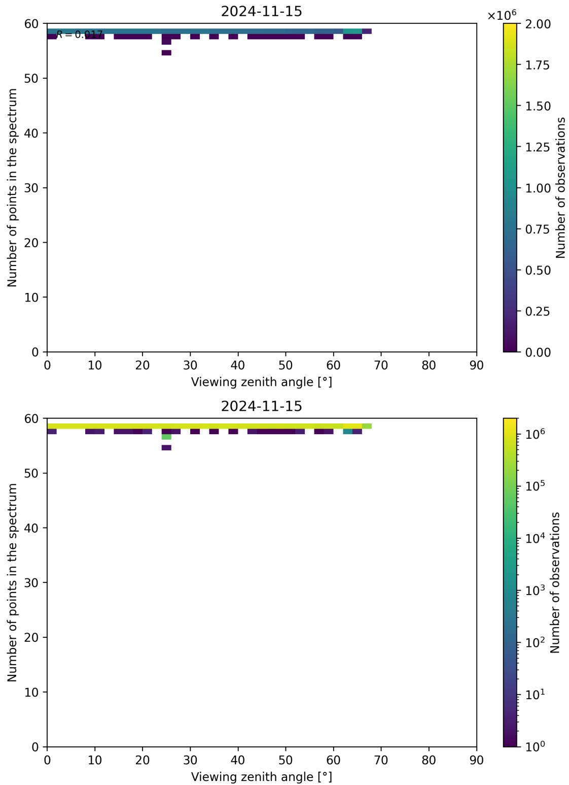
Figure 137: Scatter density plot of “Viewing zenith angle” against “Number of points in the spectrum” for 2024-11-14 to 2024-11-16.
