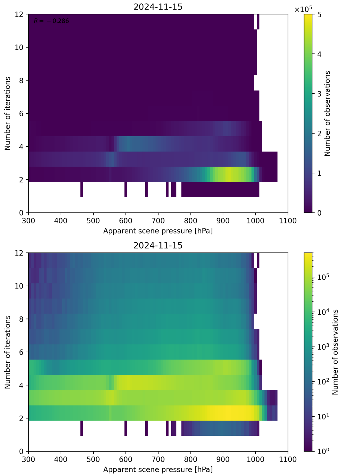
Figure 66: Scatter density plot of “Apparent scene pressure” against “Number of iterations” for 2024-11-14 to 2024-11-16.
