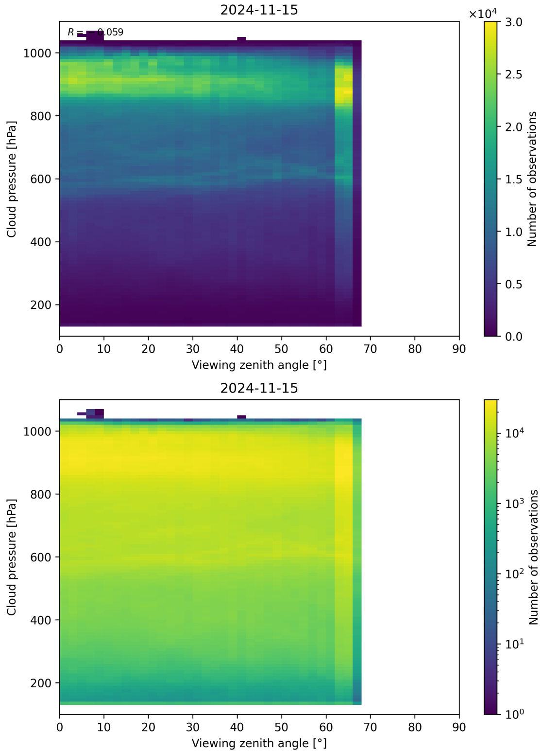
Figure 133: Scatter density plot of “Viewing zenith angle” against “Cloud pressure” for 2024-11-14 to 2024-11-16.
