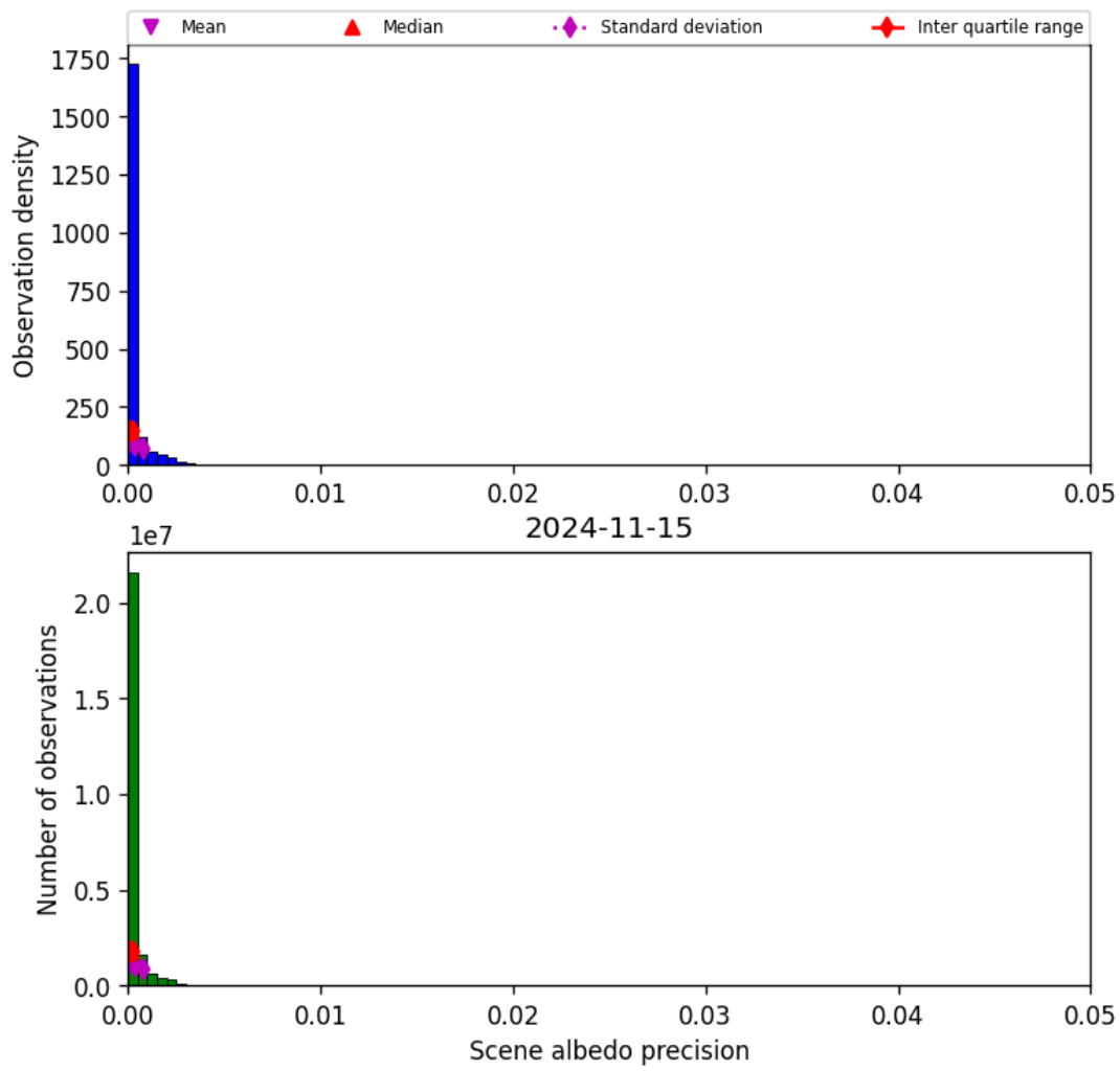
Figure 35: Histogram of “Scene albedo precision” for 2024-11-14 to 2024-11-16
