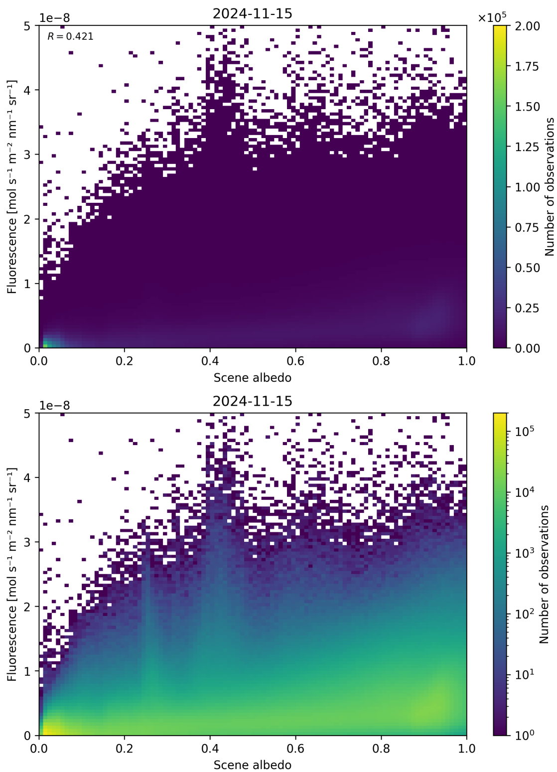
Figure 114: Scatter density plot of "Scene albedo" against "Fluorescence" for 2024-11-14 to 2024-11-16.
