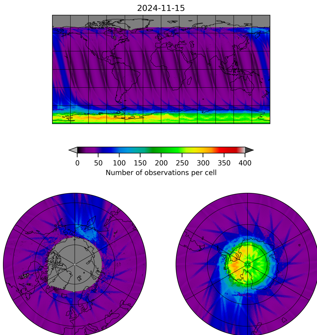
Figure 11: Map of the number of observations for 2024-11-14 to 2024-11-16
