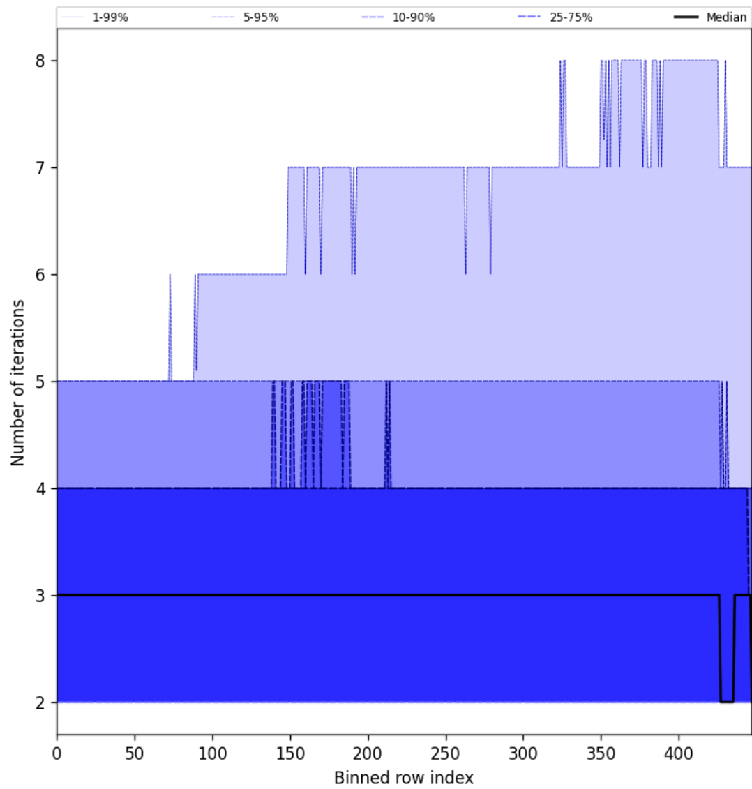
Figure 56: Along track statistics of “Number of iterations” for 2024-11-14 to 2024-11-16
