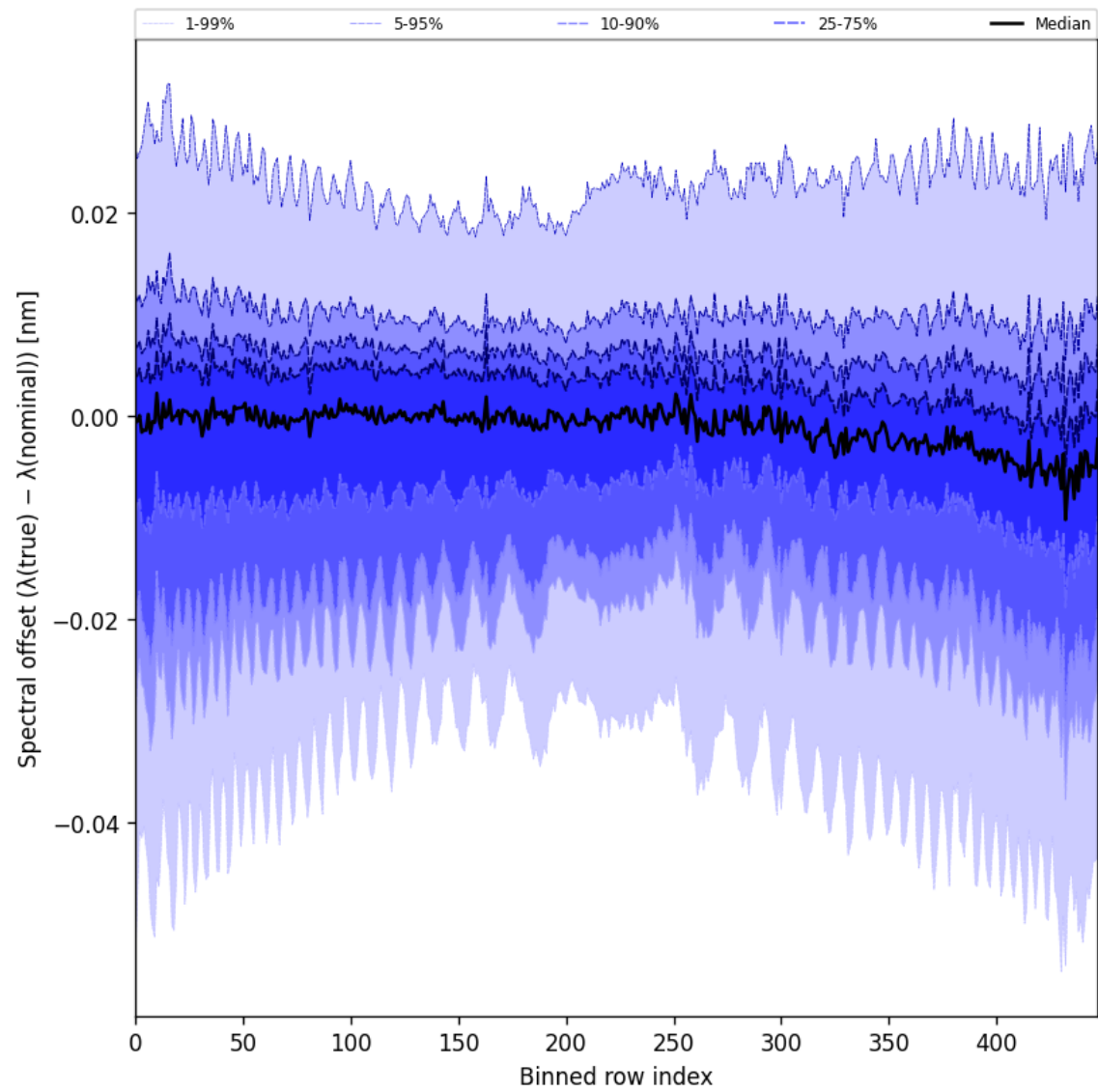
Figure 62: Along track statistics of “Spectral offset ( \lambda_{\text{true}} - \lambda_{\text{nominal}} )” for 2024-11-14 to 2024-11-16
