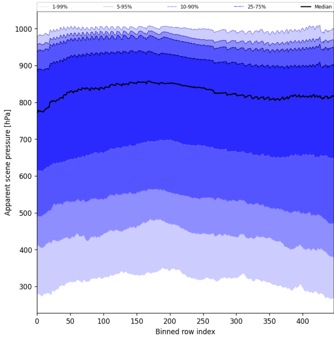
Figure 53: Along track statistics of “Apparent scene pressure” for 2024-11-14 to 2024-11-16
