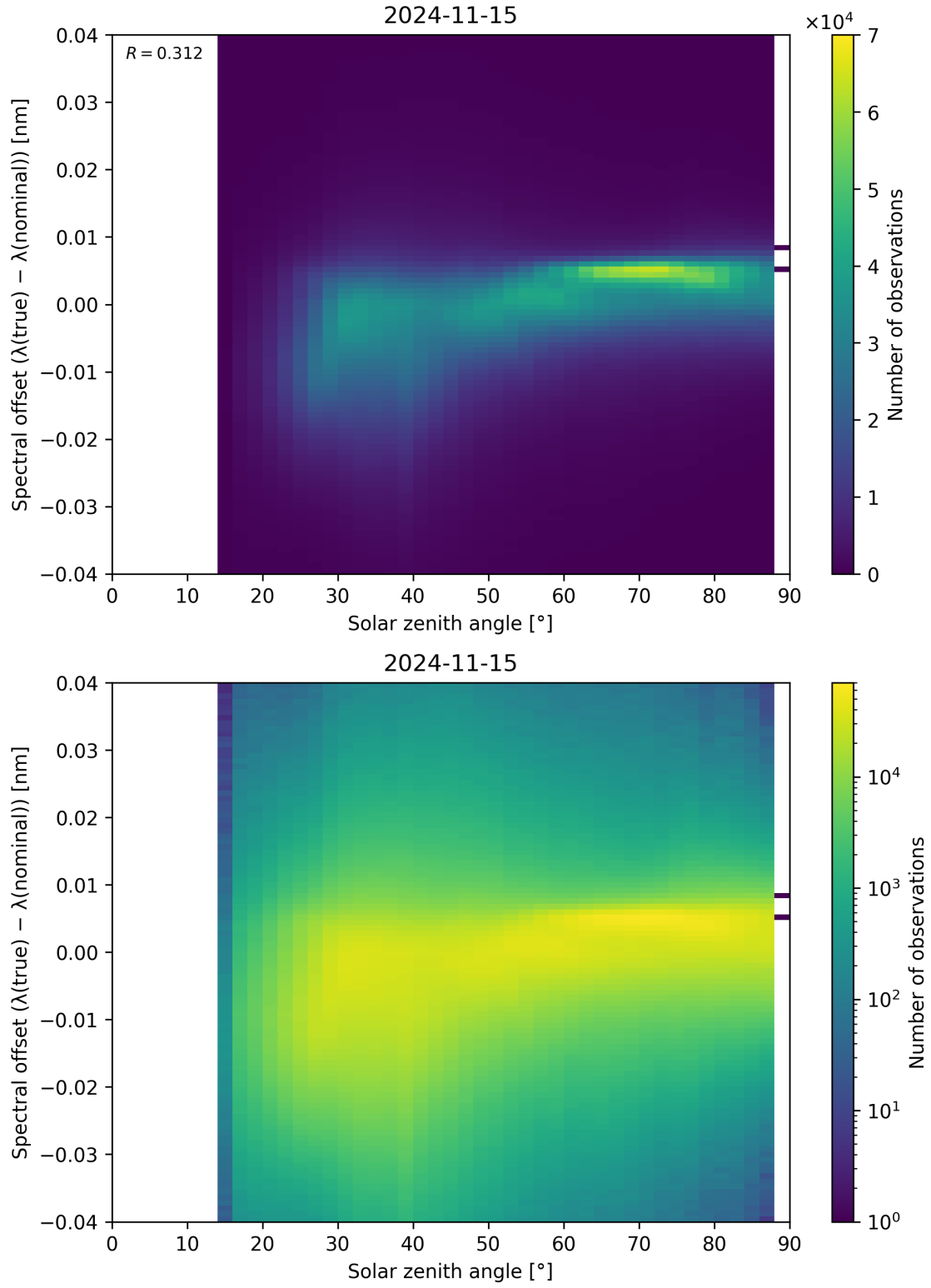
Figure 128: Scatter density plot of “Solar zenith angle” against “Spectral offset ( \lambda_{\text{true}} - \lambda_{\text{nominal}} )” for 2024-11-14 to 2024-11-16.
