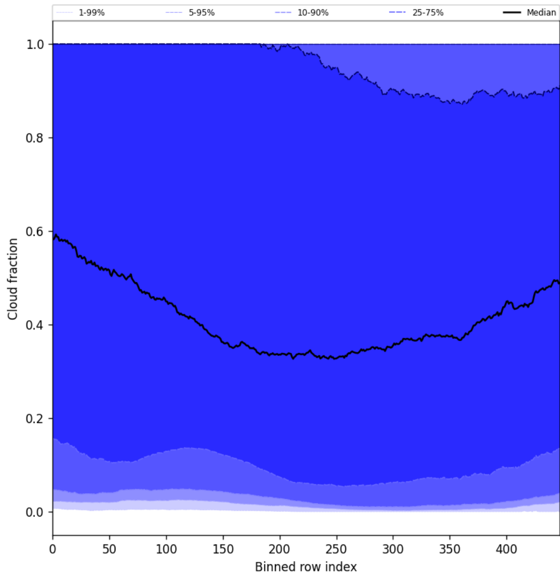
Figure 49: Along track statistics of “Cloud fraction” for 2024-11-14 to 2024-11-16
