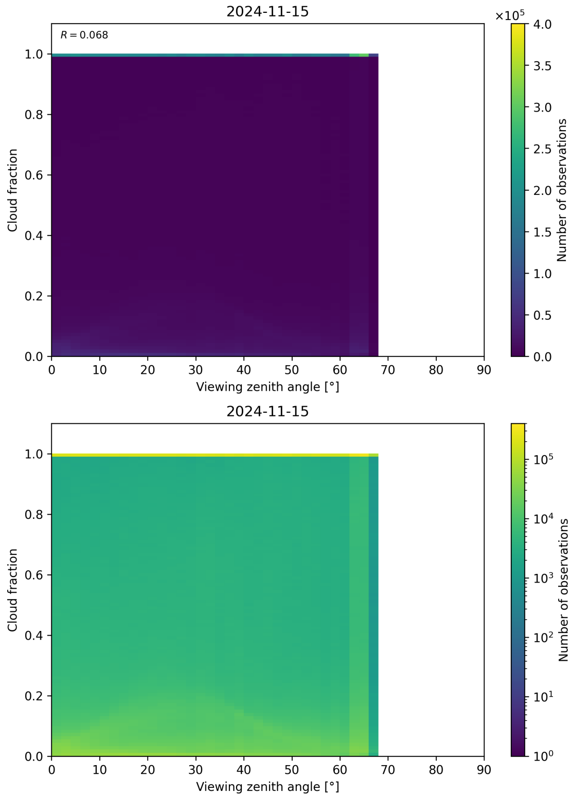
Figure 132: Scatter density plot of “Viewing zenith angle” against “Cloud fraction” for 2024-11-14 to 2024-11-16.
