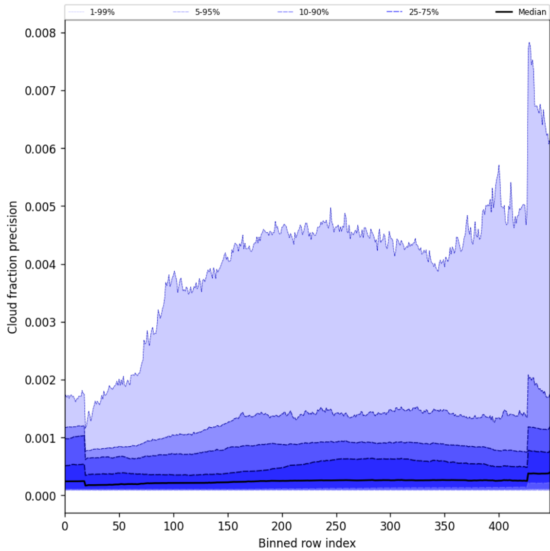
Figure 50: Along track statistics of “Cloud fraction precision” for 2024-11-14 to 2024-11-16
