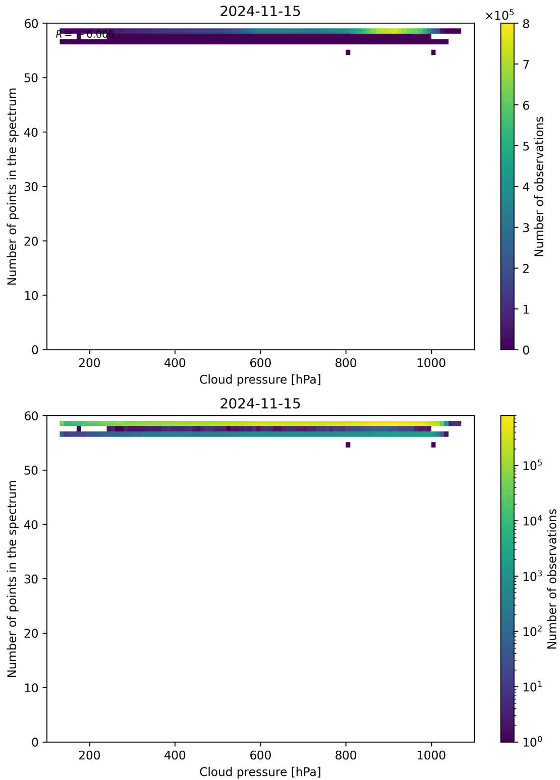
Figure 90: Scatter density plot of “Cloud pressure” against “Number of points in the spectrum” for 2024-11-14 to 2024-11-16.
