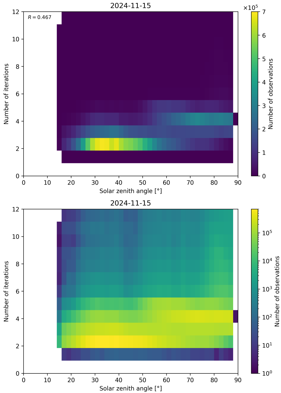
Figure 125: Scatter density plot of “Solar zenith angle” against “Number of iterations” for 2024-11-14 to 2024-11-16.
