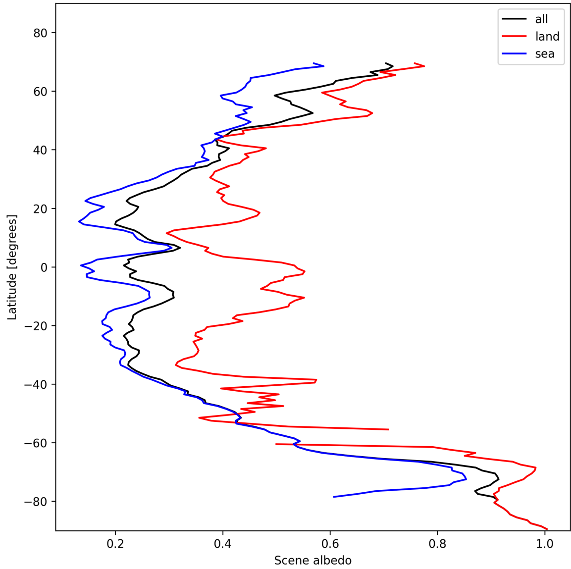
Figure 17: Zonal average of “Scene albedo” for 2024-11-14 to 2024-11-16.
