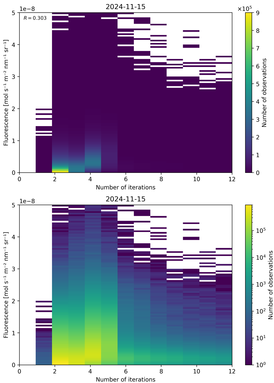
Figure 107: Scatter density plot of “Number of iterations” against “Fluorescence” for 2024-11-14 to 2024-11-16.
