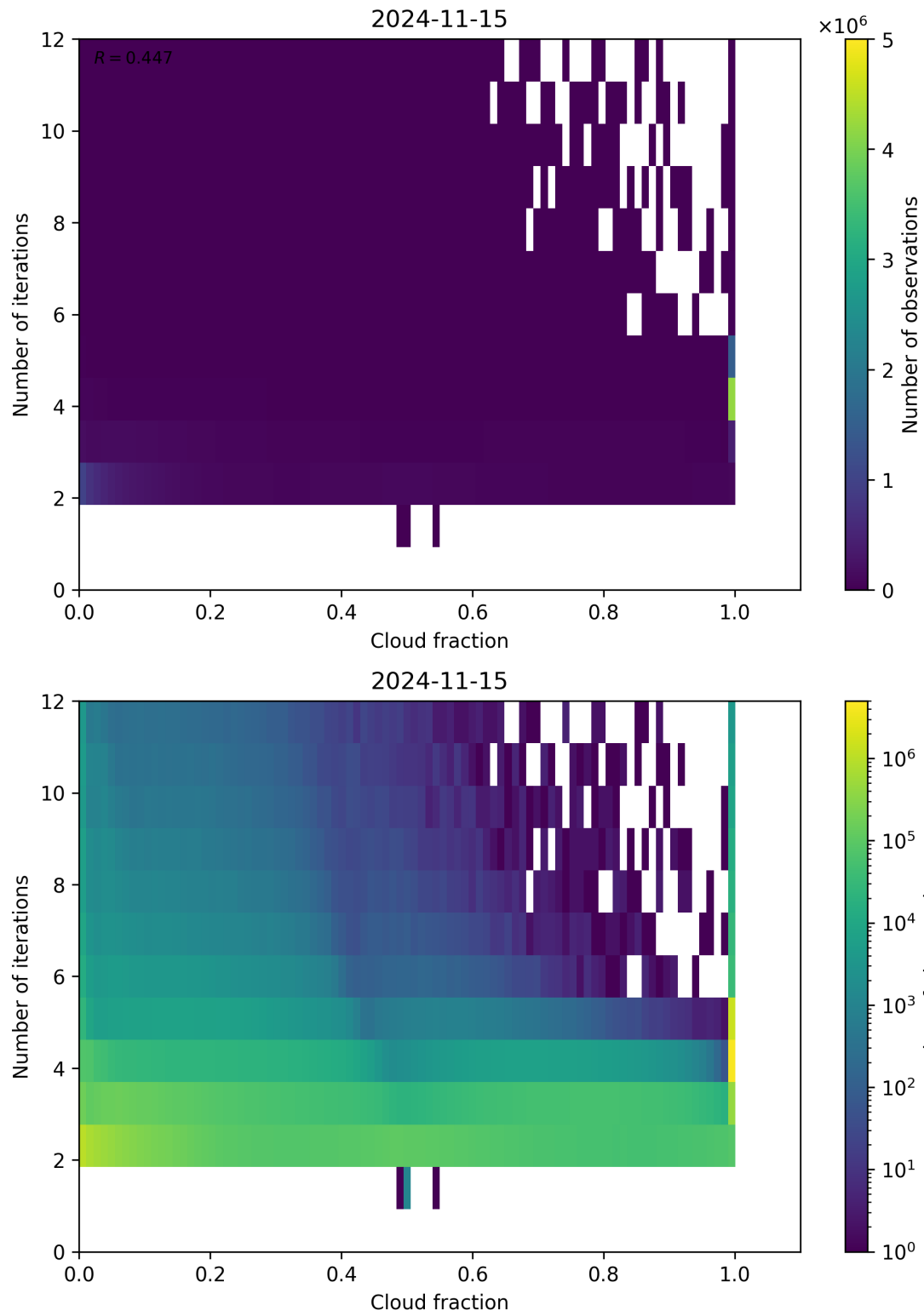
Figure 80: Scatter density plot of “Cloud fraction” against “Number of iterations” for 2024-11-14 to 2024-11-16.
