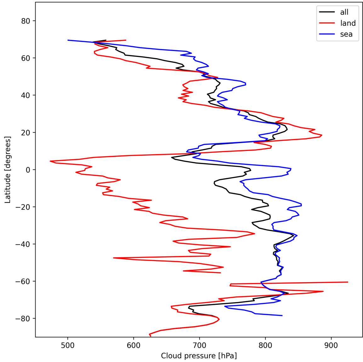
Figure 13: Zonal average of “Cloud pressure” for 2024-11-14 to 2024-11-16.
