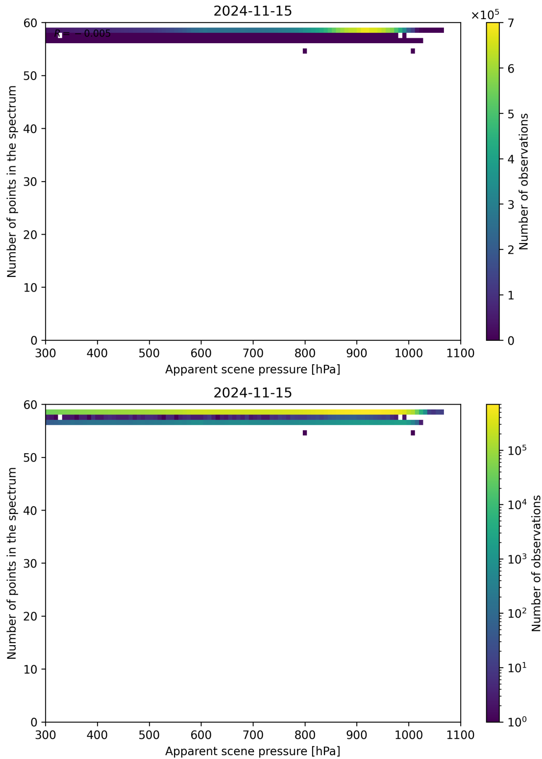
Figure 67: Scatter density plot of “Apparent scene pressure” against “Number of points in the spectrum” for 2024-11-14 to 2024-11-16.
