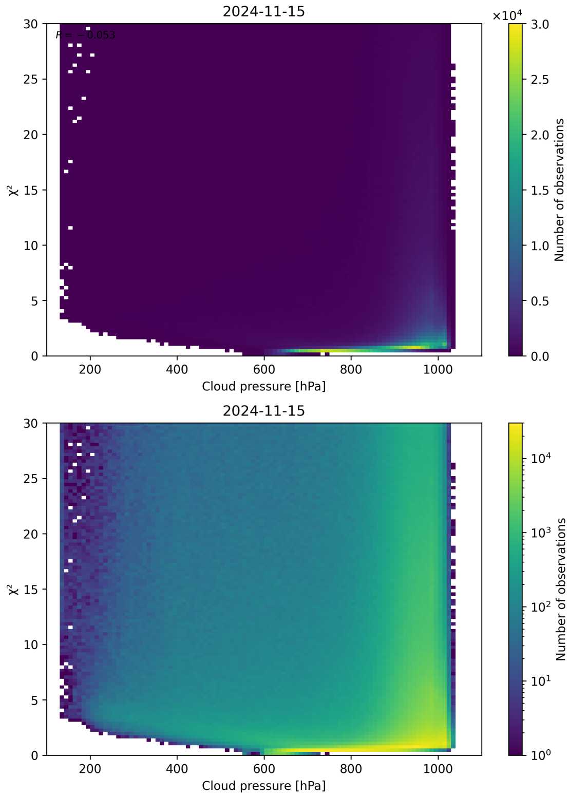
Figure 85: Scatter density plot of “Cloud pressure” against “ \chi^2 ” for 2024-11-14 to 2024-11-16.
