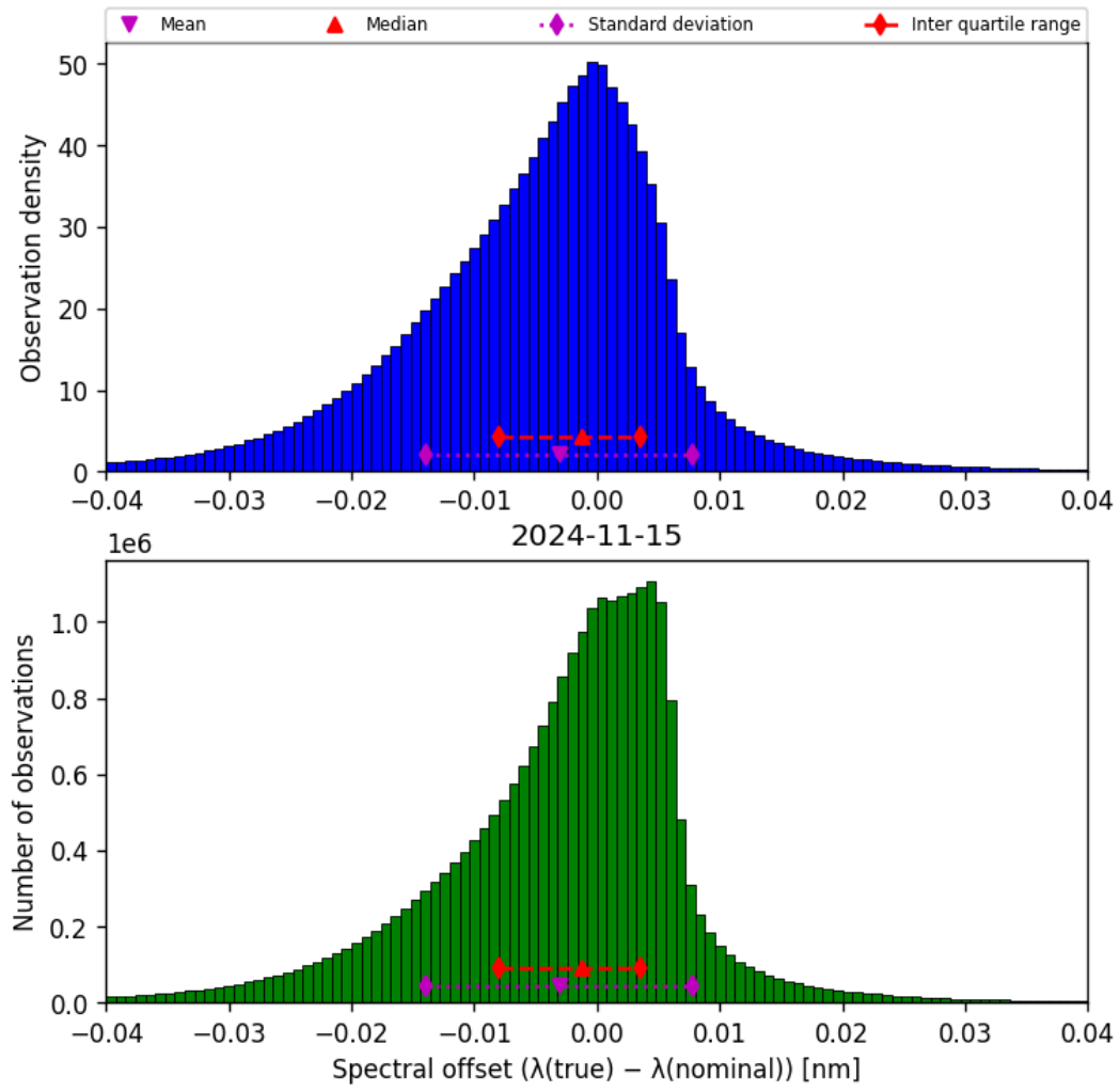
Figure 45: Histogram of “Spectral offset ( \lambda_{\text{true}} - \lambda_{\text{nominal}} )” for 2024-11-14 to 2024-11-16
