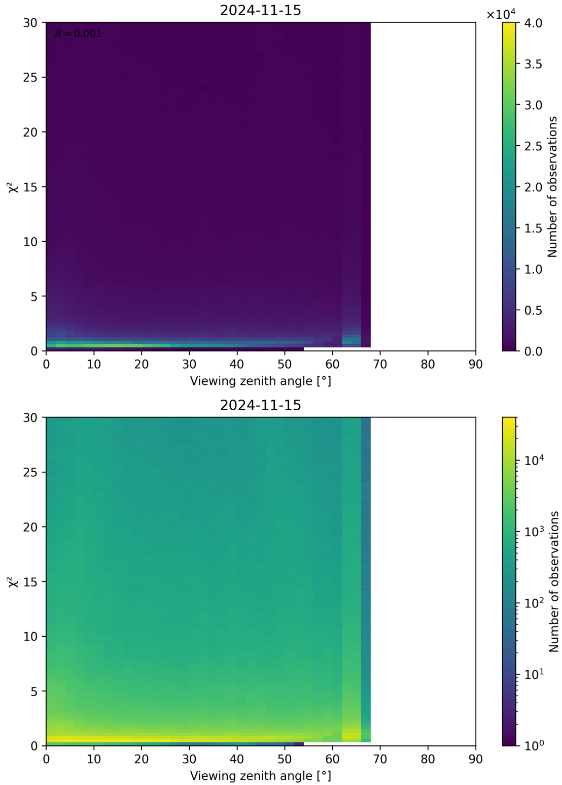
Figure 130: Scatter density plot of “Viewing zenith angle” against “ \chi^2 ” for 2024-11-14 to 2024-11-16.
