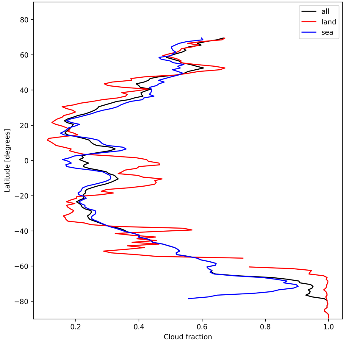
Figure 15: Zonal average of “Cloud fraction” for 2024-11-14 to 2024-11-16.
