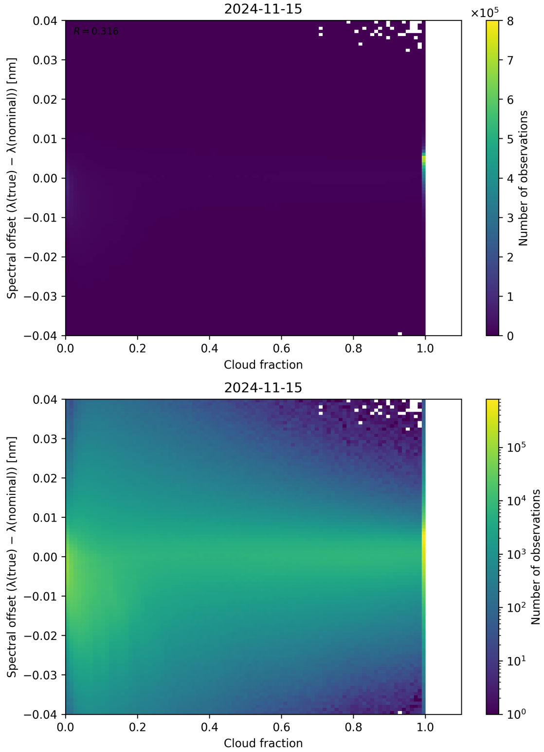
Figure 83: Scatter density plot of “Cloud fraction” against “Spectral offset ( \lambda_{\text{true}} - \lambda_{\text{nominal}} )” for 2024-11-14 to 2024-11-16.
