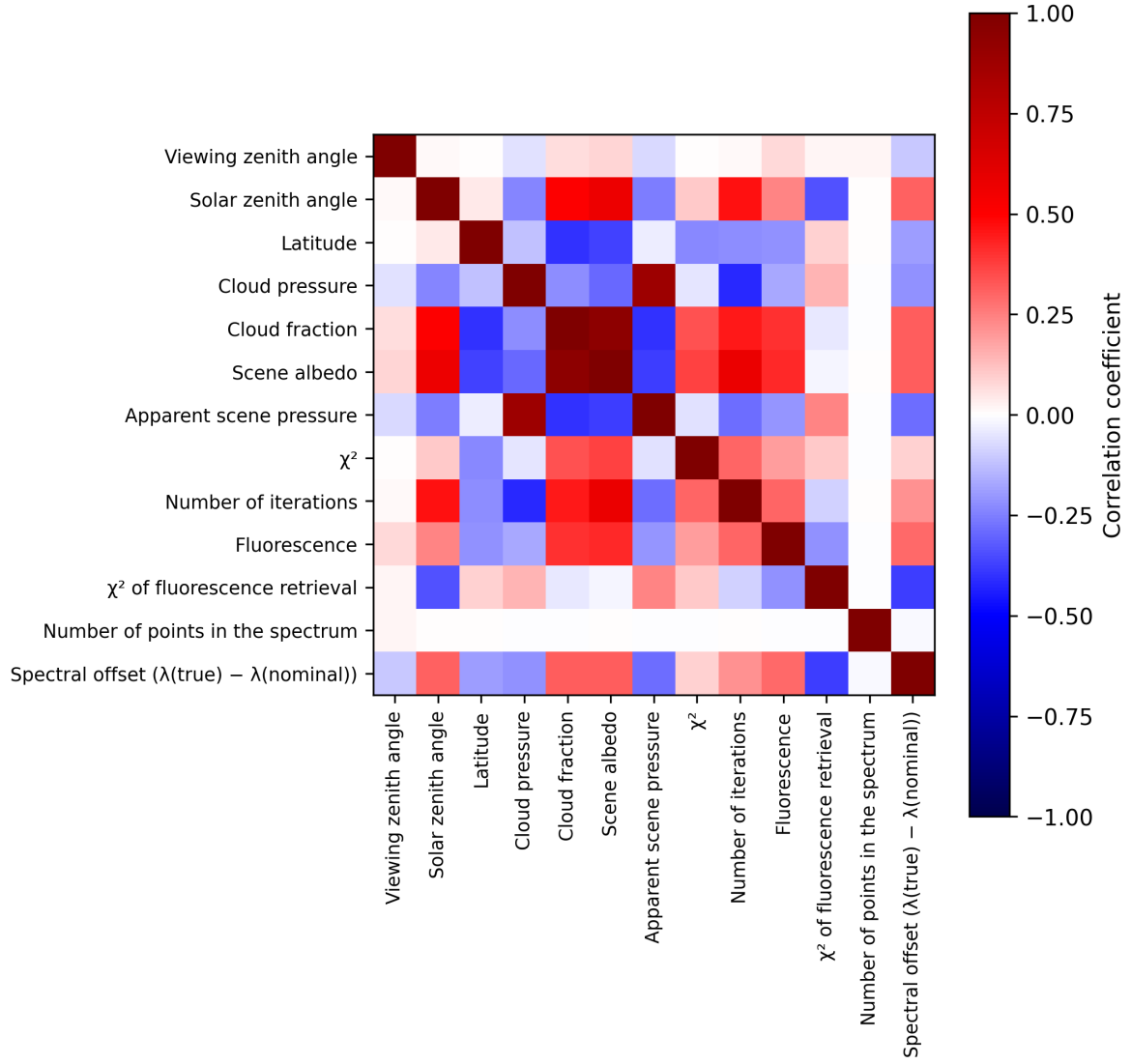
Figure 2: Map of correlation matrix for 2024-11-14 to 2024-11-16.
