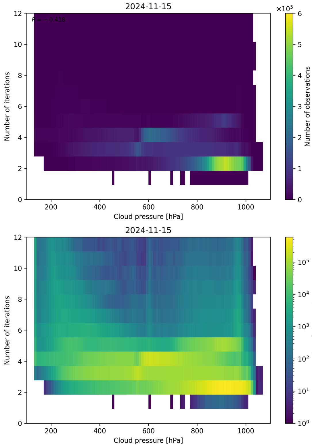
Figure 89: Scatter density plot of “Cloud pressure” against “Number of iterations” for 2024-11-14 to 2024-11-16.
