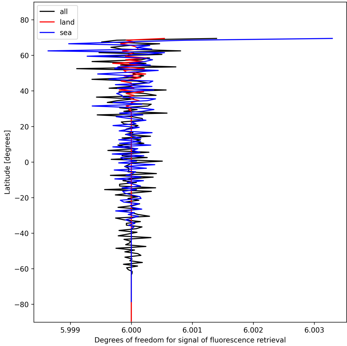
Figure 26: Zonal average of “Degrees of freedom for signal of fluorescence retrieval” for 2024-11-14 to 2024-11-16.
