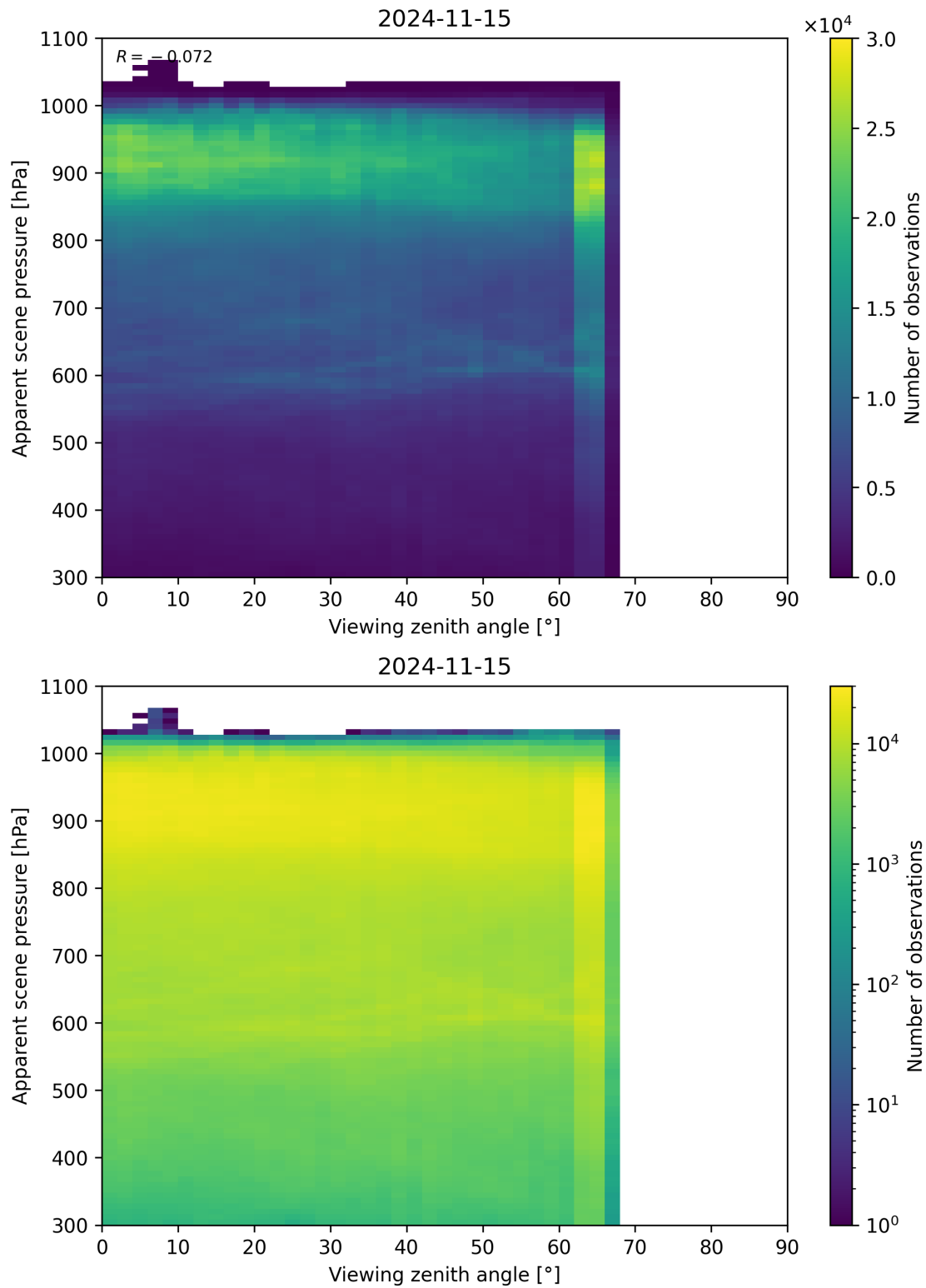
Figure 129: Scatter density plot of “Viewing zenith angle” against “Apparent scene pressure” for 2024-11-14 to 2024-11-16.
