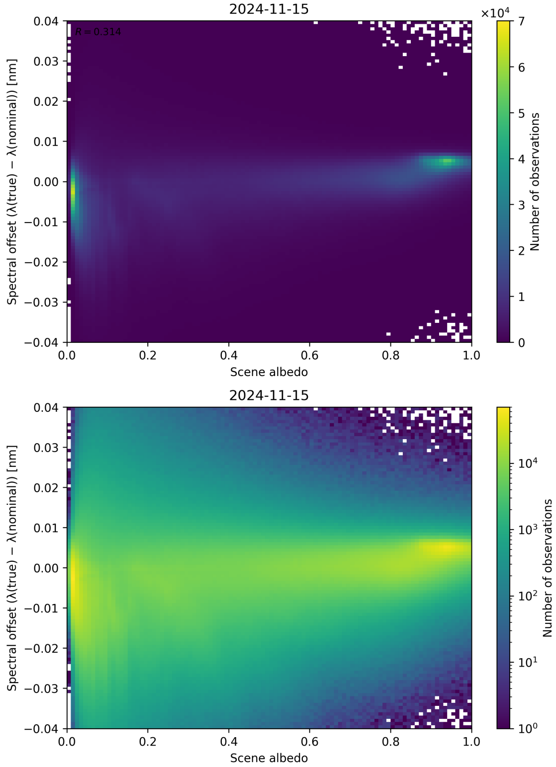
Figure 117: Scatter density plot of “Scene albedo” against “Spectral offset ( \lambda_{\text{true}} - \lambda_{\text{nominal}} )” for 2024-11-14 to 2024-11-16.
