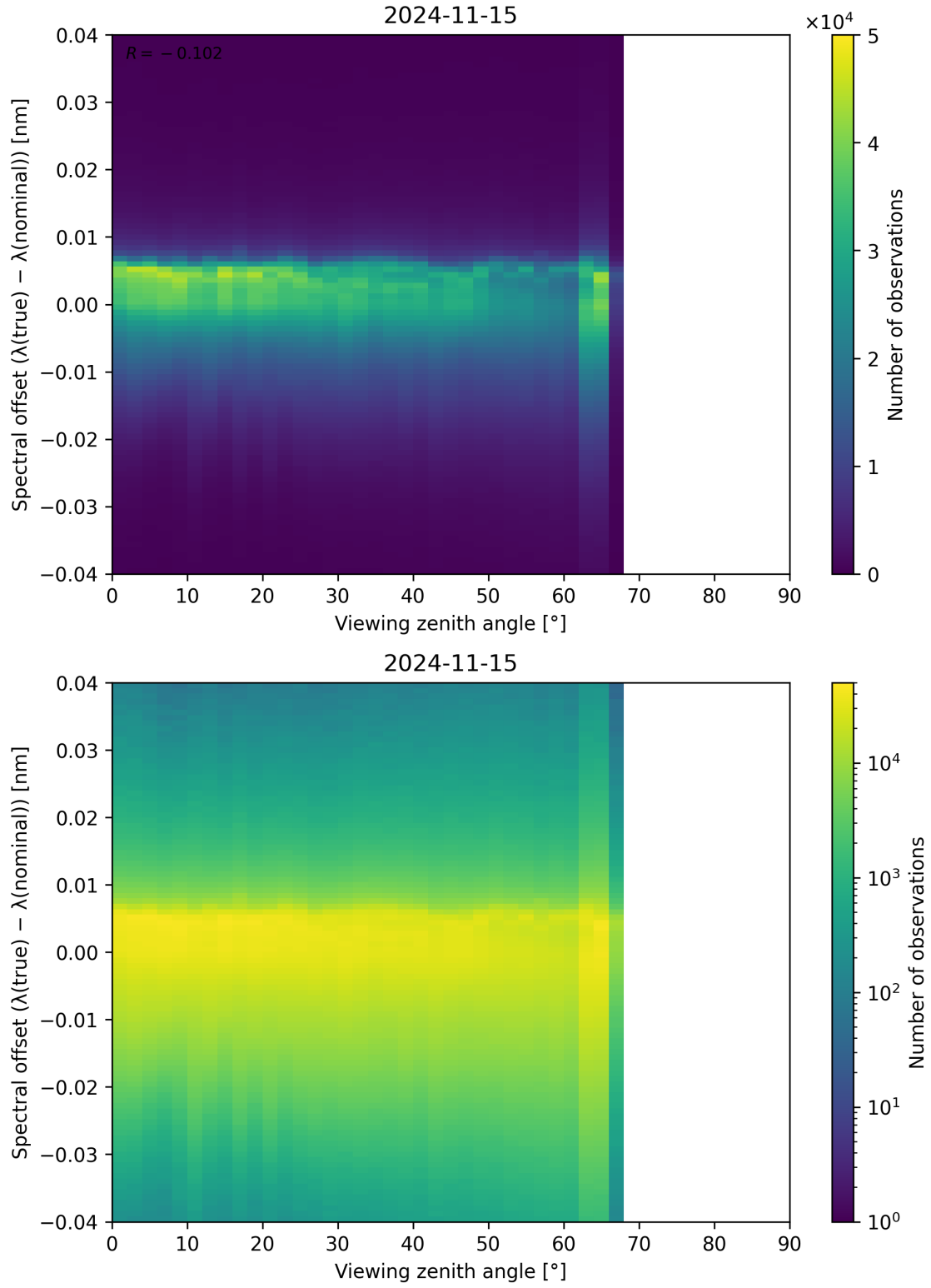
Figure 140: Scatter density plot of “Viewing zenith angle” against “Spectral offset ( \lambda_{\text{true}} - \lambda_{\text{nominal}} )” for 2024-11-14 to 2024-11-16.
