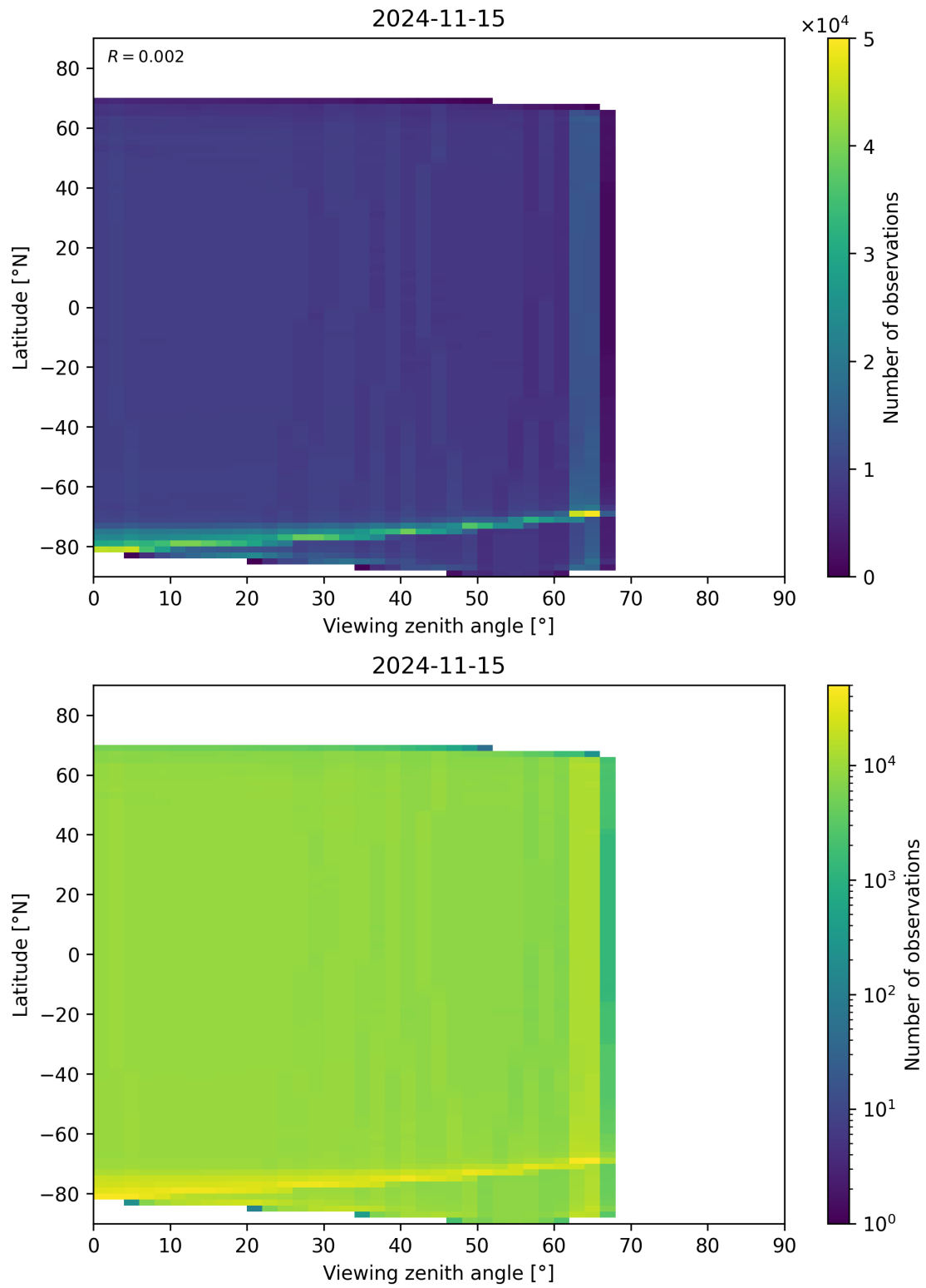
Figure 135: Scatter density plot of “Viewing zenith angle” against “Latitude” for 2024-11-14 to 2024-11-16.
