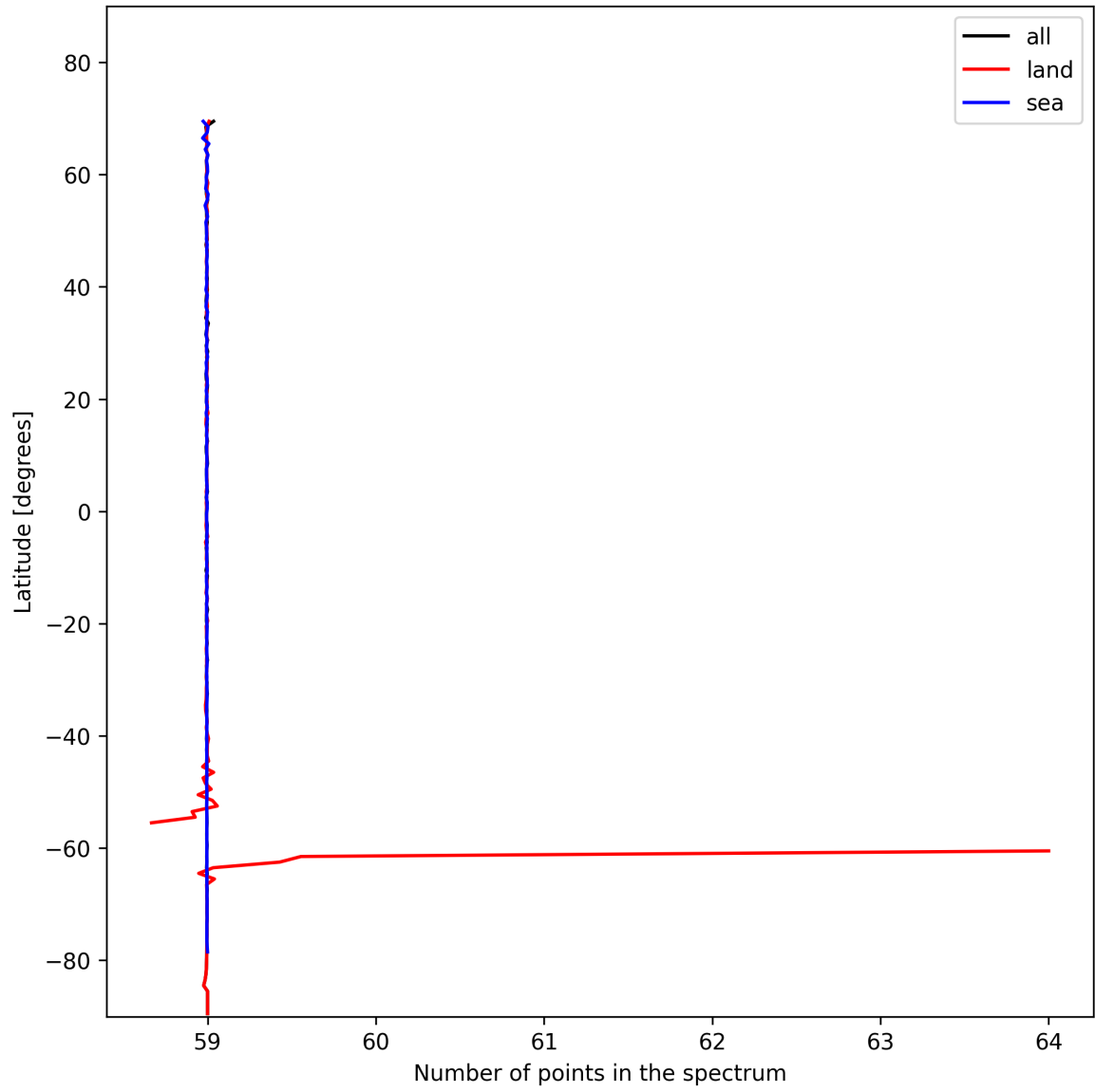
Figure 27: Zonal average of “Number of points in the spectrum” for 2024-11-14 to 2024-11-16.
