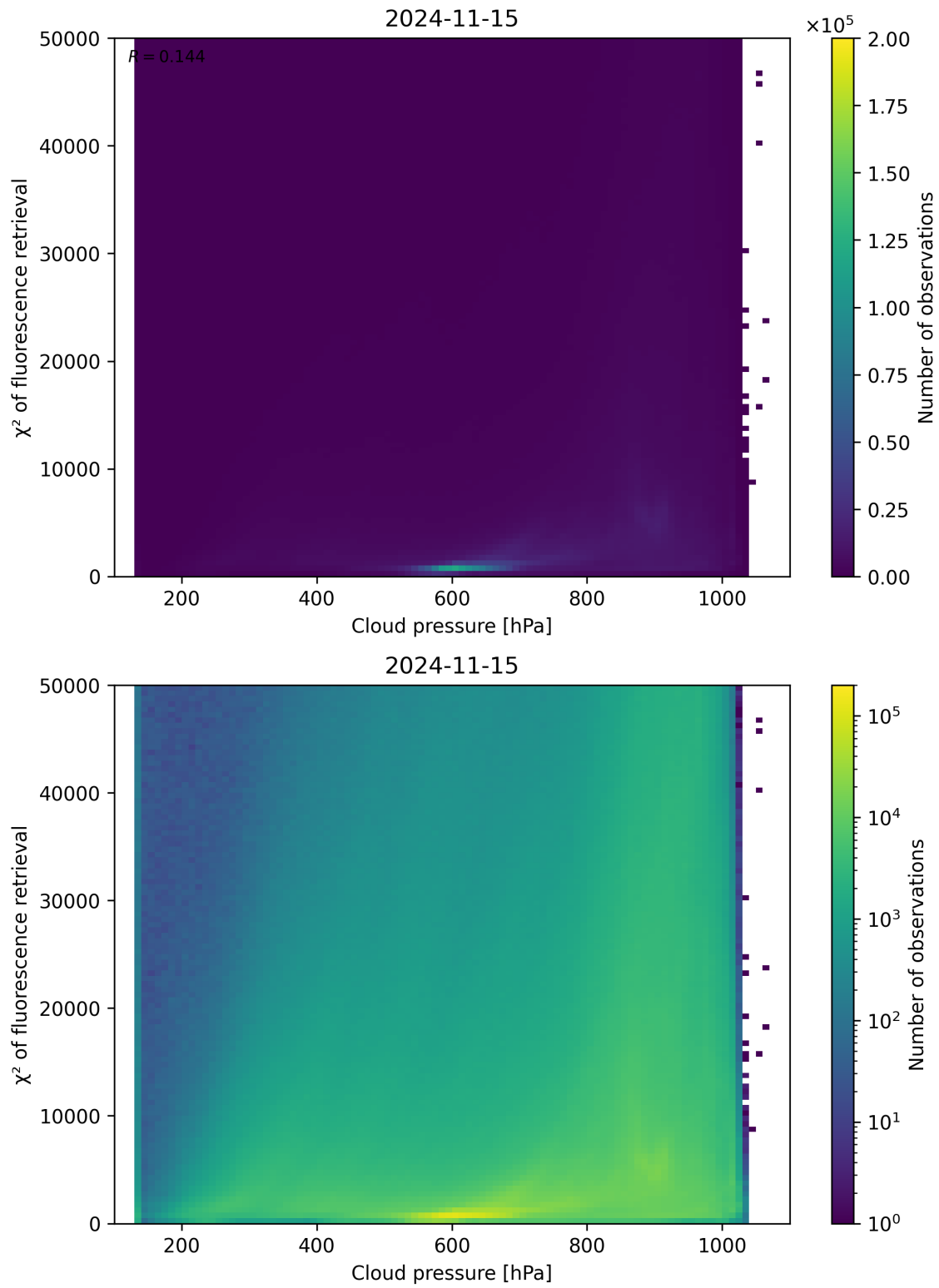
Figure 86: Scatter density plot of “Cloud pressure” against “ \chi^2 of fluorescence retrieval” for 2024-11-14 to 2024-11-16.
