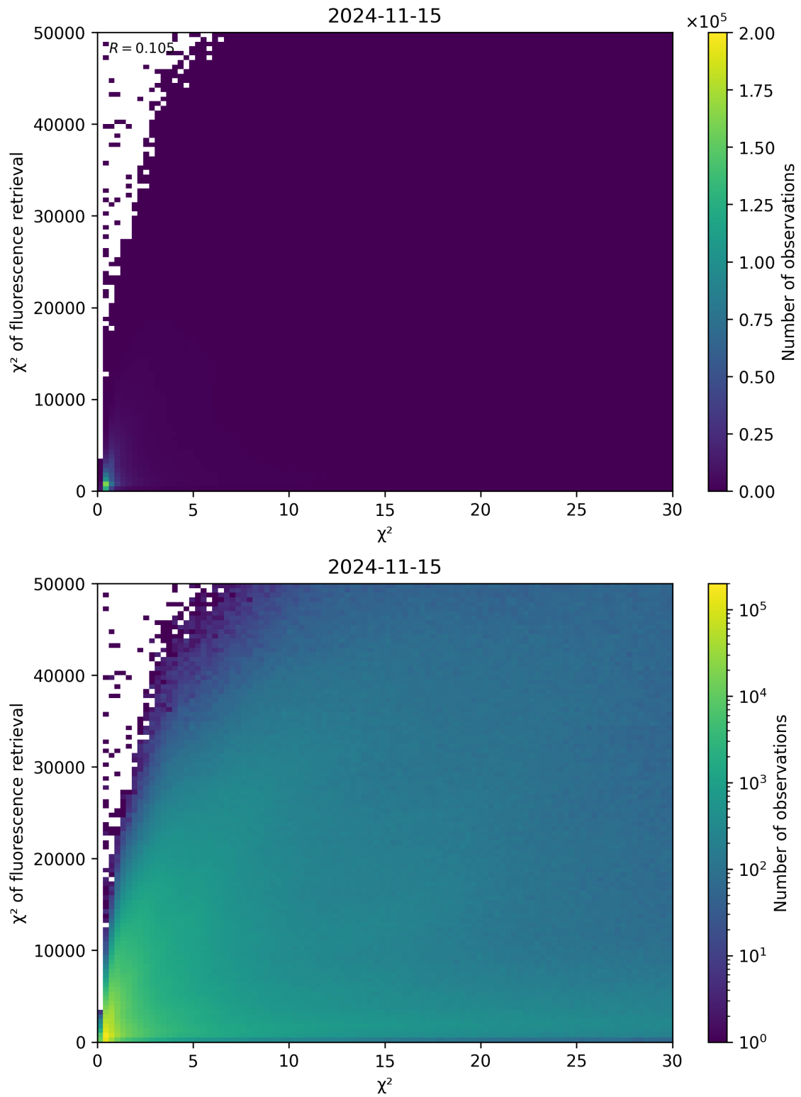
Figure 69: Scatter density plot of “ \chi^2 ” against “ \chi^2 of fluorescence retrieval” for 2024-11-14 to 2024-11-16.
