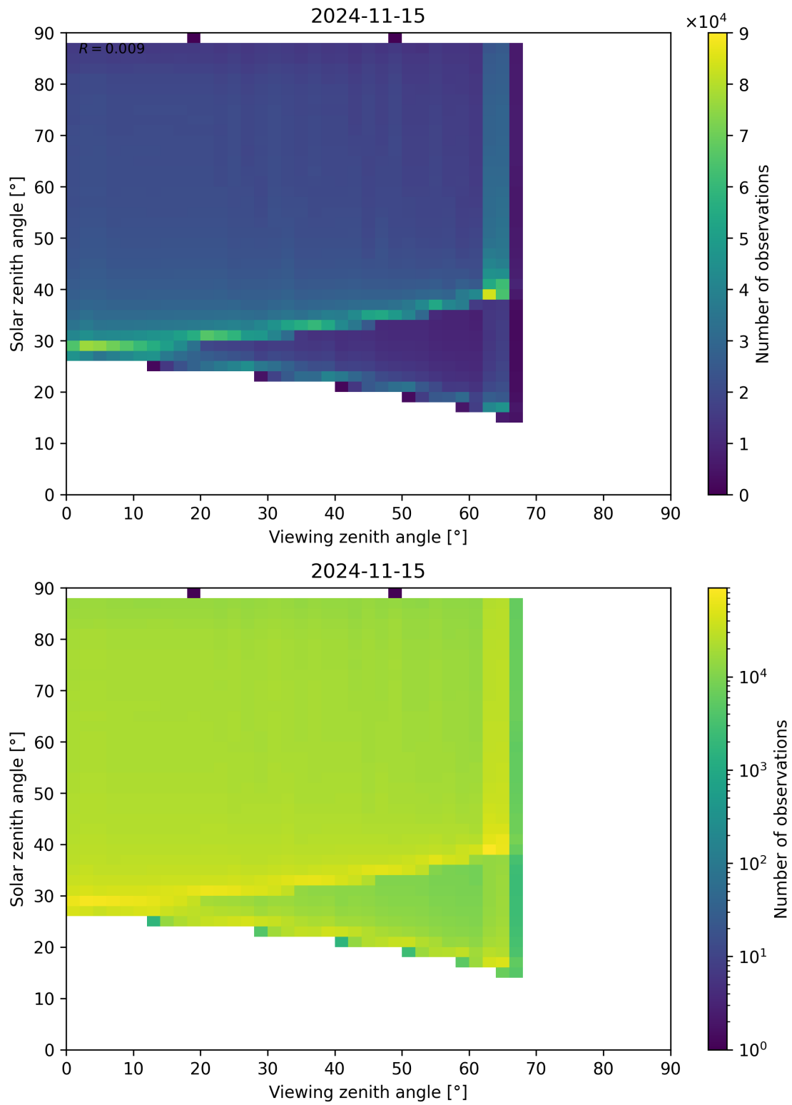
Figure 139: Scatter density plot of “Viewing zenith angle” against “Solar zenith angle” for 2024-11-14 to 2024-11-16.
