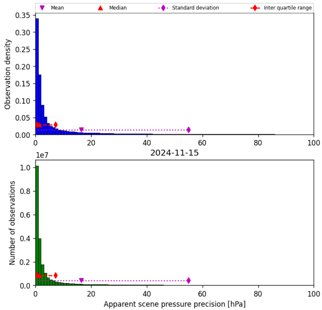
Figure 37: Histogram of “Apparent scene pressure precision” for 2024-11-14 to 2024-11-16
