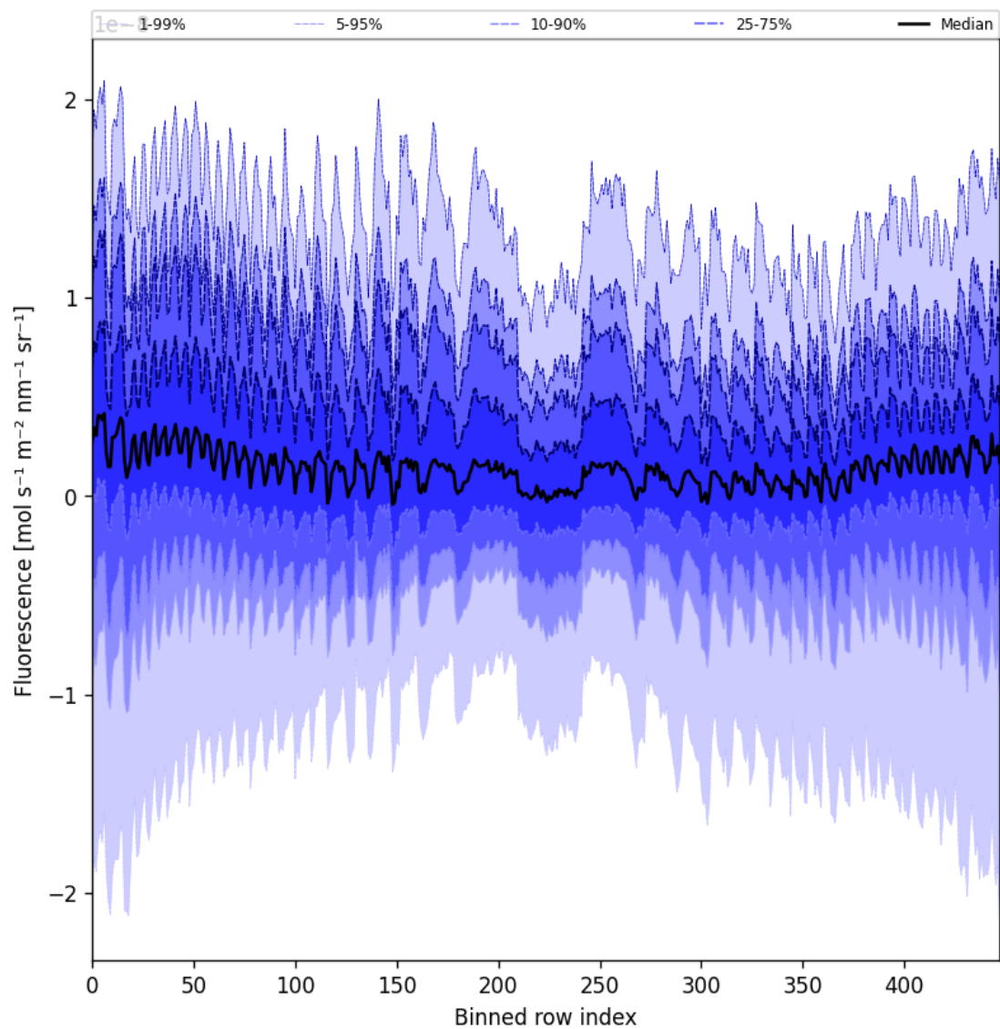
Figure 57: Along track statistics of “Fluorescence” for 2024-11-14 to 2024-11-16
